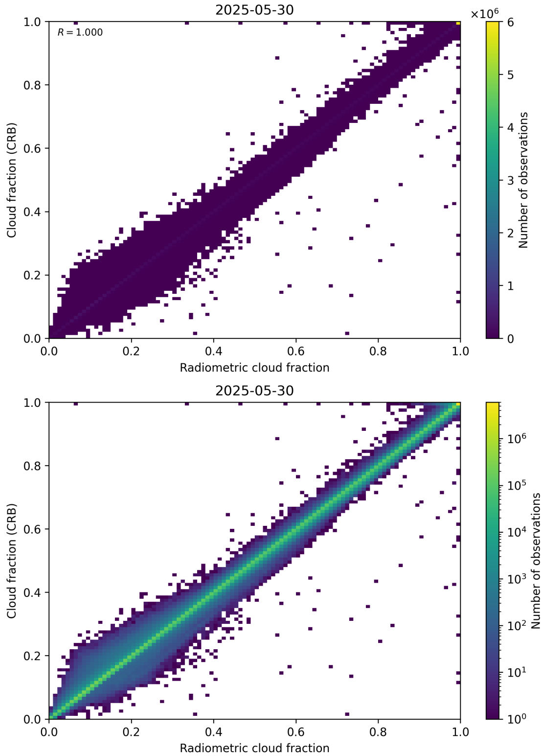
Figure 73: Scatter density plot of “Radiometric cloud fraction” against “Cloud fraction (CRB)” for 2025-05-29 to 2025-05-31.
