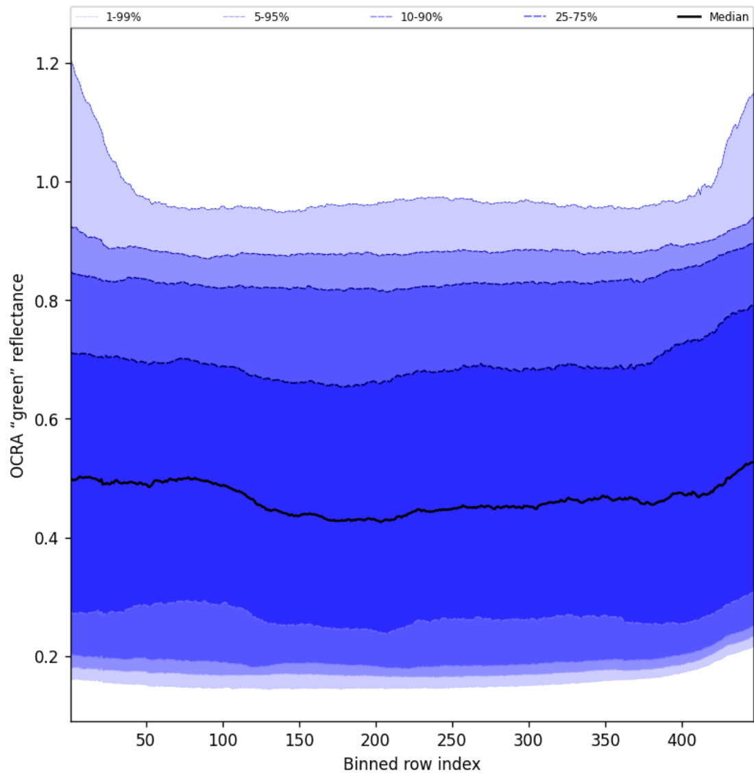
Figure 68: Along track statistics of “OCRA “green” reflectance” for 2025-05-29 to 2025-05-31
