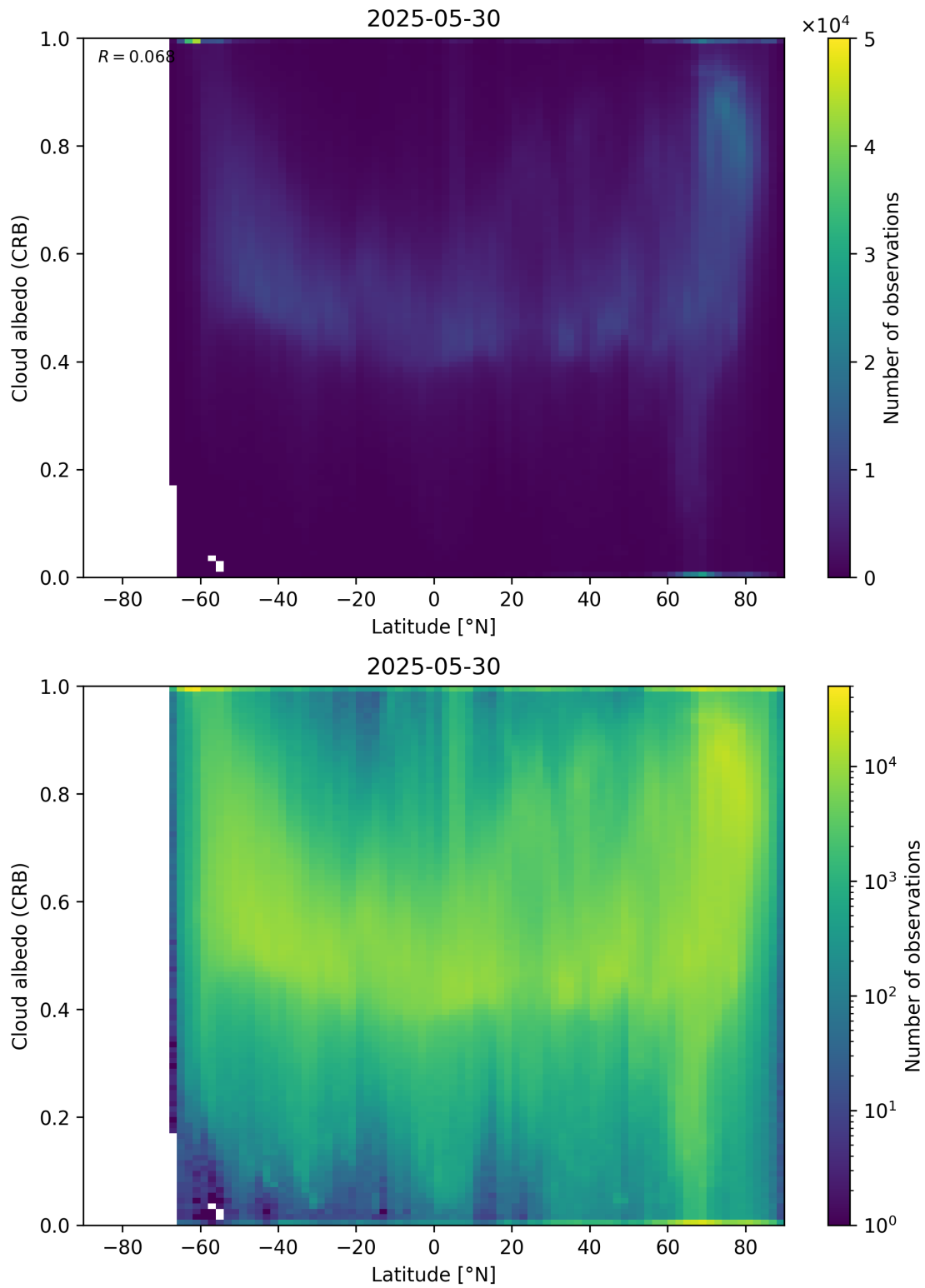
Figure 91: Scatter density plot of “Latitude” against “Cloud albedo (CRB)” for 2025-05-29 to 2025-05-31.
