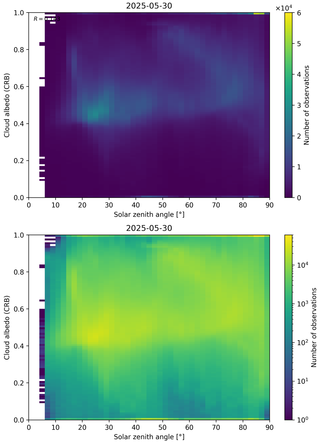
Figure 98: Scatter density plot of “Solar zenith angle” against “Cloud albedo (CRB)” for 2025-05-29 to 2025-05-31.
