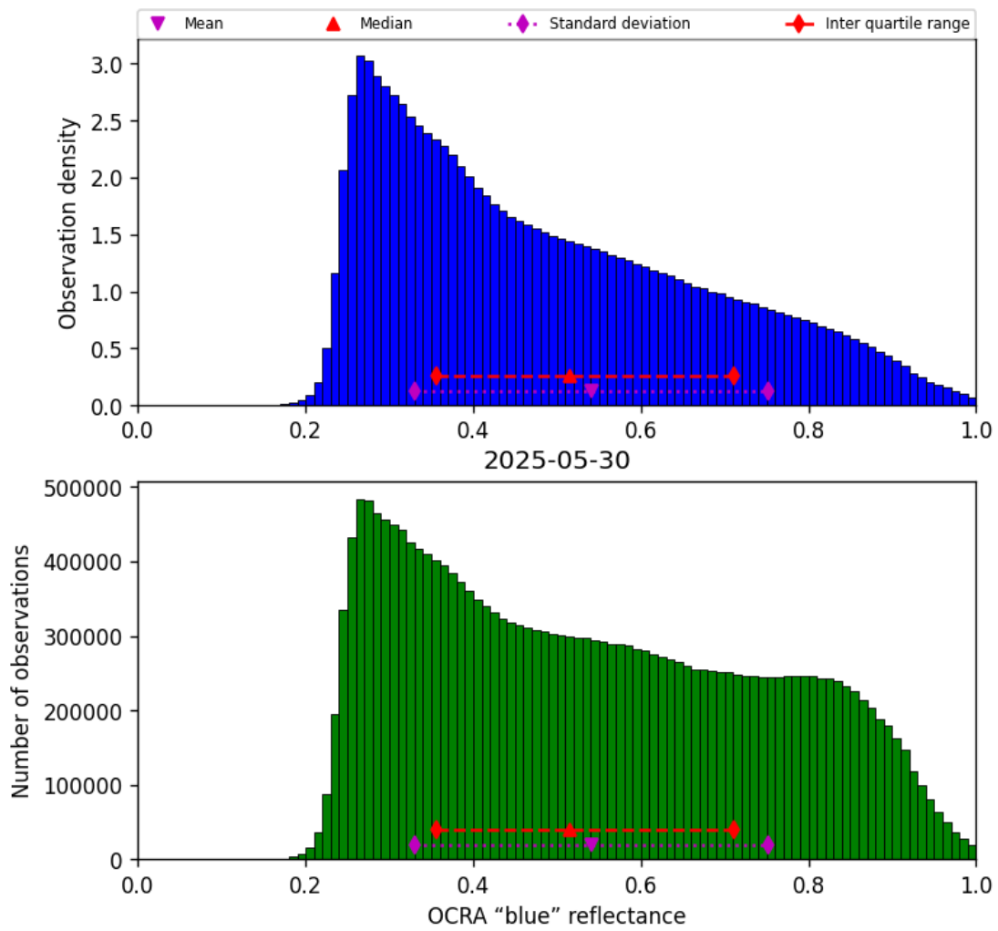
Figure 51: Histogram of “OCRA “blue” reflectance” for 2025-05-29 to 2025-05-31
