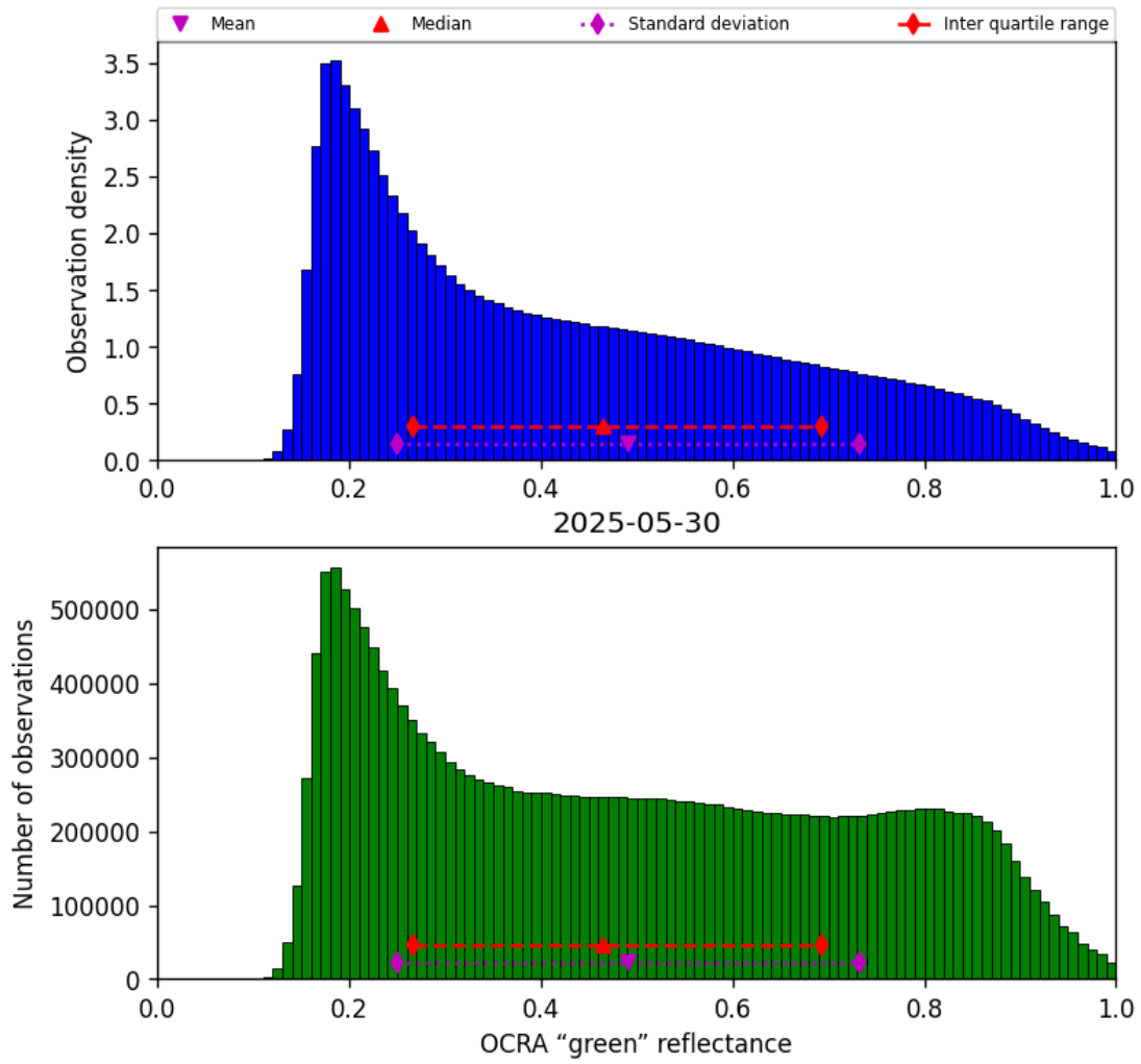
Figure 52: Histogram of “OCRA “green” reflectance” for 2025-05-29 to 2025-05-31
