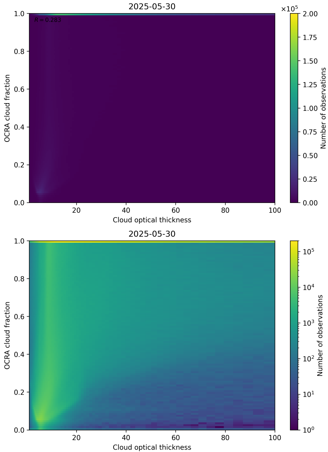
Figure 83: Scatter density plot of “Cloud optical thickness” against “OCRA cloud fraction” for 2025-05-29 to 2025-05-31.
