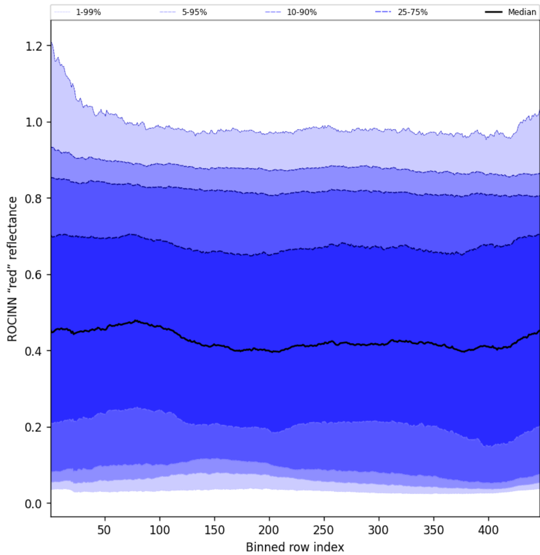
Figure 69: Along track statistics of “ROCINN “red” reflectance” for 2025-05-29 to 2025-05-31
