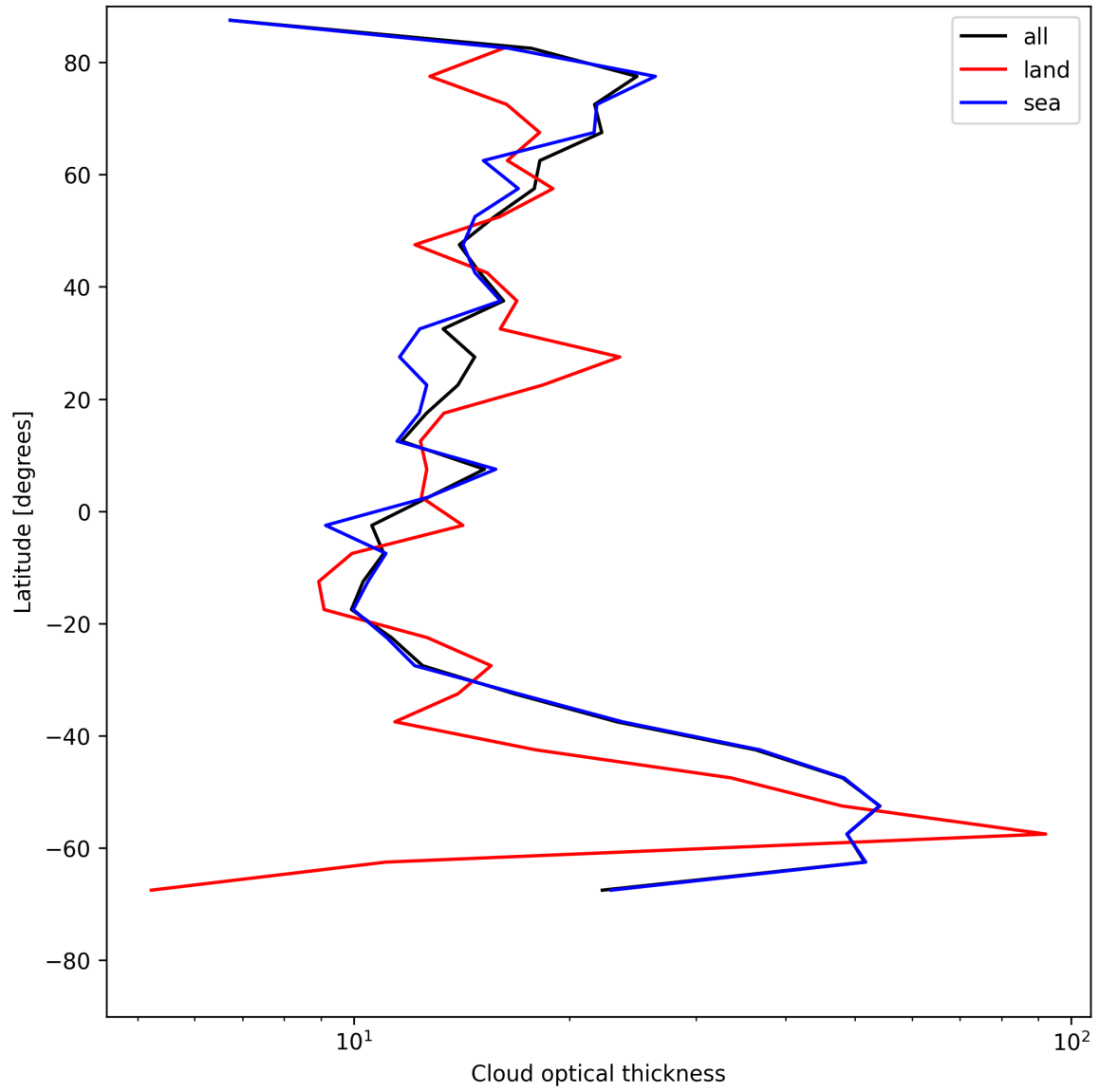
Figure 25: Zonal average of “Cloud optical thickness” for 2025-05-29 to 2025-05-31.
