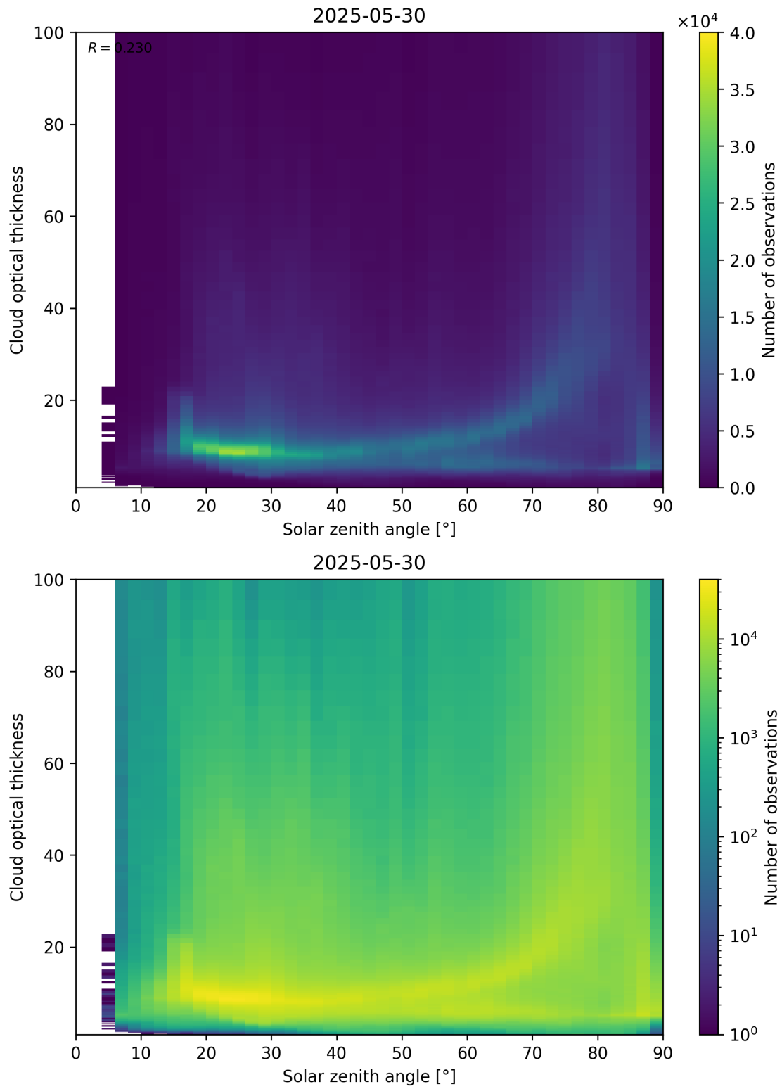
Figure 103: Scatter density plot of “Solar zenith angle” against “Cloud optical thickness” for 2025-05-29 to 2025-05-31.
