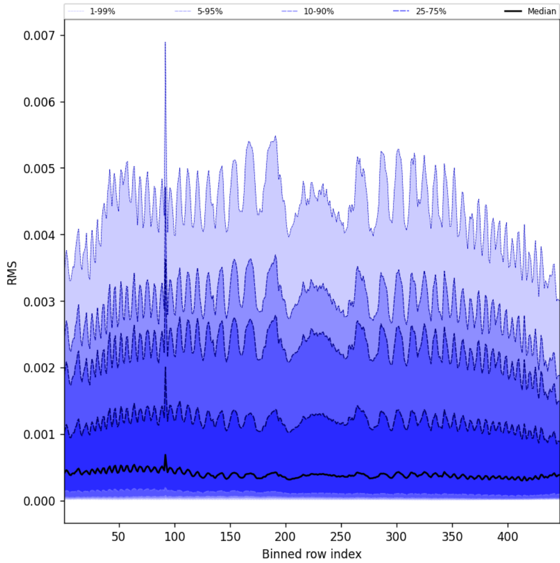
Figure 63: Along track statistics of “RMS” for 2025-05-29 to 2025-05-31
