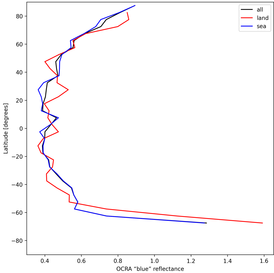
Figure 35: Zonal average of “OCRA “blue” reflectance” for 2025-05-29 to 2025-05-31.
