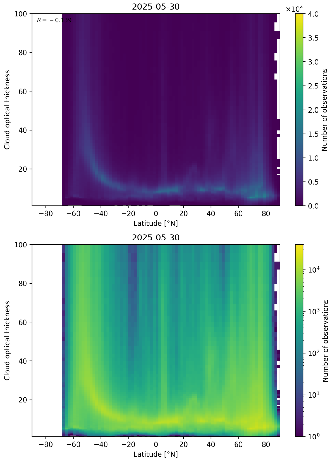
Figure 96: Scatter density plot of “Latitude” against “Cloud optical thickness” for 2025-05-29 to 2025-05-31.
