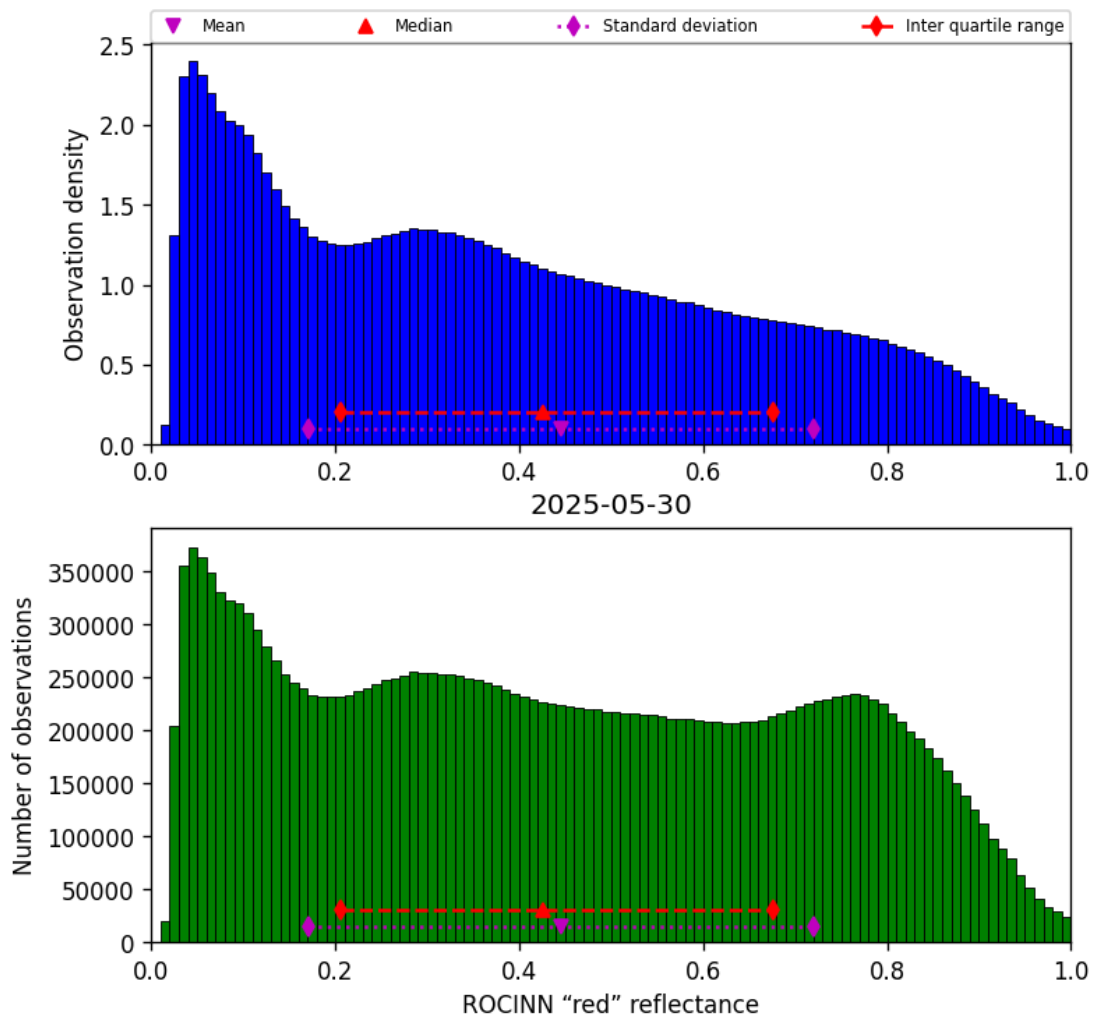
Figure 53: Histogram of “ROCINN “red” reflectance” for 2025-05-29 to 2025-05-31
