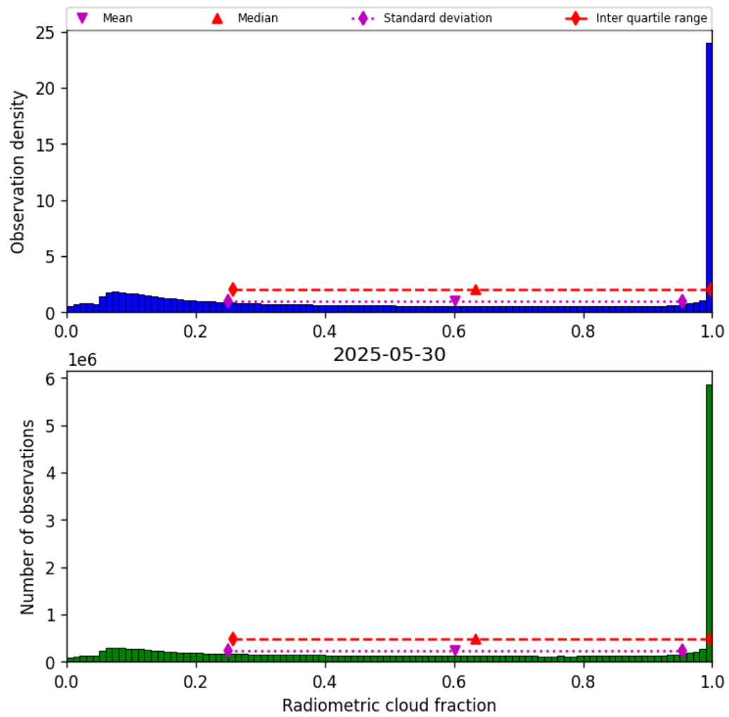
Figure 39: Histogram of “Radiometric cloud fraction” for 2025-05-29 to 2025-05-31
