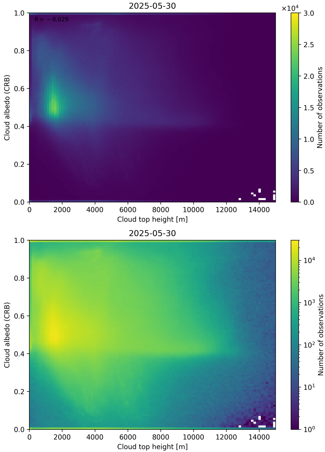
Figure 86: Scatter density plot of “Cloud top height” against “Cloud albedo (CRB)” for 2025-05-29 to 2025-05-31.
