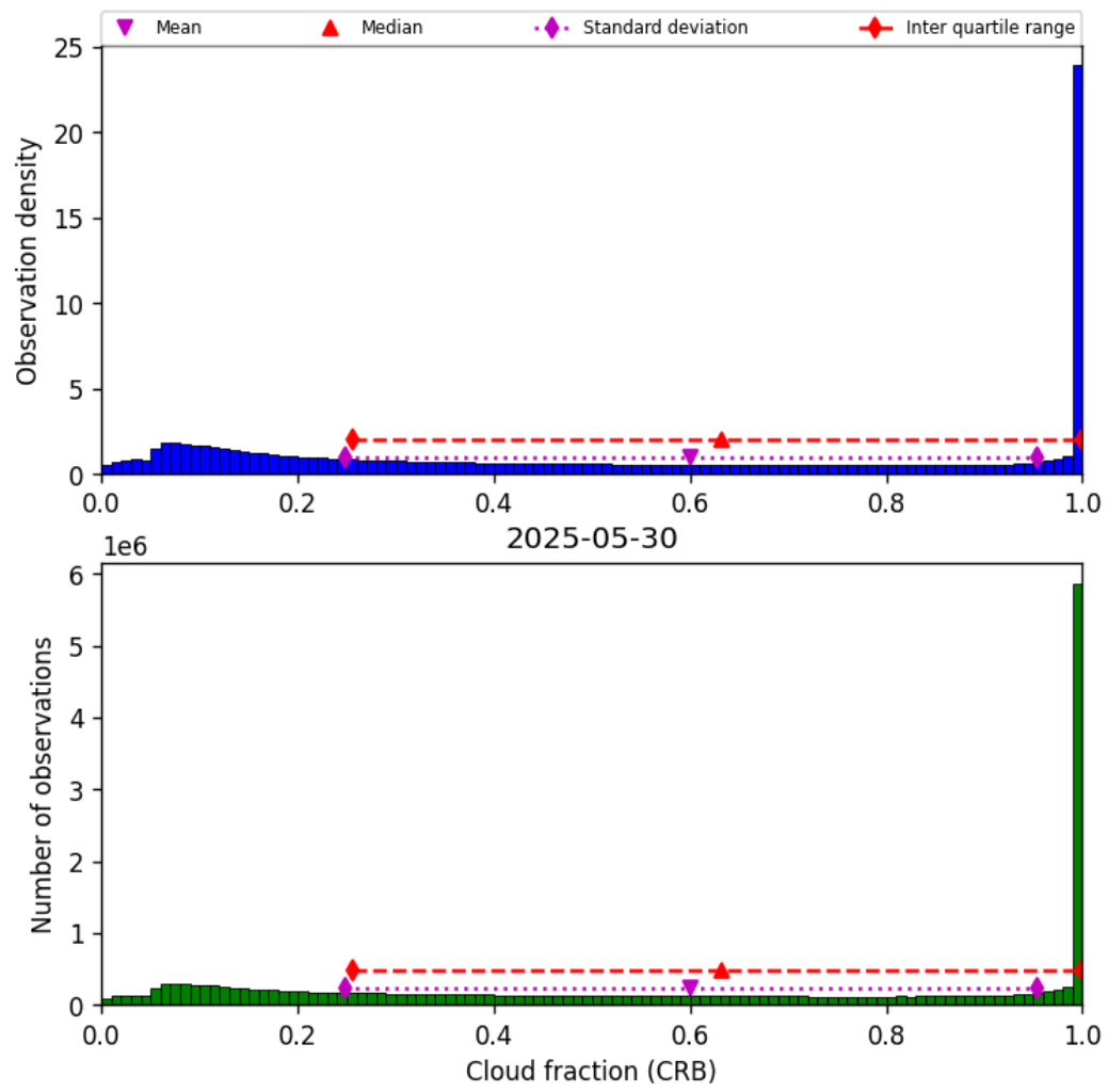
Figure 42: Histogram of “Cloud fraction (CRB)” for 2025-05-29 to 2025-05-31
