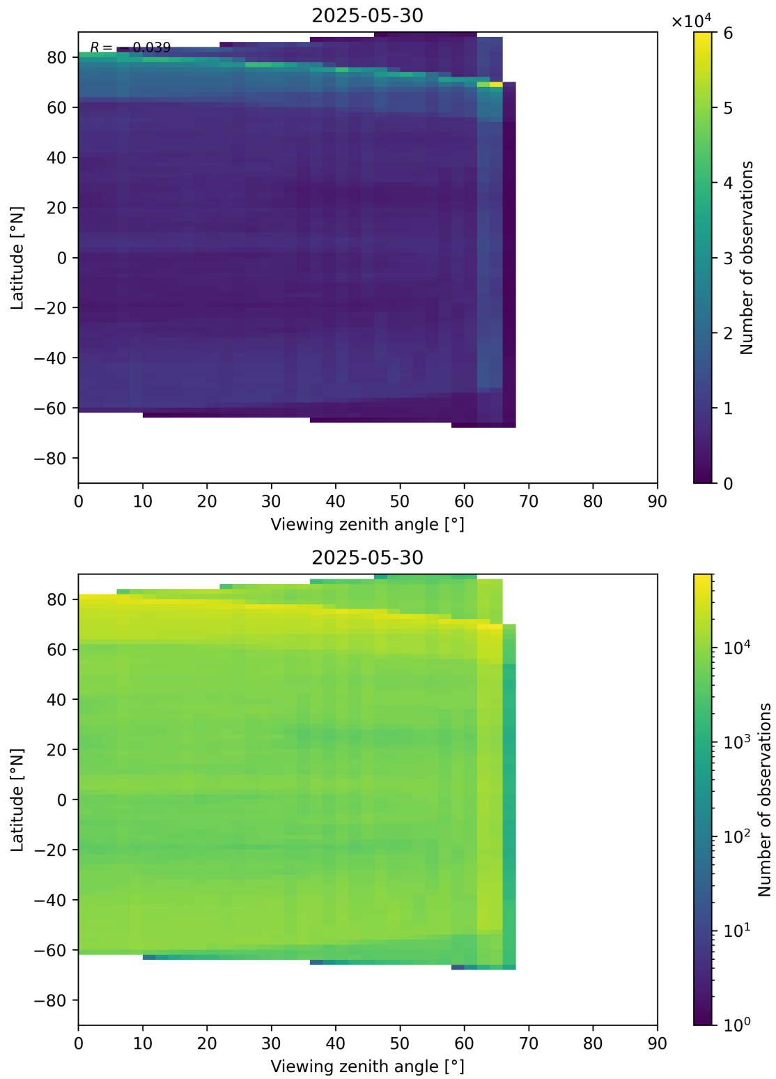
Figure 113: Scatter density plot of “Viewing zenith angle” against “Latitude” for 2025-05-29 to 2025-05-31.
