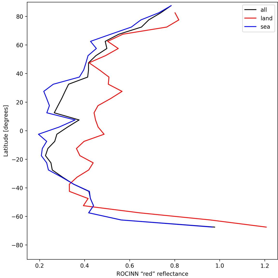
Figure 37: Zonal average of “ROCINN “red” reflectance” for 2025-05-29 to 2025-05-31.
