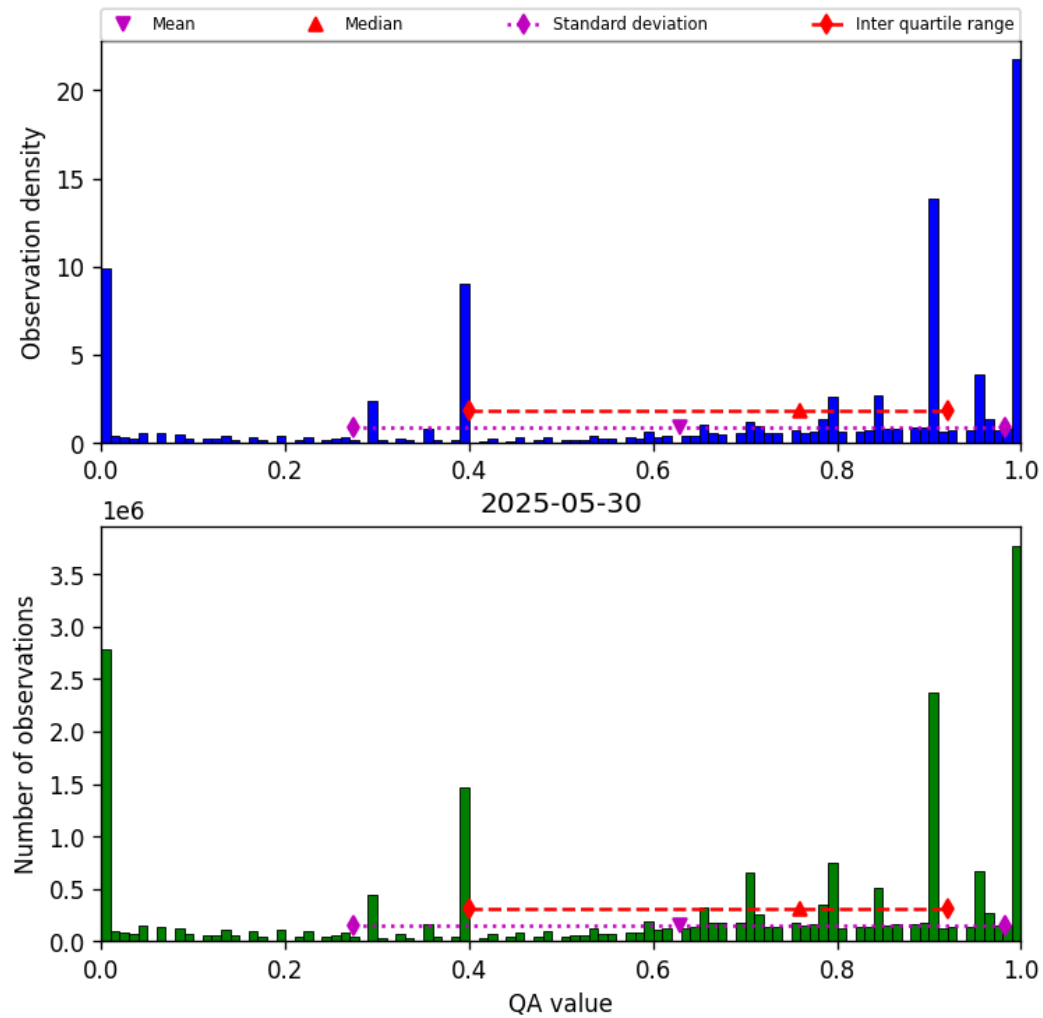
Figure 38: Histogram of “QA value” for 2025-05-29 to 2025-05-31
