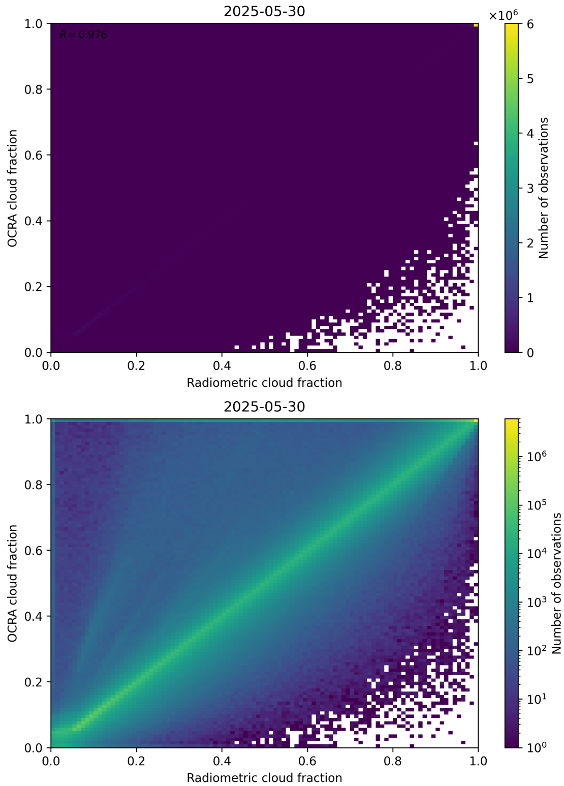
Figure 72: Scatter density plot of “Radiometric cloud fraction” against “OCRA cloud fraction” for 2025-05-29 to 2025-05-31.
