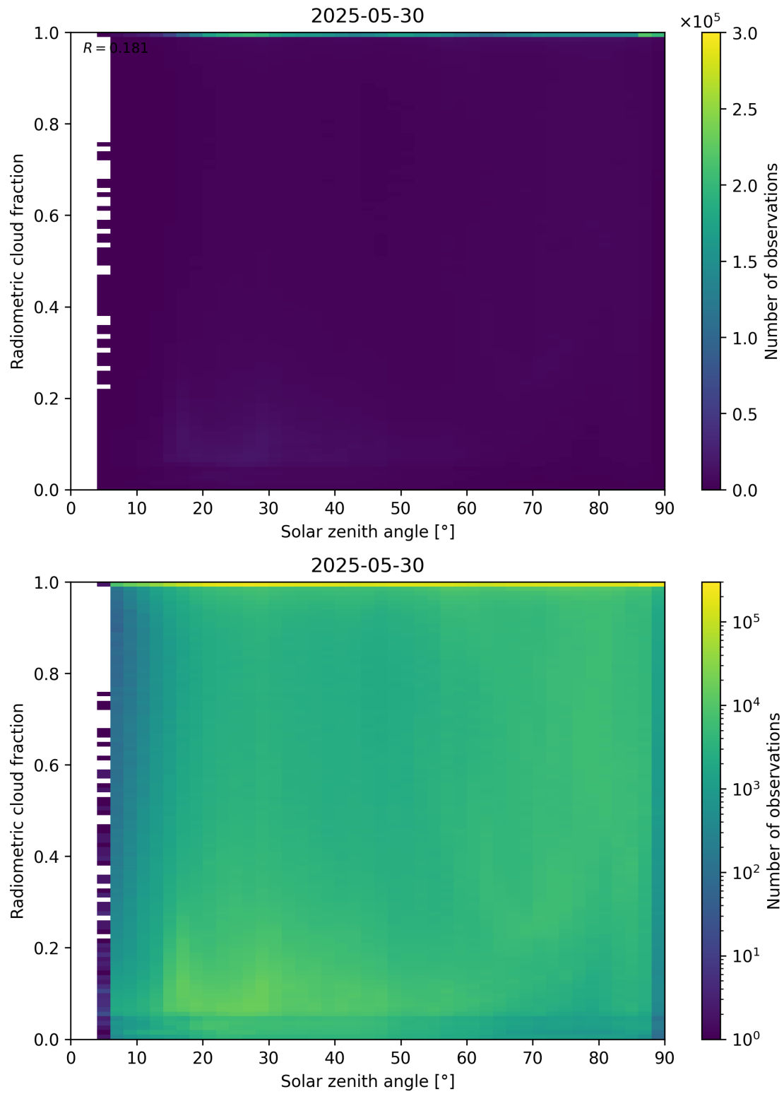
Figure 99: Scatter density plot of “Solar zenith angle” against “Radiometric cloud fraction” for 2025-05-29 to 2025-05-31.
