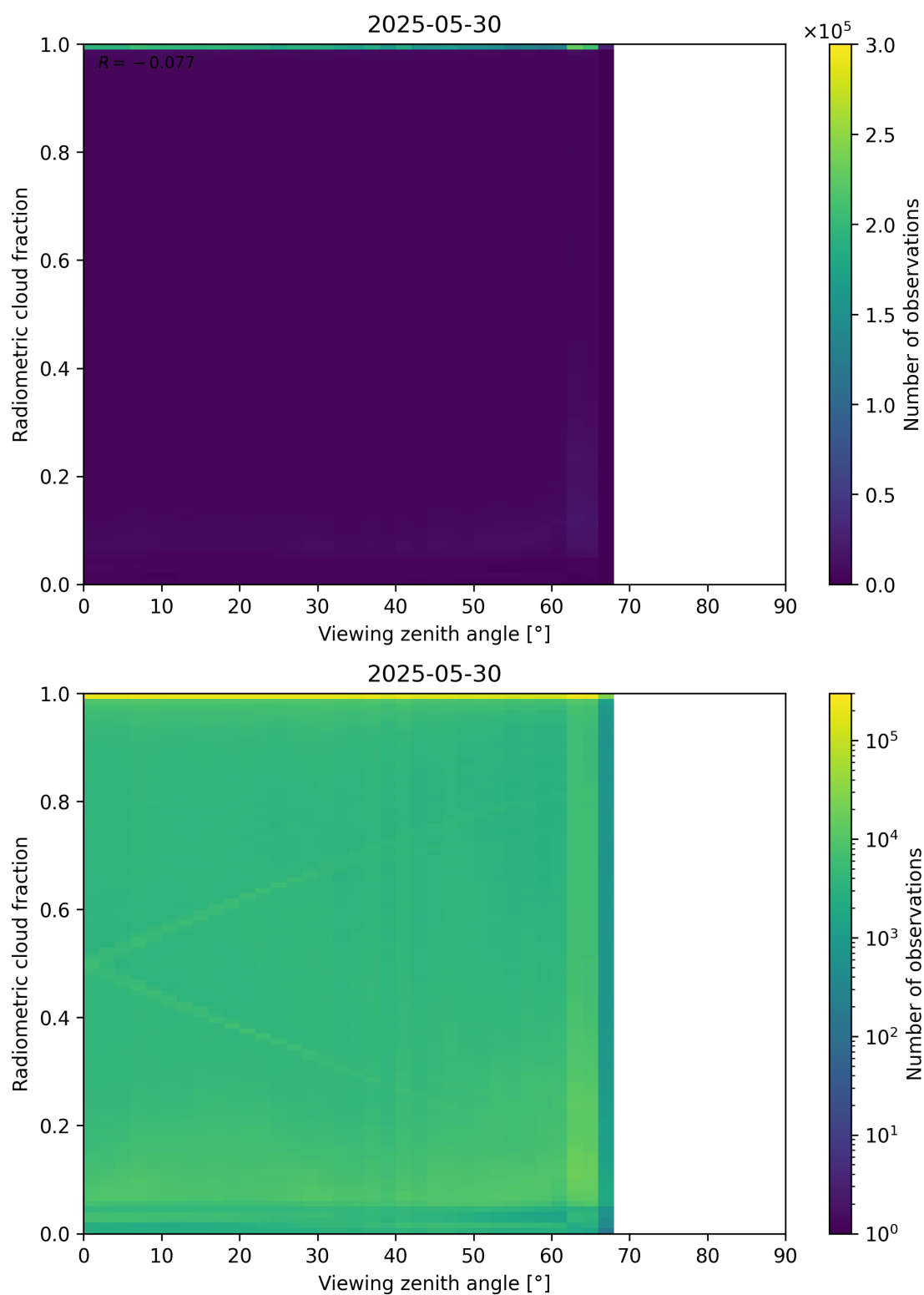
Figure 107: Scatter density plot of “Viewing zenith angle” against “Radiometric cloud fraction” for 2025-05-29 to 2025-05-31.
