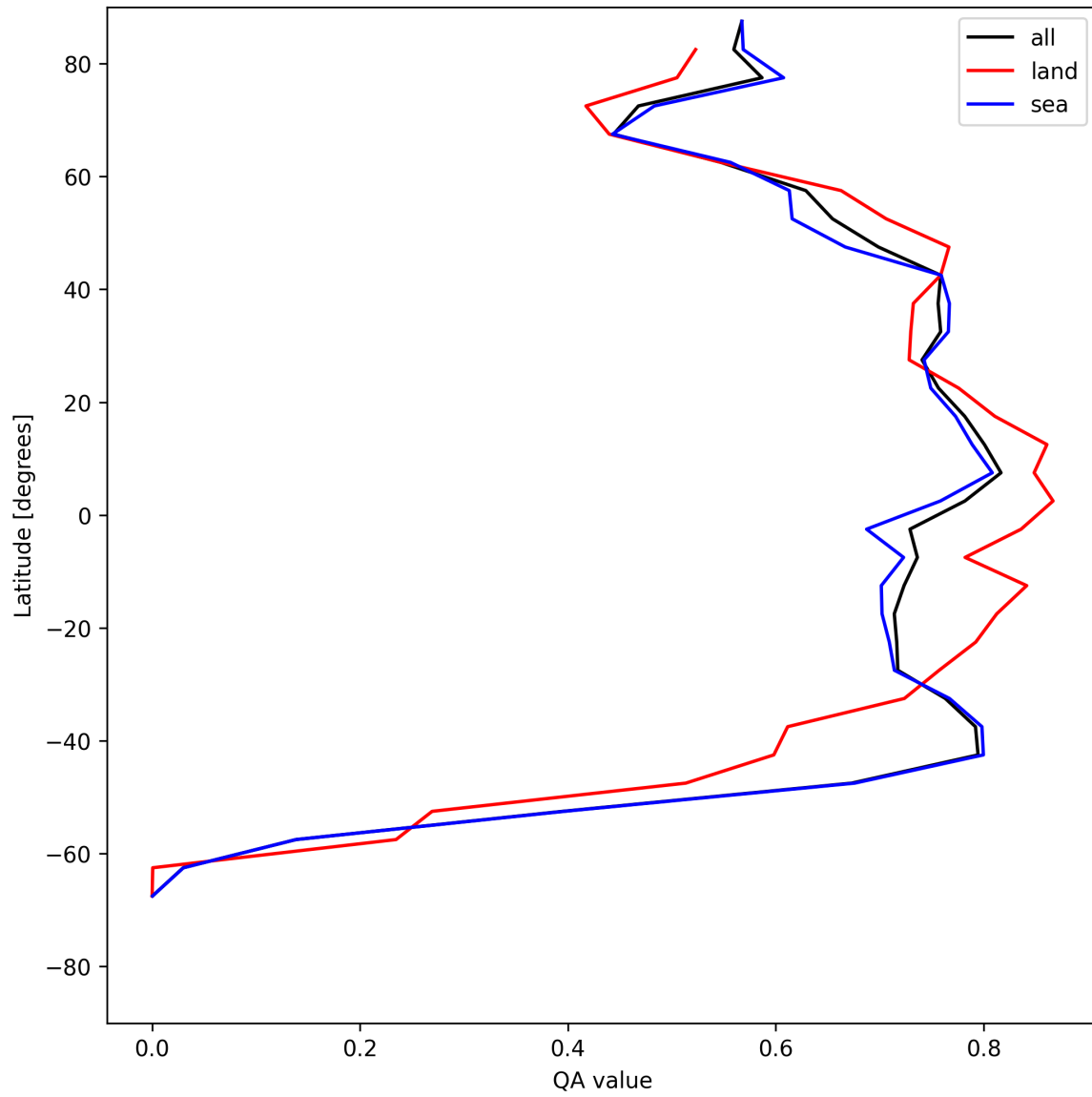
Figure 22: Zonal average of “QA value” for 2025-05-29 to 2025-05-31.
