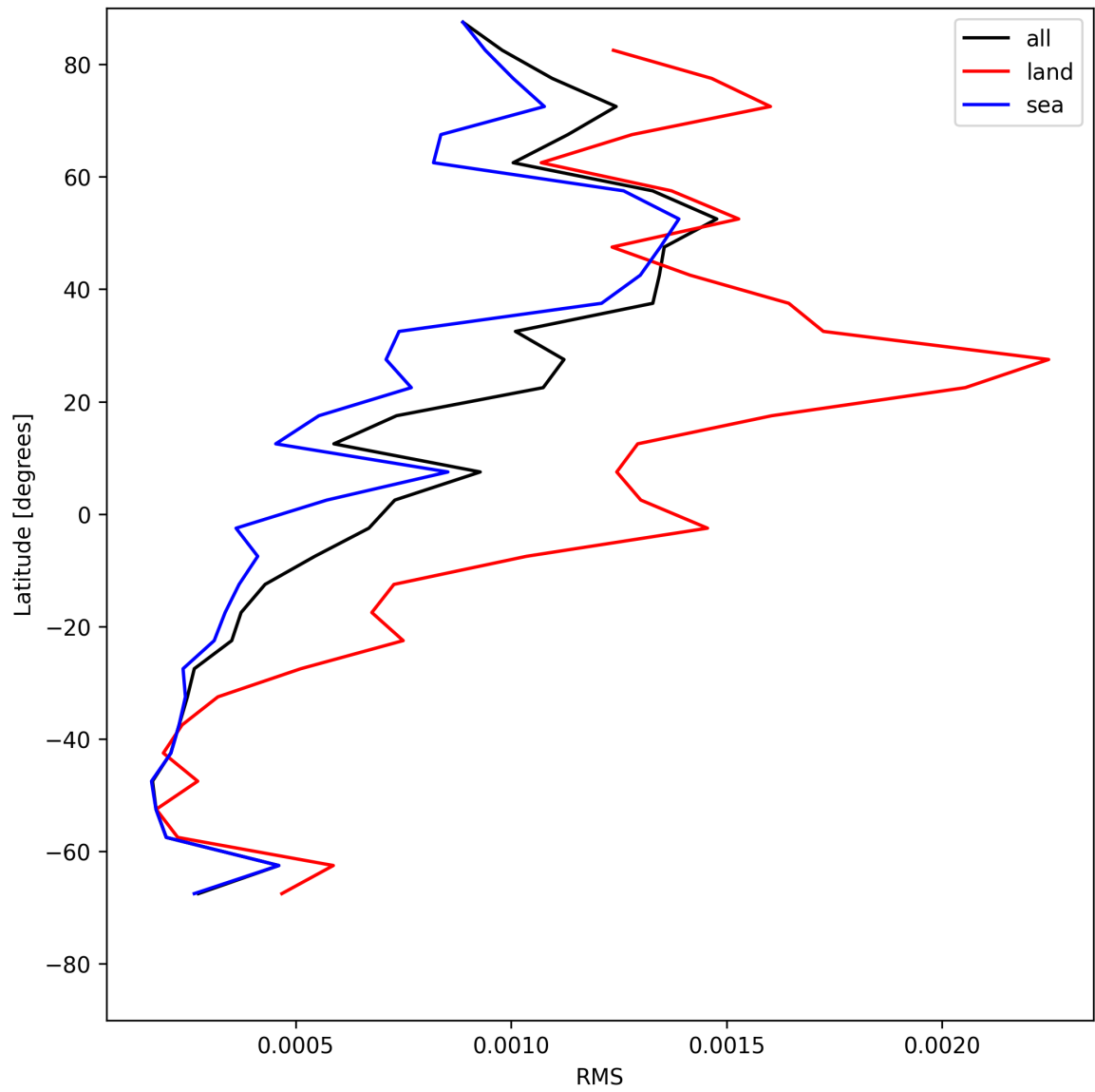
Figure 31: Zonal average of “RMS” for 2025-05-29 to 2025-05-31.
