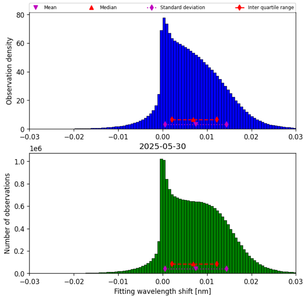
Figure 49: Histogram of “Fitting wavelength shift” for 2025-05-29 to 2025-05-31
