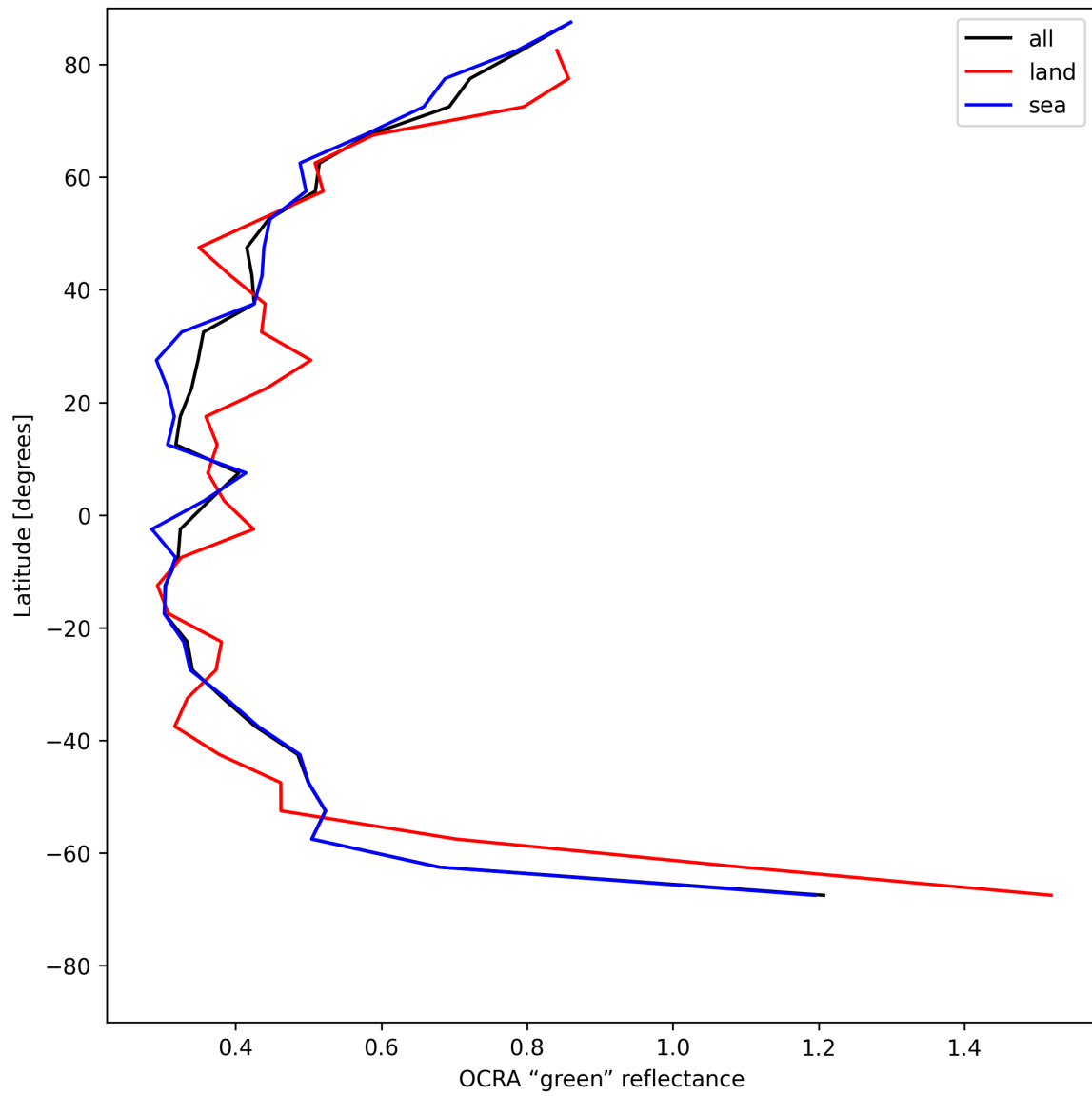
Figure 36: Zonal average of “OCRA “green” reflectance” for 2025-05-29 to 2025-05-31.
