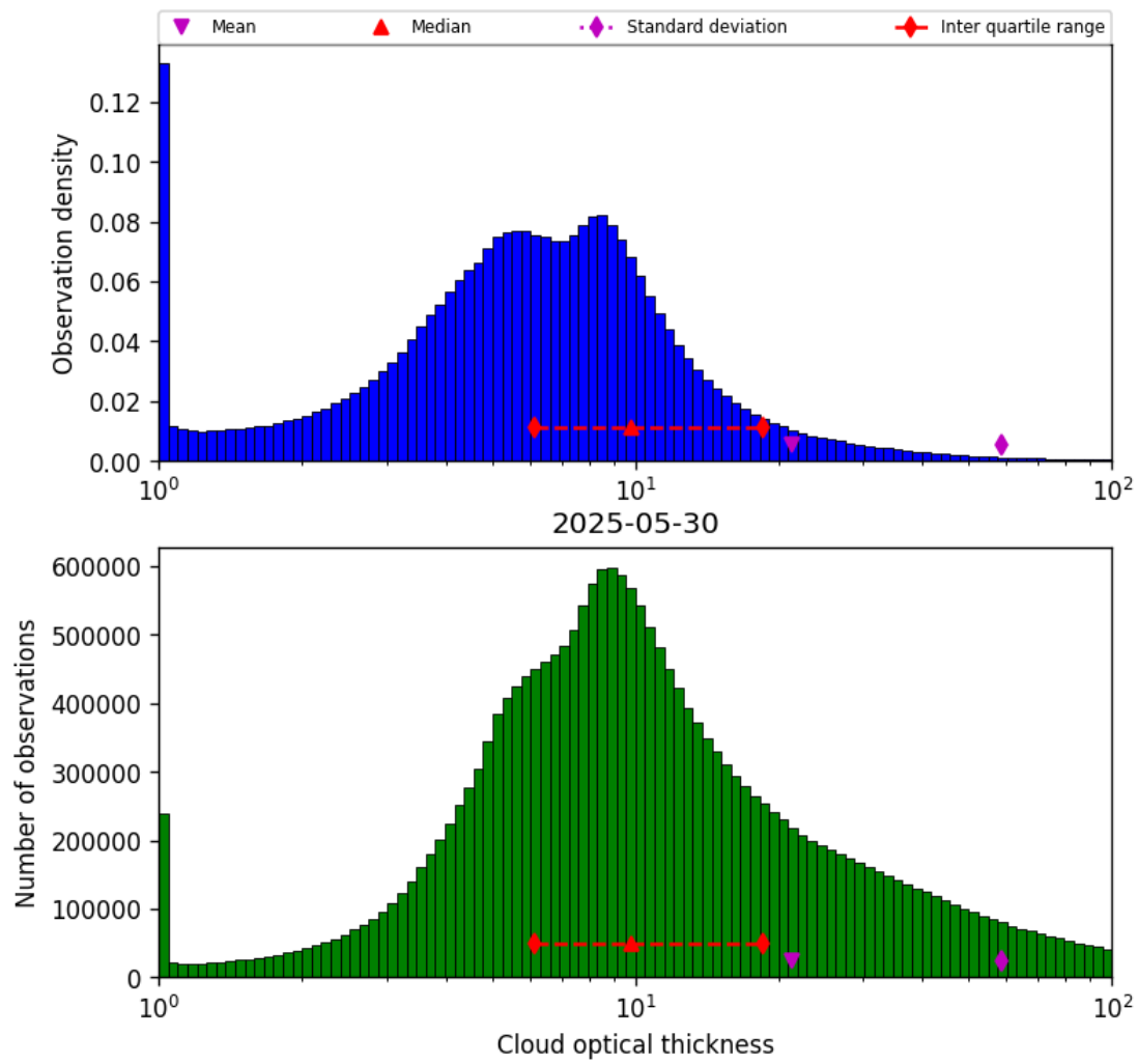
Figure 41: Histogram of “Cloud optical thickness” for 2025-05-29 to 2025-05-31
