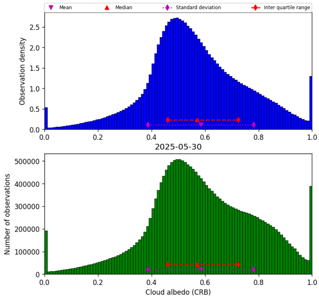
Figure 44: Histogram of “Cloud albedo (CRB)” for 2025-05-29 to 2025-05-31
