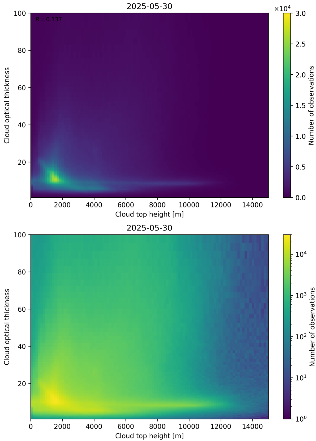
Figure 90: Scatter density plot of “Cloud top height” against “Cloud optical thickness” for 2025-05-29 to 2025-05-31.
