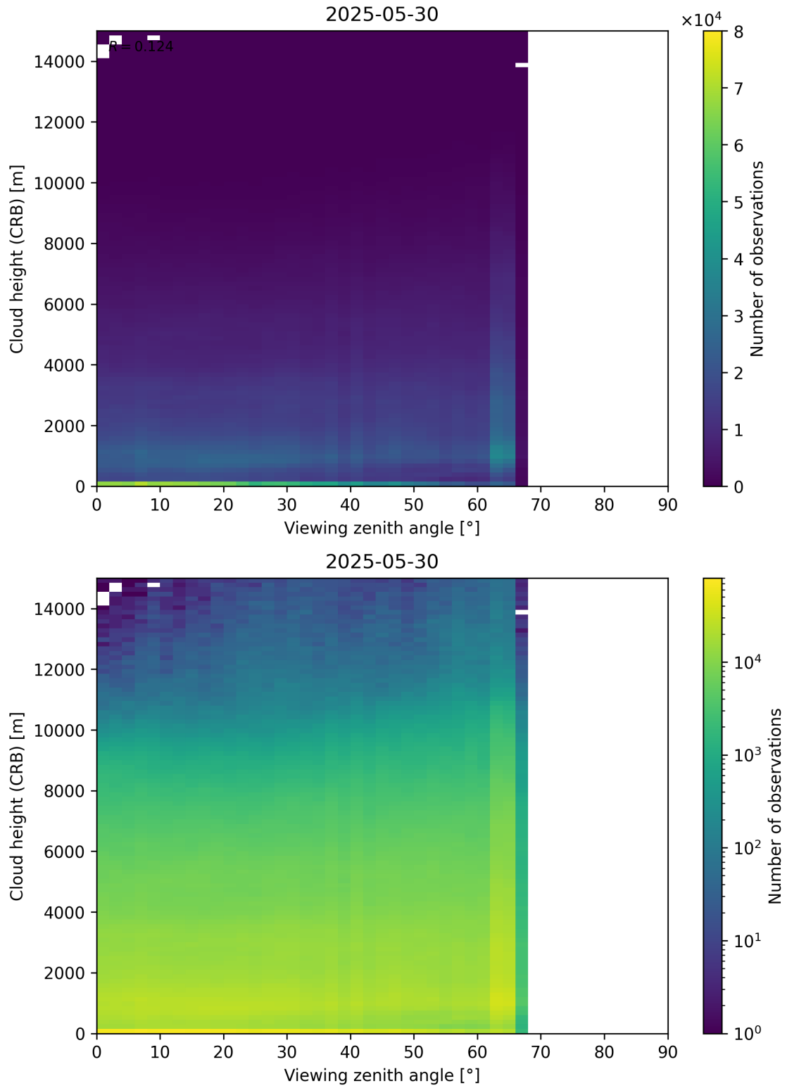
Figure 110: Scatter density plot of “Viewing zenith angle” against “Cloud height (CRB)” for 2025-05-29 to 2025-05-31.
