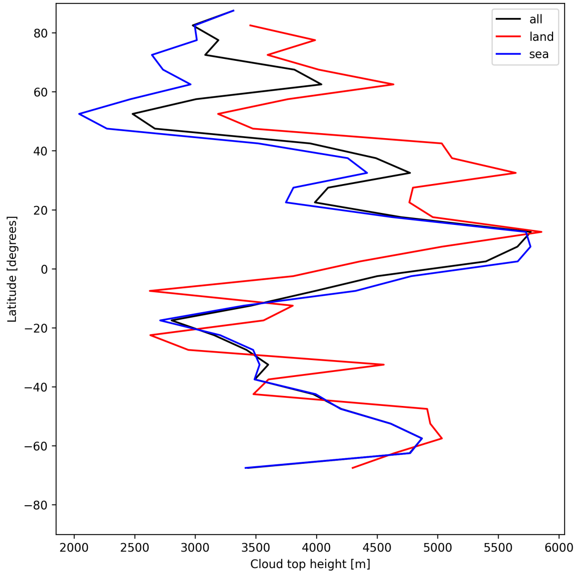
Figure 24: Zonal average of “Cloud top height” for 2025-05-29 to 2025-05-31.
