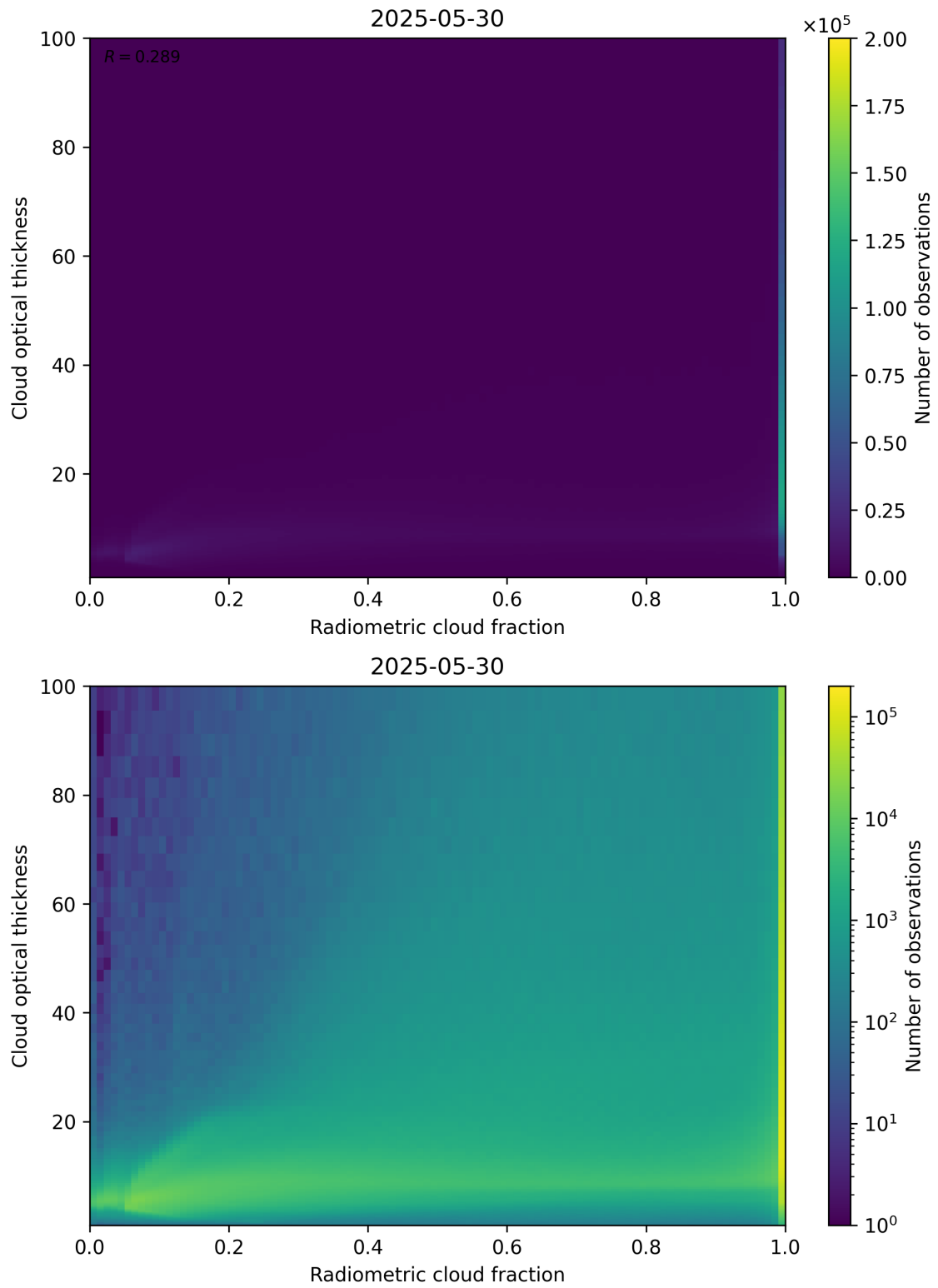
Figure 75: Scatter density plot of “Radiometric cloud fraction” against “Cloud optical thickness” for 2025-05-29 to 2025-05-31.
