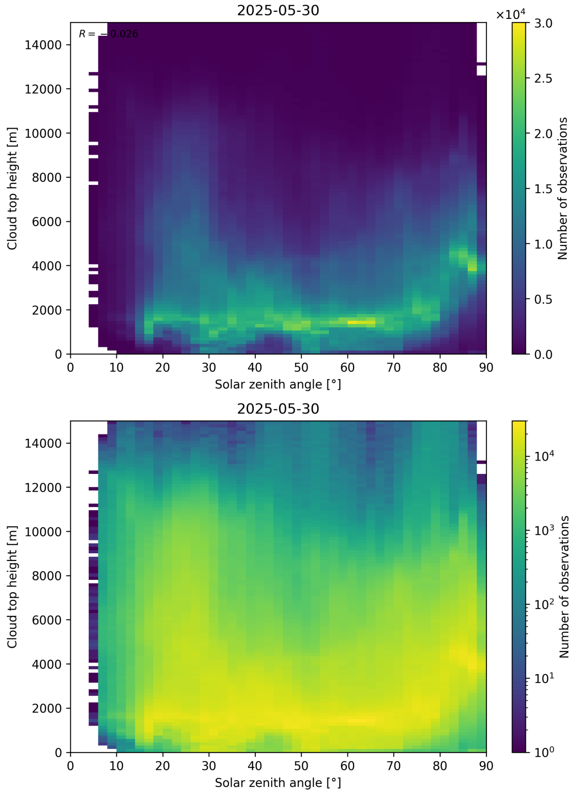
Figure 104: Scatter density plot of “Solar zenith angle” against “Cloud top height” for 2025-05-29 to 2025-05-31.
