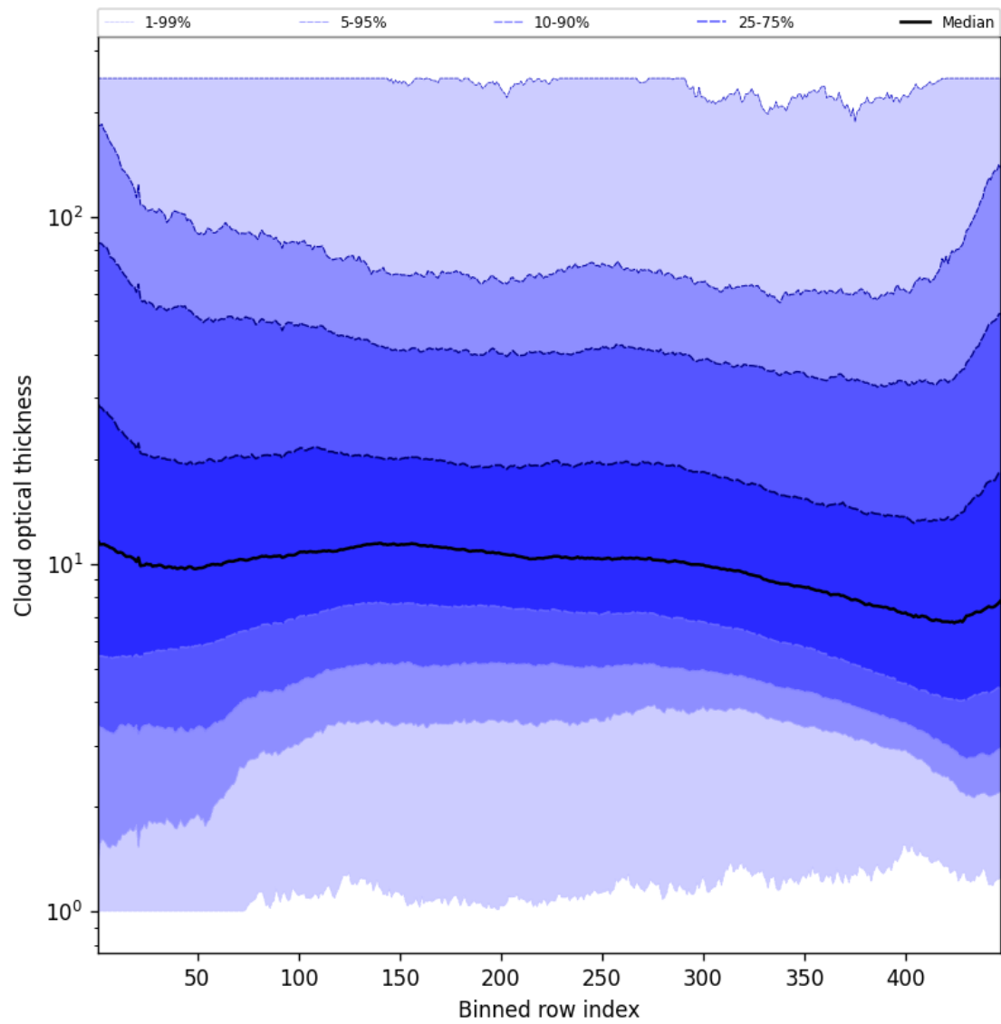
Figure 57: Along track statistics of “Cloud optical thickness” for 2025-05-29 to 2025-05-31
