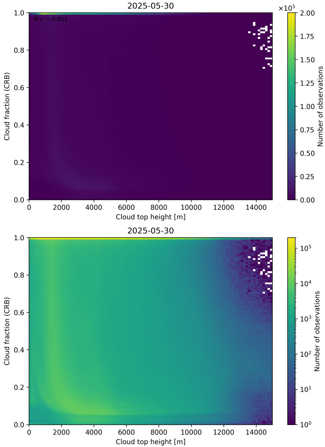
Figure 88: Scatter density plot of “Cloud top height” against “Cloud fraction (CRB)” for 2025-05-29 to 2025-05-31.
