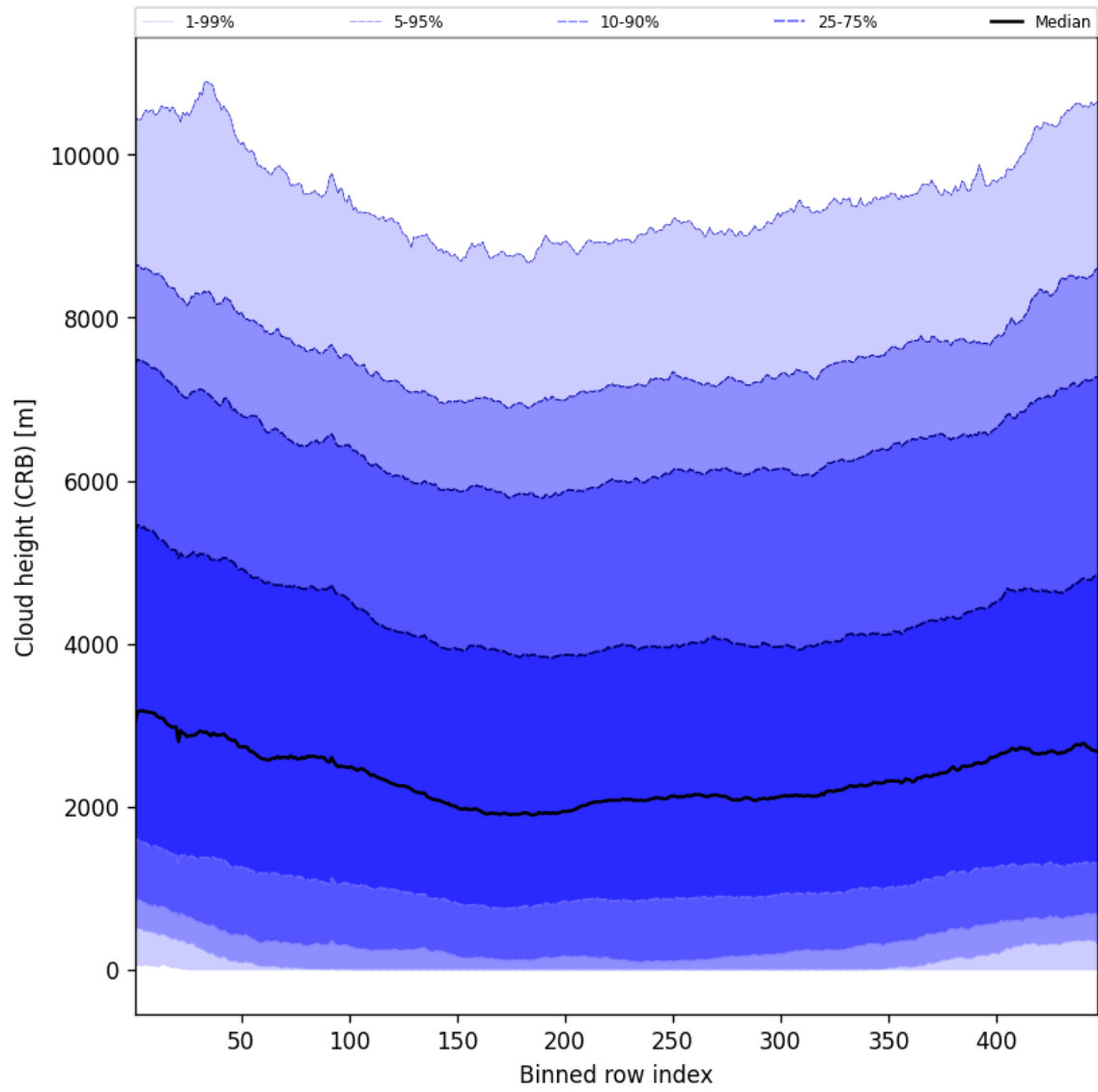
Figure 59: Along track statistics of “Cloud height (CRB)” for 2025-05-29 to 2025-05-31
