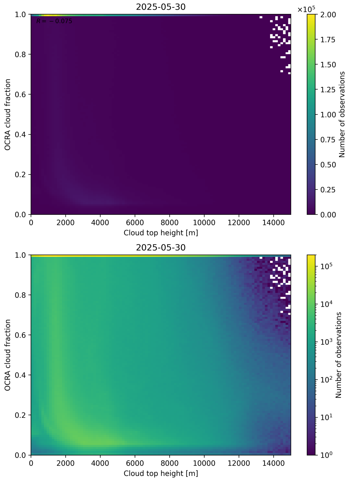
Figure 87: Scatter density plot of “Cloud top height” against “OCRA cloud fraction” for 2025-05-29 to 2025-05-31.
