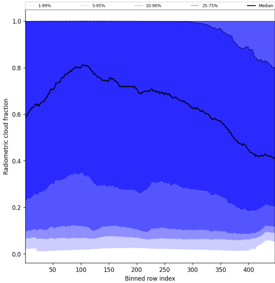
Figure 55: Along track statistics of “Radiometric cloud fraction” for 2025-05-29 to 2025-05-31
