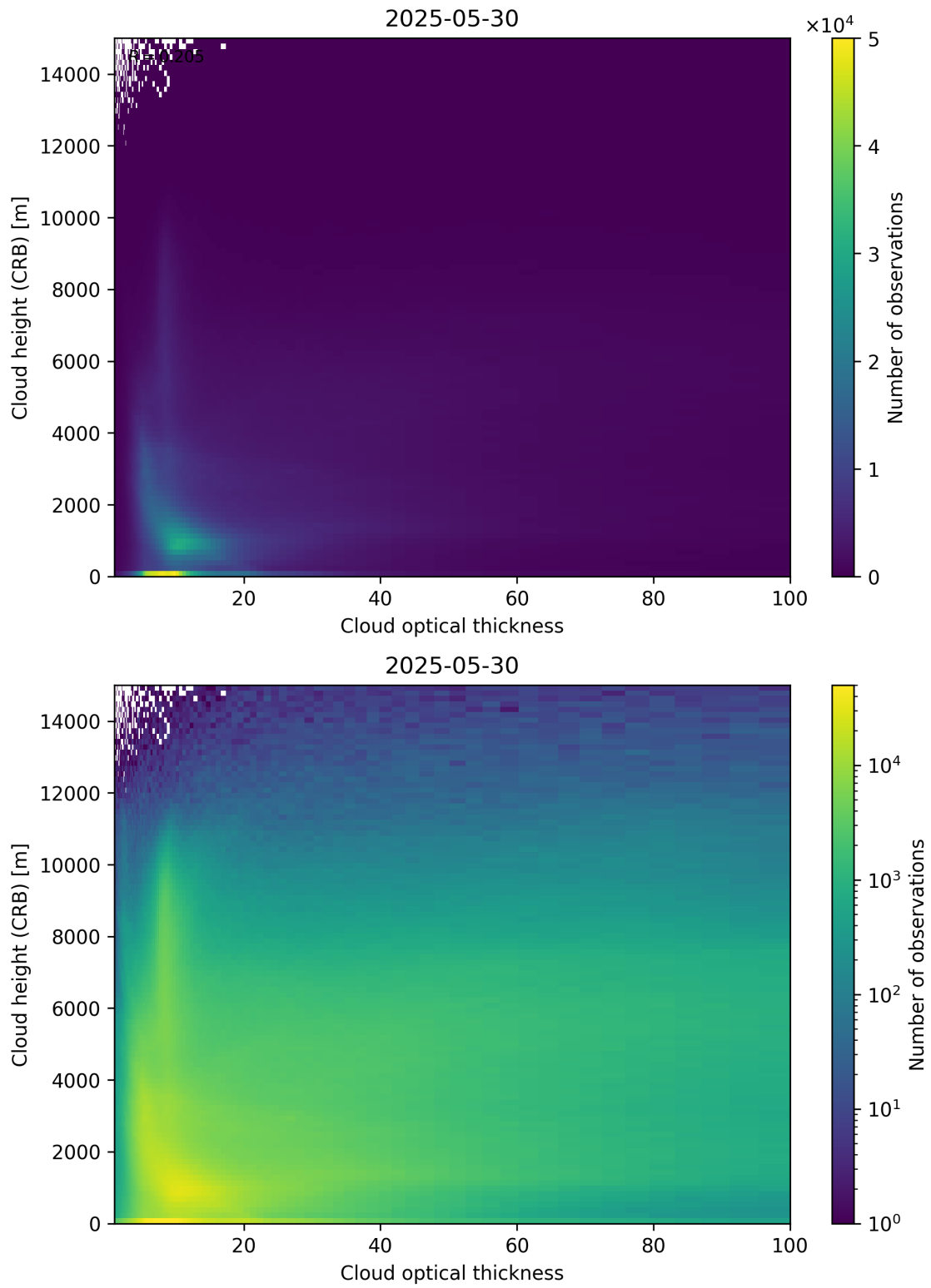
Figure 85: Scatter density plot of “Cloud optical thickness” against “Cloud height (CRB)” for 2025-05-29 to 2025-05-31.
