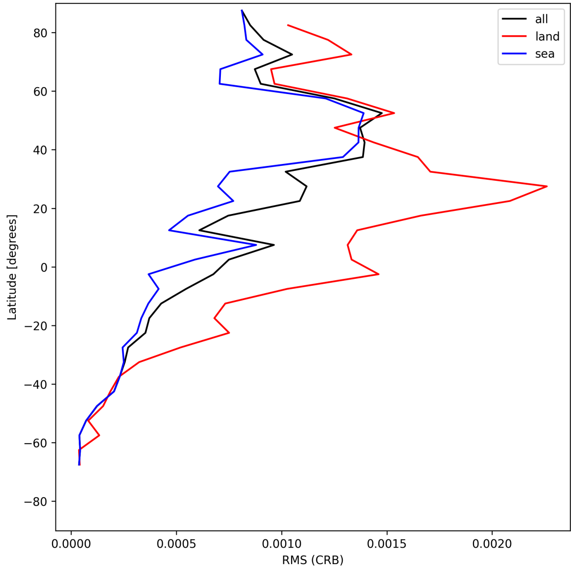
Figure 32: Zonal average of “RMS (CRB)” for 2025-05-29 to 2025-05-31.
