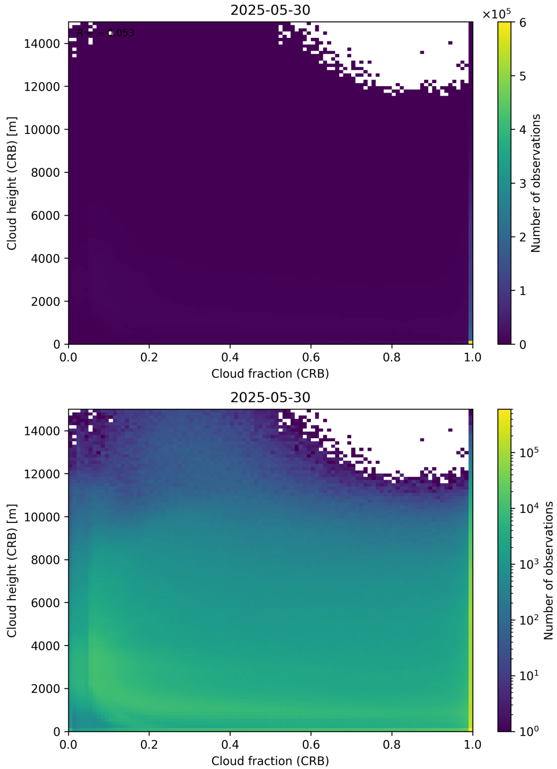
Figure 79: Scatter density plot of “Cloud fraction (CRB)” against “Cloud height (CRB)” for 2025-05-29 to 2025-05-31.
