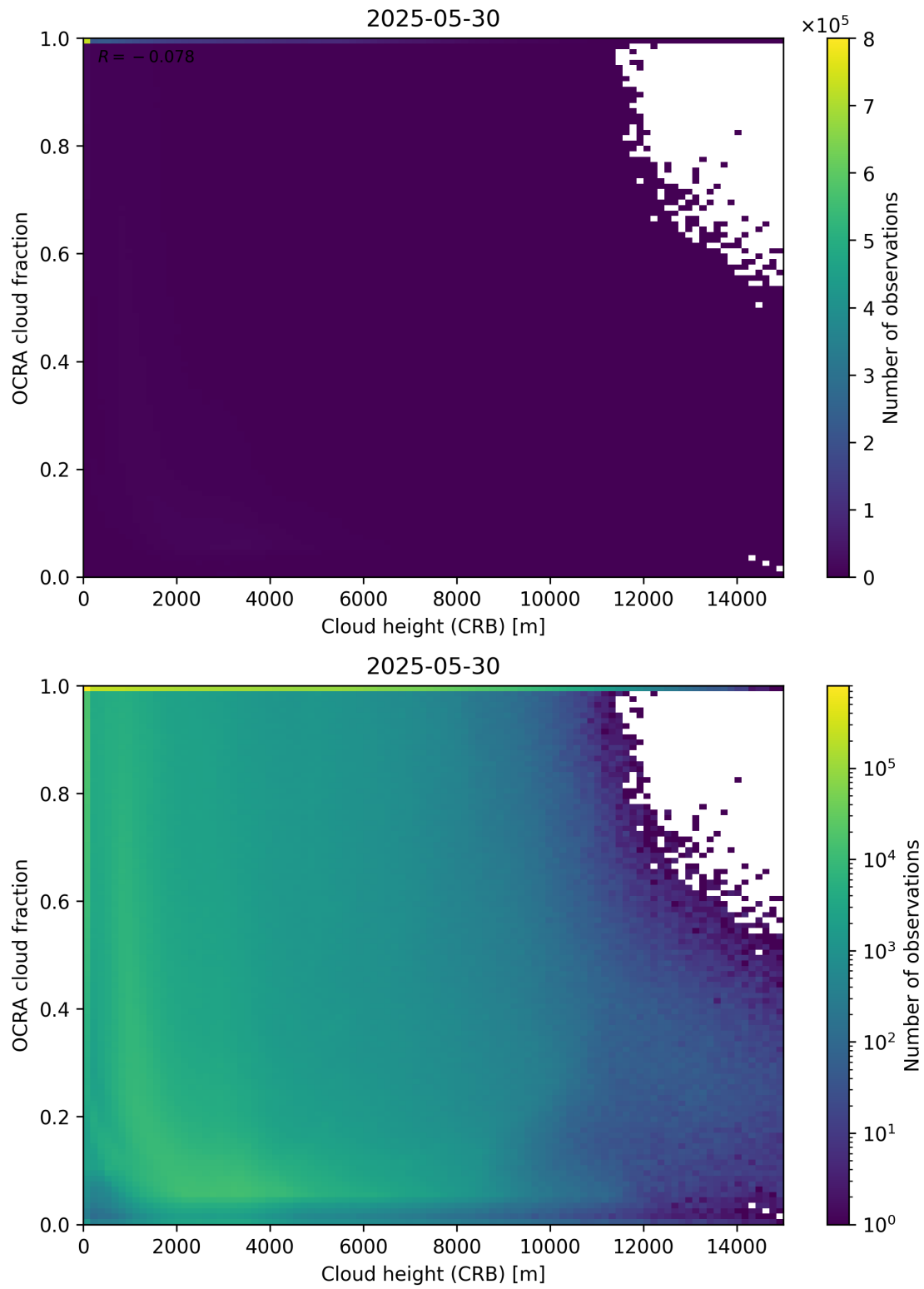
Figure 81: Scatter density plot of “Cloud height (CRB)” against “OCRA cloud fraction” for 2025-05-29 to 2025-05-31.
