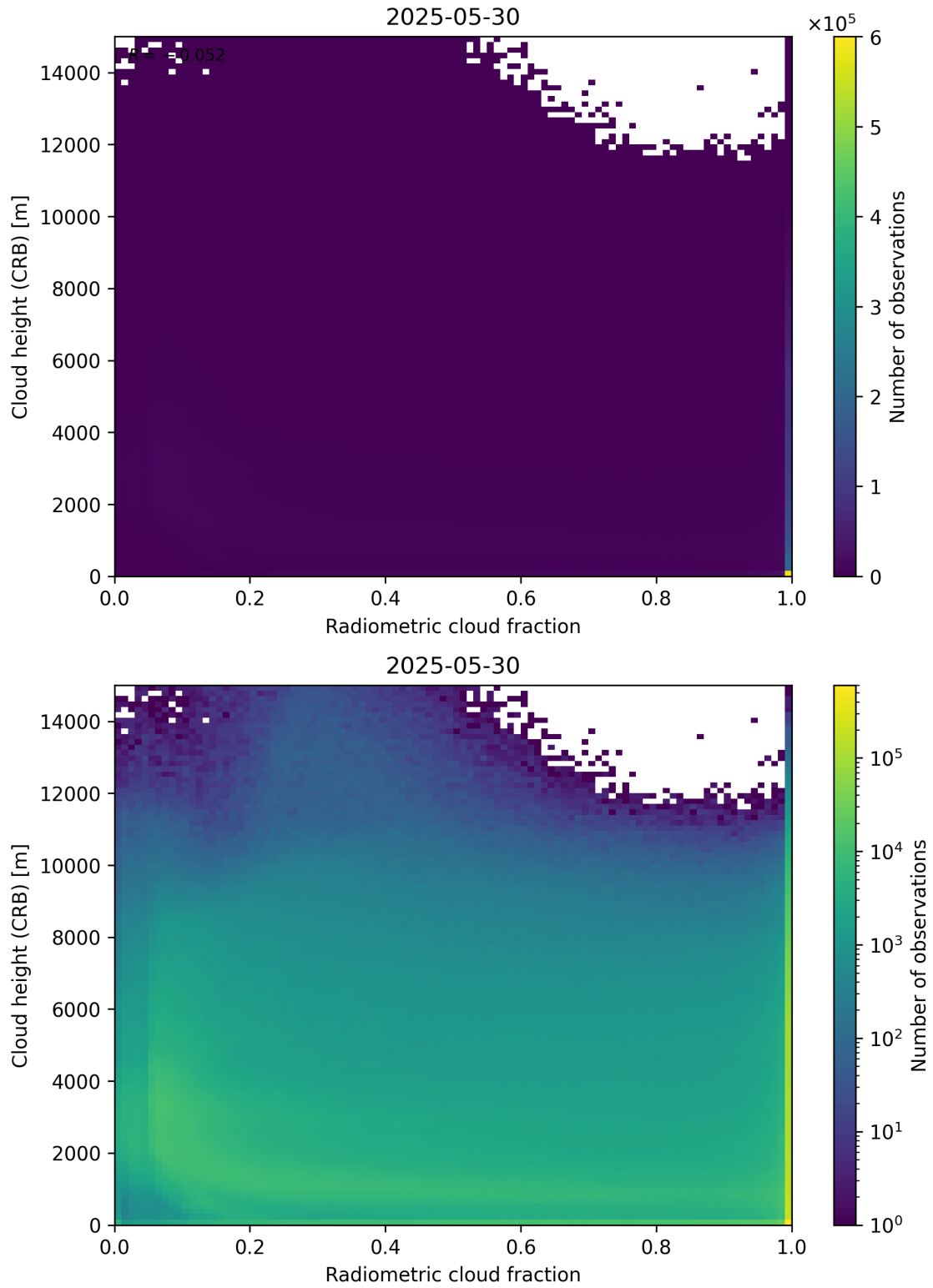
Figure 74: Scatter density plot of “Radiometric cloud fraction” against “Cloud height (CRB)” for 2025-05-29 to 2025-05-31.
