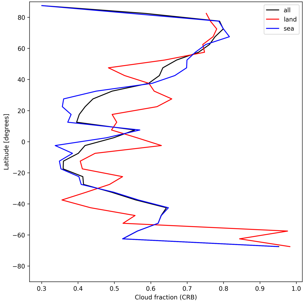
Figure 26: Zonal average of “Cloud fraction (CRB)” for 2025-05-29 to 2025-05-31.
