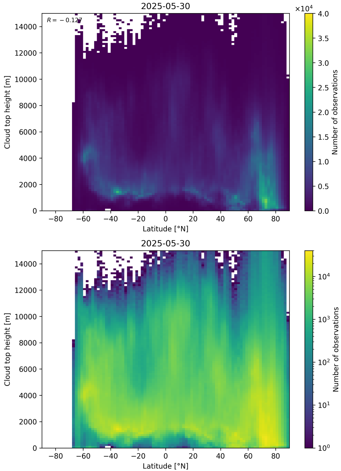
Figure 97: Scatter density plot of “Latitude” against “Cloud top height” for 2025-05-29 to 2025-05-31.
