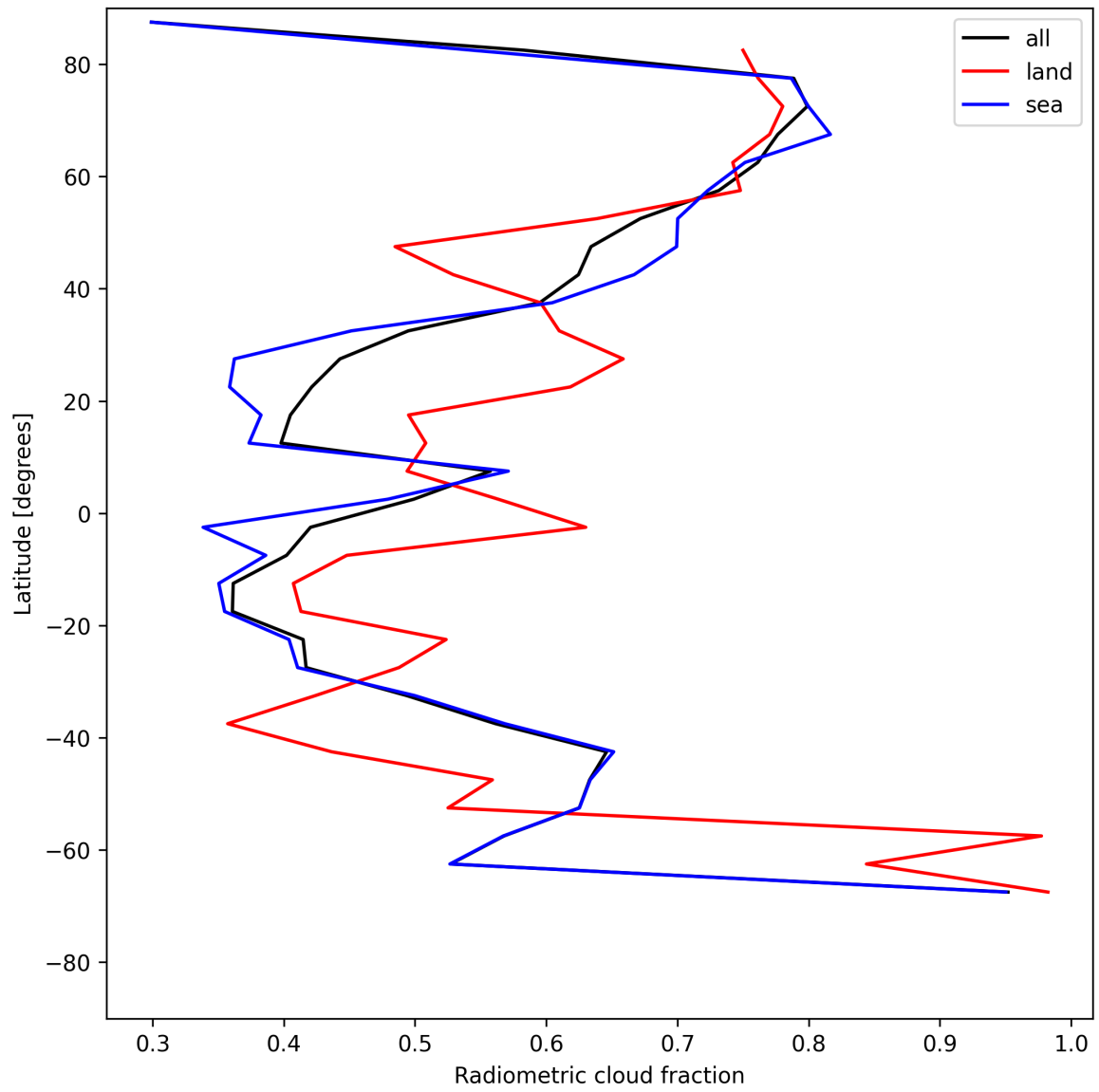
Figure 23: Zonal average of “Radiometric cloud fraction” for 2025-05-29 to 2025-05-31.
