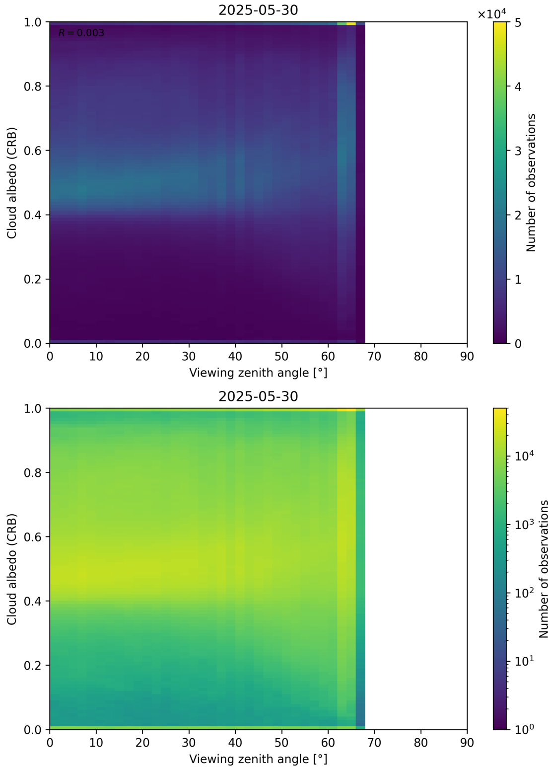
Figure 106: Scatter density plot of “Viewing zenith angle” against “Cloud albedo (CRB)” for 2025-05-29 to 2025-05-31.
