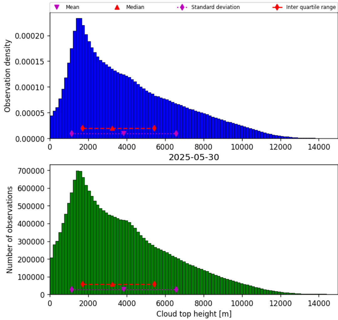
Figure 40: Histogram of “Cloud top height” for 2025-05-29 to 2025-05-31
