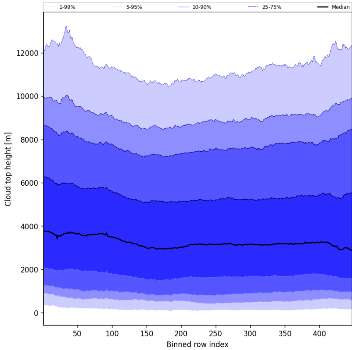
Figure 56: Along track statistics of “Cloud top height” for 2025-05-29 to 2025-05-31
