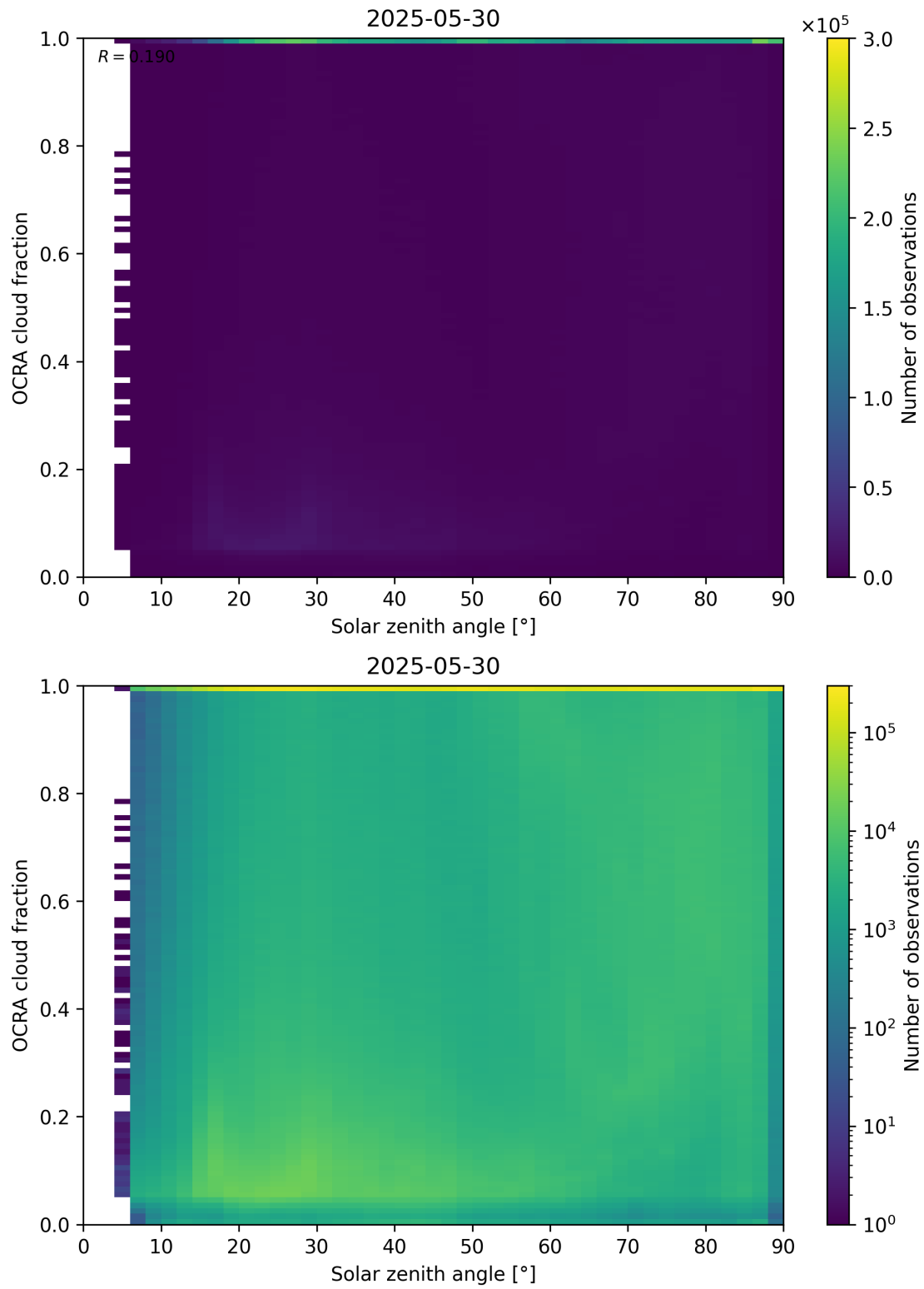
Figure 100: Scatter density plot of “Solar zenith angle” against “OCRA cloud fraction” for 2025-05-29 to 2025-05-31.
