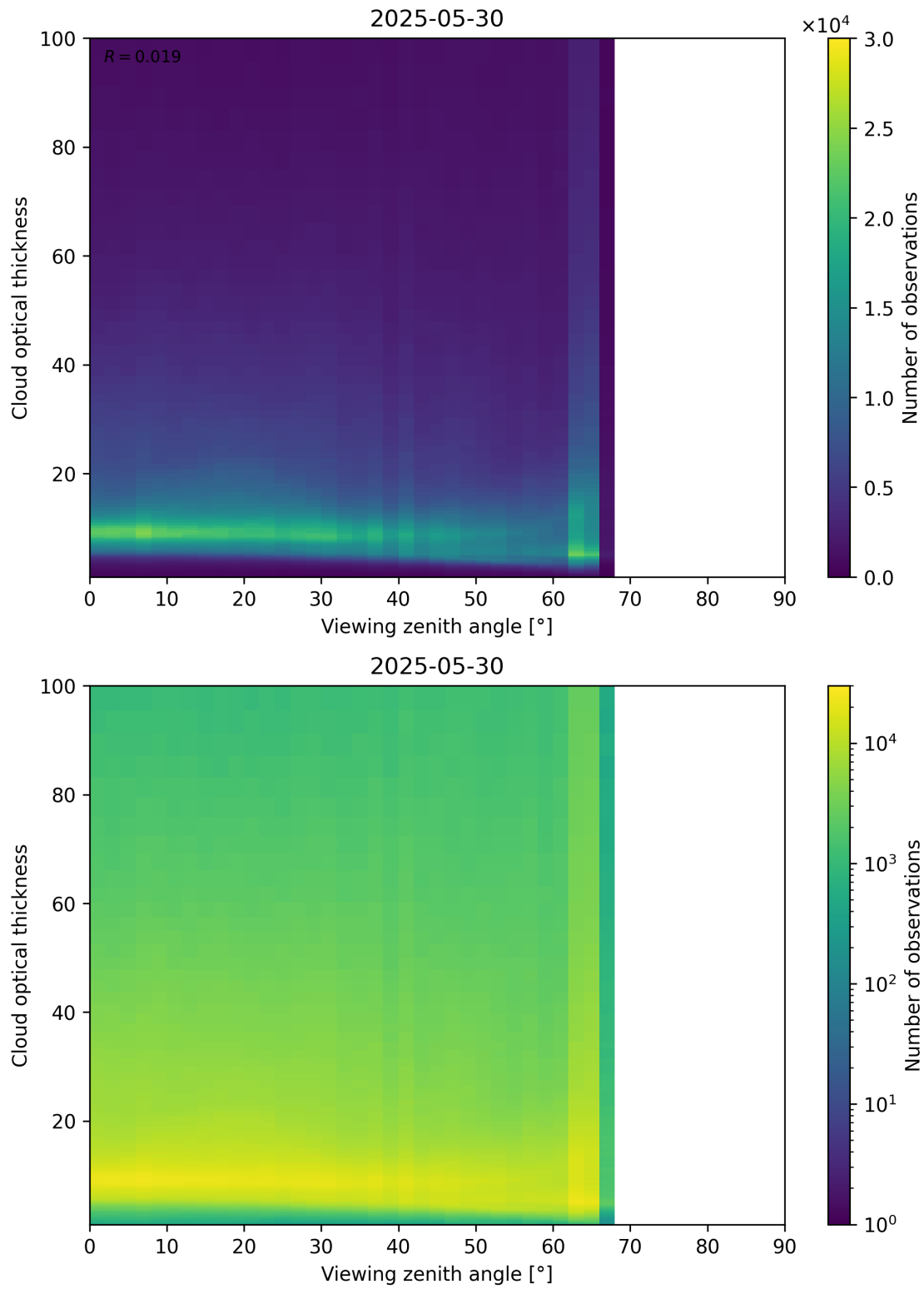
Figure 111: Scatter density plot of “Viewing zenith angle” against “Cloud optical thickness” for 2025-05-29 to 2025-05-31.
