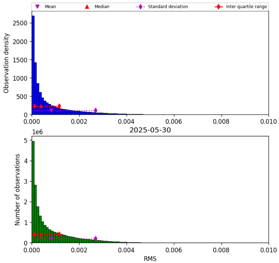
Figure 47: Histogram of “RMS” for 2025-05-29 to 2025-05-31
