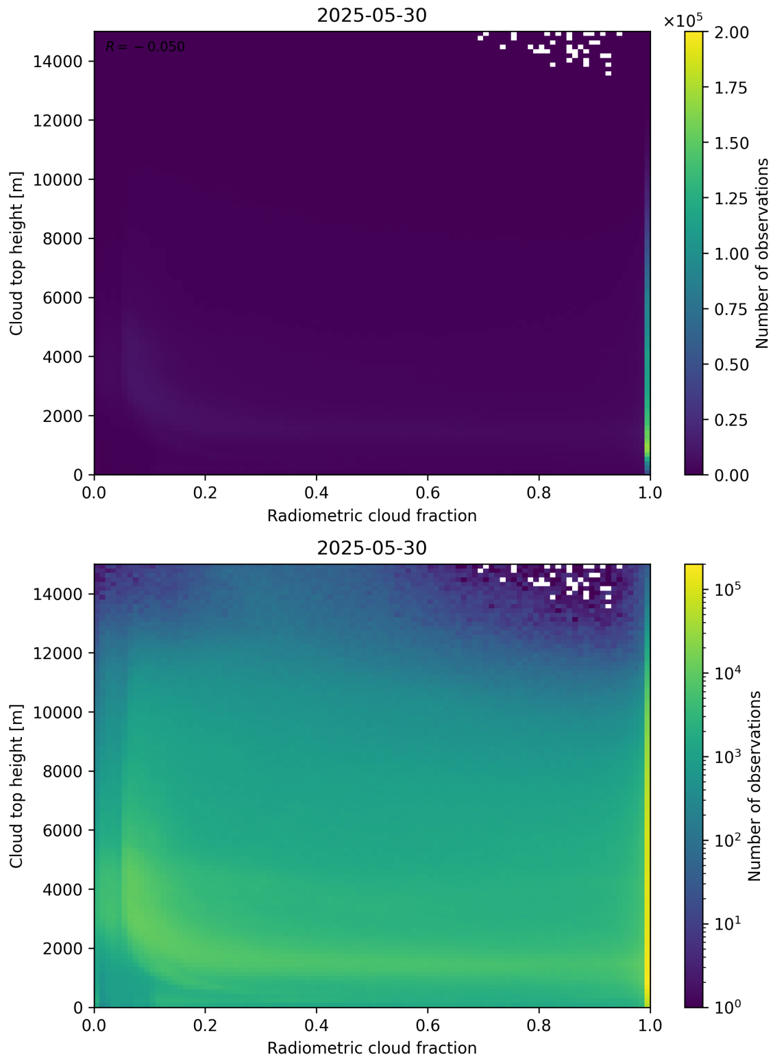
Figure 76: Scatter density plot of “Radiometric cloud fraction” against “Cloud top height” for 2025-05-29 to 2025-05-31.
