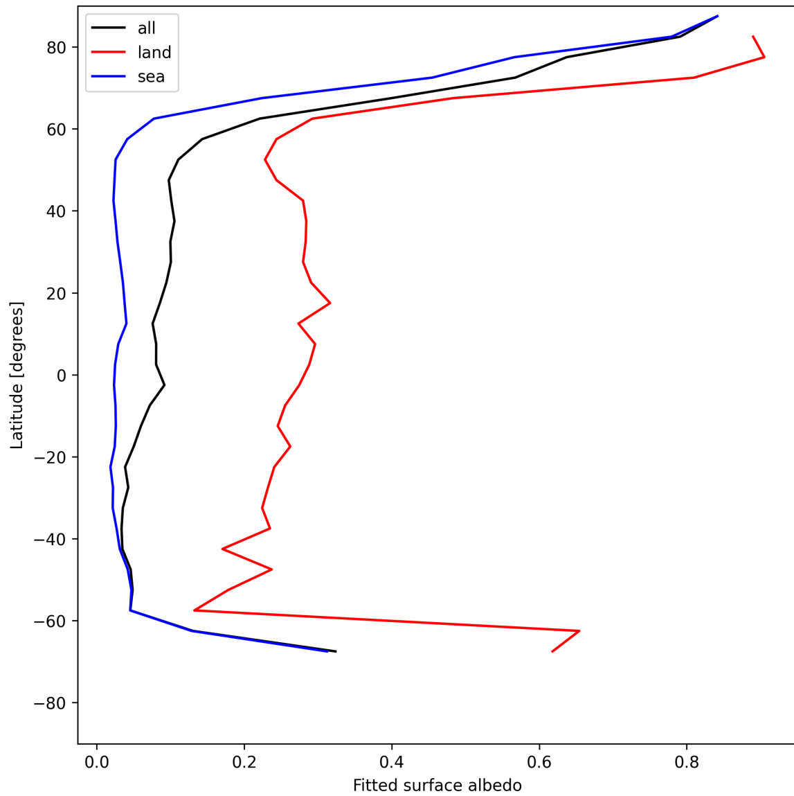
Figure 29: Zonal average of “Fitted surface albedo” for 2025-05-29 to 2025-05-31.
