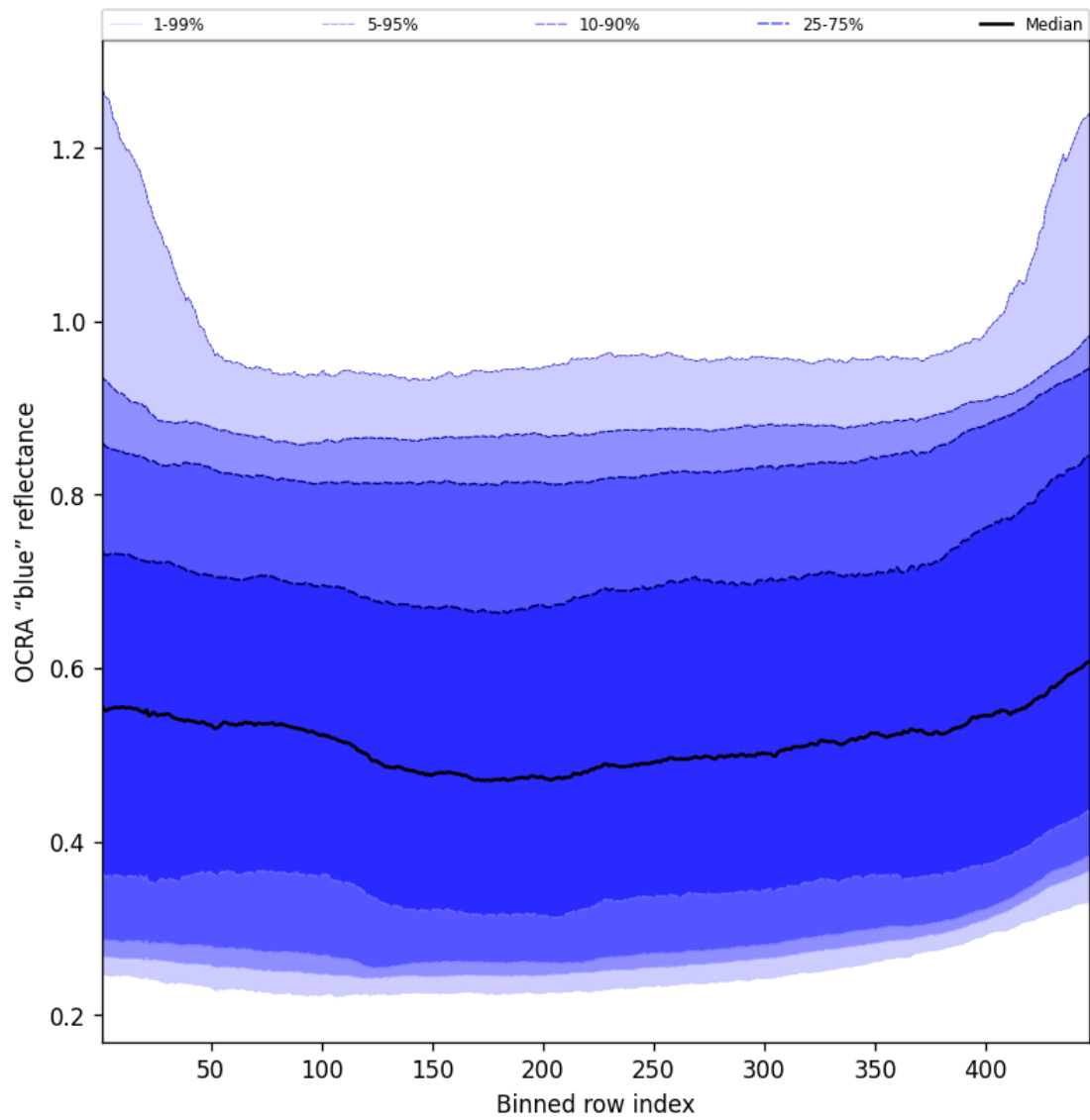
Figure 67: Along track statistics of “OCRA “blue” reflectance” for 2025-05-29 to 2025-05-31
