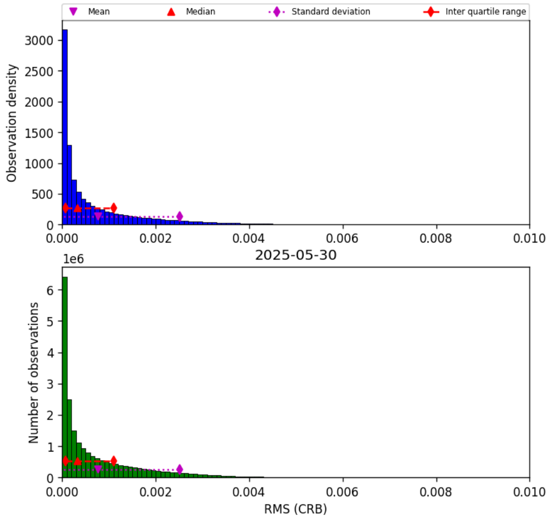
Figure 48: Histogram of “RMS (CRB)” for 2025-05-29 to 2025-05-31
