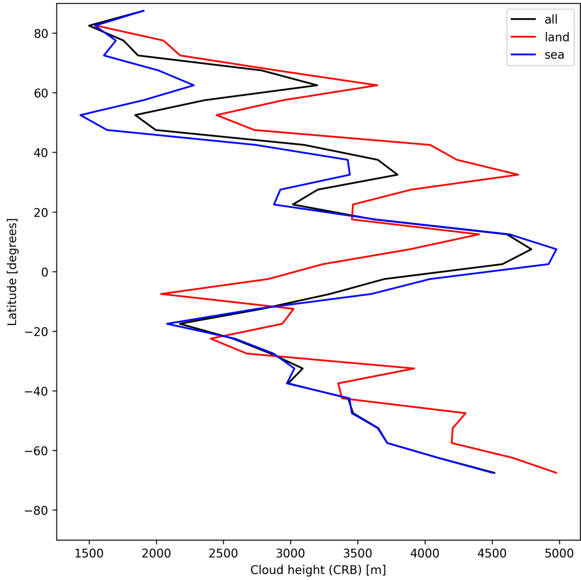
Figure 27: Zonal average of “Cloud height (CRB)” for 2025-05-29 to 2025-05-31.
