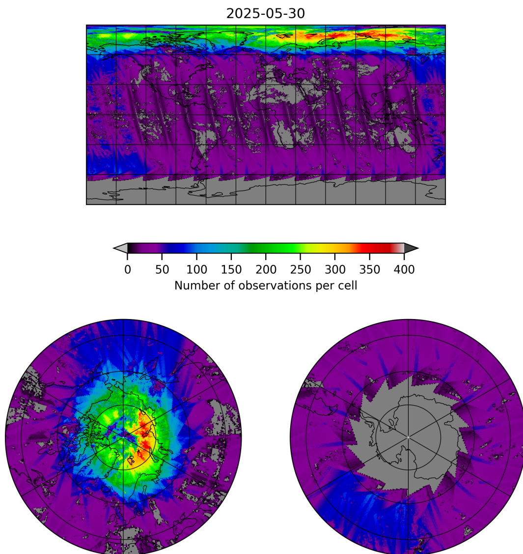
Figure 21: Map of the number of observations for 2025-05-29 to 2025-05-31
