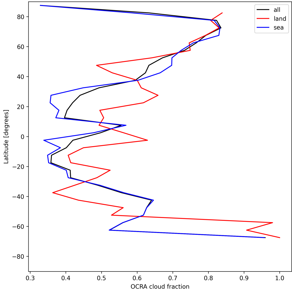
Figure 34: Zonal average of “OCRA cloud fraction” for 2025-05-29 to 2025-05-31.
