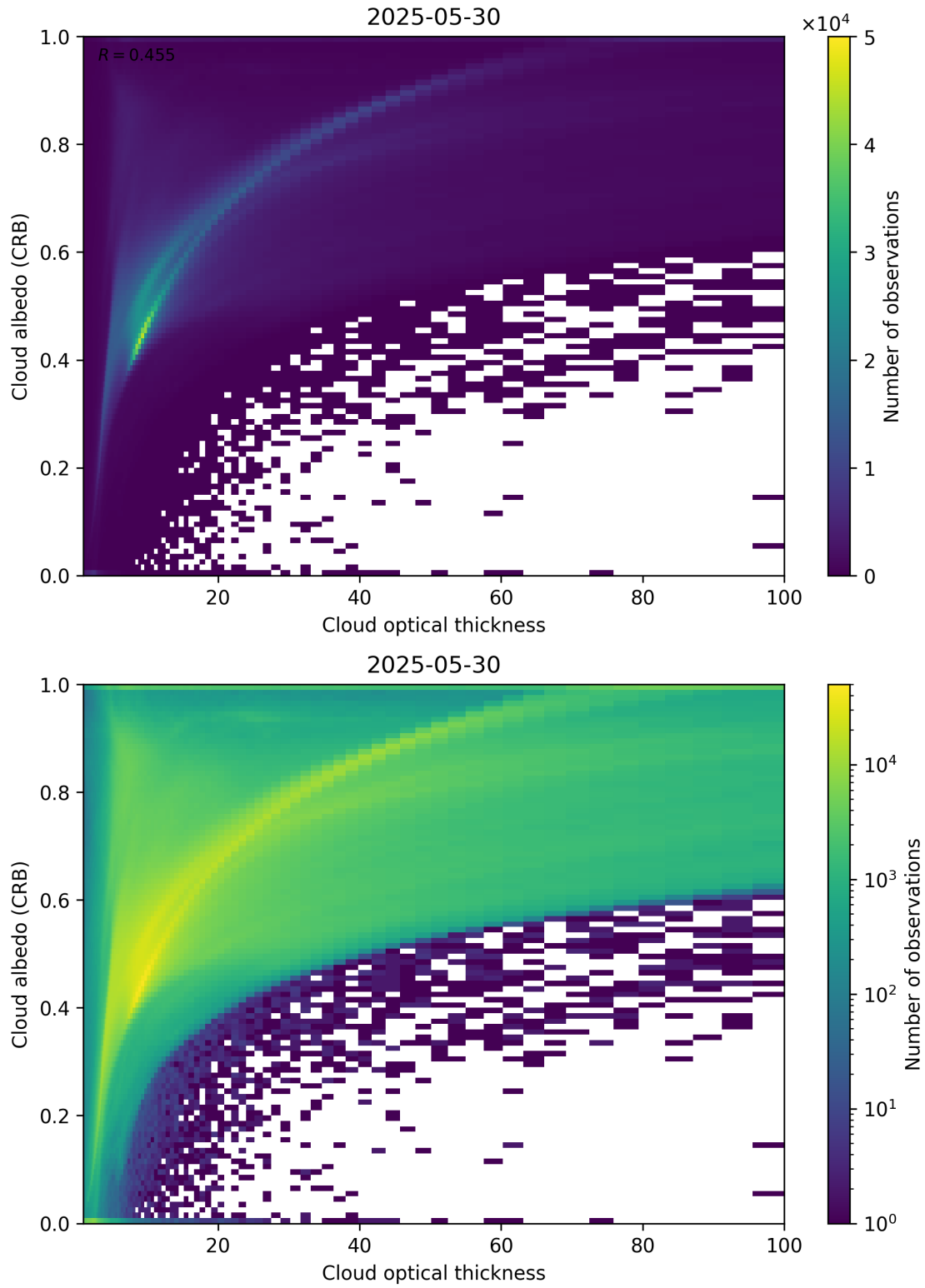
Figure 82: Scatter density plot of “Cloud optical thickness” against “Cloud albedo (CRB)” for 2025-05-29 to 2025-05-31.
