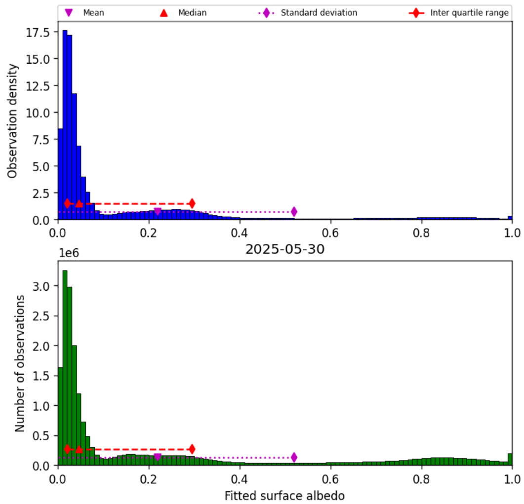
Figure 45: Histogram of “Fitted surface albedo” for 2025-05-29 to 2025-05-31
