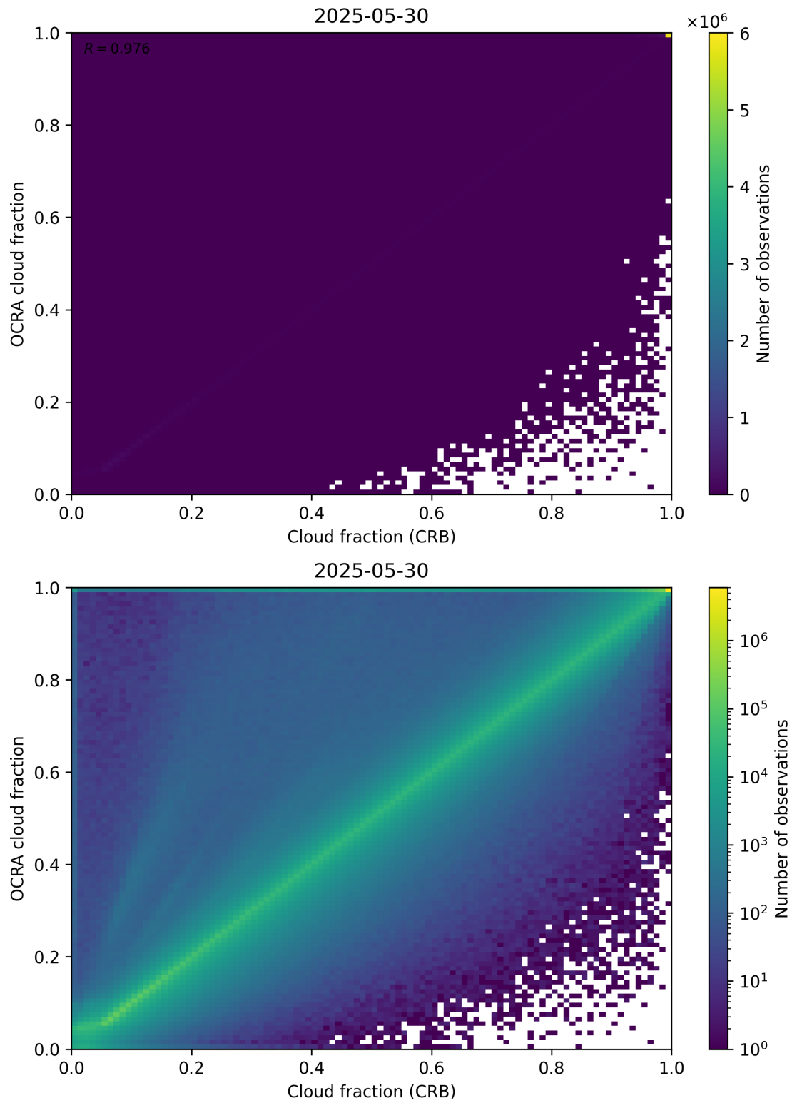
Figure 78: Scatter density plot of “Cloud fraction (CRB)” against “OCRA cloud fraction” for 2025-05-29 to 2025-05-31.
