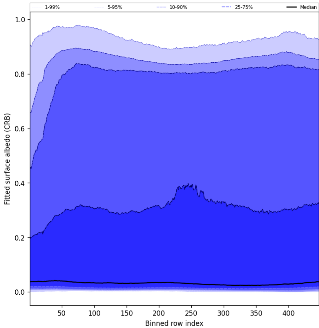
Figure 62: Along track statistics of “Fitted surface albedo (CRB)” for 2025-05-29 to 2025-05-31
