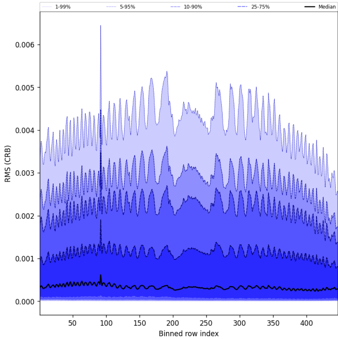
Figure 64: Along track statistics of “RMS (CRB)” for 2025-05-29 to 2025-05-31
