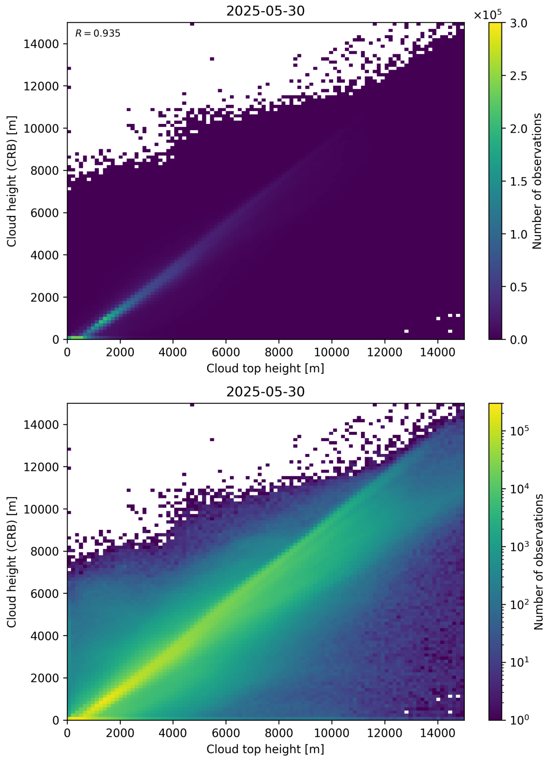
Figure 89: Scatter density plot of “Cloud top height” against “Cloud height (CRB)” for 2025-05-29 to 2025-05-31.
