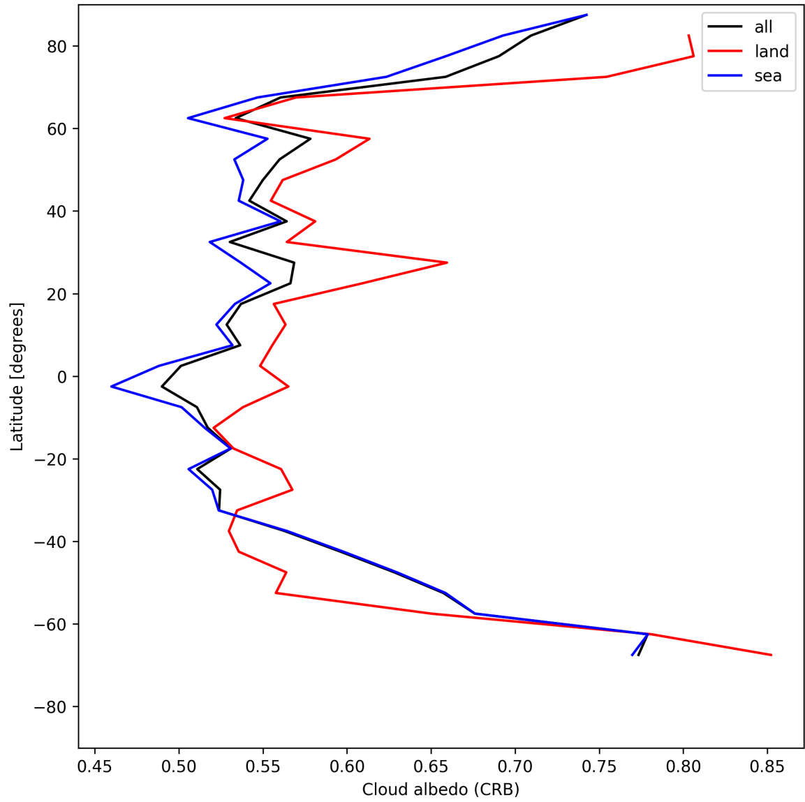
Figure 28: Zonal average of “Cloud albedo (CRB)” for 2025-05-29 to 2025-05-31.
