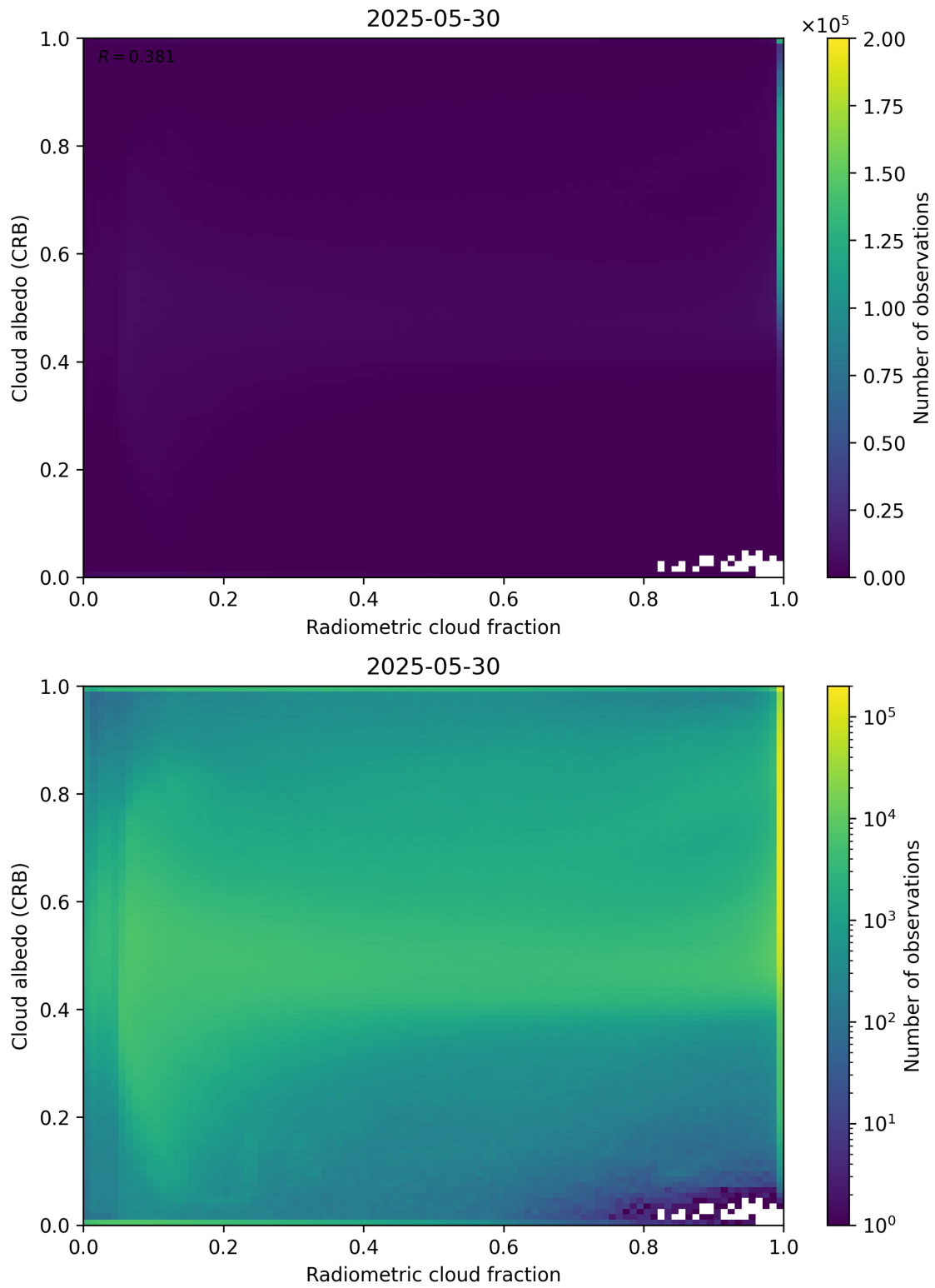
Figure 71: Scatter density plot of “Radiometric cloud fraction” against “Cloud albedo (CRB)” for 2025-05-29 to 2025-05-31.
