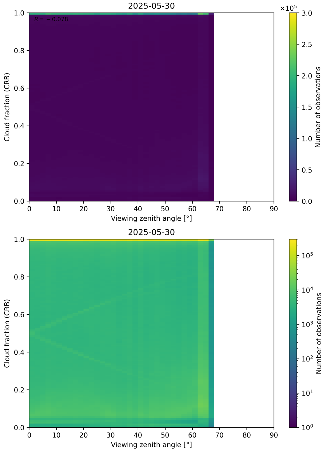
Figure 109: Scatter density plot of “Viewing zenith angle” against “Cloud fraction (CRB)” for 2025-05-29 to 2025-05-31.
