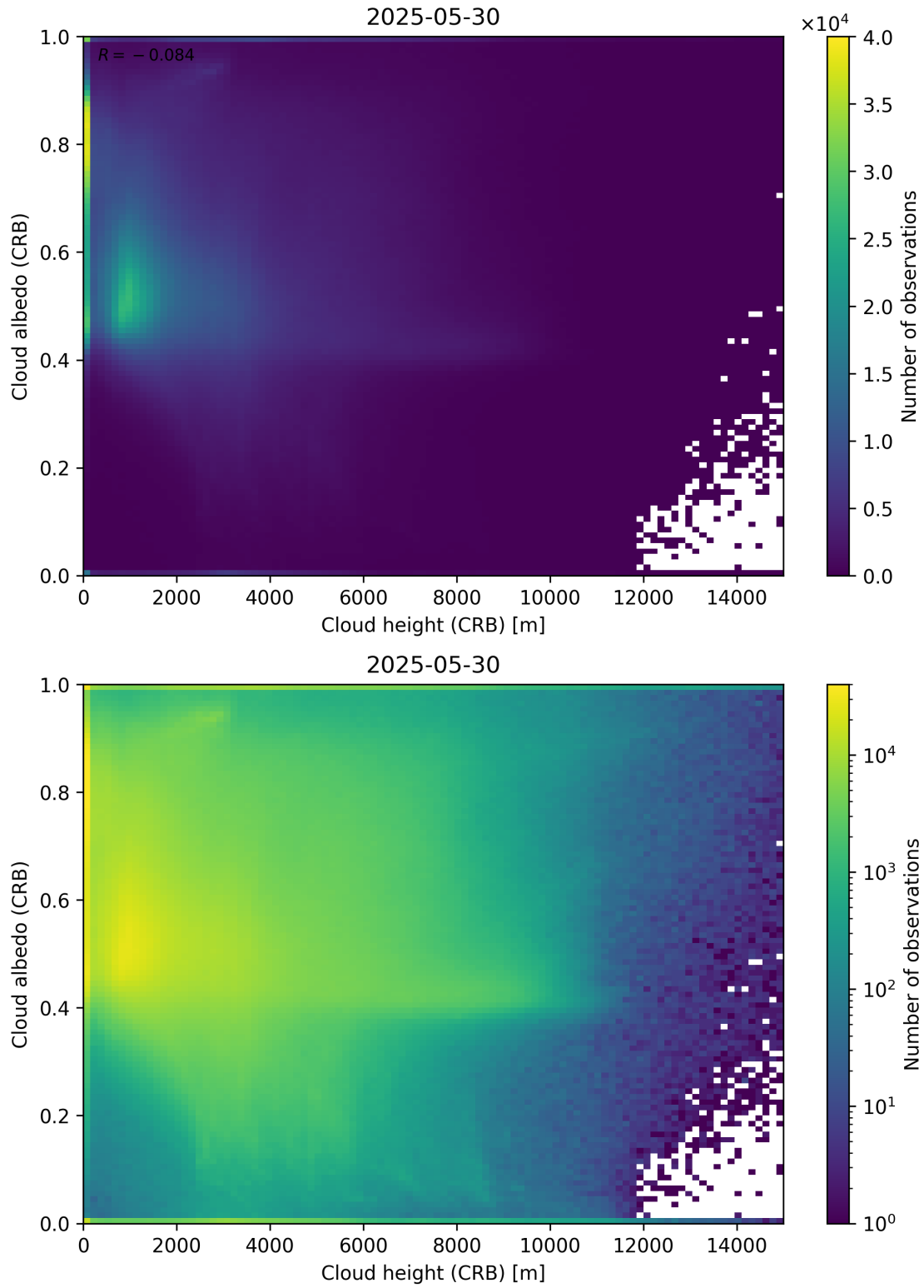
Figure 80: Scatter density plot of “Cloud height (CRB)” against “Cloud albedo (CRB)” for 2025-05-29 to 2025-05-31.
