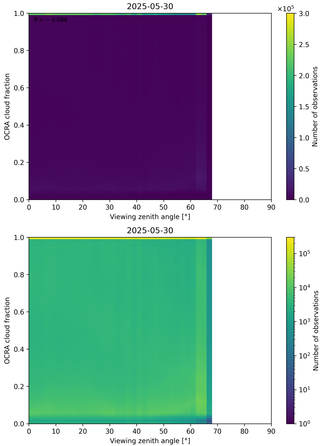
Figure 108: Scatter density plot of “Viewing zenith angle” against “OCRA cloud fraction” for 2025-05-29 to 2025-05-31.
