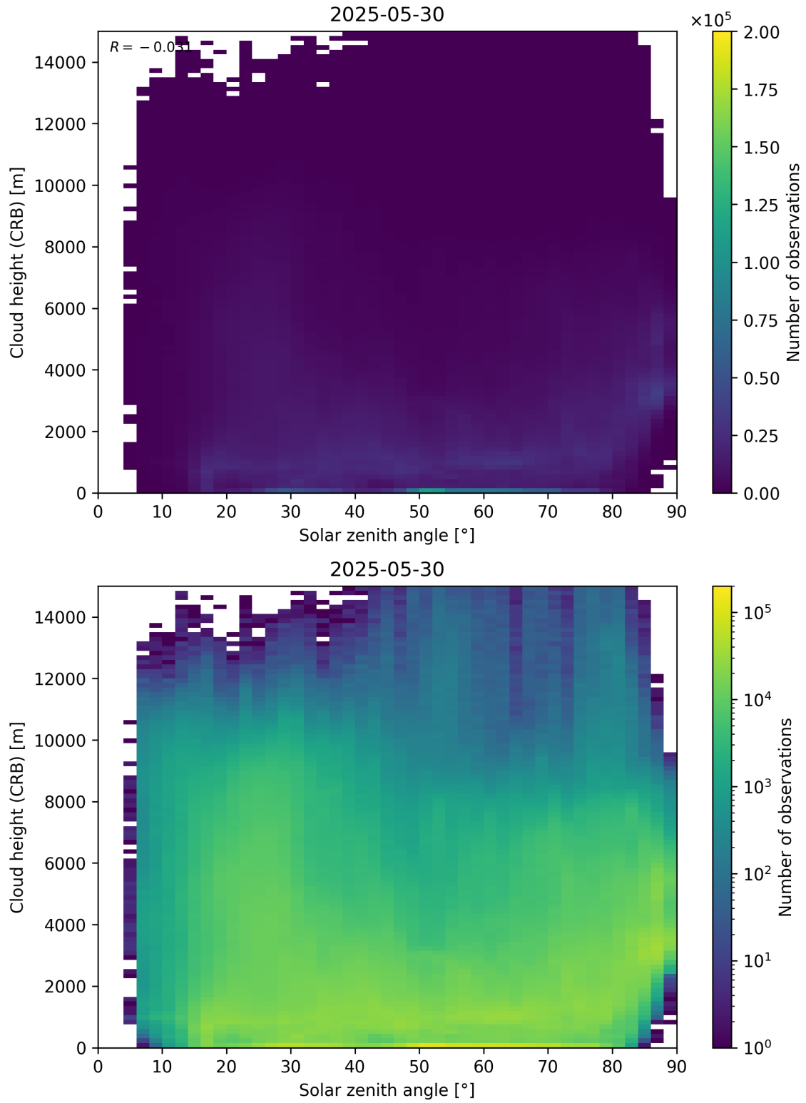
Figure 102: Scatter density plot of “Solar zenith angle” against “Cloud height (CRB)” for 2025-05-29 to 2025-05-31.
