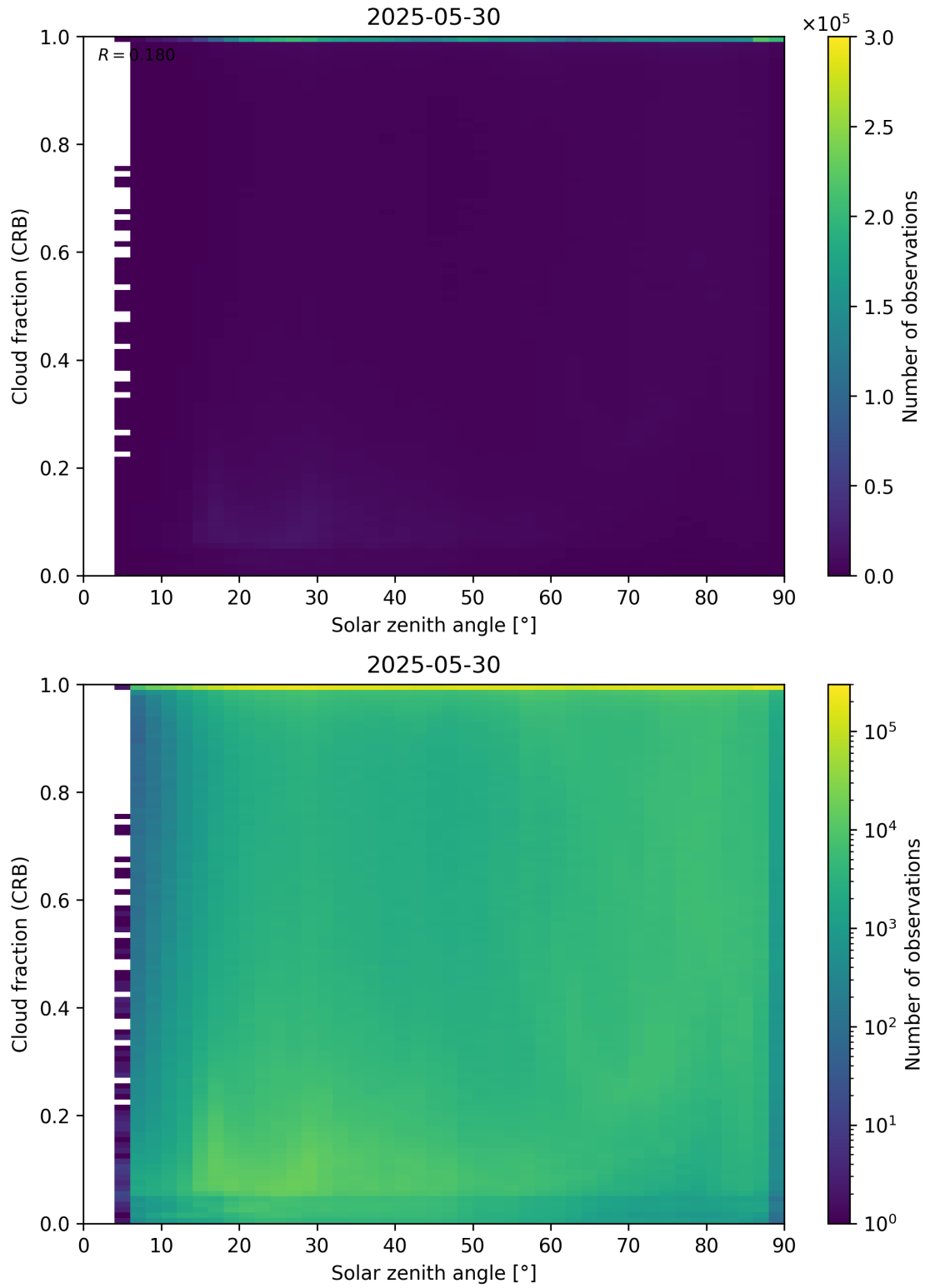
Figure 101: Scatter density plot of “Solar zenith angle” against “Cloud fraction (CRB)” for 2025-05-29 to 2025-05-31.
