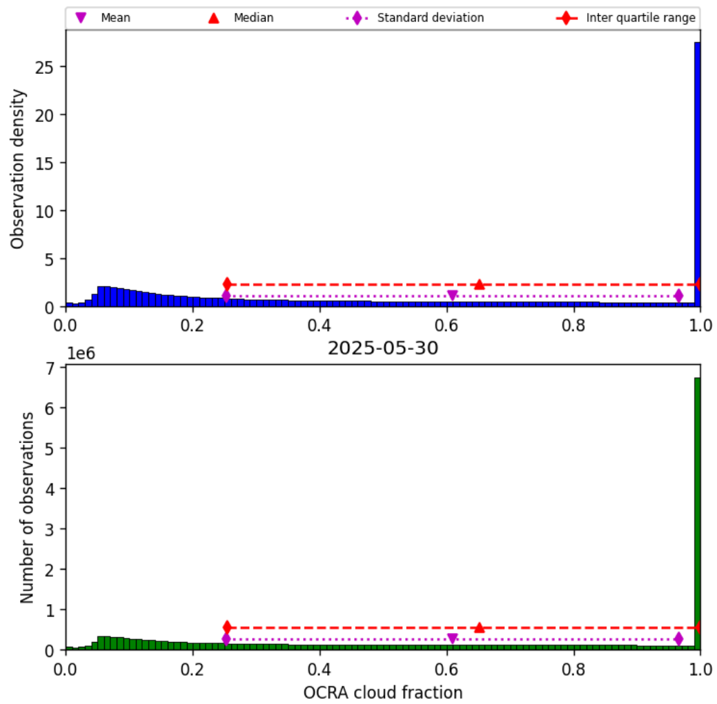
Figure 50: Histogram of “OCRA cloud fraction” for 2025-05-29 to 2025-05-31
