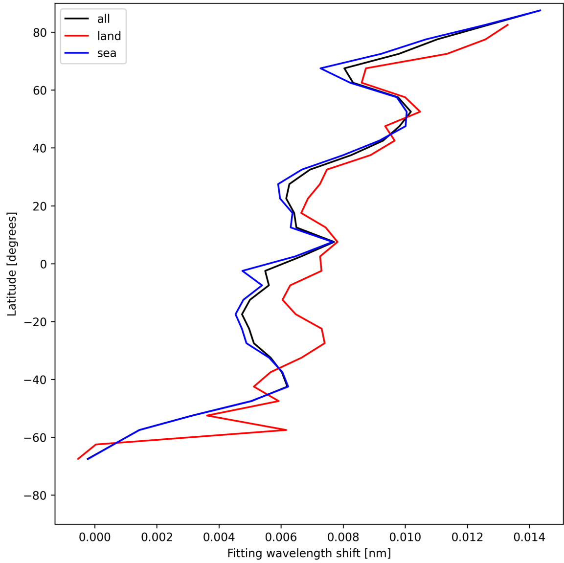
Figure 33: Zonal average of “Fitting wavelength shift” for 2025-05-29 to 2025-05-31.
