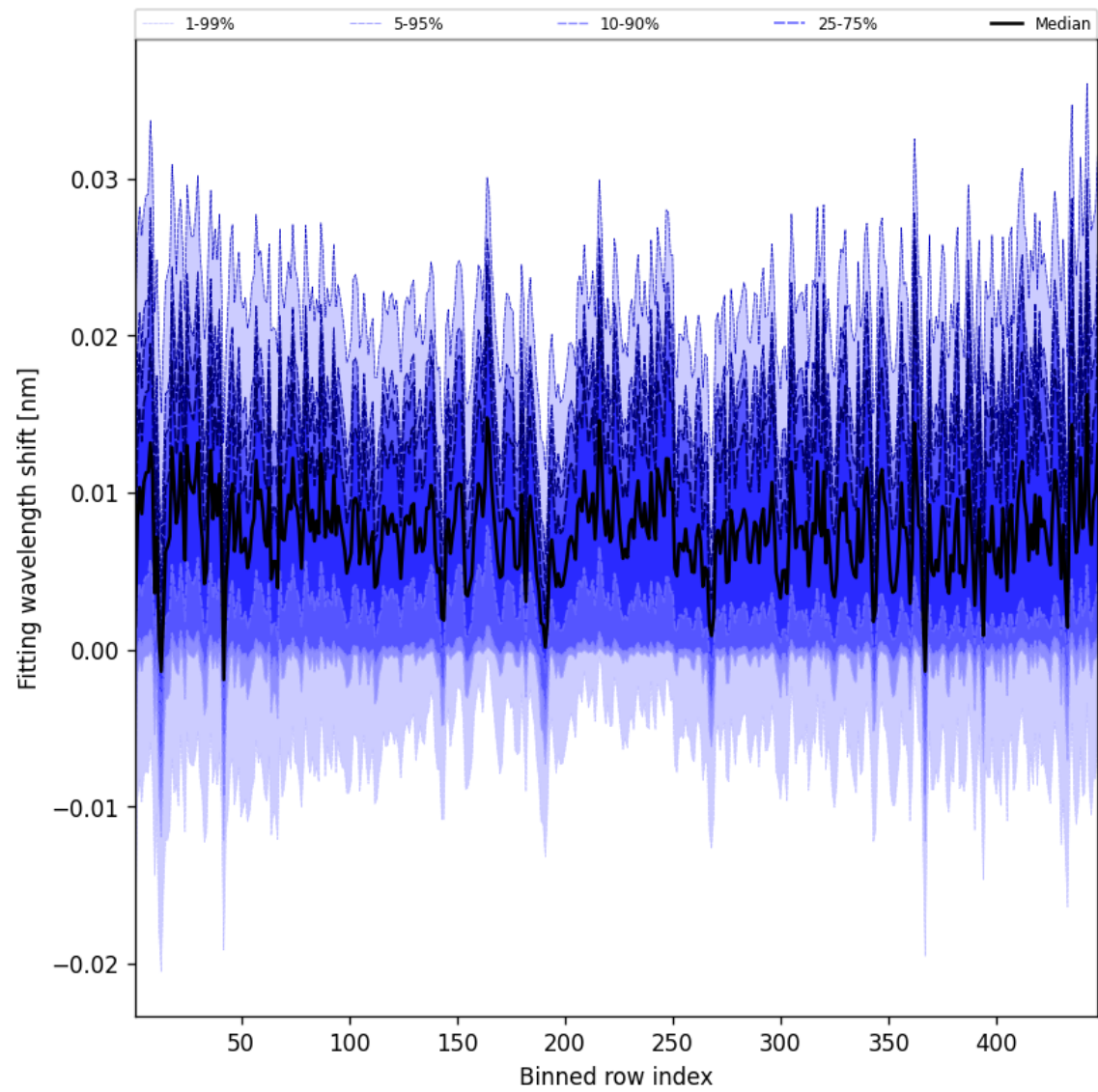
Figure 65: Along track statistics of “Fitting wavelength shift” for 2025-05-29 to 2025-05-31
