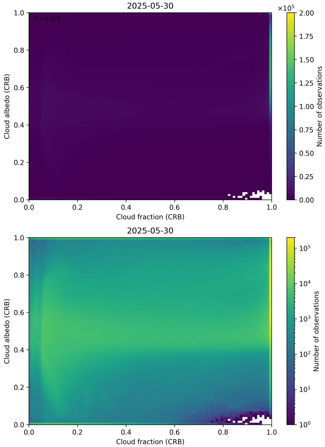
Figure 77: Scatter density plot of “Cloud fraction (CRB)” against “Cloud albedo (CRB)” for 2025-05-29 to 2025-05-31.
