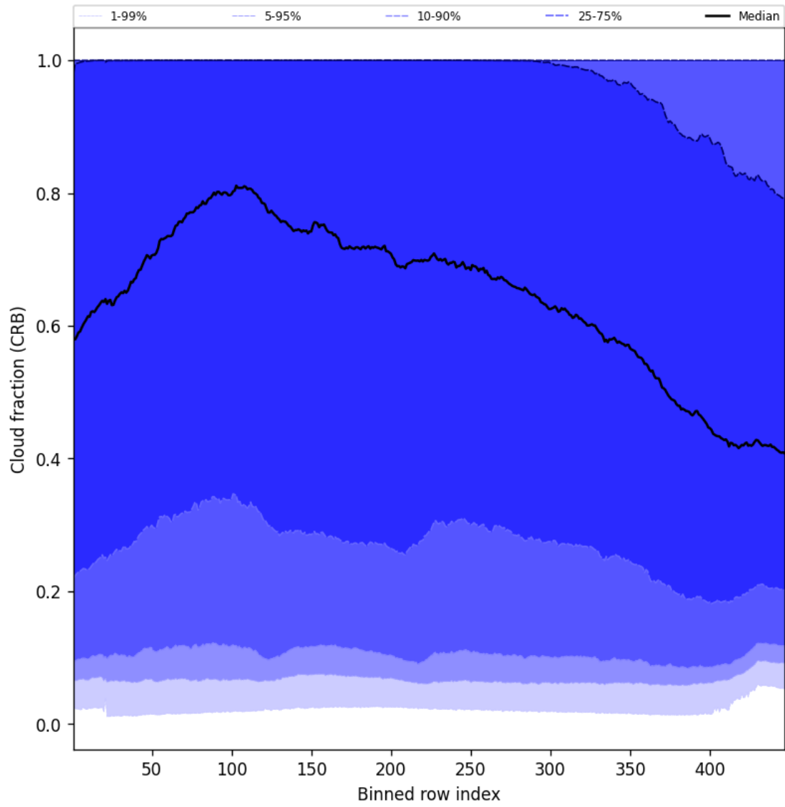
Figure 58: Along track statistics of “Cloud fraction (CRB)” for 2025-05-29 to 2025-05-31
