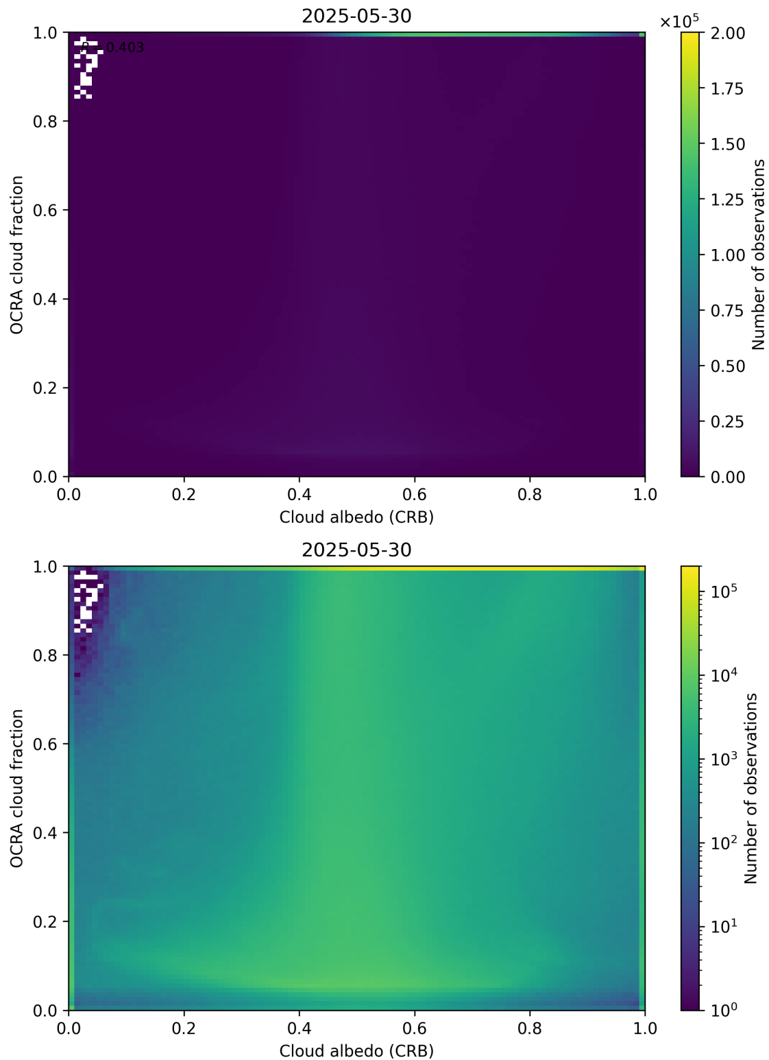
Figure 70: Scatter density plot of “Cloud albedo (CRB)” against “OCRA cloud fraction” for 2025-05-29 to 2025-05-31.
