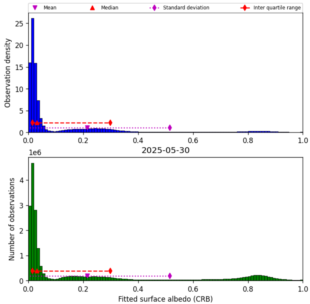
Figure 46: Histogram of “Fitted surface albedo (CRB)” for 2025-05-29 to 2025-05-31
