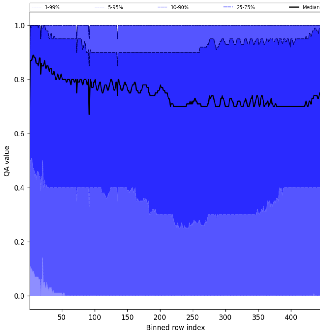
Figure 54: Along track statistics of “QA value” for 2025-05-29 to 2025-05-31
