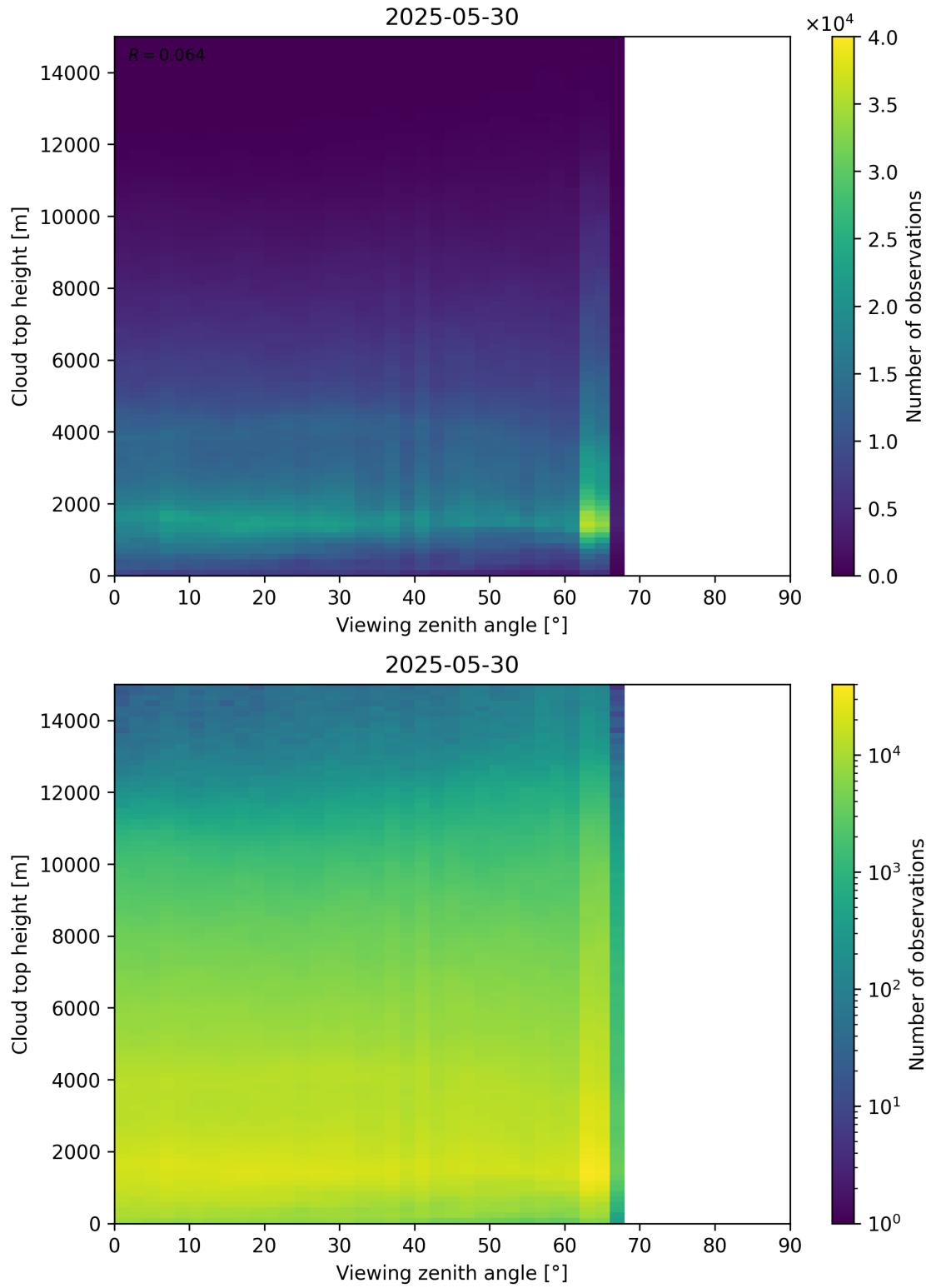
Figure 112: Scatter density plot of “Viewing zenith angle” against “Cloud top height” for 2025-05-29 to 2025-05-31.
