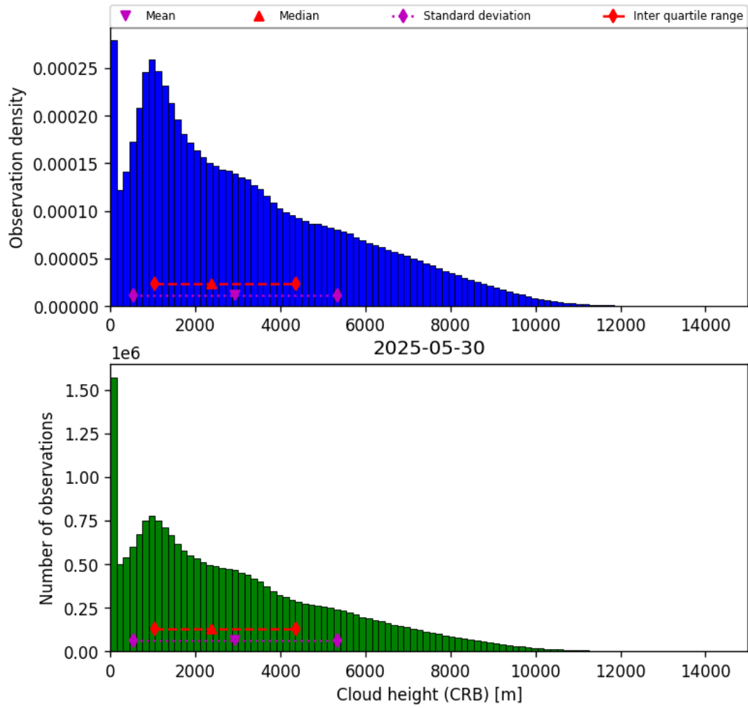
Figure 43: Histogram of “Cloud height (CRB)” for 2025-05-29 to 2025-05-31
