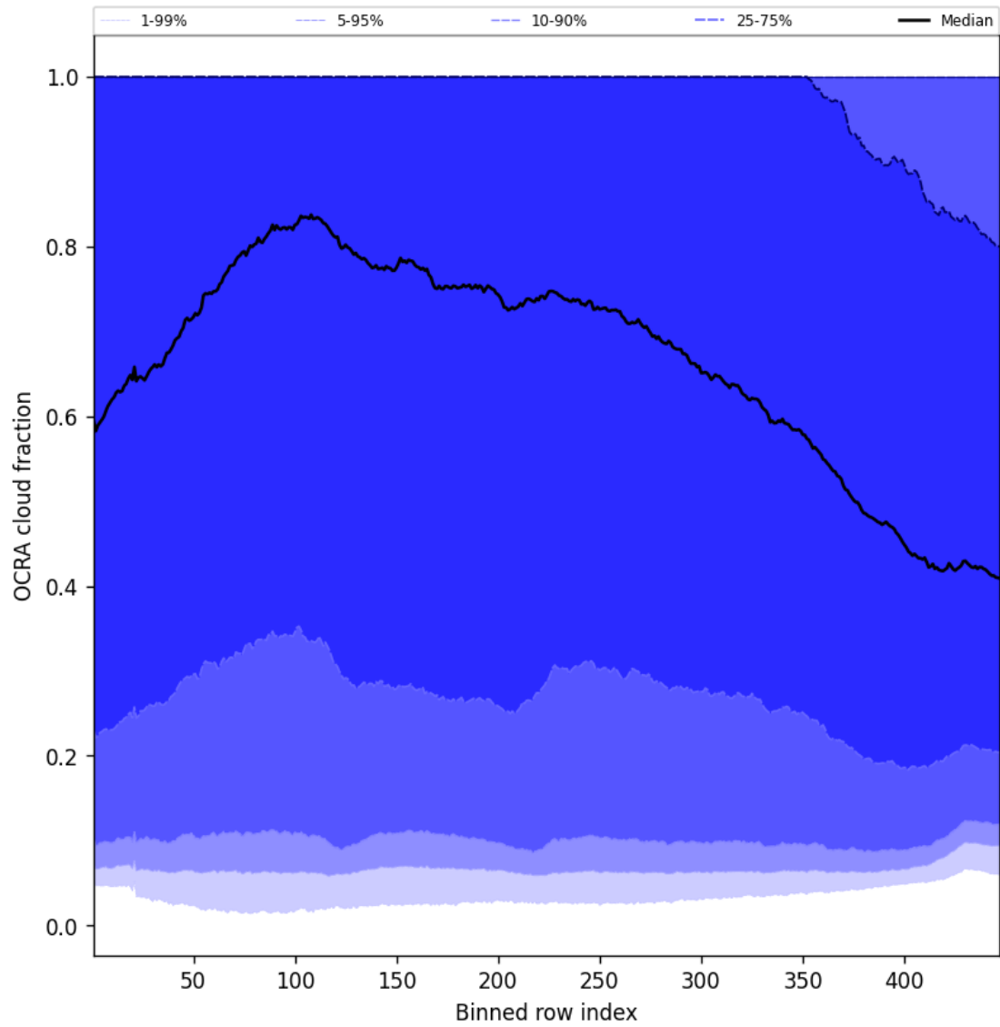
Figure 66: Along track statistics of “OCRA cloud fraction” for 2025-05-29 to 2025-05-31
