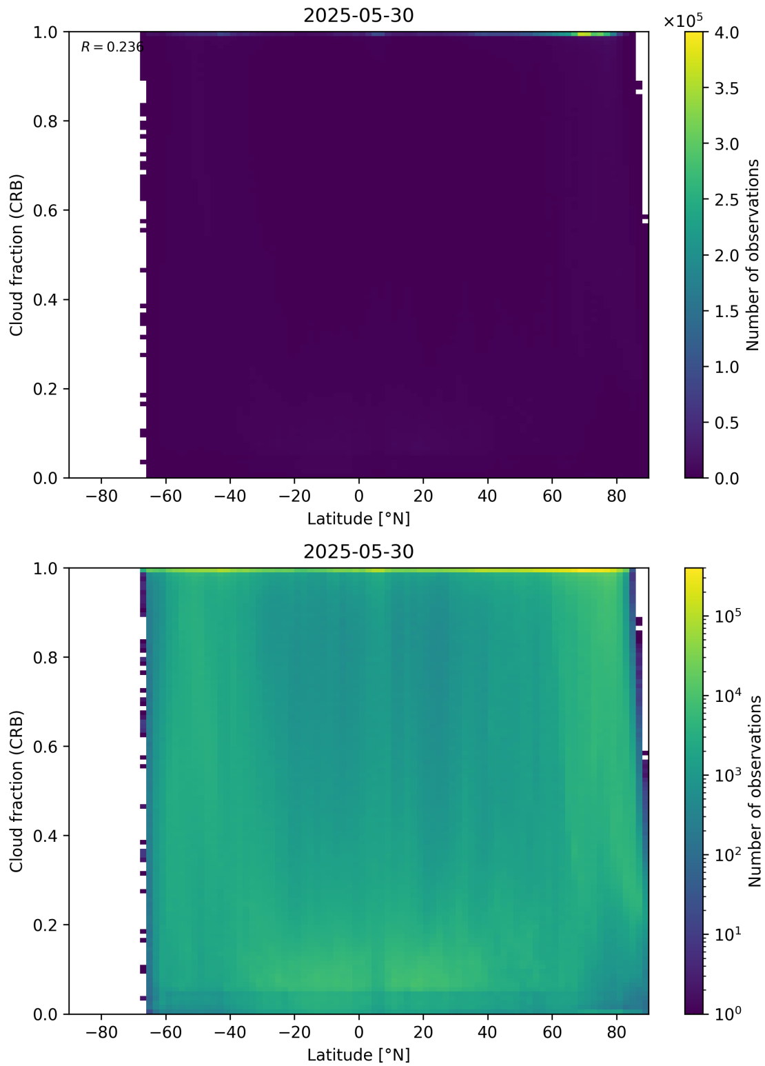
Figure 94: Scatter density plot of “Latitude” against “Cloud fraction (CRB)” for 2025-05-29 to 2025-05-31.
