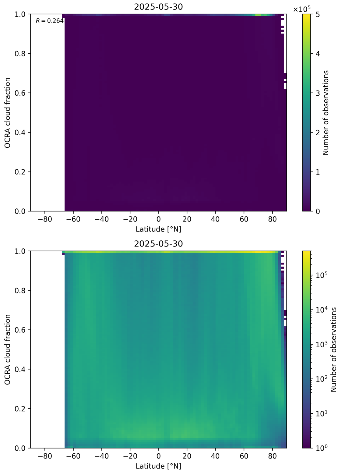
Figure 93: Scatter density plot of “Latitude” against “OCRA cloud fraction” for 2025-05-29 to 2025-05-31.
