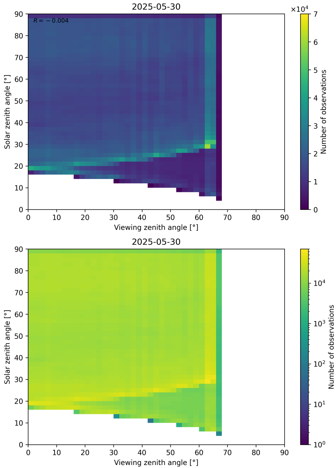
Figure 114: Scatter density plot of “Viewing zenith angle” against “Solar zenith angle” for 2025-05-29 to 2025-05-31.
