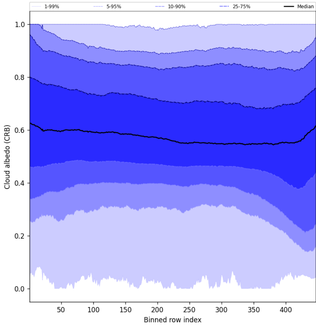
Figure 60: Along track statistics of “Cloud albedo (CRB)” for 2025-05-29 to 2025-05-31
