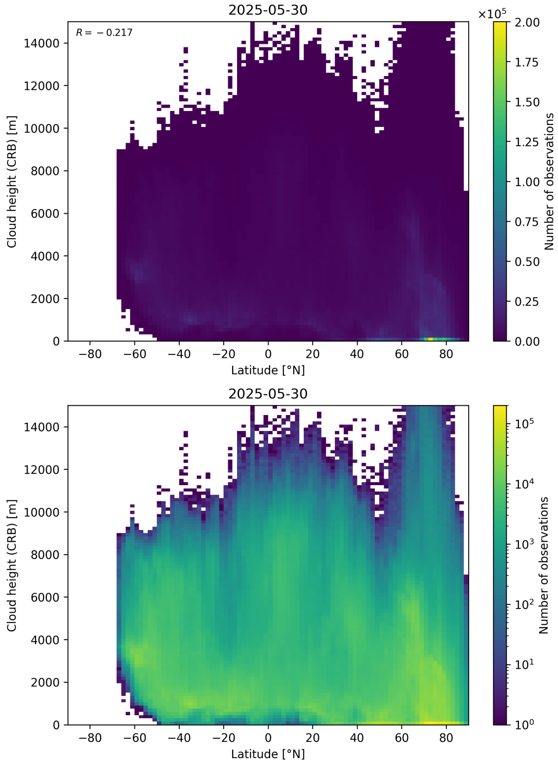
Figure 95: Scatter density plot of “Latitude” against “Cloud height (CRB)” for 2025-05-29 to 2025-05-31.
