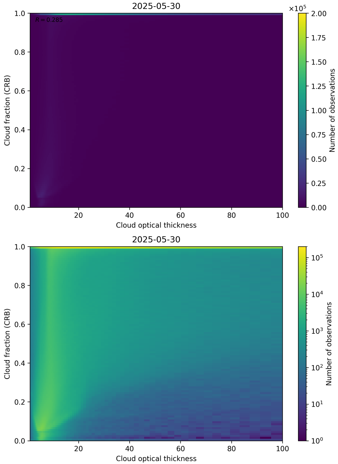
Figure 84: Scatter density plot of “Cloud optical thickness” against “Cloud fraction (CRB)” for 2025-05-29 to 2025-05-31.
