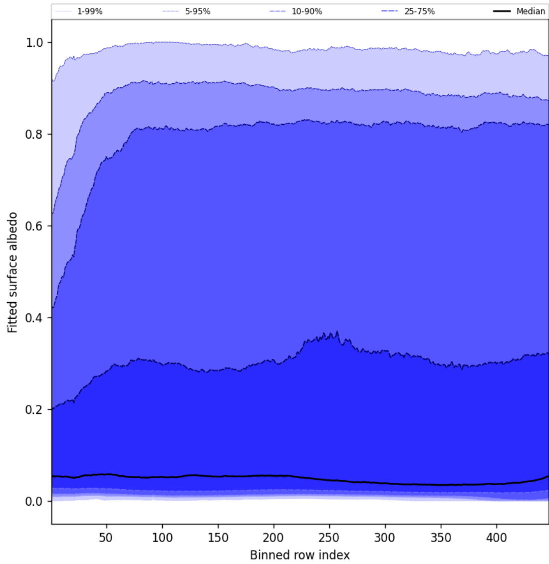
Figure 61: Along track statistics of “Fitted surface albedo” for 2025-05-29 to 2025-05-31
