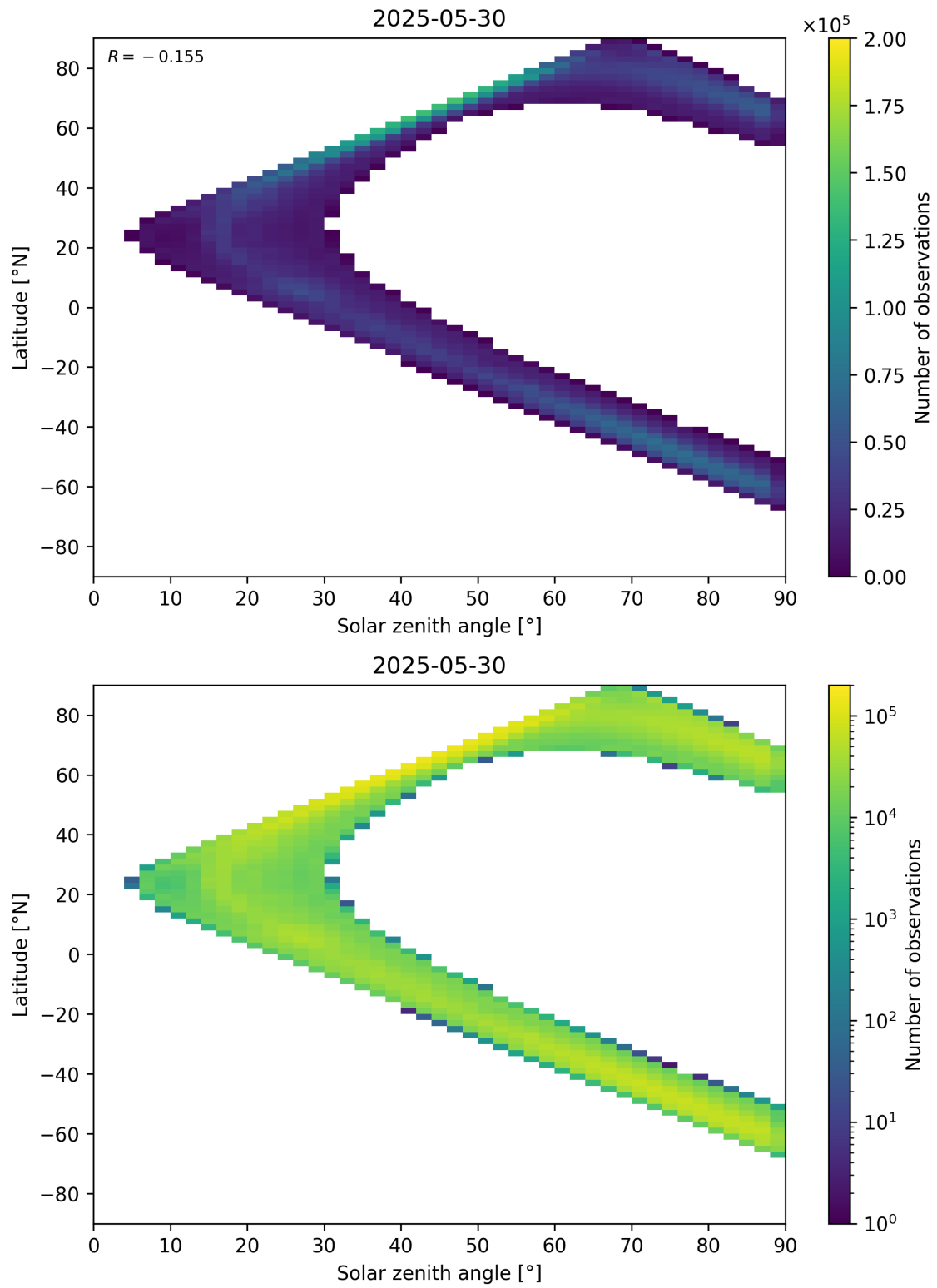
Figure 105: Scatter density plot of “Solar zenith angle” against “Latitude” for 2025-05-29 to 2025-05-31.
