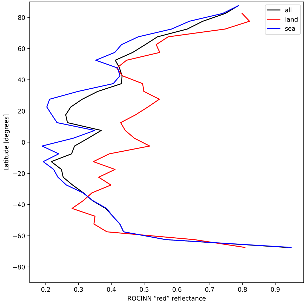
Figure 37: Zonal average of “ROCINN “red” reflectance” for 2025-05-31 to 2025-06-01.
