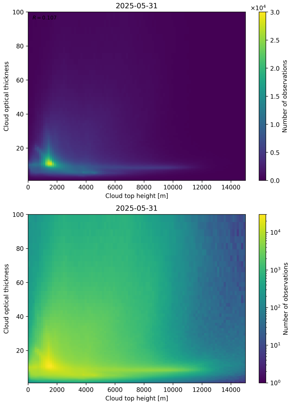
Figure 90: Scatter density plot of “Cloud top height” against “Cloud optical thickness” for 2025-05-31 to 2025-06-01.
