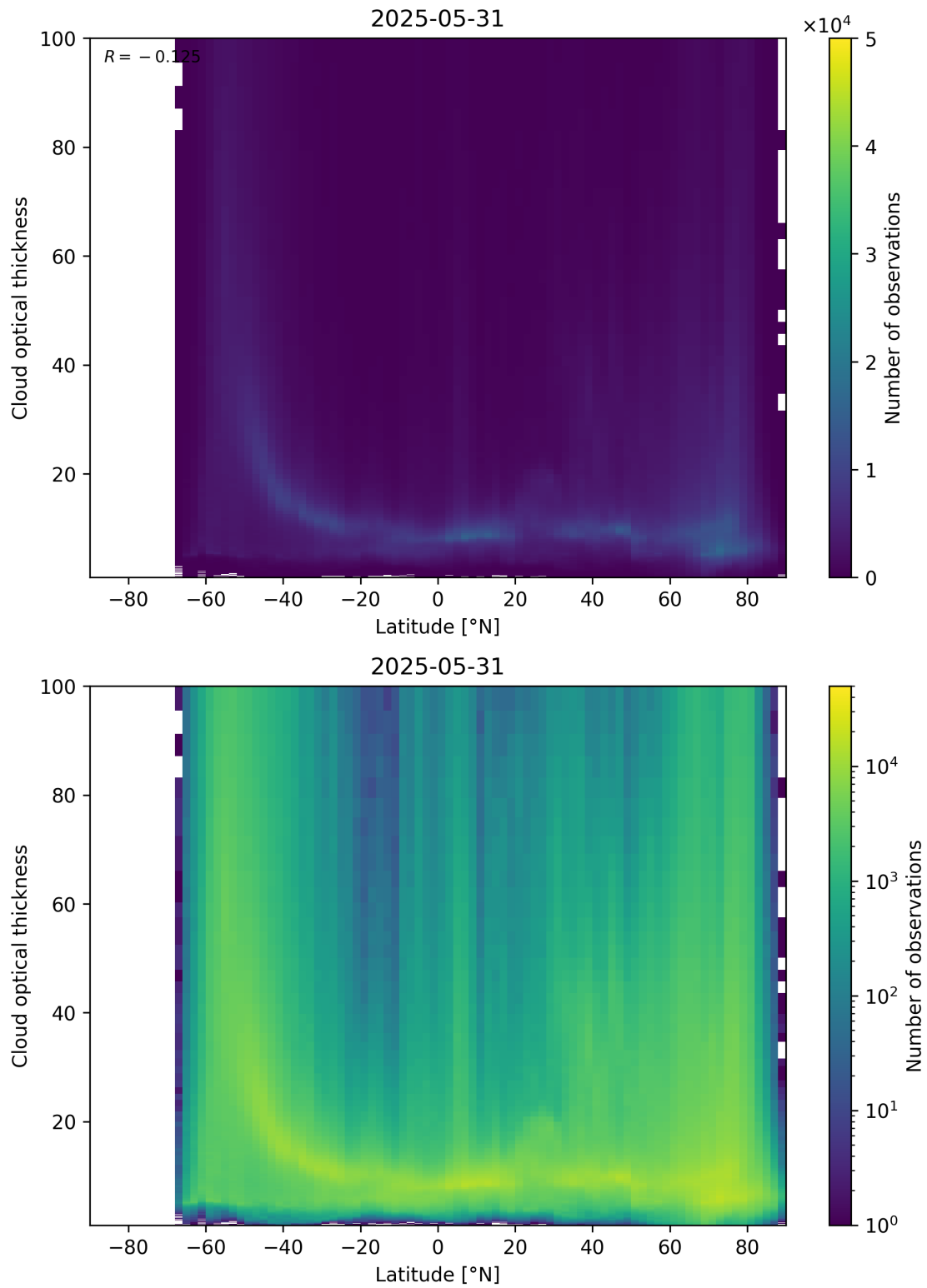
Figure 96: Scatter density plot of “Latitude” against “Cloud optical thickness” for 2025-05-31 to 2025-06-01.
