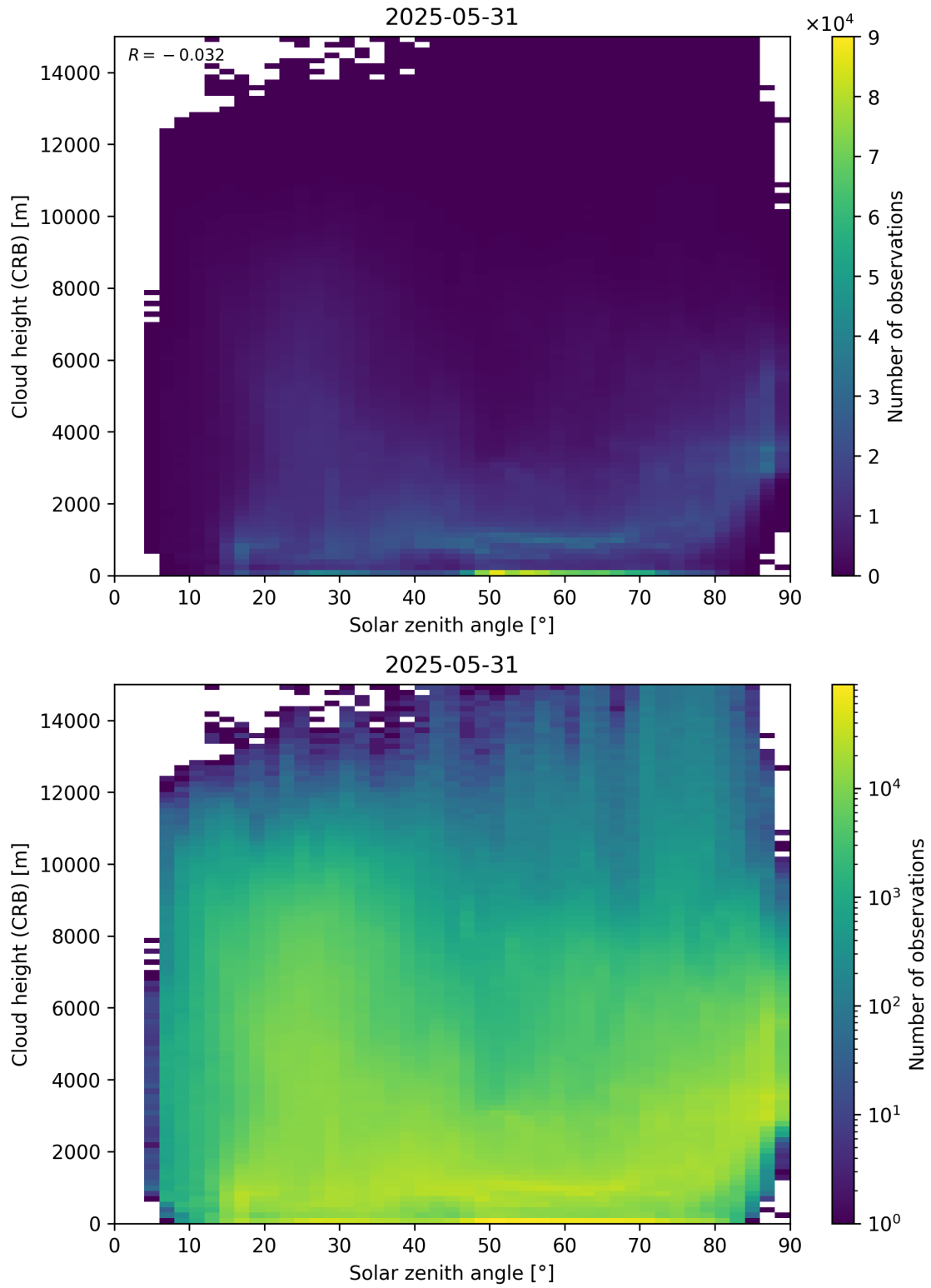
Figure 102: Scatter density plot of “Solar zenith angle” against “Cloud height (CRB)” for 2025-05-31 to 2025-06-01.
