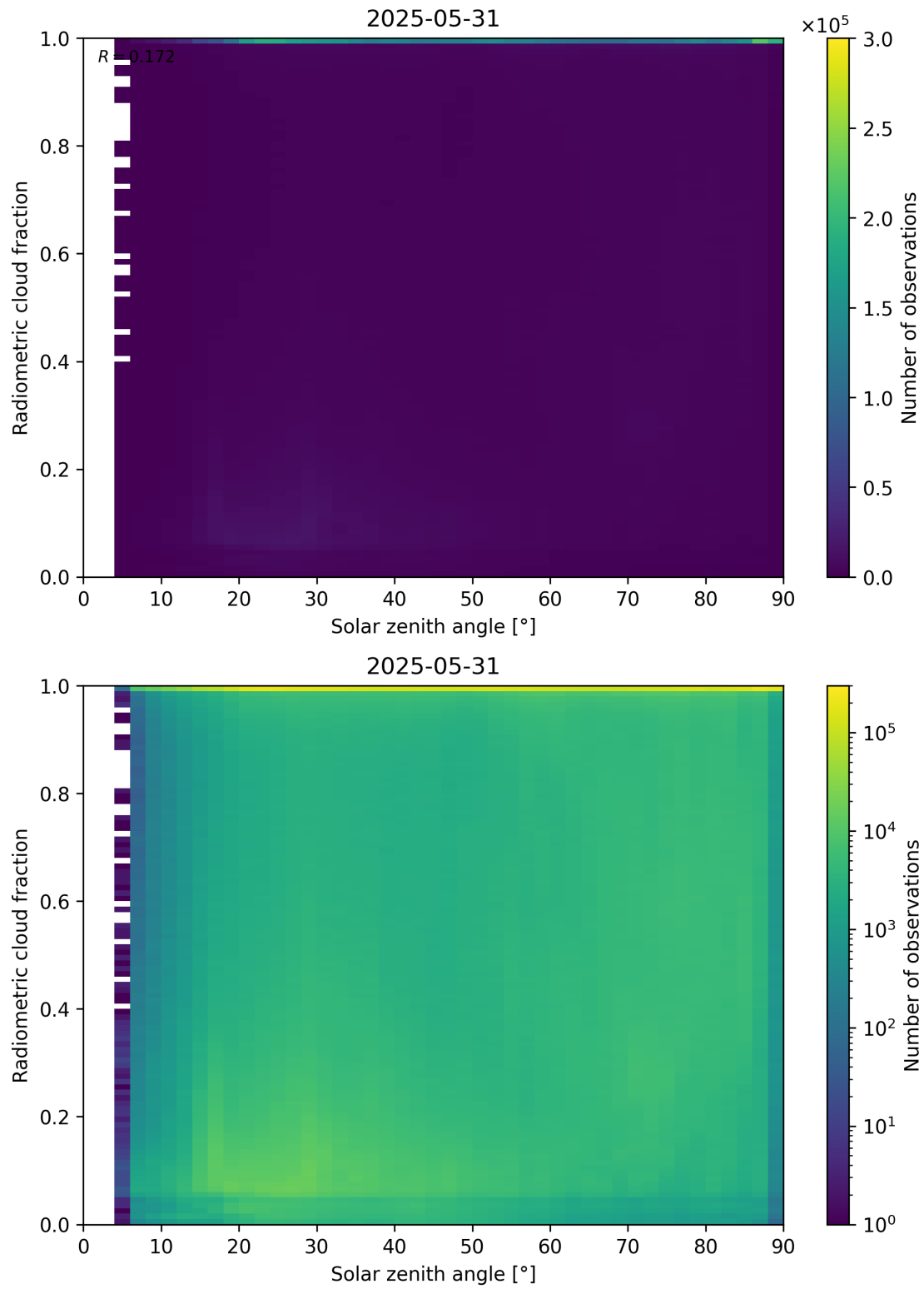
Figure 99: Scatter density plot of “Solar zenith angle” against “Radiometric cloud fraction” for 2025-05-31 to 2025-06-01.
