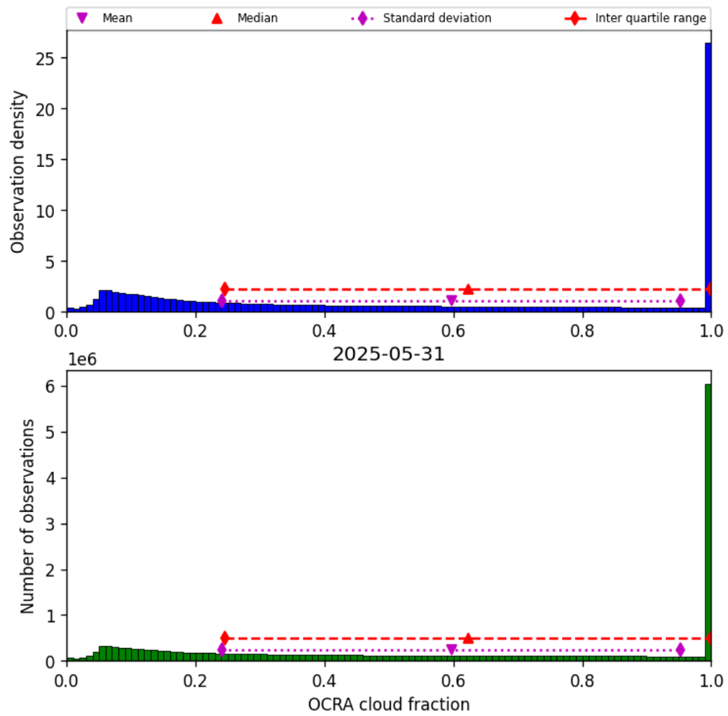
Figure 50: Histogram of “OCRA cloud fraction” for 2025-05-31 to 2025-06-01
