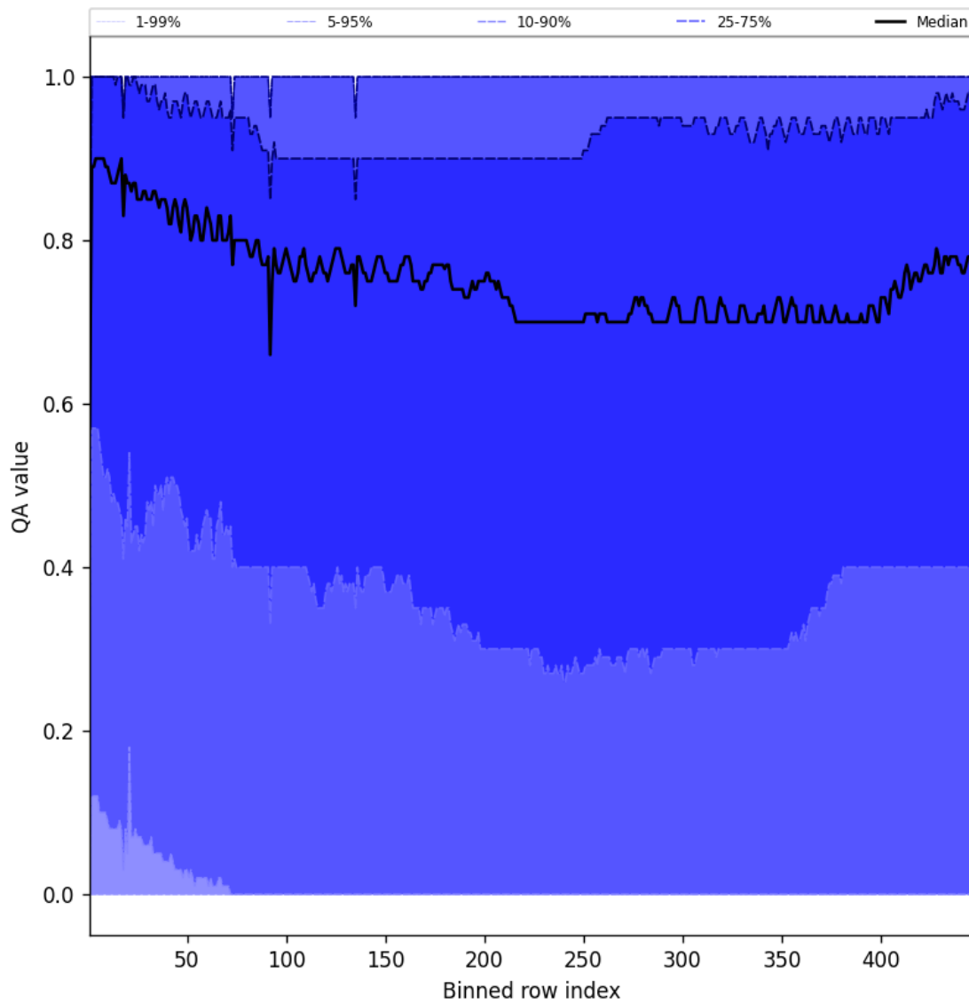
Figure 54: Along track statistics of “QA value” for 2025-05-31 to 2025-06-01
