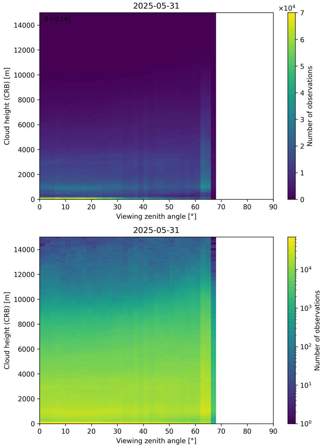
Figure 110: Scatter density plot of “Viewing zenith angle” against “Cloud height (CRB)” for 2025-05-31 to 2025-06-01.
