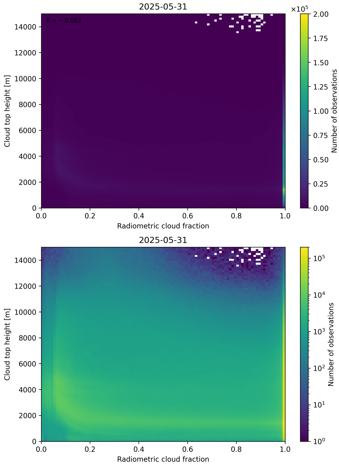
Figure 76: Scatter density plot of “Radiometric cloud fraction” against “Cloud top height” for 2025-05-31 to 2025-06-01.
