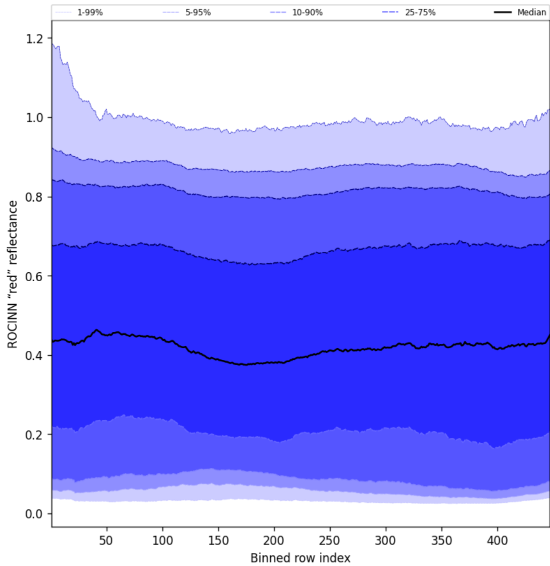
Figure 69: Along track statistics of "ROCINN "red" reflectance" for 2025-05-31 to 2025-06-01
