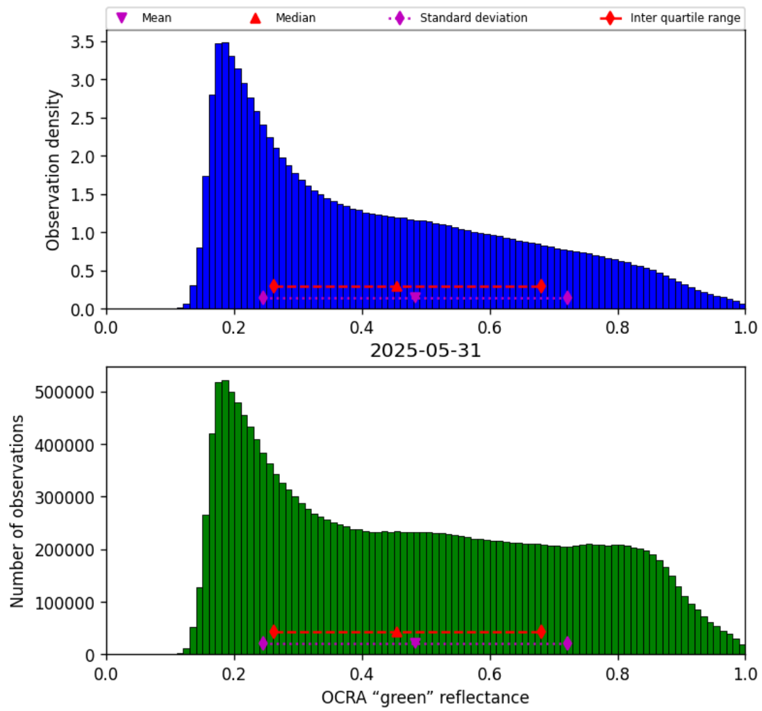
Figure 52: Histogram of “OCRA “green” reflectance” for 2025-05-31 to 2025-06-01
