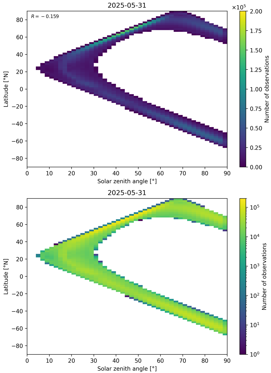
Figure 105: Scatter density plot of “Solar zenith angle” against “Latitude” for 2025-05-31 to 2025-06-01.
