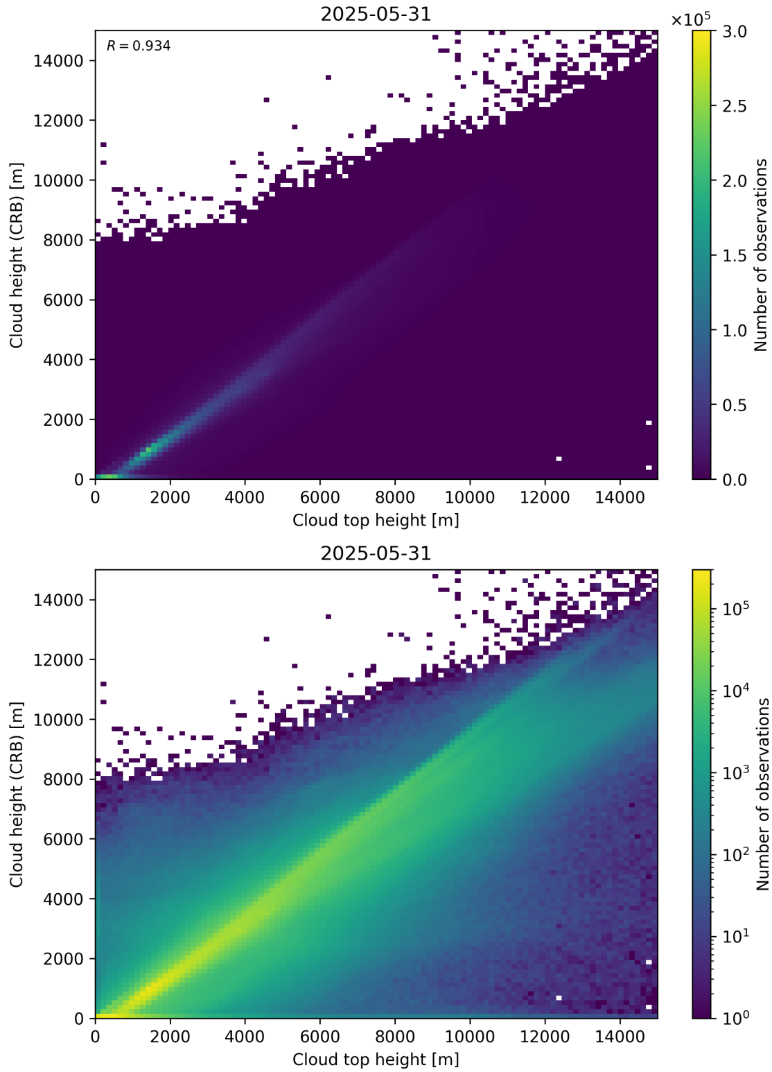
Figure 89: Scatter density plot of “Cloud top height” against “Cloud height (CRB)” for 2025-05-31 to 2025-06-01.
