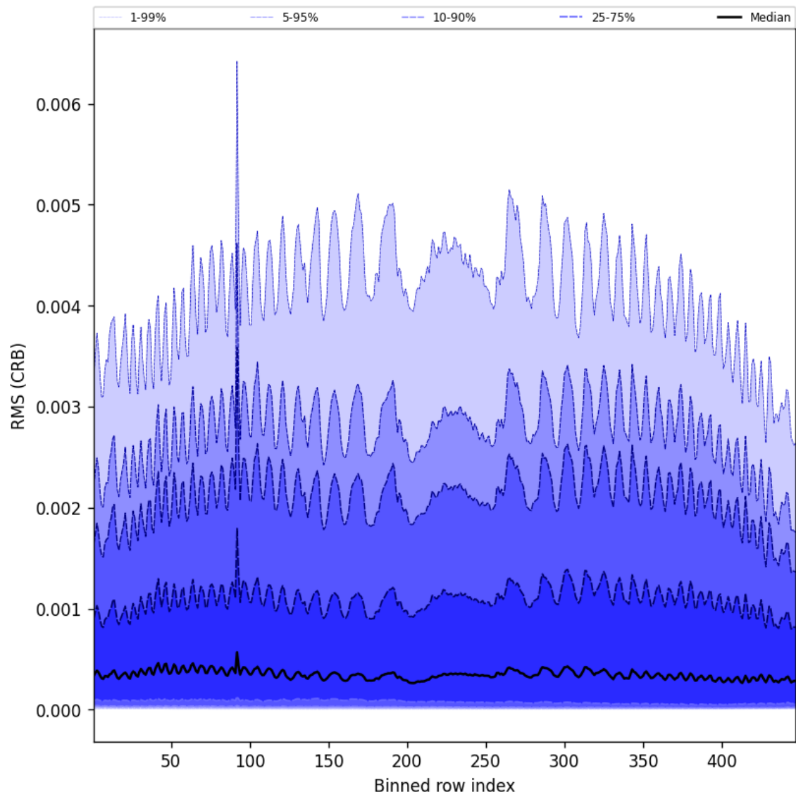
Figure 64: Along track statistics of “RMS (CRB)” for 2025-05-31 to 2025-06-01
