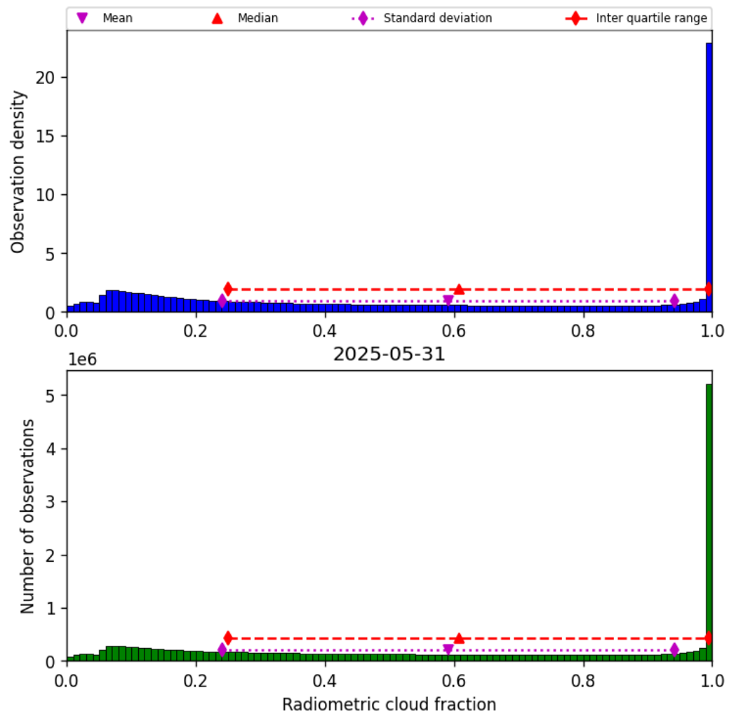
Figure 39: Histogram of “Radiometric cloud fraction” for 2025-05-31 to 2025-06-01
