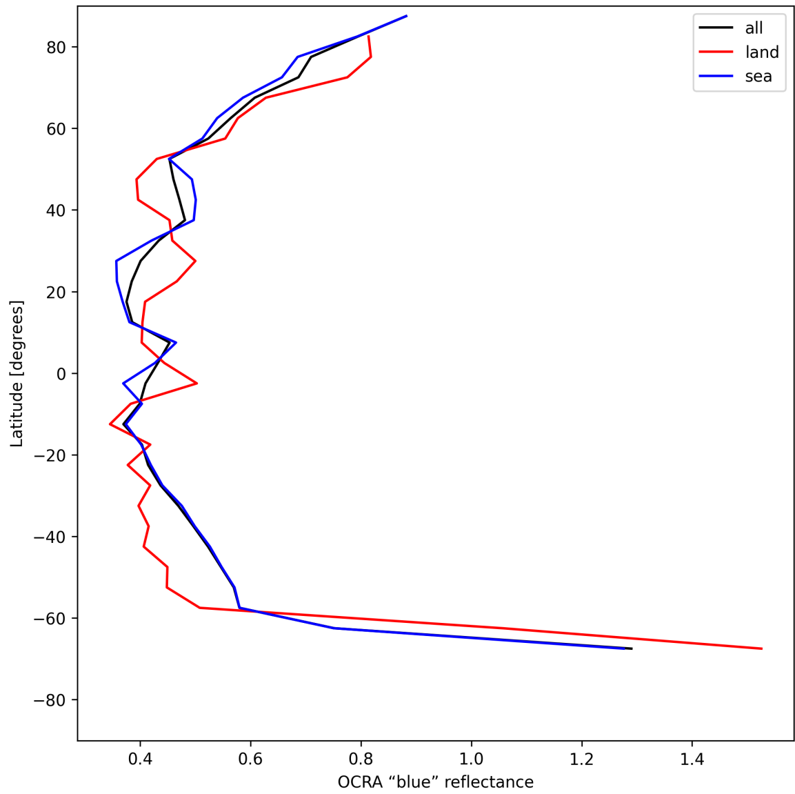
Figure 35: Zonal average of "OCRA "blue" reflectance" for 2025-05-31 to 2025-06-01.
