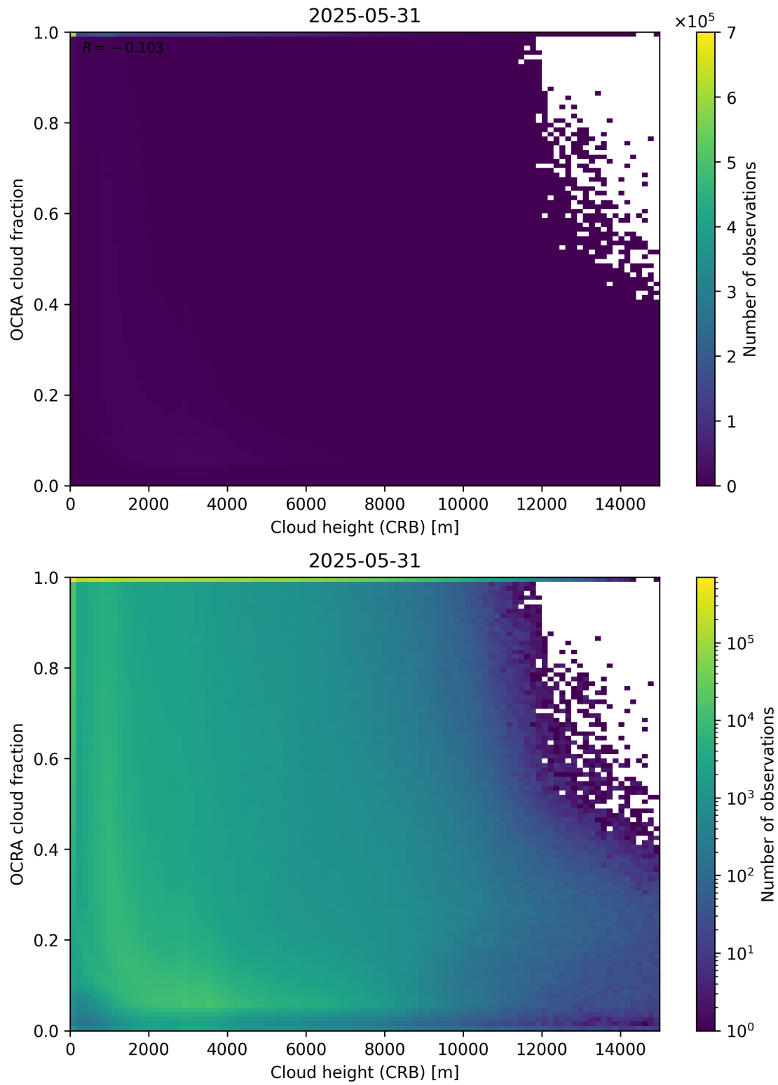
Figure 81: Scatter density plot of “Cloud height (CRB)” against “OCRA cloud fraction” for 2025-05-31 to 2025-06-01.
