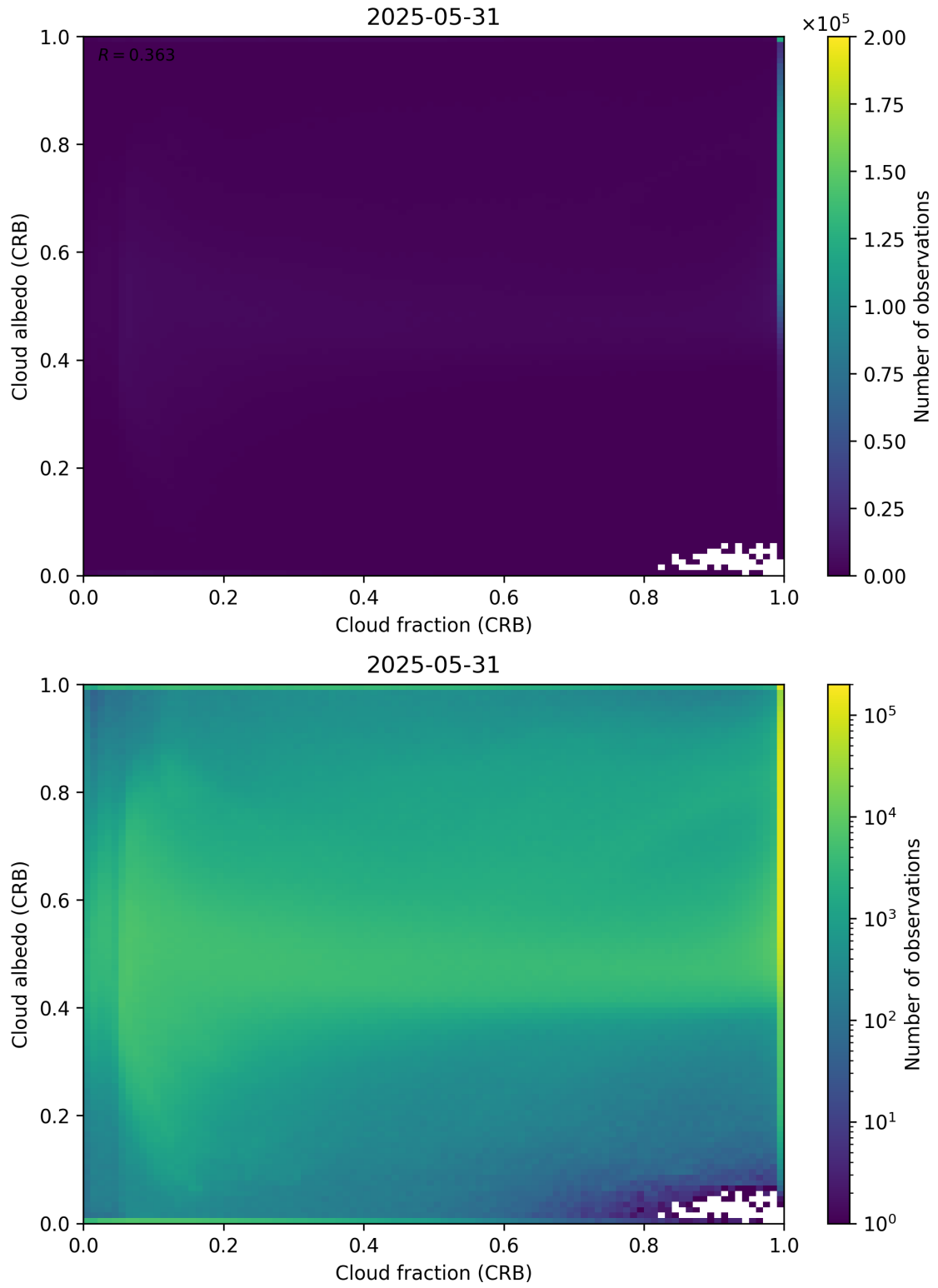
Figure 77: Scatter density plot of “Cloud fraction (CRB)” against “Cloud albedo (CRB)” for 2025-05-31 to 2025-06-01.
