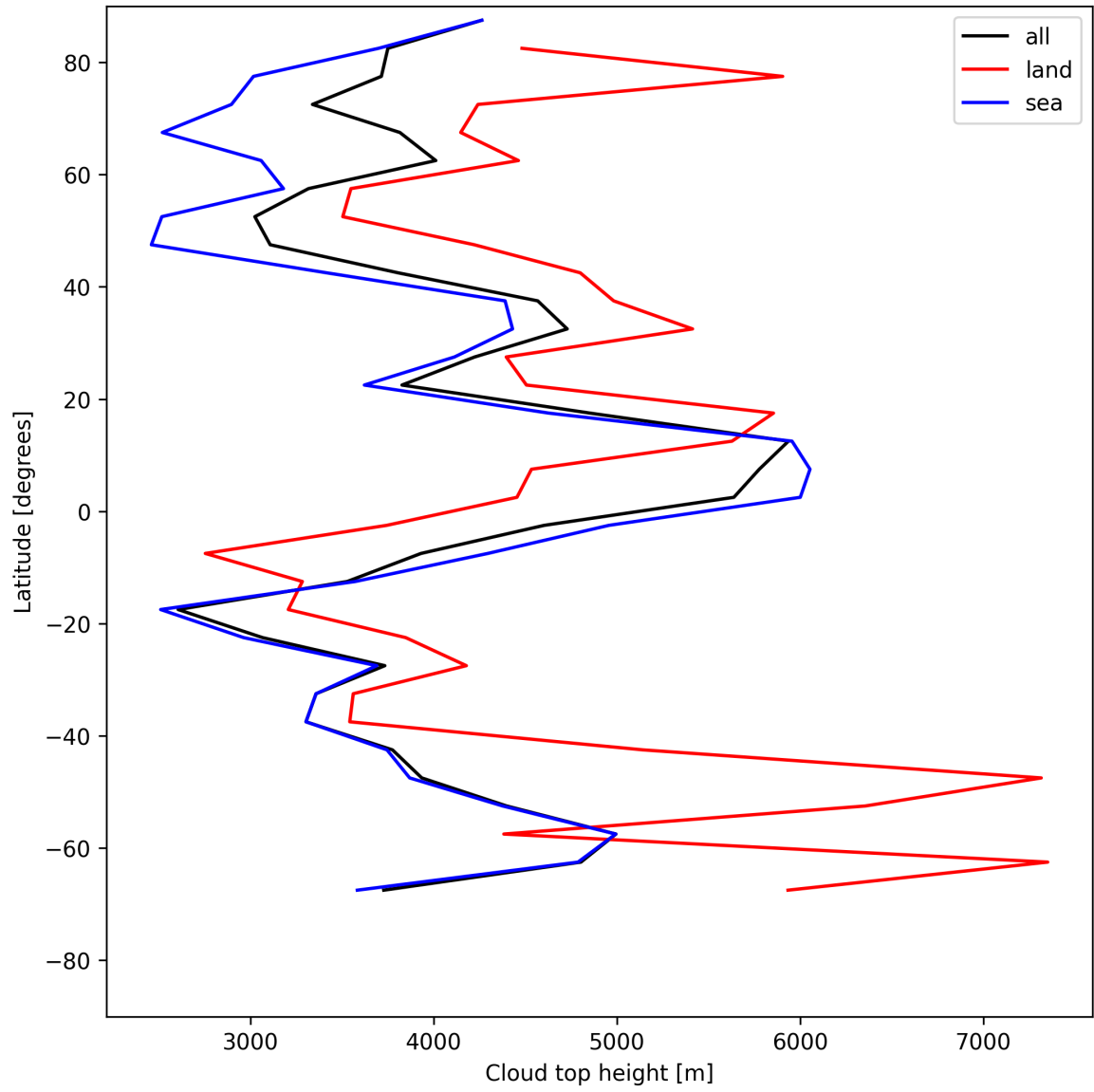
Figure 24: Zonal average of “Cloud top height” for 2025-05-31 to 2025-06-01.
