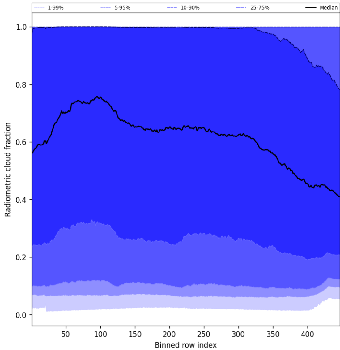
Figure 55: Along track statistics of “Radiometric cloud fraction” for 2025-05-31 to 2025-06-01
