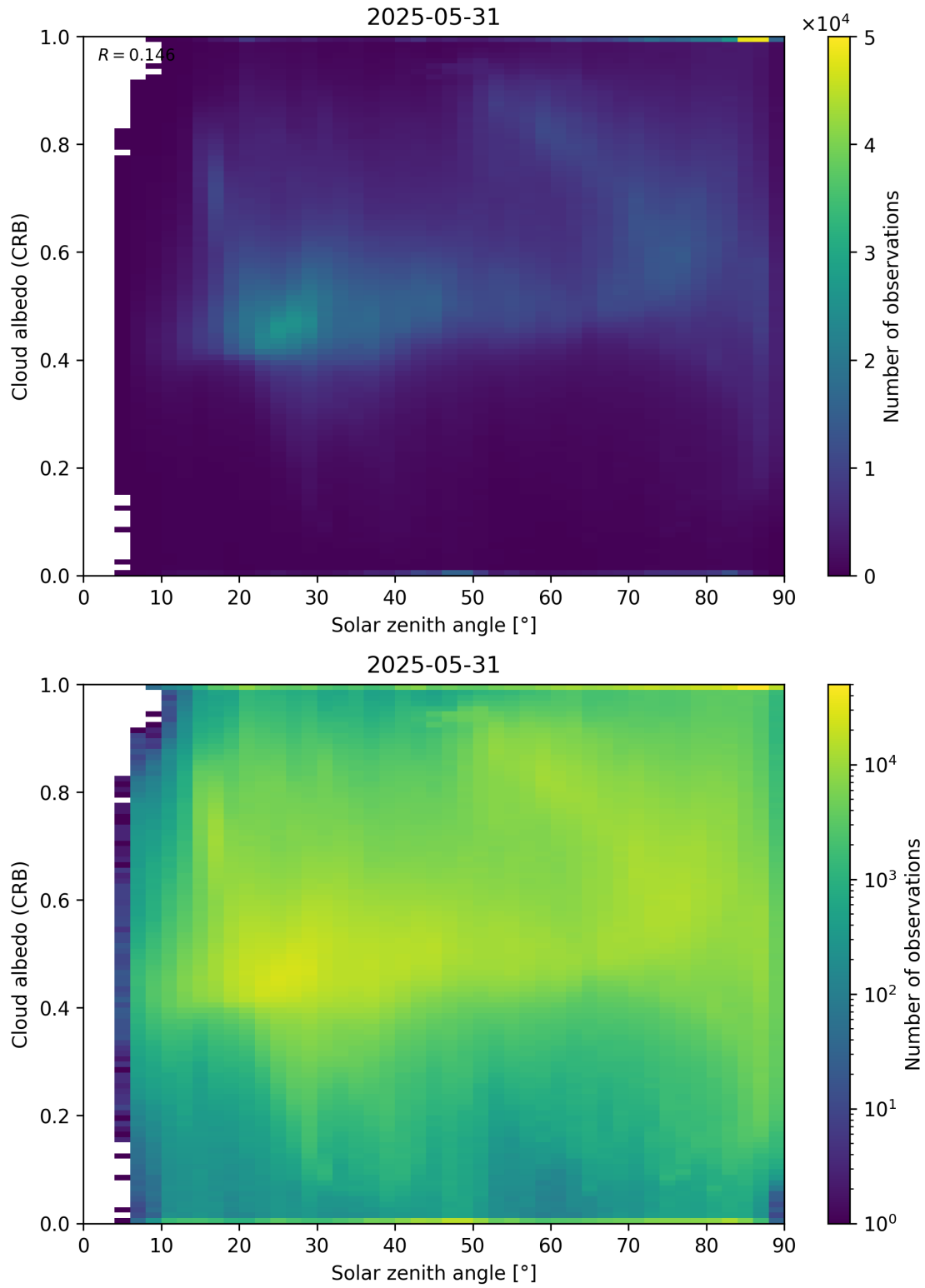
Figure 98: Scatter density plot of “Solar zenith angle” against “Cloud albedo (CRB)” for 2025-05-31 to 2025-06-01.
