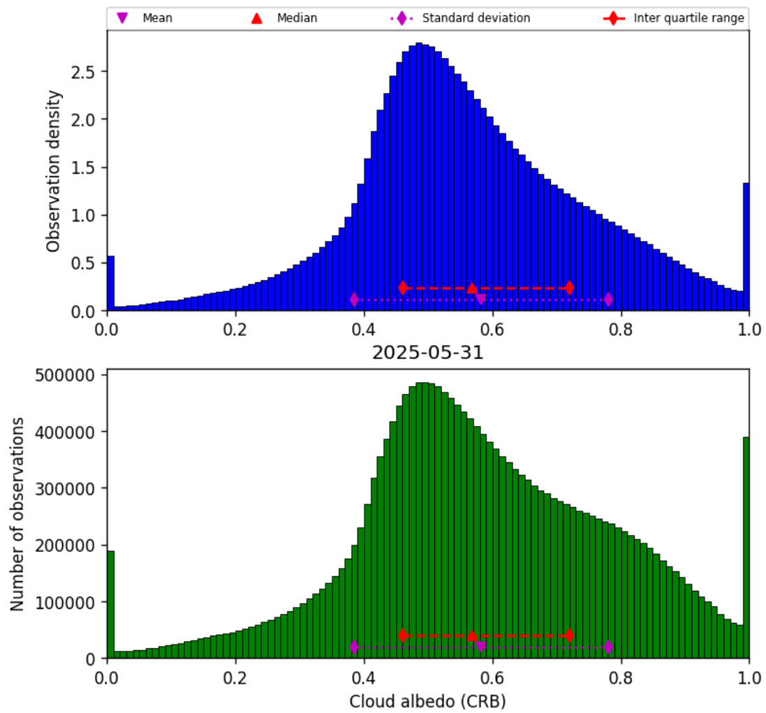
Figure 44: Histogram of “Cloud albedo (CRB)” for 2025-05-31 to 2025-06-01
