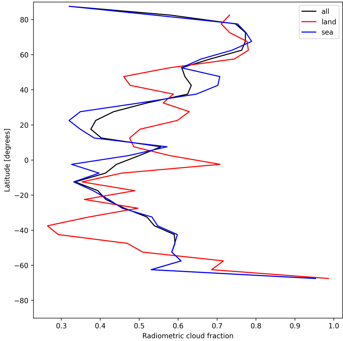
Figure 23: Zonal average of “Radiometric cloud fraction” for 2025-05-31 to 2025-06-01.
