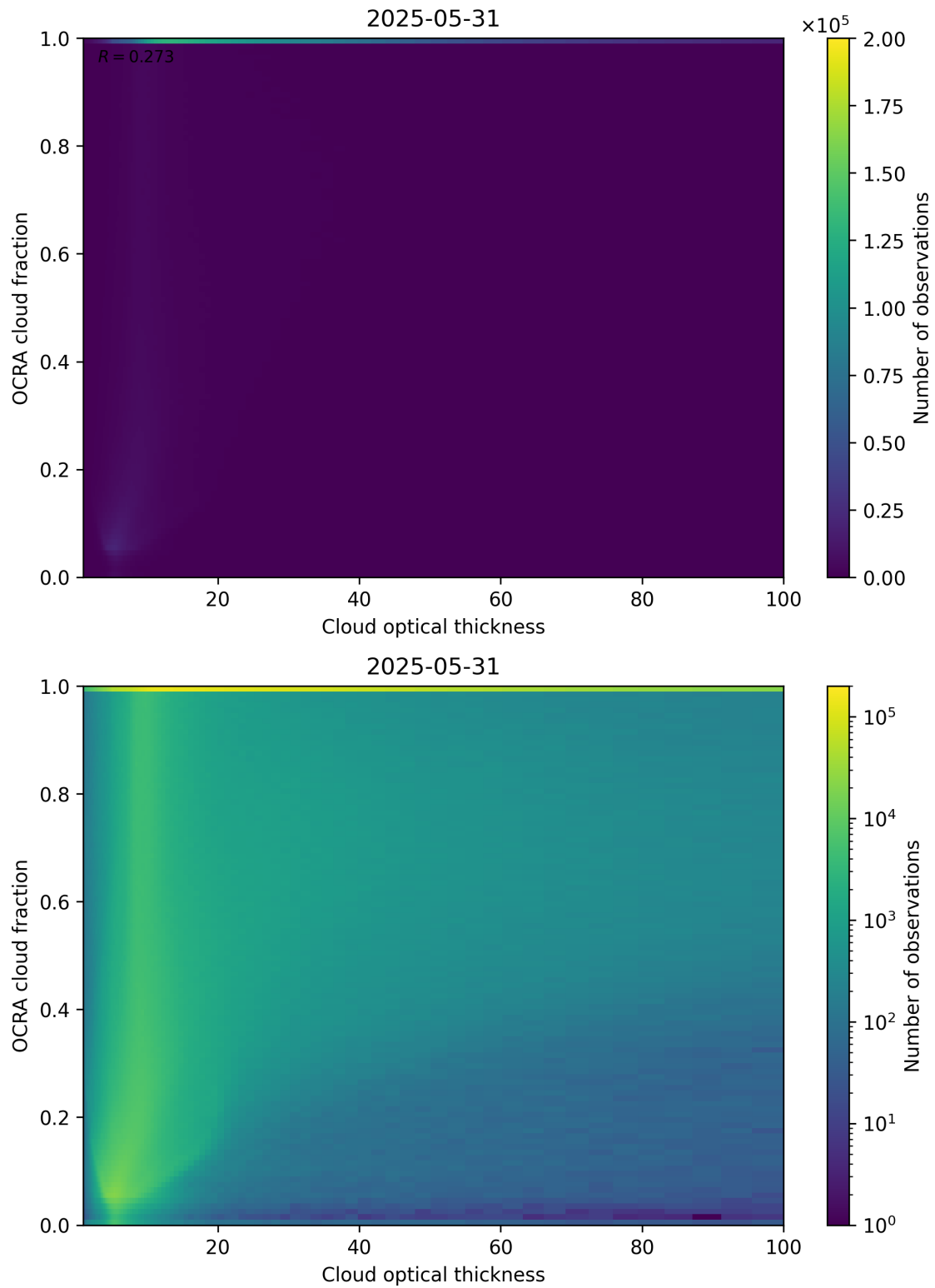
Figure 83: Scatter density plot of “Cloud optical thickness” against “OCRA cloud fraction” for 2025-05-31 to 2025-06-01.
