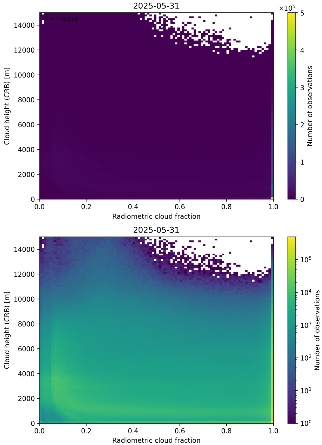
Figure 74: Scatter density plot of “Radiometric cloud fraction” against “Cloud height (CRB)” for 2025-05-31 to 2025-06-01.
