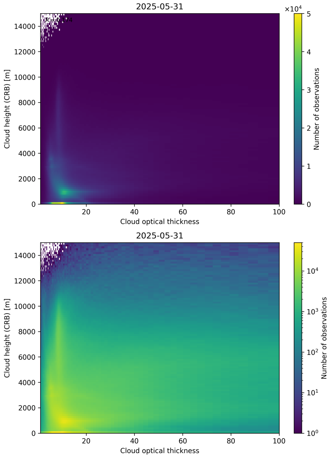
Figure 85: Scatter density plot of “Cloud optical thickness” against “Cloud height (CRB)” for 2025-05-31 to 2025-06-01.
