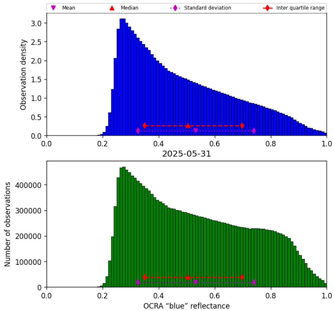
Figure 51: Histogram of “OCRA “blue” reflectance” for 2025-05-31 to 2025-06-01
