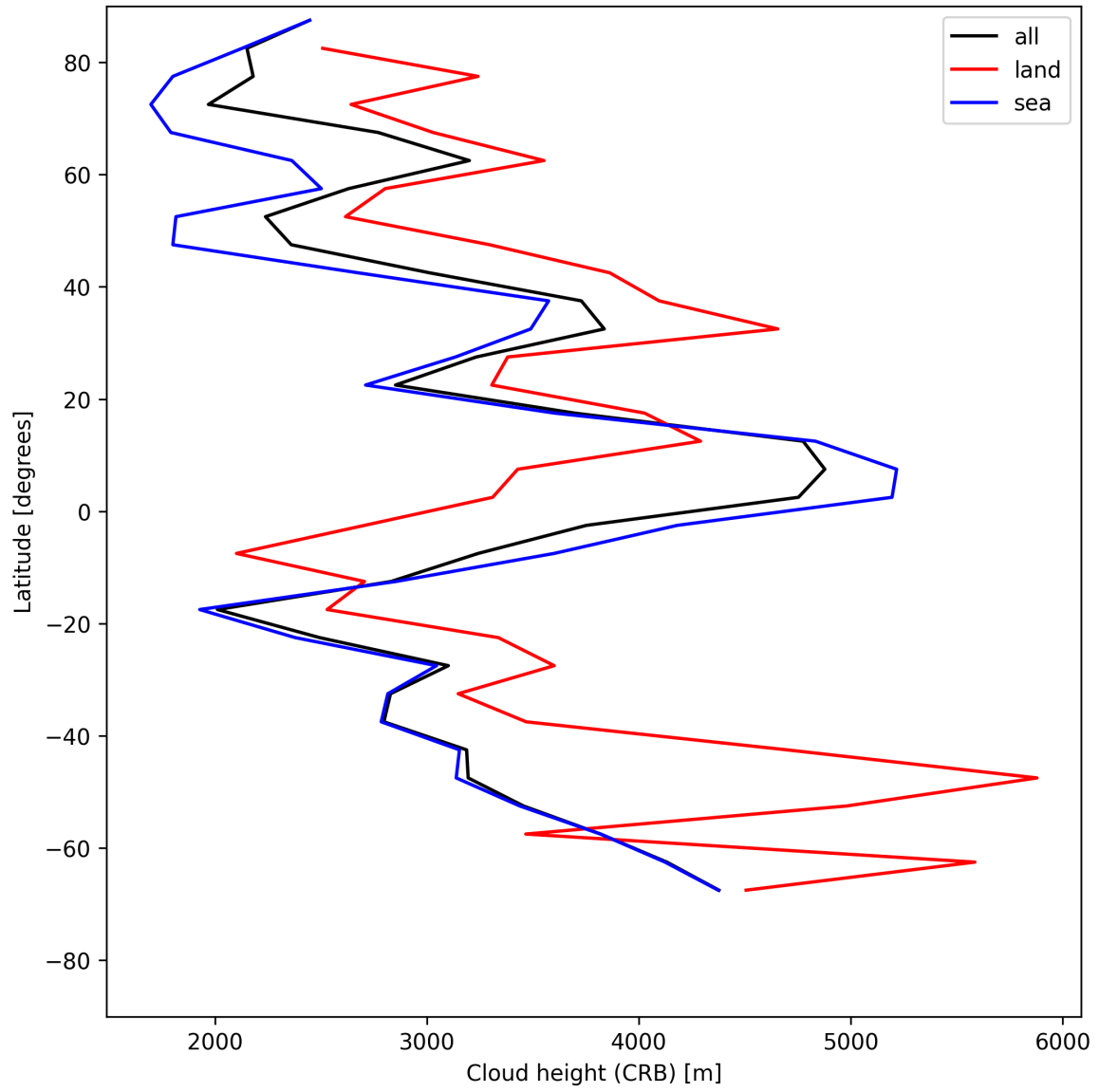
Figure 27: Zonal average of “Cloud height (CRB)” for 2025-05-31 to 2025-06-01.
