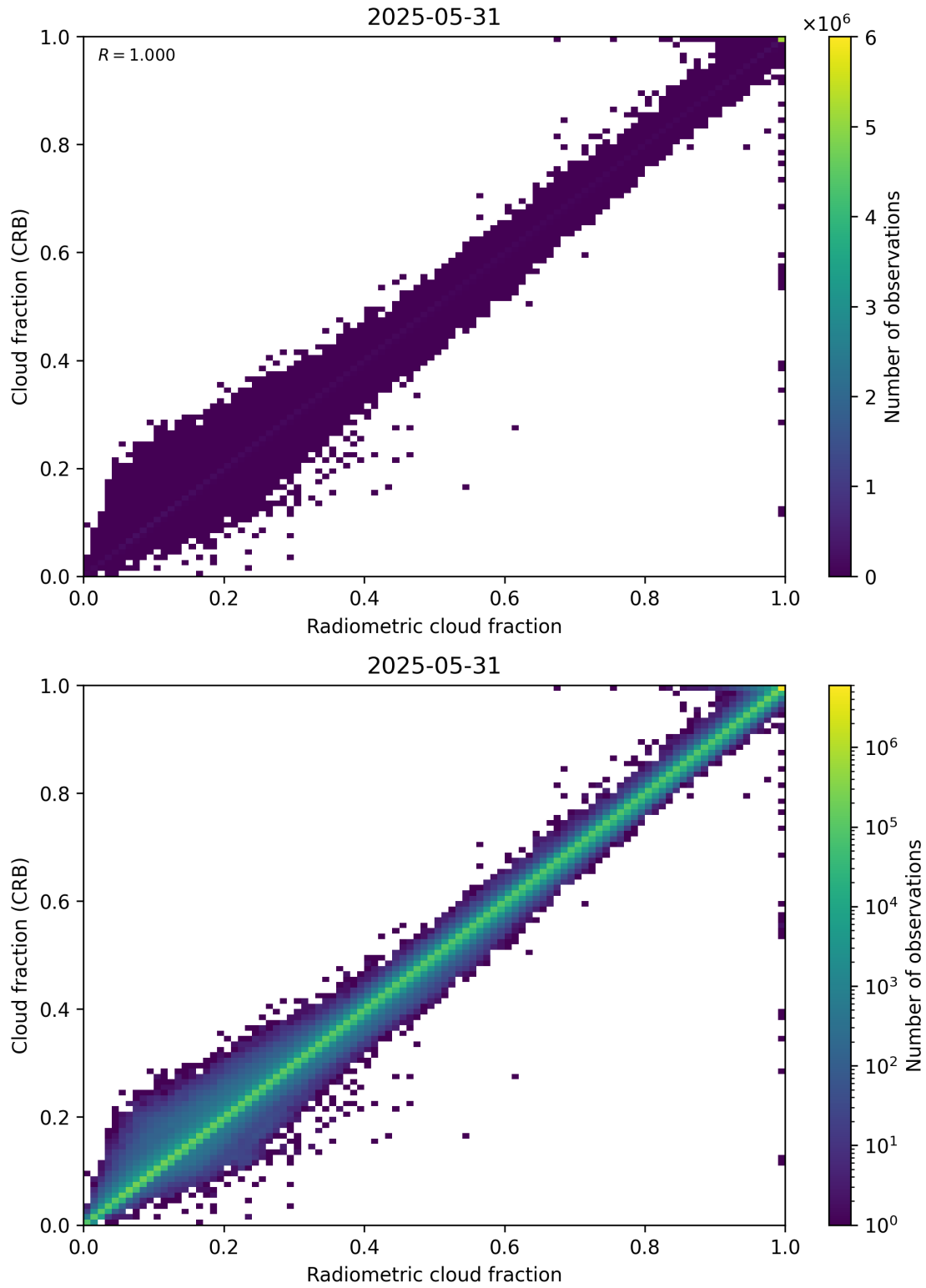
Figure 73: Scatter density plot of “Radiometric cloud fraction” against “Cloud fraction (CRB)” for 2025-05-31 to 2025-06-01.
