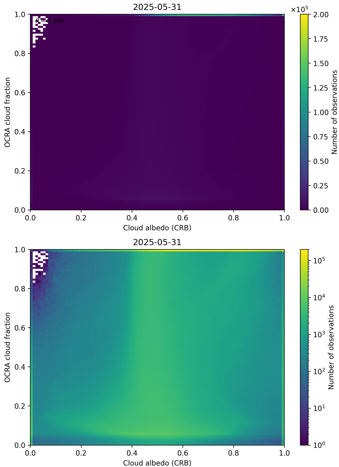
Figure 70: Scatter density plot of “Cloud albedo (CRB)” against “OCRA cloud fraction” for 2025-05-31 to 2025-06-01.
