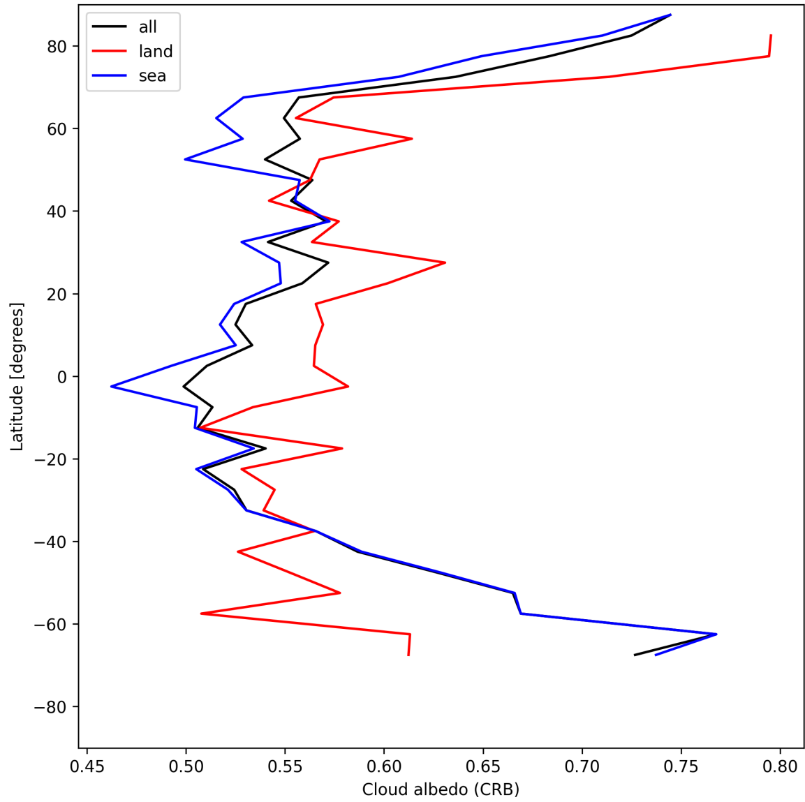
Figure 28: Zonal average of “Cloud albedo (CRB)” for 2025-05-31 to 2025-06-01.
