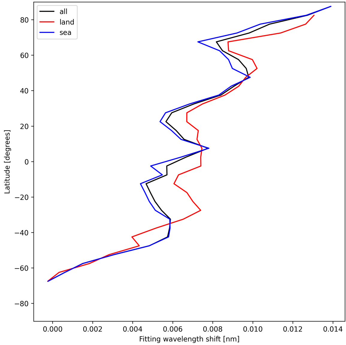
Figure 33: Zonal average of “Fitting wavelength shift” for 2025-05-31 to 2025-06-01.
