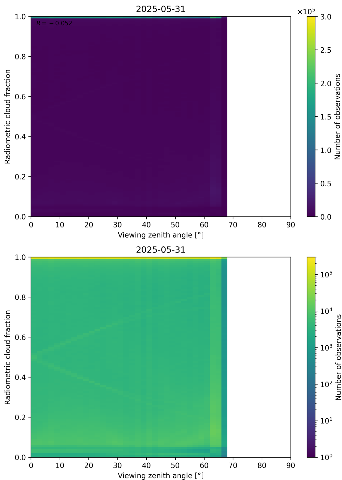
Figure 107: Scatter density plot of “Viewing zenith angle” against “Radiometric cloud fraction” for 2025-05-31 to 2025-06-01.
