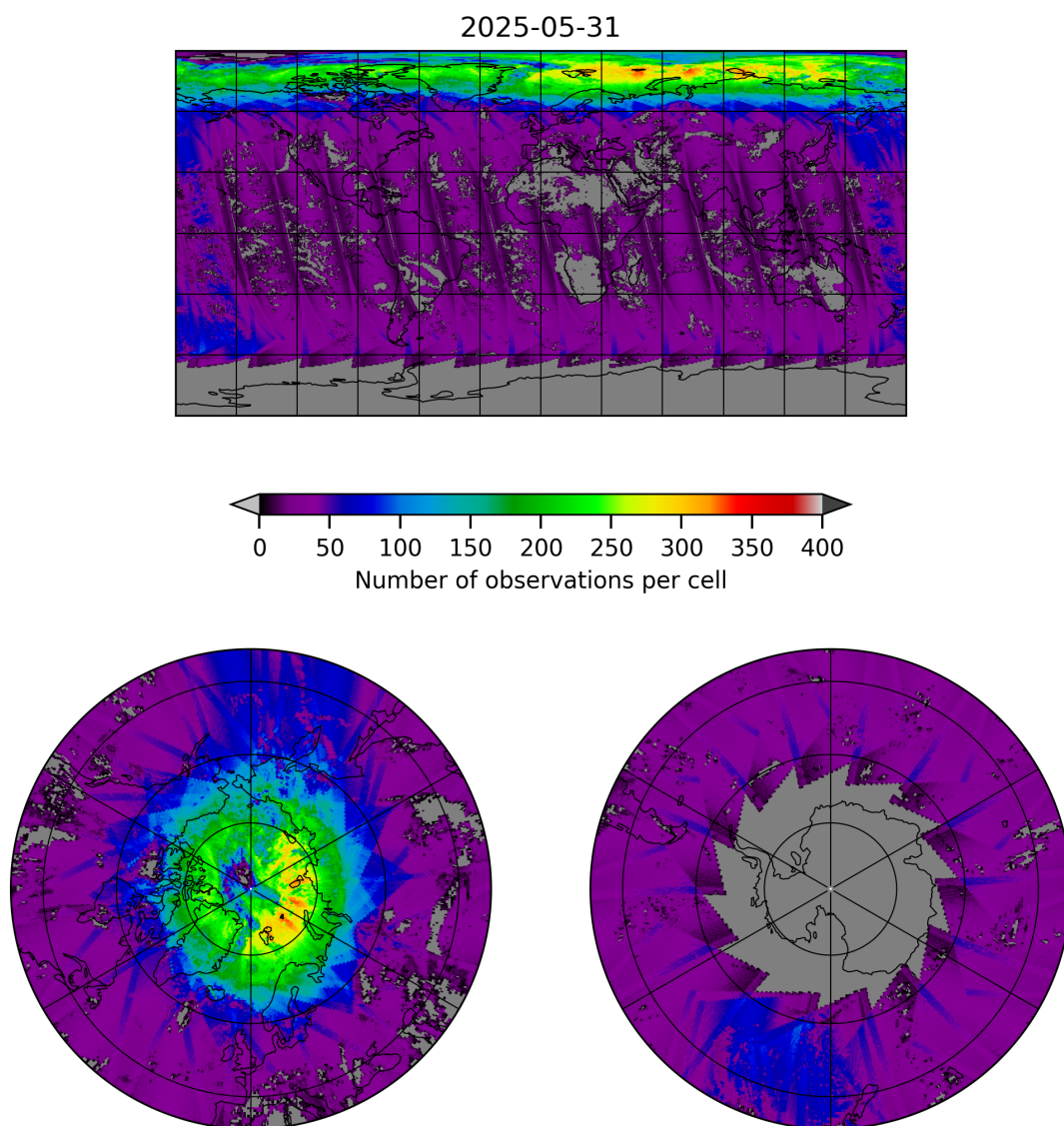
Figure 21: Map of the number of observations for 2025-05-31 to 2025-06-01
