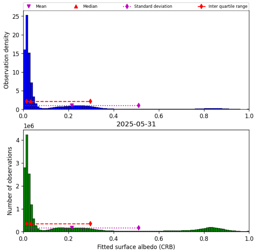
Figure 46: Histogram of “Fitted surface albedo (CRB)” for 2025-05-31 to 2025-06-01
