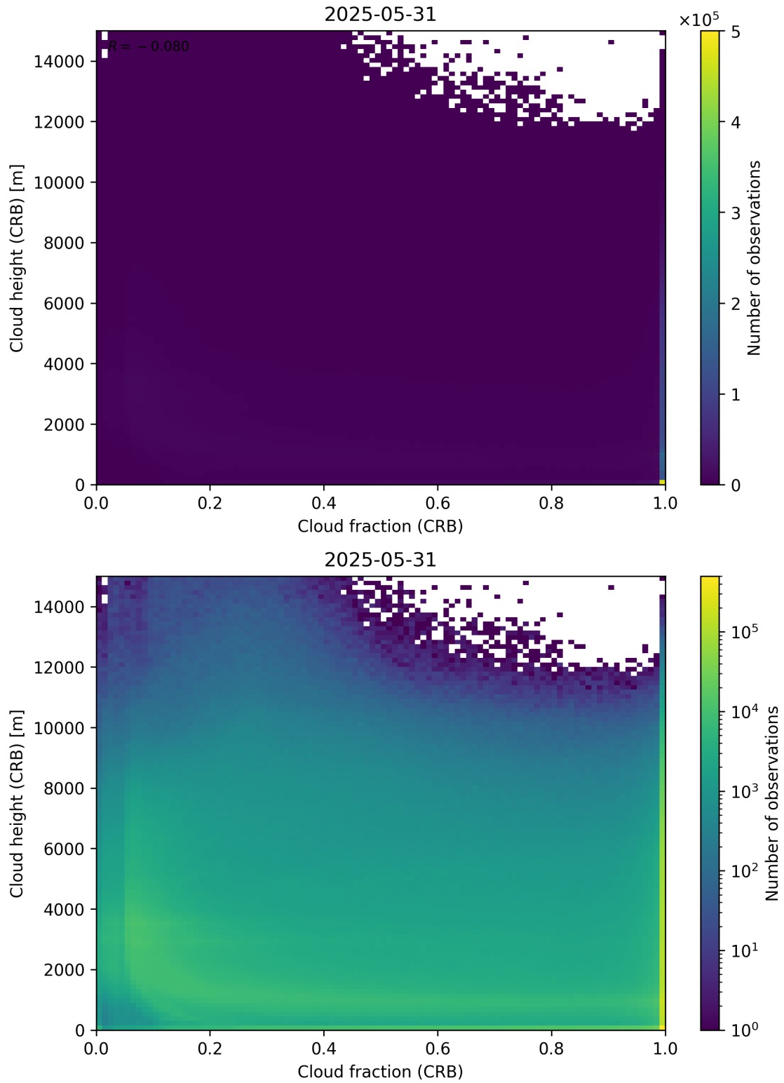
Figure 79: Scatter density plot of “Cloud fraction (CRB)” against “Cloud height (CRB)” for 2025-05-31 to 2025-06-01.
