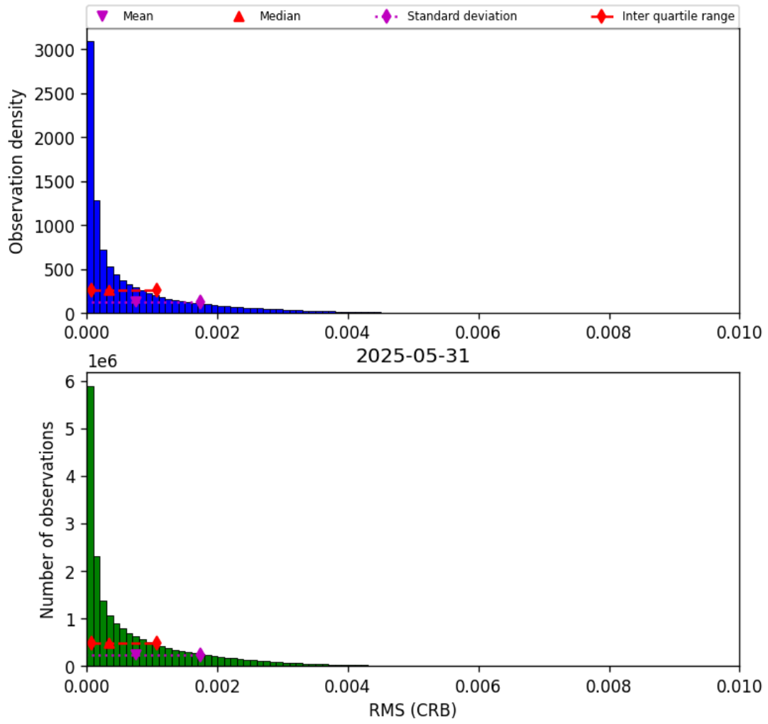
Figure 48: Histogram of “RMS (CRB)” for 2025-05-31 to 2025-06-01
