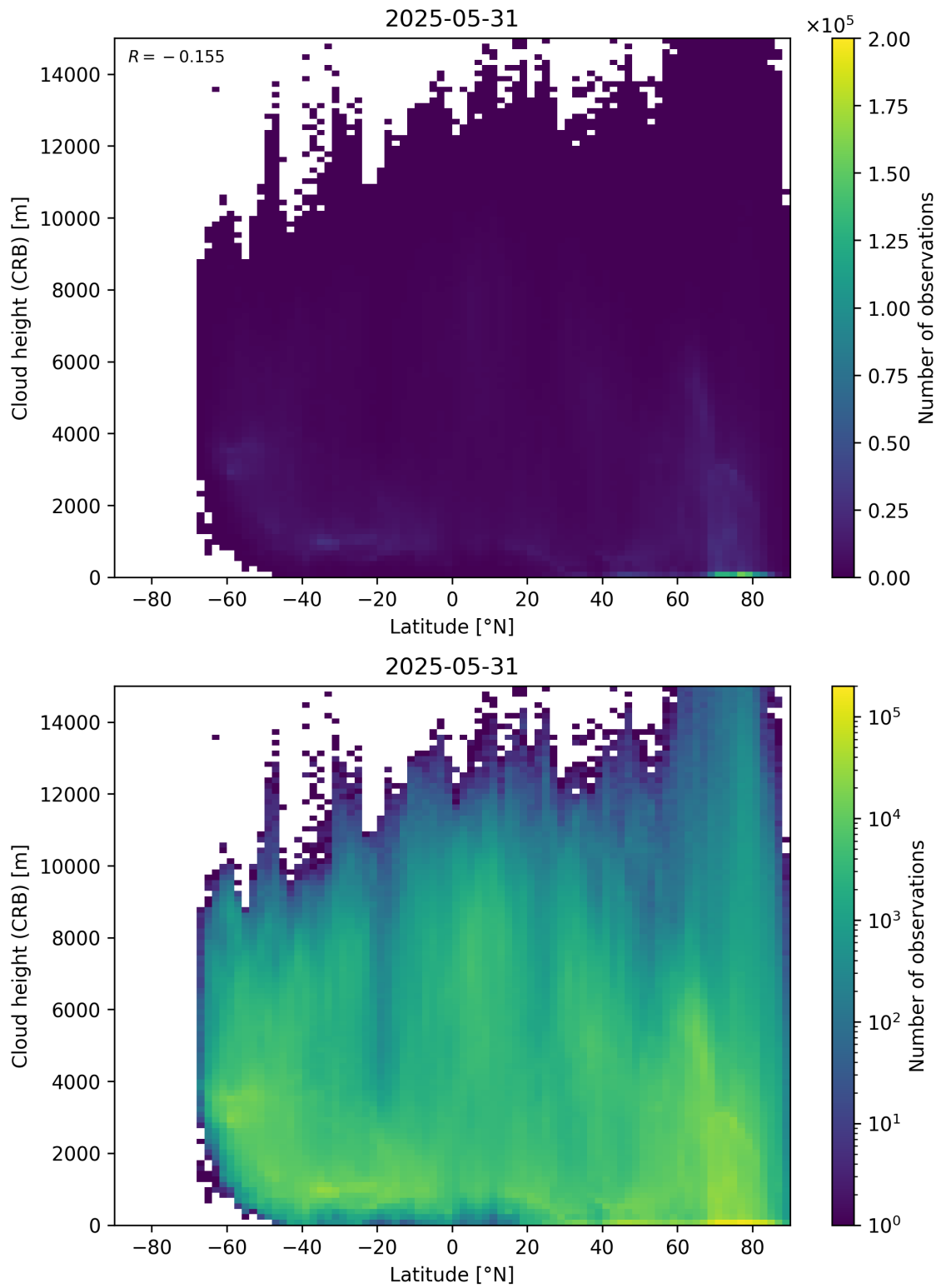
Figure 95: Scatter density plot of “Latitude” against “Cloud height (CRB)” for 2025-05-31 to 2025-06-01.
