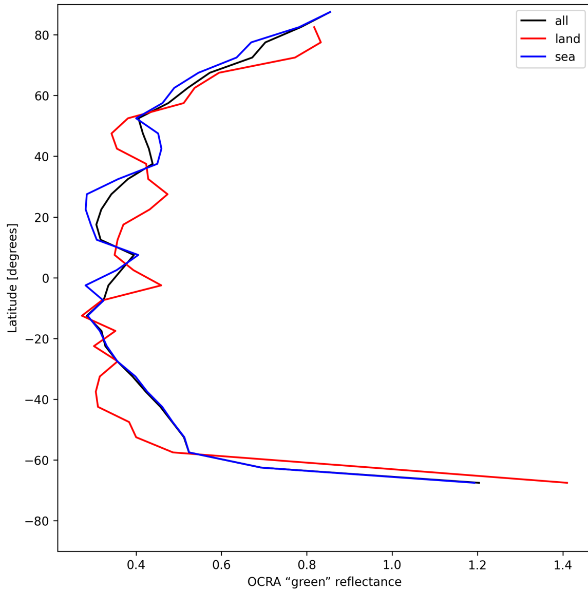
Figure 36: Zonal average of “OCRA “green” reflectance” for 2025-05-31 to 2025-06-01.
