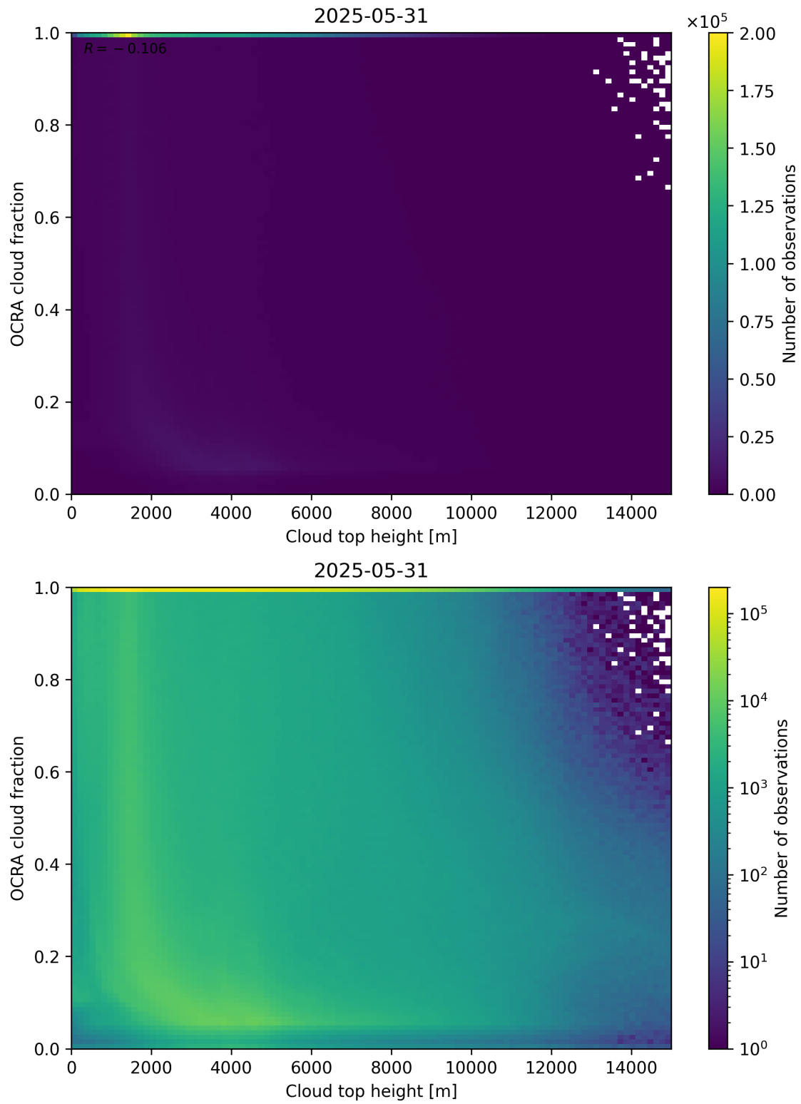
Figure 87: Scatter density plot of “Cloud top height” against “OCRA cloud fraction” for 2025-05-31 to 2025-06-01.
