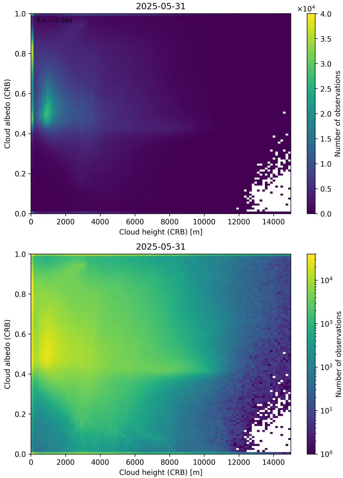
Figure 80: Scatter density plot of “Cloud height (CRB)” against “Cloud albedo (CRB)” for 2025-05-31 to 2025-06-01.
