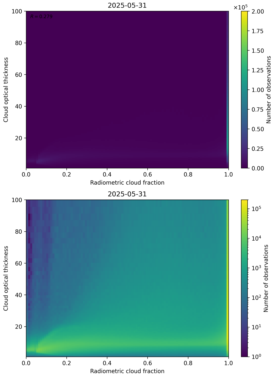
Figure 75: Scatter density plot of “Radiometric cloud fraction” against “Cloud optical thickness” for 2025-05-31 to 2025-06-01.
