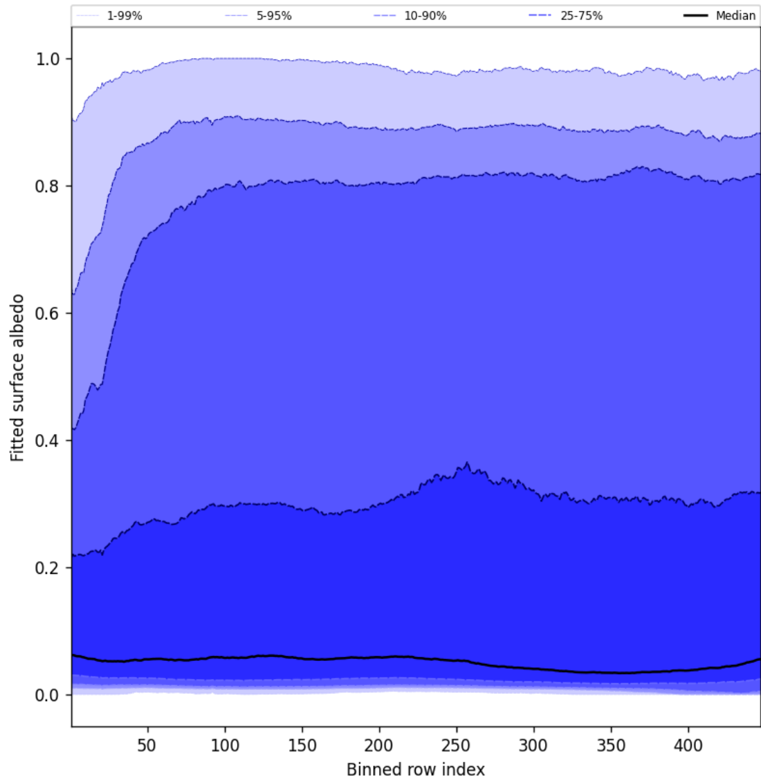
Figure 61: Along track statistics of “Fitted surface albedo” for 2025-05-31 to 2025-06-01
