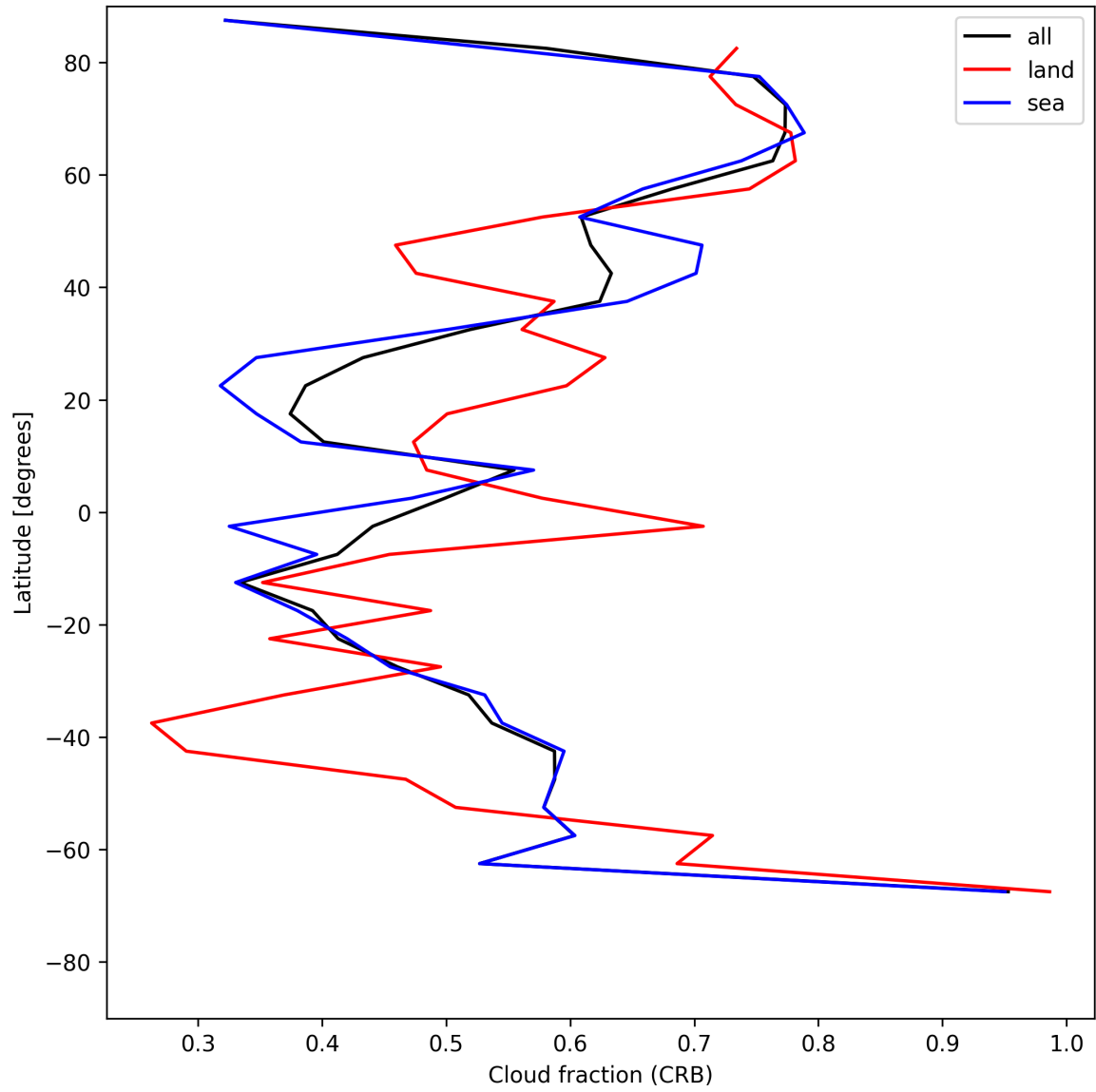
Figure 26: Zonal average of “Cloud fraction (CRB)” for 2025-05-31 to 2025-06-01.
