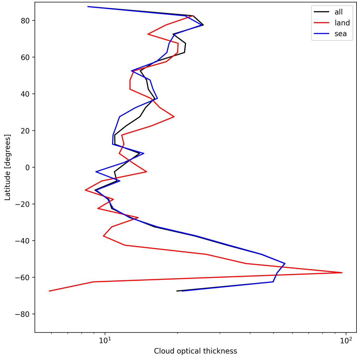
Figure 25: Zonal average of “Cloud optical thickness” for 2025-05-31 to 2025-06-01.
