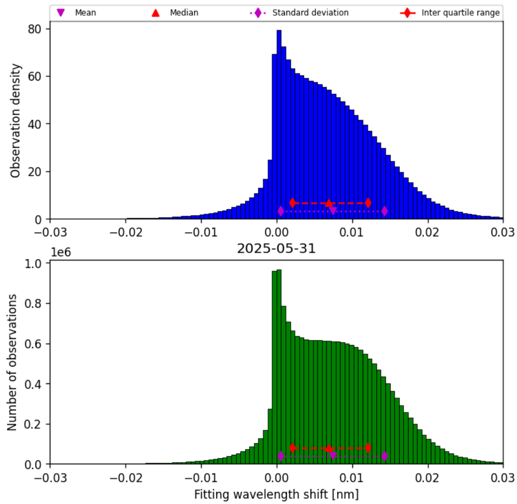
Figure 49: Histogram of “Fitting wavelength shift” for 2025-05-31 to 2025-06-01
