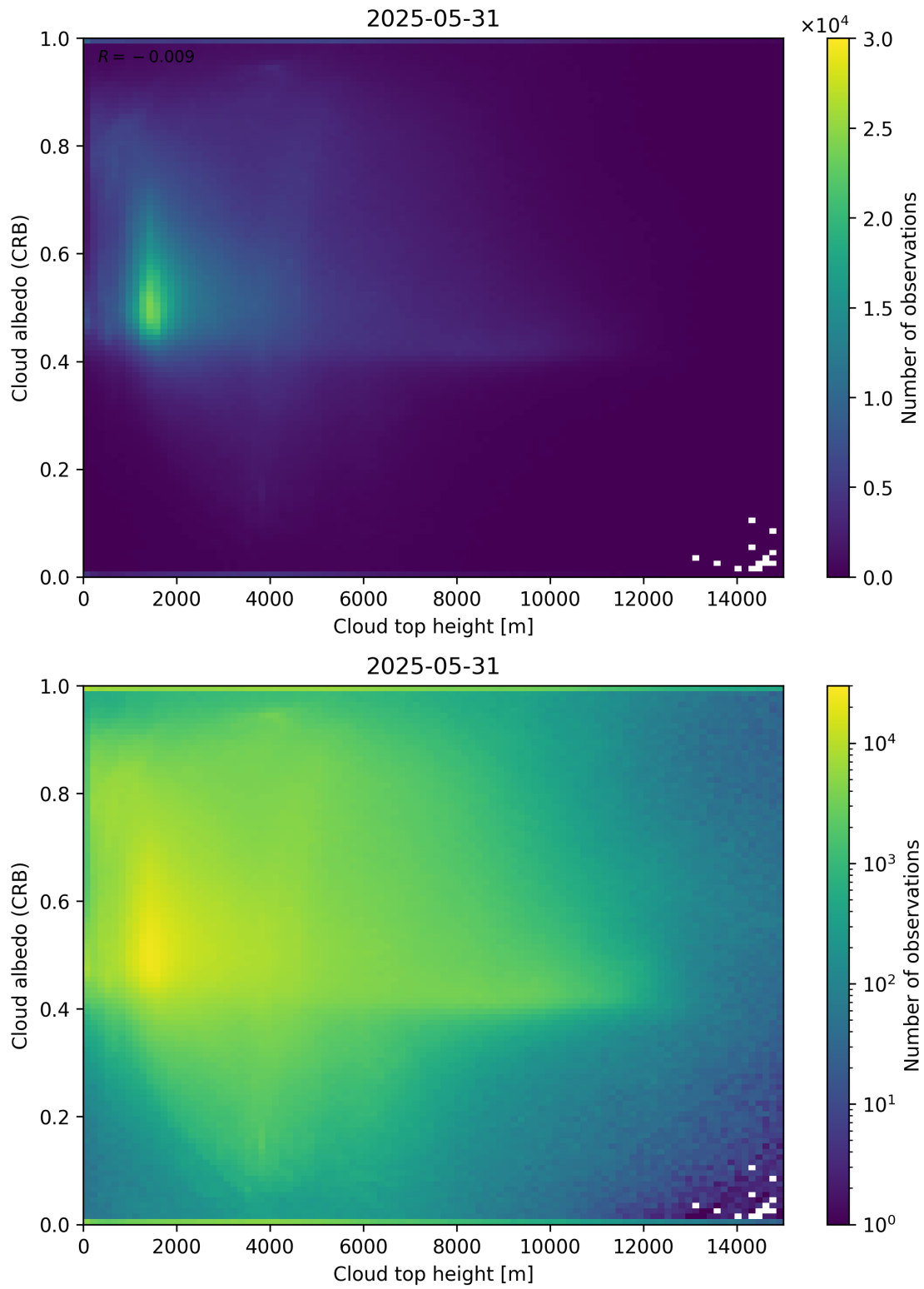
Figure 86: Scatter density plot of “Cloud top height” against “Cloud albedo (CRB)” for 2025-05-31 to 2025-06-01.
