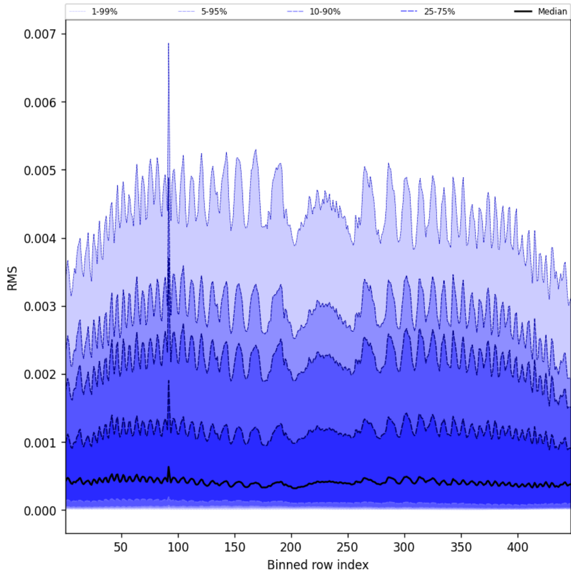
Figure 63: Along track statistics of “RMS” for 2025-05-31 to 2025-06-01
