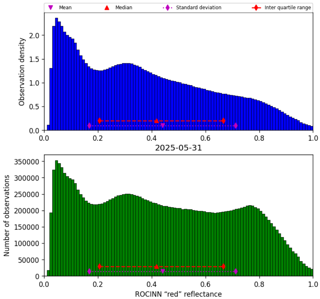
Figure 53: Histogram of “ROCINN “red” reflectance” for 2025-05-31 to 2025-06-01
