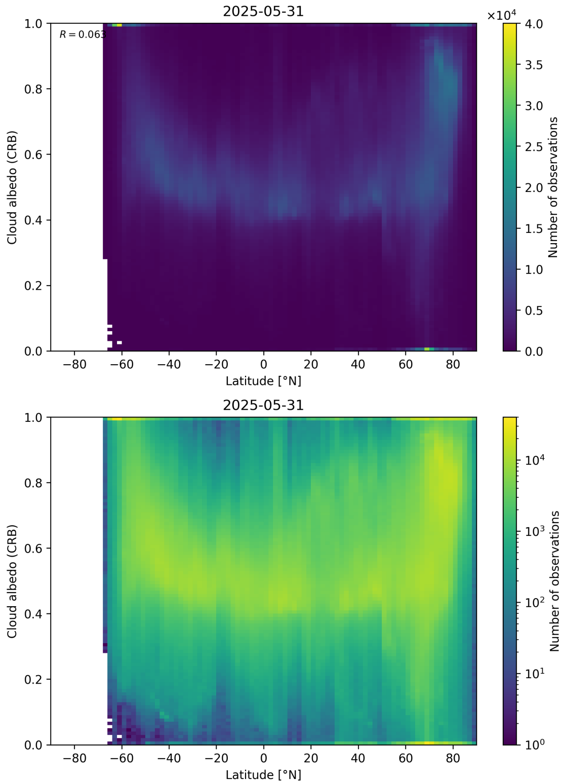
Figure 91: Scatter density plot of “Latitude” against “Cloud albedo (CRB)” for 2025-05-31 to 2025-06-01.
