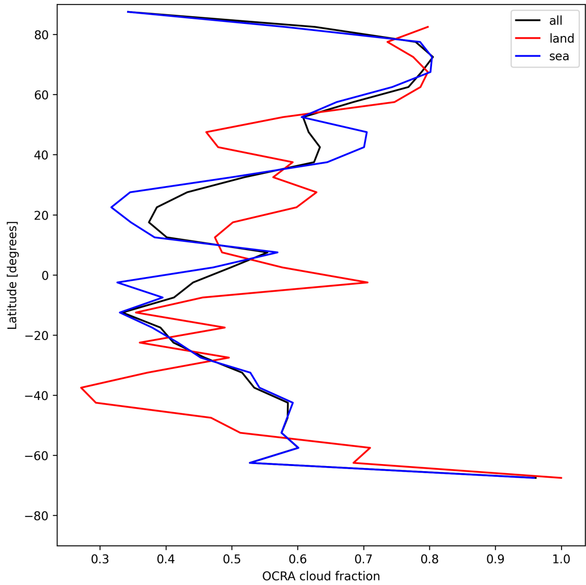
Figure 34: Zonal average of “OCRA cloud fraction” for 2025-05-31 to 2025-06-01.
