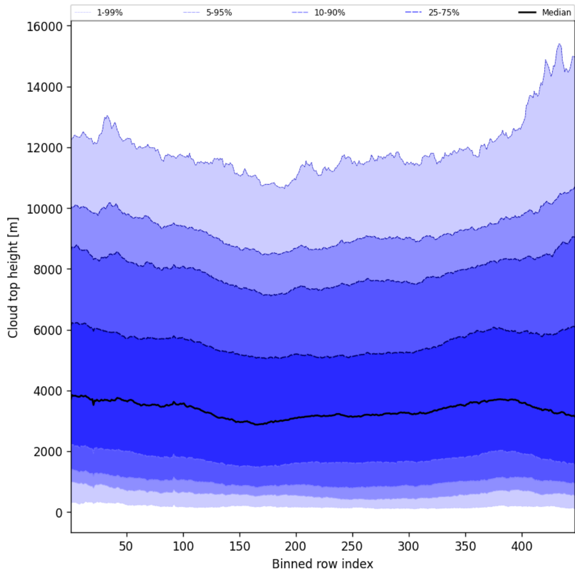
Figure 56: Along track statistics of “Cloud top height” for 2025-05-31 to 2025-06-01
