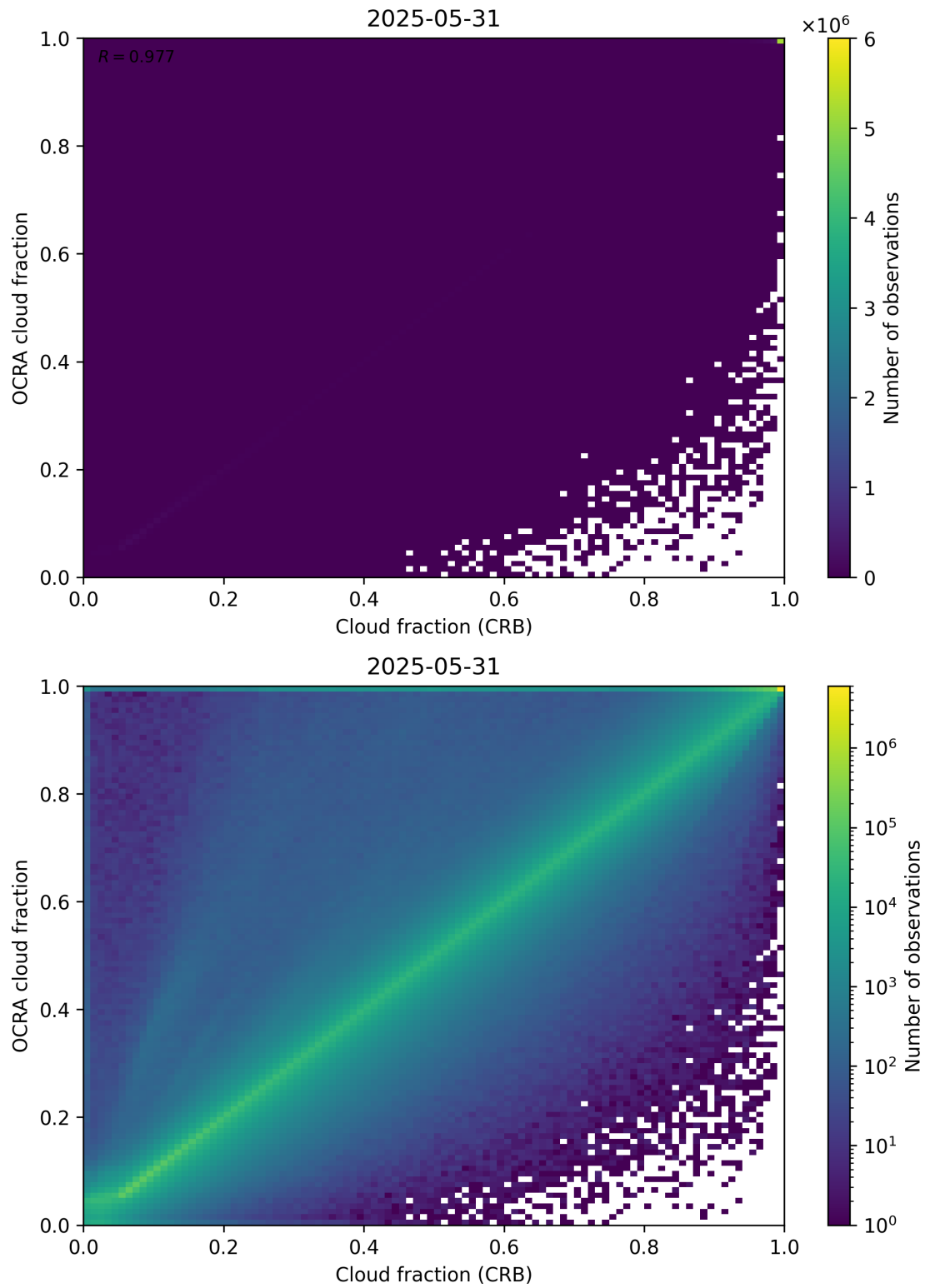
Figure 78: Scatter density plot of “Cloud fraction (CRB)” against “OCRA cloud fraction” for 2025-05-31 to 2025-06-01.
