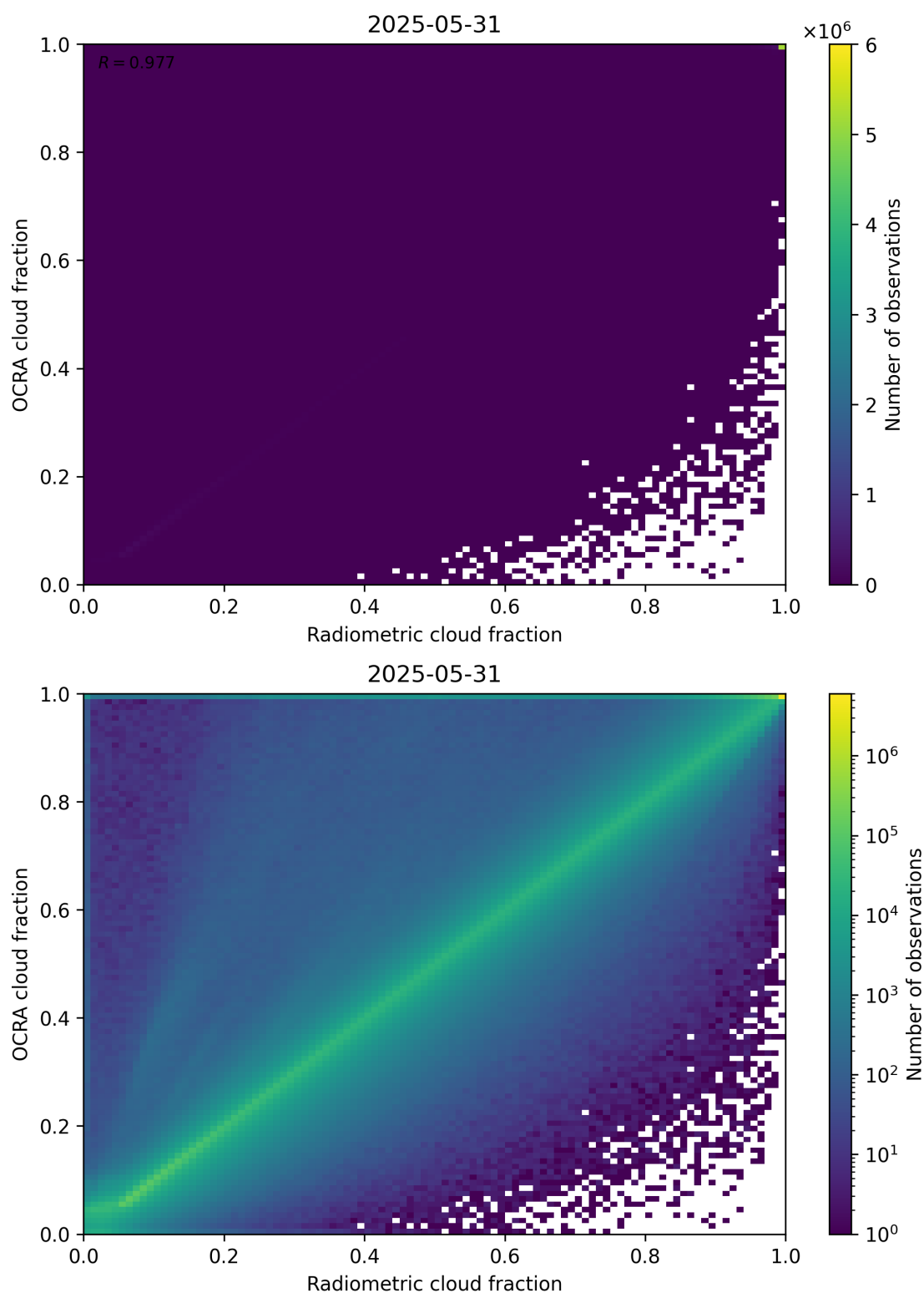
Figure 72: Scatter density plot of “Radiometric cloud fraction” against “OCRA cloud fraction” for 2025-05-31 to 2025-06-01.
