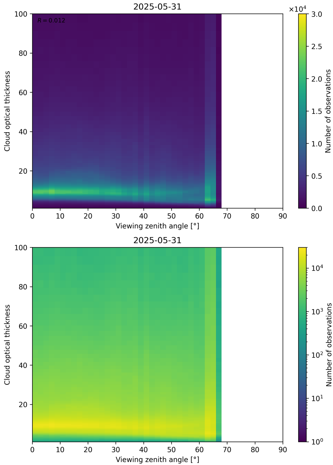
Figure 111: Scatter density plot of “Viewing zenith angle” against “Cloud optical thickness” for 2025-05-31 to 2025-06-01.
