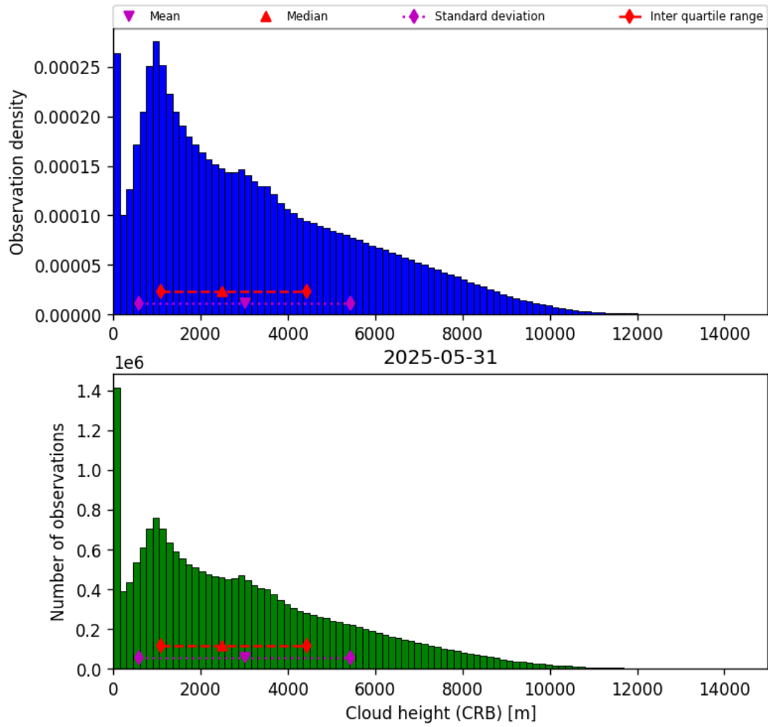
Figure 43: Histogram of “Cloud height (CRB)” for 2025-05-31 to 2025-06-01
