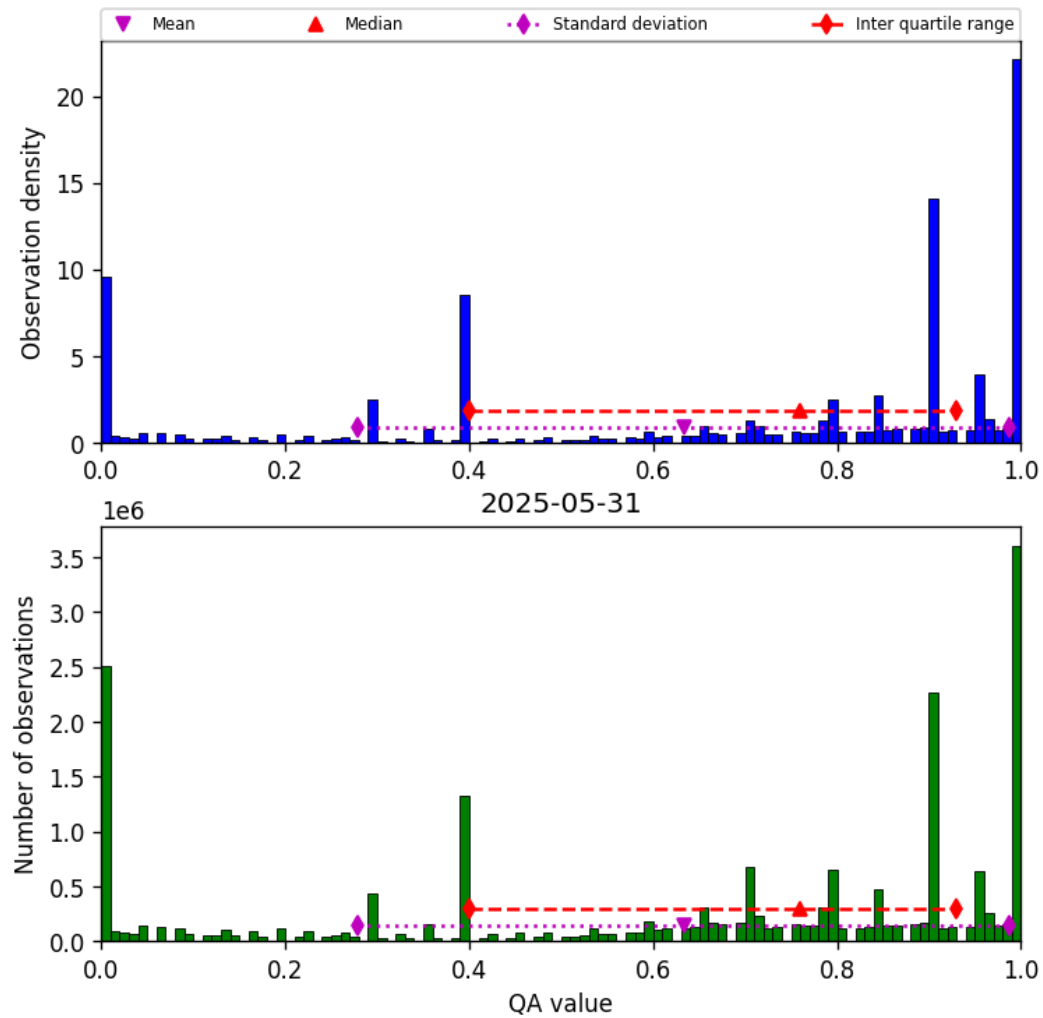
Figure 38: Histogram of “QA value” for 2025-05-31 to 2025-06-01
