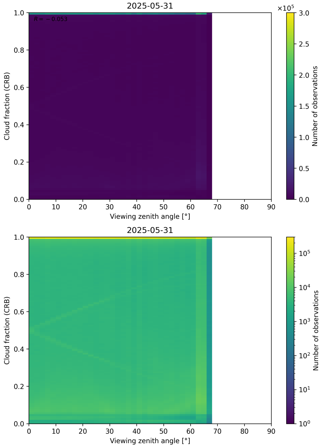
Figure 109: Scatter density plot of “Viewing zenith angle” against “Cloud fraction (CRB)” for 2025-05-31 to 2025-06-01.
