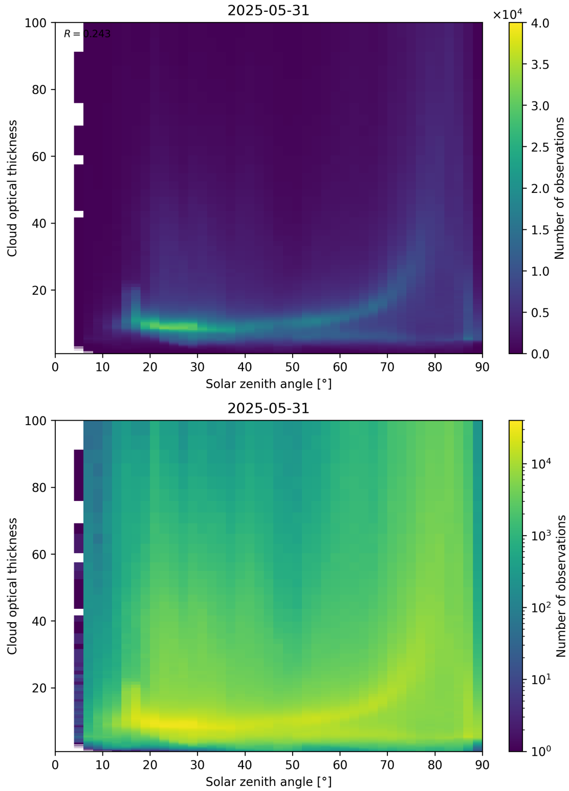
Figure 103: Scatter density plot of “Solar zenith angle” against “Cloud optical thickness” for 2025-05-31 to 2025-06-01.
