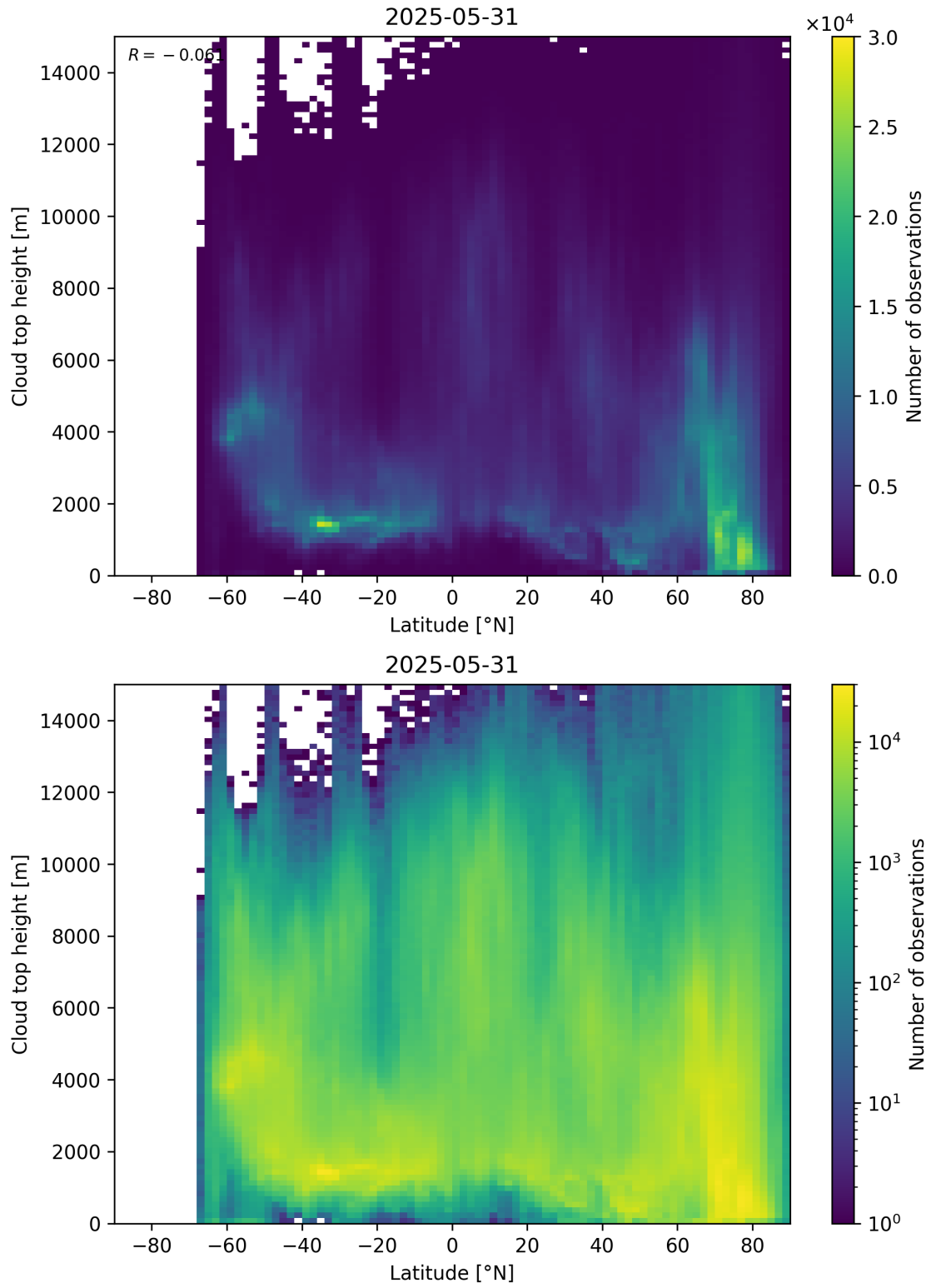
Figure 97: Scatter density plot of “Latitude” against “Cloud top height” for 2025-05-31 to 2025-06-01.
