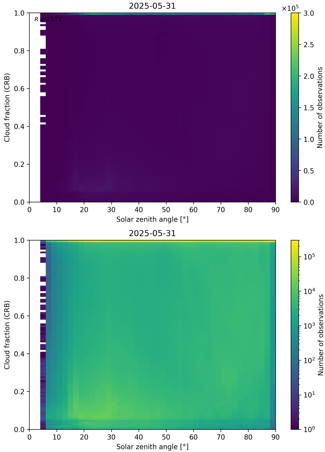
Figure 101: Scatter density plot of “Solar zenith angle” against “Cloud fraction (CRB)” for 2025-05-31 to 2025-06-01.
