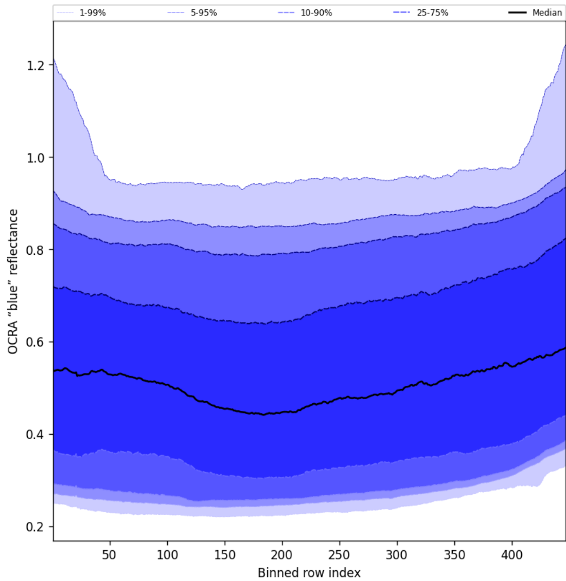
Figure 67: Along track statistics of “OCRA “blue” reflectance” for 2025-05-31 to 2025-06-01
