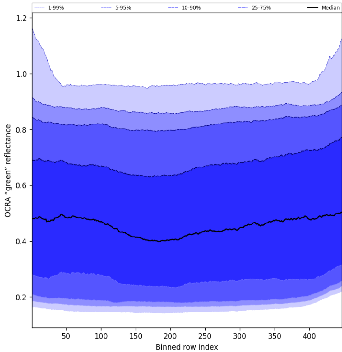
Figure 68: Along track statistics of "OCRA "green" reflectance" for 2025-05-31 to 2025-06-01
