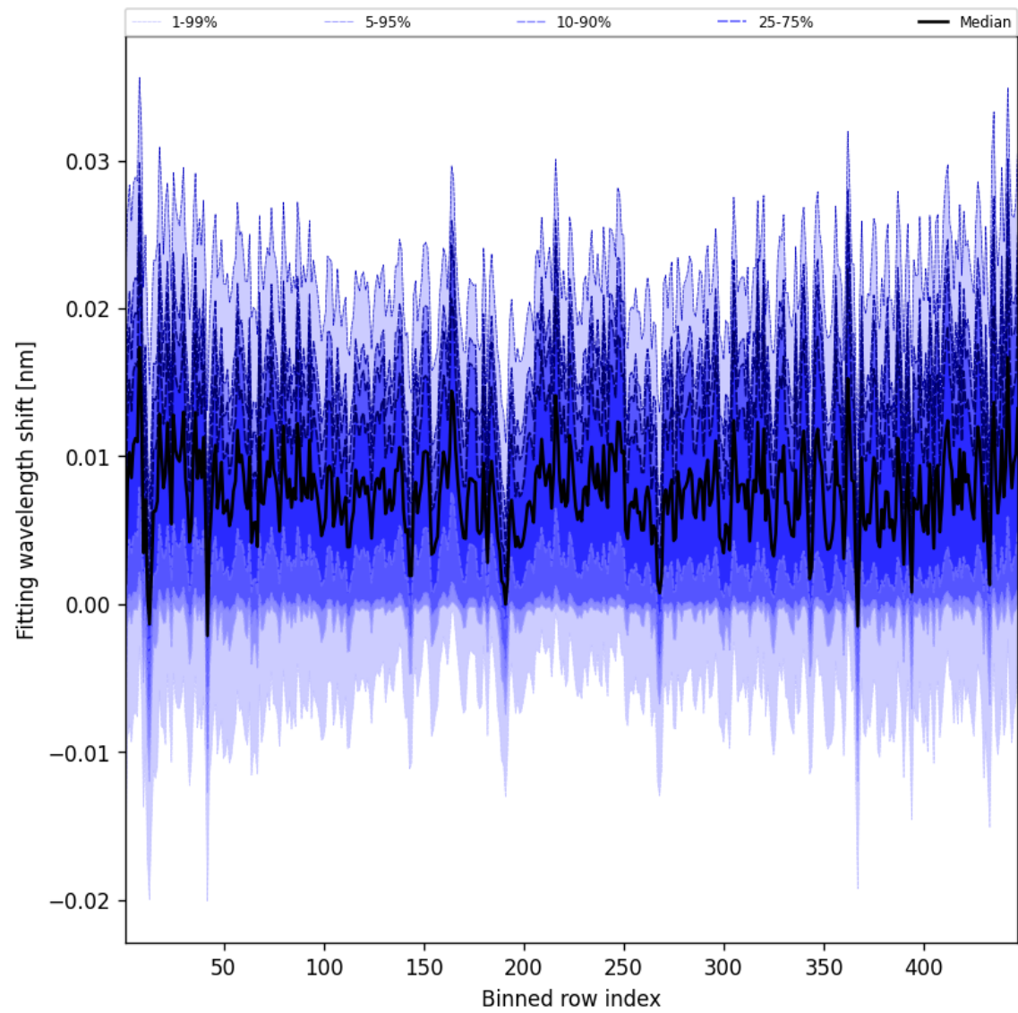
Figure 65: Along track statistics of “Fitting wavelength shift” for 2025-05-31 to 2025-06-01
