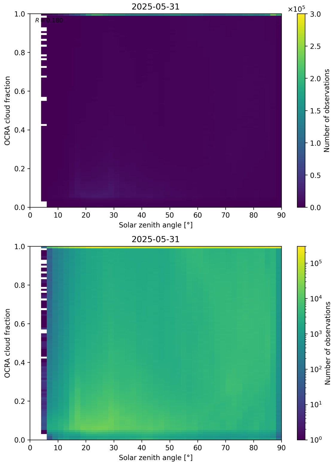
Figure 100: Scatter density plot of “Solar zenith angle” against “OCRA cloud fraction” for 2025-05-31 to 2025-06-01.
