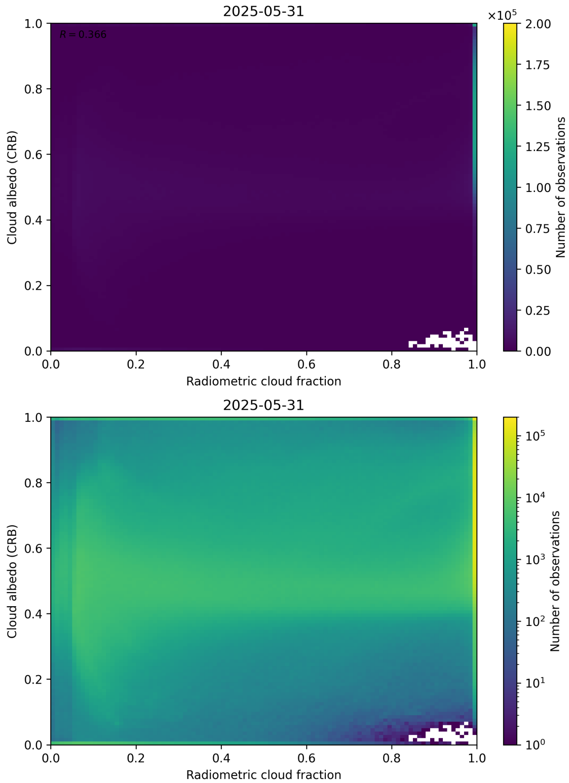
Figure 71: Scatter density plot of “Radiometric cloud fraction” against “Cloud albedo (CRB)” for 2025-05-31 to 2025-06-01.
