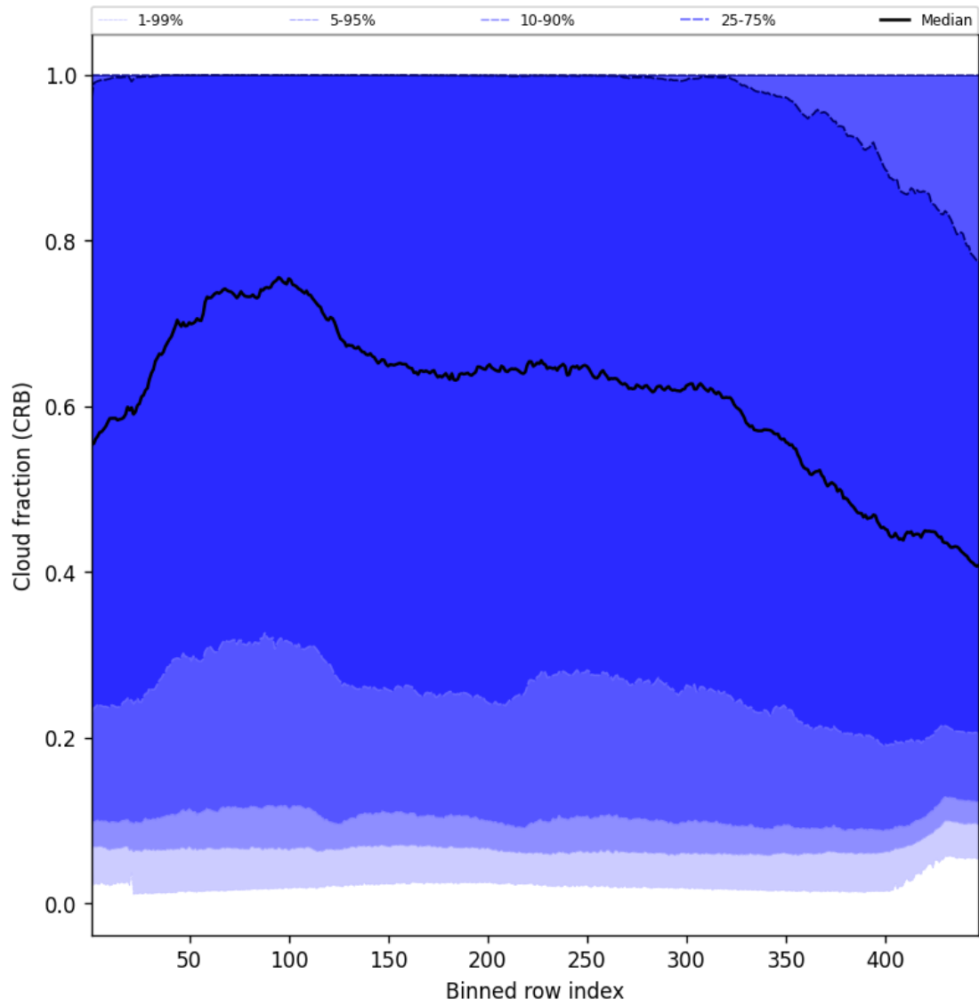
Figure 58: Along track statistics of “Cloud fraction (CRB)” for 2025-05-31 to 2025-06-01
