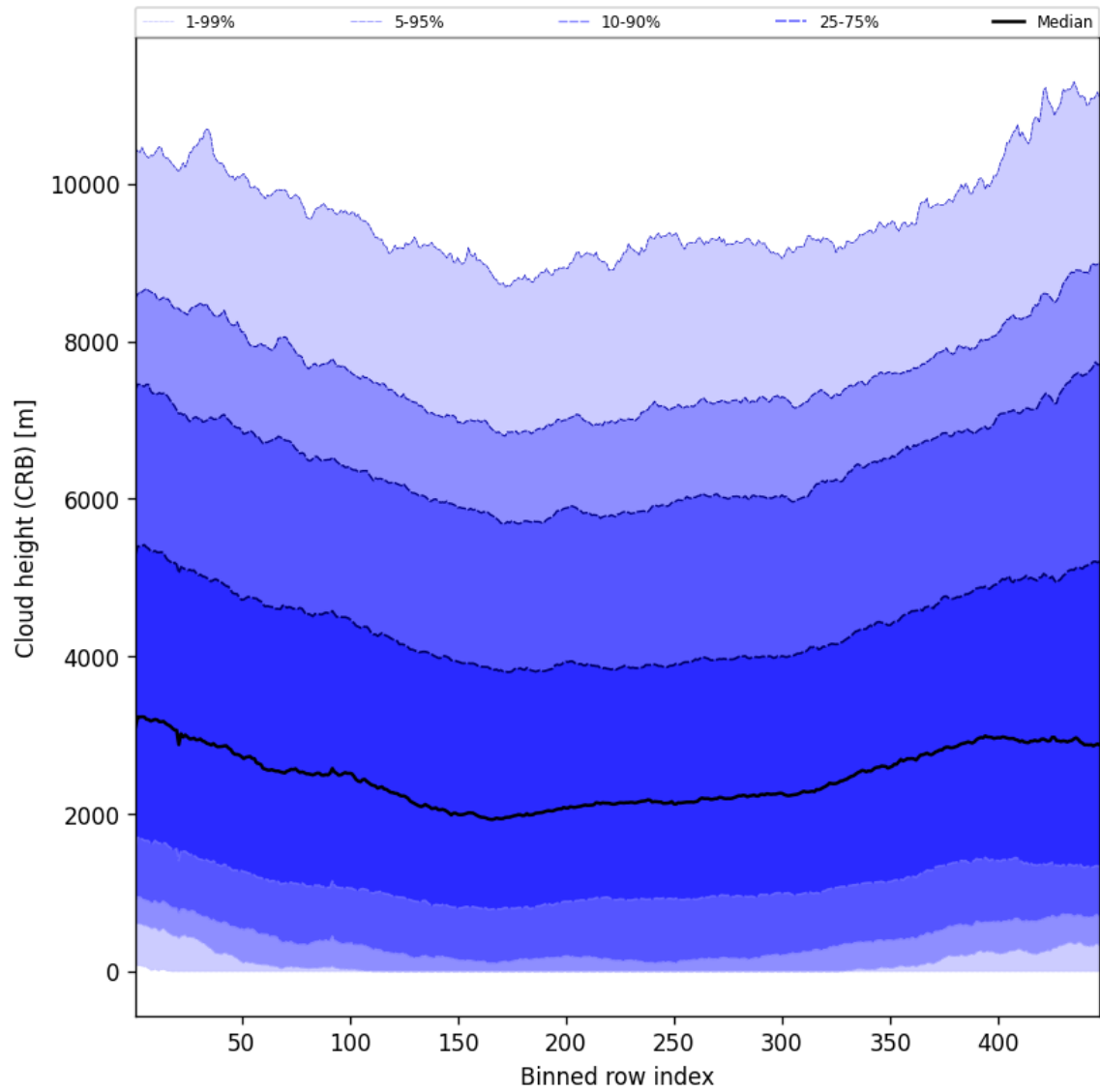
Figure 59: Along track statistics of “Cloud height (CRB)” for 2025-05-31 to 2025-06-01
