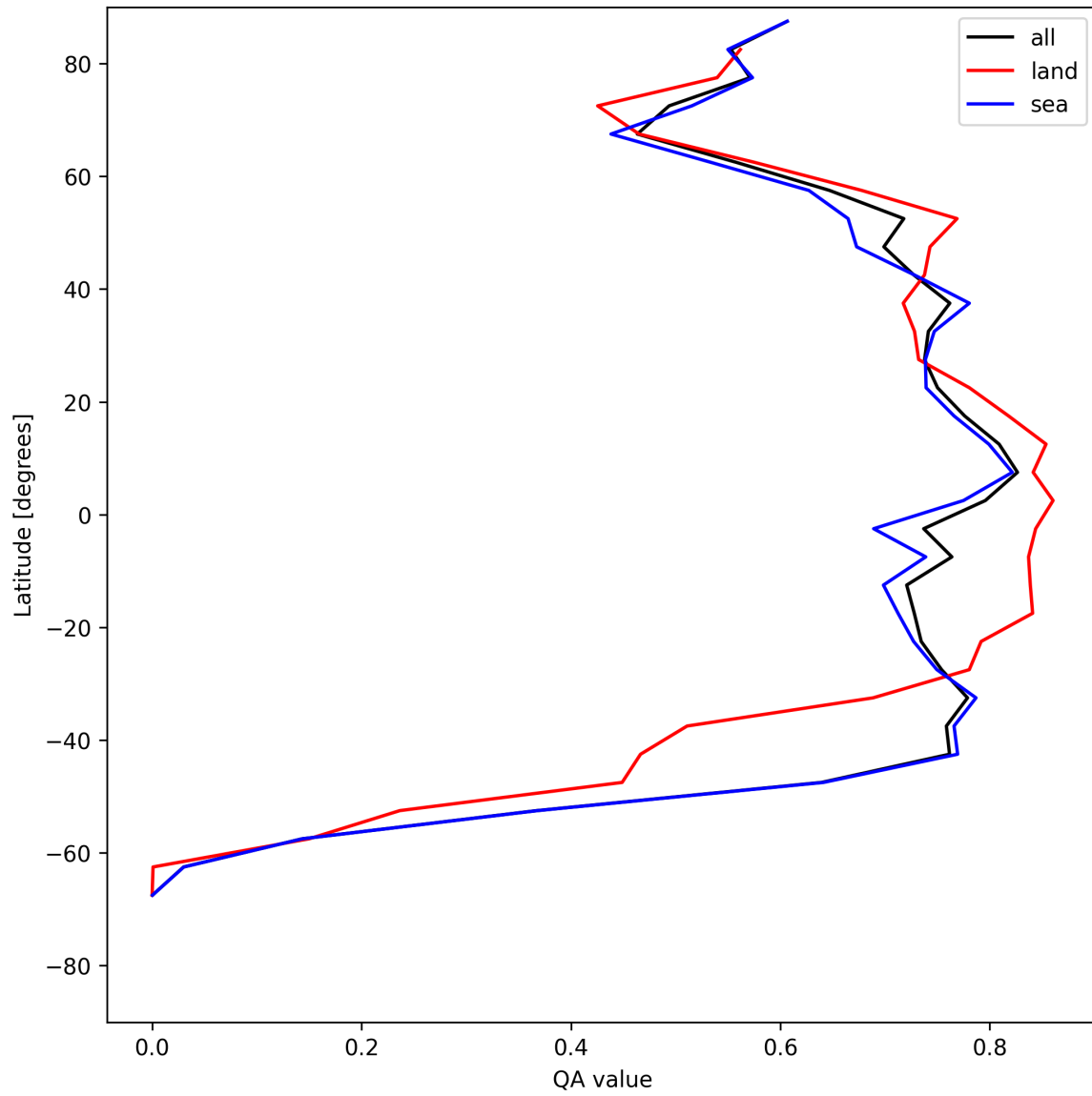
Figure 22: Zonal average of “QA value” for 2025-05-31 to 2025-06-01.
