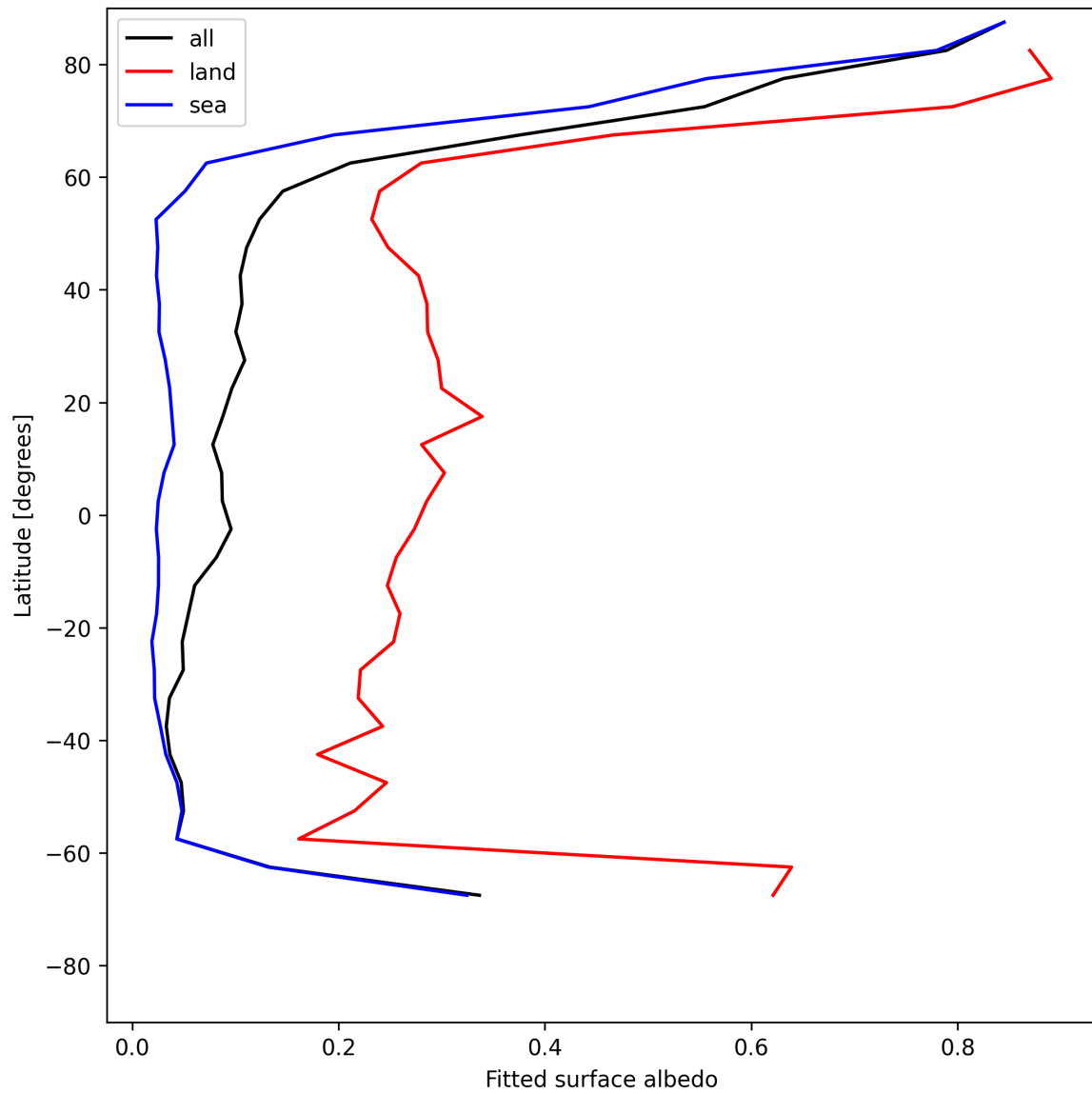
Figure 29: Zonal average of “Fitted surface albedo” for 2025-05-31 to 2025-06-01.
