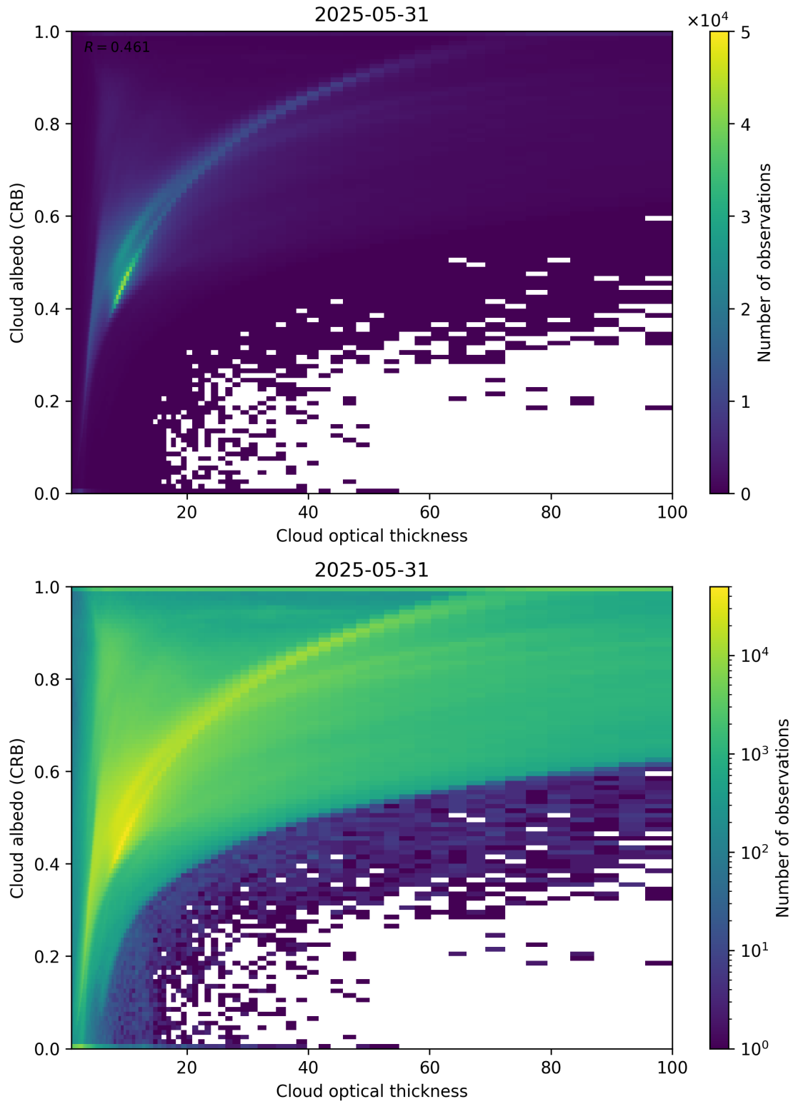
Figure 82: Scatter density plot of “Cloud optical thickness” against “Cloud albedo (CRB)” for 2025-05-31 to 2025-06-01.
