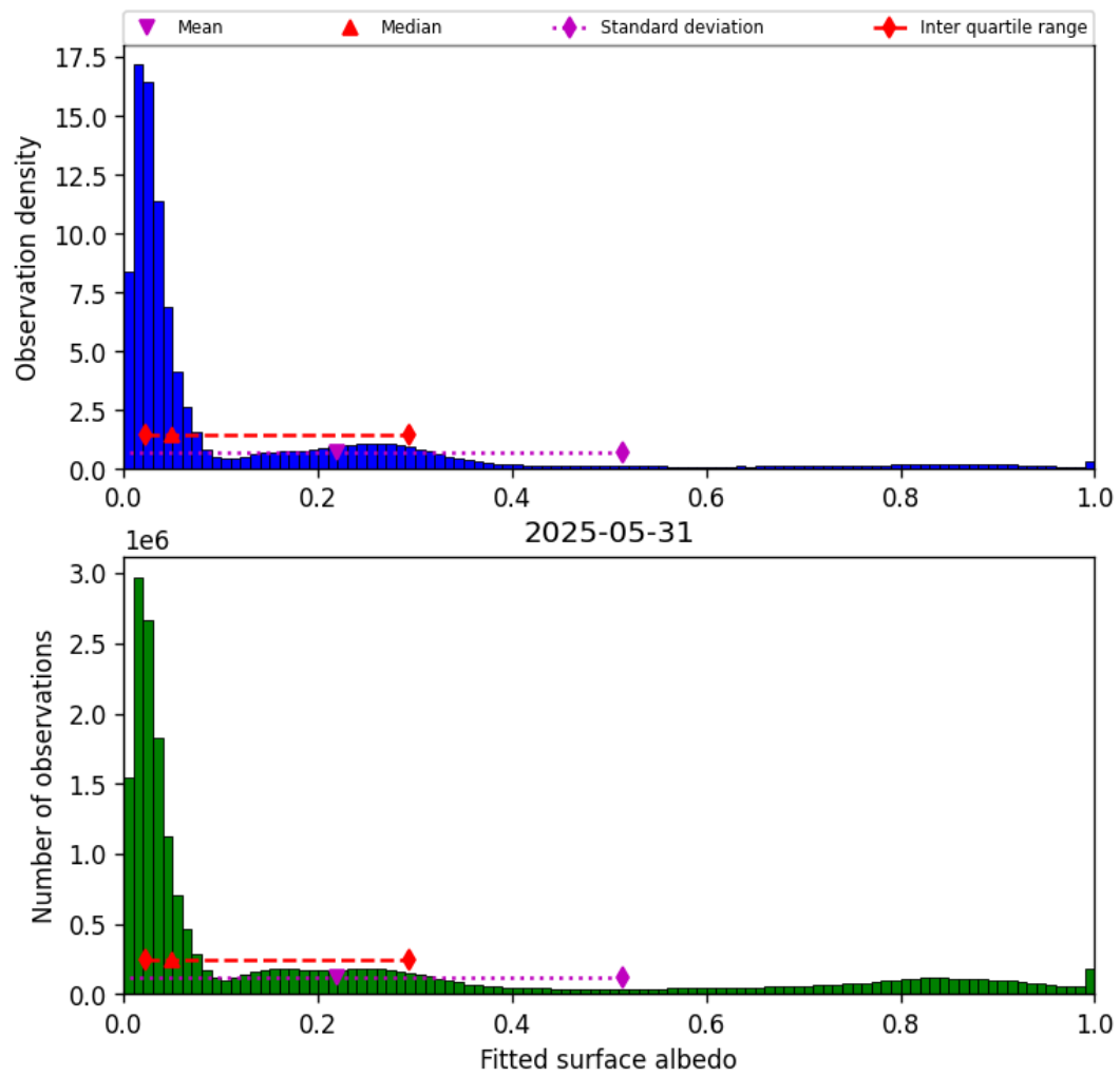
Figure 45: Histogram of “Fitted surface albedo” for 2025-05-31 to 2025-06-01
