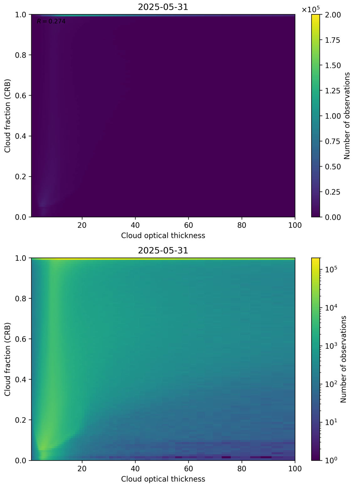
Figure 84: Scatter density plot of “Cloud optical thickness” against “Cloud fraction (CRB)” for 2025-05-31 to 2025-06-01.
