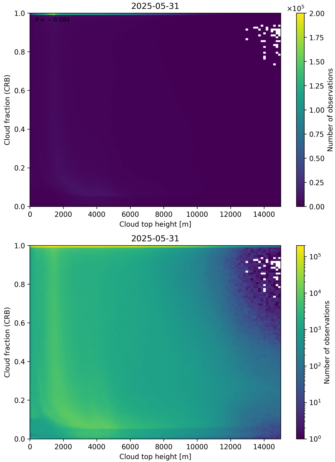
Figure 88: Scatter density plot of “Cloud top height” against “Cloud fraction (CRB)” for 2025-05-31 to 2025-06-01.
