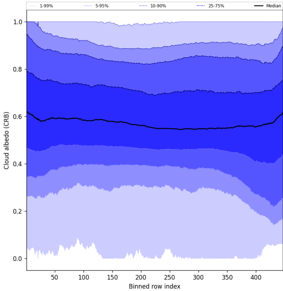
Figure 60: Along track statistics of “Cloud albedo (CRB)” for 2025-05-31 to 2025-06-01
