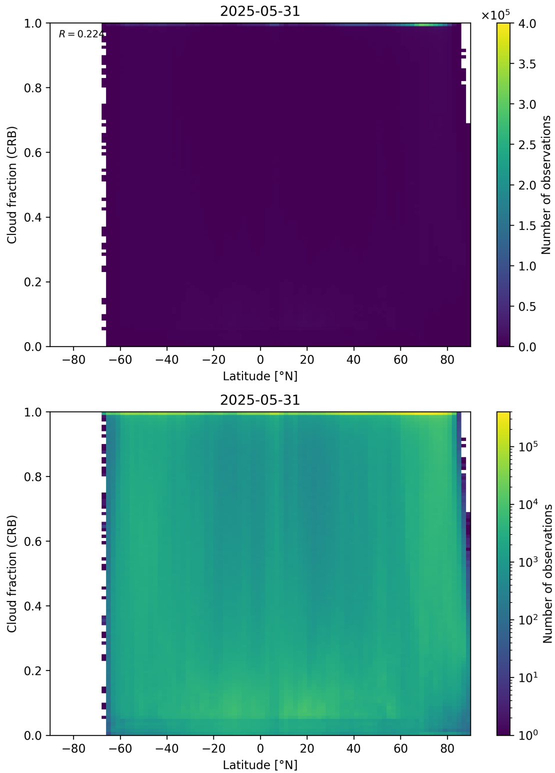
Figure 94: Scatter density plot of “Latitude” against “Cloud fraction (CRB)” for 2025-05-31 to 2025-06-01.
