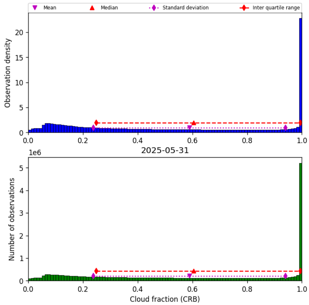
Figure 42: Histogram of “Cloud fraction (CRB)” for 2025-05-31 to 2025-06-01
