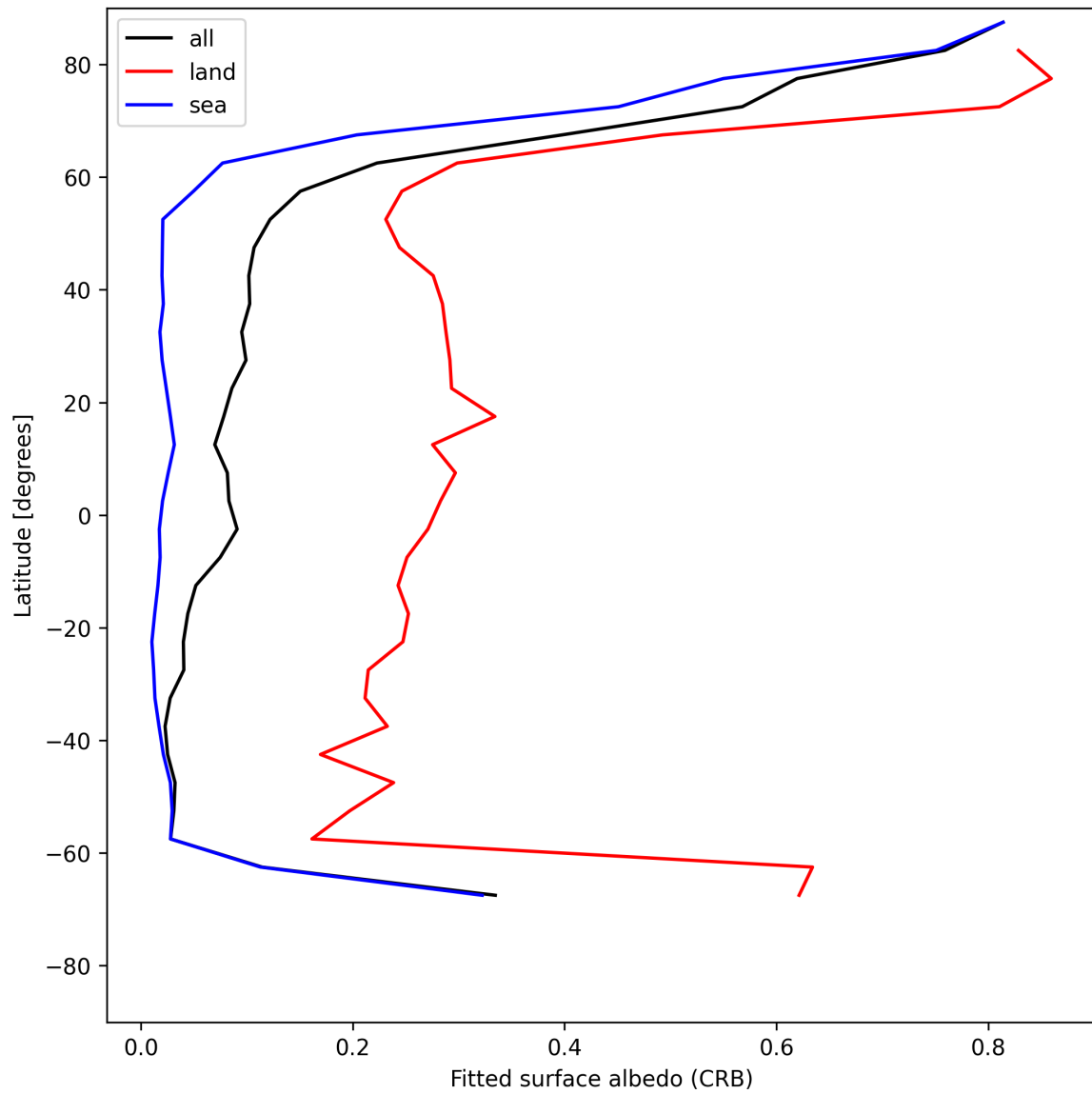
Figure 30: Zonal average of “Fitted surface albedo (CRB)” for 2025-05-31 to 2025-06-01.
