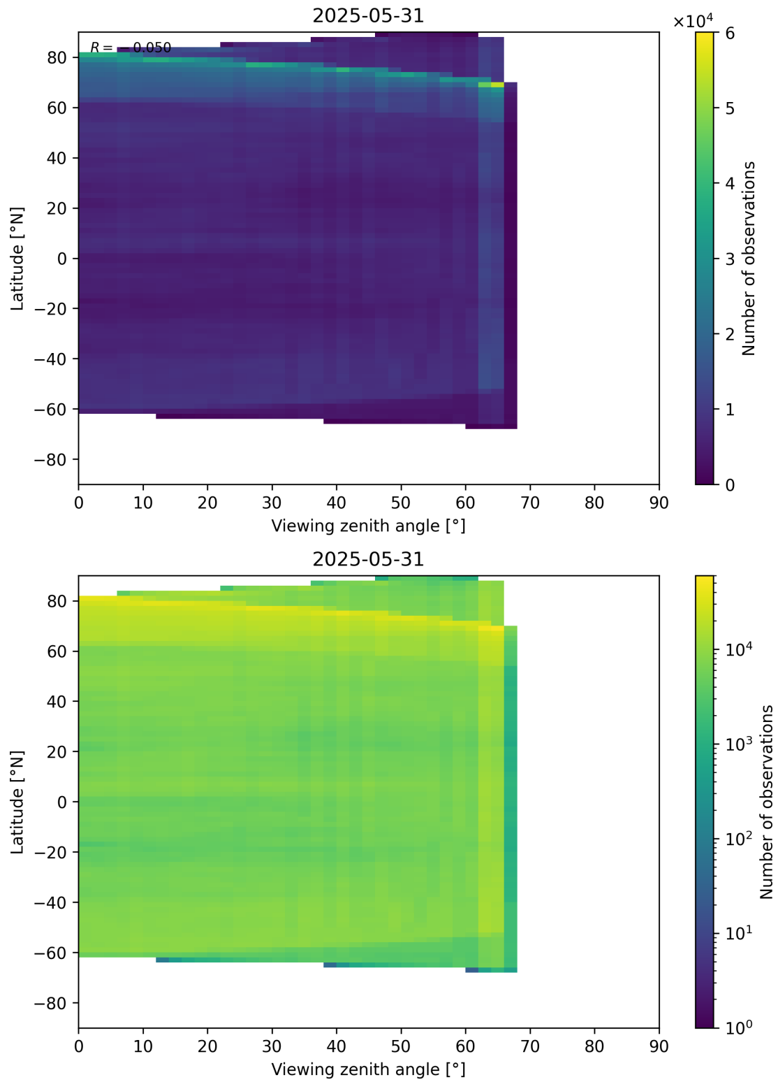
Figure 113: Scatter density plot of “Viewing zenith angle” against “Latitude” for 2025-05-31 to 2025-06-01.
