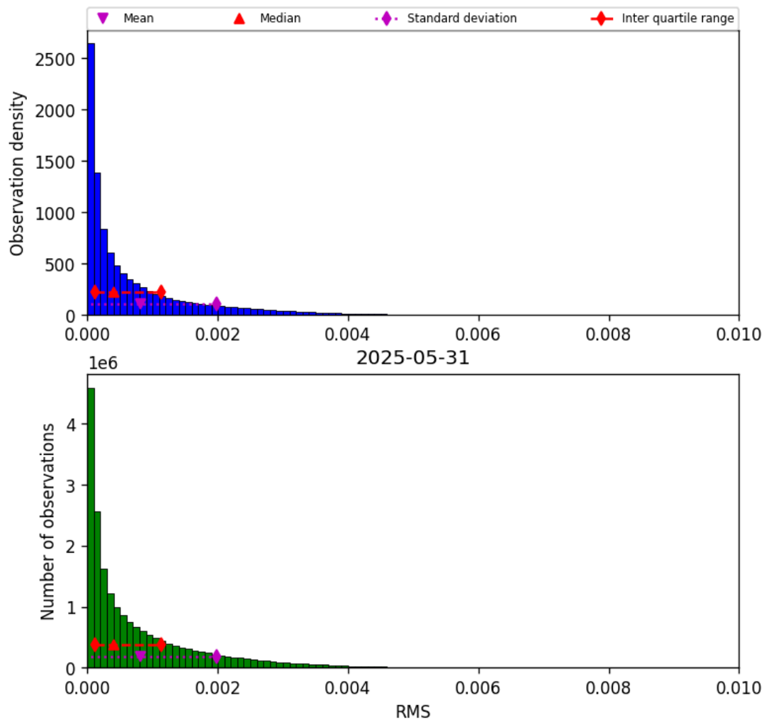
Figure 47: Histogram of “RMS” for 2025-05-31 to 2025-06-01
