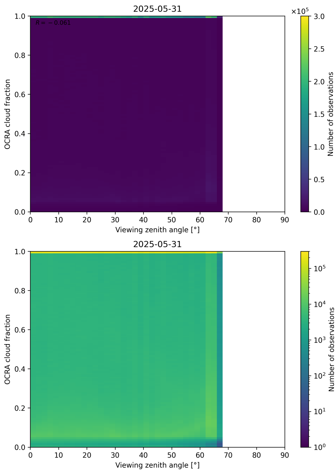
Figure 108: Scatter density plot of “Viewing zenith angle” against “OCRA cloud fraction” for 2025-05-31 to 2025-06-01.
