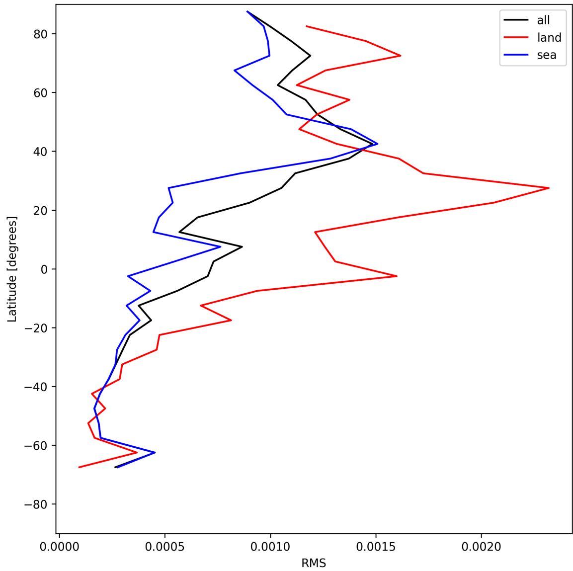
Figure 31: Zonal average of “RMS” for 2025-05-31 to 2025-06-01.
