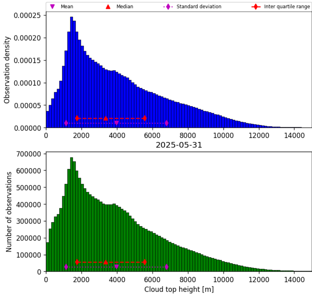
Figure 40: Histogram of “Cloud top height” for 2025-05-31 to 2025-06-01
