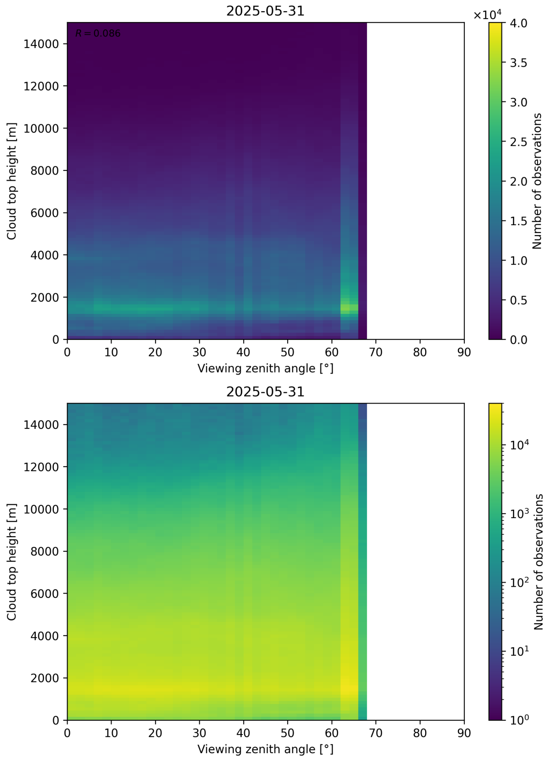
Figure 112: Scatter density plot of “Viewing zenith angle” against “Cloud top height” for 2025-05-31 to 2025-06-01.
