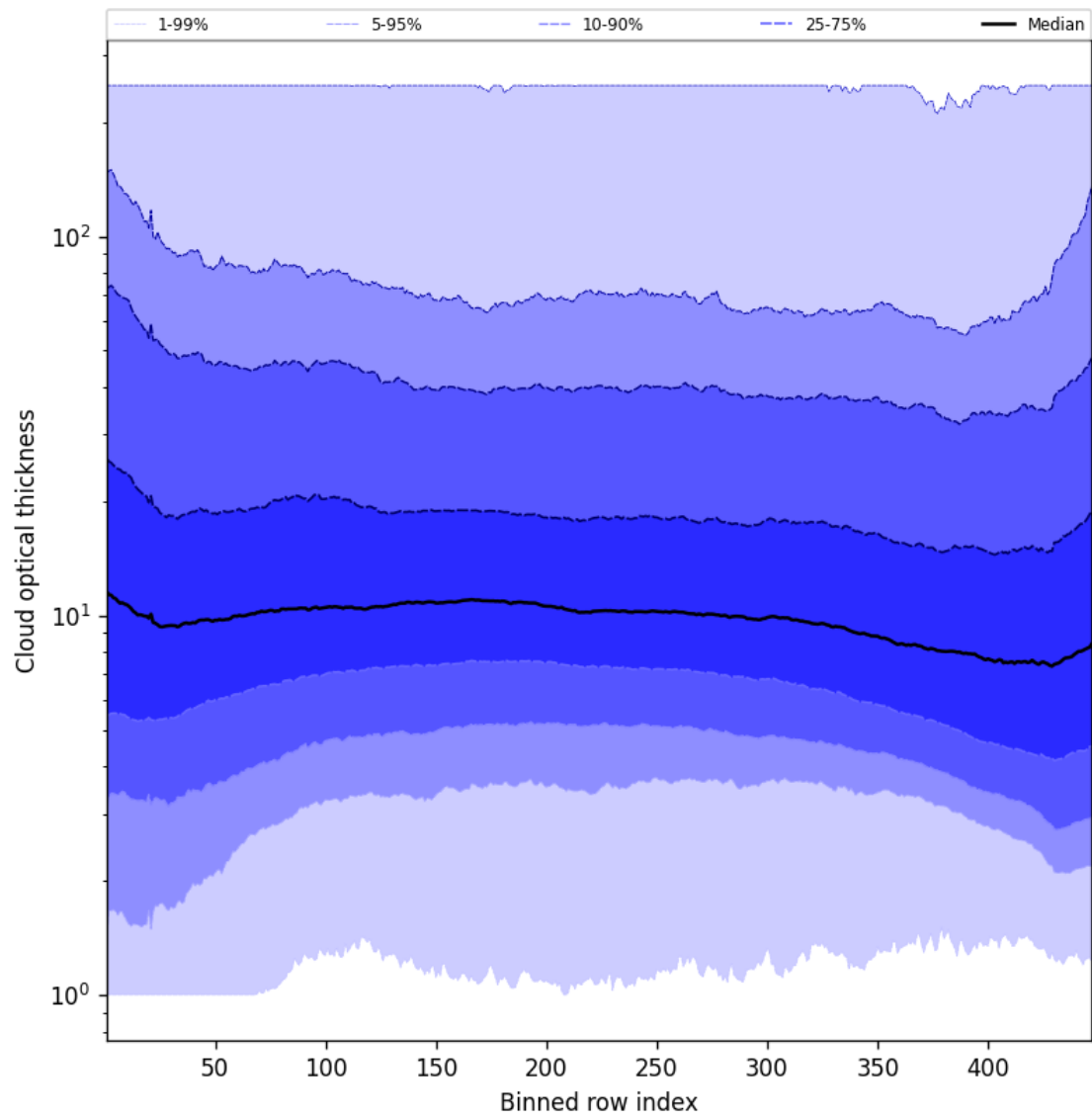
Figure 57: Along track statistics of “Cloud optical thickness” for 2025-05-31 to 2025-06-01
