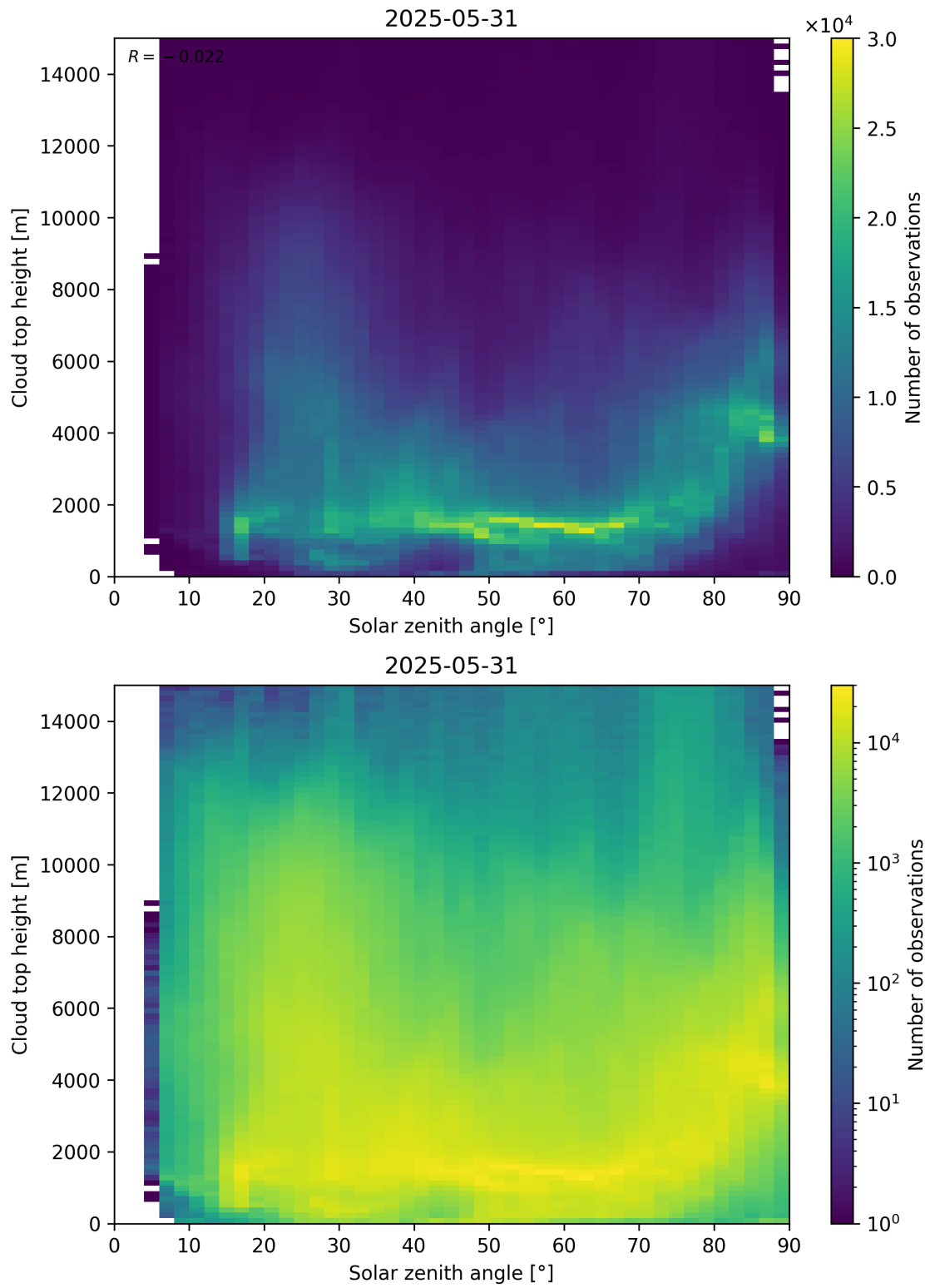
Figure 104: Scatter density plot of “Solar zenith angle” against “Cloud top height” for 2025-05-31 to 2025-06-01.
