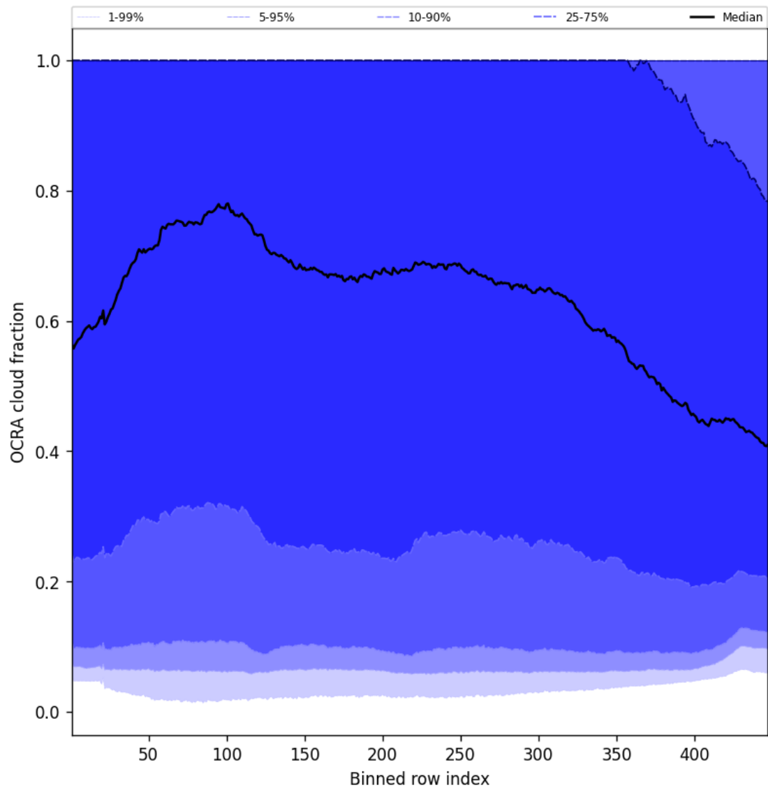
Figure 66: Along track statistics of “OCRA cloud fraction” for 2025-05-31 to 2025-06-01
