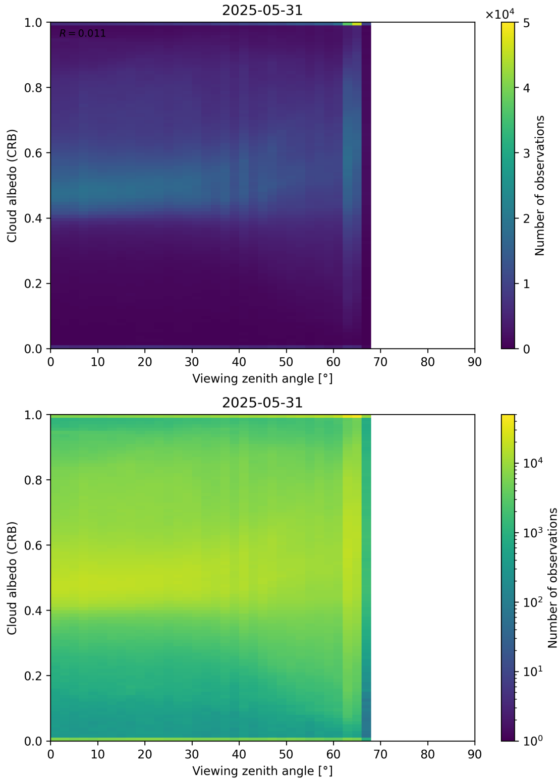
Figure 106: Scatter density plot of “Viewing zenith angle” against “Cloud albedo (CRB)” for 2025-05-31 to 2025-06-01.
