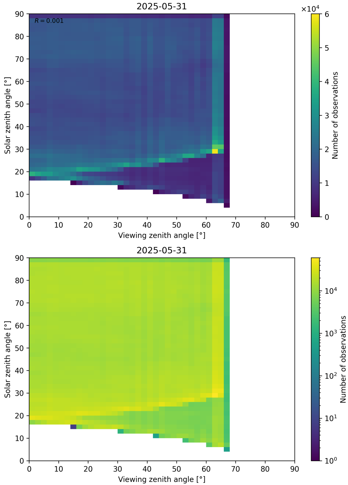
Figure 114: Scatter density plot of “Viewing zenith angle” against “Solar zenith angle” for 2025-05-31 to 2025-06-01.
