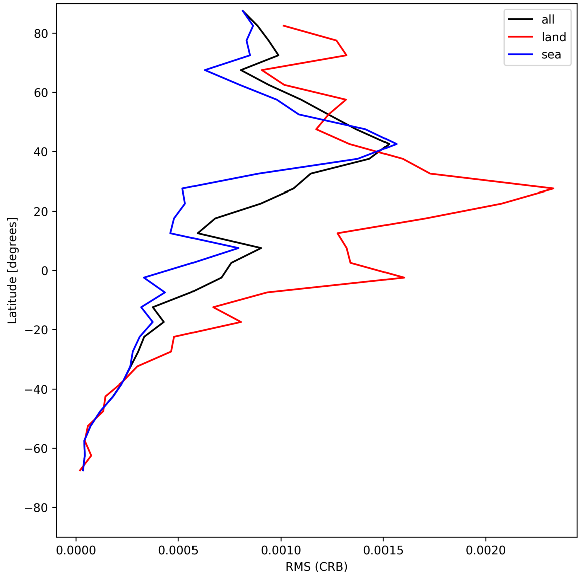
Figure 32: Zonal average of “RMS (CRB)” for 2025-05-31 to 2025-06-01.
