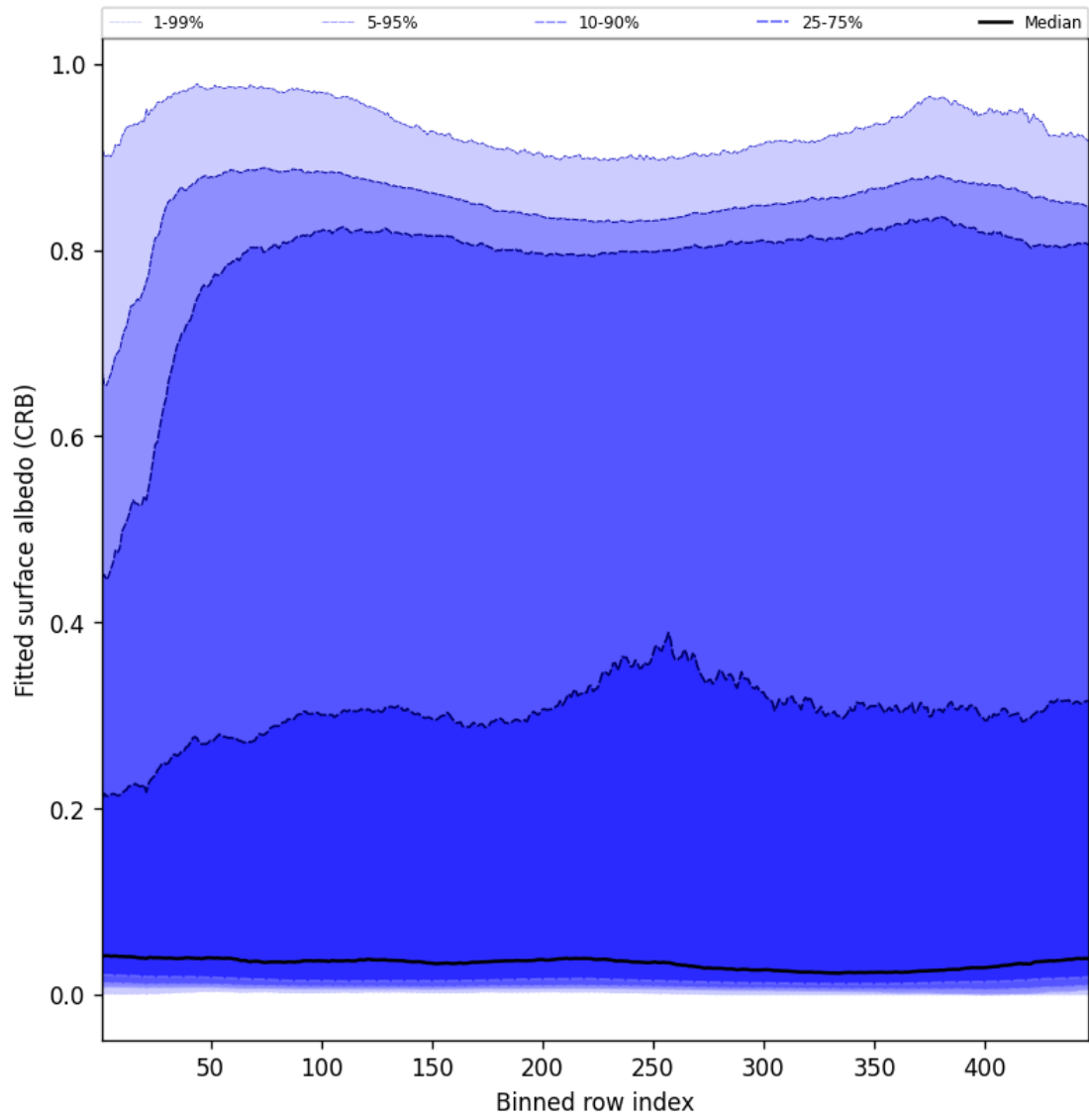
Figure 62: Along track statistics of “Fitted surface albedo (CRB)” for 2025-05-31 to 2025-06-01
