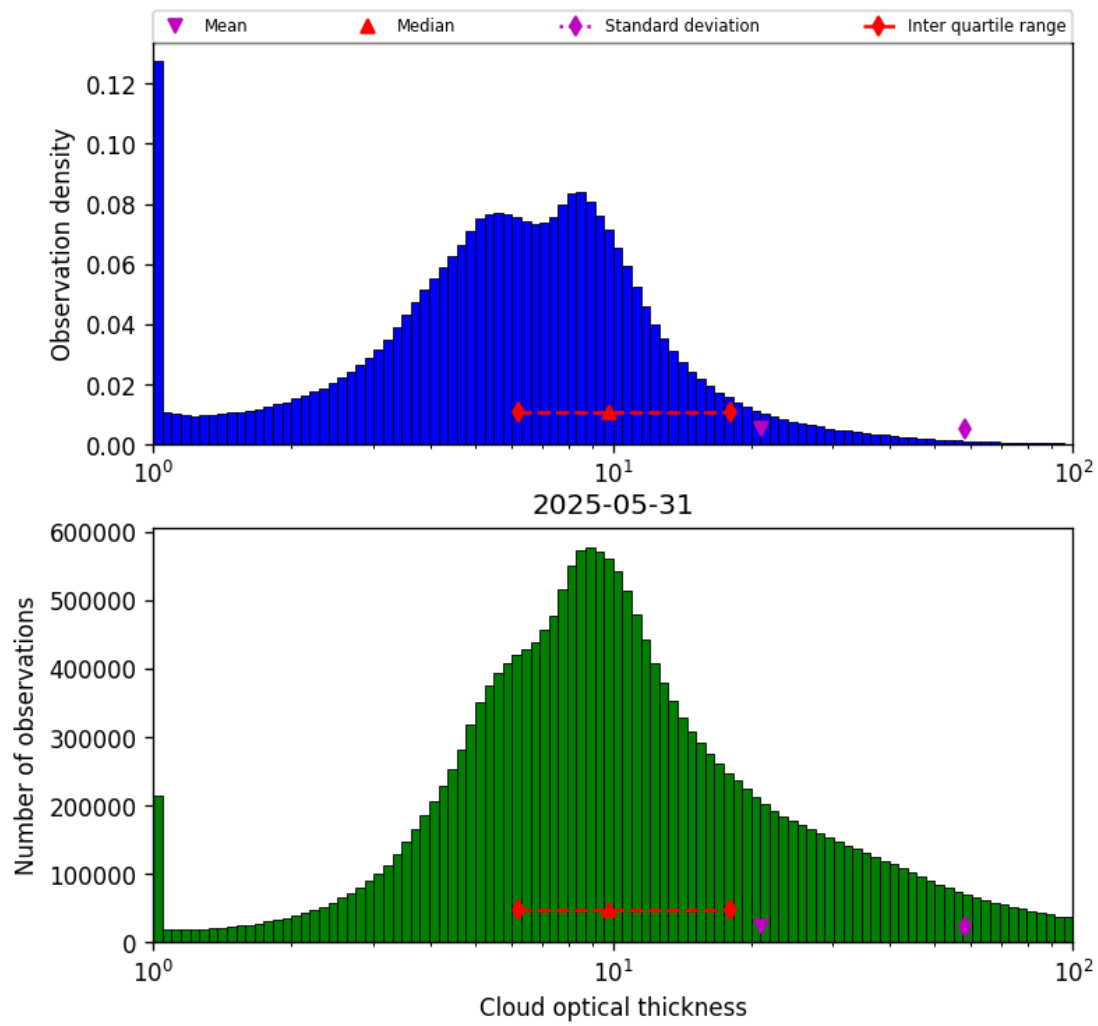
Figure 41: Histogram of “Cloud optical thickness” for 2025-05-31 to 2025-06-01
