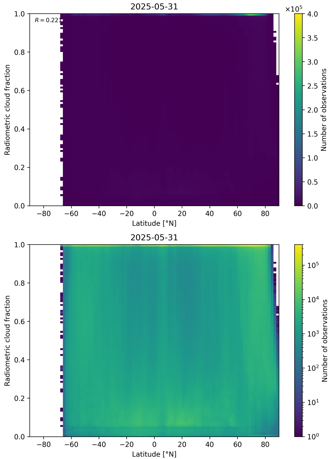
Figure 92: Scatter density plot of “Latitude” against “Radiometric cloud fraction” for 2025-05-31 to 2025-06-01.
