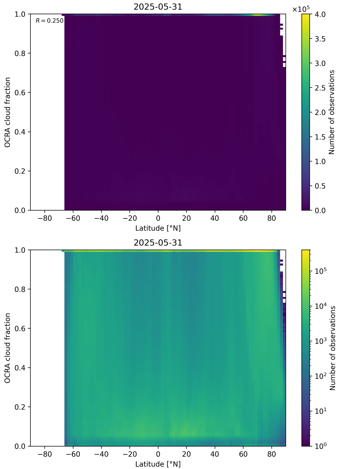
Figure 93: Scatter density plot of “Latitude” against “OCRA cloud fraction” for 2025-05-31 to 2025-06-01.
