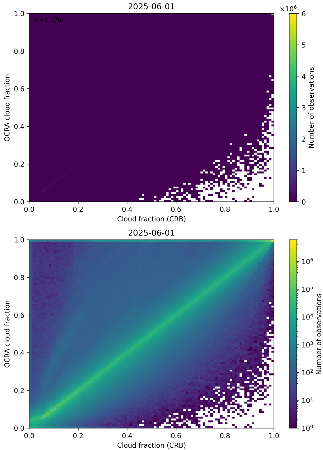
Figure 78: Scatter density plot of “Cloud fraction (CRB)” against “OCRA cloud fraction” for 2025-06-01 to 2025-06-02.
