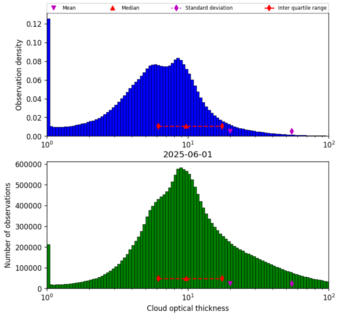
Figure 41: Histogram of “Cloud optical thickness” for 2025-06-01 to 2025-06-02
