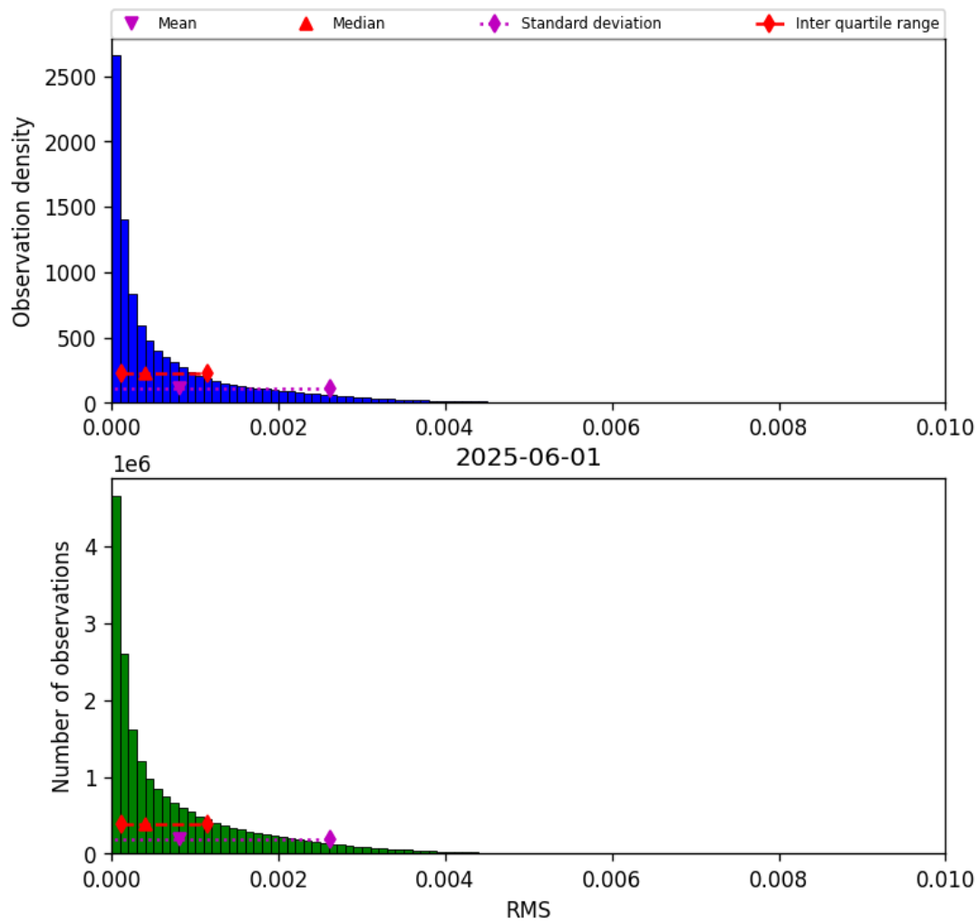
Figure 47: Histogram of “RMS” for 2025-06-01 to 2025-06-02
