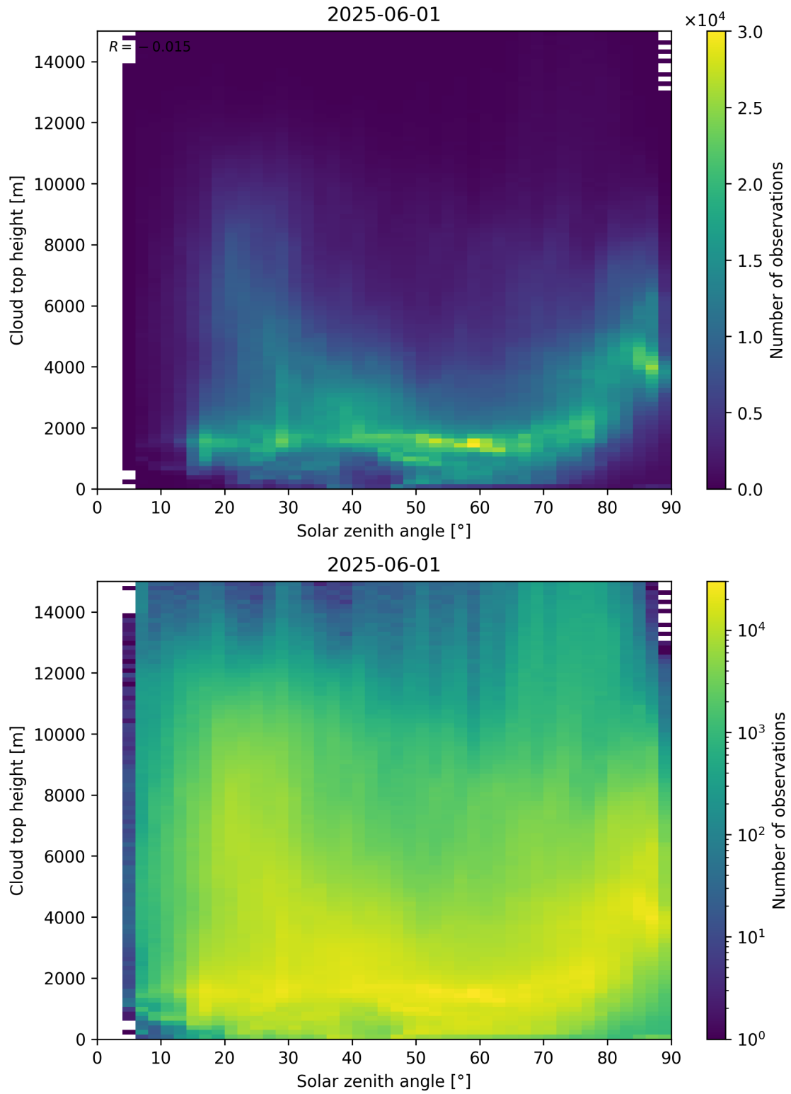
Figure 104: Scatter density plot of “Solar zenith angle” against “Cloud top height” for 2025-06-01 to 2025-06-02.
