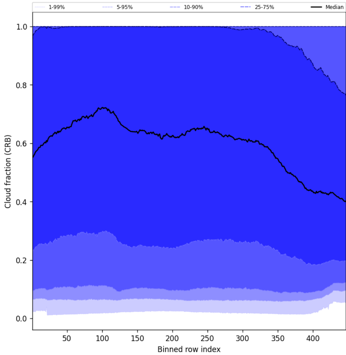
Figure 58: Along track statistics of “Cloud fraction (CRB)” for 2025-06-01 to 2025-06-02
