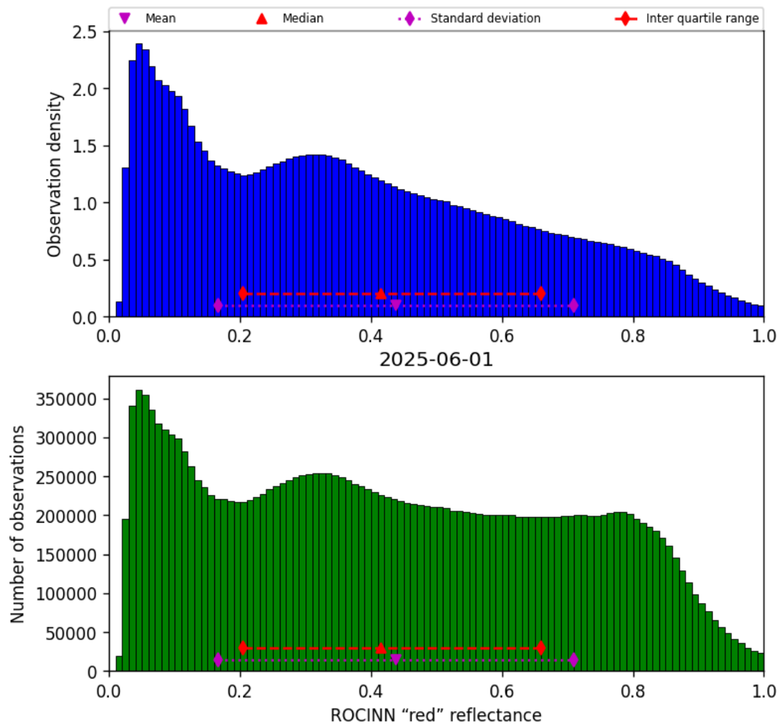
Figure 53: Histogram of “ROCINN “red” reflectance” for 2025-06-01 to 2025-06-02
