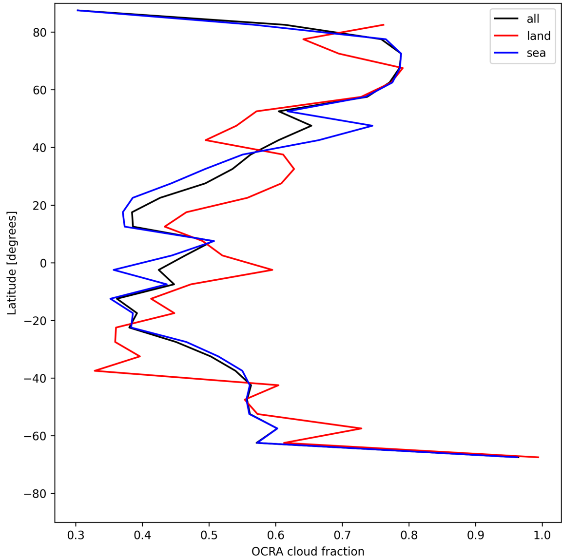
Figure 34: Zonal average of “OCRA cloud fraction” for 2025-06-01 to 2025-06-02.
