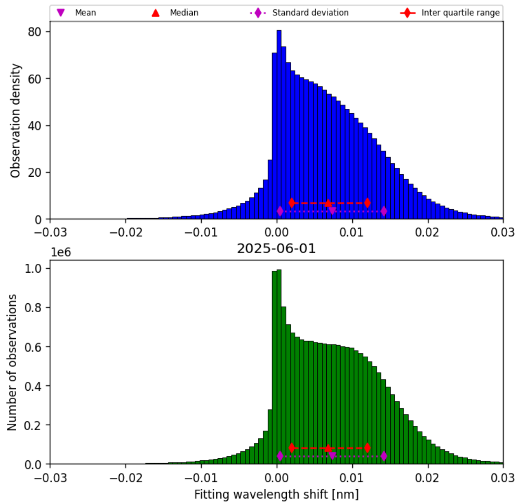
Figure 49: Histogram of “Fitting wavelength shift” for 2025-06-01 to 2025-06-02
