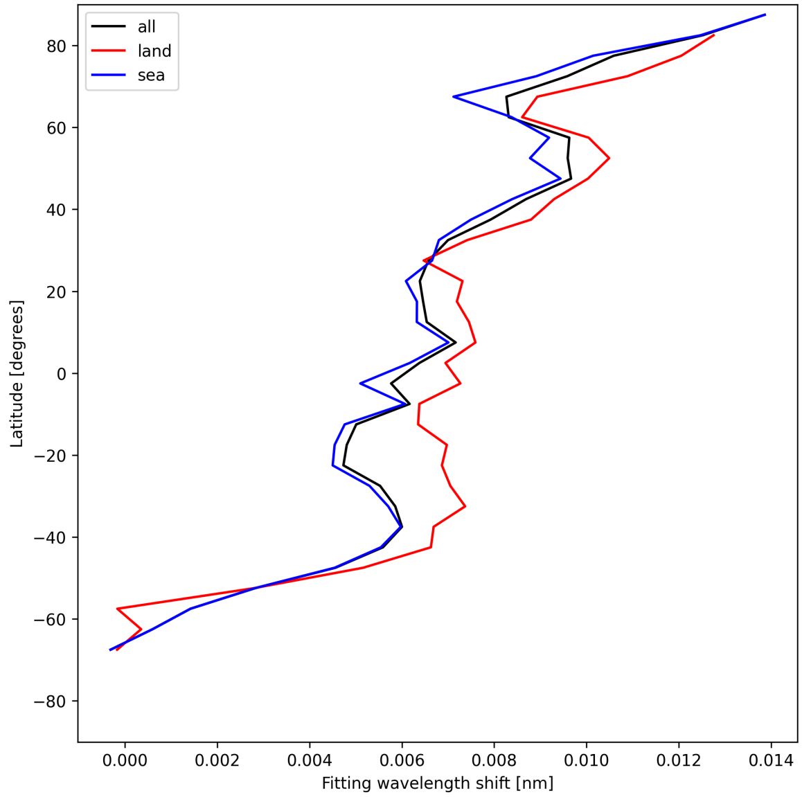
Figure 33: Zonal average of “Fitting wavelength shift” for 2025-06-01 to 2025-06-02.
