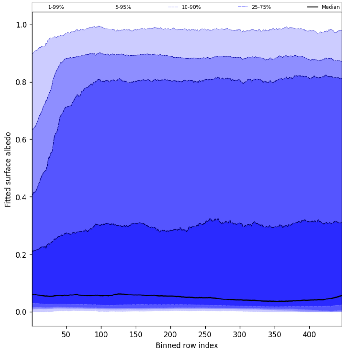
Figure 61: Along track statistics of “Fitted surface albedo” for 2025-06-01 to 2025-06-02
