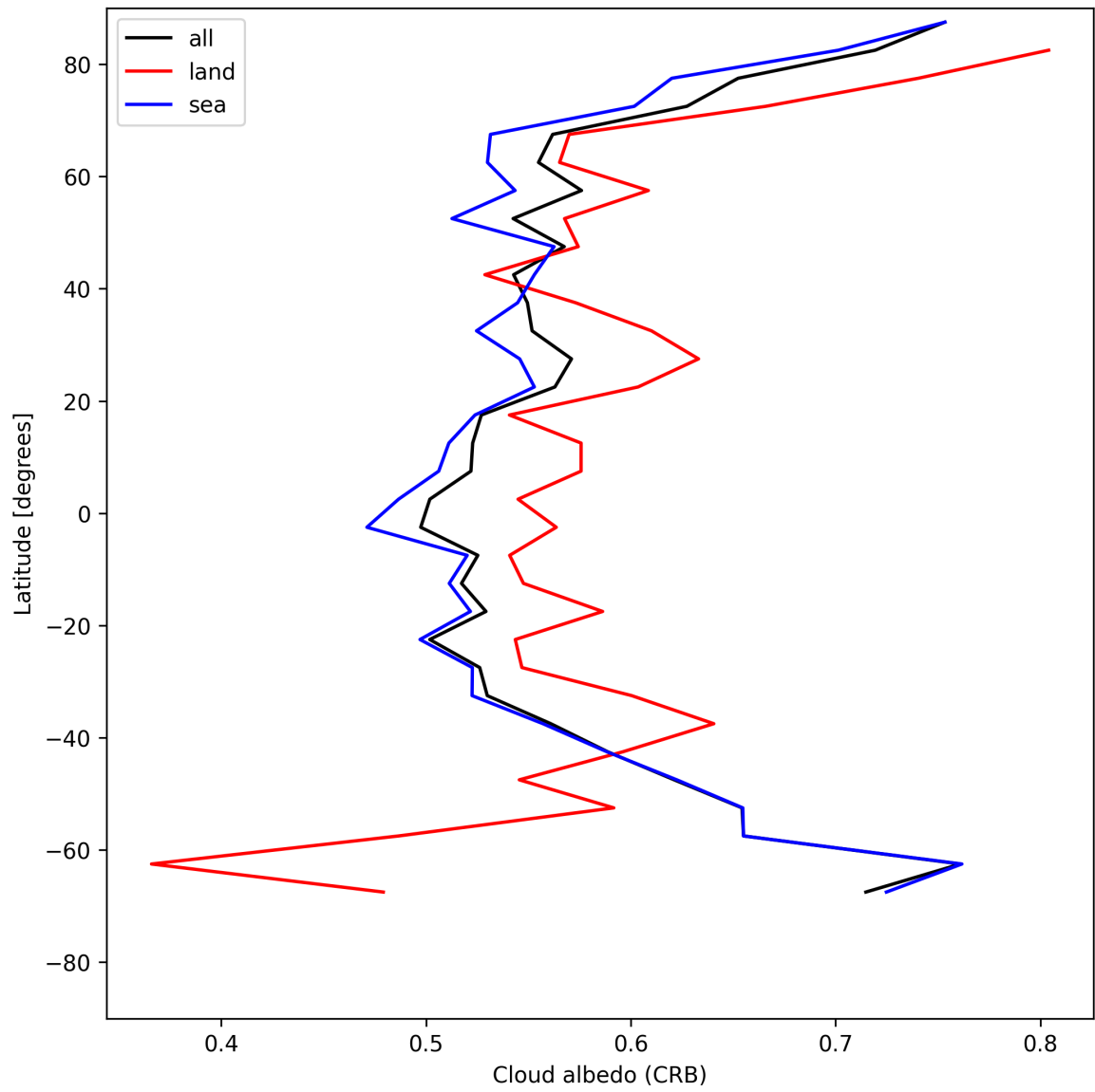
Figure 28: Zonal average of “Cloud albedo (CRB)” for 2025-06-01 to 2025-06-02.
