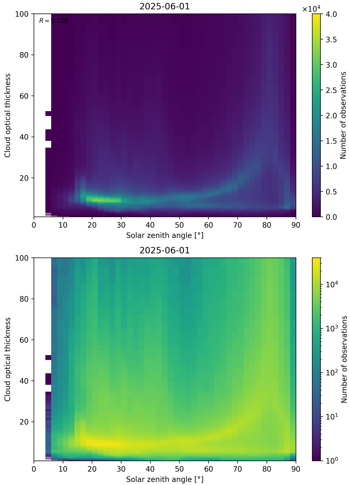
Figure 103: Scatter density plot of “Solar zenith angle” against “Cloud optical thickness” for 2025-06-01 to 2025-06-02.
