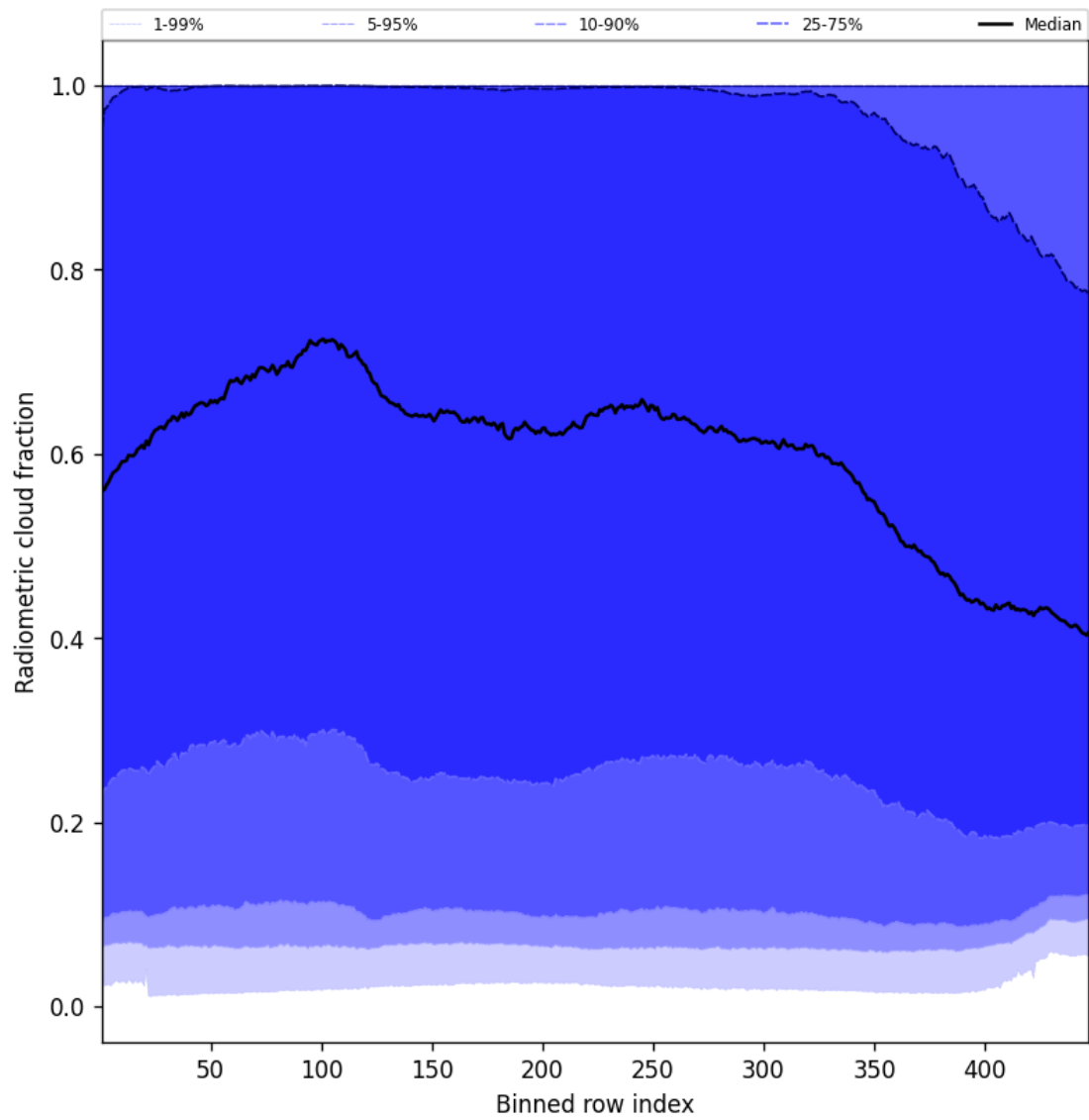
Figure 55: Along track statistics of “Radiometric cloud fraction” for 2025-06-01 to 2025-06-02
