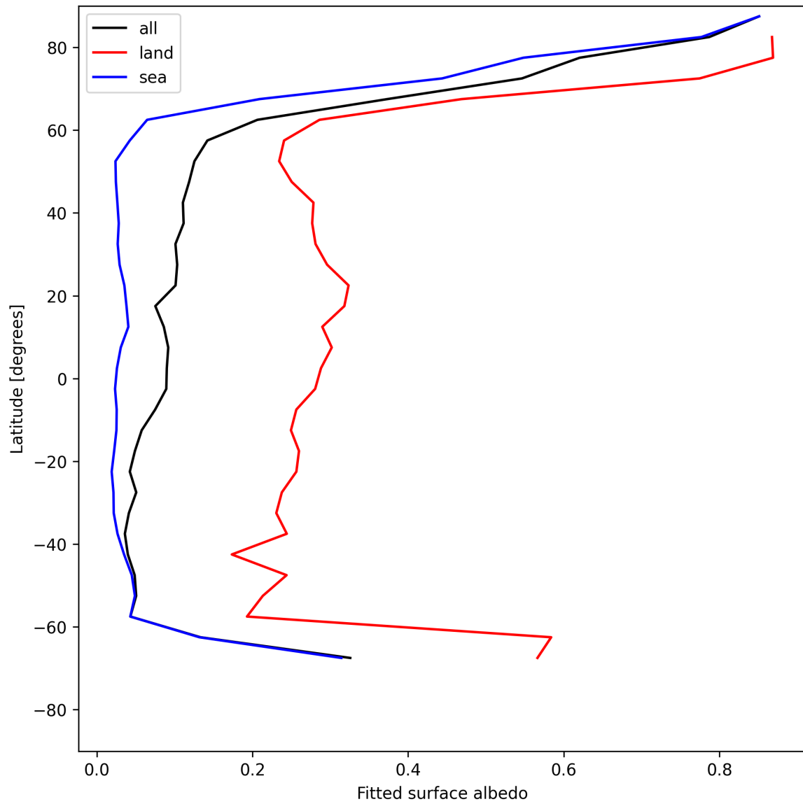
Figure 29: Zonal average of “Fitted surface albedo” for 2025-06-01 to 2025-06-02.
