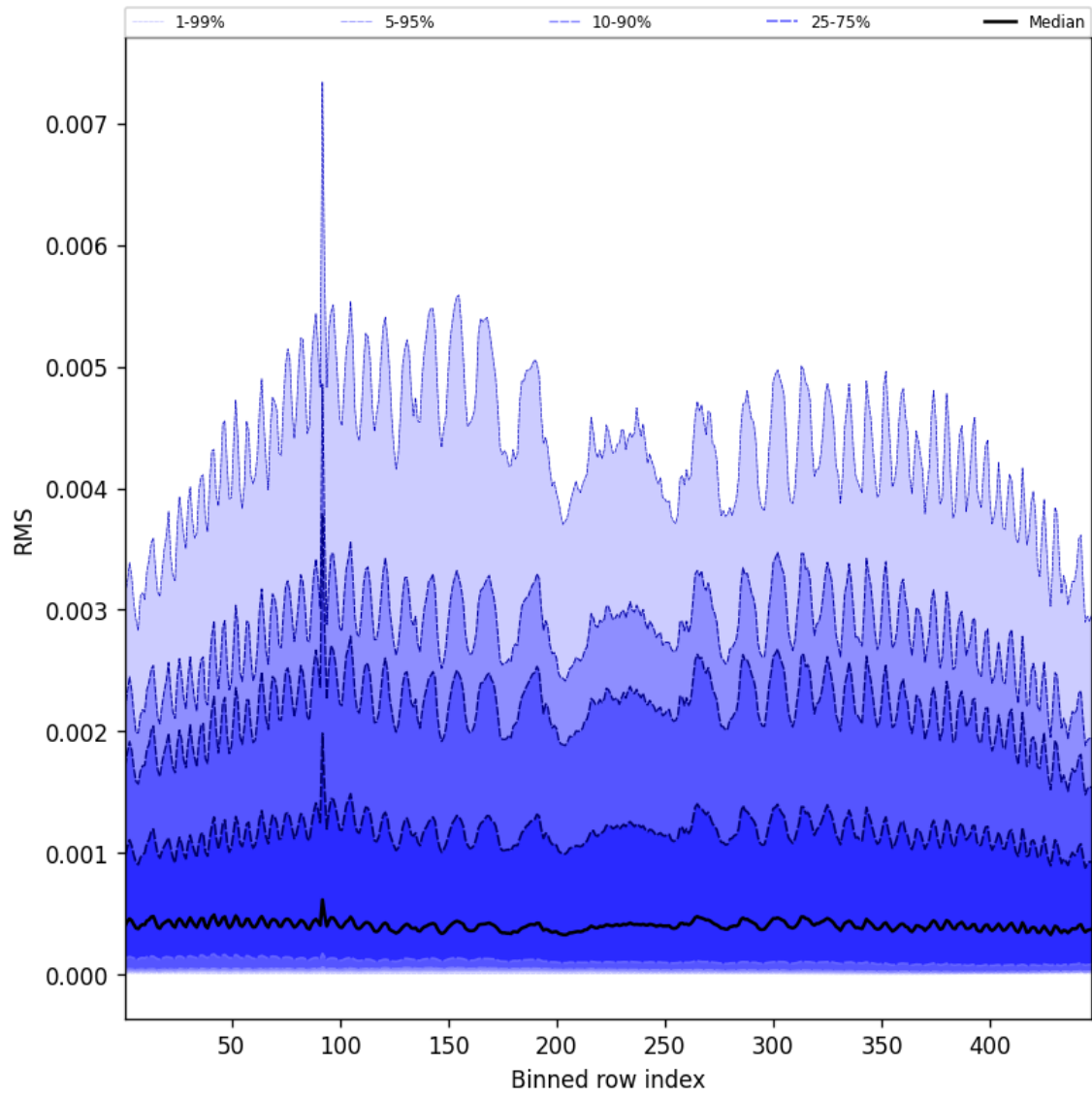
Figure 63: Along track statistics of “RMS” for 2025-06-01 to 2025-06-02
