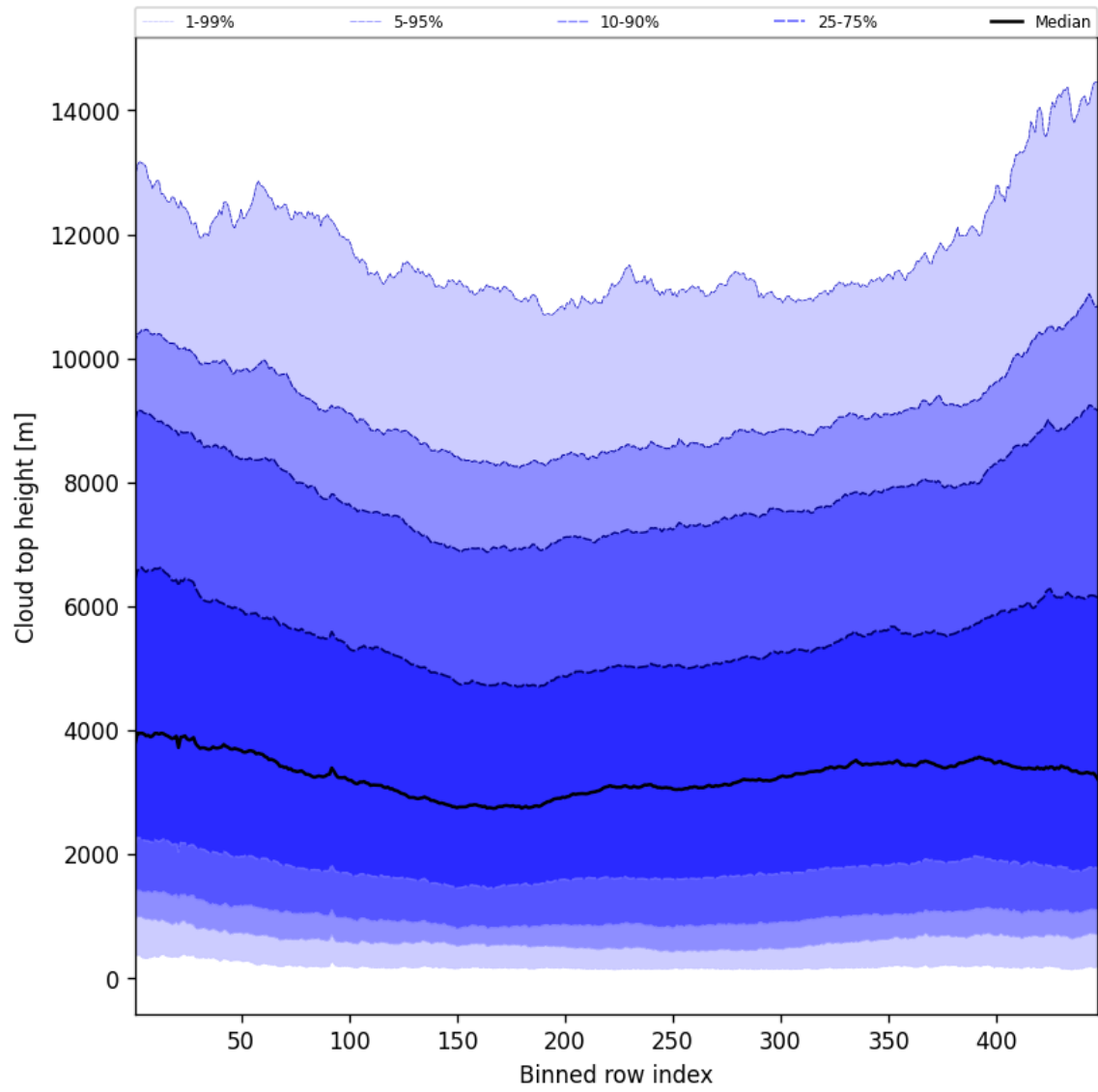
Figure 56: Along track statistics of “Cloud top height” for 2025-06-01 to 2025-06-02
