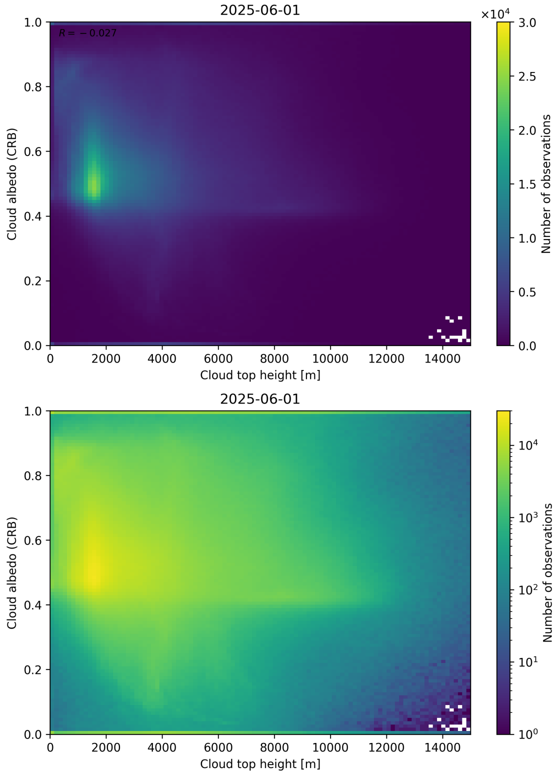
Figure 86: Scatter density plot of “Cloud top height” against “Cloud albedo (CRB)” for 2025-06-01 to 2025-06-02.
