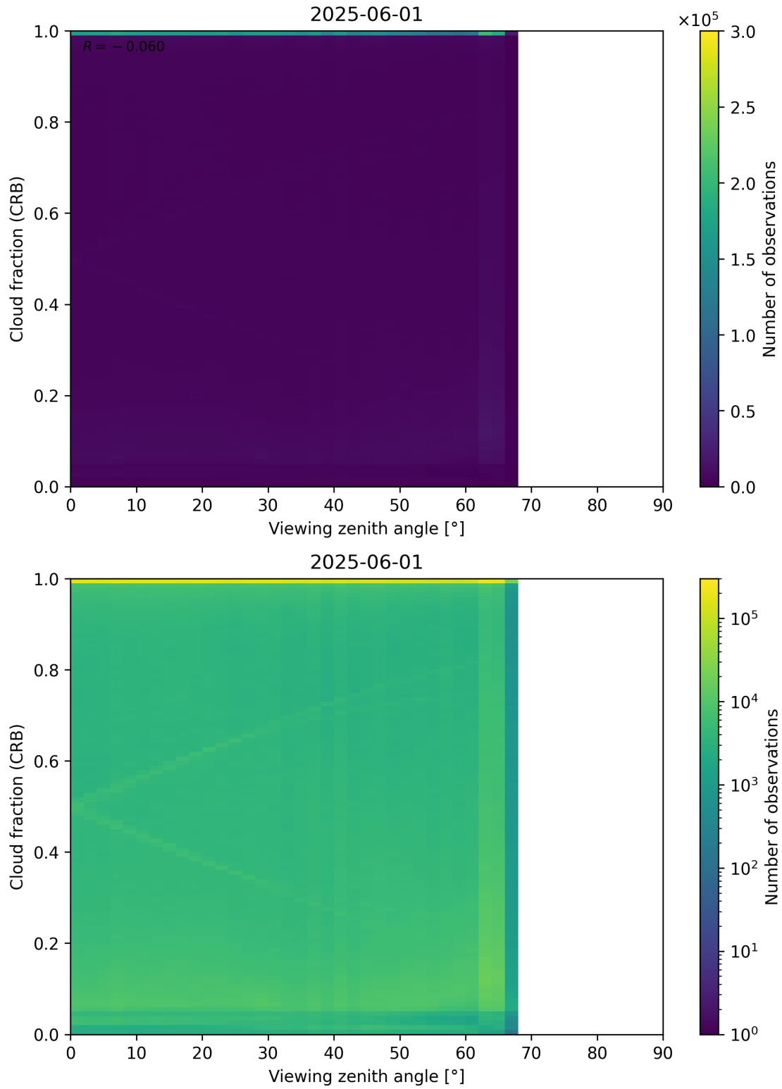
Figure 109: Scatter density plot of “Viewing zenith angle” against “Cloud fraction (CRB)” for 2025-06-01 to 2025-06-02.
