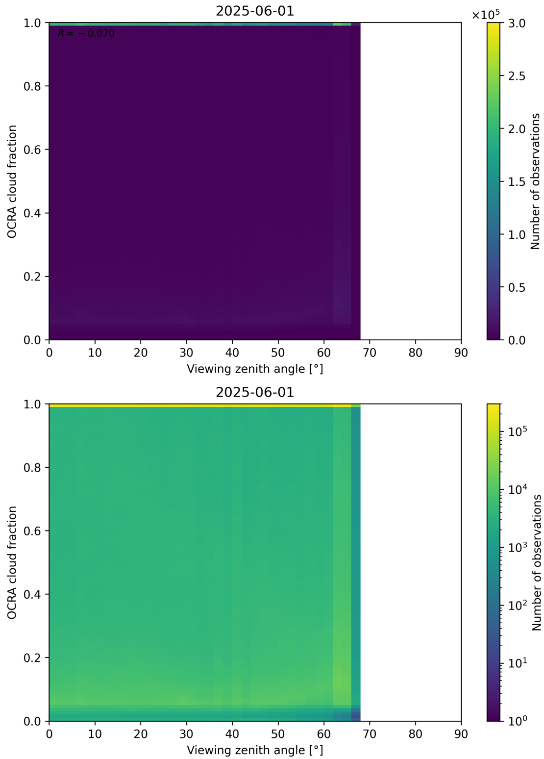
Figure 108: Scatter density plot of “Viewing zenith angle” against “OCRA cloud fraction” for 2025-06-01 to 2025-06-02.
