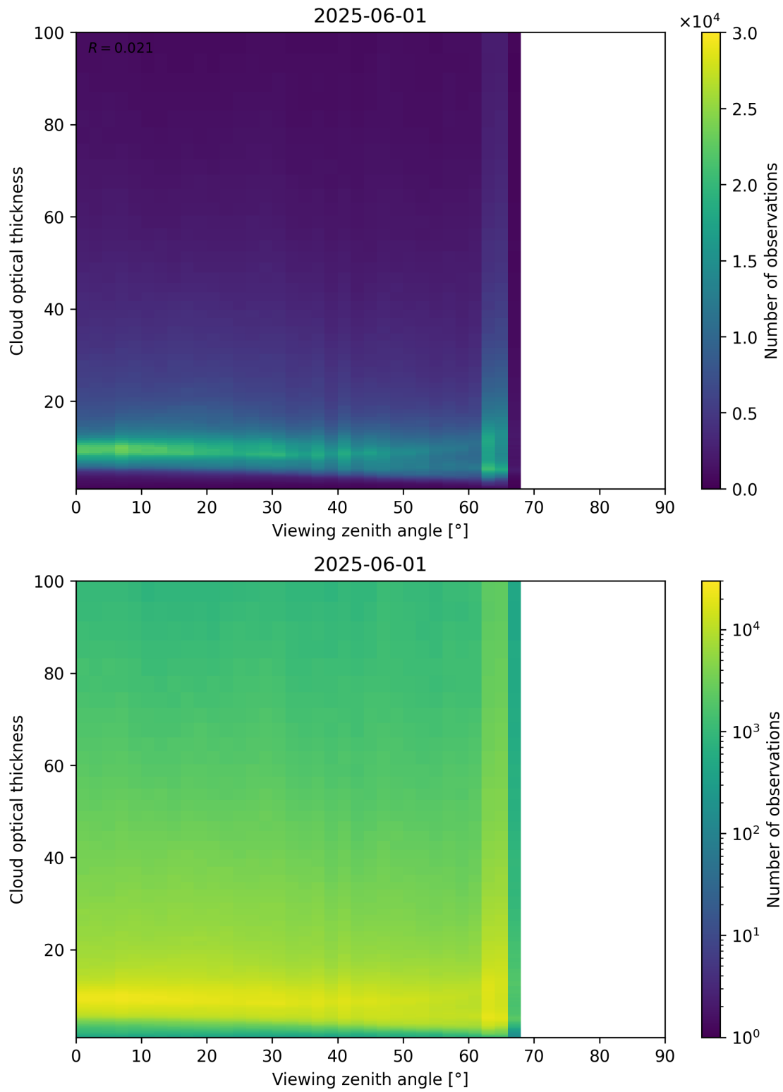
Figure 111: Scatter density plot of “Viewing zenith angle” against “Cloud optical thickness” for 2025-06-01 to 2025-06-02.
