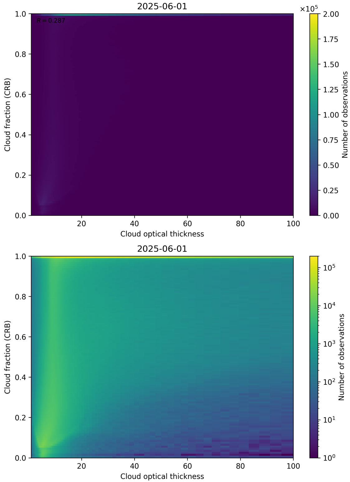
Figure 84: Scatter density plot of “Cloud optical thickness” against “Cloud fraction (CRB)” for 2025-06-01 to 2025-06-02.
