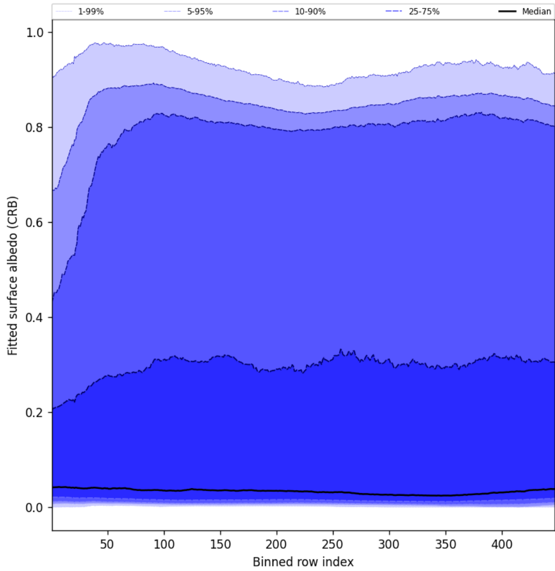
Figure 62: Along track statistics of “Fitted surface albedo (CRB)” for 2025-06-01 to 2025-06-02
