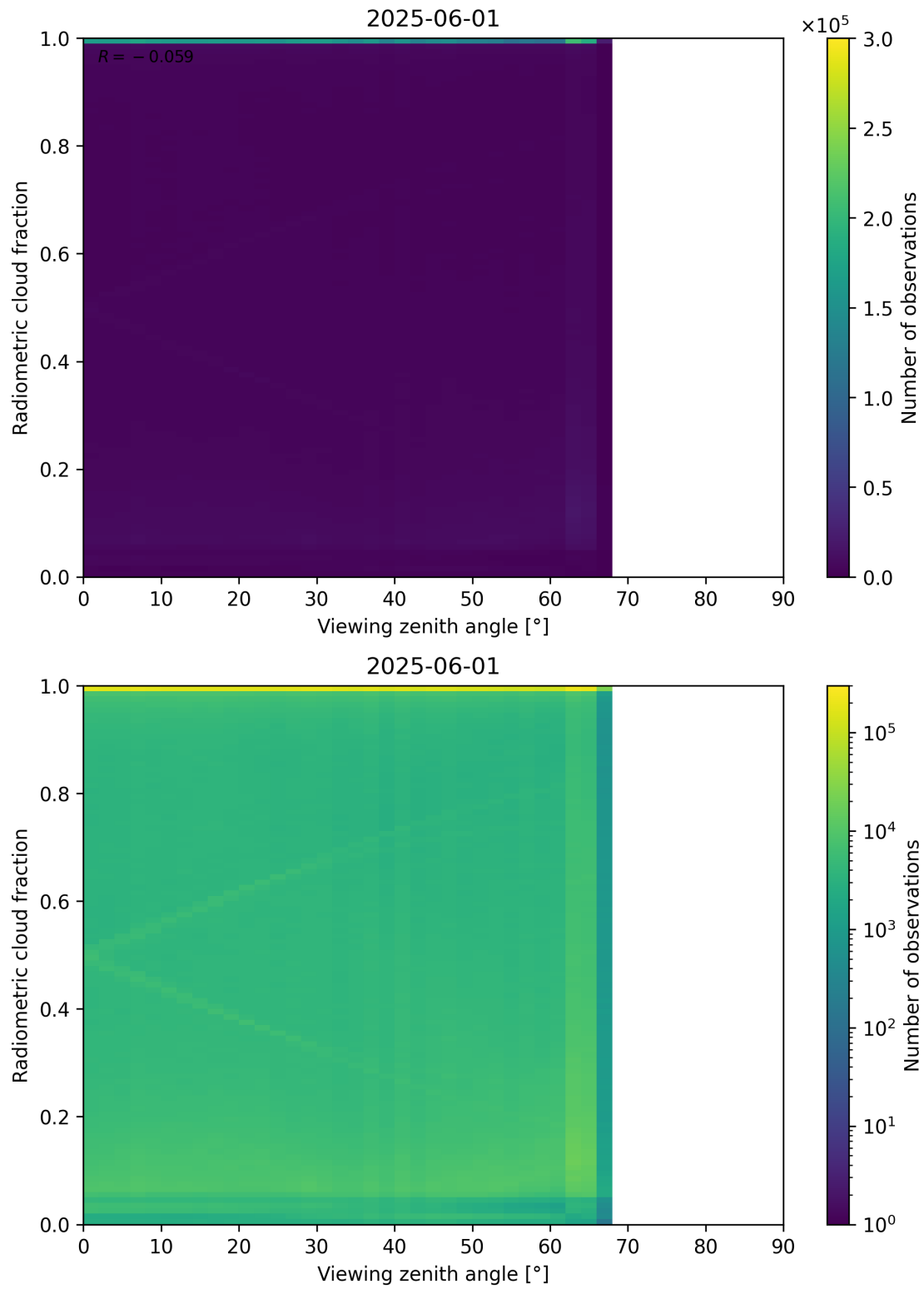
Figure 107: Scatter density plot of “Viewing zenith angle” against “Radiometric cloud fraction” for 2025-06-01 to 2025-06-02.
