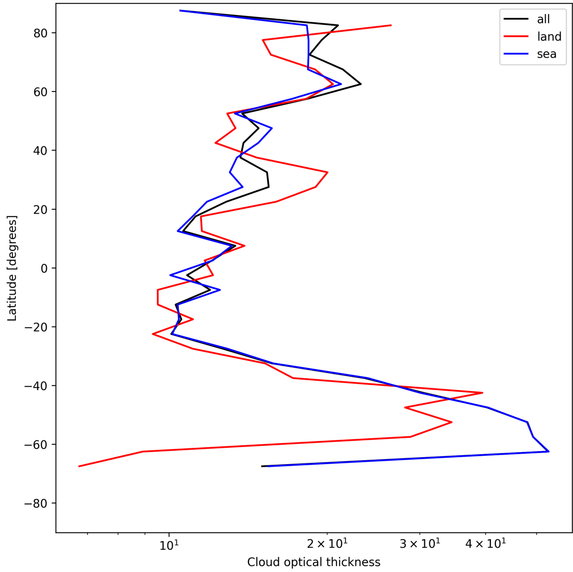
Figure 25: Zonal average of “Cloud optical thickness” for 2025-06-01 to 2025-06-02.
