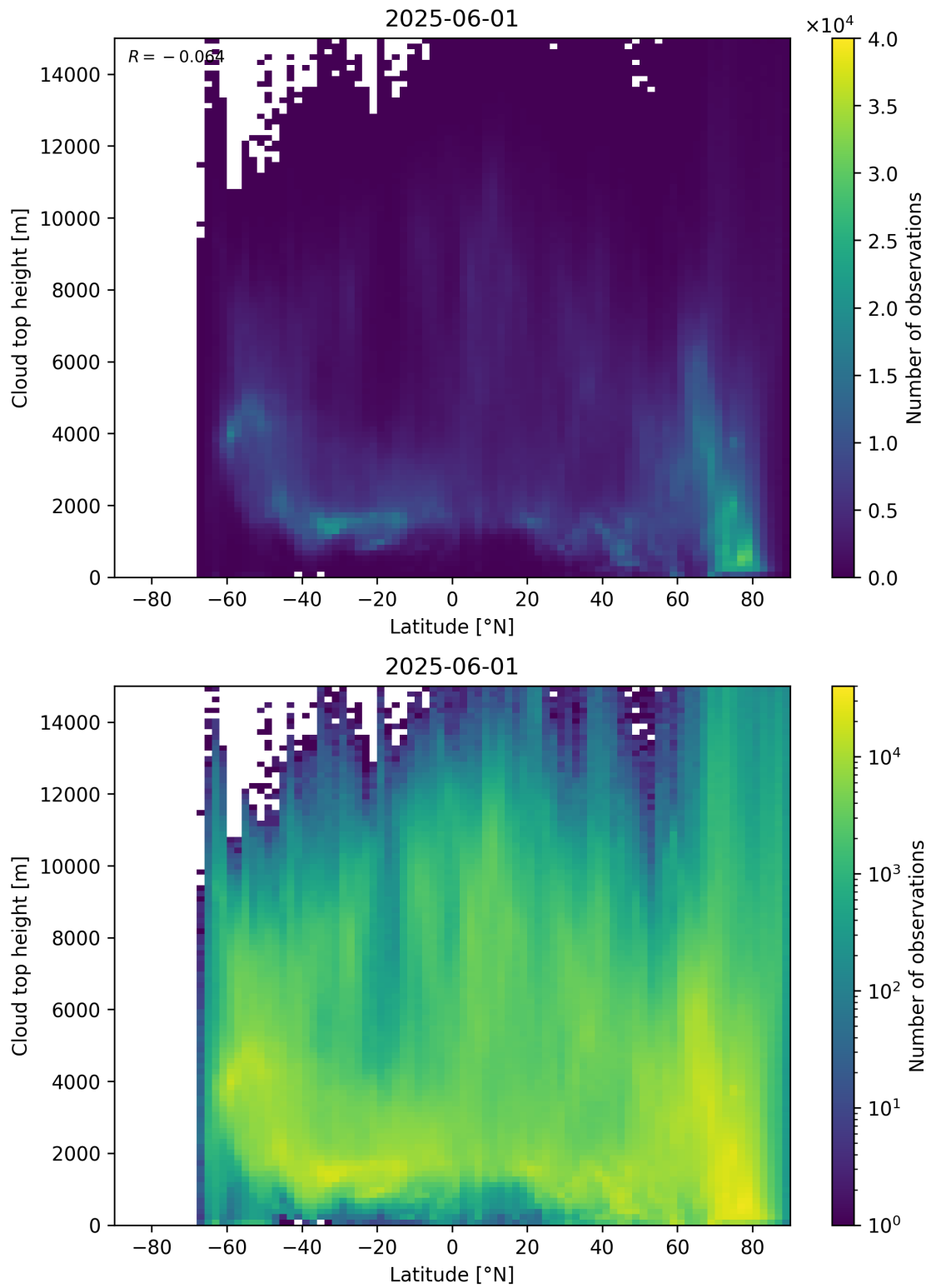
Figure 97: Scatter density plot of “Latitude” against “Cloud top height” for 2025-06-01 to 2025-06-02.
