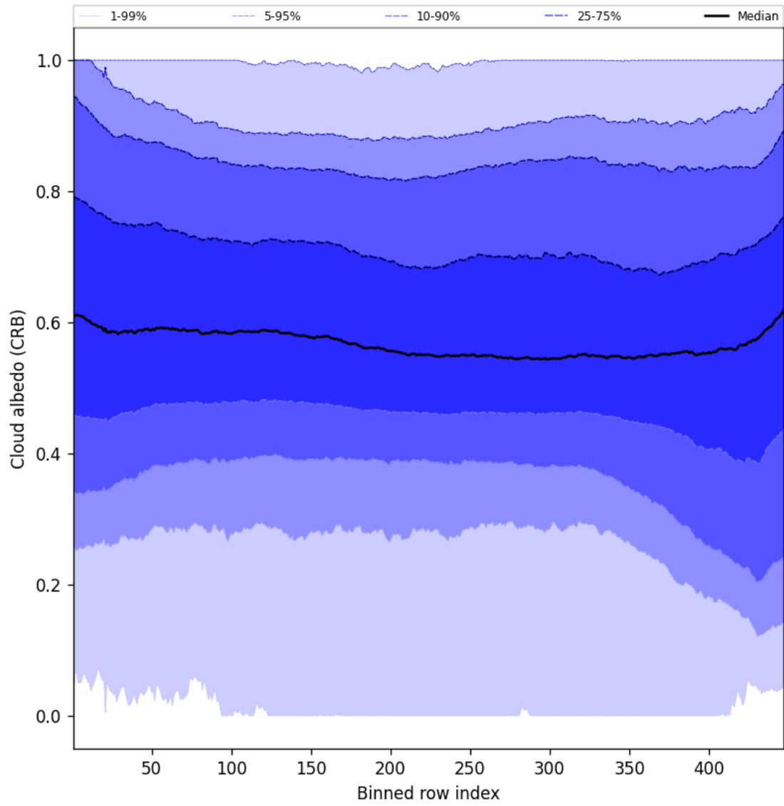
Figure 60: Along track statistics of “Cloud albedo (CRB)” for 2025-06-01 to 2025-06-02
