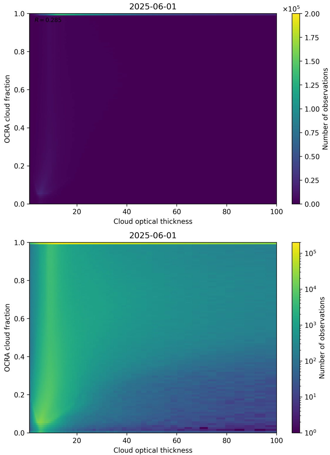
Figure 83: Scatter density plot of “Cloud optical thickness” against “OCRA cloud fraction” for 2025-06-01 to 2025-06-02.
