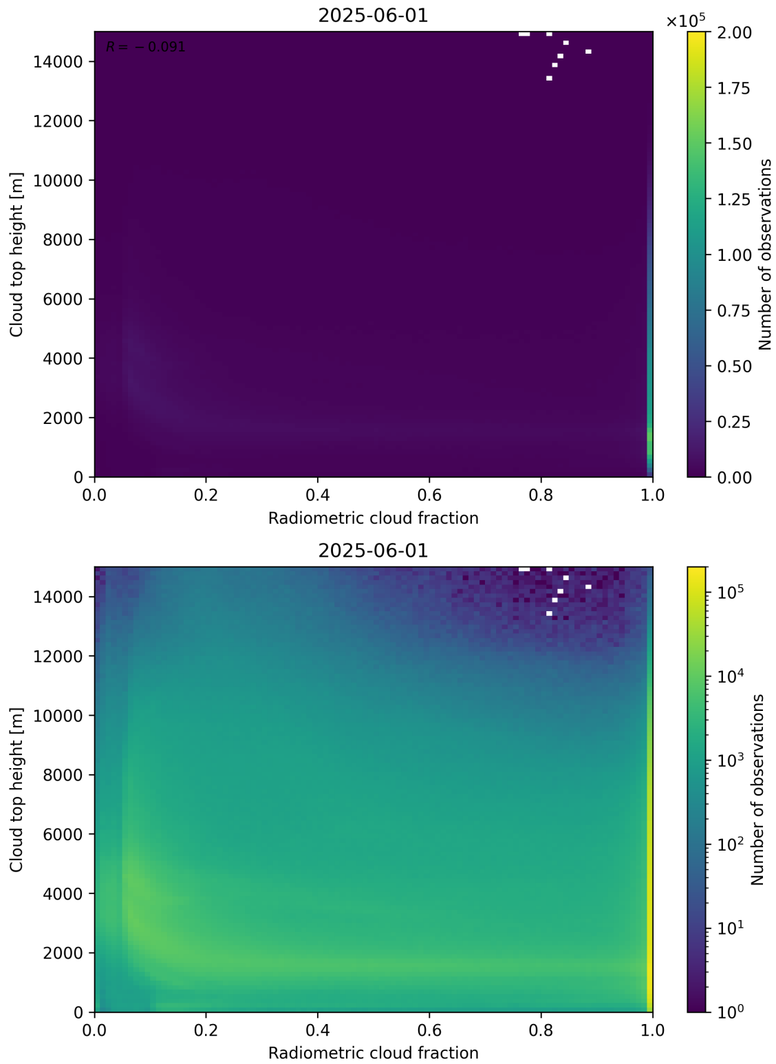
Figure 76: Scatter density plot of “Radiometric cloud fraction” against “Cloud top height” for 2025-06-01 to 2025-06-02.
