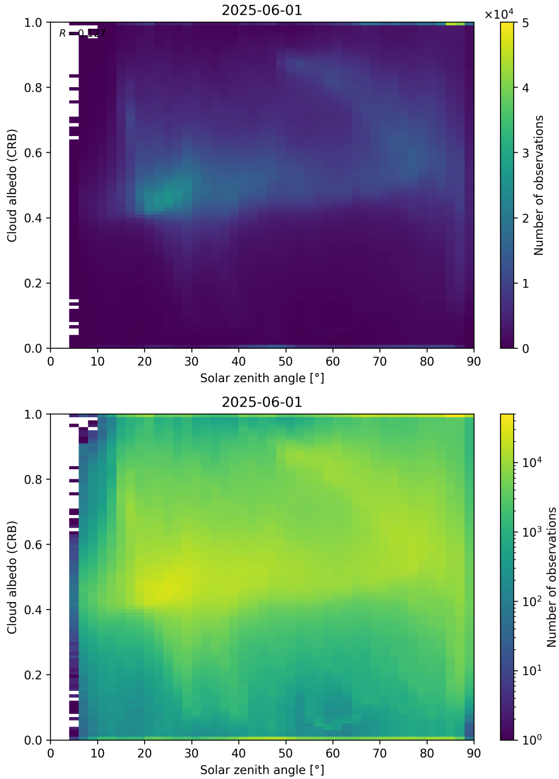
Figure 98: Scatter density plot of “Solar zenith angle” against “Cloud albedo (CRB)” for 2025-06-01 to 2025-06-02.
