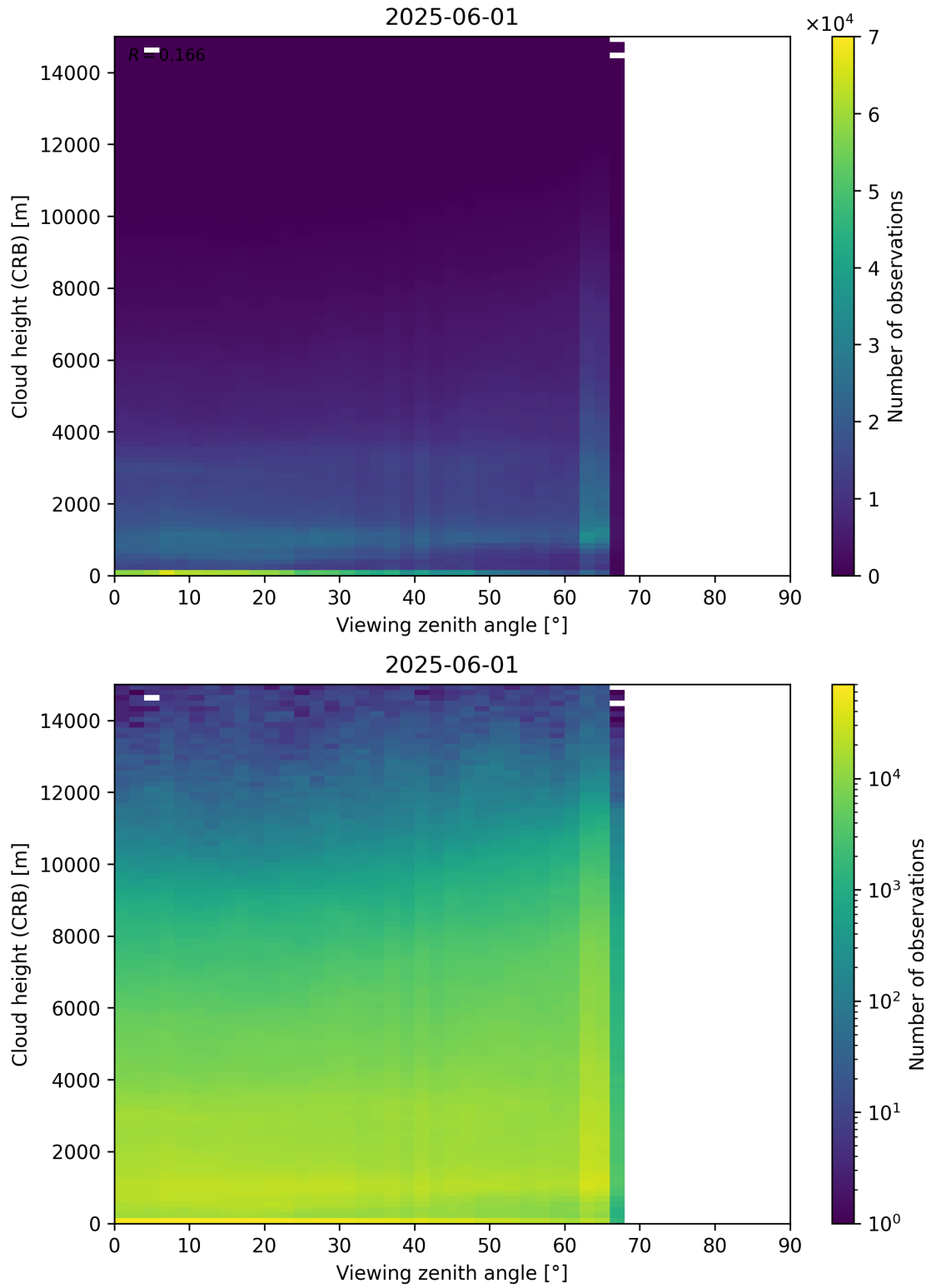
Figure 110: Scatter density plot of “Viewing zenith angle” against “Cloud height (CRB)” for 2025-06-01 to 2025-06-02.
