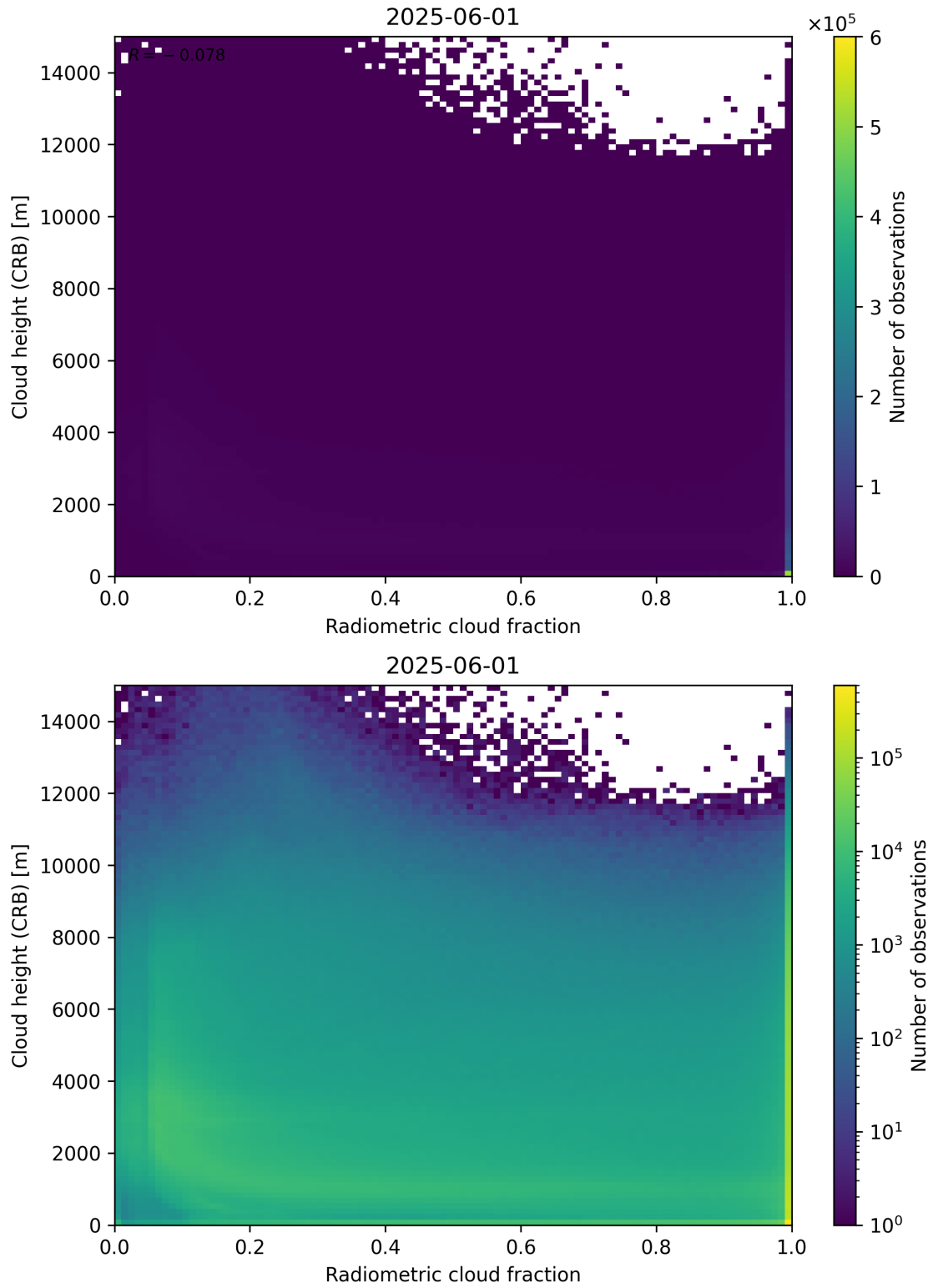
Figure 74: Scatter density plot of “Radiometric cloud fraction” against “Cloud height (CRB)” for 2025-06-01 to 2025-06-02.
