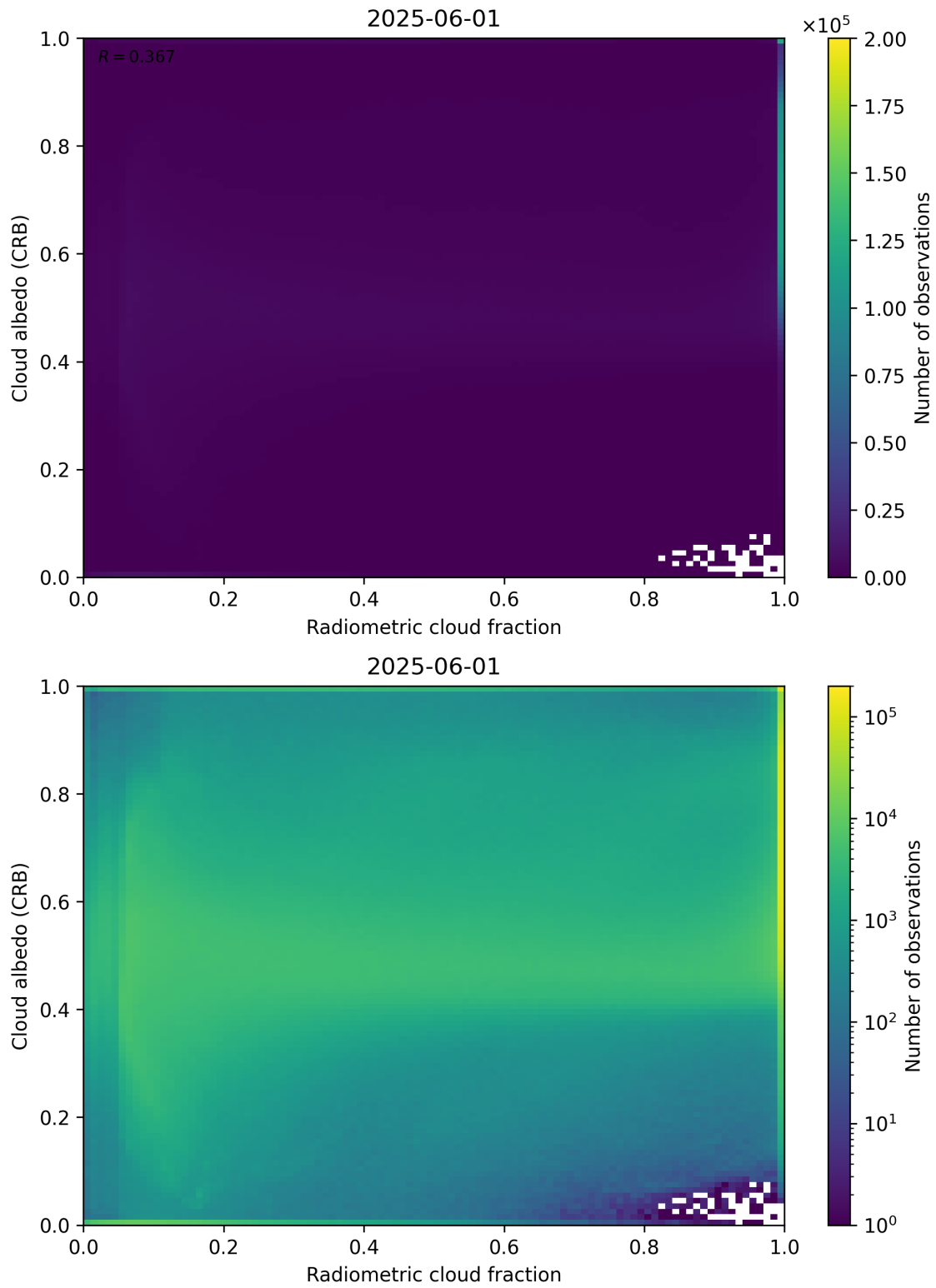
Figure 71: Scatter density plot of “Radiometric cloud fraction” against “Cloud albedo (CRB)” for 2025-06-01 to 2025-06-02.
