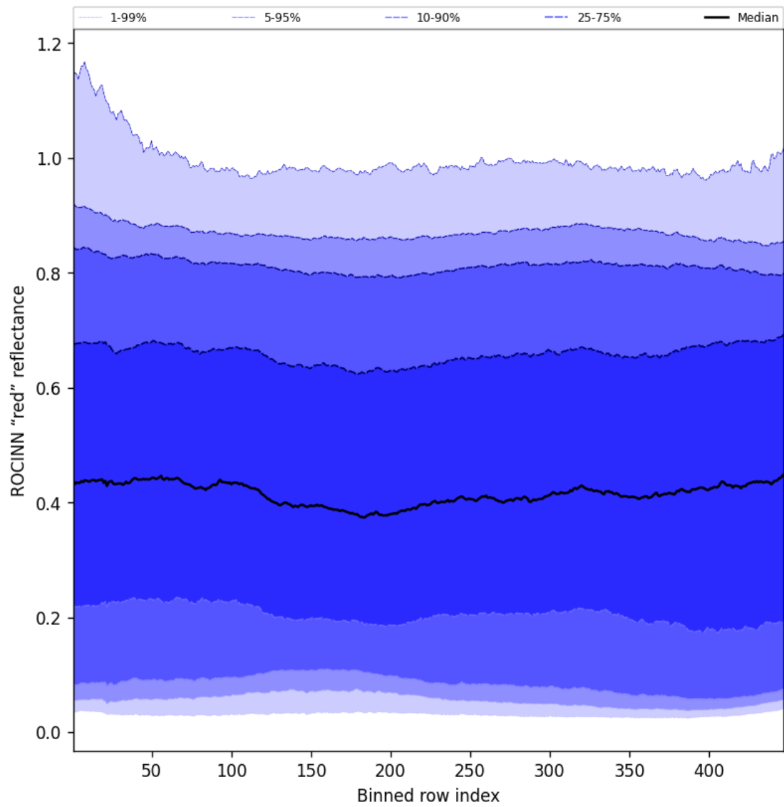
Figure 69: Along track statistics of "ROCINN "red" reflectance" for 2025-06-01 to 2025-06-02
