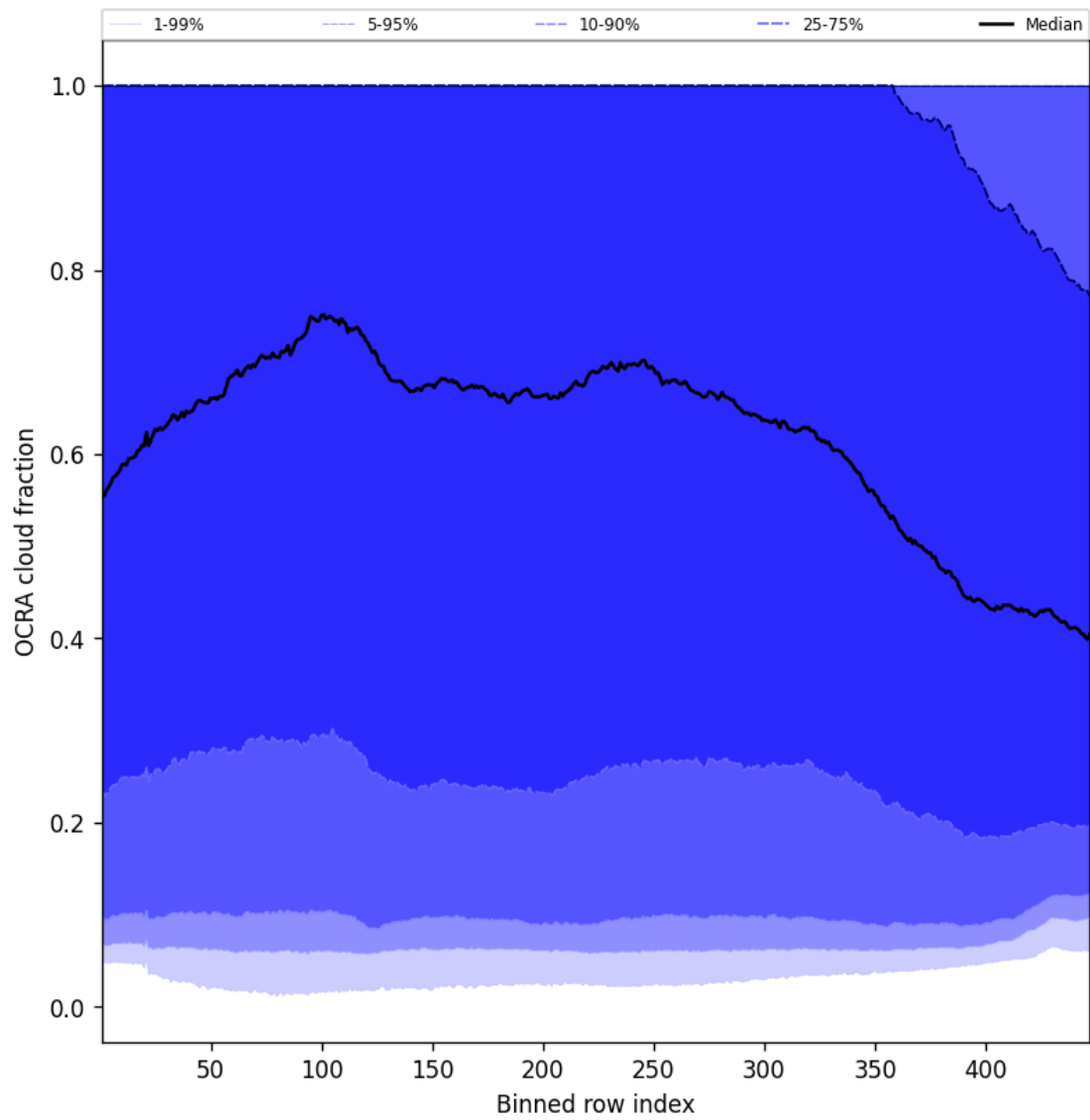
Figure 66: Along track statistics of “OCRA cloud fraction” for 2025-06-01 to 2025-06-02
