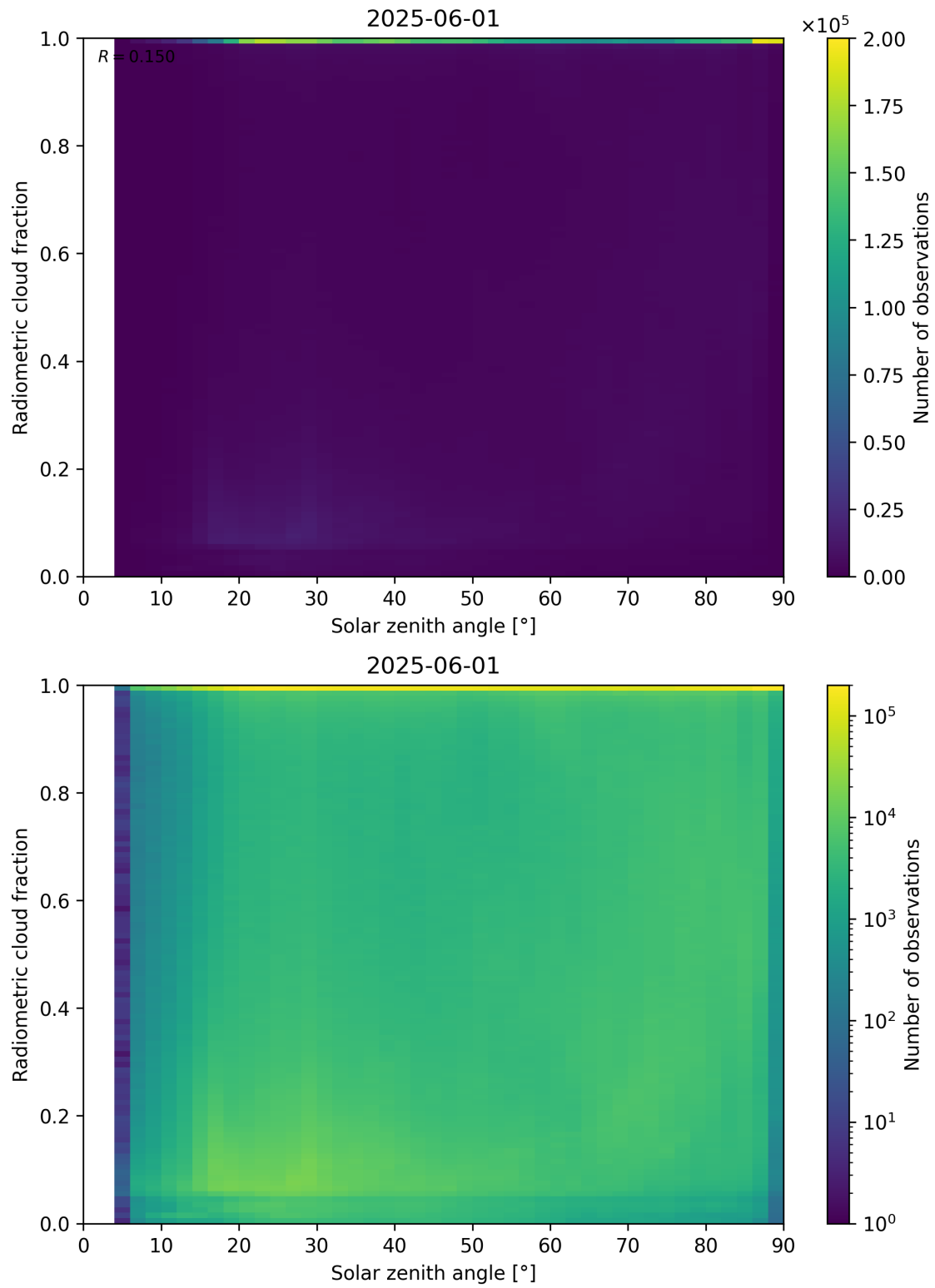
Figure 99: Scatter density plot of “Solar zenith angle” against “Radiometric cloud fraction” for 2025-06-01 to 2025-06-02.
