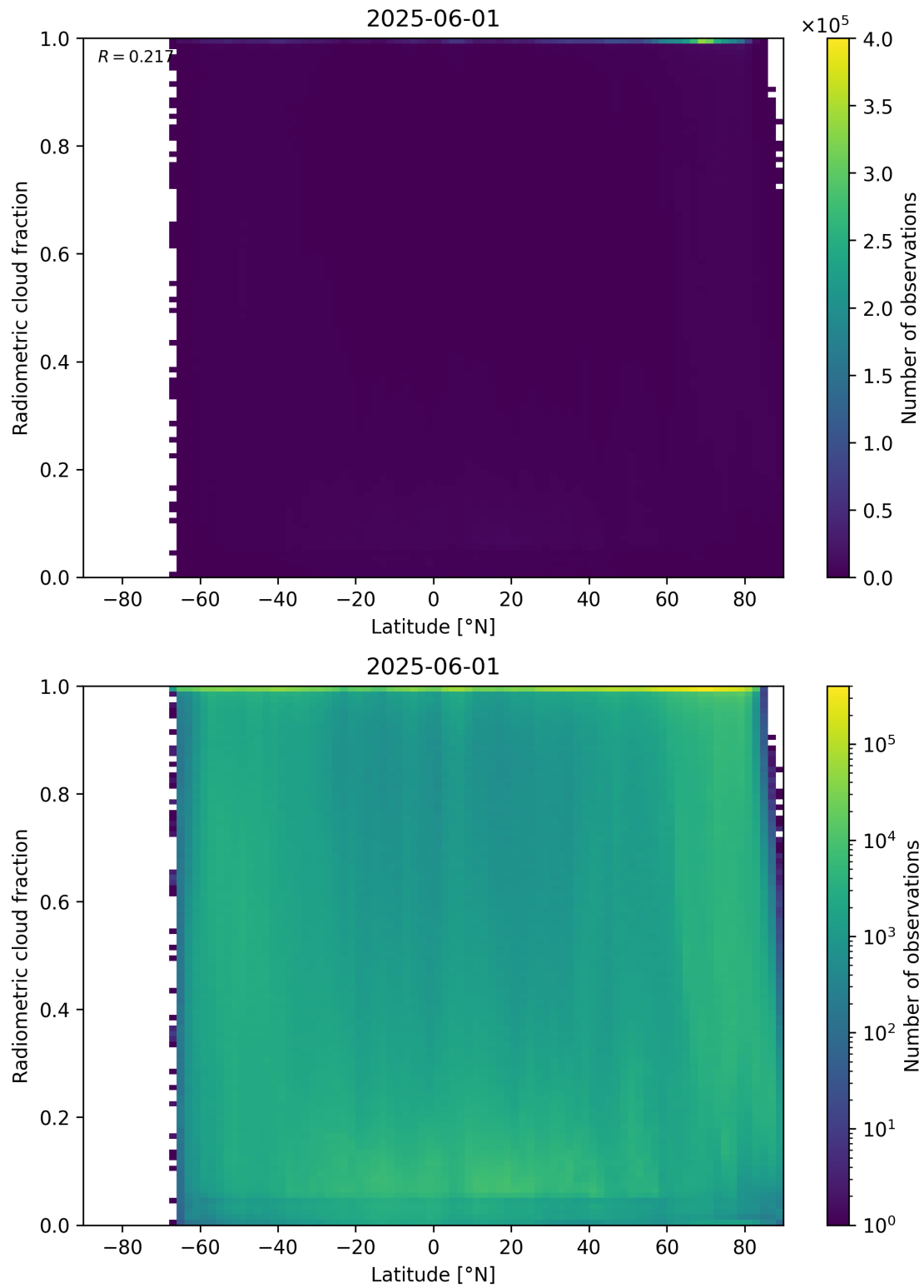
Figure 92: Scatter density plot of “Latitude” against “Radiometric cloud fraction” for 2025-06-01 to 2025-06-02.
