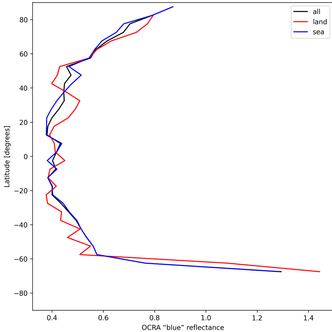
Figure 35: Zonal average of "OCRA "blue" reflectance" for 2025-06-01 to 2025-06-02.
