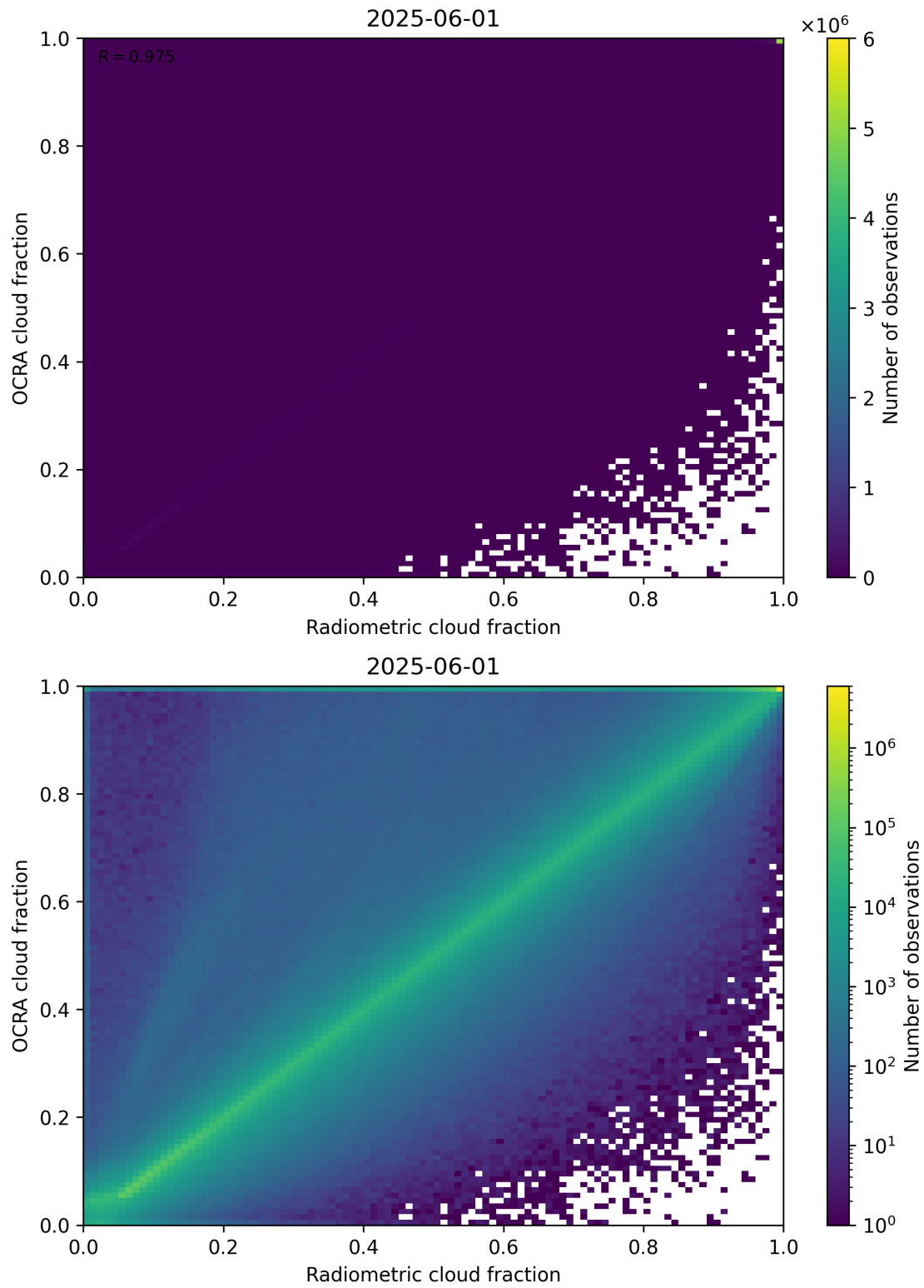
Figure 72: Scatter density plot of “Radiometric cloud fraction” against “OCRA cloud fraction” for 2025-06-01 to 2025-06-02.
