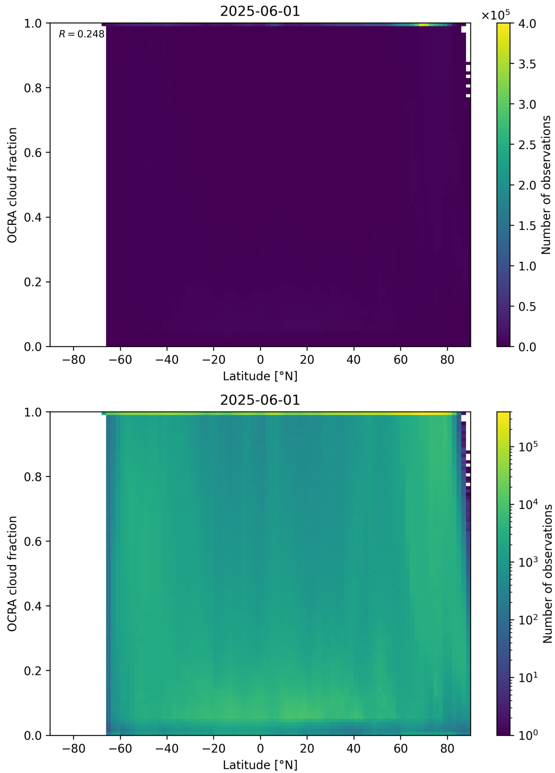
Figure 93: Scatter density plot of “Latitude” against “OCRA cloud fraction” for 2025-06-01 to 2025-06-02.
