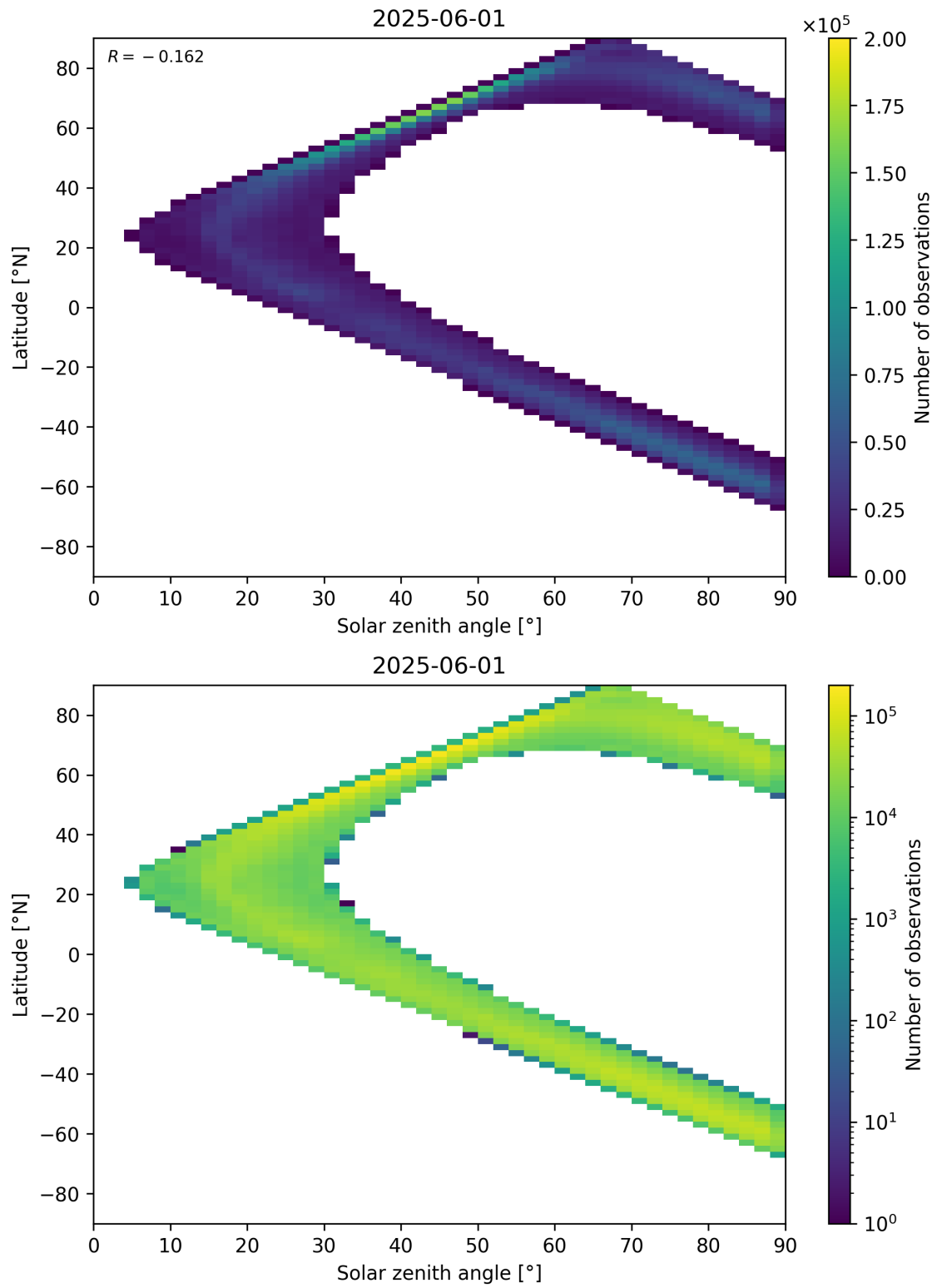
Figure 105: Scatter density plot of “Solar zenith angle” against “Latitude” for 2025-06-01 to 2025-06-02.
