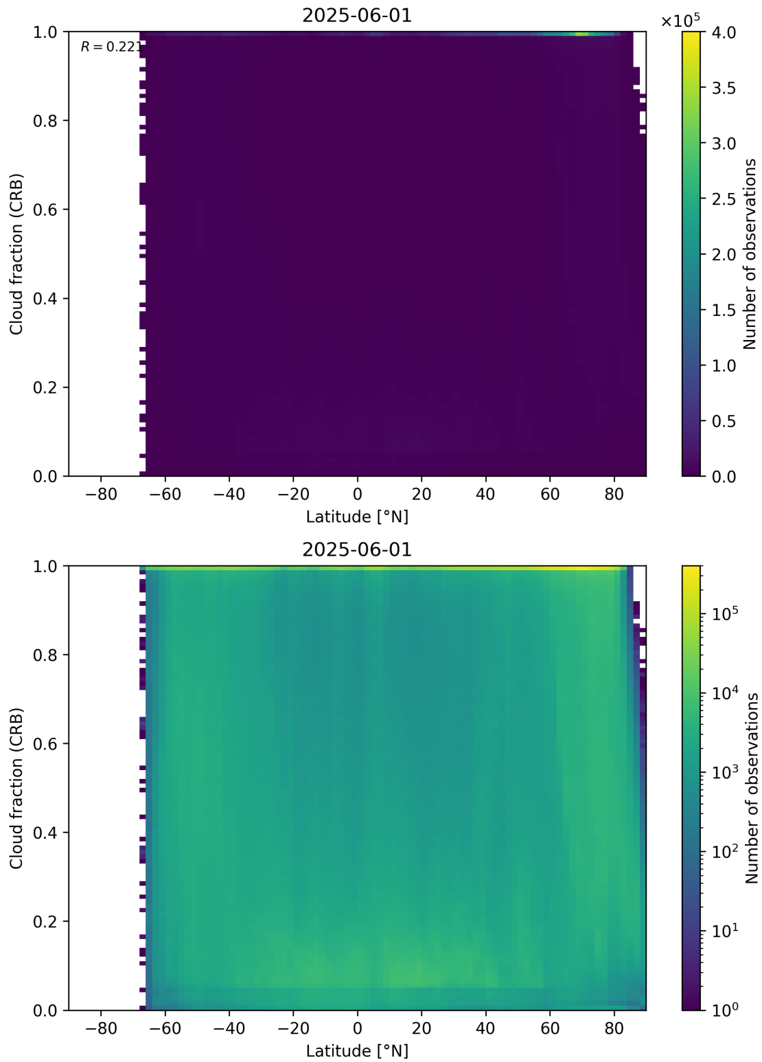
Figure 94: Scatter density plot of “Latitude” against “Cloud fraction (CRB)” for 2025-06-01 to 2025-06-02.
