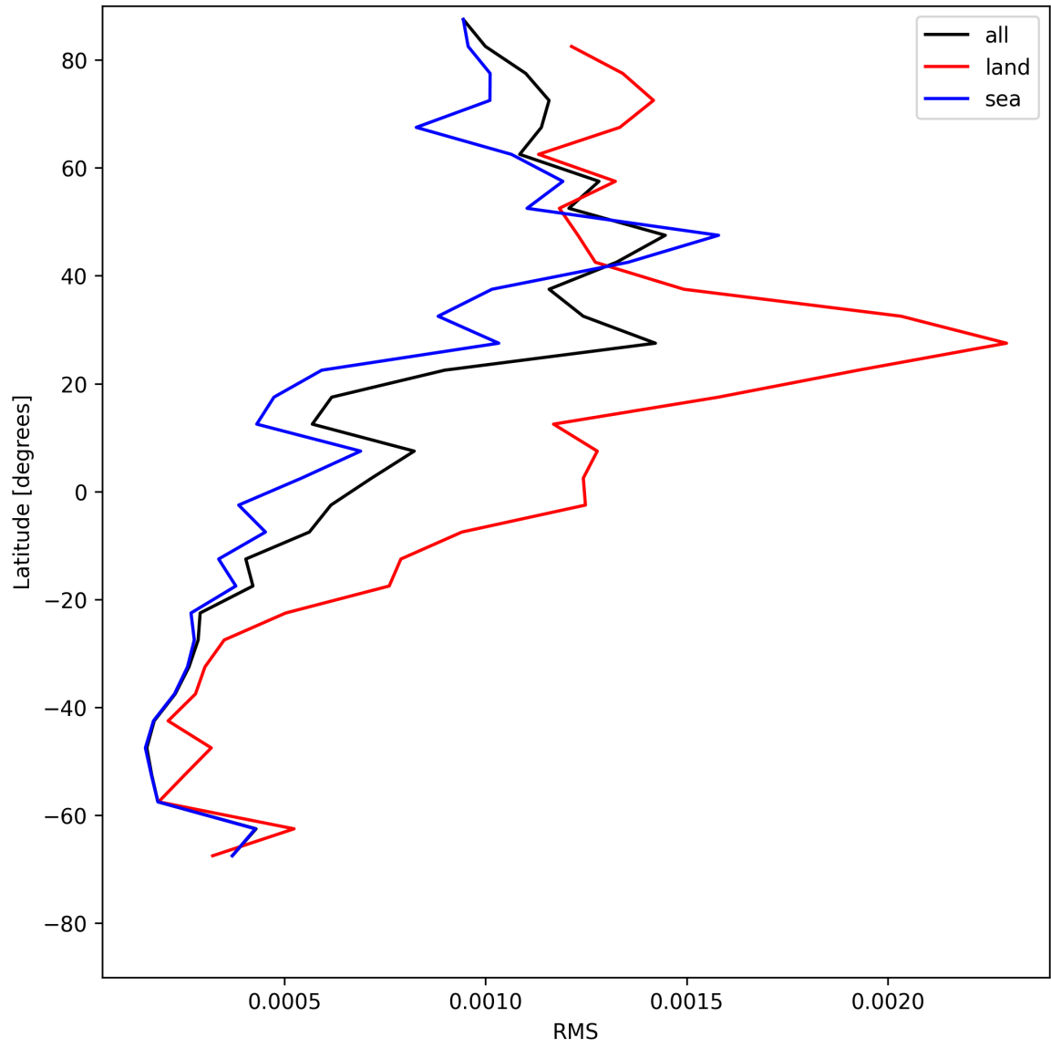
Figure 31: Zonal average of “RMS” for 2025-06-01 to 2025-06-02.
