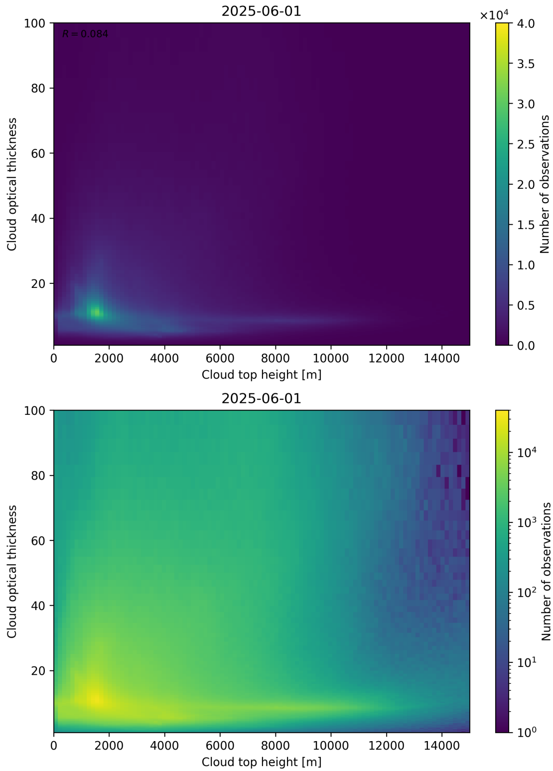
Figure 90: Scatter density plot of “Cloud top height” against “Cloud optical thickness” for 2025-06-01 to 2025-06-02.
