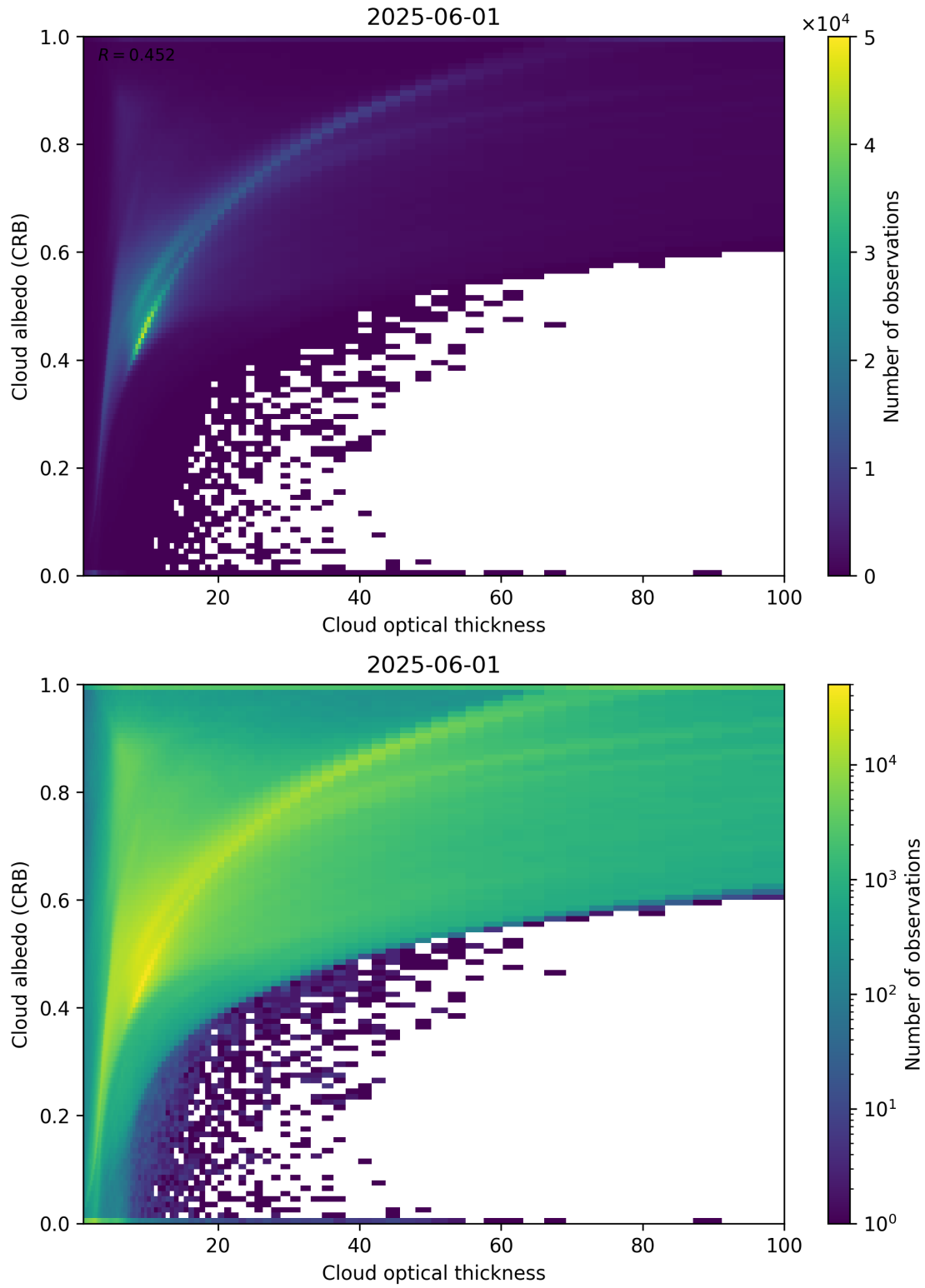
Figure 82: Scatter density plot of “Cloud optical thickness” against “Cloud albedo (CRB)” for 2025-06-01 to 2025-06-02.
