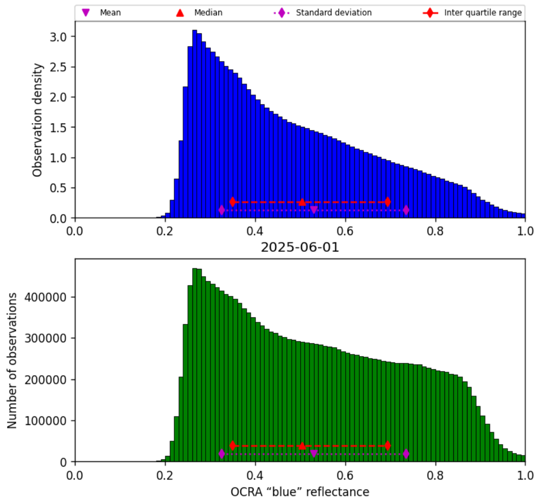
Figure 51: Histogram of “OCRA “blue” reflectance” for 2025-06-01 to 2025-06-02
