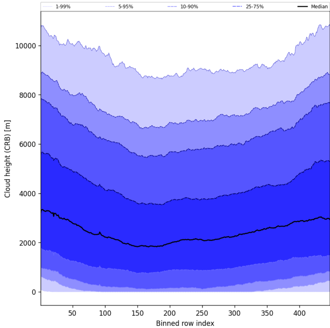
Figure 59: Along track statistics of “Cloud height (CRB)” for 2025-06-01 to 2025-06-02
