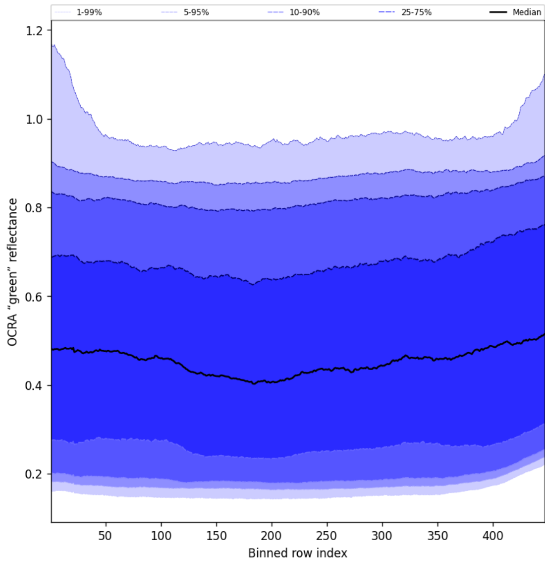
Figure 68: Along track statistics of "OCRA "green" reflectance" for 2025-06-01 to 2025-06-02
