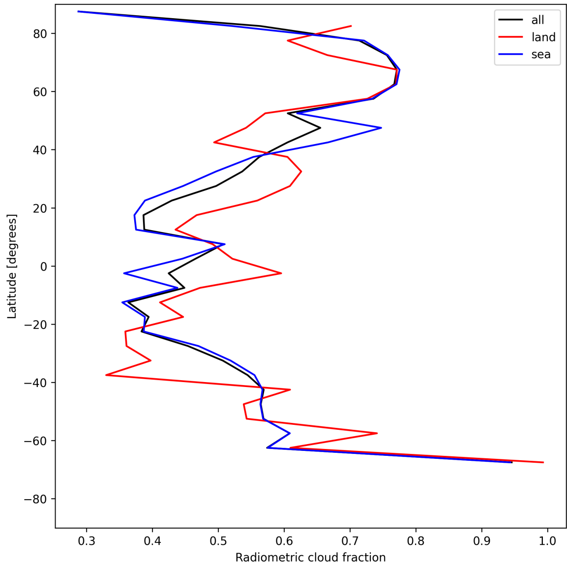
Figure 23: Zonal average of “Radiometric cloud fraction” for 2025-06-01 to 2025-06-02.
