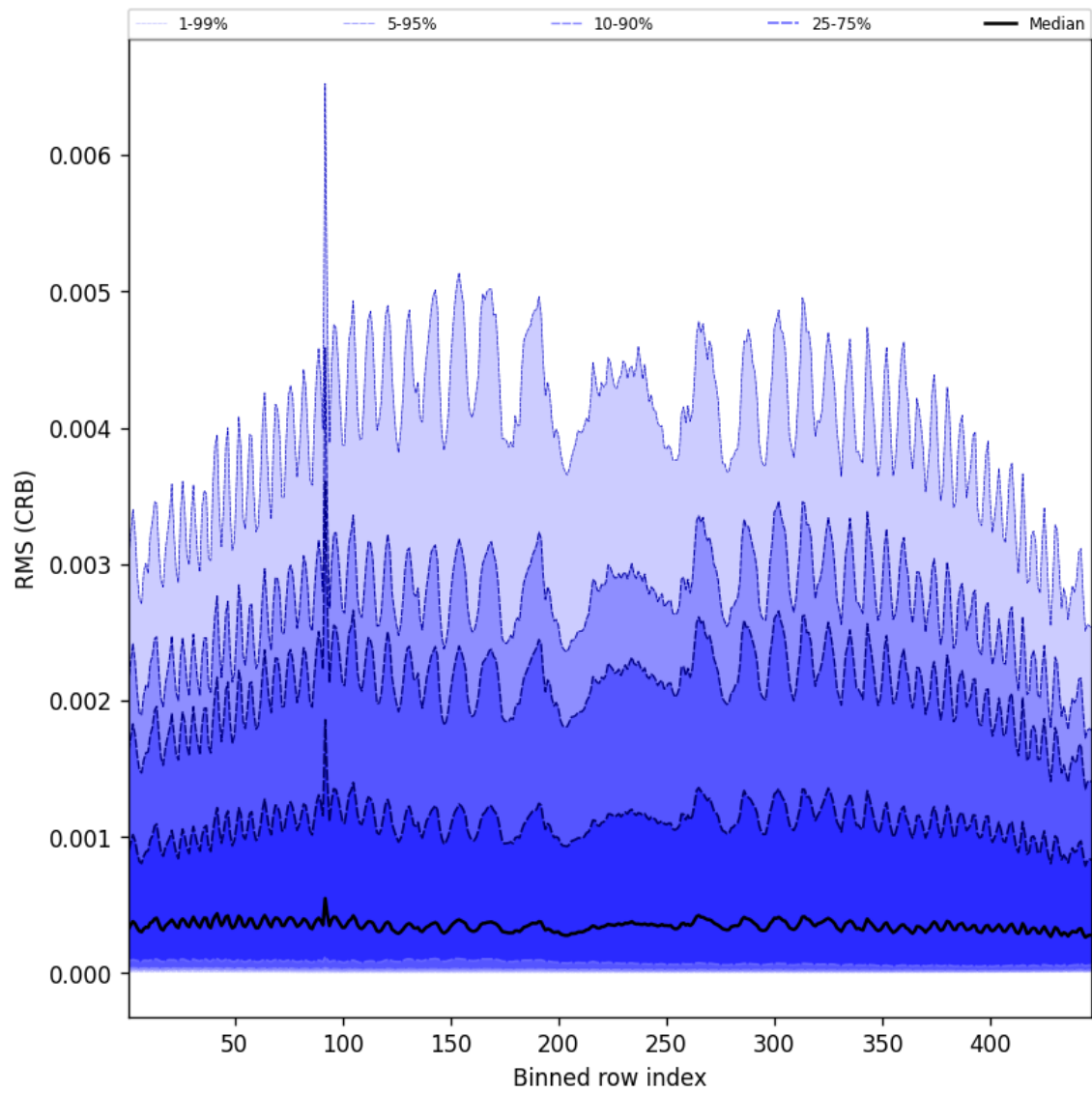
Figure 64: Along track statistics of “RMS (CRB)” for 2025-06-01 to 2025-06-02
