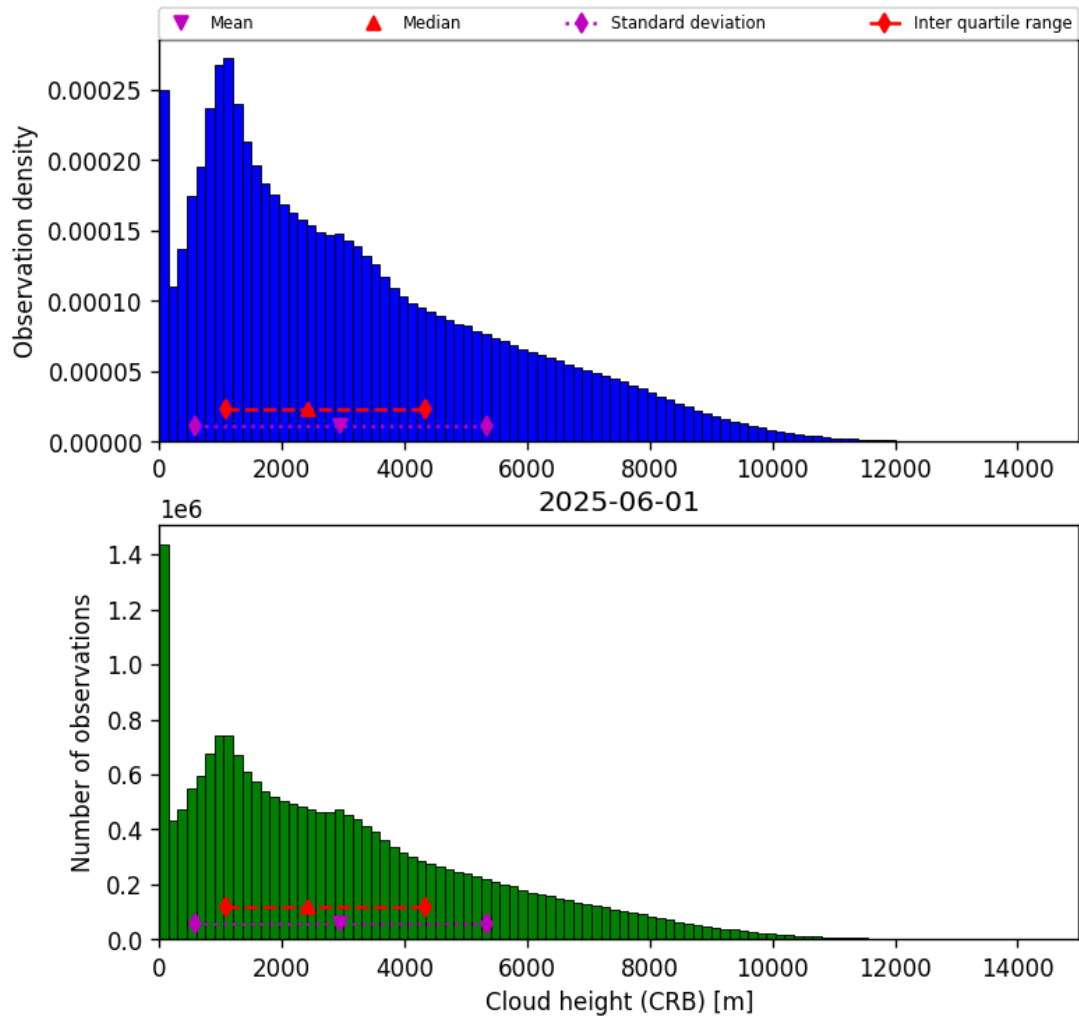
Figure 43: Histogram of “Cloud height (CRB)” for 2025-06-01 to 2025-06-02
