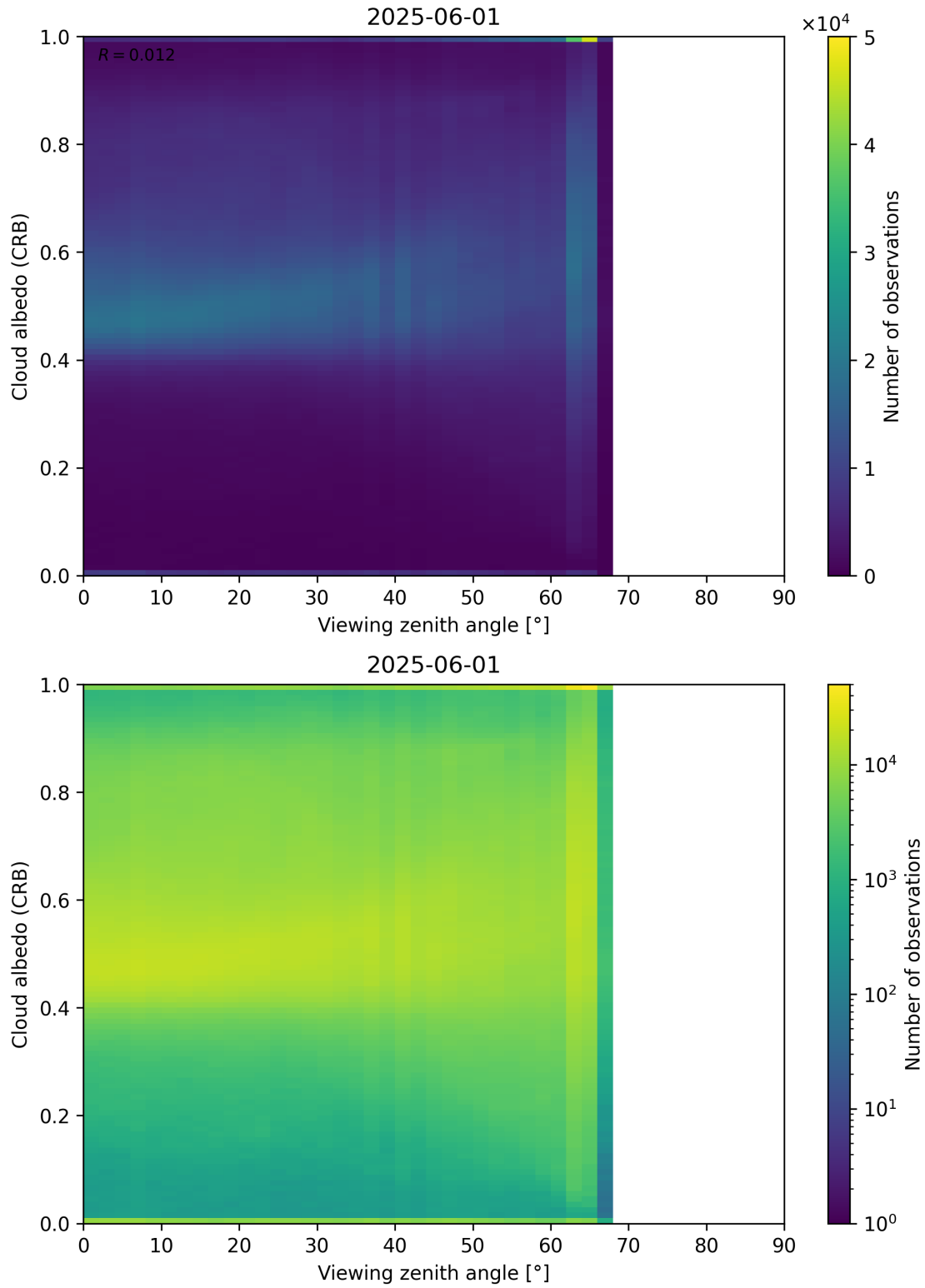
Figure 106: Scatter density plot of “Viewing zenith angle” against “Cloud albedo (CRB)” for 2025-06-01 to 2025-06-02.
