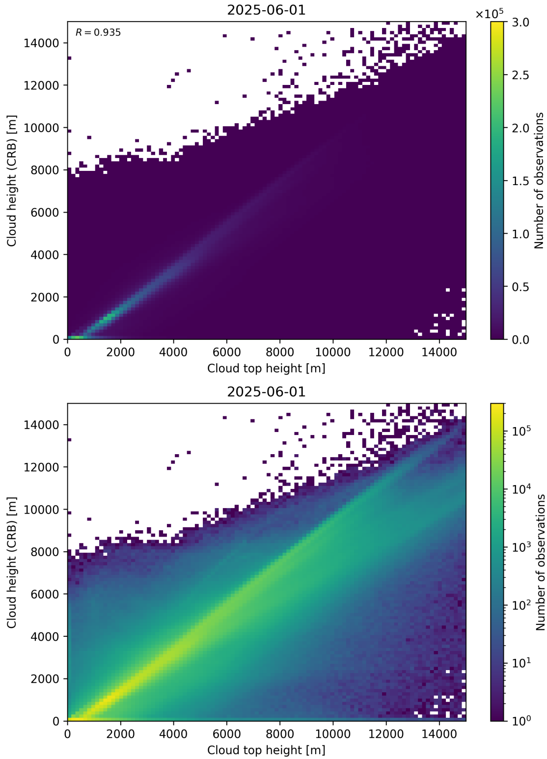
Figure 89: Scatter density plot of “Cloud top height” against “Cloud height (CRB)” for 2025-06-01 to 2025-06-02.
