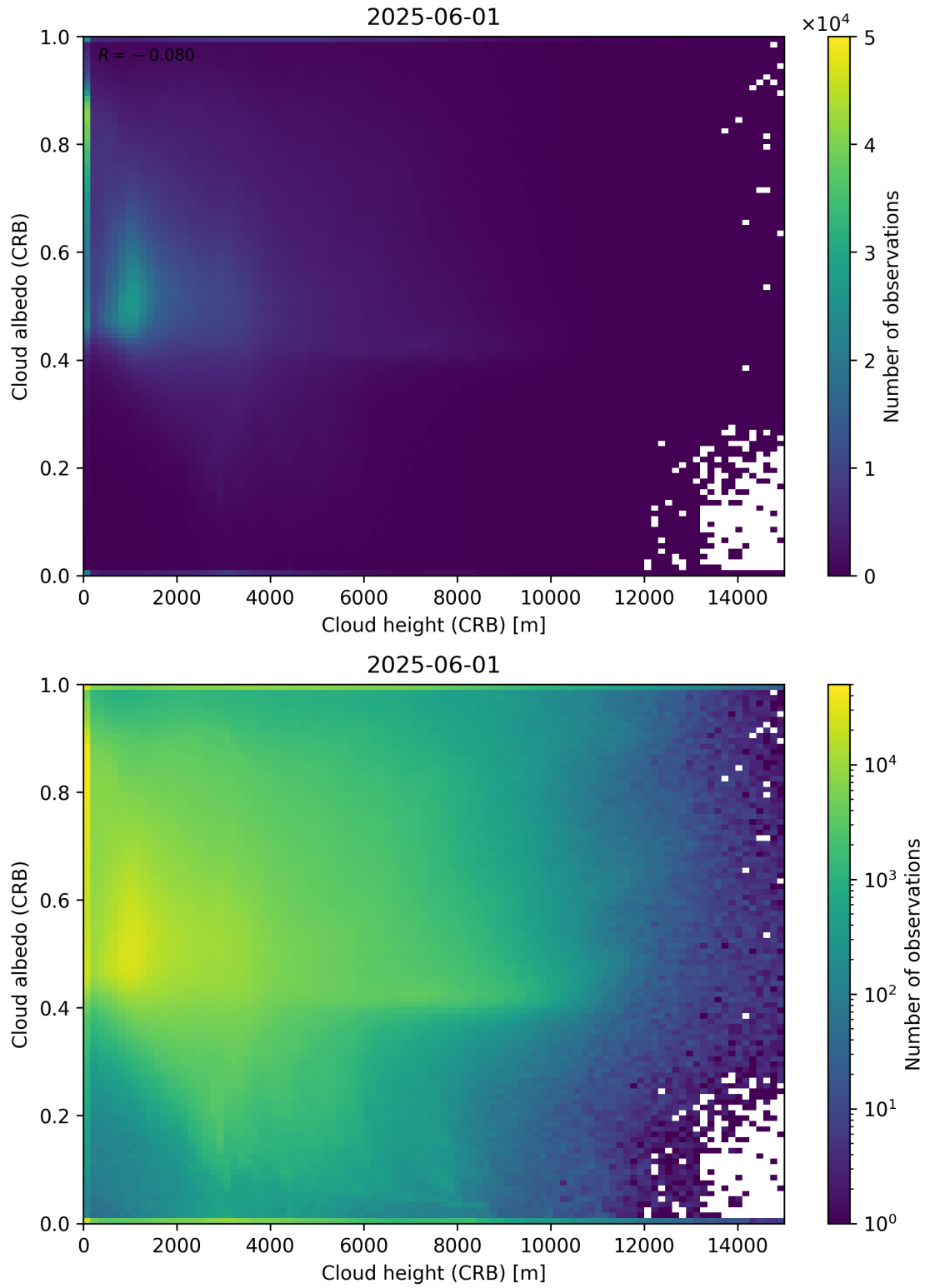
Figure 80: Scatter density plot of “Cloud height (CRB)” against “Cloud albedo (CRB)” for 2025-06-01 to 2025-06-02.
