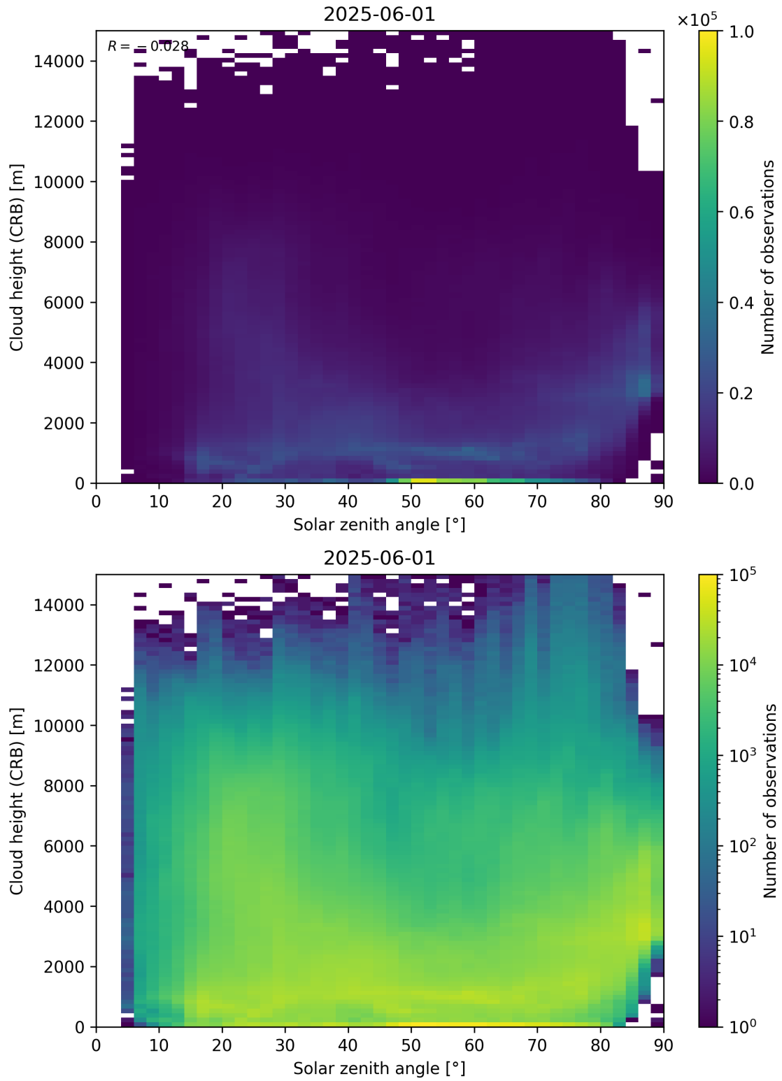
Figure 102: Scatter density plot of “Solar zenith angle” against “Cloud height (CRB)” for 2025-06-01 to 2025-06-02.
