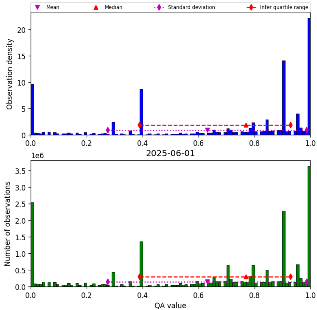
Figure 38: Histogram of “QA value” for 2025-06-01 to 2025-06-02
