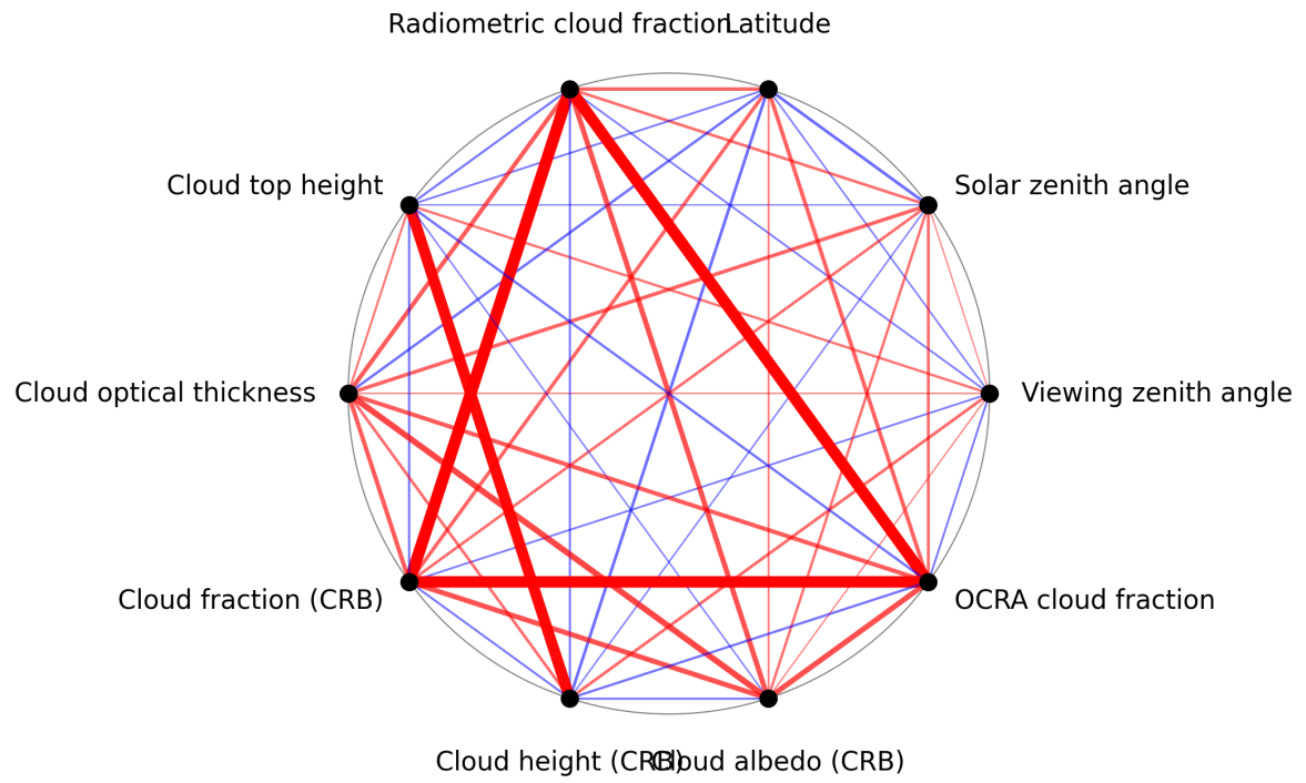
Figure 1: Map of correlation graph for 2025-06-01 to 2025-06-02.
