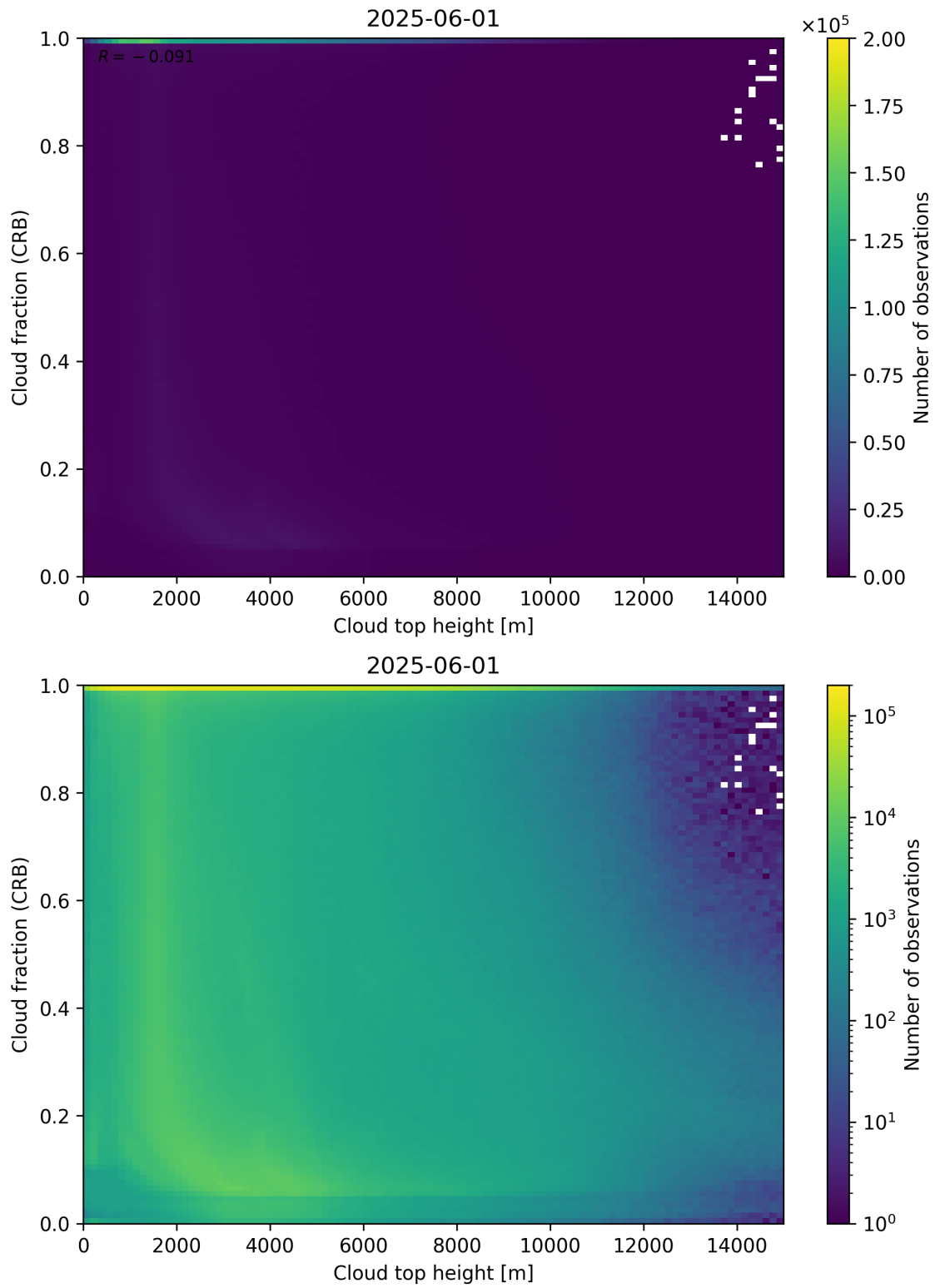
Figure 88: Scatter density plot of “Cloud top height” against “Cloud fraction (CRB)” for 2025-06-01 to 2025-06-02.
