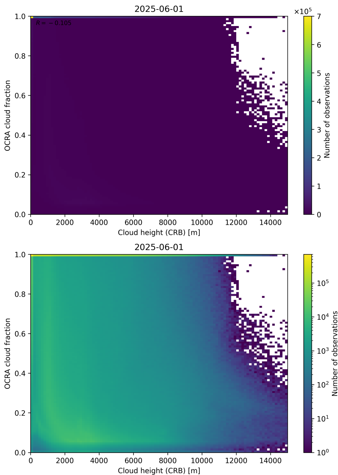
Figure 81: Scatter density plot of “Cloud height (CRB)” against “OCRA cloud fraction” for 2025-06-01 to 2025-06-02.
