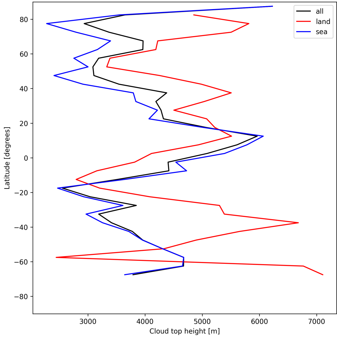
Figure 24: Zonal average of “Cloud top height” for 2025-06-01 to 2025-06-02.
