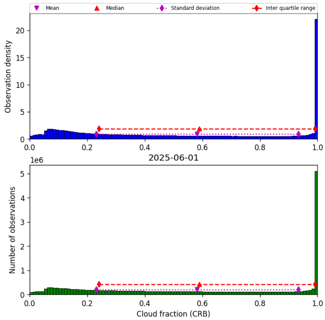
Figure 42: Histogram of “Cloud fraction (CRB)” for 2025-06-01 to 2025-06-02
