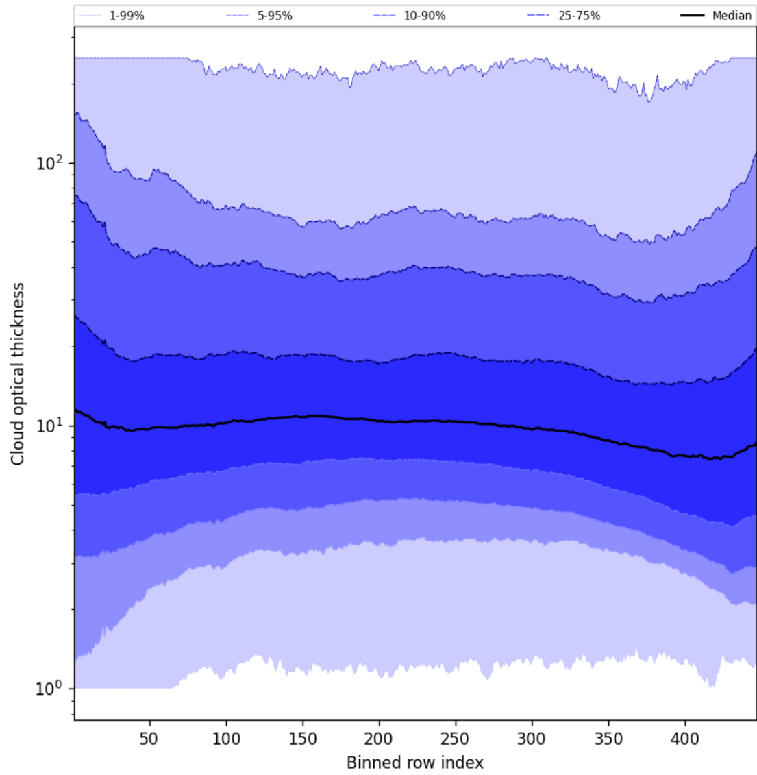
Figure 57: Along track statistics of “Cloud optical thickness” for 2025-06-01 to 2025-06-02
