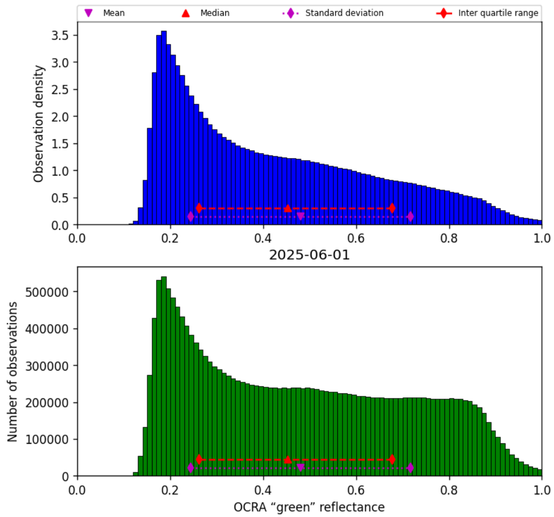
Figure 52: Histogram of “OCRA “green” reflectance” for 2025-06-01 to 2025-06-02
