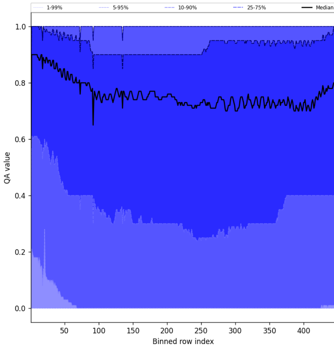
Figure 54: Along track statistics of “QA value” for 2025-06-01 to 2025-06-02
