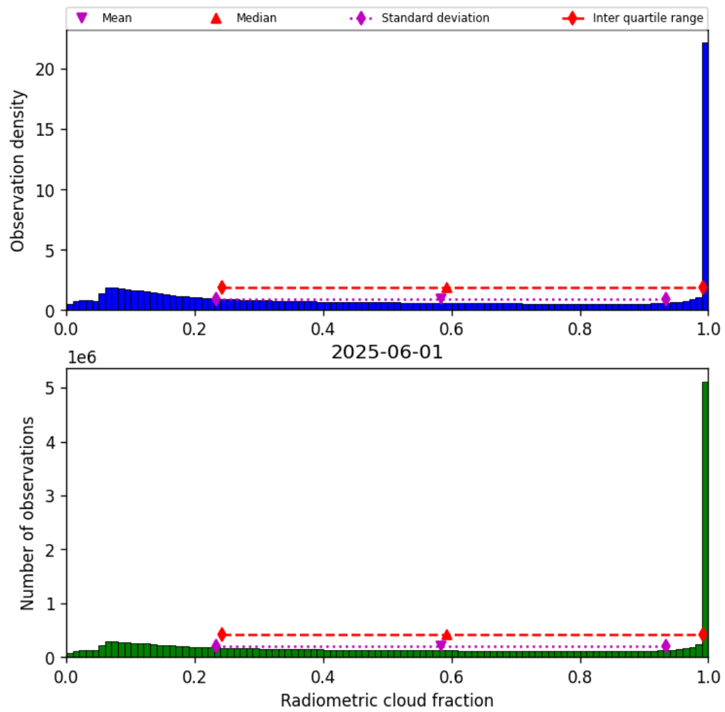
Figure 39: Histogram of “Radiometric cloud fraction” for 2025-06-01 to 2025-06-02
