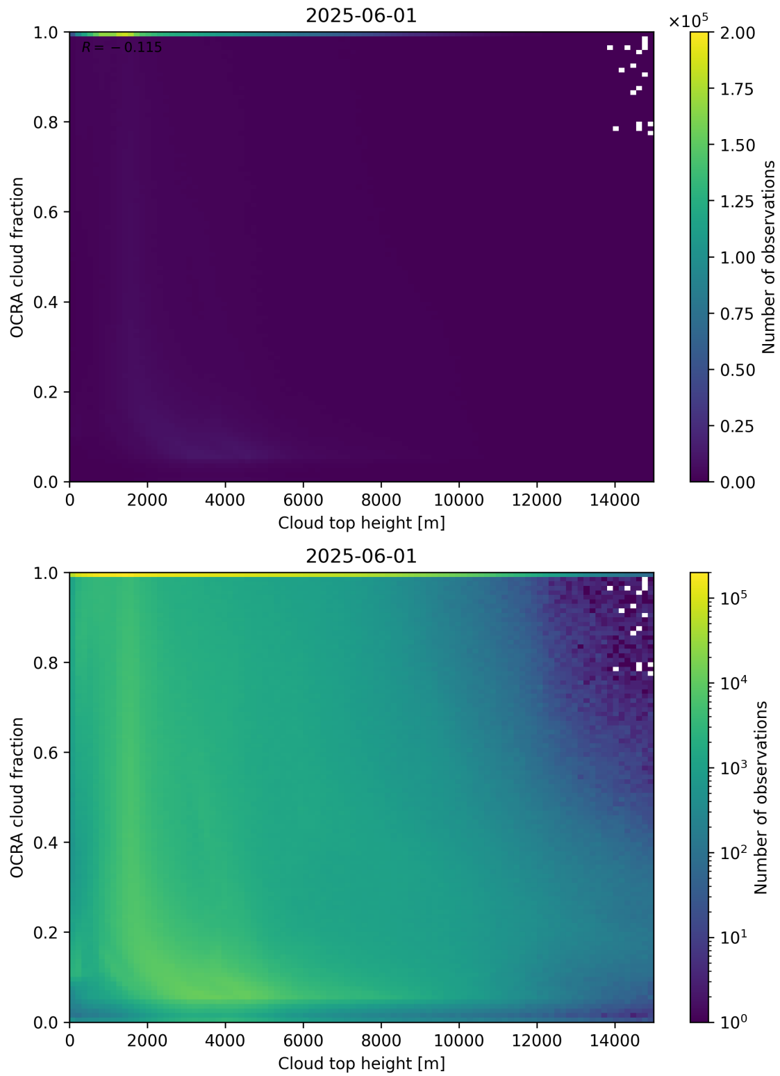
Figure 87: Scatter density plot of “Cloud top height” against “OCRA cloud fraction” for 2025-06-01 to 2025-06-02.
