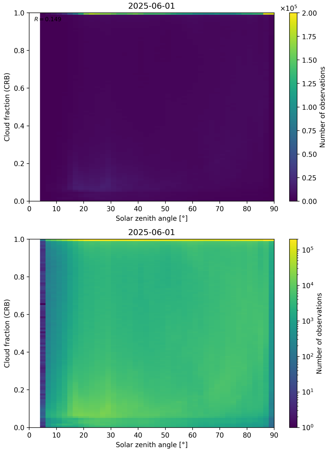
Figure 101: Scatter density plot of “Solar zenith angle” against “Cloud fraction (CRB)” for 2025-06-01 to 2025-06-02.
