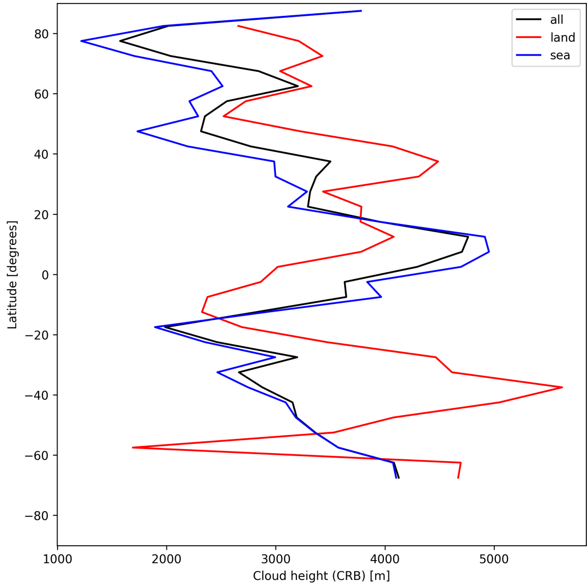
Figure 27: Zonal average of “Cloud height (CRB)” for 2025-06-01 to 2025-06-02.
