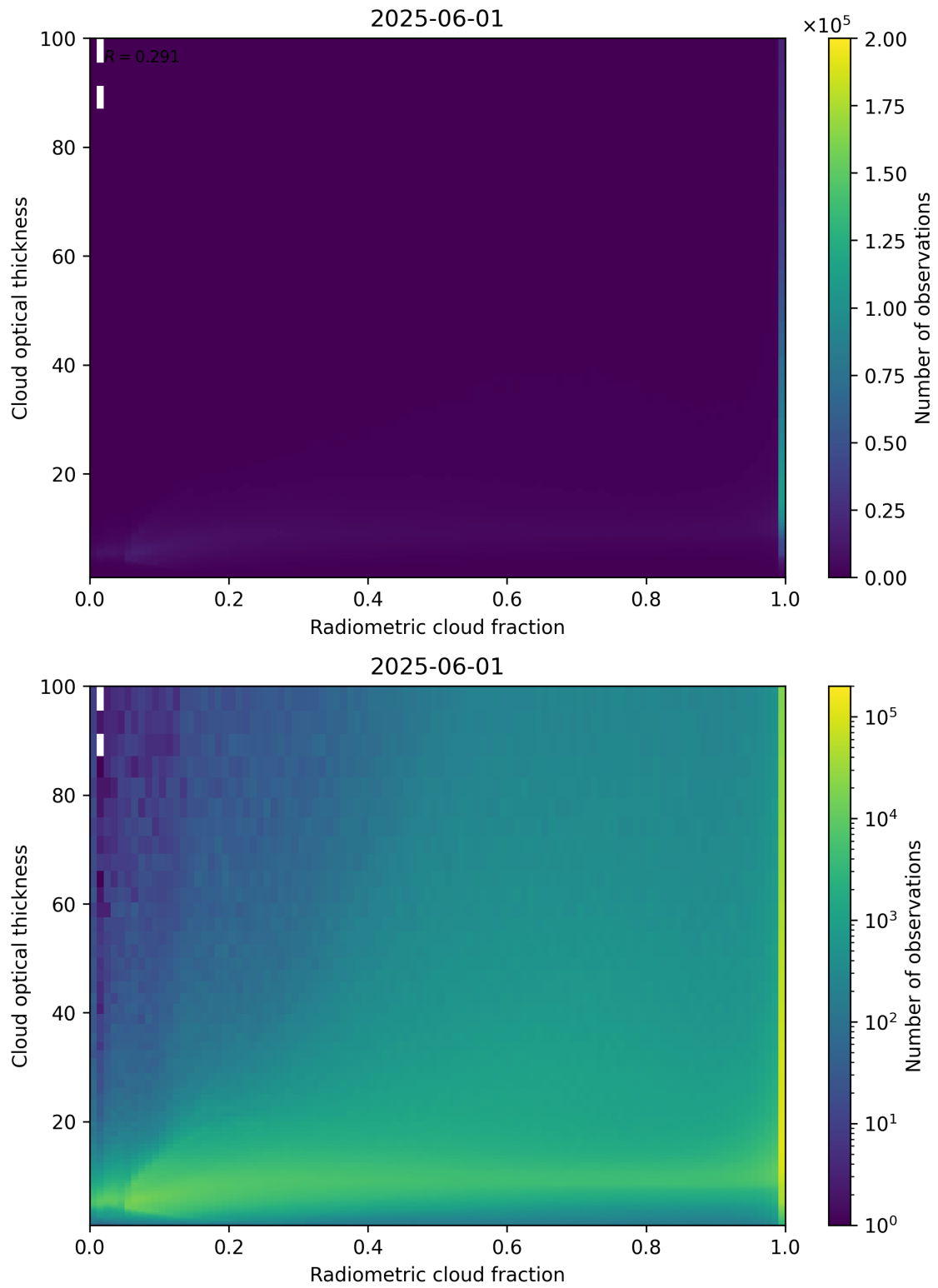
Figure 75: Scatter density plot of “Radiometric cloud fraction” against “Cloud optical thickness” for 2025-06-01 to 2025-06-02.
