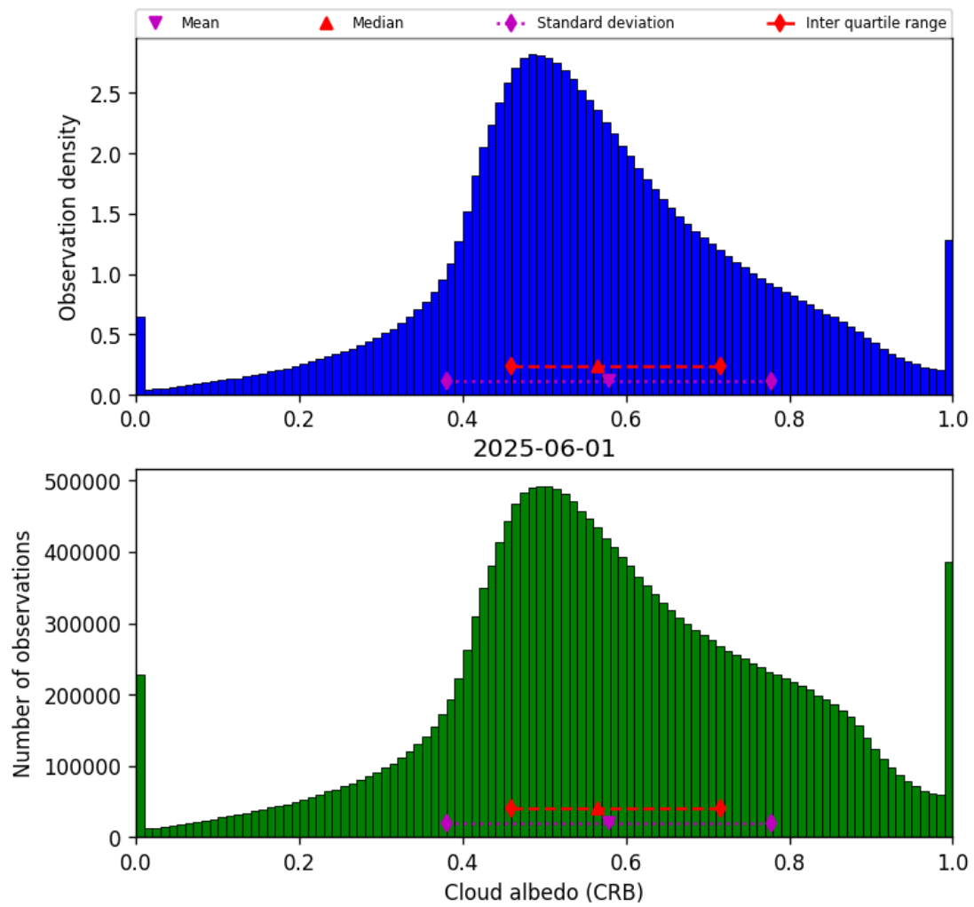
Figure 44: Histogram of “Cloud albedo (CRB)” for 2025-06-01 to 2025-06-02
