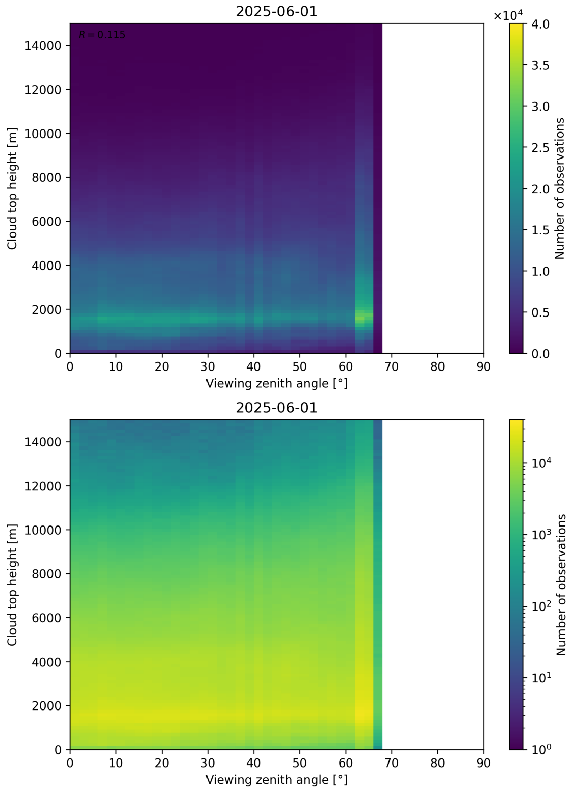
Figure 112: Scatter density plot of “Viewing zenith angle” against “Cloud top height” for 2025-06-01 to 2025-06-02.
