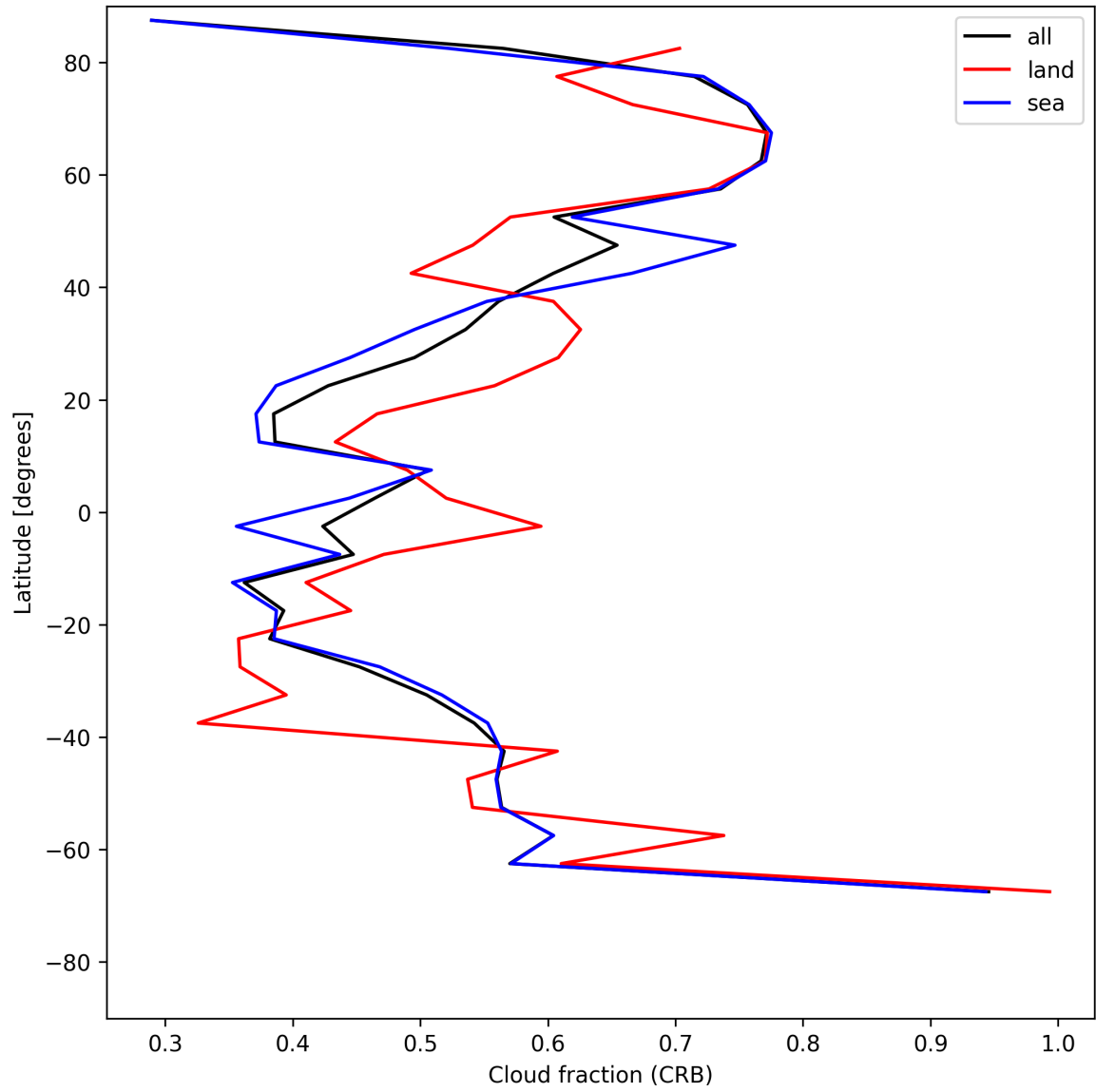
Figure 26: Zonal average of “Cloud fraction (CRB)” for 2025-06-01 to 2025-06-02.
