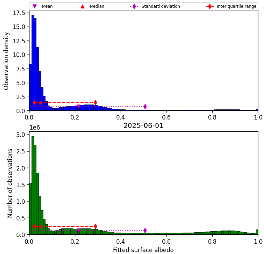
Figure 45: Histogram of “Fitted surface albedo” for 2025-06-01 to 2025-06-02
