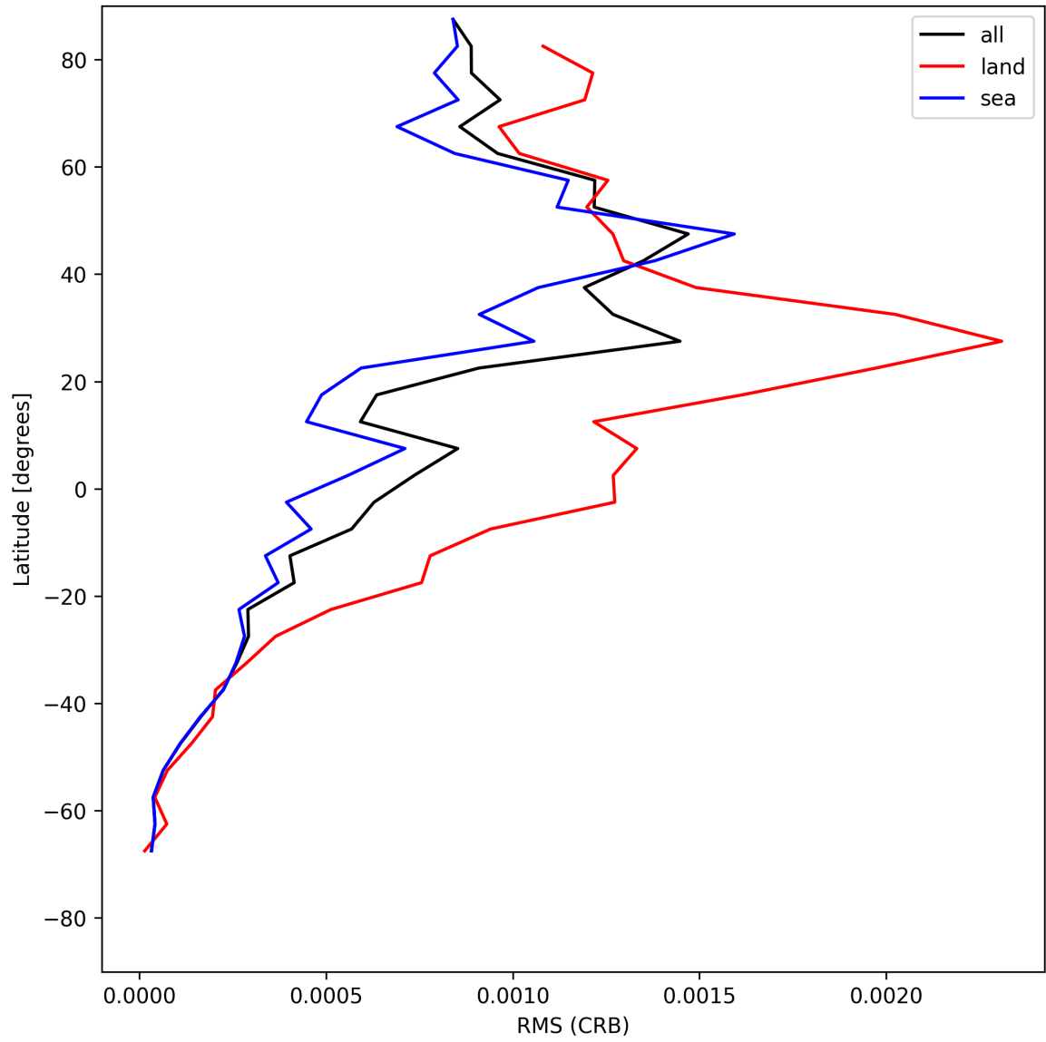
Figure 32: Zonal average of “RMS (CRB)” for 2025-06-01 to 2025-06-02.
