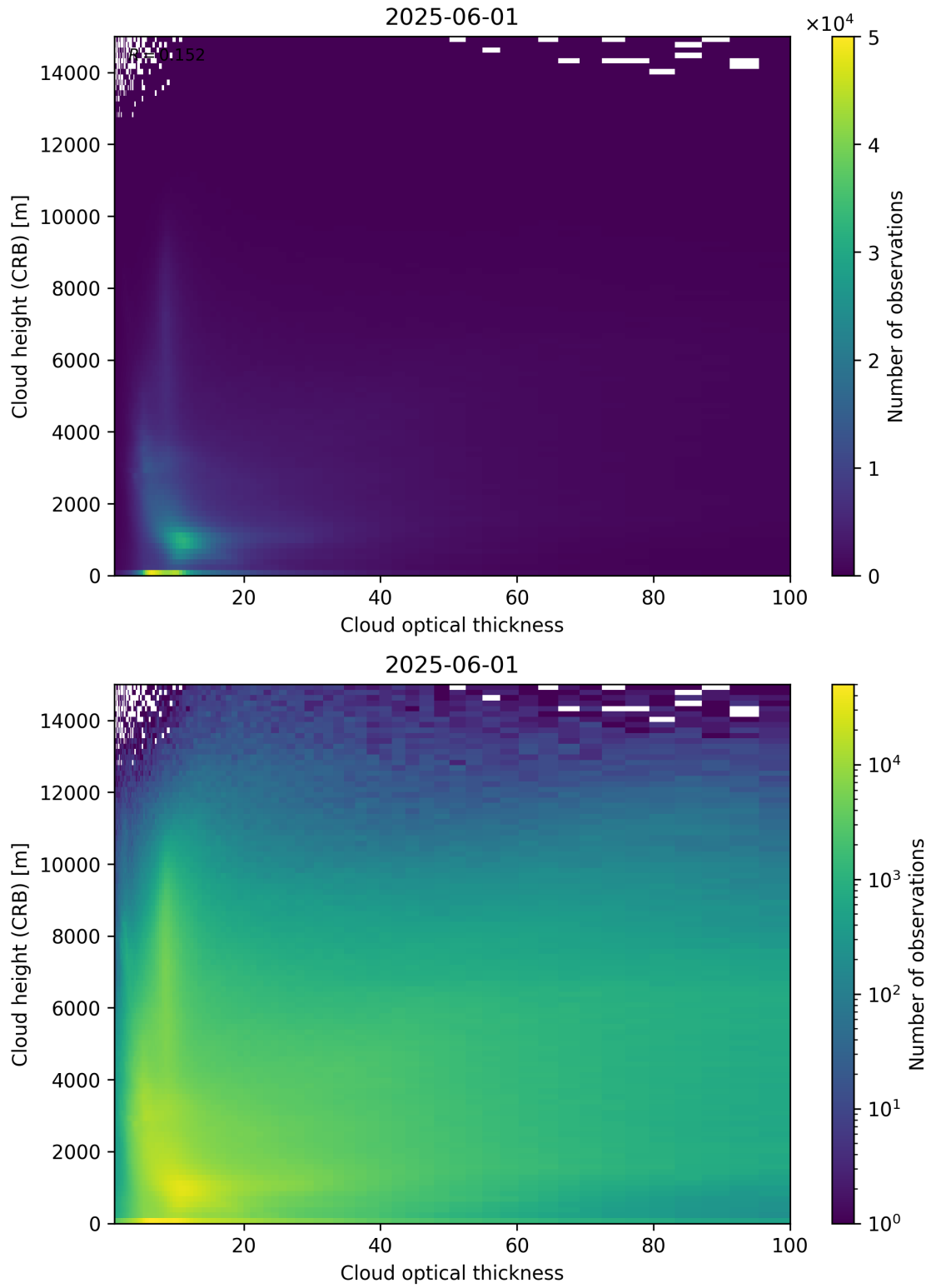
Figure 85: Scatter density plot of “Cloud optical thickness” against “Cloud height (CRB)” for 2025-06-01 to 2025-06-02.
