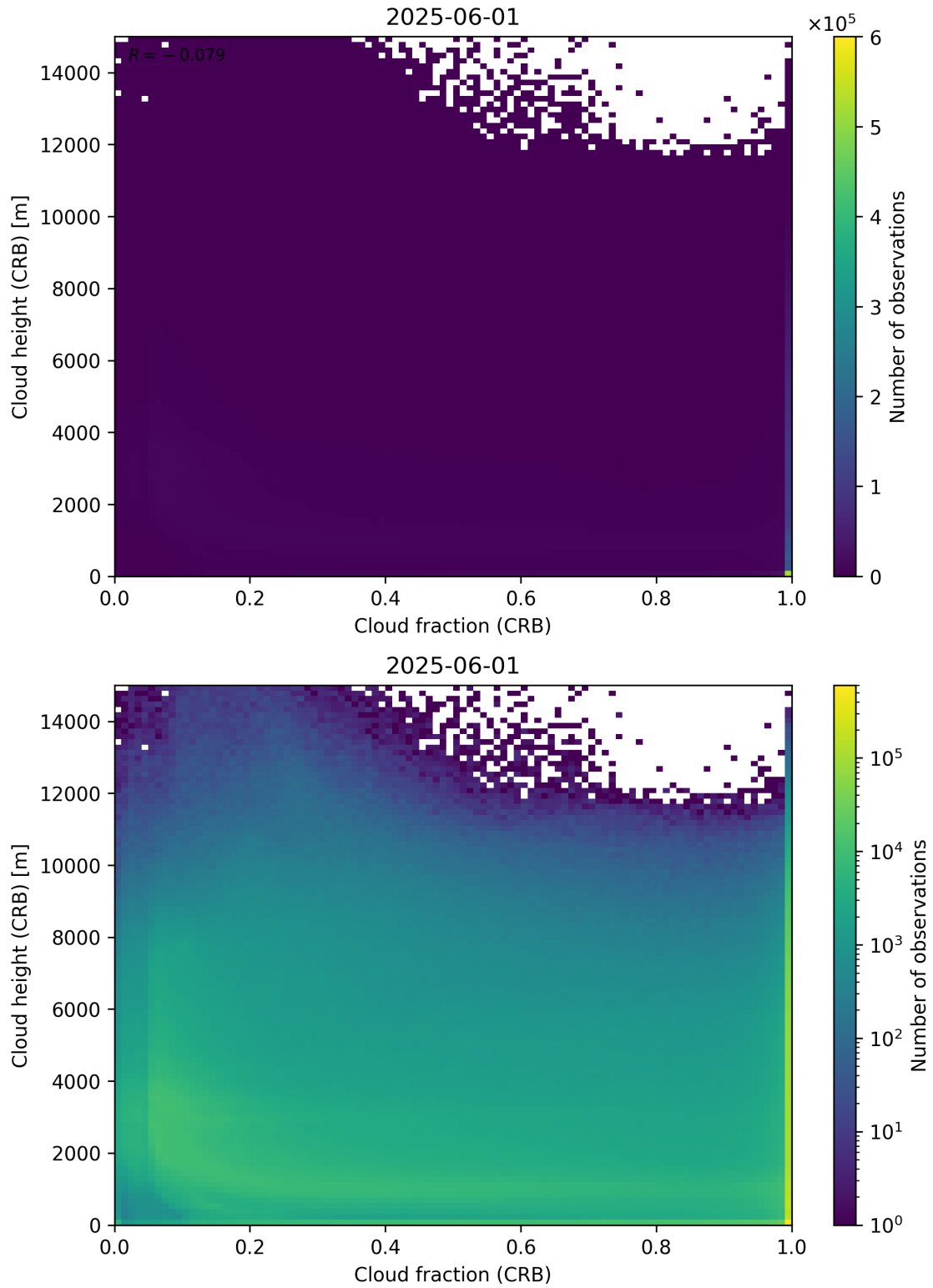
Figure 79: Scatter density plot of “Cloud fraction (CRB)” against “Cloud height (CRB)” for 2025-06-01 to 2025-06-02.
