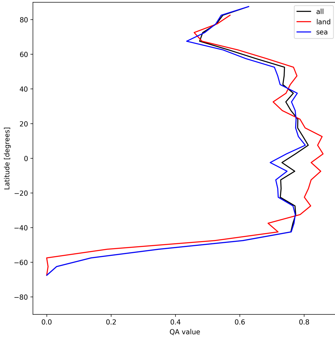
Figure 22: Zonal average of “QA value” for 2025-06-01 to 2025-06-02.
