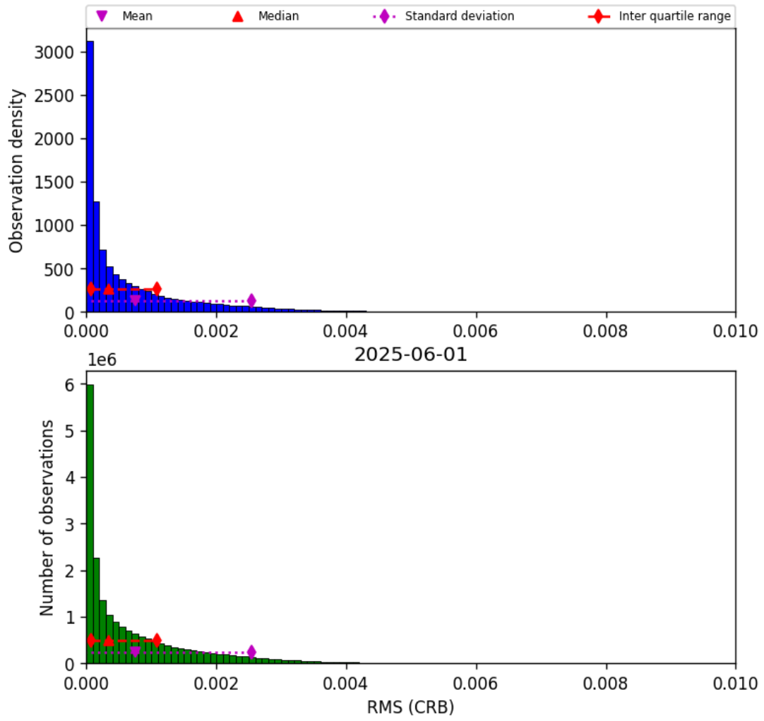
Figure 48: Histogram of “RMS (CRB)” for 2025-06-01 to 2025-06-02
