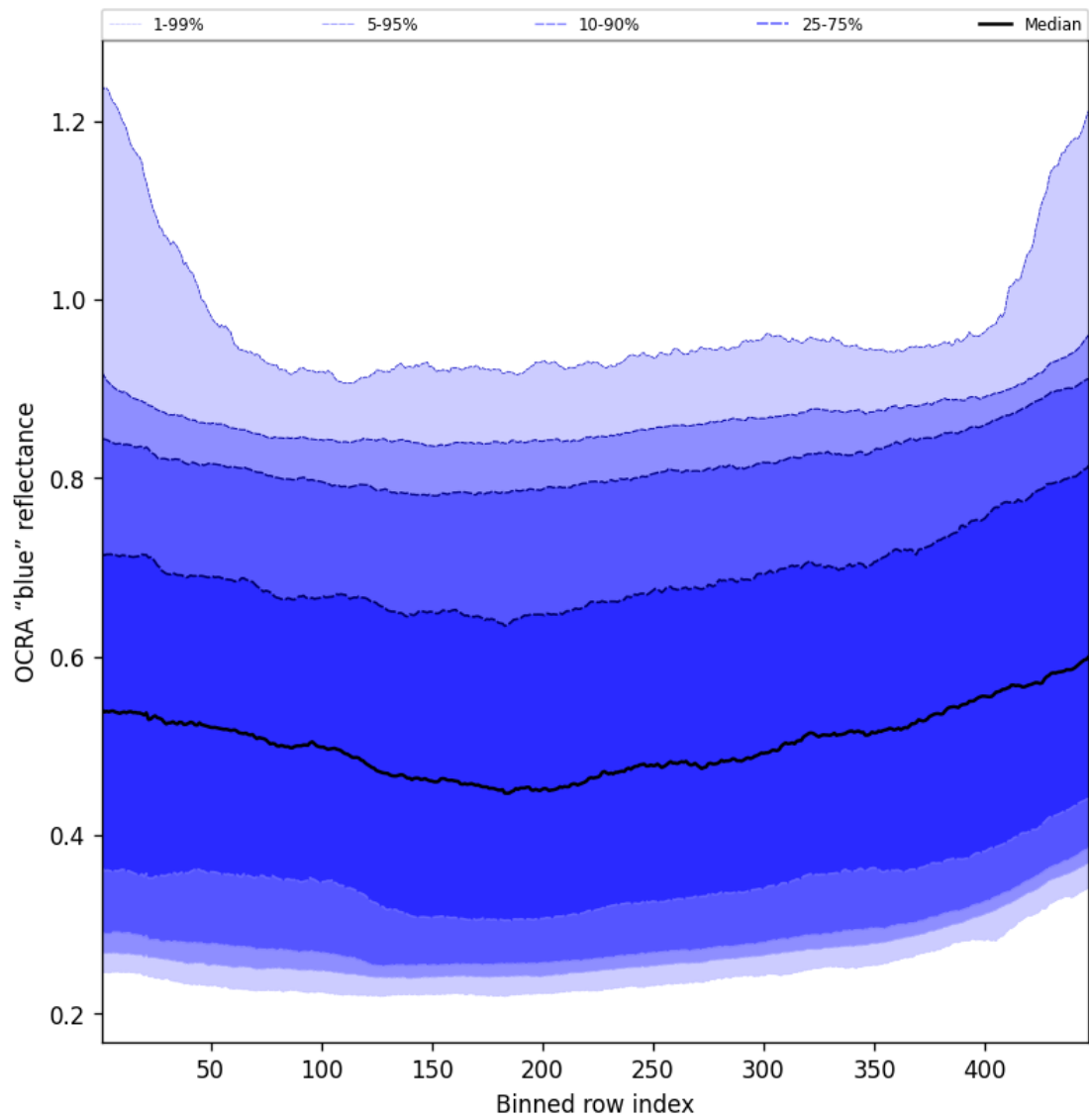
Figure 67: Along track statistics of “OCRA “blue” reflectance” for 2025-06-01 to 2025-06-02
