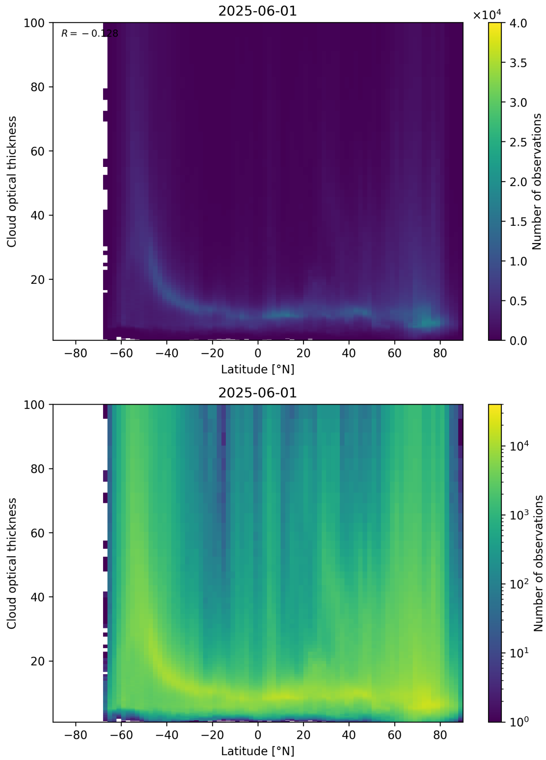
Figure 96: Scatter density plot of “Latitude” against “Cloud optical thickness” for 2025-06-01 to 2025-06-02.
