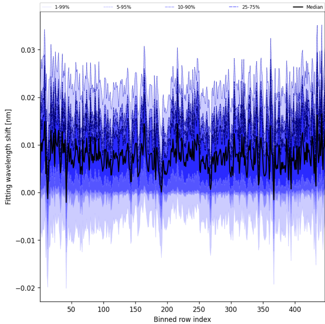
Figure 65: Along track statistics of “Fitting wavelength shift” for 2025-06-01 to 2025-06-02
