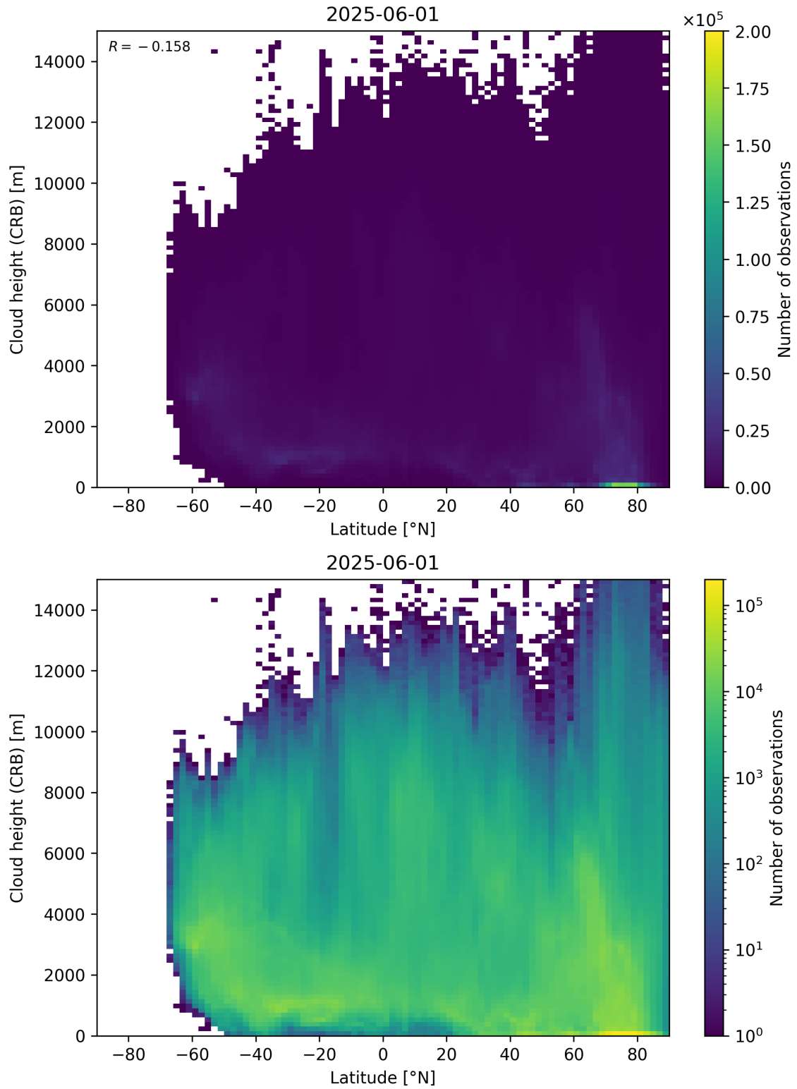
Figure 95: Scatter density plot of “Latitude” against “Cloud height (CRB)” for 2025-06-01 to 2025-06-02.
