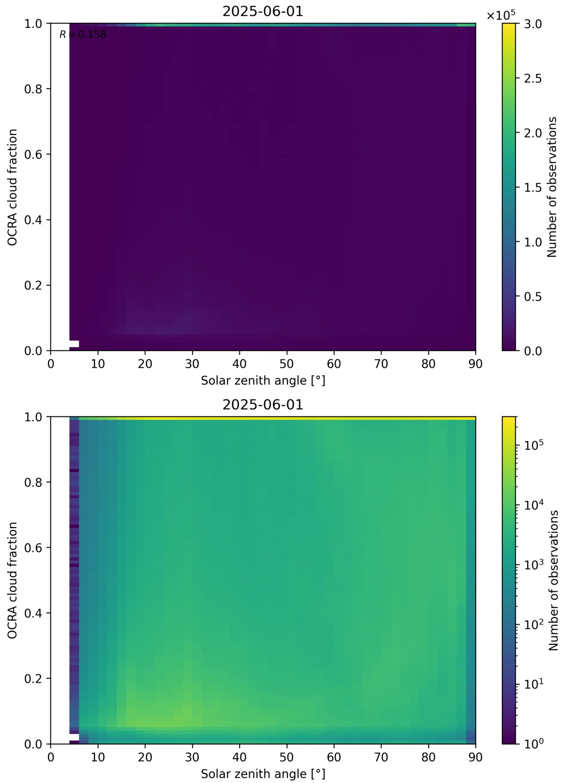
Figure 100: Scatter density plot of “Solar zenith angle” against “OCRA cloud fraction” for 2025-06-01 to 2025-06-02.
