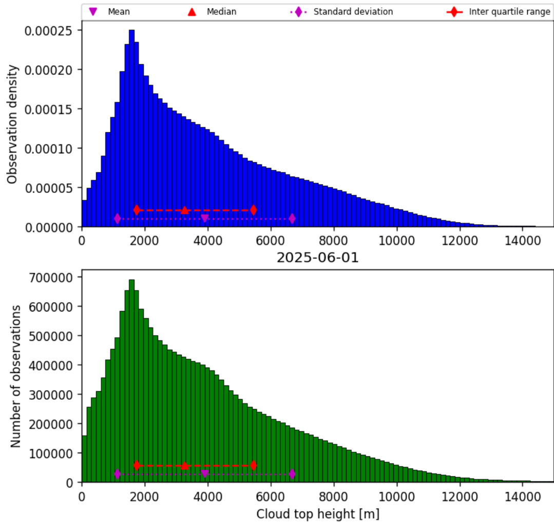
Figure 40: Histogram of “Cloud top height” for 2025-06-01 to 2025-06-02
