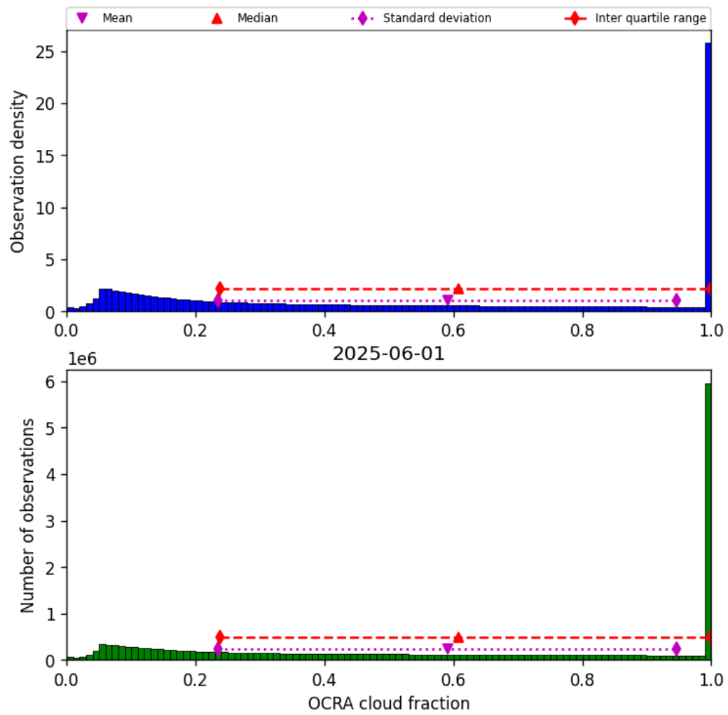
Figure 50: Histogram of “OCRA cloud fraction” for 2025-06-01 to 2025-06-02
