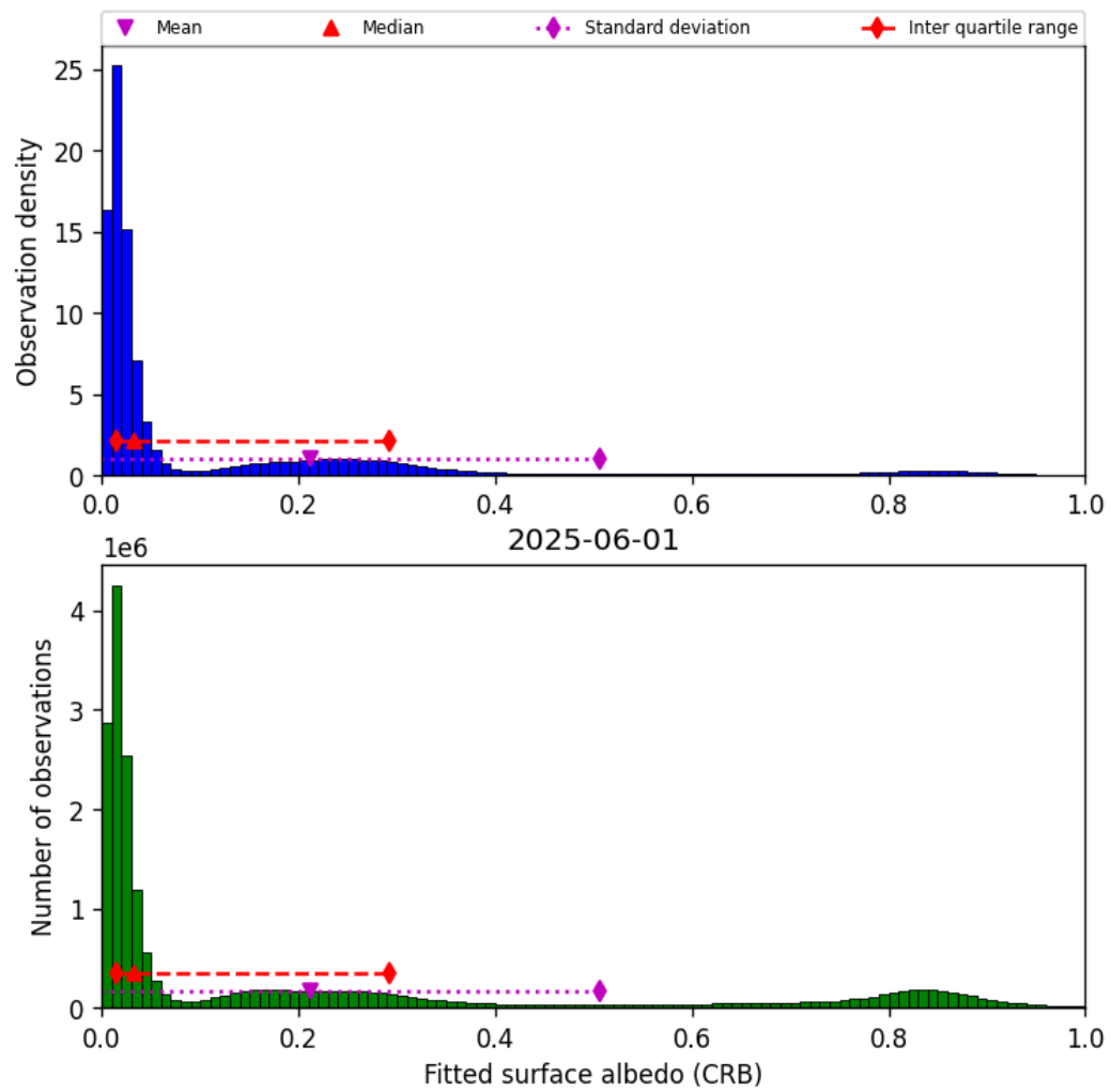
Figure 46: Histogram of “Fitted surface albedo (CRB)” for 2025-06-01 to 2025-06-02
