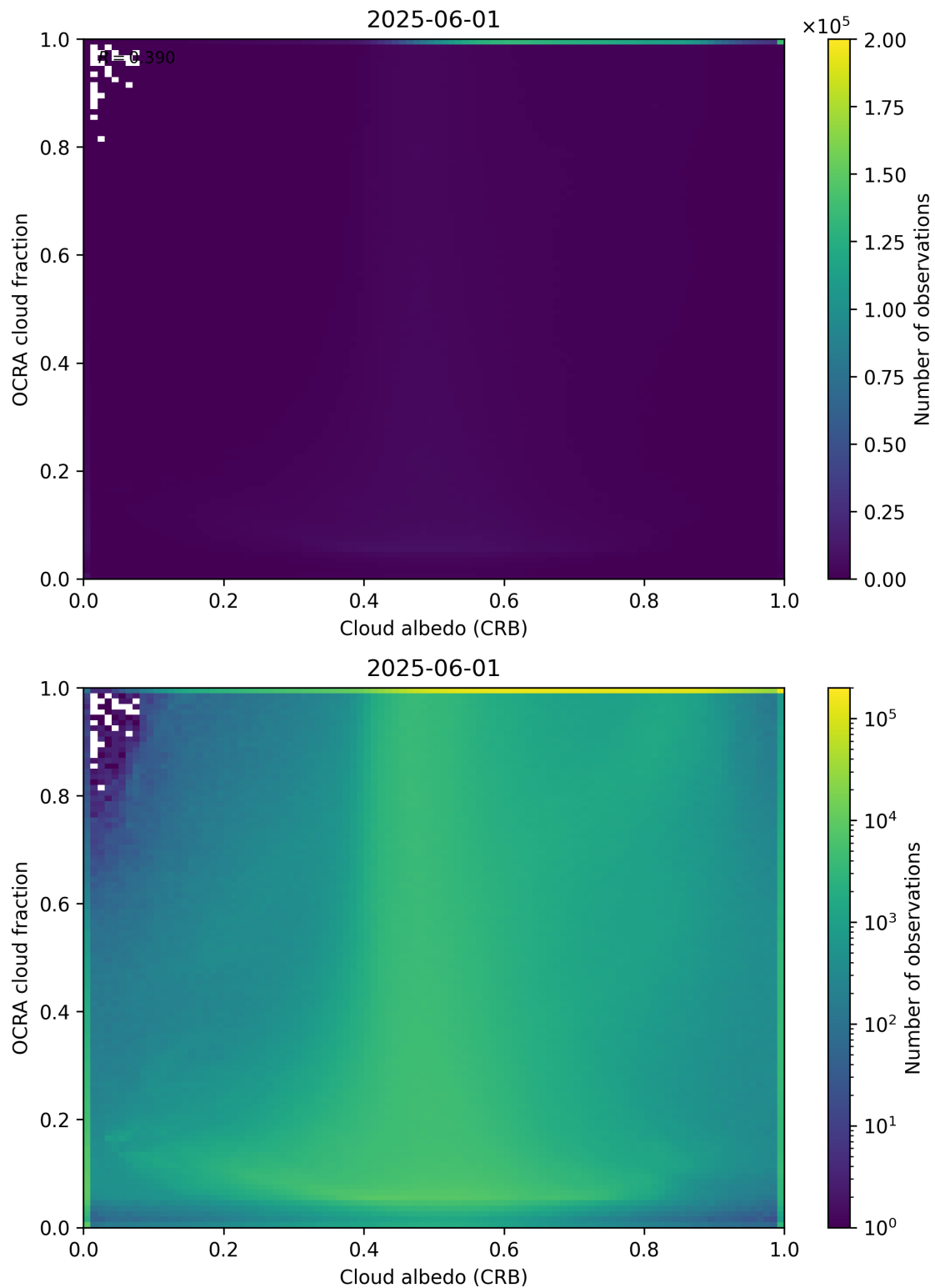
Figure 70: Scatter density plot of “Cloud albedo (CRB)” against “OCRA cloud fraction” for 2025-06-01 to 2025-06-02.
