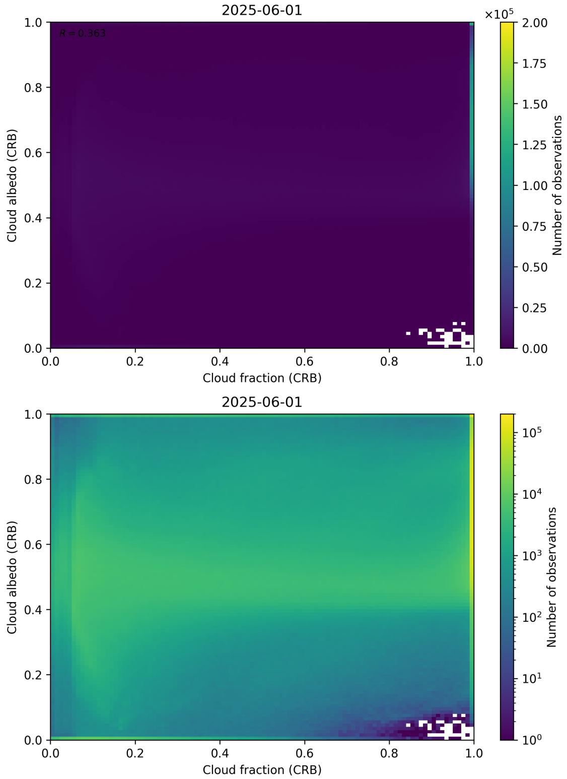
Figure 77: Scatter density plot of “Cloud fraction (CRB)” against “Cloud albedo (CRB)” for 2025-06-01 to 2025-06-02.
