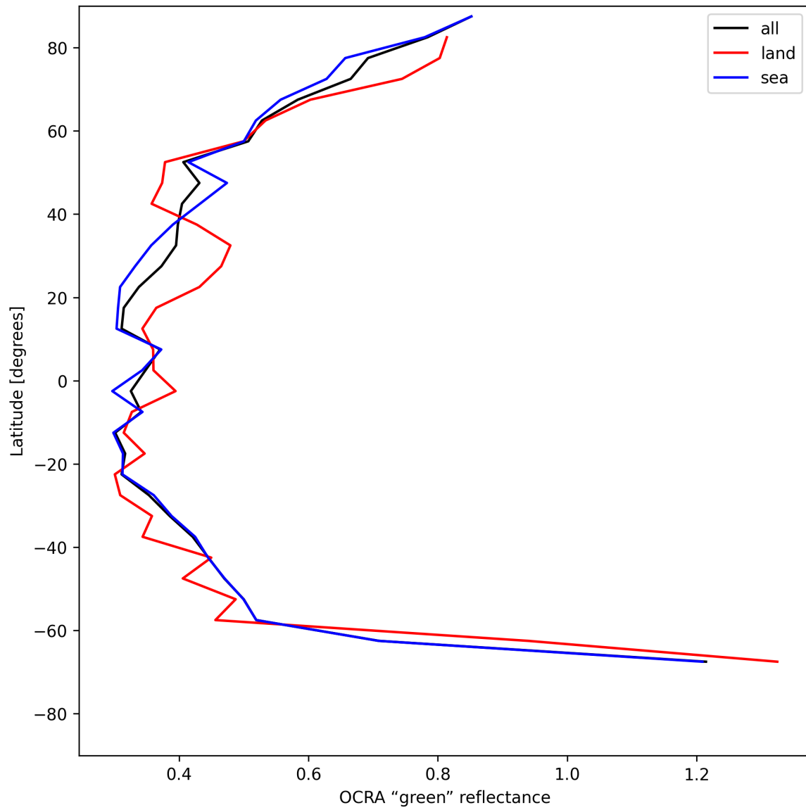
Figure 36: Zonal average of “OCRA “green” reflectance” for 2025-06-01 to 2025-06-02.
