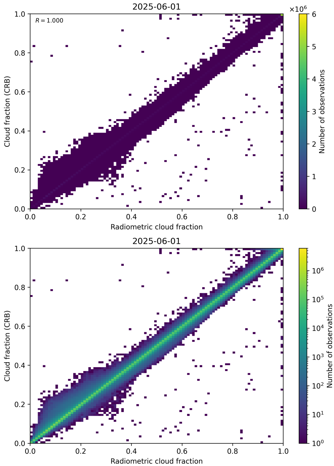
Figure 73: Scatter density plot of “Radiometric cloud fraction” against “Cloud fraction (CRB)” for 2025-06-01 to 2025-06-02.
