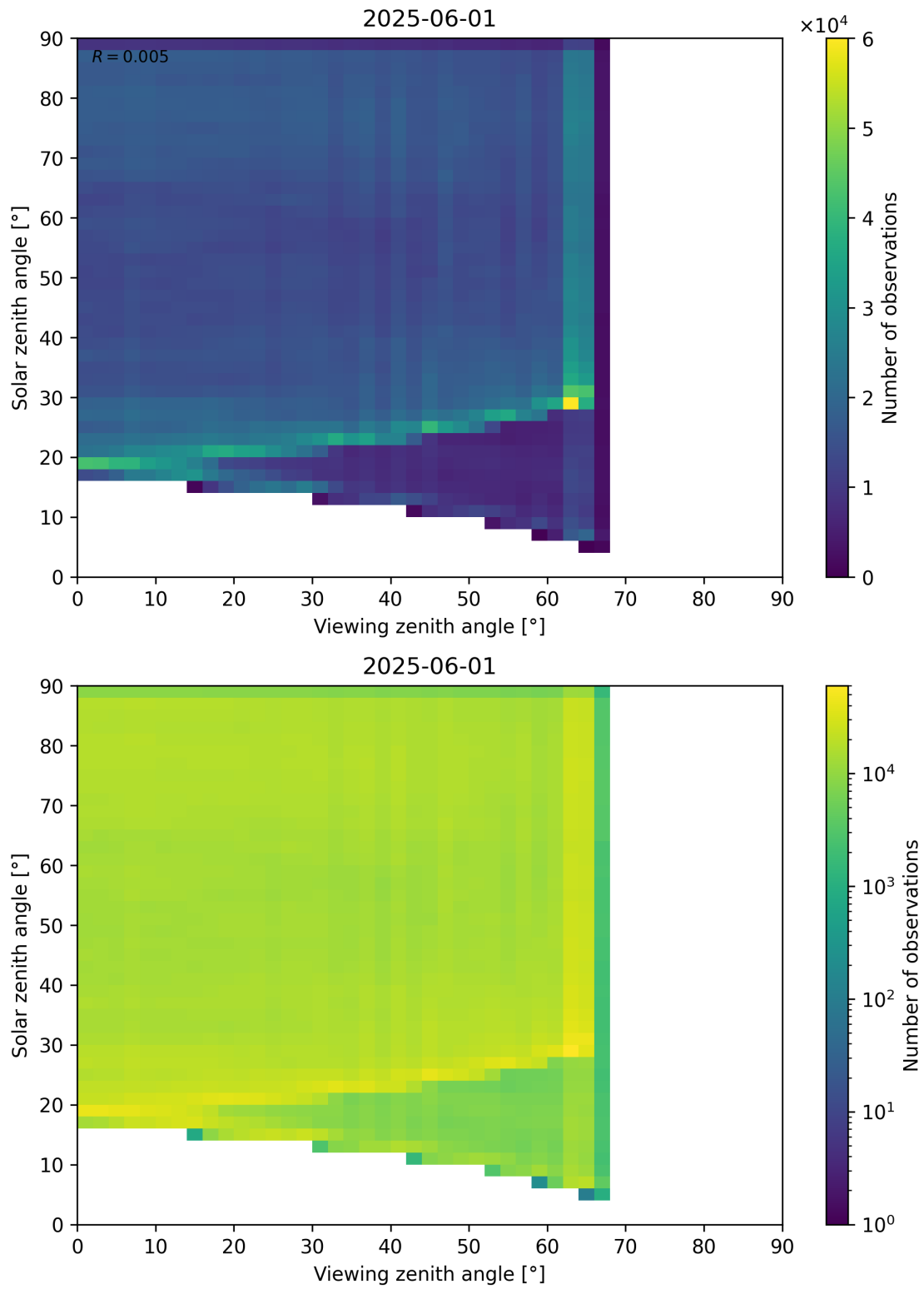
Figure 114: Scatter density plot of “Viewing zenith angle” against “Solar zenith angle” for 2025-06-01 to 2025-06-02.
