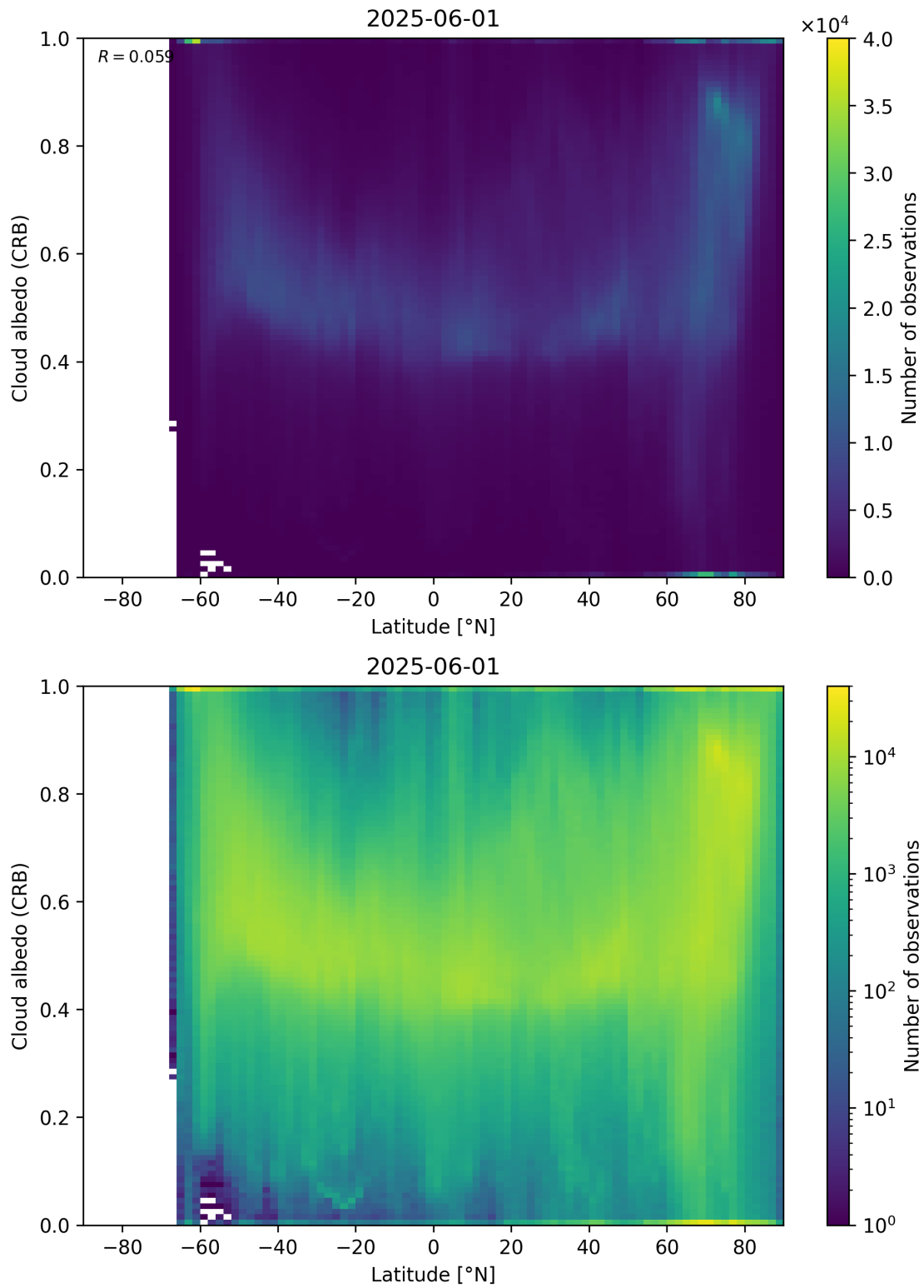
Figure 91: Scatter density plot of “Latitude” against “Cloud albedo (CRB)” for 2025-06-01 to 2025-06-02.
