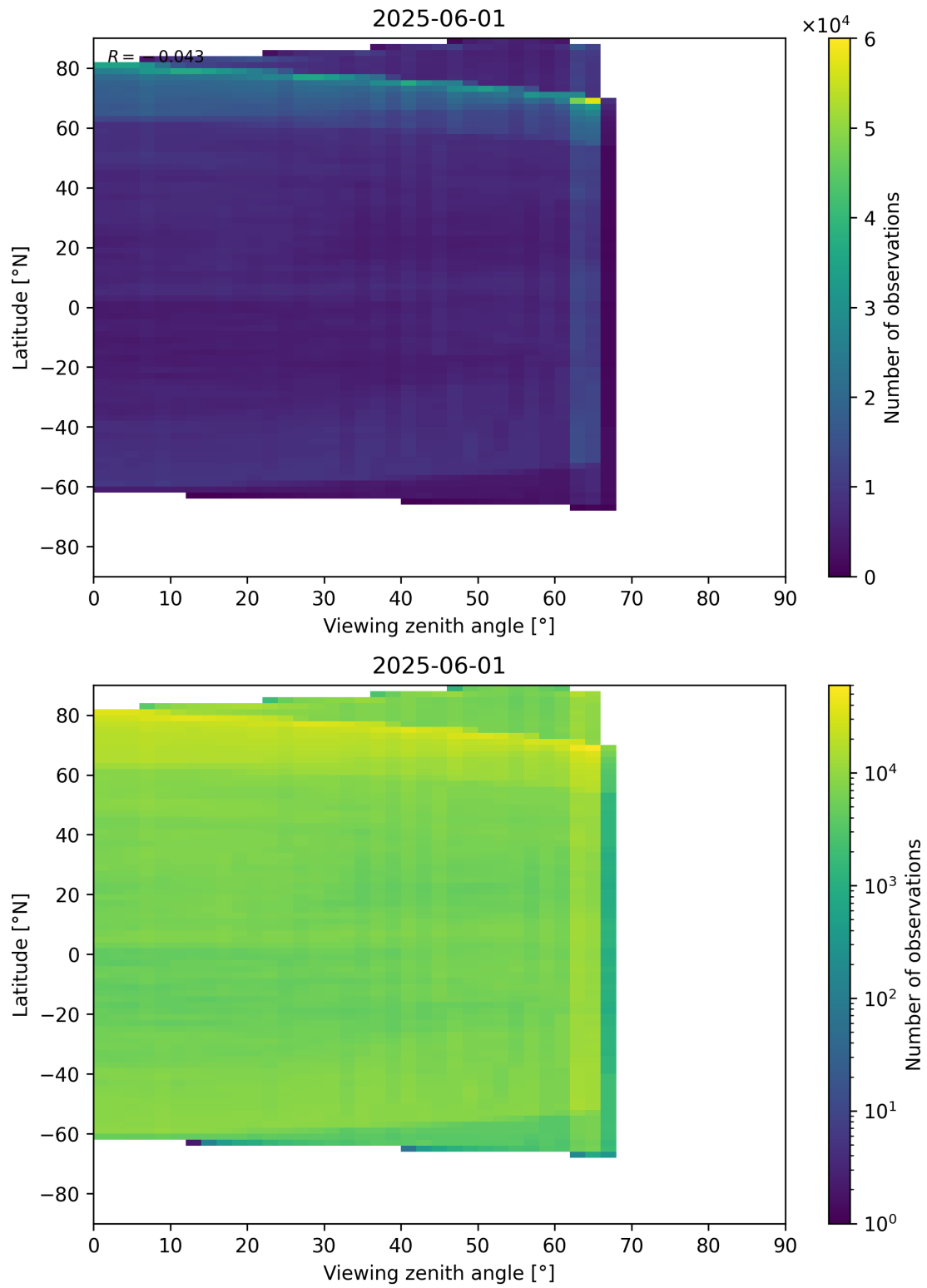
Figure 113: Scatter density plot of “Viewing zenith angle” against “Latitude” for 2025-06-01 to 2025-06-02.
