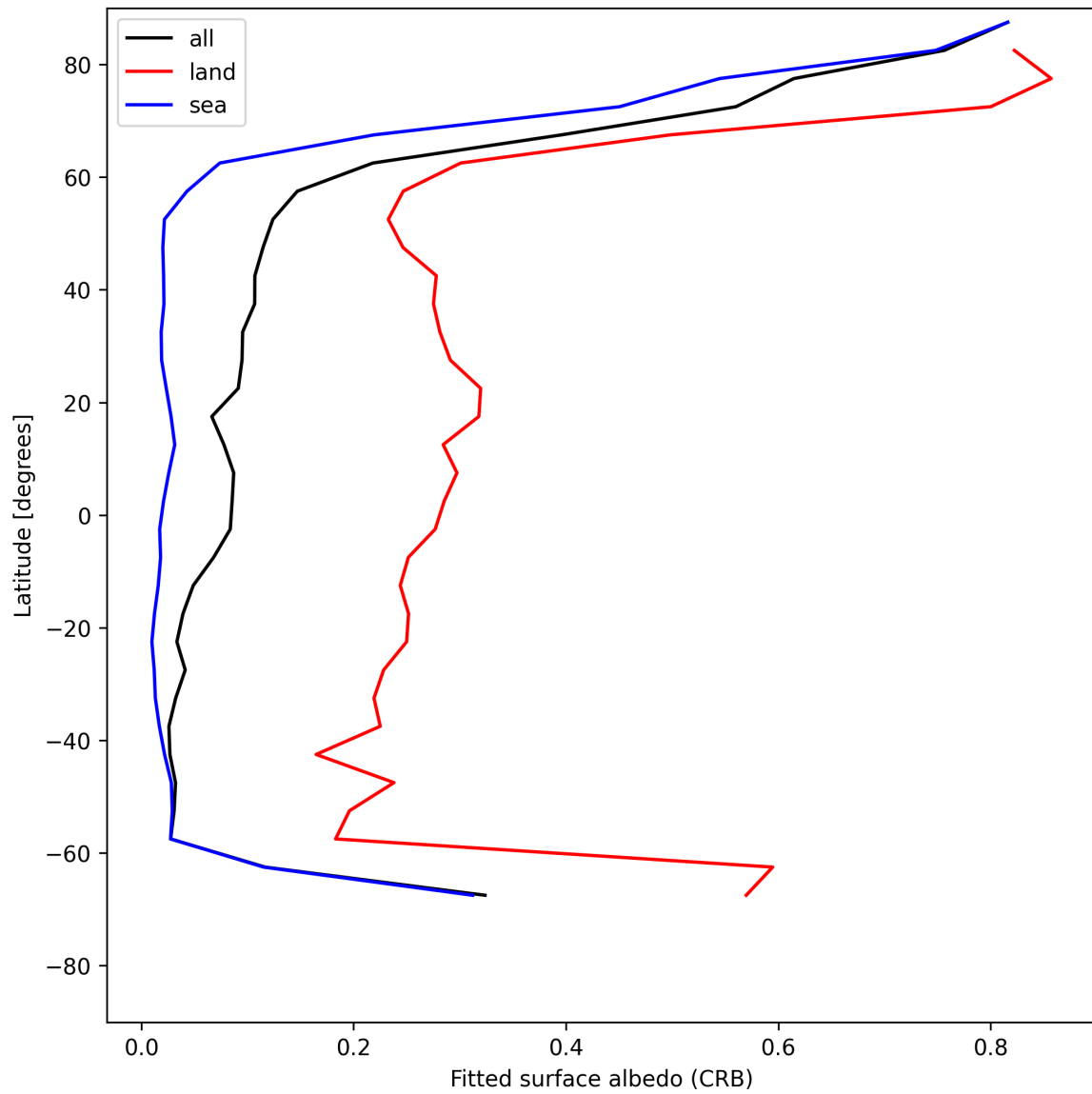
Figure 30: Zonal average of “Fitted surface albedo (CRB)” for 2025-06-01 to 2025-06-02.
