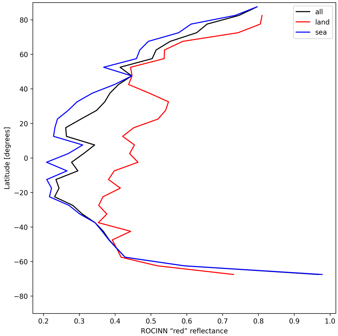
Figure 37: Zonal average of “ROCINN “red” reflectance” for 2025-06-01 to 2025-06-02.
