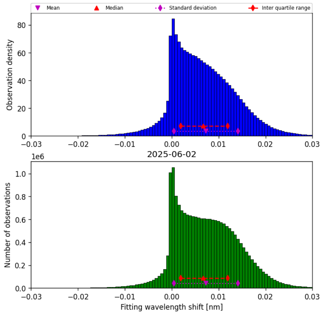
Figure 49: Histogram of “Fitting wavelength shift” for 2025-06-01 to 2025-06-03
