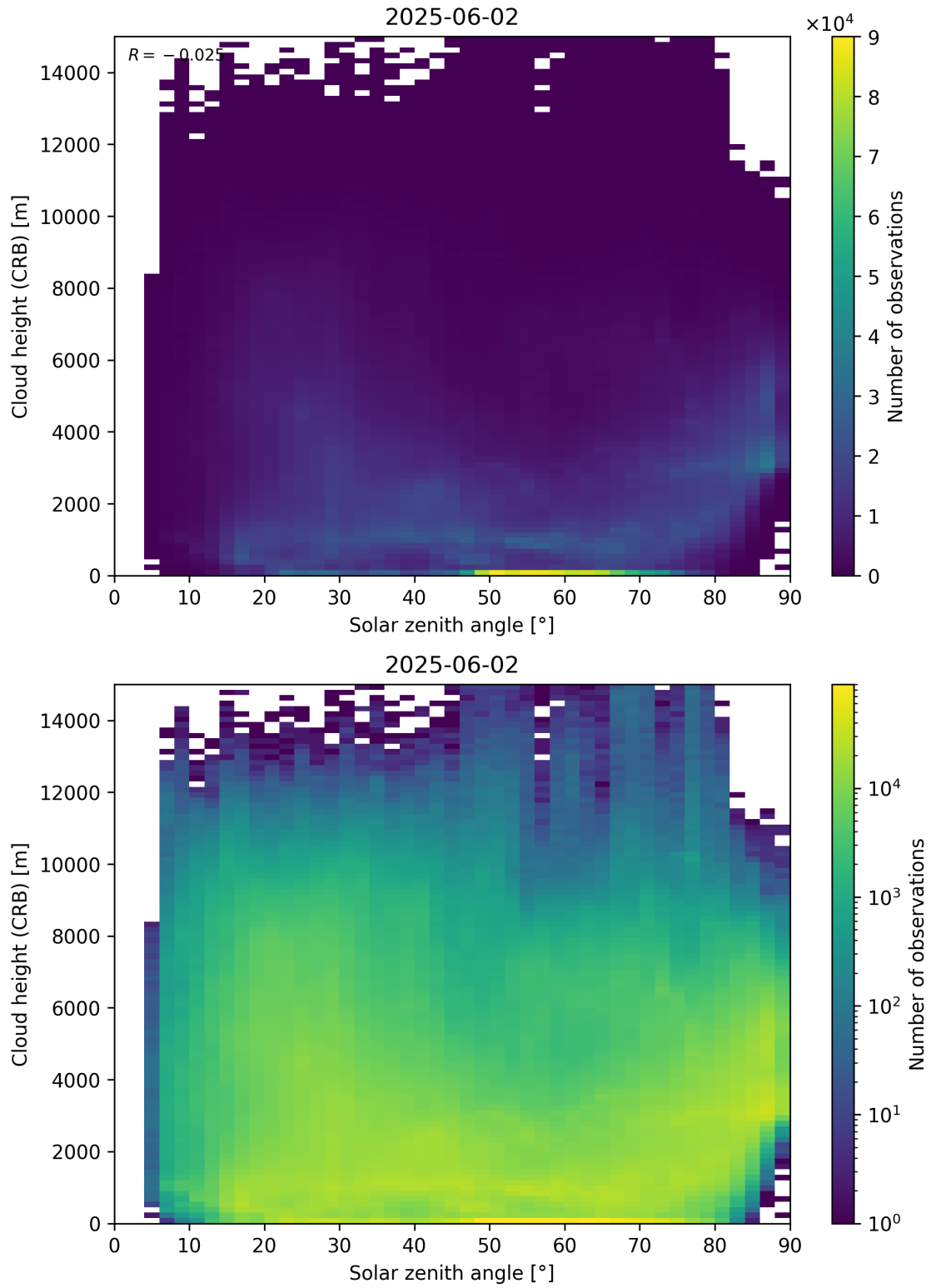
Figure 102: Scatter density plot of “Solar zenith angle” against “Cloud height (CRB)” for 2025-06-01 to 2025-06-03.
