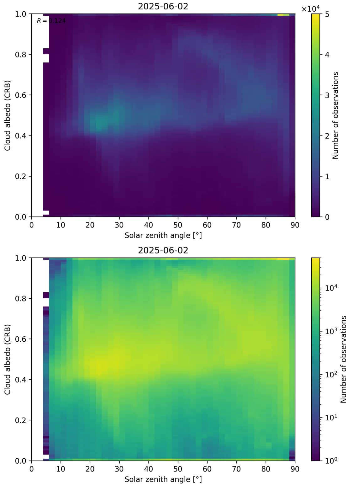
Figure 98: Scatter density plot of “Solar zenith angle” against “Cloud albedo (CRB)” for 2025-06-01 to 2025-06-03.
