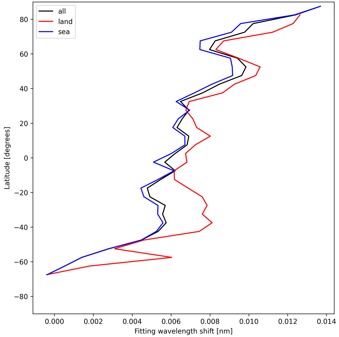
Figure 33: Zonal average of “Fitting wavelength shift” for 2025-06-01 to 2025-06-03.
