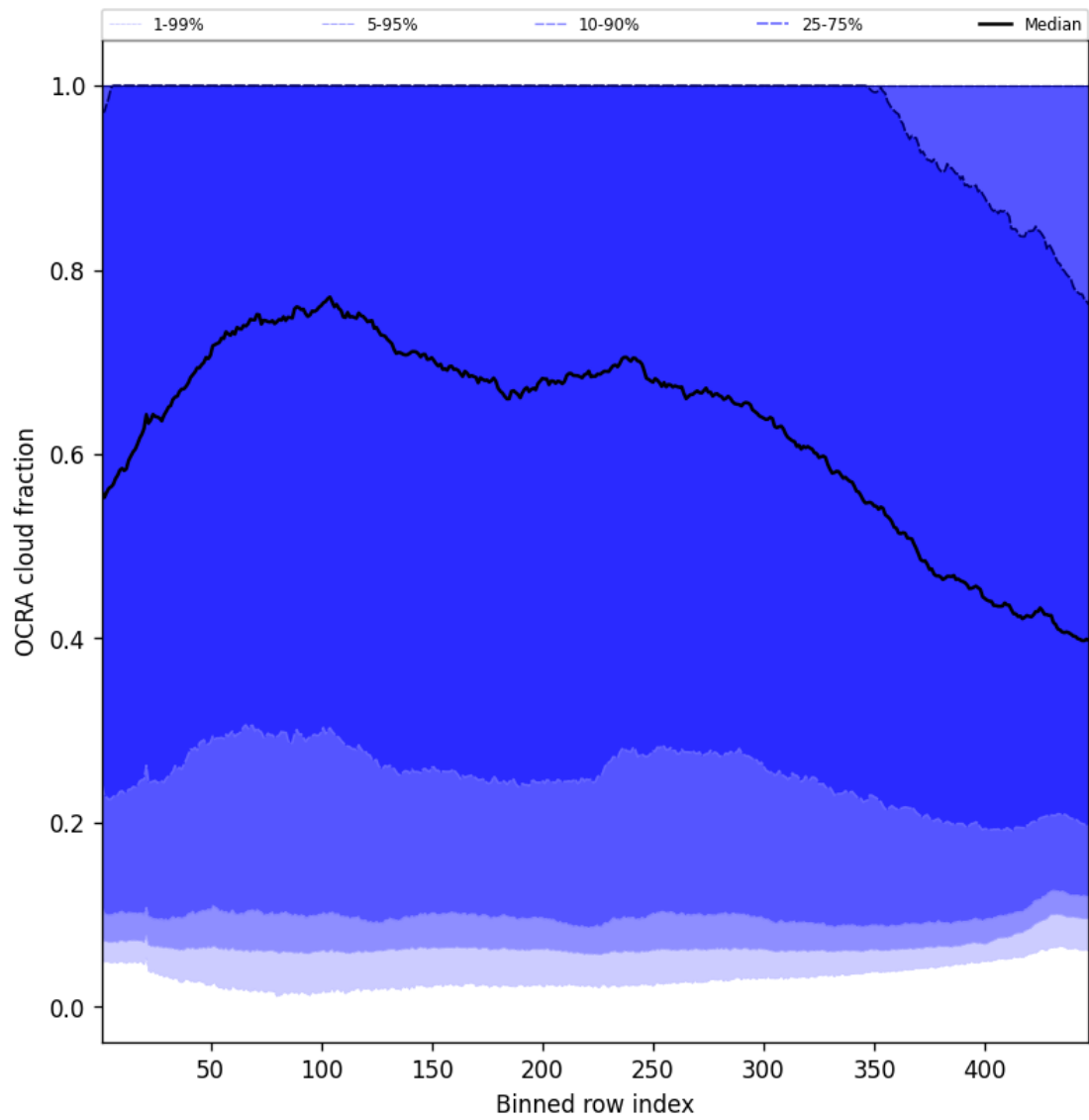
Figure 66: Along track statistics of “OCRA cloud fraction” for 2025-06-01 to 2025-06-03
