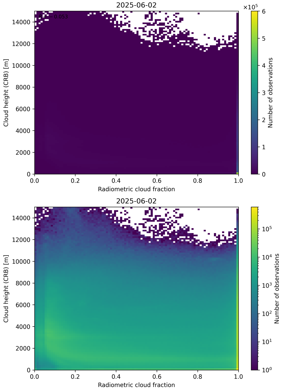
Figure 74: Scatter density plot of “Radiometric cloud fraction” against “Cloud height (CRB)” for 2025-06-01 to 2025-06-03.
