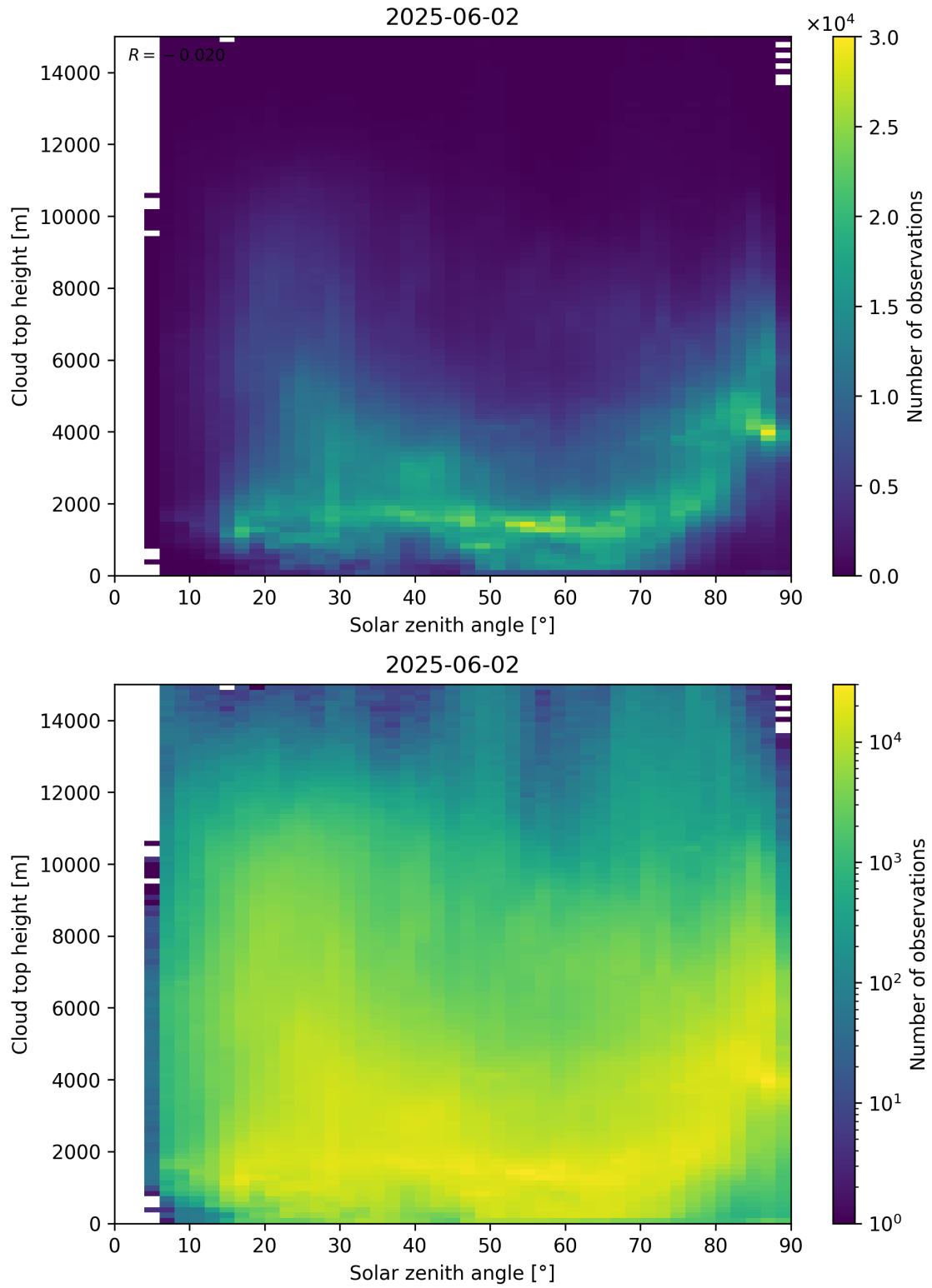
Figure 104: Scatter density plot of “Solar zenith angle” against “Cloud top height” for 2025-06-01 to 2025-06-03.
