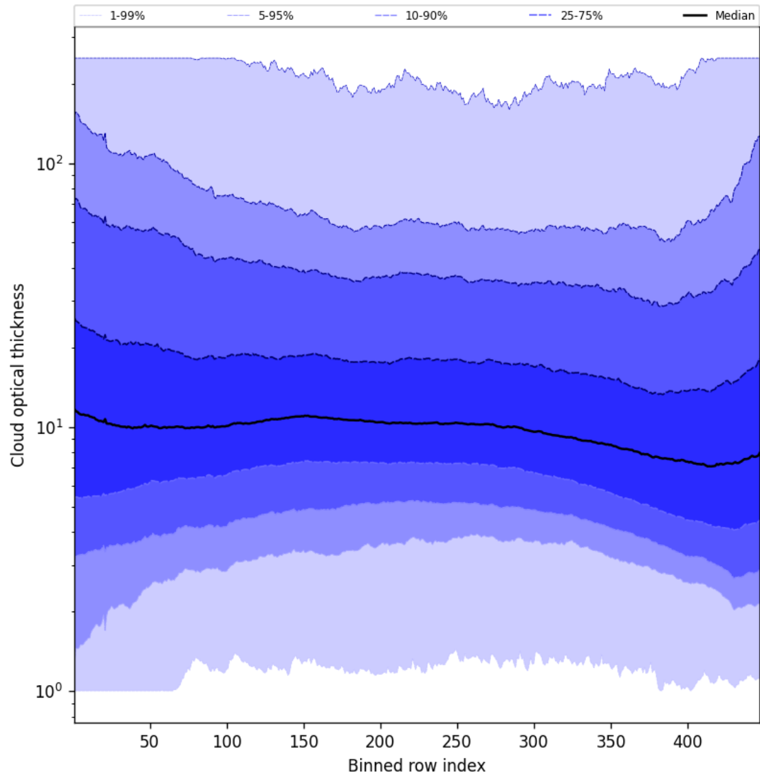
Figure 57: Along track statistics of “Cloud optical thickness” for 2025-06-01 to 2025-06-03
