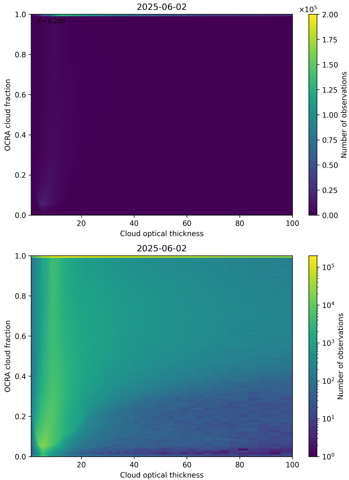
Figure 83: Scatter density plot of “Cloud optical thickness” against “OCRA cloud fraction” for 2025-06-01 to 2025-06-03.
