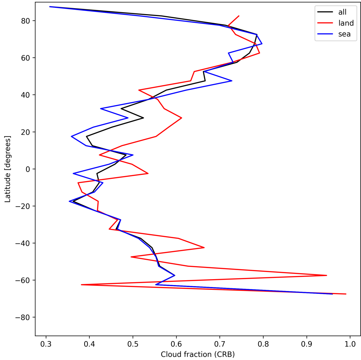
Figure 26: Zonal average of “Cloud fraction (CRB)” for 2025-06-01 to 2025-06-03.
