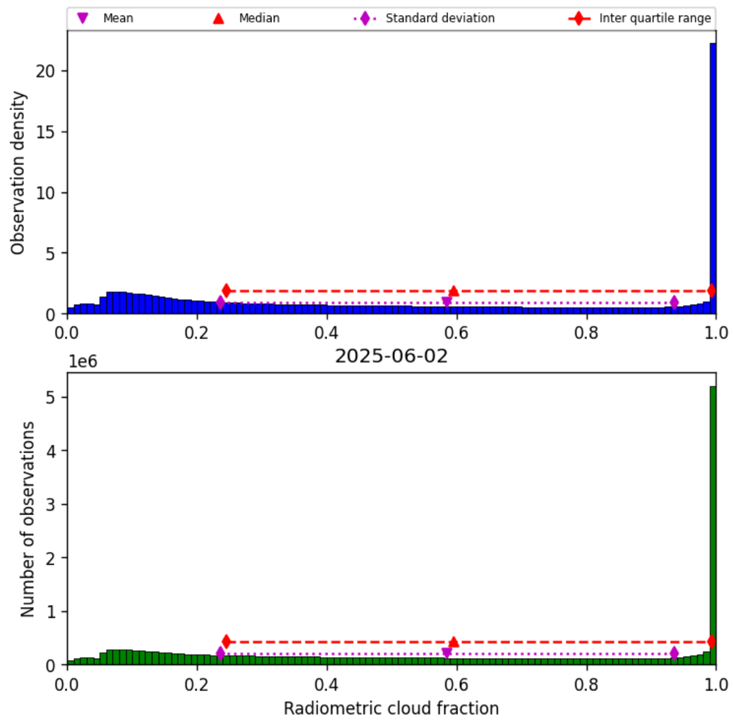
Figure 39: Histogram of “Radiometric cloud fraction” for 2025-06-01 to 2025-06-03
