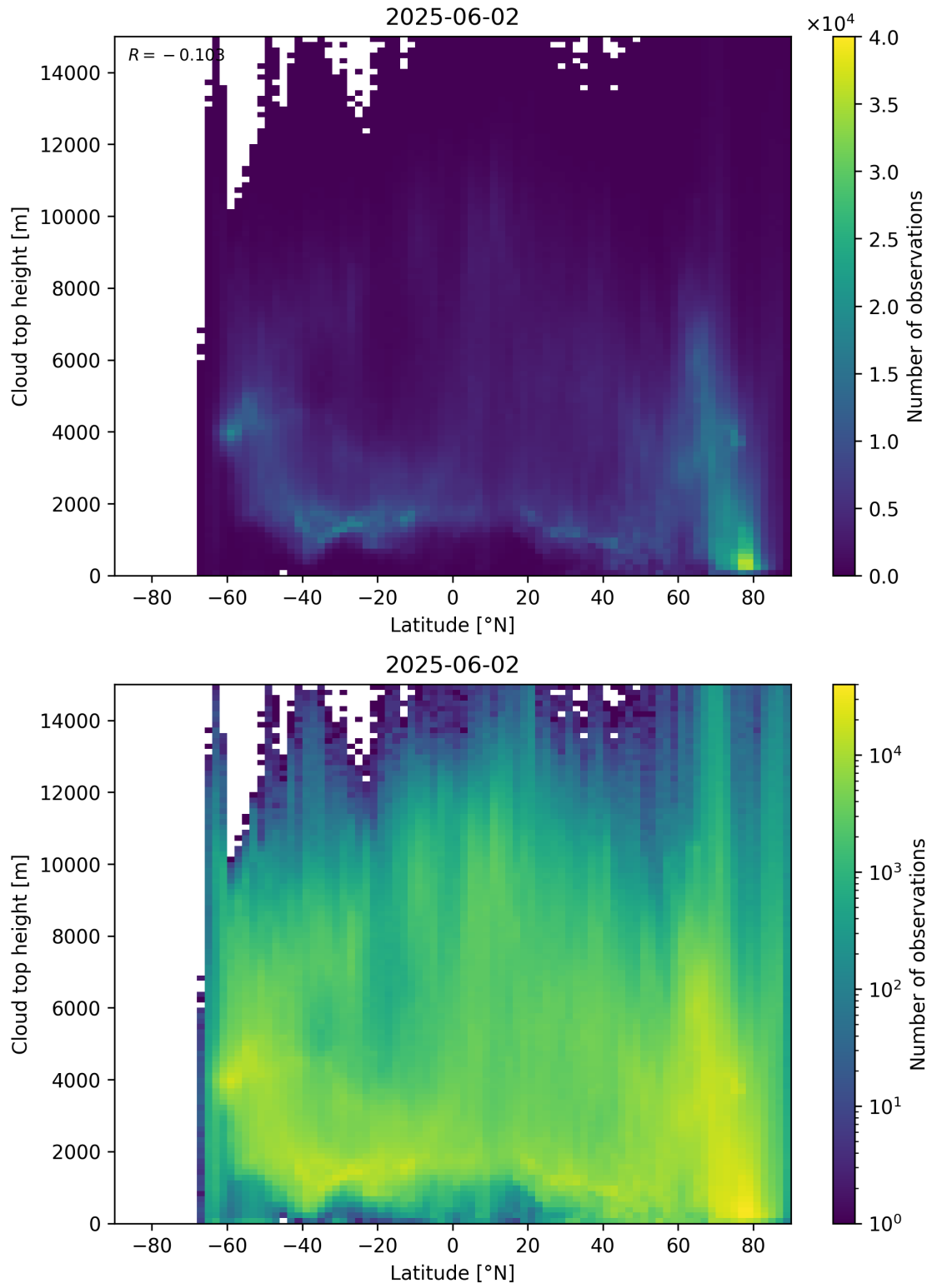
Figure 97: Scatter density plot of “Latitude” against “Cloud top height” for 2025-06-01 to 2025-06-03.
