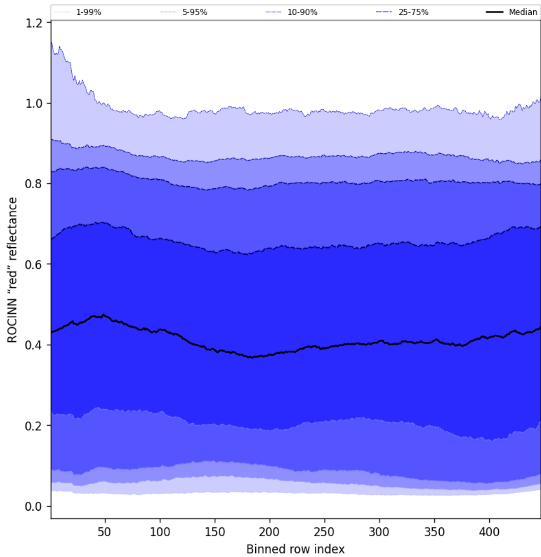
Figure 69: Along track statistics of “ROCINN “red” reflectance” for 2025-06-01 to 2025-06-03
