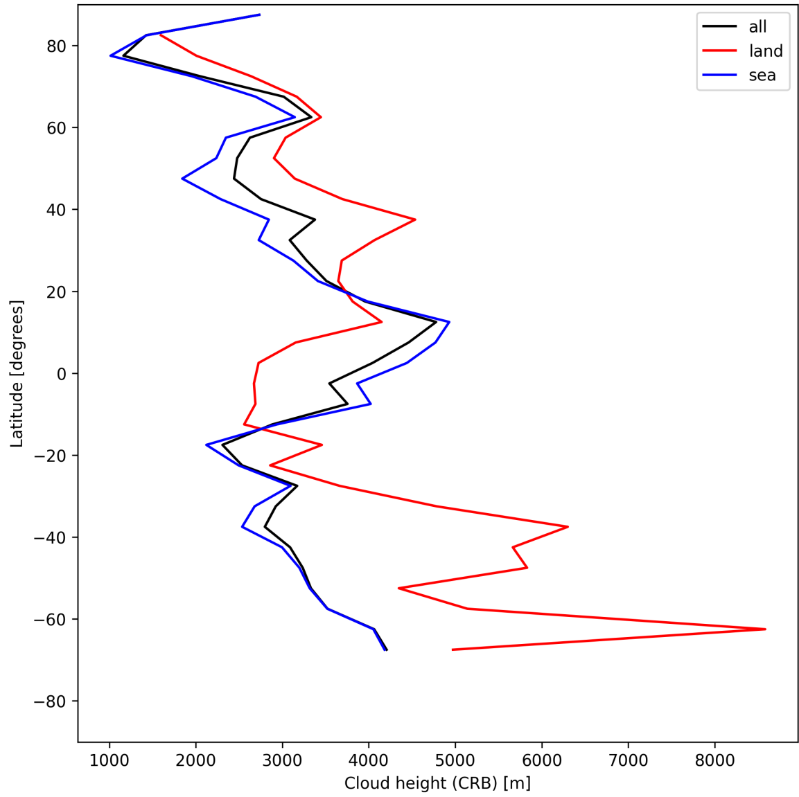
Figure 27: Zonal average of “Cloud height (CRB)” for 2025-06-01 to 2025-06-03.
