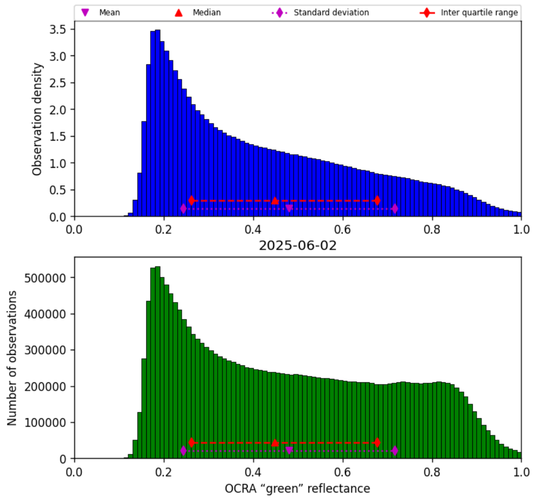
Figure 52: Histogram of “OCRA “green” reflectance” for 2025-06-01 to 2025-06-03
