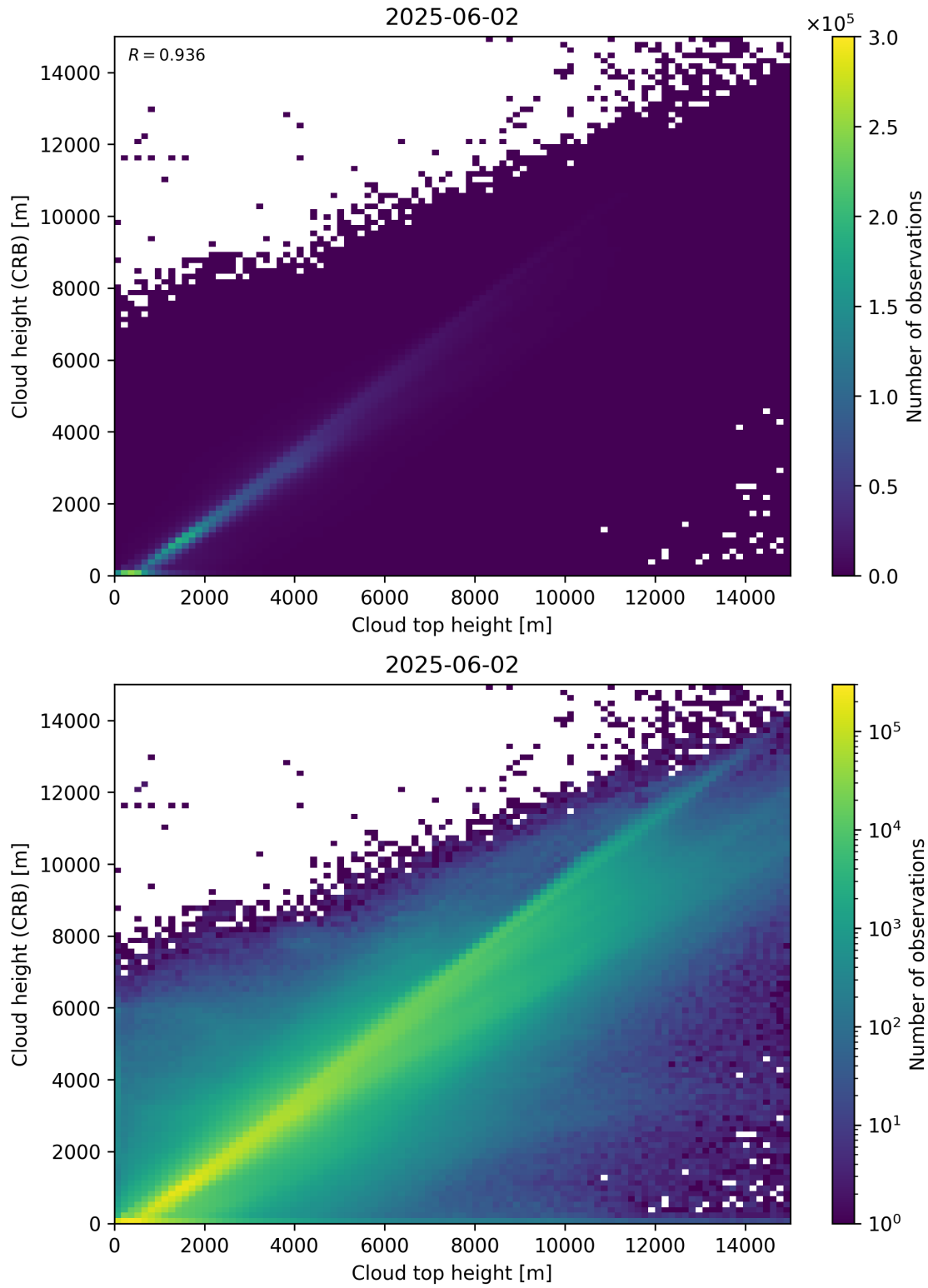
Figure 89: Scatter density plot of “Cloud top height” against “Cloud height (CRB)” for 2025-06-01 to 2025-06-03.
