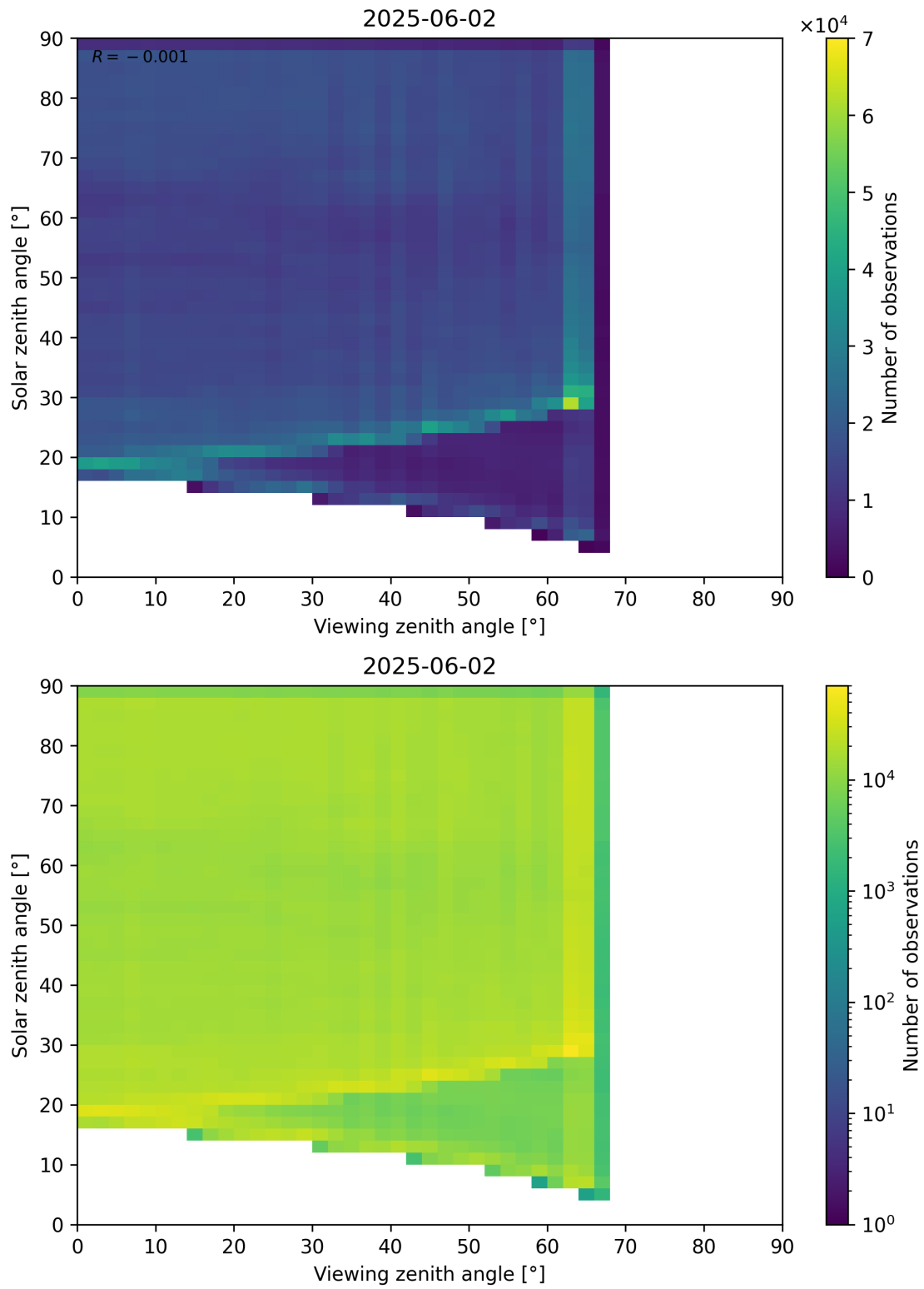
Figure 114: Scatter density plot of “Viewing zenith angle” against “Solar zenith angle” for 2025-06-01 to 2025-06-03.
