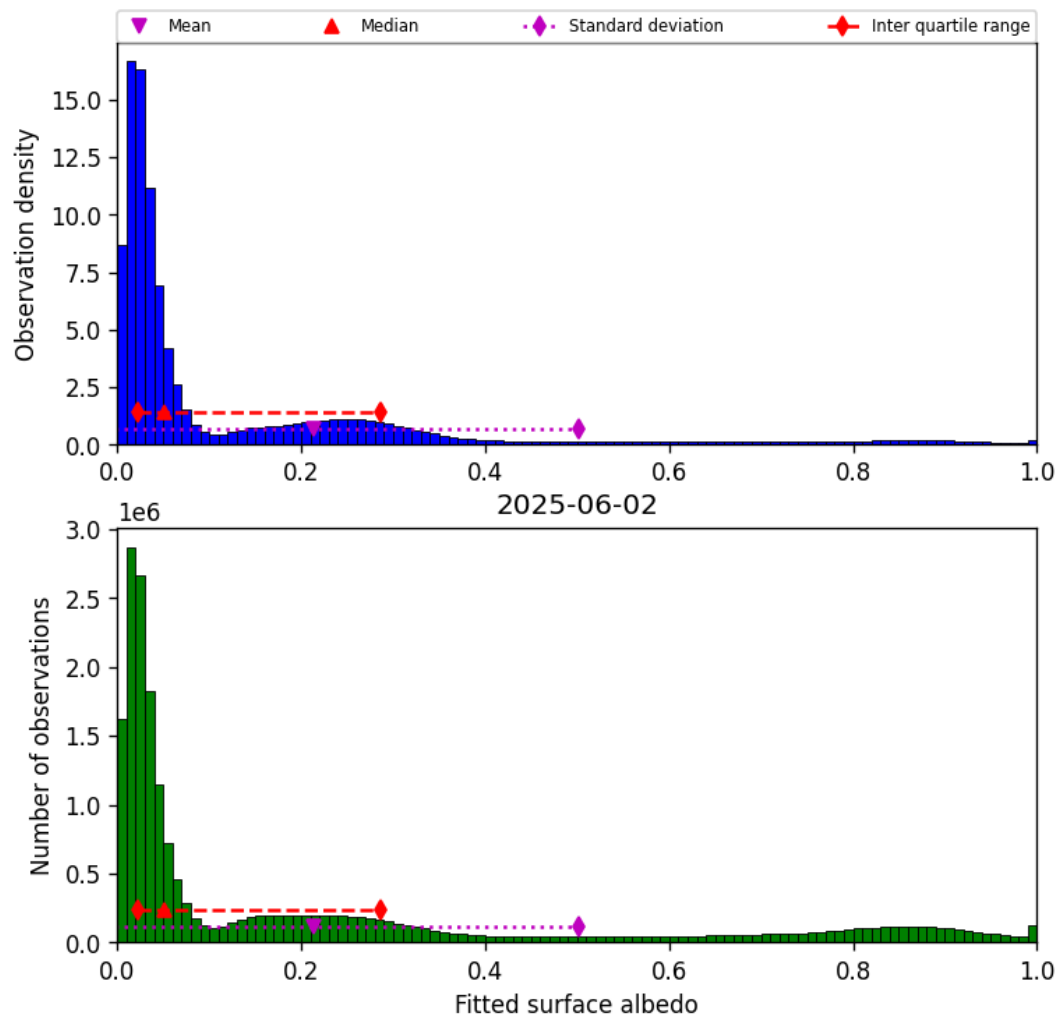
Figure 45: Histogram of “Fitted surface albedo” for 2025-06-01 to 2025-06-03
