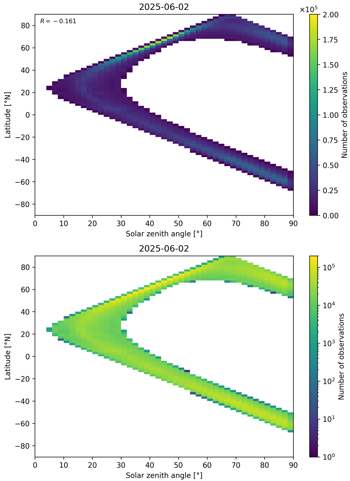
Figure 105: Scatter density plot of “Solar zenith angle” against “Latitude” for 2025-06-01 to 2025-06-03.
