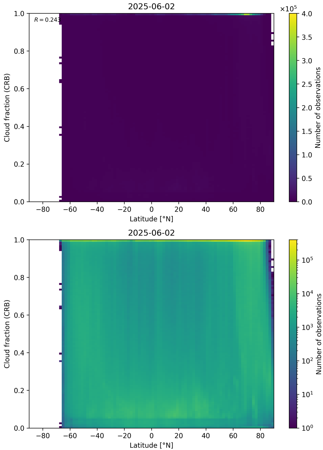
Figure 94: Scatter density plot of “Latitude” against “Cloud fraction (CRB)” for 2025-06-01 to 2025-06-03.
