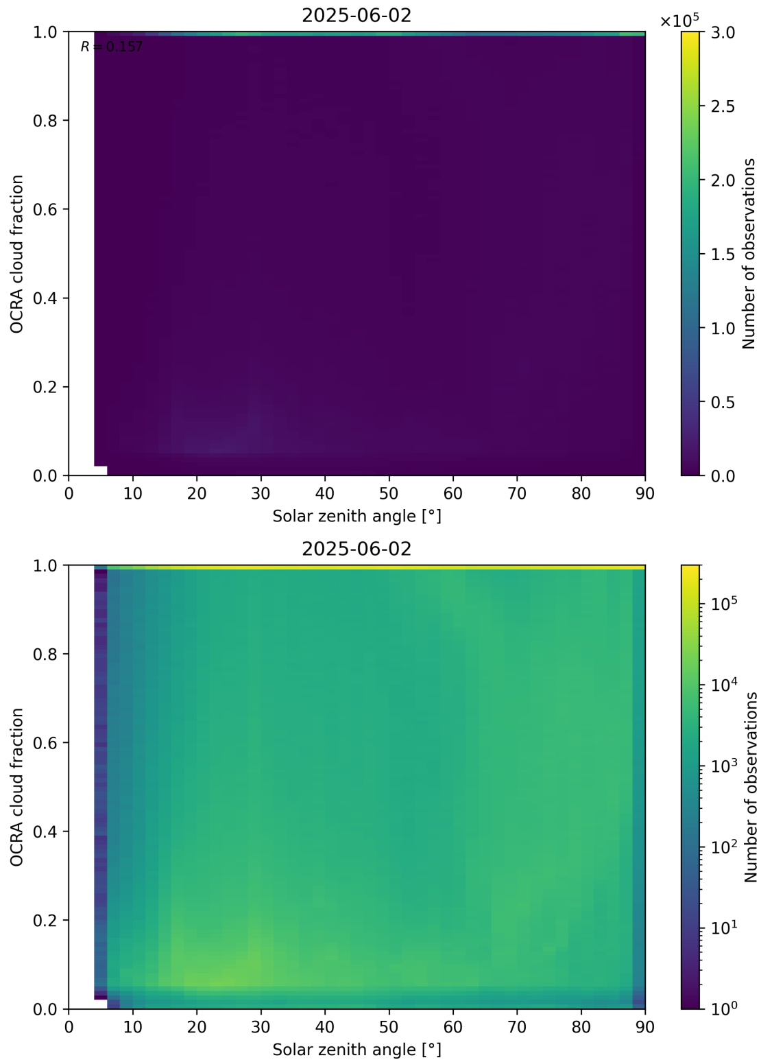
Figure 100: Scatter density plot of “Solar zenith angle” against “OCRA cloud fraction” for 2025-06-01 to 2025-06-03.
