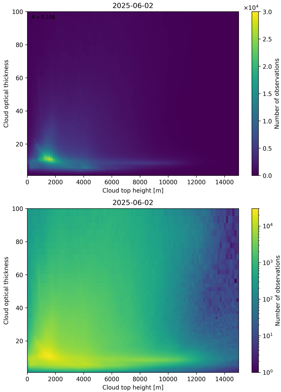
Figure 90: Scatter density plot of “Cloud top height” against “Cloud optical thickness” for 2025-06-01 to 2025-06-03.
