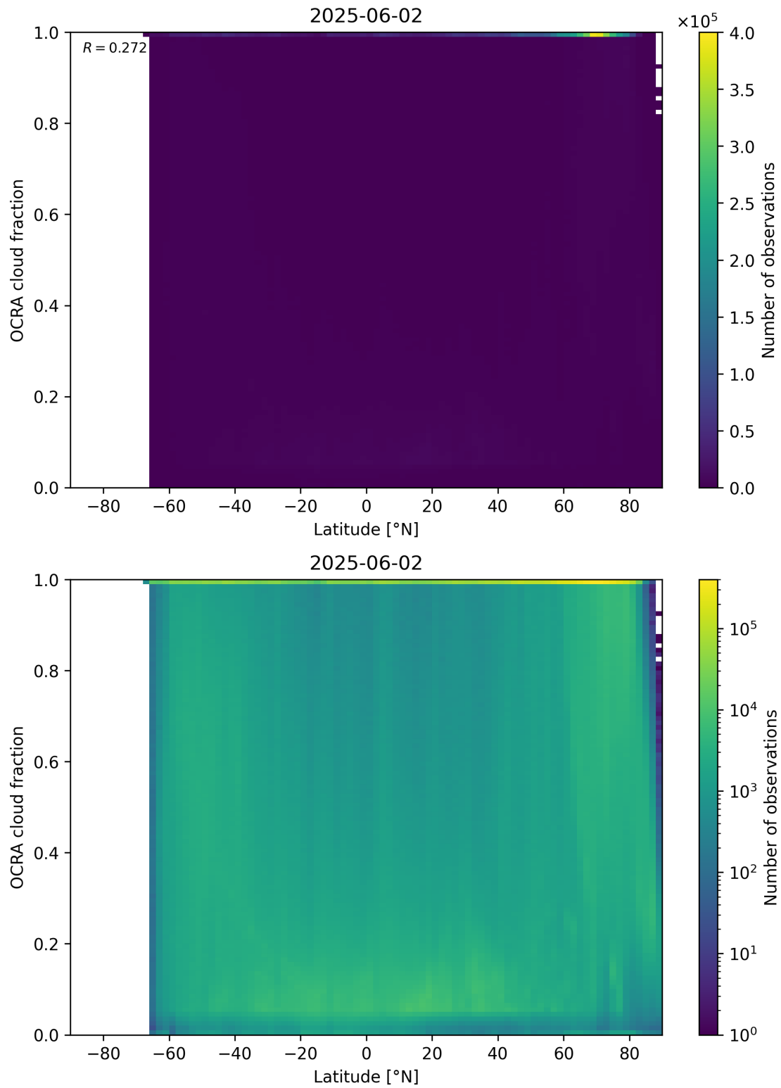
Figure 93: Scatter density plot of “Latitude” against “OCRA cloud fraction” for 2025-06-01 to 2025-06-03.
