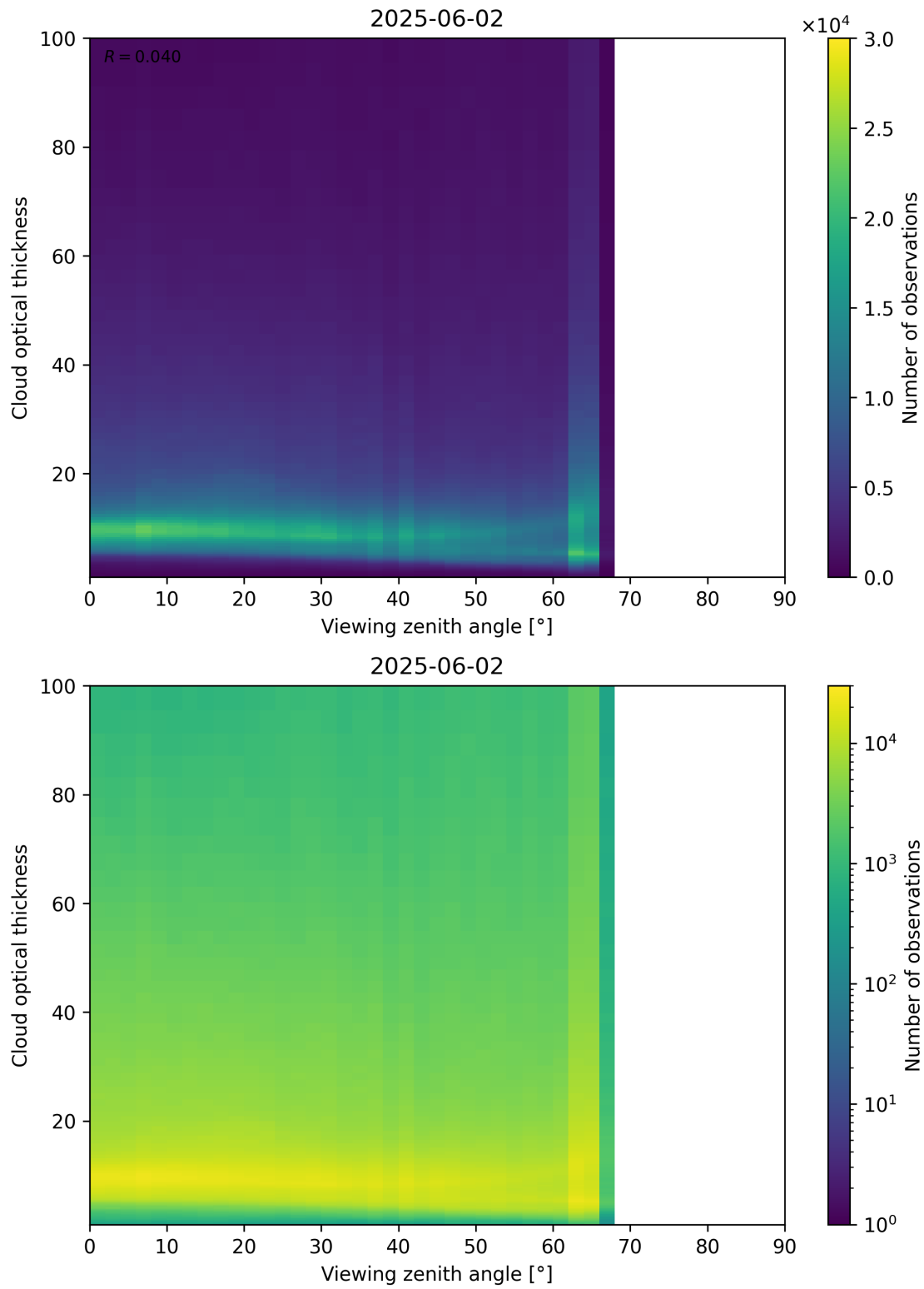
Figure 111: Scatter density plot of “Viewing zenith angle” against “Cloud optical thickness” for 2025-06-01 to 2025-06-03.
