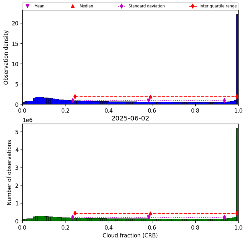
Figure 42: Histogram of “Cloud fraction (CRB)” for 2025-06-01 to 2025-06-03
