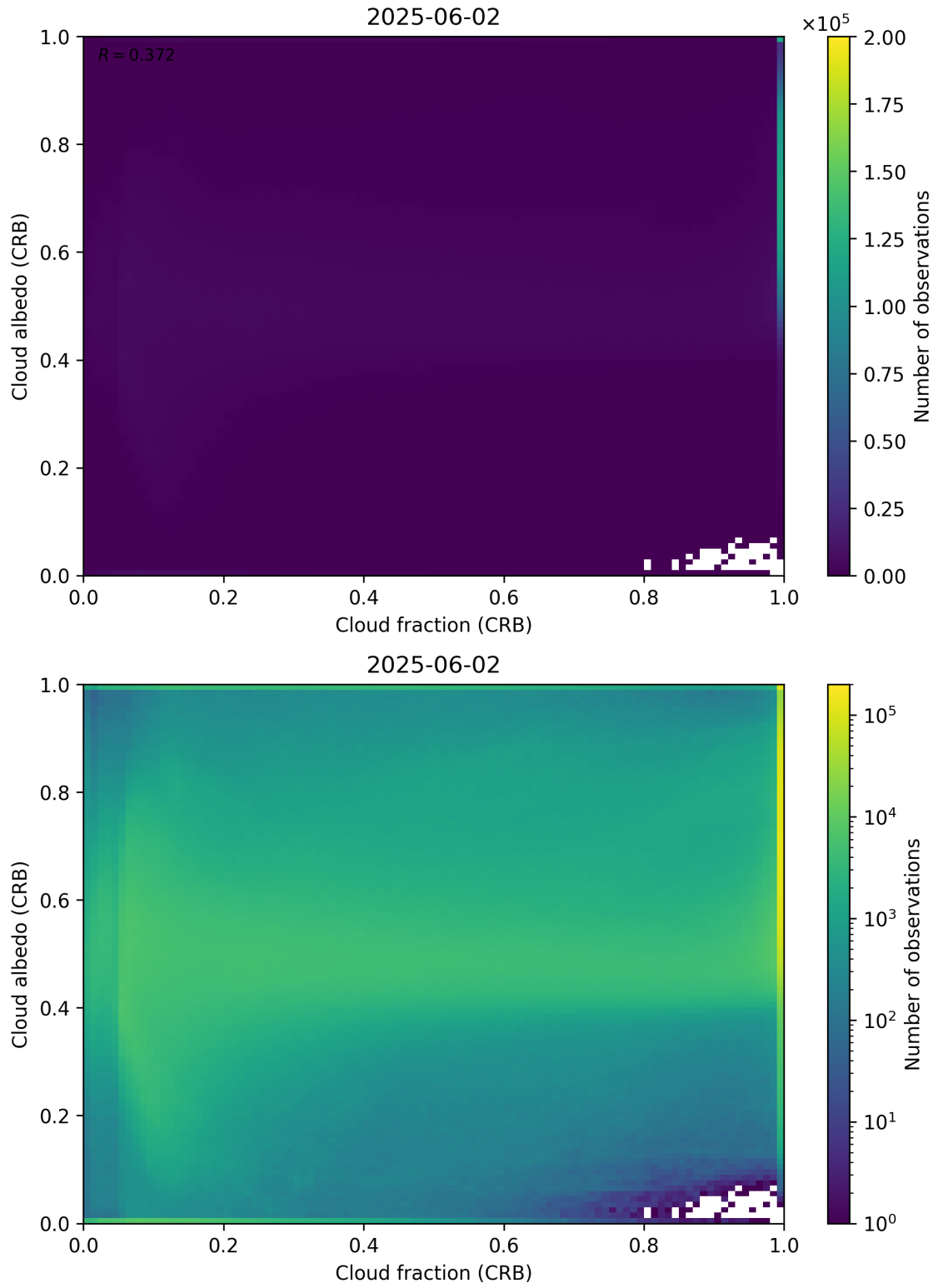
Figure 77: Scatter density plot of “Cloud fraction (CRB)” against “Cloud albedo (CRB)” for 2025-06-01 to 2025-06-03.
