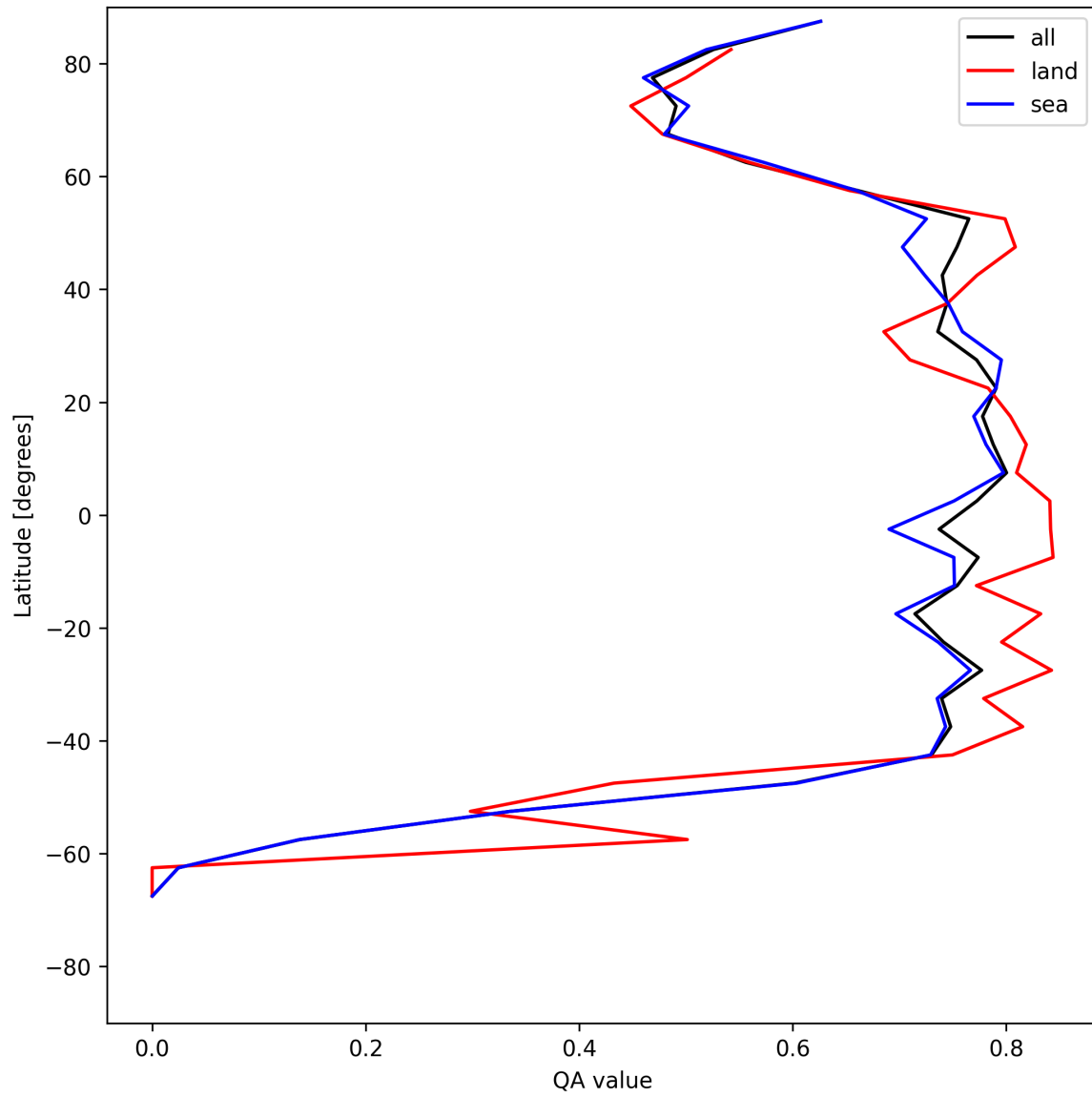
Figure 22: Zonal average of “QA value” for 2025-06-01 to 2025-06-03.
