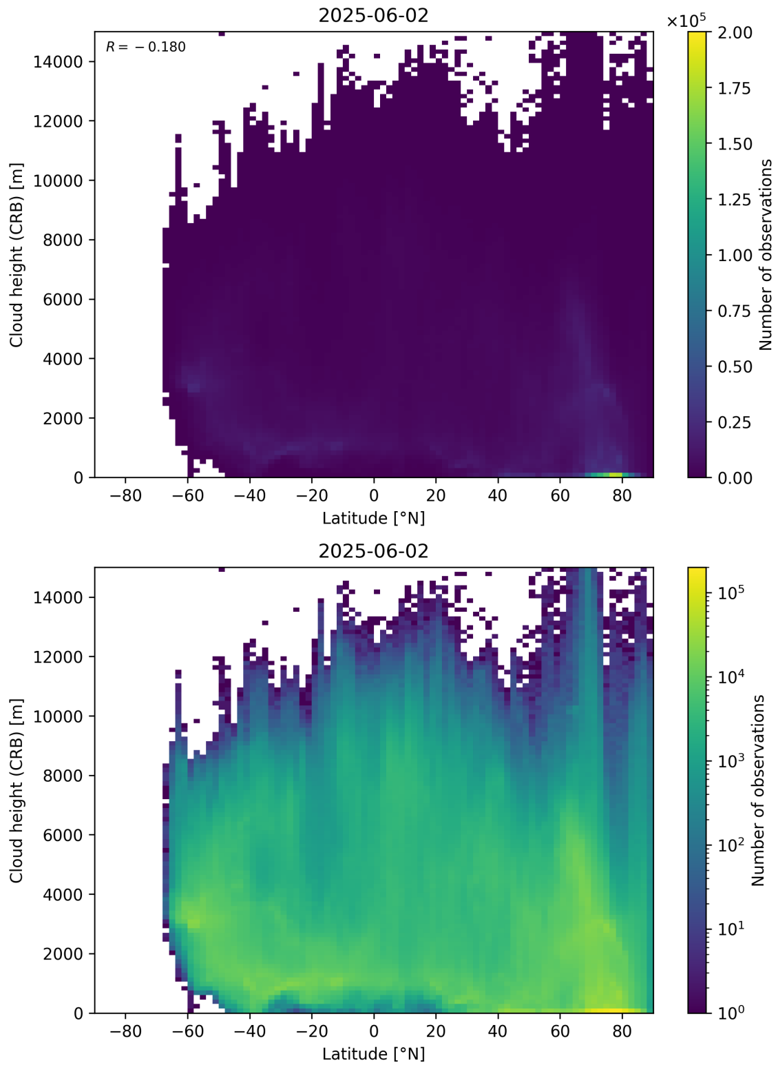
Figure 95: Scatter density plot of “Latitude” against “Cloud height (CRB)” for 2025-06-01 to 2025-06-03.
