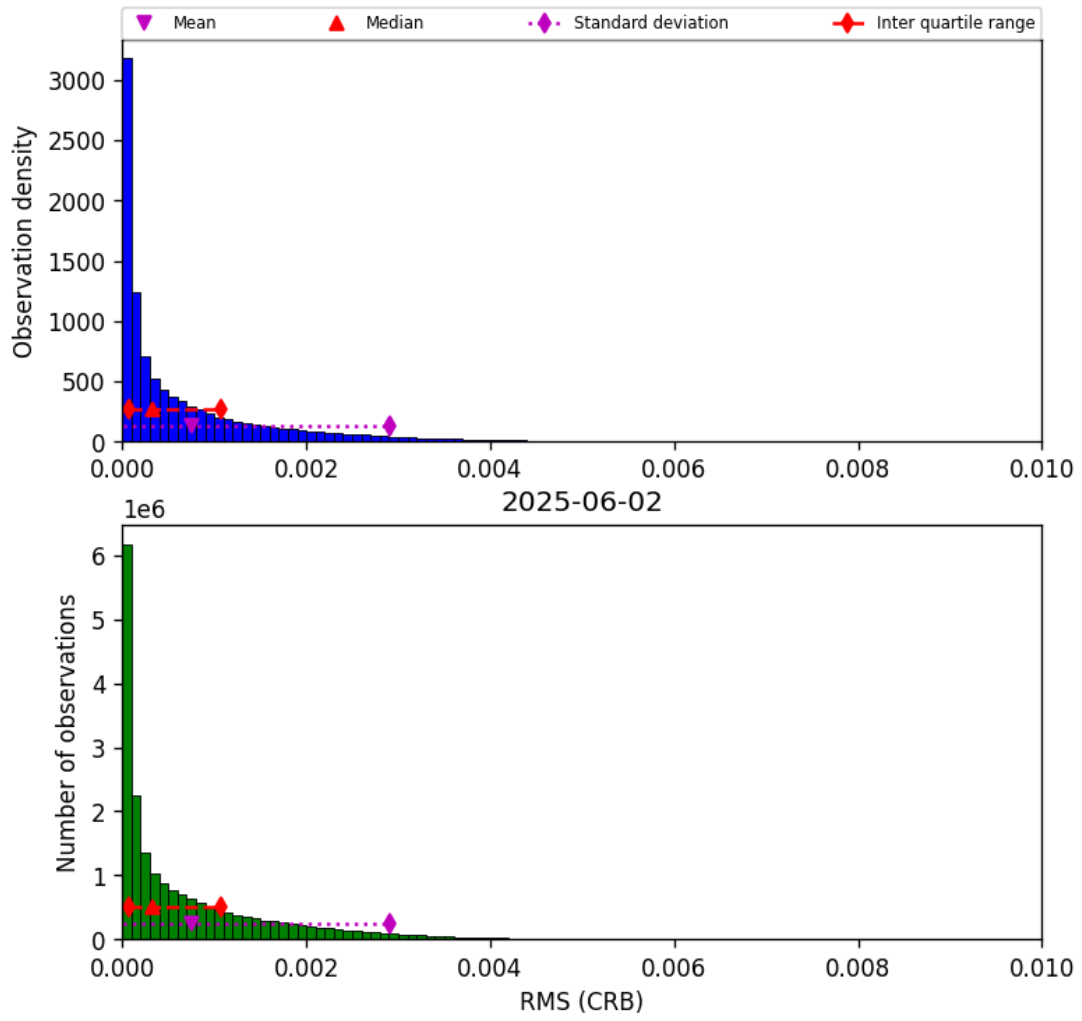
Figure 48: Histogram of “RMS (CRB)” for 2025-06-01 to 2025-06-03
