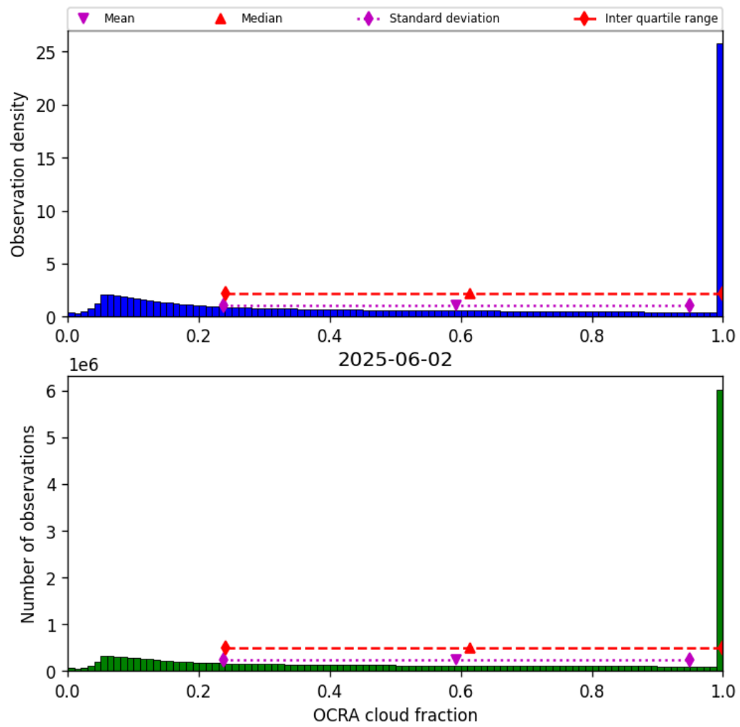
Figure 50: Histogram of “OCRA cloud fraction” for 2025-06-01 to 2025-06-03
