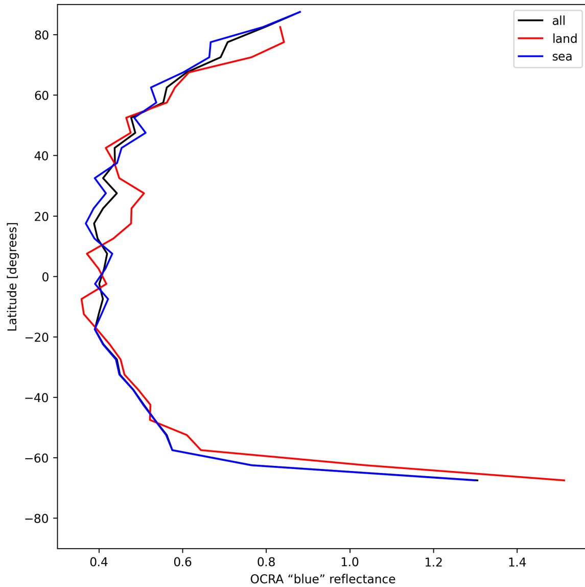
Figure 35: Zonal average of "OCRA "blue" reflectance" for 2025-06-01 to 2025-06-03.
