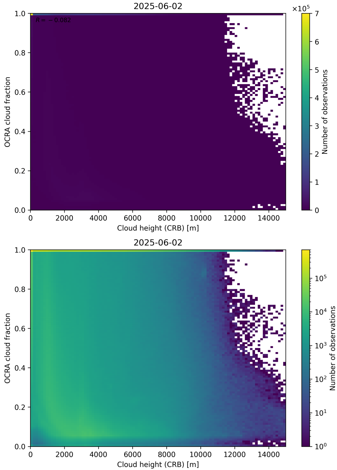
Figure 81: Scatter density plot of “Cloud height (CRB)” against “OCRA cloud fraction” for 2025-06-01 to 2025-06-03.
