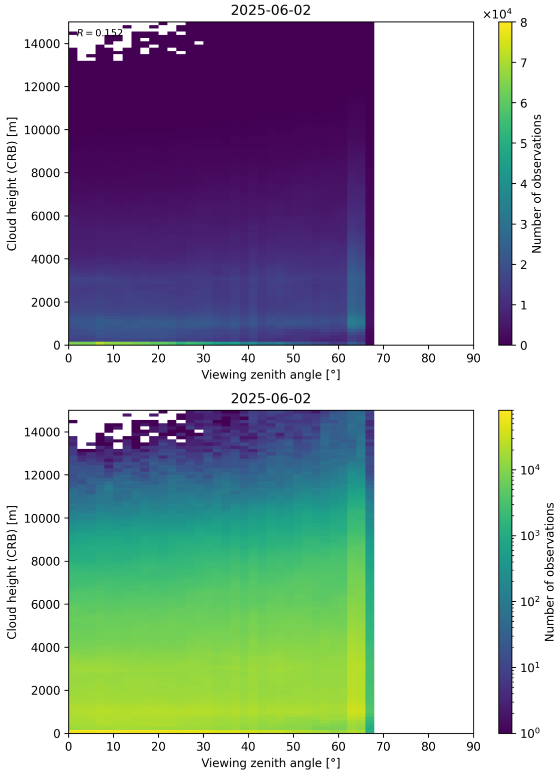
Figure 110: Scatter density plot of “Viewing zenith angle” against “Cloud height (CRB)” for 2025-06-01 to 2025-06-03.
