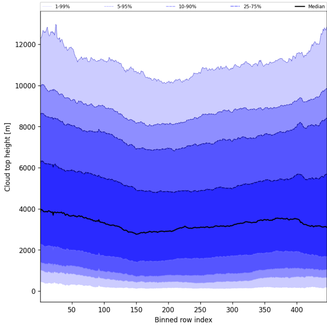
Figure 56: Along track statistics of “Cloud top height” for 2025-06-01 to 2025-06-03
