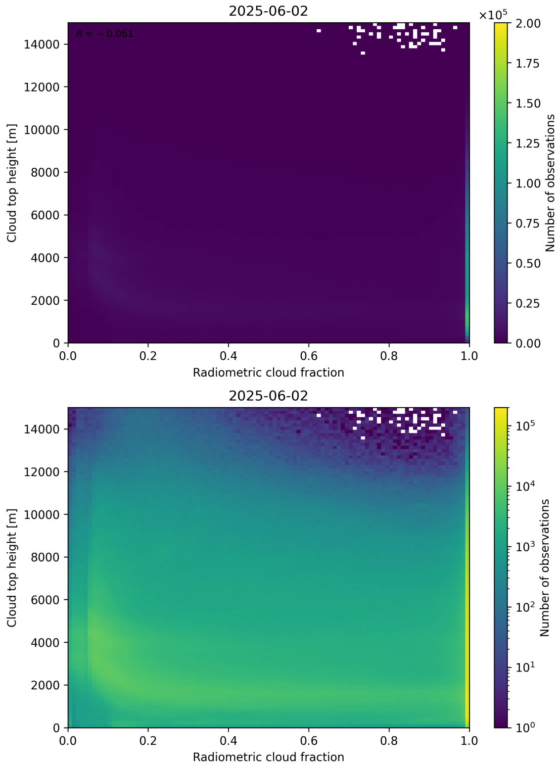
Figure 76: Scatter density plot of “Radiometric cloud fraction” against “Cloud top height” for 2025-06-01 to 2025-06-03.
