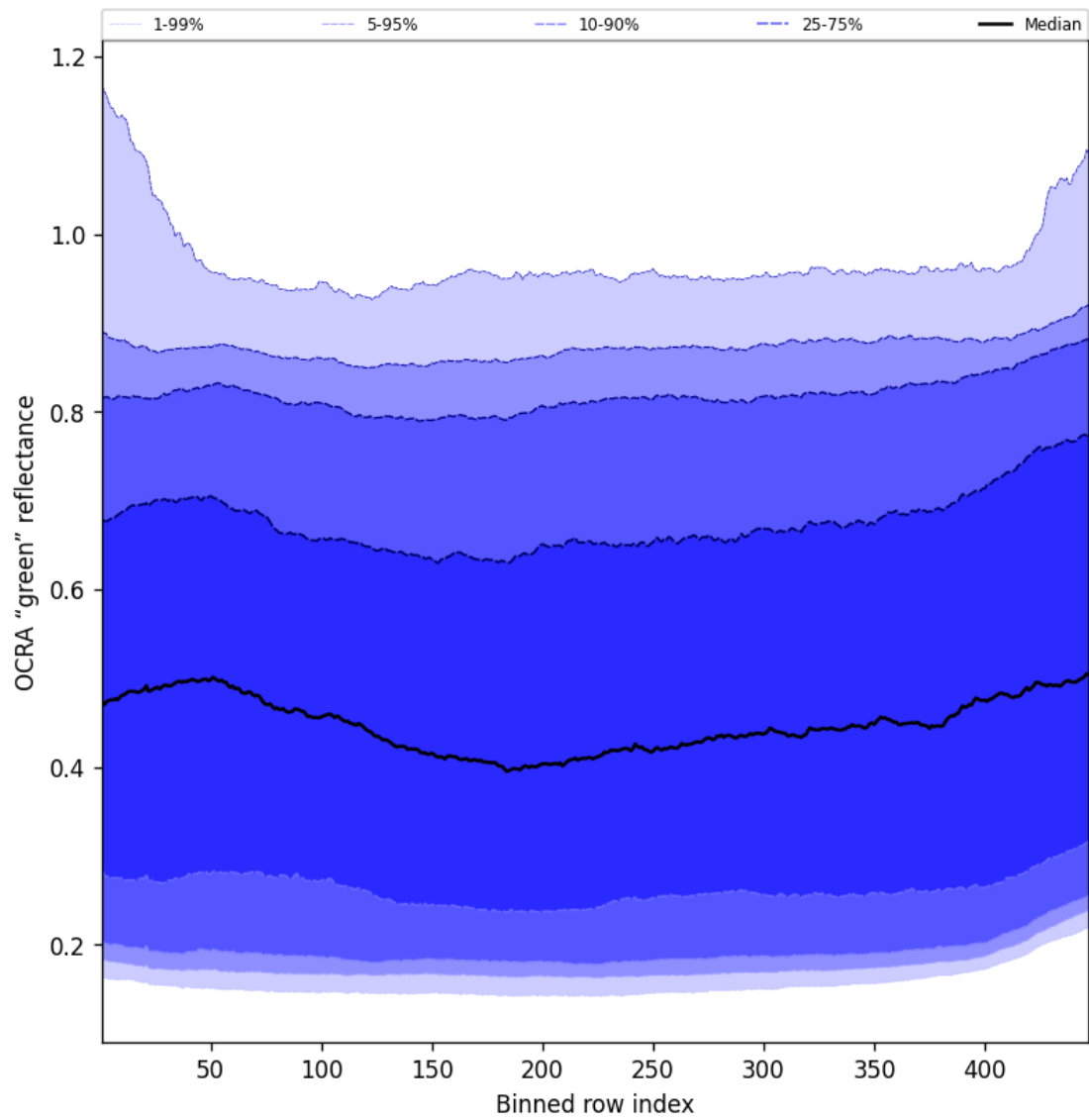
Figure 68: Along track statistics of “OCRA “green” reflectance” for 2025-06-01 to 2025-06-03
