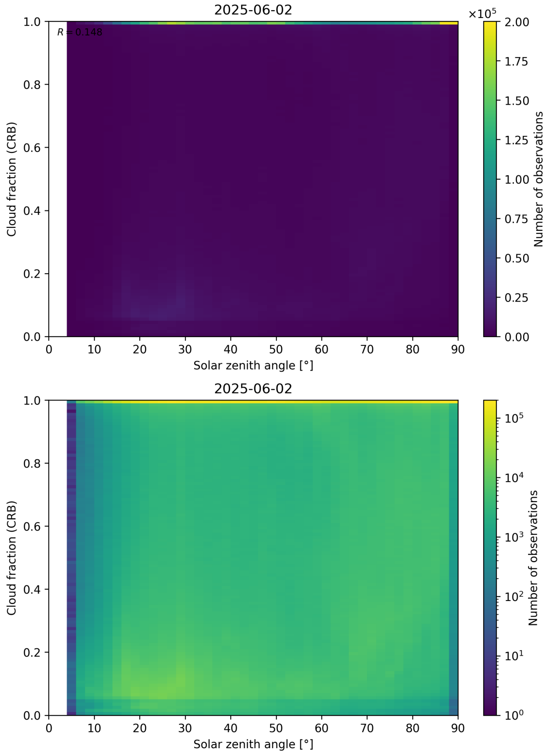
Figure 101: Scatter density plot of “Solar zenith angle” against “Cloud fraction (CRB)” for 2025-06-01 to 2025-06-03.
