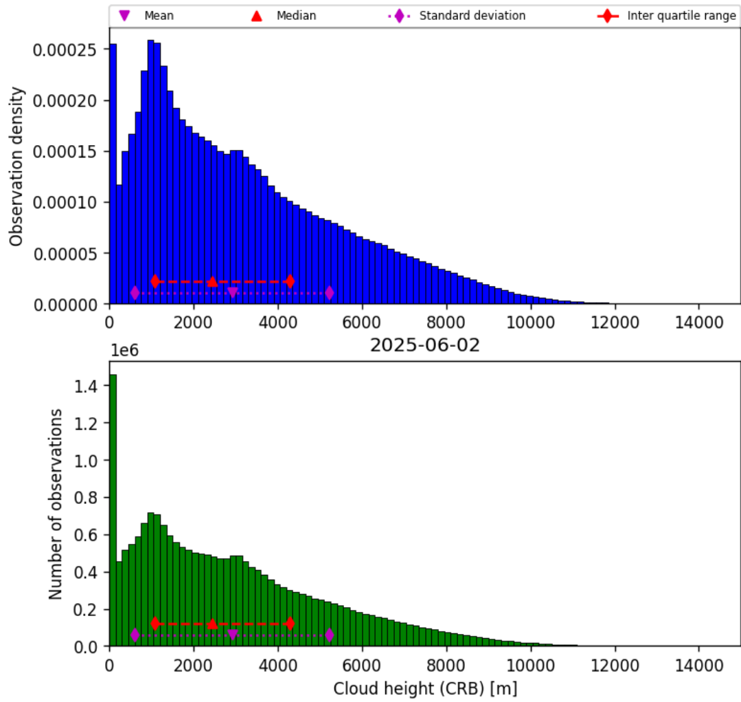
Figure 43: Histogram of “Cloud height (CRB)” for 2025-06-01 to 2025-06-03
