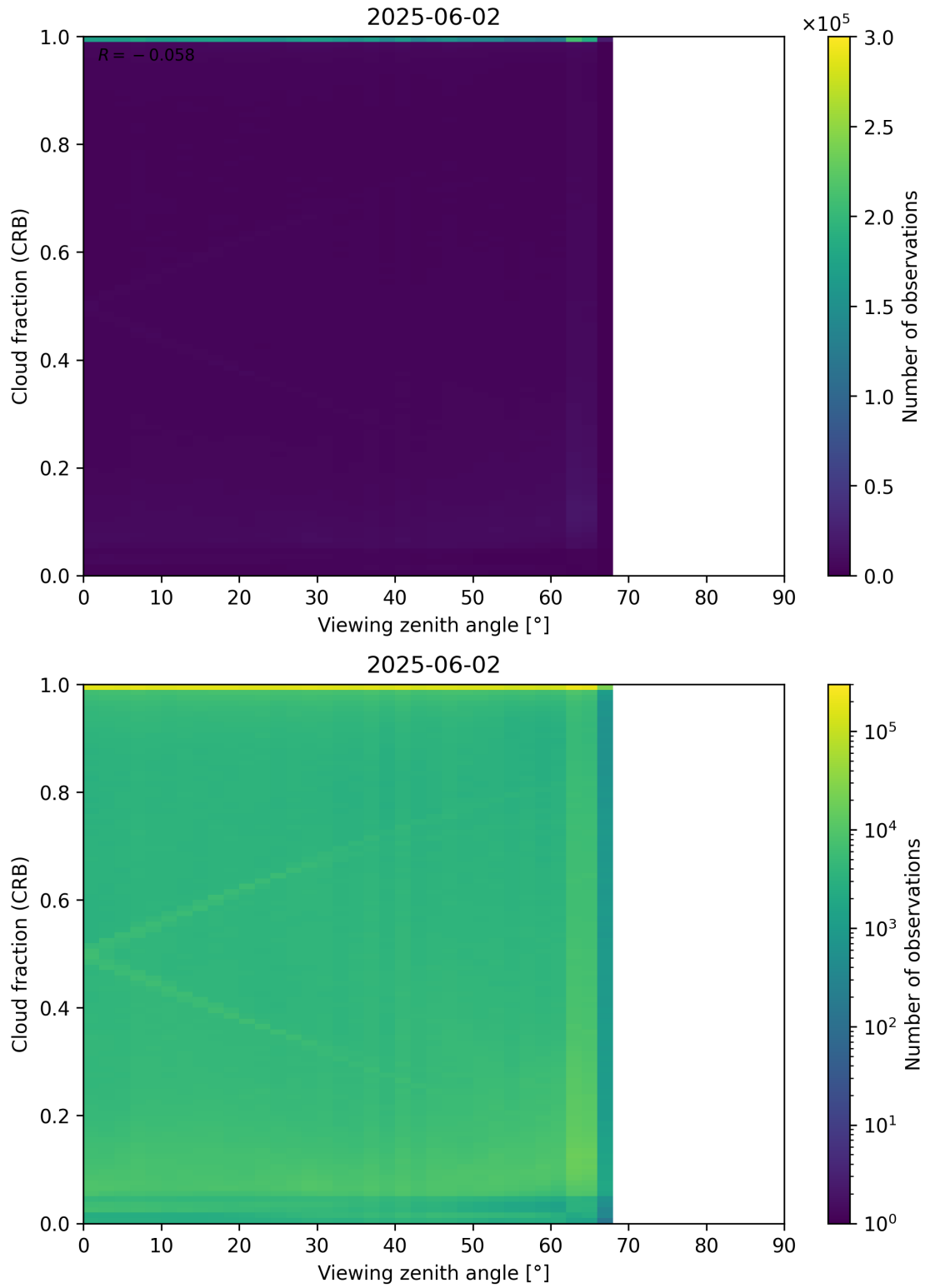
Figure 109: Scatter density plot of “Viewing zenith angle” against “Cloud fraction (CRB)” for 2025-06-01 to 2025-06-03.
