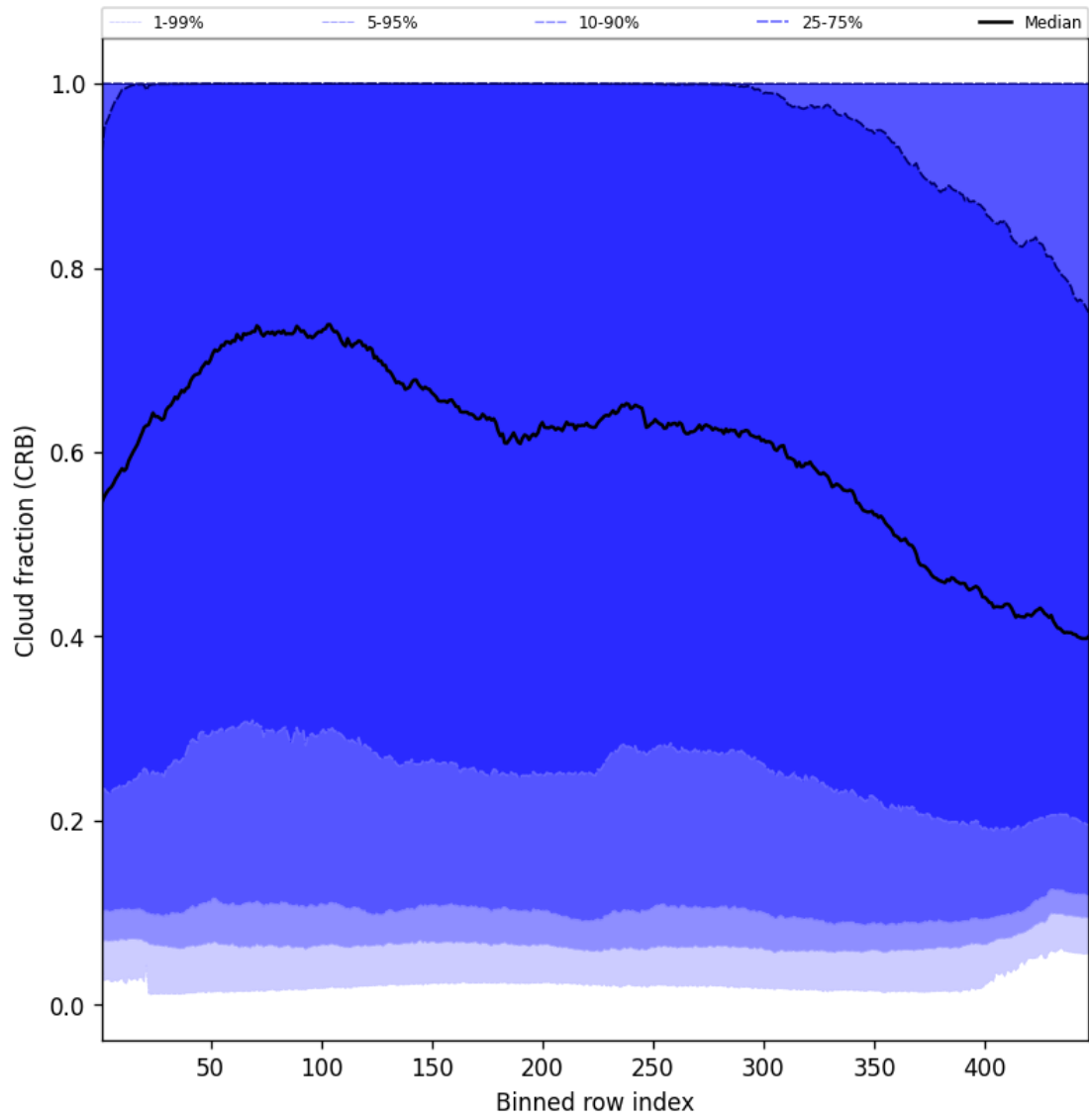
Figure 58: Along track statistics of “Cloud fraction (CRB)” for 2025-06-01 to 2025-06-03
