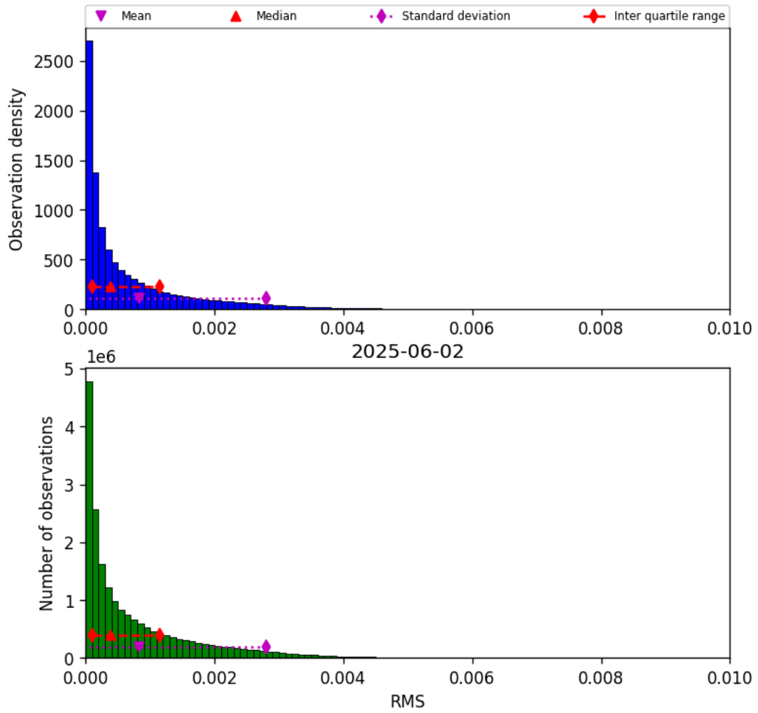
Figure 47: Histogram of “RMS” for 2025-06-01 to 2025-06-03
