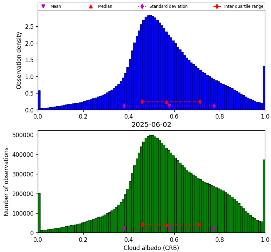
Figure 44: Histogram of “Cloud albedo (CRB)” for 2025-06-01 to 2025-06-03
