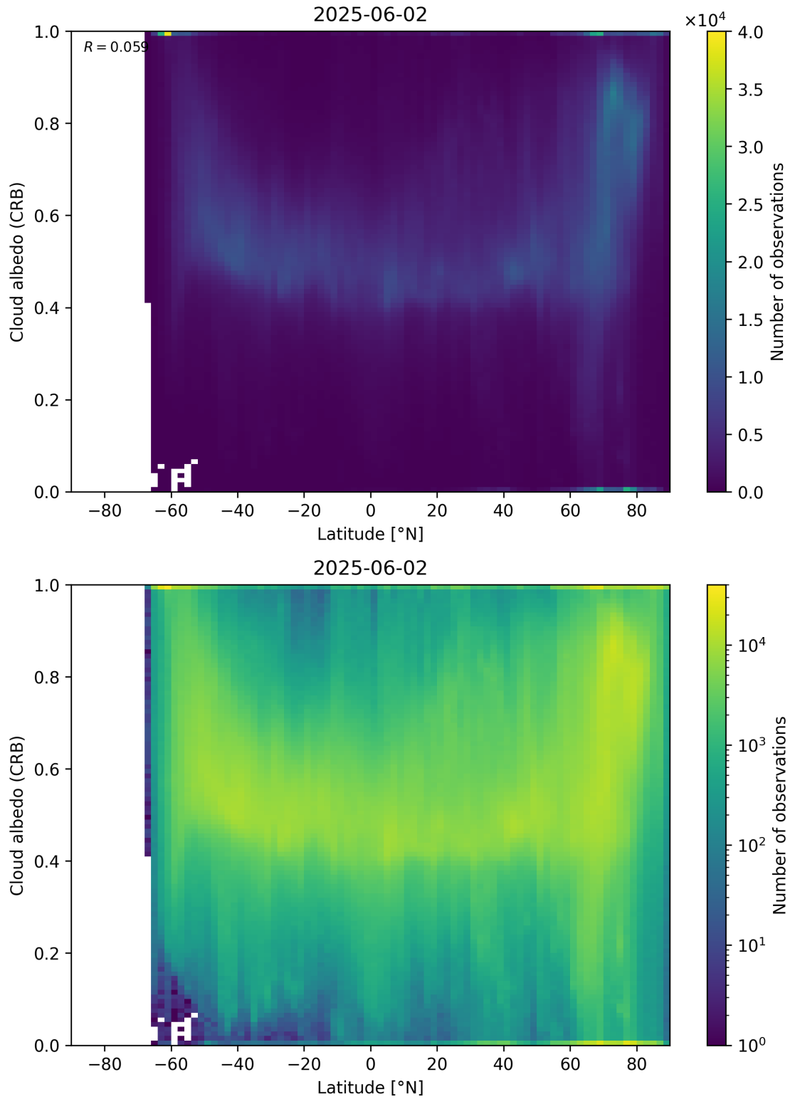
Figure 91: Scatter density plot of “Latitude” against “Cloud albedo (CRB)” for 2025-06-01 to 2025-06-03.
