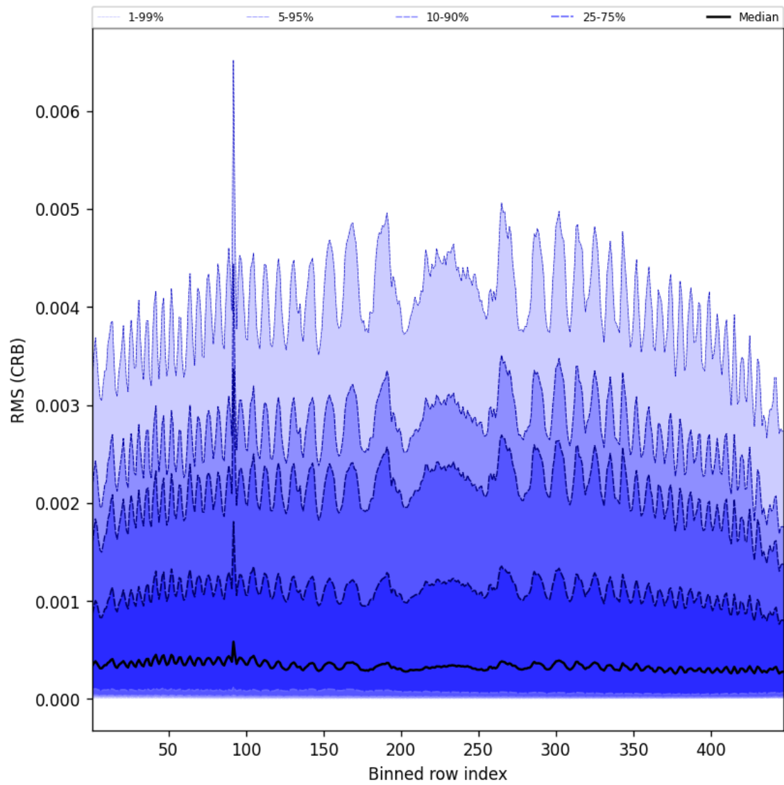
Figure 64: Along track statistics of “RMS (CRB)” for 2025-06-01 to 2025-06-03
