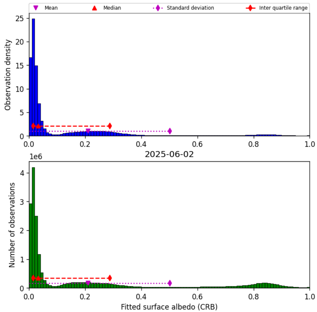
Figure 46: Histogram of “Fitted surface albedo (CRB)” for 2025-06-01 to 2025-06-03
