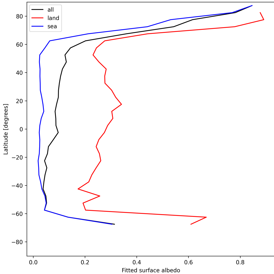
Figure 29: Zonal average of “Fitted surface albedo” for 2025-06-01 to 2025-06-03.
