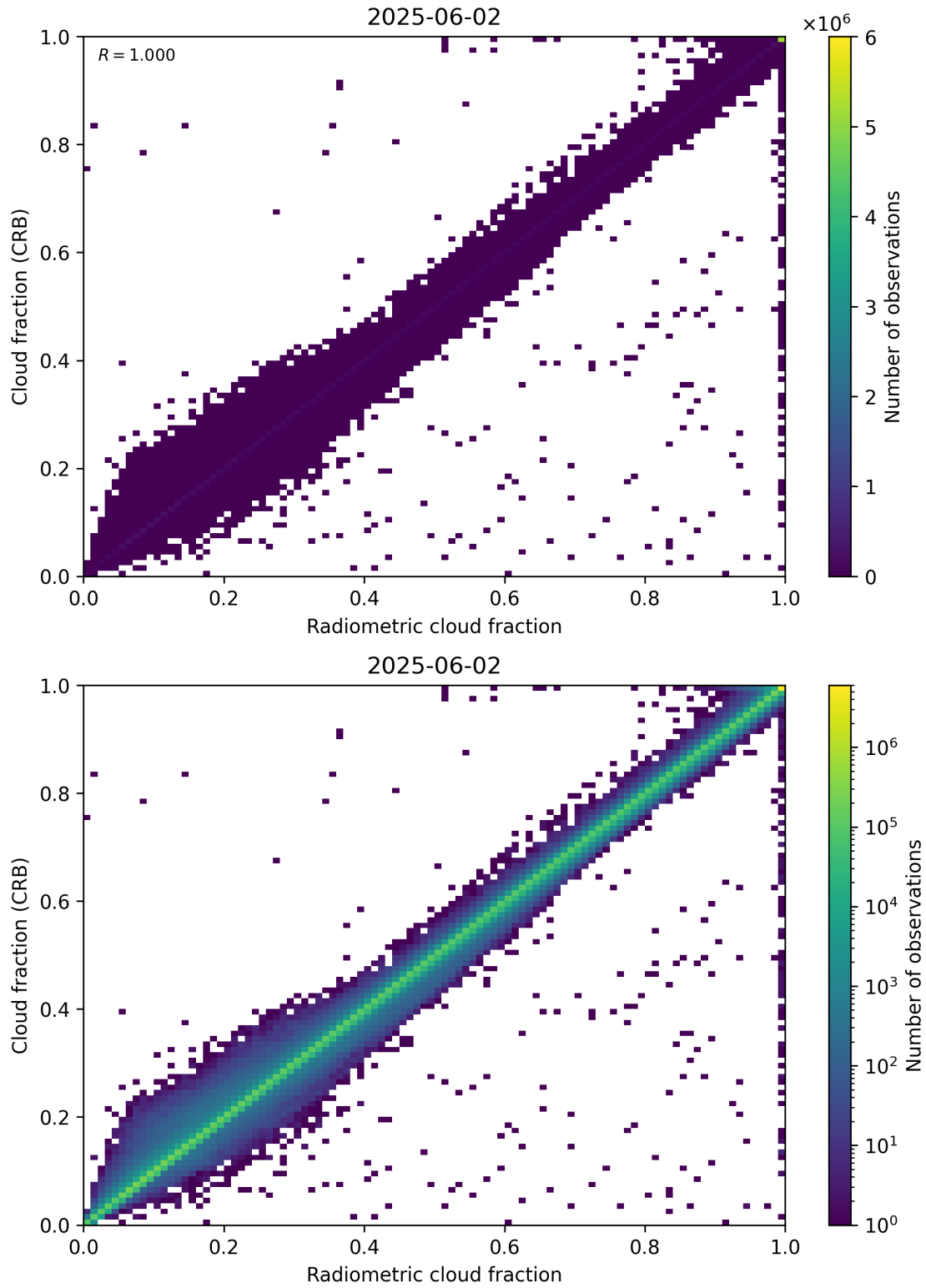
Figure 73: Scatter density plot of “Radiometric cloud fraction” against “Cloud fraction (CRB)” for 2025-06-01 to 2025-06-03.
