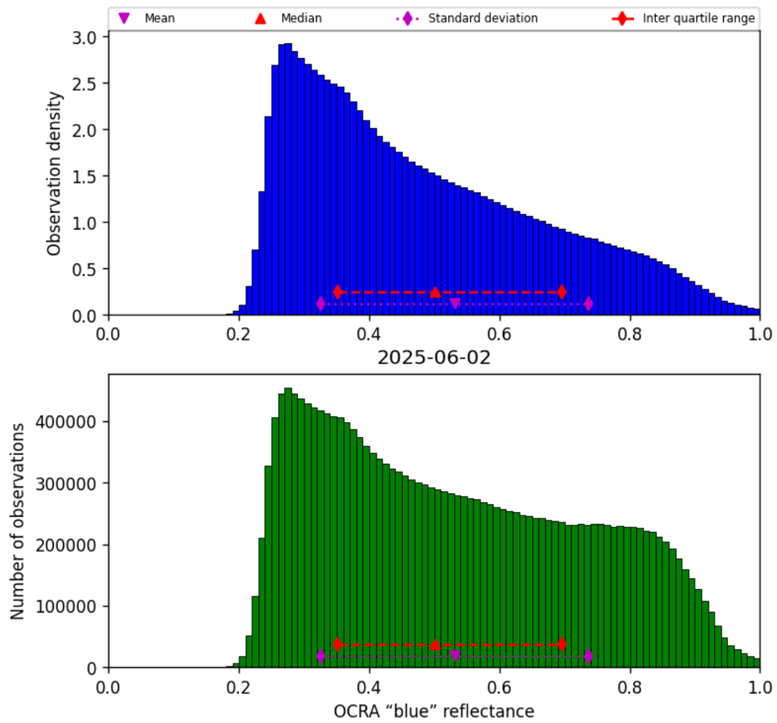
Figure 51: Histogram of “OCRA “blue” reflectance” for 2025-06-01 to 2025-06-03
