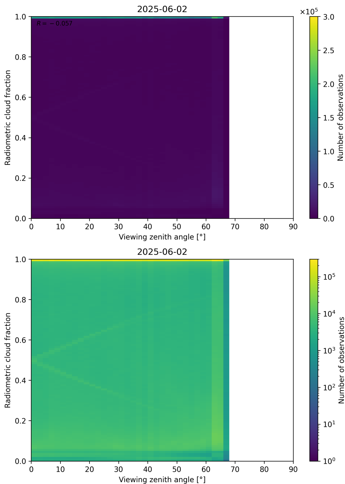
Figure 107: Scatter density plot of “Viewing zenith angle” against “Radiometric cloud fraction” for 2025-06-01 to 2025-06-03.
