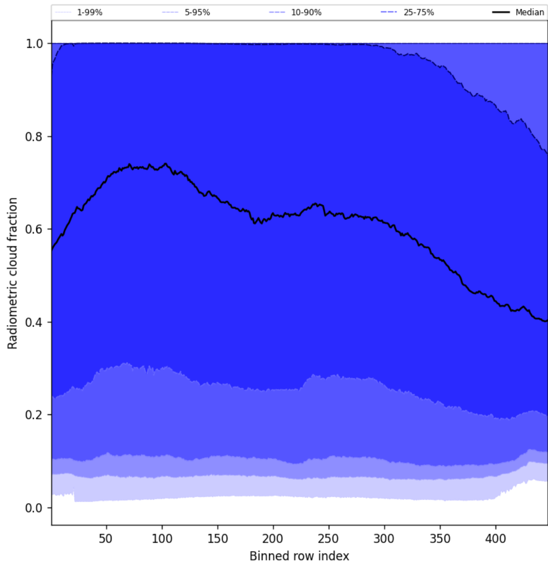
Figure 55: Along track statistics of “Radiometric cloud fraction” for 2025-06-01 to 2025-06-03
