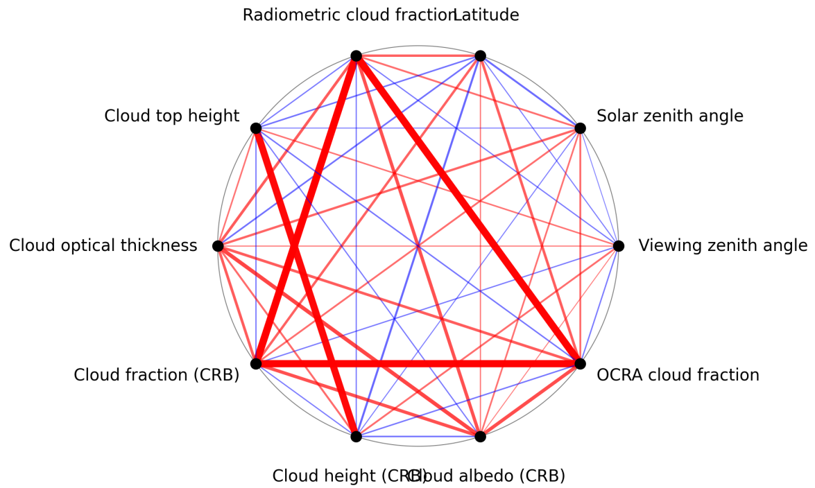
Figure 1: Map of correlation graph for 2025-06-01 to 2025-06-03.
