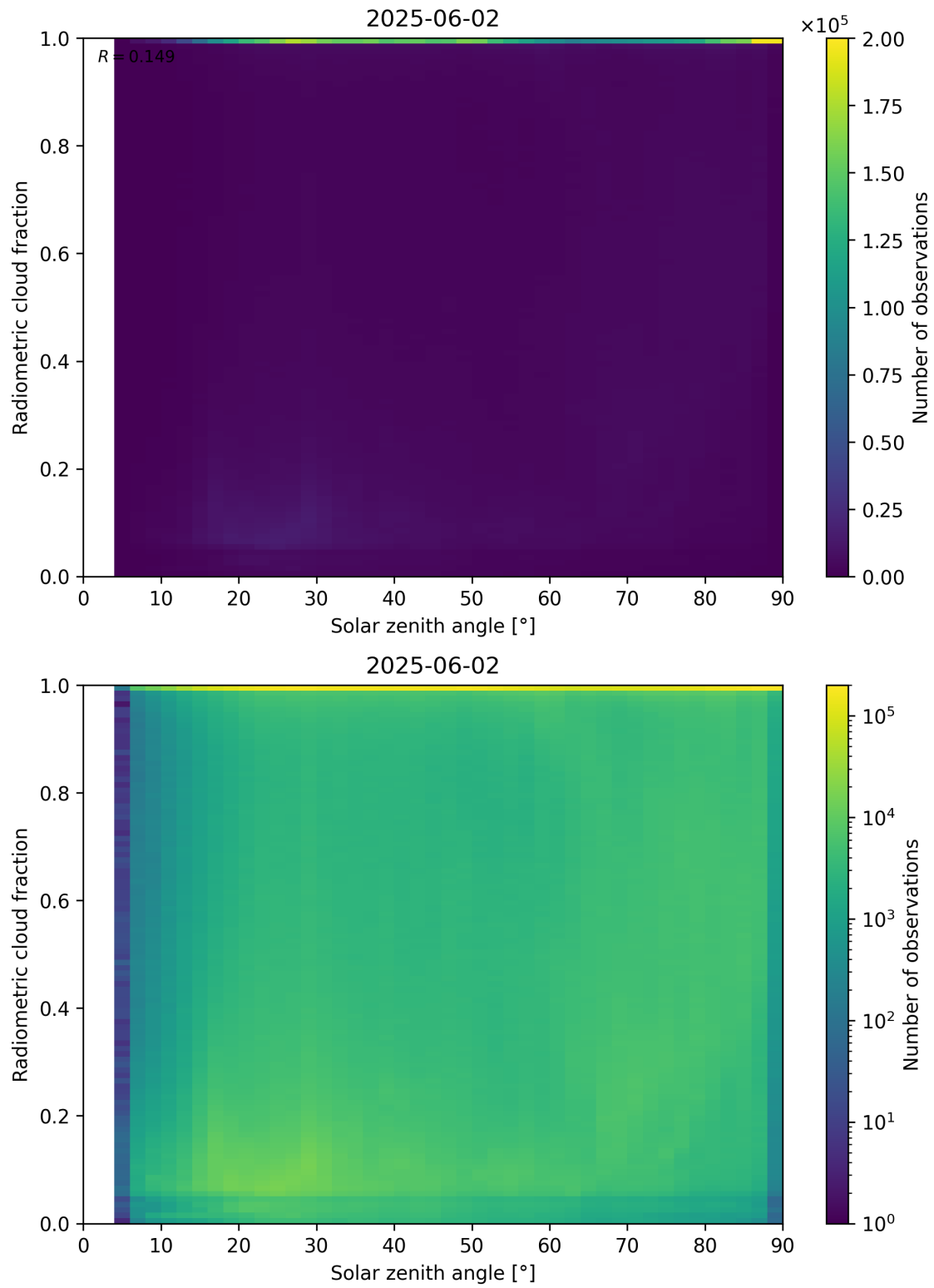
Figure 99: Scatter density plot of “Solar zenith angle” against “Radiometric cloud fraction” for 2025-06-01 to 2025-06-03.
