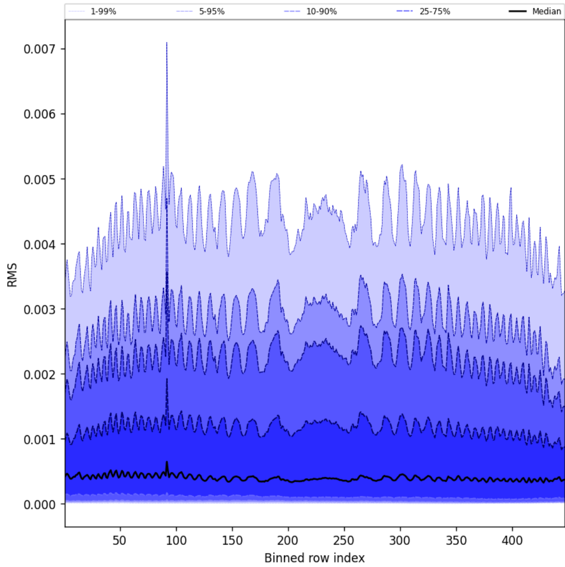
Figure 63: Along track statistics of “RMS” for 2025-06-01 to 2025-06-03
