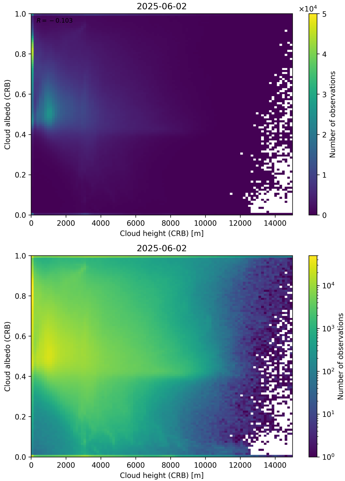
Figure 80: Scatter density plot of “Cloud height (CRB)” against “Cloud albedo (CRB)” for 2025-06-01 to 2025-06-03.
