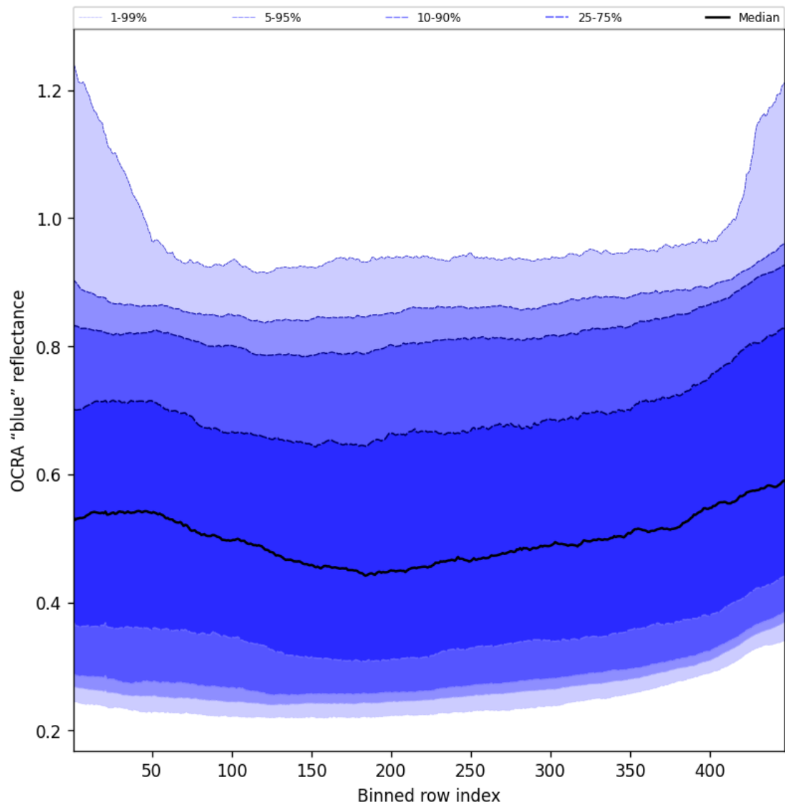
Figure 67: Along track statistics of “OCRA “blue” reflectance” for 2025-06-01 to 2025-06-03
