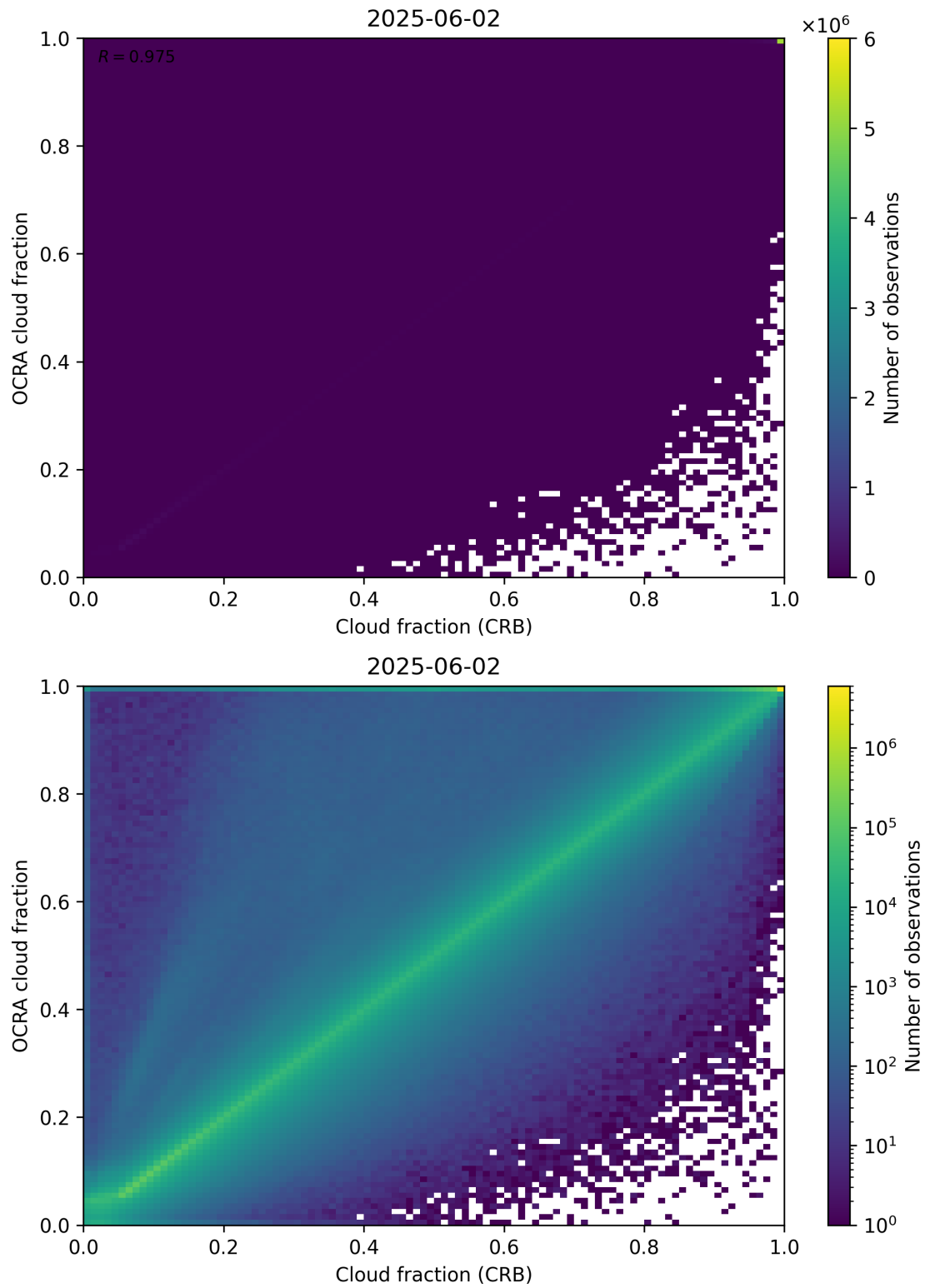
Figure 78: Scatter density plot of “Cloud fraction (CRB)” against “OCRA cloud fraction” for 2025-06-01 to 2025-06-03.
