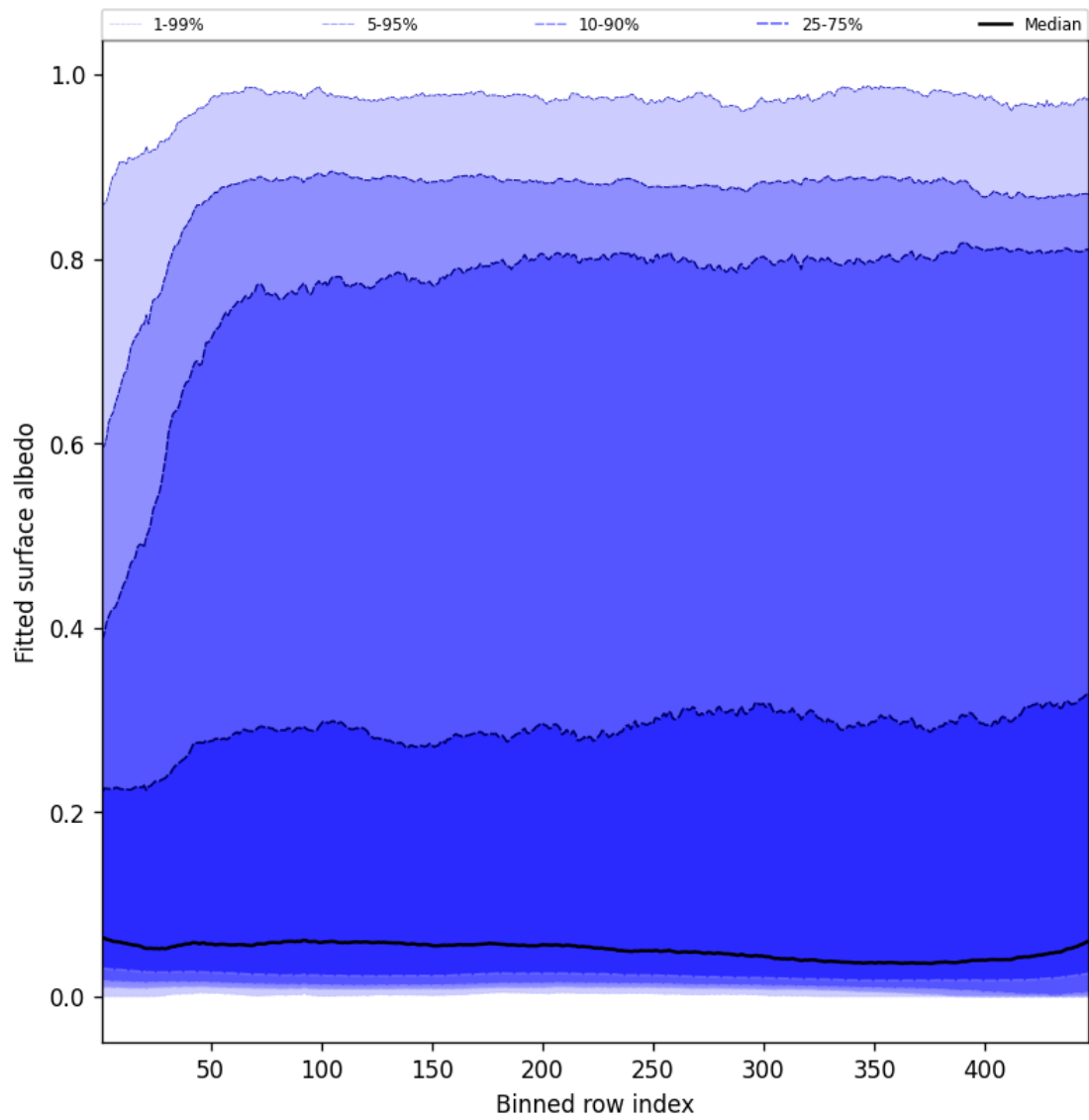
Figure 61: Along track statistics of “Fitted surface albedo” for 2025-06-01 to 2025-06-03
