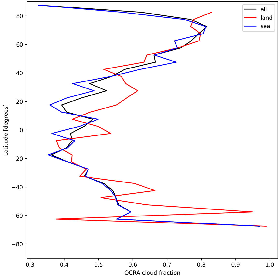
Figure 34: Zonal average of “OCRA cloud fraction” for 2025-06-01 to 2025-06-03.
