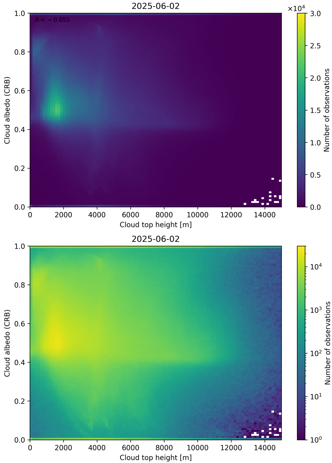
Figure 86: Scatter density plot of “Cloud top height” against “Cloud albedo (CRB)” for 2025-06-01 to 2025-06-03.
