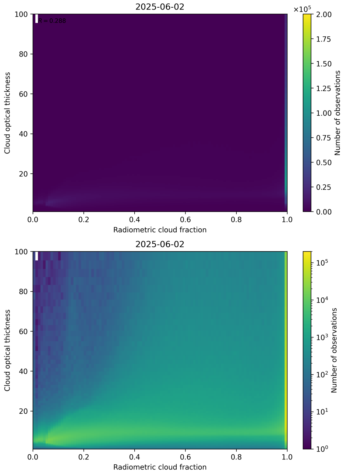
Figure 75: Scatter density plot of “Radiometric cloud fraction” against “Cloud optical thickness” for 2025-06-01 to 2025-06-03.
