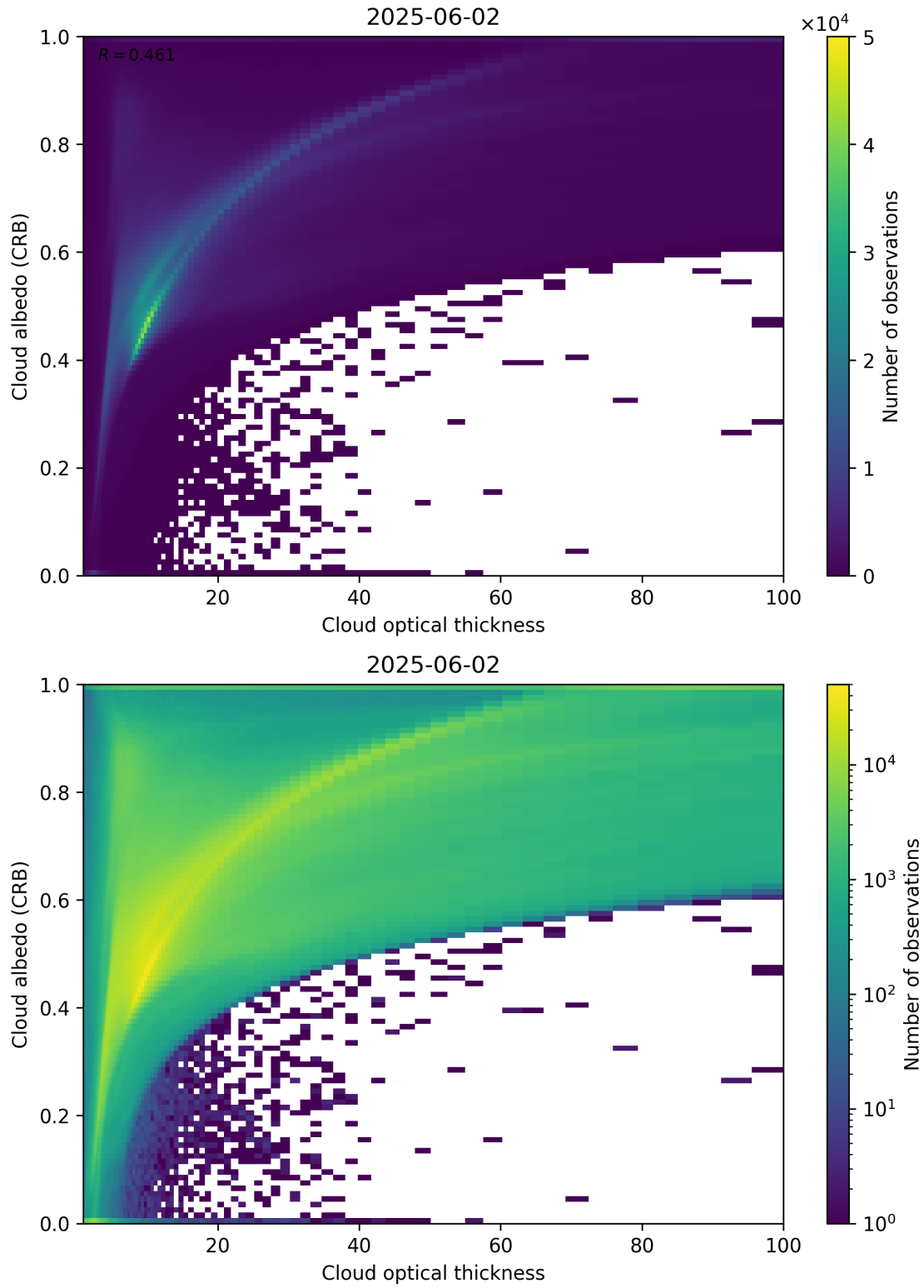
Figure 82: Scatter density plot of “Cloud optical thickness” against “Cloud albedo (CRB)” for 2025-06-01 to 2025-06-03.
