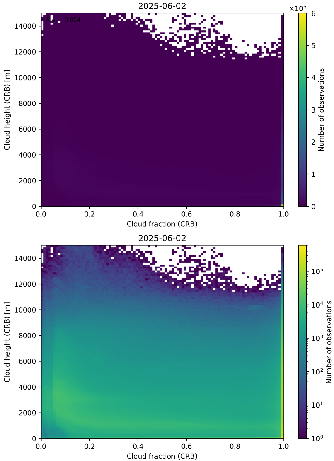
Figure 79: Scatter density plot of “Cloud fraction (CRB)” against “Cloud height (CRB)” for 2025-06-01 to 2025-06-03.
