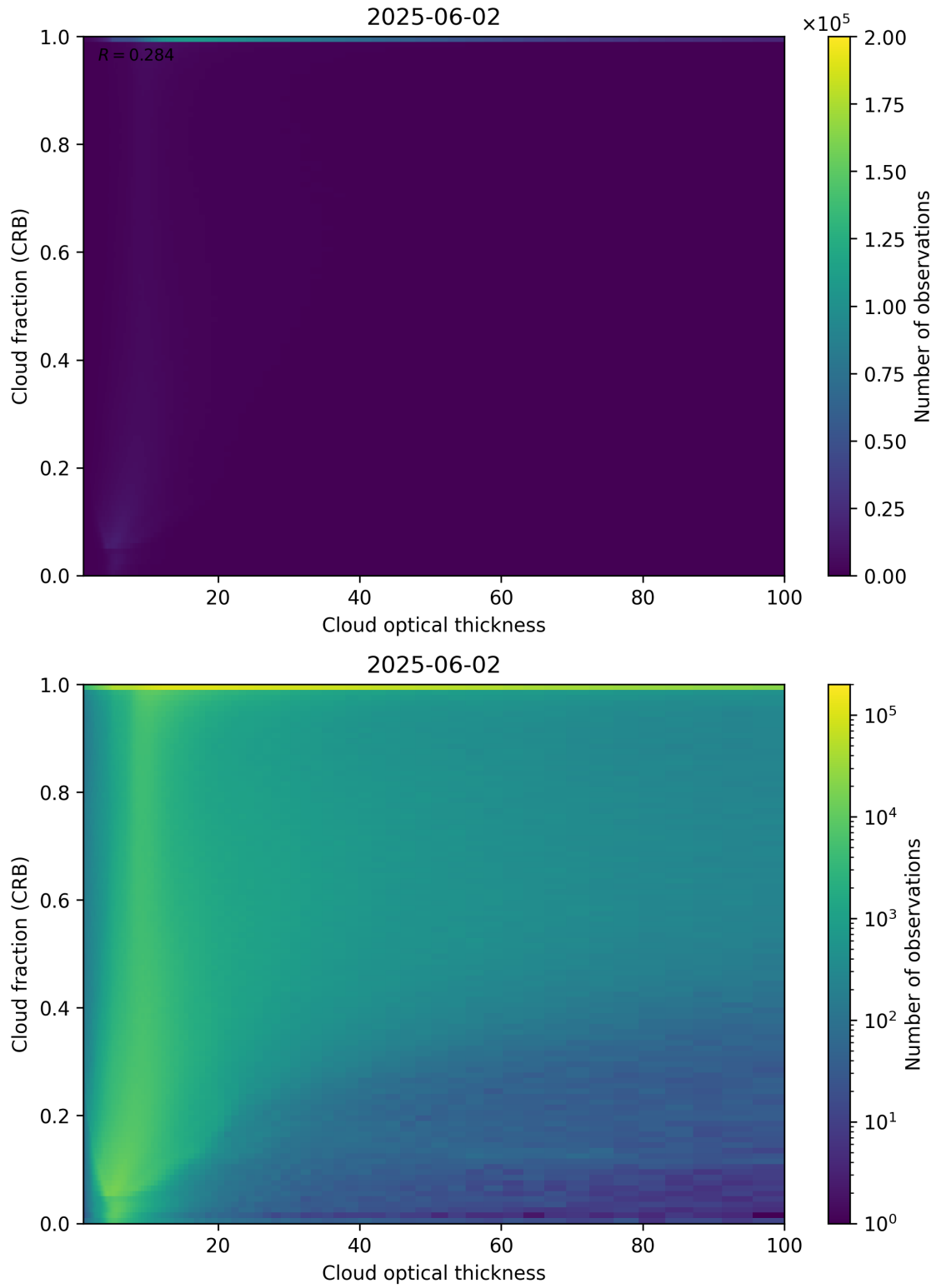
Figure 84: Scatter density plot of “Cloud optical thickness” against “Cloud fraction (CRB)” for 2025-06-01 to 2025-06-03.
