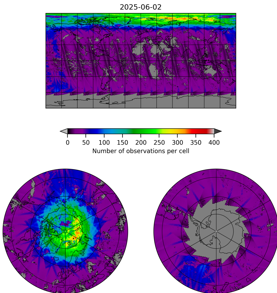
Figure 21: Map of the number of observations for 2025-06-01 to 2025-06-03
