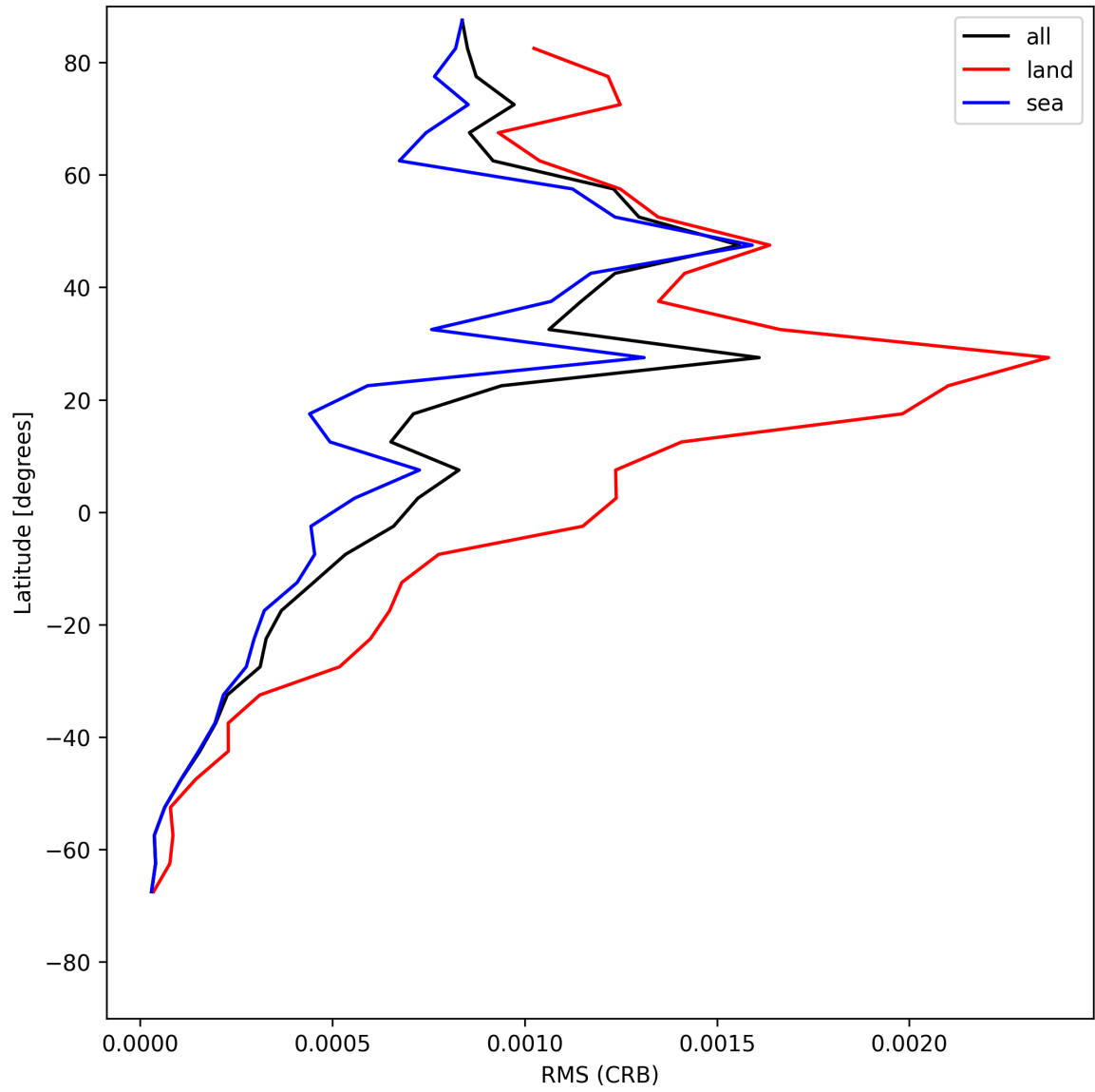
Figure 32: Zonal average of “RMS (CRB)” for 2025-06-01 to 2025-06-03.
