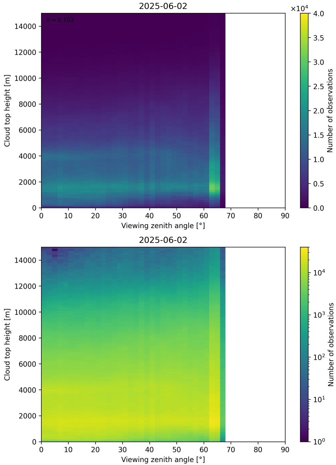
Figure 112: Scatter density plot of “Viewing zenith angle” against “Cloud top height” for 2025-06-01 to 2025-06-03.
