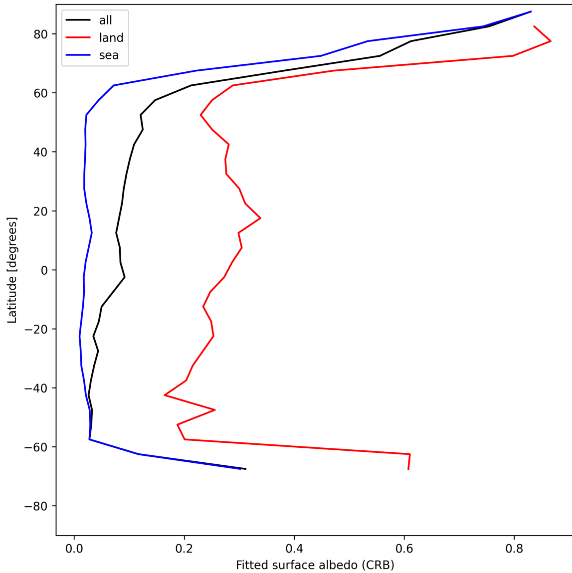
Figure 30: Zonal average of “Fitted surface albedo (CRB)” for 2025-06-01 to 2025-06-03.
