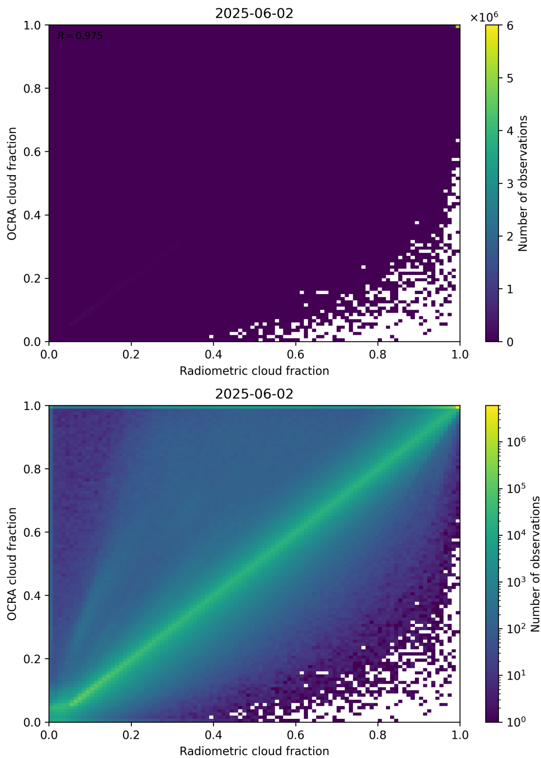
Figure 72: Scatter density plot of “Radiometric cloud fraction” against “OCRA cloud fraction” for 2025-06-01 to 2025-06-03.
