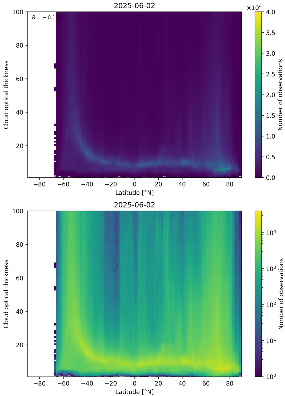
Figure 96: Scatter density plot of “Latitude” against “Cloud optical thickness” for 2025-06-01 to 2025-06-03.
