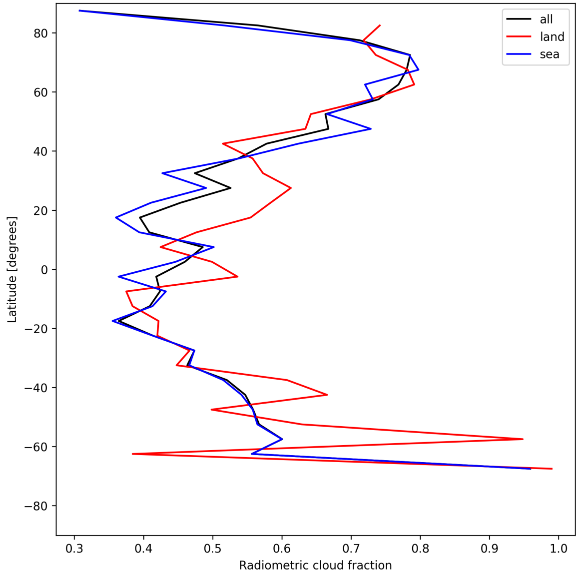
Figure 23: Zonal average of “Radiometric cloud fraction” for 2025-06-01 to 2025-06-03.
