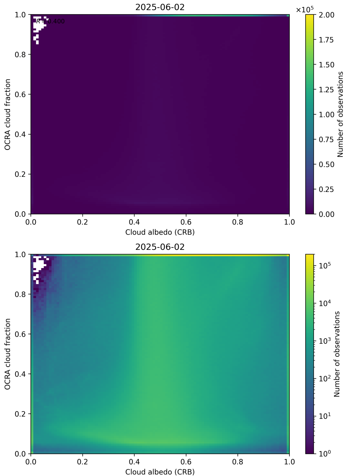
Figure 70: Scatter density plot of “Cloud albedo (CRB)” against “OCRA cloud fraction” for 2025-06-01 to 2025-06-03.
