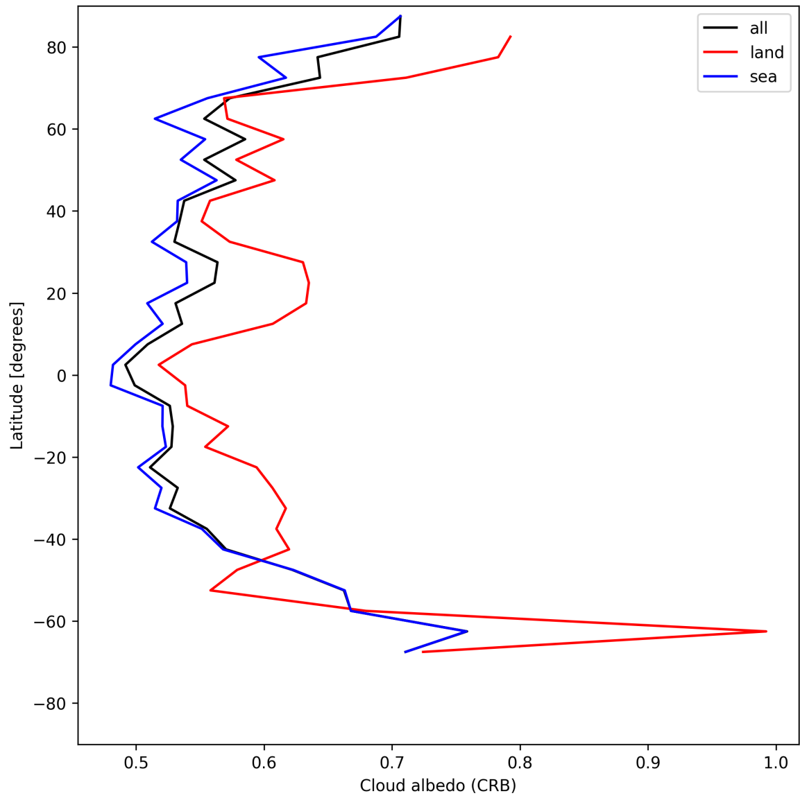
Figure 28: Zonal average of “Cloud albedo (CRB)” for 2025-06-01 to 2025-06-03.
