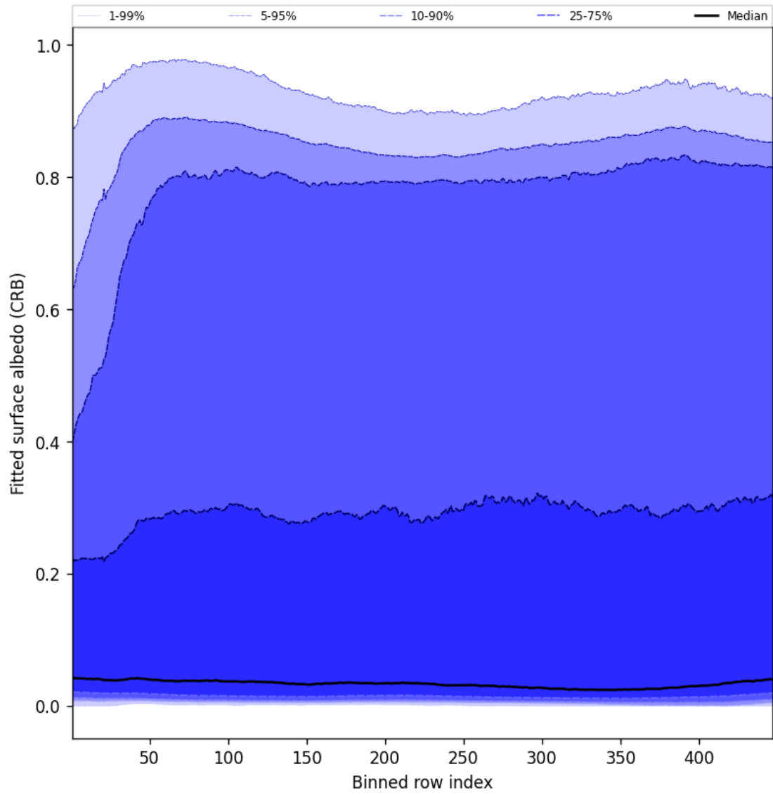
Figure 62: Along track statistics of “Fitted surface albedo (CRB)” for 2025-06-01 to 2025-06-03
