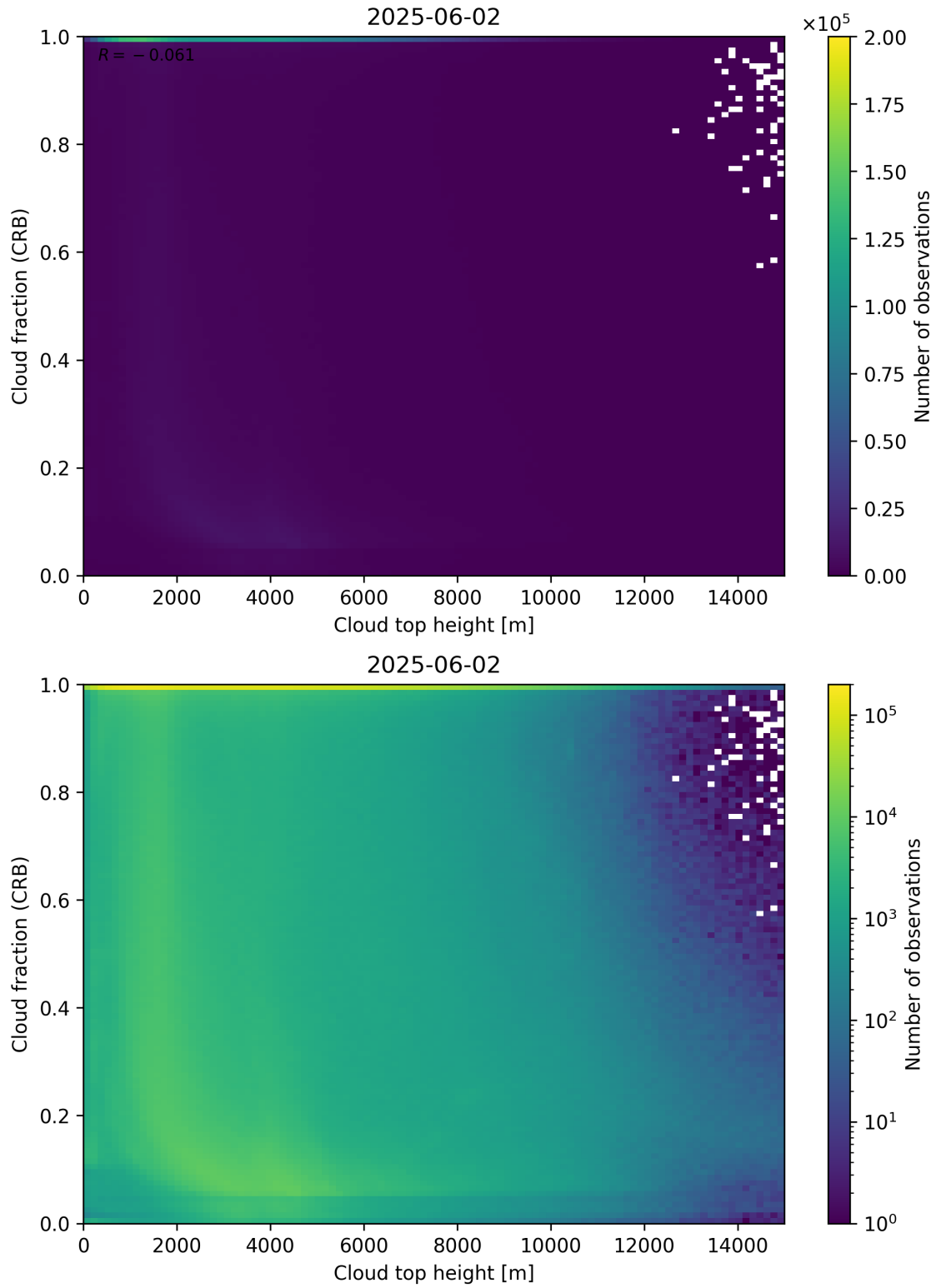
Figure 88: Scatter density plot of “Cloud top height” against “Cloud fraction (CRB)” for 2025-06-01 to 2025-06-03.
