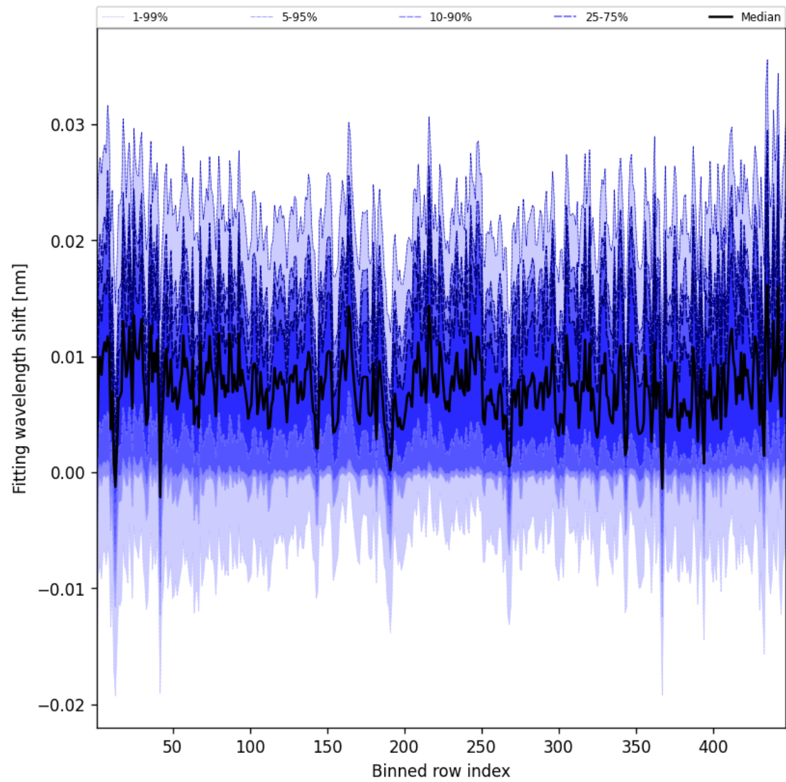
Figure 65: Along track statistics of “Fitting wavelength shift” for 2025-06-01 to 2025-06-03
