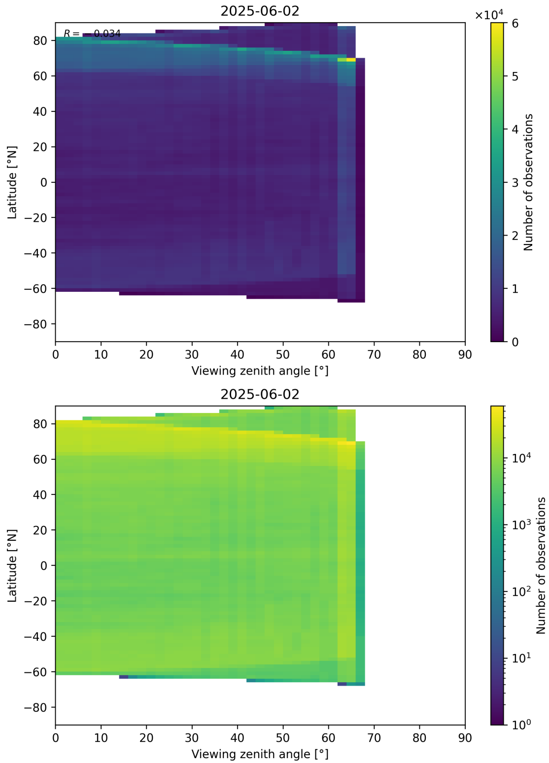
Figure 113: Scatter density plot of “Viewing zenith angle” against “Latitude” for 2025-06-01 to 2025-06-03.
