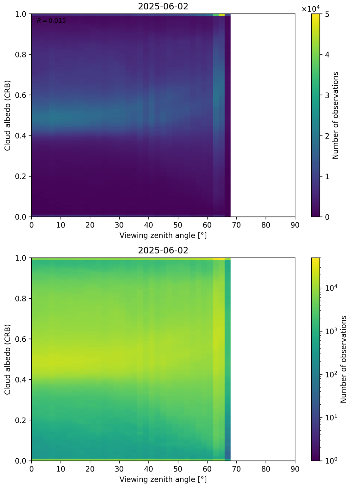
Figure 106: Scatter density plot of “Viewing zenith angle” against “Cloud albedo (CRB)” for 2025-06-01 to 2025-06-03.
