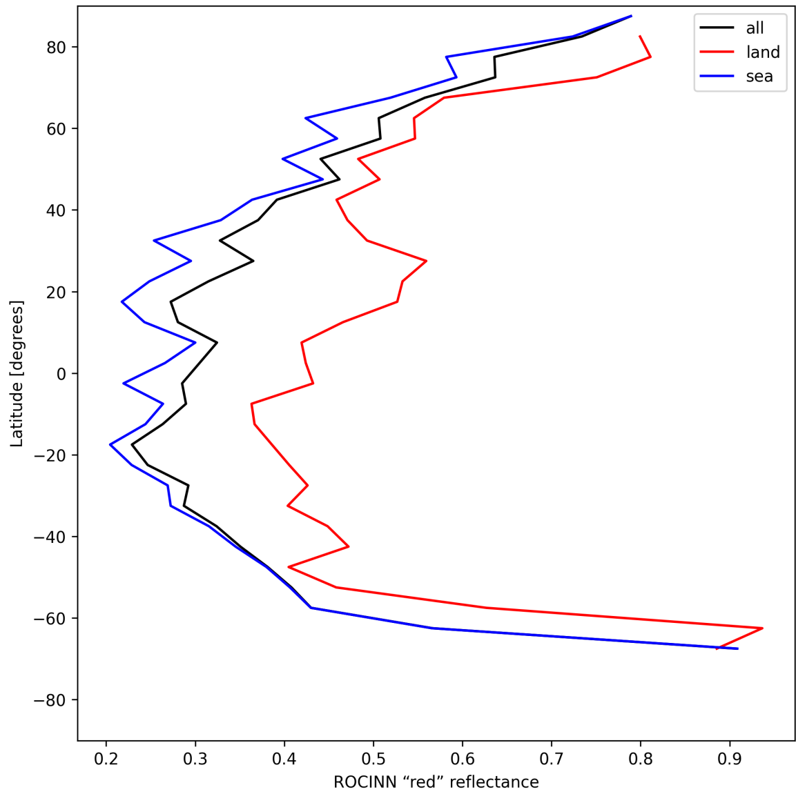
Figure 37: Zonal average of “ROCINN “red” reflectance” for 2025-06-01 to 2025-06-03.
