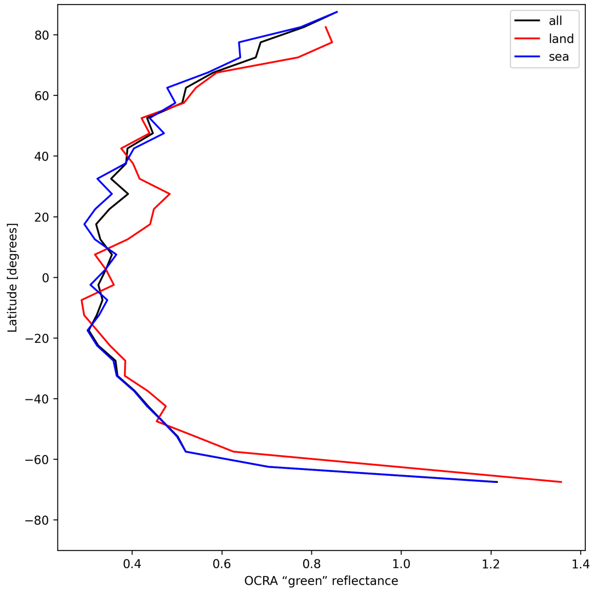
Figure 36: Zonal average of “OCRA “green” reflectance” for 2025-06-01 to 2025-06-03.
