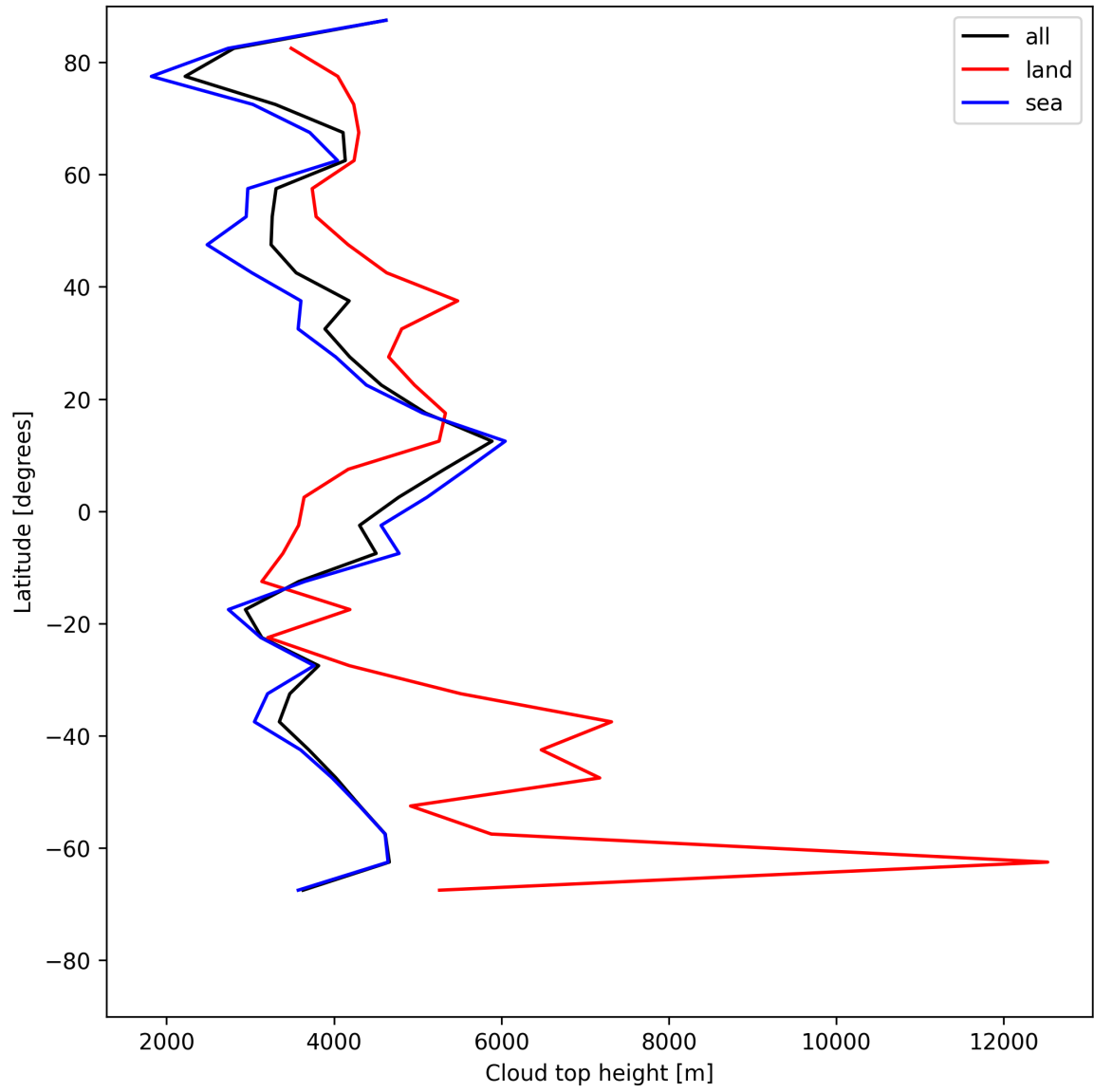
Figure 24: Zonal average of “Cloud top height” for 2025-06-01 to 2025-06-03.
