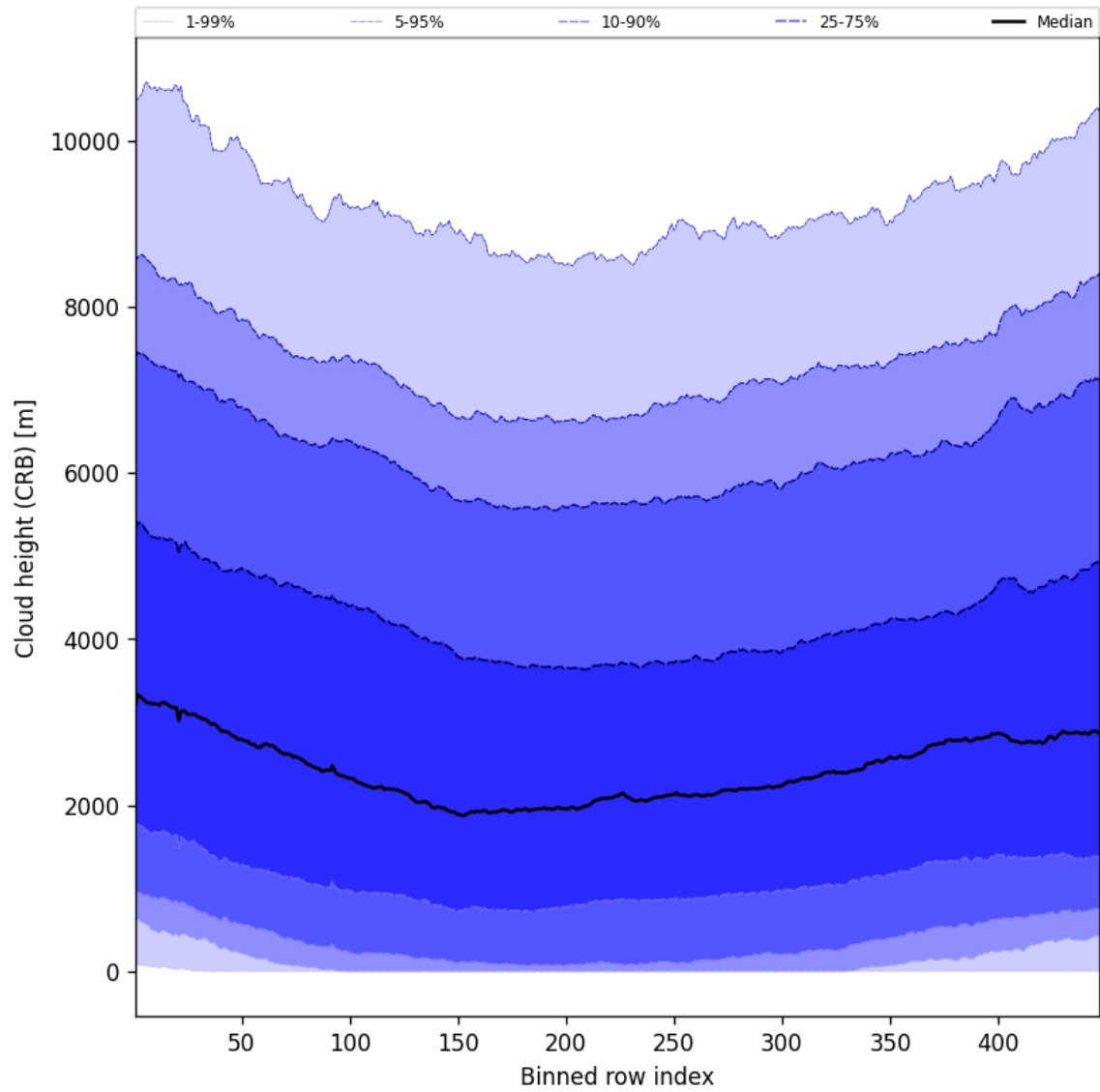
Figure 59: Along track statistics of “Cloud height (CRB)” for 2025-06-01 to 2025-06-03
