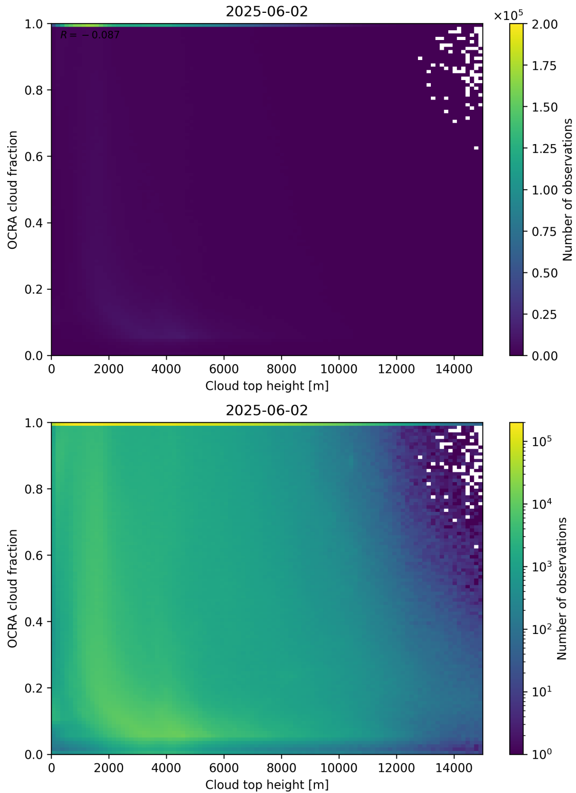
Figure 87: Scatter density plot of “Cloud top height” against “OCRA cloud fraction” for 2025-06-01 to 2025-06-03.
