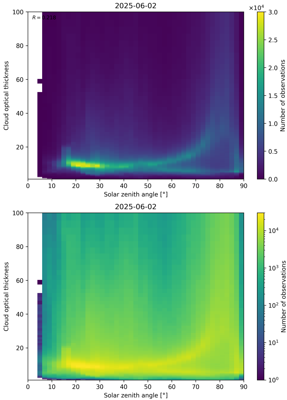
Figure 103: Scatter density plot of “Solar zenith angle” against “Cloud optical thickness” for 2025-06-01 to 2025-06-03.
