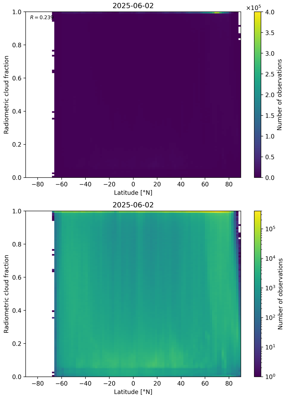
Figure 92: Scatter density plot of “Latitude” against “Radiometric cloud fraction” for 2025-06-01 to 2025-06-03.
