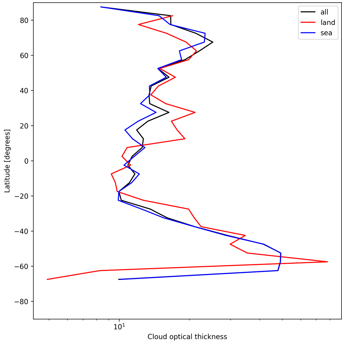
Figure 25: Zonal average of “Cloud optical thickness” for 2025-06-01 to 2025-06-03.
