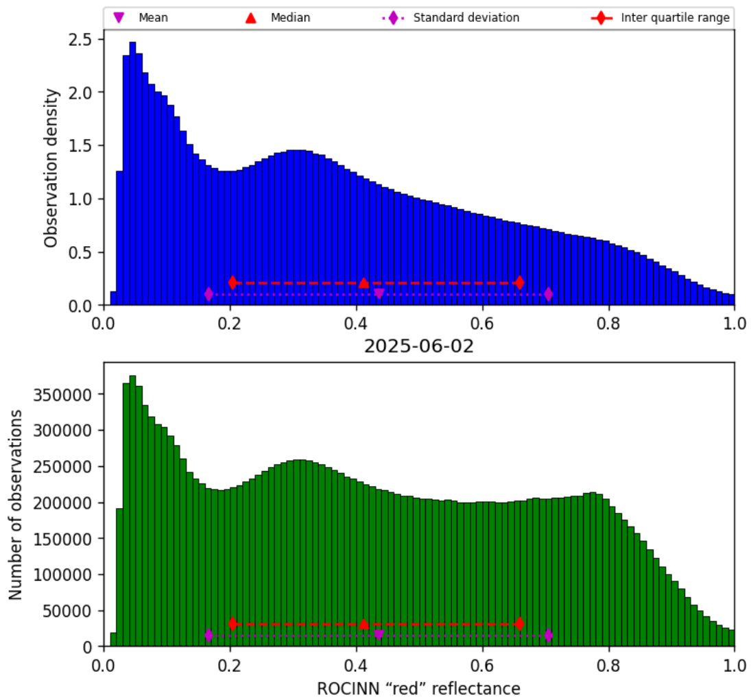
Figure 53: Histogram of “ROCINN “red” reflectance” for 2025-06-01 to 2025-06-03
