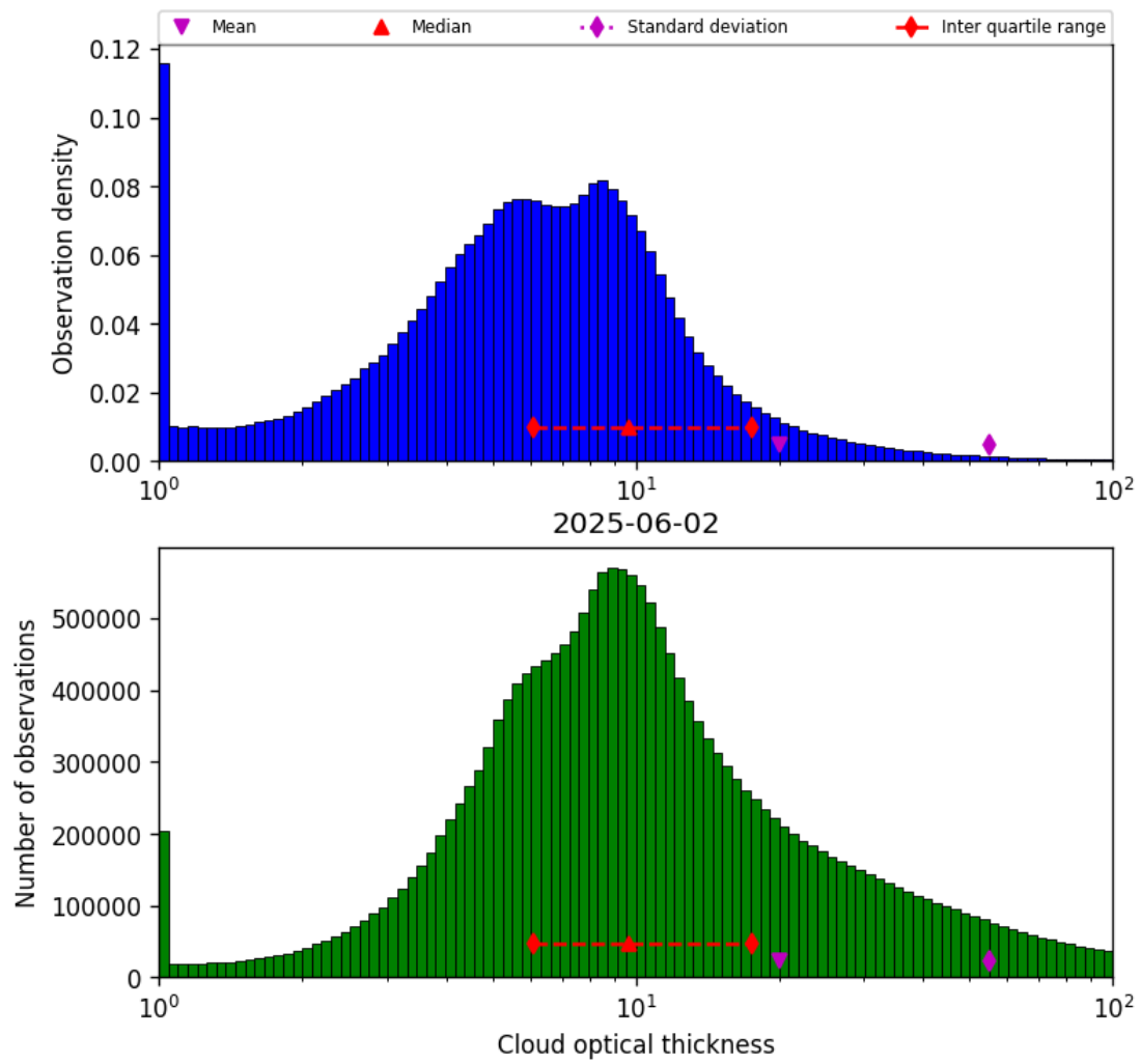
Figure 41: Histogram of “Cloud optical thickness” for 2025-06-01 to 2025-06-03
