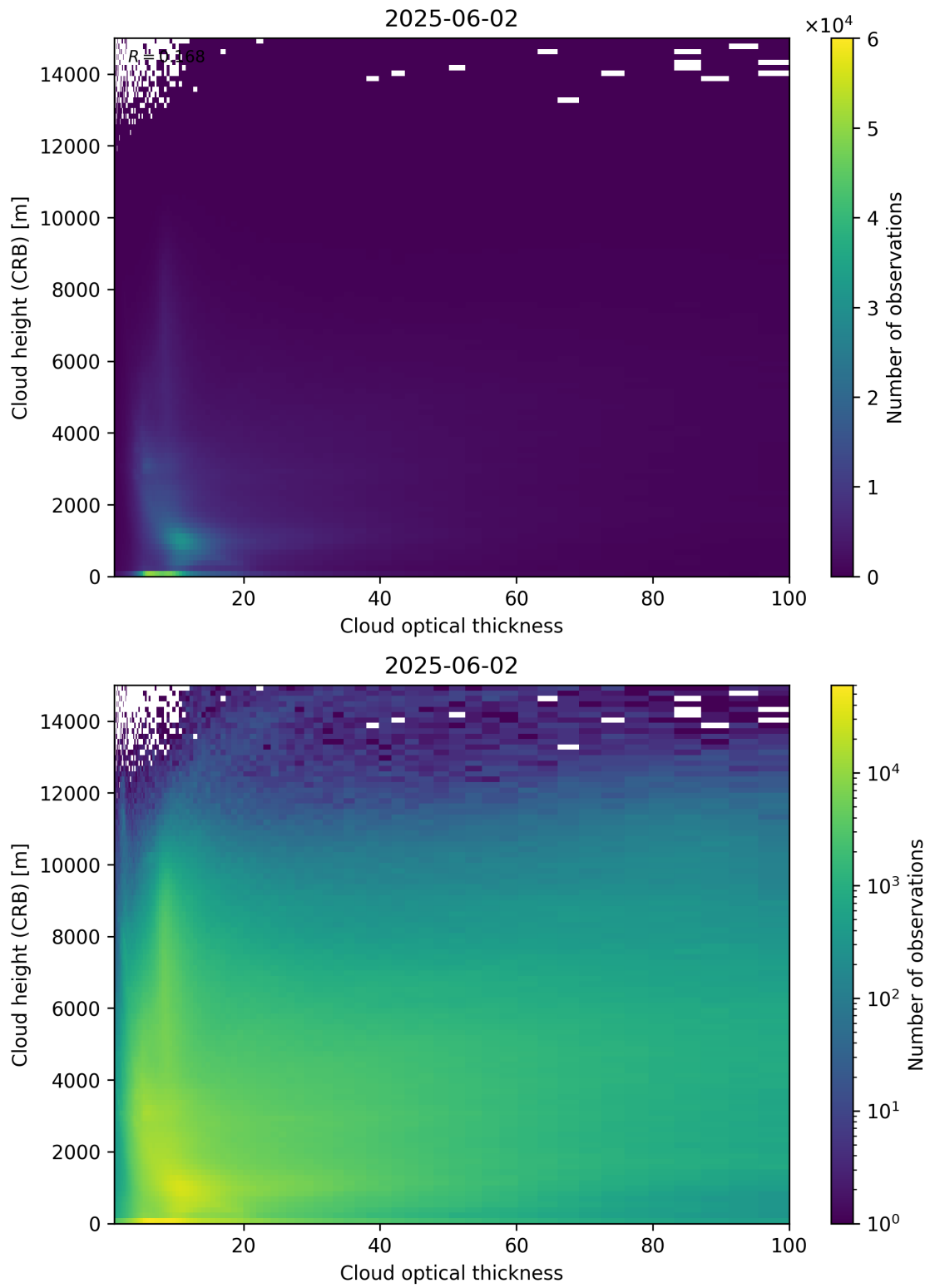
Figure 85: Scatter density plot of “Cloud optical thickness” against “Cloud height (CRB)” for 2025-06-01 to 2025-06-03.
