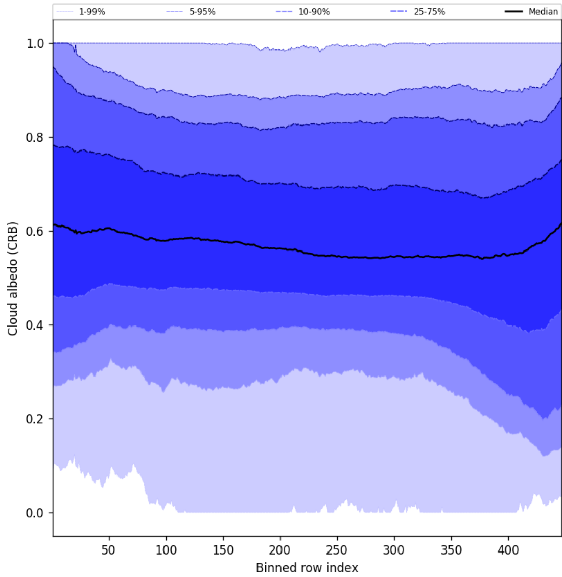
Figure 60: Along track statistics of “Cloud albedo (CRB)” for 2025-06-01 to 2025-06-03
