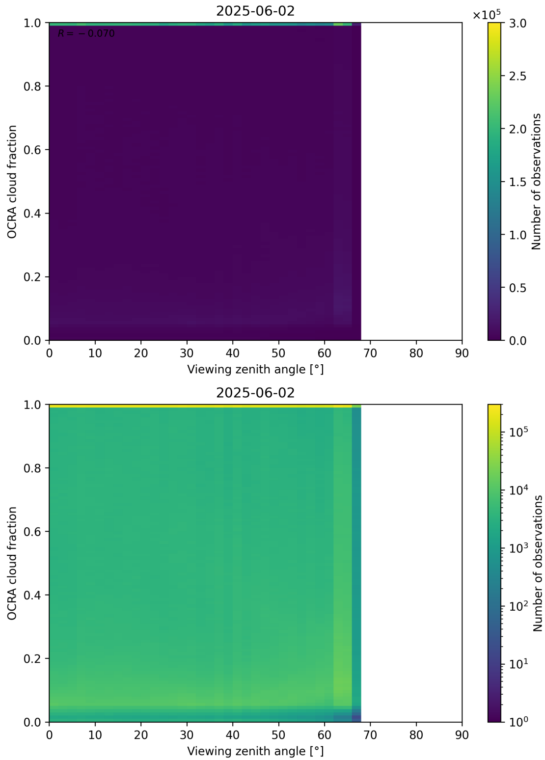
Figure 108: Scatter density plot of “Viewing zenith angle” against “OCRA cloud fraction” for 2025-06-01 to 2025-06-03.
