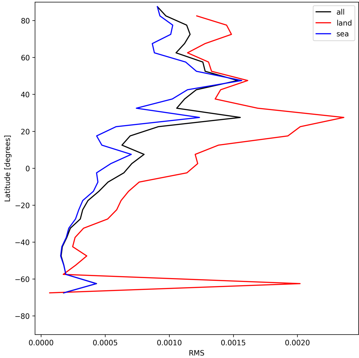
Figure 31: Zonal average of “RMS” for 2025-06-01 to 2025-06-03.
