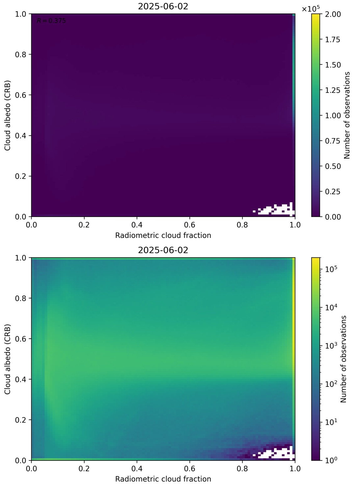
Figure 71: Scatter density plot of “Radiometric cloud fraction” against “Cloud albedo (CRB)” for 2025-06-01 to 2025-06-03.
