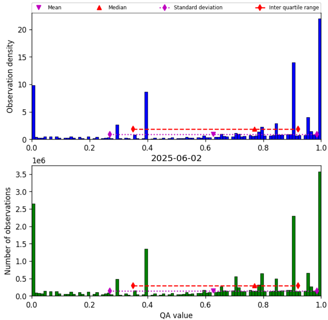
Figure 38: Histogram of “QA value” for 2025-06-01 to 2025-06-03
