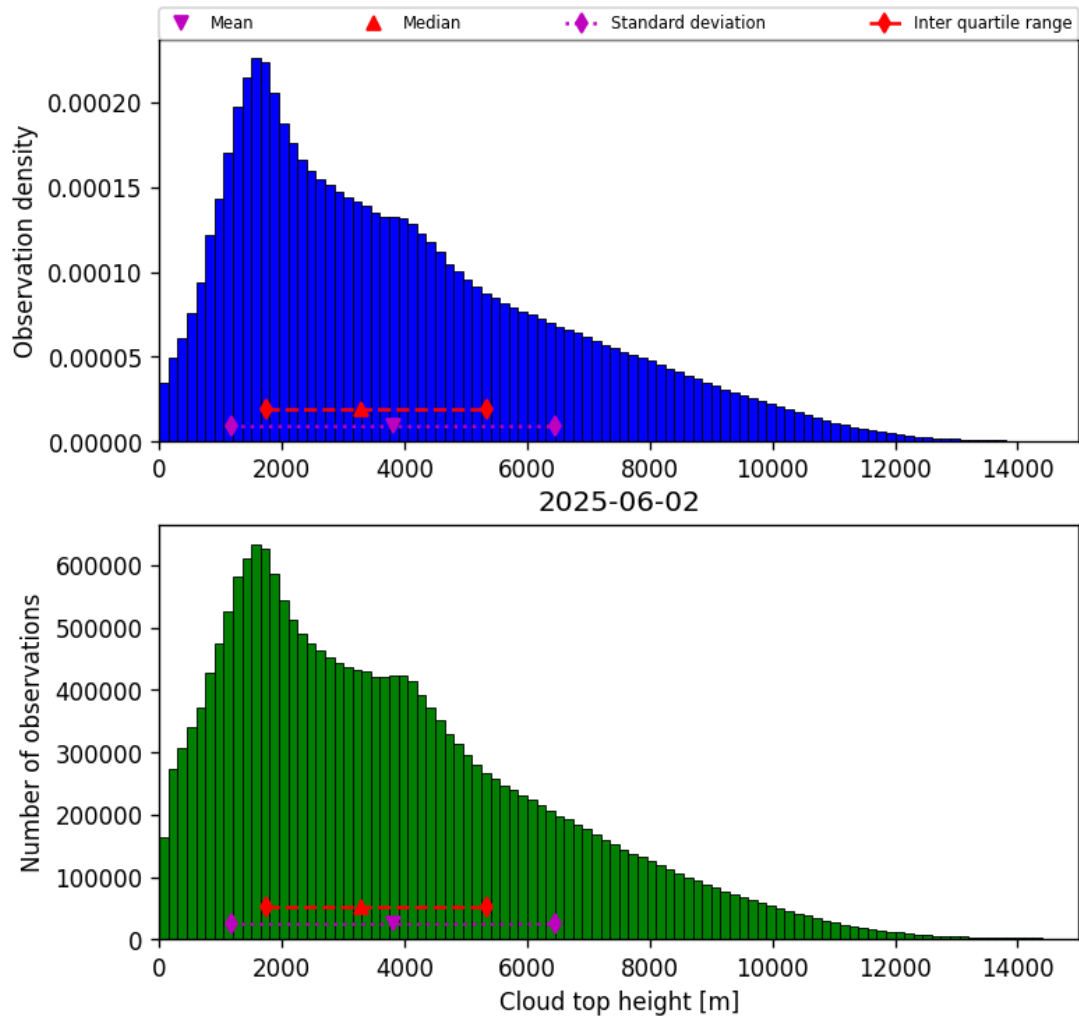
Figure 40: Histogram of “Cloud top height” for 2025-06-01 to 2025-06-03
