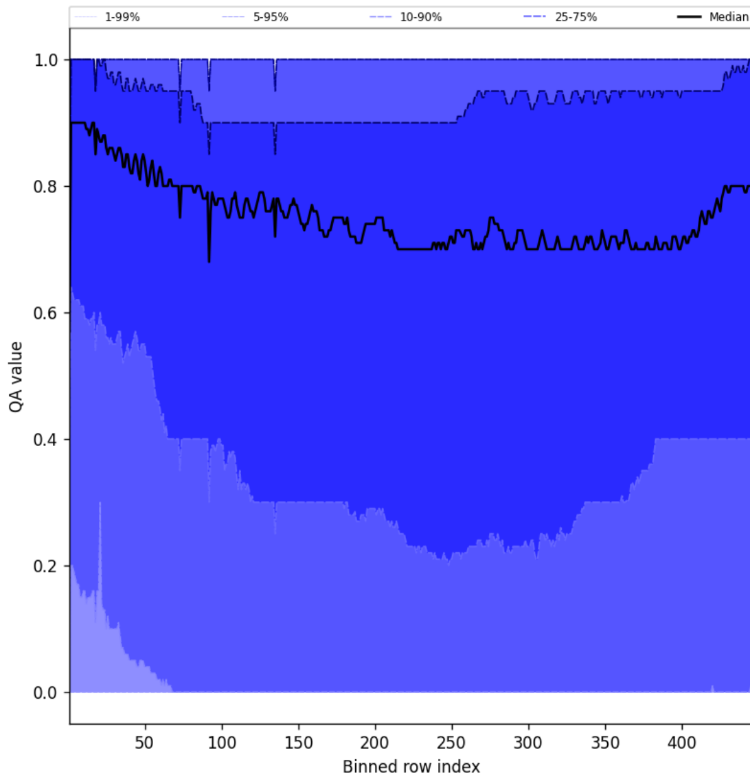
Figure 54: Along track statistics of “QA value” for 2025-06-01 to 2025-06-03
