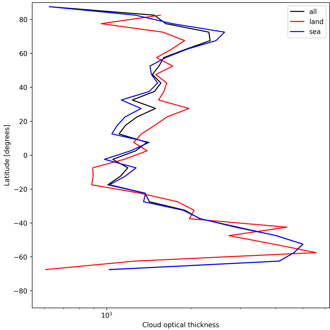
Figure 25: Zonal average of “Cloud optical thickness” for 2025-06-02 to 2025-06-04.
