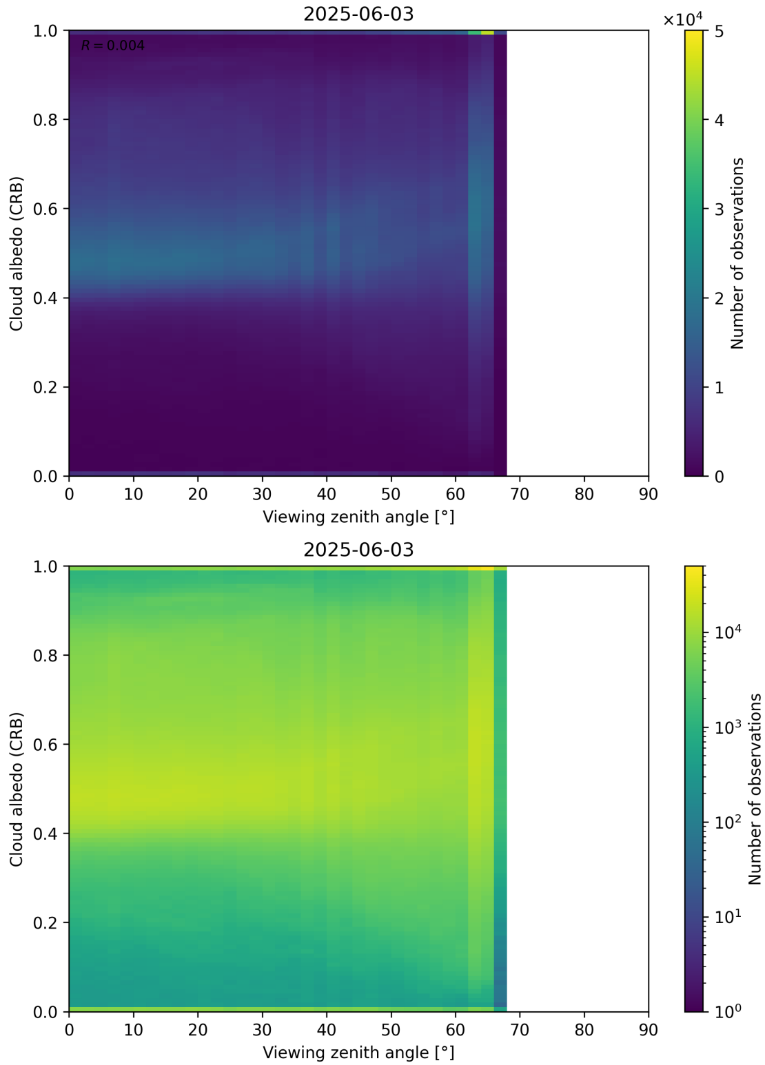
Figure 106: Scatter density plot of “Viewing zenith angle” against “Cloud albedo (CRB)” for 2025-06-02 to 2025-06-04.
