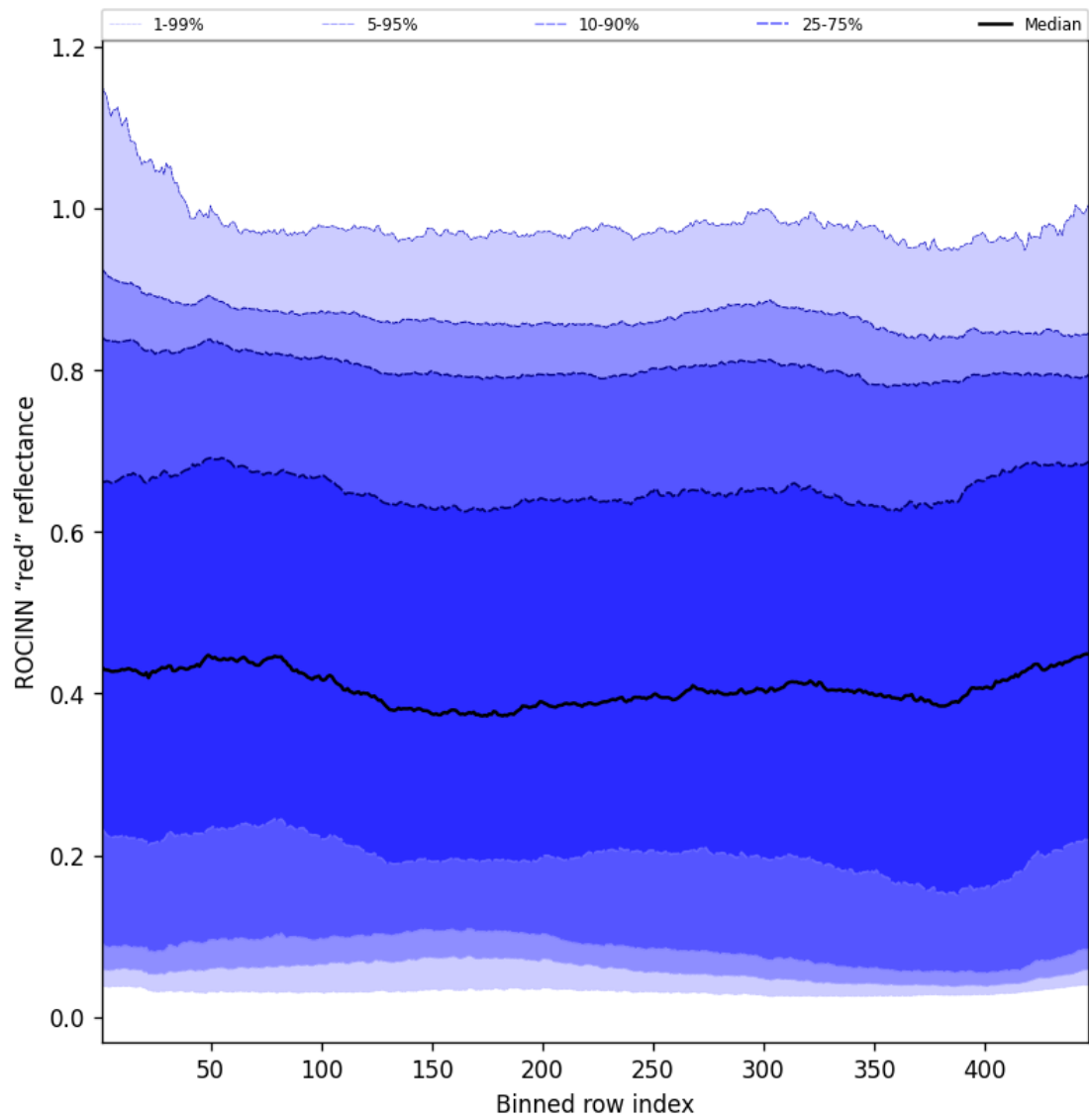
Figure 69: Along track statistics of “ROCINN “red” reflectance” for 2025-06-02 to 2025-06-04
