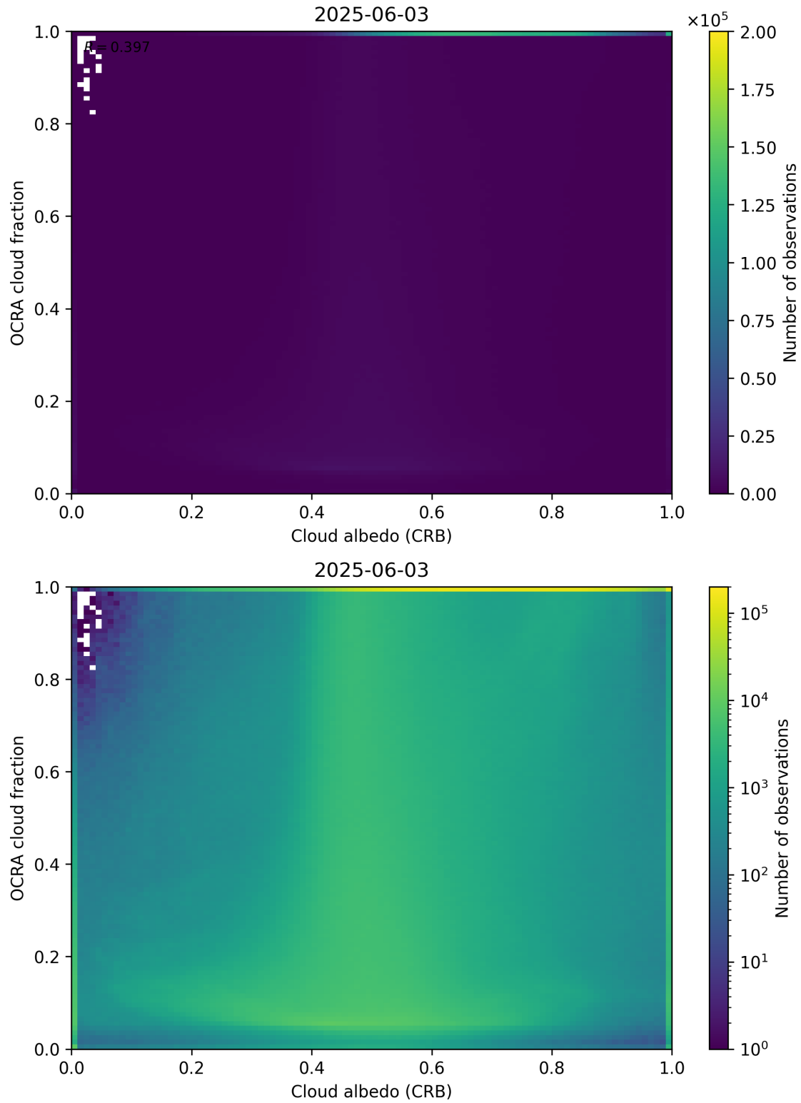
Figure 70: Scatter density plot of “Cloud albedo (CRB)” against “OCRA cloud fraction” for 2025-06-02 to 2025-06-04.
