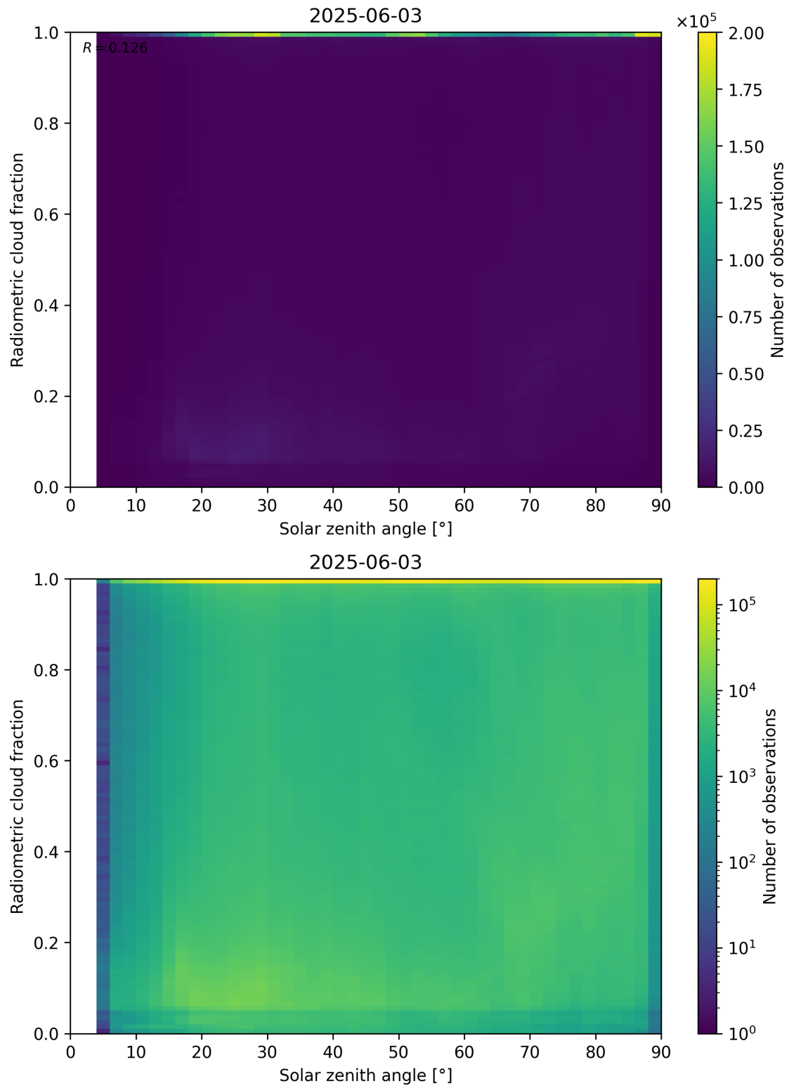
Figure 99: Scatter density plot of “Solar zenith angle” against “Radiometric cloud fraction” for 2025-06-02 to 2025-06-04.
