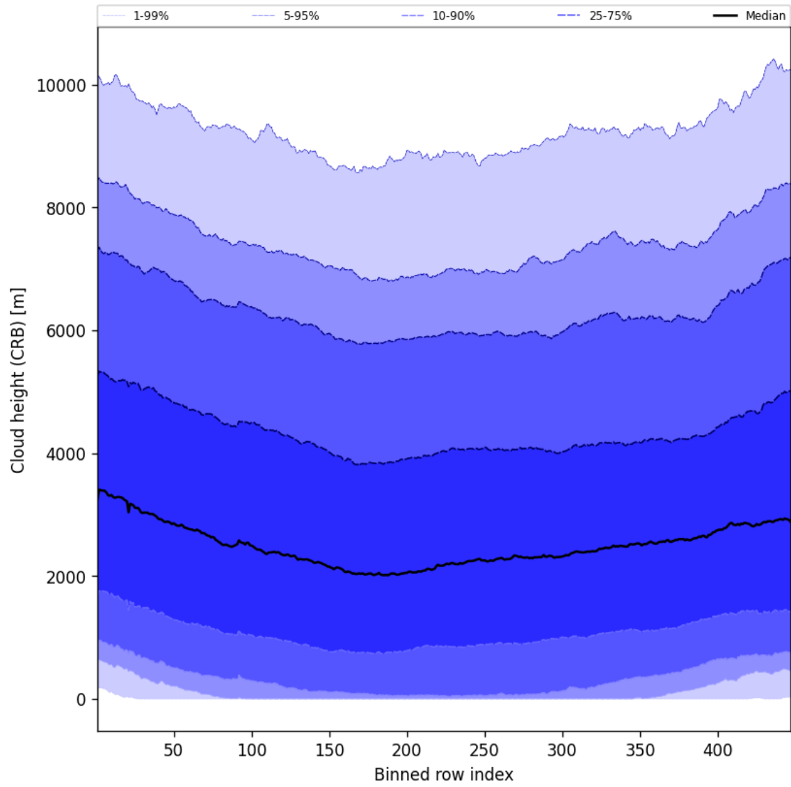
Figure 59: Along track statistics of “Cloud height (CRB)” for 2025-06-02 to 2025-06-04
