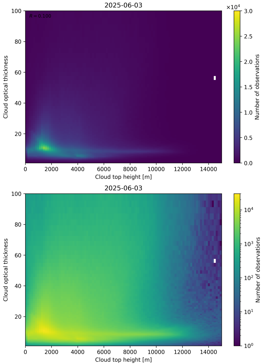
Figure 90: Scatter density plot of “Cloud top height” against “Cloud optical thickness” for 2025-06-02 to 2025-06-04.
