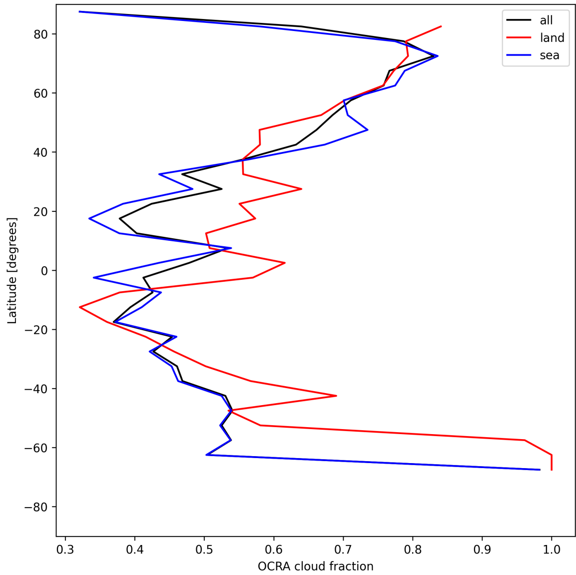
Figure 34: Zonal average of “OCRA cloud fraction” for 2025-06-02 to 2025-06-04.
