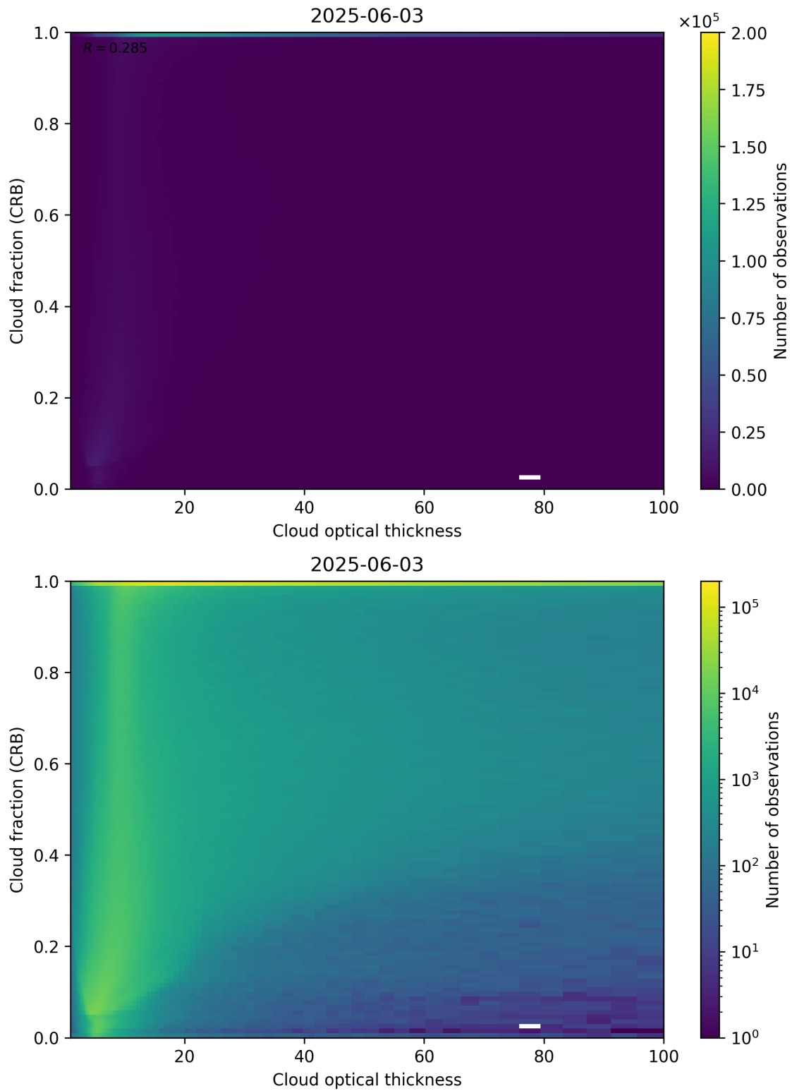
Figure 84: Scatter density plot of “Cloud optical thickness” against “Cloud fraction (CRB)” for 2025-06-02 to 2025-06-04.
