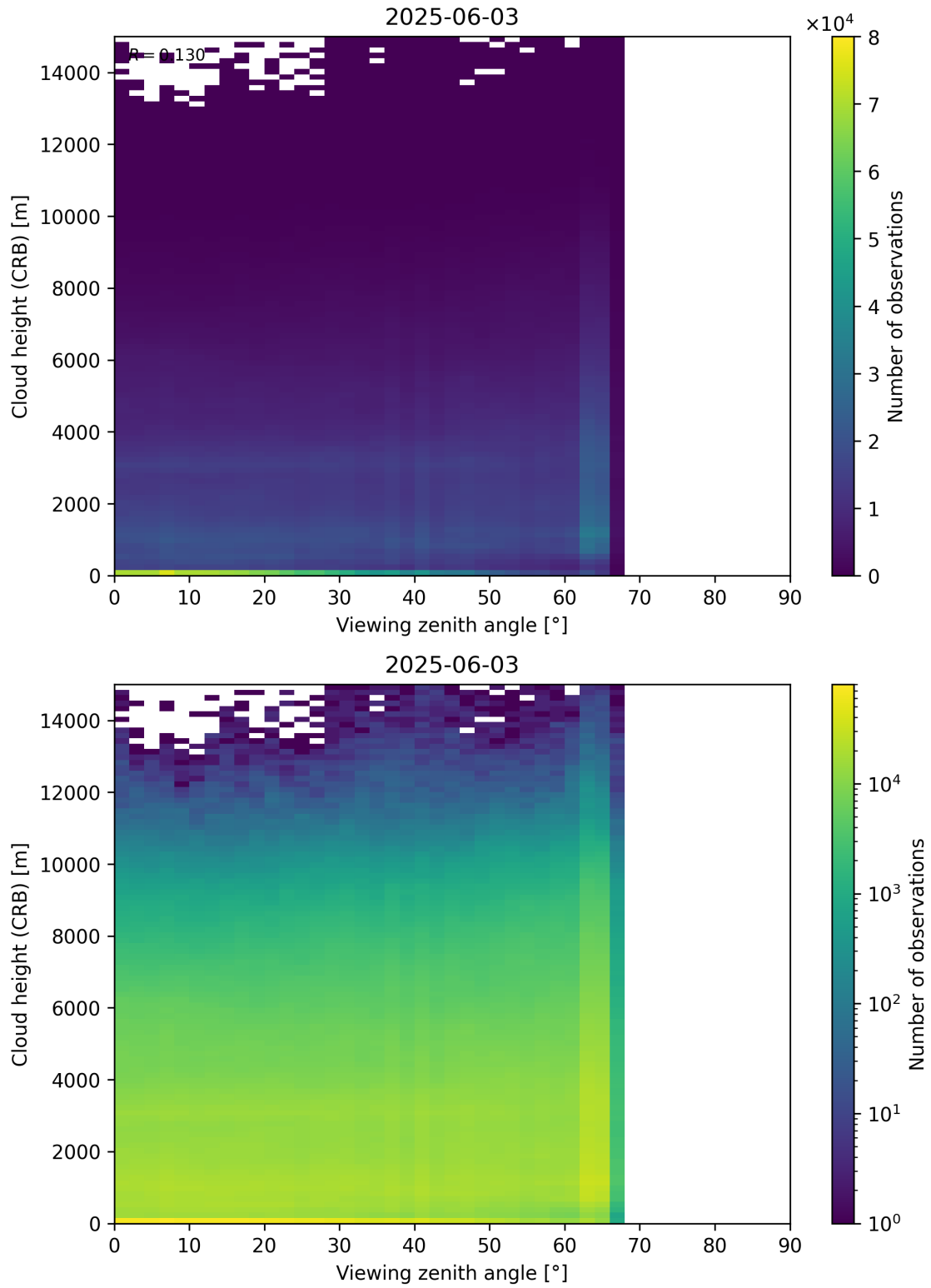
Figure 110: Scatter density plot of “Viewing zenith angle” against “Cloud height (CRB)” for 2025-06-02 to 2025-06-04.
