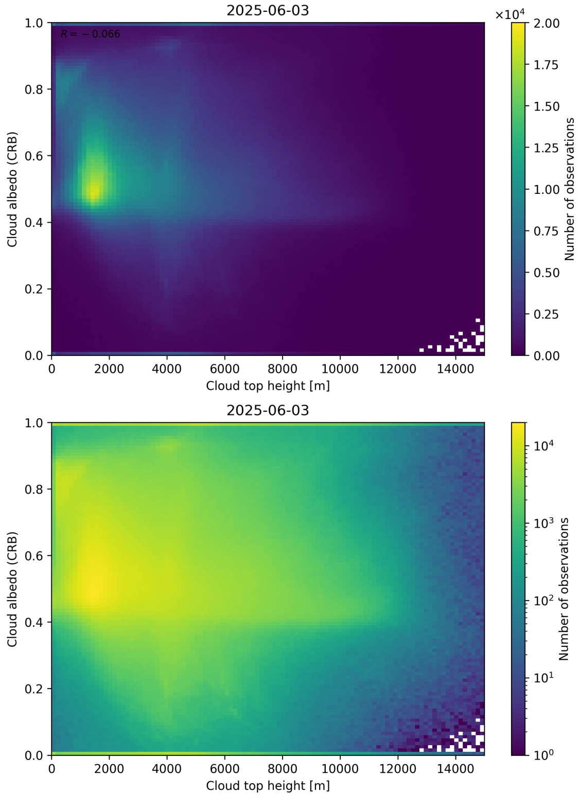
Figure 86: Scatter density plot of “Cloud top height” against “Cloud albedo (CRB)” for 2025-06-02 to 2025-06-04.
