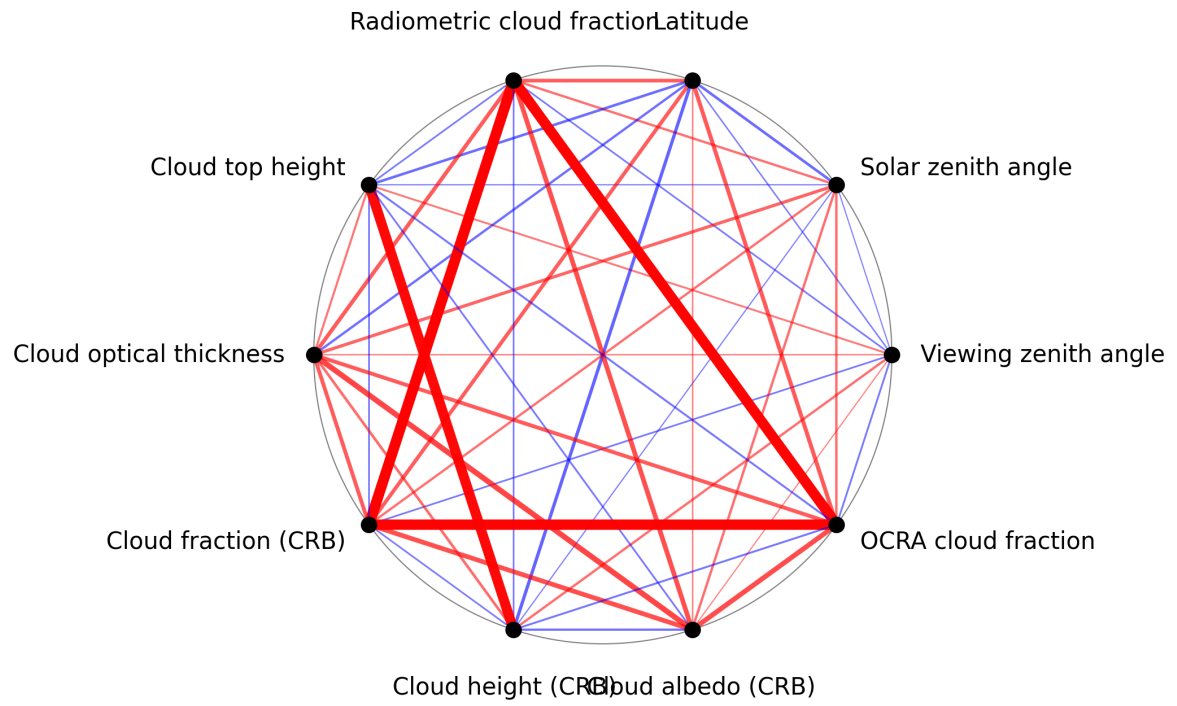
Figure 1: Map of correlation graph for 2025-06-02 to 2025-06-04.
