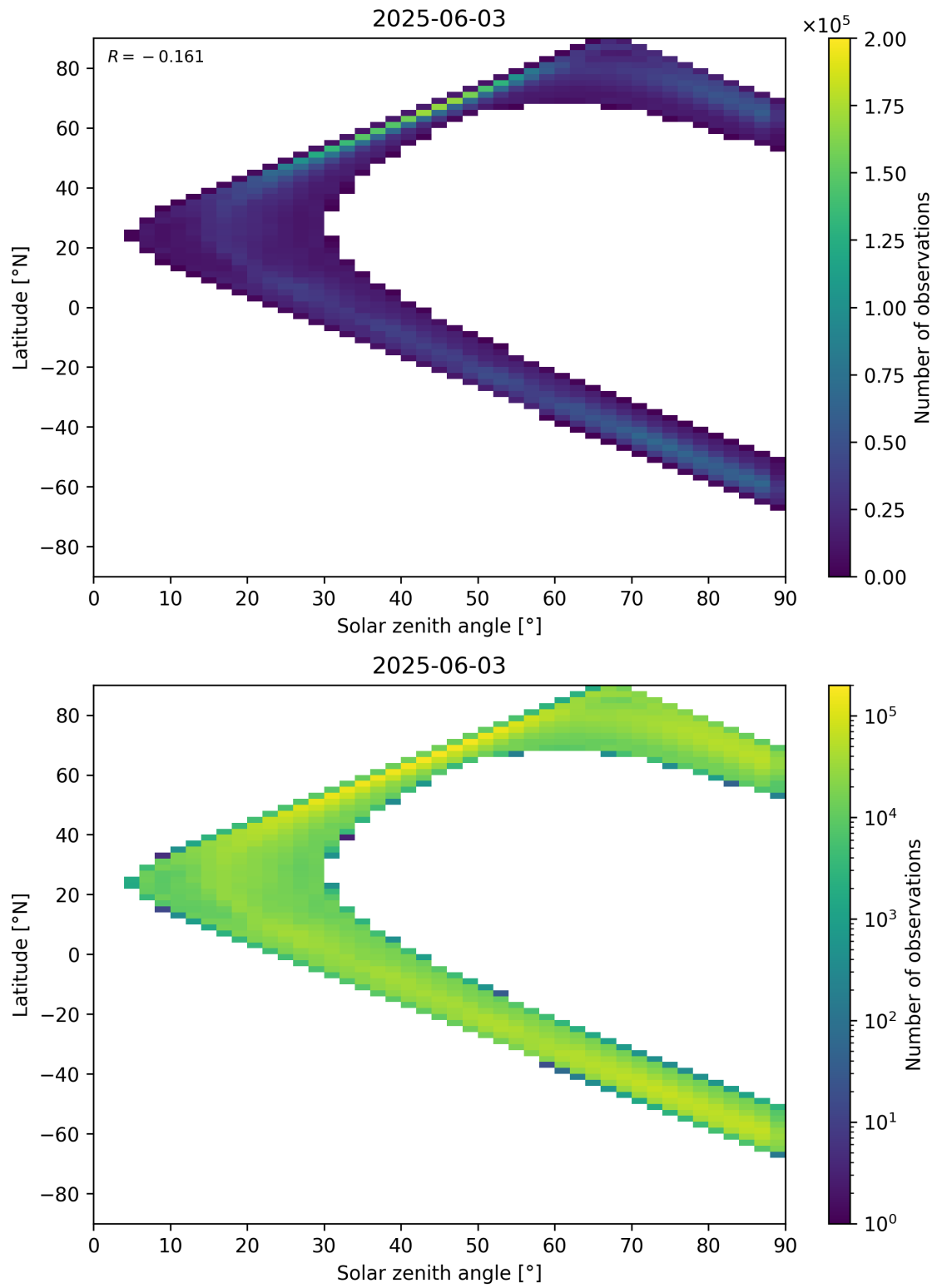
Figure 105: Scatter density plot of “Solar zenith angle” against “Latitude” for 2025-06-02 to 2025-06-04.
