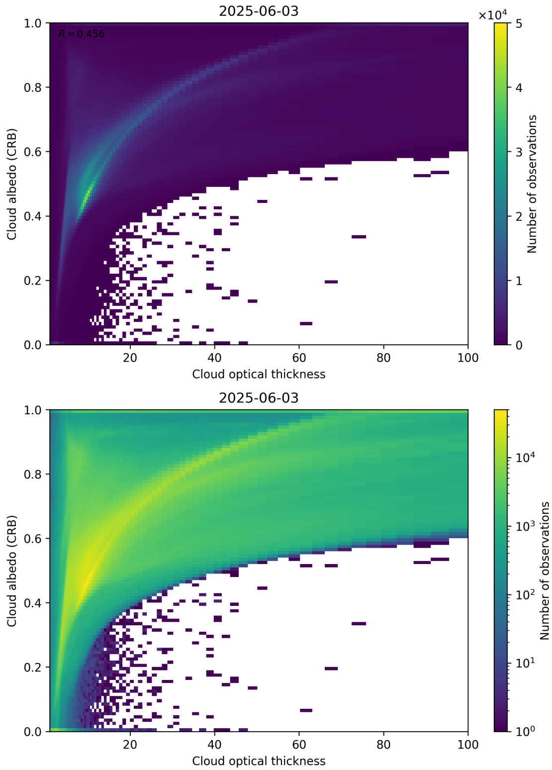
Figure 82: Scatter density plot of “Cloud optical thickness” against “Cloud albedo (CRB)” for 2025-06-02 to 2025-06-04.
