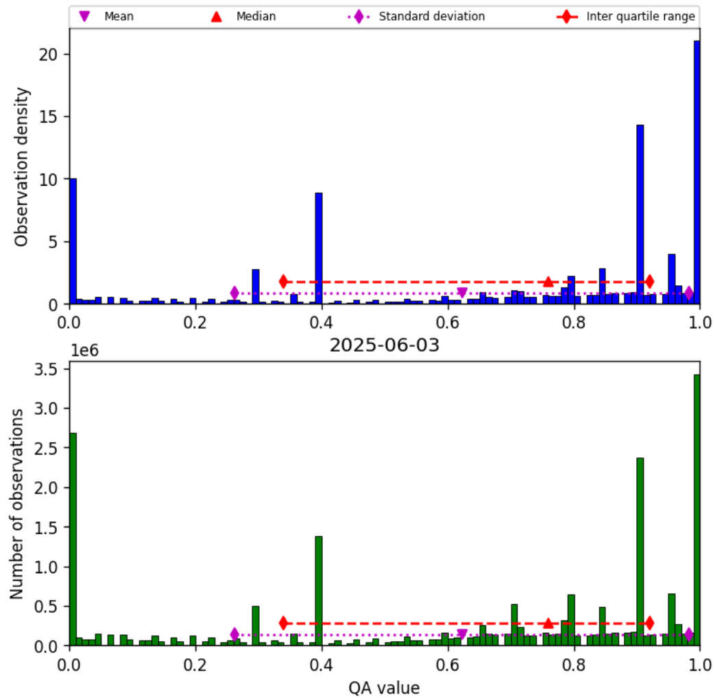
Figure 38: Histogram of “QA value” for 2025-06-02 to 2025-06-04
