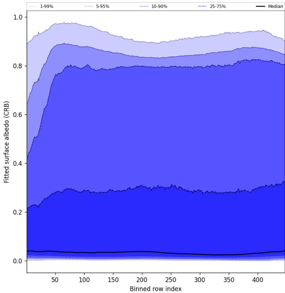
Figure 62: Along track statistics of “Fitted surface albedo (CRB)” for 2025-06-02 to 2025-06-04
