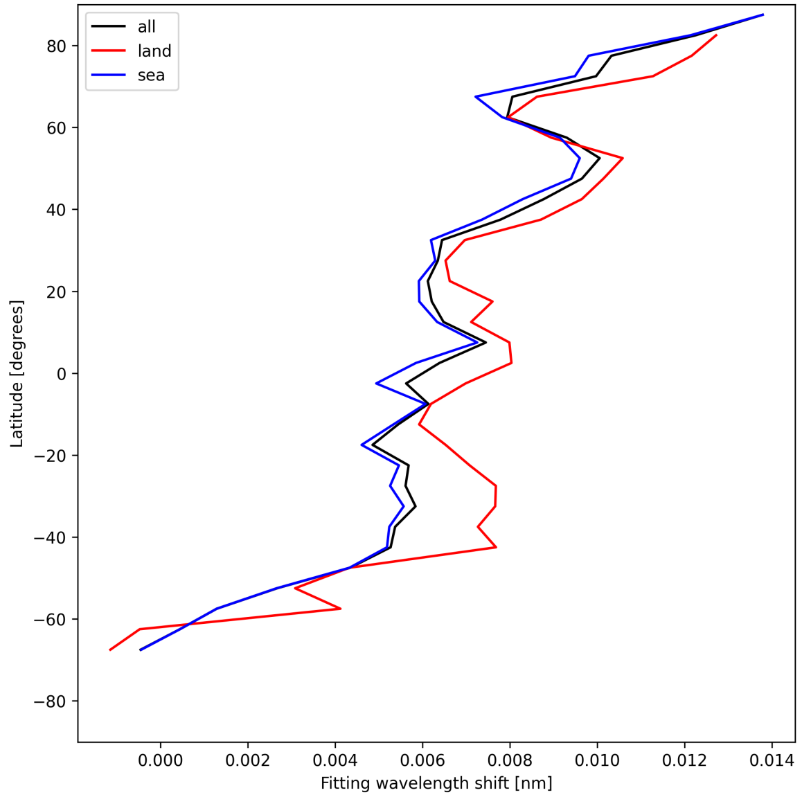
Figure 33: Zonal average of “Fitting wavelength shift” for 2025-06-02 to 2025-06-04.
