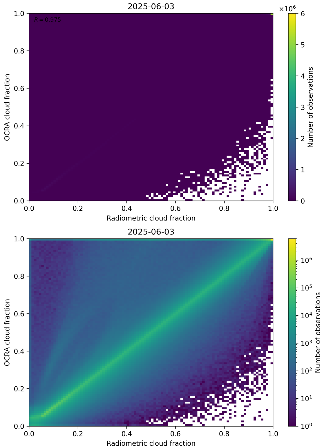
Figure 72: Scatter density plot of “Radiometric cloud fraction” against “OCRA cloud fraction” for 2025-06-02 to 2025-06-04.
