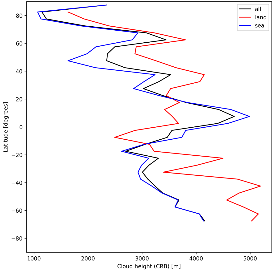
Figure 27: Zonal average of “Cloud height (CRB)” for 2025-06-02 to 2025-06-04.
