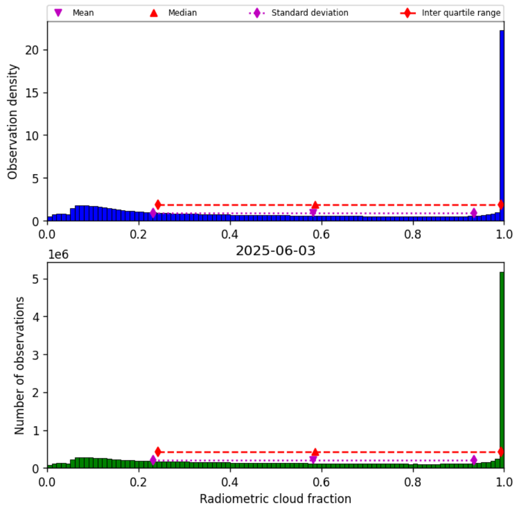
Figure 39: Histogram of “Radiometric cloud fraction” for 2025-06-02 to 2025-06-04
