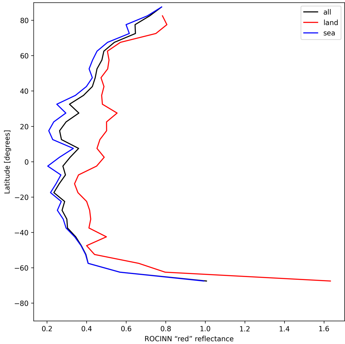
Figure 37: Zonal average of “ROCINN “red” reflectance” for 2025-06-02 to 2025-06-04.
