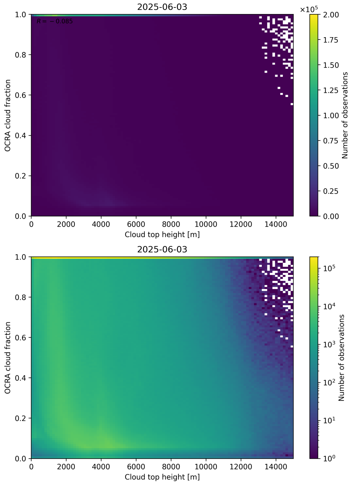
Figure 87: Scatter density plot of “Cloud top height” against “OCRA cloud fraction” for 2025-06-02 to 2025-06-04.
