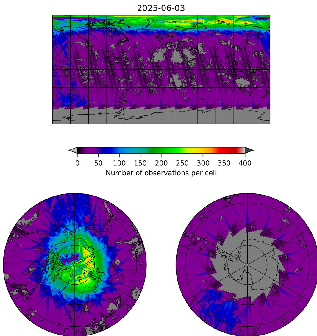
Figure 21: Map of the number of observations for 2025-06-02 to 2025-06-04
