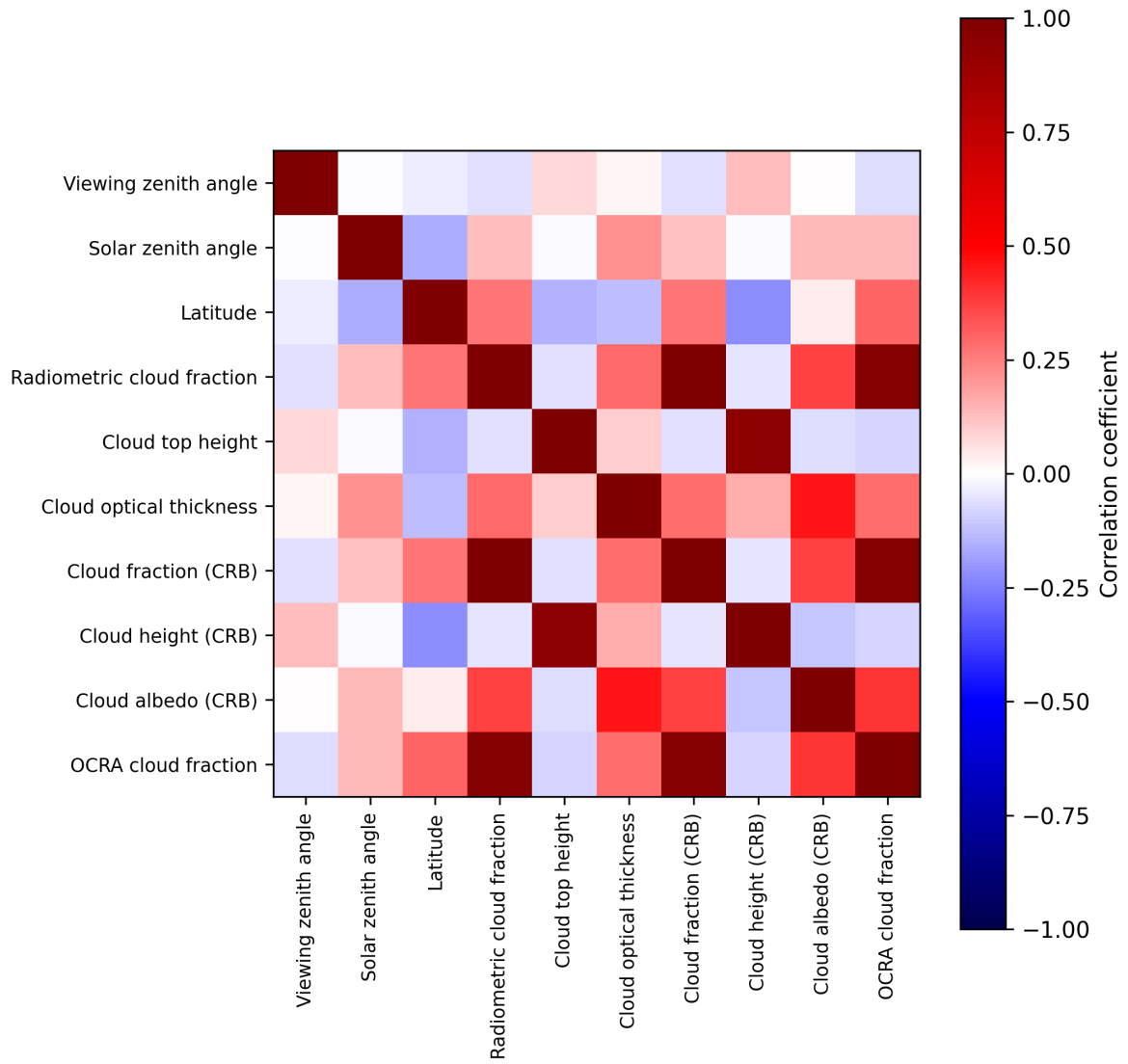
Figure 2: Map of correlation matrix for 2025-06-02 to 2025-06-04.
