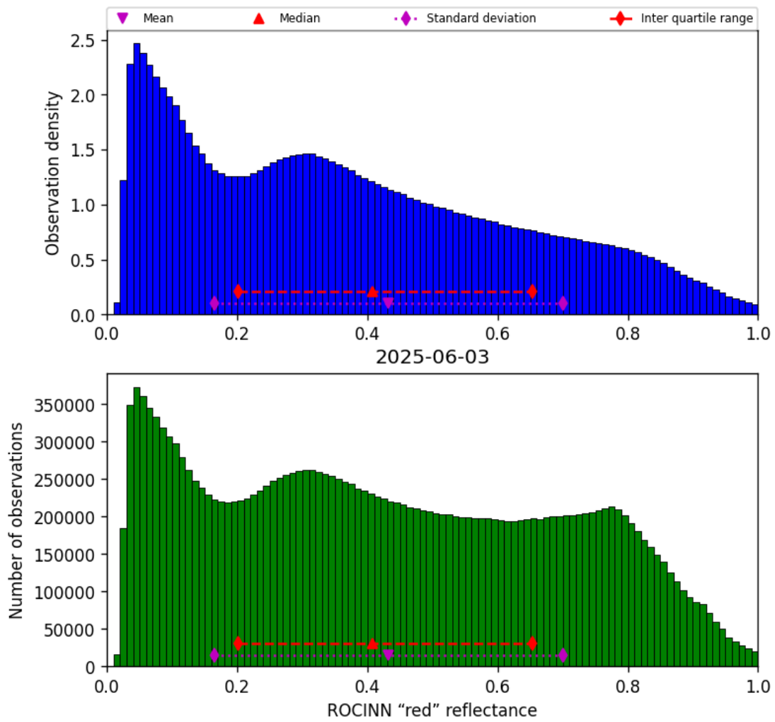
Figure 53: Histogram of “ROCINN “red” reflectance” for 2025-06-02 to 2025-06-04
