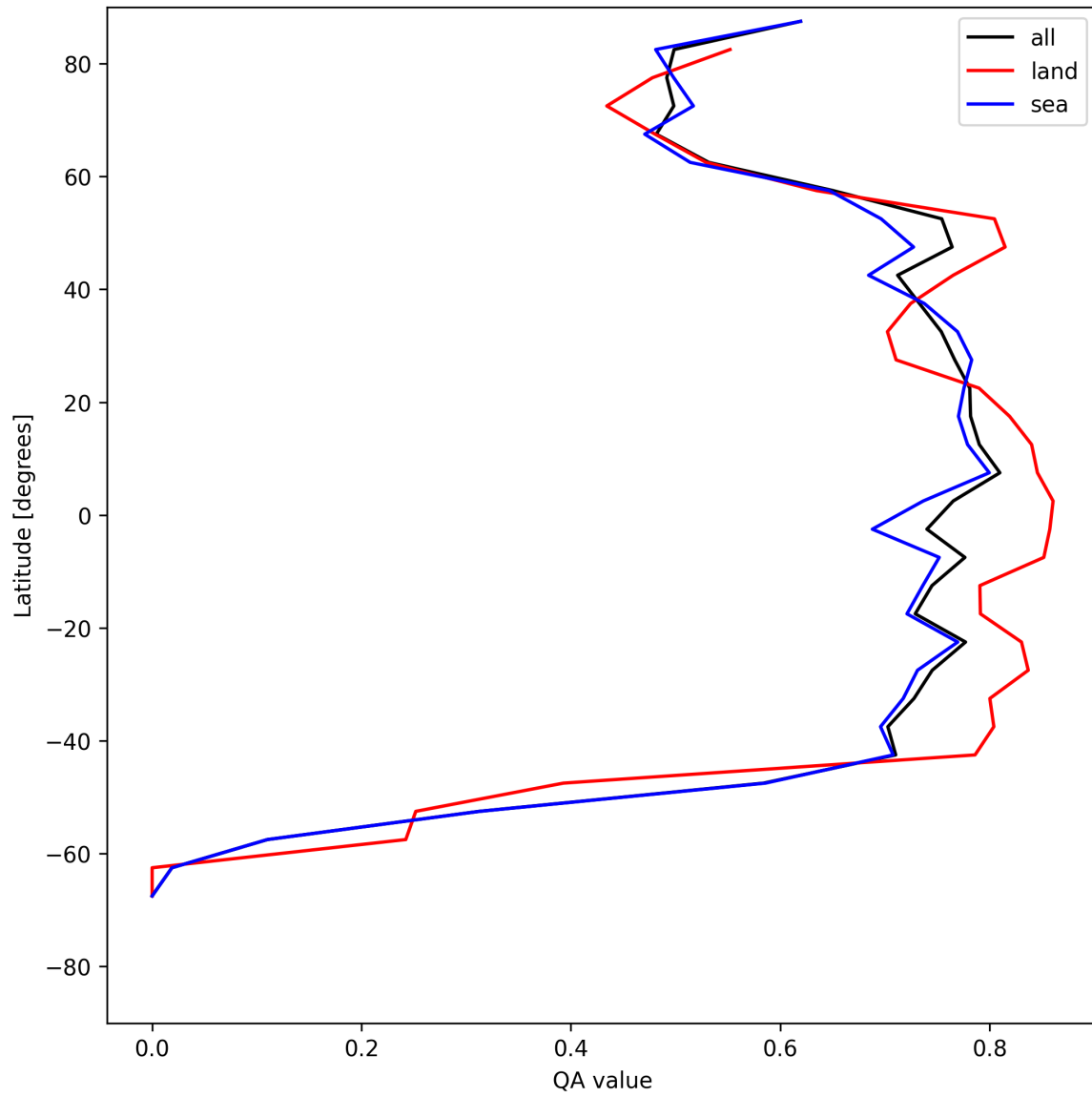
Figure 22: Zonal average of “QA value” for 2025-06-02 to 2025-06-04.
