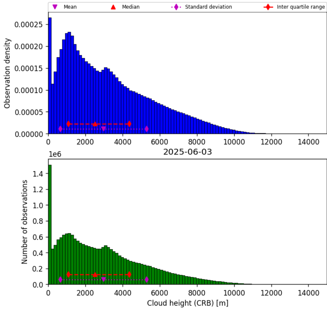
Figure 43: Histogram of “Cloud height (CRB)” for 2025-06-02 to 2025-06-04
