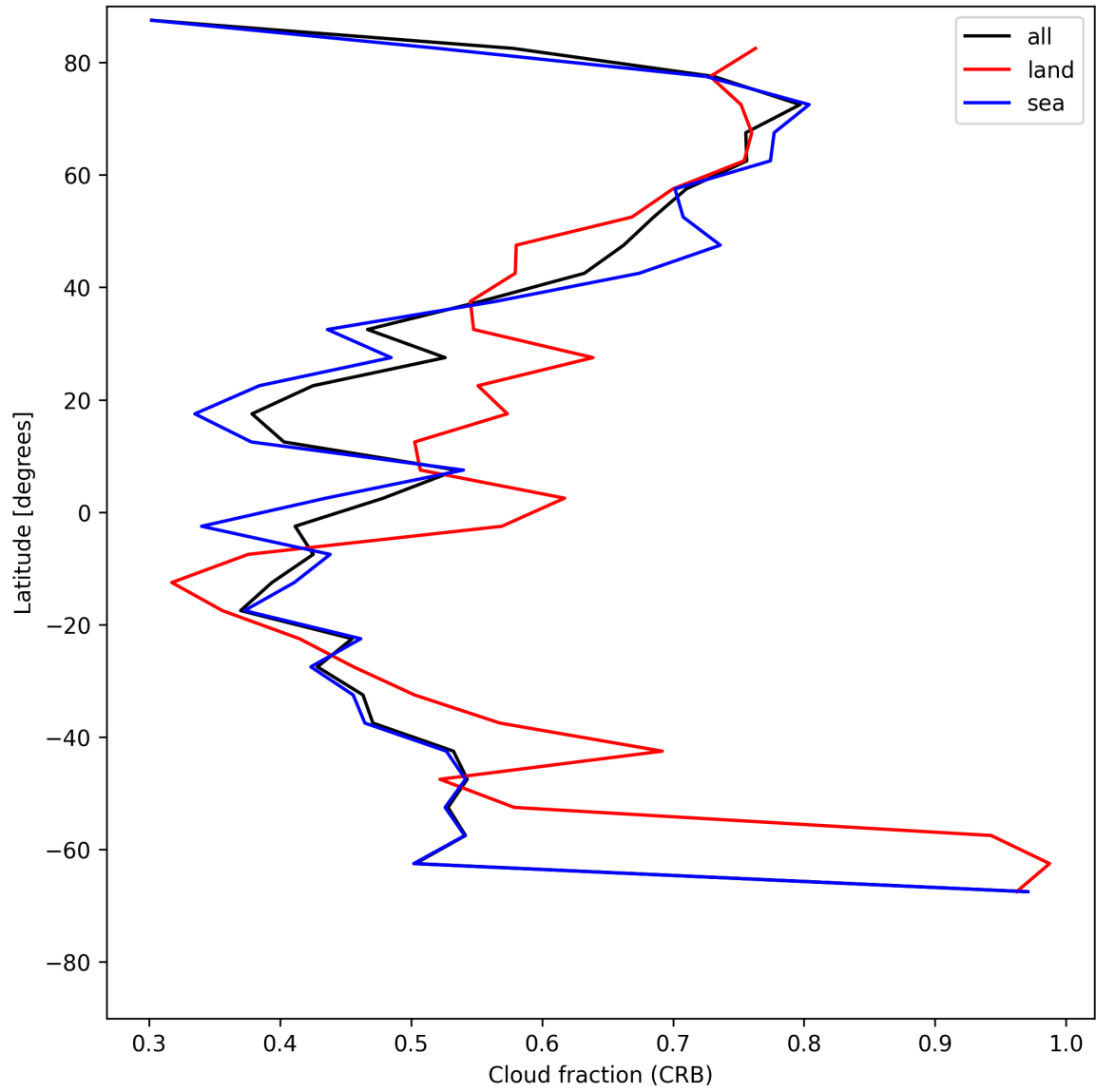
Figure 26: Zonal average of “Cloud fraction (CRB)” for 2025-06-02 to 2025-06-04.
