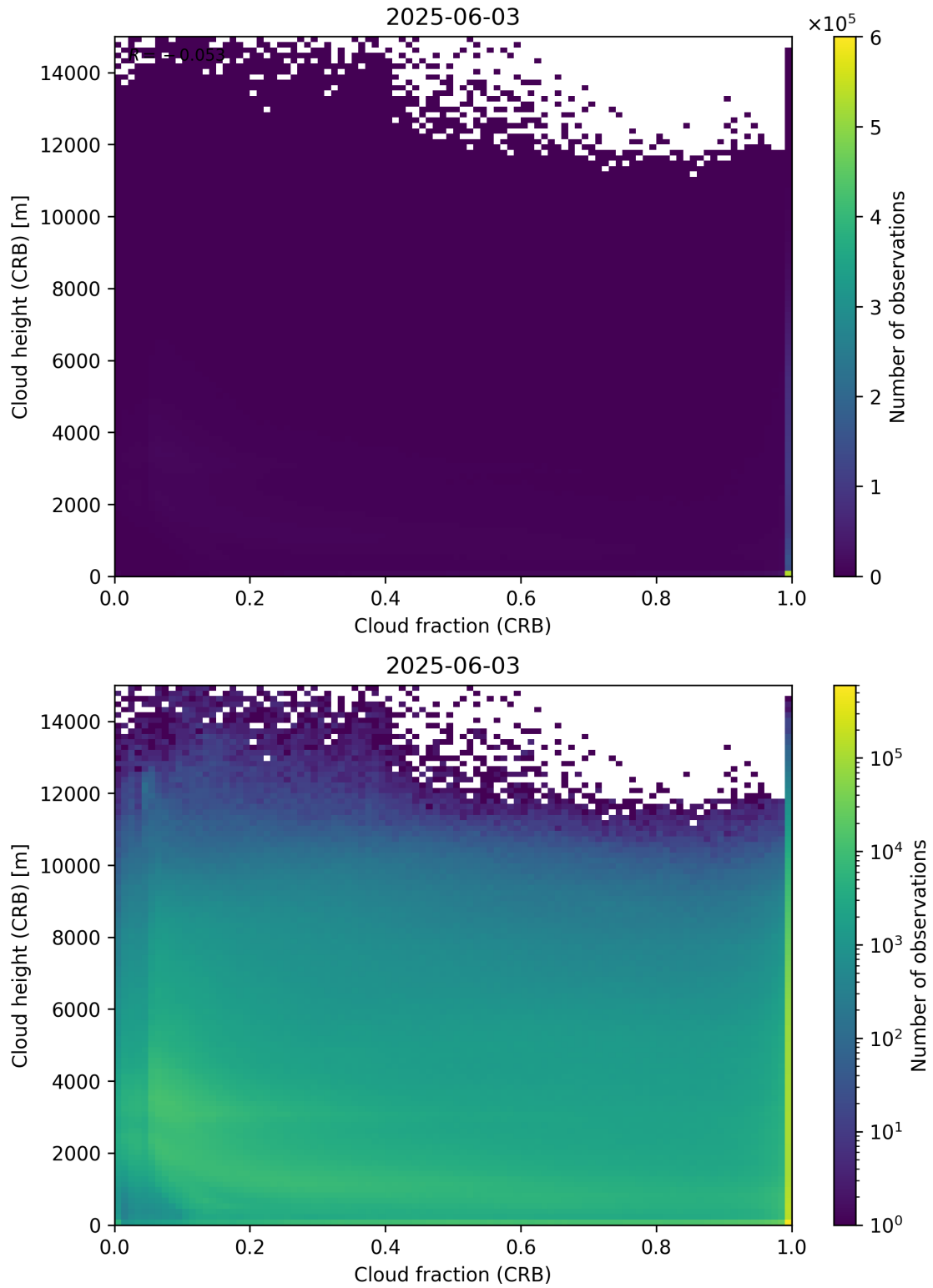
Figure 79: Scatter density plot of “Cloud fraction (CRB)” against “Cloud height (CRB)” for 2025-06-02 to 2025-06-04.
