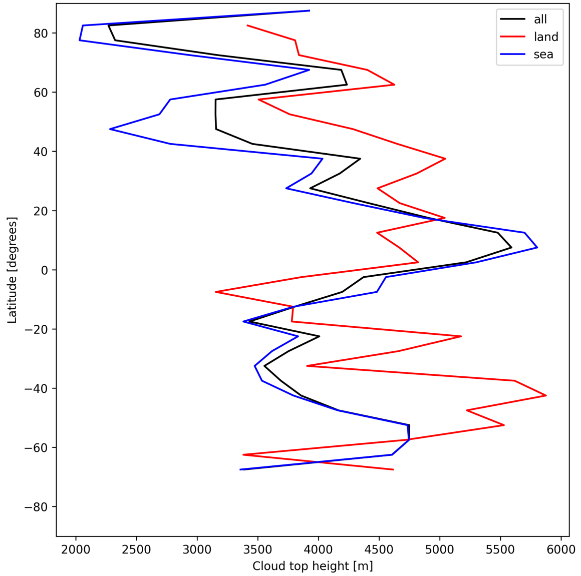
Figure 24: Zonal average of “Cloud top height” for 2025-06-02 to 2025-06-04.
