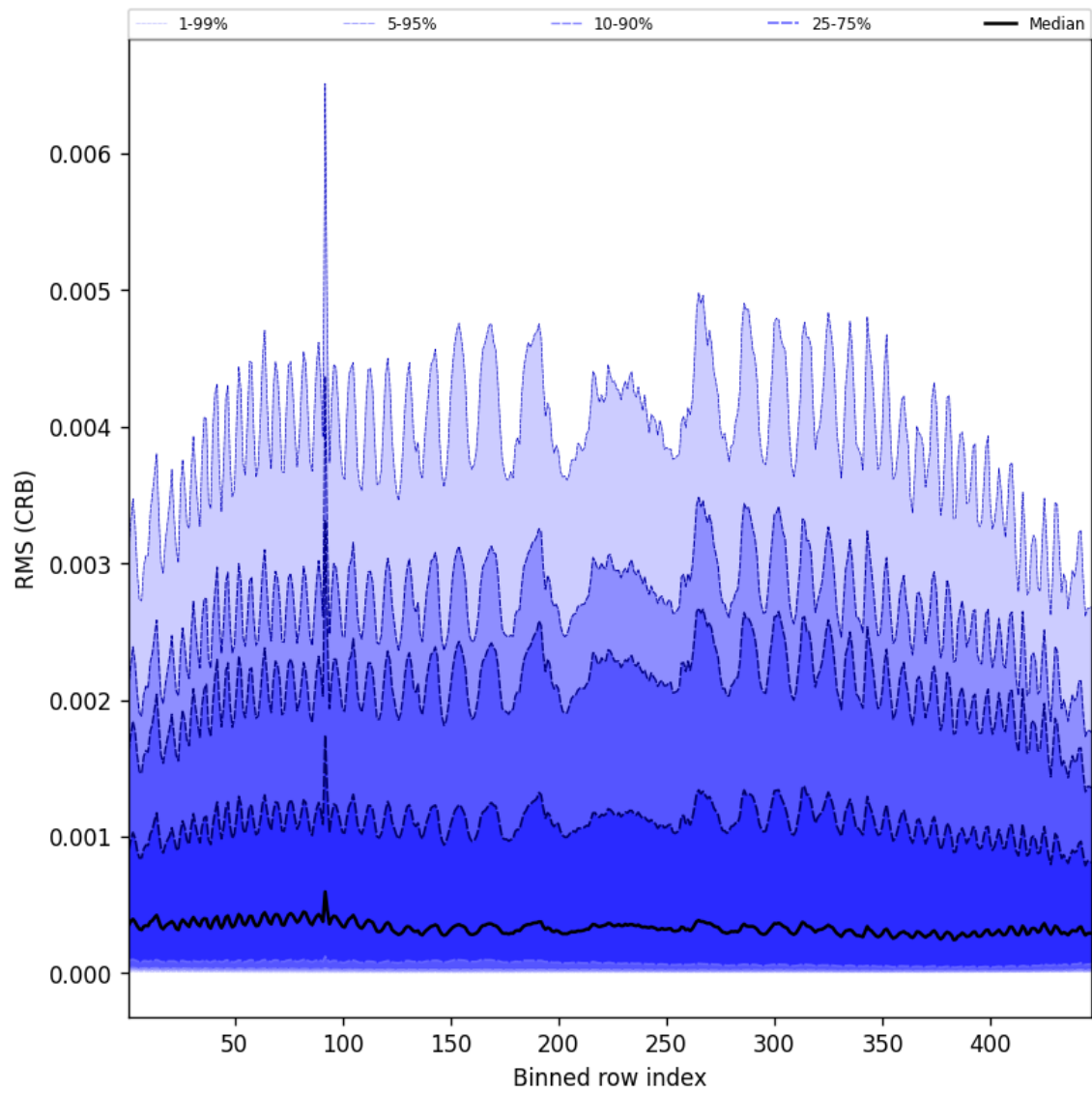
Figure 64: Along track statistics of “RMS (CRB)” for 2025-06-02 to 2025-06-04
