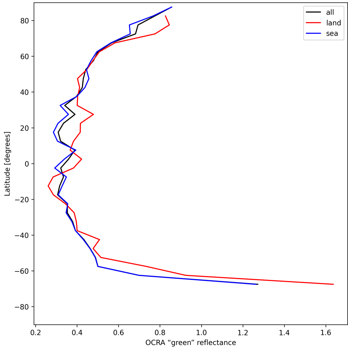
Figure 36: Zonal average of “OCRA “green” reflectance” for 2025-06-02 to 2025-06-04.
