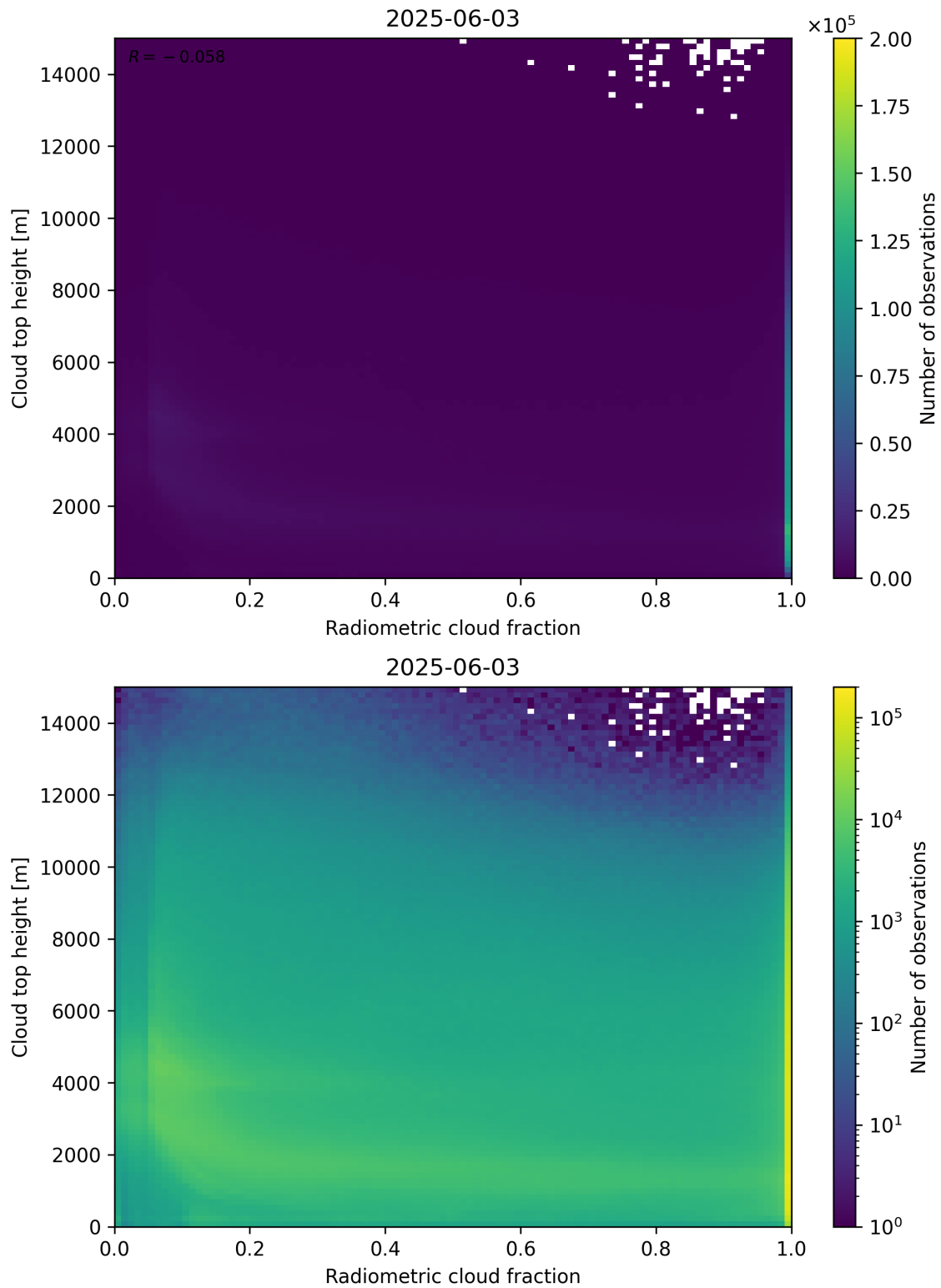
Figure 76: Scatter density plot of “Radiometric cloud fraction” against “Cloud top height” for 2025-06-02 to 2025-06-04.
