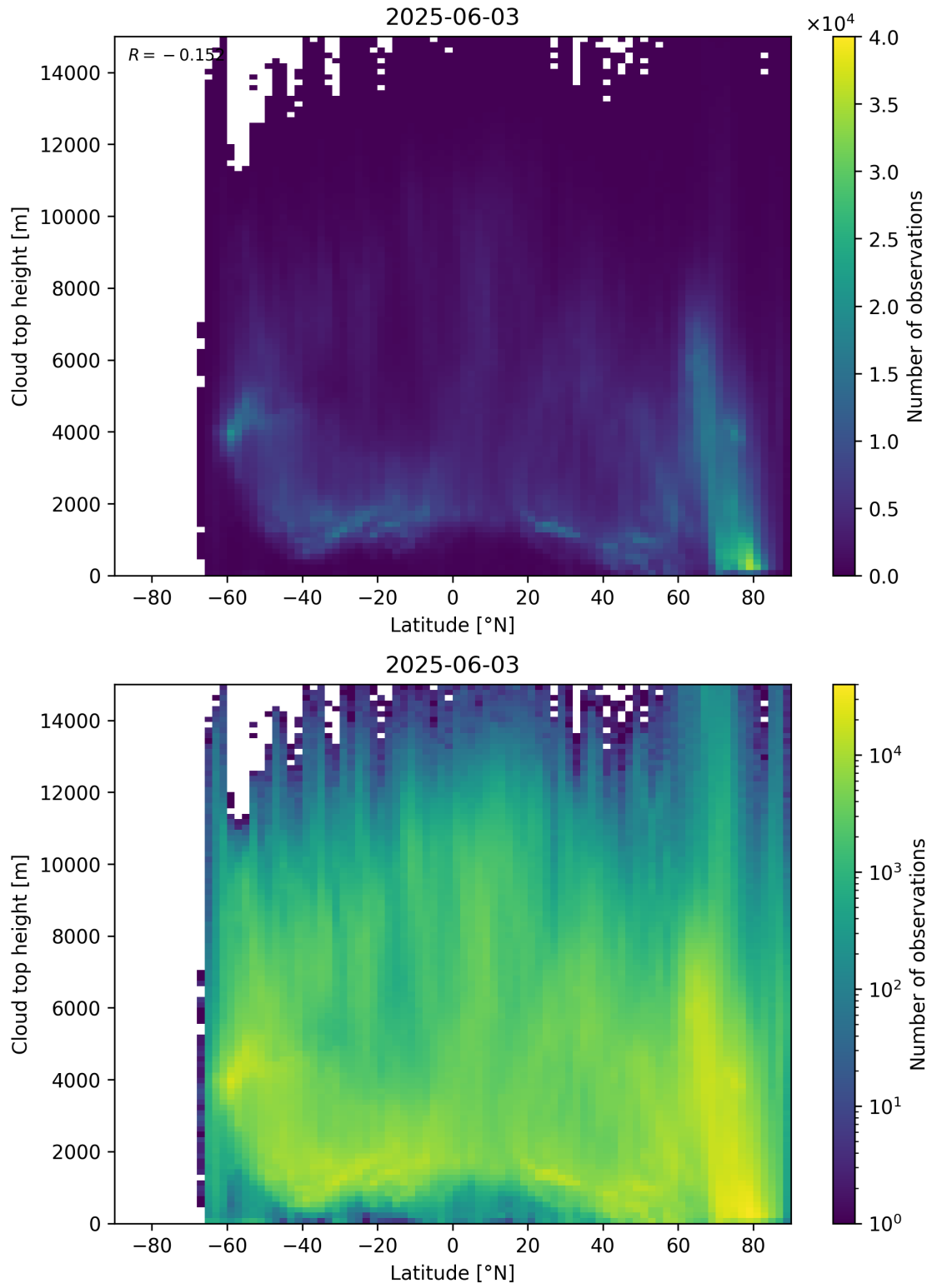
Figure 97: Scatter density plot of “Latitude” against “Cloud top height” for 2025-06-02 to 2025-06-04.
