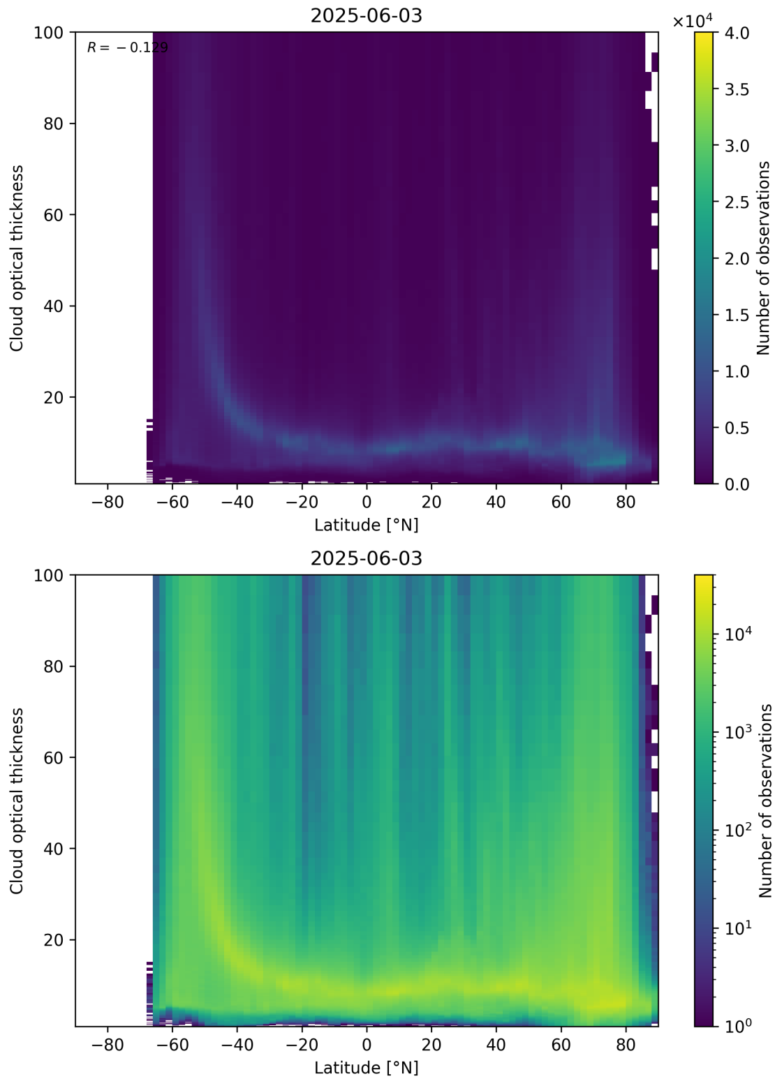
Figure 96: Scatter density plot of “Latitude” against “Cloud optical thickness” for 2025-06-02 to 2025-06-04.
