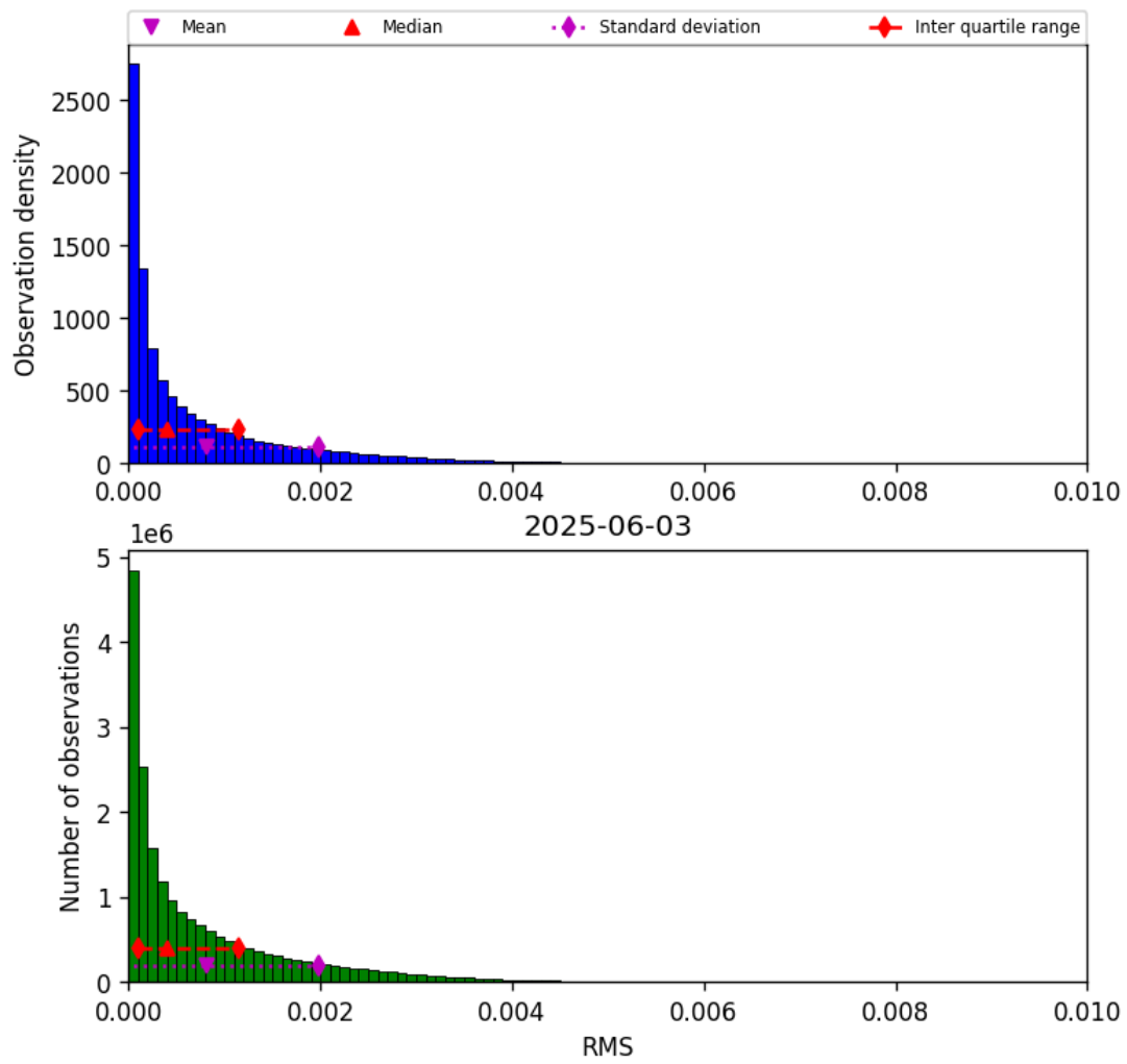
Figure 47: Histogram of “RMS” for 2025-06-02 to 2025-06-04
