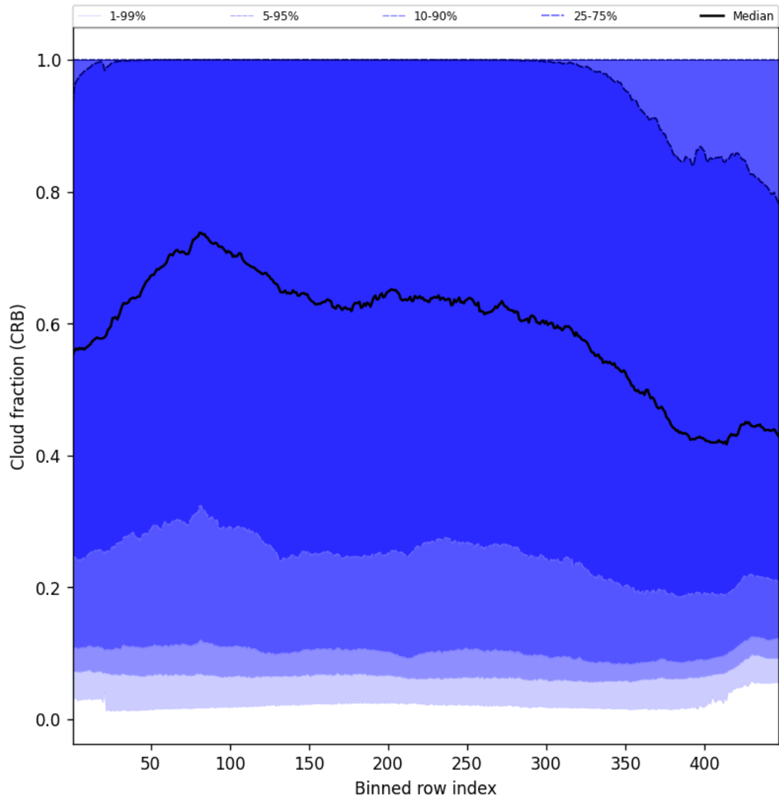
Figure 58: Along track statistics of “Cloud fraction (CRB)” for 2025-06-02 to 2025-06-04
