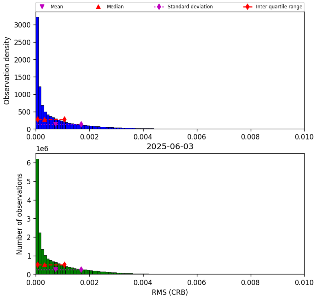
Figure 48: Histogram of “RMS (CRB)” for 2025-06-02 to 2025-06-04
