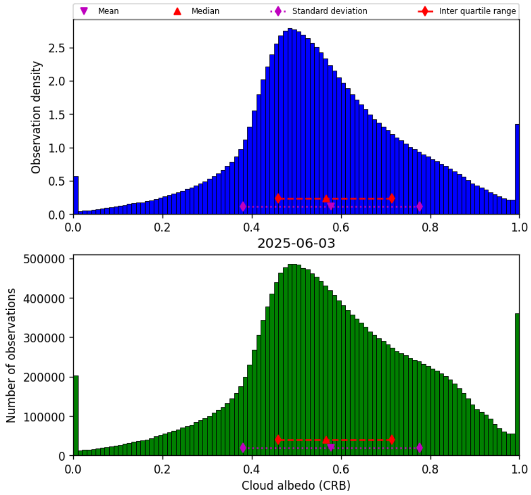
Figure 44: Histogram of “Cloud albedo (CRB)” for 2025-06-02 to 2025-06-04
