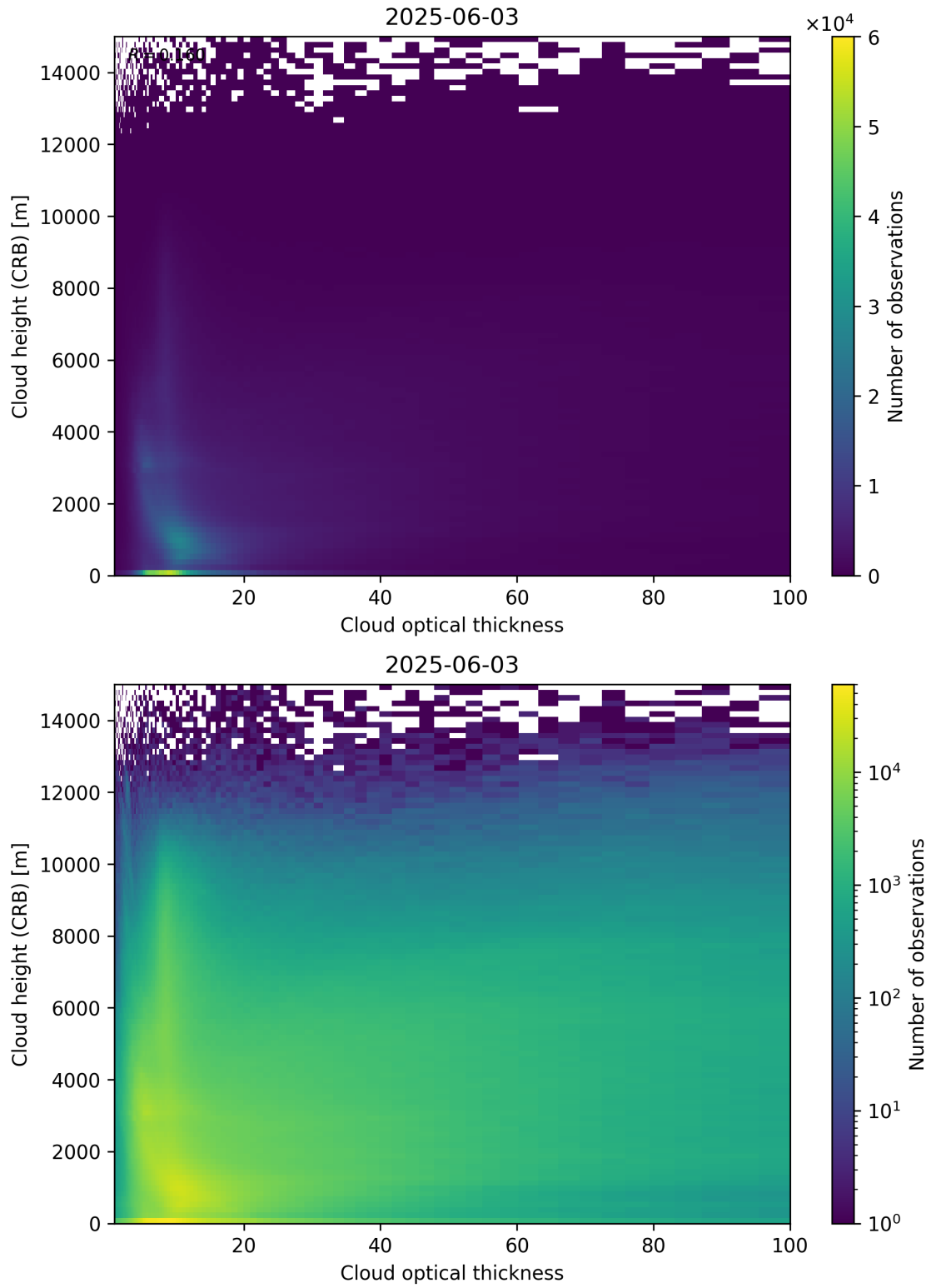
Figure 85: Scatter density plot of “Cloud optical thickness” against “Cloud height (CRB)” for 2025-06-02 to 2025-06-04.
