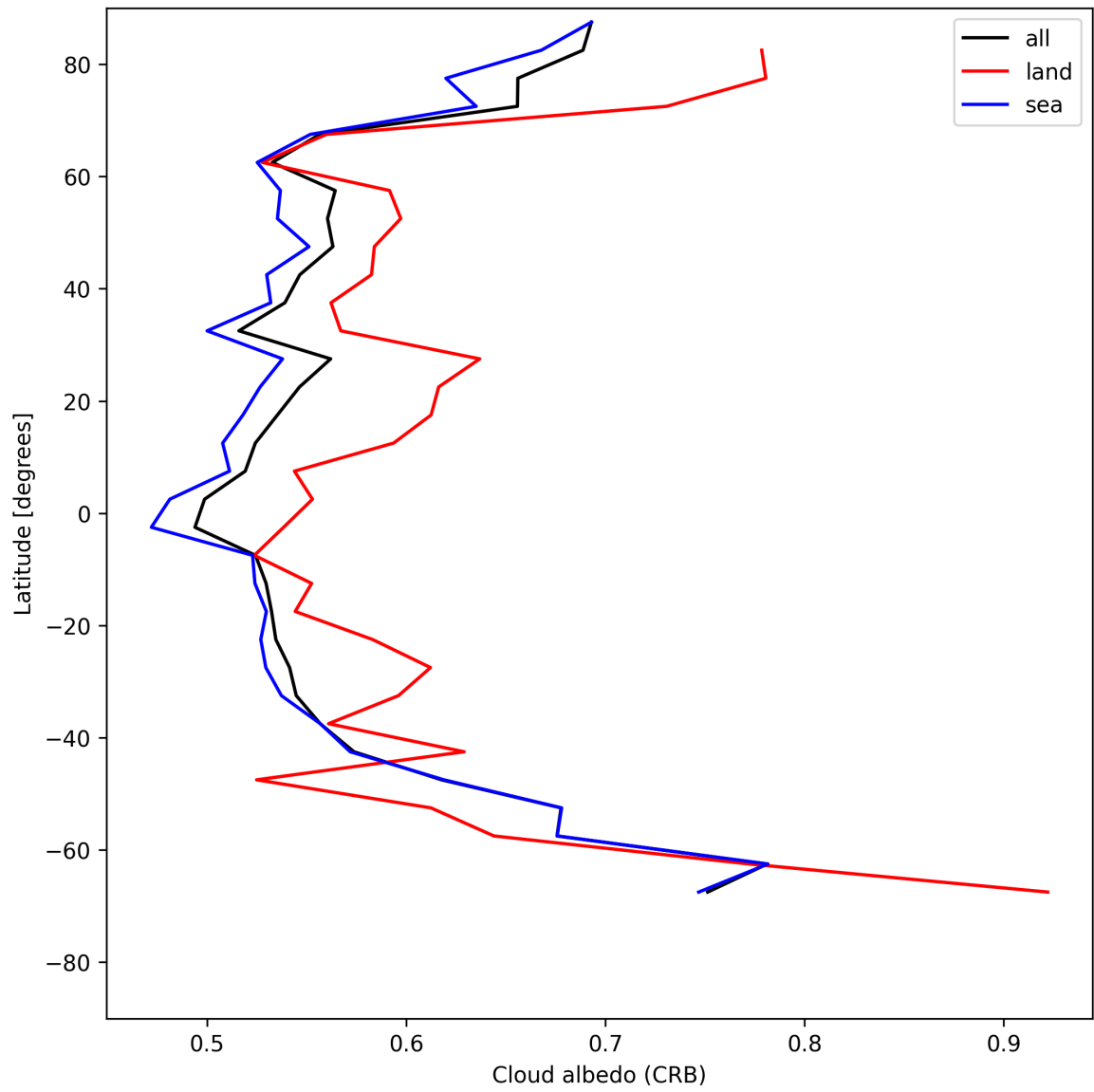
Figure 28: Zonal average of “Cloud albedo (CRB)” for 2025-06-02 to 2025-06-04.
