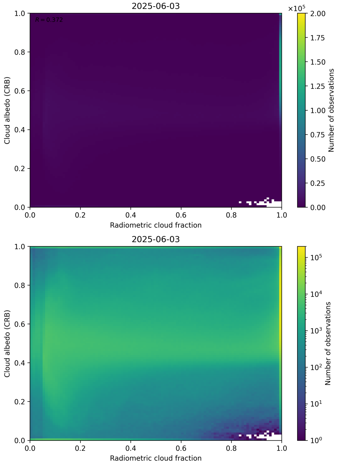
Figure 71: Scatter density plot of “Radiometric cloud fraction” against “Cloud albedo (CRB)” for 2025-06-02 to 2025-06-04.
