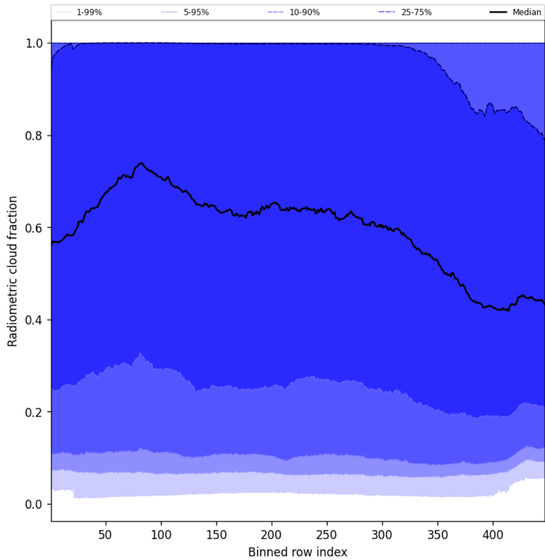
Figure 55: Along track statistics of “Radiometric cloud fraction” for 2025-06-02 to 2025-06-04
