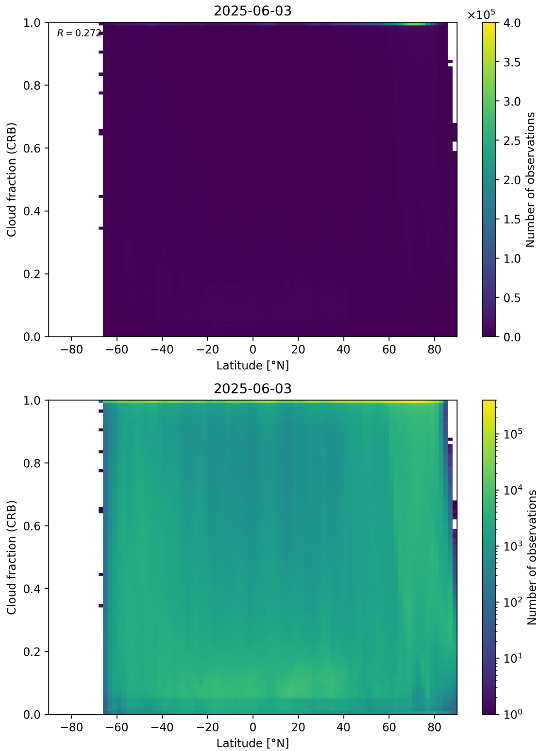
Figure 94: Scatter density plot of “Latitude” against “Cloud fraction (CRB)” for 2025-06-02 to 2025-06-04.
