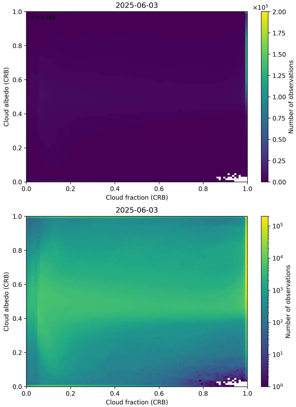
Figure 77: Scatter density plot of “Cloud fraction (CRB)” against “Cloud albedo (CRB)” for 2025-06-02 to 2025-06-04.
