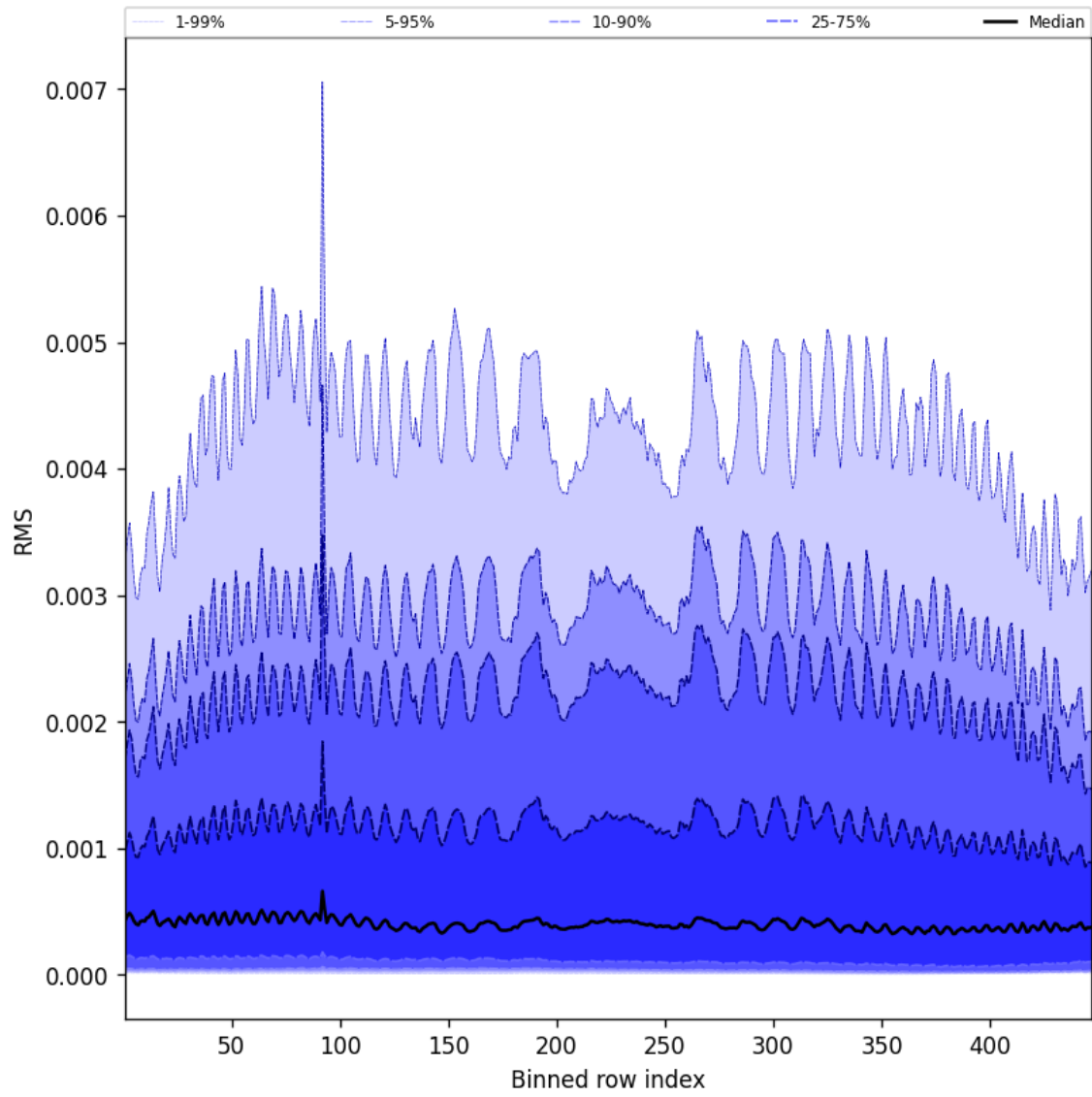
Figure 63: Along track statistics of “RMS” for 2025-06-02 to 2025-06-04
