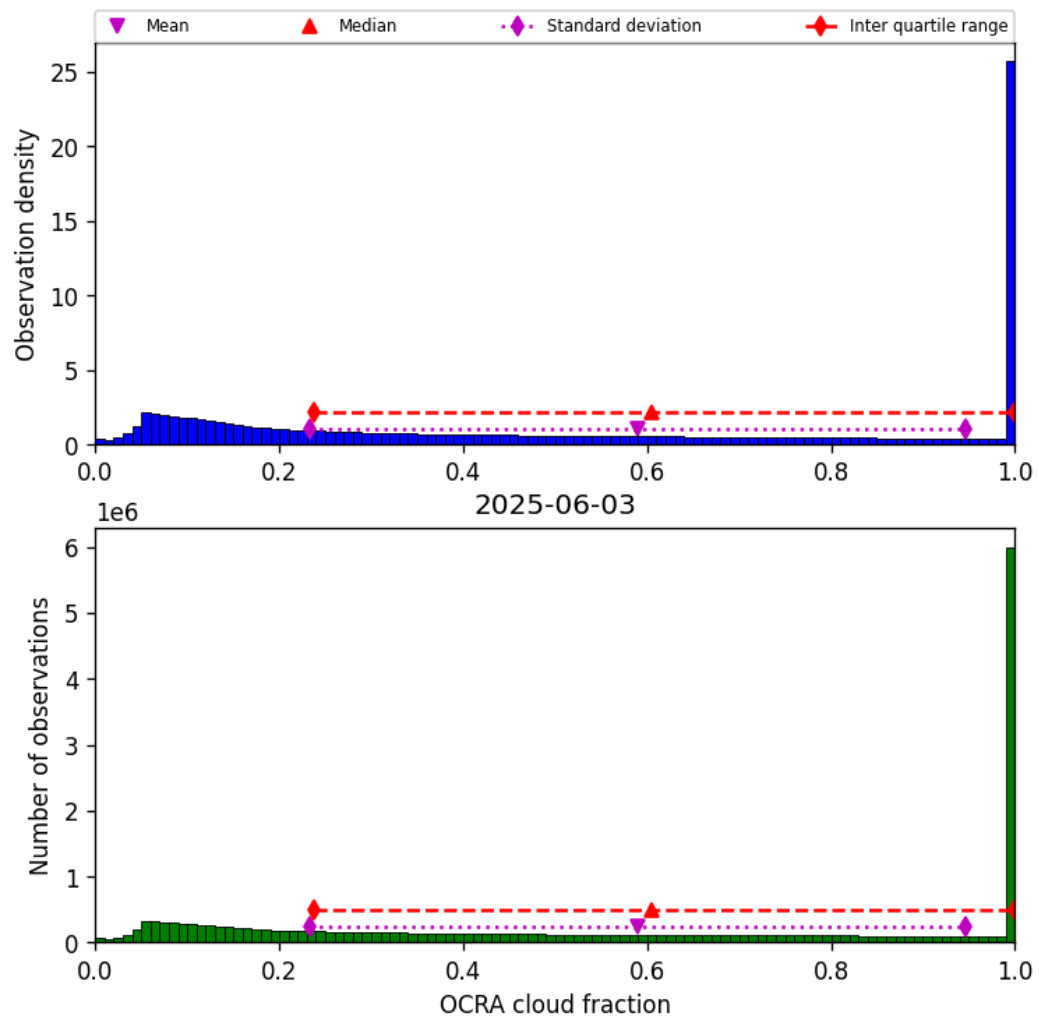
Figure 50: Histogram of “OCRA cloud fraction” for 2025-06-02 to 2025-06-04
