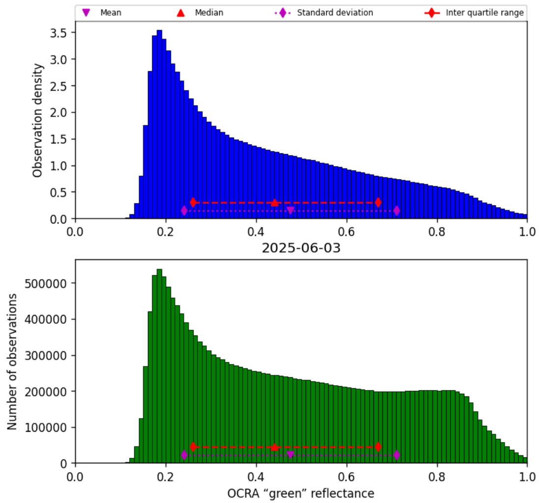
Figure 52: Histogram of “OCRA “green” reflectance” for 2025-06-02 to 2025-06-04
