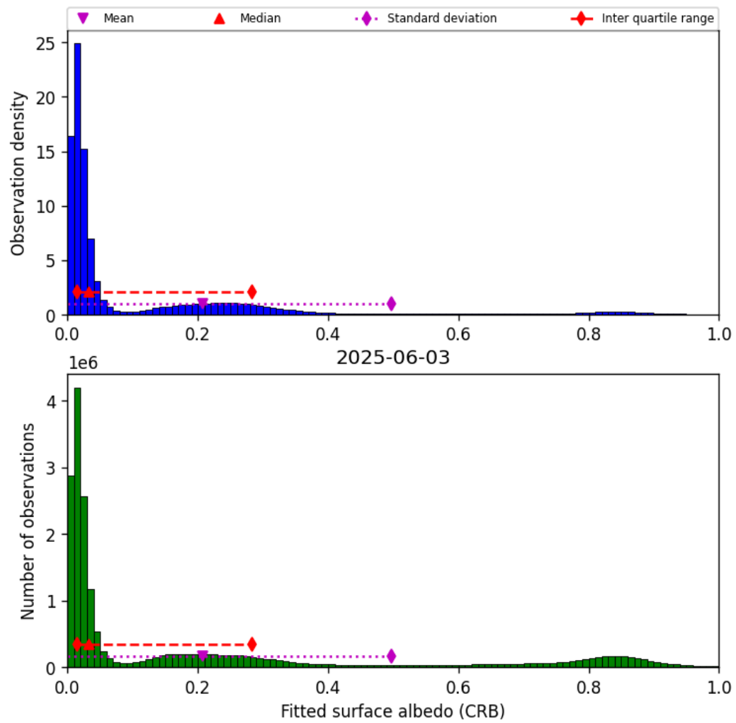
Figure 46: Histogram of “Fitted surface albedo (CRB)” for 2025-06-02 to 2025-06-04
