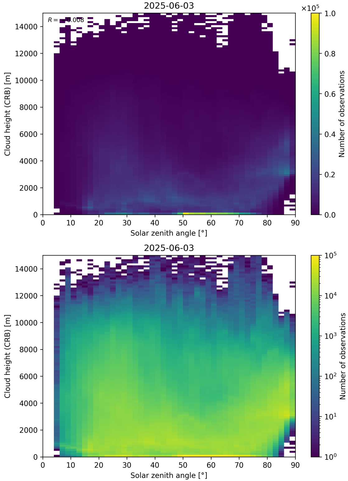
Figure 102: Scatter density plot of “Solar zenith angle” against “Cloud height (CRB)” for 2025-06-02 to 2025-06-04.
