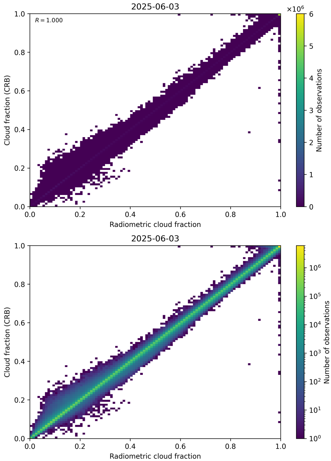
Figure 73: Scatter density plot of “Radiometric cloud fraction” against “Cloud fraction (CRB)” for 2025-06-02 to 2025-06-04.
