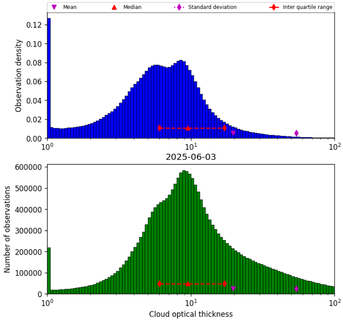
Figure 41: Histogram of “Cloud optical thickness” for 2025-06-02 to 2025-06-04
