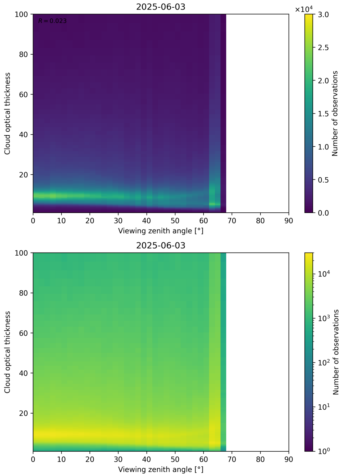
Figure 111: Scatter density plot of “Viewing zenith angle” against “Cloud optical thickness” for 2025-06-02 to 2025-06-04.
