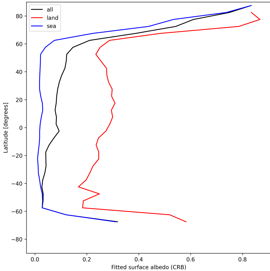
Figure 30: Zonal average of “Fitted surface albedo (CRB)” for 2025-06-02 to 2025-06-04.
