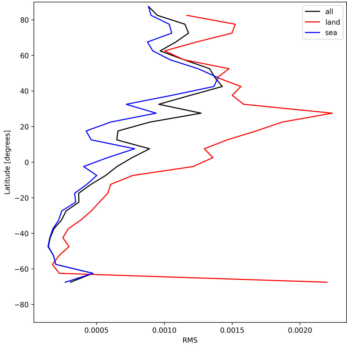
Figure 31: Zonal average of “RMS” for 2025-06-02 to 2025-06-04.
