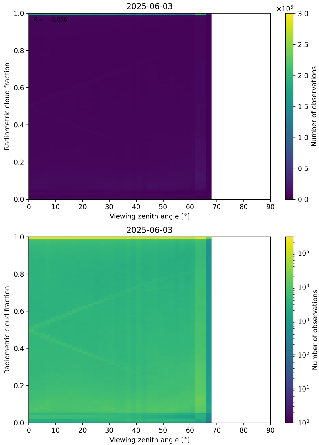
Figure 107: Scatter density plot of “Viewing zenith angle” against “Radiometric cloud fraction” for 2025-06-02 to 2025-06-04.
