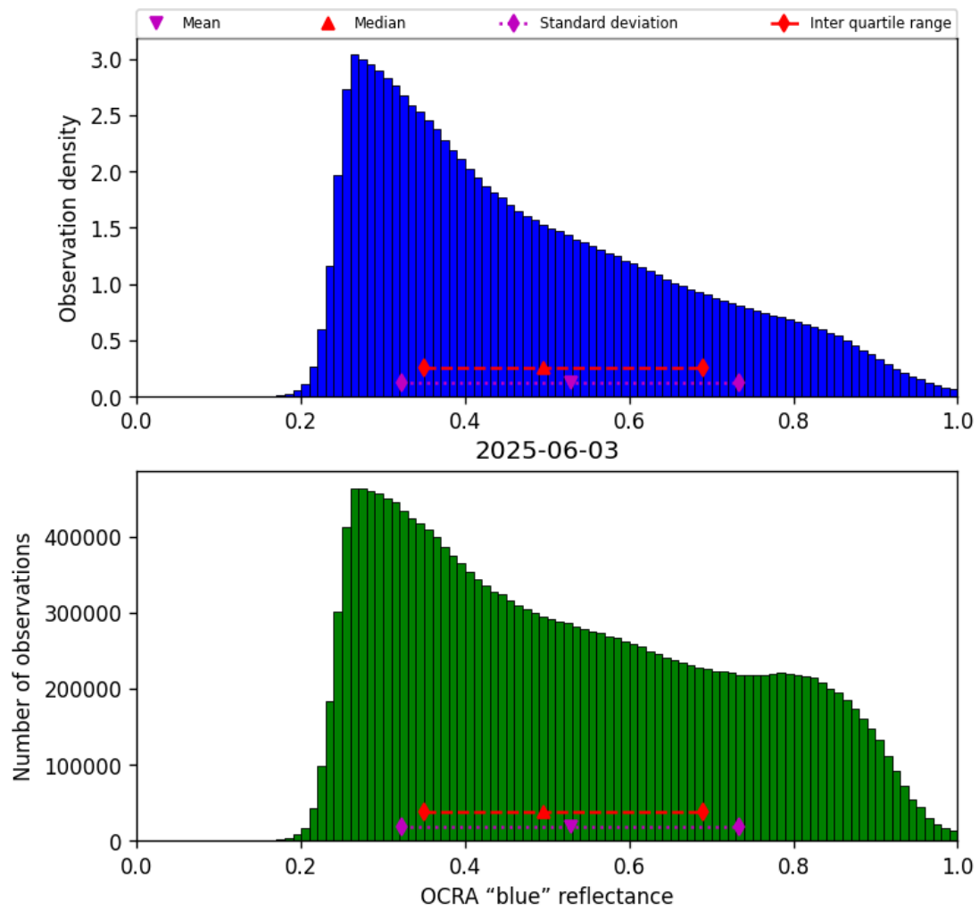
Figure 51: Histogram of “OCRA “blue” reflectance” for 2025-06-02 to 2025-06-04
