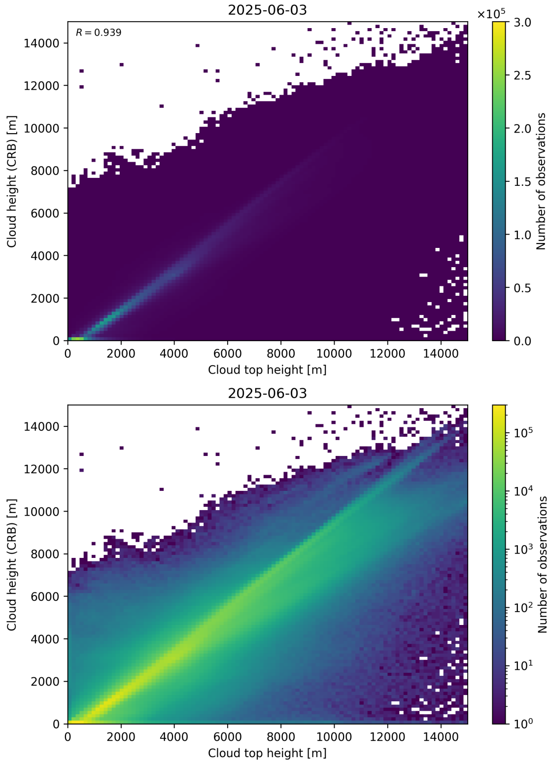
Figure 89: Scatter density plot of “Cloud top height” against “Cloud height (CRB)” for 2025-06-02 to 2025-06-04.
