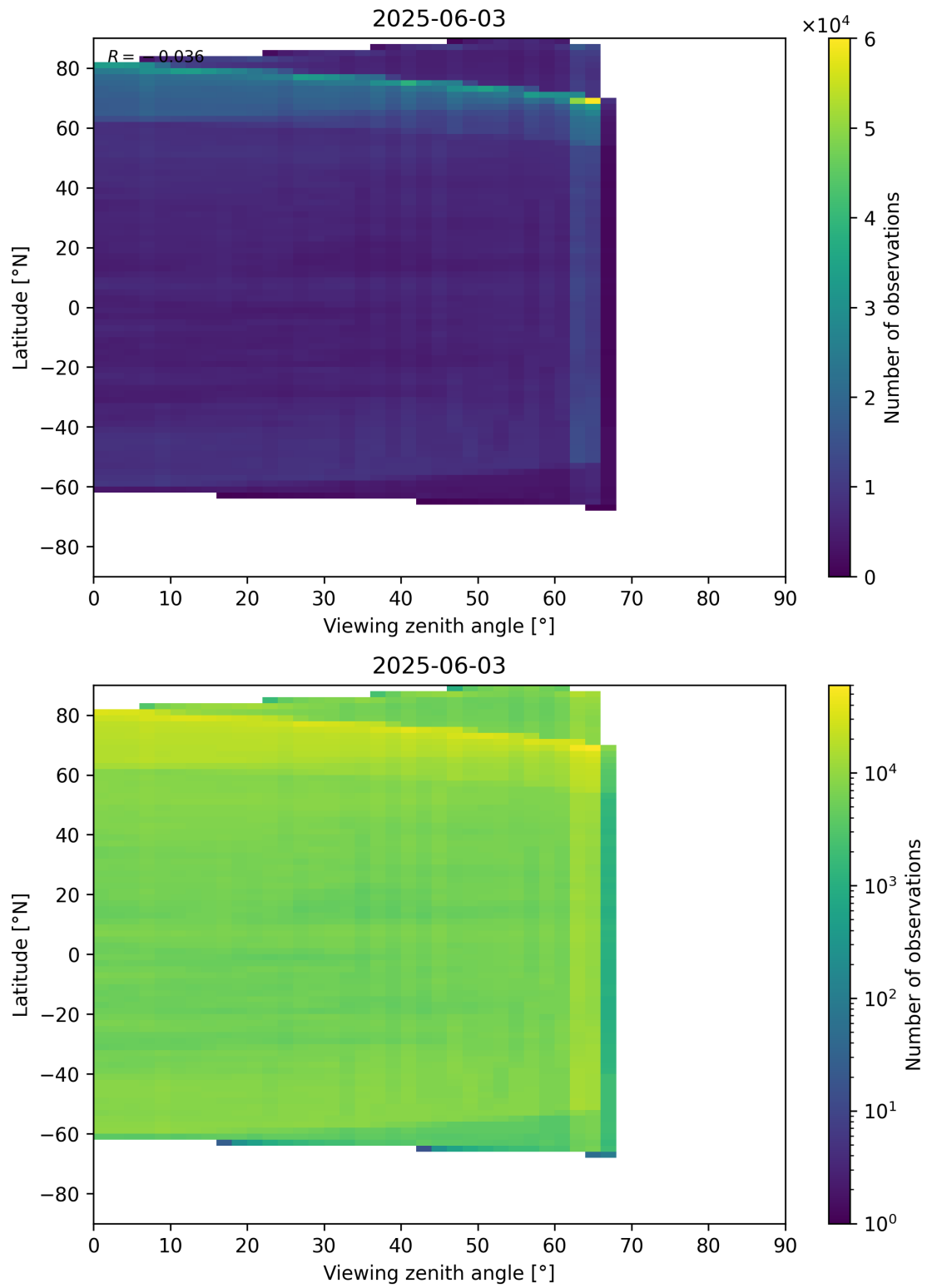
Figure 113: Scatter density plot of “Viewing zenith angle” against “Latitude” for 2025-06-02 to 2025-06-04.
