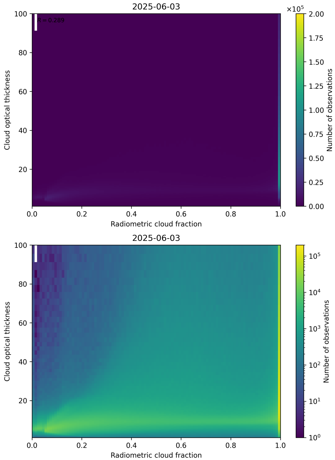
Figure 75: Scatter density plot of “Radiometric cloud fraction” against “Cloud optical thickness” for 2025-06-02 to 2025-06-04.
