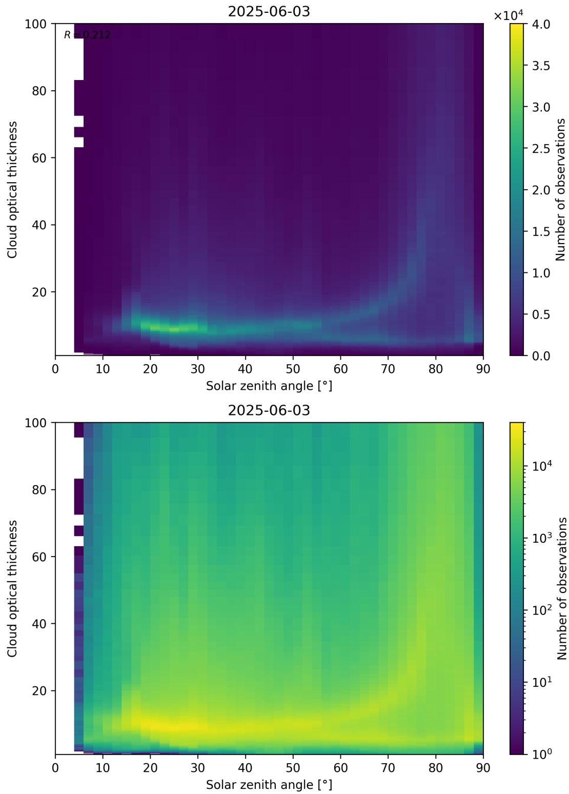
Figure 103: Scatter density plot of “Solar zenith angle” against “Cloud optical thickness” for 2025-06-02 to 2025-06-04.
