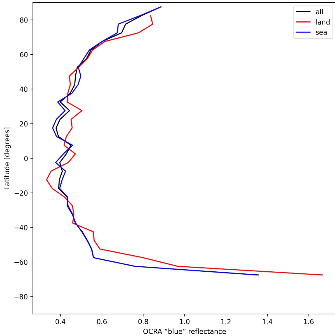
Figure 35: Zonal average of "OCRA "blue" reflectance" for 2025-06-02 to 2025-06-04.
