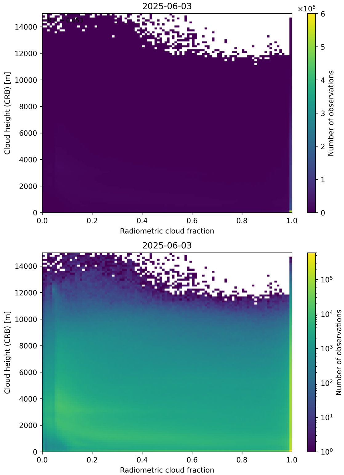
Figure 74: Scatter density plot of “Radiometric cloud fraction” against “Cloud height (CRB)” for 2025-06-02 to 2025-06-04.
