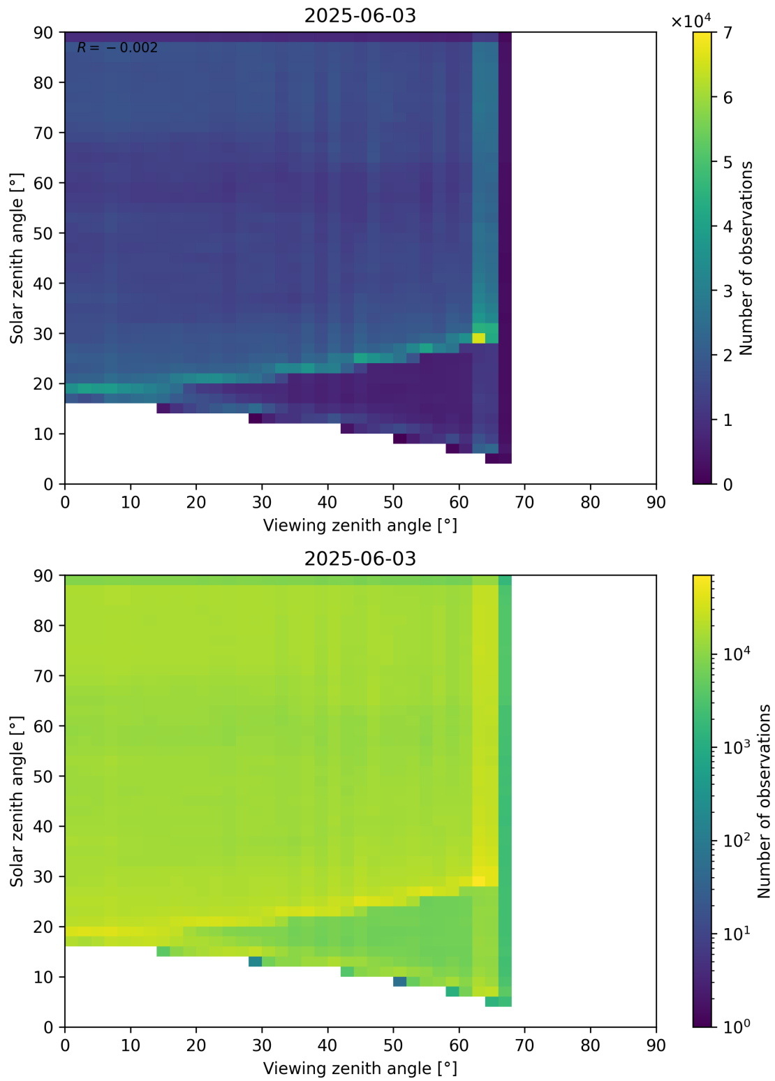
Figure 114: Scatter density plot of “Viewing zenith angle” against “Solar zenith angle” for 2025-06-02 to 2025-06-04.
