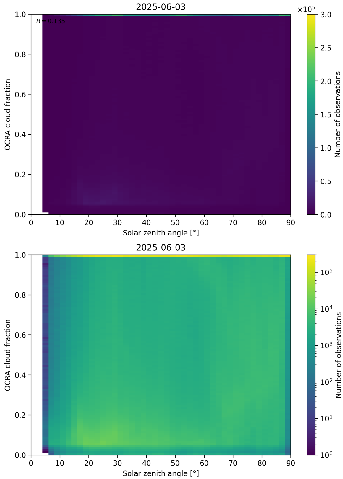
Figure 100: Scatter density plot of “Solar zenith angle” against “OCRA cloud fraction” for 2025-06-02 to 2025-06-04.
