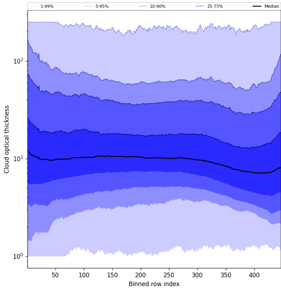
Figure 57: Along track statistics of “Cloud optical thickness” for 2025-06-02 to 2025-06-04
