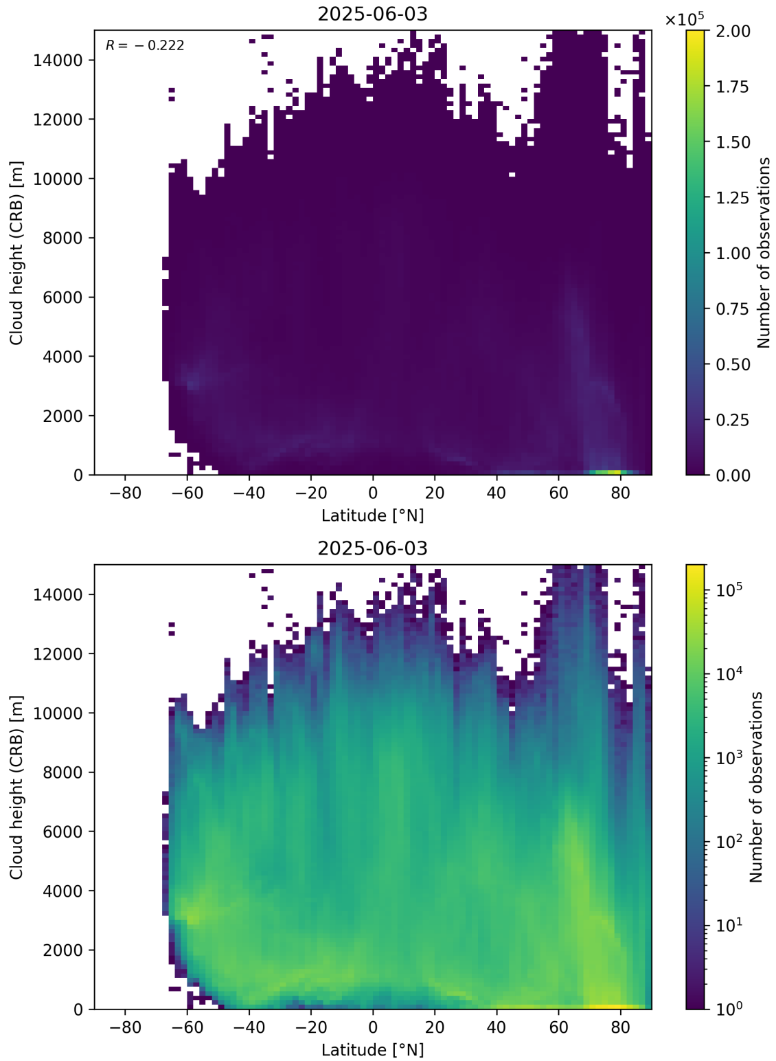
Figure 95: Scatter density plot of “Latitude” against “Cloud height (CRB)” for 2025-06-02 to 2025-06-04.
