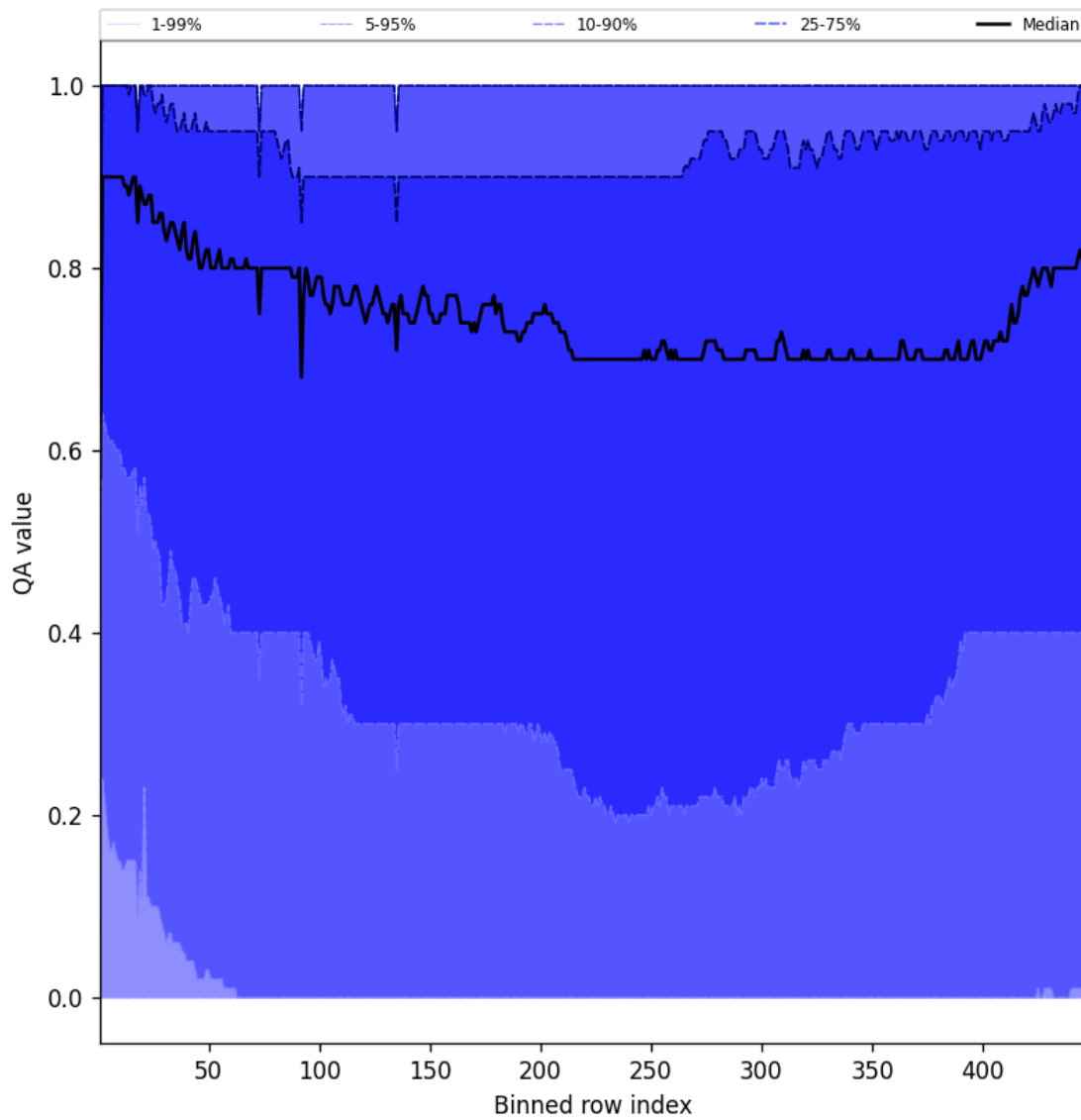
Figure 54: Along track statistics of “QA value” for 2025-06-02 to 2025-06-04
