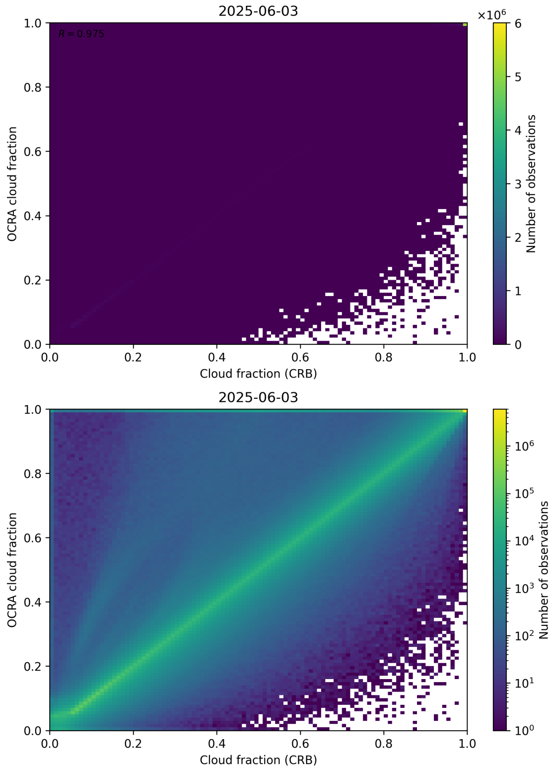
Figure 78: Scatter density plot of “Cloud fraction (CRB)” against “OCRA cloud fraction” for 2025-06-02 to 2025-06-04.
