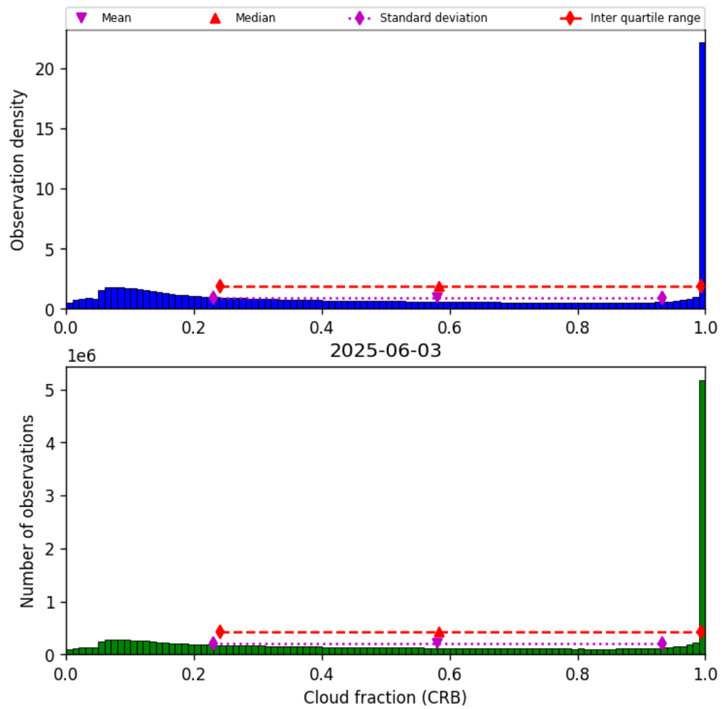
Figure 42: Histogram of “Cloud fraction (CRB)” for 2025-06-02 to 2025-06-04
