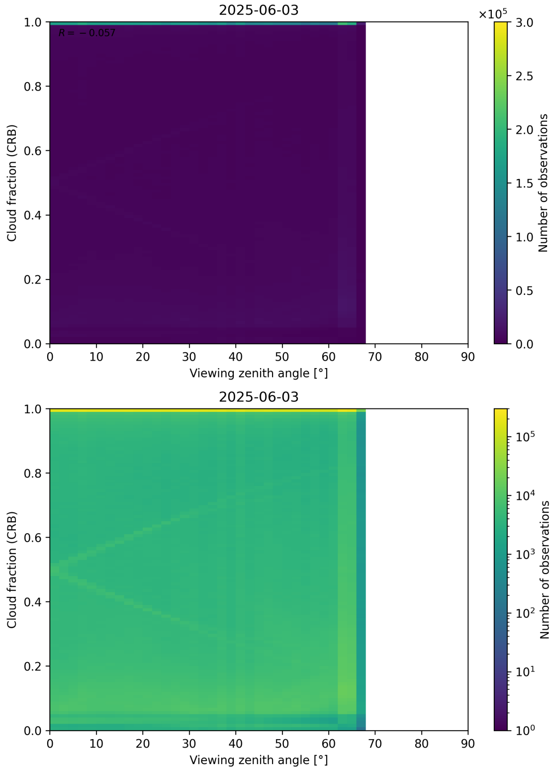
Figure 109: Scatter density plot of “Viewing zenith angle” against “Cloud fraction (CRB)” for 2025-06-02 to 2025-06-04.
