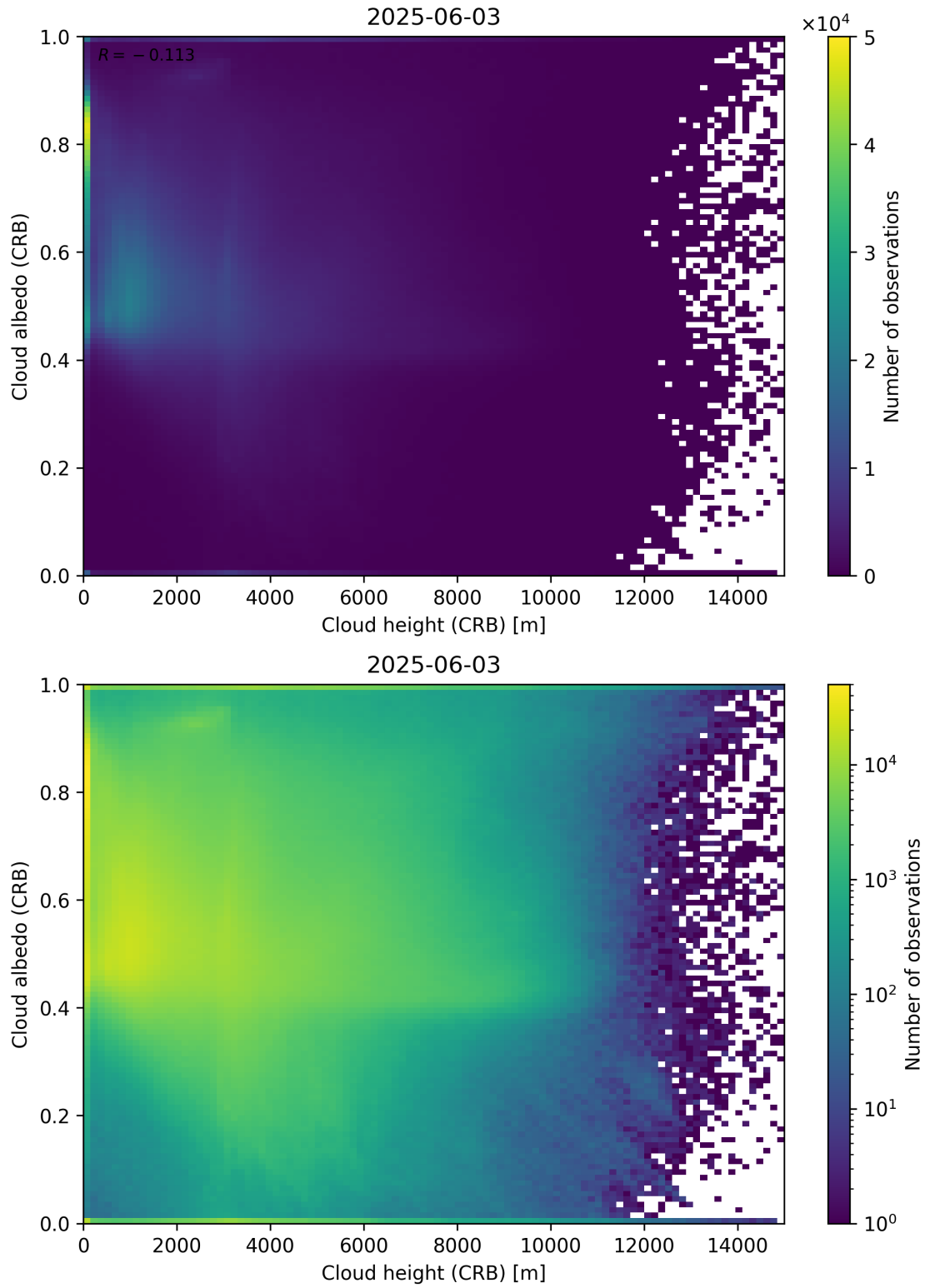
Figure 80: Scatter density plot of “Cloud height (CRB)” against “Cloud albedo (CRB)” for 2025-06-02 to 2025-06-04.
