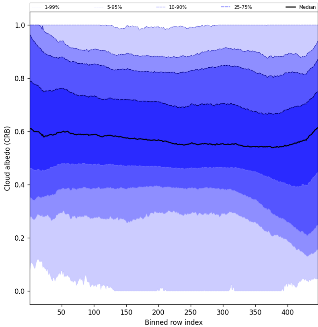
Figure 60: Along track statistics of “Cloud albedo (CRB)” for 2025-06-02 to 2025-06-04
