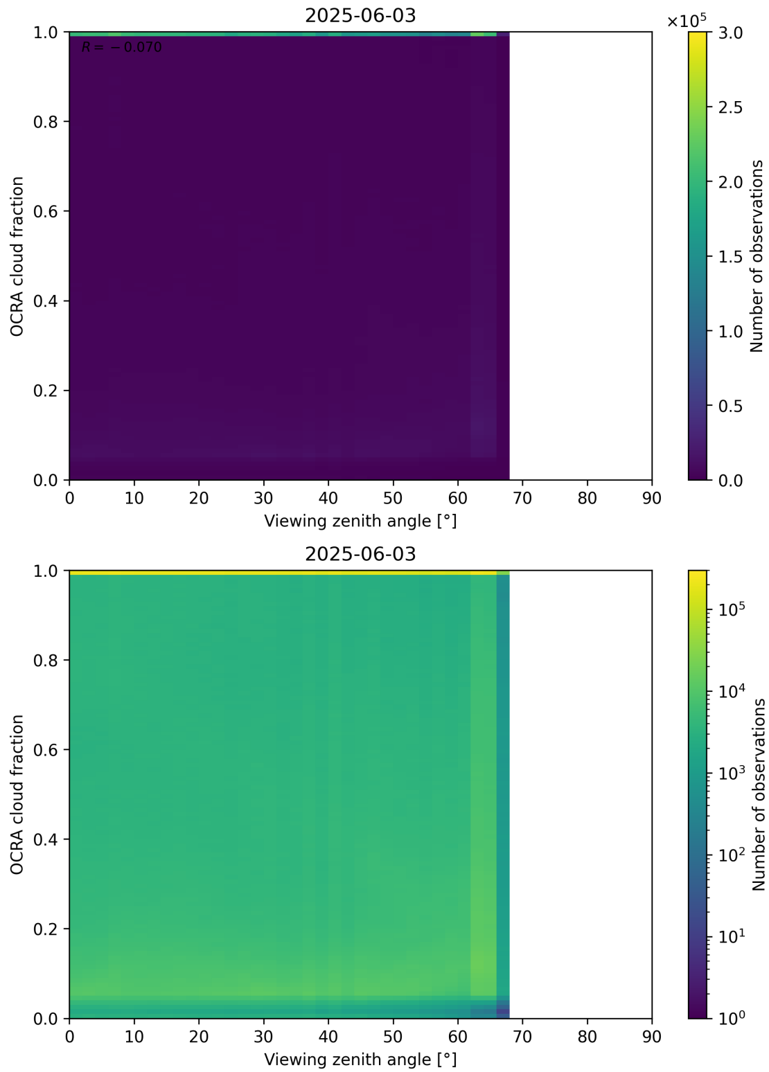
Figure 108: Scatter density plot of “Viewing zenith angle” against “OCRA cloud fraction” for 2025-06-02 to 2025-06-04.
