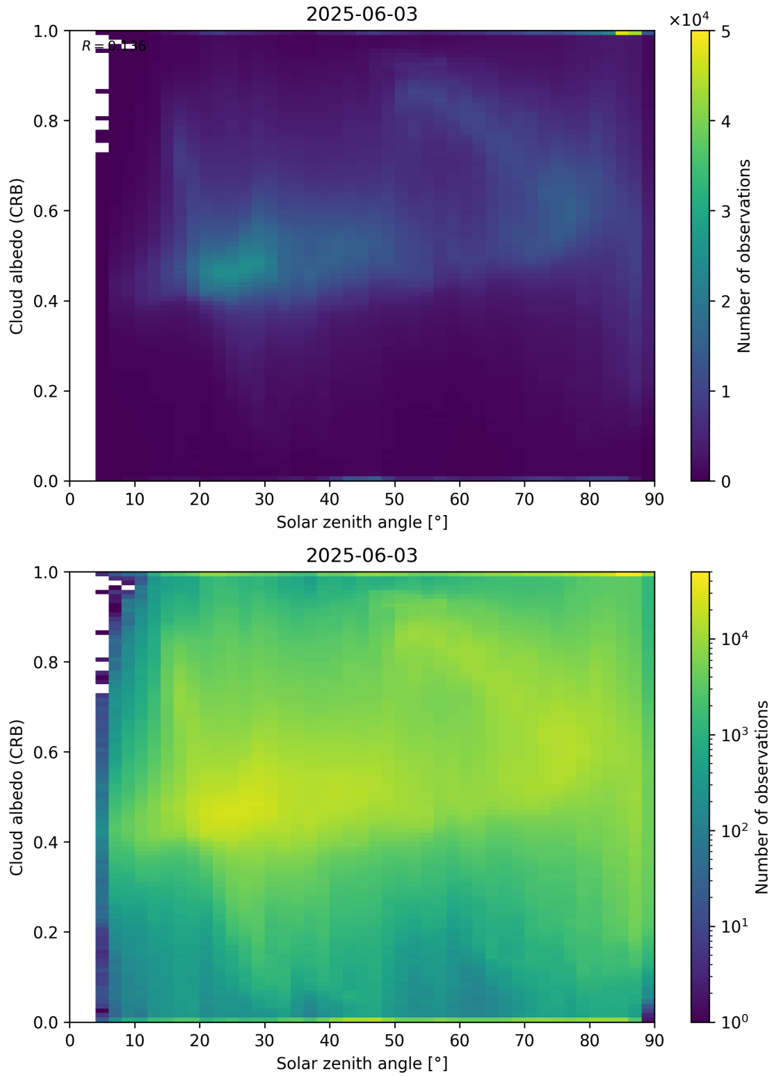
Figure 98: Scatter density plot of “Solar zenith angle” against “Cloud albedo (CRB)” for 2025-06-02 to 2025-06-04.
