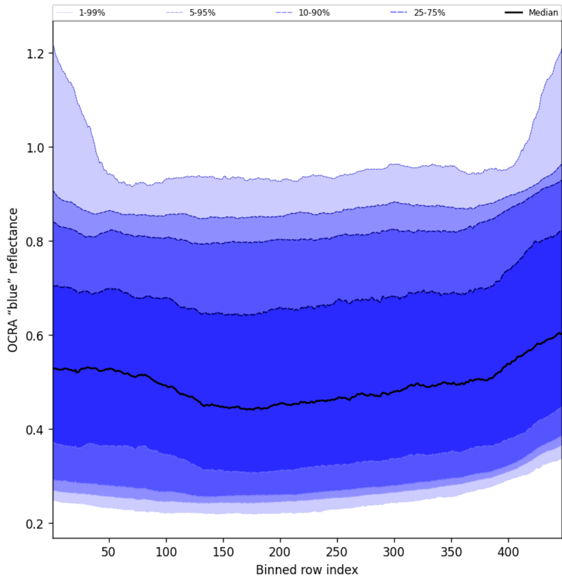
Figure 67: Along track statistics of “OCRA “blue” reflectance” for 2025-06-02 to 2025-06-04
