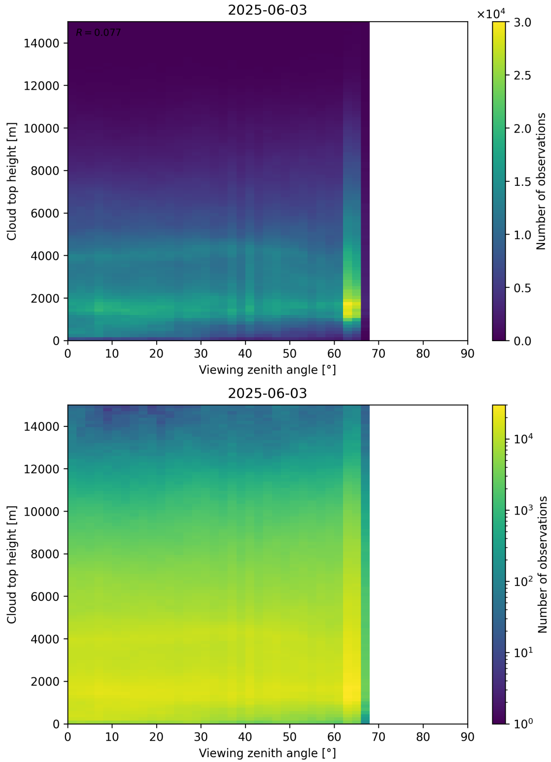
Figure 112: Scatter density plot of “Viewing zenith angle” against “Cloud top height” for 2025-06-02 to 2025-06-04.
