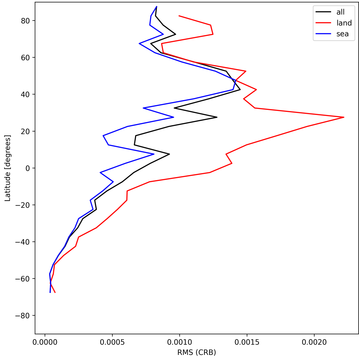
Figure 32: Zonal average of “RMS (CRB)” for 2025-06-02 to 2025-06-04.
