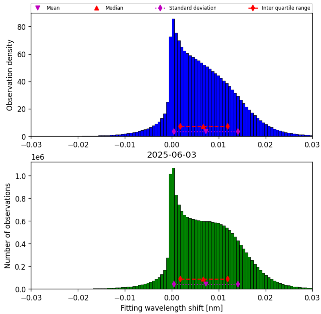
Figure 49: Histogram of “Fitting wavelength shift” for 2025-06-02 to 2025-06-04
