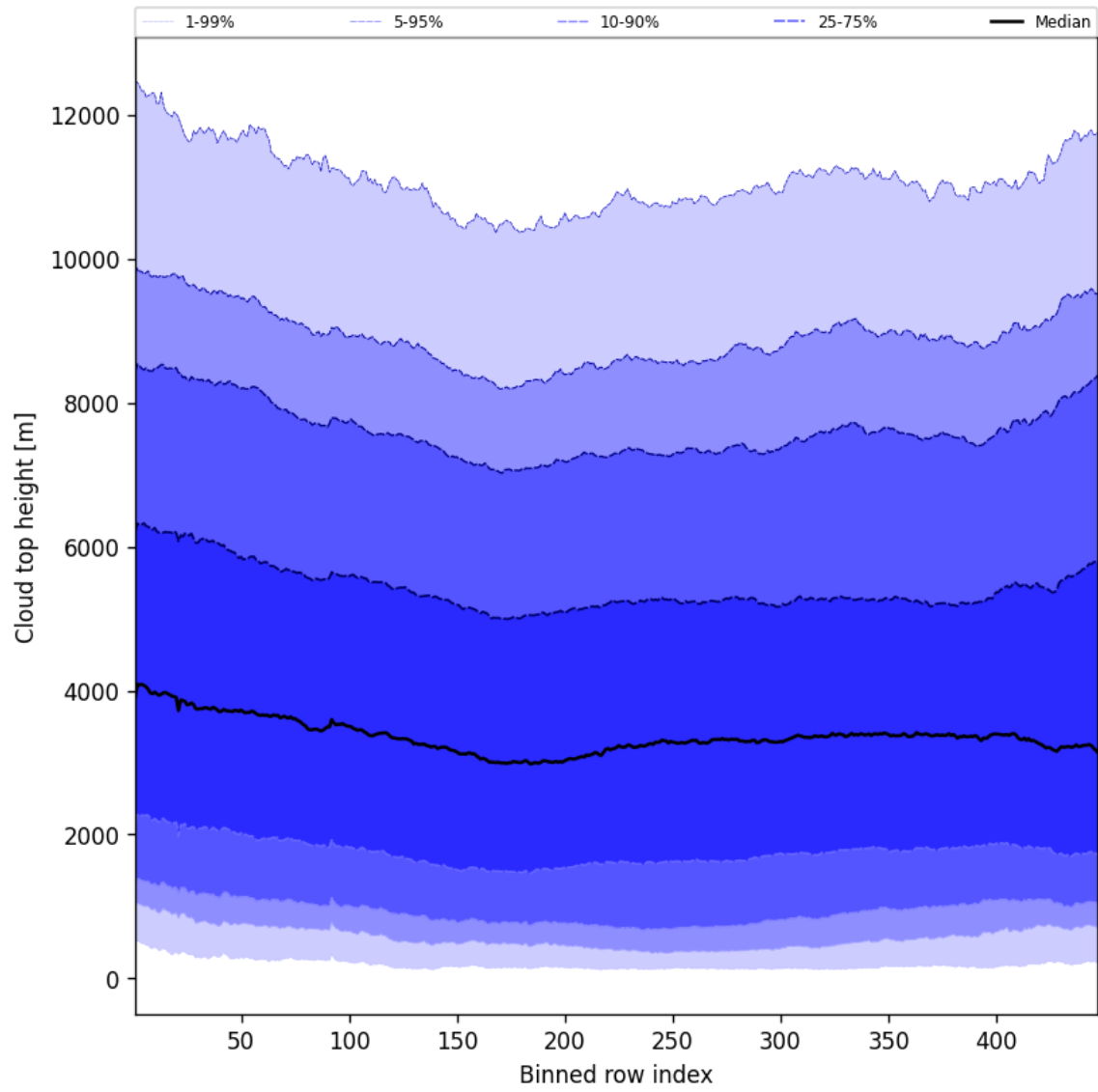
Figure 56: Along track statistics of “Cloud top height” for 2025-06-02 to 2025-06-04
