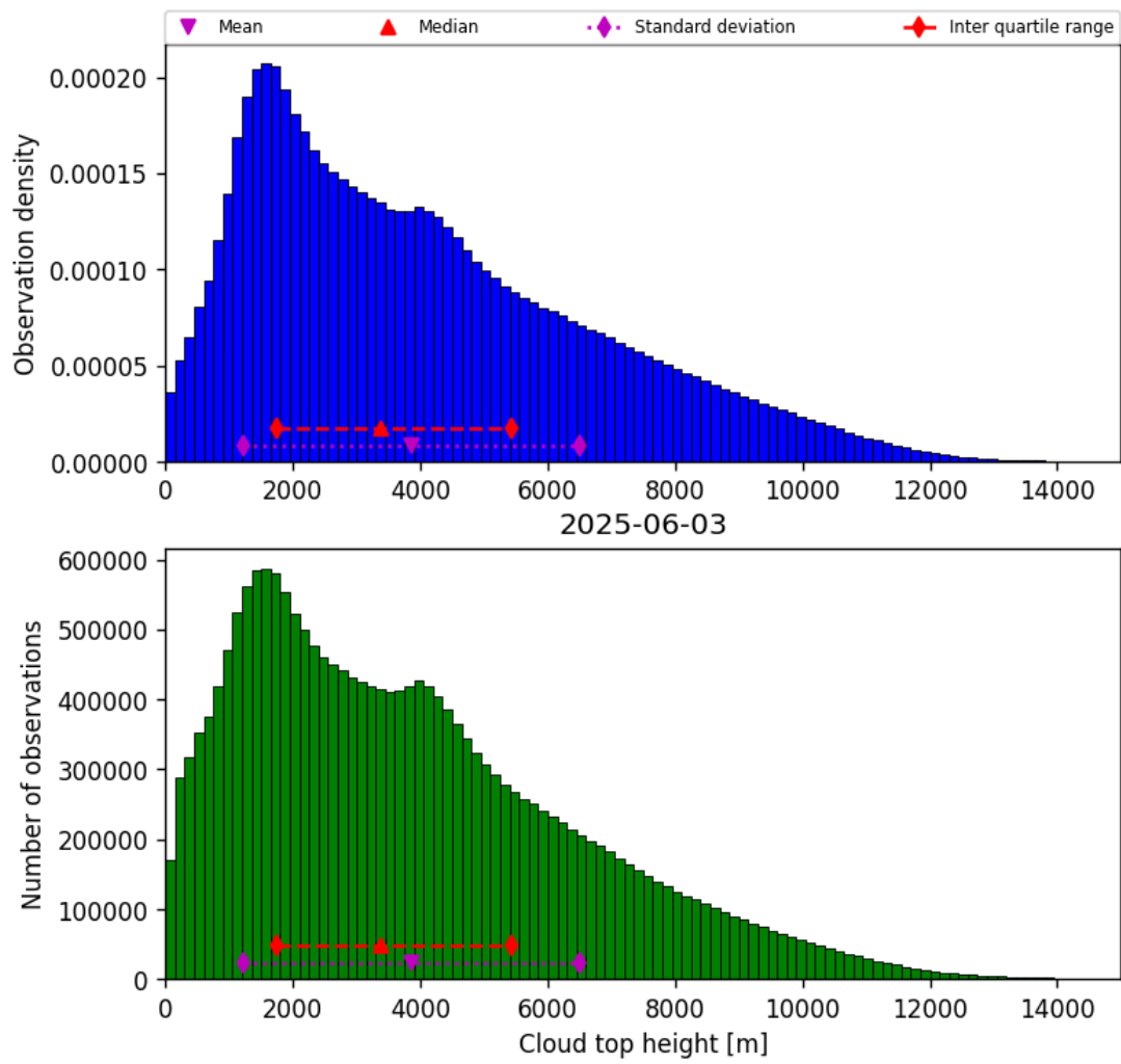
Figure 40: Histogram of “Cloud top height” for 2025-06-02 to 2025-06-04
