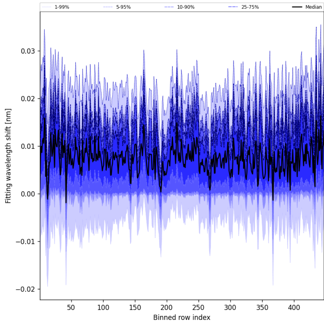
Figure 65: Along track statistics of “Fitting wavelength shift” for 2025-06-02 to 2025-06-04
