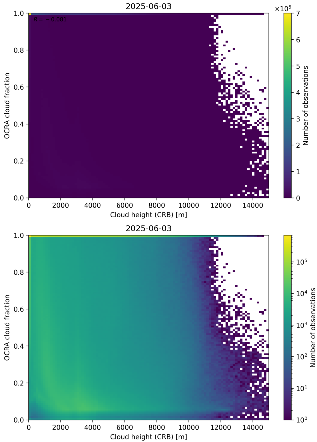
Figure 81: Scatter density plot of “Cloud height (CRB)” against “OCRA cloud fraction” for 2025-06-02 to 2025-06-04.
