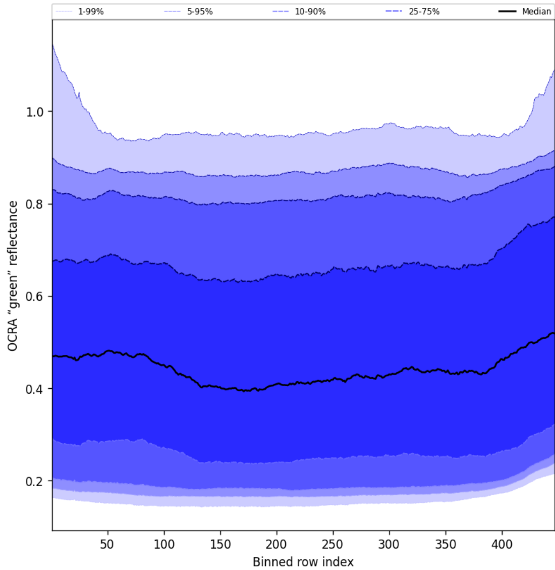
Figure 68: Along track statistics of “OCRA “green” reflectance” for 2025-06-02 to 2025-06-04
