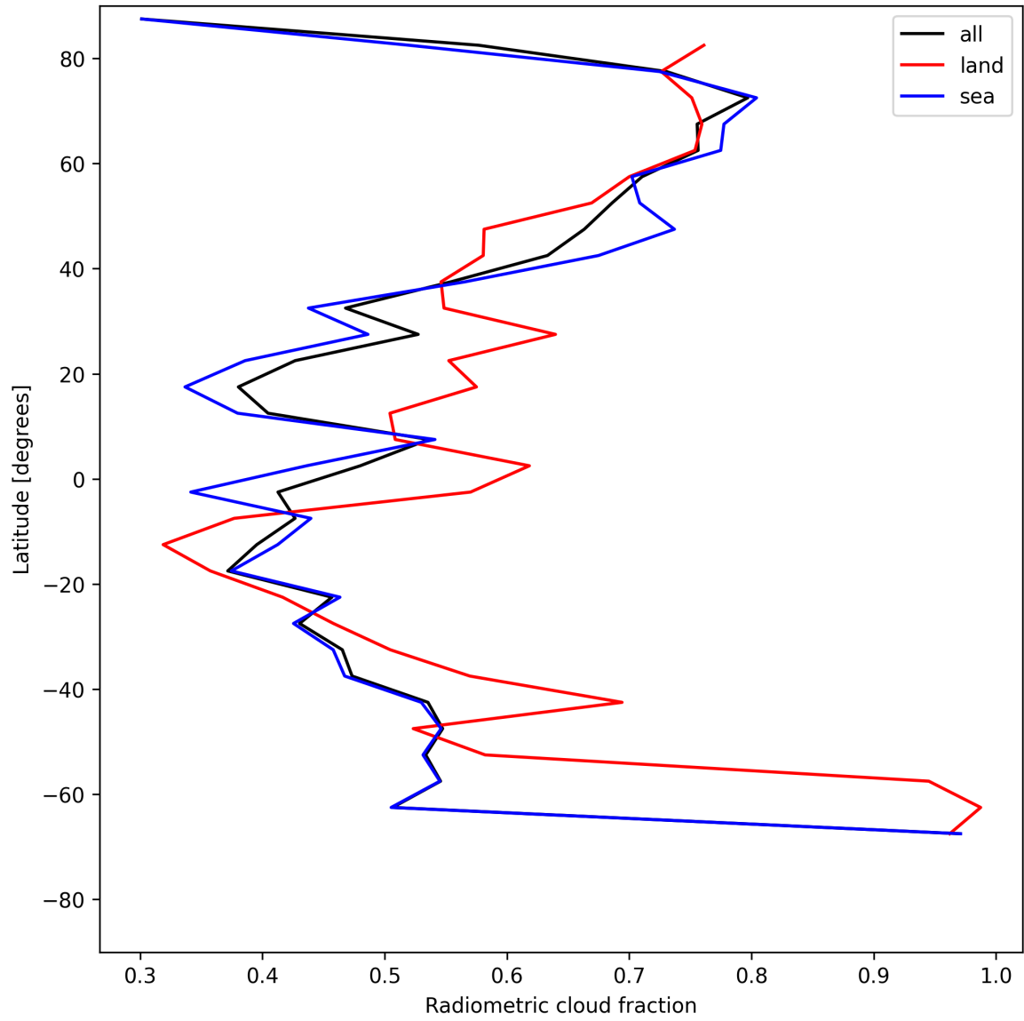
Figure 23: Zonal average of “Radiometric cloud fraction” for 2025-06-02 to 2025-06-04.
