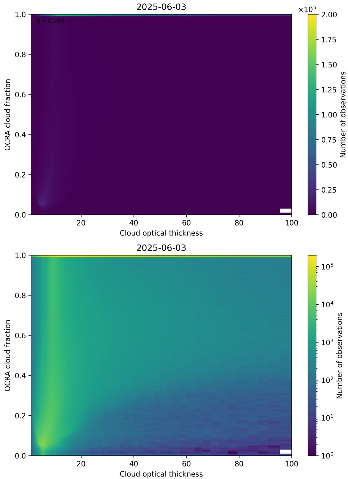
Figure 83: Scatter density plot of “Cloud optical thickness” against “OCRA cloud fraction” for 2025-06-02 to 2025-06-04.
