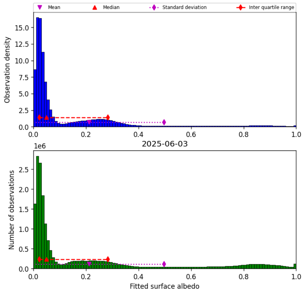
Figure 45: Histogram of “Fitted surface albedo” for 2025-06-02 to 2025-06-04
