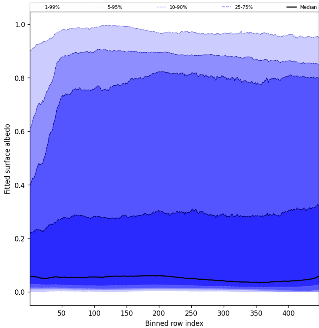
Figure 61: Along track statistics of “Fitted surface albedo” for 2025-06-02 to 2025-06-04
