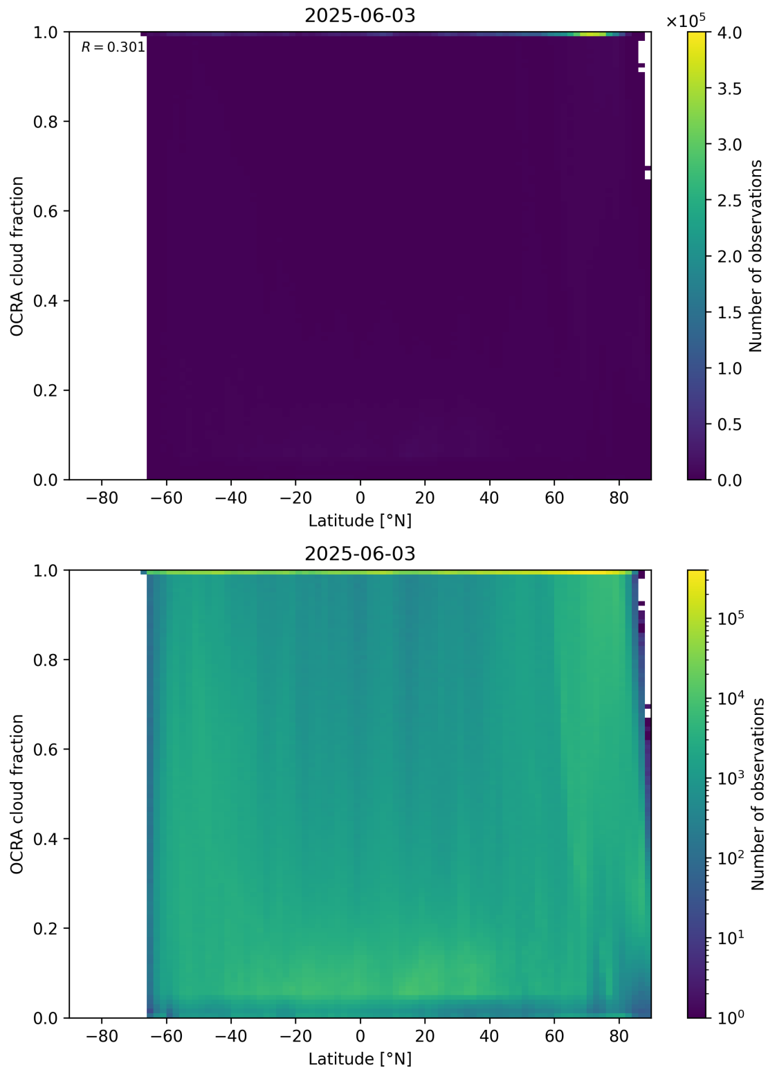
Figure 93: Scatter density plot of “Latitude” against “OCRA cloud fraction” for 2025-06-02 to 2025-06-04.
