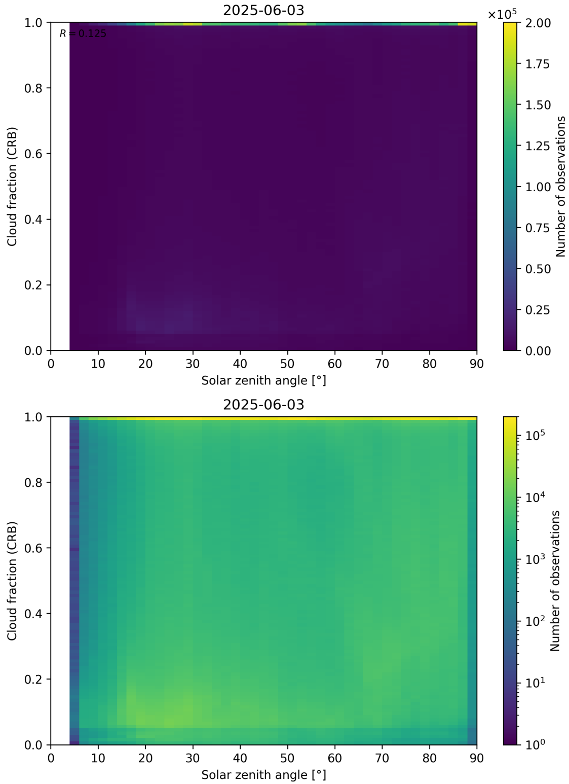
Figure 101: Scatter density plot of “Solar zenith angle” against “Cloud fraction (CRB)” for 2025-06-02 to 2025-06-04.
