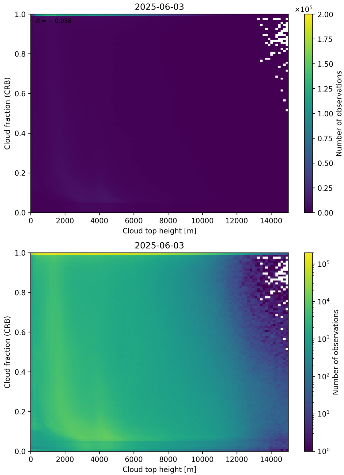
Figure 88: Scatter density plot of “Cloud top height” against “Cloud fraction (CRB)” for 2025-06-02 to 2025-06-04.
