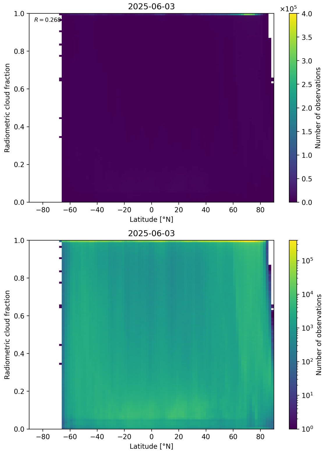
Figure 92: Scatter density plot of “Latitude” against “Radiometric cloud fraction” for 2025-06-02 to 2025-06-04.
