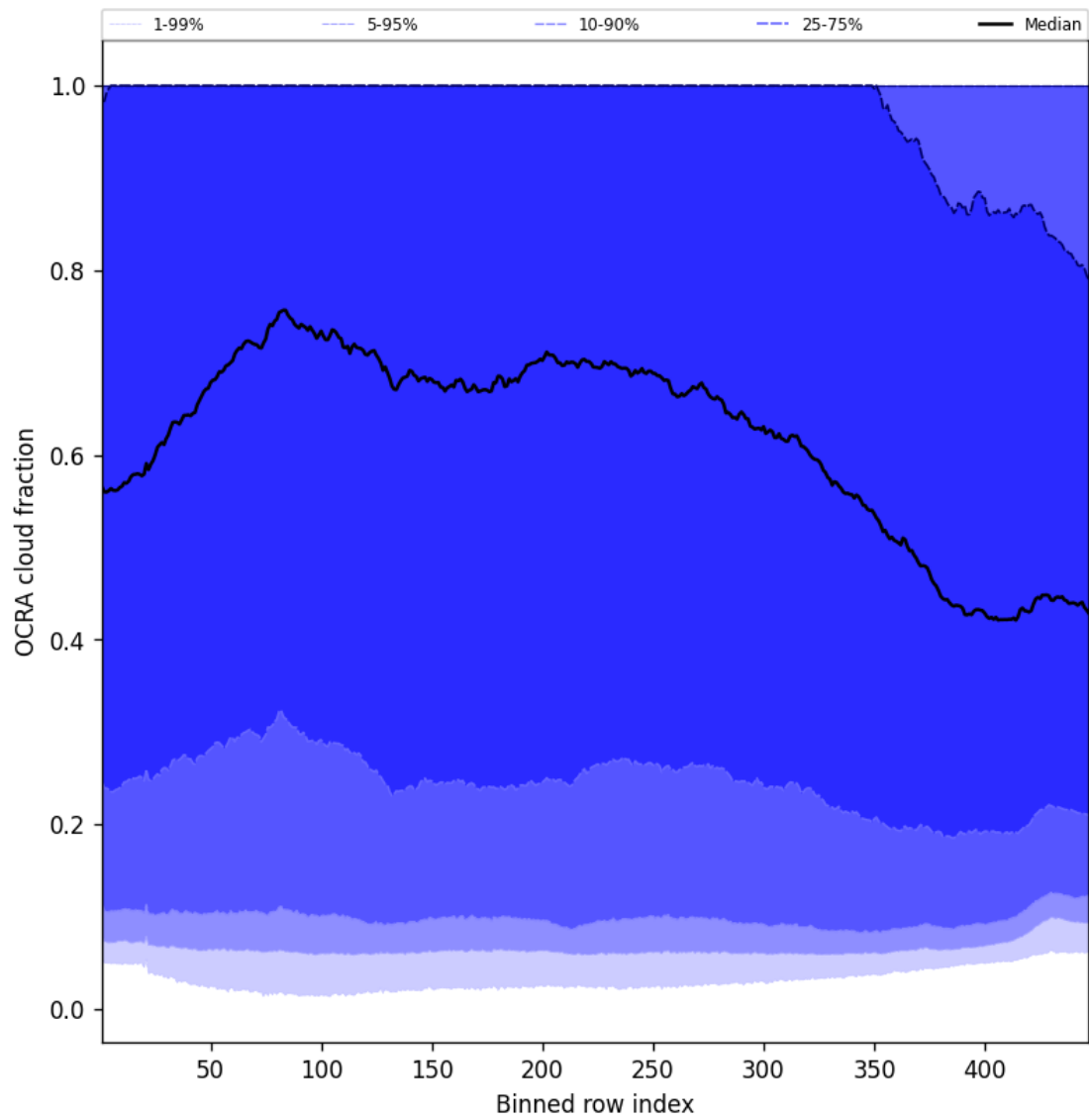
Figure 66: Along track statistics of “OCRA cloud fraction” for 2025-06-02 to 2025-06-04
