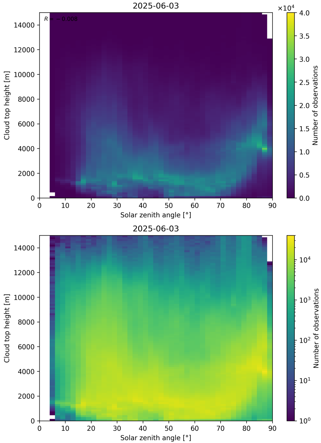
Figure 104: Scatter density plot of “Solar zenith angle” against “Cloud top height” for 2025-06-02 to 2025-06-04.
