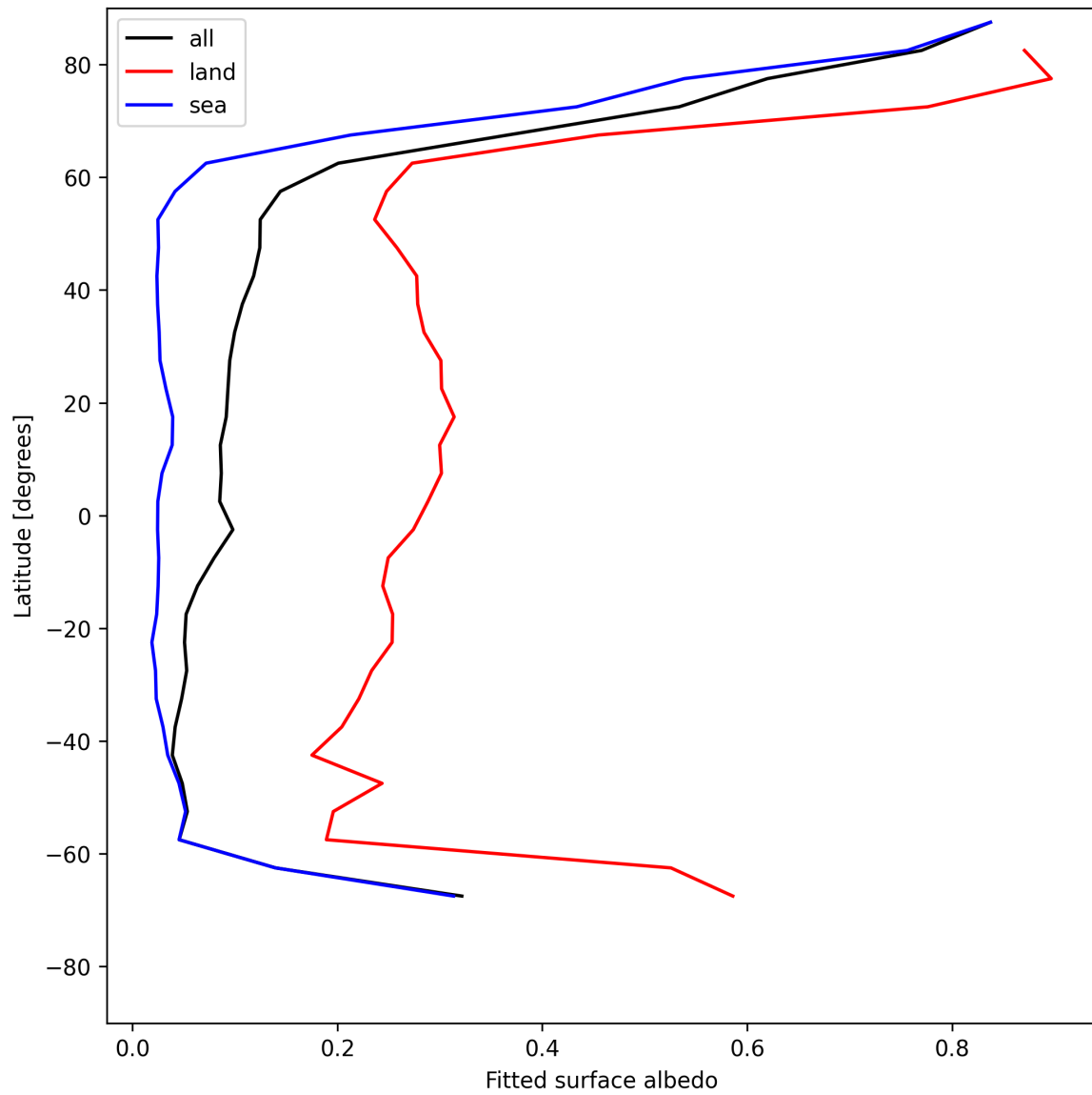
Figure 29: Zonal average of “Fitted surface albedo” for 2025-06-02 to 2025-06-04.
