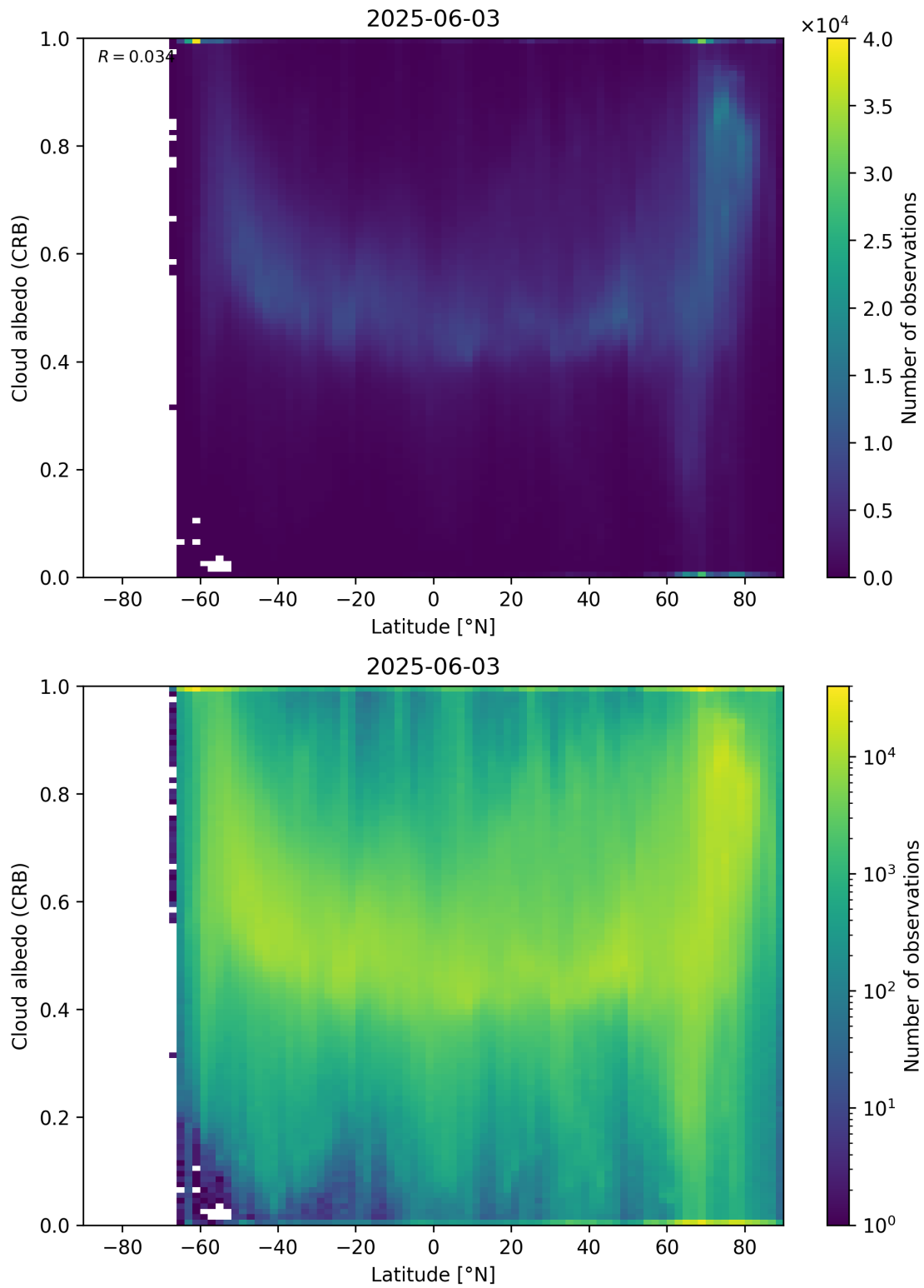
Figure 91: Scatter density plot of “Latitude” against “Cloud albedo (CRB)” for 2025-06-02 to 2025-06-04.
