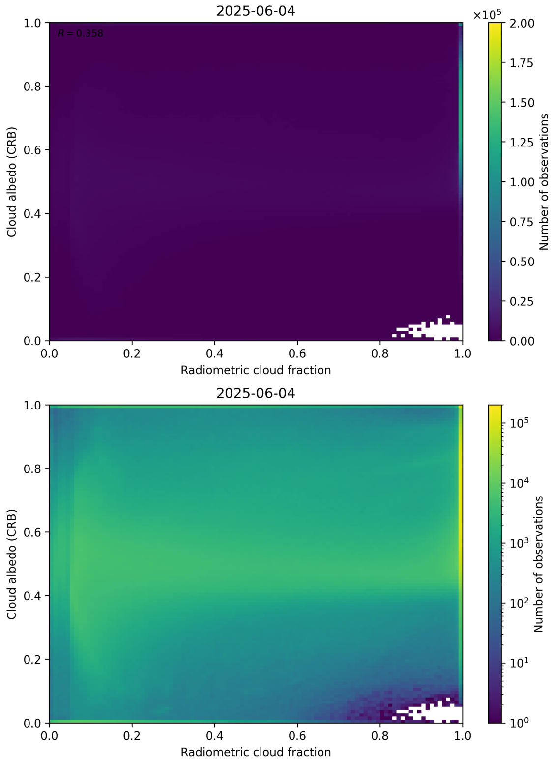
Figure 71: Scatter density plot of “Radiometric cloud fraction” against “Cloud albedo (CRB)” for 2025-06-03 to 2025-06-05.
