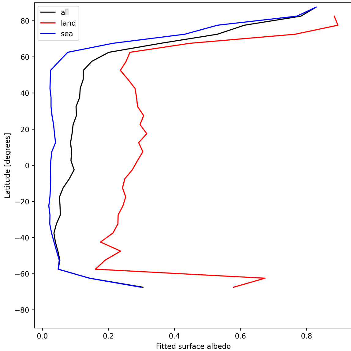
Figure 29: Zonal average of “Fitted surface albedo” for 2025-06-03 to 2025-06-05.
