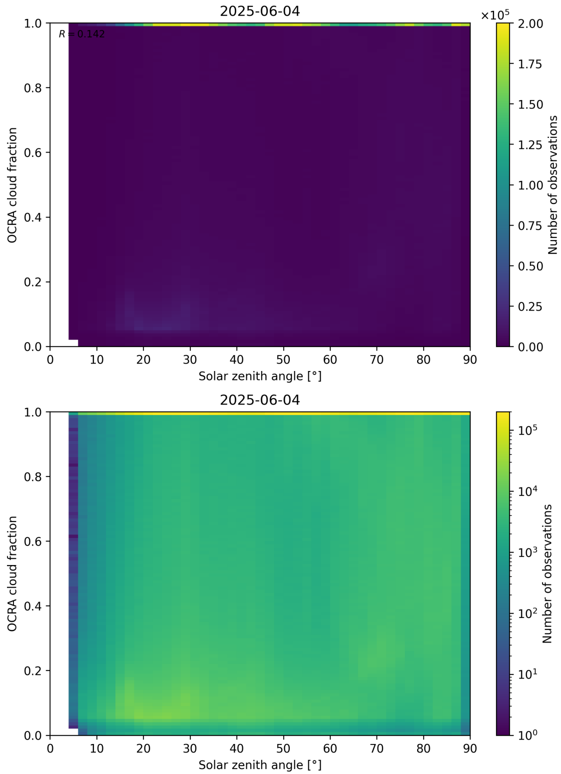
Figure 100: Scatter density plot of “Solar zenith angle” against “OCRA cloud fraction” for 2025-06-03 to 2025-06-05.
