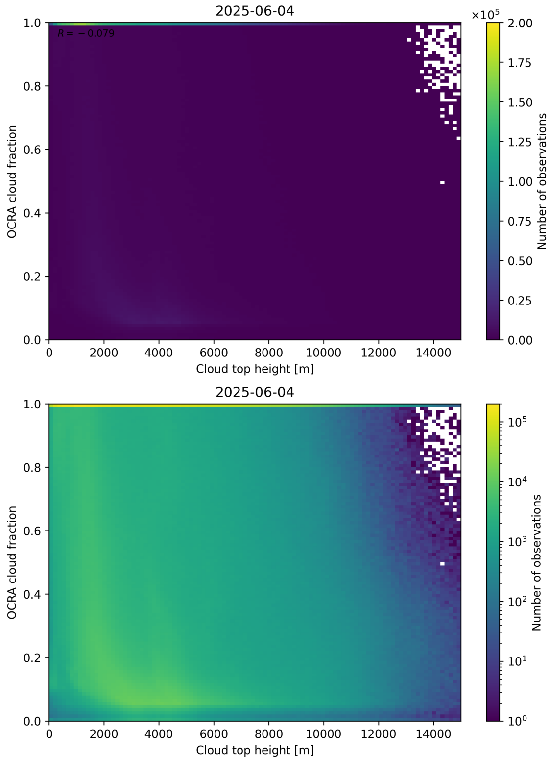
Figure 87: Scatter density plot of “Cloud top height” against “OCRA cloud fraction” for 2025-06-03 to 2025-06-05.
