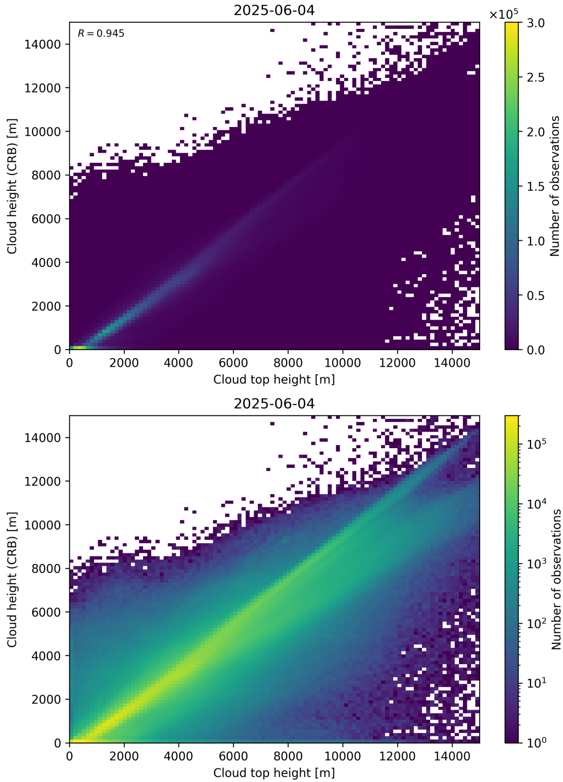
Figure 89: Scatter density plot of “Cloud top height” against “Cloud height (CRB)” for 2025-06-03 to 2025-06-05.
