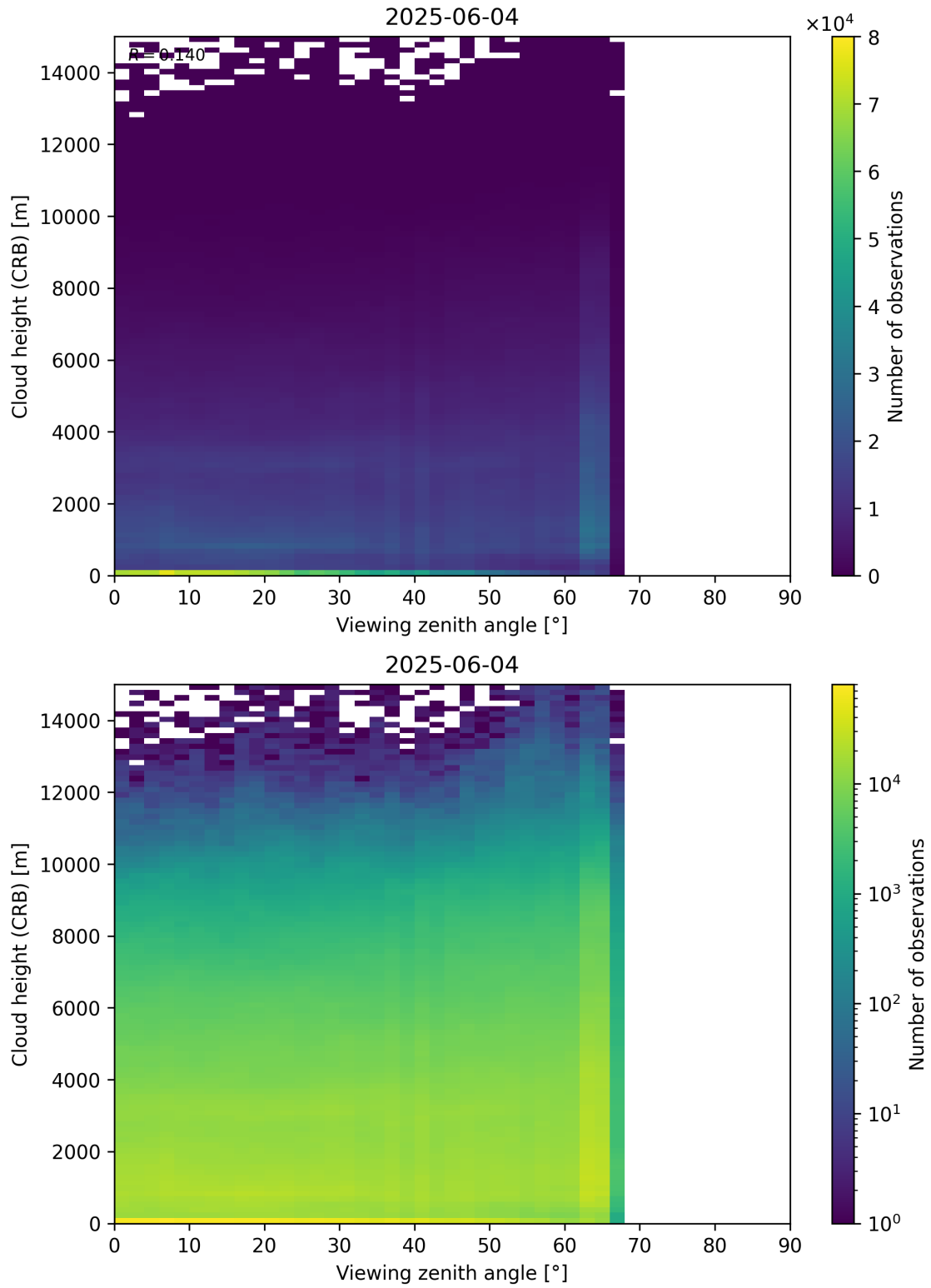
Figure 110: Scatter density plot of “Viewing zenith angle” against “Cloud height (CRB)” for 2025-06-03 to 2025-06-05.
