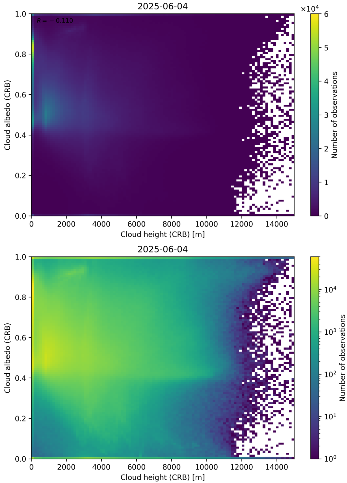
Figure 80: Scatter density plot of “Cloud height (CRB)” against “Cloud albedo (CRB)” for 2025-06-03 to 2025-06-05.
