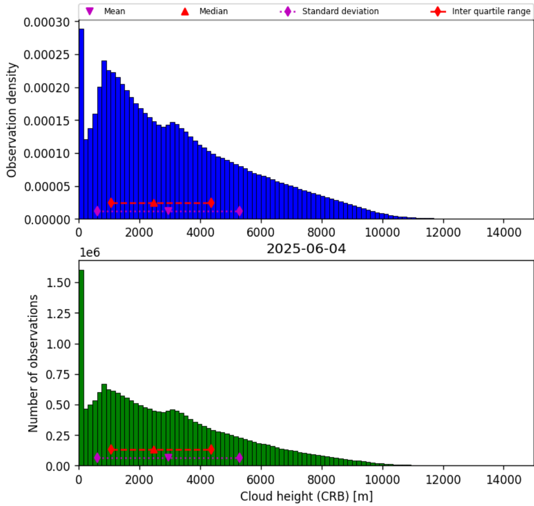
Figure 43: Histogram of “Cloud height (CRB)” for 2025-06-03 to 2025-06-05
