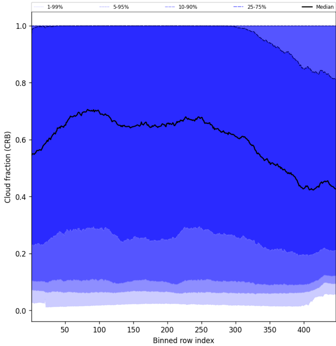
Figure 58: Along track statistics of “Cloud fraction (CRB)” for 2025-06-03 to 2025-06-05
