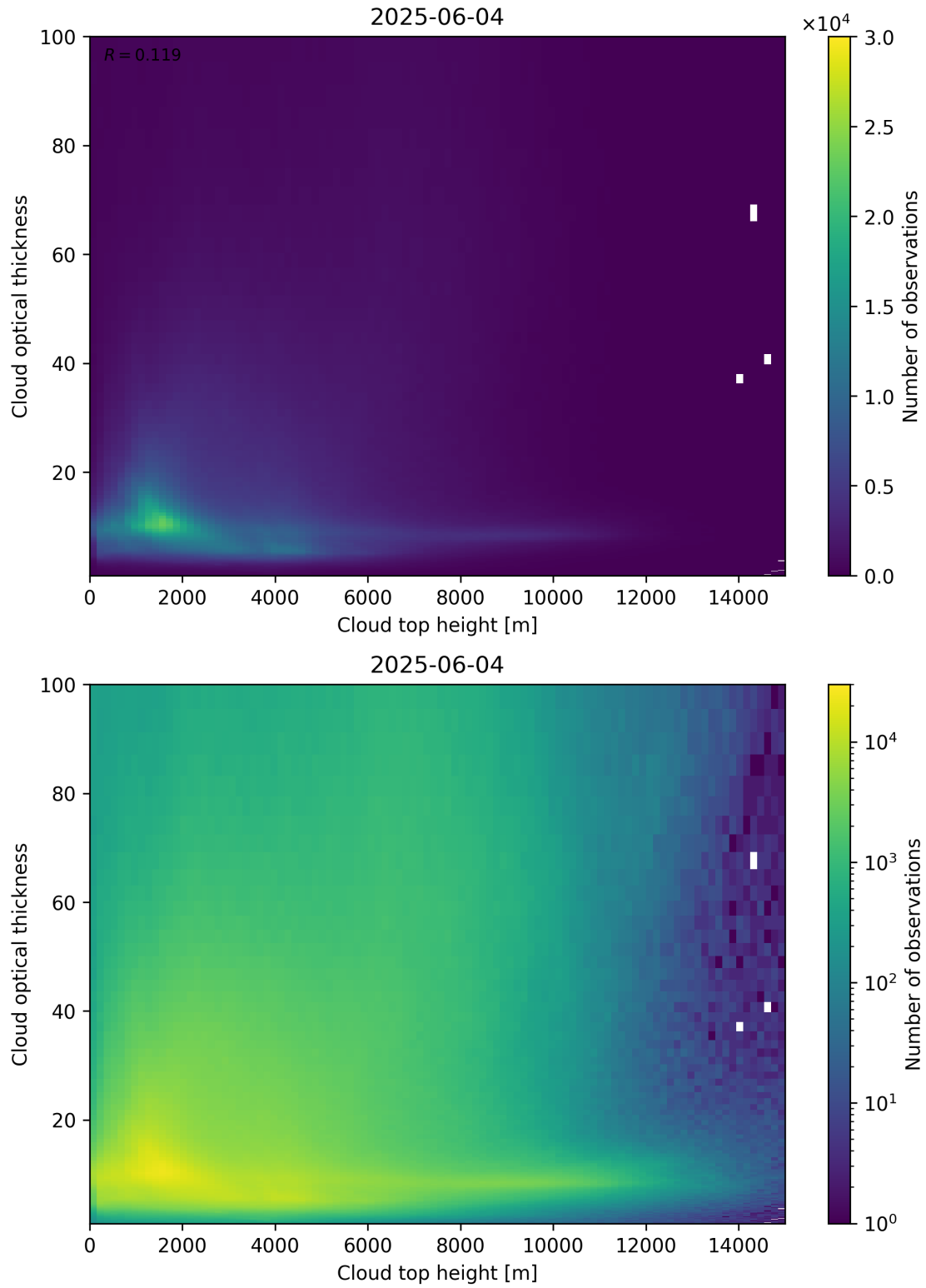
Figure 90: Scatter density plot of “Cloud top height” against “Cloud optical thickness” for 2025-06-03 to 2025-06-05.
