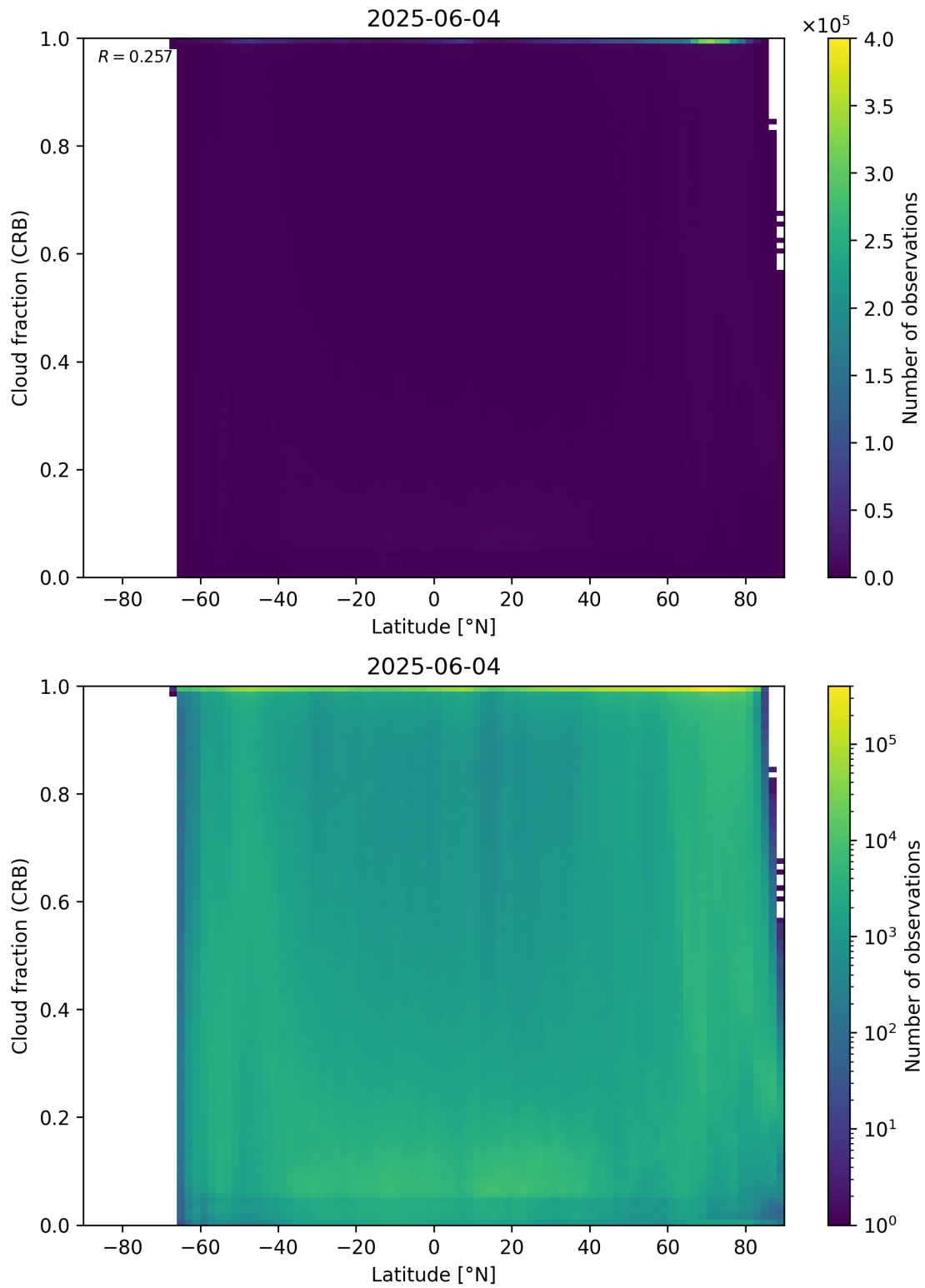
Figure 94: Scatter density plot of “Latitude” against “Cloud fraction (CRB)” for 2025-06-03 to 2025-06-05.
