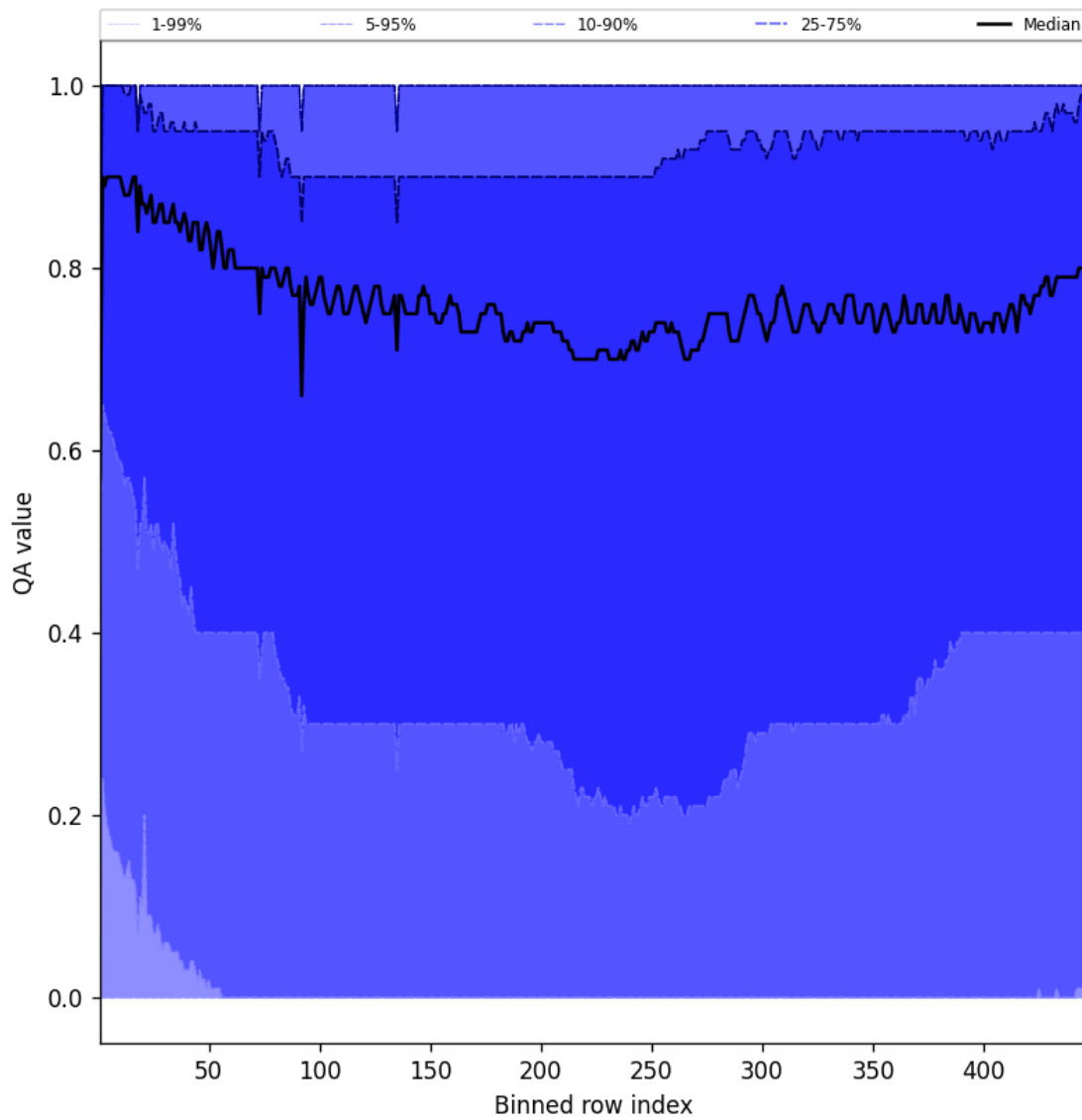
Figure 54: Along track statistics of “QA value” for 2025-06-03 to 2025-06-05
