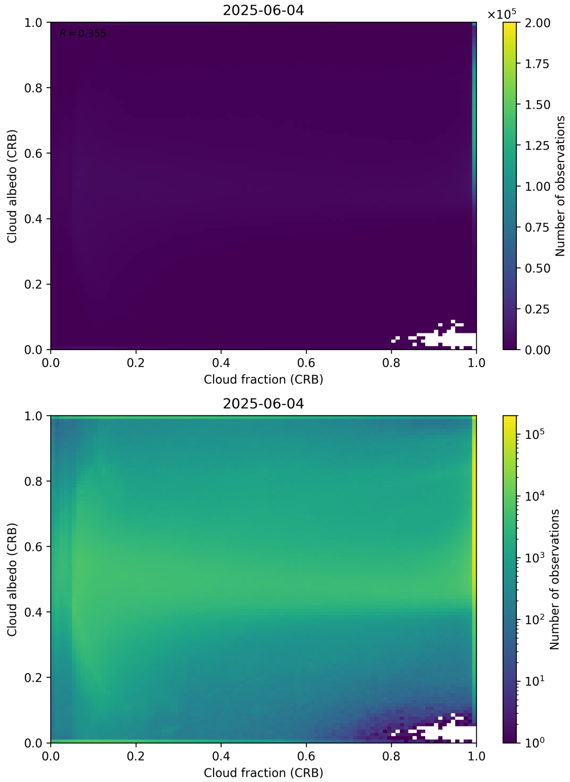
Figure 77: Scatter density plot of “Cloud fraction (CRB)” against “Cloud albedo (CRB)” for 2025-06-03 to 2025-06-05.
