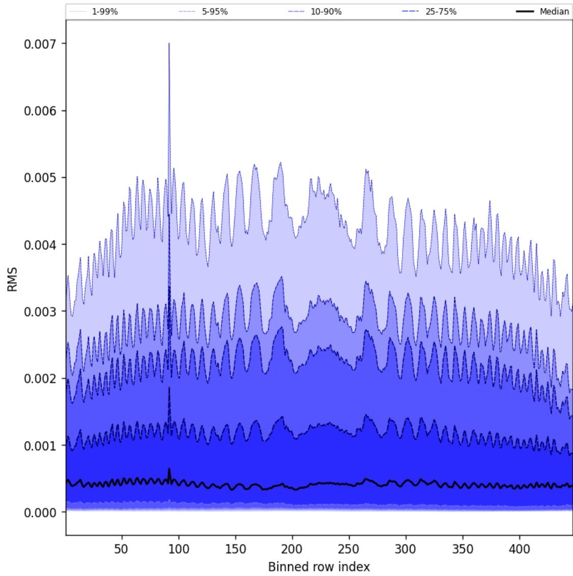
Figure 63: Along track statistics of “RMS” for 2025-06-03 to 2025-06-05
