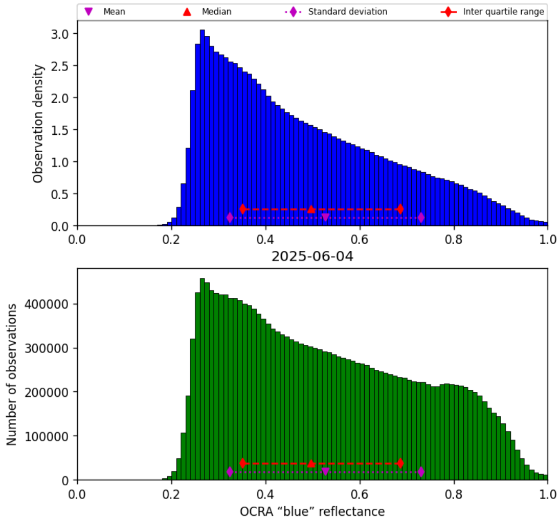
Figure 51: Histogram of “OCRA “blue” reflectance” for 2025-06-03 to 2025-06-05
