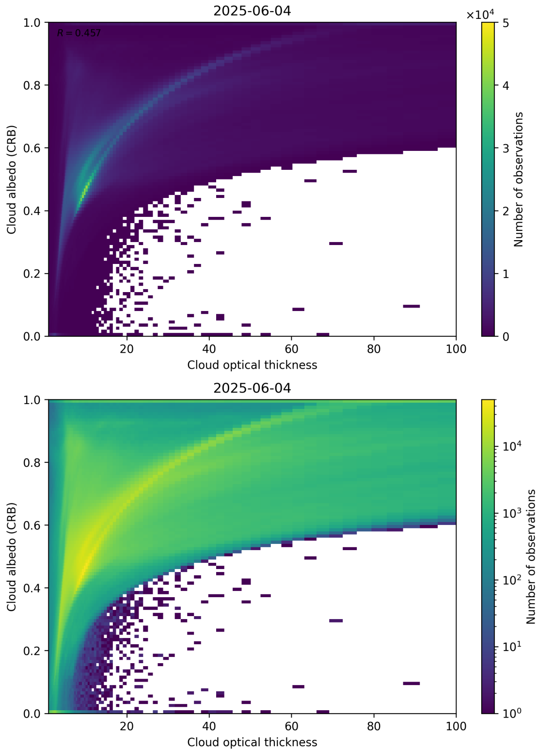
Figure 82: Scatter density plot of “Cloud optical thickness” against “Cloud albedo (CRB)” for 2025-06-03 to 2025-06-05.
