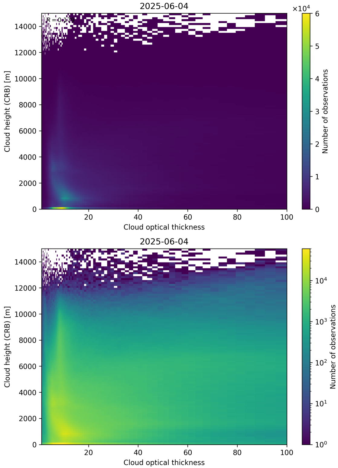
Figure 85: Scatter density plot of “Cloud optical thickness” against “Cloud height (CRB)” for 2025-06-03 to 2025-06-05.
