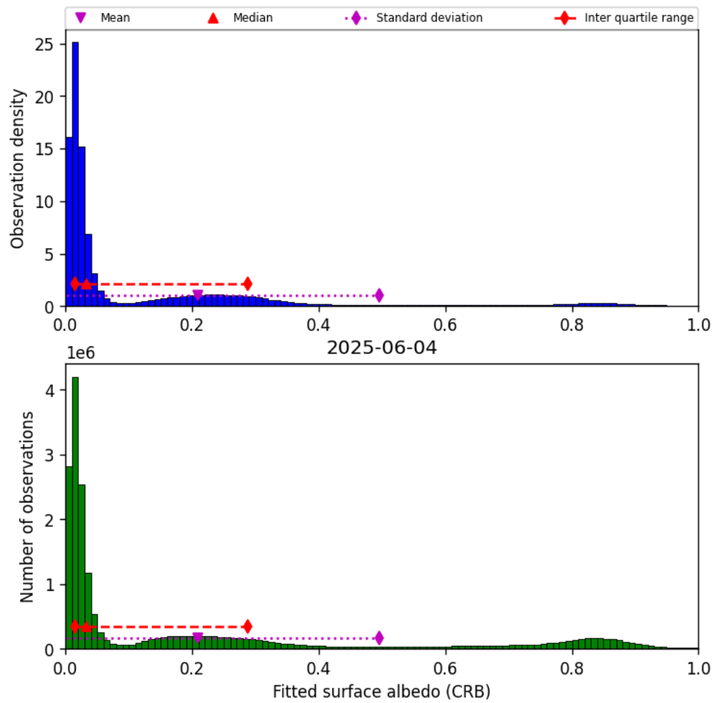
Figure 46: Histogram of “Fitted surface albedo (CRB)” for 2025-06-03 to 2025-06-05
