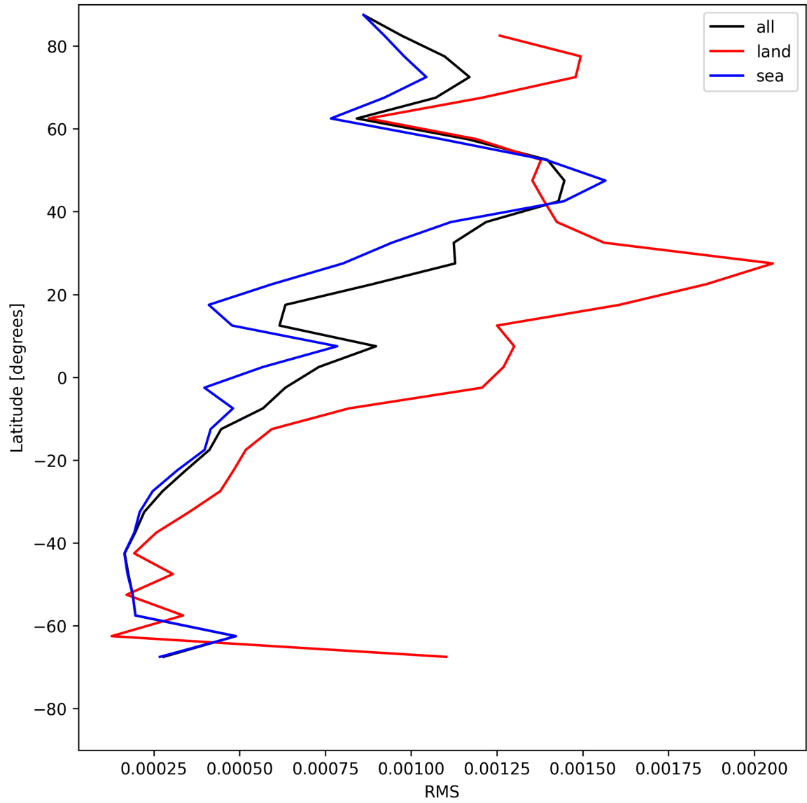
Figure 31: Zonal average of “RMS” for 2025-06-03 to 2025-06-05.
