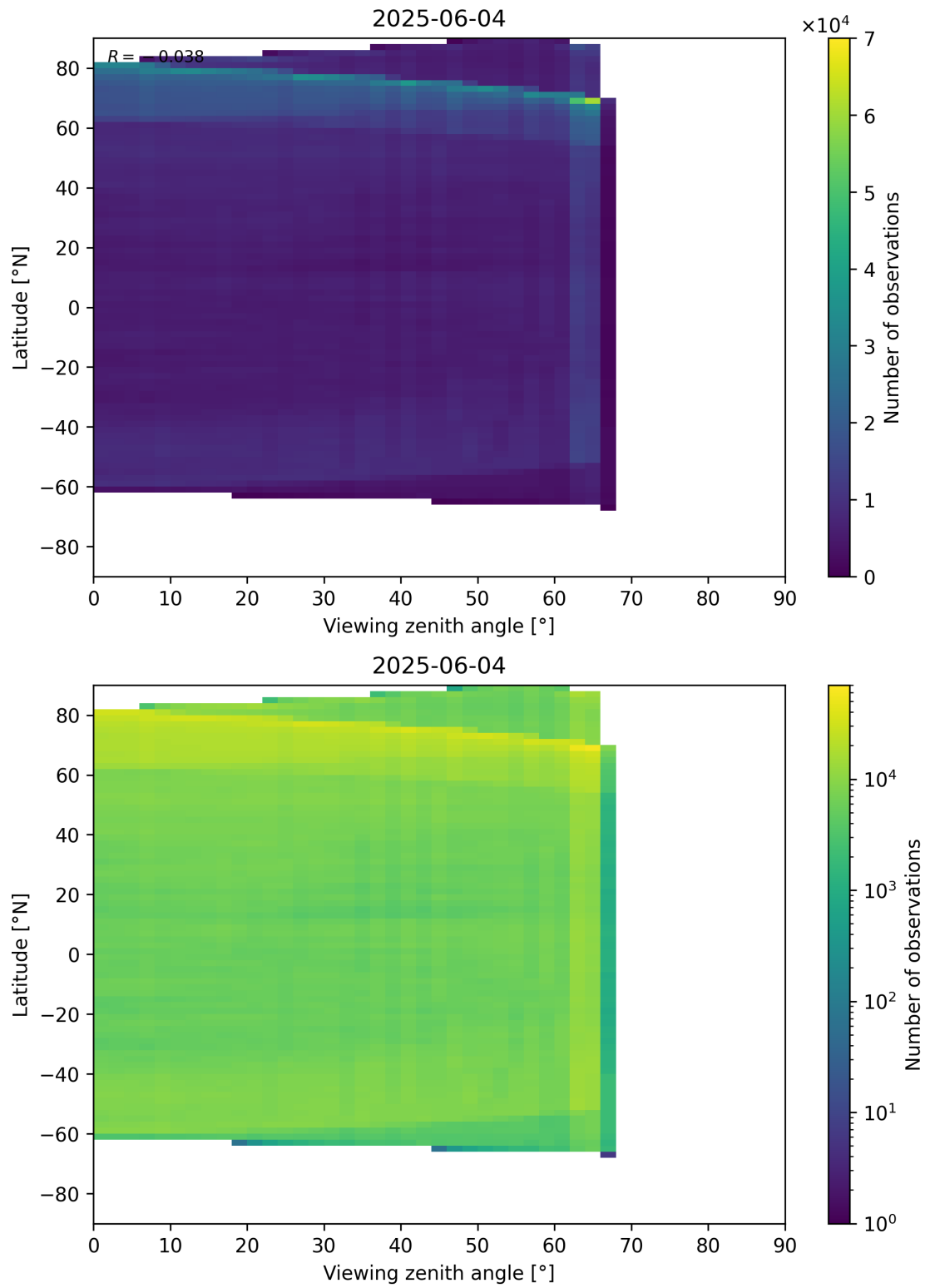
Figure 113: Scatter density plot of “Viewing zenith angle” against “Latitude” for 2025-06-03 to 2025-06-05.
