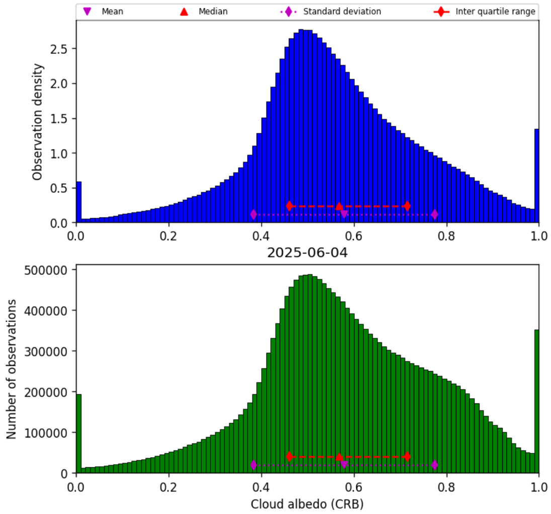
Figure 44: Histogram of “Cloud albedo (CRB)” for 2025-06-03 to 2025-06-05
