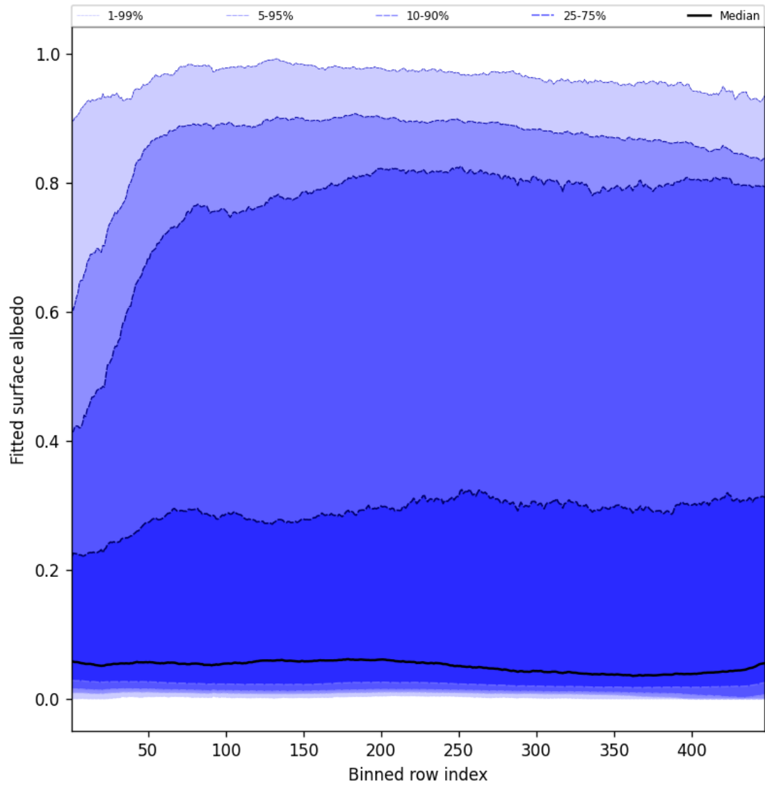
Figure 61: Along track statistics of “Fitted surface albedo” for 2025-06-03 to 2025-06-05
