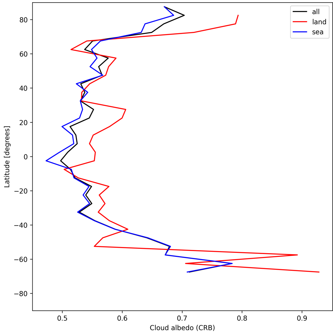
Figure 28: Zonal average of “Cloud albedo (CRB)” for 2025-06-03 to 2025-06-05.
