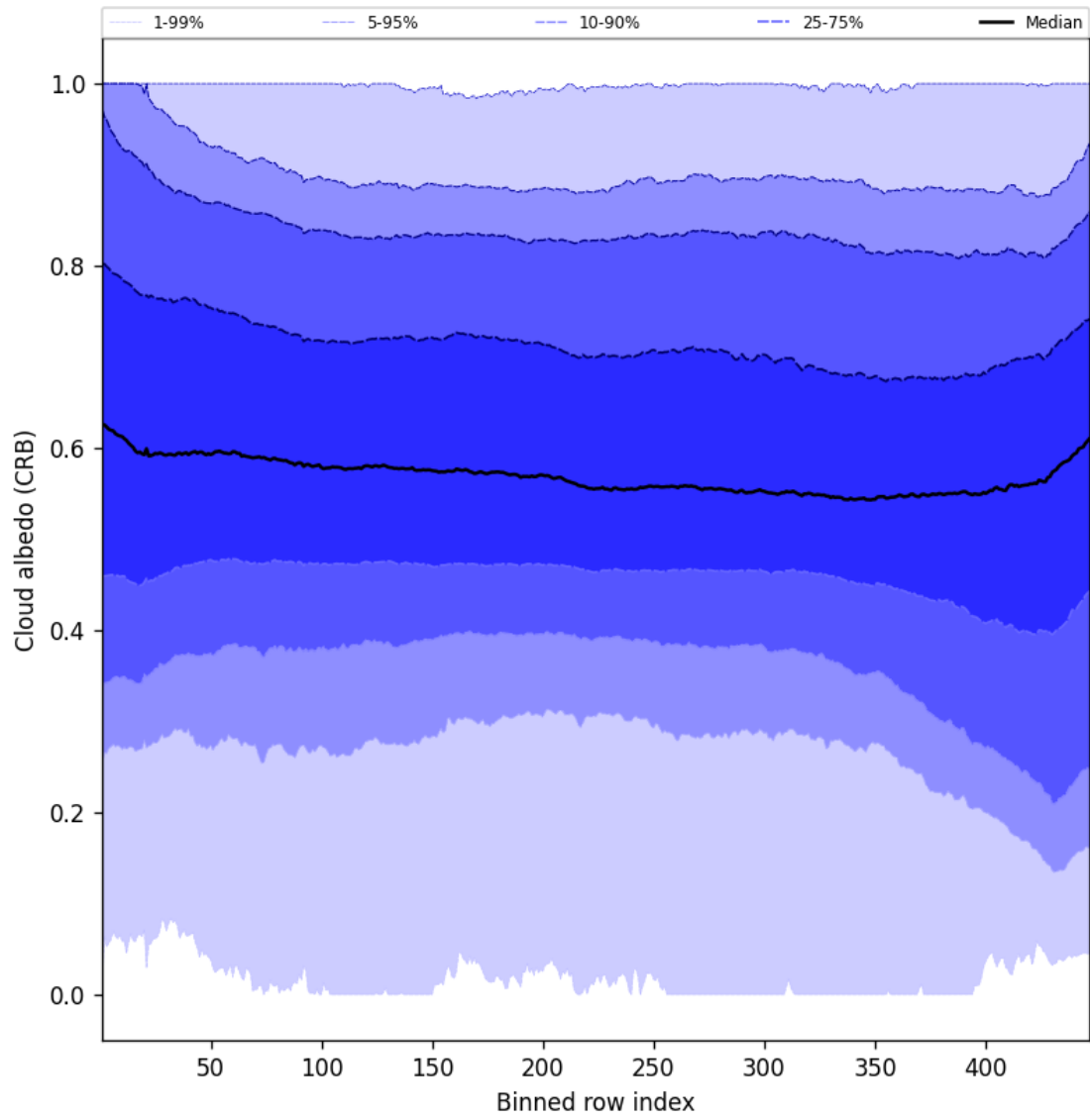
Figure 60: Along track statistics of “Cloud albedo (CRB)” for 2025-06-03 to 2025-06-05
