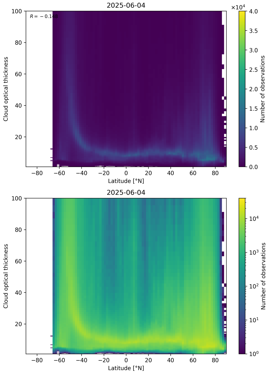
Figure 96: Scatter density plot of “Latitude” against “Cloud optical thickness” for 2025-06-03 to 2025-06-05.
