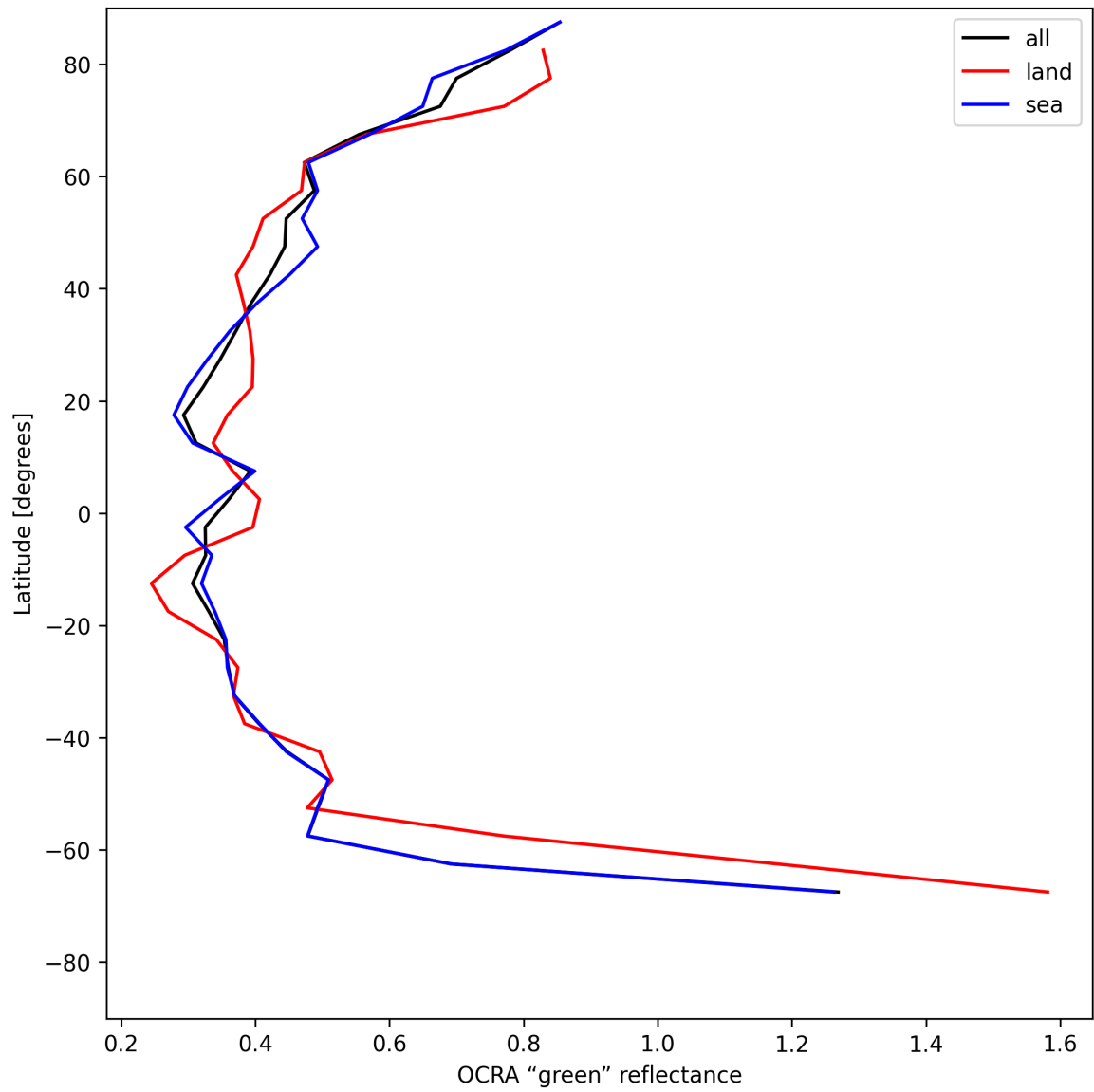
Figure 36: Zonal average of “OCRA “green” reflectance” for 2025-06-03 to 2025-06-05.
