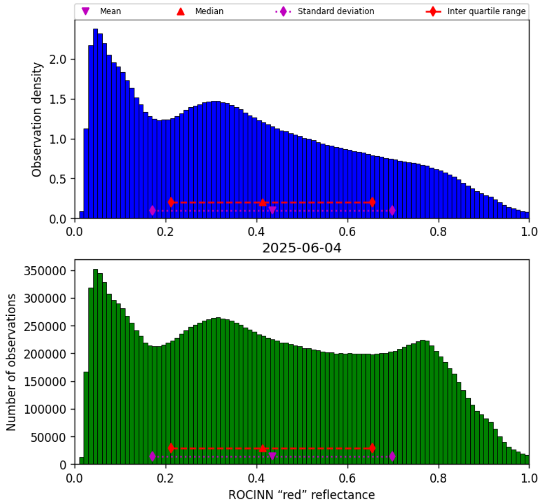
Figure 53: Histogram of “ROCINN “red” reflectance” for 2025-06-03 to 2025-06-05
