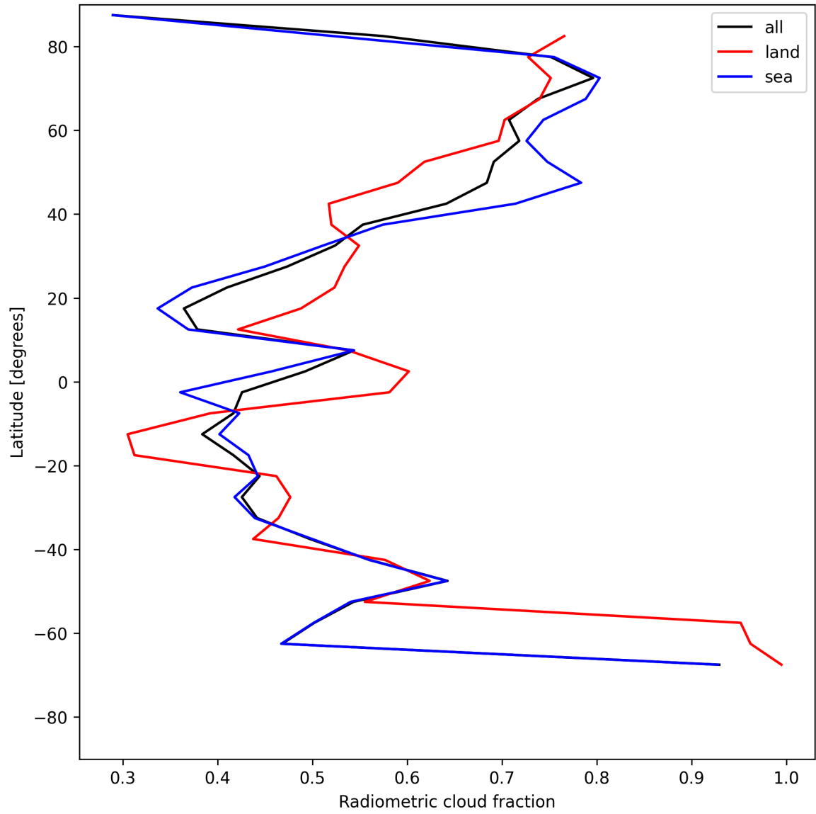
Figure 23: Zonal average of “Radiometric cloud fraction” for 2025-06-03 to 2025-06-05.
