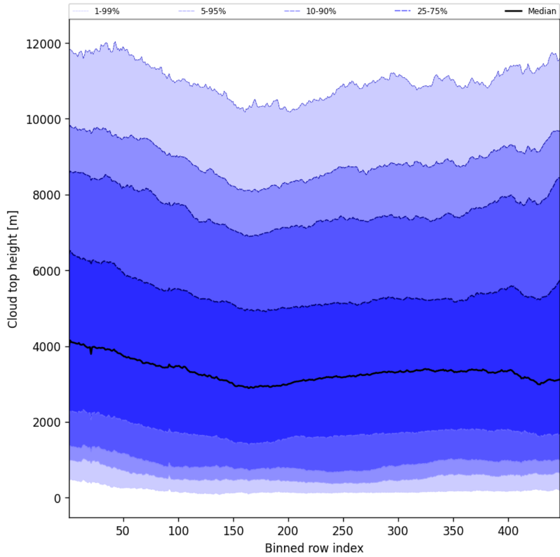
Figure 56: Along track statistics of “Cloud top height” for 2025-06-03 to 2025-06-05
