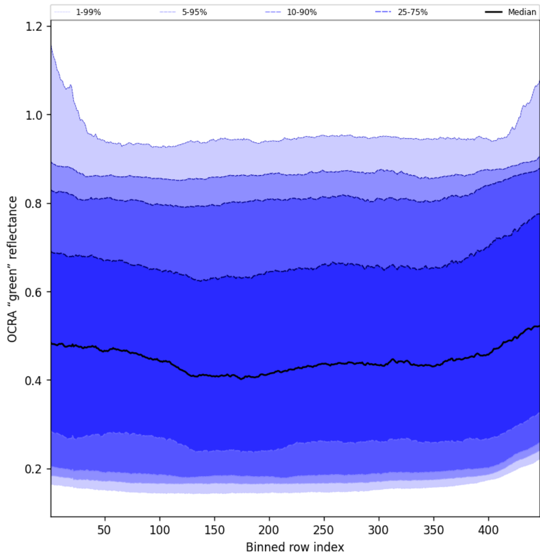
Figure 68: Along track statistics of “OCRA “green” reflectance” for 2025-06-03 to 2025-06-05
