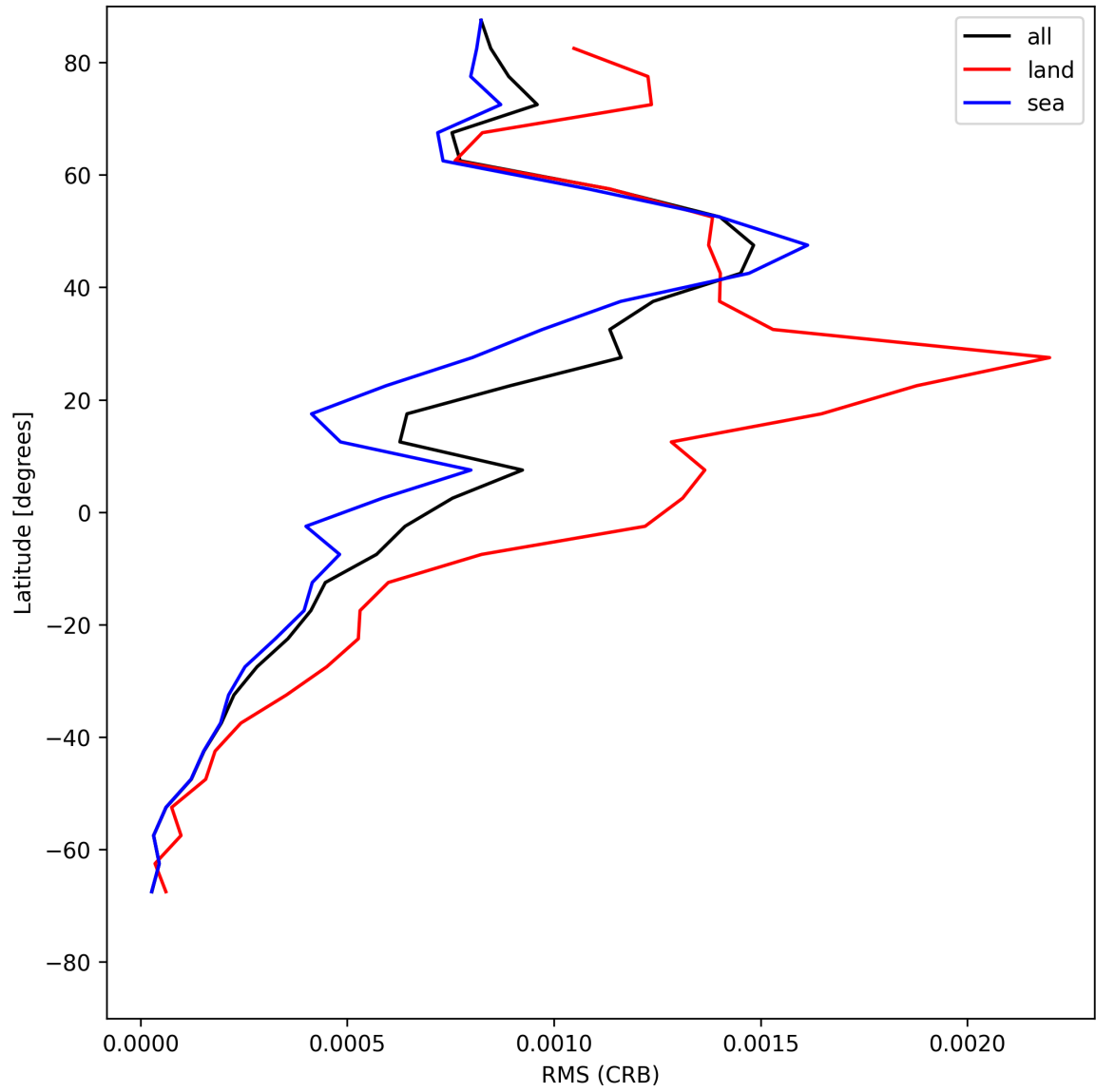
Figure 32: Zonal average of “RMS (CRB)” for 2025-06-03 to 2025-06-05.
