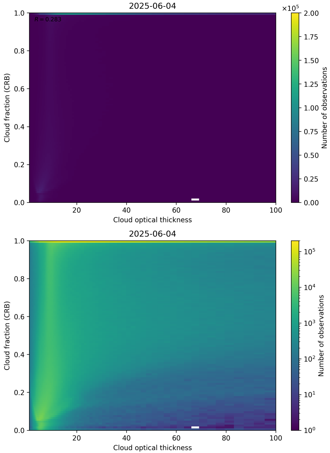
Figure 84: Scatter density plot of “Cloud optical thickness” against “Cloud fraction (CRB)” for 2025-06-03 to 2025-06-05.
