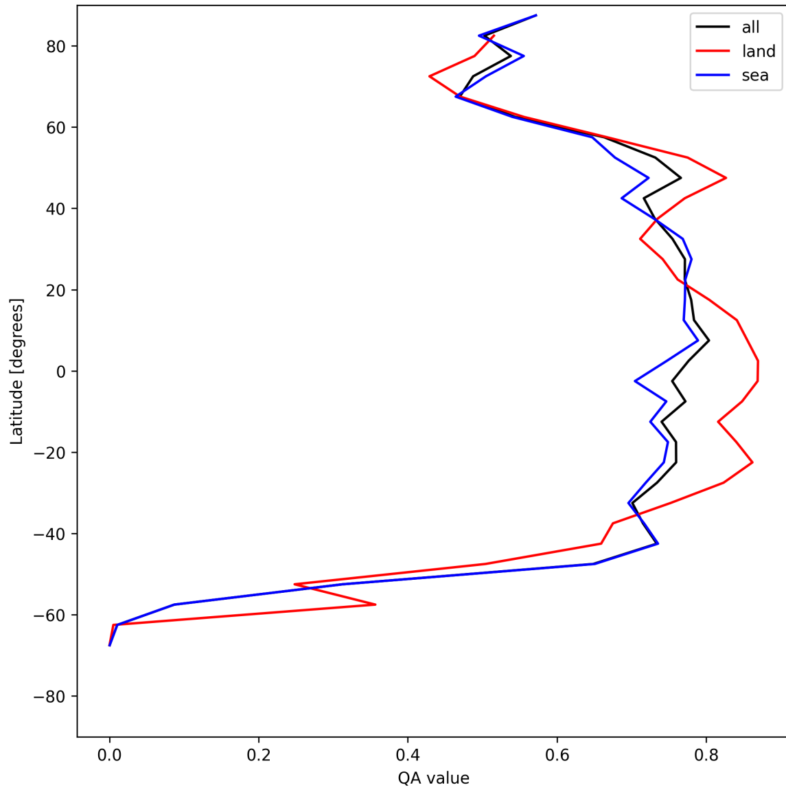
Figure 22: Zonal average of “QA value” for 2025-06-03 to 2025-06-05.
