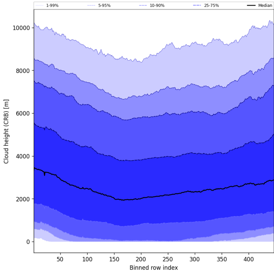
Figure 59: Along track statistics of “Cloud height (CRB)” for 2025-06-03 to 2025-06-05
