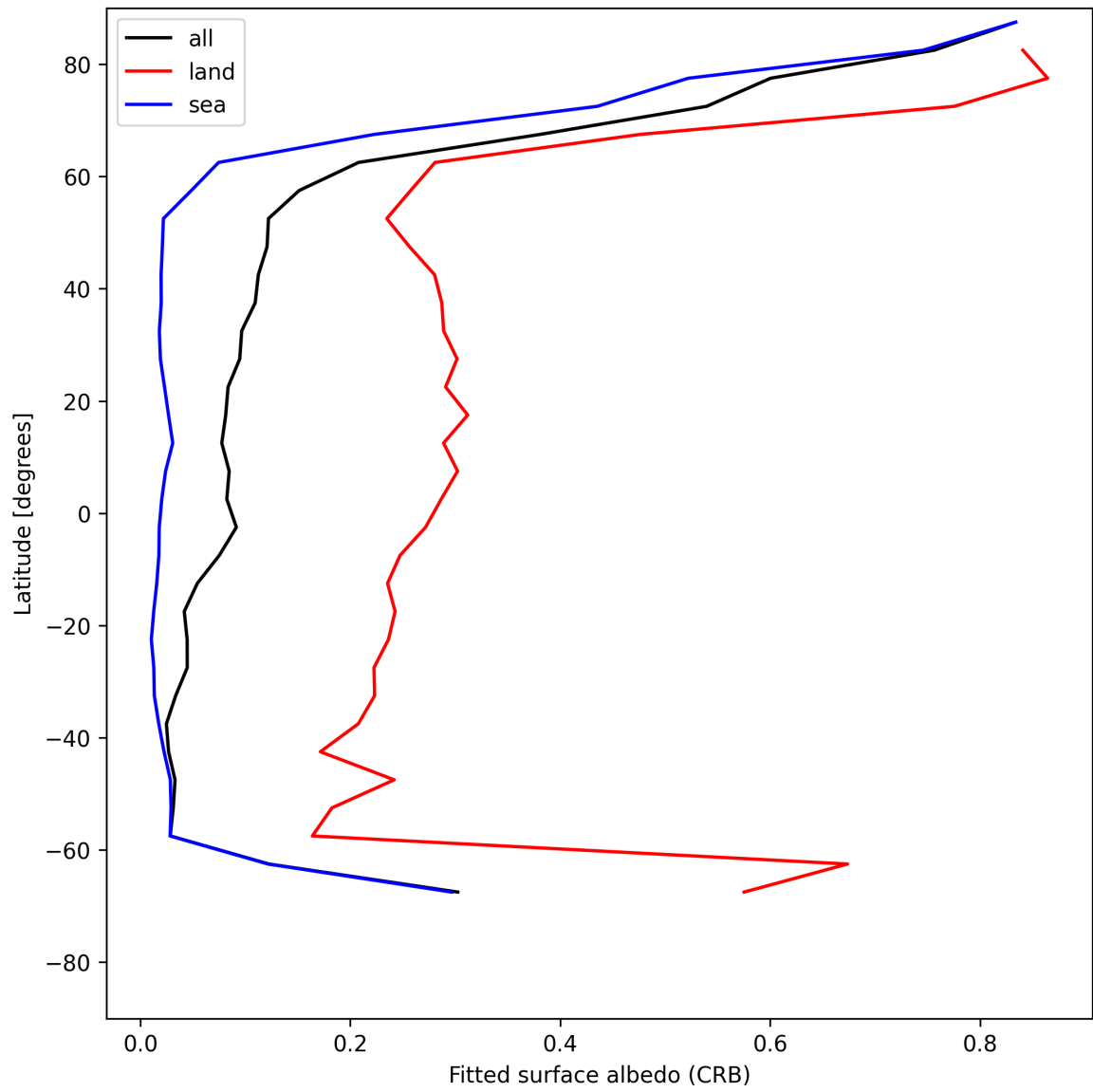
Figure 30: Zonal average of “Fitted surface albedo (CRB)” for 2025-06-03 to 2025-06-05.
