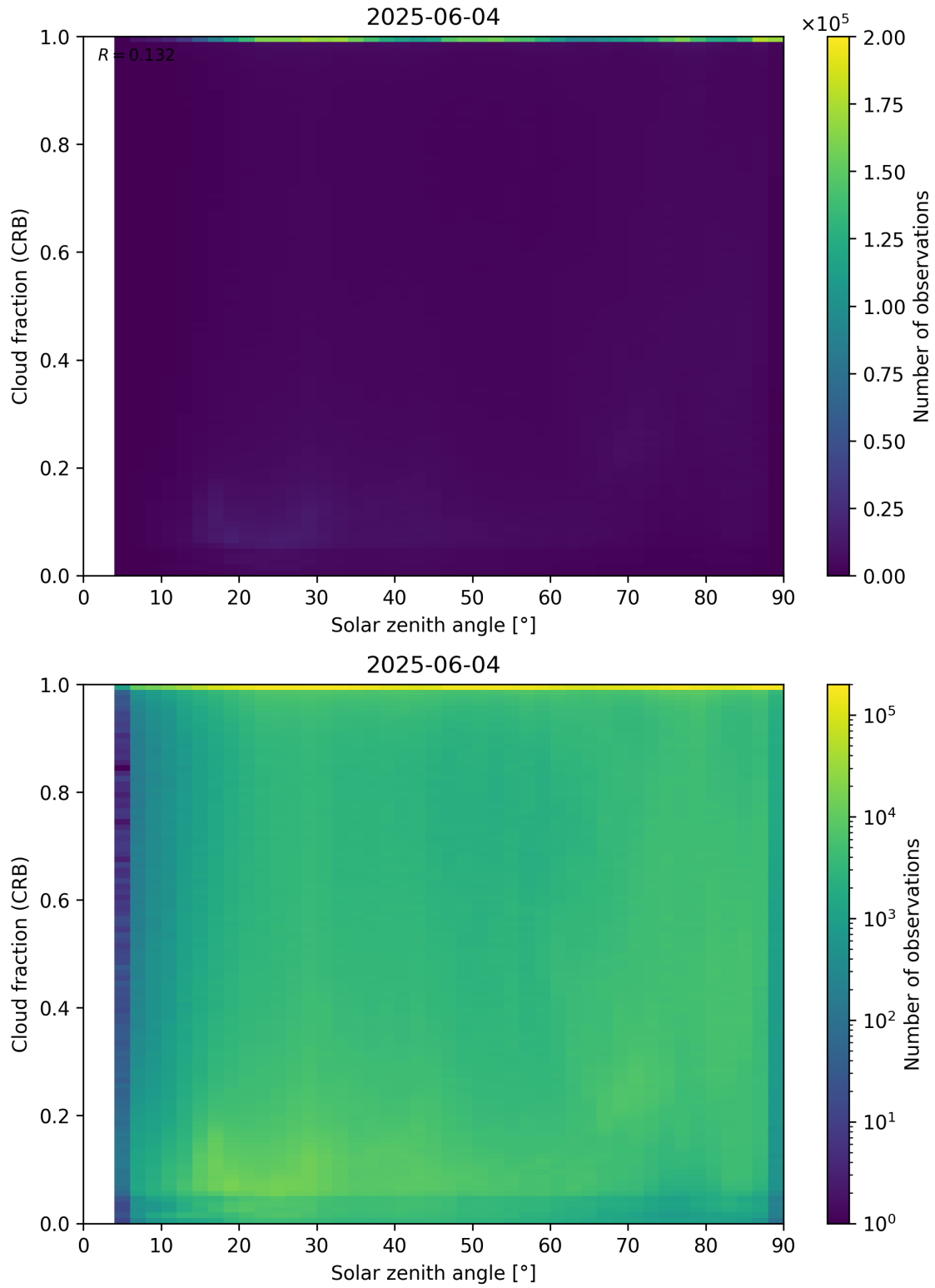
Figure 101: Scatter density plot of “Solar zenith angle” against “Cloud fraction (CRB)” for 2025-06-03 to 2025-06-05.
