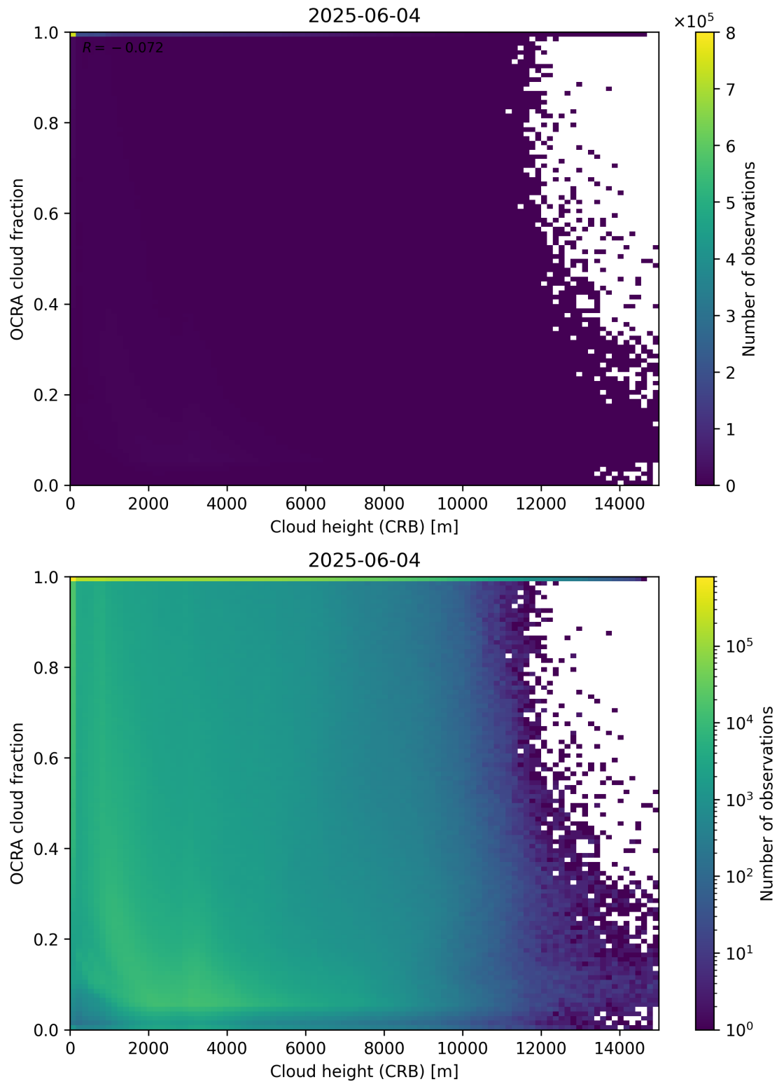
Figure 81: Scatter density plot of “Cloud height (CRB)” against “OCRA cloud fraction” for 2025-06-03 to 2025-06-05.
