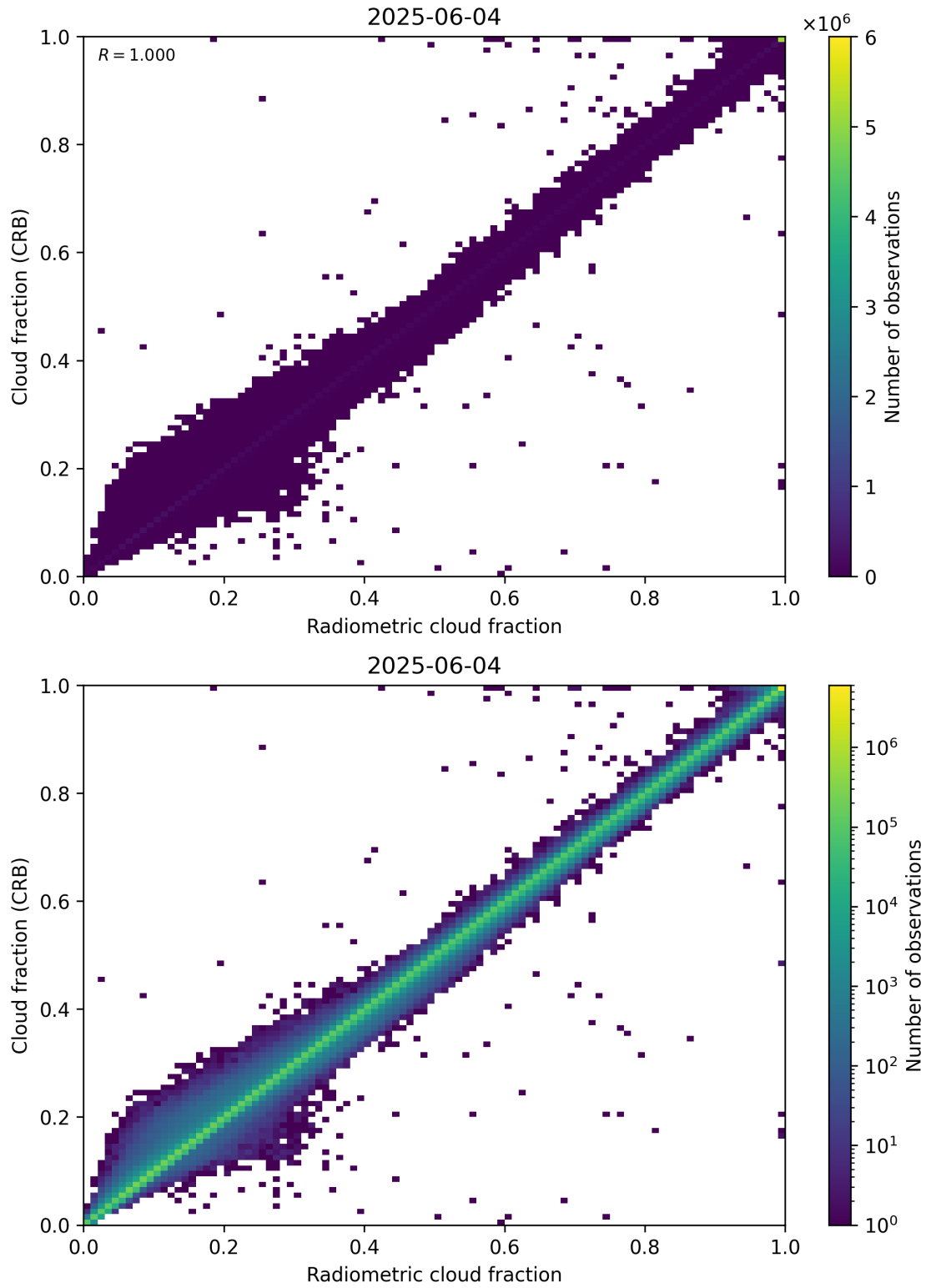
Figure 73: Scatter density plot of “Radiometric cloud fraction” against “Cloud fraction (CRB)” for 2025-06-03 to 2025-06-05.
