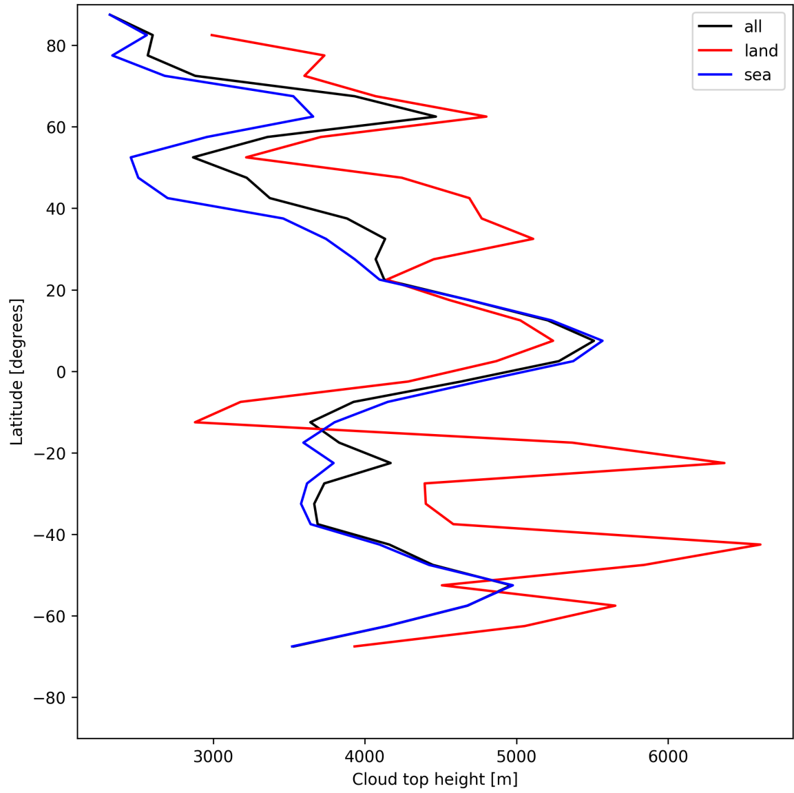
Figure 24: Zonal average of “Cloud top height” for 2025-06-03 to 2025-06-05.
