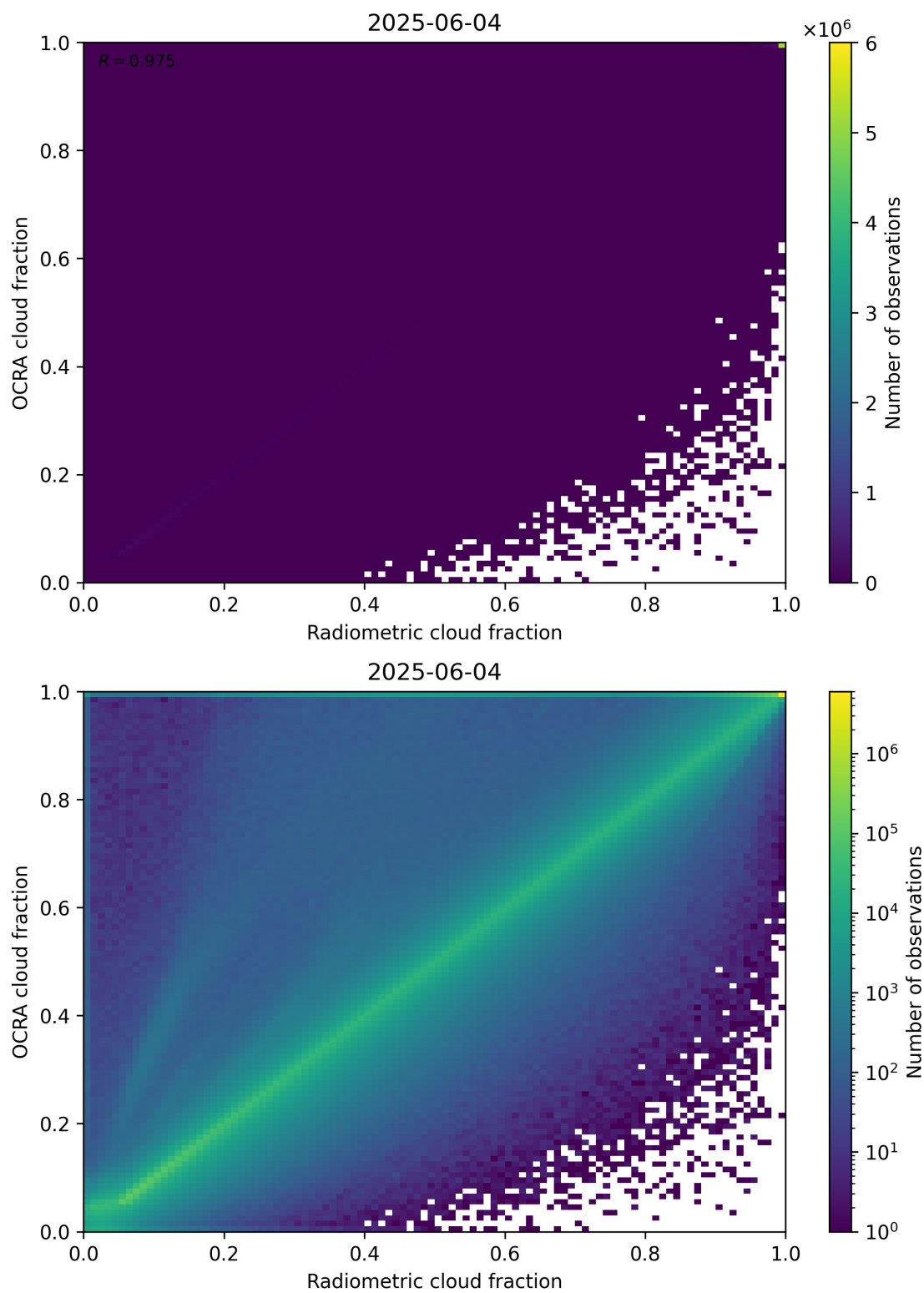
Figure 72: Scatter density plot of “Radiometric cloud fraction” against “OCRA cloud fraction” for 2025-06-03 to 2025-06-05.
