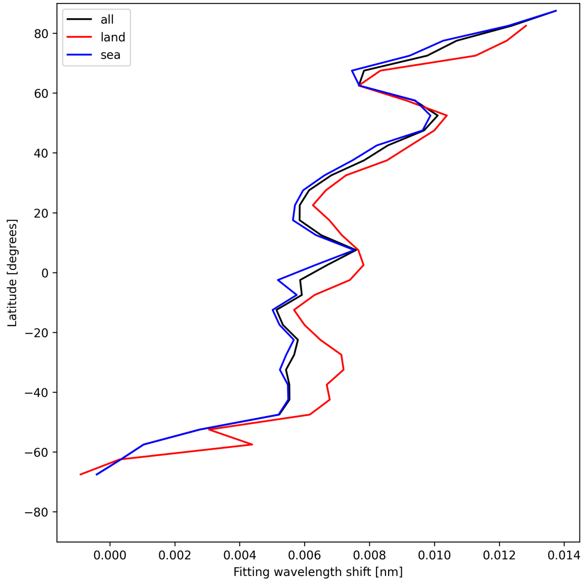
Figure 33: Zonal average of “Fitting wavelength shift” for 2025-06-03 to 2025-06-05.
