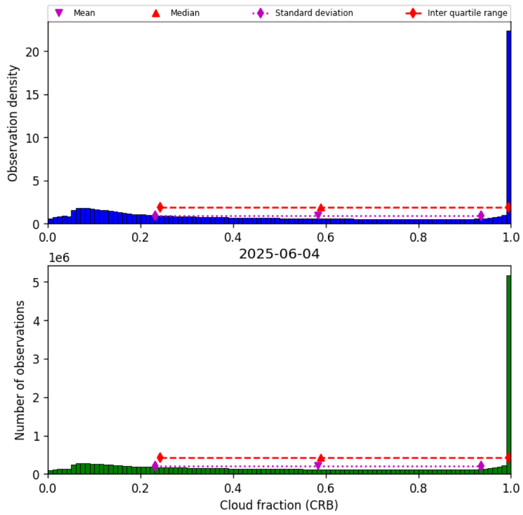
Figure 42: Histogram of “Cloud fraction (CRB)” for 2025-06-03 to 2025-06-05
