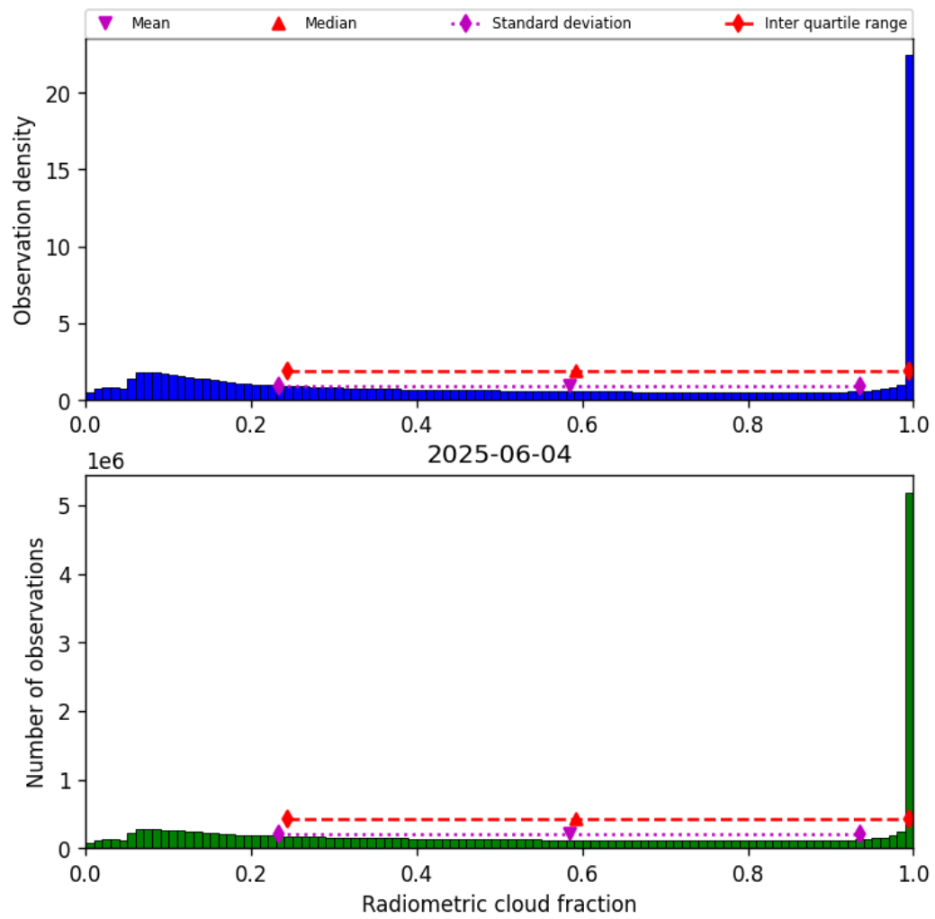
Figure 39: Histogram of “Radiometric cloud fraction” for 2025-06-03 to 2025-06-05
