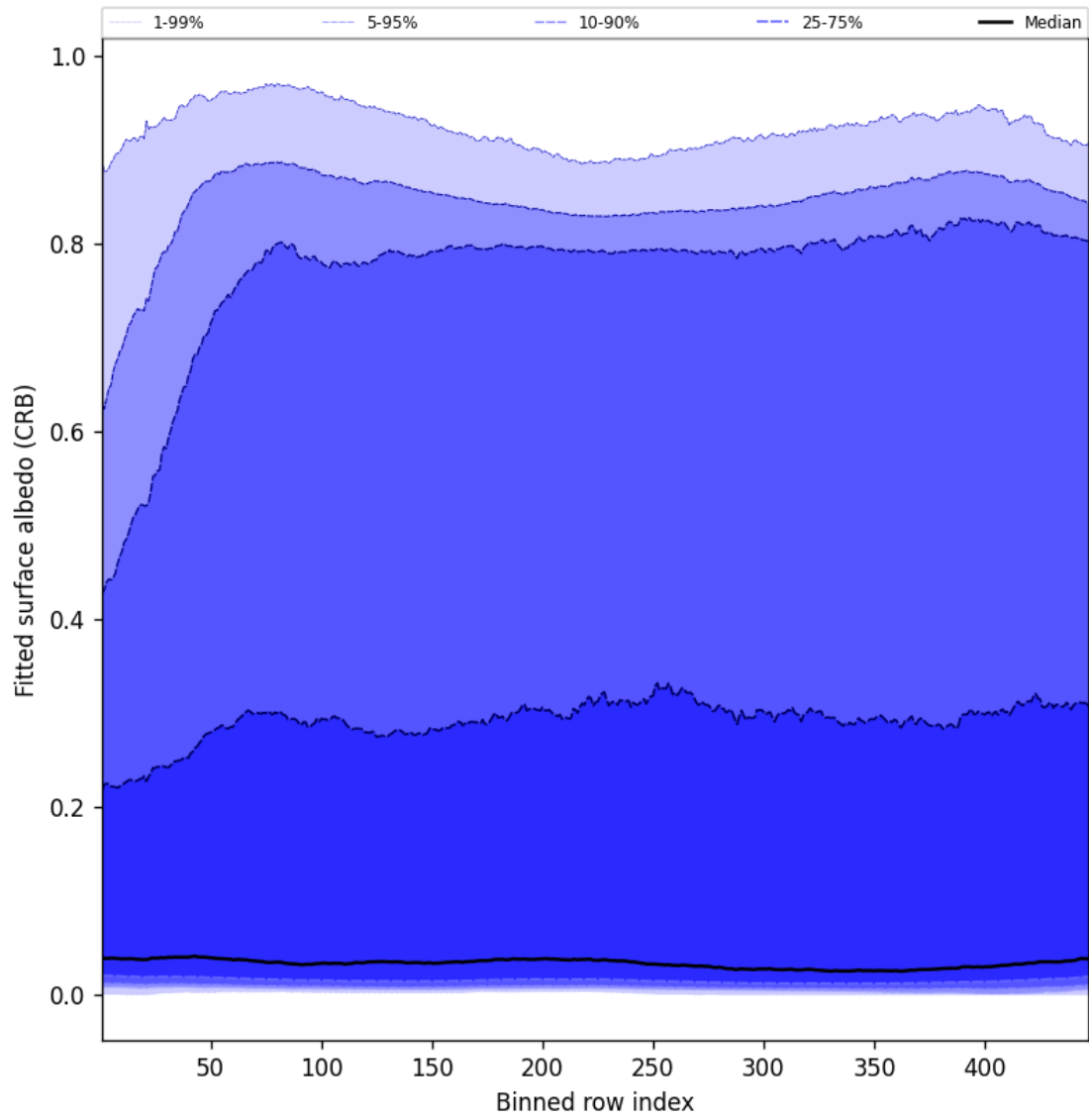
Figure 62: Along track statistics of “Fitted surface albedo (CRB)” for 2025-06-03 to 2025-06-05
