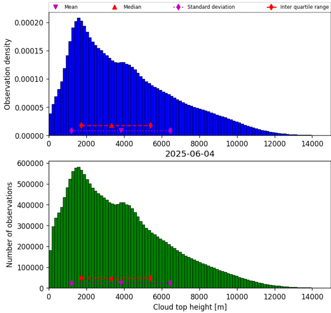
Figure 40: Histogram of “Cloud top height” for 2025-06-03 to 2025-06-05
