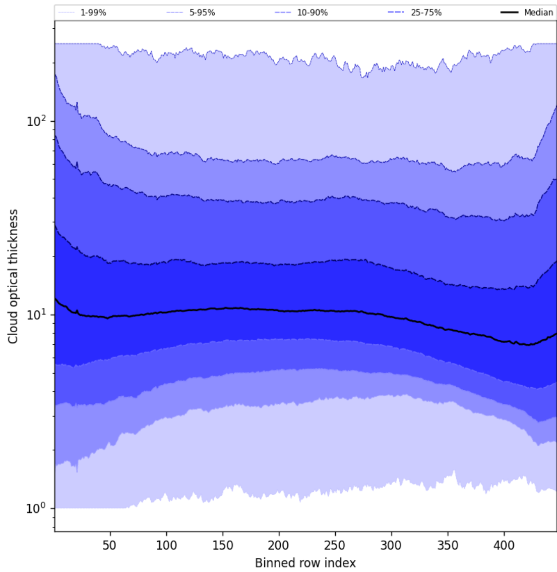
Figure 57: Along track statistics of “Cloud optical thickness” for 2025-06-03 to 2025-06-05
