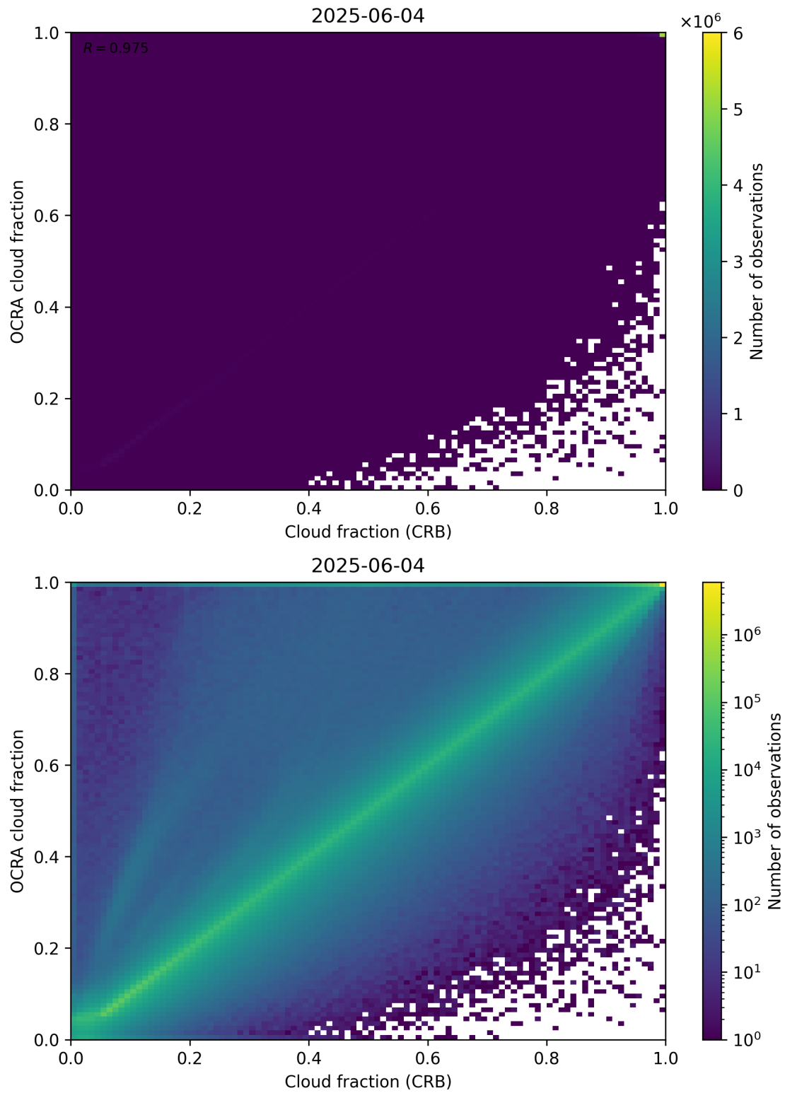
Figure 78: Scatter density plot of “Cloud fraction (CRB)” against “OCRA cloud fraction” for 2025-06-03 to 2025-06-05.
