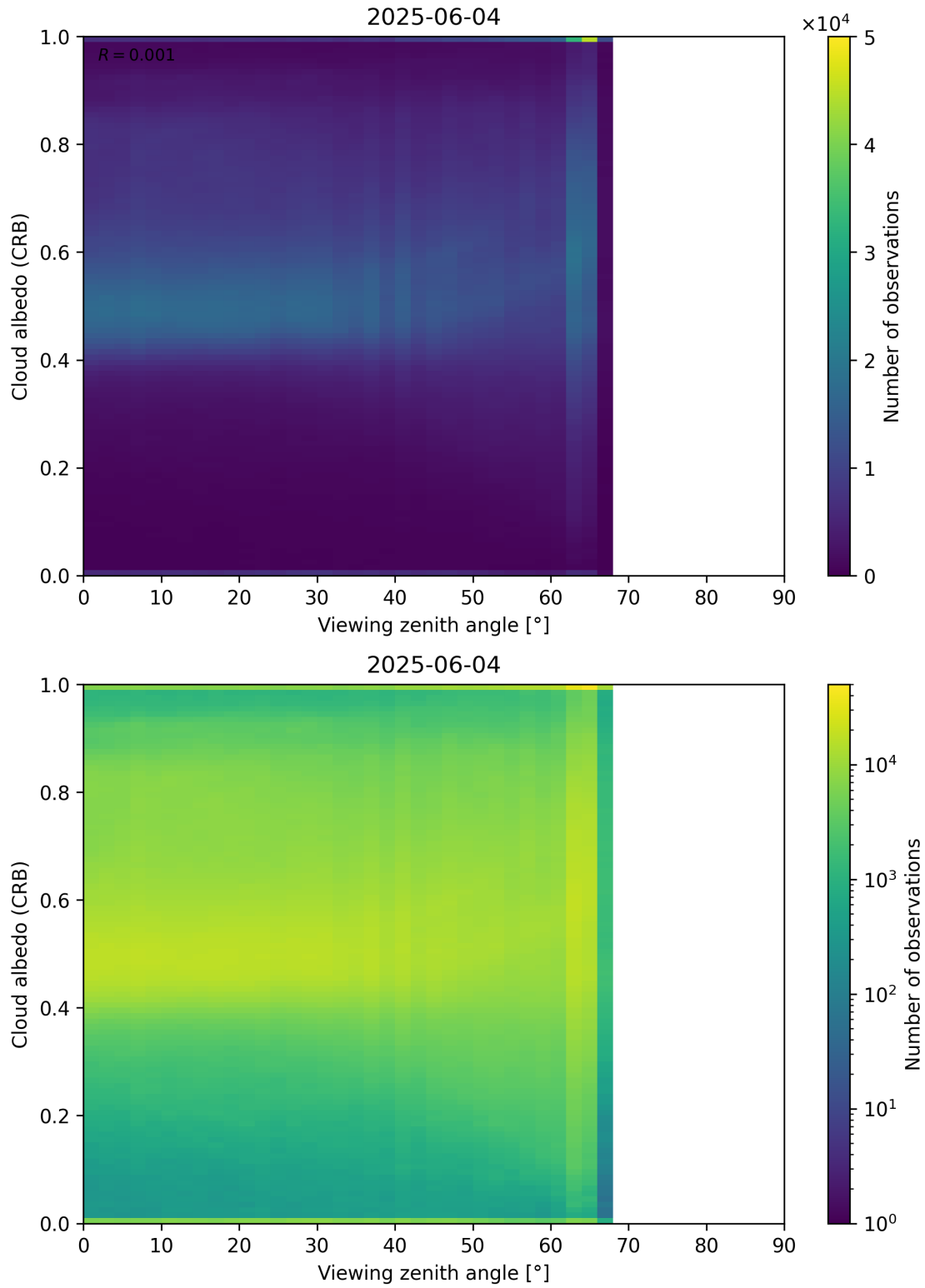
Figure 106: Scatter density plot of “Viewing zenith angle” against “Cloud albedo (CRB)” for 2025-06-03 to 2025-06-05.
