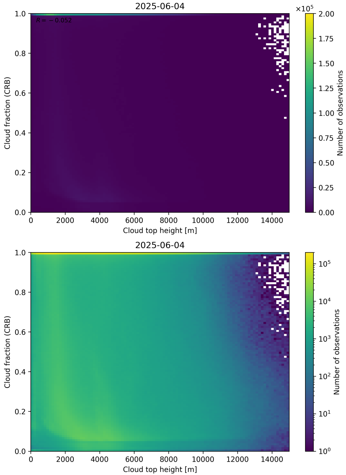
Figure 88: Scatter density plot of “Cloud top height” against “Cloud fraction (CRB)” for 2025-06-03 to 2025-06-05.
