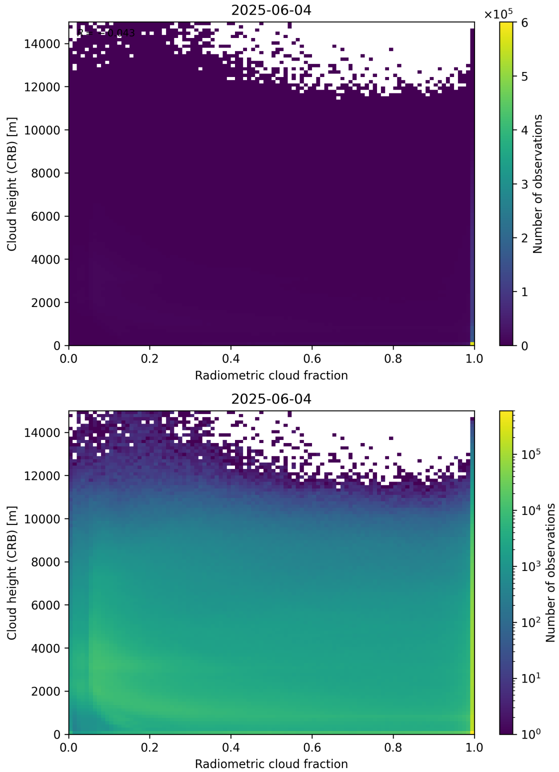
Figure 74: Scatter density plot of “Radiometric cloud fraction” against “Cloud height (CRB)” for 2025-06-03 to 2025-06-05.
