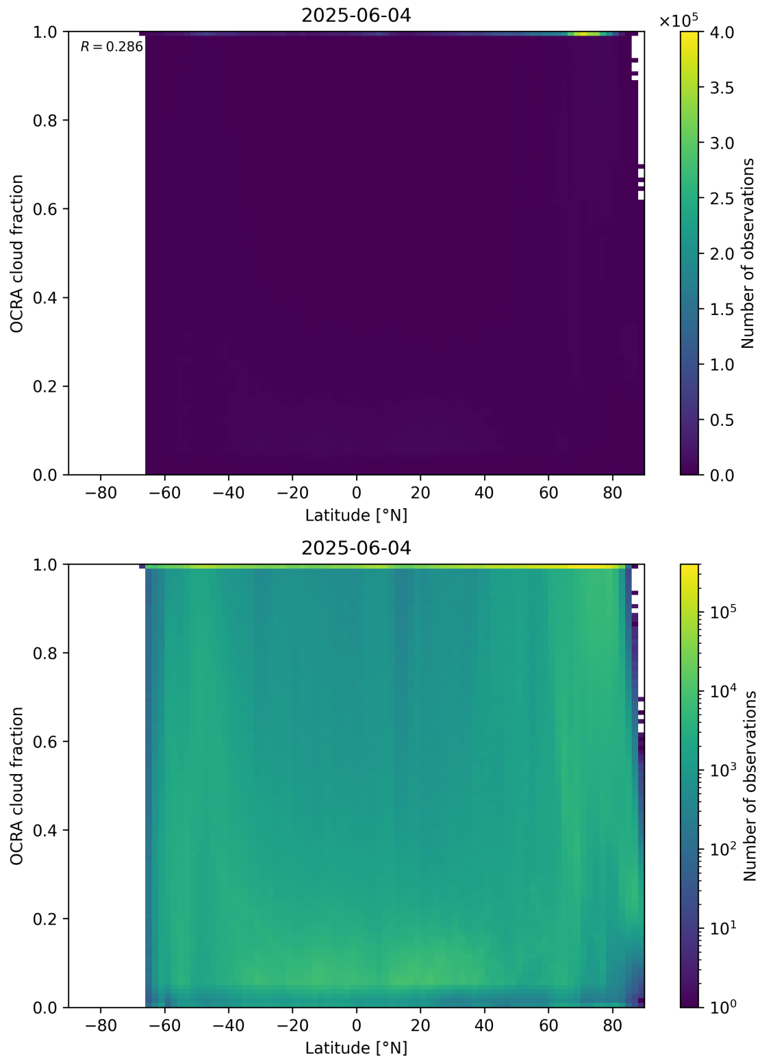
Figure 93: Scatter density plot of “Latitude” against “OCRA cloud fraction” for 2025-06-03 to 2025-06-05.
