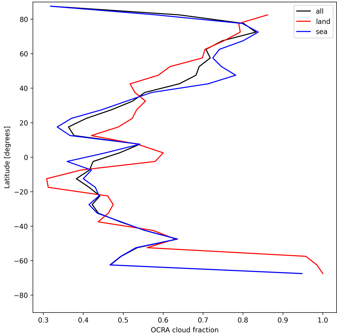
Figure 34: Zonal average of “OCRA cloud fraction” for 2025-06-03 to 2025-06-05.
