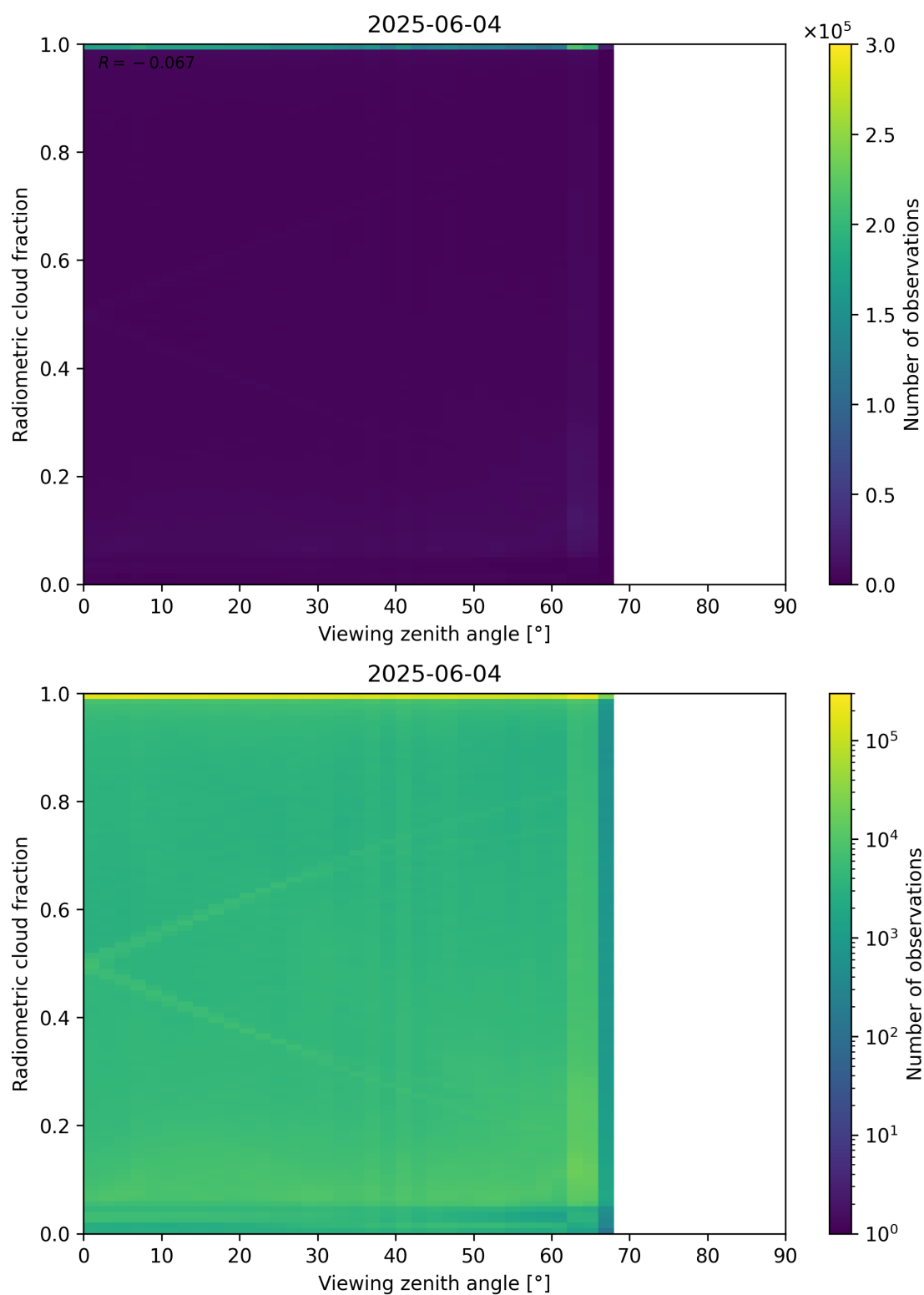
Figure 107: Scatter density plot of “Viewing zenith angle” against “Radiometric cloud fraction” for 2025-06-03 to 2025-06-05.
