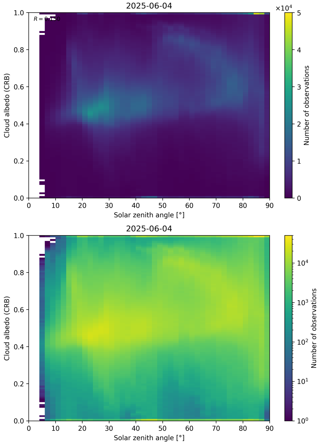
Figure 98: Scatter density plot of “Solar zenith angle” against “Cloud albedo (CRB)” for 2025-06-03 to 2025-06-05.
