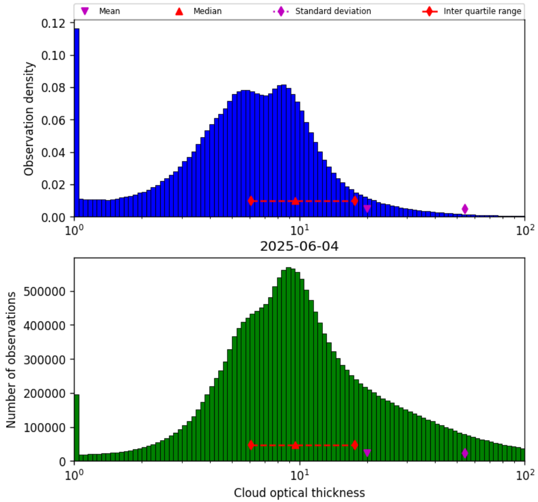
Figure 41: Histogram of “Cloud optical thickness” for 2025-06-03 to 2025-06-05
