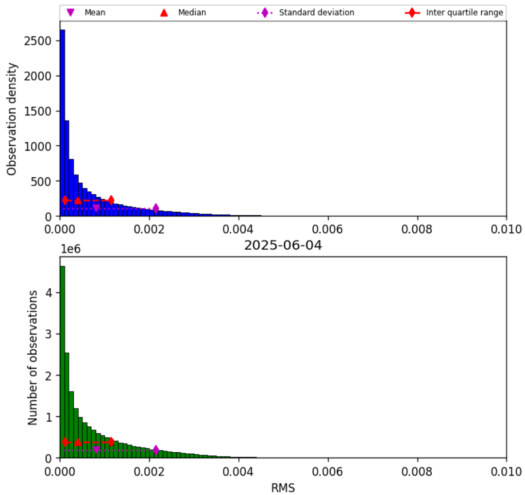
Figure 47: Histogram of “RMS” for 2025-06-03 to 2025-06-05
