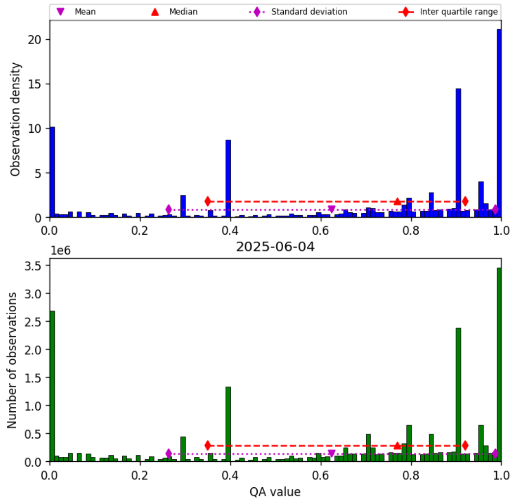
Figure 38: Histogram of “QA value” for 2025-06-03 to 2025-06-05
