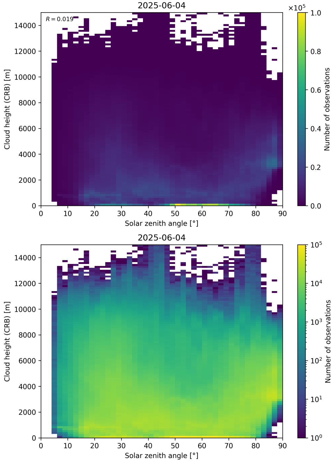
Figure 102: Scatter density plot of “Solar zenith angle” against “Cloud height (CRB)” for 2025-06-03 to 2025-06-05.
