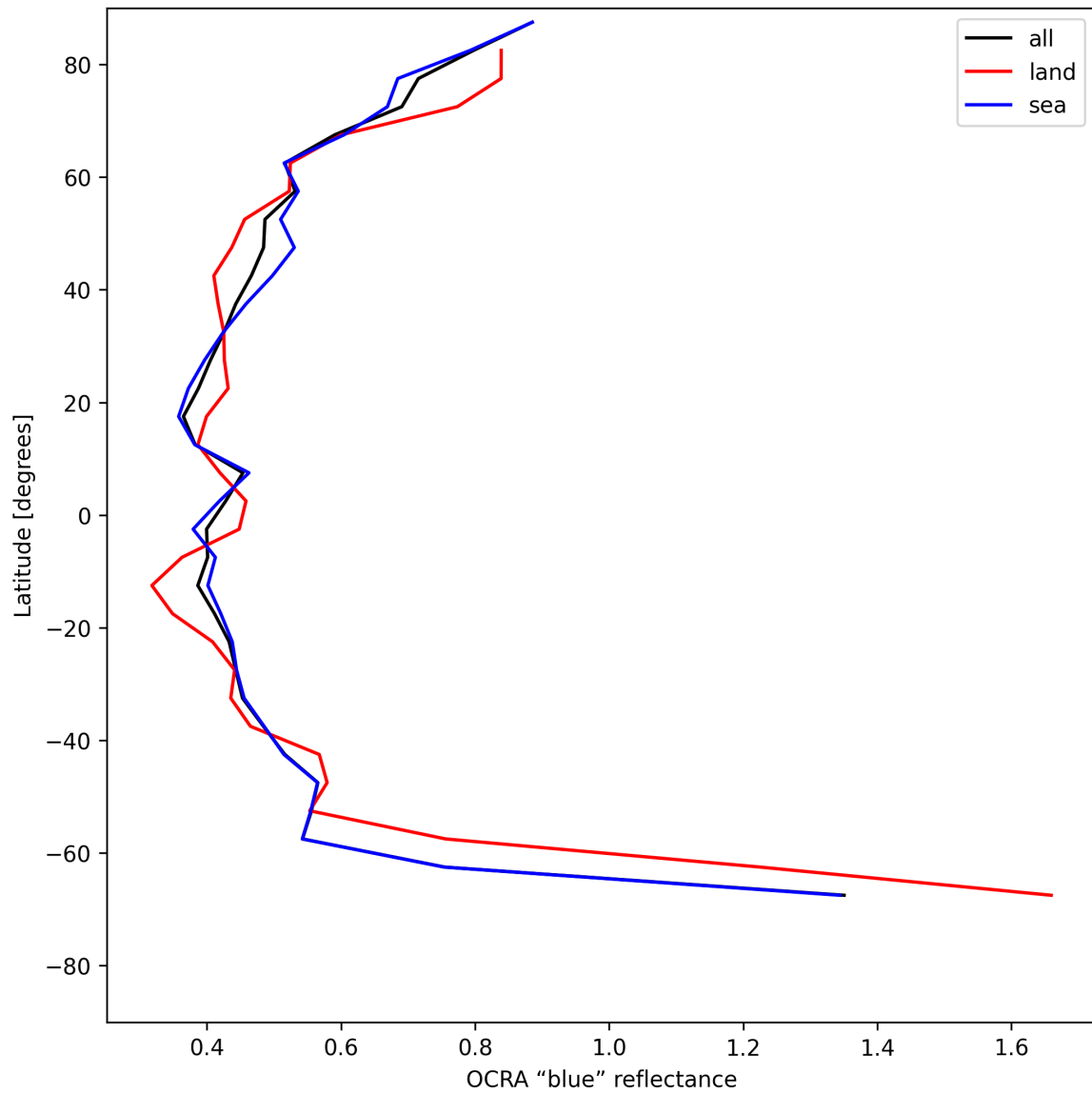
Figure 35: Zonal average of “OCRA “blue” reflectance” for 2025-06-03 to 2025-06-05.
