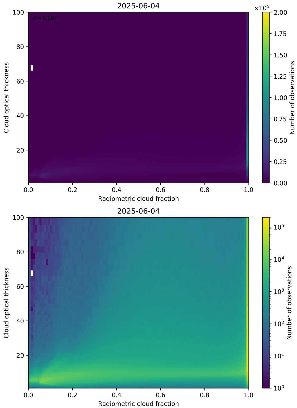
Figure 75: Scatter density plot of “Radiometric cloud fraction” against “Cloud optical thickness” for 2025-06-03 to 2025-06-05.
