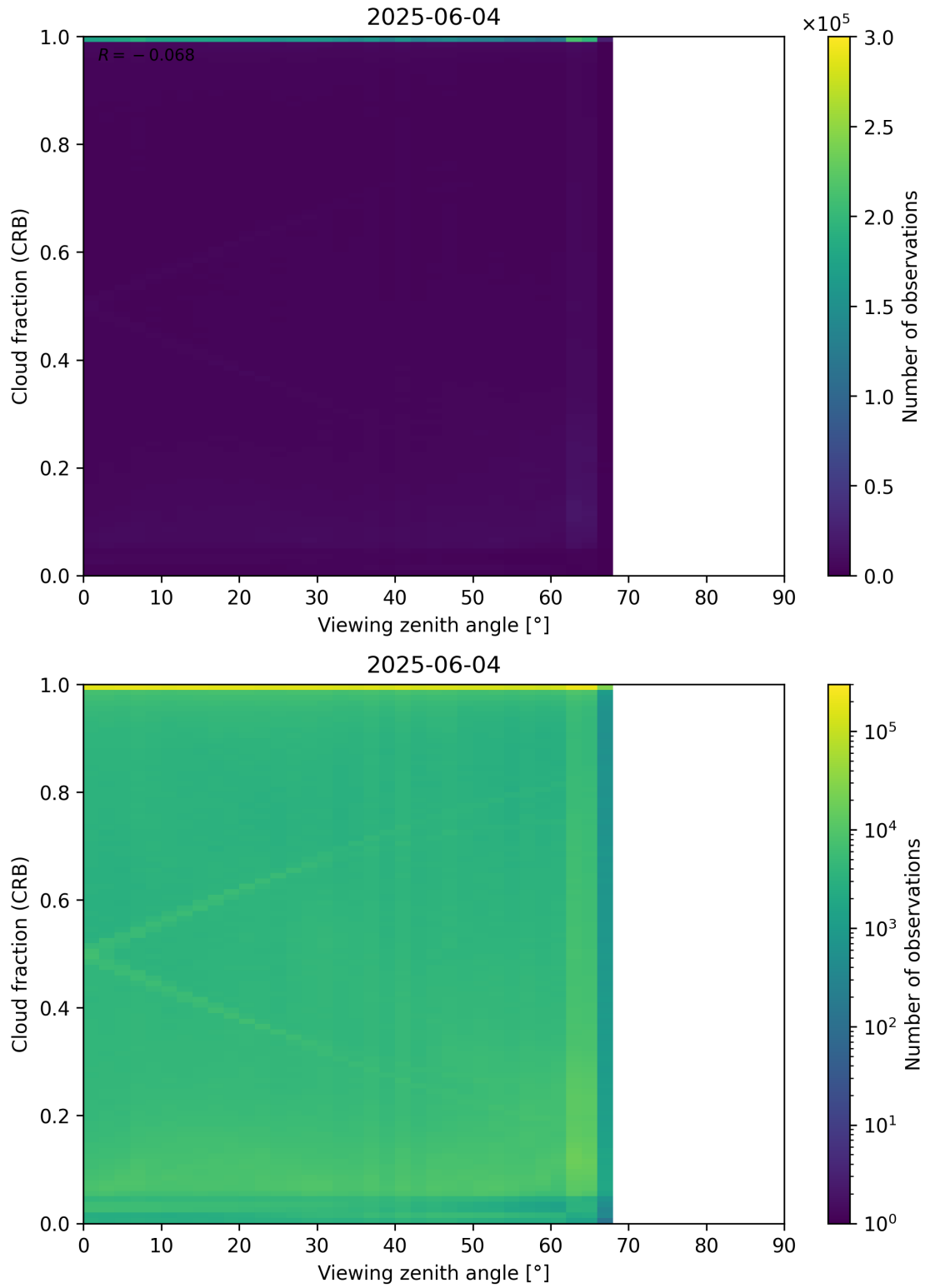
Figure 109: Scatter density plot of “Viewing zenith angle” against “Cloud fraction (CRB)” for 2025-06-03 to 2025-06-05.
