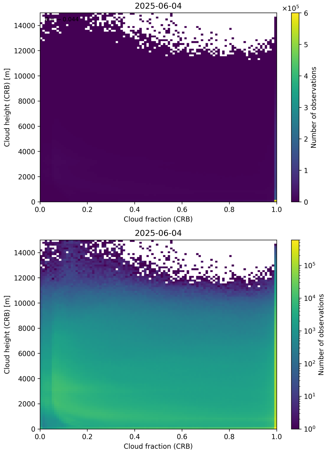
Figure 79: Scatter density plot of “Cloud fraction (CRB)” against “Cloud height (CRB)” for 2025-06-03 to 2025-06-05.
