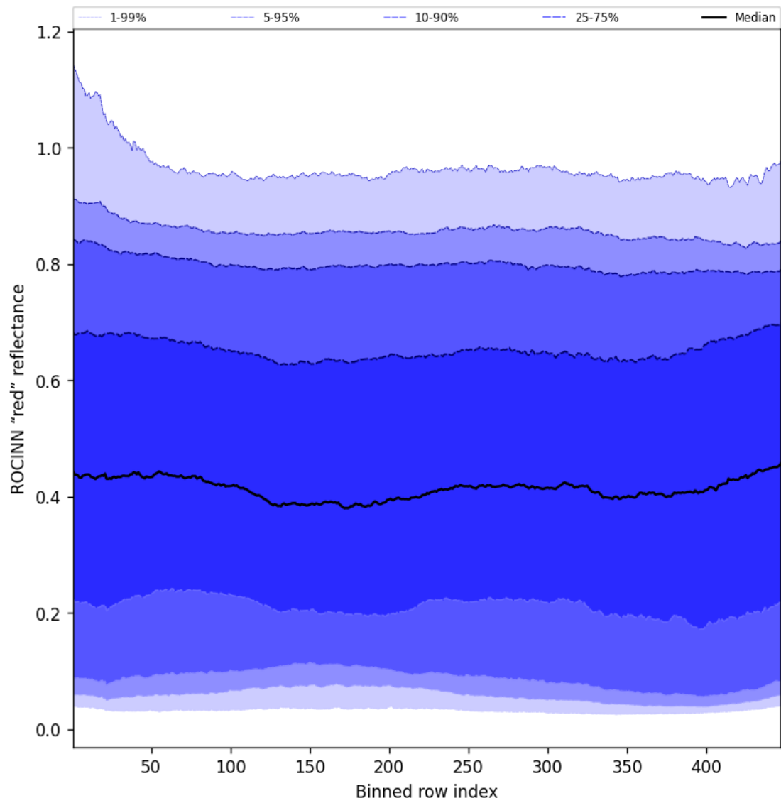
Figure 69: Along track statistics of “ROCINN “red” reflectance” for 2025-06-03 to 2025-06-05
