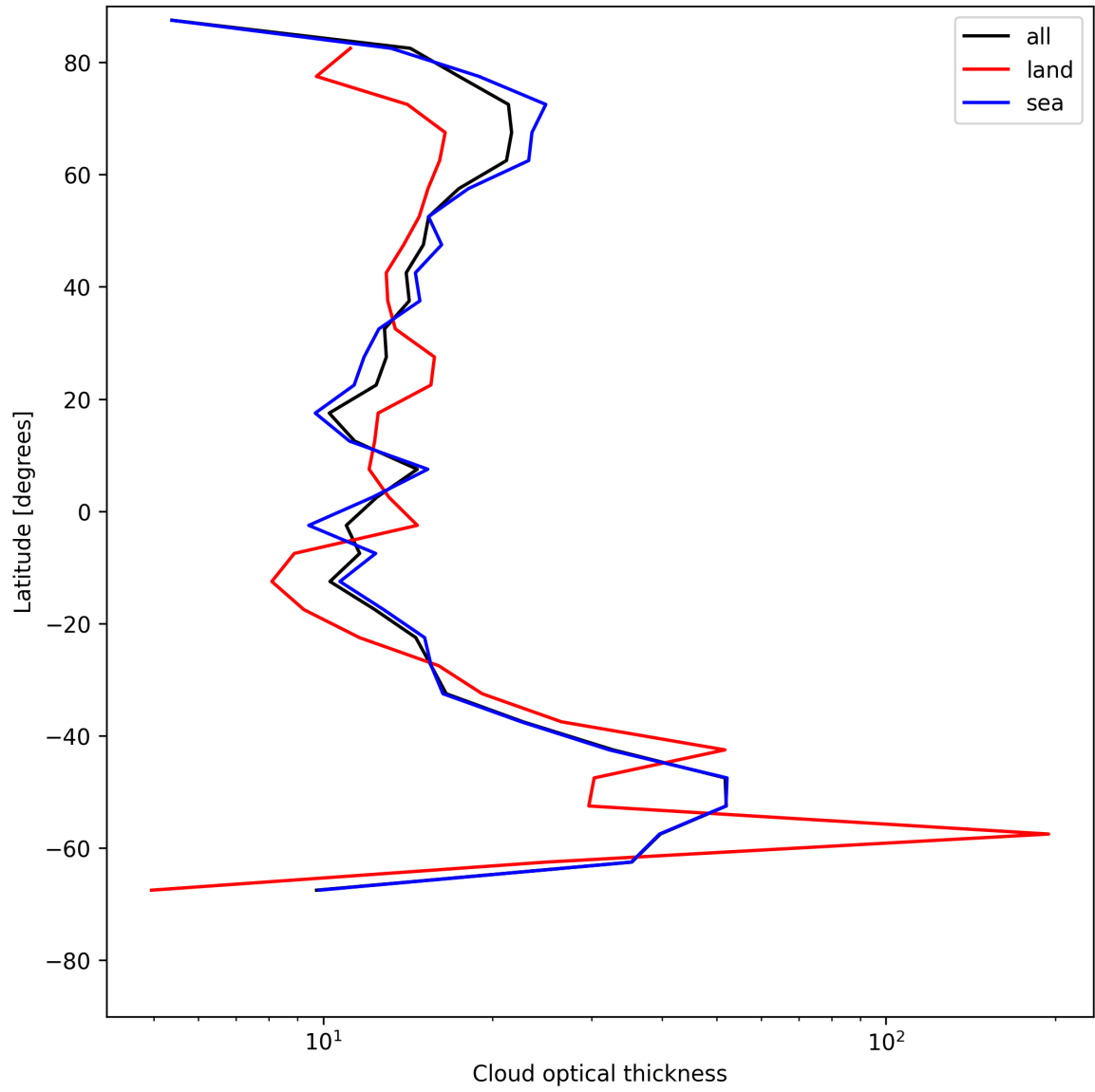
Figure 25: Zonal average of “Cloud optical thickness” for 2025-06-03 to 2025-06-05.
