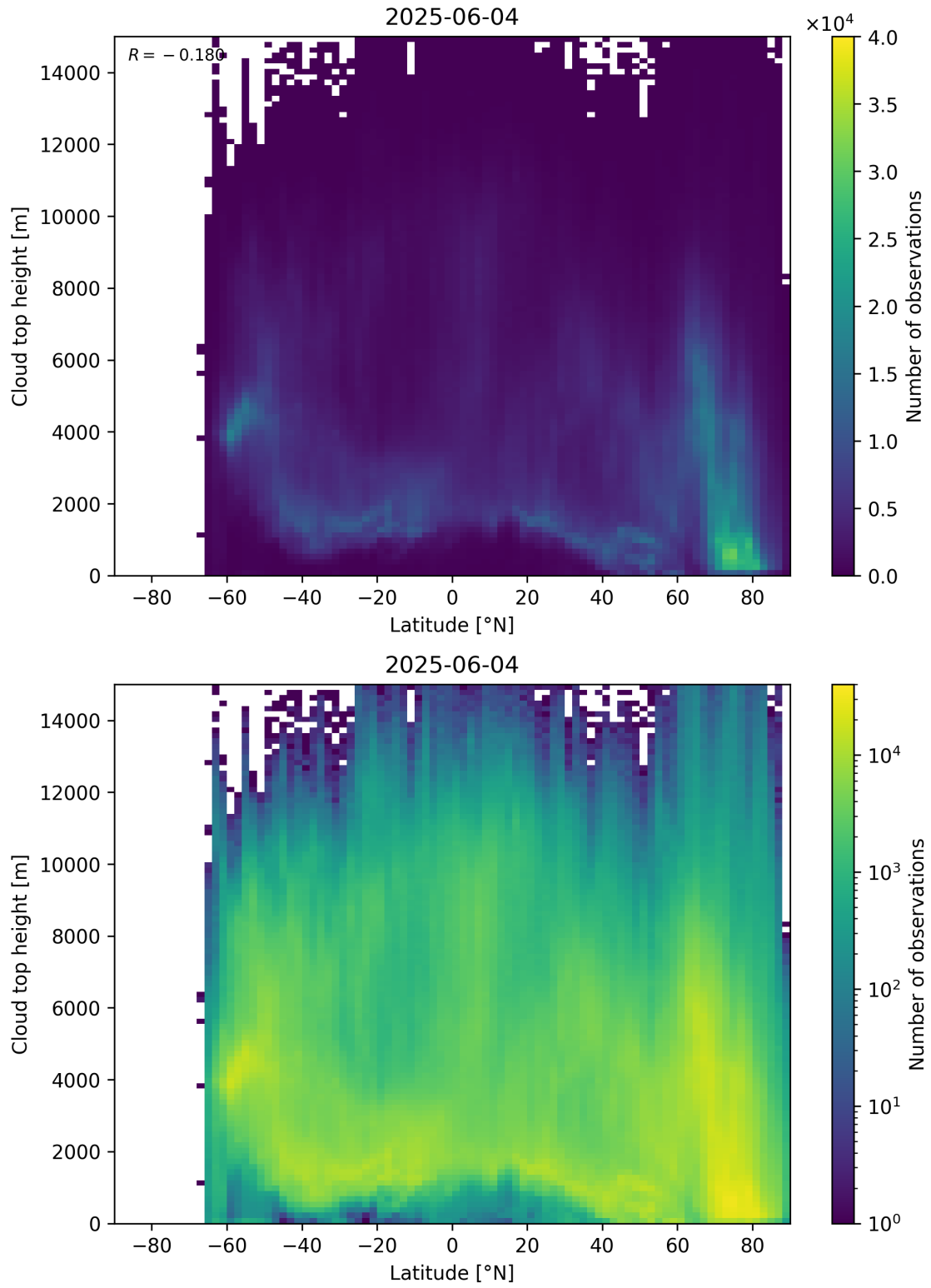
Figure 97: Scatter density plot of “Latitude” against “Cloud top height” for 2025-06-03 to 2025-06-05.
