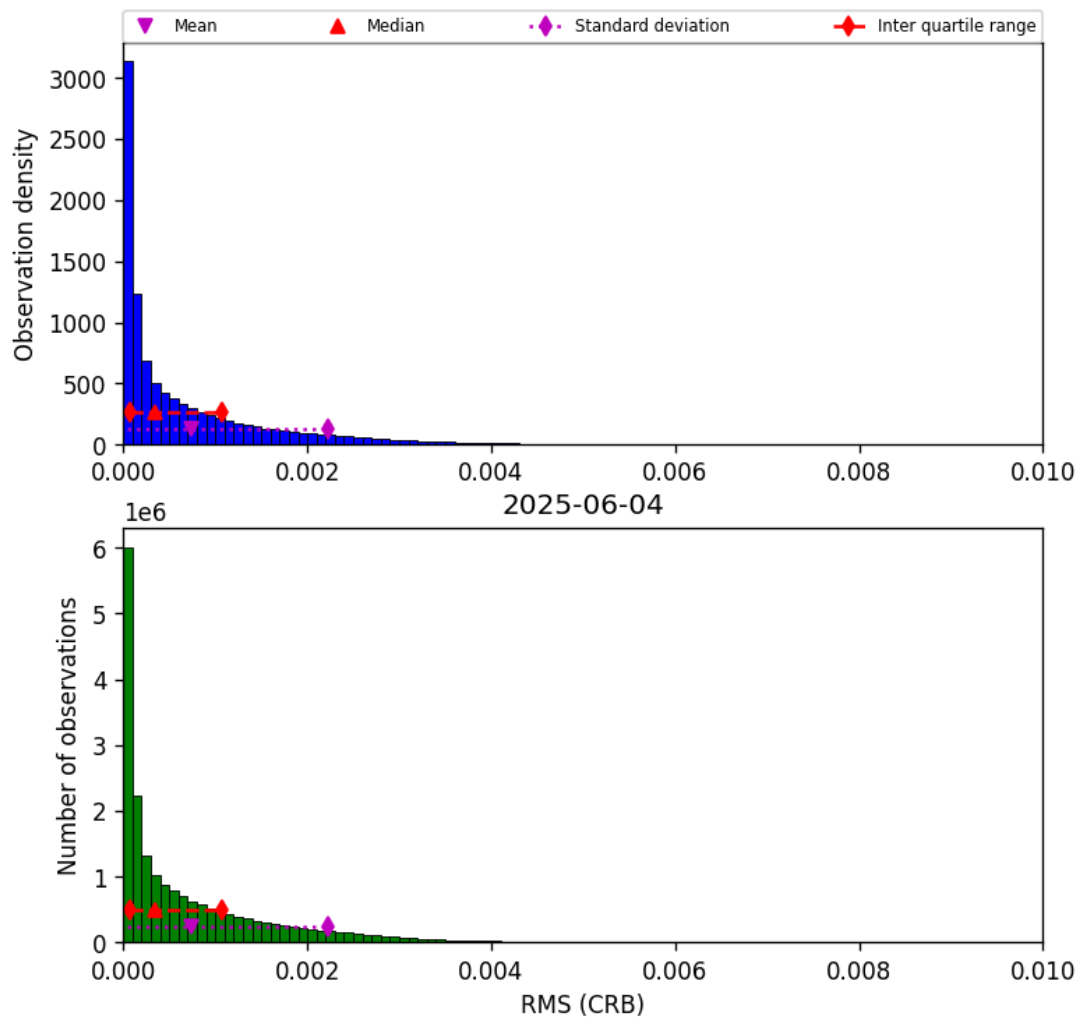
Figure 48: Histogram of “RMS (CRB)” for 2025-06-03 to 2025-06-05
