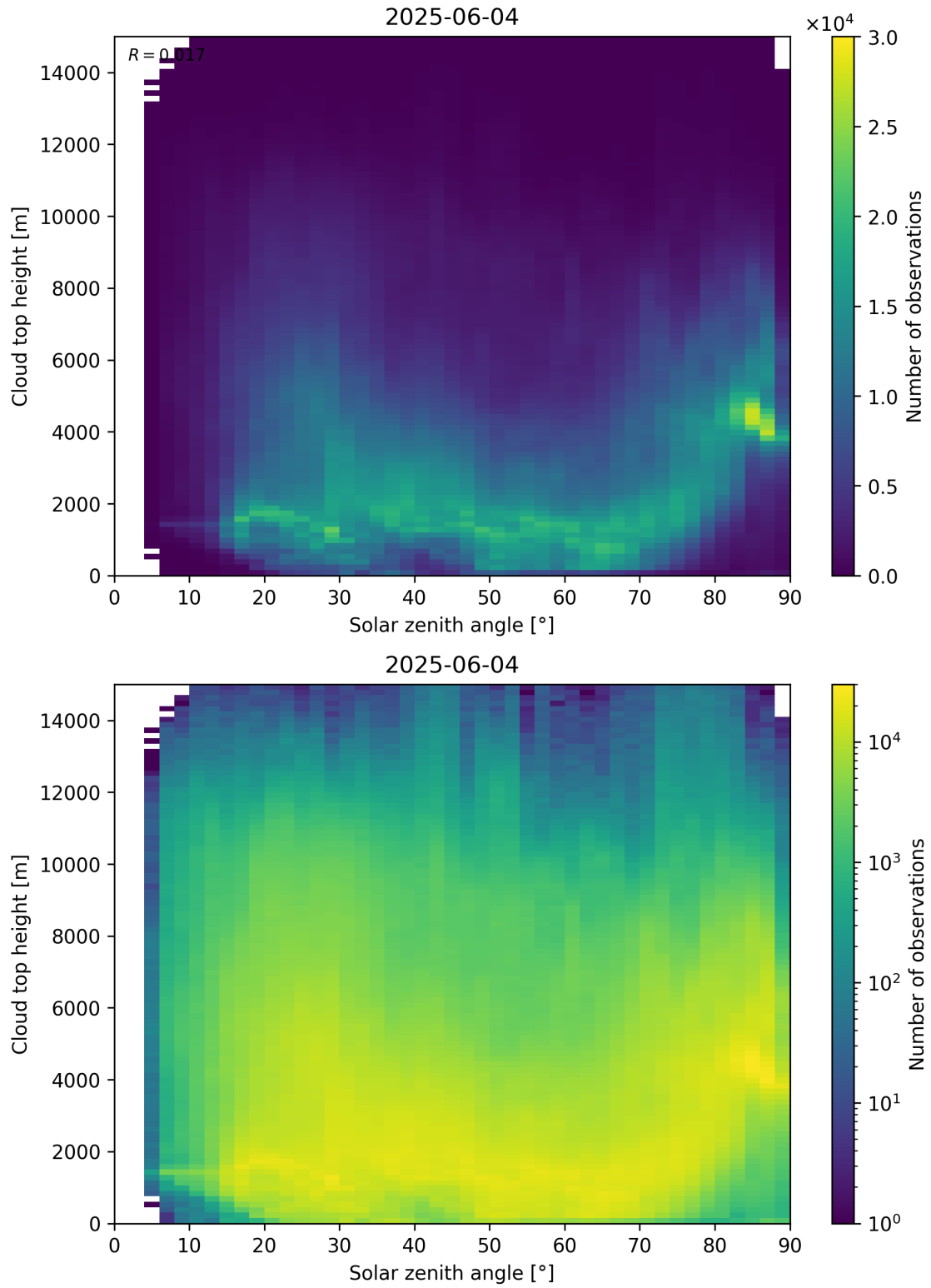
Figure 104: Scatter density plot of “Solar zenith angle” against “Cloud top height” for 2025-06-03 to 2025-06-05.
