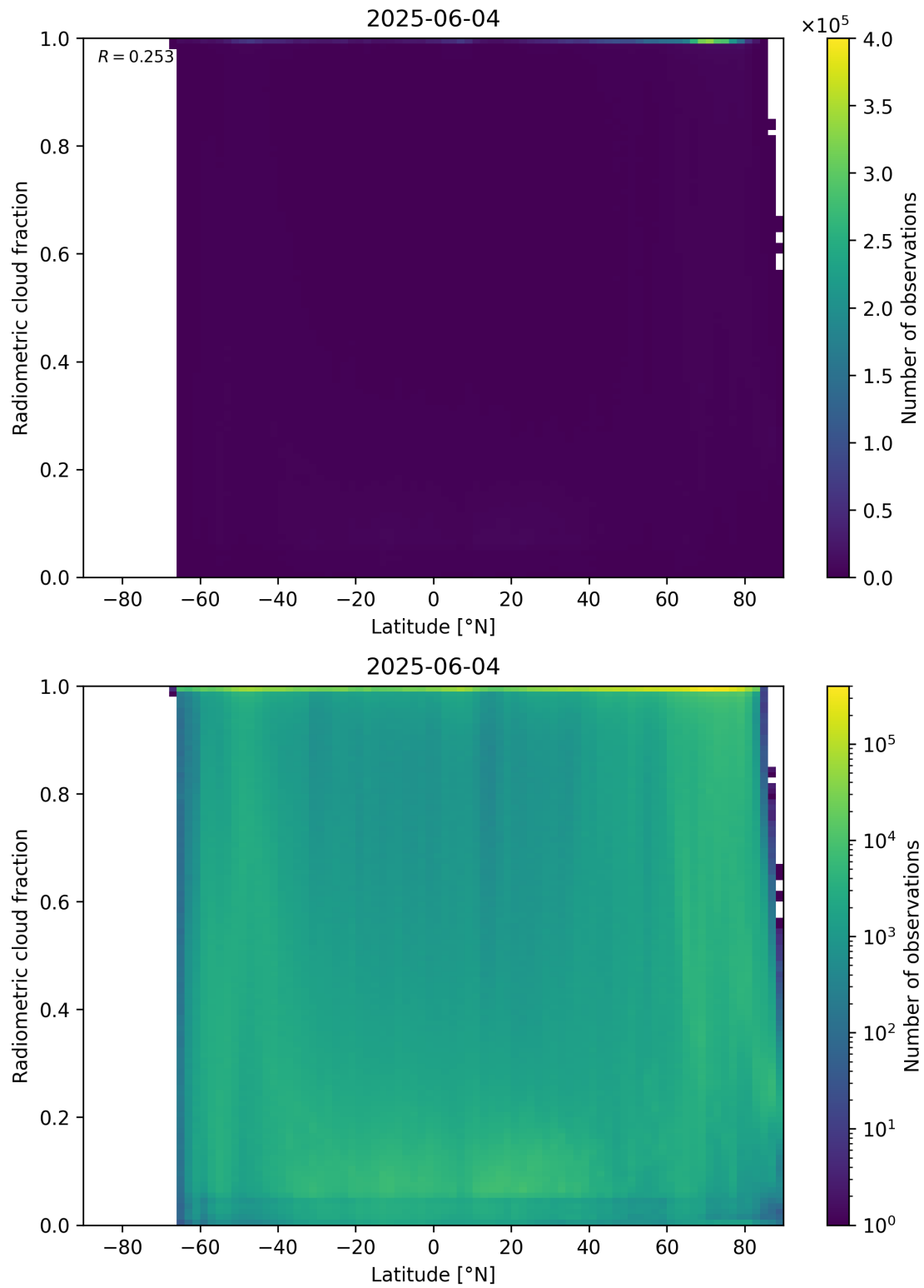
Figure 92: Scatter density plot of “Latitude” against “Radiometric cloud fraction” for 2025-06-03 to 2025-06-05.
