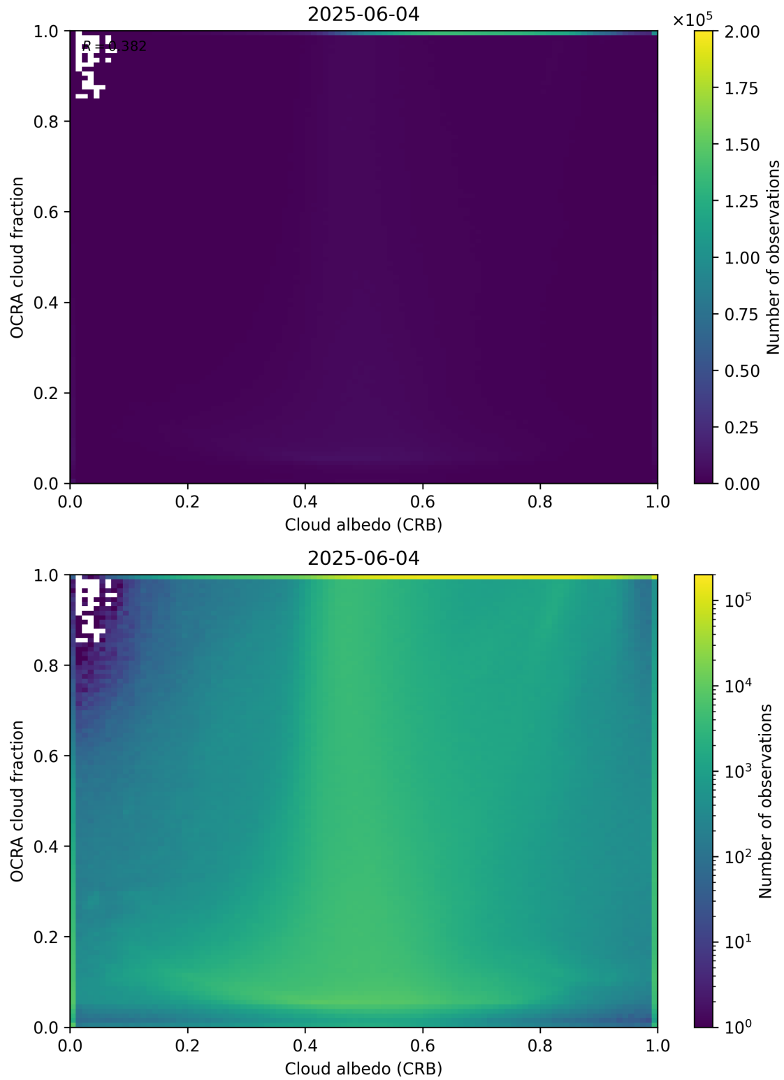
Figure 70: Scatter density plot of “Cloud albedo (CRB)” against “OCRA cloud fraction” for 2025-06-03 to 2025-06-05.
