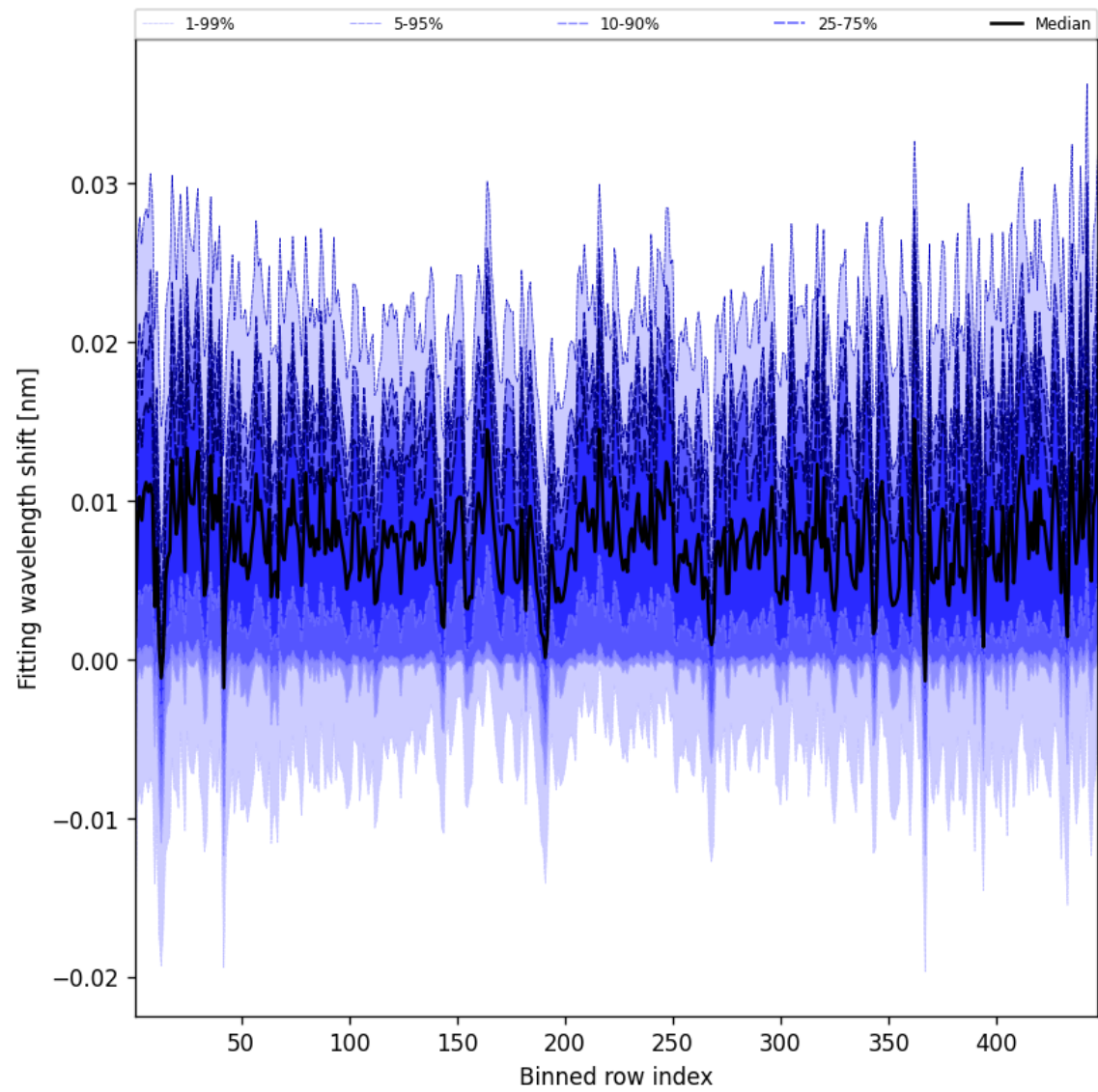
Figure 65: Along track statistics of “Fitting wavelength shift” for 2025-06-03 to 2025-06-05
