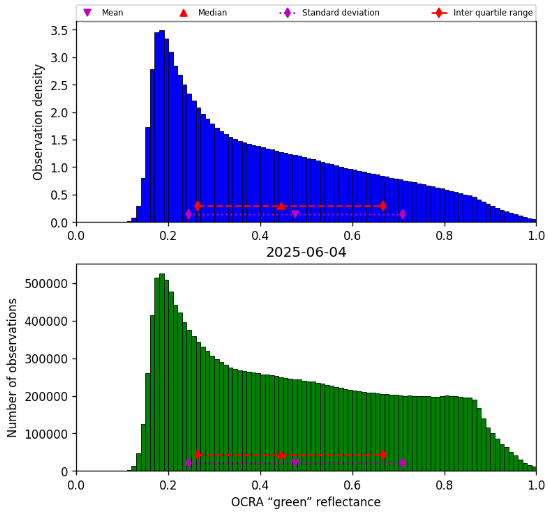
Figure 52: Histogram of “OCRA “green” reflectance” for 2025-06-03 to 2025-06-05
