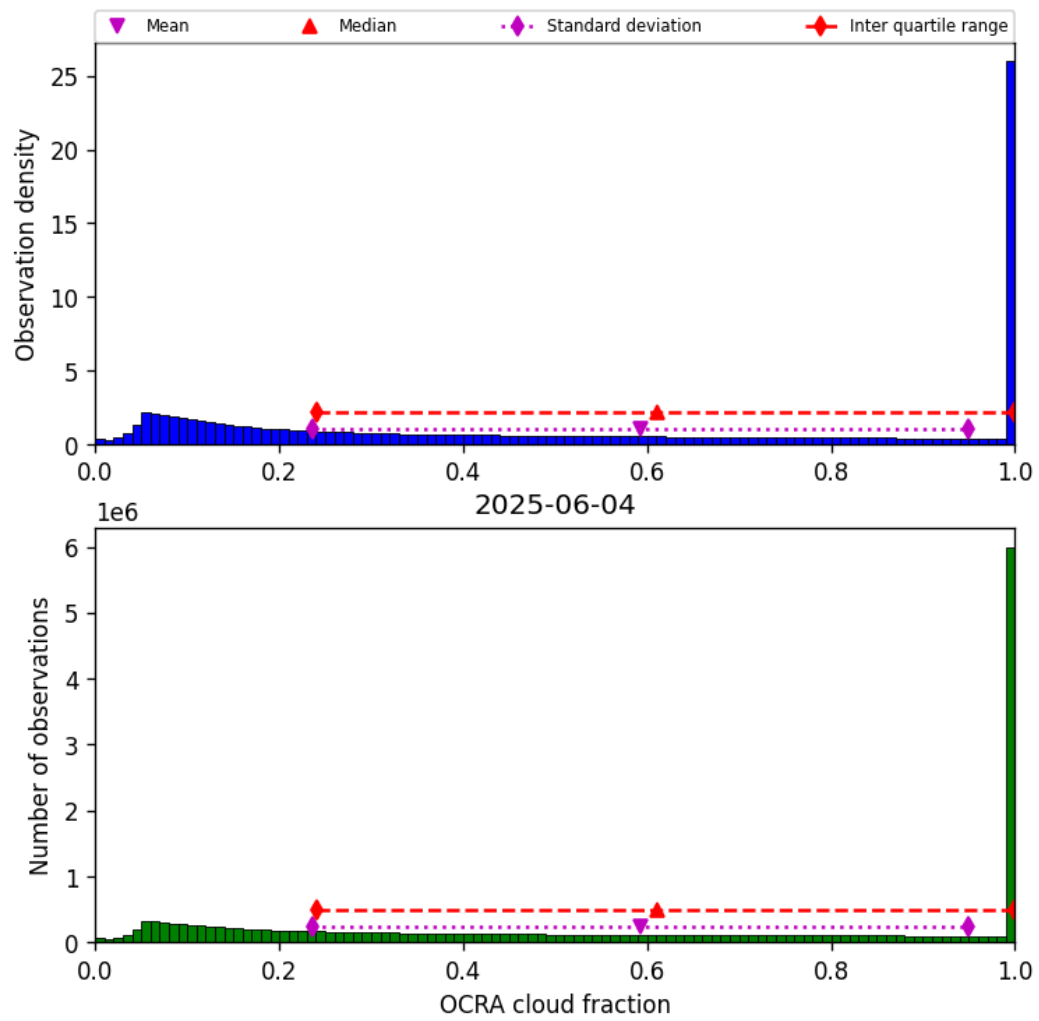
Figure 50: Histogram of “OCRA cloud fraction” for 2025-06-03 to 2025-06-05
