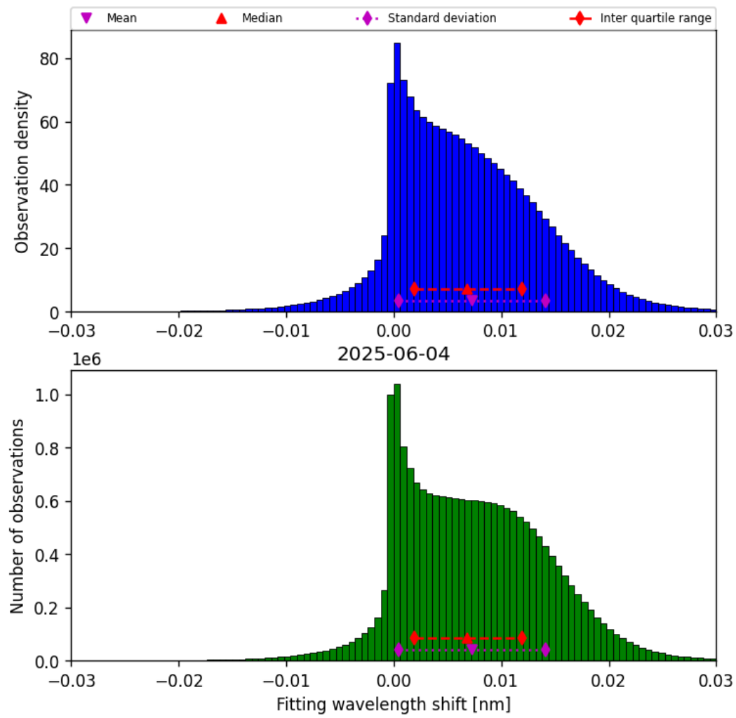
Figure 49: Histogram of “Fitting wavelength shift” for 2025-06-03 to 2025-06-05
