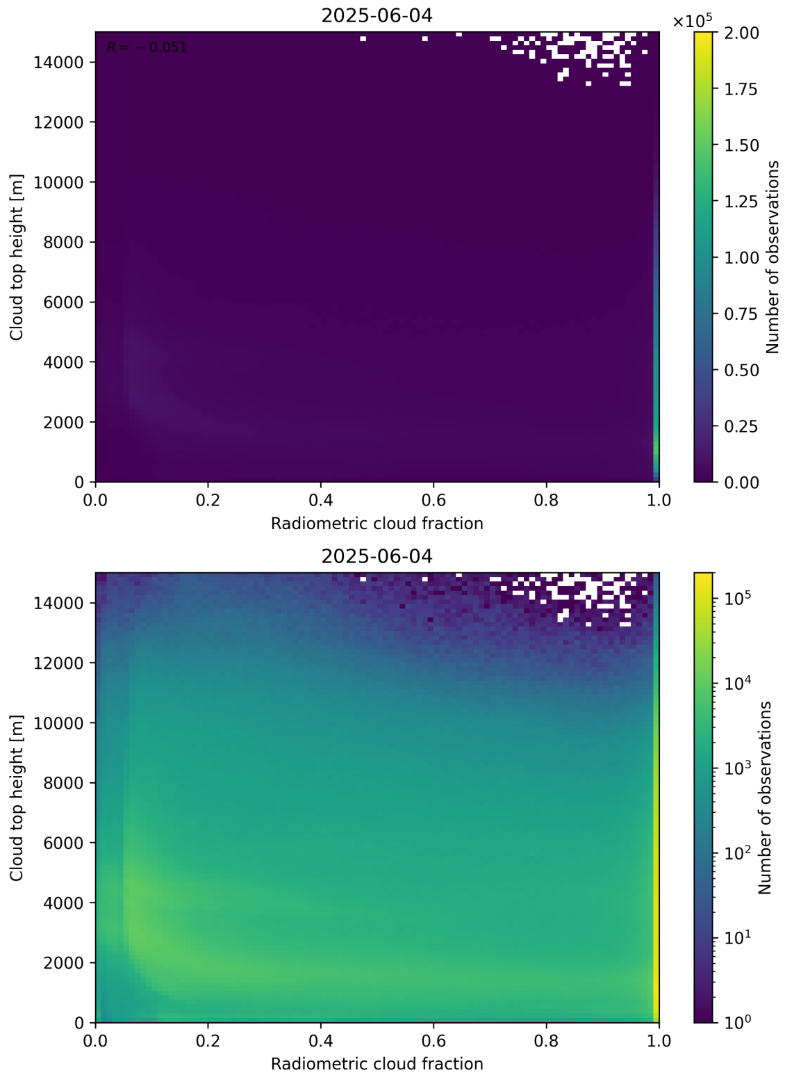
Figure 76: Scatter density plot of “Radiometric cloud fraction” against “Cloud top height” for 2025-06-03 to 2025-06-05.
