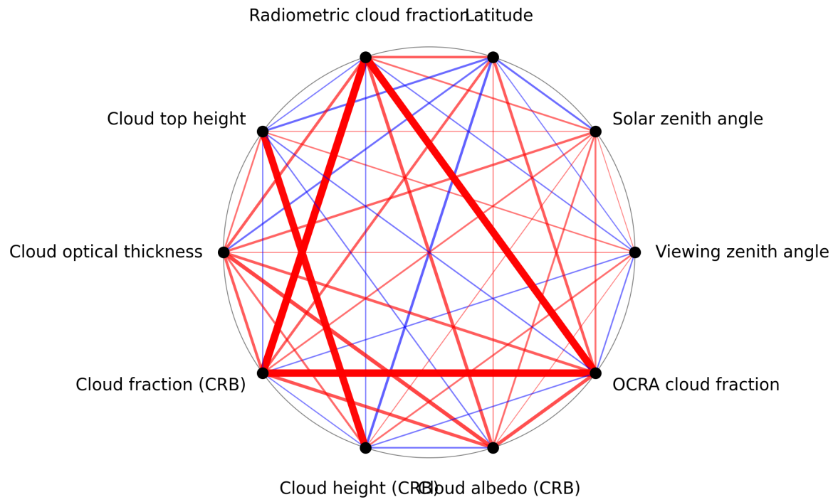
Figure 1: Map of correlation graph for 2025-06-03 to 2025-06-05.
