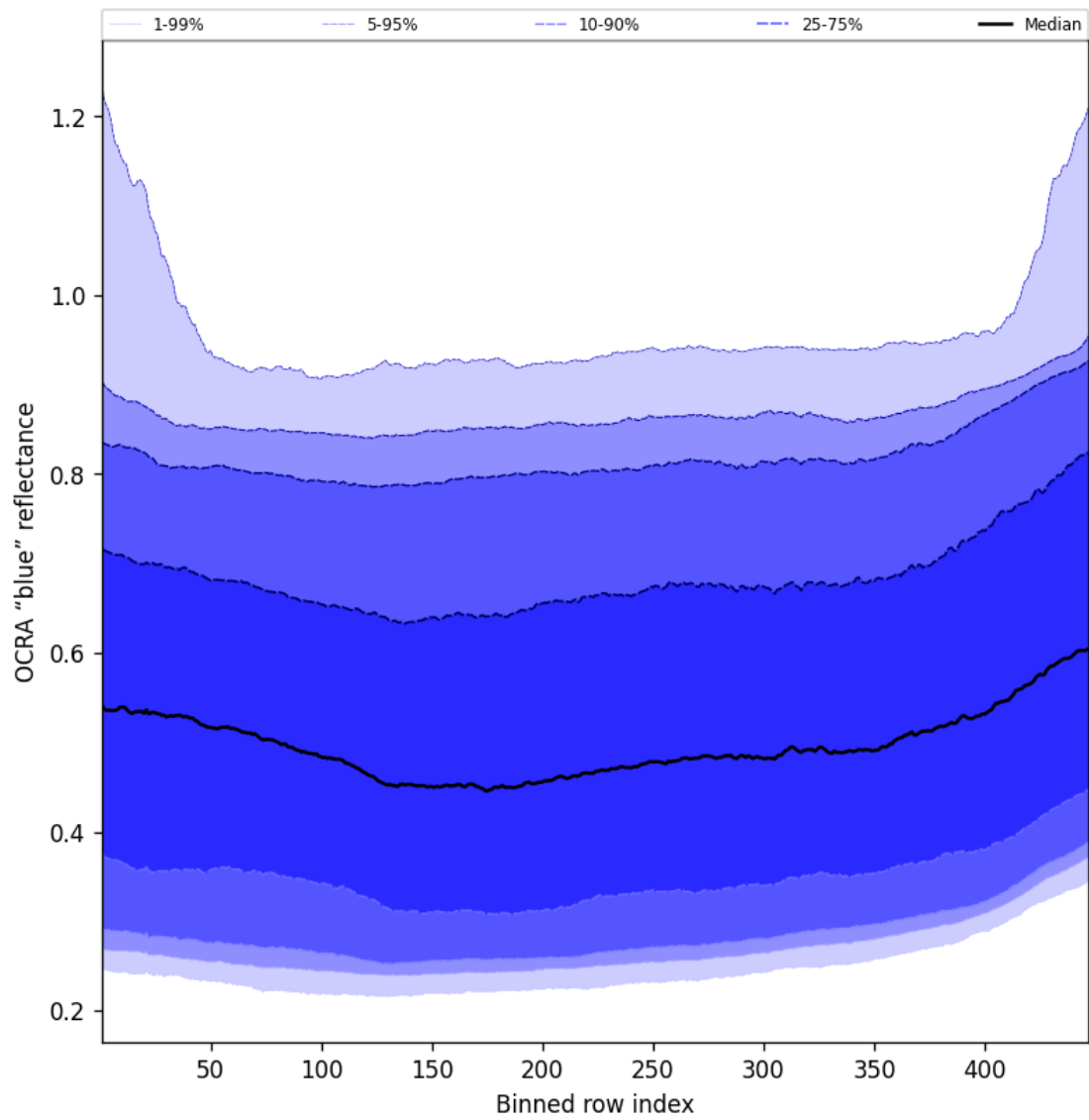
Figure 67: Along track statistics of “OCRA “blue” reflectance” for 2025-06-03 to 2025-06-05
