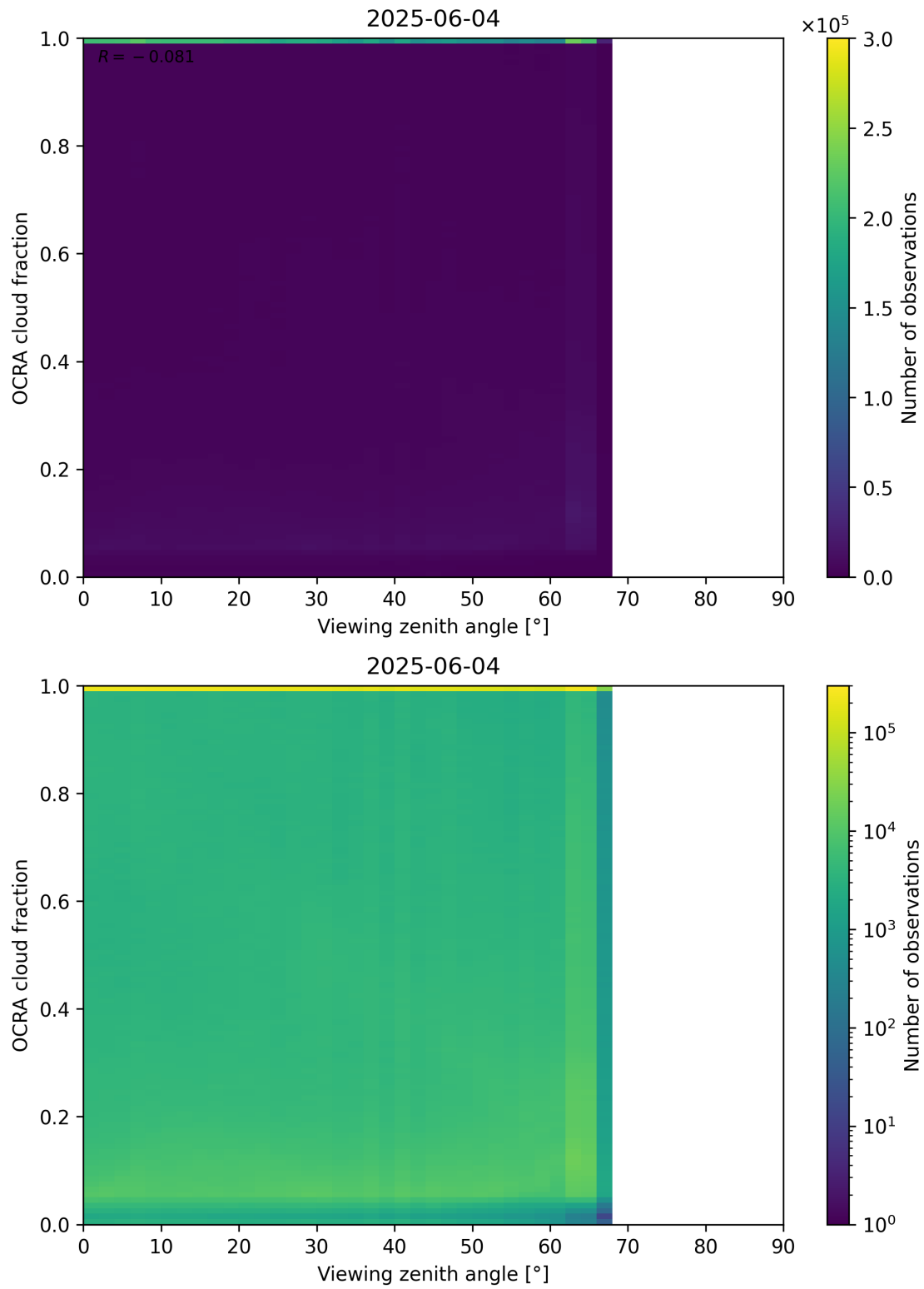
Figure 108: Scatter density plot of “Viewing zenith angle” against “OCRA cloud fraction” for 2025-06-03 to 2025-06-05.
