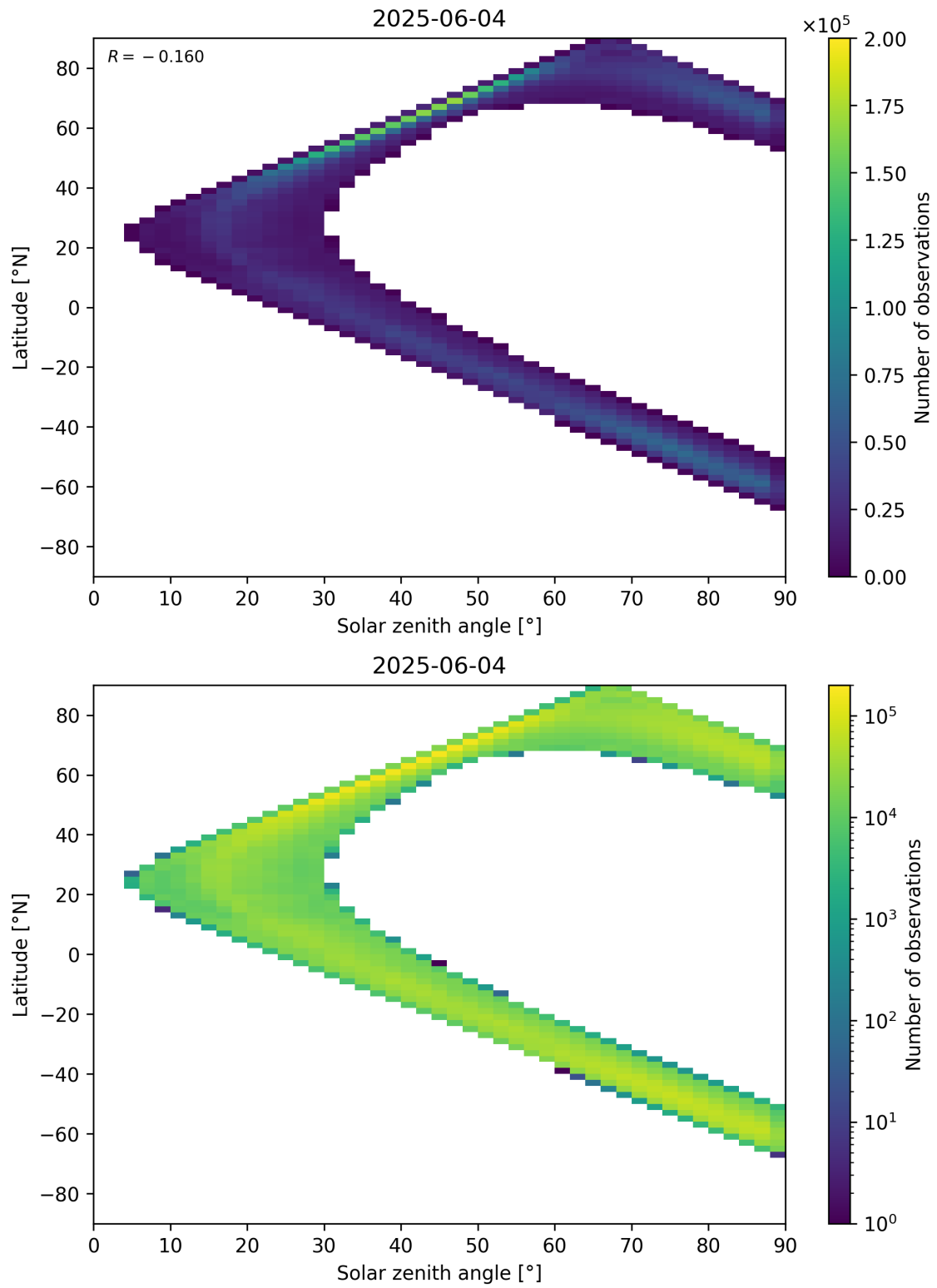
Figure 105: Scatter density plot of “Solar zenith angle” against “Latitude” for 2025-06-03 to 2025-06-05.
