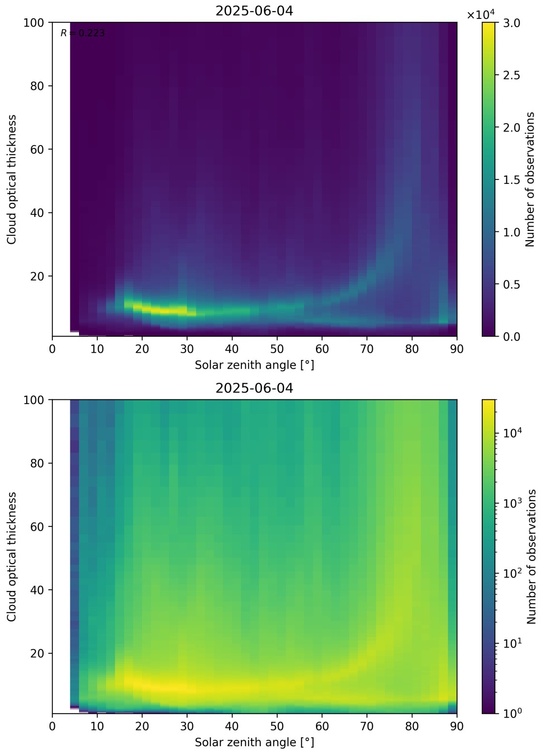
Figure 103: Scatter density plot of “Solar zenith angle” against “Cloud optical thickness” for 2025-06-03 to 2025-06-05.
