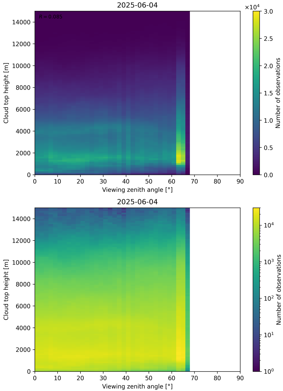
Figure 112: Scatter density plot of “Viewing zenith angle” against “Cloud top height” for 2025-06-03 to 2025-06-05.
