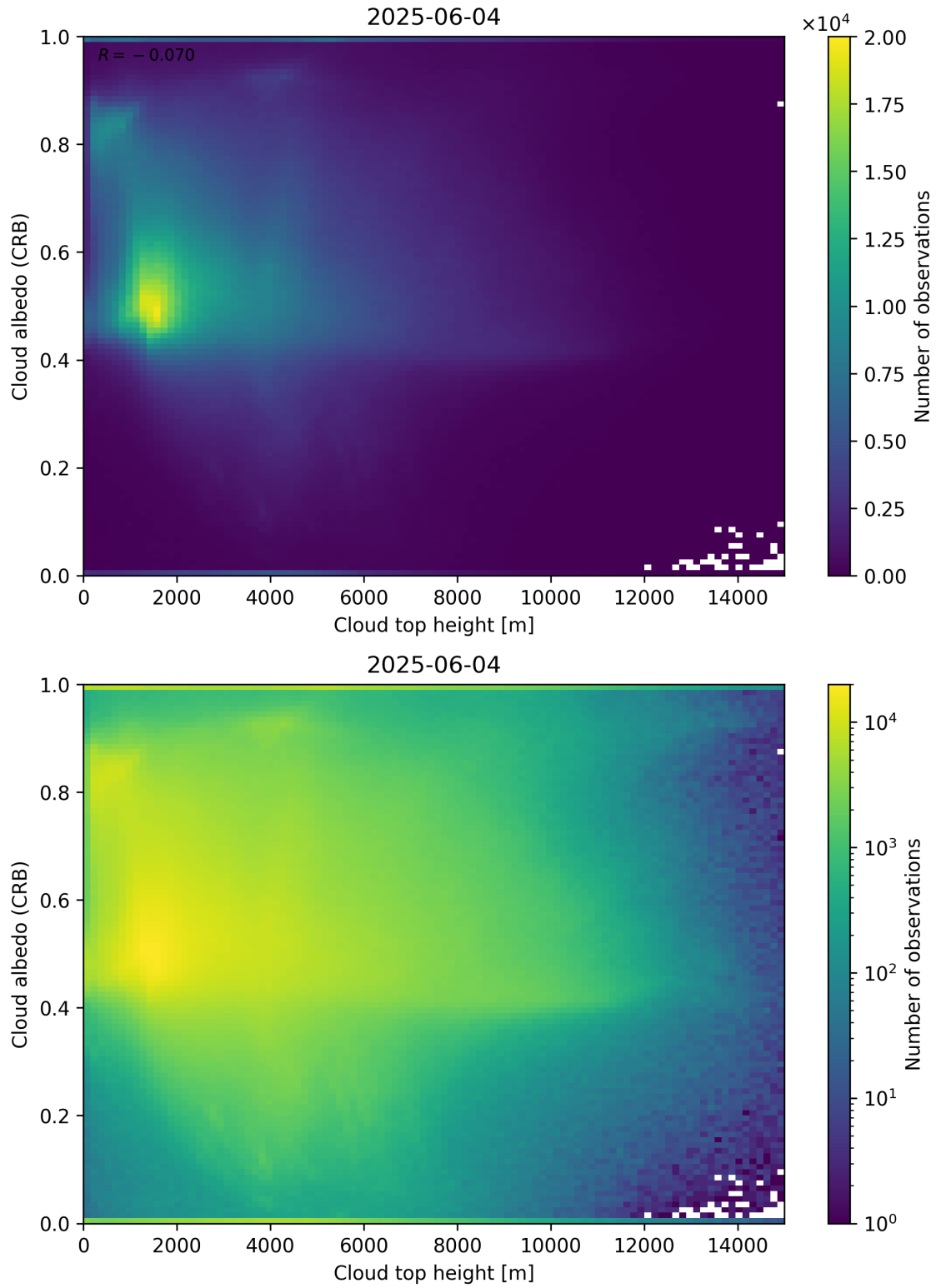
Figure 86: Scatter density plot of “Cloud top height” against “Cloud albedo (CRB)” for 2025-06-03 to 2025-06-05.
