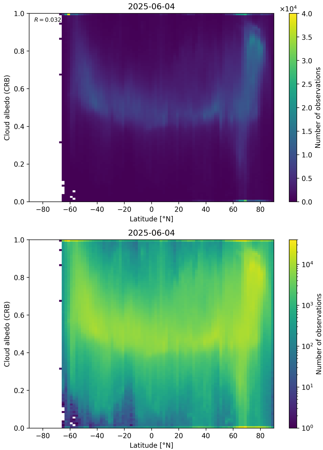
Figure 91: Scatter density plot of “Latitude” against “Cloud albedo (CRB)” for 2025-06-03 to 2025-06-05.
