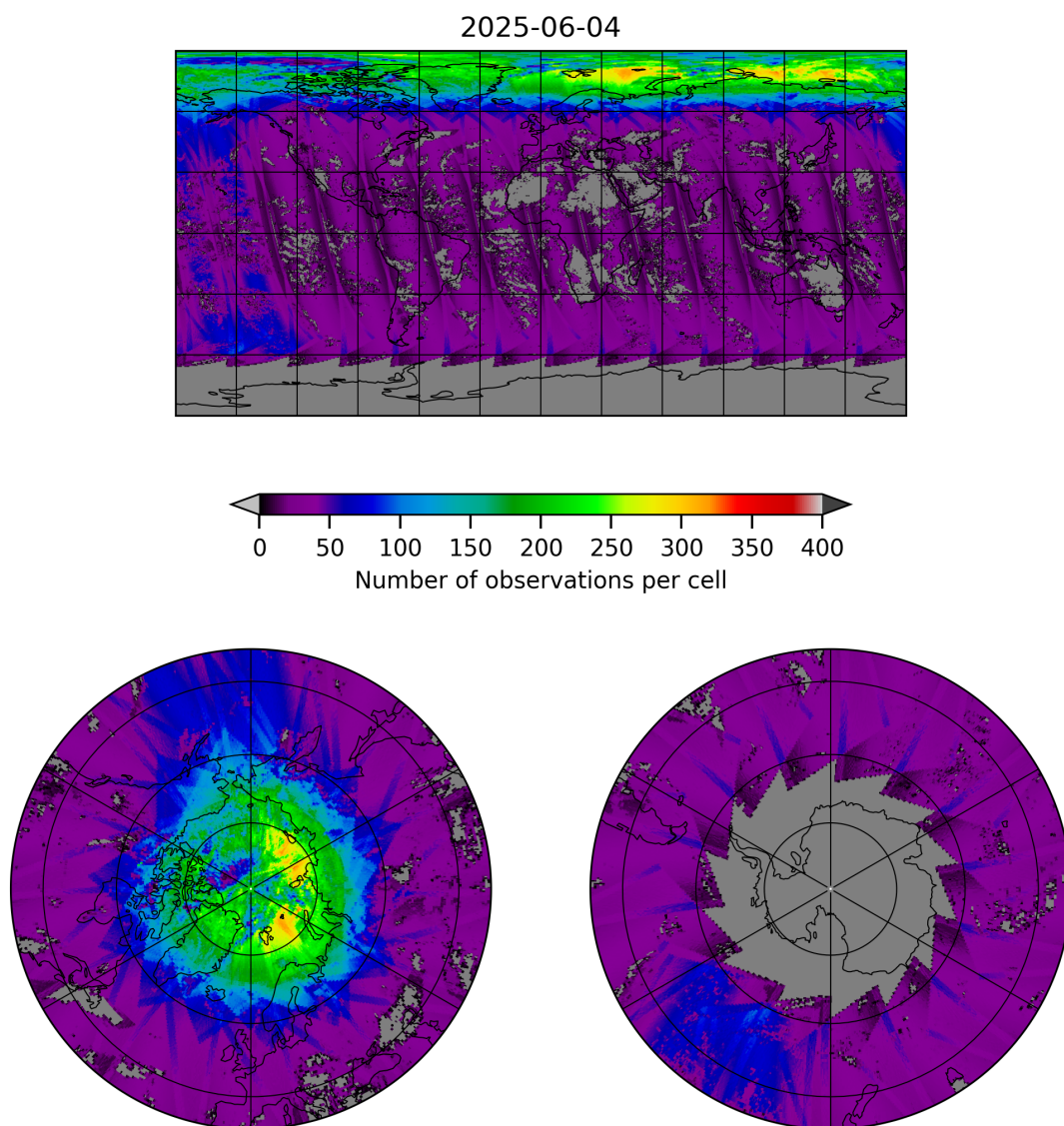
Figure 21: Map of the number of observations for 2025-06-03 to 2025-06-05
