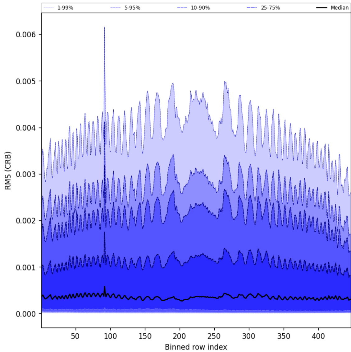
Figure 64: Along track statistics of “RMS (CRB)” for 2025-06-03 to 2025-06-05
