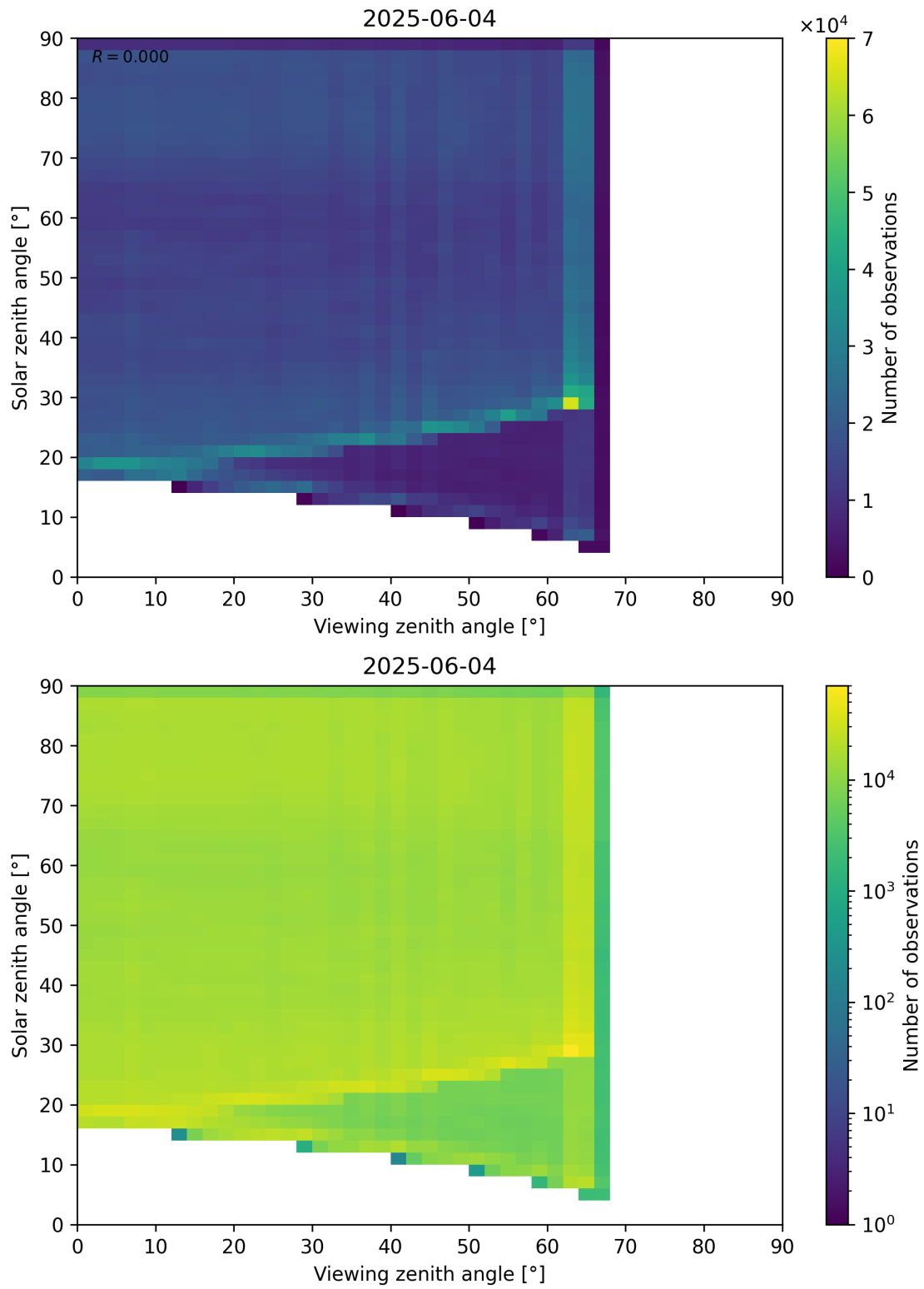
Figure 114: Scatter density plot of “Viewing zenith angle” against “Solar zenith angle” for 2025-06-03 to 2025-06-05.
