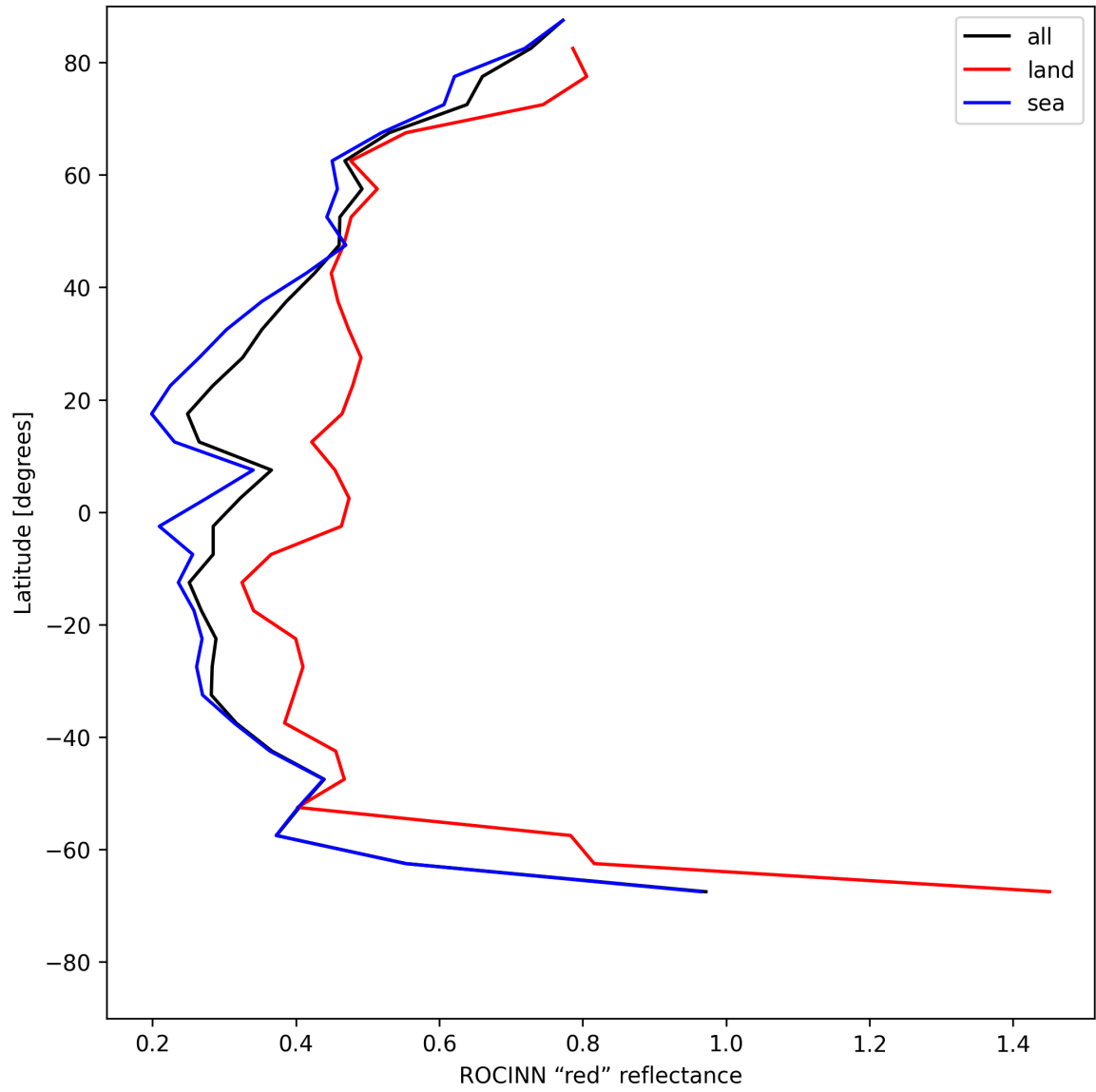
Figure 37: Zonal average of “ROCINN “red” reflectance” for 2025-06-03 to 2025-06-05.
