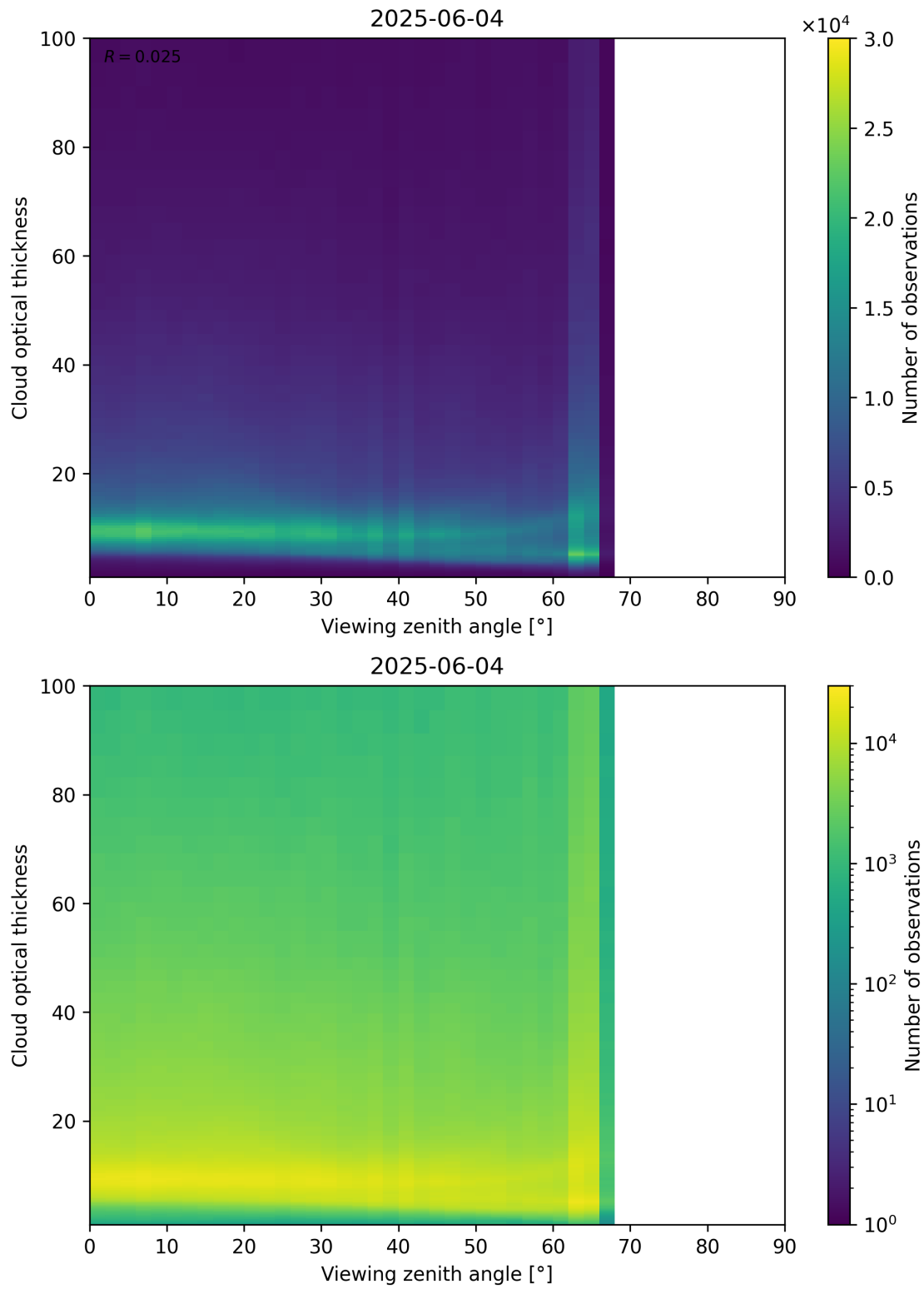
Figure 111: Scatter density plot of “Viewing zenith angle” against “Cloud optical thickness” for 2025-06-03 to 2025-06-05.
