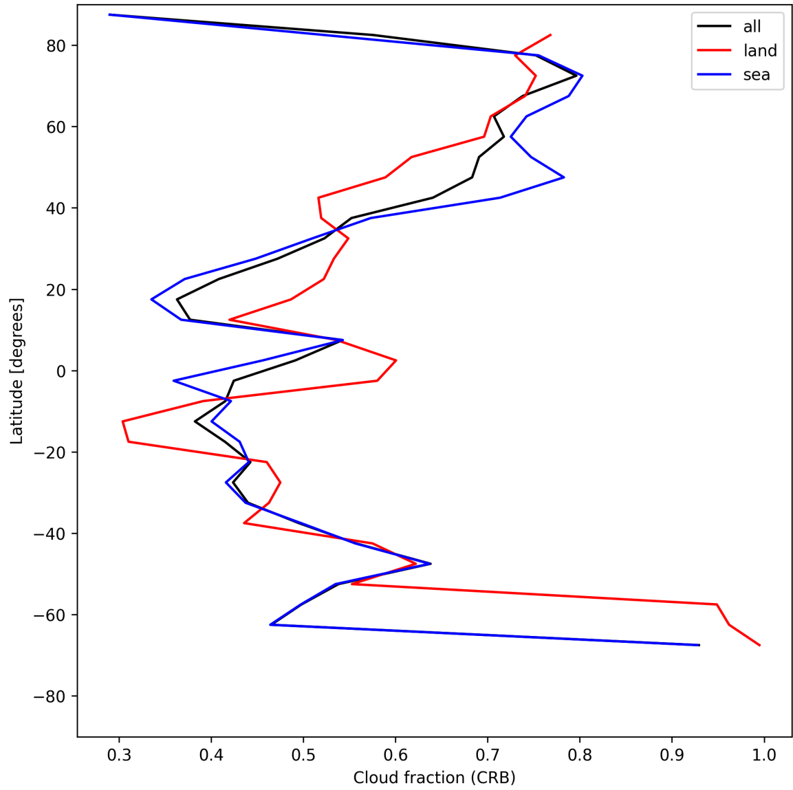
Figure 26: Zonal average of “Cloud fraction (CRB)” for 2025-06-03 to 2025-06-05.
