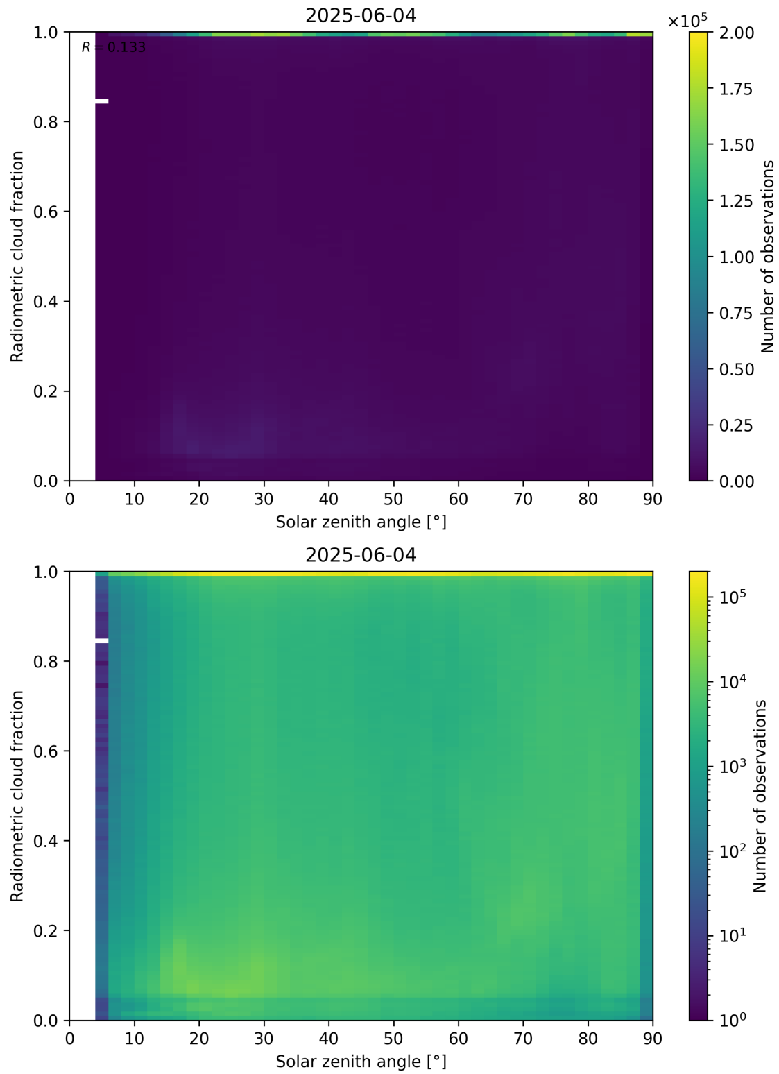
Figure 99: Scatter density plot of “Solar zenith angle” against “Radiometric cloud fraction” for 2025-06-03 to 2025-06-05.
