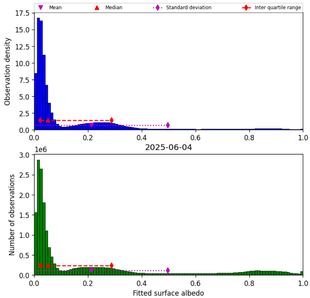
Figure 45: Histogram of “Fitted surface albedo” for 2025-06-03 to 2025-06-05
