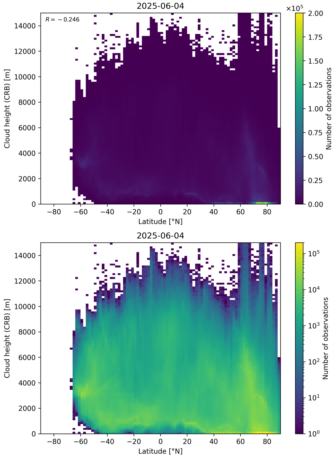
Figure 95: Scatter density plot of “Latitude” against “Cloud height (CRB)” for 2025-06-03 to 2025-06-05.
