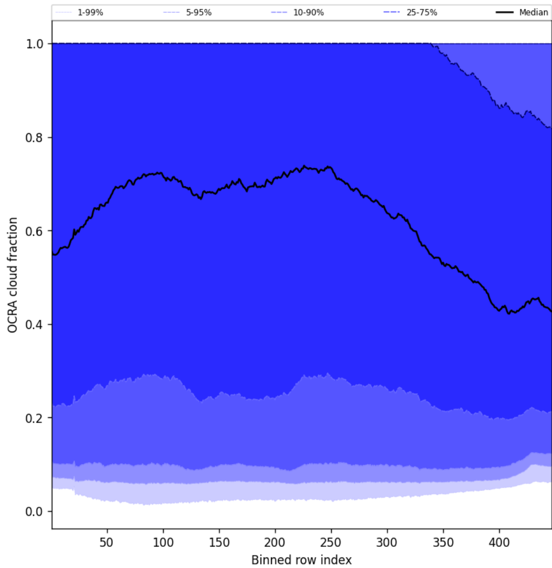
Figure 66: Along track statistics of “OCRA cloud fraction” for 2025-06-03 to 2025-06-05
