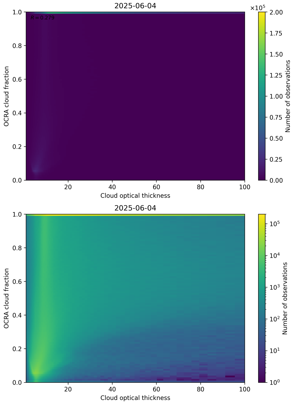
Figure 83: Scatter density plot of “Cloud optical thickness” against “OCRA cloud fraction” for 2025-06-03 to 2025-06-05.
