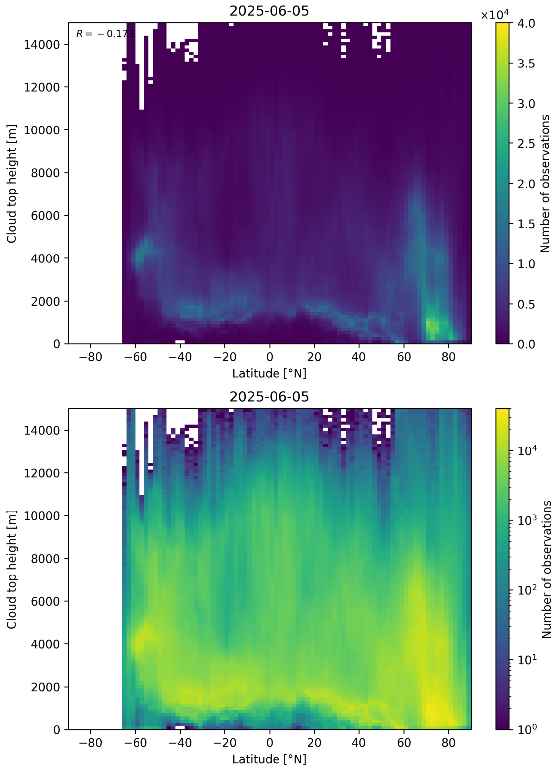
Figure 97: Scatter density plot of “Latitude” against “Cloud top height” for 2025-06-04 to 2025-06-06.
