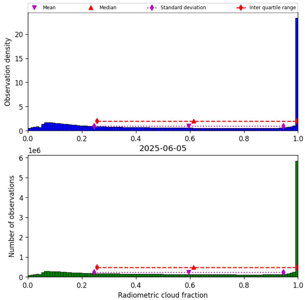
Figure 39: Histogram of “Radiometric cloud fraction” for 2025-06-04 to 2025-06-06
