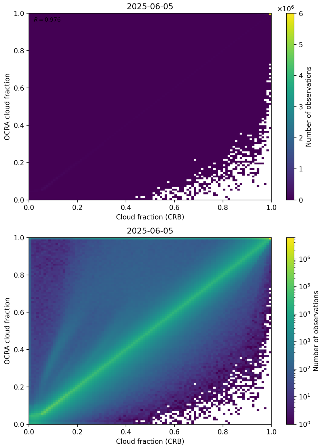
Figure 78: Scatter density plot of “Cloud fraction (CRB)” against “OCRA cloud fraction” for 2025-06-04 to 2025-06-06.
