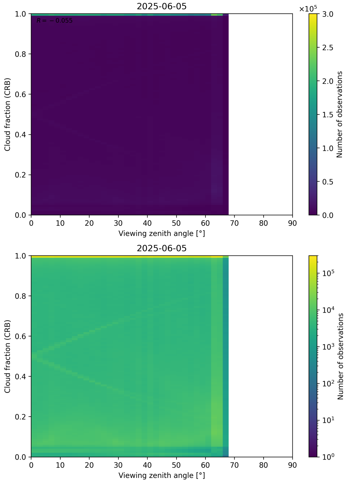
Figure 109: Scatter density plot of “Viewing zenith angle” against “Cloud fraction (CRB)” for 2025-06-04 to 2025-06-06.
