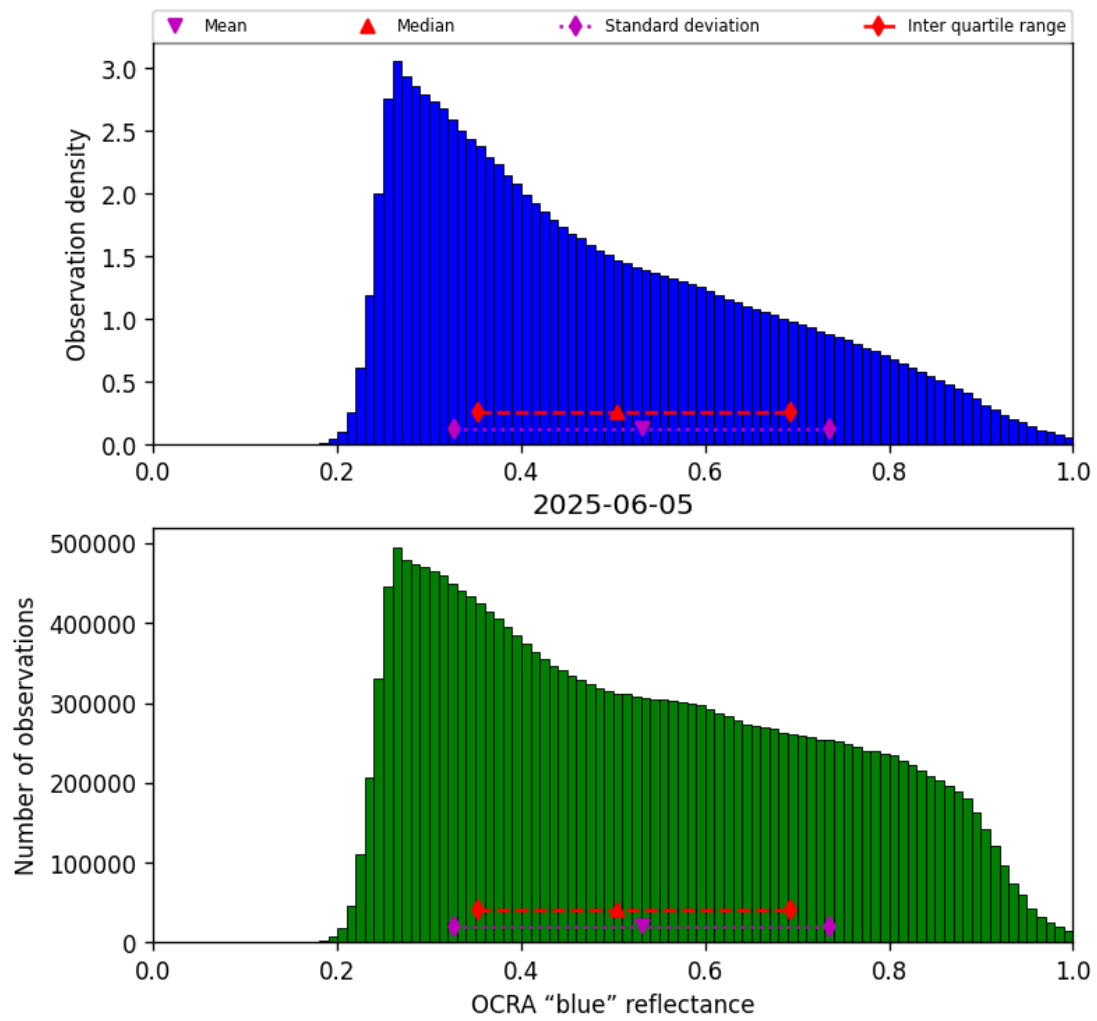
Figure 51: Histogram of “OCRA “blue” reflectance” for 2025-06-04 to 2025-06-06
