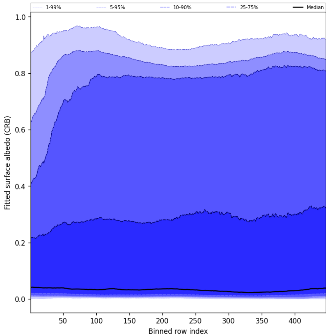
Figure 62: Along track statistics of “Fitted surface albedo (CRB)” for 2025-06-04 to 2025-06-06
