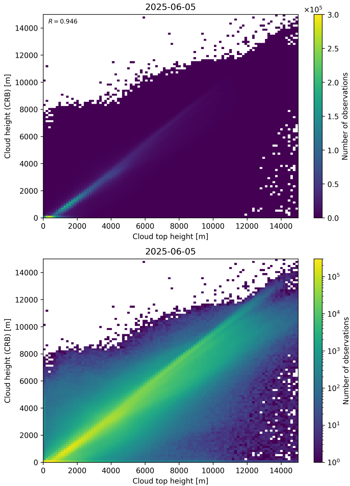
Figure 89: Scatter density plot of “Cloud top height” against “Cloud height (CRB)” for 2025-06-04 to 2025-06-06.
