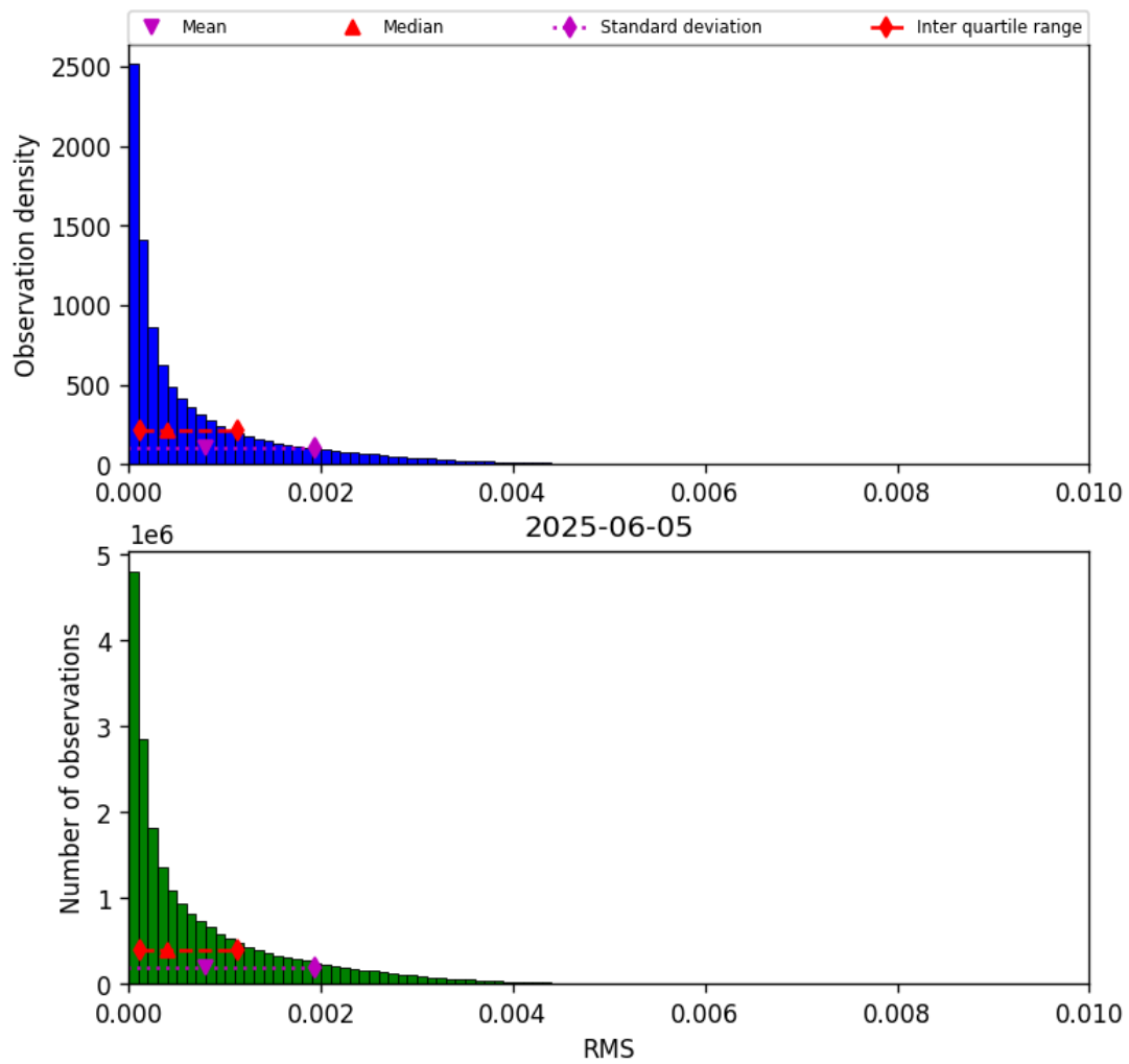
Figure 47: Histogram of “RMS” for 2025-06-04 to 2025-06-06
