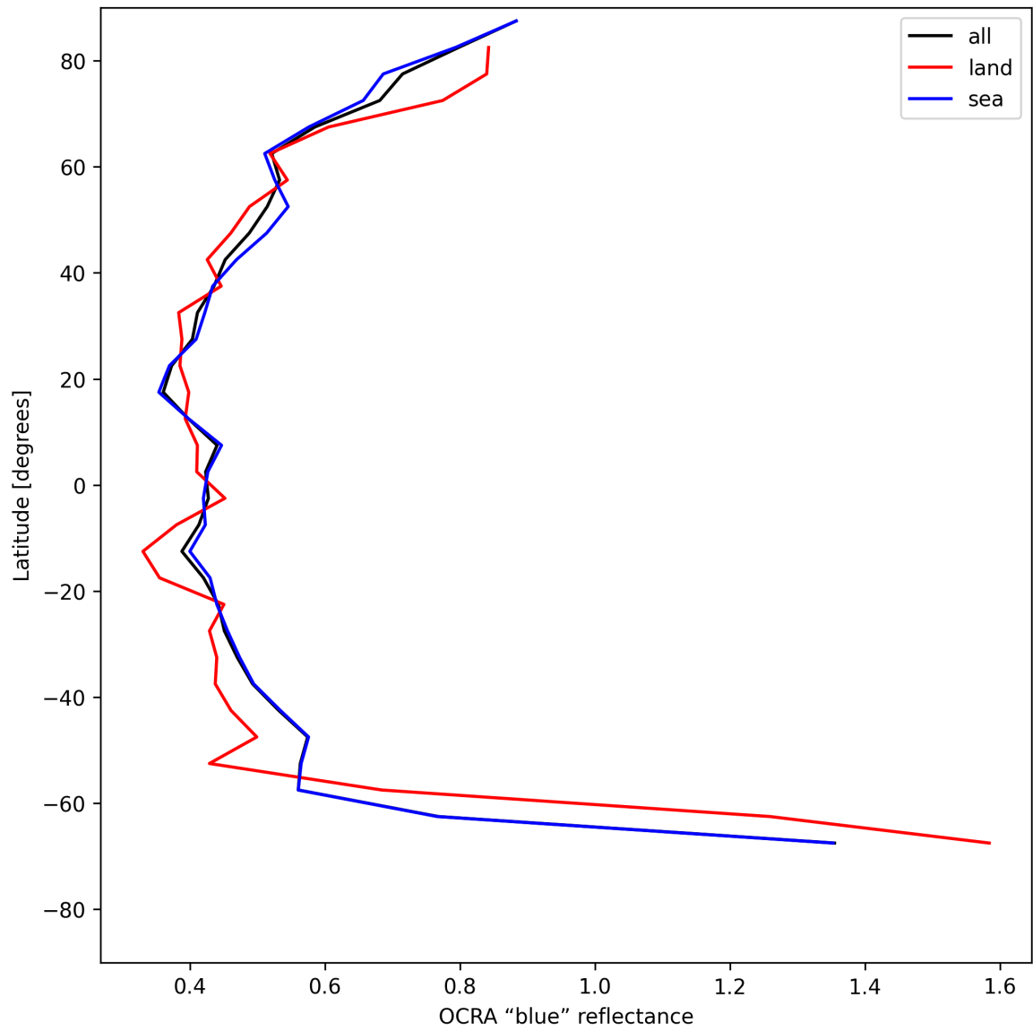
Figure 35: Zonal average of “OCRA “blue” reflectance” for 2025-06-04 to 2025-06-06.
