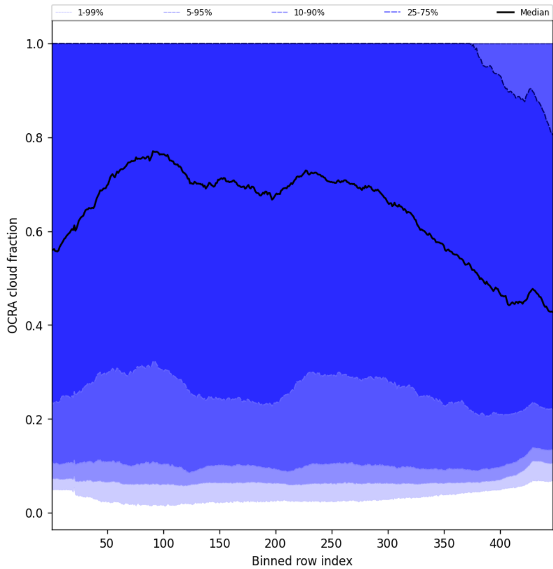
Figure 66: Along track statistics of “OCRA cloud fraction” for 2025-06-04 to 2025-06-06
