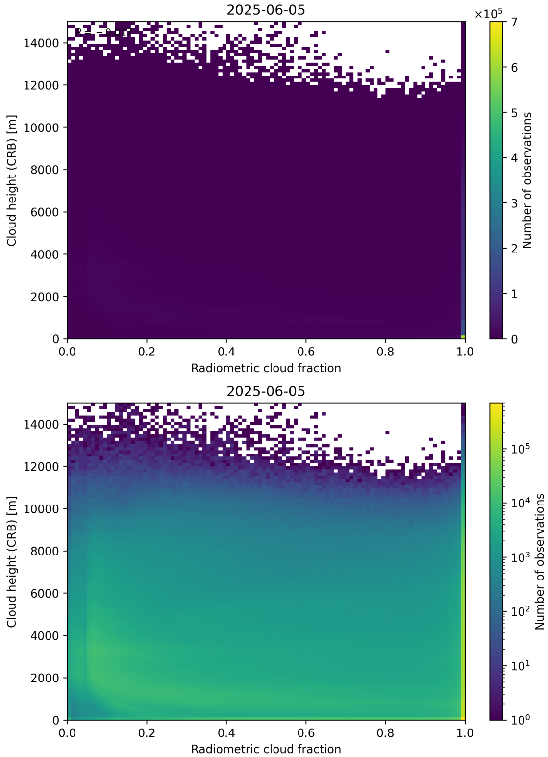
Figure 74: Scatter density plot of “Radiometric cloud fraction” against “Cloud height (CRB)” for 2025-06-04 to 2025-06-06.
