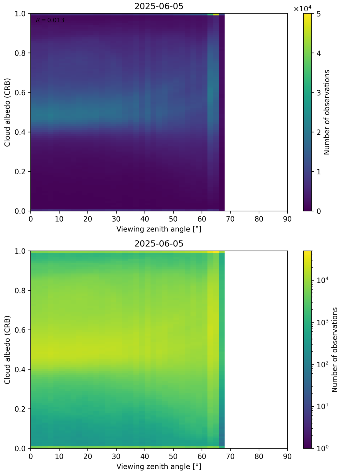
Figure 106: Scatter density plot of “Viewing zenith angle” against “Cloud albedo (CRB)” for 2025-06-04 to 2025-06-06.
