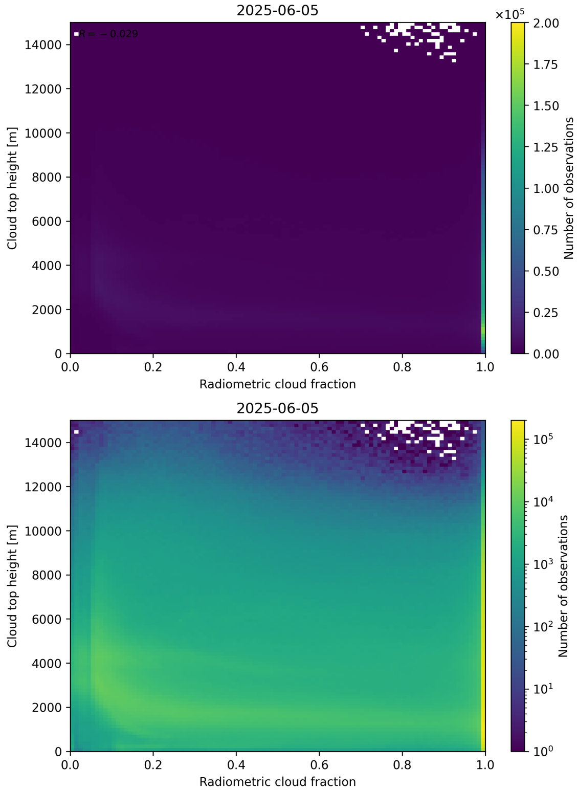
Figure 76: Scatter density plot of “Radiometric cloud fraction” against “Cloud top height” for 2025-06-04 to 2025-06-06.
