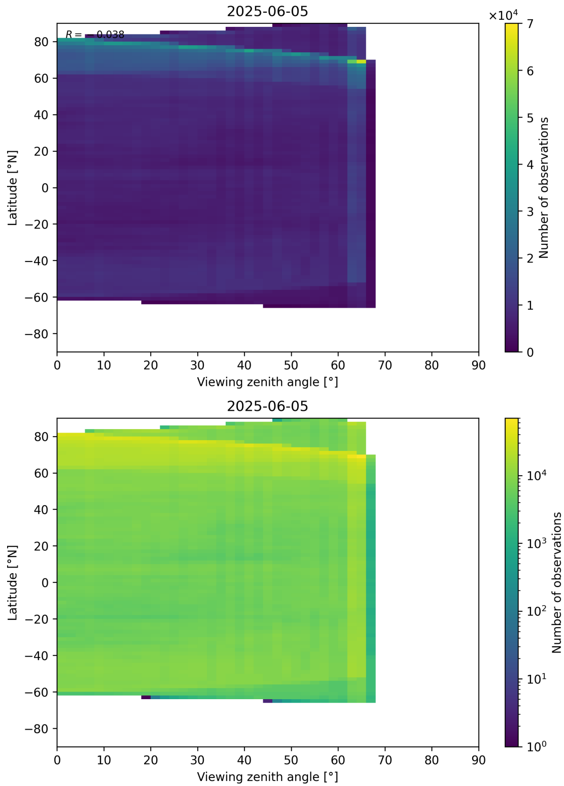
Figure 113: Scatter density plot of “Viewing zenith angle” against “Latitude” for 2025-06-04 to 2025-06-06.
