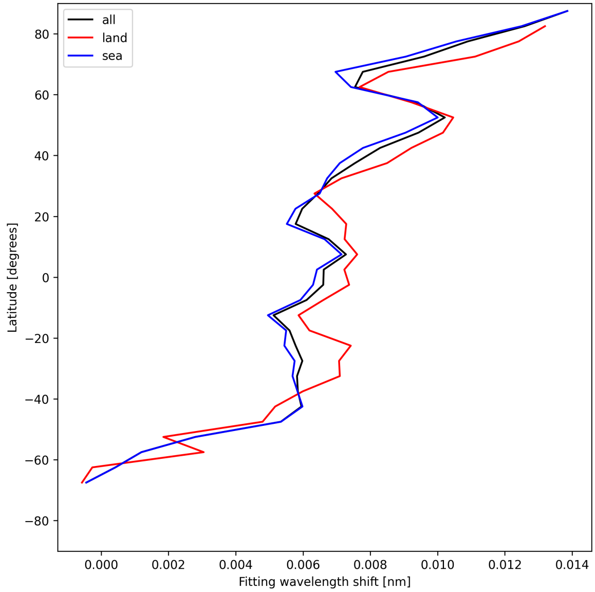
Figure 33: Zonal average of “Fitting wavelength shift” for 2025-06-04 to 2025-06-06.
