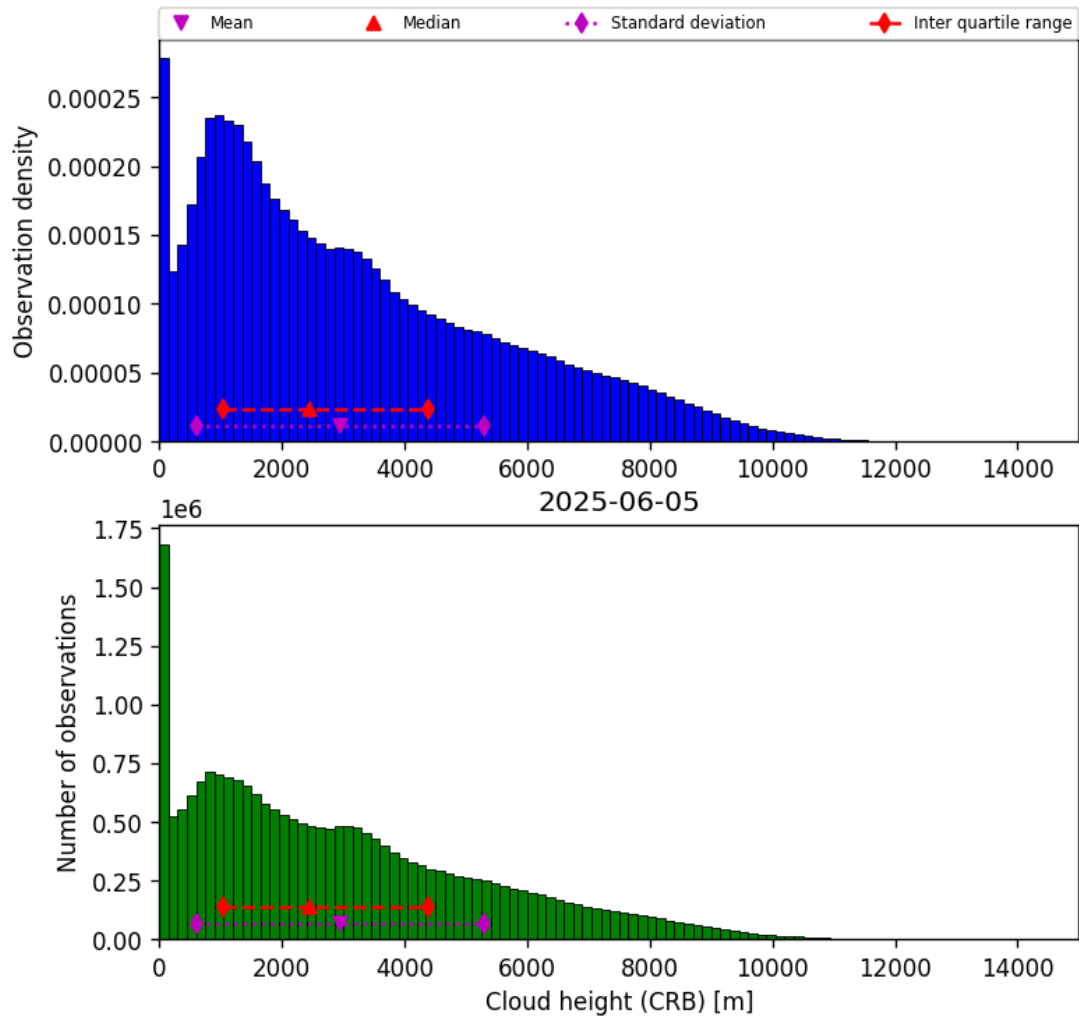
Figure 43: Histogram of “Cloud height (CRB)” for 2025-06-04 to 2025-06-06
