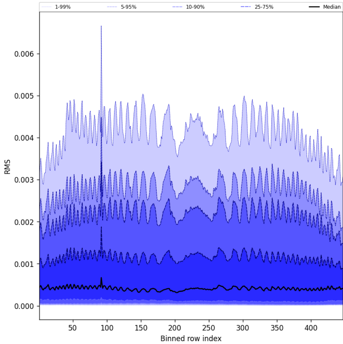
Figure 63: Along track statistics of “RMS” for 2025-06-04 to 2025-06-06
