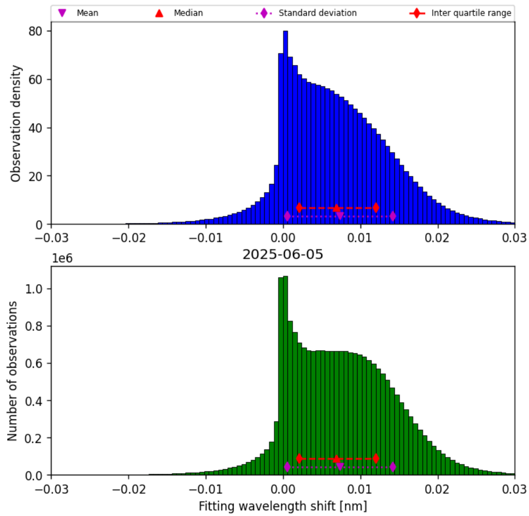
Figure 49: Histogram of “Fitting wavelength shift” for 2025-06-04 to 2025-06-06
