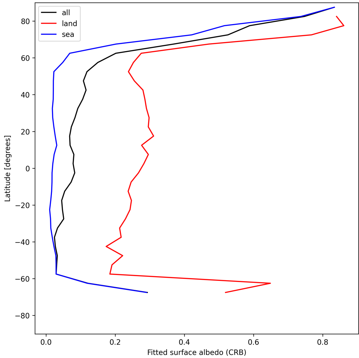
Figure 30: Zonal average of “Fitted surface albedo (CRB)” for 2025-06-04 to 2025-06-06.
