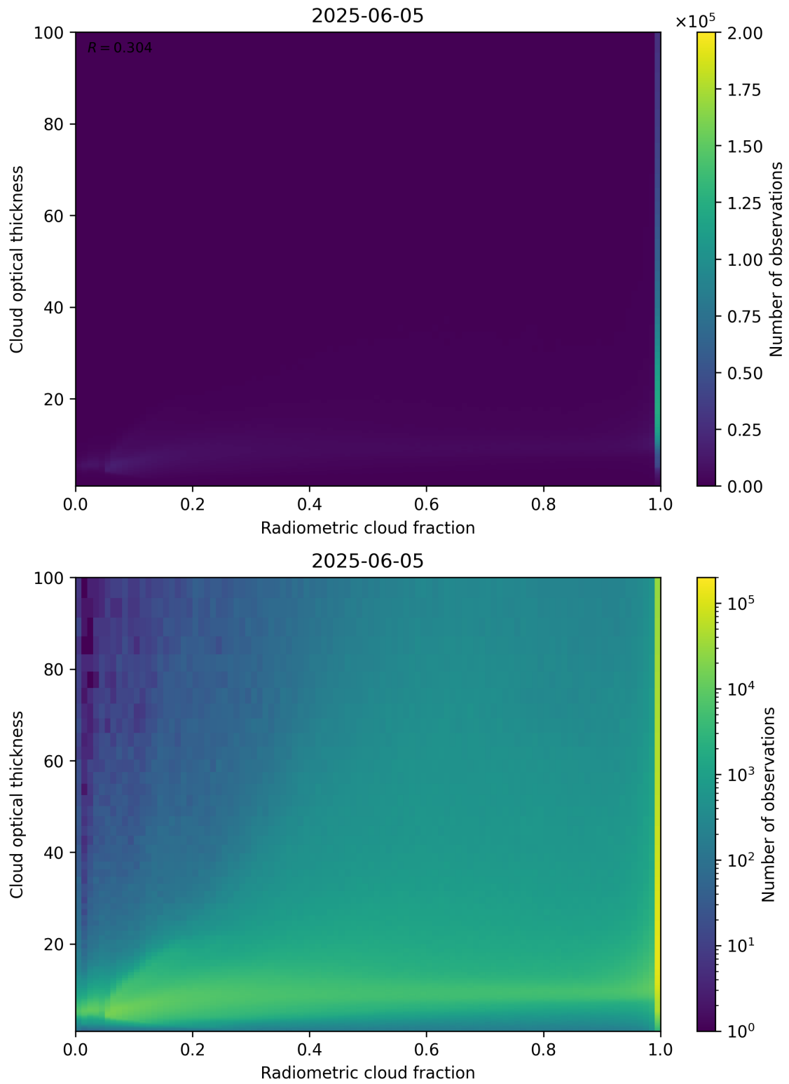
Figure 75: Scatter density plot of “Radiometric cloud fraction” against “Cloud optical thickness” for 2025-06-04 to 2025-06-06.
