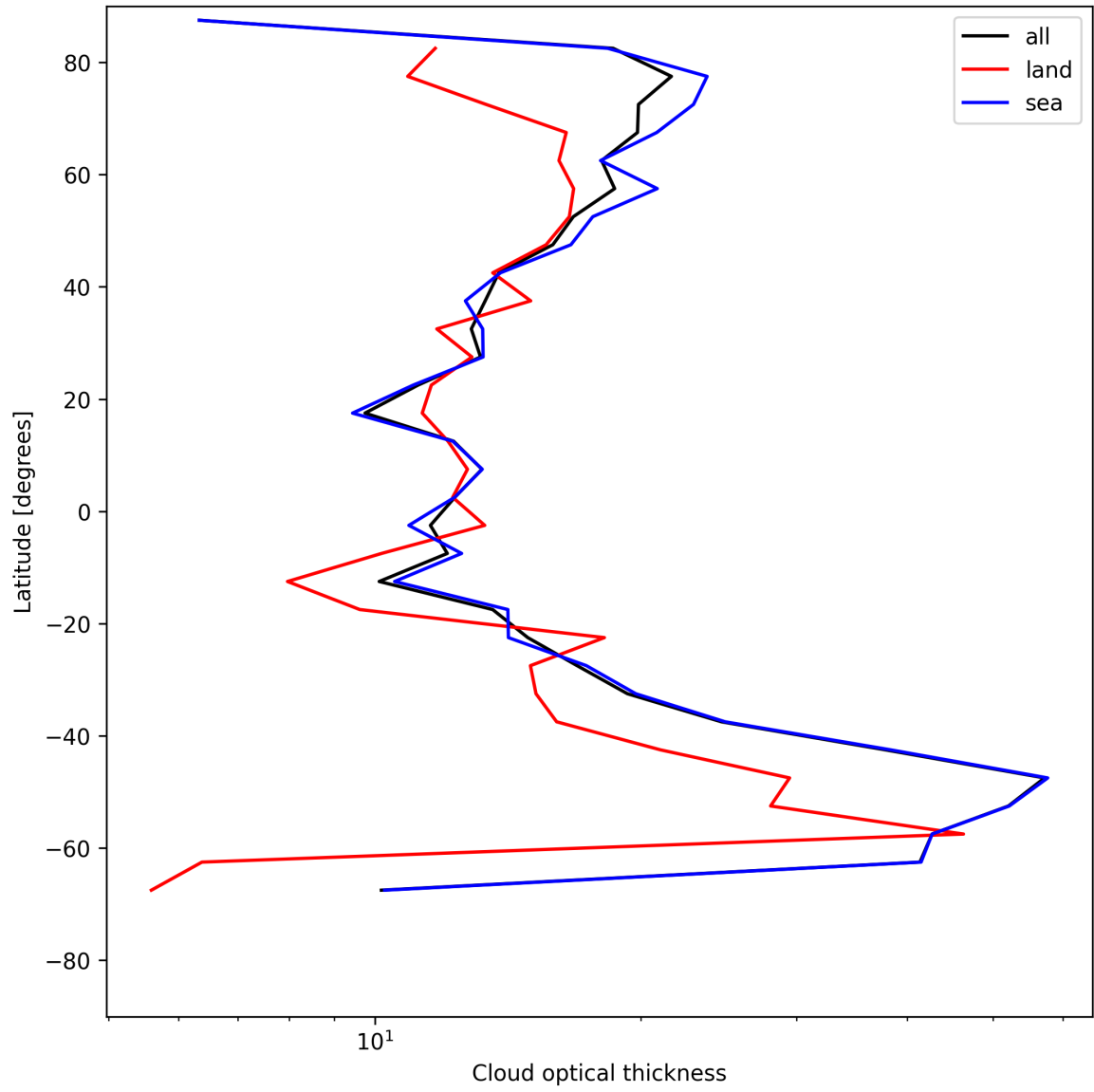
Figure 25: Zonal average of “Cloud optical thickness” for 2025-06-04 to 2025-06-06.
