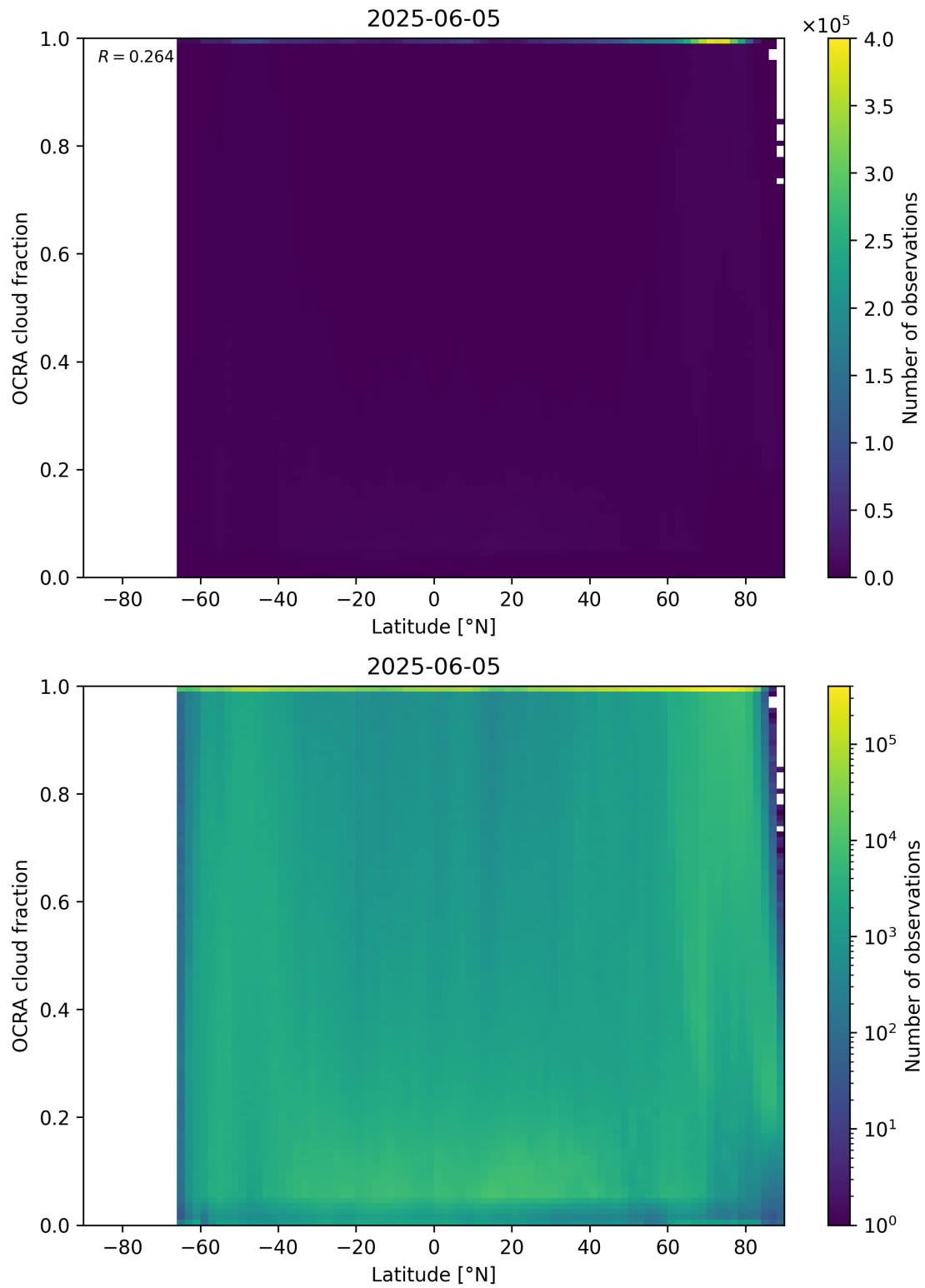
Figure 93: Scatter density plot of “Latitude” against “OCRA cloud fraction” for 2025-06-04 to 2025-06-06.
