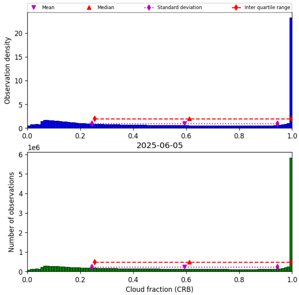
Figure 42: Histogram of “Cloud fraction (CRB)” for 2025-06-04 to 2025-06-06
