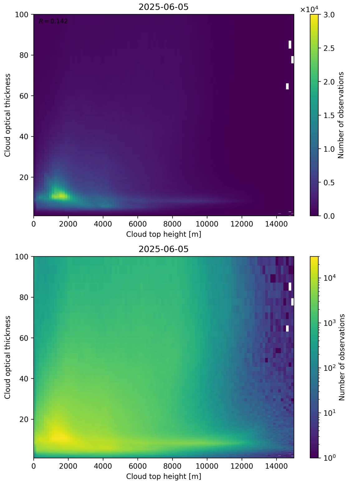
Figure 90: Scatter density plot of “Cloud top height” against “Cloud optical thickness” for 2025-06-04 to 2025-06-06.
