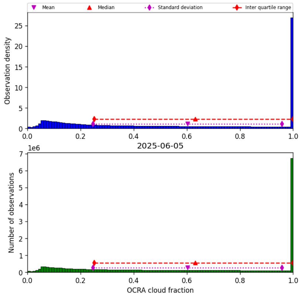
Figure 50: Histogram of “OCRA cloud fraction” for 2025-06-04 to 2025-06-06
