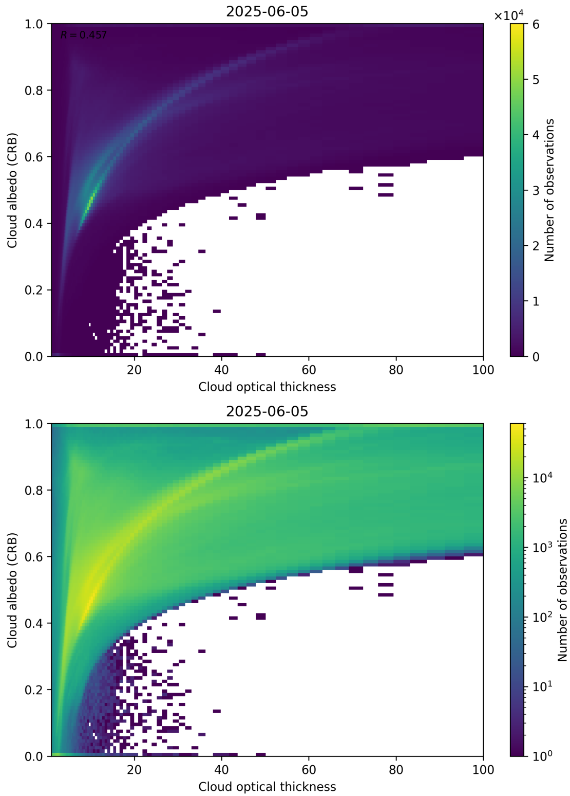
Figure 82: Scatter density plot of “Cloud optical thickness” against “Cloud albedo (CRB)” for 2025-06-04 to 2025-06-06.
