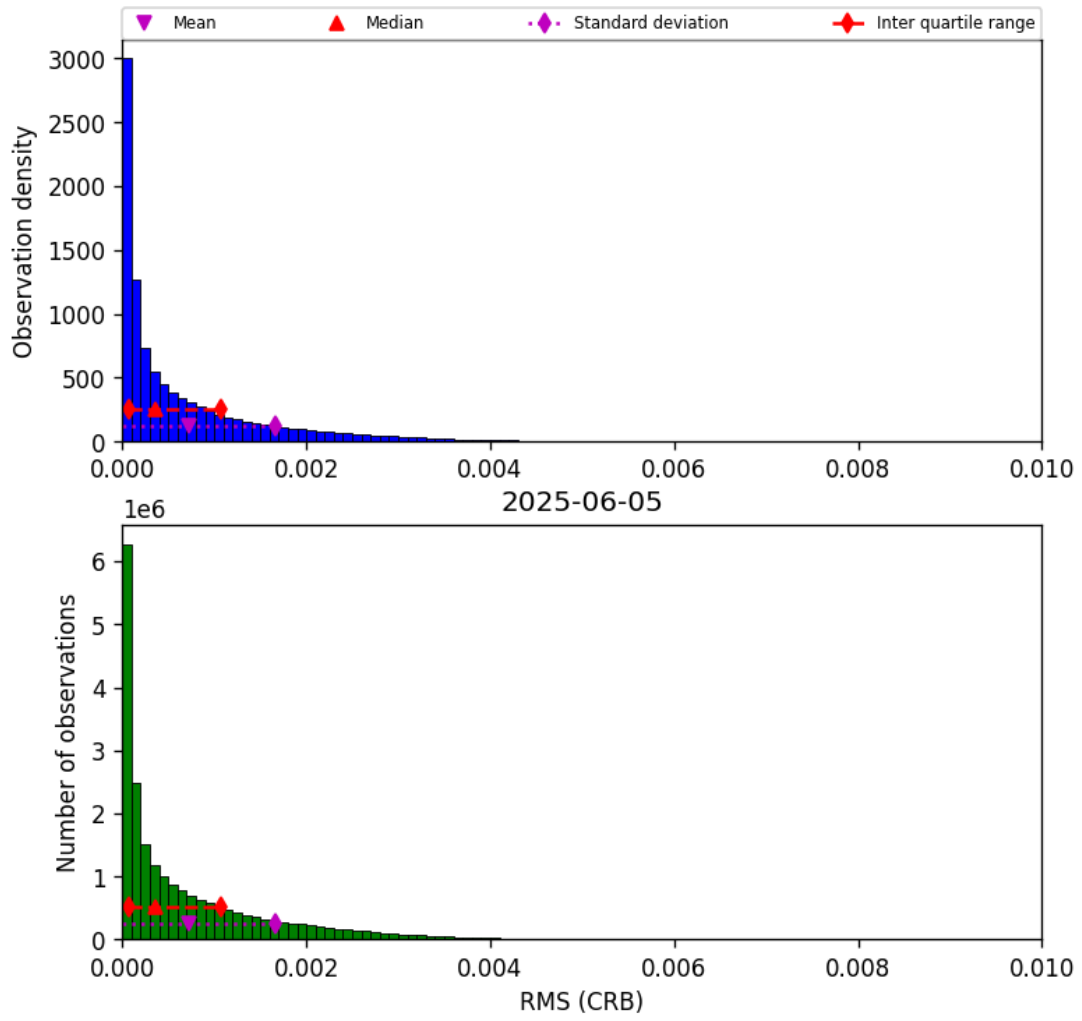
Figure 48: Histogram of “RMS (CRB)” for 2025-06-04 to 2025-06-06
