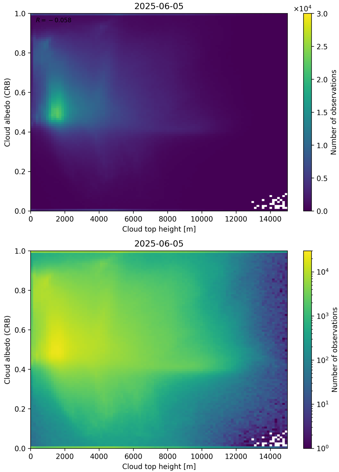
Figure 86: Scatter density plot of “Cloud top height” against “Cloud albedo (CRB)” for 2025-06-04 to 2025-06-06.
