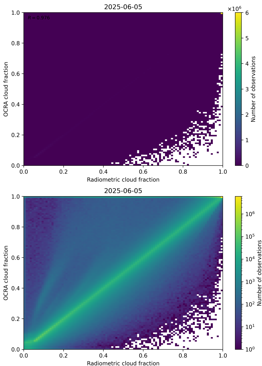
Figure 72: Scatter density plot of “Radiometric cloud fraction” against “OCRA cloud fraction” for 2025-06-04 to 2025-06-06.
