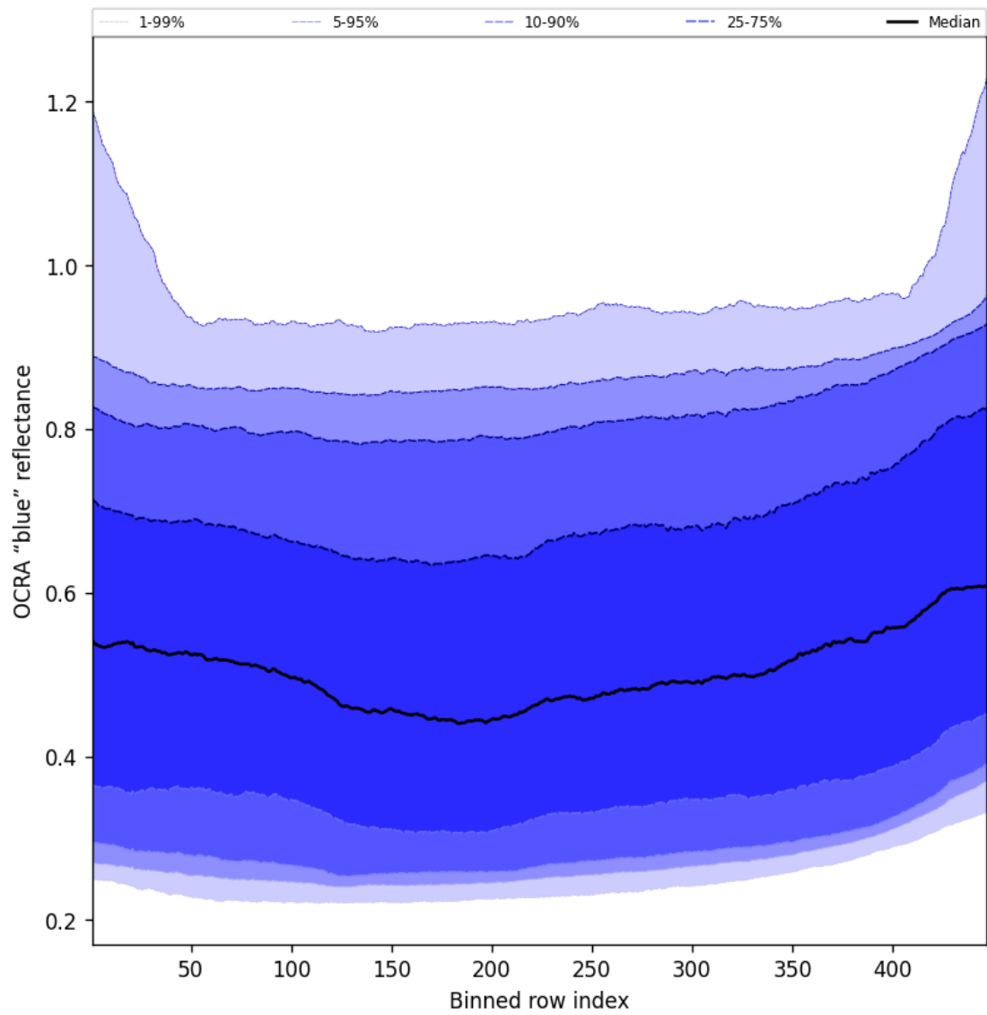
Figure 67: Along track statistics of “OCRA “blue” reflectance” for 2025-06-04 to 2025-06-06
