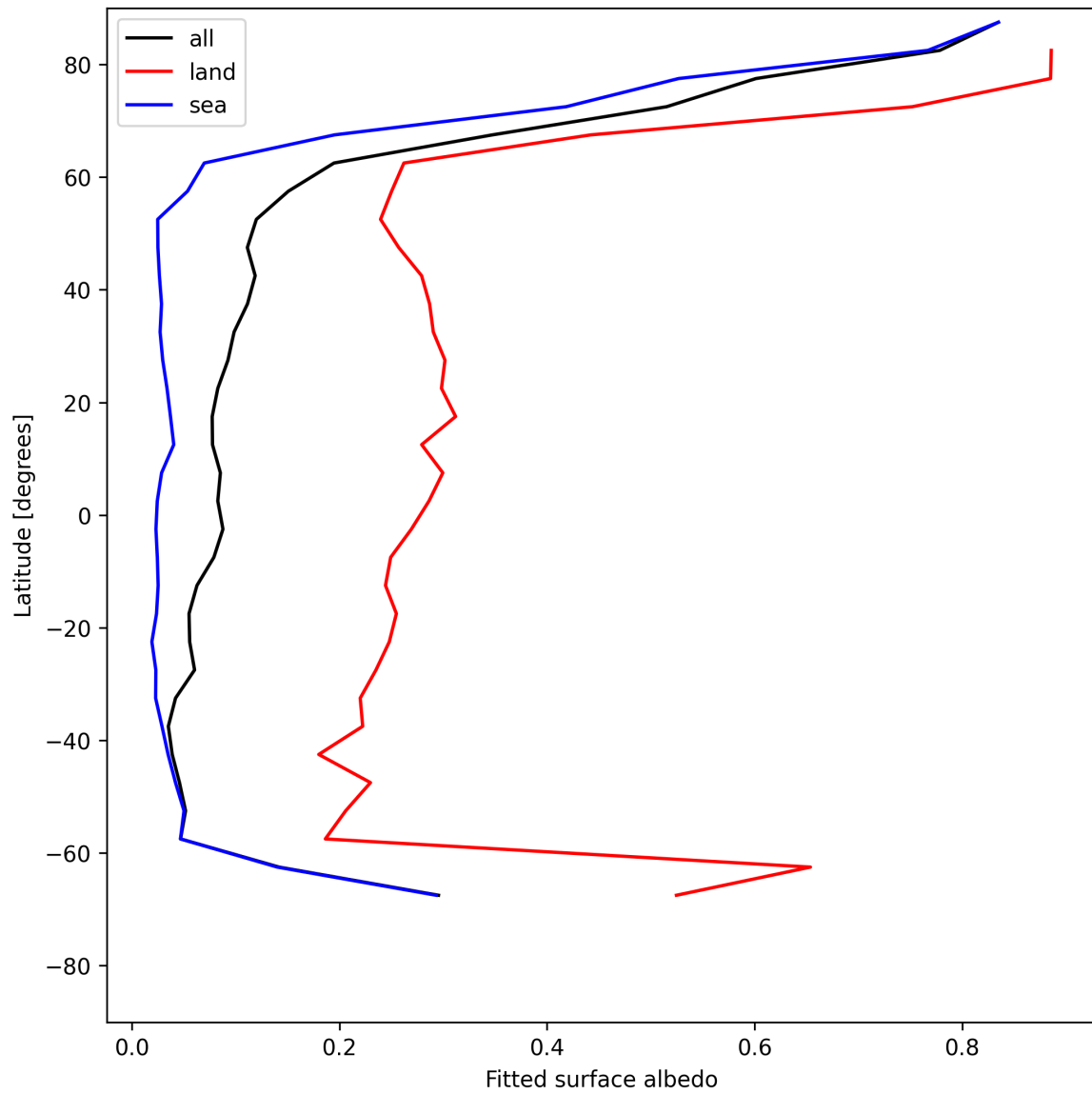
Figure 29: Zonal average of “Fitted surface albedo” for 2025-06-04 to 2025-06-06.
