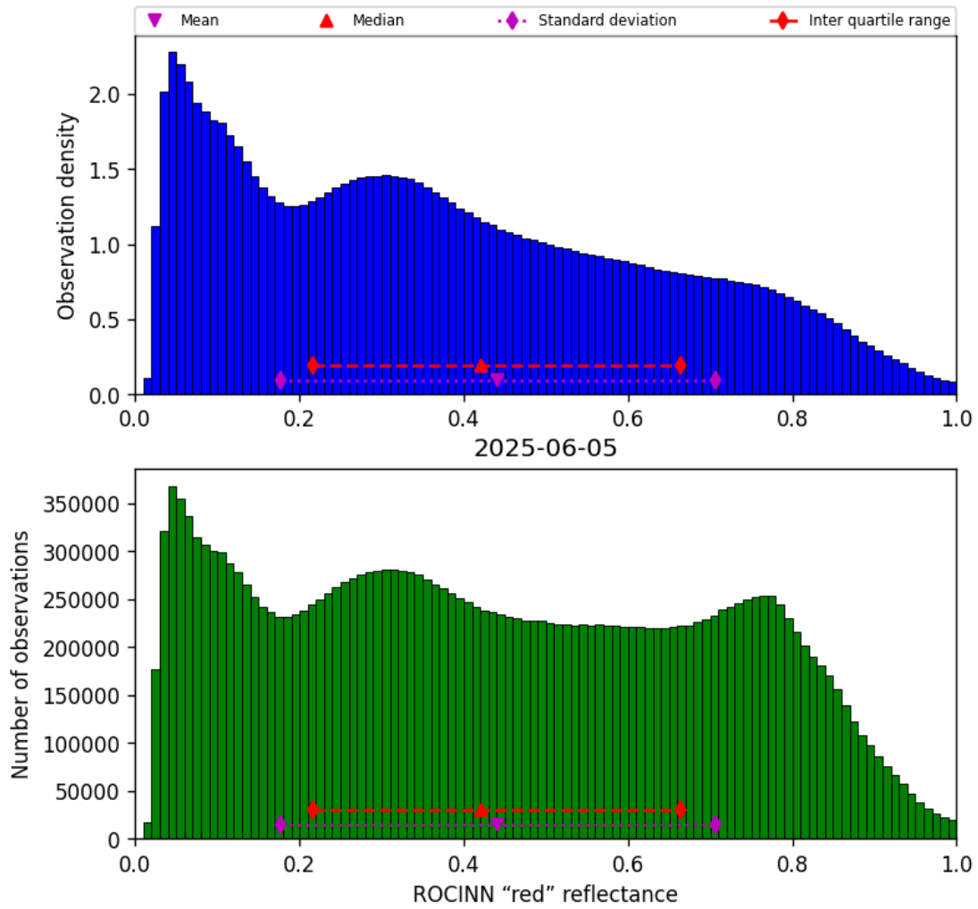
Figure 53: Histogram of “ROCINN “red” reflectance” for 2025-06-04 to 2025-06-06
