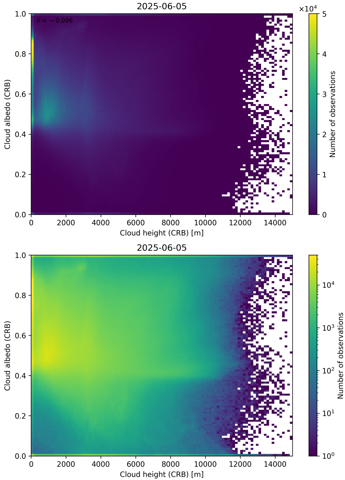
Figure 80: Scatter density plot of “Cloud height (CRB)” against “Cloud albedo (CRB)” for 2025-06-04 to 2025-06-06.
