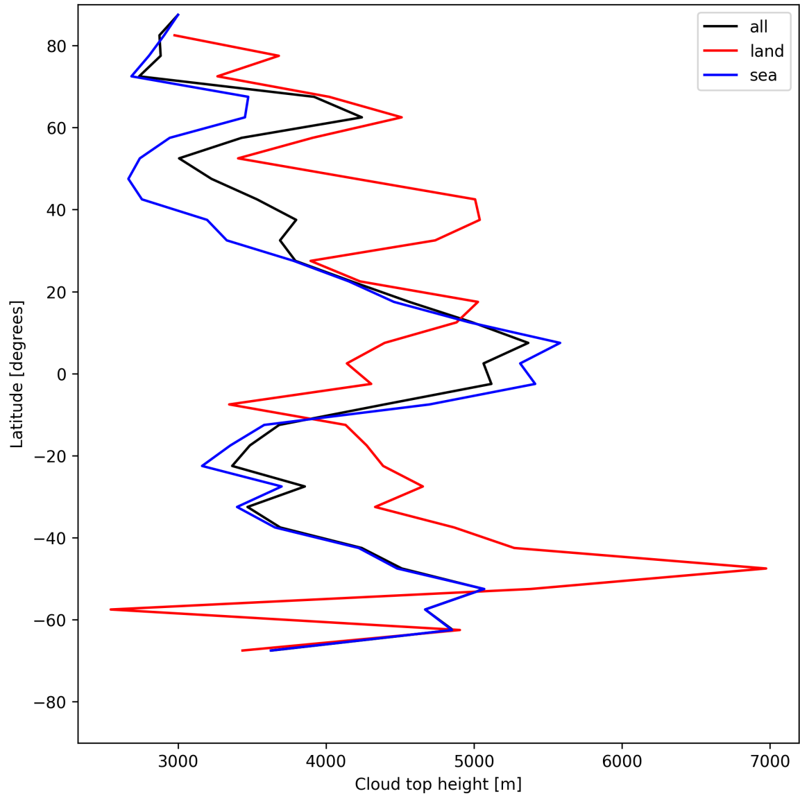
Figure 24: Zonal average of “Cloud top height” for 2025-06-04 to 2025-06-06.
