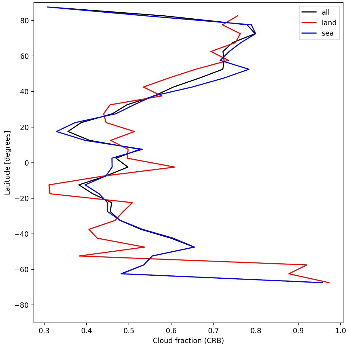
Figure 26: Zonal average of “Cloud fraction (CRB)” for 2025-06-04 to 2025-06-06.
