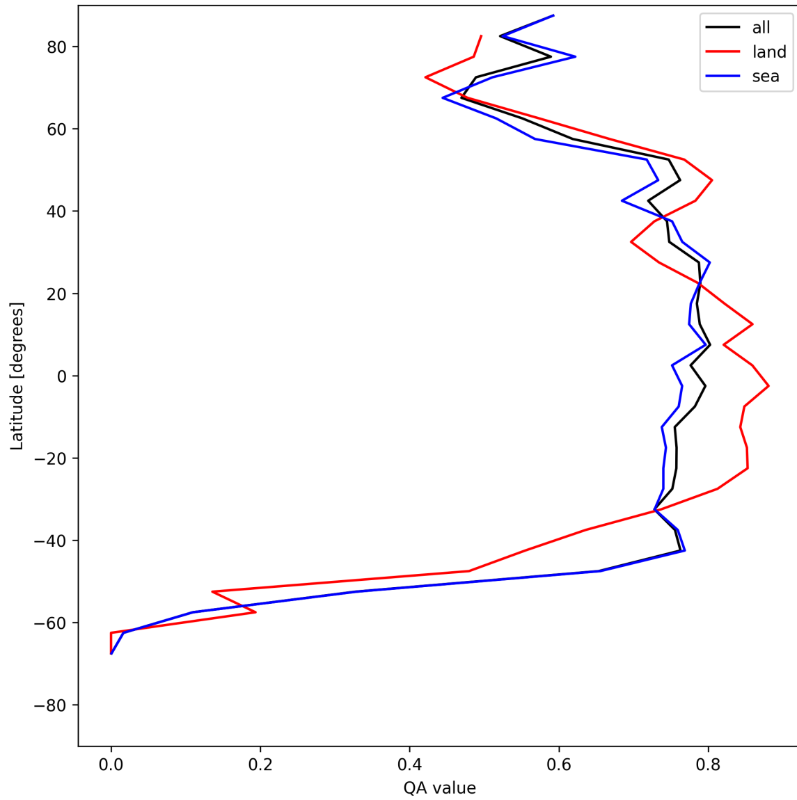
Figure 22: Zonal average of “QA value” for 2025-06-04 to 2025-06-06.
