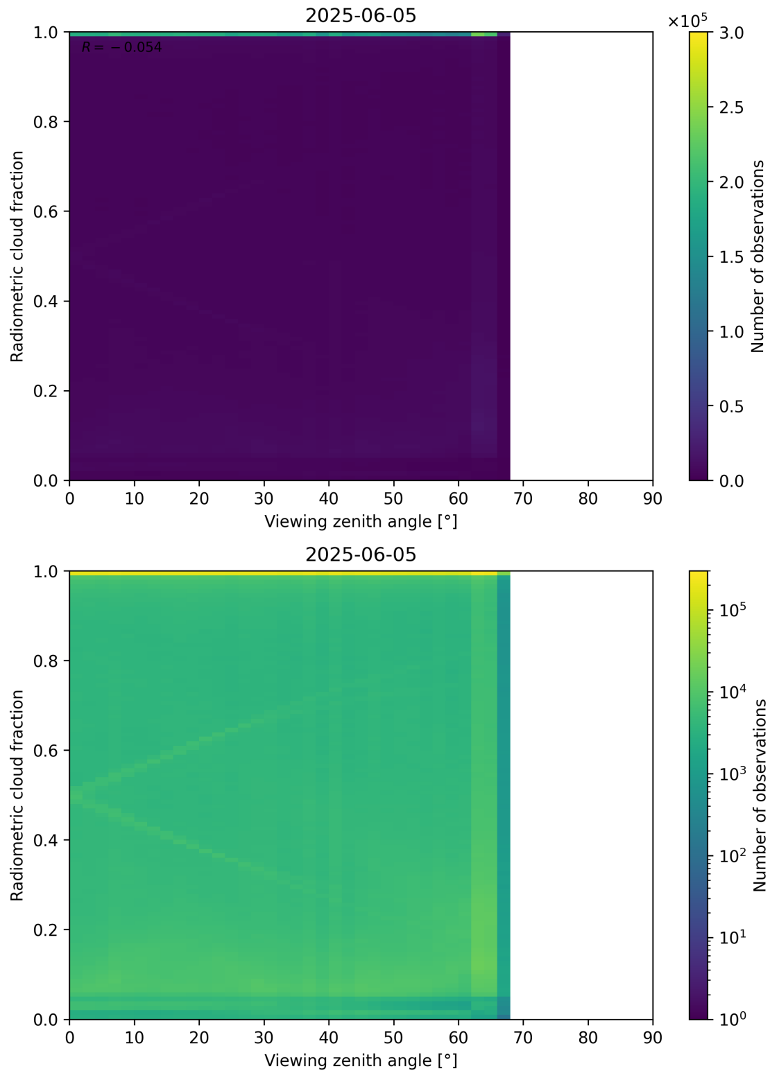
Figure 107: Scatter density plot of “Viewing zenith angle” against “Radiometric cloud fraction” for 2025-06-04 to 2025-06-06.
