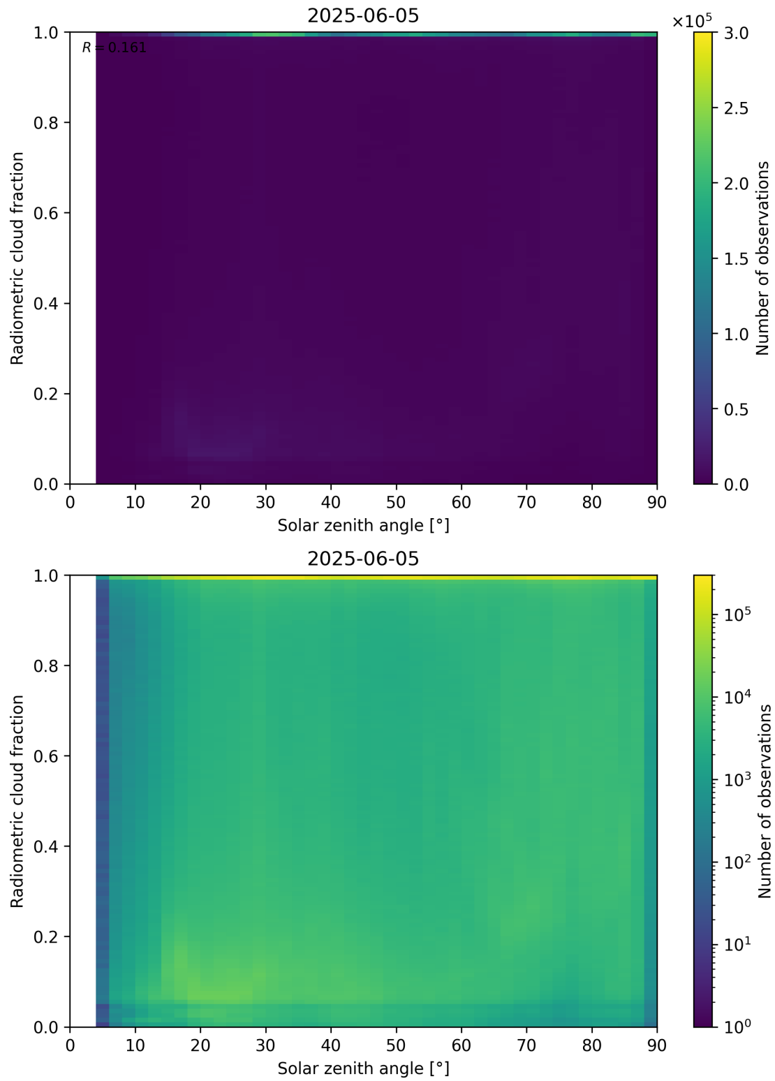
Figure 99: Scatter density plot of “Solar zenith angle” against “Radiometric cloud fraction” for 2025-06-04 to 2025-06-06.
