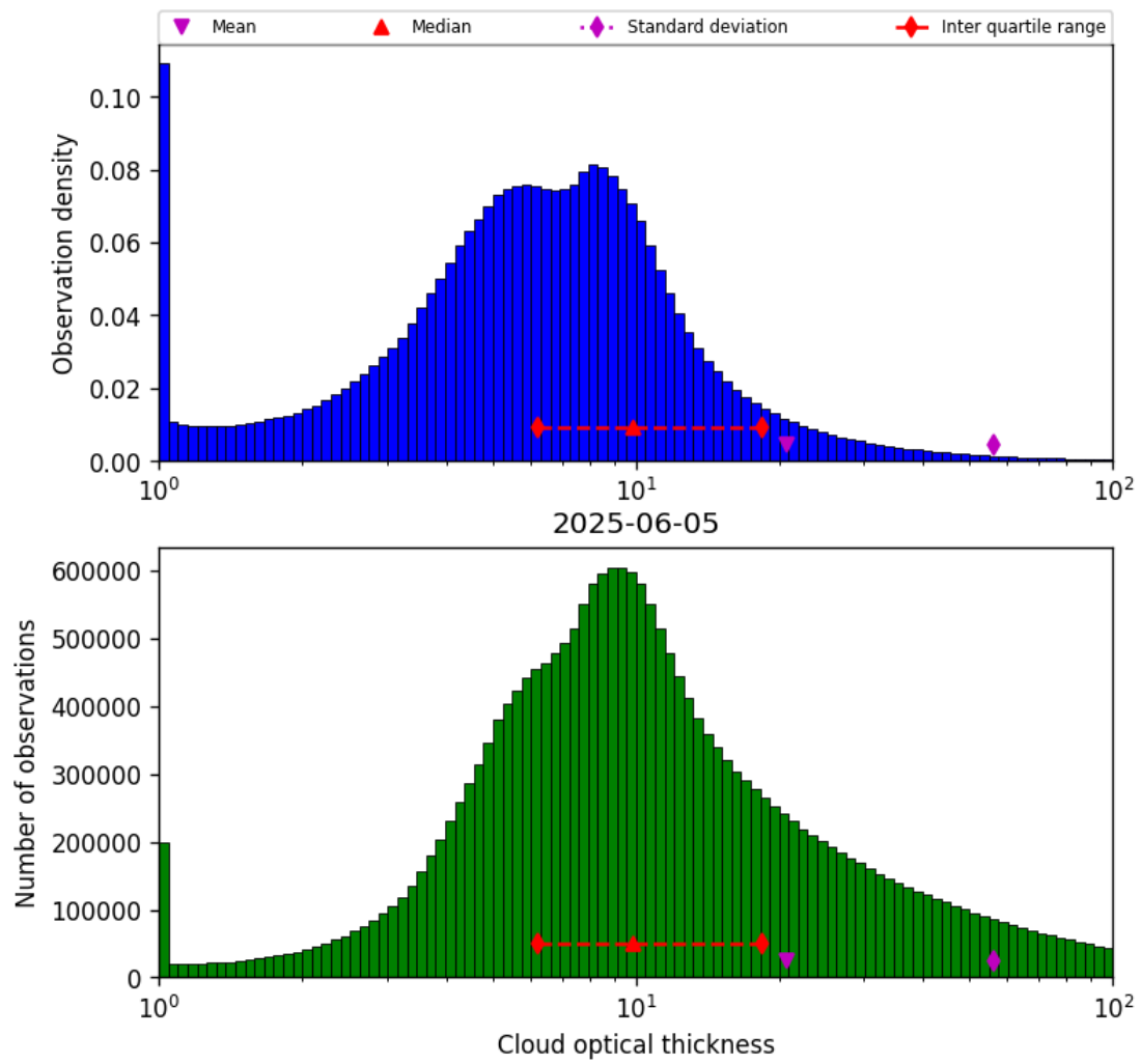
Figure 41: Histogram of “Cloud optical thickness” for 2025-06-04 to 2025-06-06
