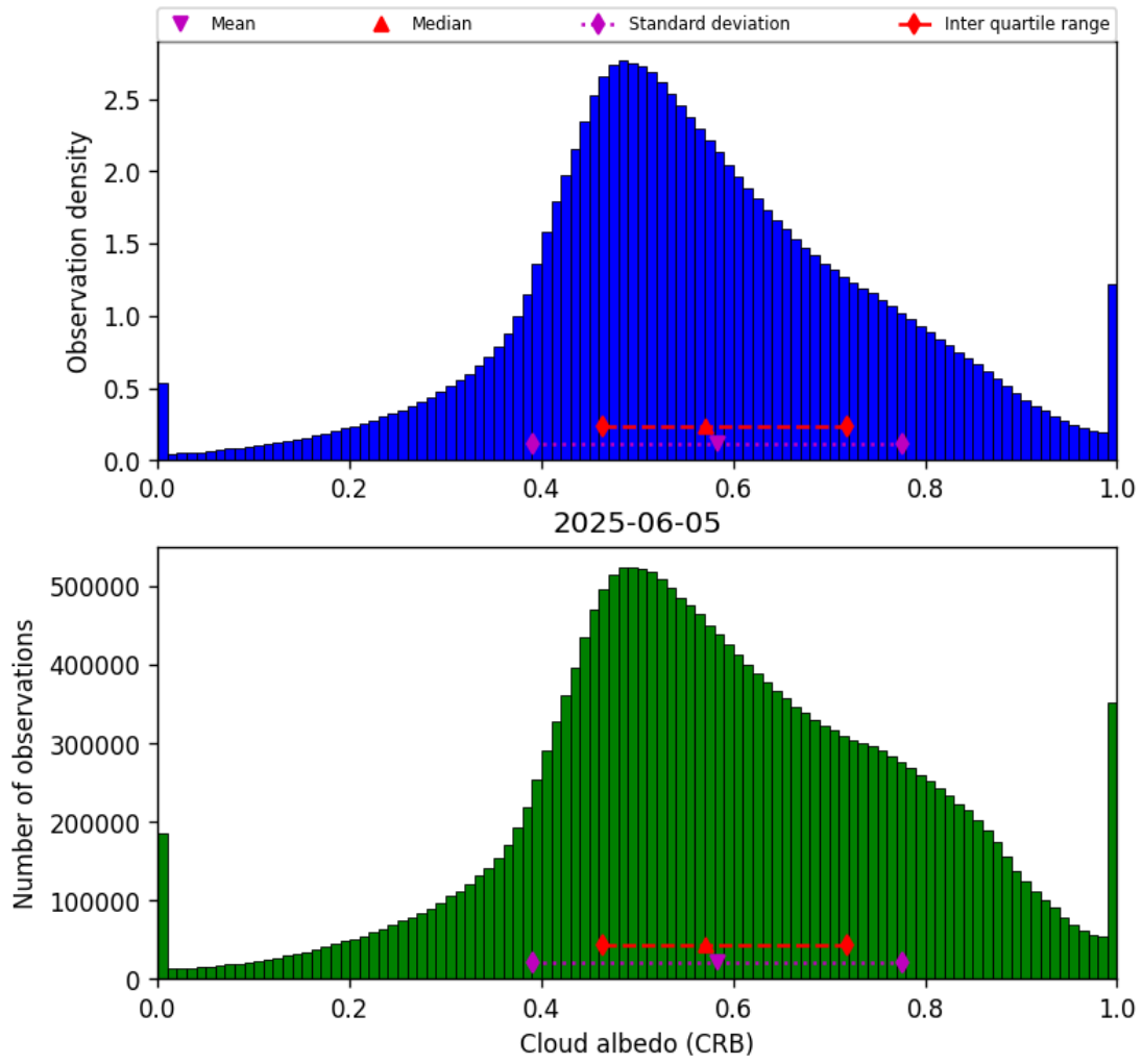
Figure 44: Histogram of “Cloud albedo (CRB)” for 2025-06-04 to 2025-06-06
