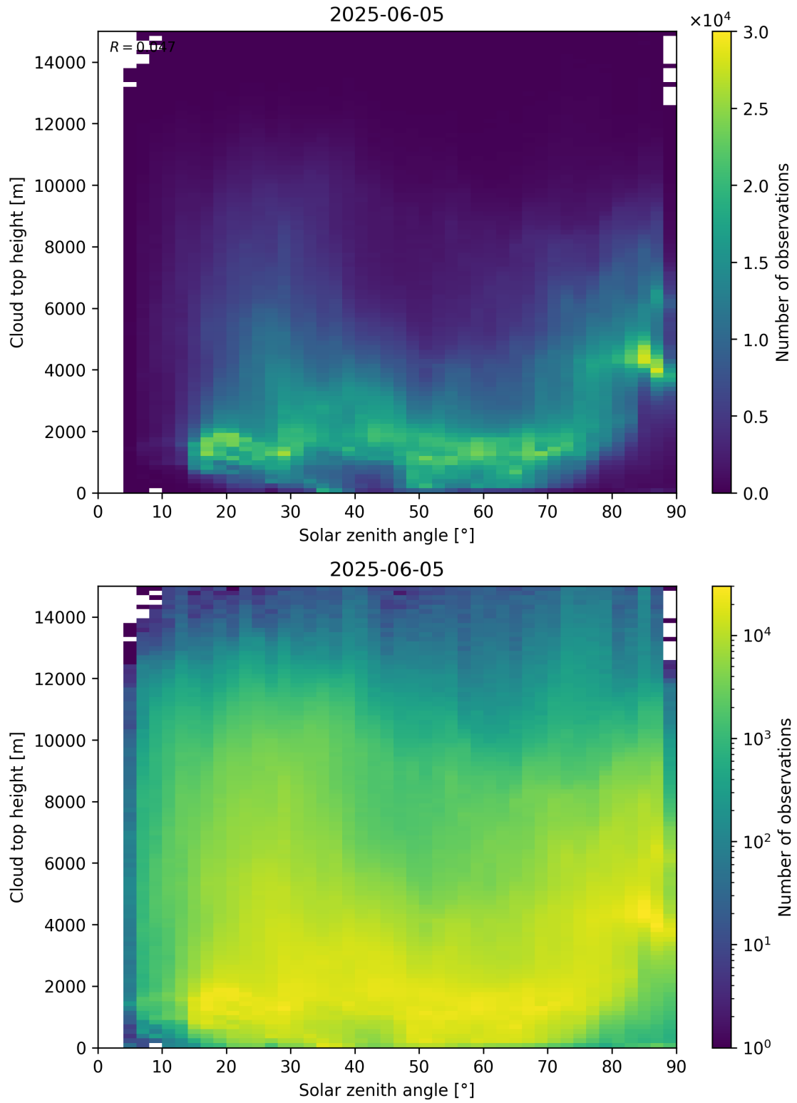
Figure 104: Scatter density plot of “Solar zenith angle” against “Cloud top height” for 2025-06-04 to 2025-06-06.
