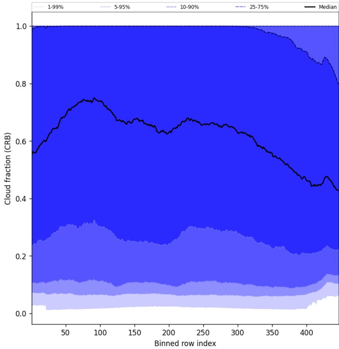
Figure 58: Along track statistics of “Cloud fraction (CRB)” for 2025-06-04 to 2025-06-06
