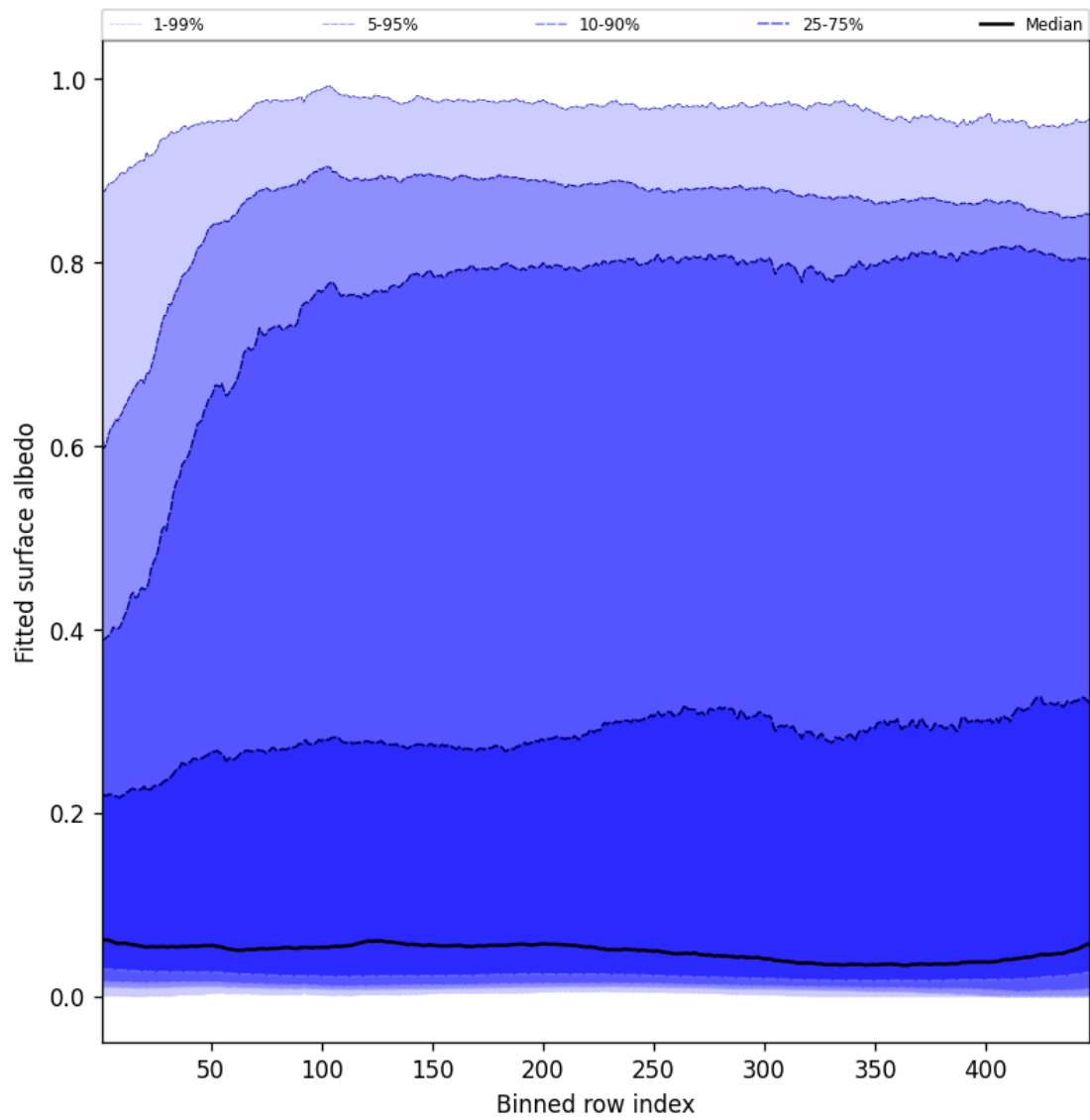
Figure 61: Along track statistics of “Fitted surface albedo” for 2025-06-04 to 2025-06-06
