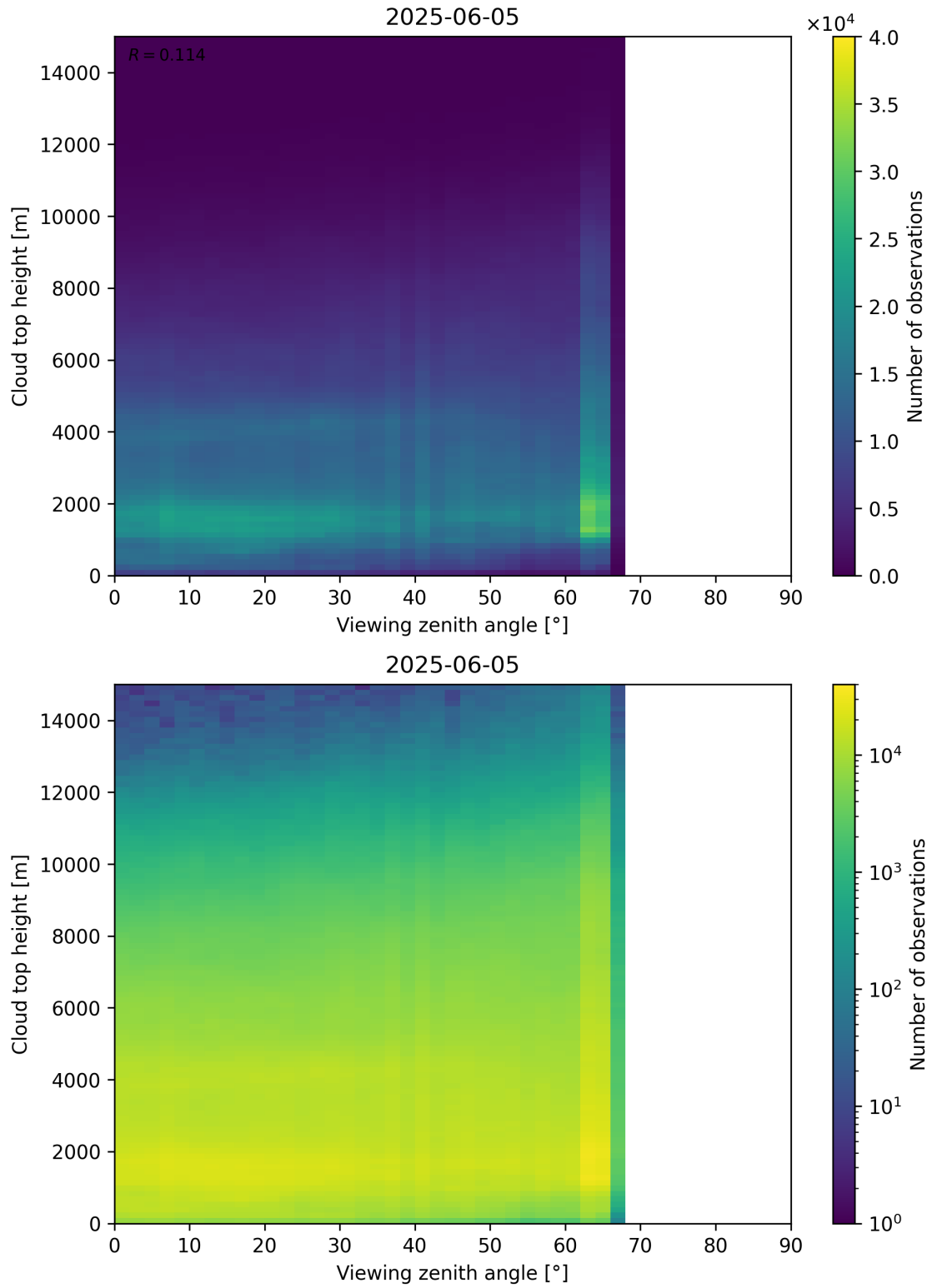
Figure 112: Scatter density plot of “Viewing zenith angle” against “Cloud top height” for 2025-06-04 to 2025-06-06.
