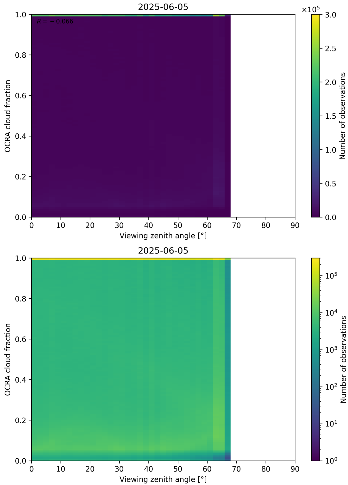
Figure 108: Scatter density plot of “Viewing zenith angle” against “OCRA cloud fraction” for 2025-06-04 to 2025-06-06.
