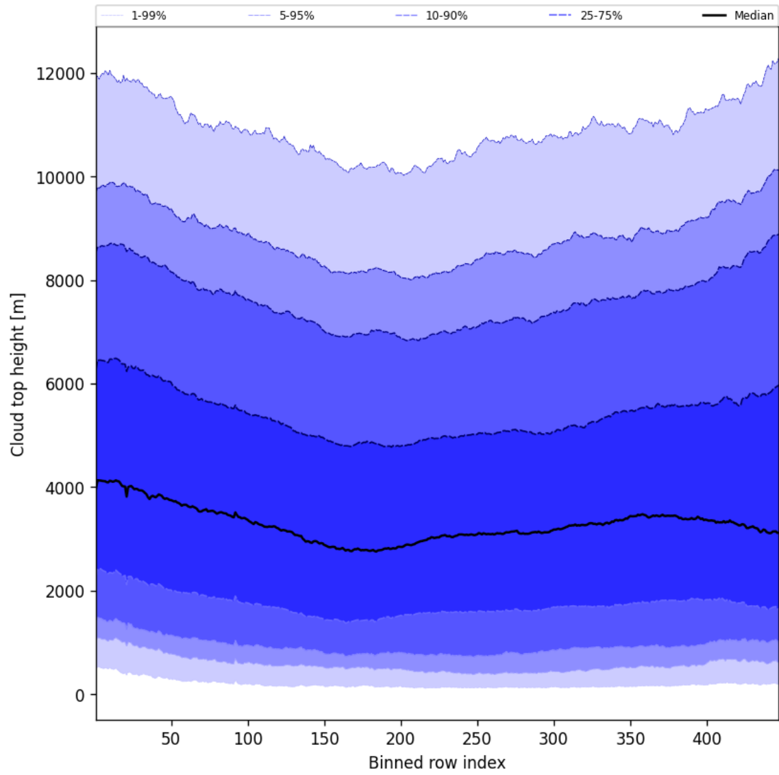
Figure 56: Along track statistics of “Cloud top height” for 2025-06-04 to 2025-06-06
