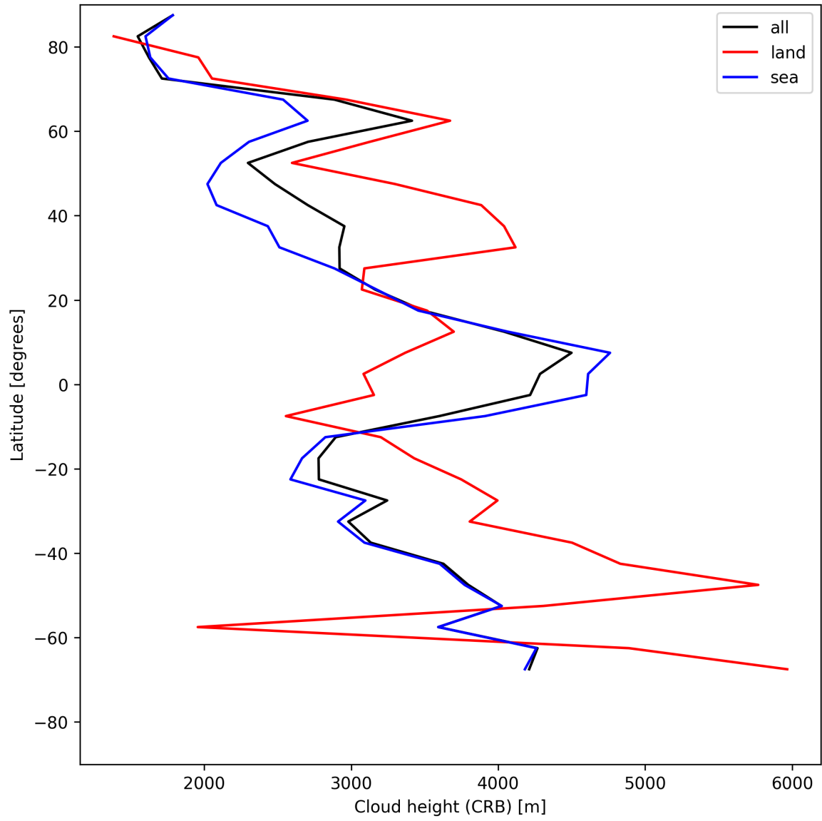
Figure 27: Zonal average of “Cloud height (CRB)” for 2025-06-04 to 2025-06-06.
