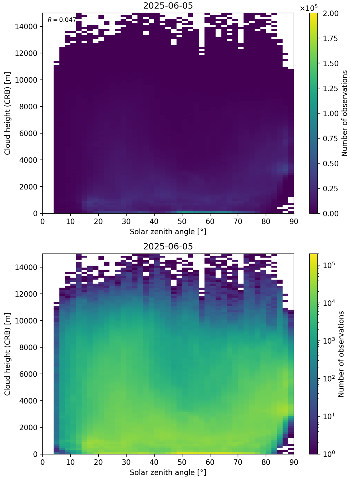
Figure 102: Scatter density plot of “Solar zenith angle” against “Cloud height (CRB)” for 2025-06-04 to 2025-06-06.
