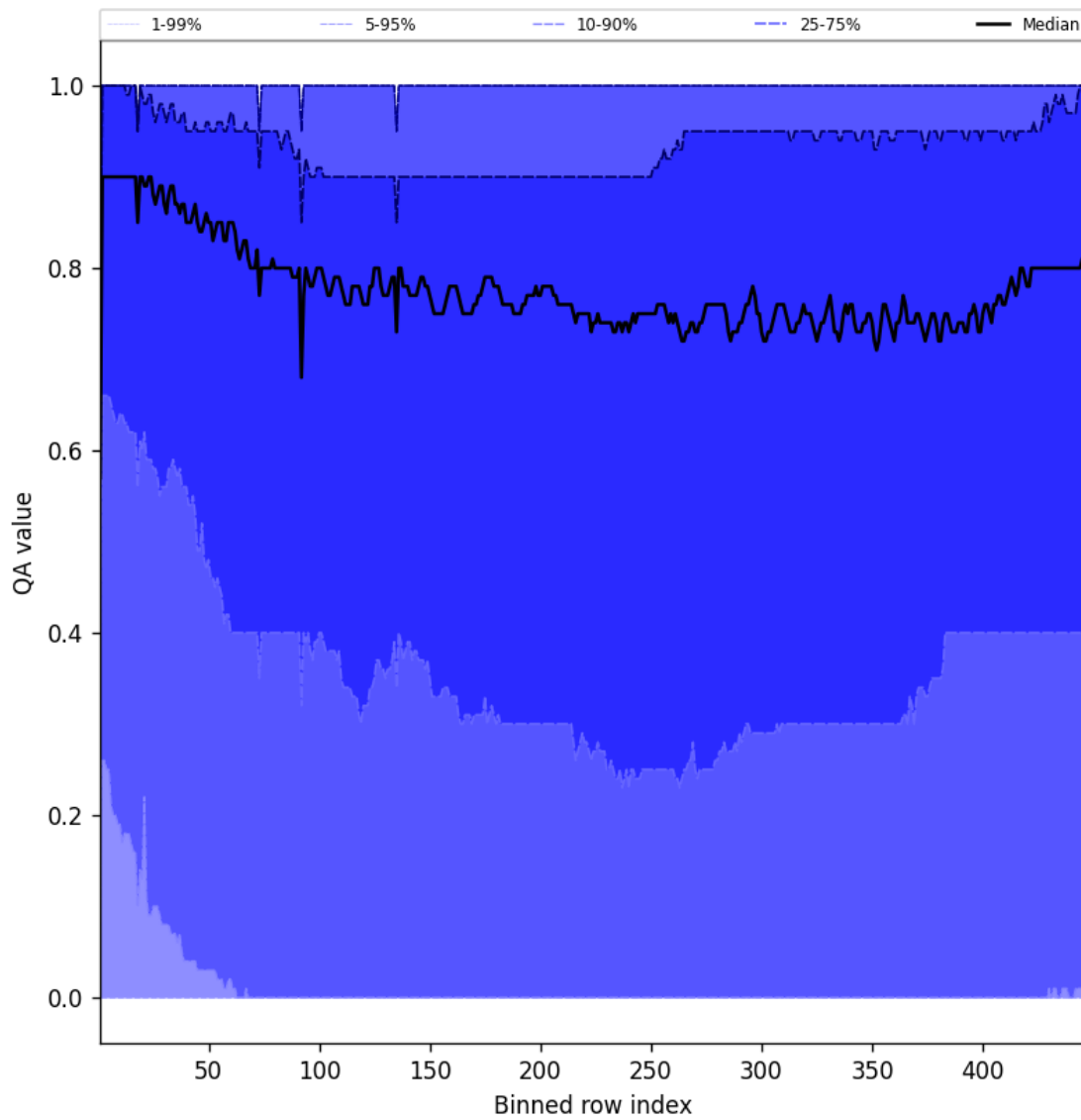
Figure 54: Along track statistics of “QA value” for 2025-06-04 to 2025-06-06
