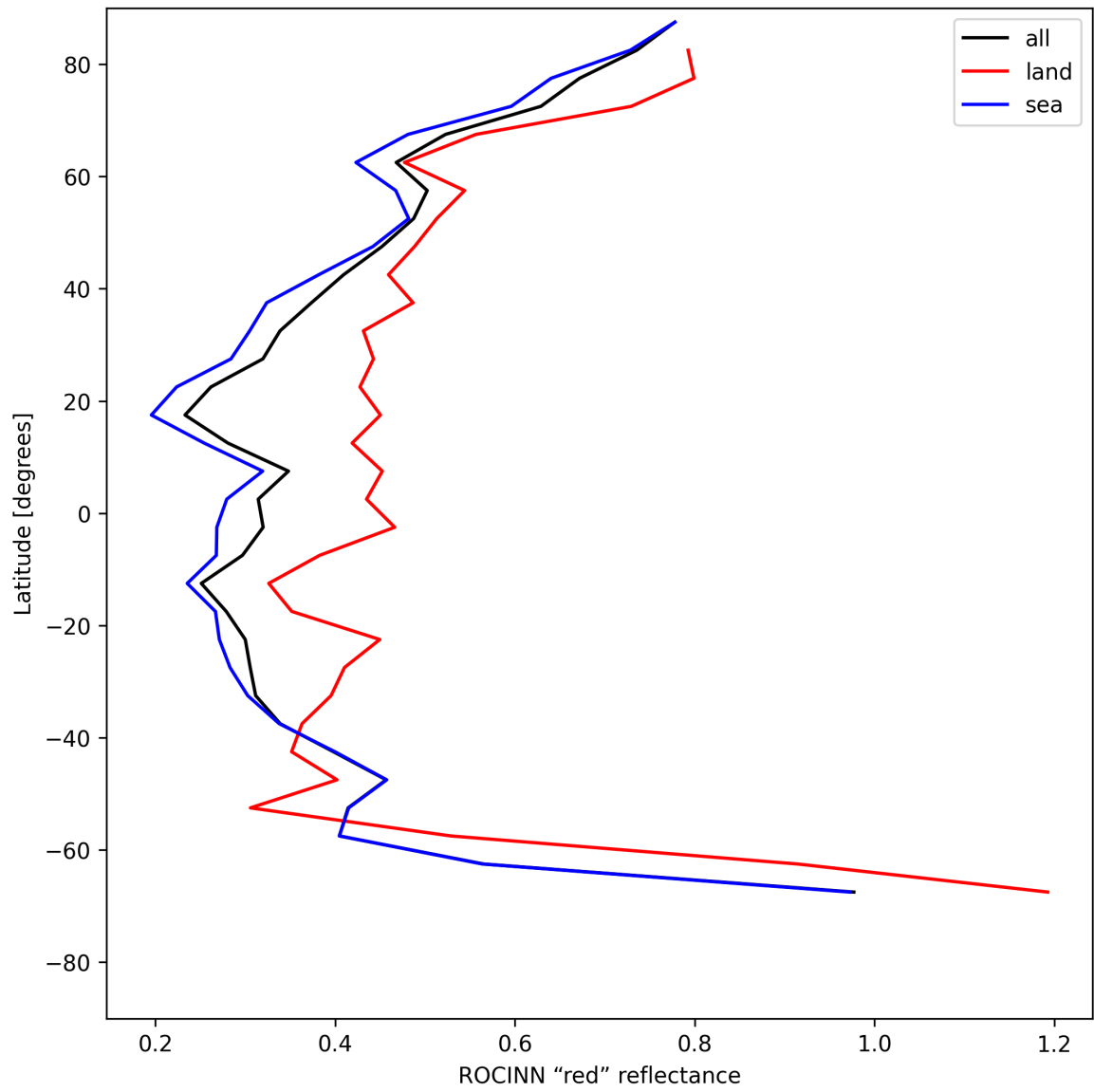
Figure 37: Zonal average of “ROCINN “red” reflectance” for 2025-06-04 to 2025-06-06.
