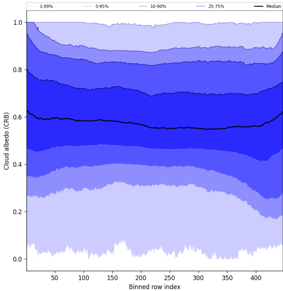
Figure 60: Along track statistics of “Cloud albedo (CRB)” for 2025-06-04 to 2025-06-06
