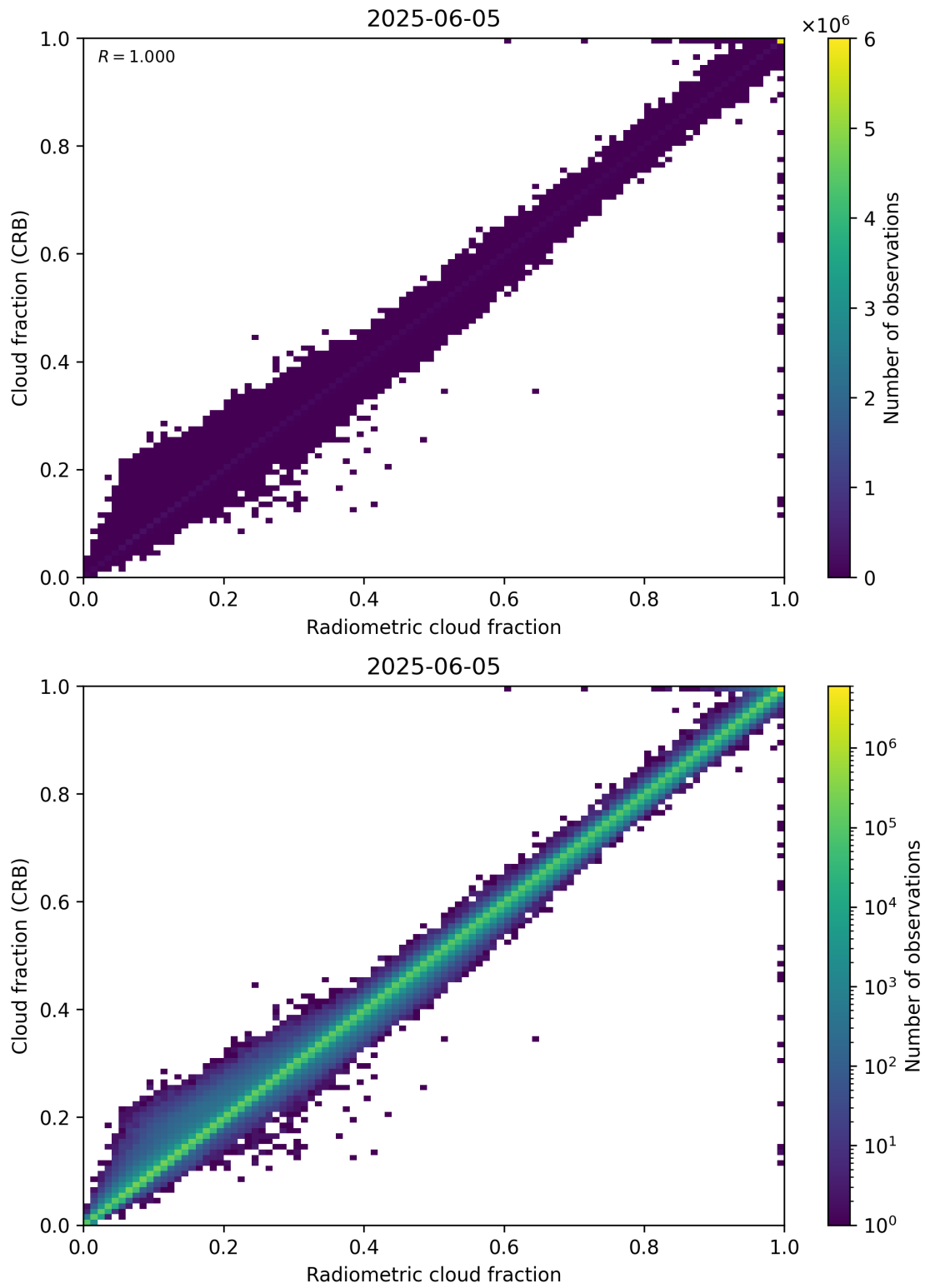
Figure 73: Scatter density plot of “Radiometric cloud fraction” against “Cloud fraction (CRB)” for 2025-06-04 to 2025-06-06.
