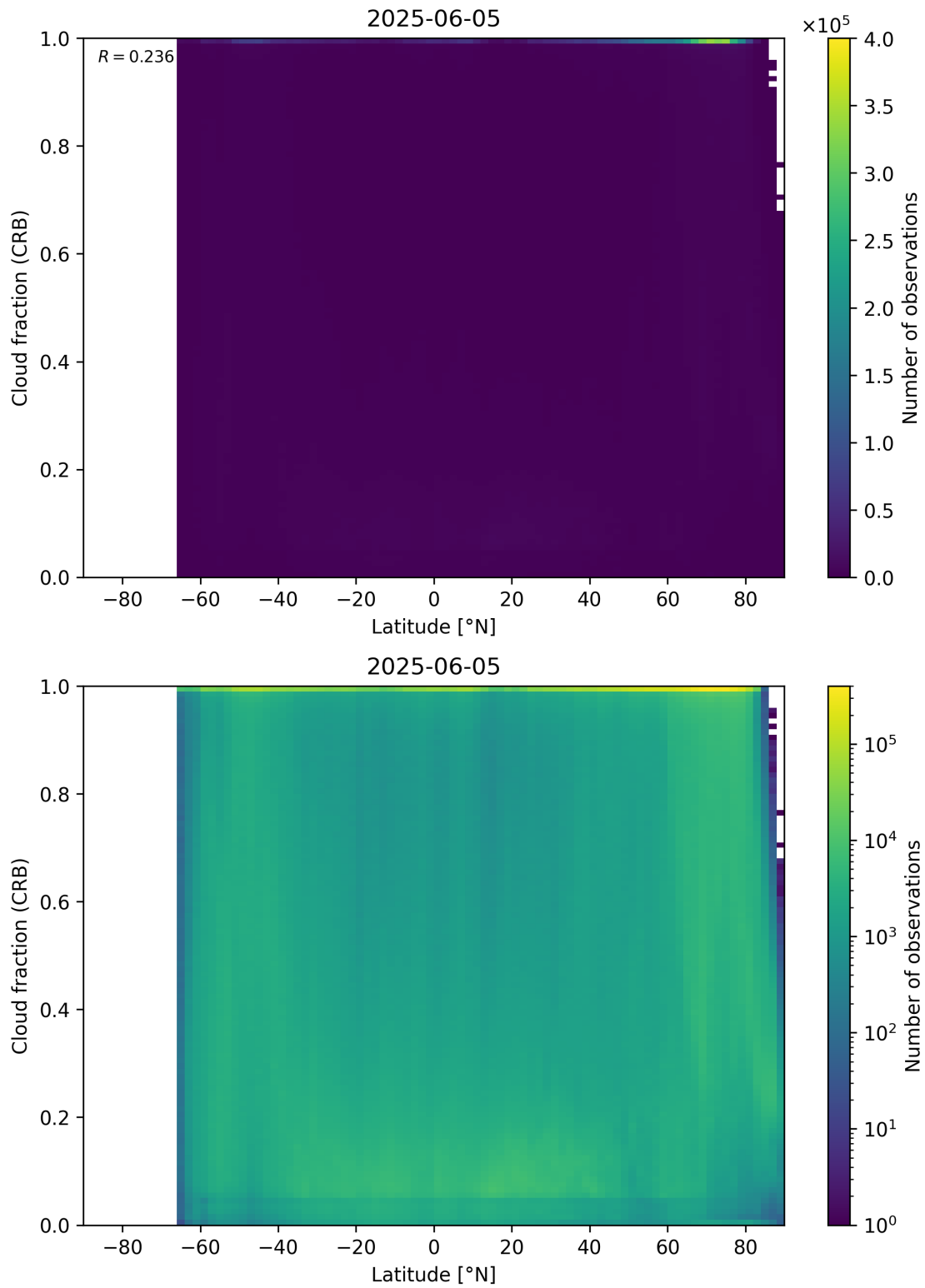
Figure 94: Scatter density plot of “Latitude” against “Cloud fraction (CRB)” for 2025-06-04 to 2025-06-06.
