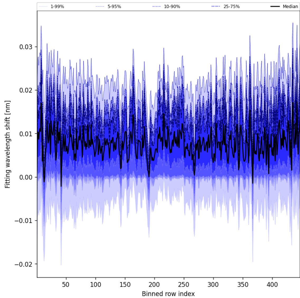
Figure 65: Along track statistics of “Fitting wavelength shift” for 2025-06-04 to 2025-06-06
