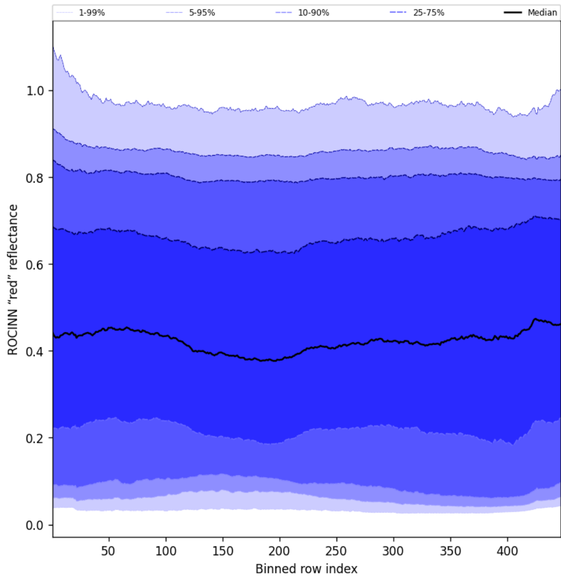
Figure 69: Along track statistics of "ROCINN "red" reflectance" for 2025-06-04 to 2025-06-06
