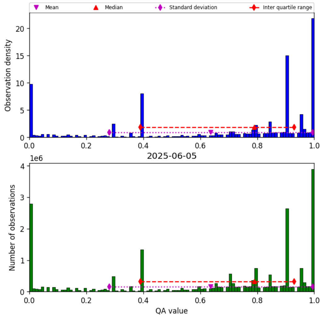
Figure 38: Histogram of “QA value” for 2025-06-04 to 2025-06-06
