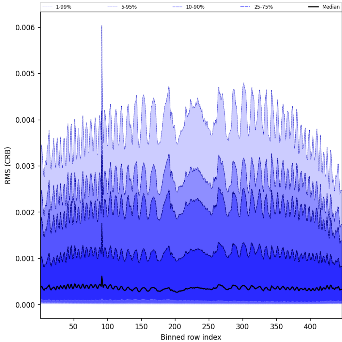
Figure 64: Along track statistics of “RMS (CRB)” for 2025-06-04 to 2025-06-06
