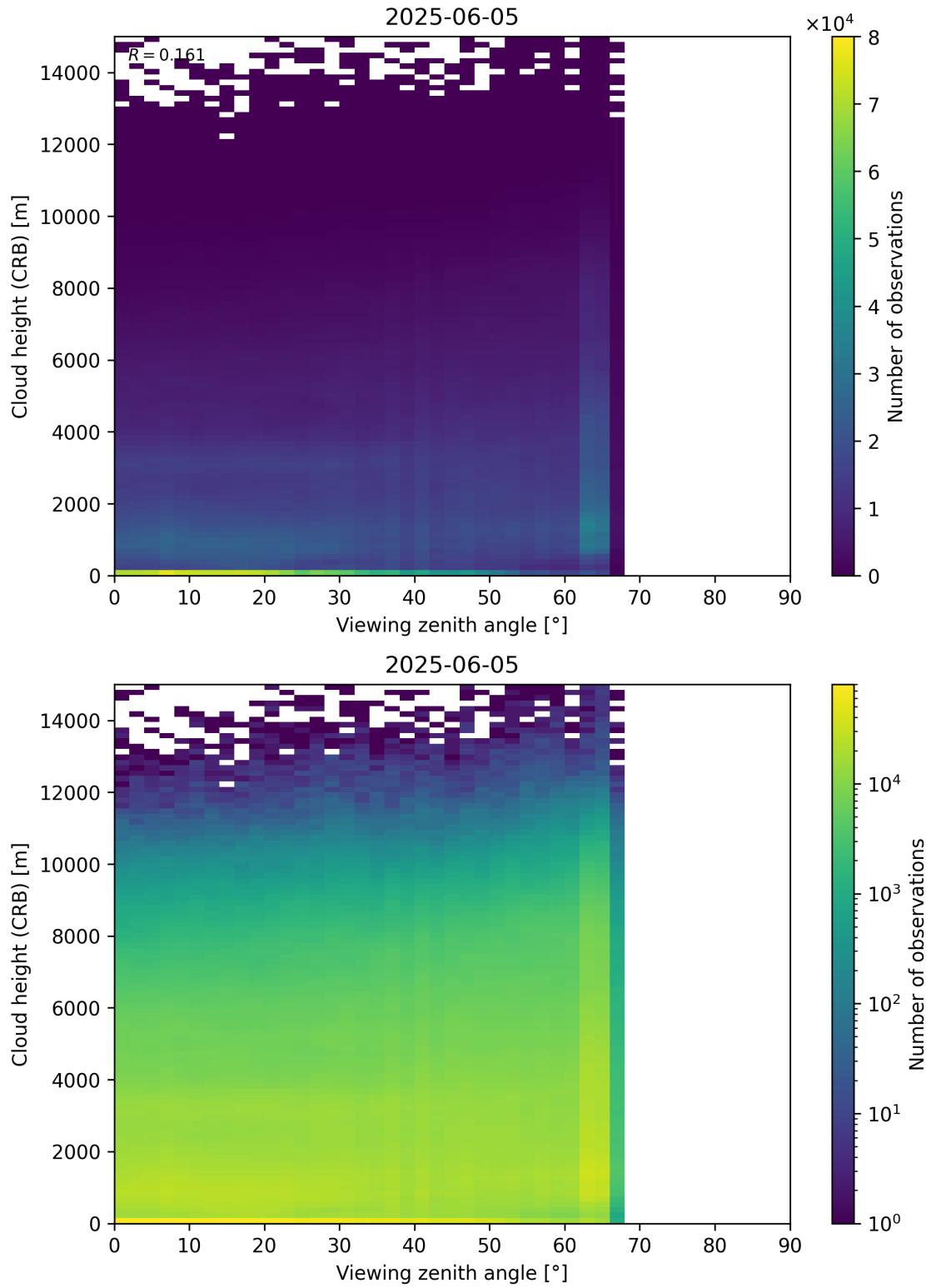
Figure 110: Scatter density plot of “Viewing zenith angle” against “Cloud height (CRB)” for 2025-06-04 to 2025-06-06.
