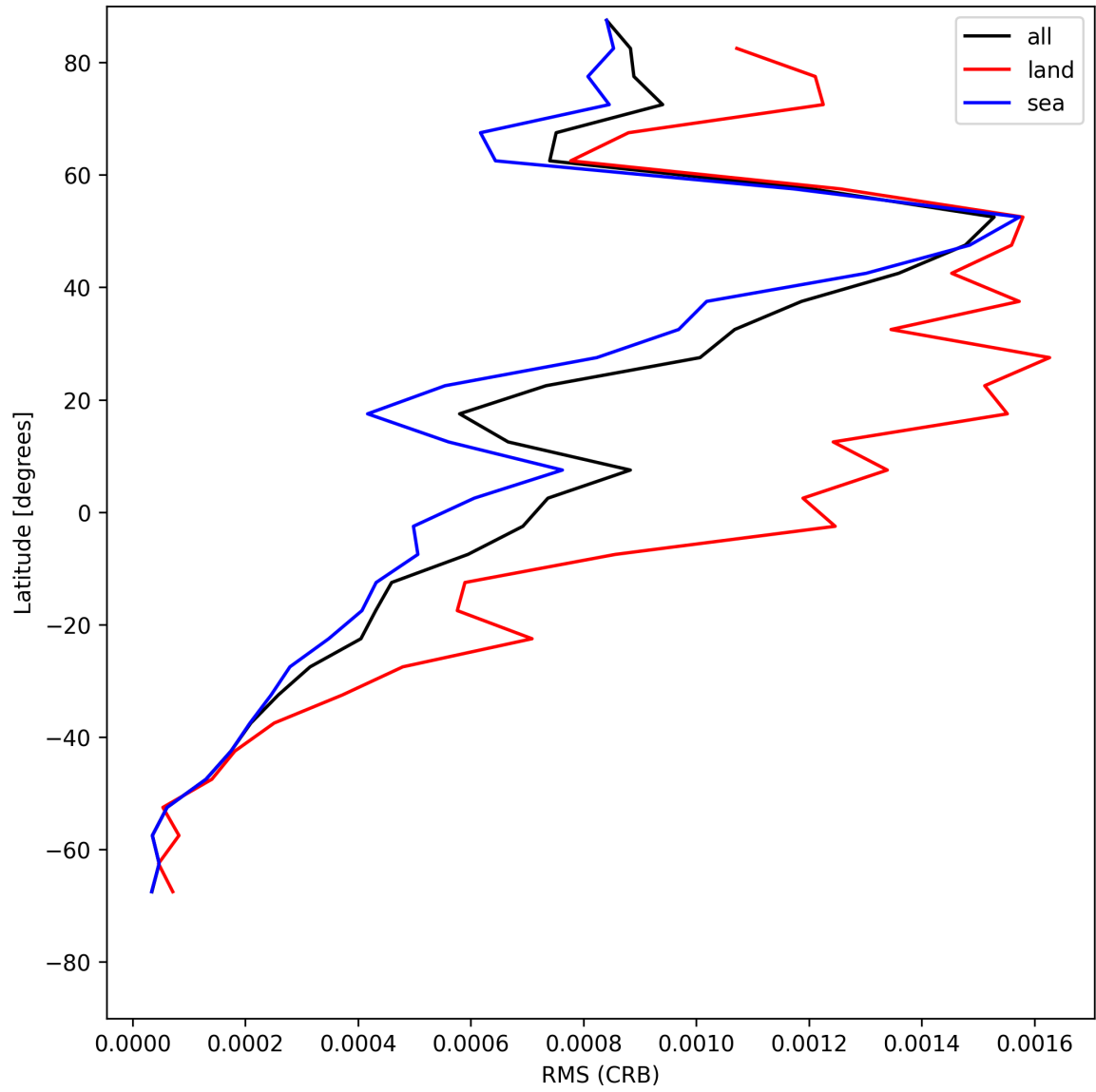
Figure 32: Zonal average of “RMS (CRB)” for 2025-06-04 to 2025-06-06.
