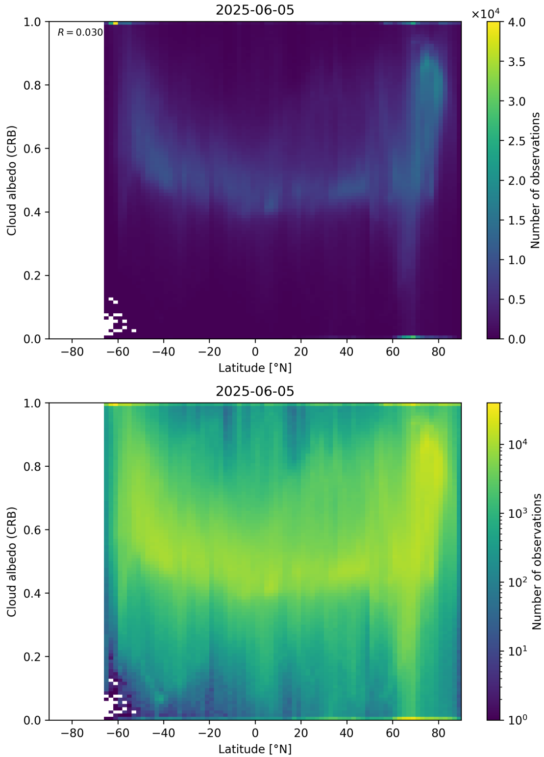
Figure 91: Scatter density plot of “Latitude” against “Cloud albedo (CRB)” for 2025-06-04 to 2025-06-06.
