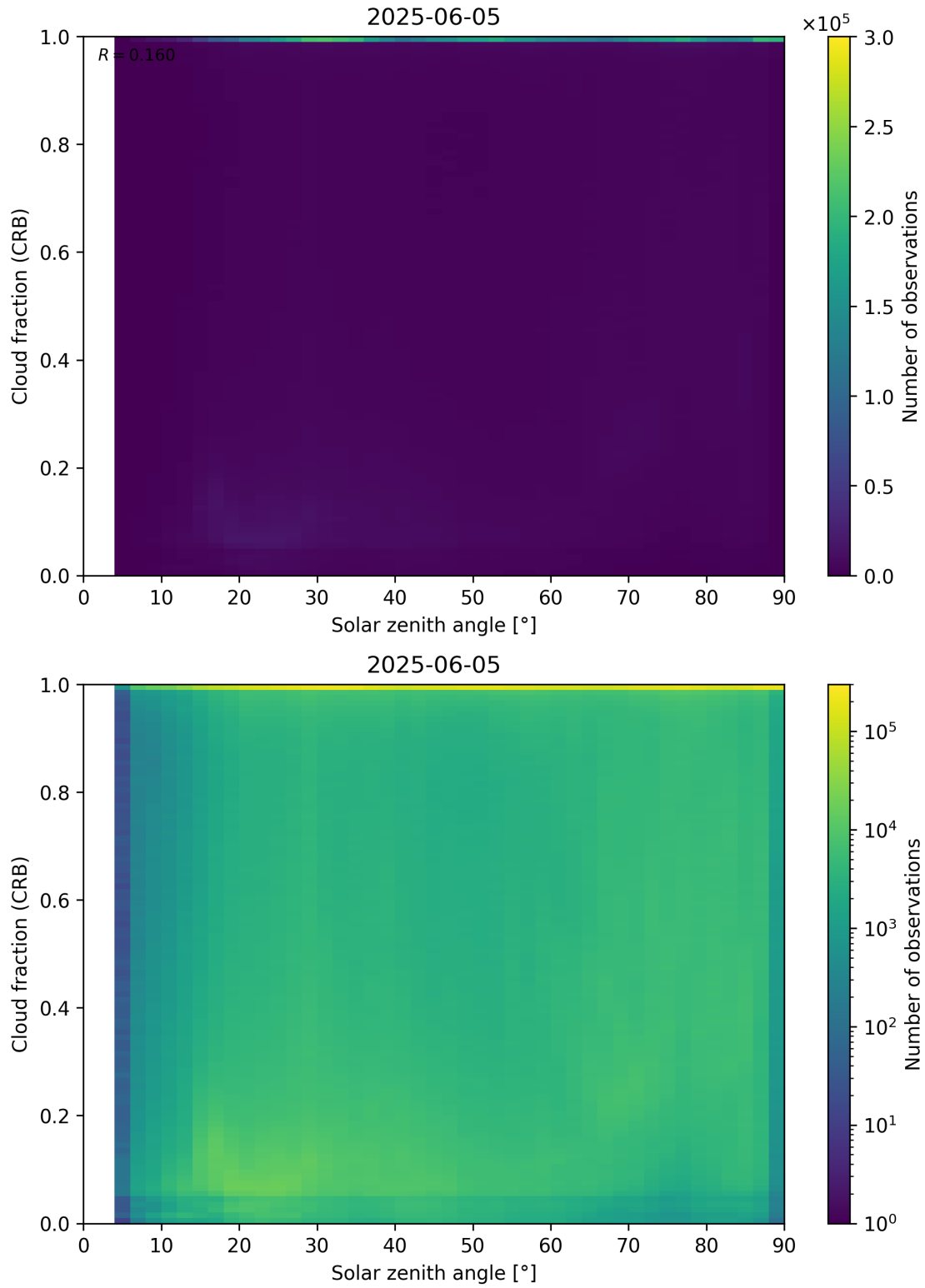
Figure 101: Scatter density plot of “Solar zenith angle” against “Cloud fraction (CRB)” for 2025-06-04 to 2025-06-06.
