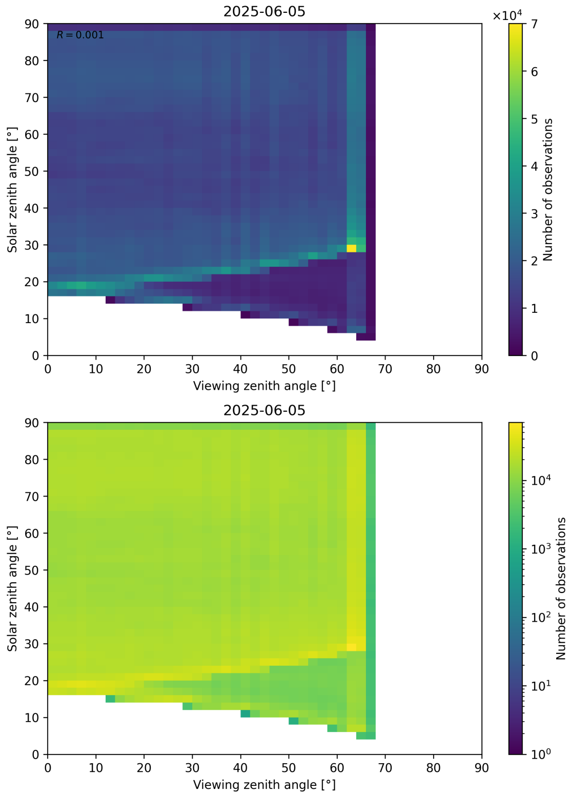
Figure 114: Scatter density plot of “Viewing zenith angle” against “Solar zenith angle” for 2025-06-04 to 2025-06-06.
