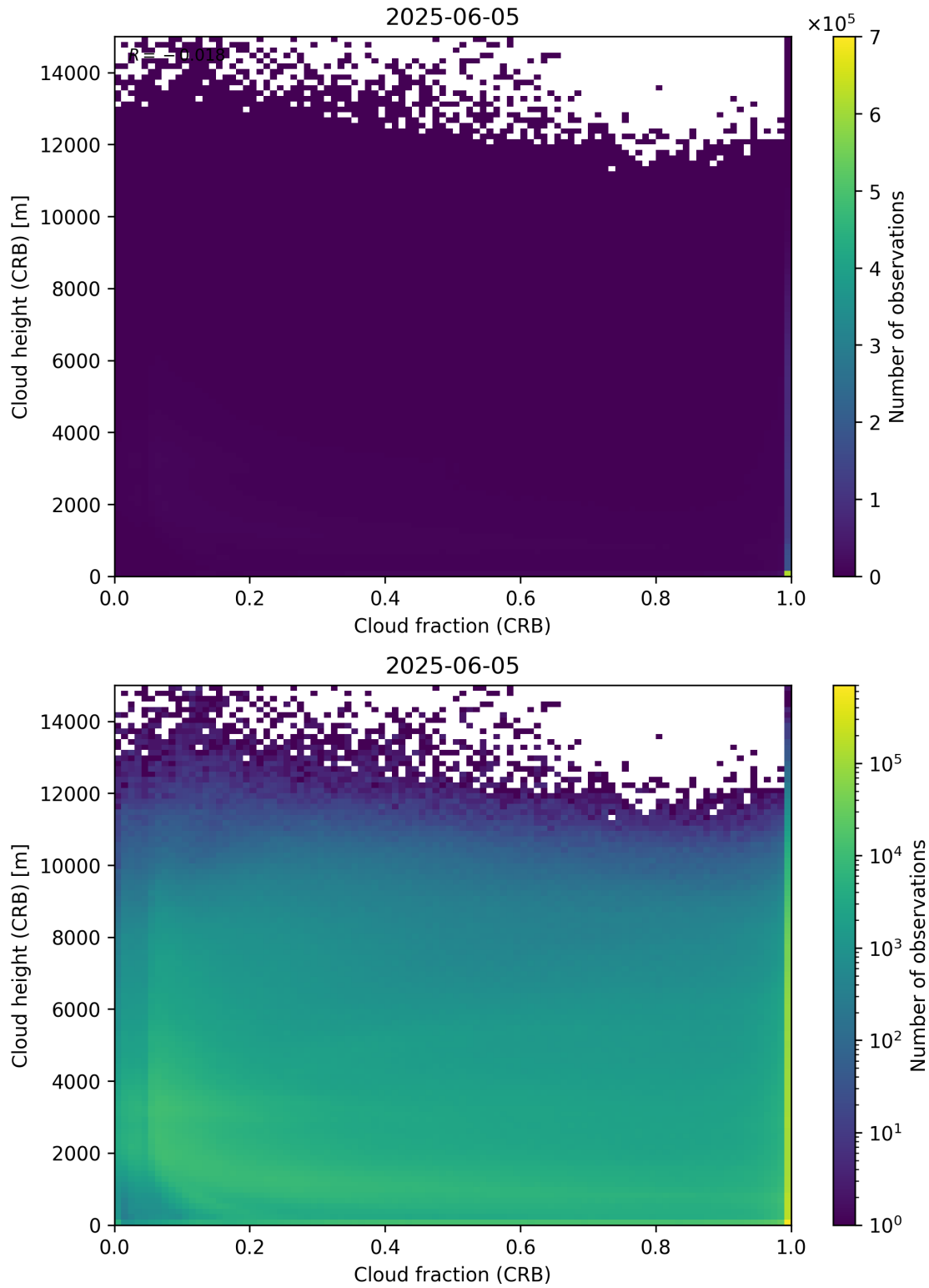
Figure 79: Scatter density plot of “Cloud fraction (CRB)” against “Cloud height (CRB)” for 2025-06-04 to 2025-06-06.
