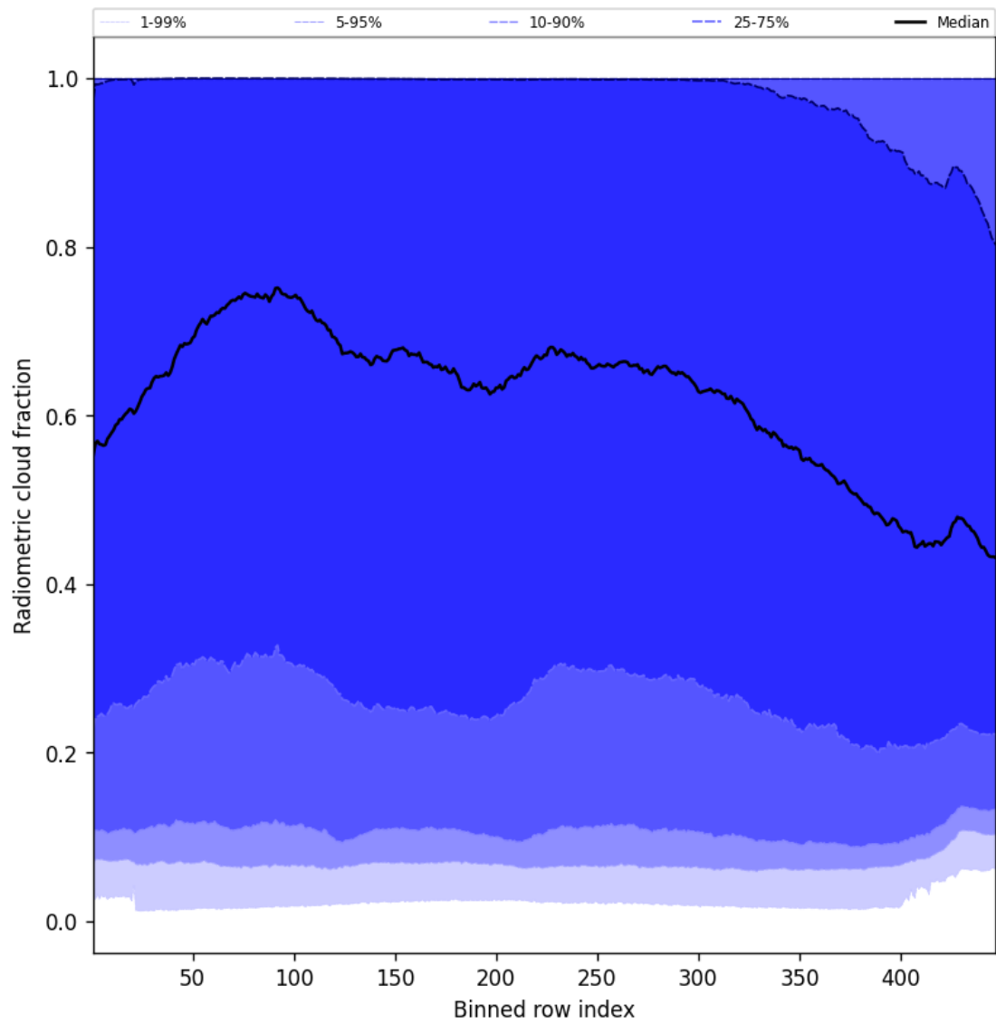
Figure 55: Along track statistics of “Radiometric cloud fraction” for 2025-06-04 to 2025-06-06
