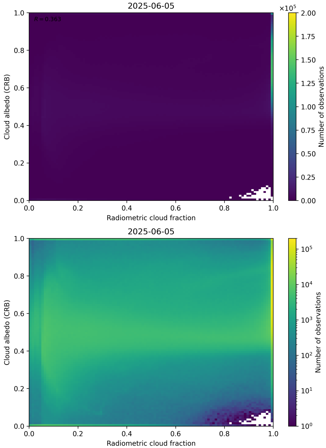
Figure 71: Scatter density plot of “Radiometric cloud fraction” against “Cloud albedo (CRB)” for 2025-06-04 to 2025-06-06.
