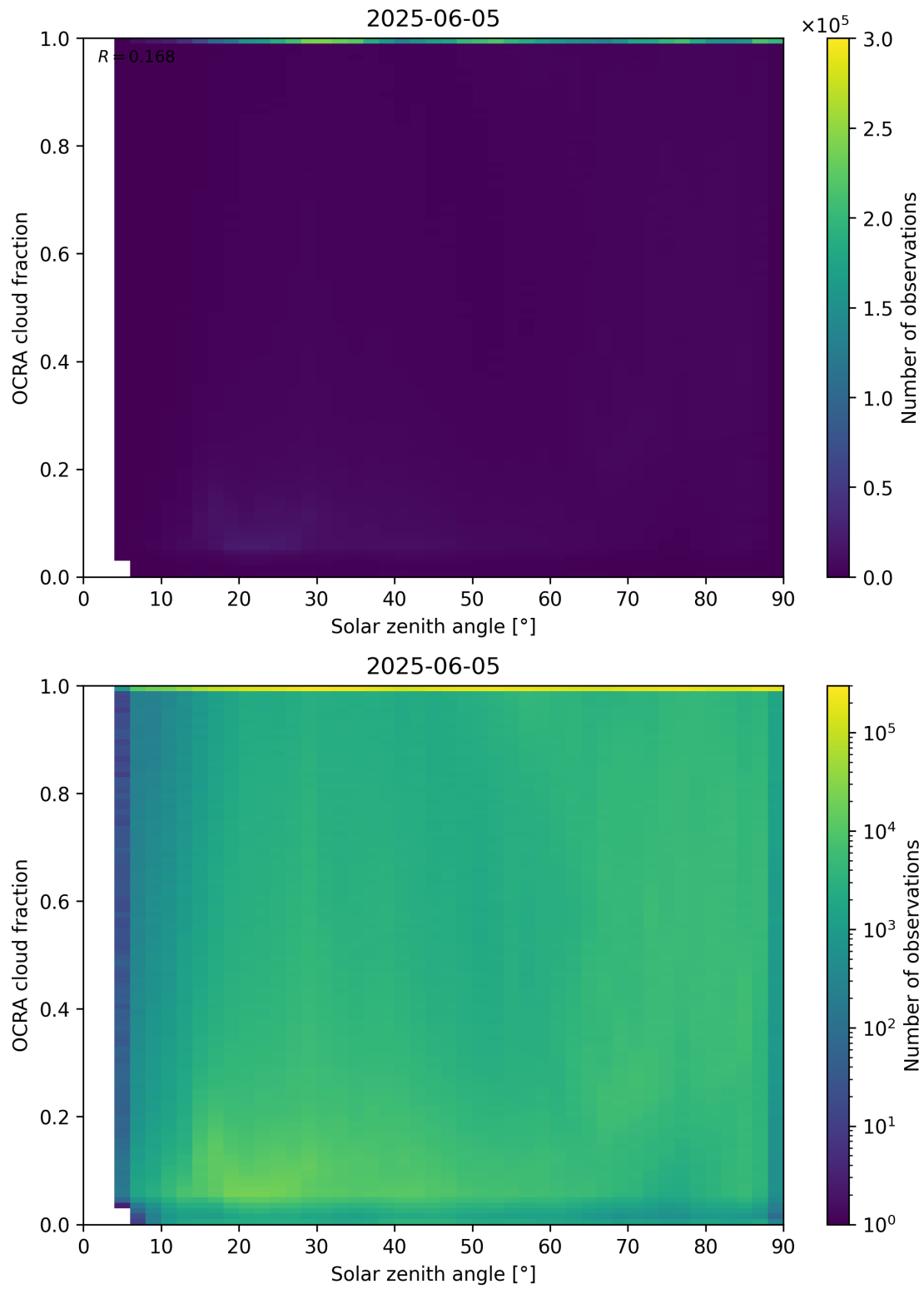
Figure 100: Scatter density plot of “Solar zenith angle” against “OCRA cloud fraction” for 2025-06-04 to 2025-06-06.
