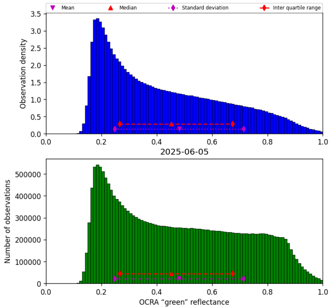
Figure 52: Histogram of “OCRA “green” reflectance” for 2025-06-04 to 2025-06-06
