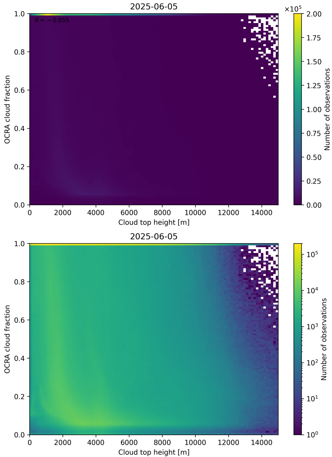
Figure 87: Scatter density plot of “Cloud top height” against “OCRA cloud fraction” for 2025-06-04 to 2025-06-06.
