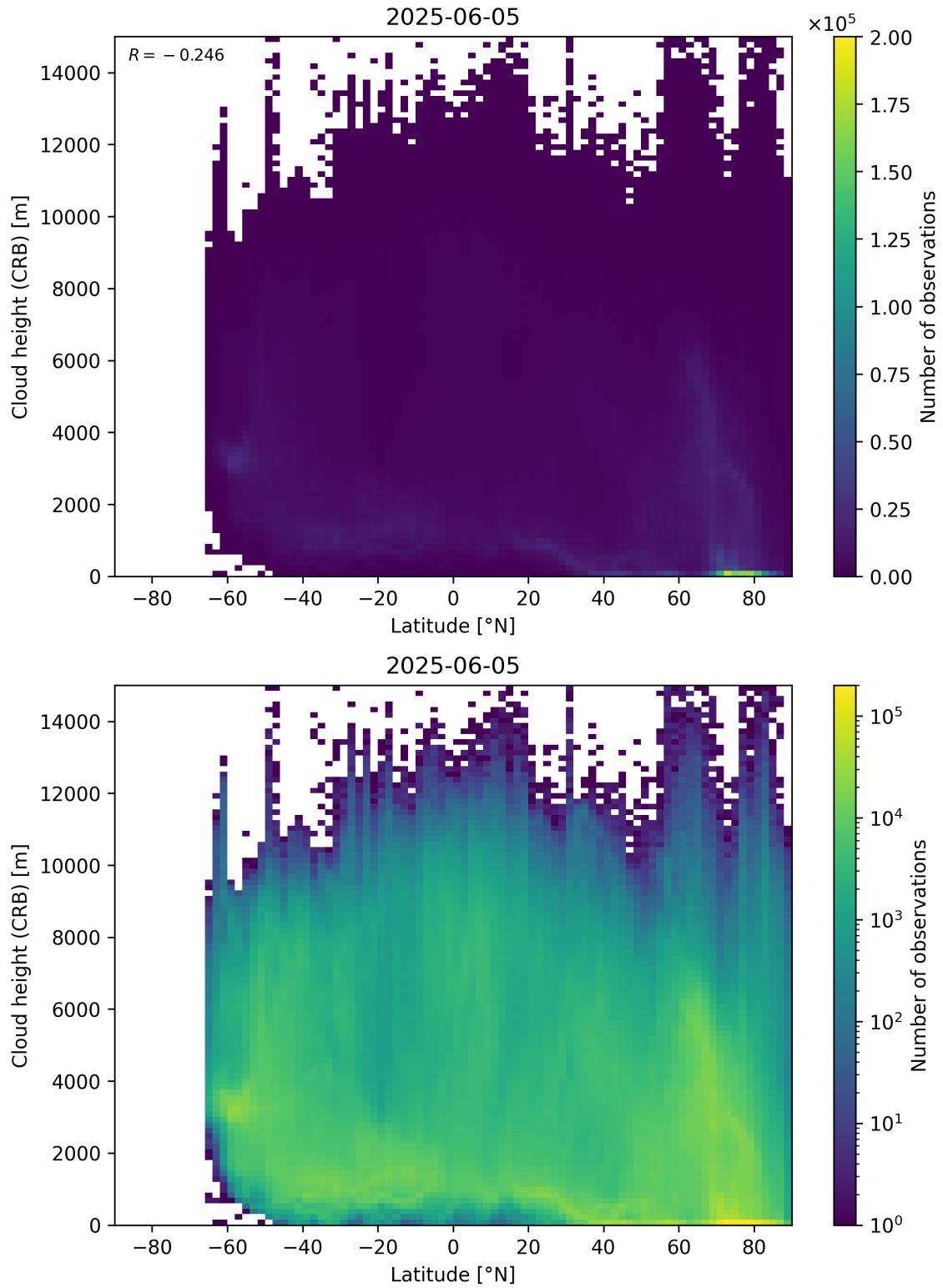
Figure 95: Scatter density plot of “Latitude” against “Cloud height (CRB)” for 2025-06-04 to 2025-06-06.
