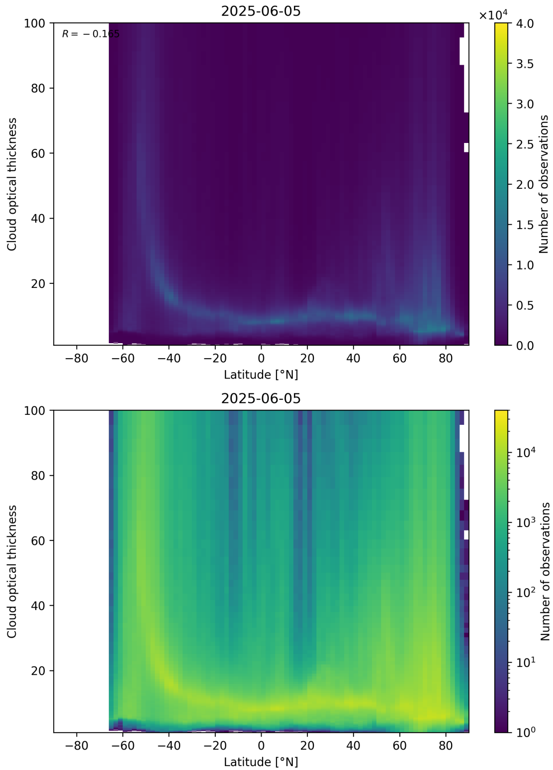
Figure 96: Scatter density plot of “Latitude” against “Cloud optical thickness” for 2025-06-04 to 2025-06-06.
