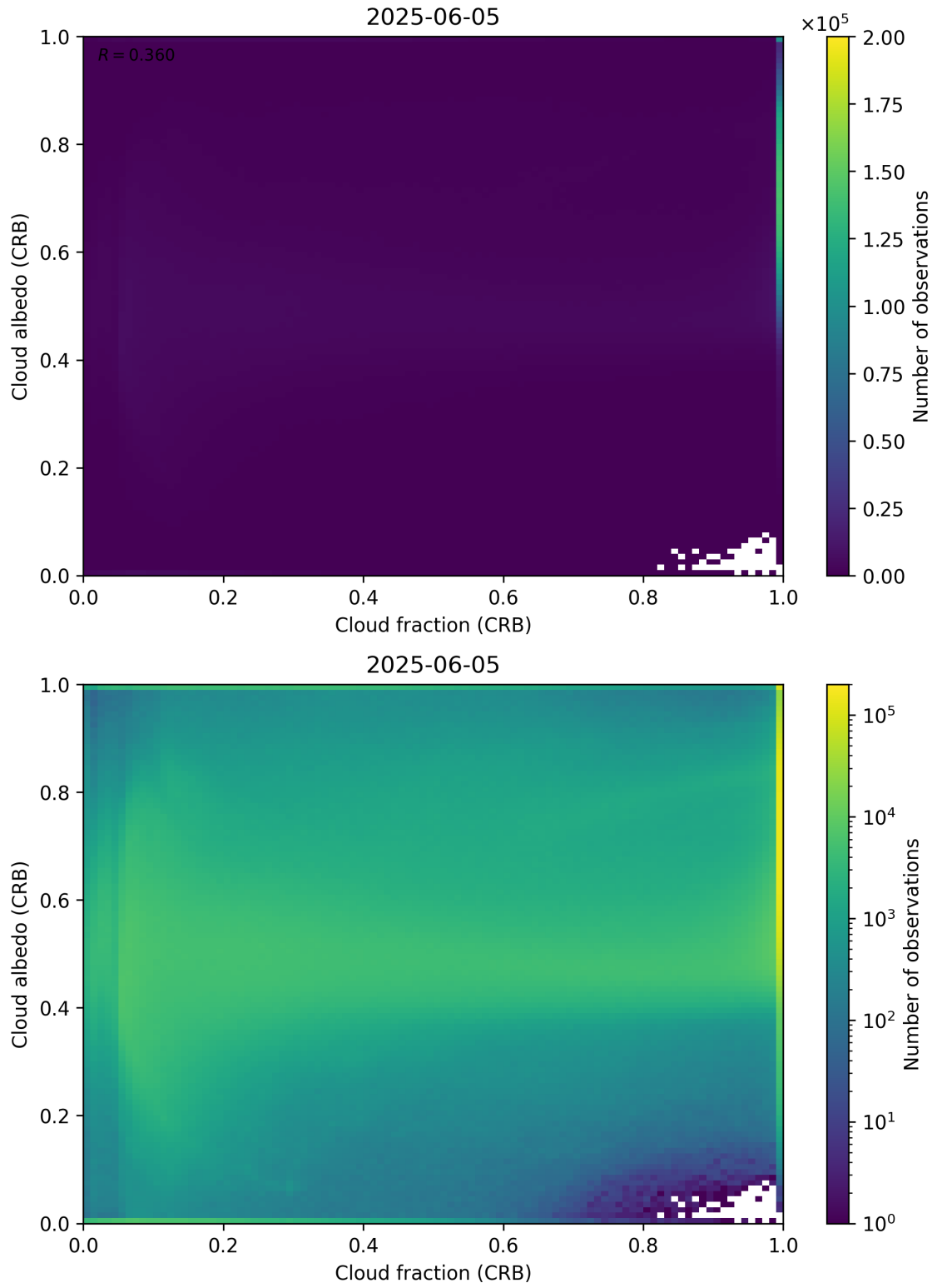
Figure 77: Scatter density plot of “Cloud fraction (CRB)” against “Cloud albedo (CRB)” for 2025-06-04 to 2025-06-06.
