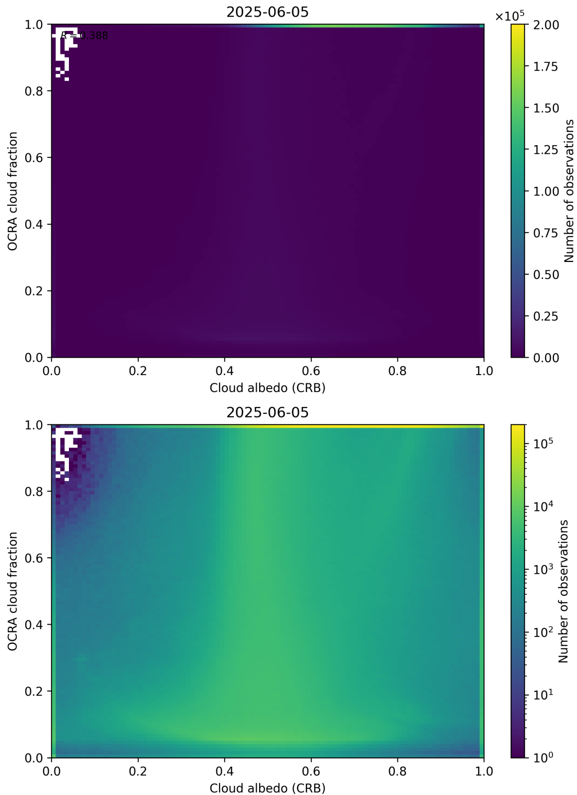
Figure 70: Scatter density plot of “Cloud albedo (CRB)” against “OCRA cloud fraction” for 2025-06-04 to 2025-06-06.
