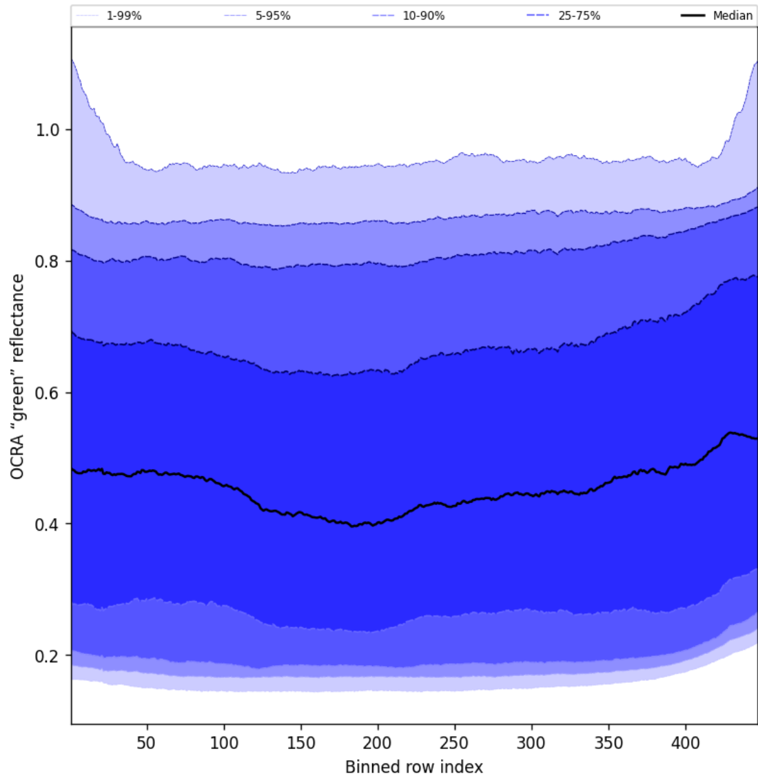
Figure 68: Along track statistics of "OCRA "green" reflectance" for 2025-06-04 to 2025-06-06
