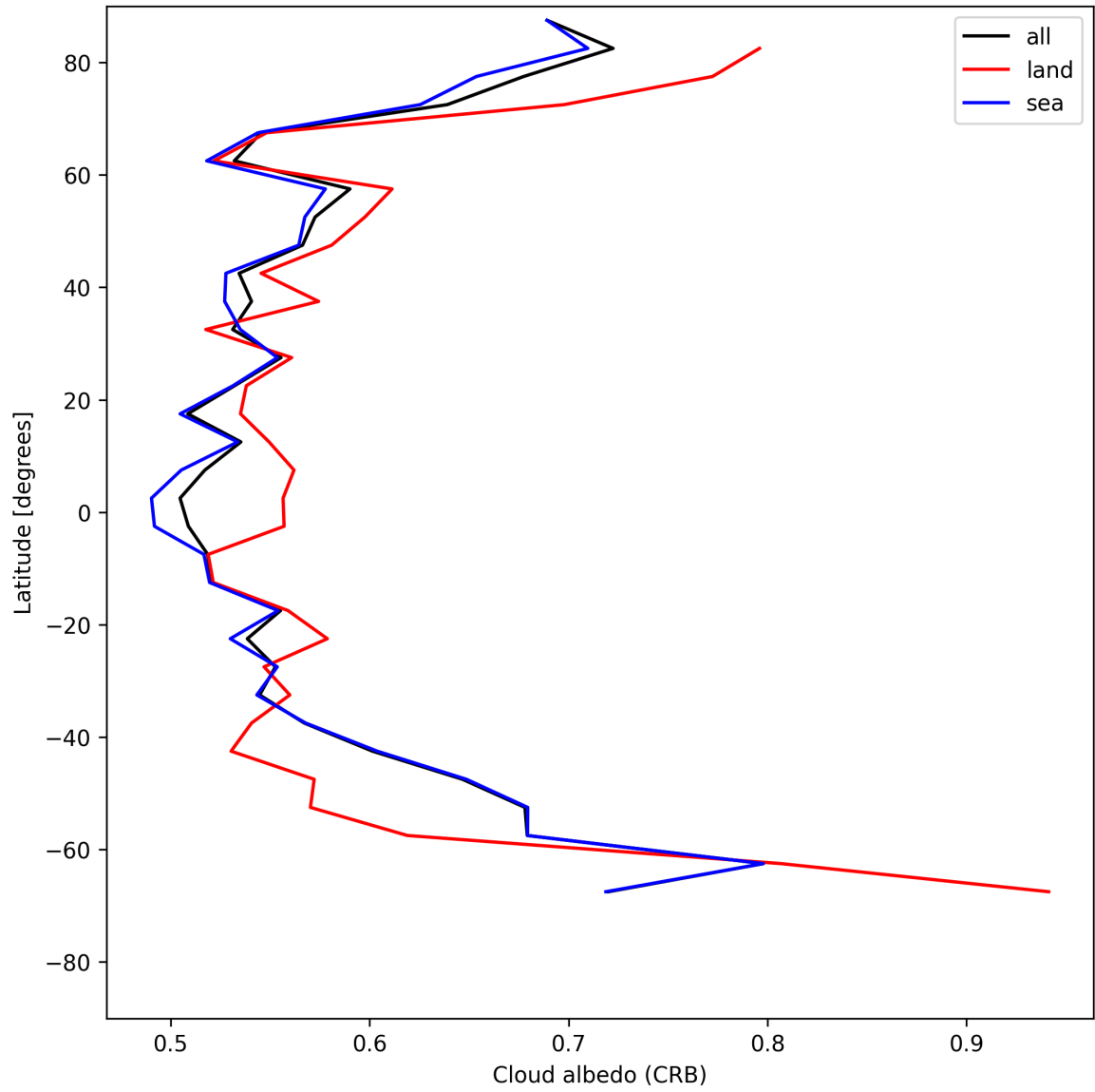
Figure 28: Zonal average of “Cloud albedo (CRB)” for 2025-06-04 to 2025-06-06.
