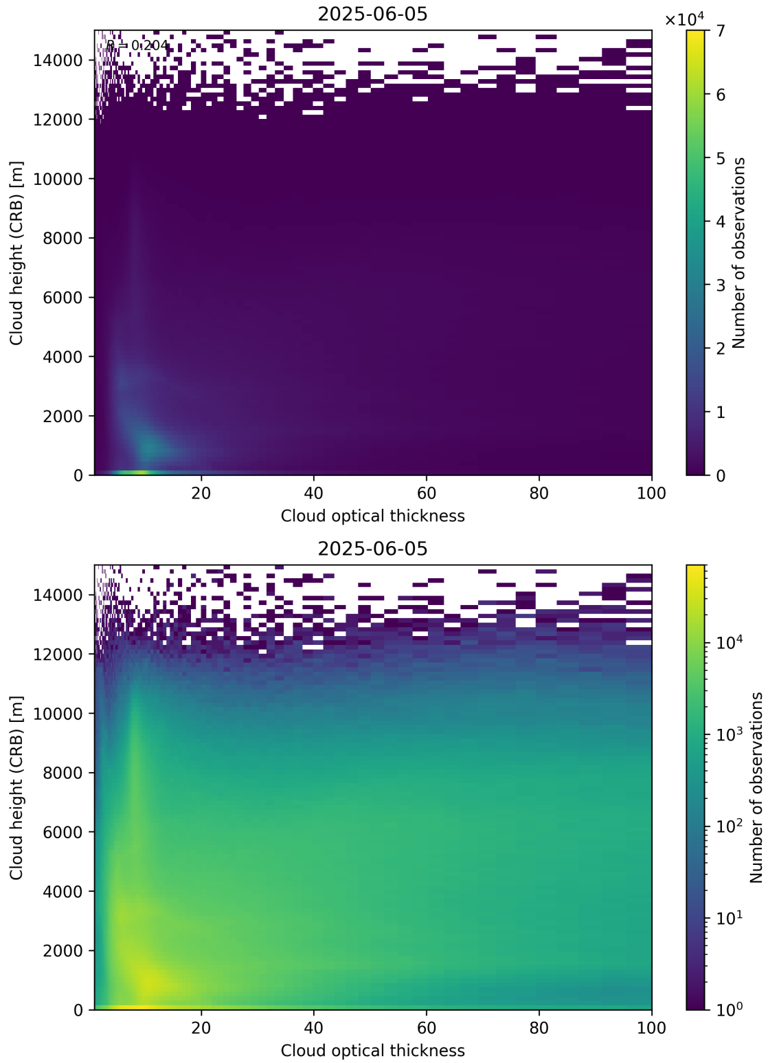
Figure 85: Scatter density plot of “Cloud optical thickness” against “Cloud height (CRB)” for 2025-06-04 to 2025-06-06.
