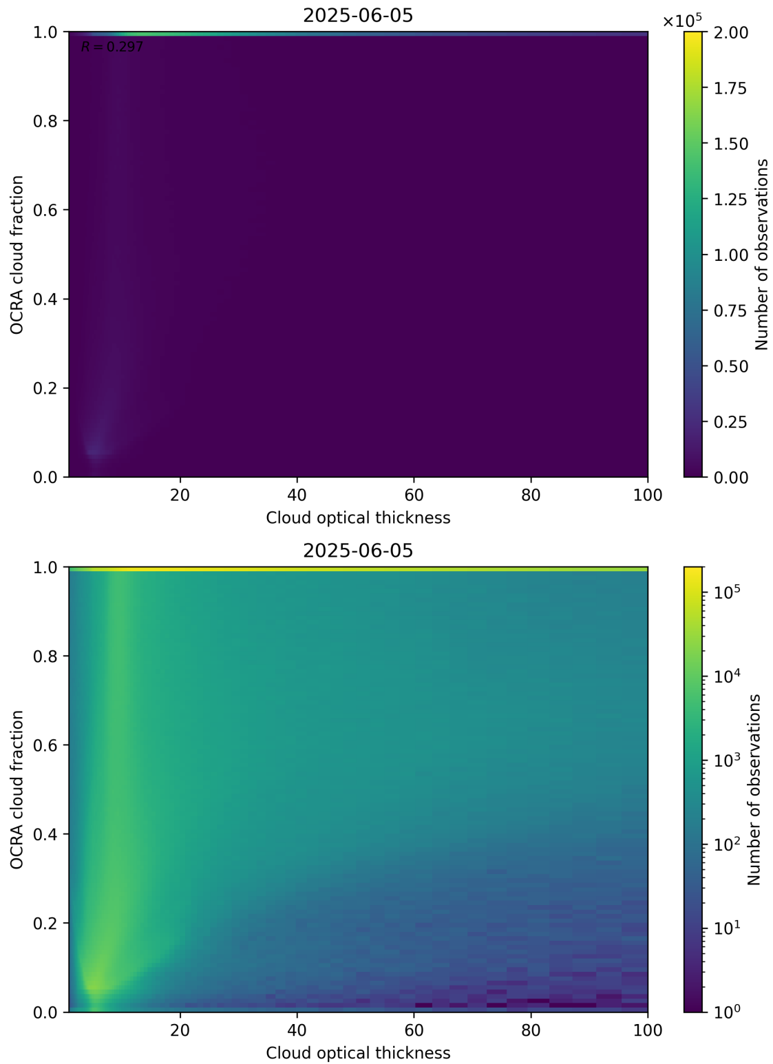
Figure 83: Scatter density plot of “Cloud optical thickness” against “OCRA cloud fraction” for 2025-06-04 to 2025-06-06.
