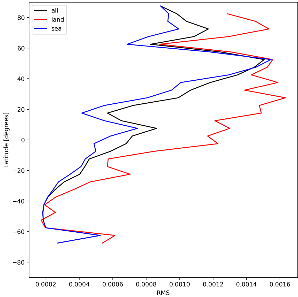
Figure 31: Zonal average of “RMS” for 2025-06-04 to 2025-06-06.
