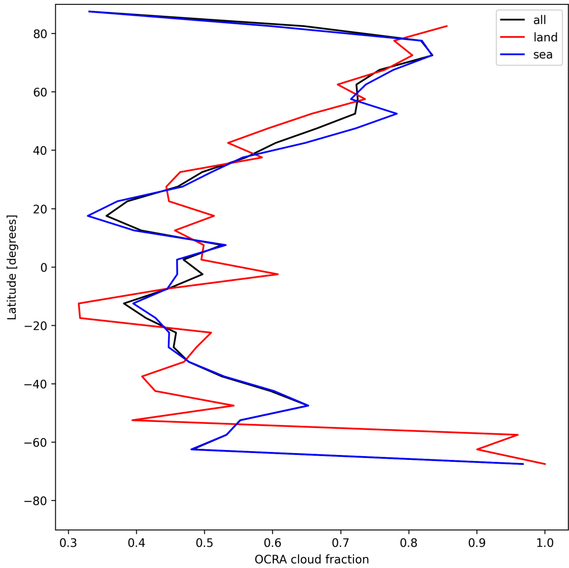
Figure 34: Zonal average of “OCRA cloud fraction” for 2025-06-04 to 2025-06-06.
