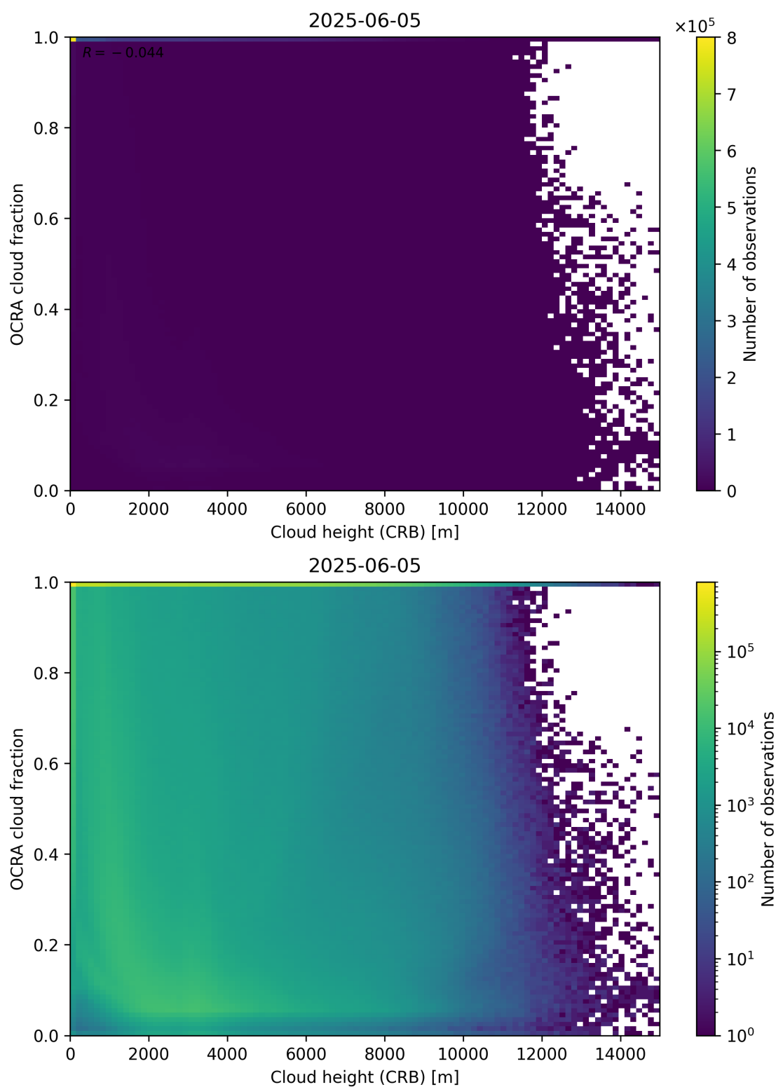
Figure 81: Scatter density plot of “Cloud height (CRB)” against “OCRA cloud fraction” for 2025-06-04 to 2025-06-06.
