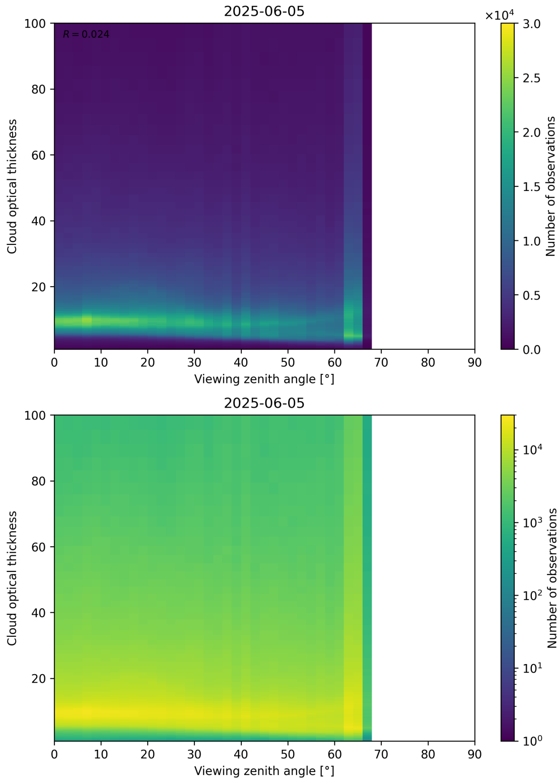
Figure 111: Scatter density plot of “Viewing zenith angle” against “Cloud optical thickness” for 2025-06-04 to 2025-06-06.
