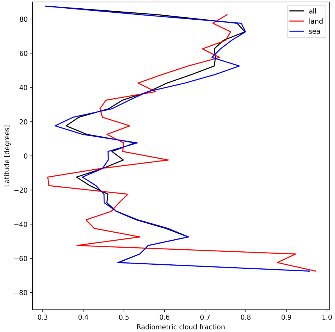
Figure 23: Zonal average of “Radiometric cloud fraction” for 2025-06-04 to 2025-06-06.
