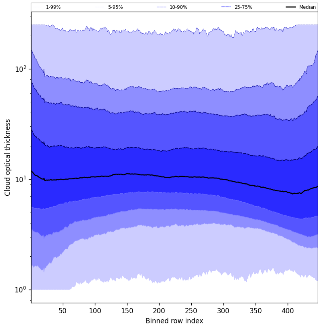
Figure 57: Along track statistics of “Cloud optical thickness” for 2025-06-04 to 2025-06-06
