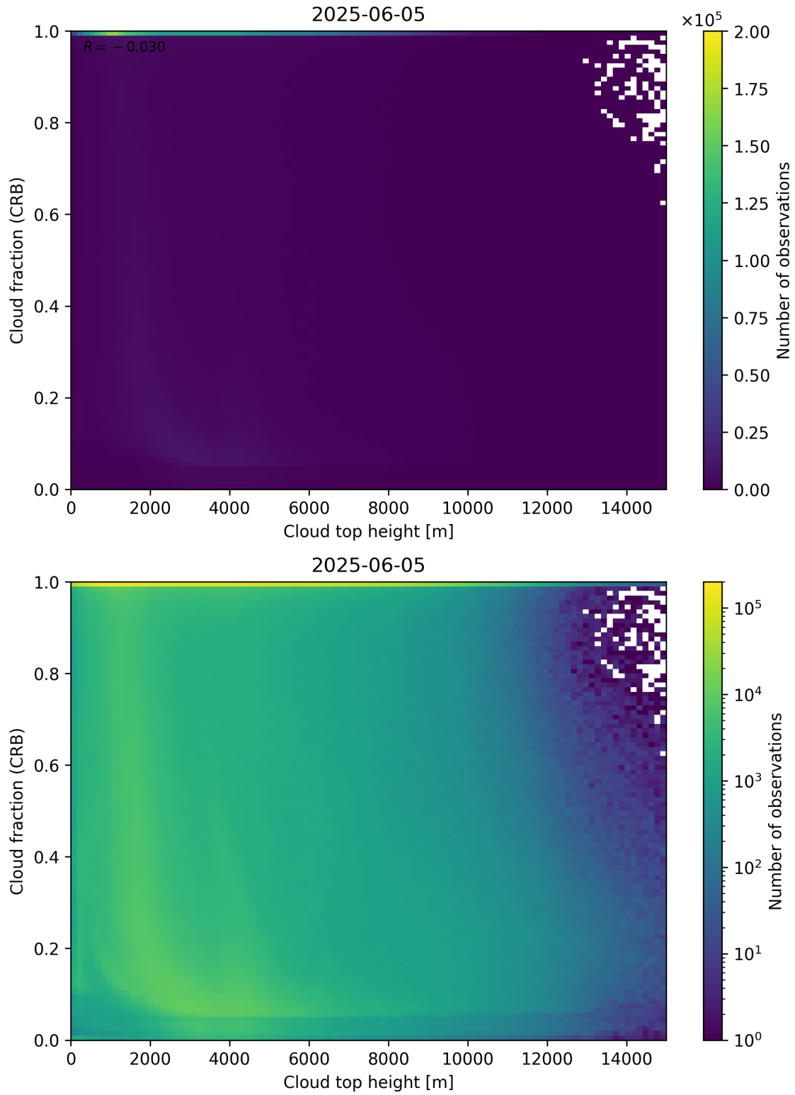
Figure 88: Scatter density plot of “Cloud top height” against “Cloud fraction (CRB)” for 2025-06-04 to 2025-06-06.
