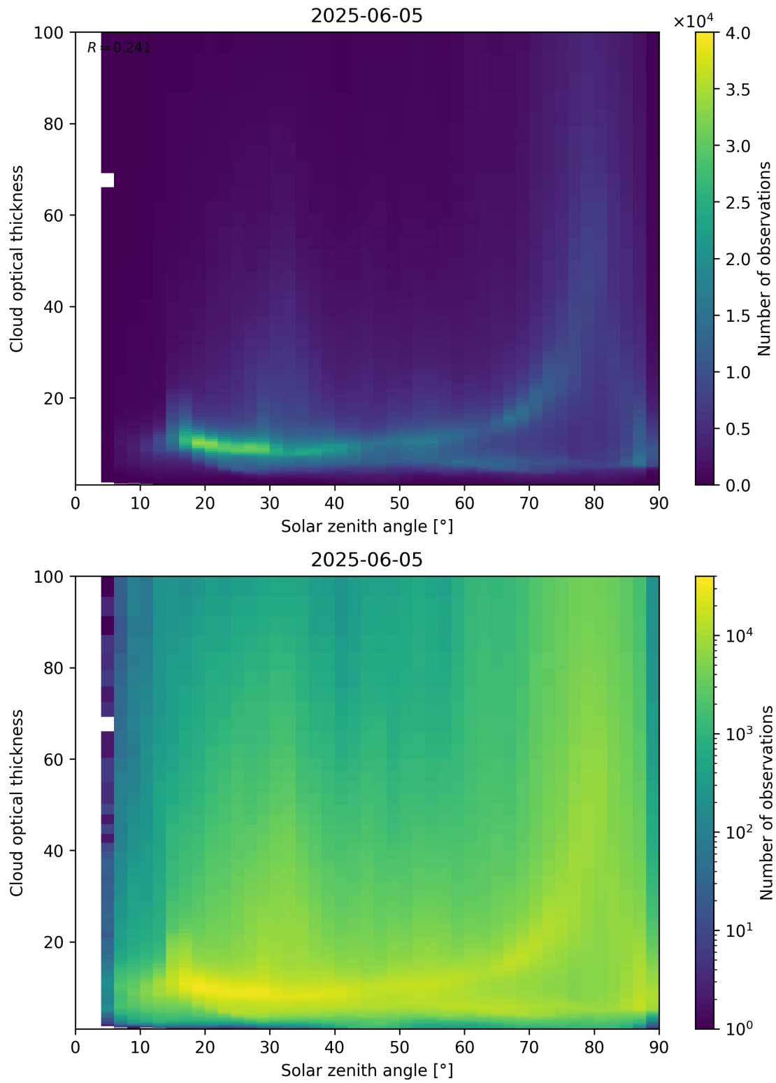
Figure 103: Scatter density plot of “Solar zenith angle” against “Cloud optical thickness” for 2025-06-04 to 2025-06-06.
