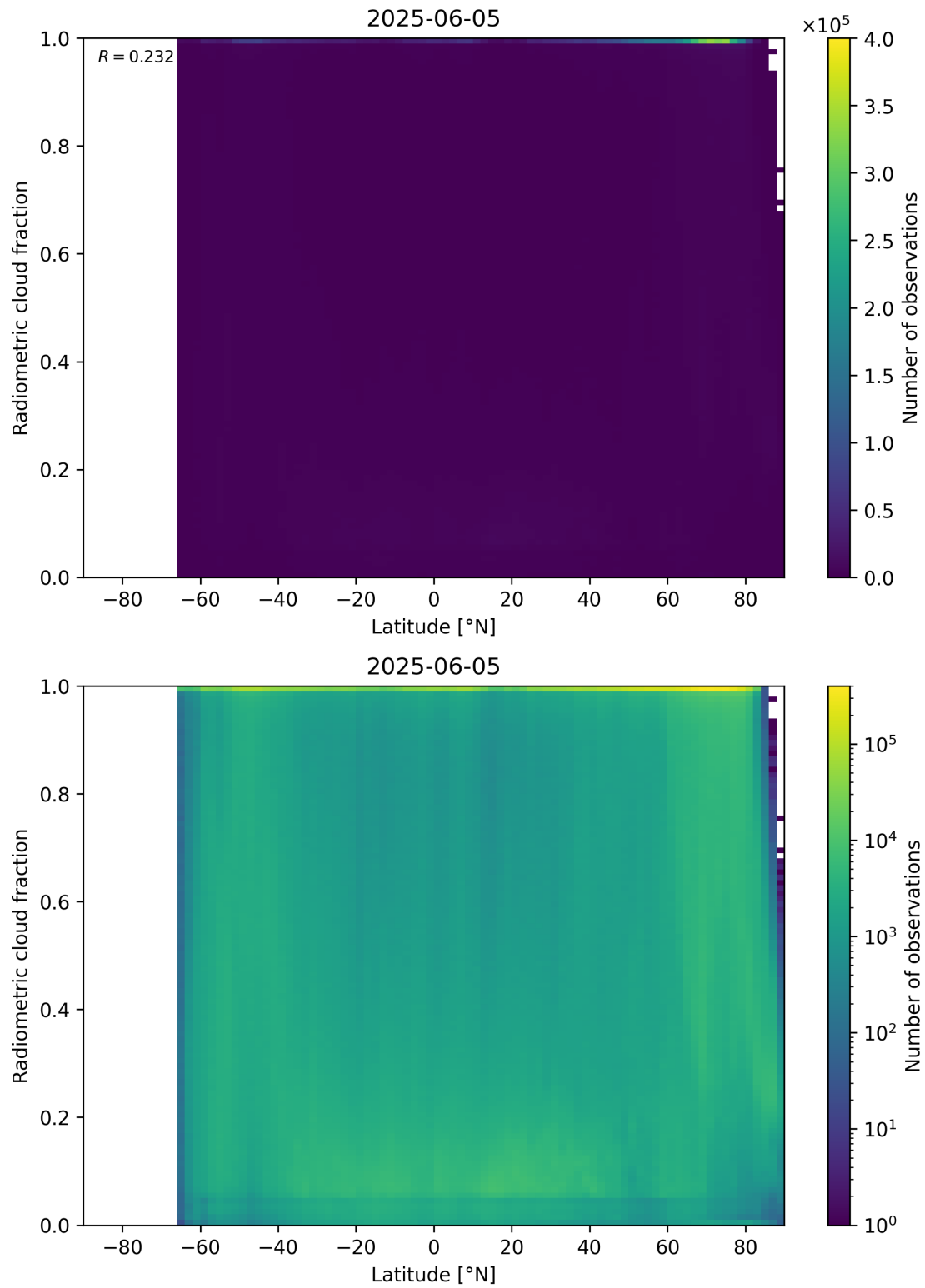
Figure 92: Scatter density plot of “Latitude” against “Radiometric cloud fraction” for 2025-06-04 to 2025-06-06.
