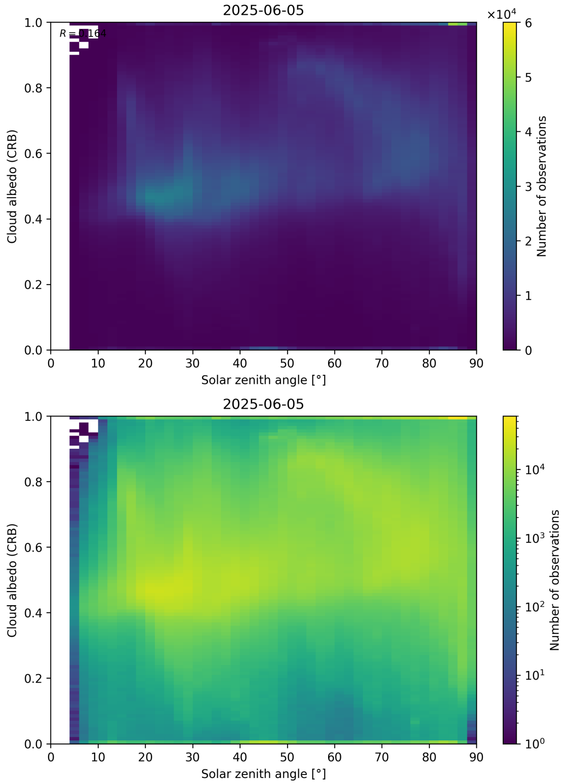
Figure 98: Scatter density plot of “Solar zenith angle” against “Cloud albedo (CRB)” for 2025-06-04 to 2025-06-06.
