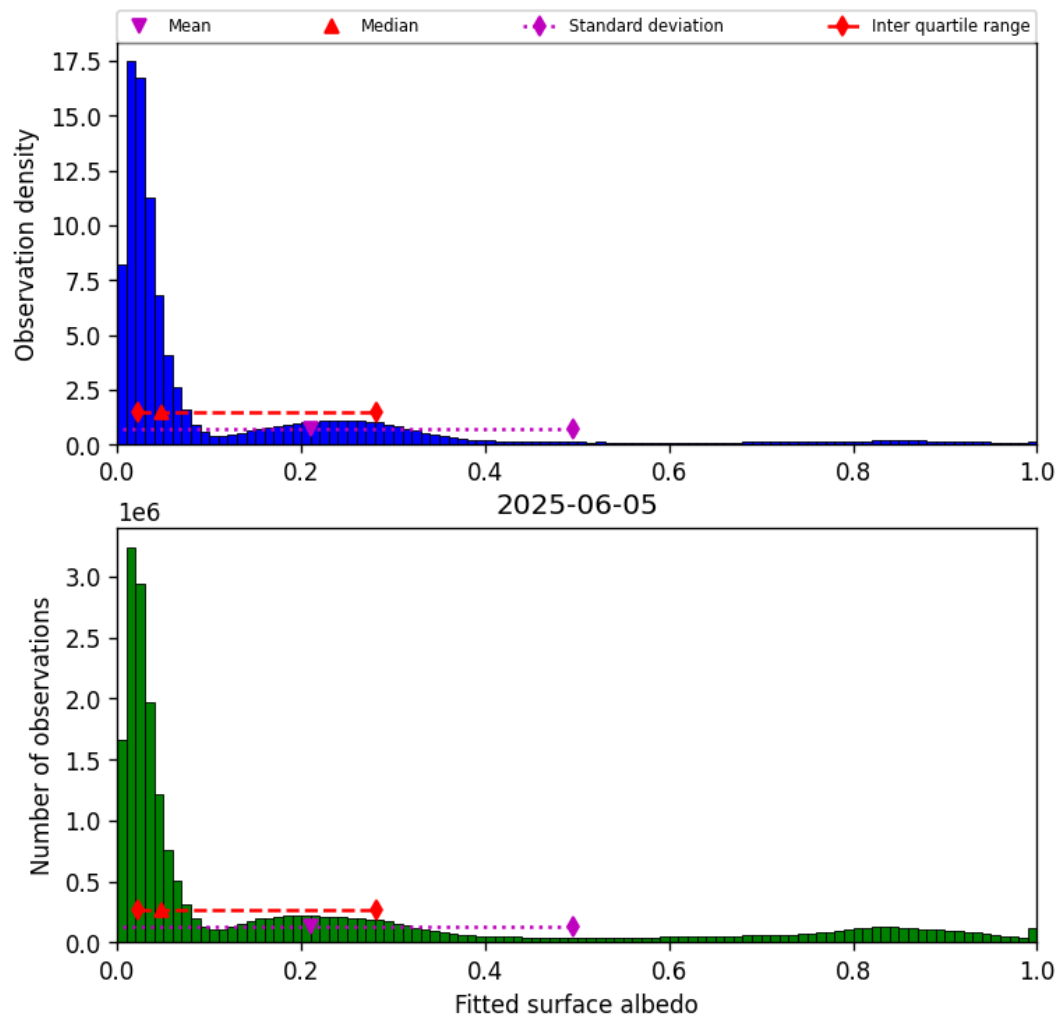
Figure 45: Histogram of “Fitted surface albedo” for 2025-06-04 to 2025-06-06
