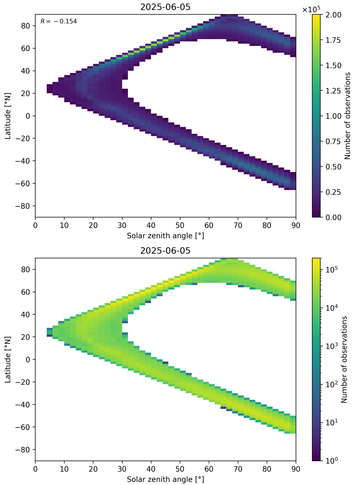
Figure 105: Scatter density plot of “Solar zenith angle” against “Latitude” for 2025-06-04 to 2025-06-06.
