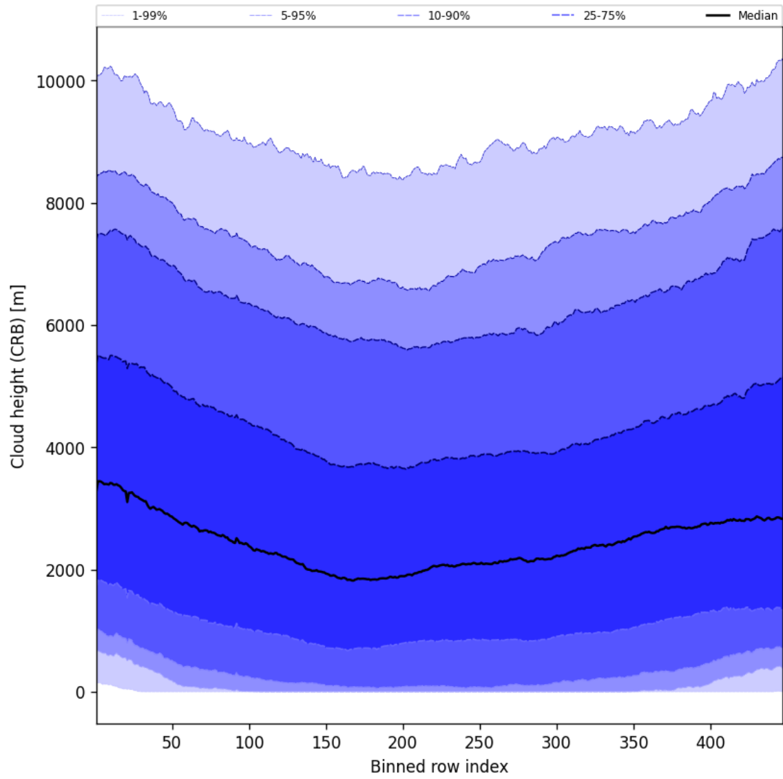
Figure 59: Along track statistics of “Cloud height (CRB)” for 2025-06-04 to 2025-06-06
