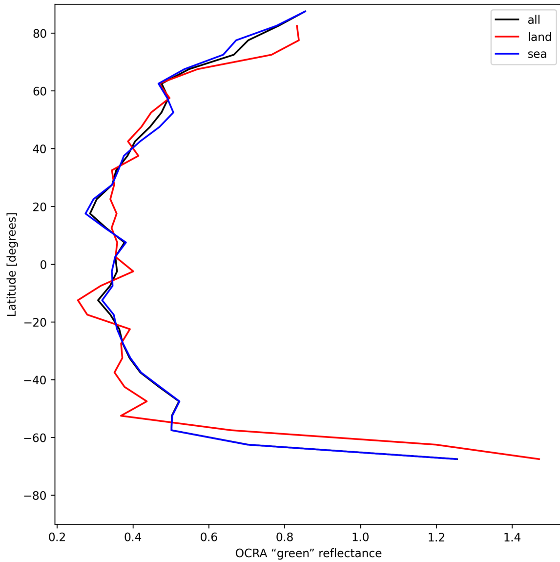
Figure 36: Zonal average of “OCRA “green” reflectance” for 2025-06-04 to 2025-06-06.
