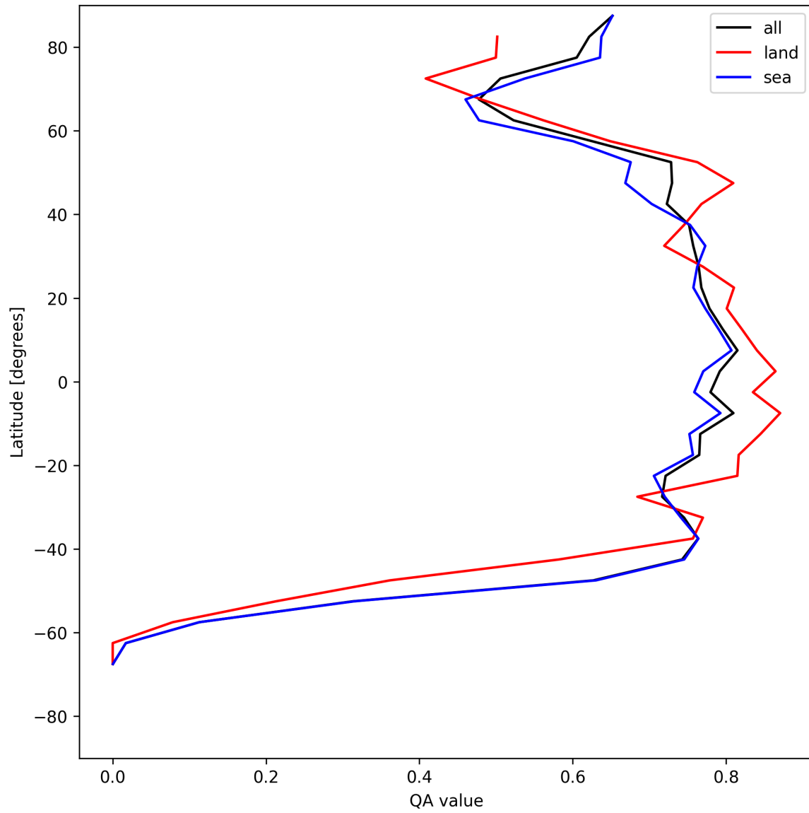
Figure 22: Zonal average of “QA value” for 2025-06-06 to 2025-06-08.
