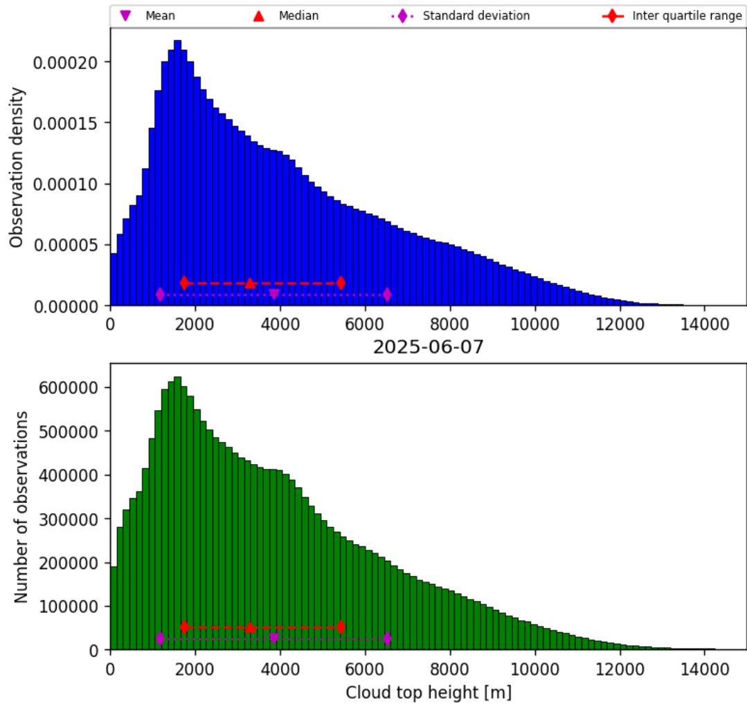
Figure 40: Histogram of “Cloud top height” for 2025-06-06 to 2025-06-08
