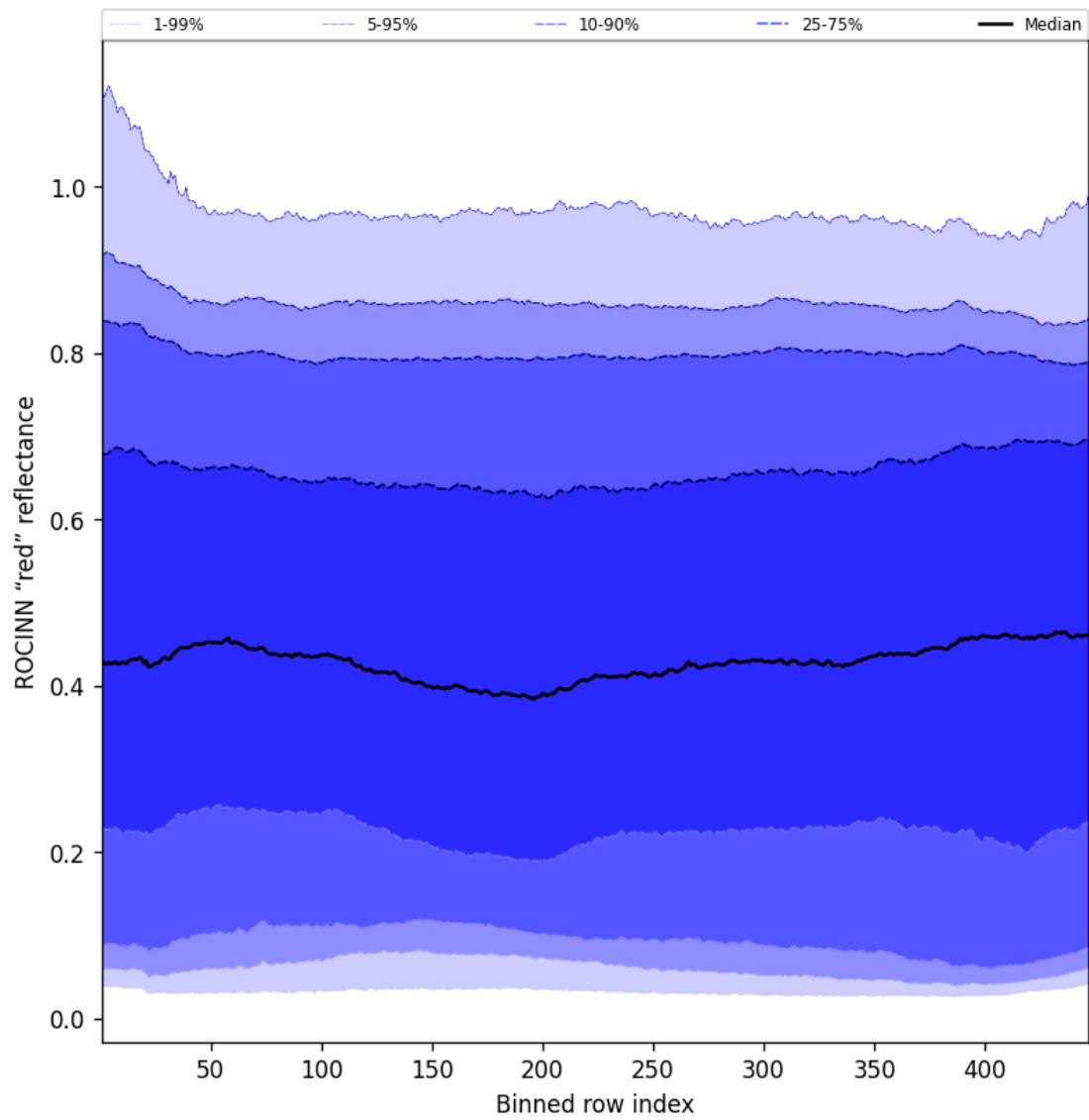
Figure 69: Along track statistics of “ROCINN “red” reflectance” for 2025-06-06 to 2025-06-08
