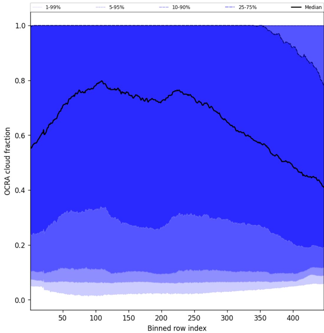
Figure 66: Along track statistics of “OCRA cloud fraction” for 2025-06-06 to 2025-06-08
