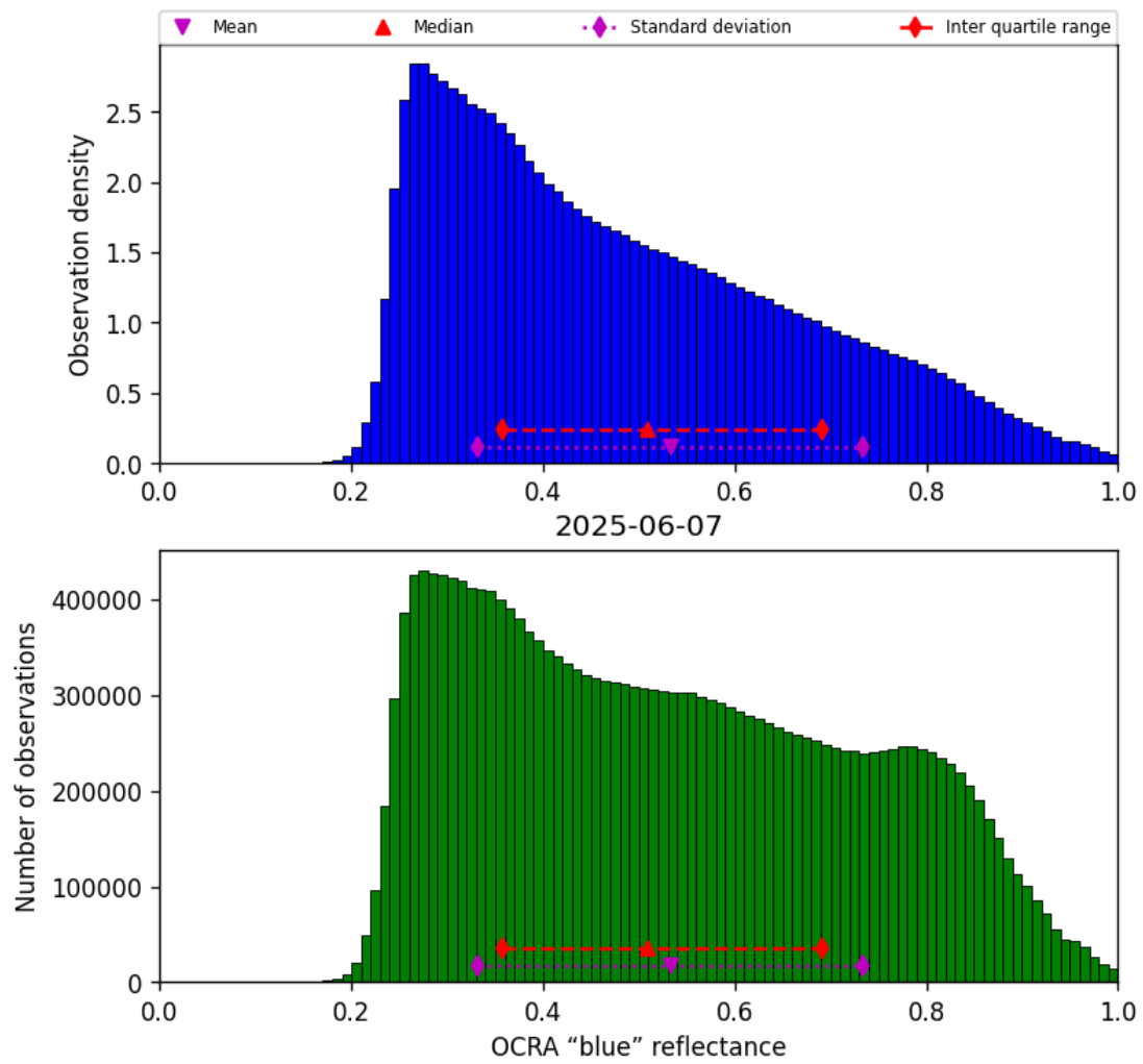
Figure 51: Histogram of “OCRA “blue” reflectance” for 2025-06-06 to 2025-06-08
