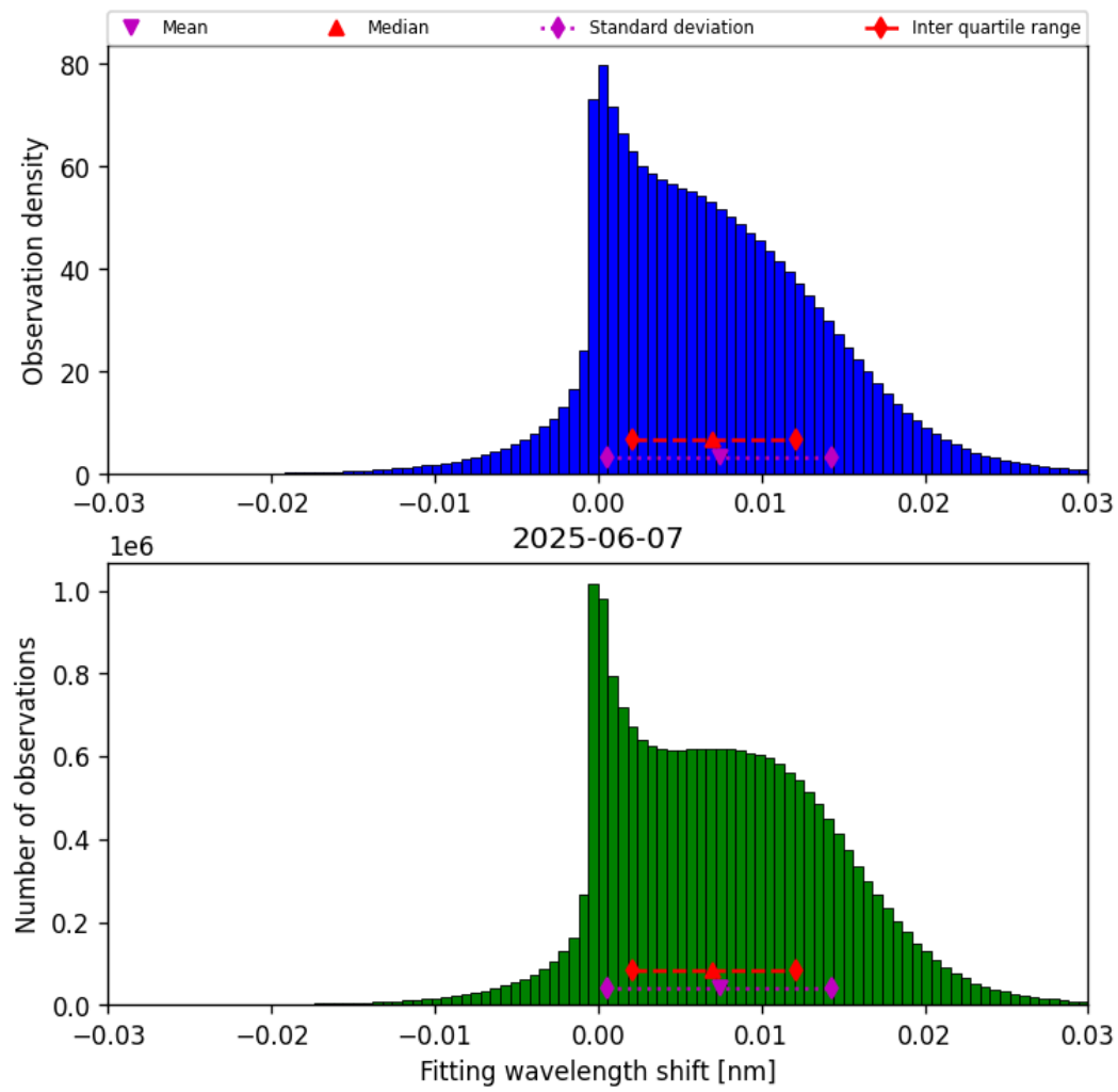
Figure 49: Histogram of “Fitting wavelength shift” for 2025-06-06 to 2025-06-08
