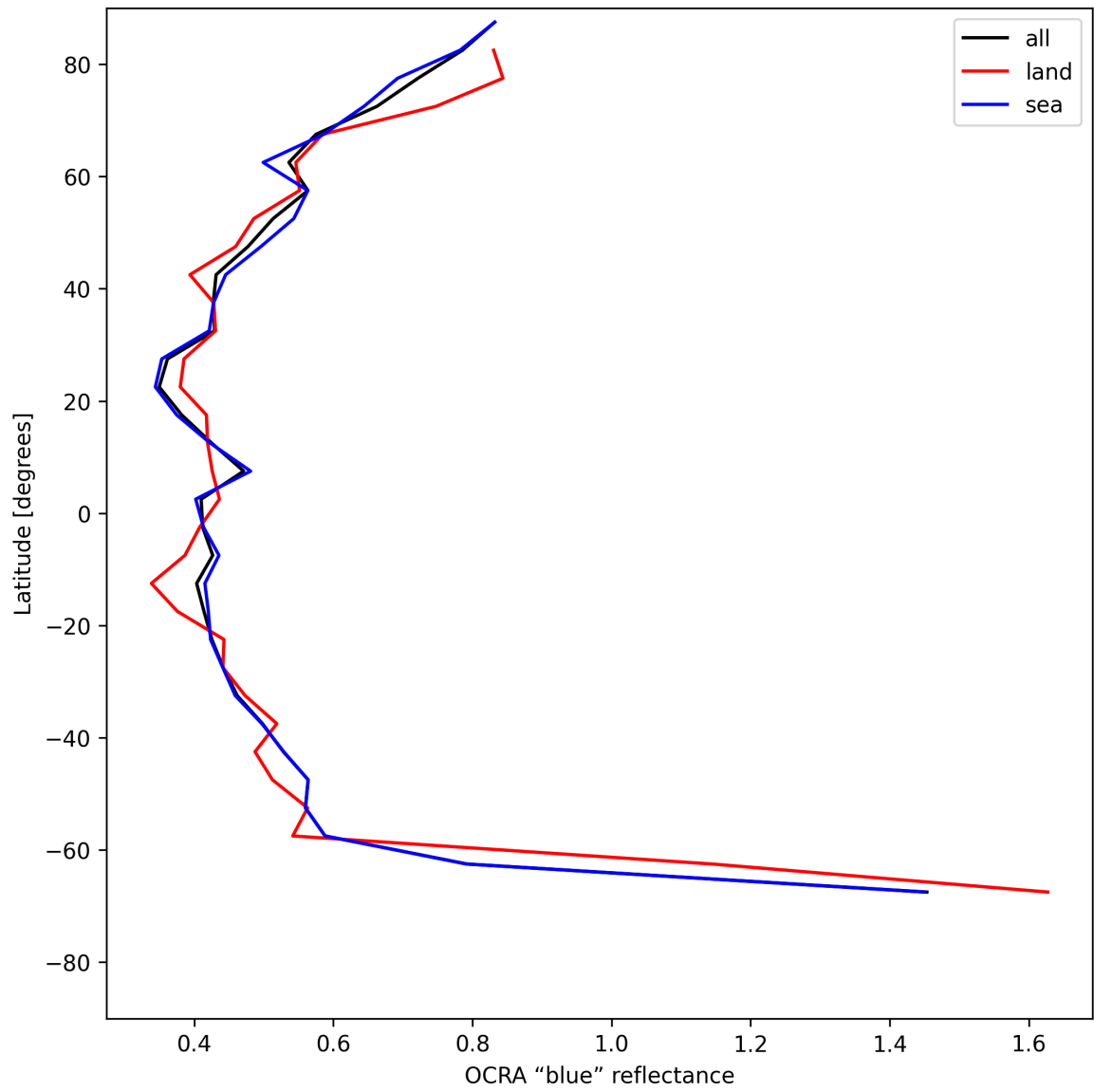
Figure 35: Zonal average of “OCRA “blue” reflectance” for 2025-06-06 to 2025-06-08.
