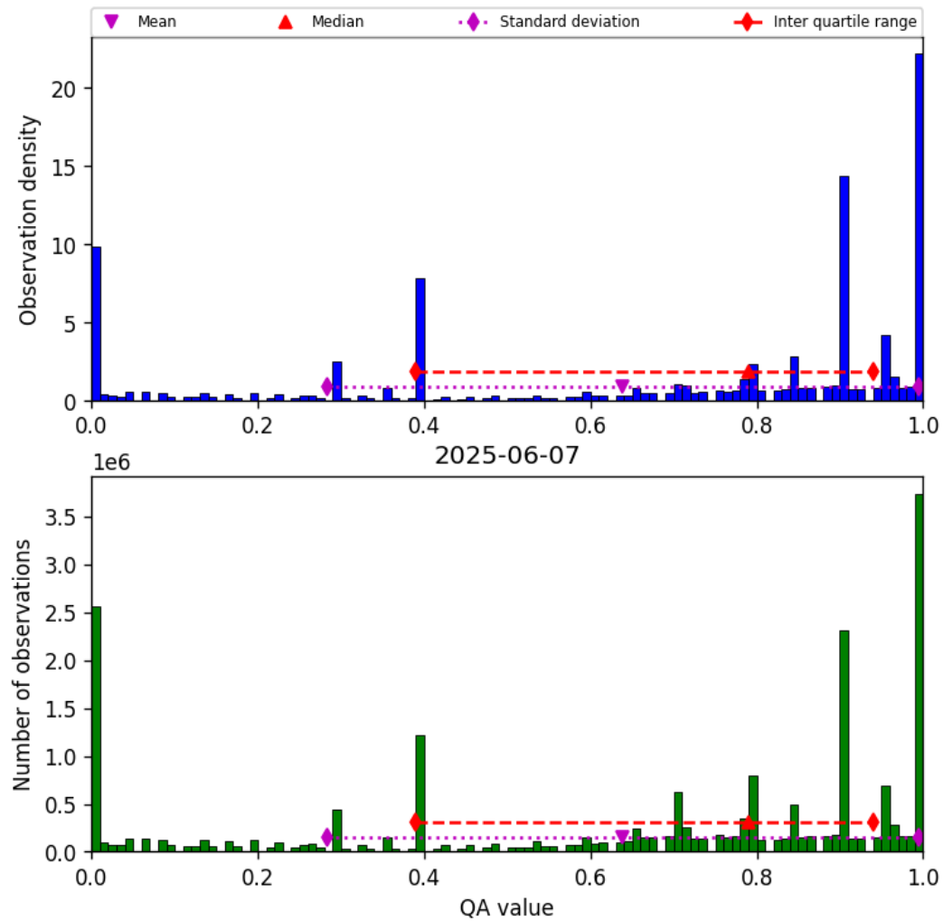
Figure 38: Histogram of “QA value” for 2025-06-06 to 2025-06-08
