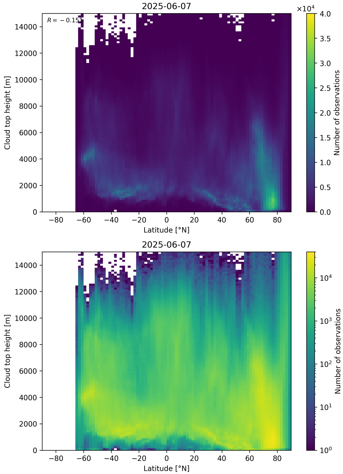
Figure 97: Scatter density plot of “Latitude” against “Cloud top height” for 2025-06-06 to 2025-06-08.
