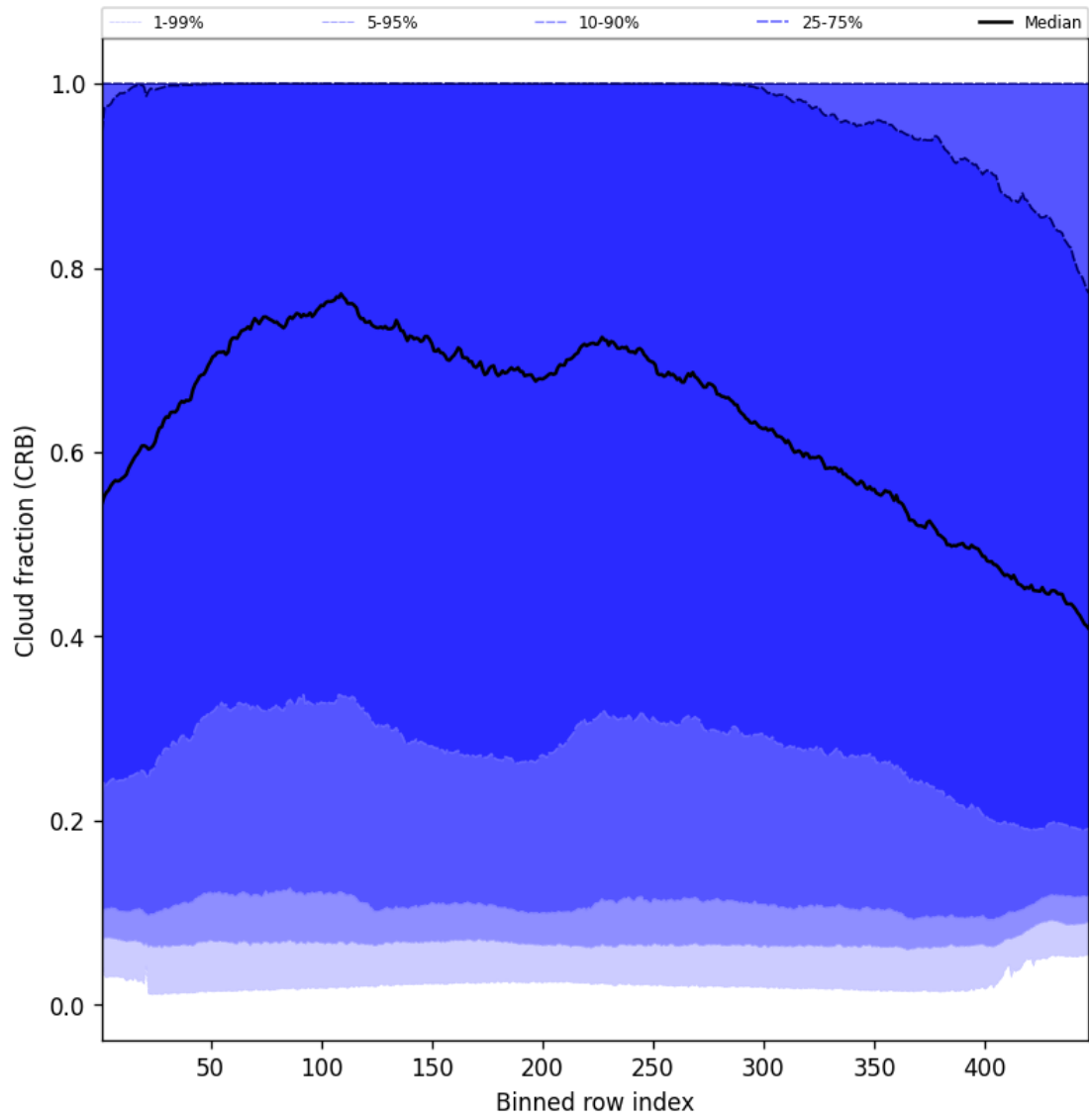
Figure 58: Along track statistics of “Cloud fraction (CRB)” for 2025-06-06 to 2025-06-08
