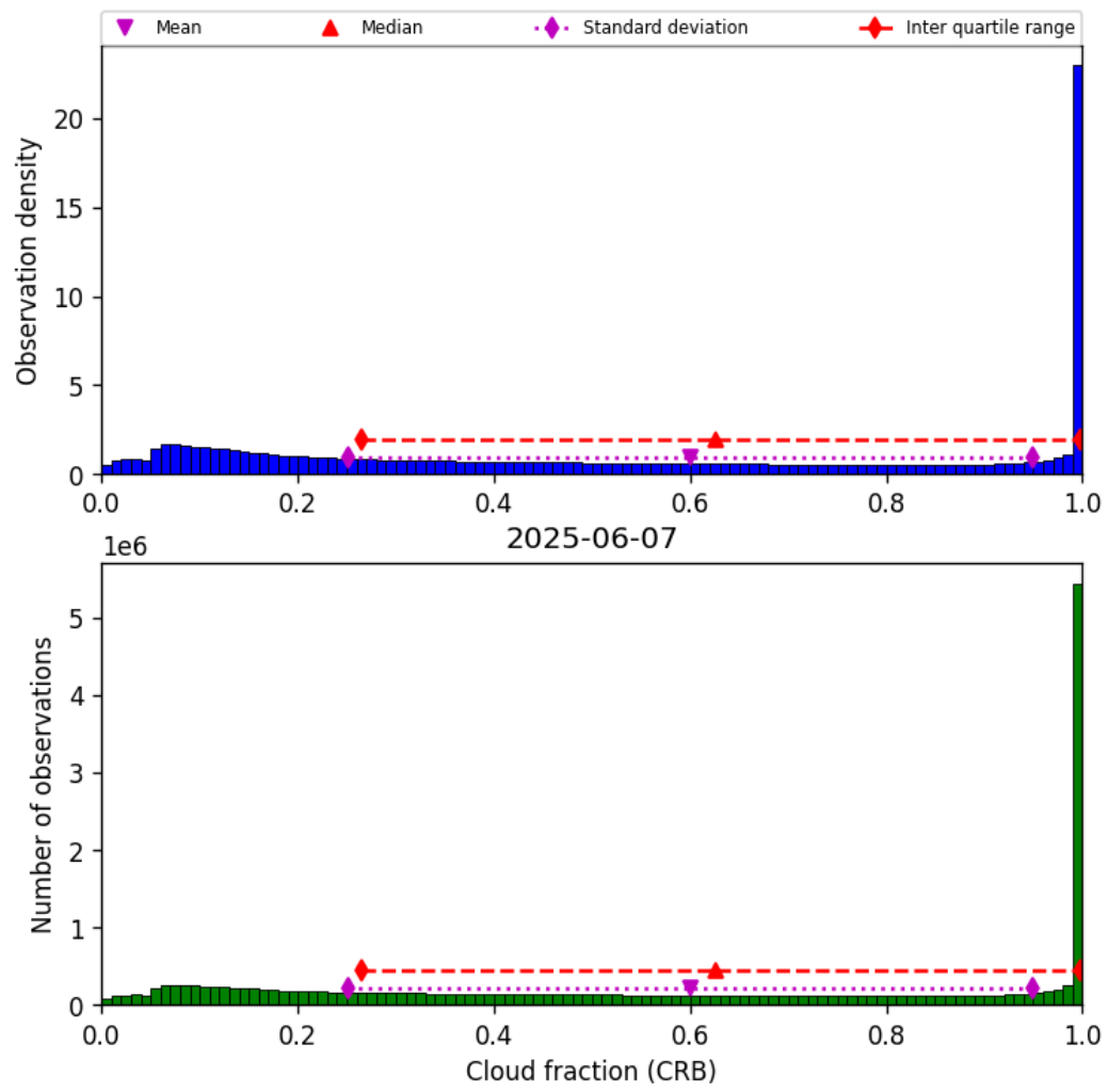
Figure 42: Histogram of “Cloud fraction (CRB)” for 2025-06-06 to 2025-06-08
