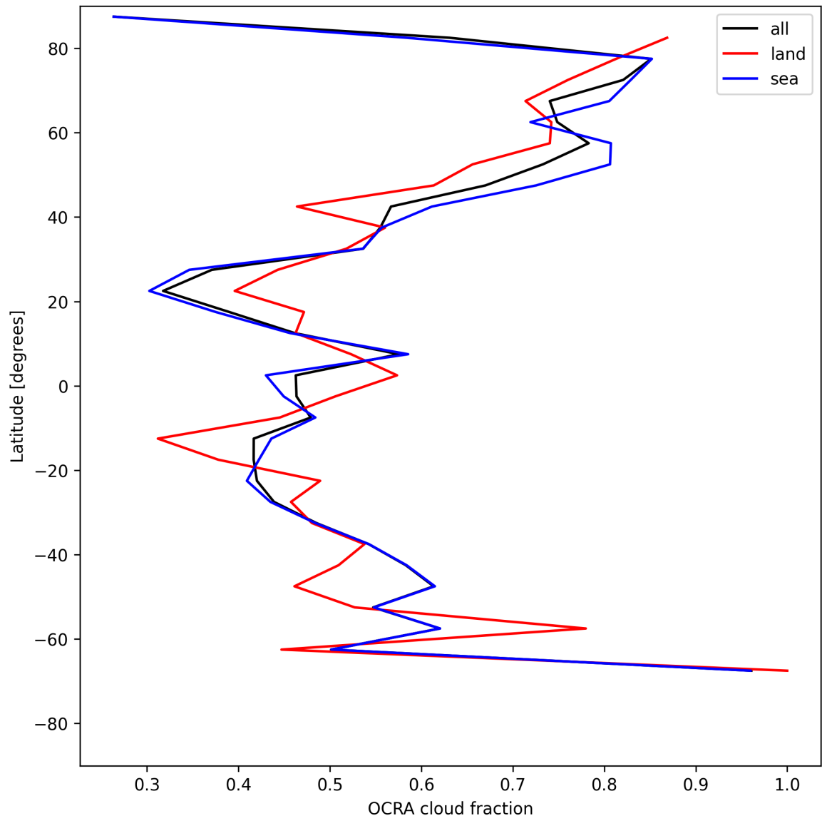
Figure 34: Zonal average of “OCRA cloud fraction” for 2025-06-06 to 2025-06-08.
