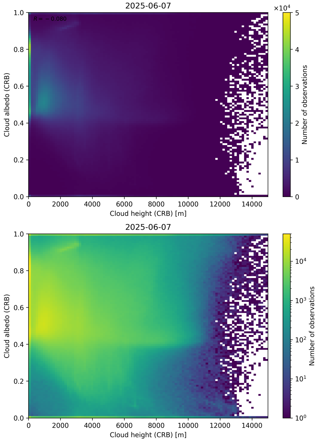
Figure 80: Scatter density plot of “Cloud height (CRB)” against “Cloud albedo (CRB)” for 2025-06-06 to 2025-06-08.
