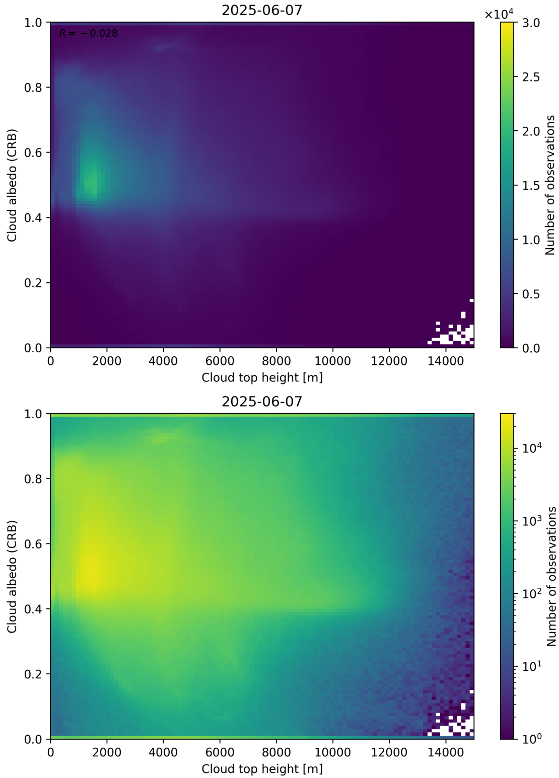
Figure 86: Scatter density plot of “Cloud top height” against “Cloud albedo (CRB)” for 2025-06-06 to 2025-06-08.
