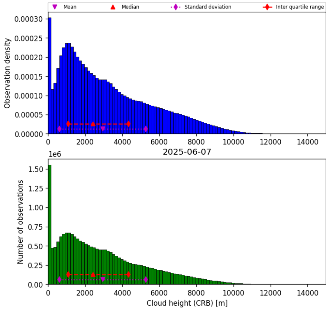
Figure 43: Histogram of “Cloud height (CRB)” for 2025-06-06 to 2025-06-08
