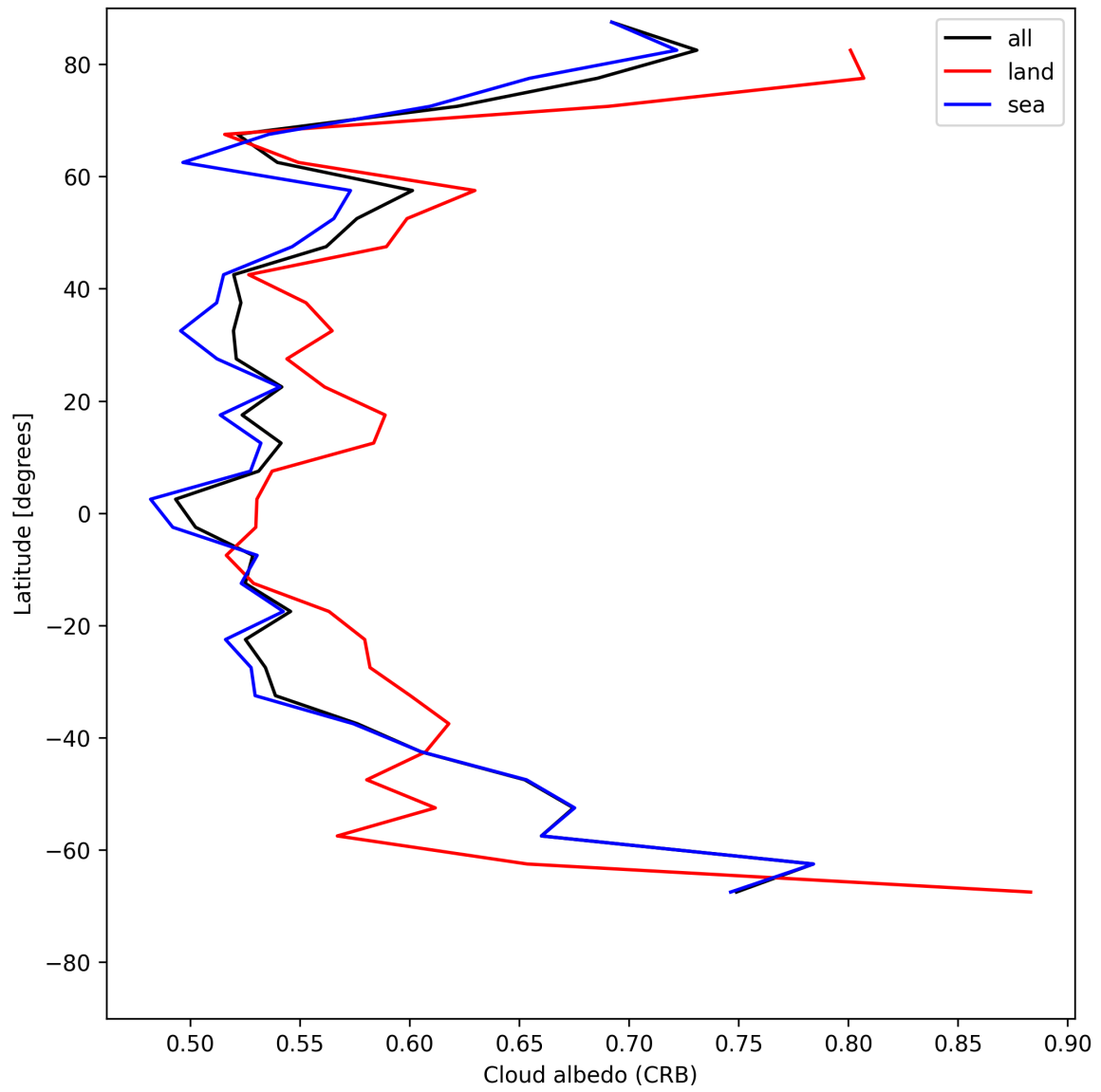
Figure 28: Zonal average of “Cloud albedo (CRB)” for 2025-06-06 to 2025-06-08.
