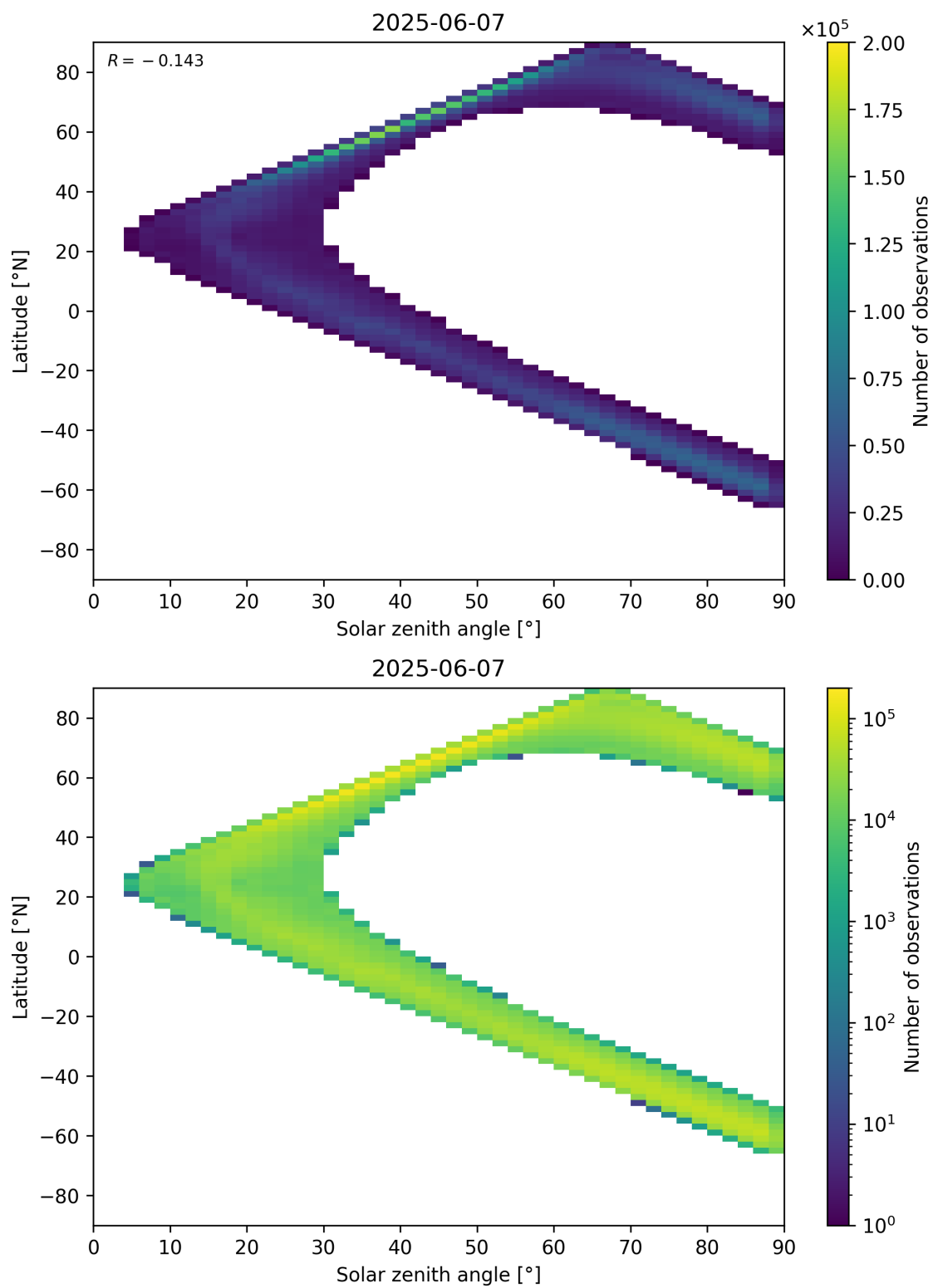
Figure 105: Scatter density plot of “Solar zenith angle” against “Latitude” for 2025-06-06 to 2025-06-08.
