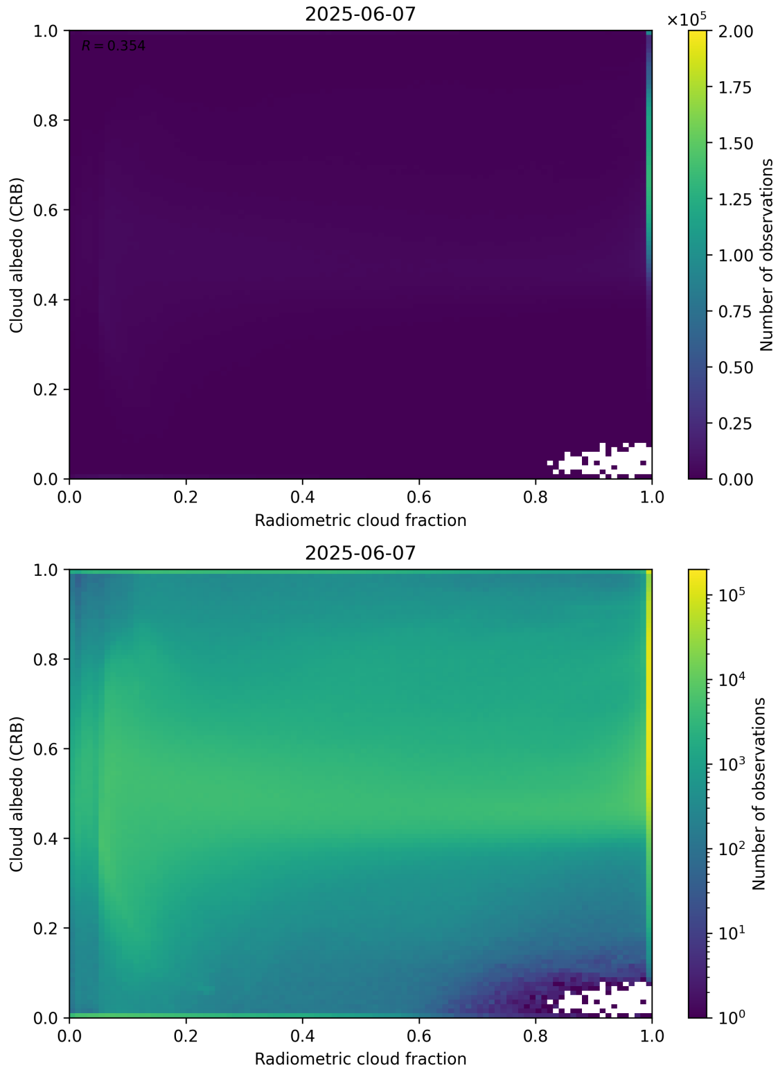
Figure 71: Scatter density plot of “Radiometric cloud fraction” against “Cloud albedo (CRB)” for 2025-06-06 to 2025-06-08.
