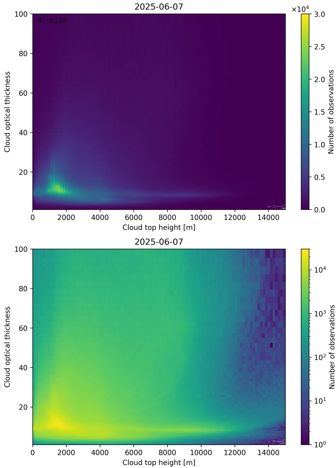
Figure 90: Scatter density plot of “Cloud top height” against “Cloud optical thickness” for 2025-06-06 to 2025-06-08.
