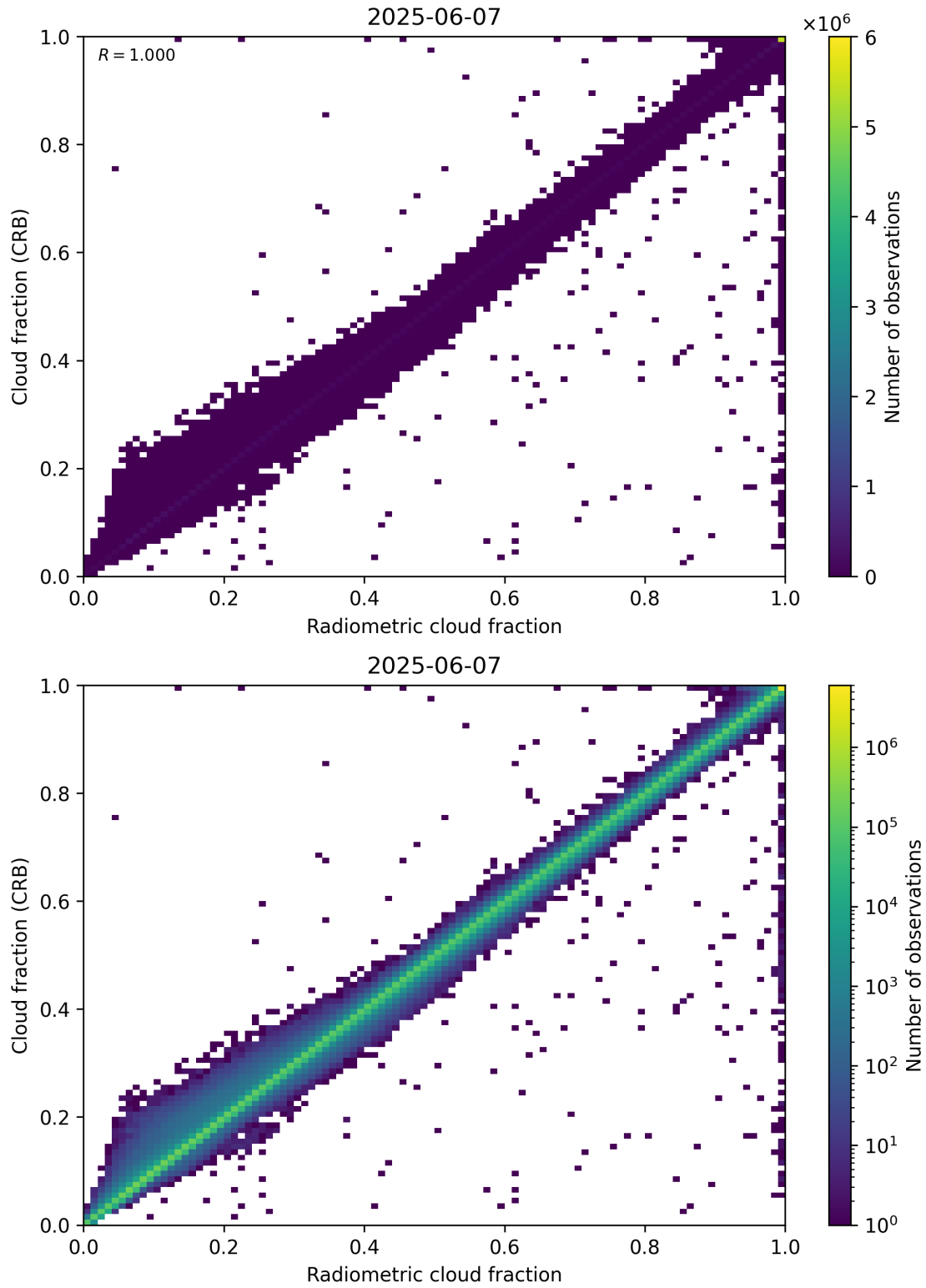
Figure 73: Scatter density plot of “Radiometric cloud fraction” against “Cloud fraction (CRB)” for 2025-06-06 to 2025-06-08.
