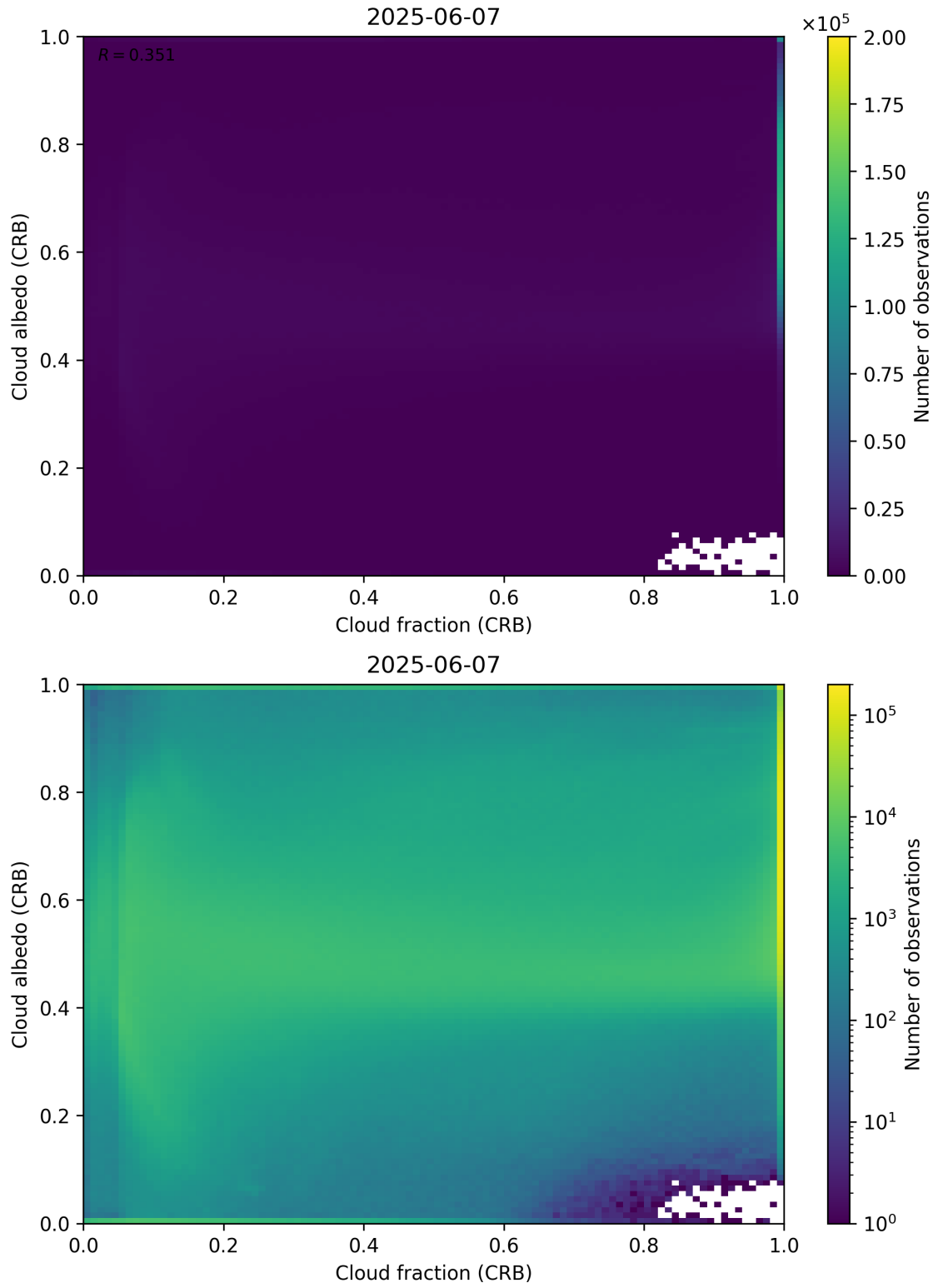
Figure 77: Scatter density plot of “Cloud fraction (CRB)” against “Cloud albedo (CRB)” for 2025-06-06 to 2025-06-08.
