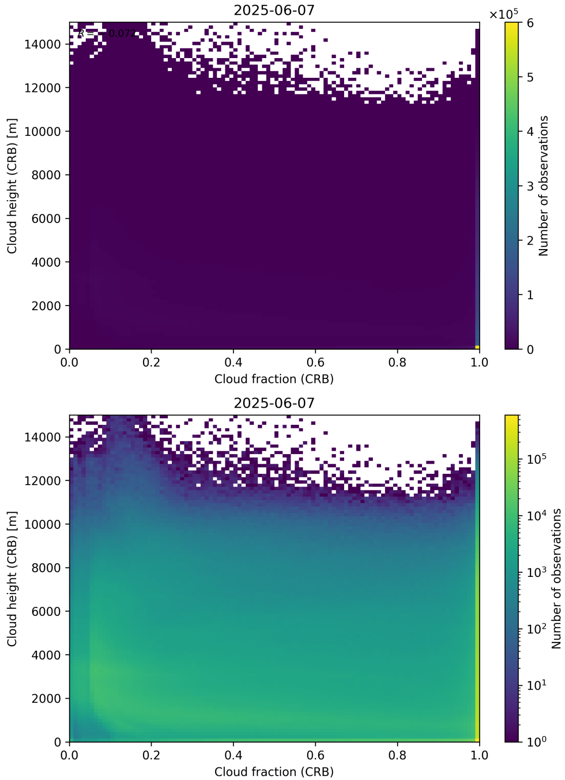
Figure 79: Scatter density plot of “Cloud fraction (CRB)” against “Cloud height (CRB)” for 2025-06-06 to 2025-06-08.
