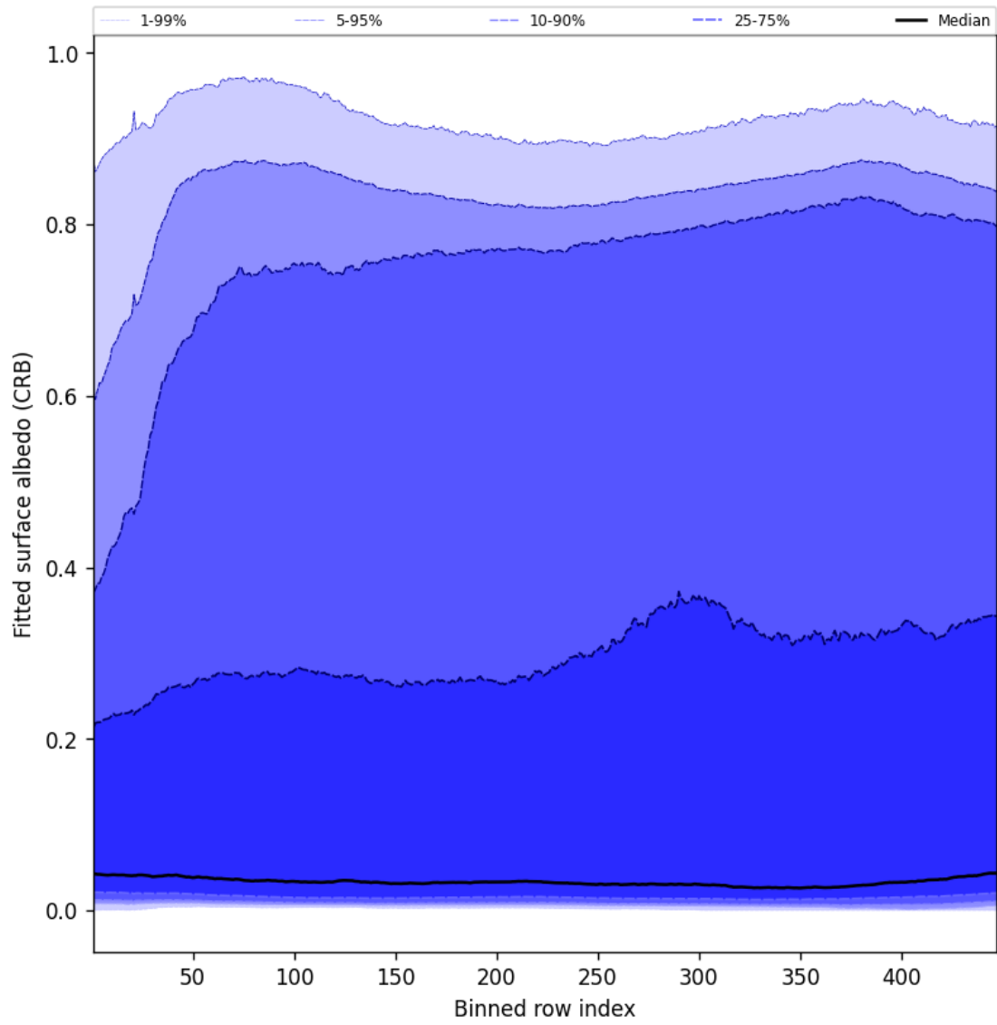
Figure 62: Along track statistics of “Fitted surface albedo (CRB)” for 2025-06-06 to 2025-06-08
