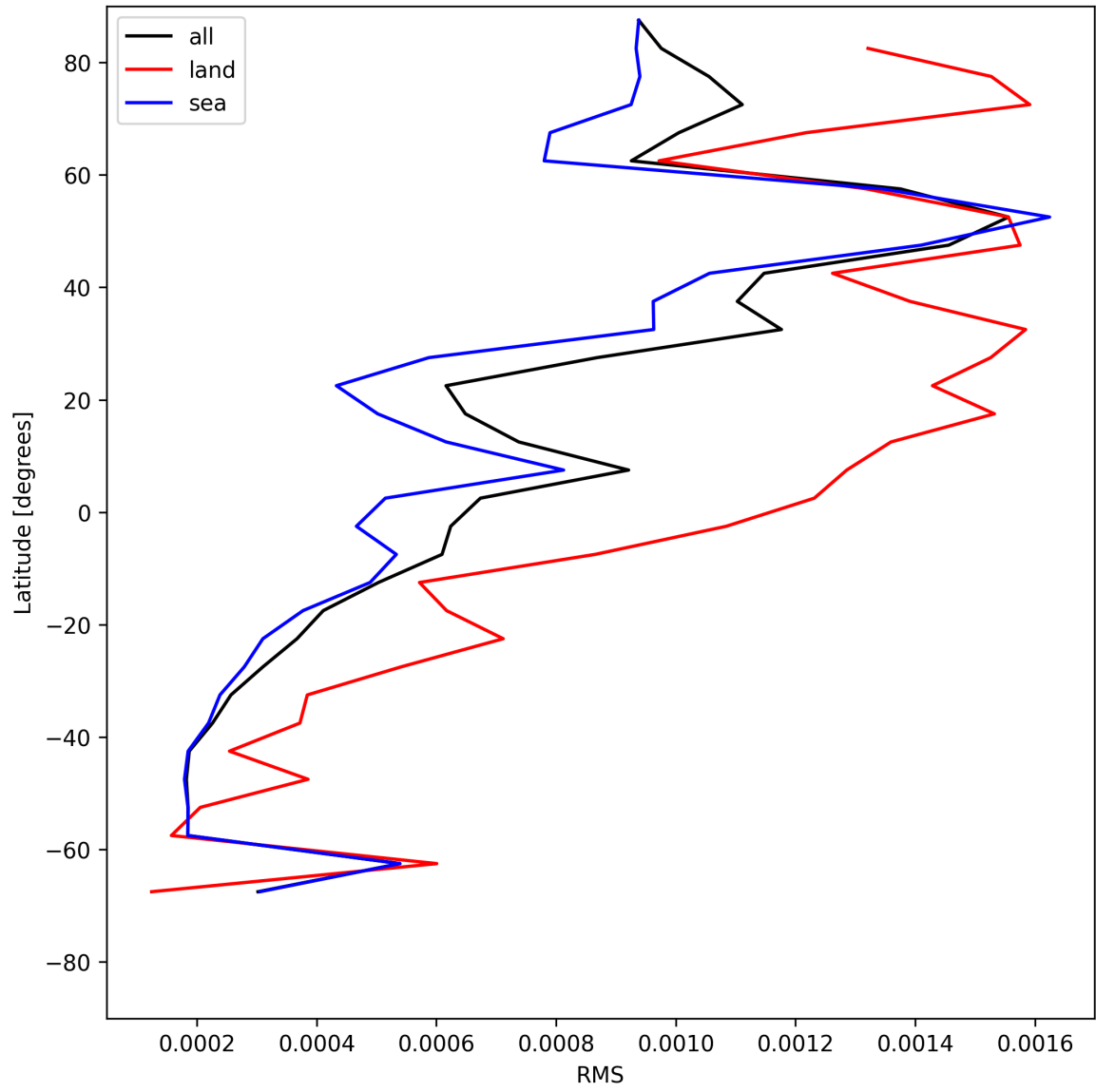
Figure 31: Zonal average of “RMS” for 2025-06-06 to 2025-06-08.
