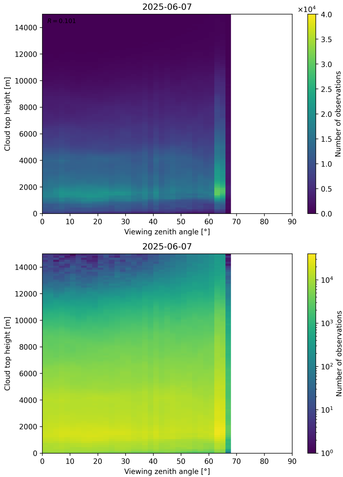
Figure 112: Scatter density plot of “Viewing zenith angle” against “Cloud top height” for 2025-06-06 to 2025-06-08.
