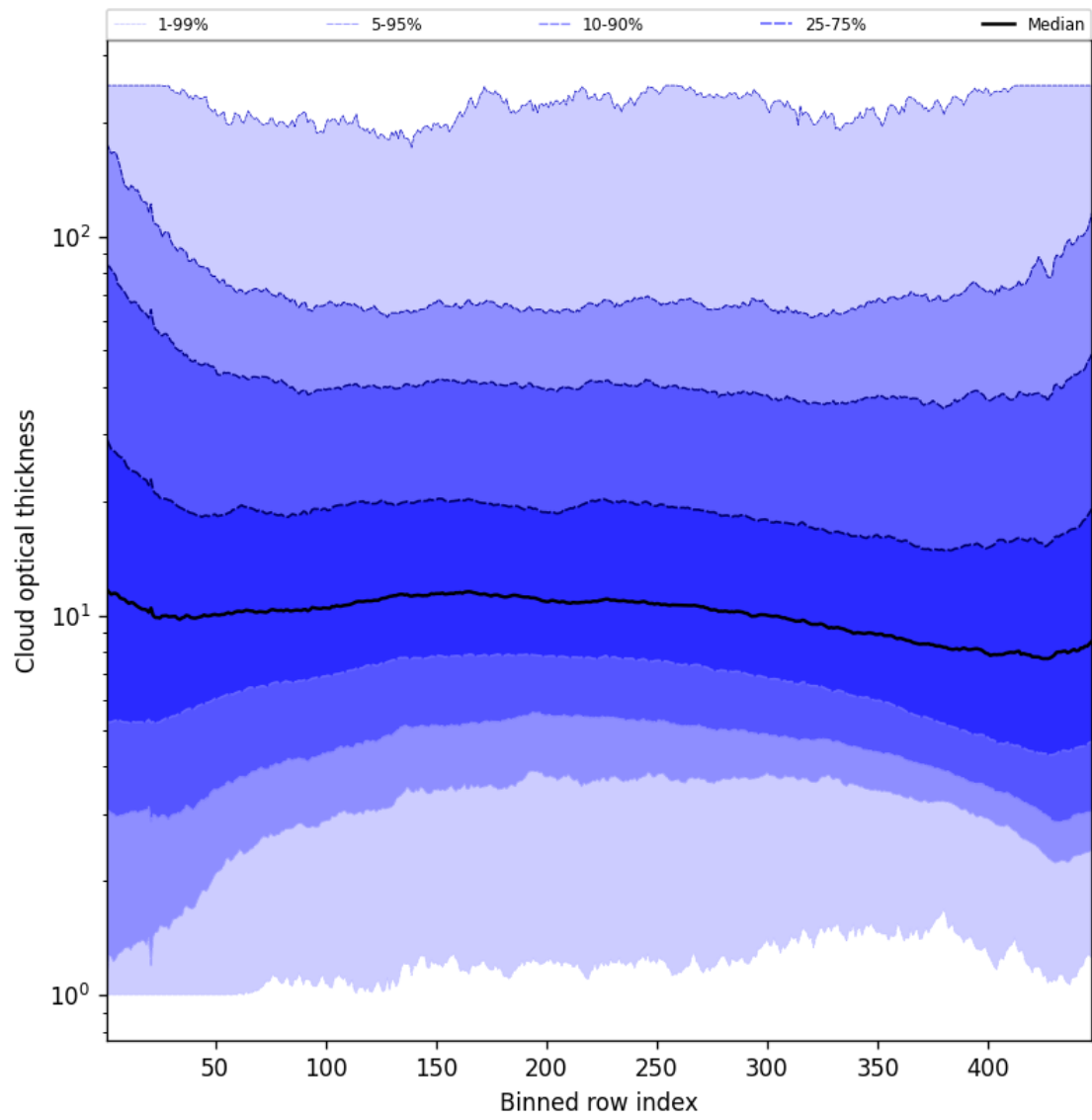
Figure 57: Along track statistics of “Cloud optical thickness” for 2025-06-06 to 2025-06-08
