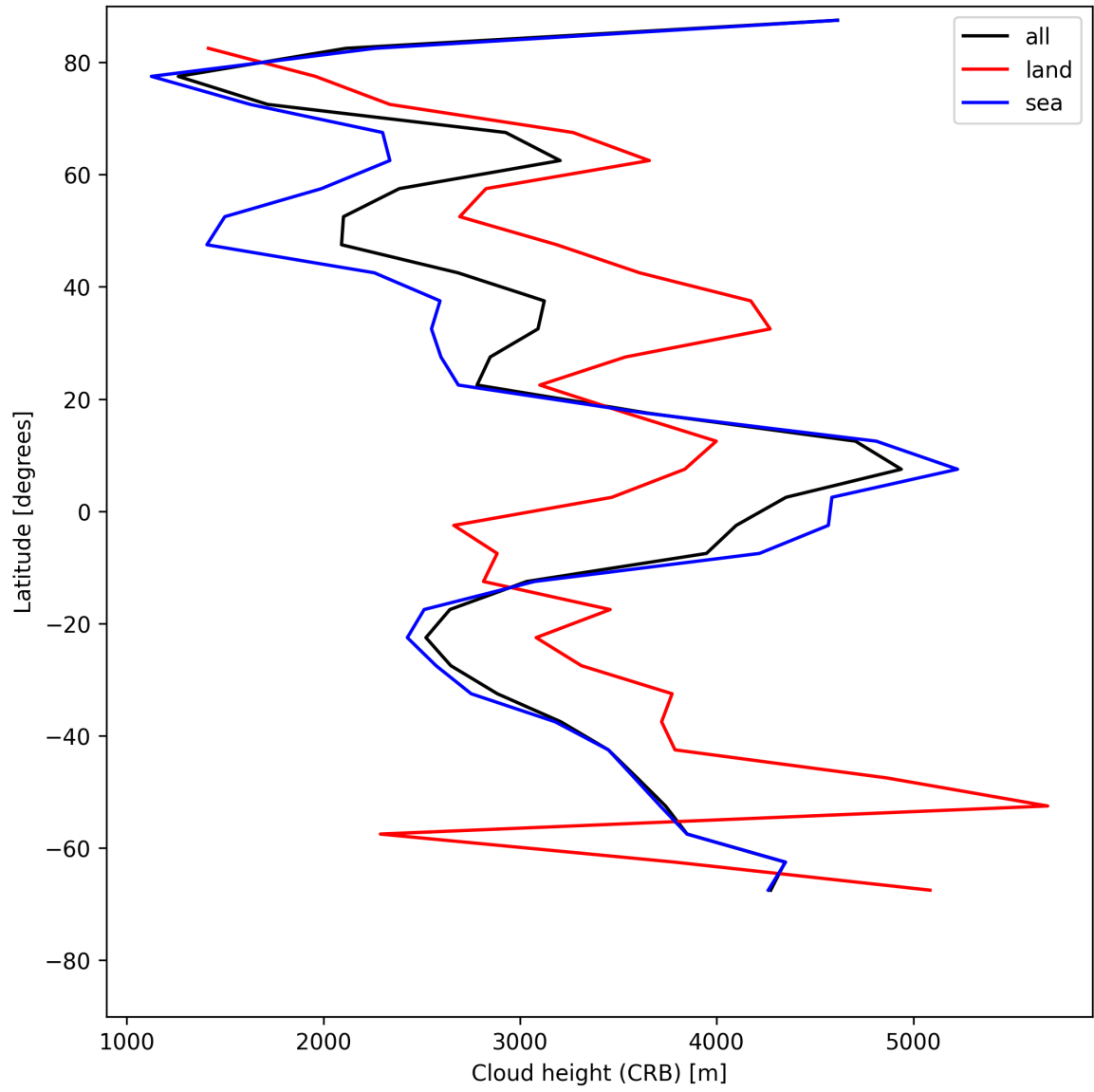
Figure 27: Zonal average of “Cloud height (CRB)” for 2025-06-06 to 2025-06-08.
