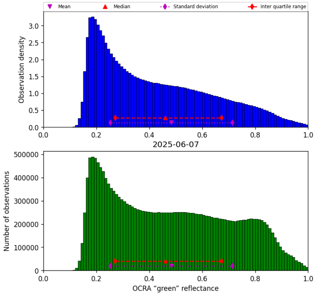
Figure 52: Histogram of “OCRA “green” reflectance” for 2025-06-06 to 2025-06-08
