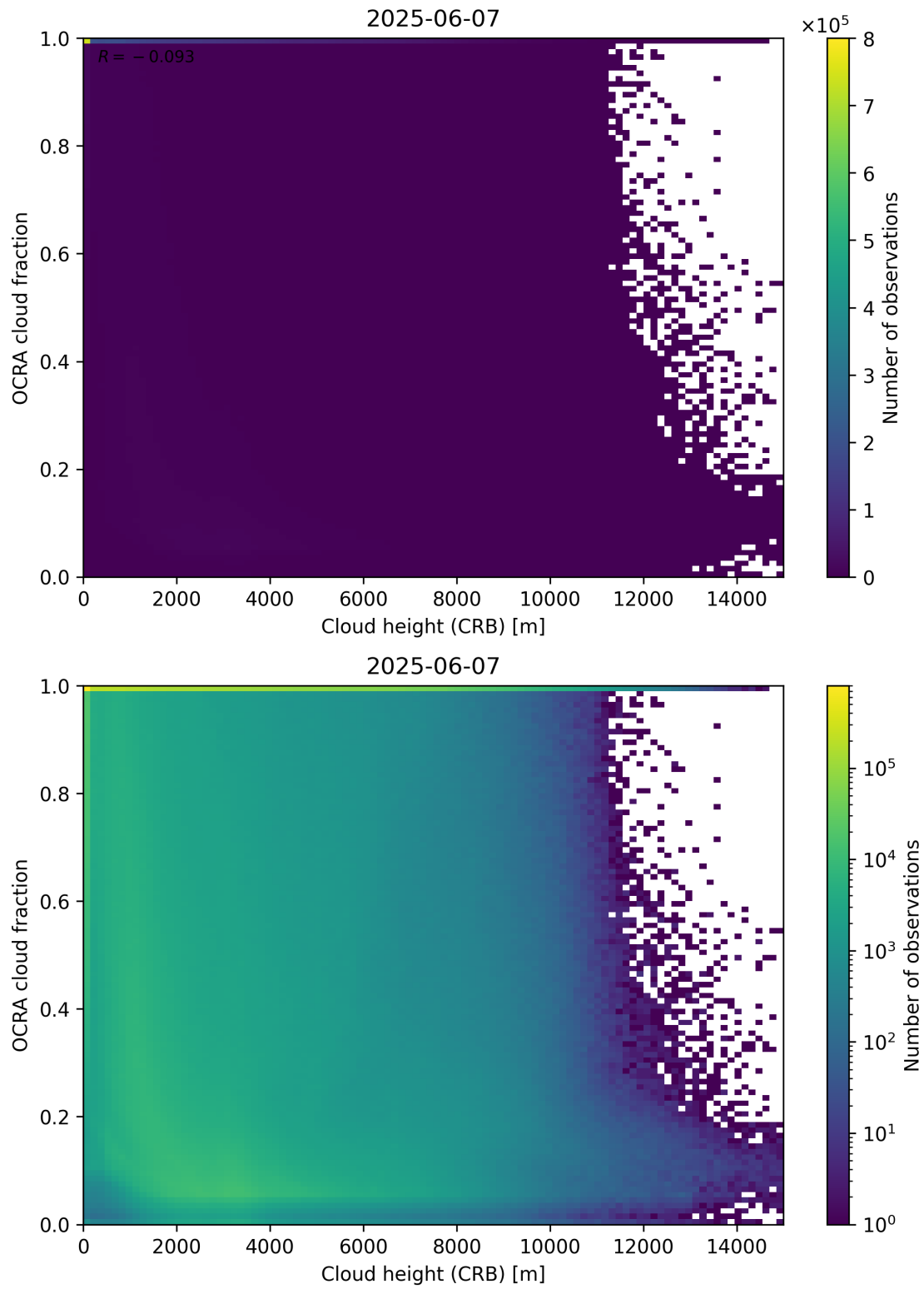
Figure 81: Scatter density plot of “Cloud height (CRB)” against “OCRA cloud fraction” for 2025-06-06 to 2025-06-08.
