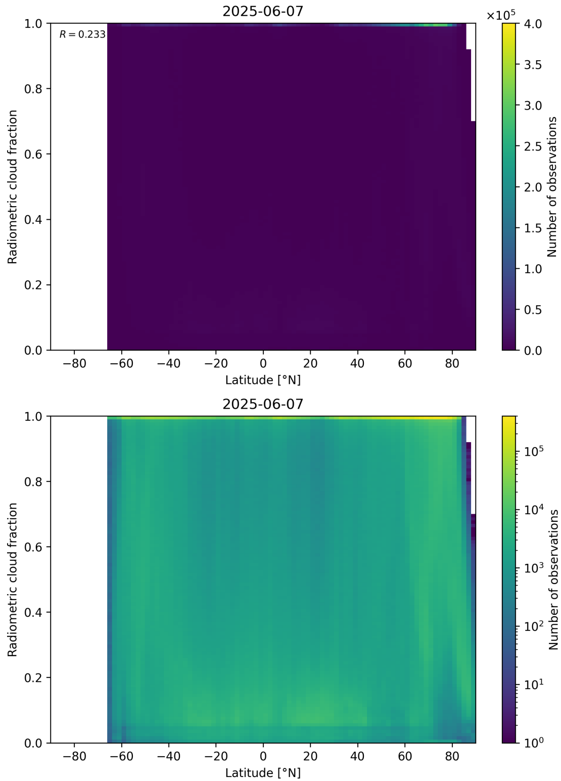
Figure 92: Scatter density plot of “Latitude” against “Radiometric cloud fraction” for 2025-06-06 to 2025-06-08.
