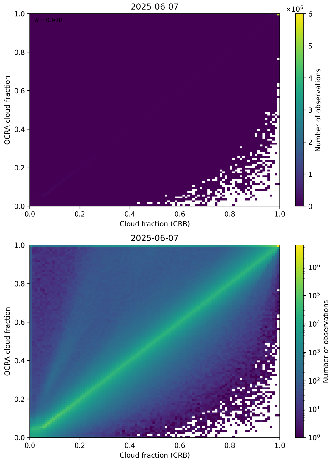
Figure 78: Scatter density plot of “Cloud fraction (CRB)” against “OCRA cloud fraction” for 2025-06-06 to 2025-06-08.
