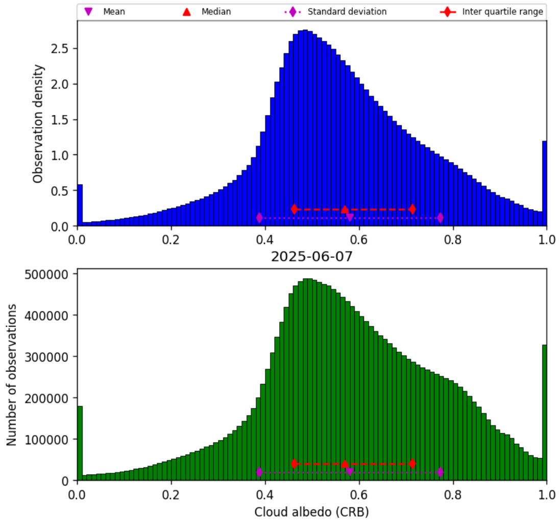
Figure 44: Histogram of “Cloud albedo (CRB)” for 2025-06-06 to 2025-06-08
