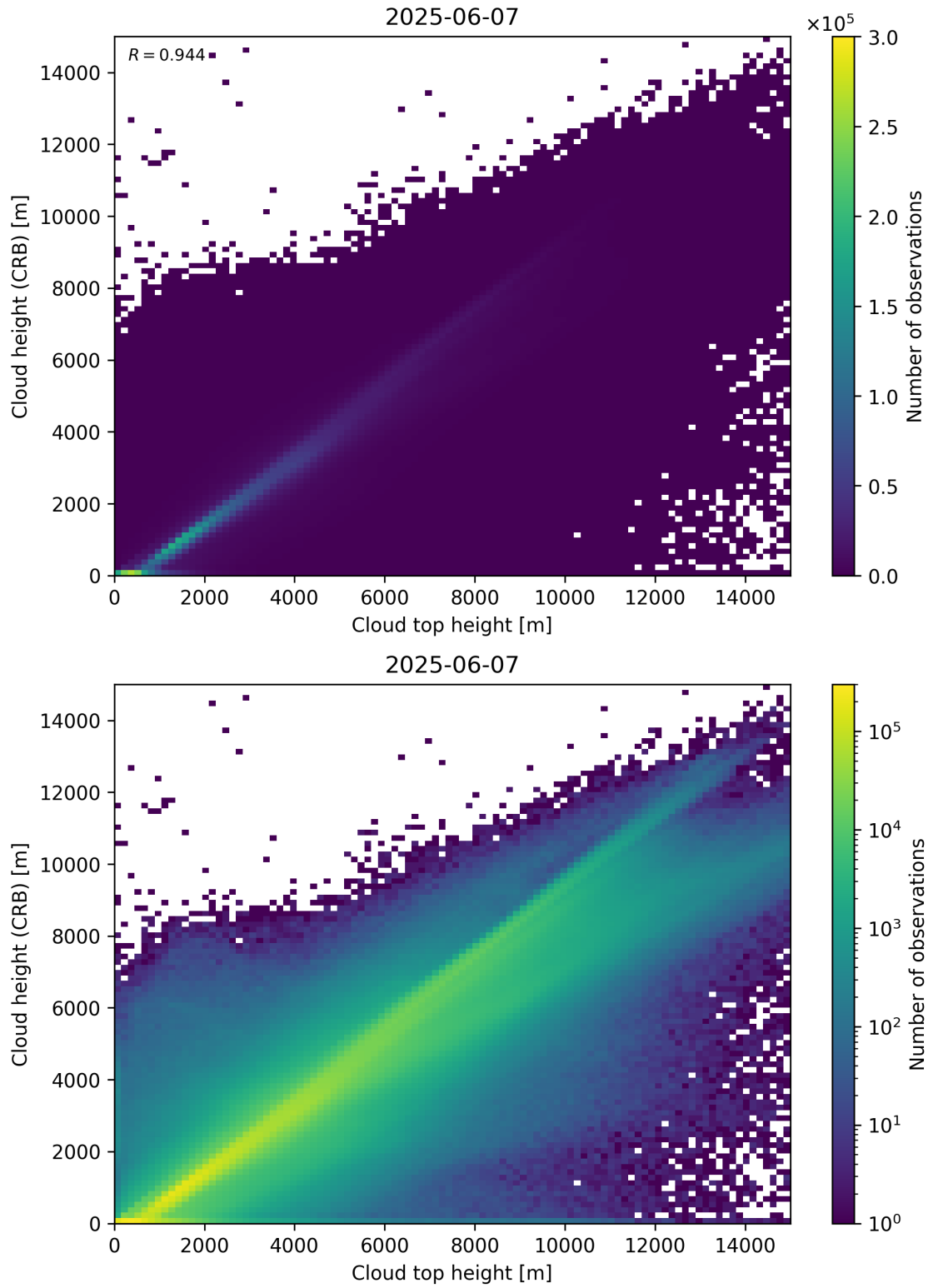
Figure 89: Scatter density plot of “Cloud top height” against “Cloud height (CRB)” for 2025-06-06 to 2025-06-08.
