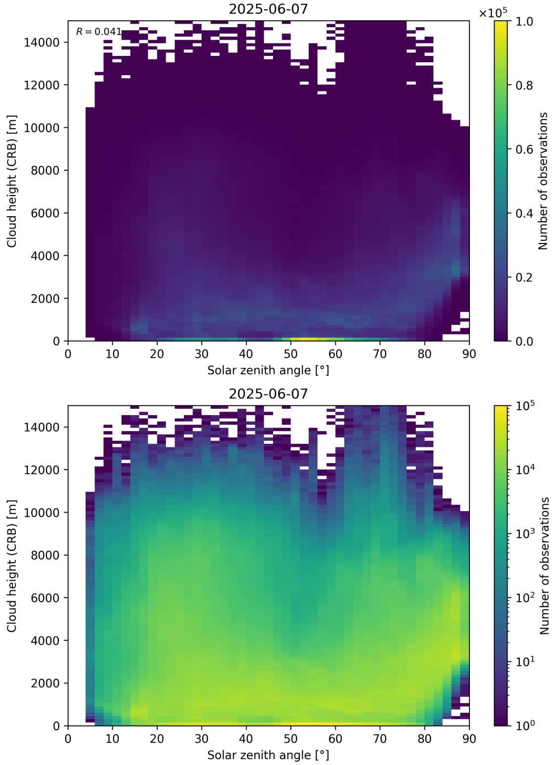
Figure 102: Scatter density plot of “Solar zenith angle” against “Cloud height (CRB)” for 2025-06-06 to 2025-06-08.
