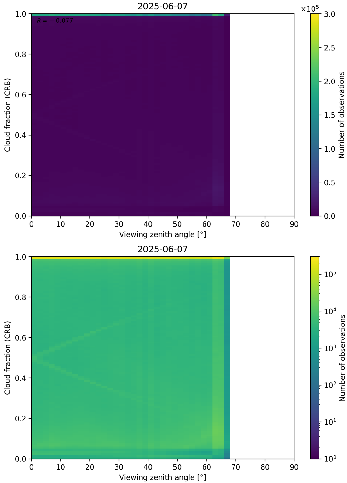
Figure 109: Scatter density plot of “Viewing zenith angle” against “Cloud fraction (CRB)” for 2025-06-06 to 2025-06-08.
