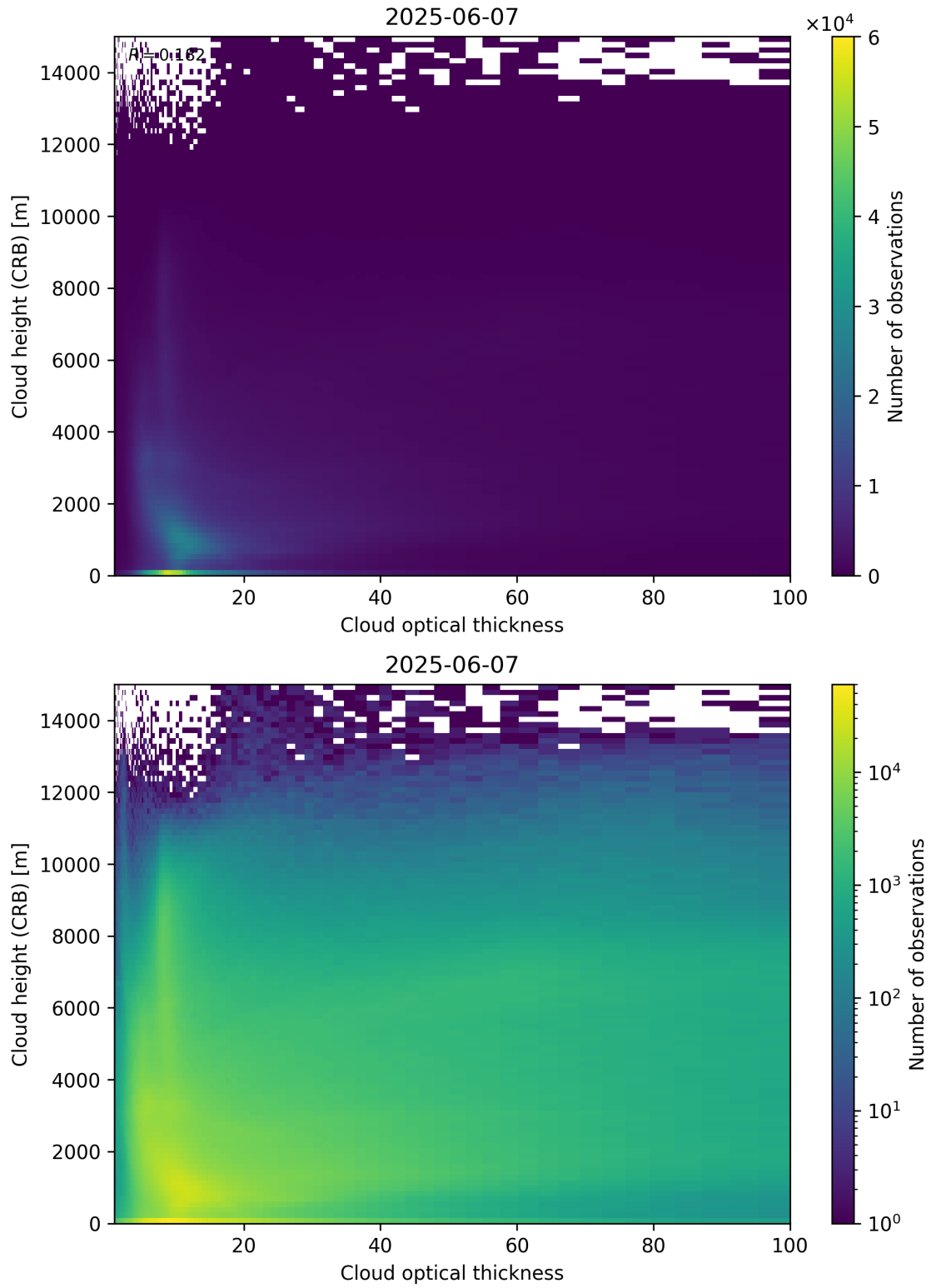
Figure 85: Scatter density plot of “Cloud optical thickness” against “Cloud height (CRB)” for 2025-06-06 to 2025-06-08.
