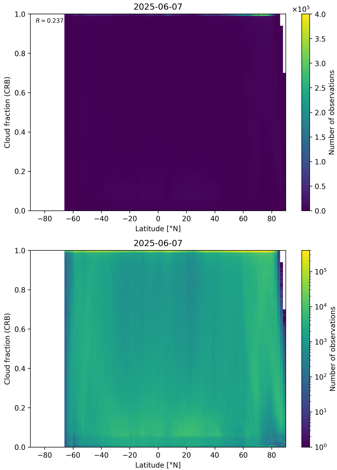
Figure 94: Scatter density plot of “Latitude” against “Cloud fraction (CRB)” for 2025-06-06 to 2025-06-08.
