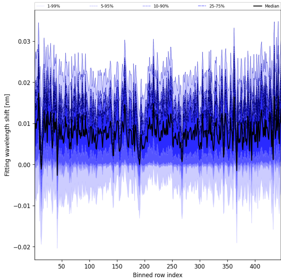
Figure 65: Along track statistics of “Fitting wavelength shift” for 2025-06-06 to 2025-06-08
