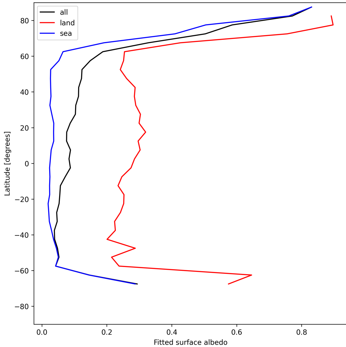
Figure 29: Zonal average of “Fitted surface albedo” for 2025-06-06 to 2025-06-08.
