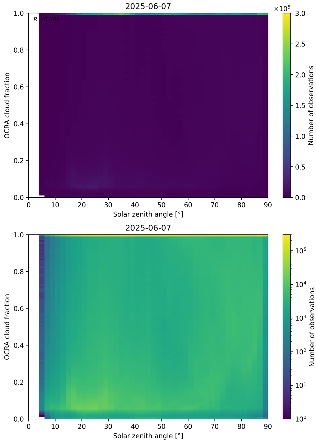
Figure 100: Scatter density plot of “Solar zenith angle” against “OCRA cloud fraction” for 2025-06-06 to 2025-06-08.
