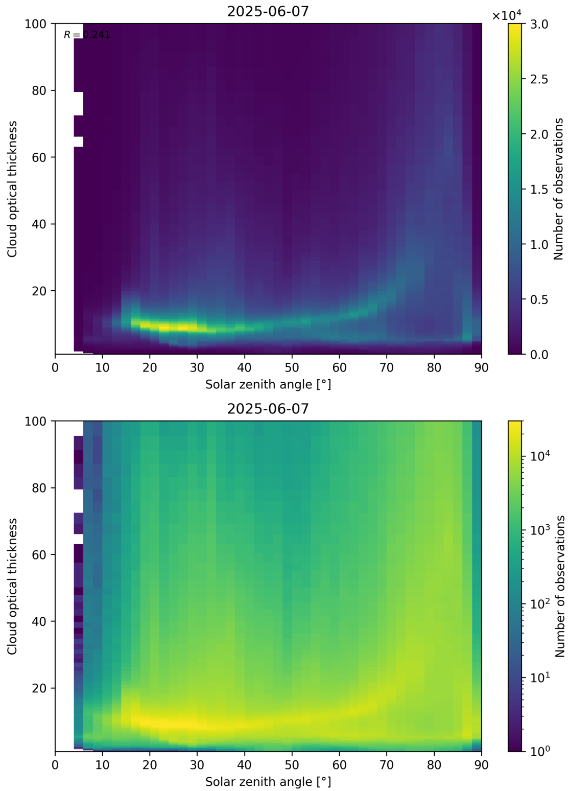
Figure 103: Scatter density plot of “Solar zenith angle” against “Cloud optical thickness” for 2025-06-06 to 2025-06-08.
