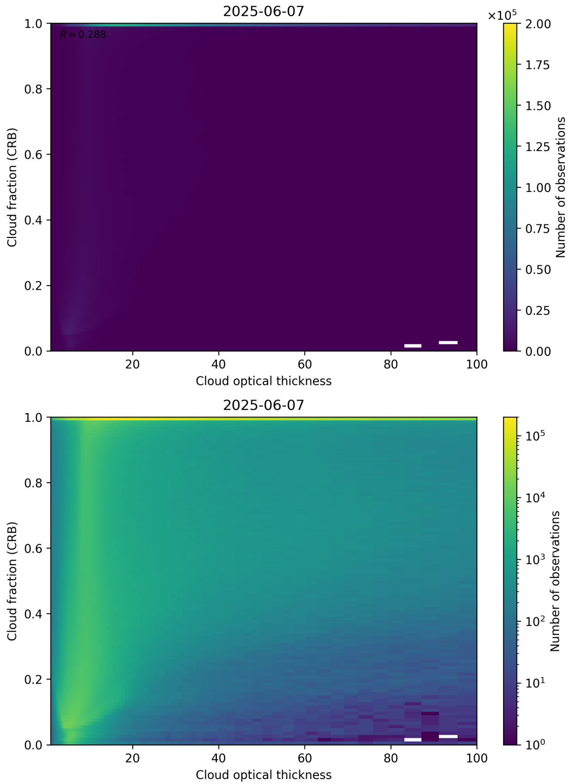
Figure 84: Scatter density plot of “Cloud optical thickness” against “Cloud fraction (CRB)” for 2025-06-06 to 2025-06-08.
