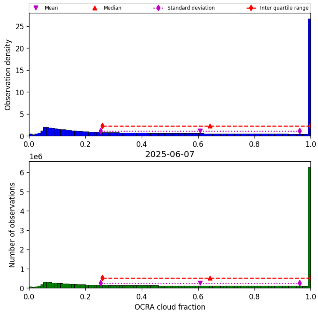
Figure 50: Histogram of “OCRA cloud fraction” for 2025-06-06 to 2025-06-08
