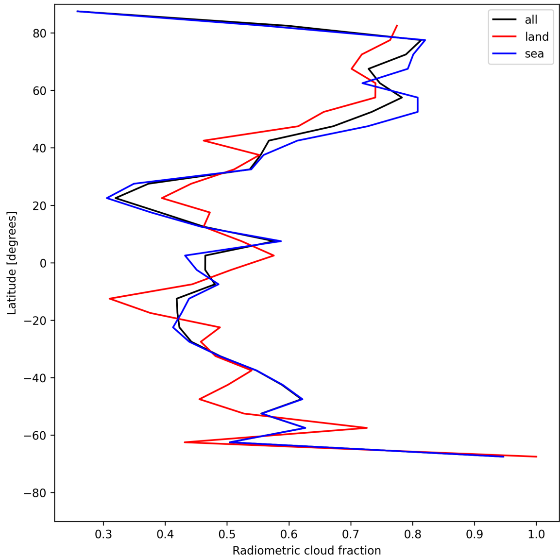
Figure 23: Zonal average of “Radiometric cloud fraction” for 2025-06-06 to 2025-06-08.
