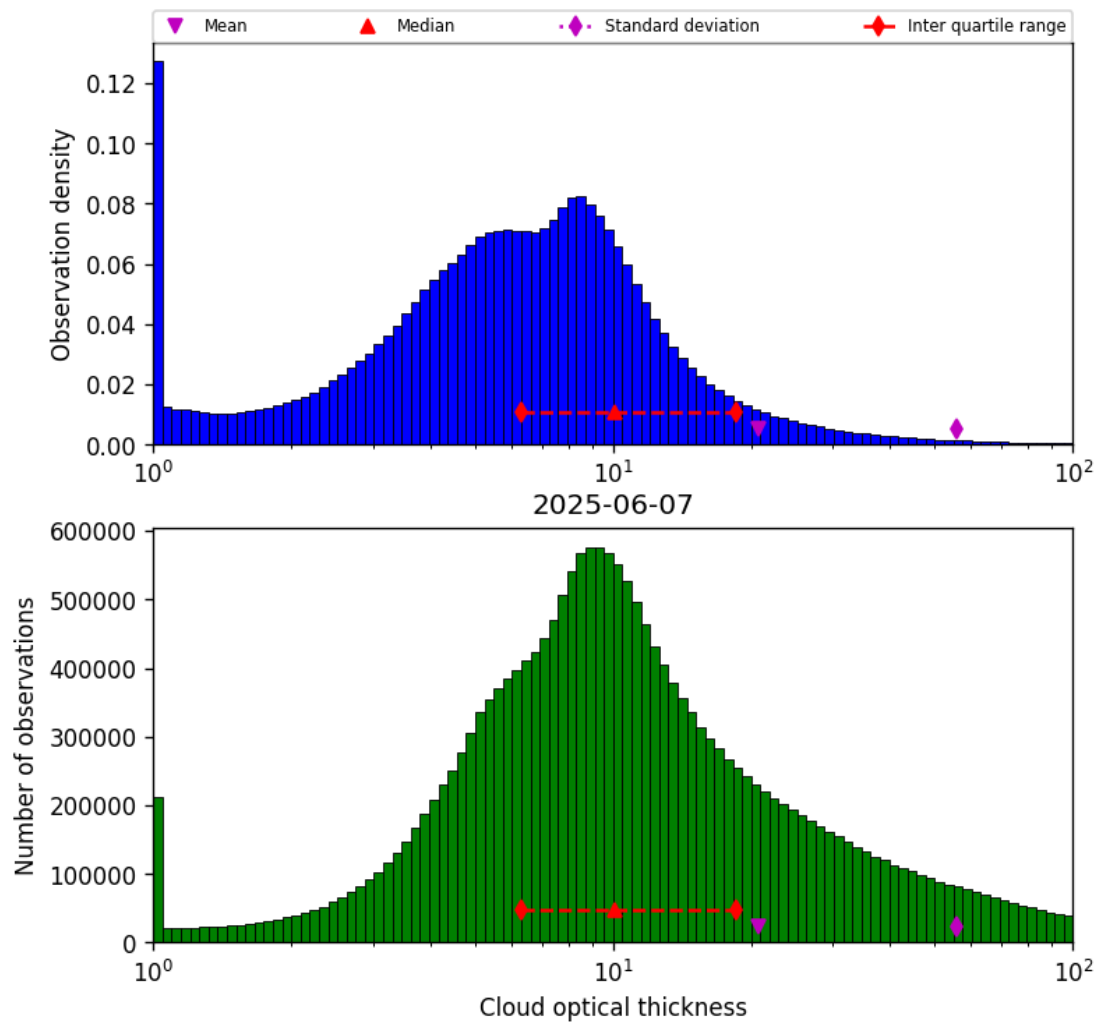
Figure 41: Histogram of “Cloud optical thickness” for 2025-06-06 to 2025-06-08
