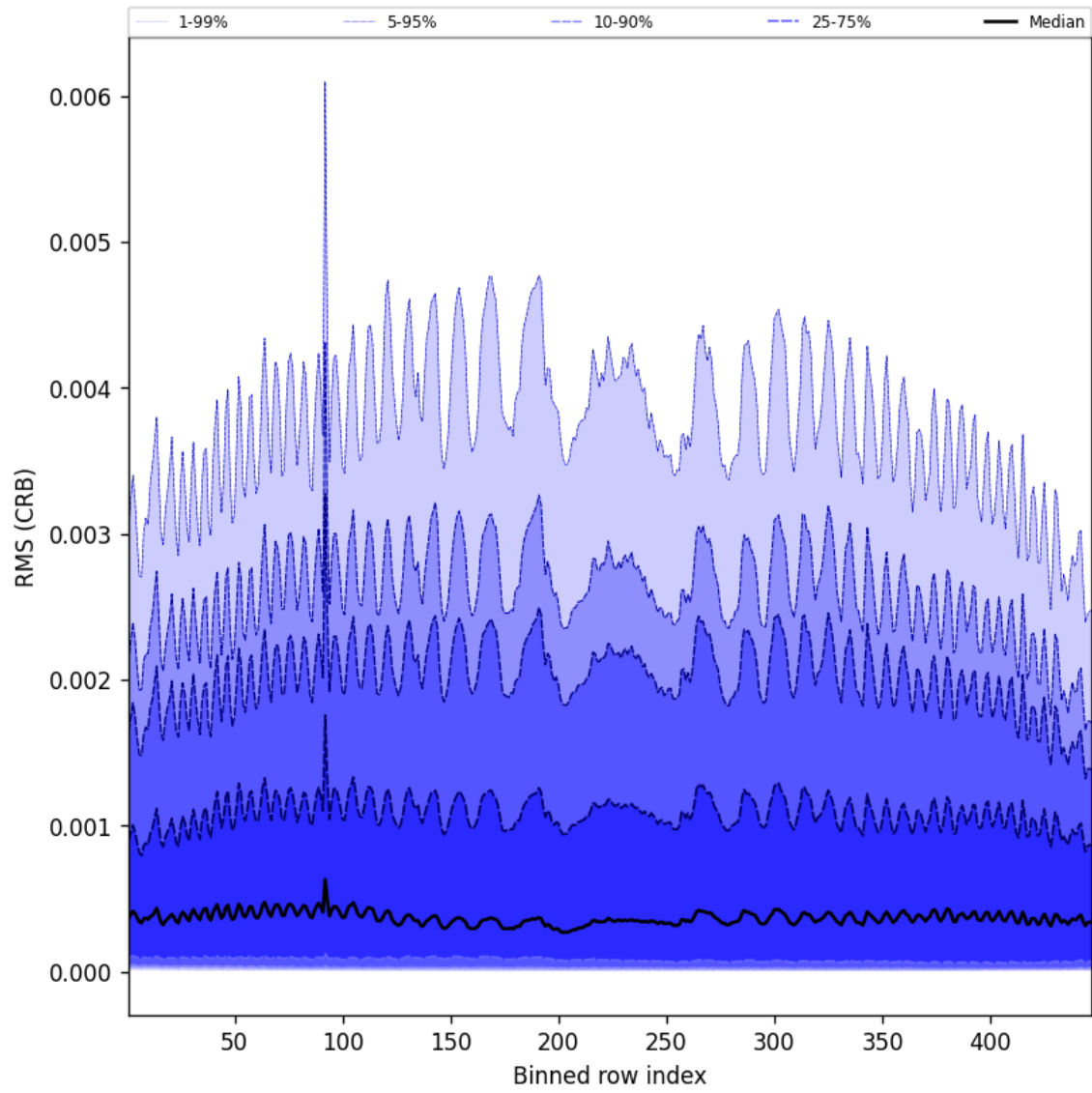
Figure 64: Along track statistics of “RMS (CRB)” for 2025-06-06 to 2025-06-08
