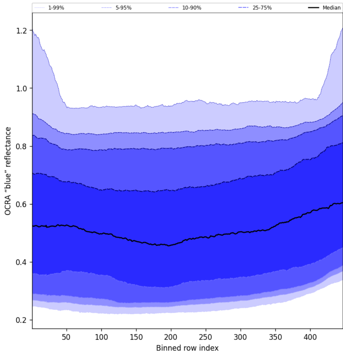
Figure 67: Along track statistics of "OCRA "blue" reflectance" for 2025-06-06 to 2025-06-08
