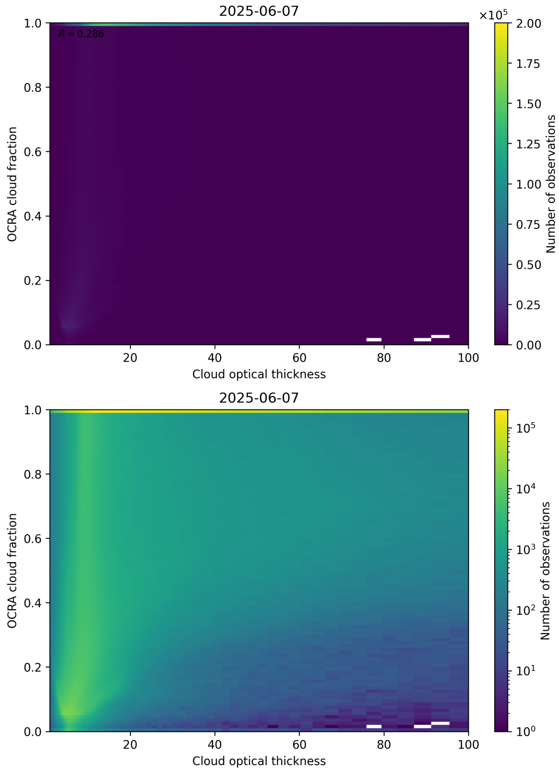
Figure 83: Scatter density plot of “Cloud optical thickness” against “OCRA cloud fraction” for 2025-06-06 to 2025-06-08.
