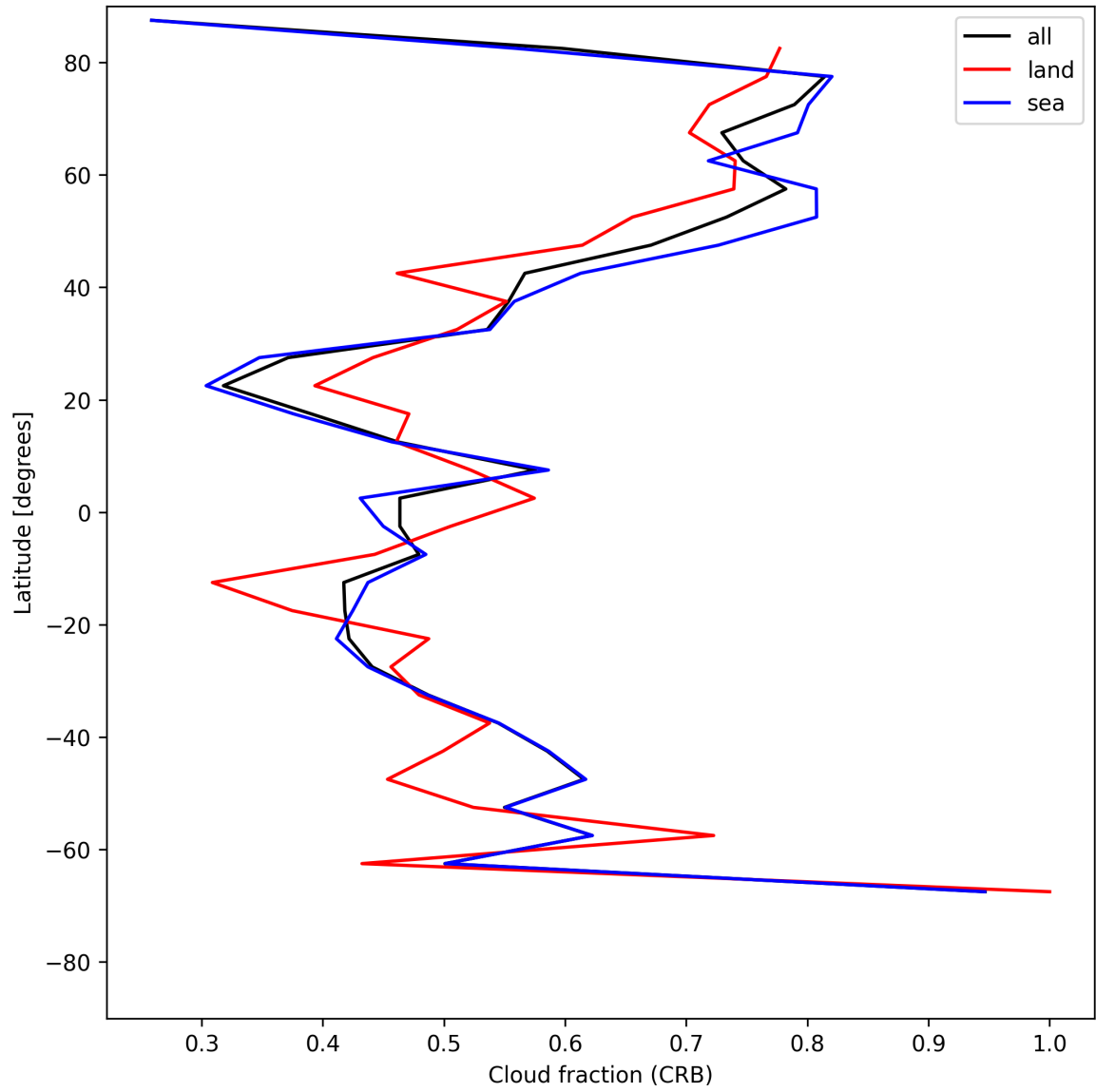
Figure 26: Zonal average of “Cloud fraction (CRB)” for 2025-06-06 to 2025-06-08.
