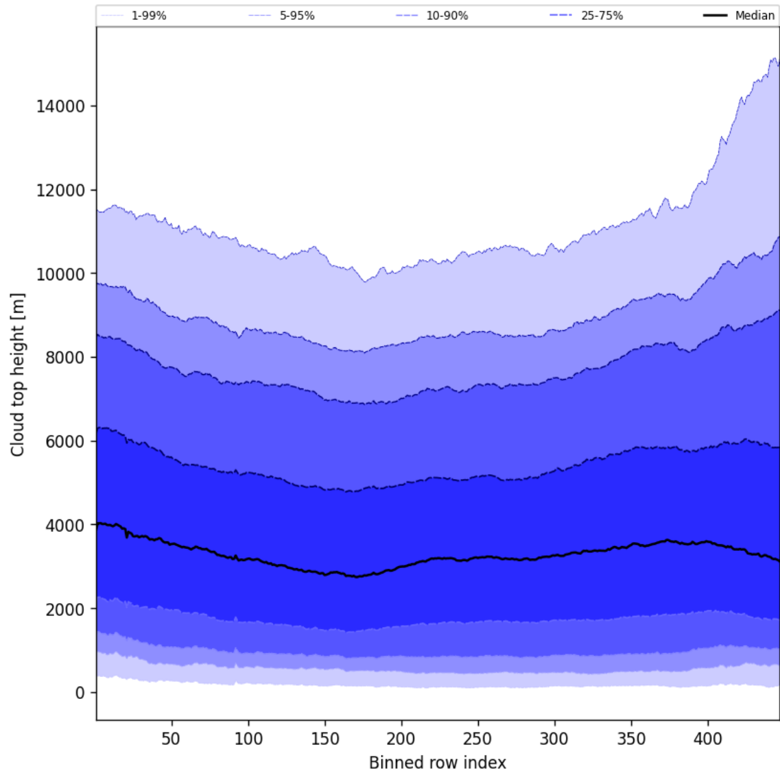
Figure 56: Along track statistics of “Cloud top height” for 2025-06-06 to 2025-06-08
