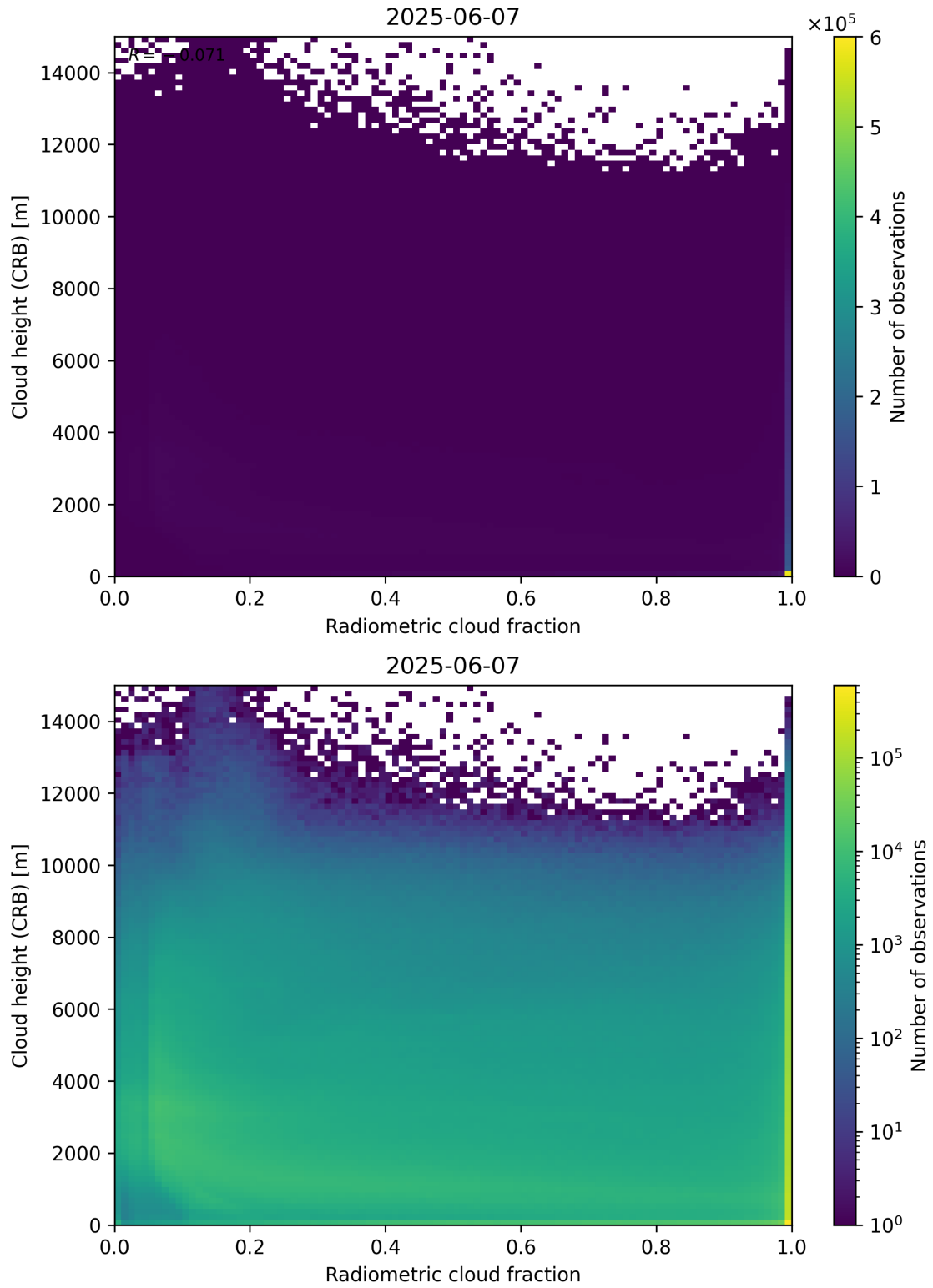
Figure 74: Scatter density plot of “Radiometric cloud fraction” against “Cloud height (CRB)” for 2025-06-06 to 2025-06-08.
