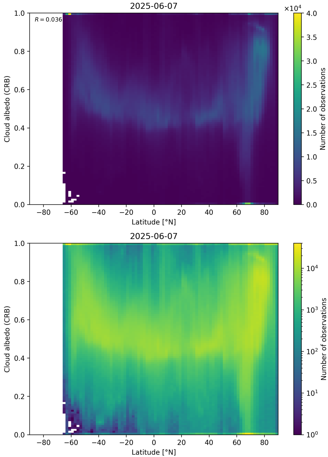
Figure 91: Scatter density plot of “Latitude” against “Cloud albedo (CRB)” for 2025-06-06 to 2025-06-08.
