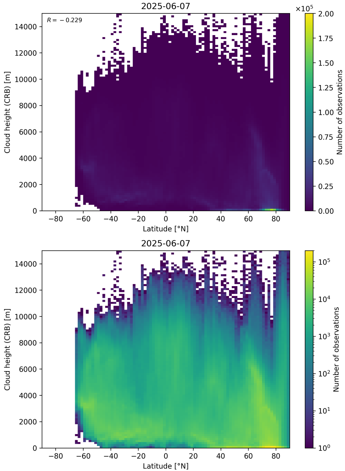
Figure 95: Scatter density plot of “Latitude” against “Cloud height (CRB)” for 2025-06-06 to 2025-06-08.
