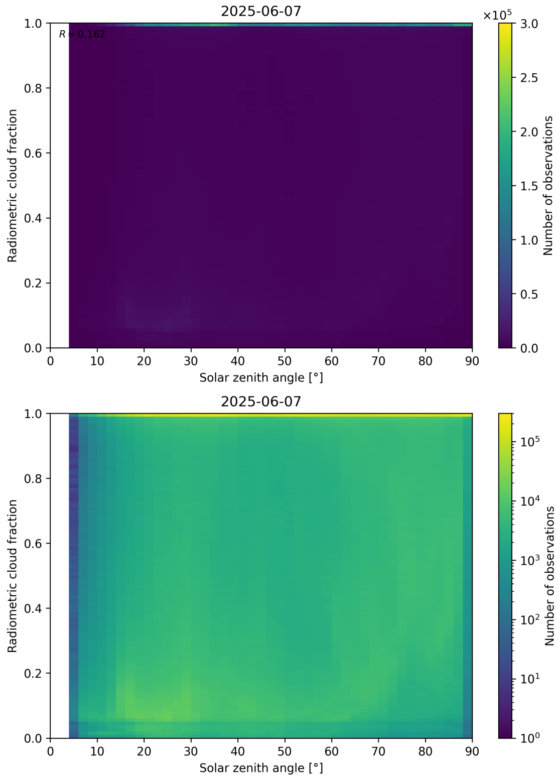
Figure 99: Scatter density plot of “Solar zenith angle” against “Radiometric cloud fraction” for 2025-06-06 to 2025-06-08.
