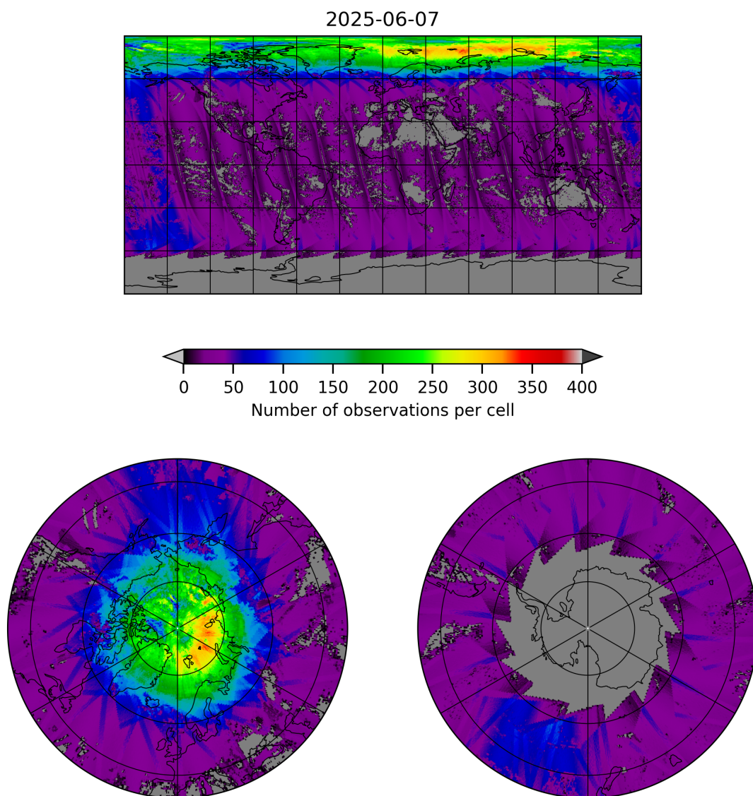
Figure 21: Map of the number of observations for 2025-06-06 to 2025-06-08
