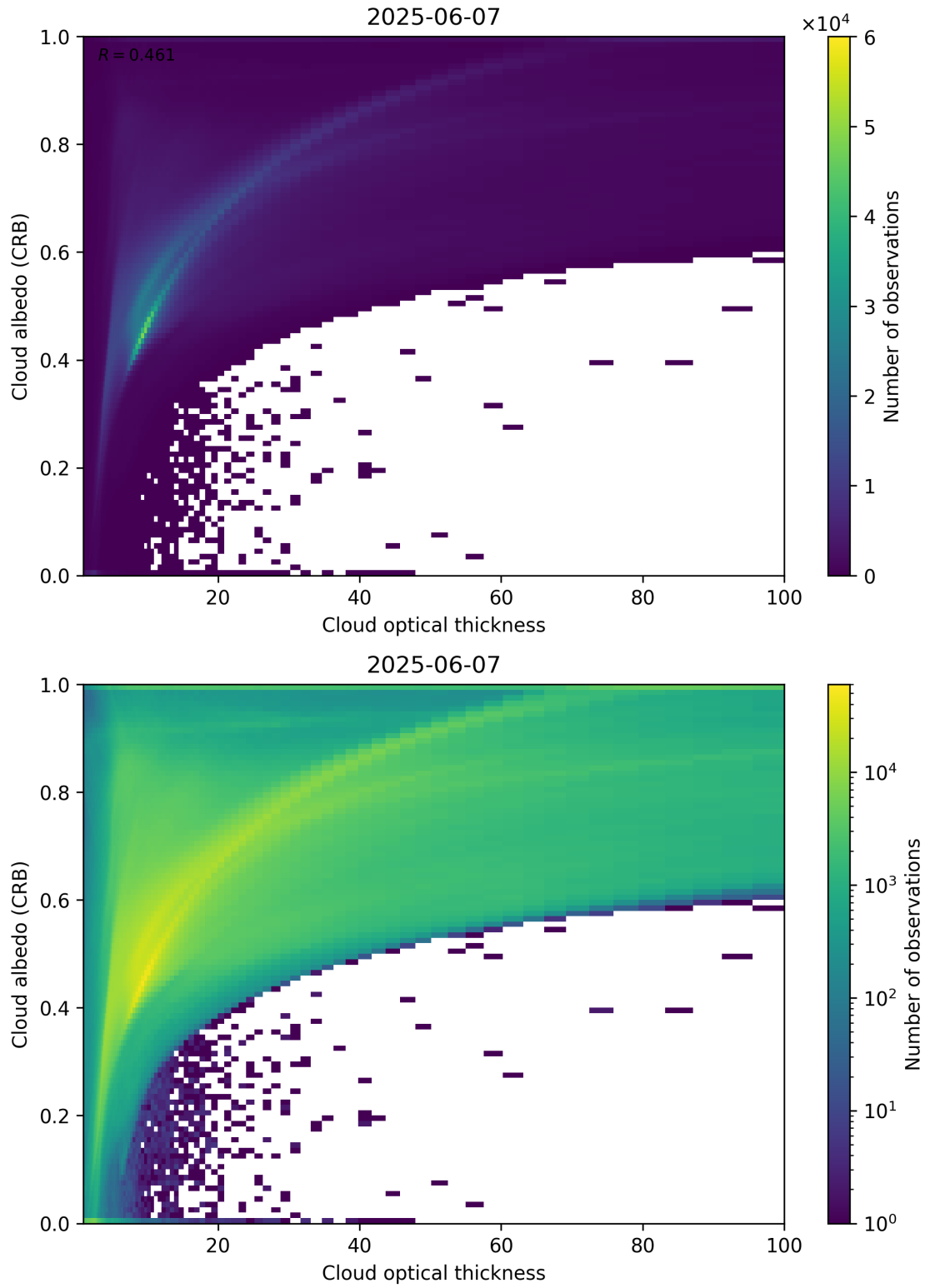
Figure 82: Scatter density plot of “Cloud optical thickness” against “Cloud albedo (CRB)” for 2025-06-06 to 2025-06-08.
