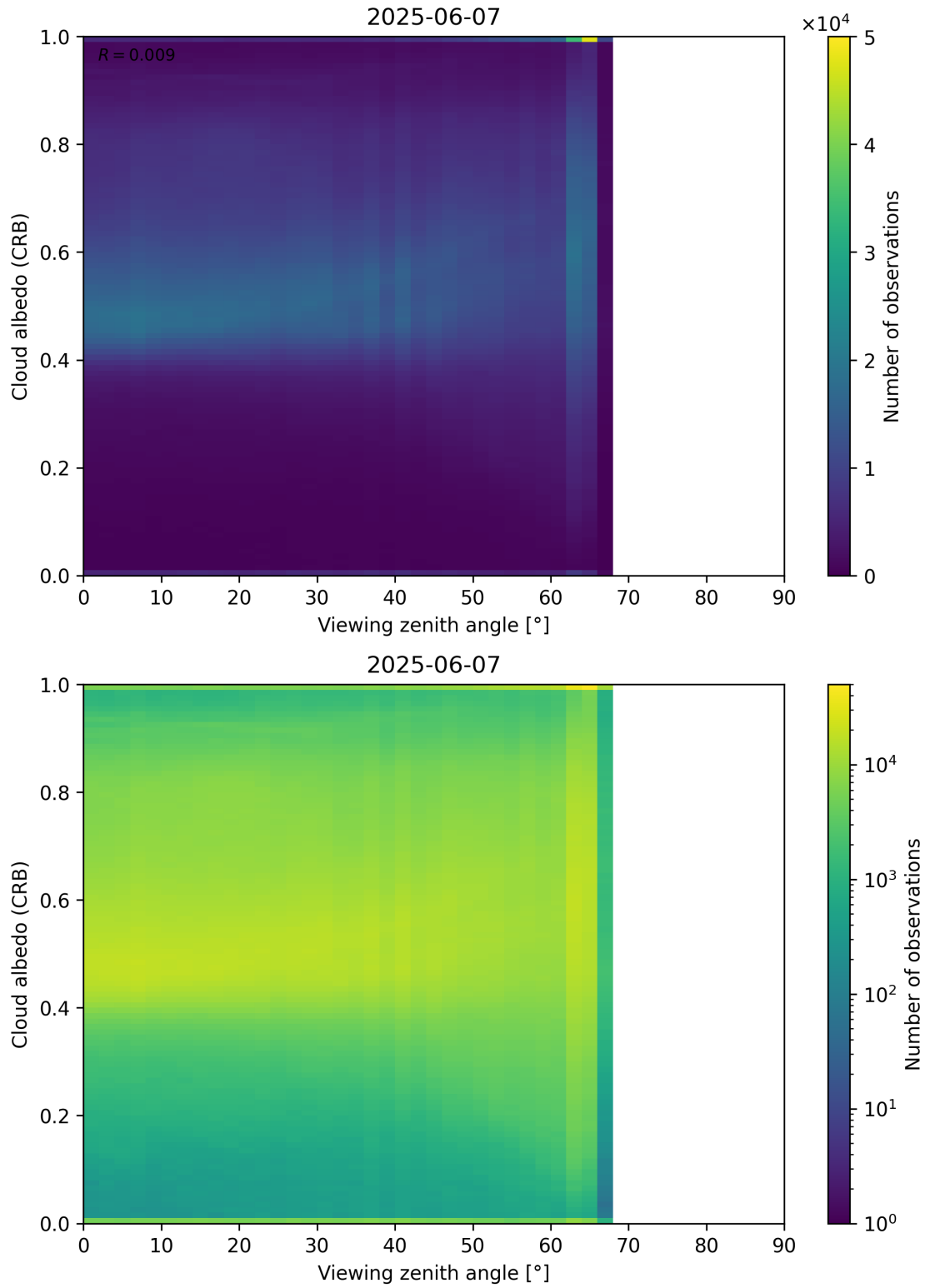
Figure 106: Scatter density plot of “Viewing zenith angle” against “Cloud albedo (CRB)” for 2025-06-06 to 2025-06-08.
