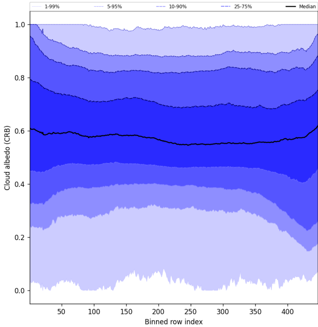
Figure 60: Along track statistics of “Cloud albedo (CRB)” for 2025-06-06 to 2025-06-08
