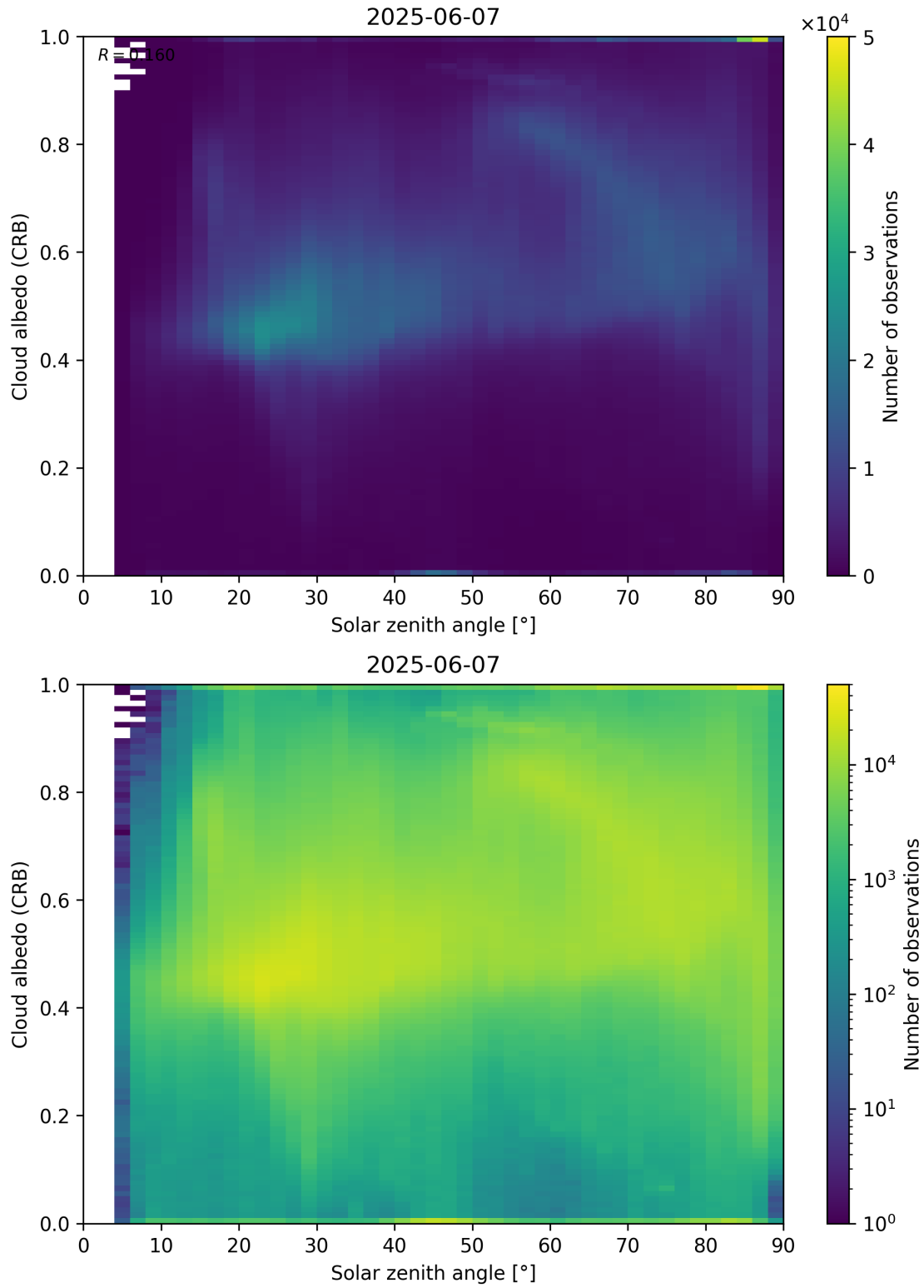
Figure 98: Scatter density plot of “Solar zenith angle” against “Cloud albedo (CRB)” for 2025-06-06 to 2025-06-08.
