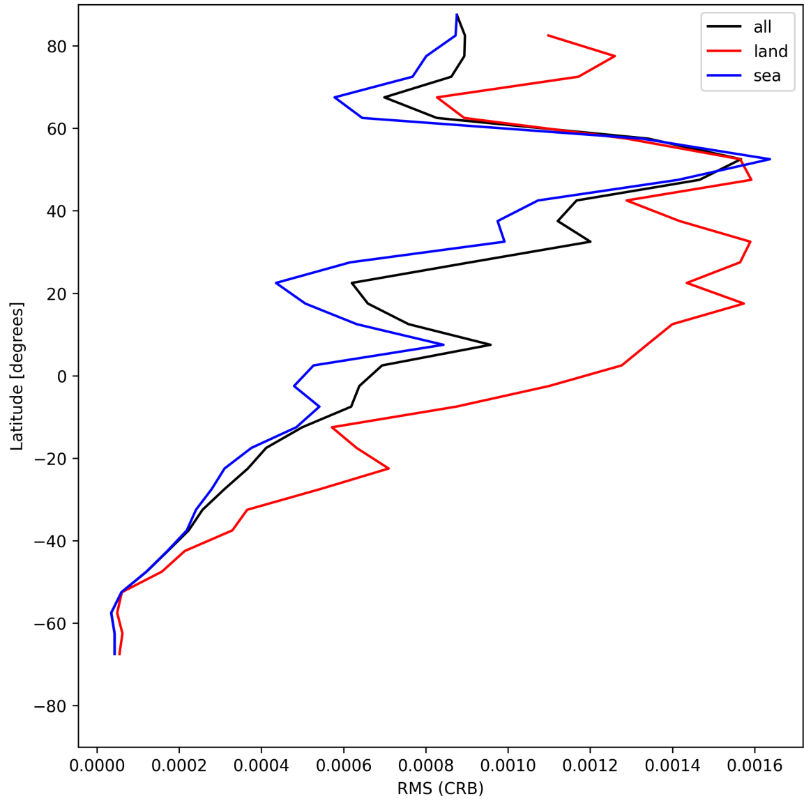
Figure 32: Zonal average of “RMS (CRB)” for 2025-06-06 to 2025-06-08.
