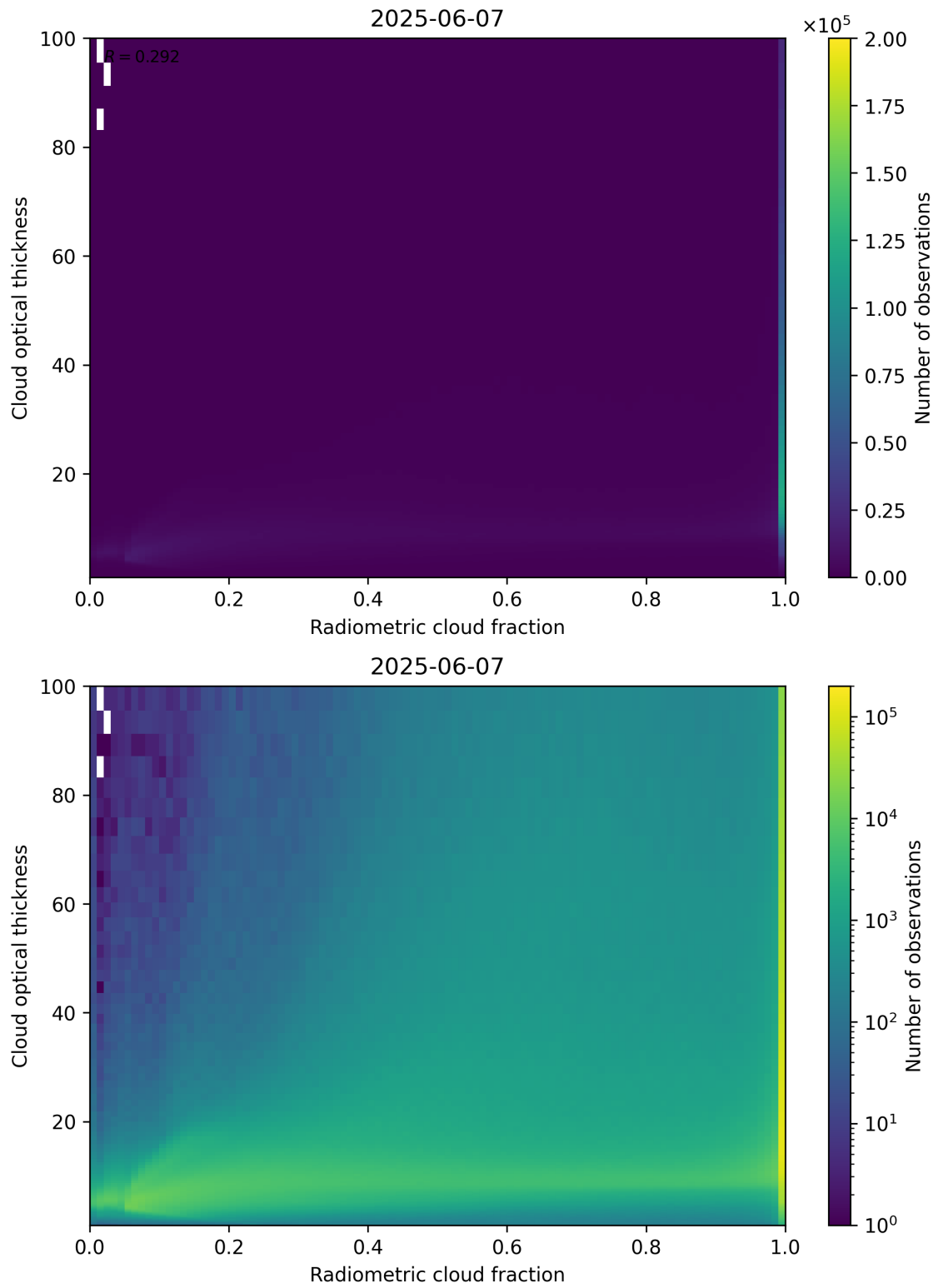
Figure 75: Scatter density plot of “Radiometric cloud fraction” against “Cloud optical thickness” for 2025-06-06 to 2025-06-08.
