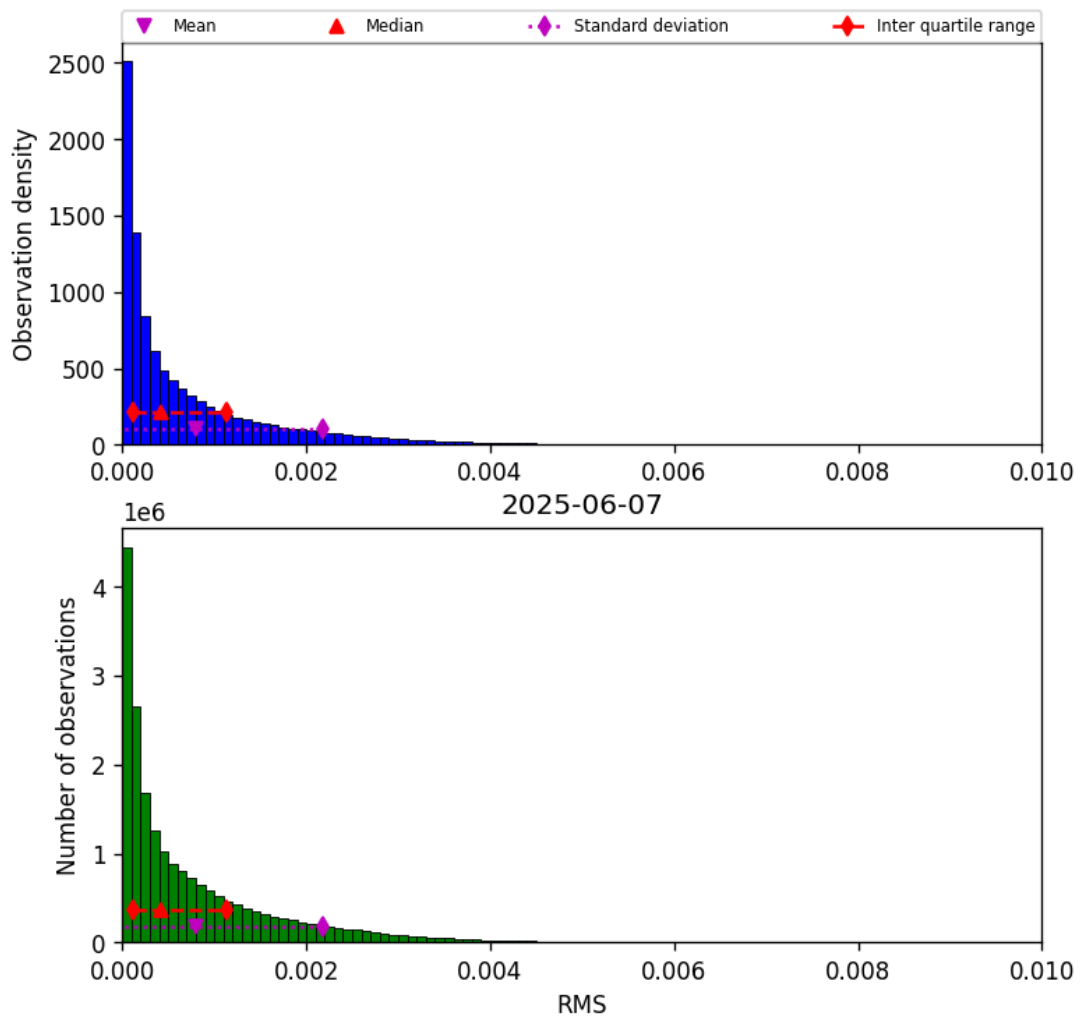
Figure 47: Histogram of “RMS” for 2025-06-06 to 2025-06-08
