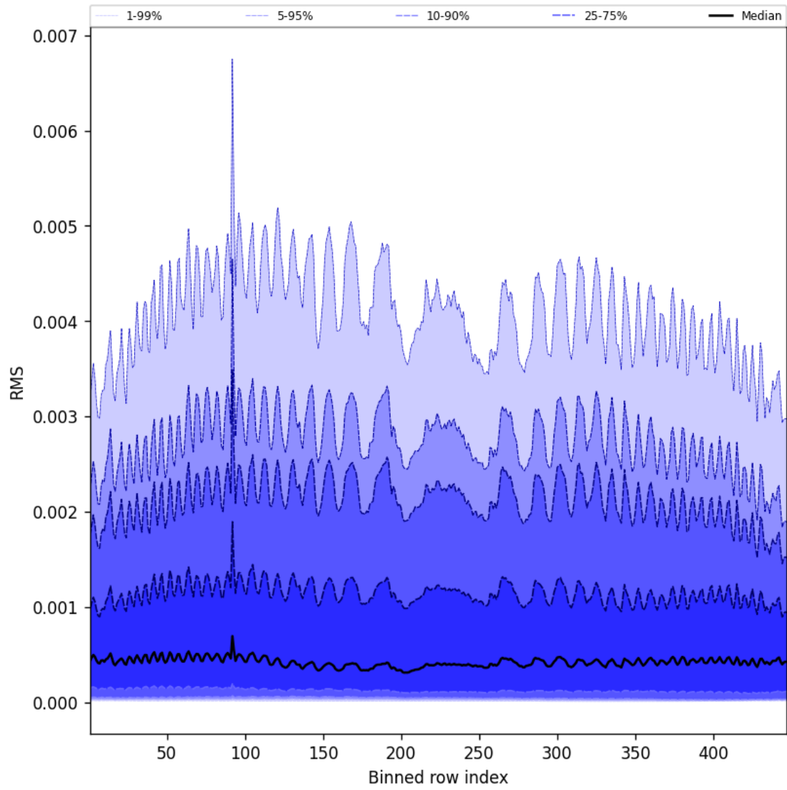
Figure 63: Along track statistics of “RMS” for 2025-06-06 to 2025-06-08
