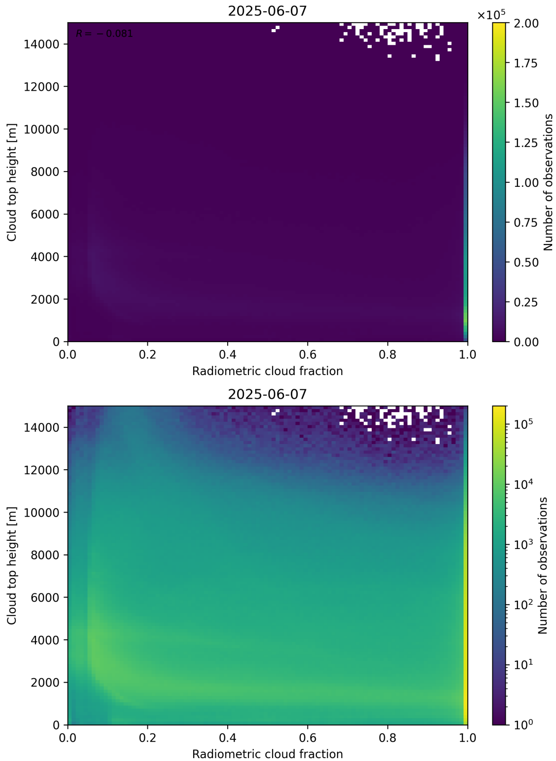
Figure 76: Scatter density plot of “Radiometric cloud fraction” against “Cloud top height” for 2025-06-06 to 2025-06-08.
