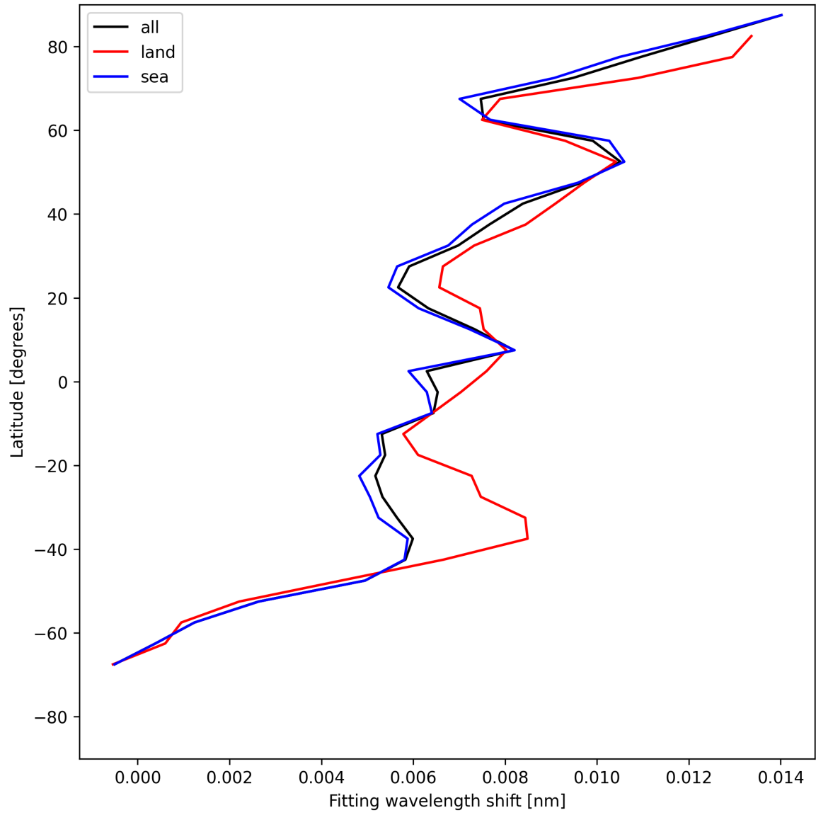
Figure 33: Zonal average of “Fitting wavelength shift” for 2025-06-06 to 2025-06-08.
