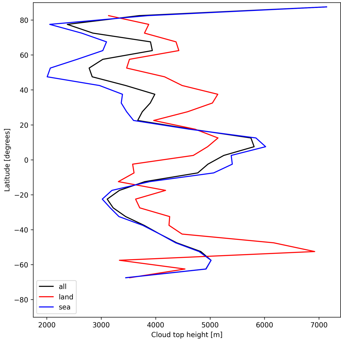
Figure 24: Zonal average of “Cloud top height” for 2025-06-06 to 2025-06-08.
