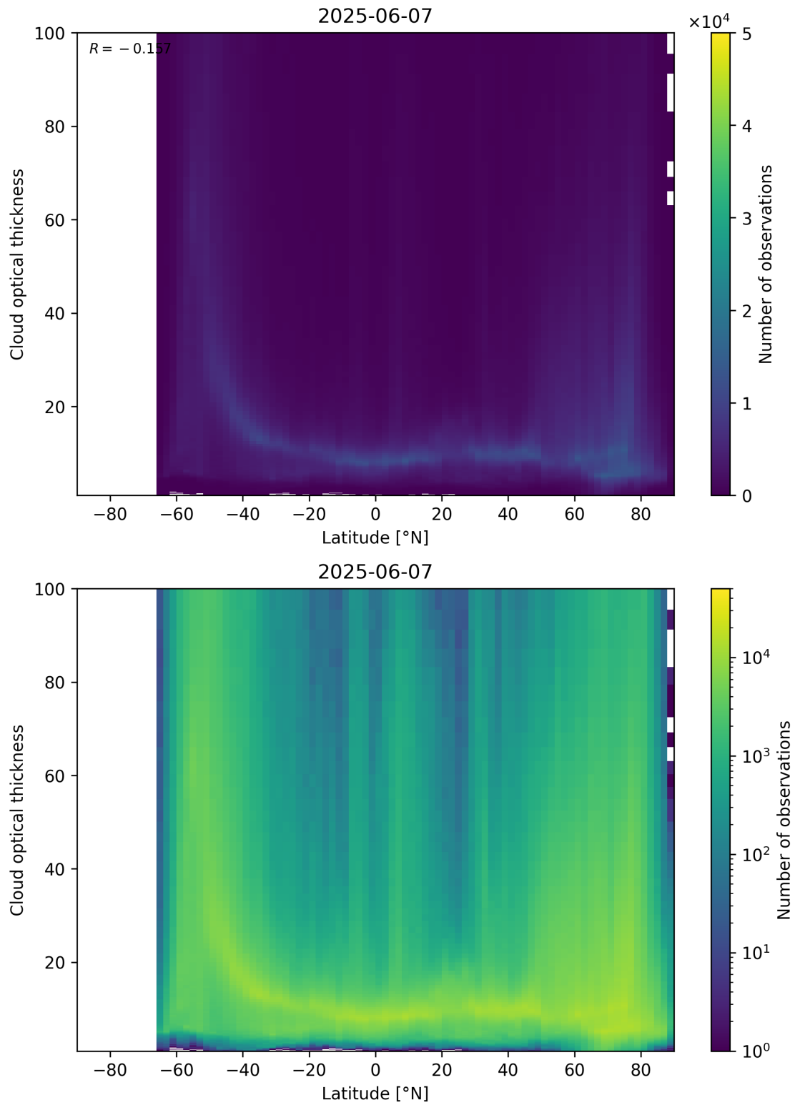
Figure 96: Scatter density plot of “Latitude” against “Cloud optical thickness” for 2025-06-06 to 2025-06-08.
