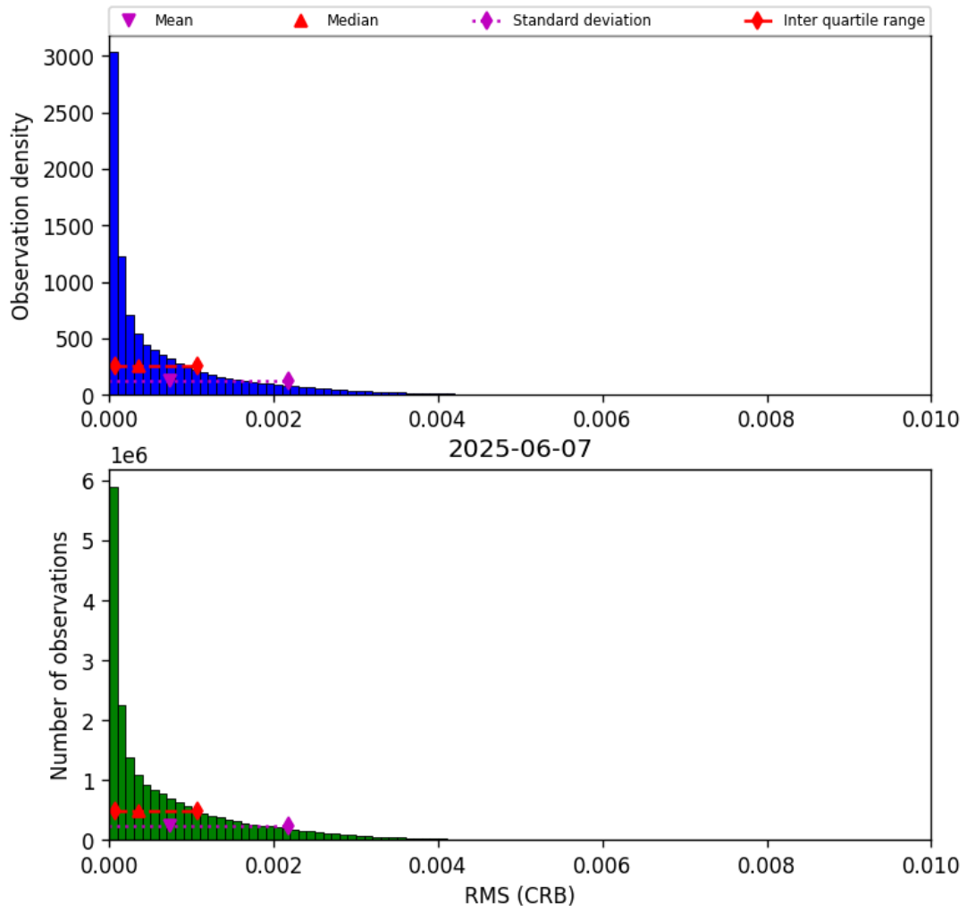
Figure 48: Histogram of “RMS (CRB)” for 2025-06-06 to 2025-06-08
