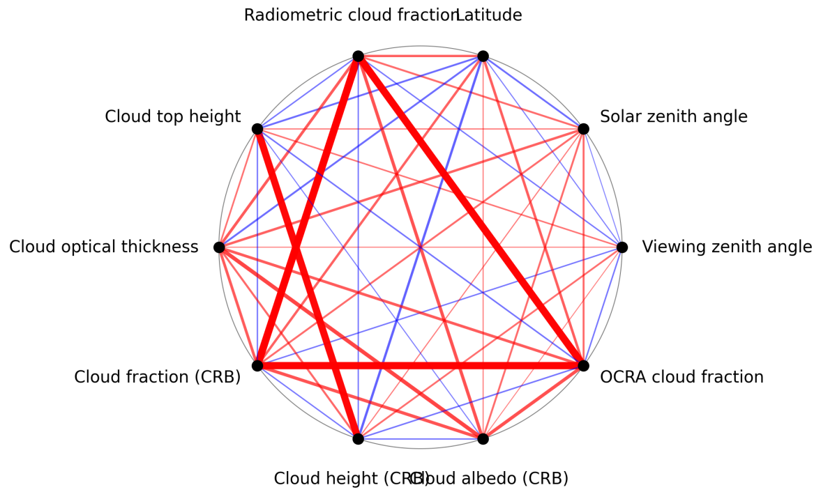
Figure 1: Map of correlation graph for 2025-06-06 to 2025-06-08.
