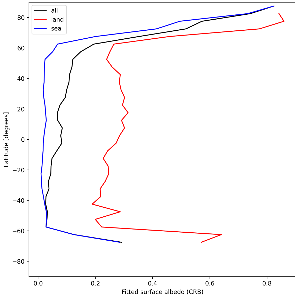
Figure 30: Zonal average of “Fitted surface albedo (CRB)” for 2025-06-06 to 2025-06-08.
