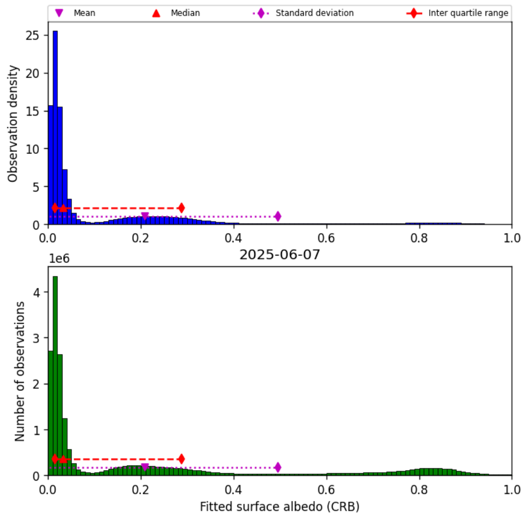
Figure 46: Histogram of “Fitted surface albedo (CRB)” for 2025-06-06 to 2025-06-08
