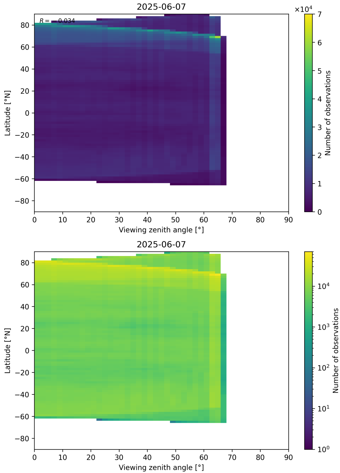
Figure 113: Scatter density plot of “Viewing zenith angle” against “Latitude” for 2025-06-06 to 2025-06-08.
