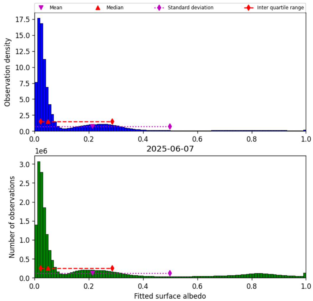
Figure 45: Histogram of “Fitted surface albedo” for 2025-06-06 to 2025-06-08
