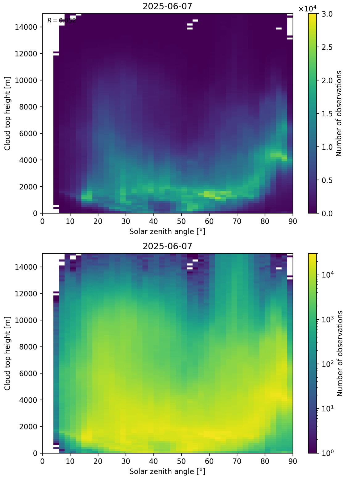
Figure 104: Scatter density plot of “Solar zenith angle” against “Cloud top height” for 2025-06-06 to 2025-06-08.
