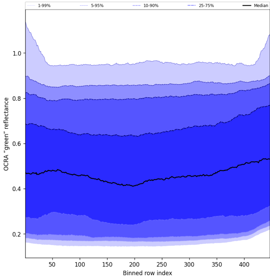
Figure 68: Along track statistics of “OCRA “green” reflectance” for 2025-06-06 to 2025-06-08
