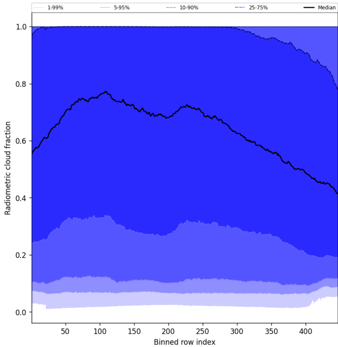
Figure 55: Along track statistics of “Radiometric cloud fraction” for 2025-06-06 to 2025-06-08
