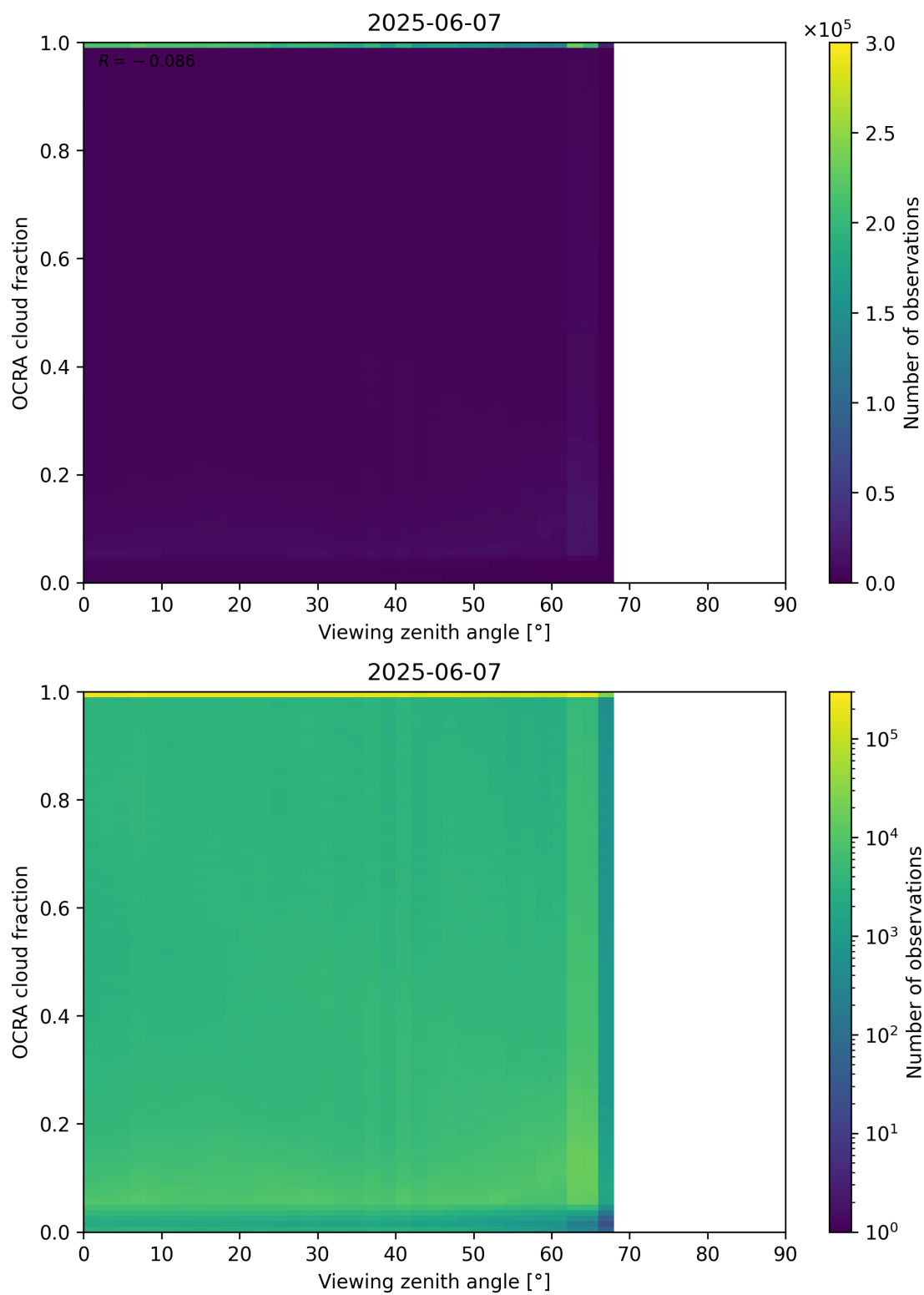
Figure 108: Scatter density plot of “Viewing zenith angle” against “OCRA cloud fraction” for 2025-06-06 to 2025-06-08.
