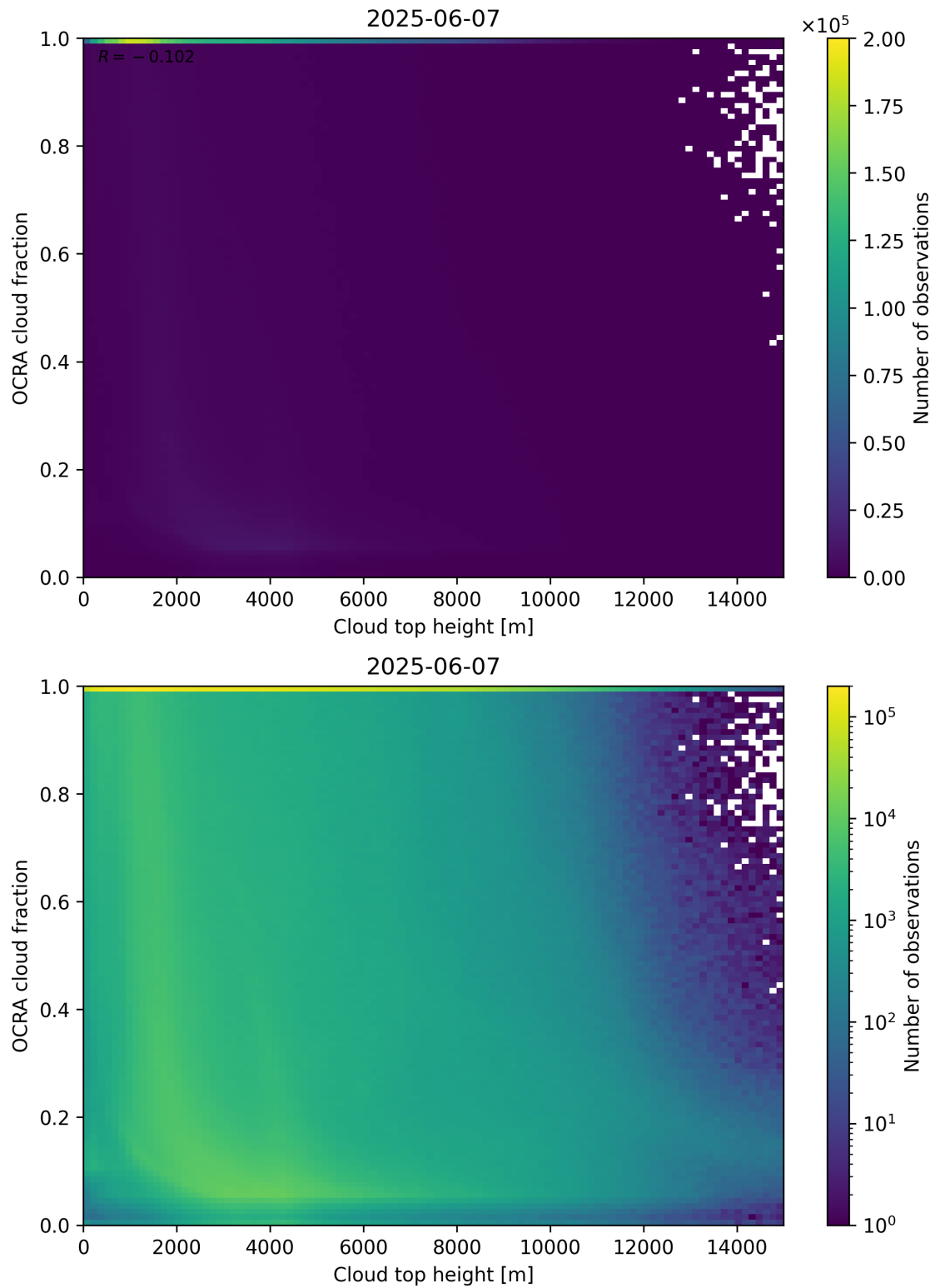
Figure 87: Scatter density plot of “Cloud top height” against “OCRA cloud fraction” for 2025-06-06 to 2025-06-08.
