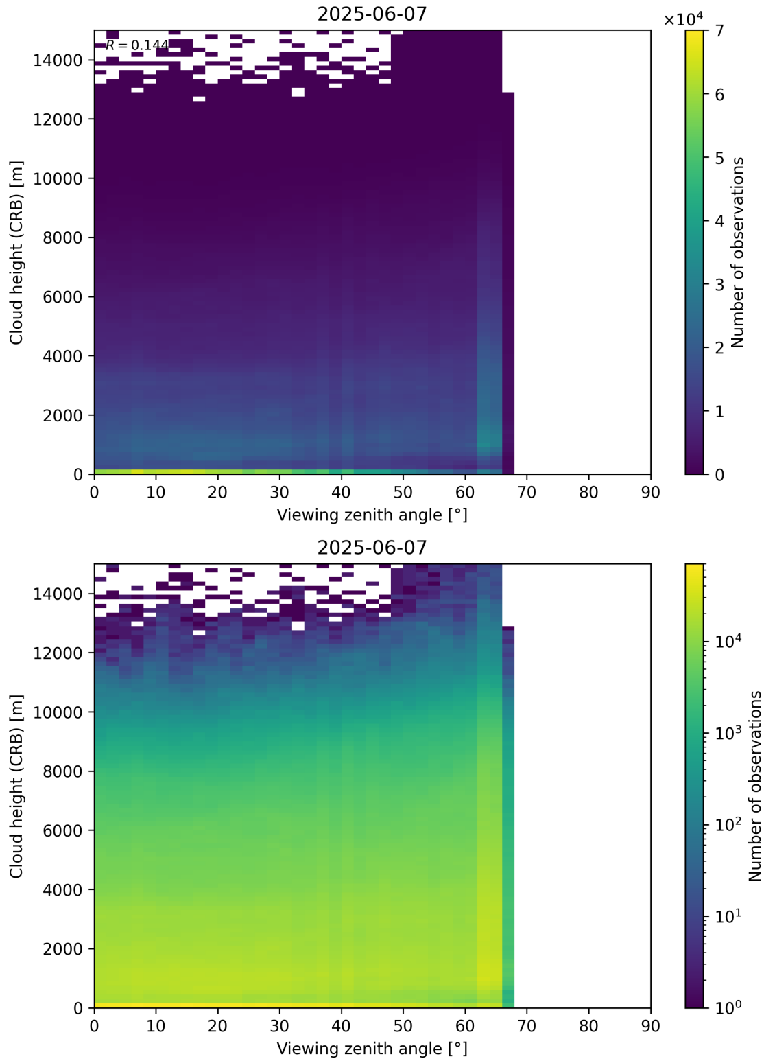
Figure 110: Scatter density plot of “Viewing zenith angle” against “Cloud height (CRB)” for 2025-06-06 to 2025-06-08.
