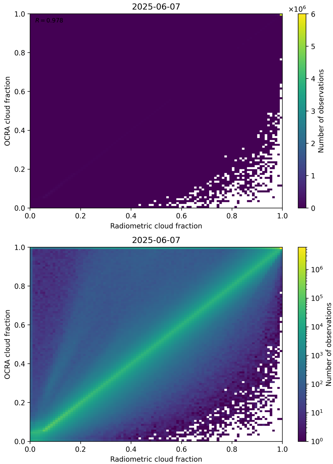
Figure 72: Scatter density plot of “Radiometric cloud fraction” against “OCRA cloud fraction” for 2025-06-06 to 2025-06-08.
