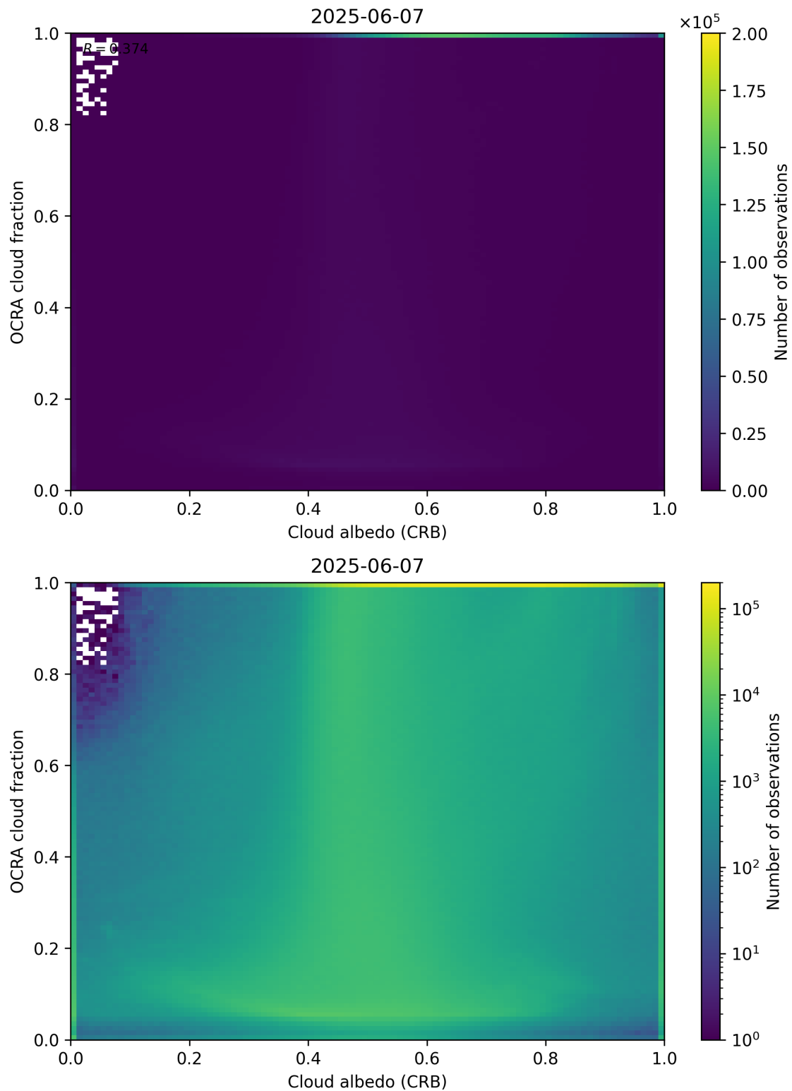
Figure 70: Scatter density plot of “Cloud albedo (CRB)” against “OCRA cloud fraction” for 2025-06-06 to 2025-06-08.
