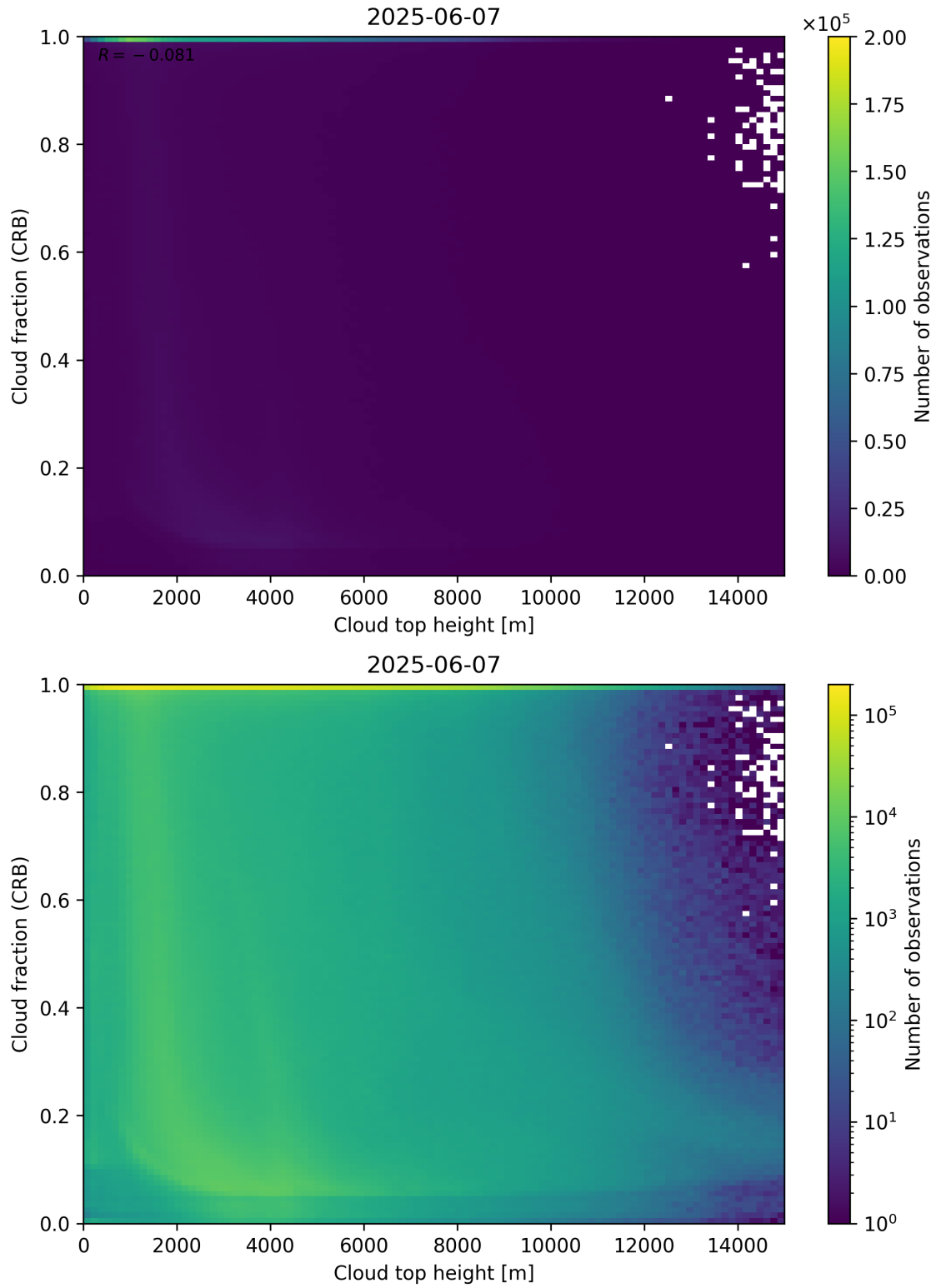
Figure 88: Scatter density plot of “Cloud top height” against “Cloud fraction (CRB)” for 2025-06-06 to 2025-06-08.
