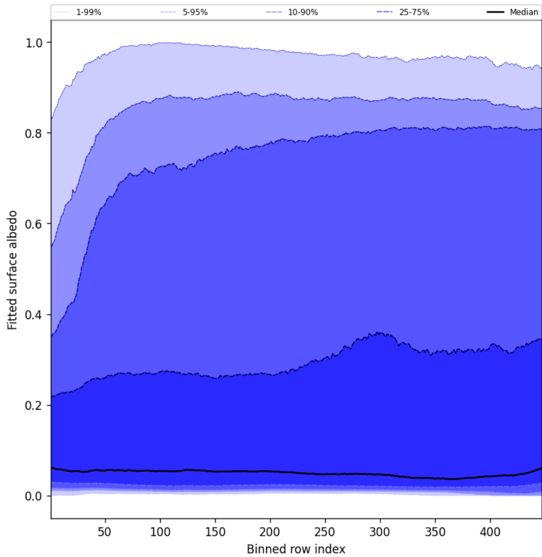
Figure 61: Along track statistics of “Fitted surface albedo” for 2025-06-06 to 2025-06-08
