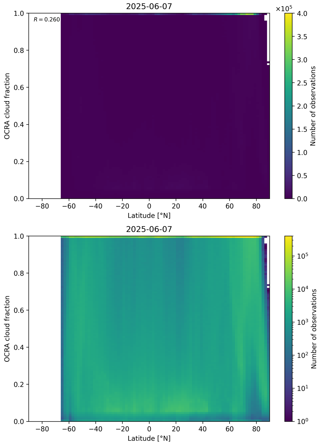
Figure 93: Scatter density plot of “Latitude” against “OCRA cloud fraction” for 2025-06-06 to 2025-06-08.
