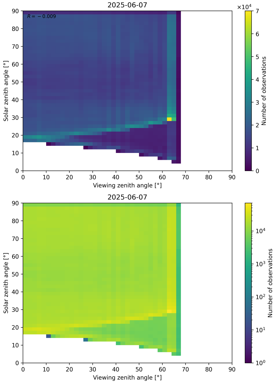
Figure 114: Scatter density plot of “Viewing zenith angle” against “Solar zenith angle” for 2025-06-06 to 2025-06-08.
