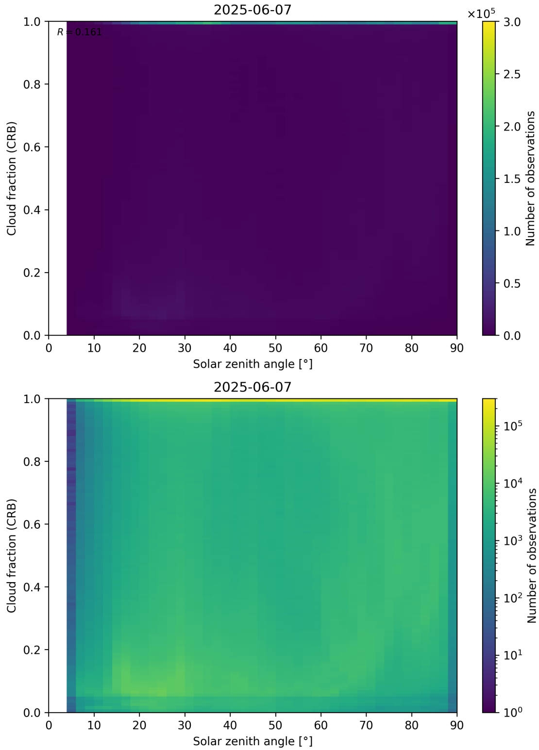
Figure 101: Scatter density plot of “Solar zenith angle” against “Cloud fraction (CRB)” for 2025-06-06 to 2025-06-08.
