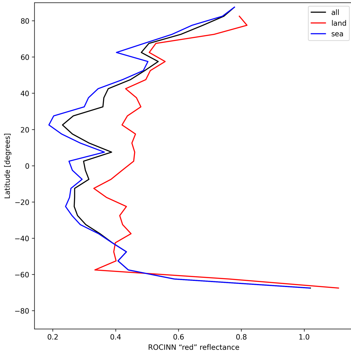
Figure 37: Zonal average of “ROCINN “red” reflectance” for 2025-06-06 to 2025-06-08.
