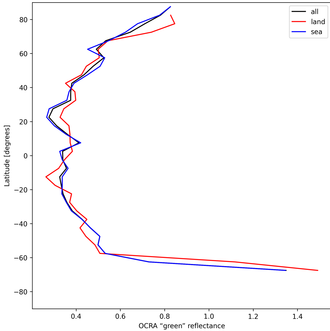
Figure 36: Zonal average of “OCRA “green” reflectance” for 2025-06-06 to 2025-06-08.
