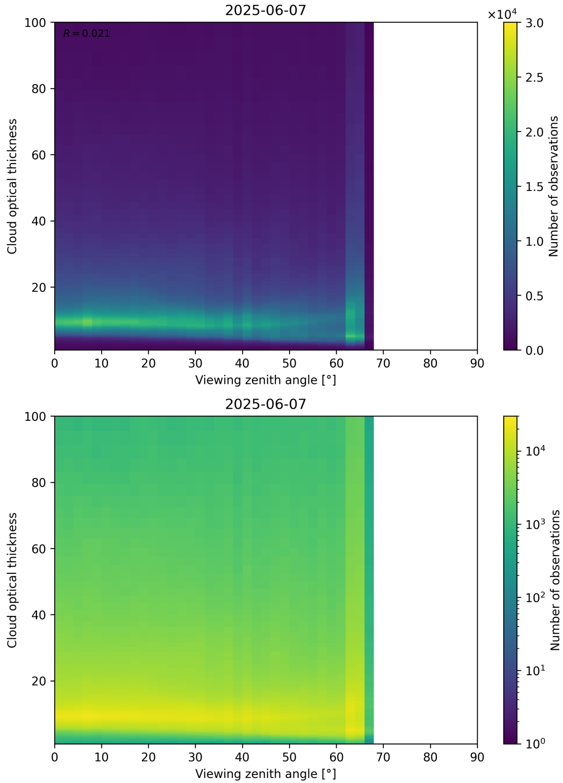
Figure 111: Scatter density plot of “Viewing zenith angle” against “Cloud optical thickness” for 2025-06-06 to 2025-06-08.
