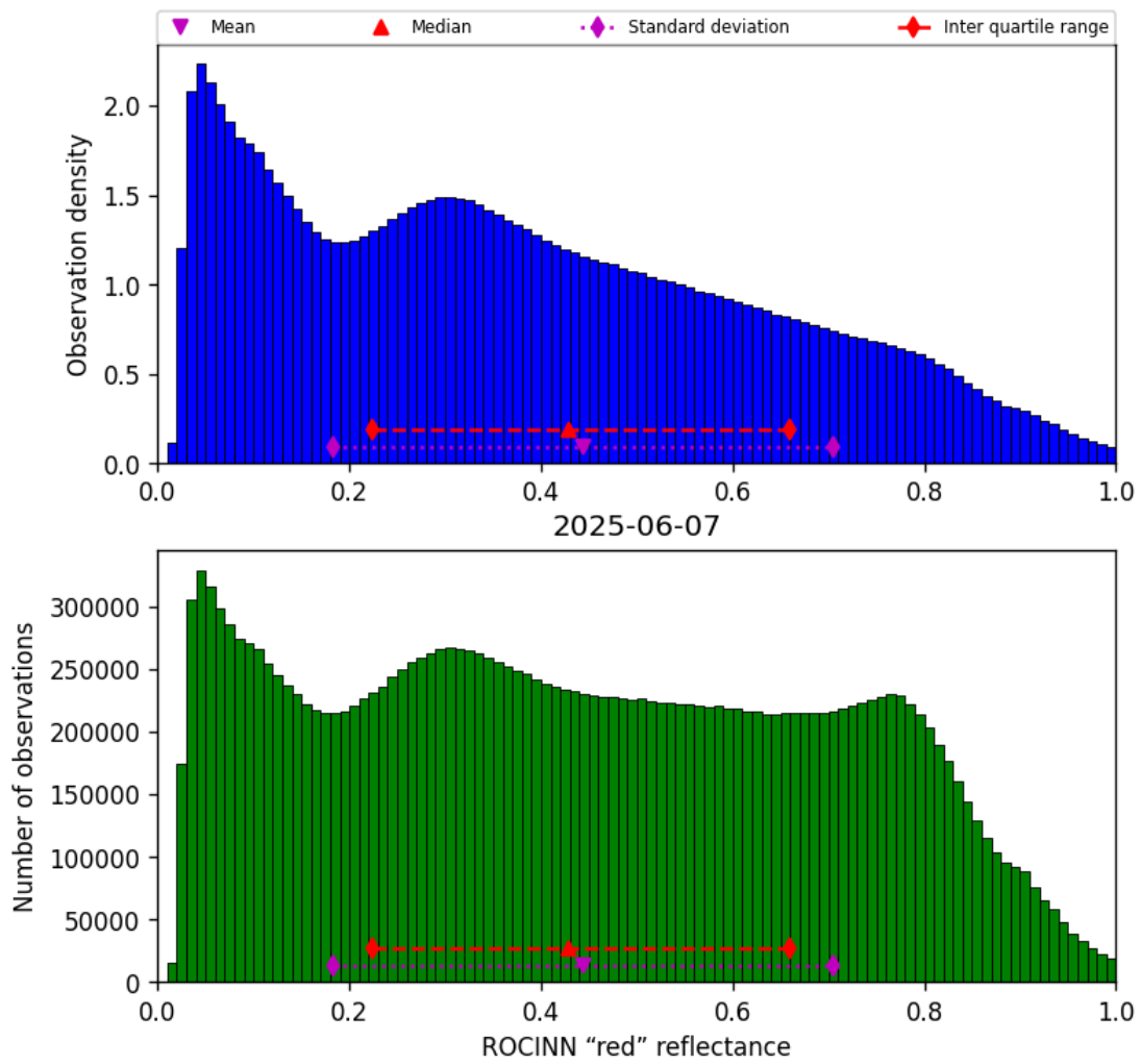
Figure 53: Histogram of “ROCINN “red” reflectance” for 2025-06-06 to 2025-06-08
