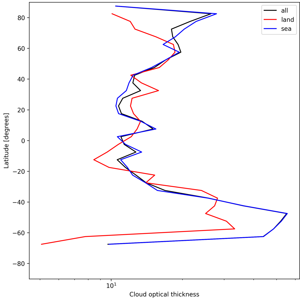
Figure 25: Zonal average of “Cloud optical thickness” for 2025-06-06 to 2025-06-08.
