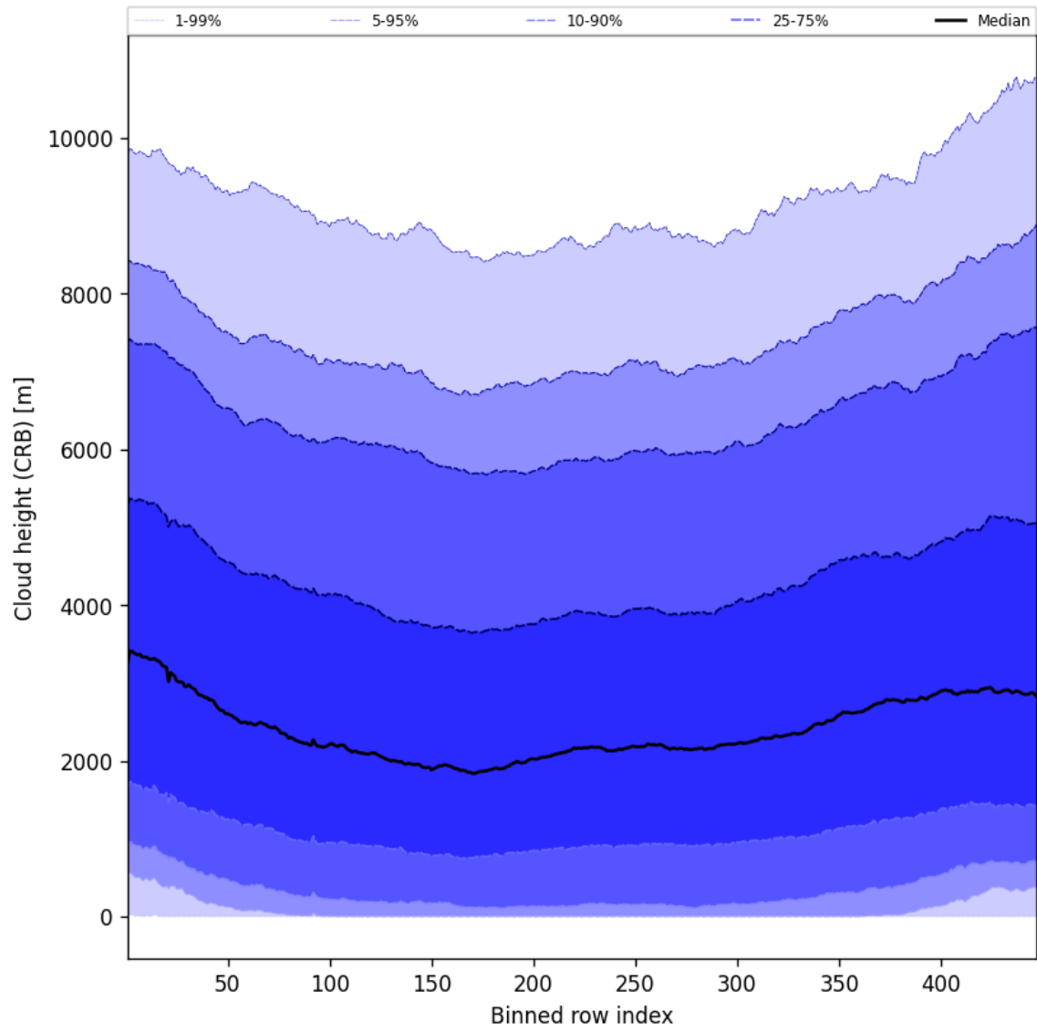
Figure 59: Along track statistics of “Cloud height (CRB)” for 2025-06-06 to 2025-06-08
