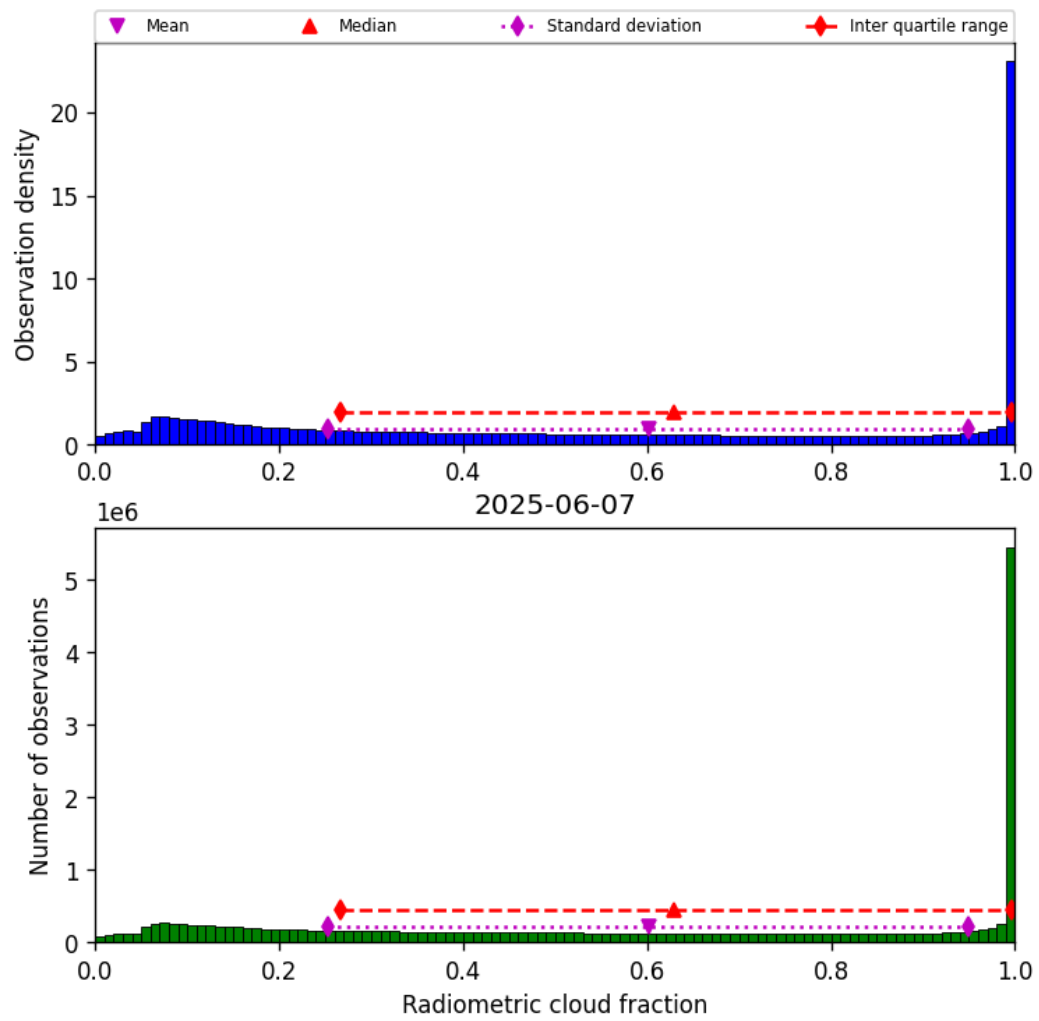
Figure 39: Histogram of “Radiometric cloud fraction” for 2025-06-06 to 2025-06-08
