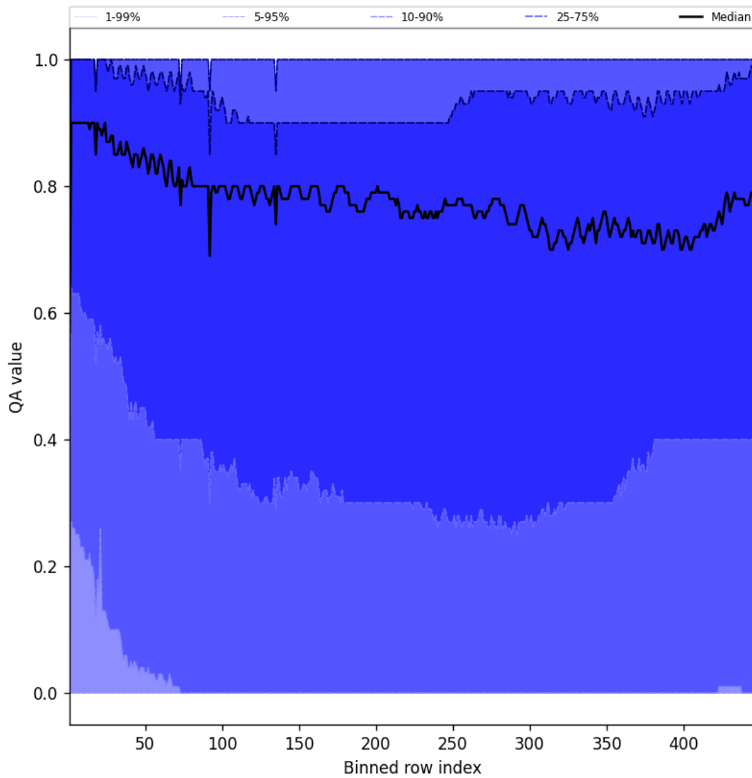
Figure 54: Along track statistics of “QA value” for 2025-06-06 to 2025-06-08
