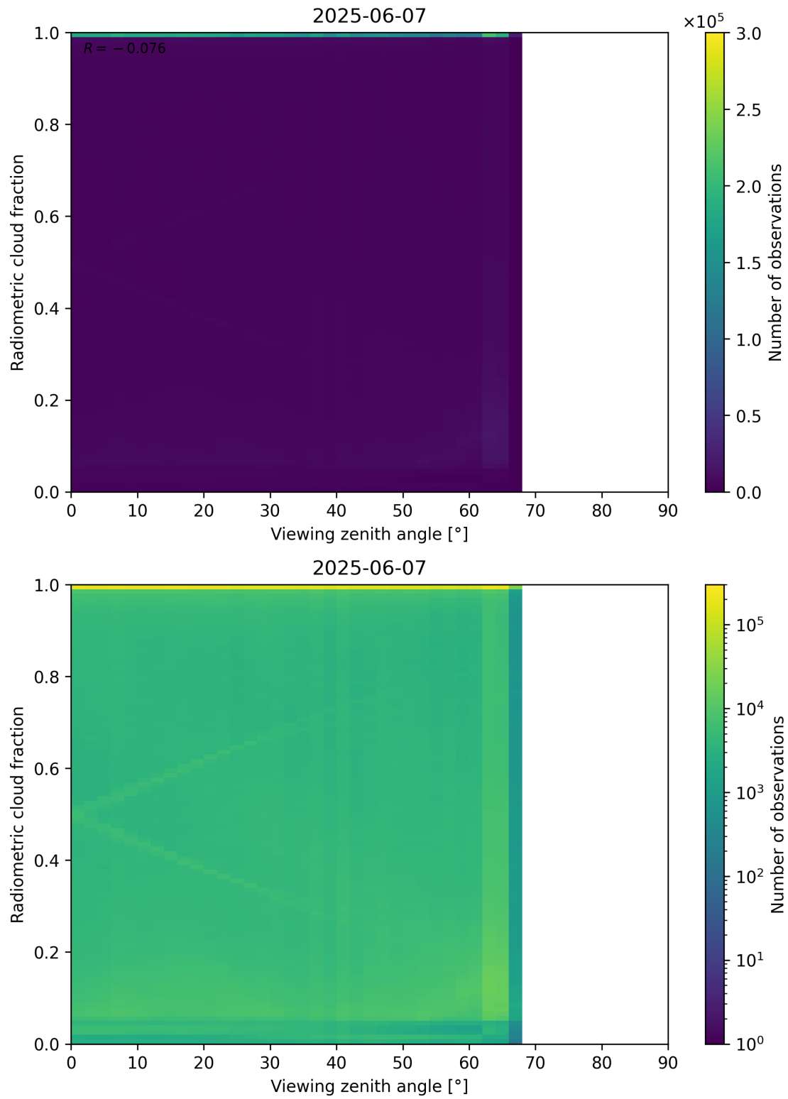
Figure 107: Scatter density plot of “Viewing zenith angle” against “Radiometric cloud fraction” for 2025-06-06 to 2025-06-08.
