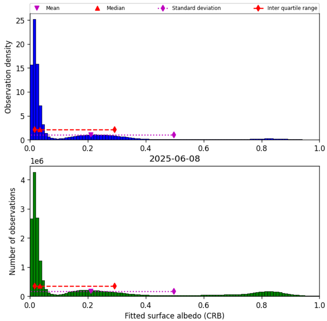
Figure 46: Histogram of “Fitted surface albedo (CRB)” for 2025-06-07 to 2025-06-09
