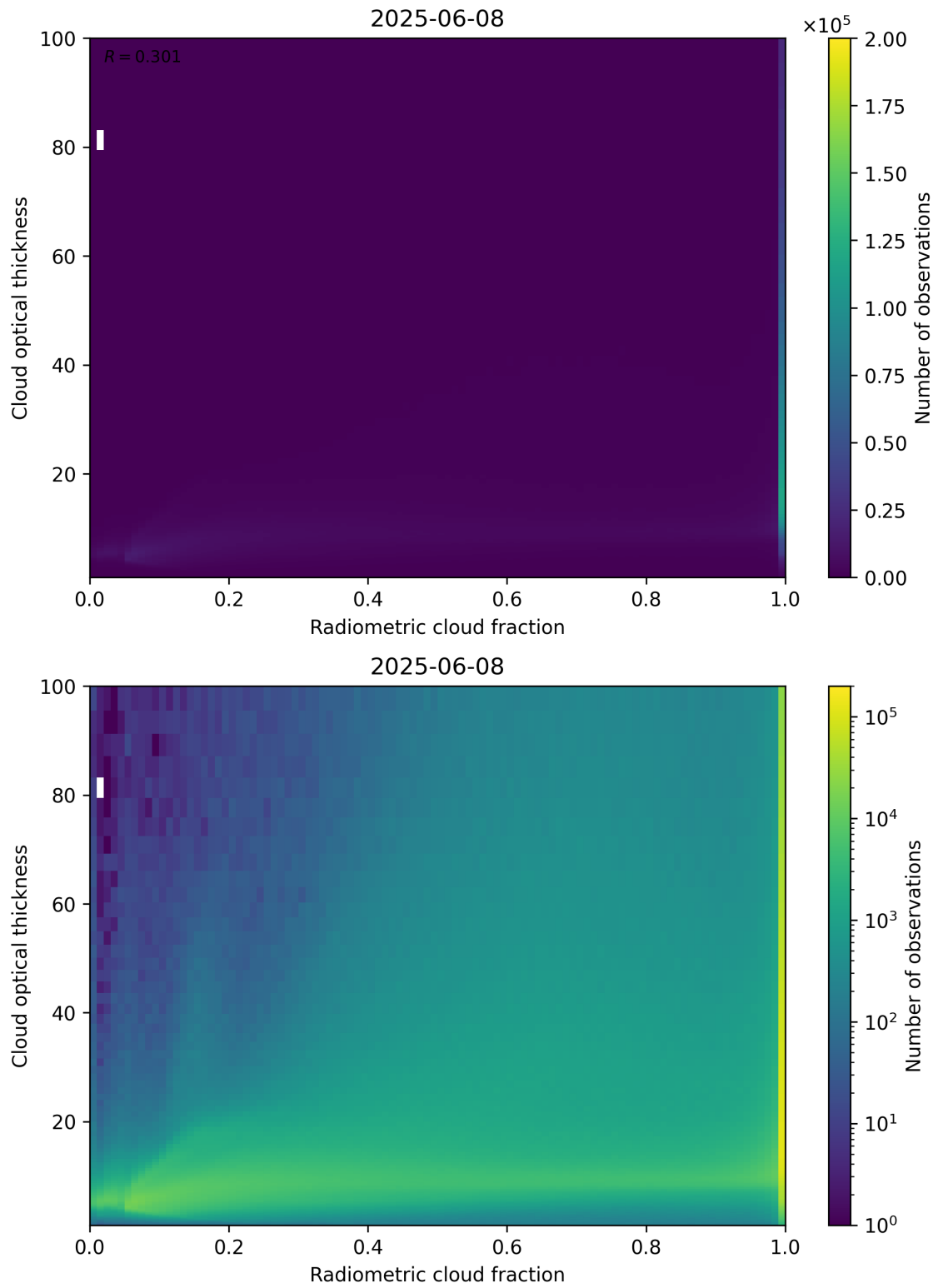
Figure 75: Scatter density plot of “Radiometric cloud fraction” against “Cloud optical thickness” for 2025-06-07 to 2025-06-09.
