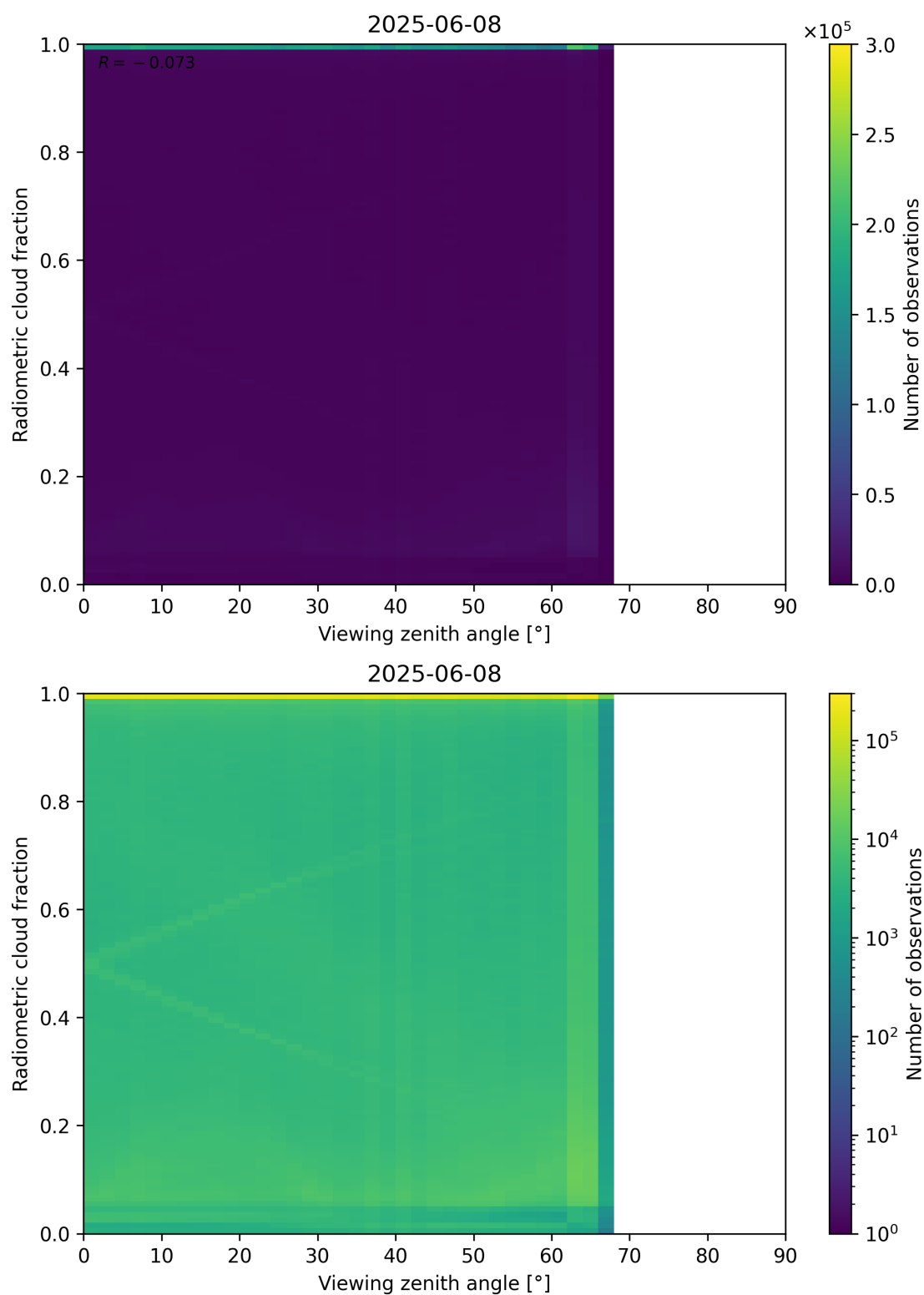
Figure 107: Scatter density plot of “Viewing zenith angle” against “Radiometric cloud fraction” for 2025-06-07 to 2025-06-09.
