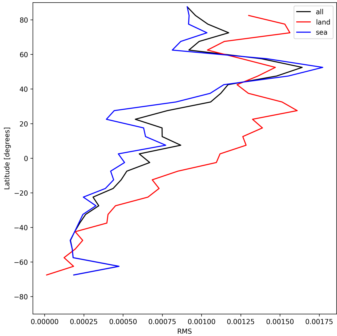
Figure 31: Zonal average of “RMS” for 2025-06-07 to 2025-06-09.
