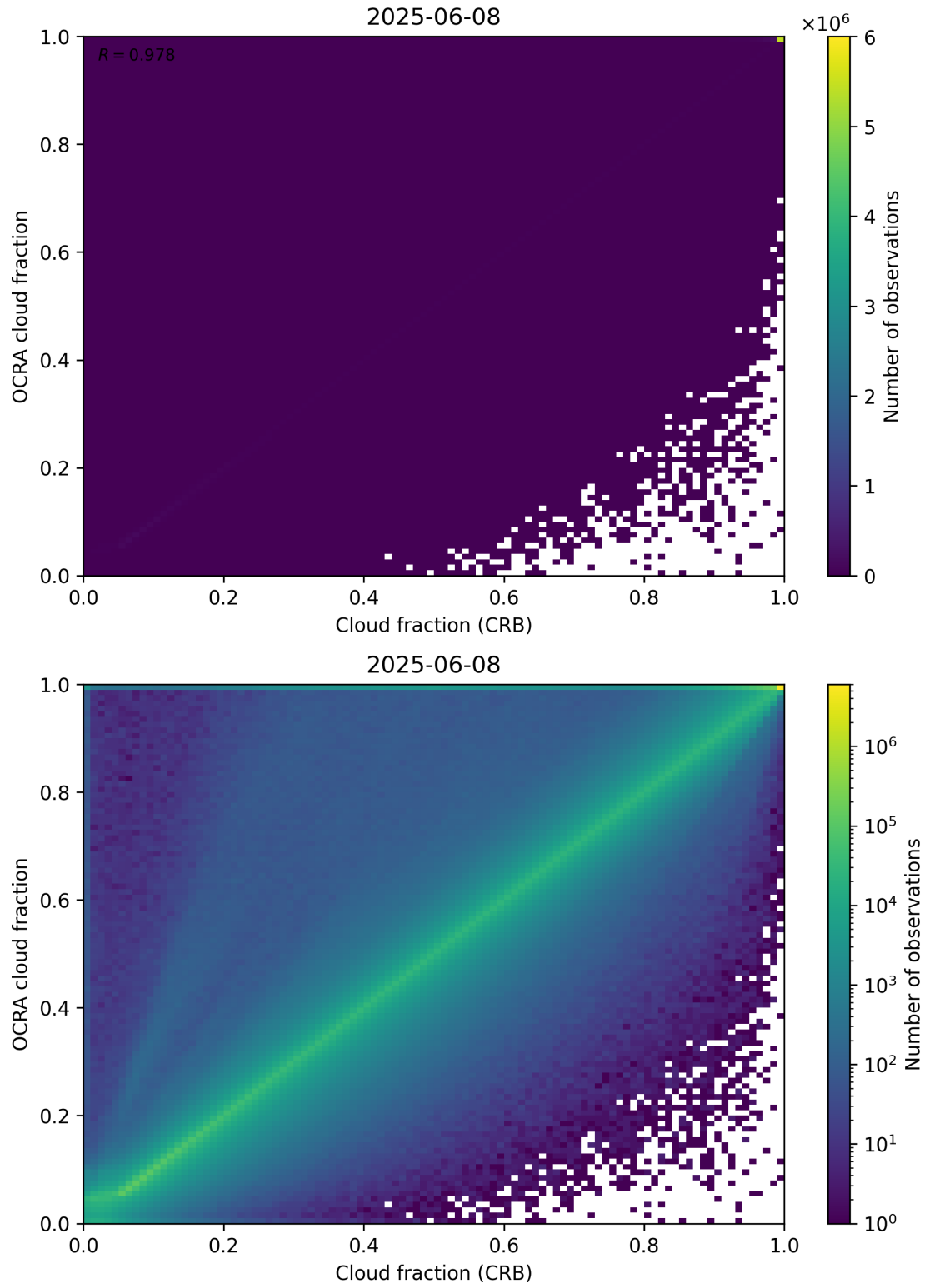
Figure 78: Scatter density plot of “Cloud fraction (CRB)” against “OCRA cloud fraction” for 2025-06-07 to 2025-06-09.
