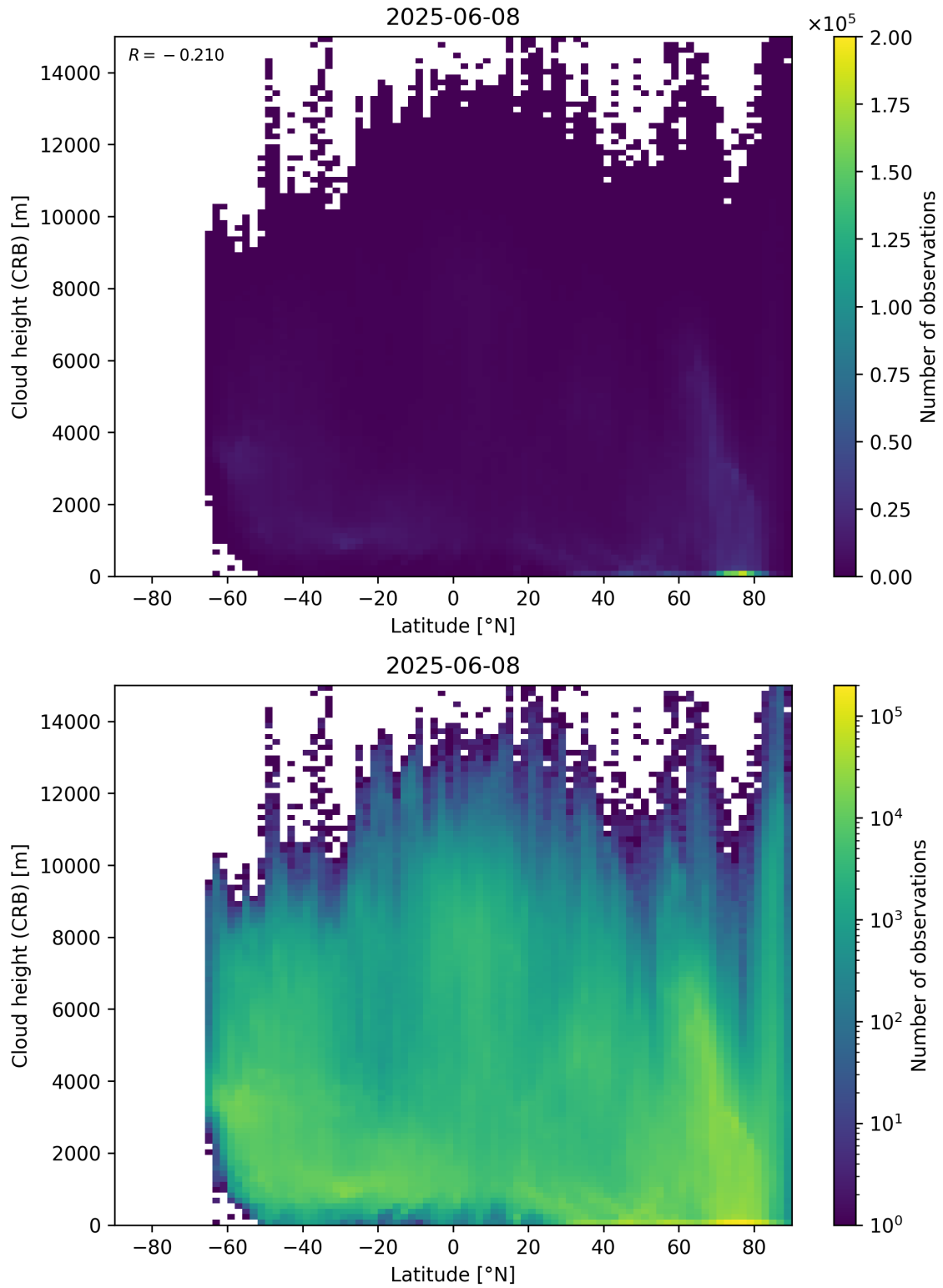
Figure 95: Scatter density plot of “Latitude” against “Cloud height (CRB)” for 2025-06-07 to 2025-06-09.
