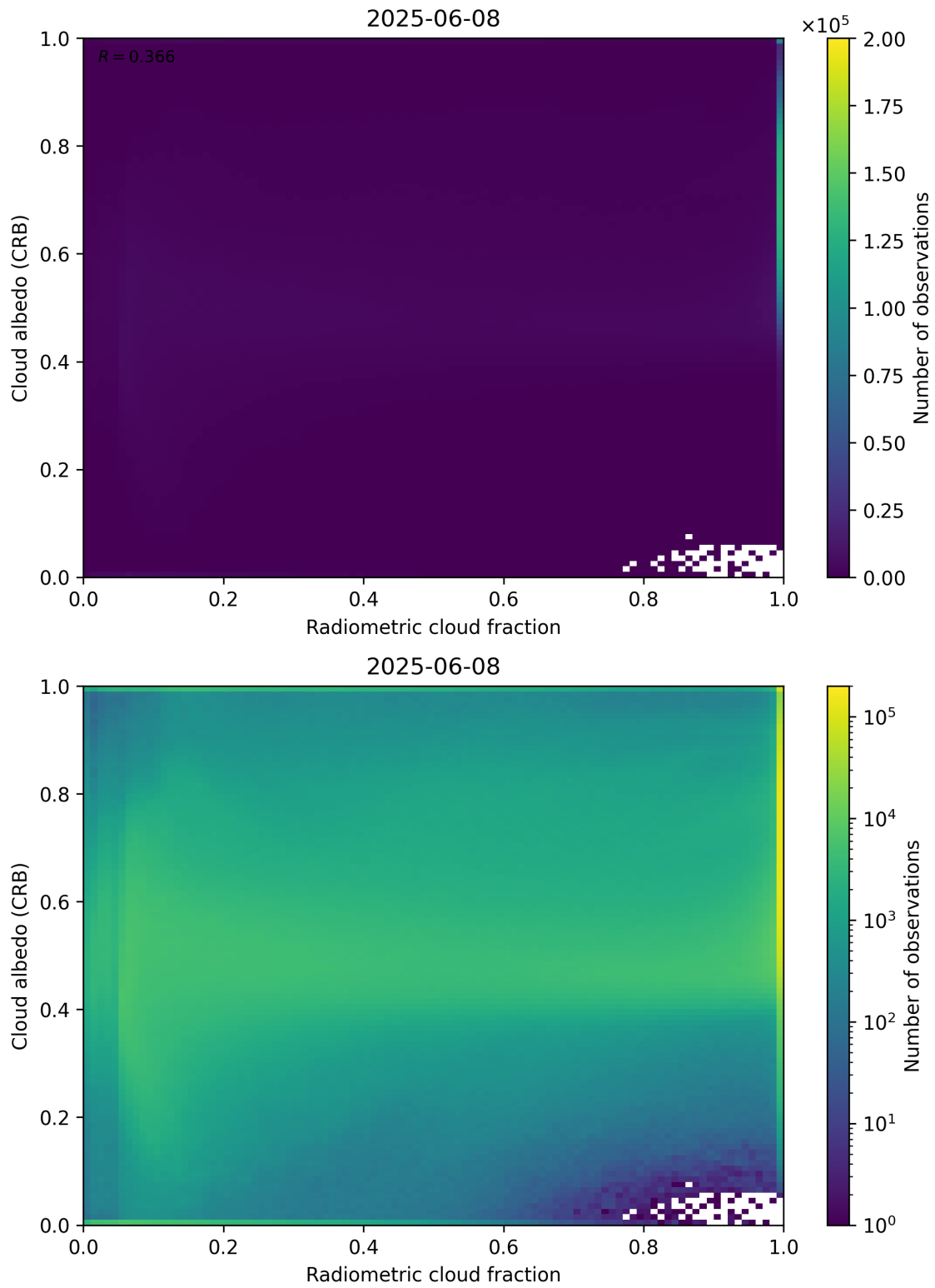
Figure 71: Scatter density plot of “Radiometric cloud fraction” against “Cloud albedo (CRB)” for 2025-06-07 to 2025-06-09.
