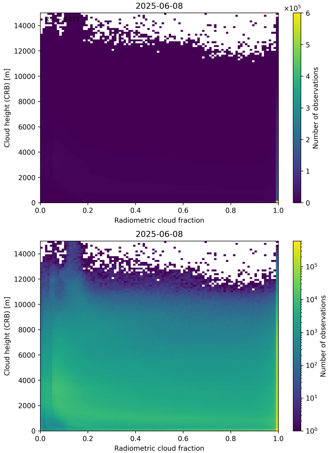
Figure 74: Scatter density plot of “Radiometric cloud fraction” against “Cloud height (CRB)” for 2025-06-07 to 2025-06-09.
