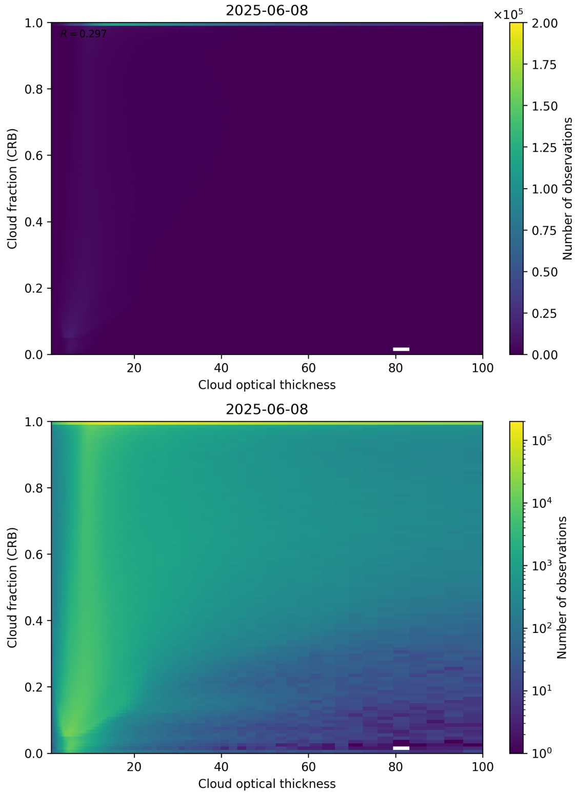
Figure 84: Scatter density plot of “Cloud optical thickness” against “Cloud fraction (CRB)” for 2025-06-07 to 2025-06-09.
