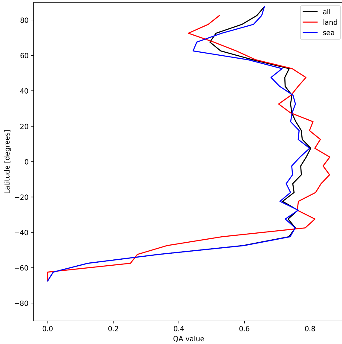
Figure 22: Zonal average of “QA value” for 2025-06-07 to 2025-06-09.
