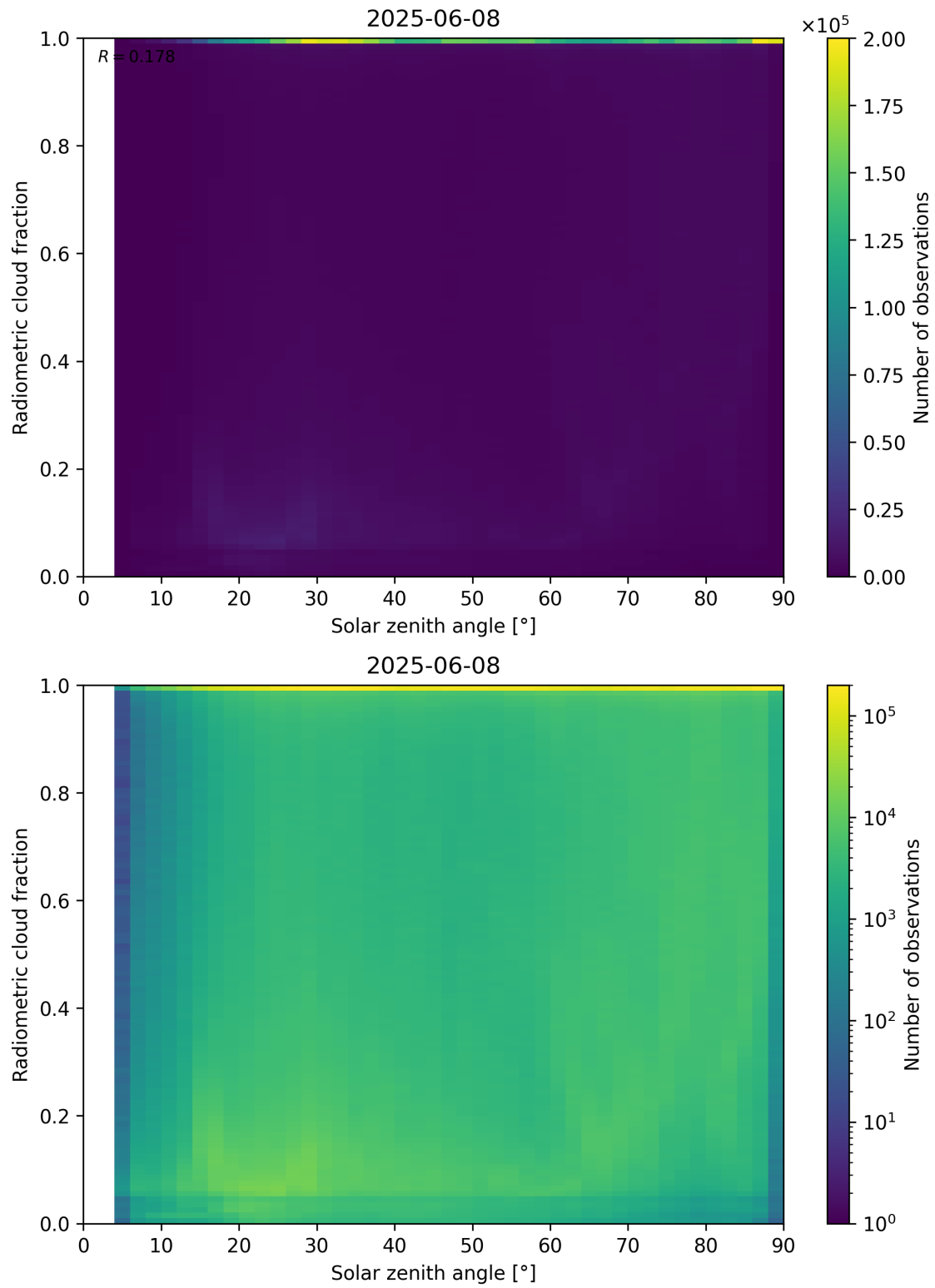
Figure 99: Scatter density plot of “Solar zenith angle” against “Radiometric cloud fraction” for 2025-06-07 to 2025-06-09.
