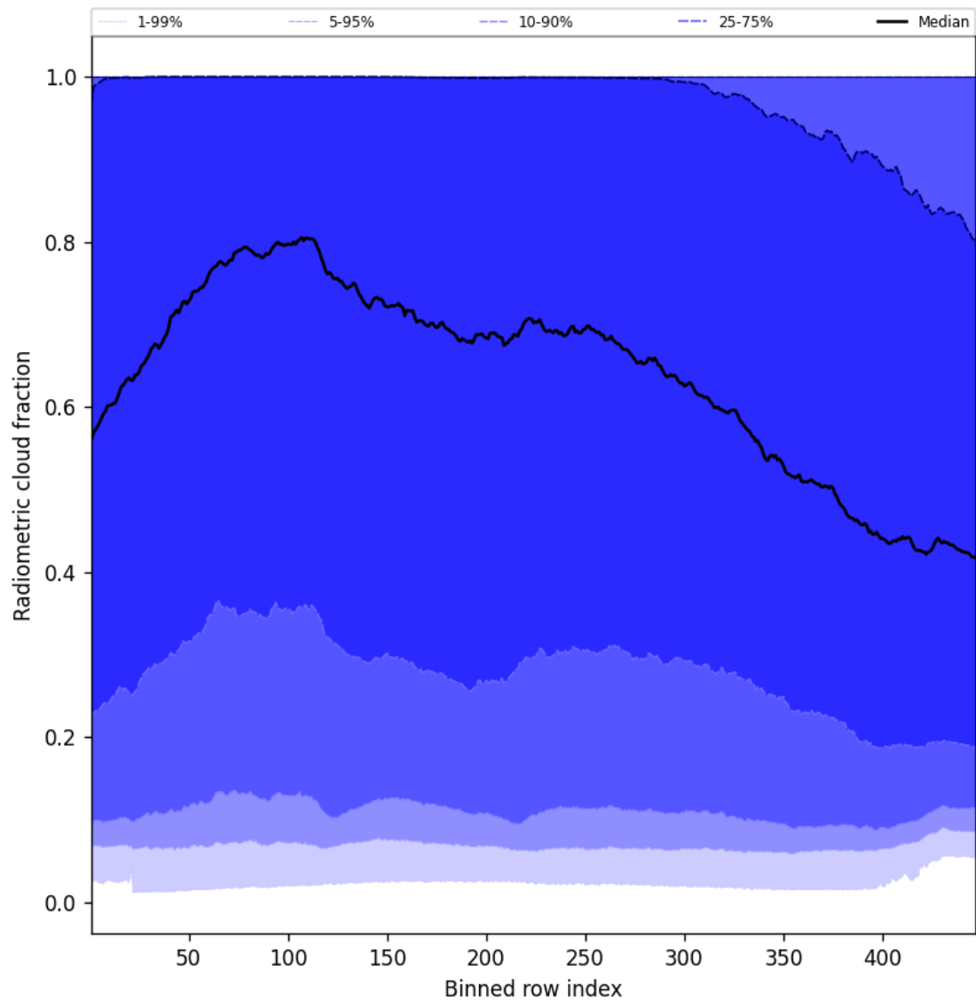
Figure 55: Along track statistics of “Radiometric cloud fraction” for 2025-06-07 to 2025-06-09
