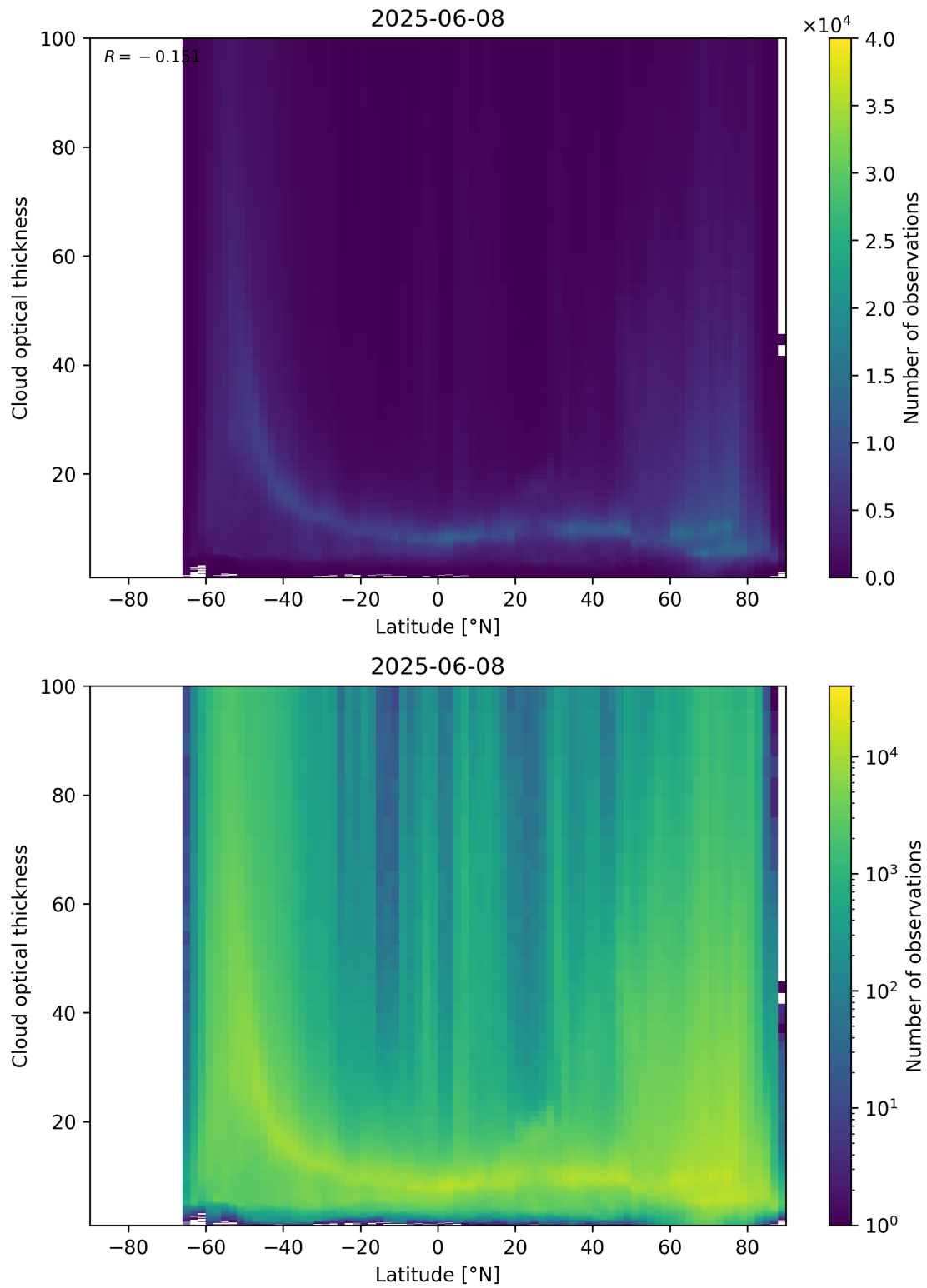
Figure 96: Scatter density plot of “Latitude” against “Cloud optical thickness” for 2025-06-07 to 2025-06-09.
