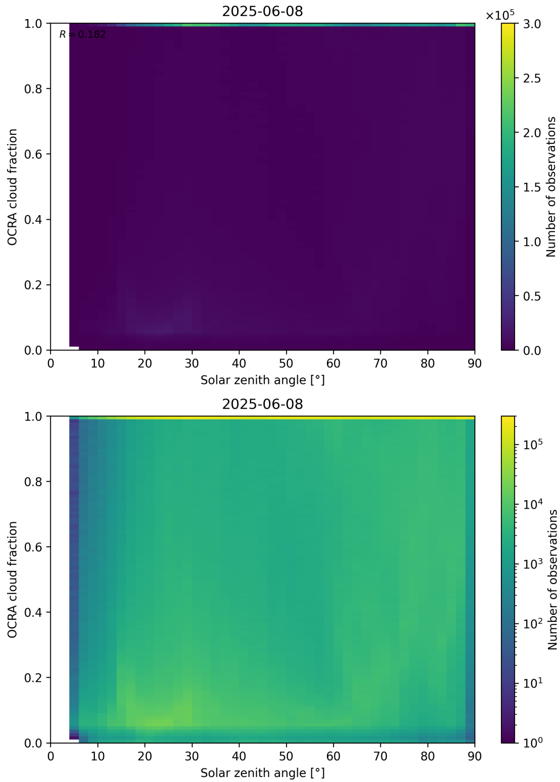
Figure 100: Scatter density plot of “Solar zenith angle” against “OCRA cloud fraction” for 2025-06-07 to 2025-06-09.
