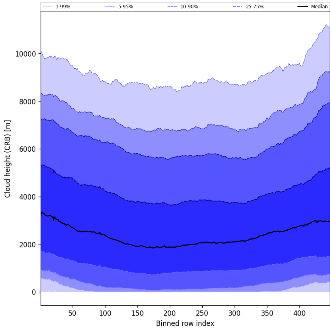
Figure 59: Along track statistics of “Cloud height (CRB)” for 2025-06-07 to 2025-06-09
