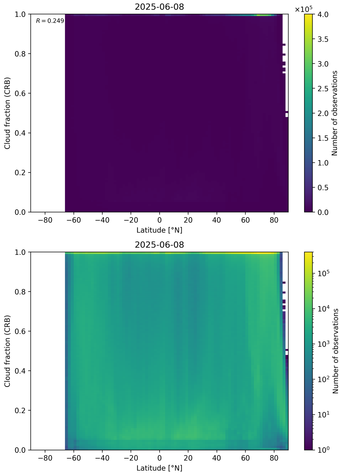
Figure 94: Scatter density plot of “Latitude” against “Cloud fraction (CRB)” for 2025-06-07 to 2025-06-09.
