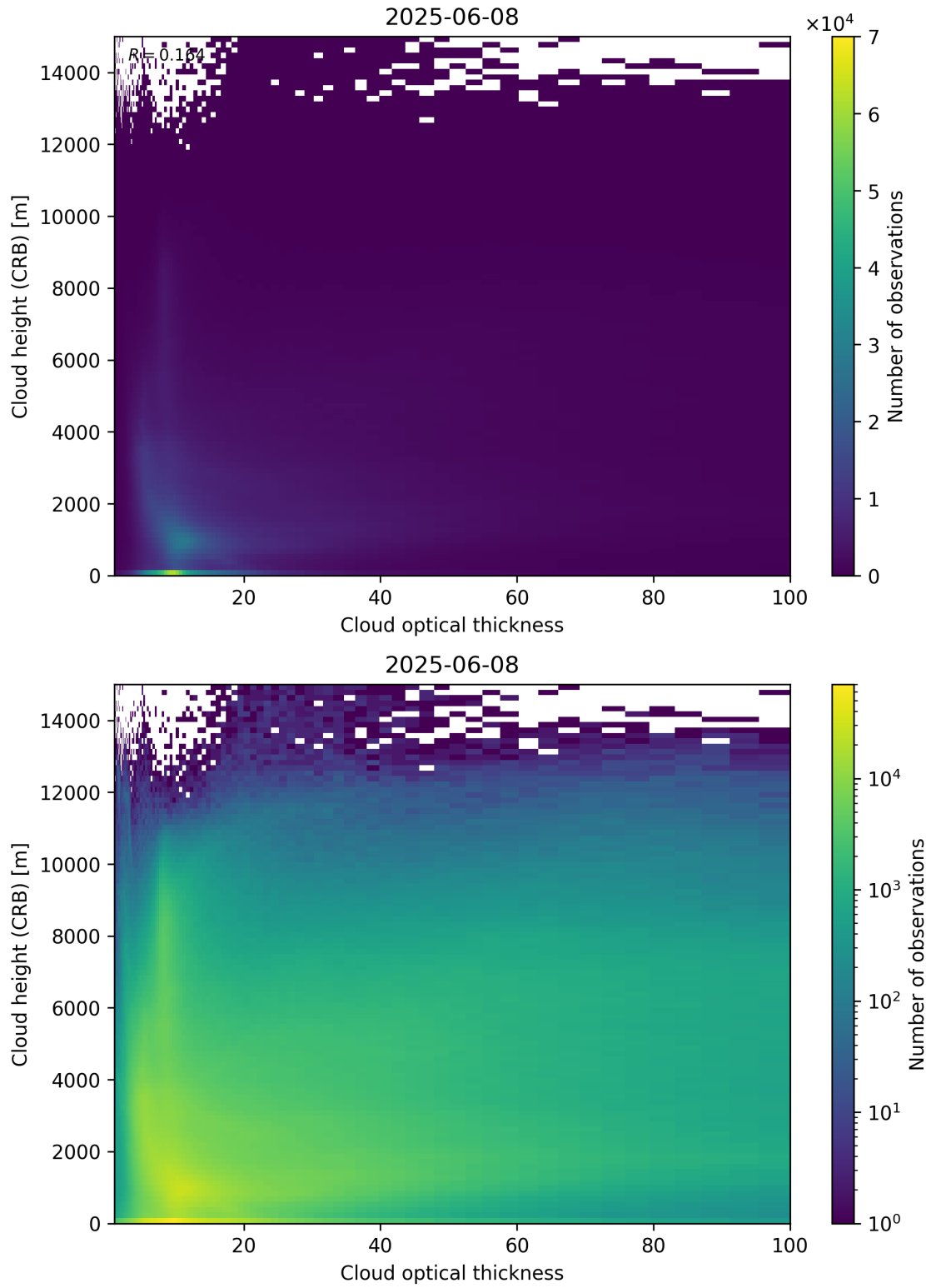
Figure 85: Scatter density plot of “Cloud optical thickness” against “Cloud height (CRB)” for 2025-06-07 to 2025-06-09.
