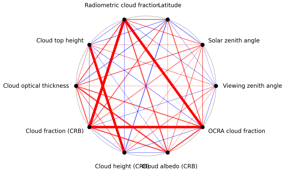
Figure 1: Map of correlation graph for 2025-06-07 to 2025-06-09.
