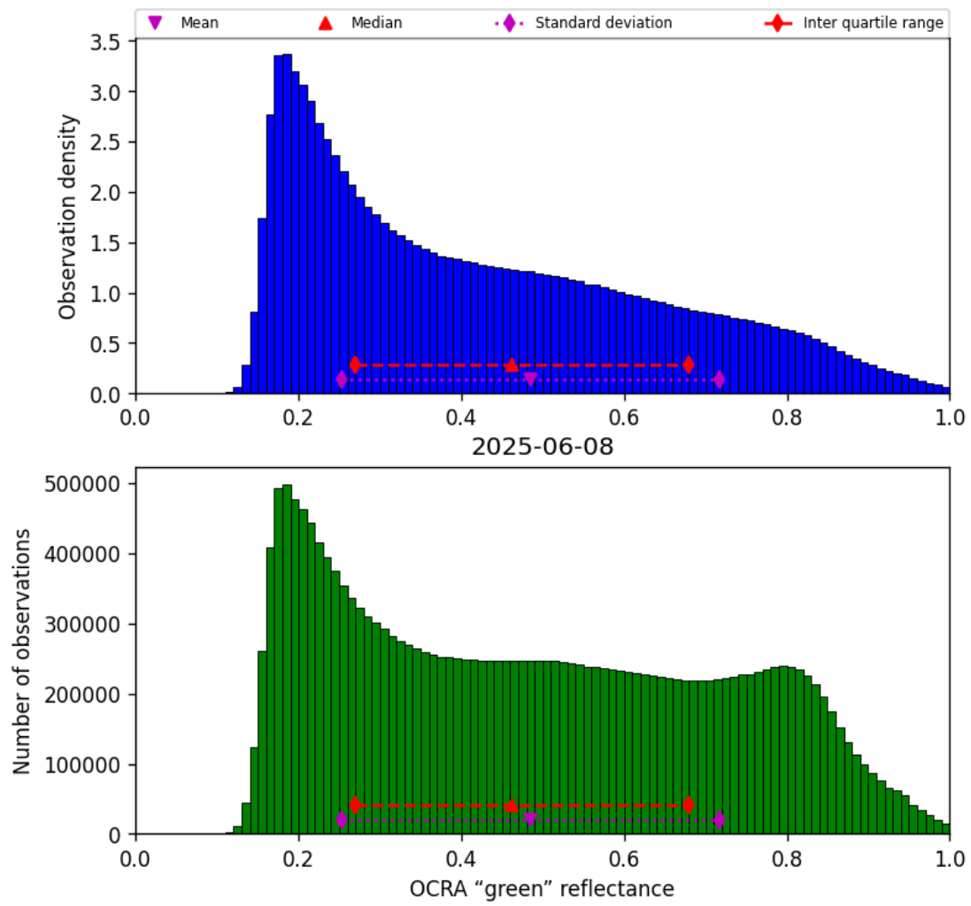
Figure 52: Histogram of “OCRA “green” reflectance” for 2025-06-07 to 2025-06-09
