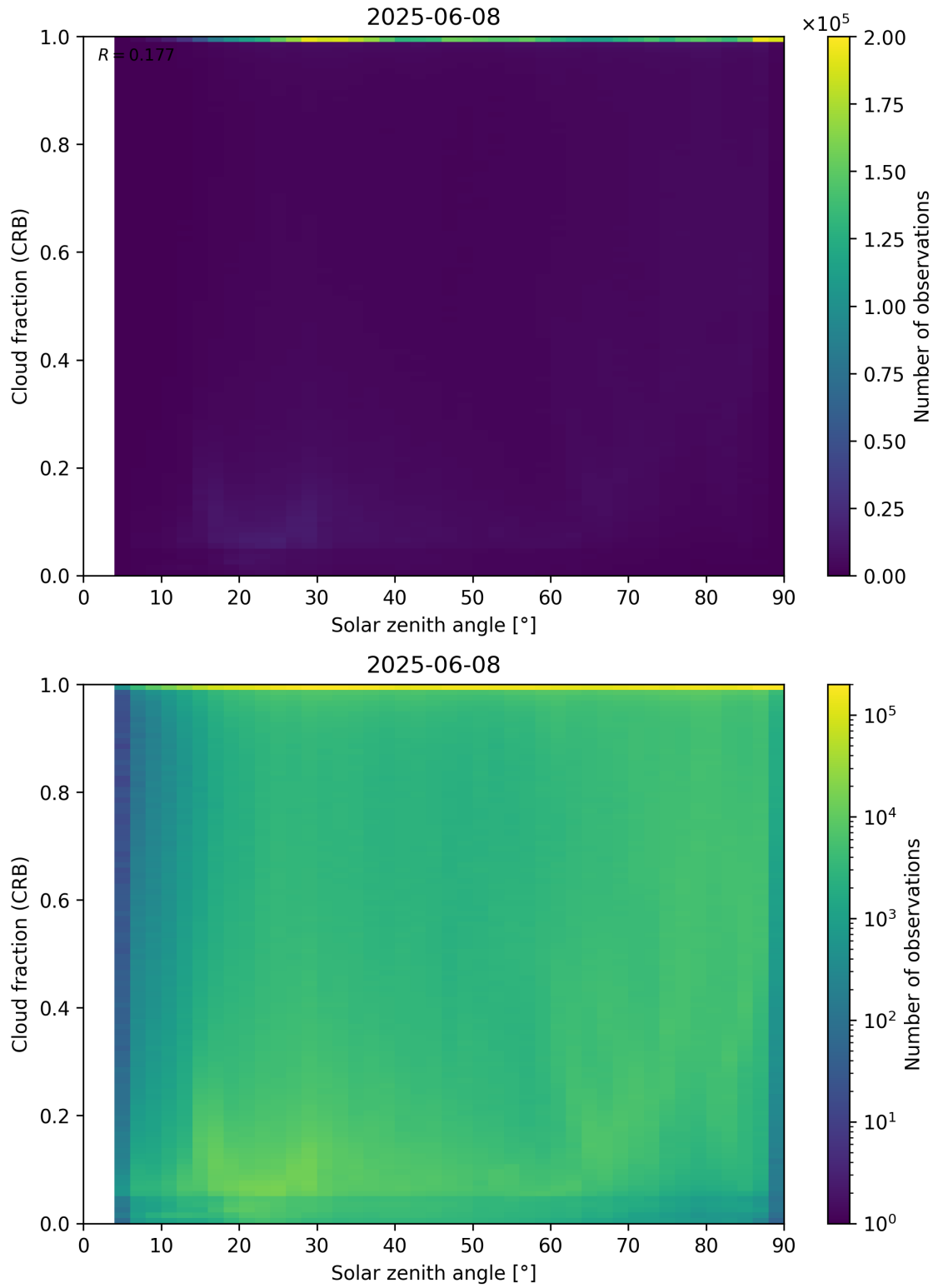
Figure 101: Scatter density plot of “Solar zenith angle” against “Cloud fraction (CRB)” for 2025-06-07 to 2025-06-09.
