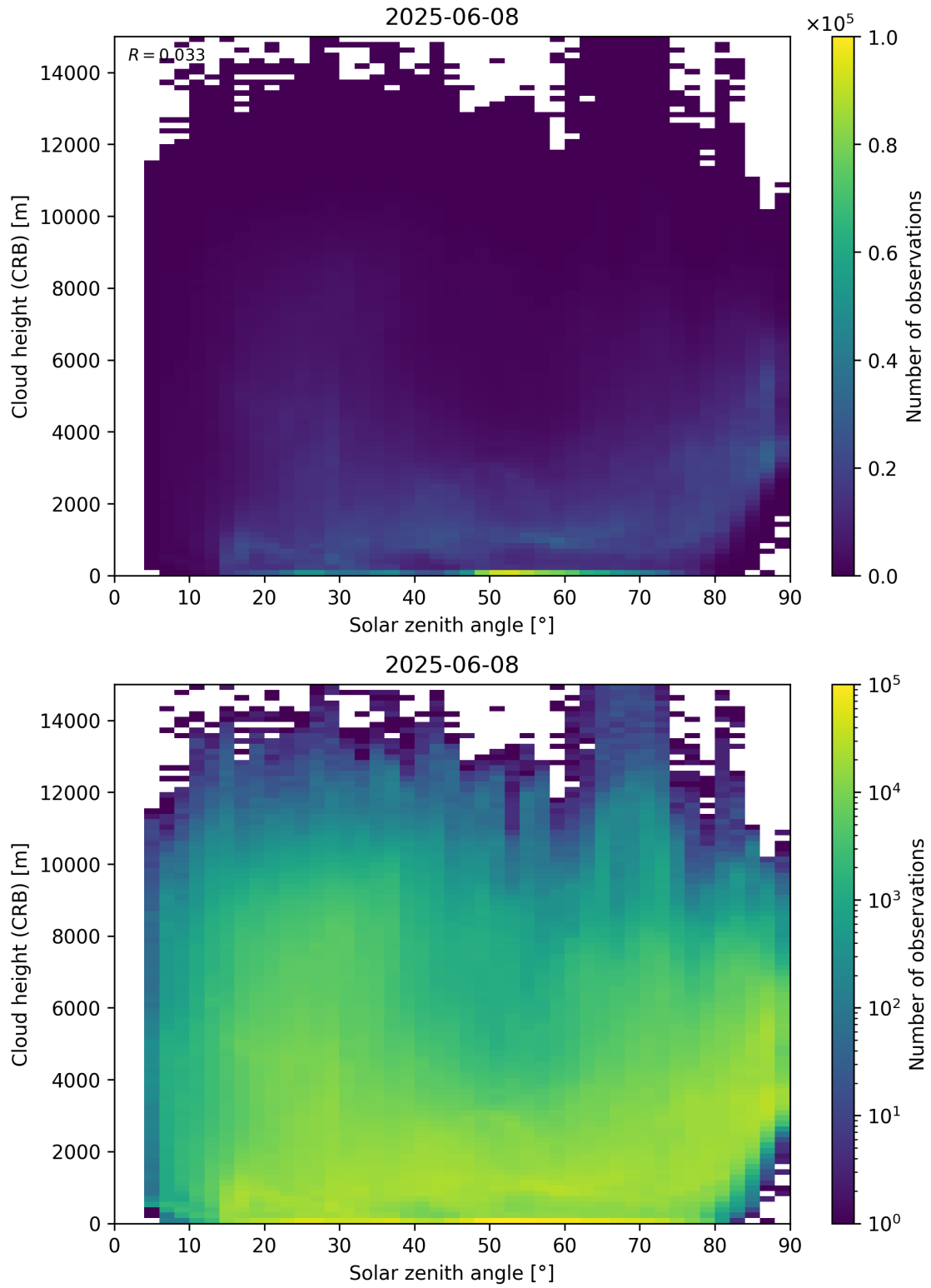
Figure 102: Scatter density plot of “Solar zenith angle” against “Cloud height (CRB)” for 2025-06-07 to 2025-06-09.
