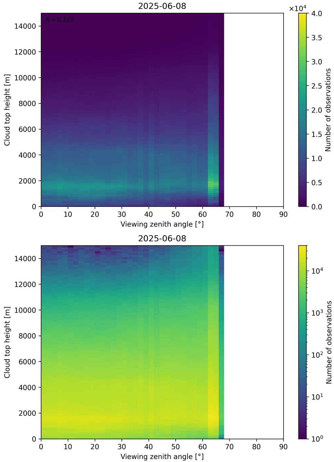
Figure 112: Scatter density plot of “Viewing zenith angle” against “Cloud top height” for 2025-06-07 to 2025-06-09.
