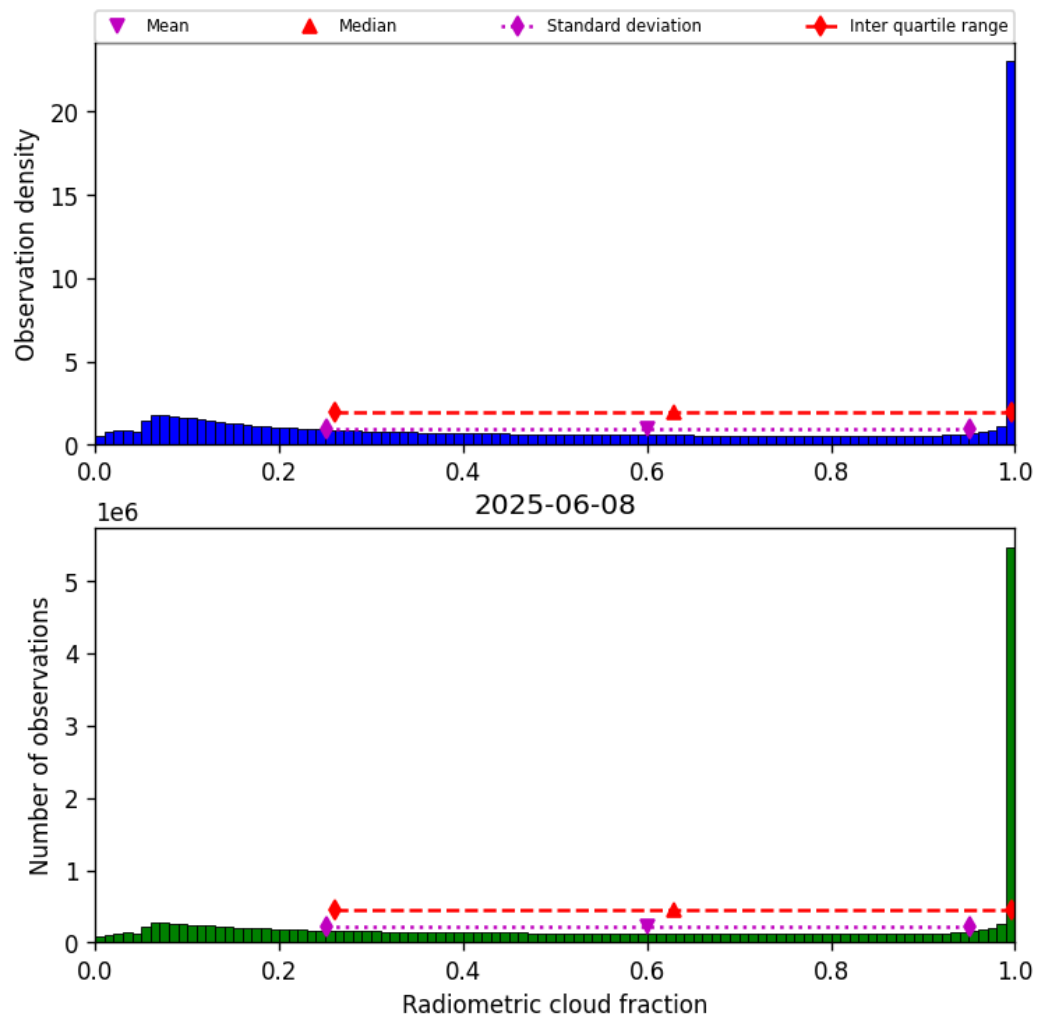
Figure 39: Histogram of “Radiometric cloud fraction” for 2025-06-07 to 2025-06-09
