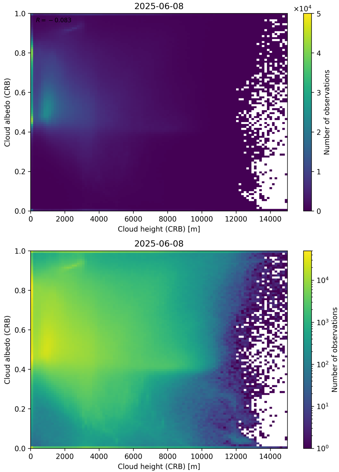
Figure 80: Scatter density plot of “Cloud height (CRB)” against “Cloud albedo (CRB)” for 2025-06-07 to 2025-06-09.
