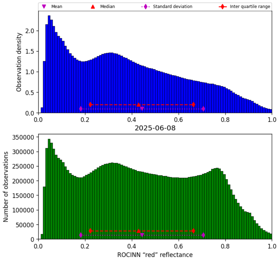
Figure 53: Histogram of “ROCINN “red” reflectance” for 2025-06-07 to 2025-06-09
