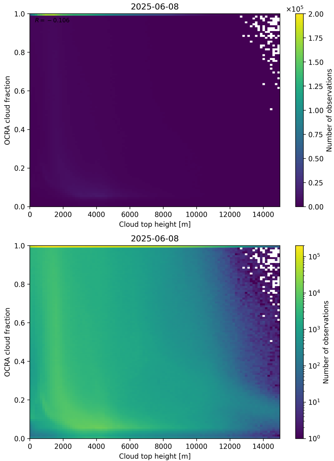
Figure 87: Scatter density plot of “Cloud top height” against “OCRA cloud fraction” for 2025-06-07 to 2025-06-09.
