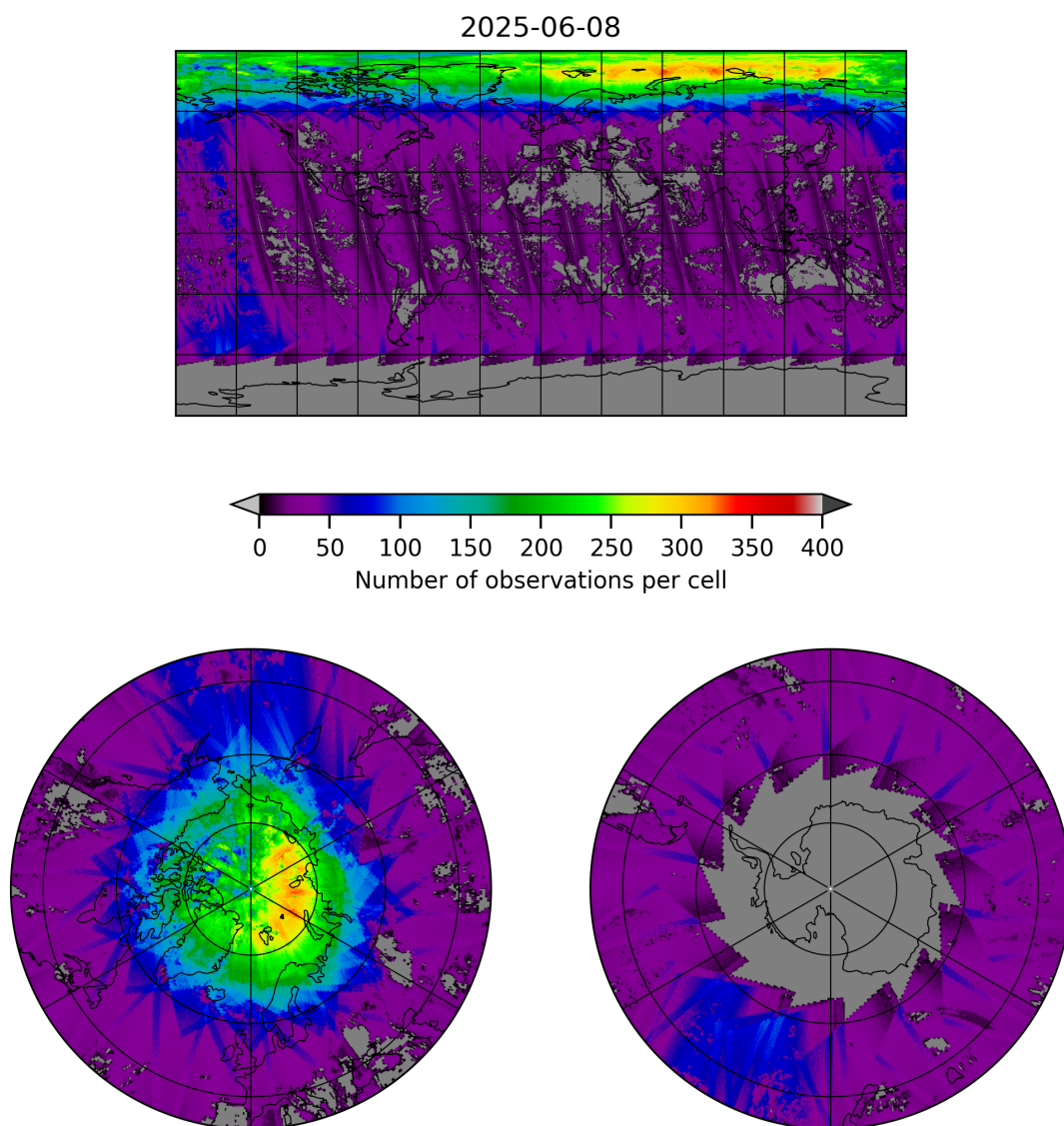
Figure 21: Map of the number of observations for 2025-06-07 to 2025-06-09
