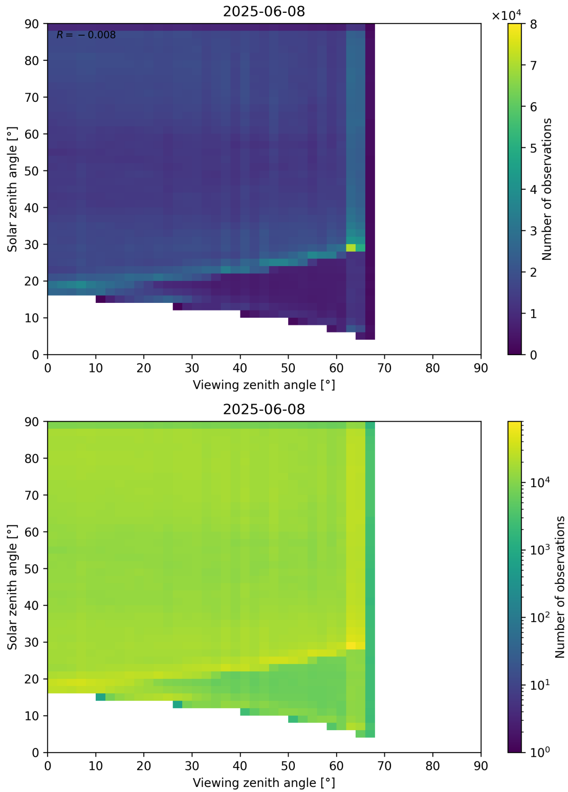
Figure 114: Scatter density plot of “Viewing zenith angle” against “Solar zenith angle” for 2025-06-07 to 2025-06-09.
