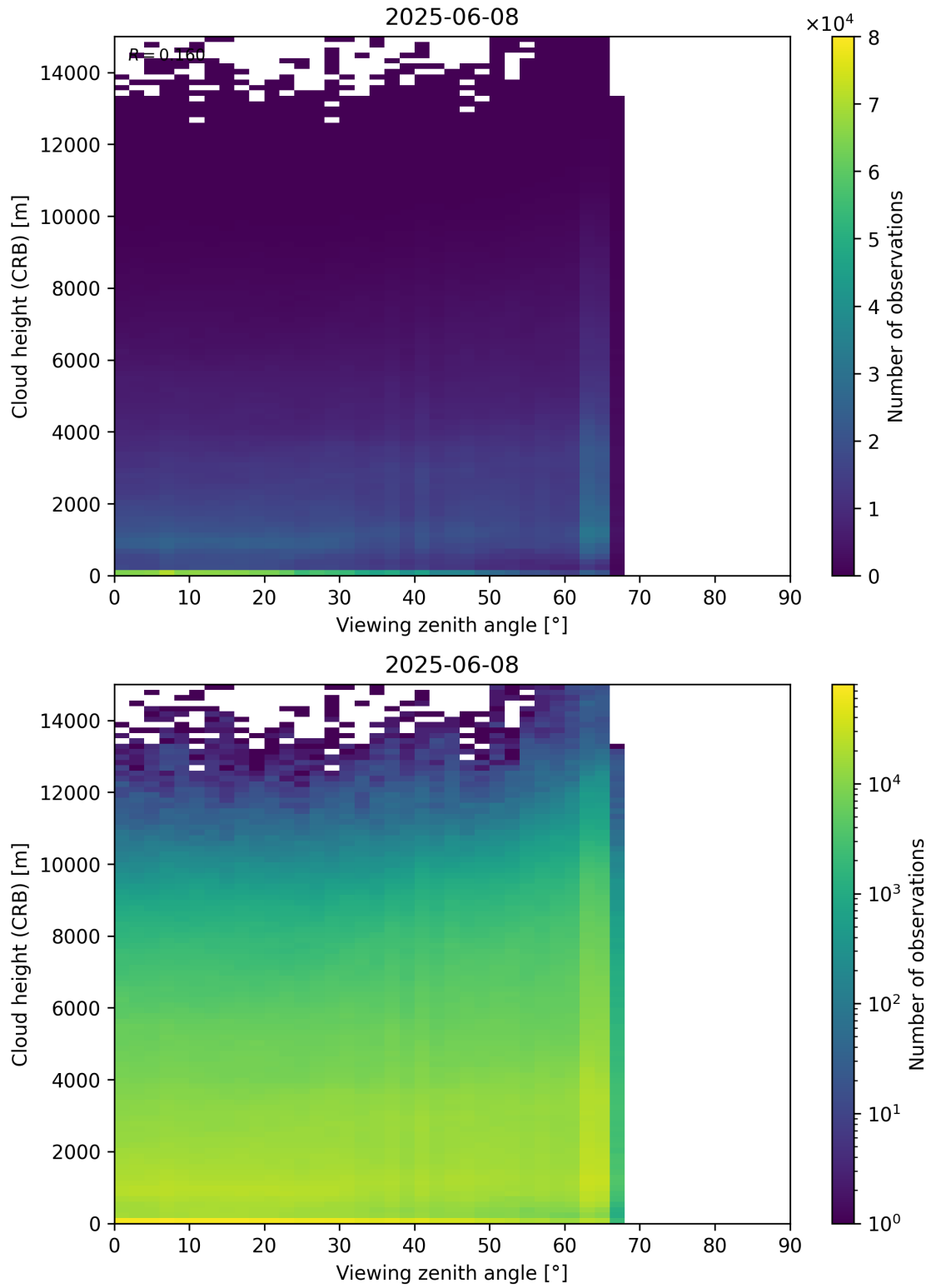
Figure 110: Scatter density plot of “Viewing zenith angle” against “Cloud height (CRB)” for 2025-06-07 to 2025-06-09.
