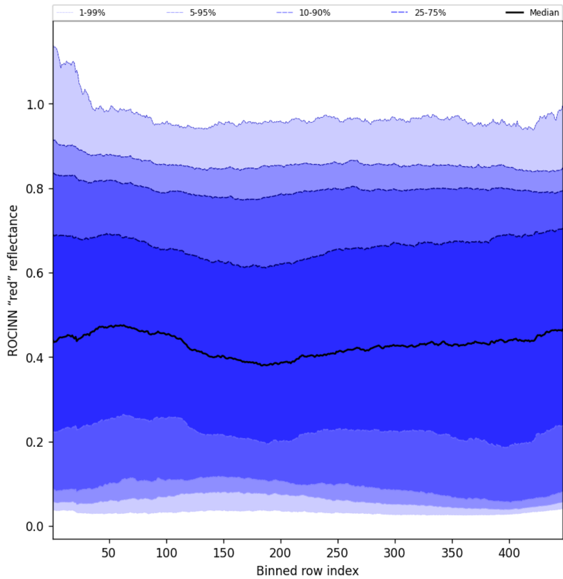
Figure 69: Along track statistics of “ROCINN “red” reflectance” for 2025-06-07 to 2025-06-09
