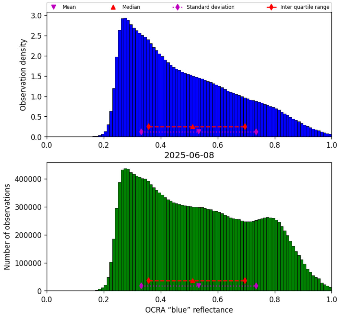
Figure 51: Histogram of “OCRA “blue” reflectance” for 2025-06-07 to 2025-06-09
