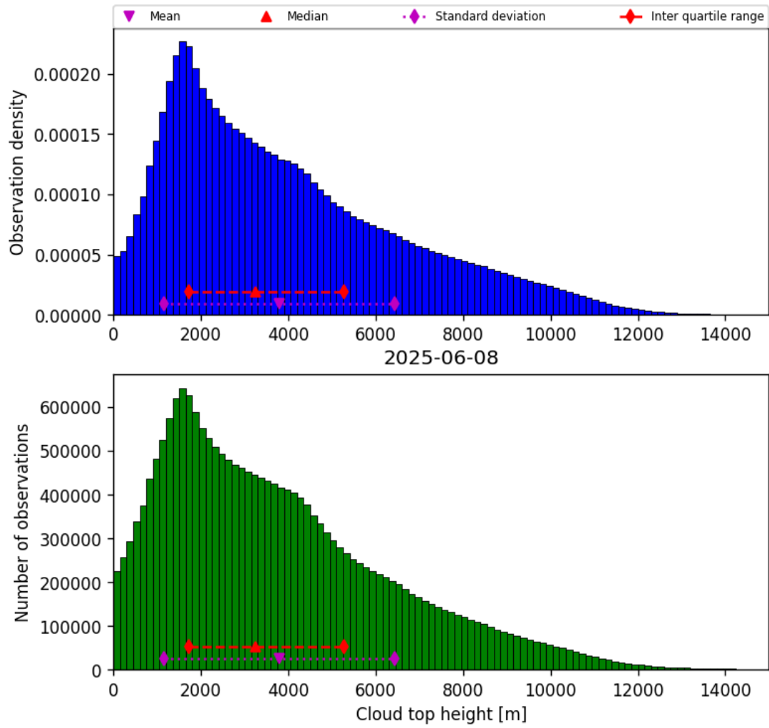
Figure 40: Histogram of “Cloud top height” for 2025-06-07 to 2025-06-09
