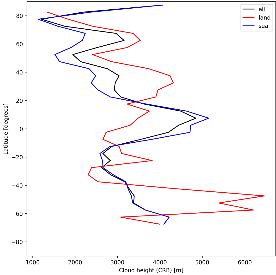
Figure 27: Zonal average of “Cloud height (CRB)” for 2025-06-07 to 2025-06-09.
