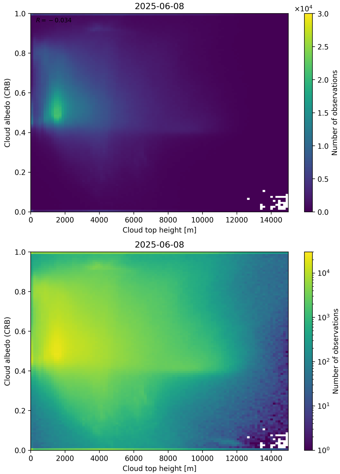
Figure 86: Scatter density plot of “Cloud top height” against “Cloud albedo (CRB)” for 2025-06-07 to 2025-06-09.
