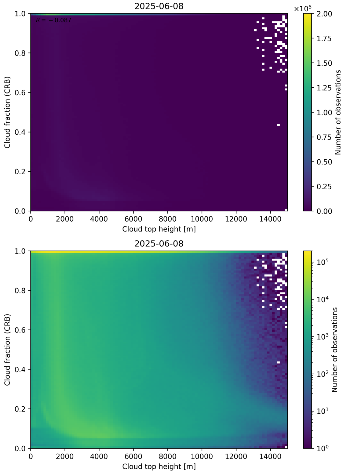
Figure 88: Scatter density plot of “Cloud top height” against “Cloud fraction (CRB)” for 2025-06-07 to 2025-06-09.
