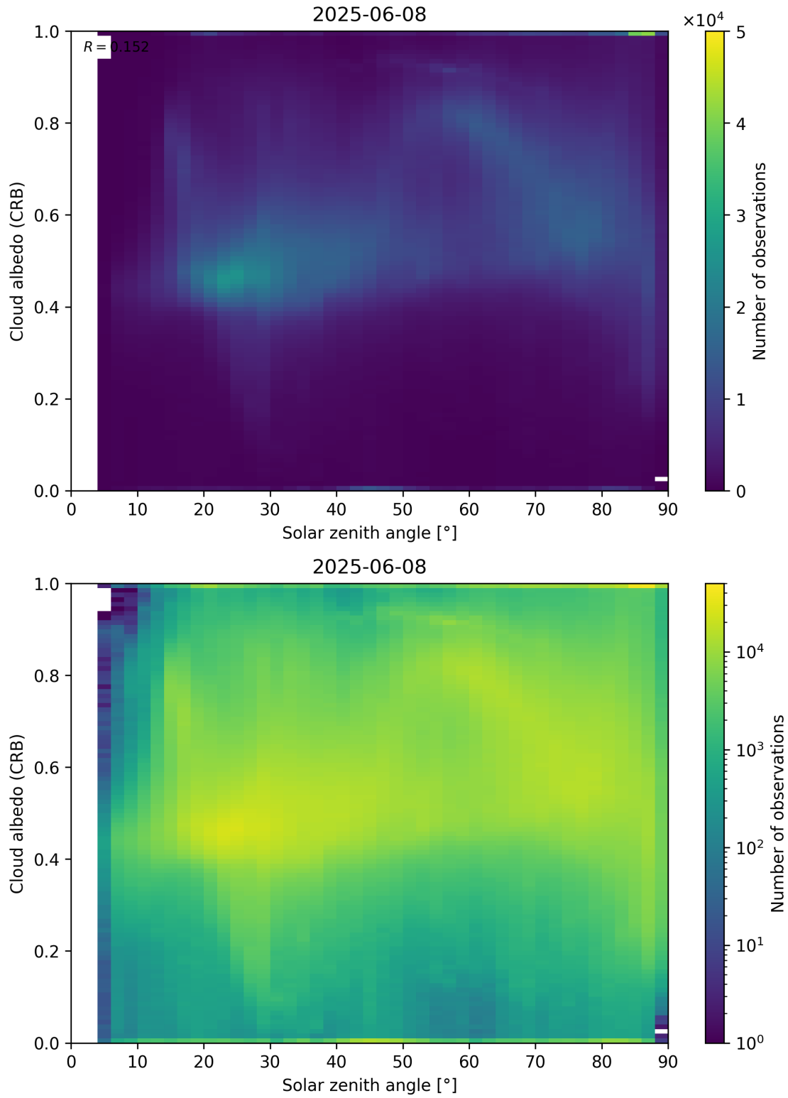
Figure 98: Scatter density plot of “Solar zenith angle” against “Cloud albedo (CRB)” for 2025-06-07 to 2025-06-09.
