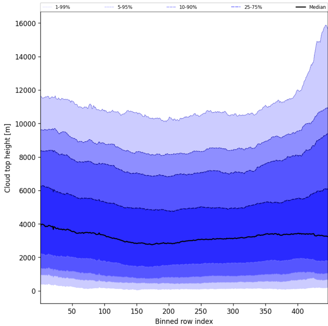
Figure 56: Along track statistics of “Cloud top height” for 2025-06-07 to 2025-06-09
