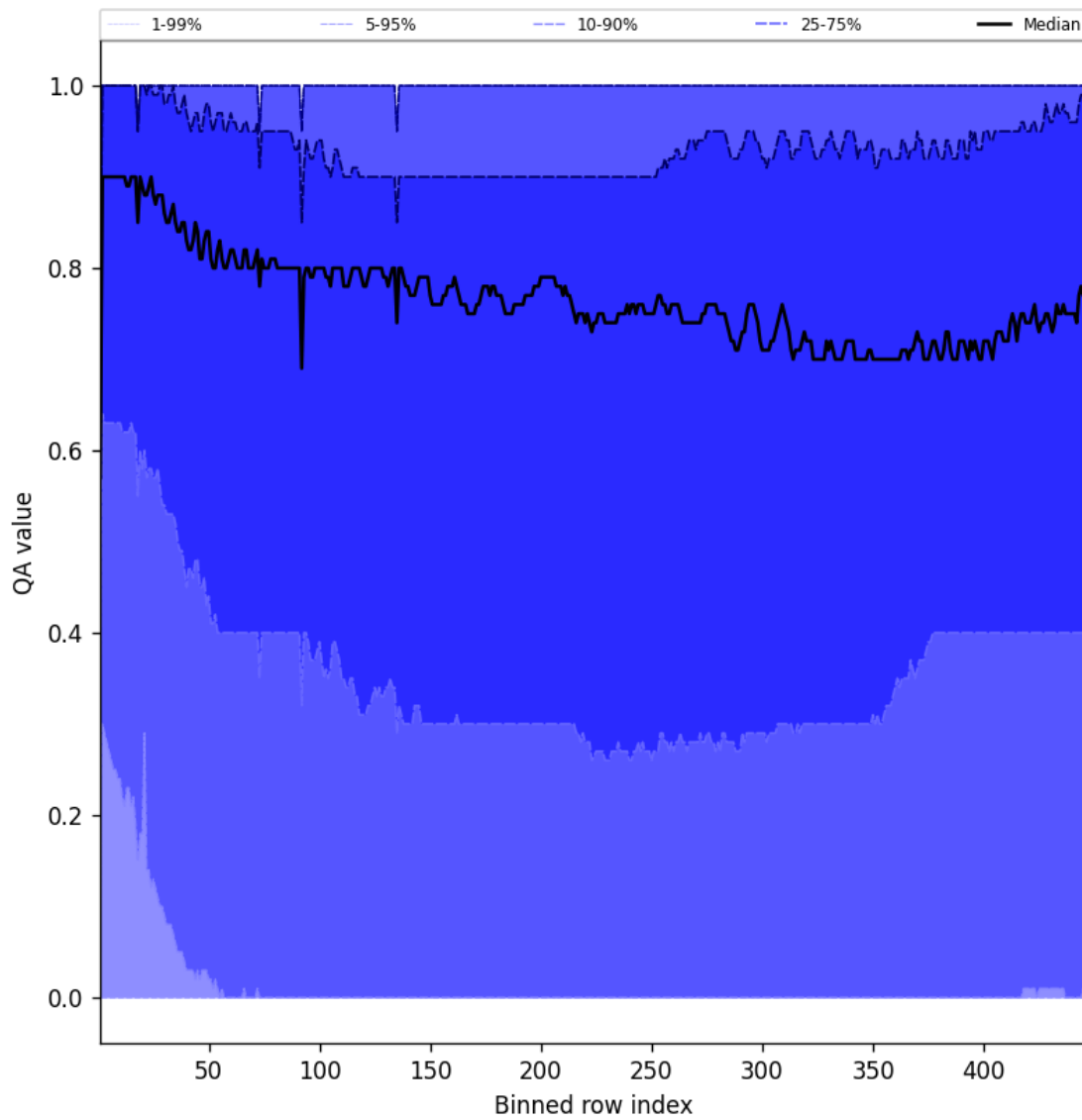
Figure 54: Along track statistics of “QA value” for 2025-06-07 to 2025-06-09
