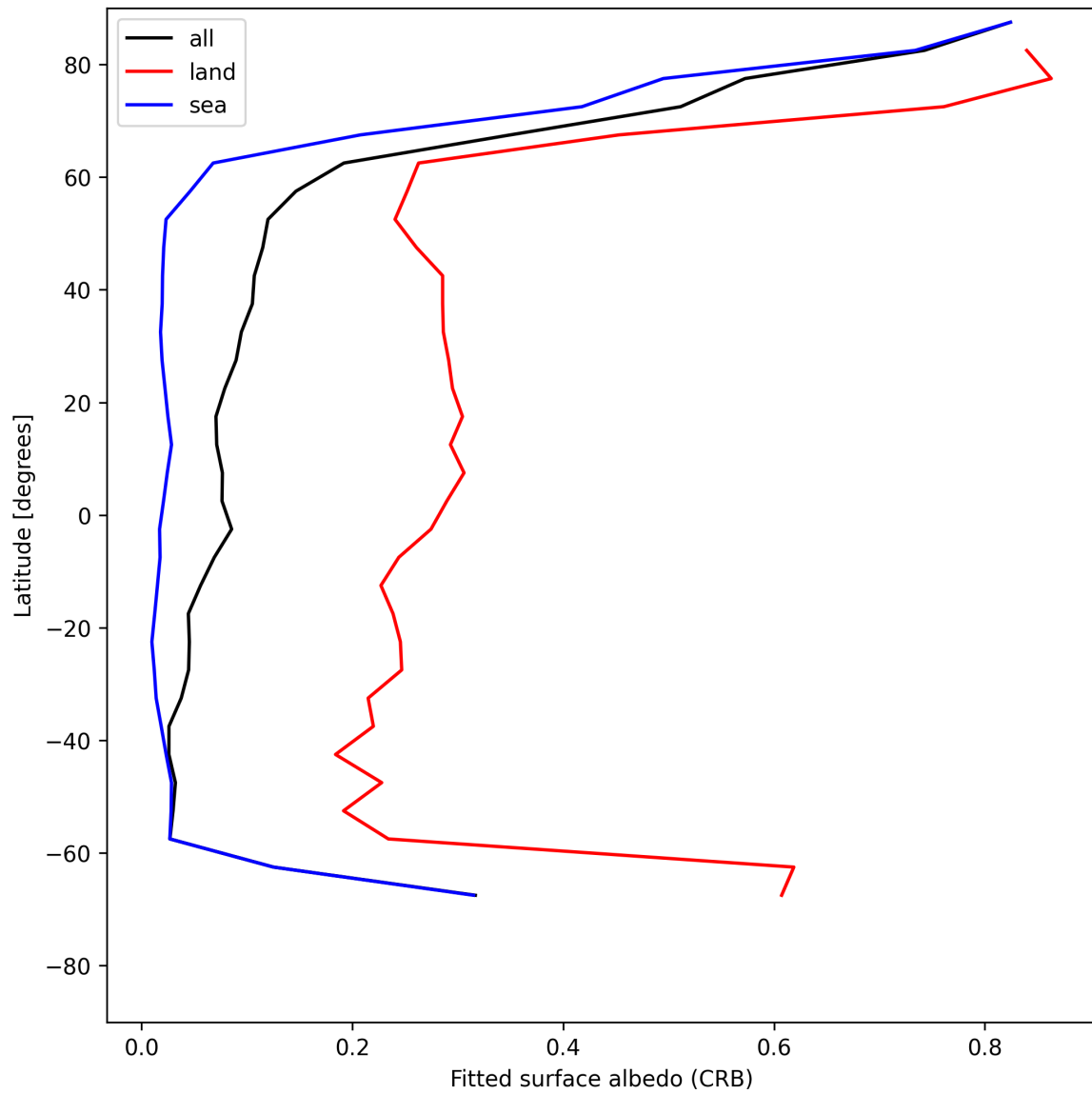
Figure 30: Zonal average of “Fitted surface albedo (CRB)” for 2025-06-07 to 2025-06-09.
