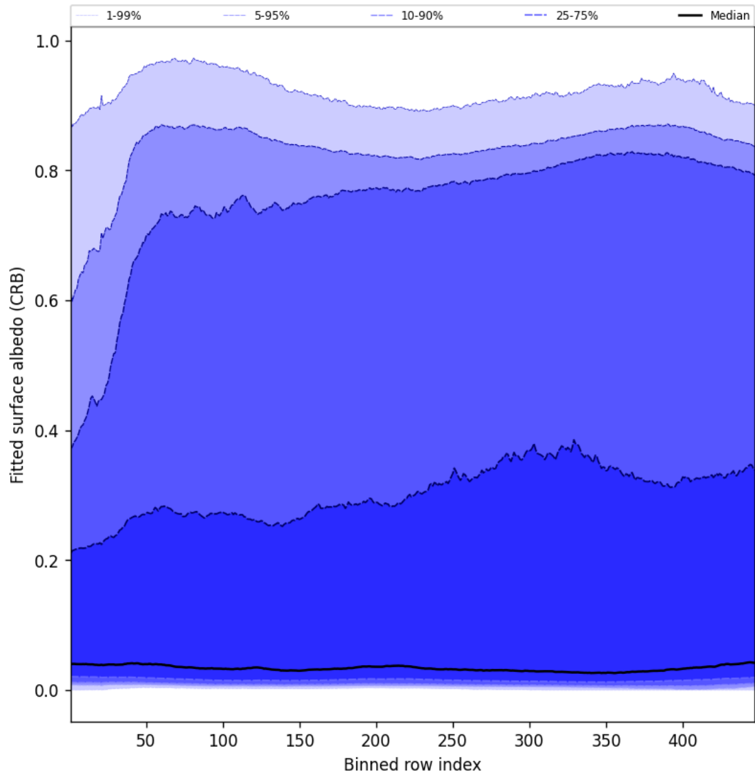
Figure 62: Along track statistics of “Fitted surface albedo (CRB)” for 2025-06-07 to 2025-06-09
