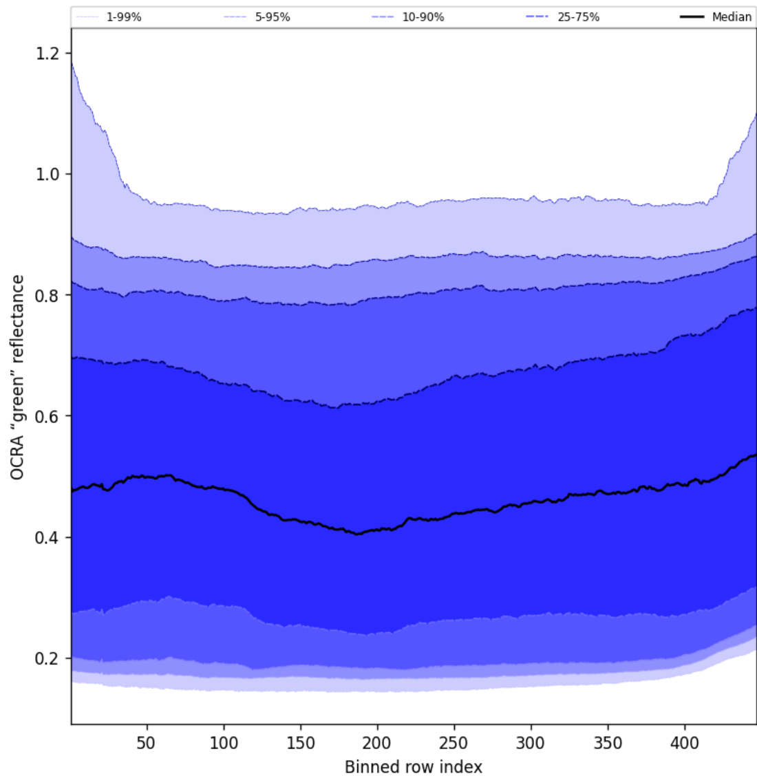
Figure 68: Along track statistics of “OCRA “green” reflectance” for 2025-06-07 to 2025-06-09
