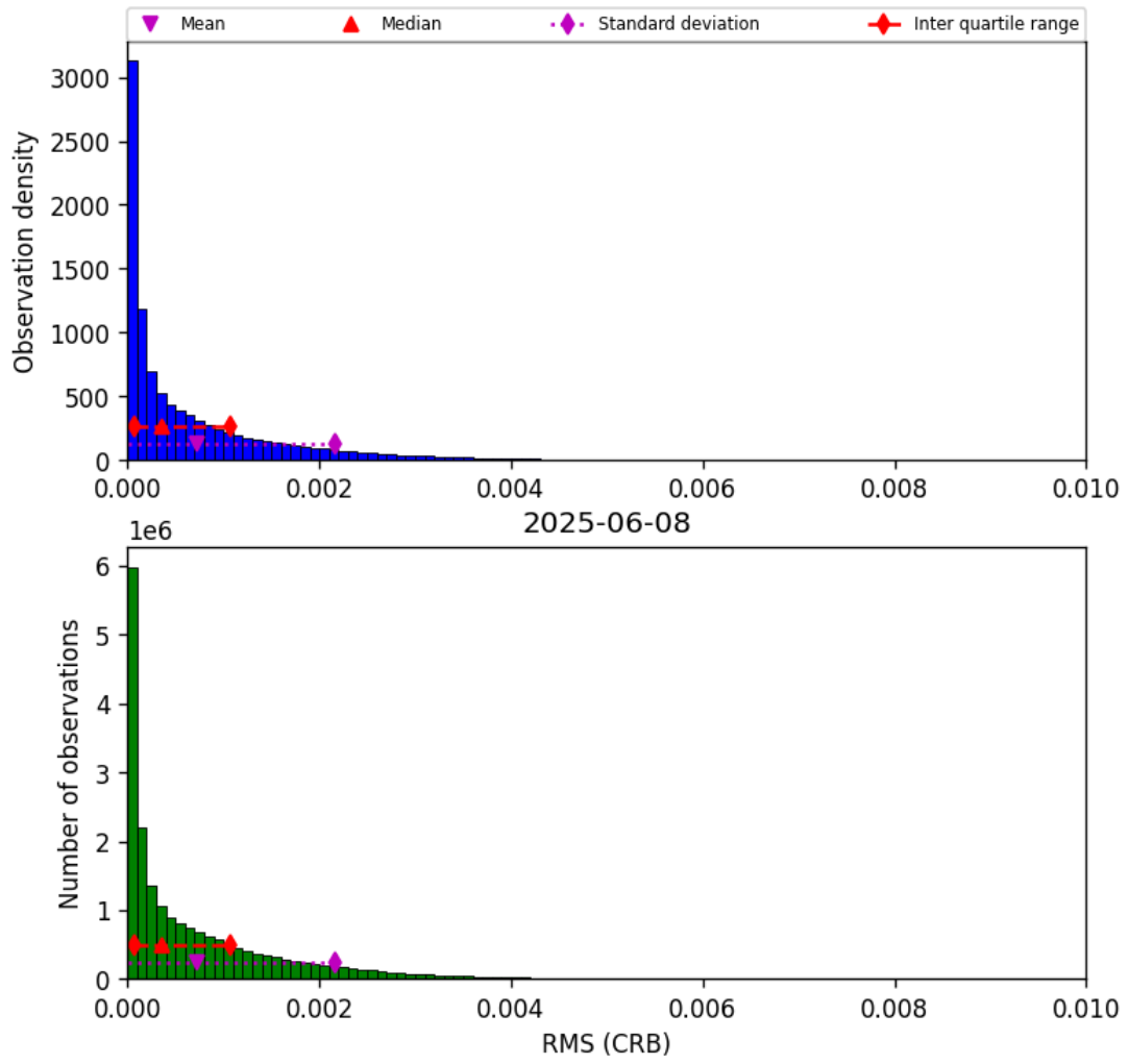
Figure 48: Histogram of “RMS (CRB)” for 2025-06-07 to 2025-06-09
