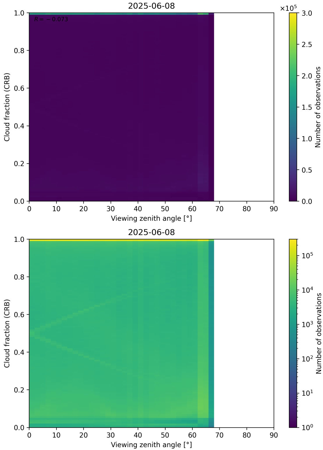
Figure 109: Scatter density plot of “Viewing zenith angle” against “Cloud fraction (CRB)” for 2025-06-07 to 2025-06-09.
