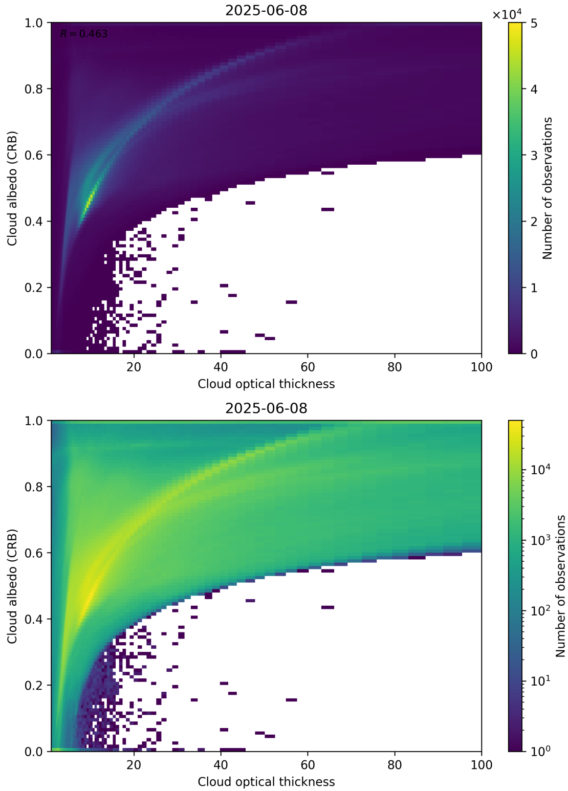
Figure 82: Scatter density plot of “Cloud optical thickness” against “Cloud albedo (CRB)” for 2025-06-07 to 2025-06-09.
