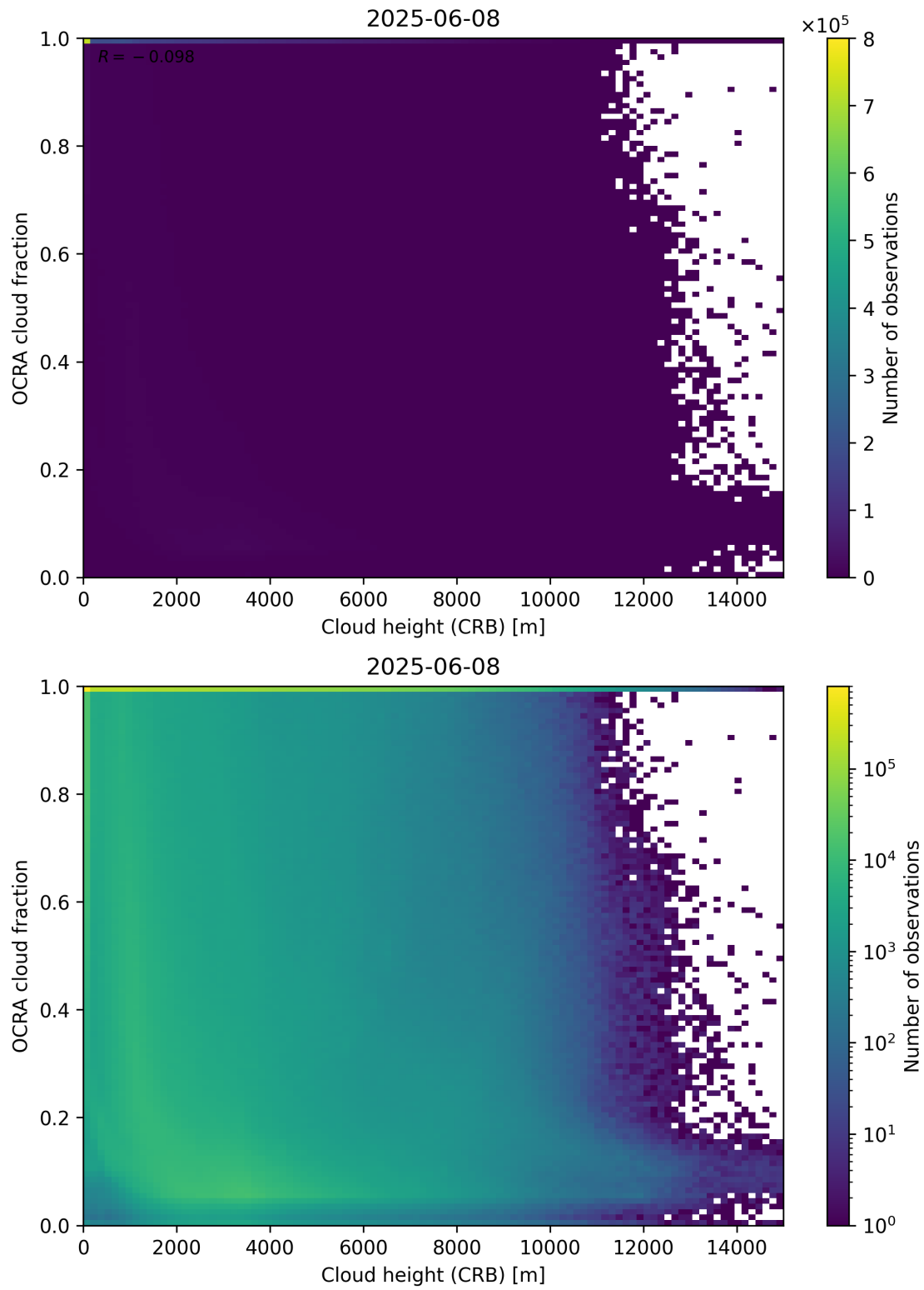
Figure 81: Scatter density plot of “Cloud height (CRB)” against “OCRA cloud fraction” for 2025-06-07 to 2025-06-09.
