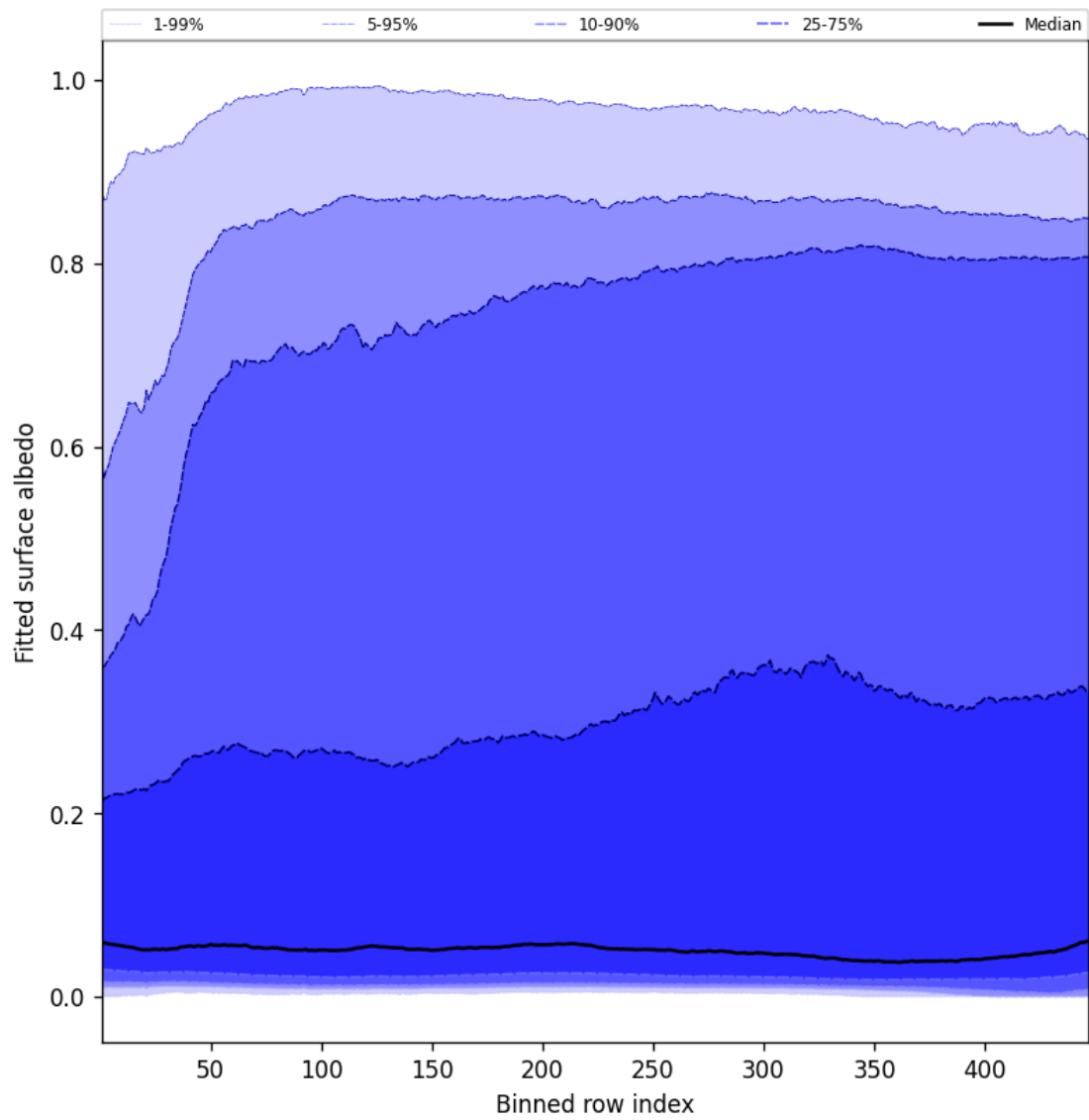
Figure 61: Along track statistics of “Fitted surface albedo” for 2025-06-07 to 2025-06-09
