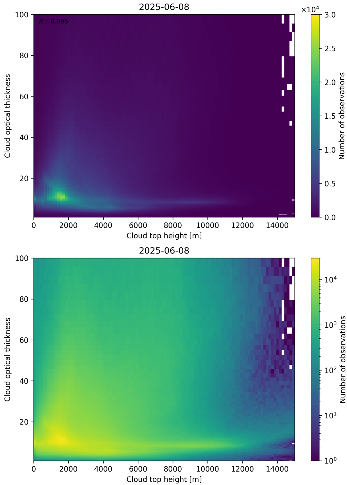
Figure 90: Scatter density plot of “Cloud top height” against “Cloud optical thickness” for 2025-06-07 to 2025-06-09.
