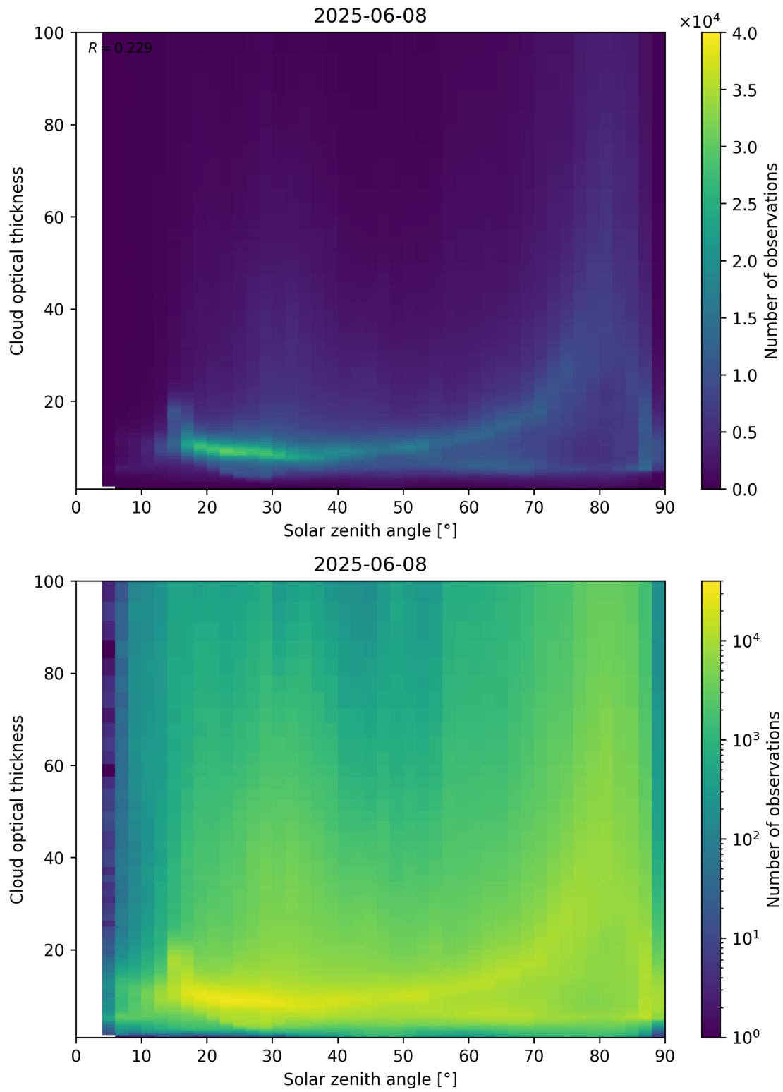
Figure 103: Scatter density plot of “Solar zenith angle” against “Cloud optical thickness” for 2025-06-07 to 2025-06-09.
