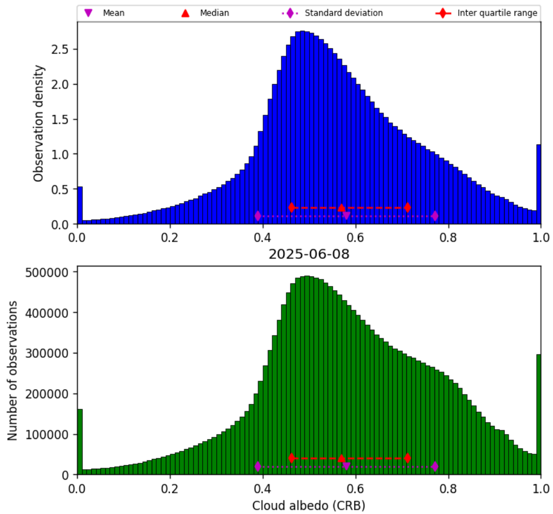
Figure 44: Histogram of “Cloud albedo (CRB)” for 2025-06-07 to 2025-06-09
