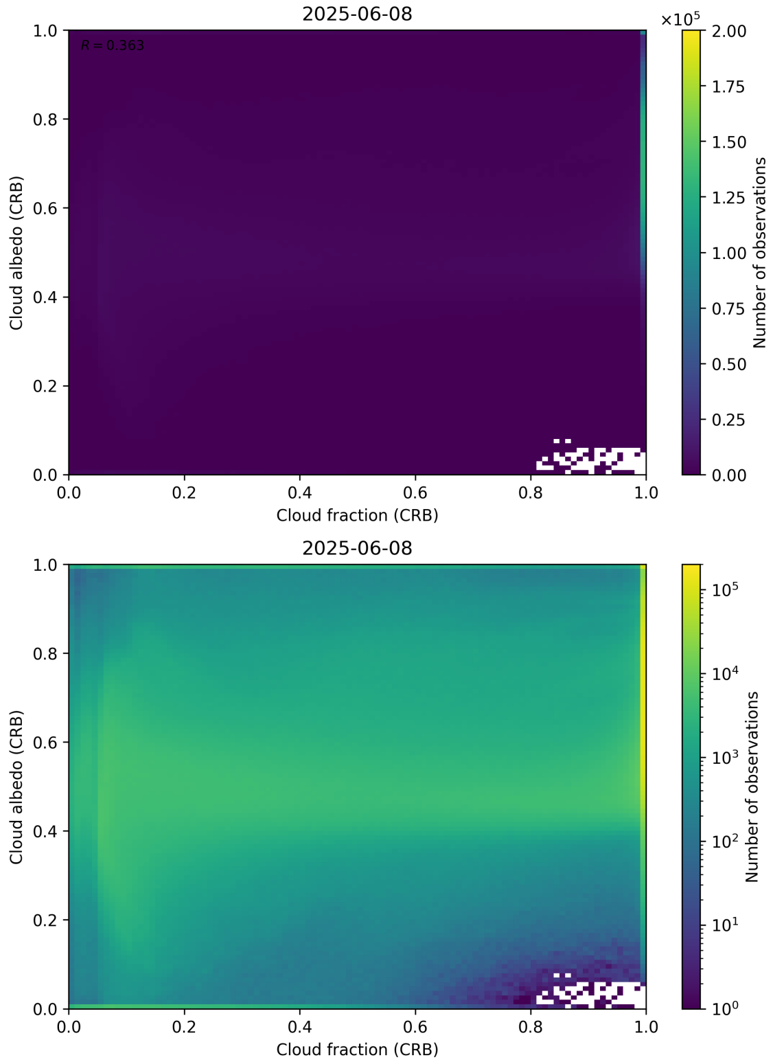
Figure 77: Scatter density plot of “Cloud fraction (CRB)” against “Cloud albedo (CRB)” for 2025-06-07 to 2025-06-09.
