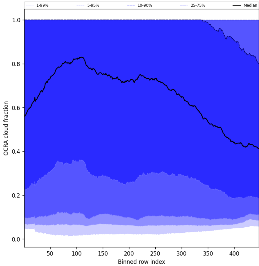
Figure 66: Along track statistics of “OCRA cloud fraction” for 2025-06-07 to 2025-06-09
