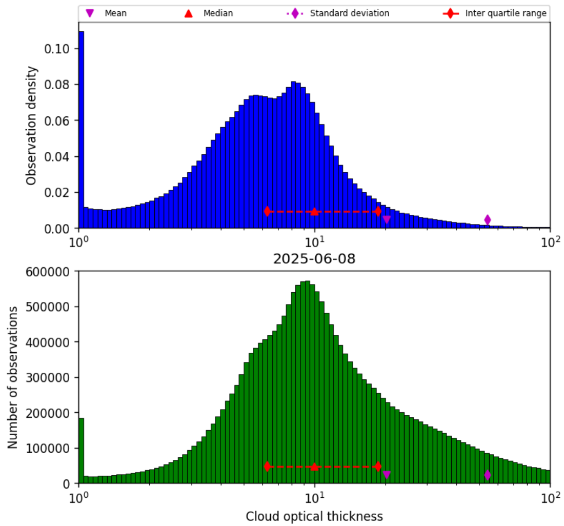
Figure 41: Histogram of “Cloud optical thickness” for 2025-06-07 to 2025-06-09
