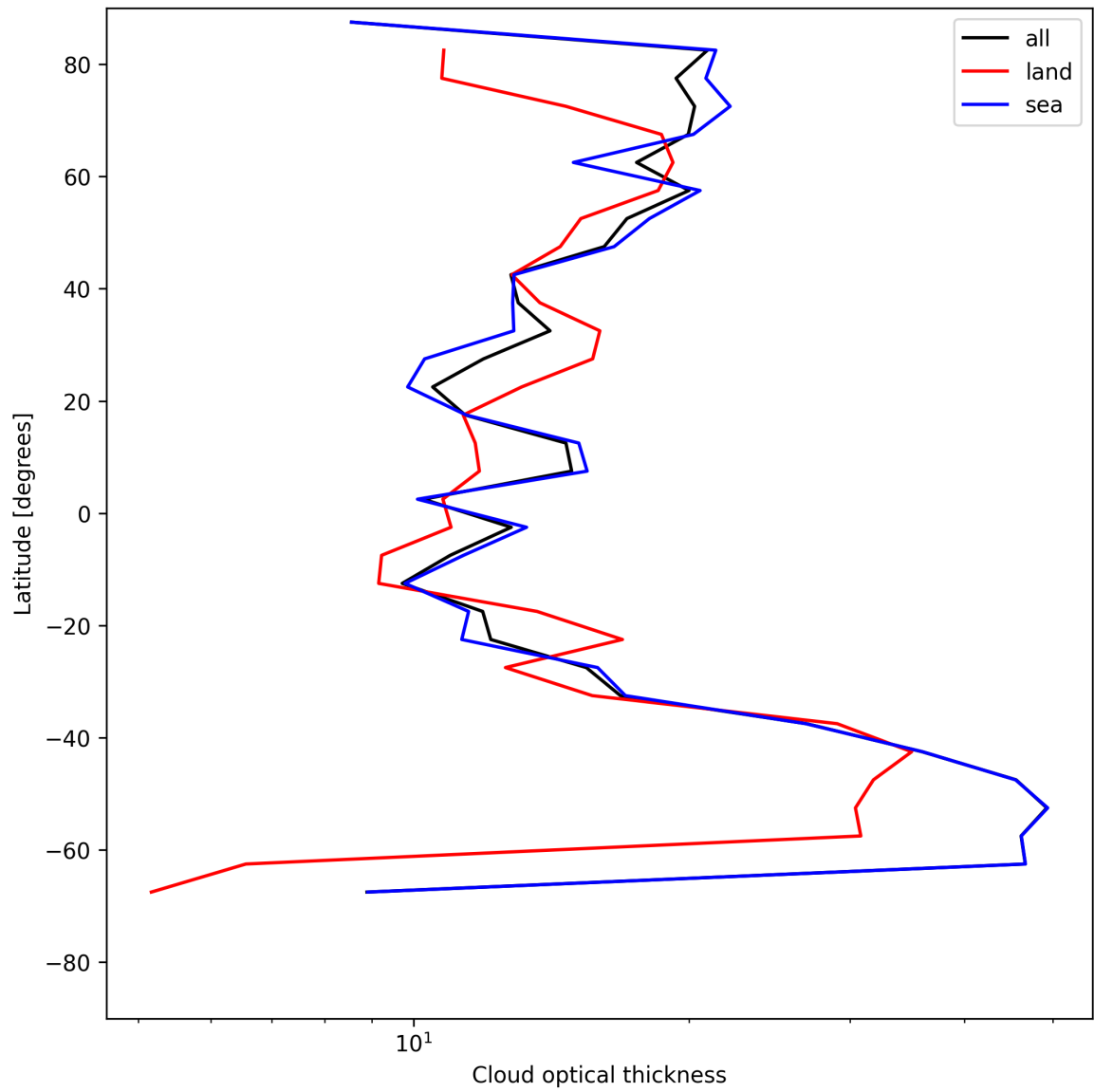
Figure 25: Zonal average of “Cloud optical thickness” for 2025-06-07 to 2025-06-09.
