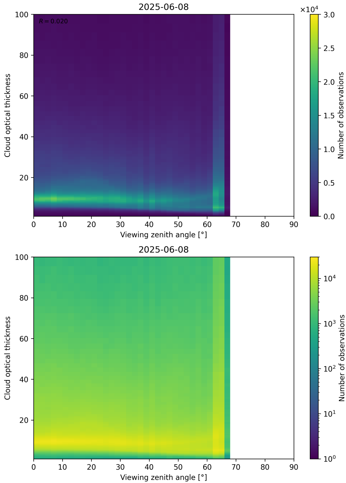
Figure 111: Scatter density plot of “Viewing zenith angle” against “Cloud optical thickness” for 2025-06-07 to 2025-06-09.
