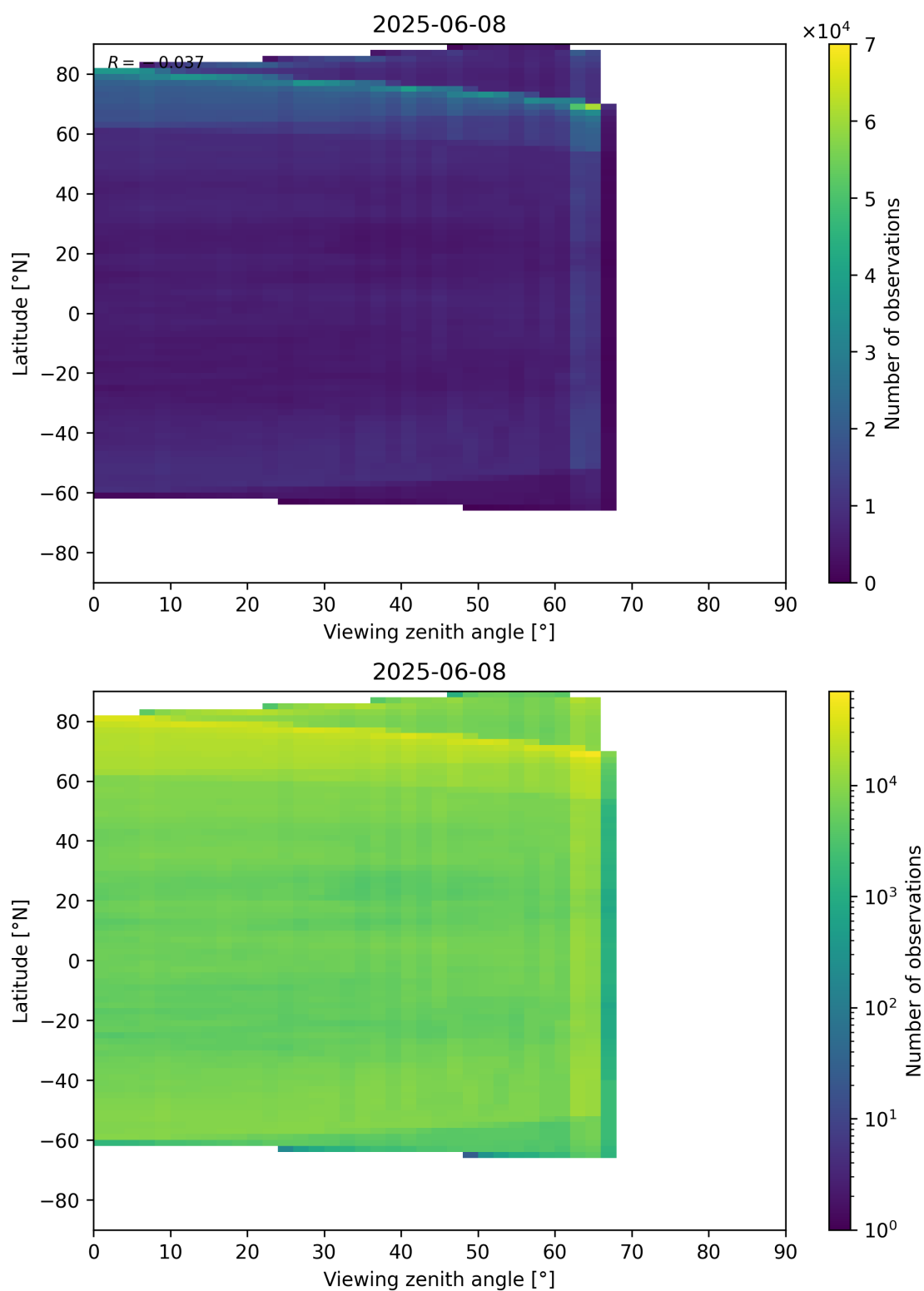
Figure 113: Scatter density plot of “Viewing zenith angle” against “Latitude” for 2025-06-07 to 2025-06-09.
