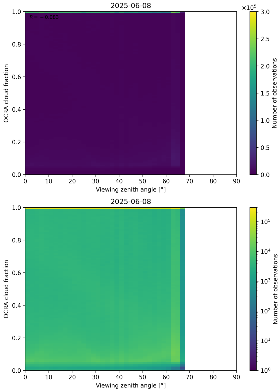
Figure 108: Scatter density plot of “Viewing zenith angle” against “OCRA cloud fraction” for 2025-06-07 to 2025-06-09.
