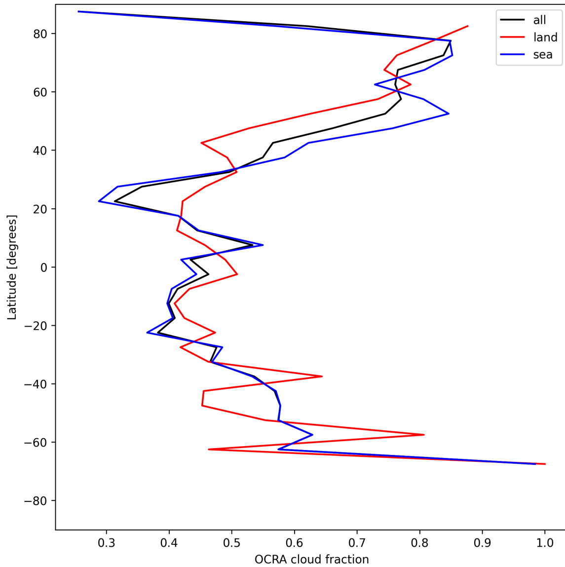
Figure 34: Zonal average of “OCRA cloud fraction” for 2025-06-07 to 2025-06-09.
