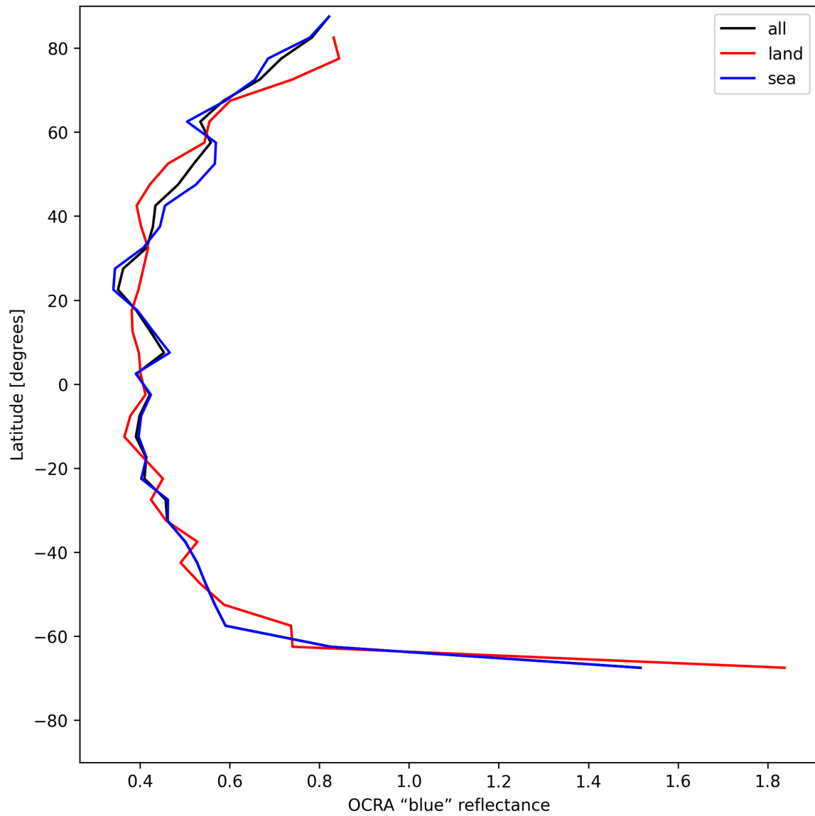
Figure 35: Zonal average of “OCRA “blue” reflectance” for 2025-06-07 to 2025-06-09.
