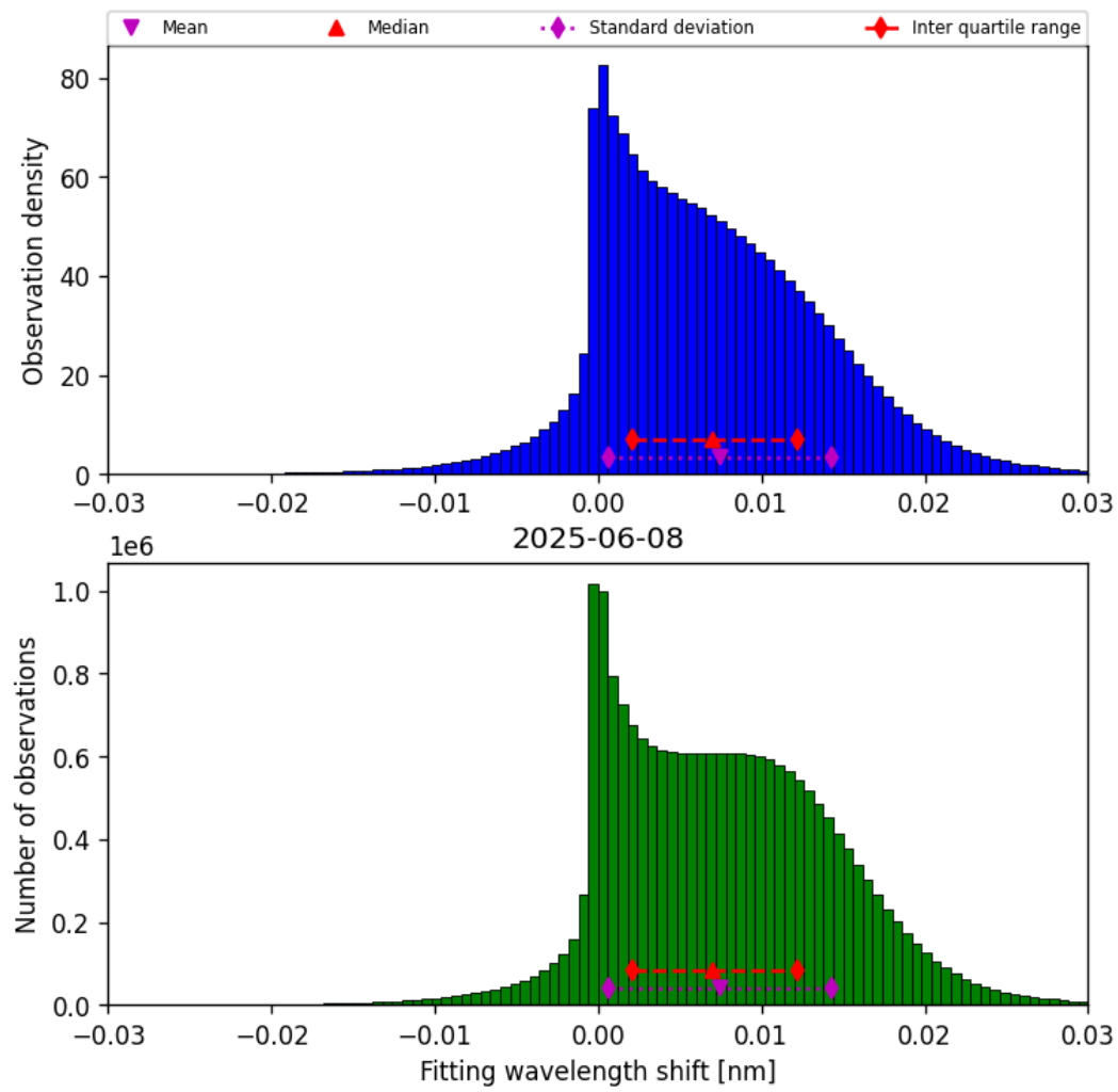
Figure 49: Histogram of “Fitting wavelength shift” for 2025-06-07 to 2025-06-09
