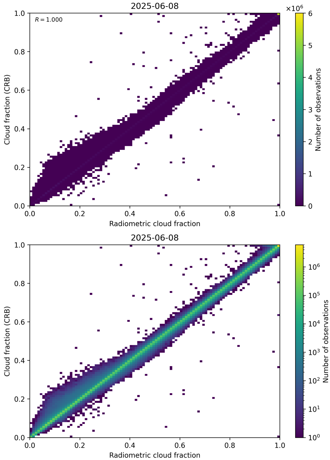
Figure 73: Scatter density plot of “Radiometric cloud fraction” against “Cloud fraction (CRB)” for 2025-06-07 to 2025-06-09.
