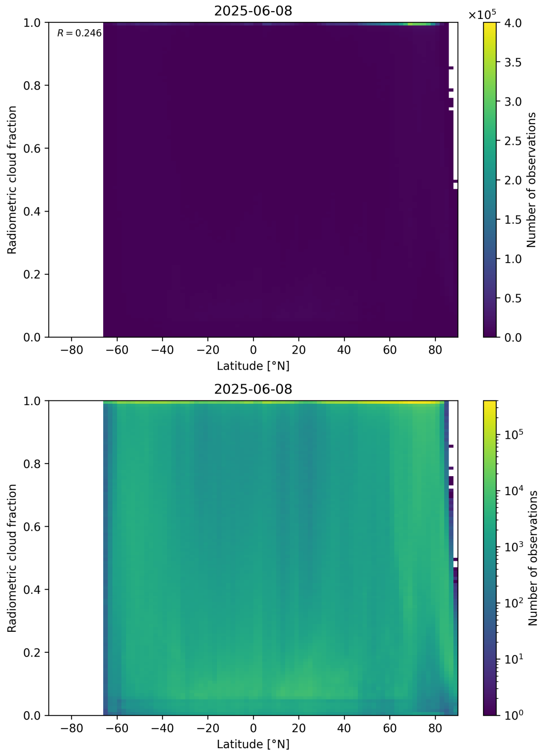
Figure 92: Scatter density plot of “Latitude” against “Radiometric cloud fraction” for 2025-06-07 to 2025-06-09.
