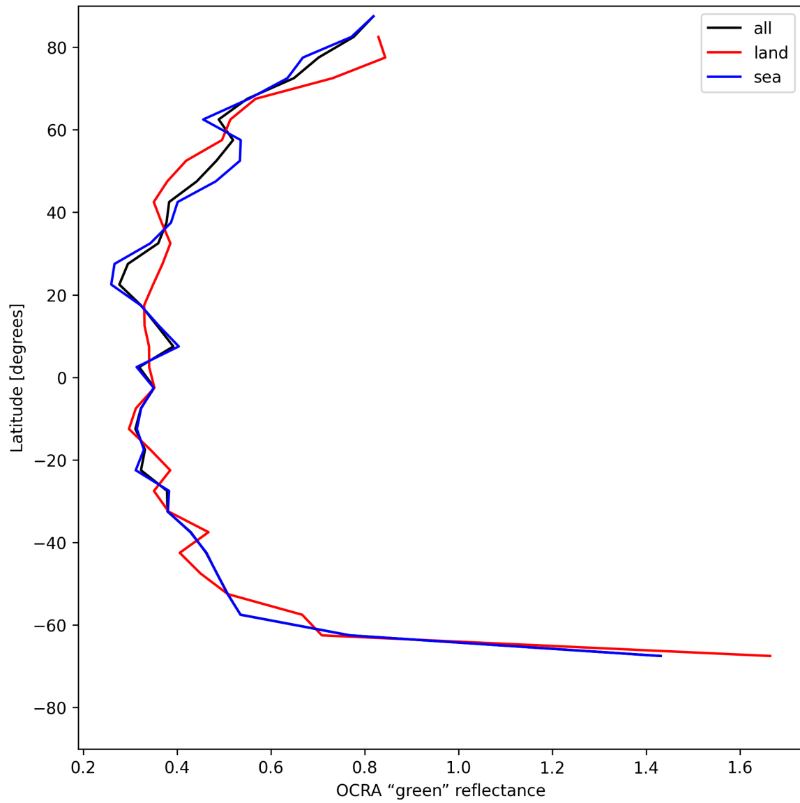
Figure 36: Zonal average of “OCRA “green” reflectance” for 2025-06-07 to 2025-06-09.
