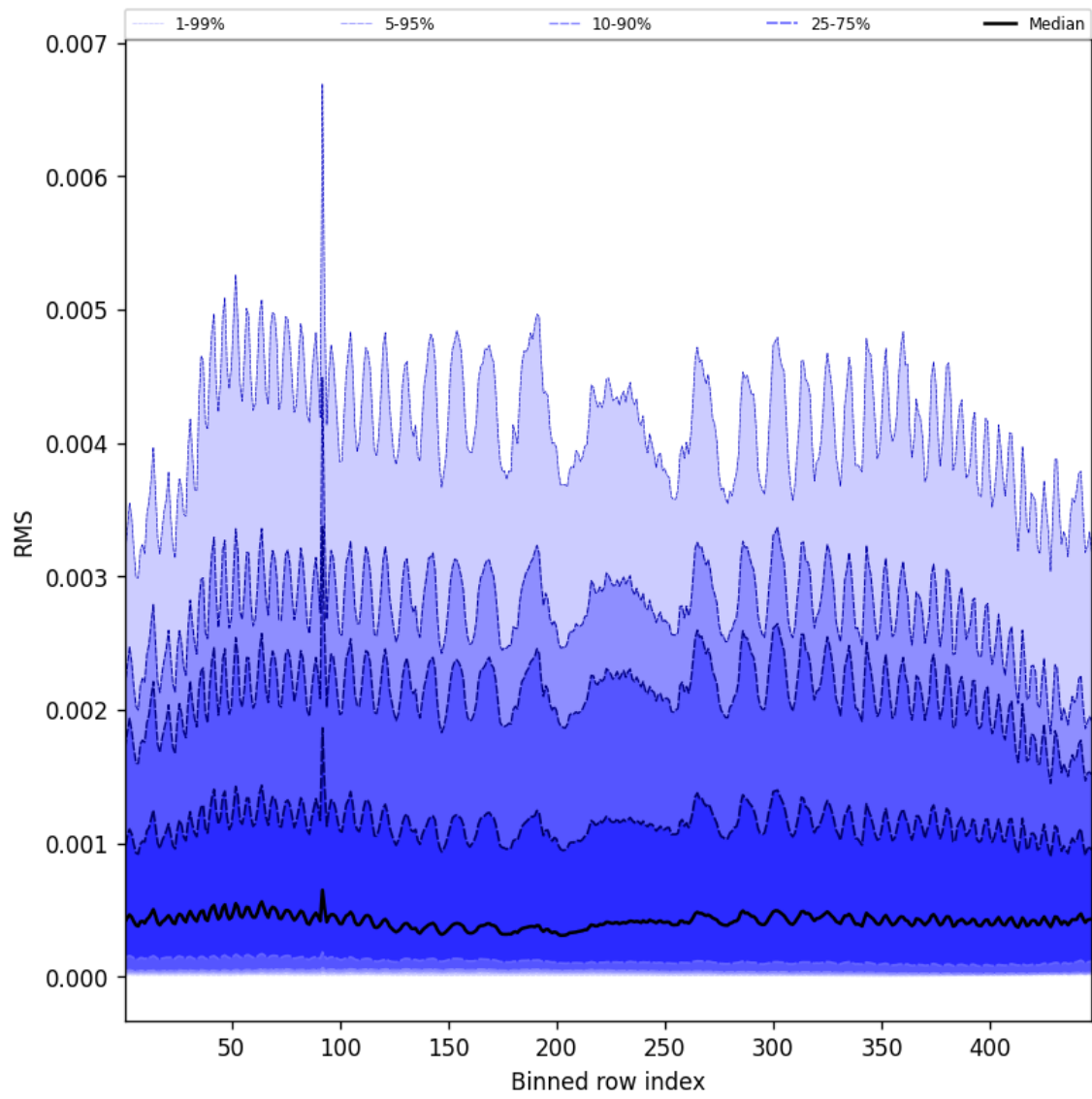
Figure 63: Along track statistics of “RMS” for 2025-06-07 to 2025-06-09
