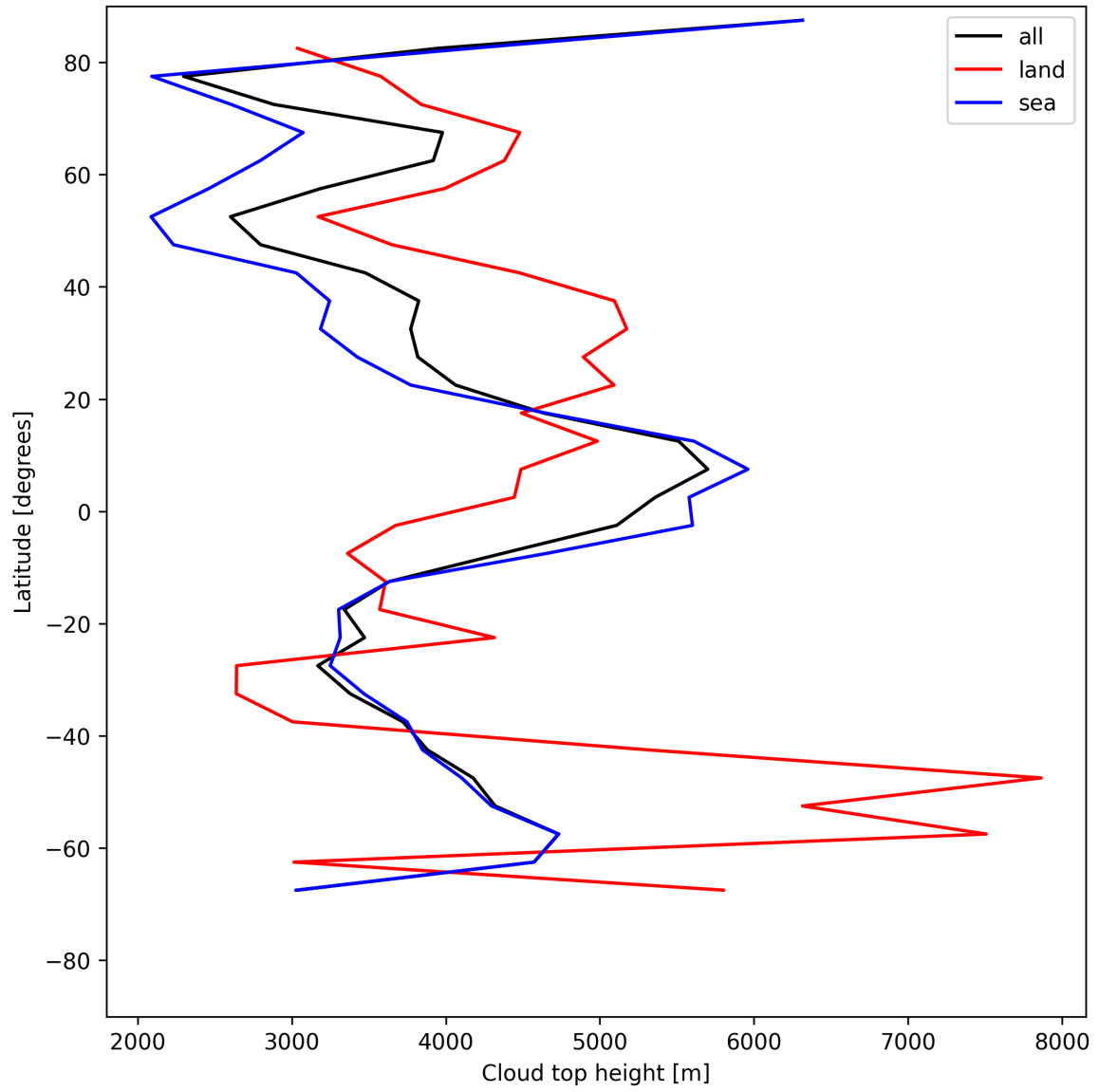
Figure 24: Zonal average of “Cloud top height” for 2025-06-07 to 2025-06-09.
