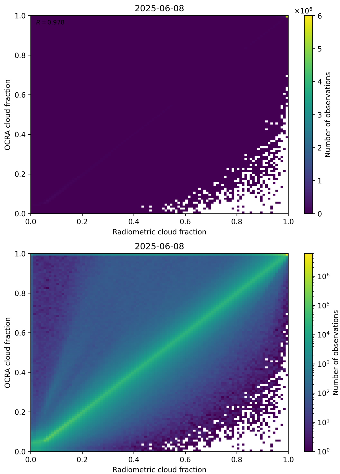
Figure 72: Scatter density plot of “Radiometric cloud fraction” against “OCRA cloud fraction” for 2025-06-07 to 2025-06-09.
