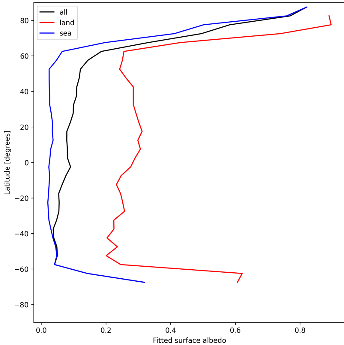
Figure 29: Zonal average of “Fitted surface albedo” for 2025-06-07 to 2025-06-09.
