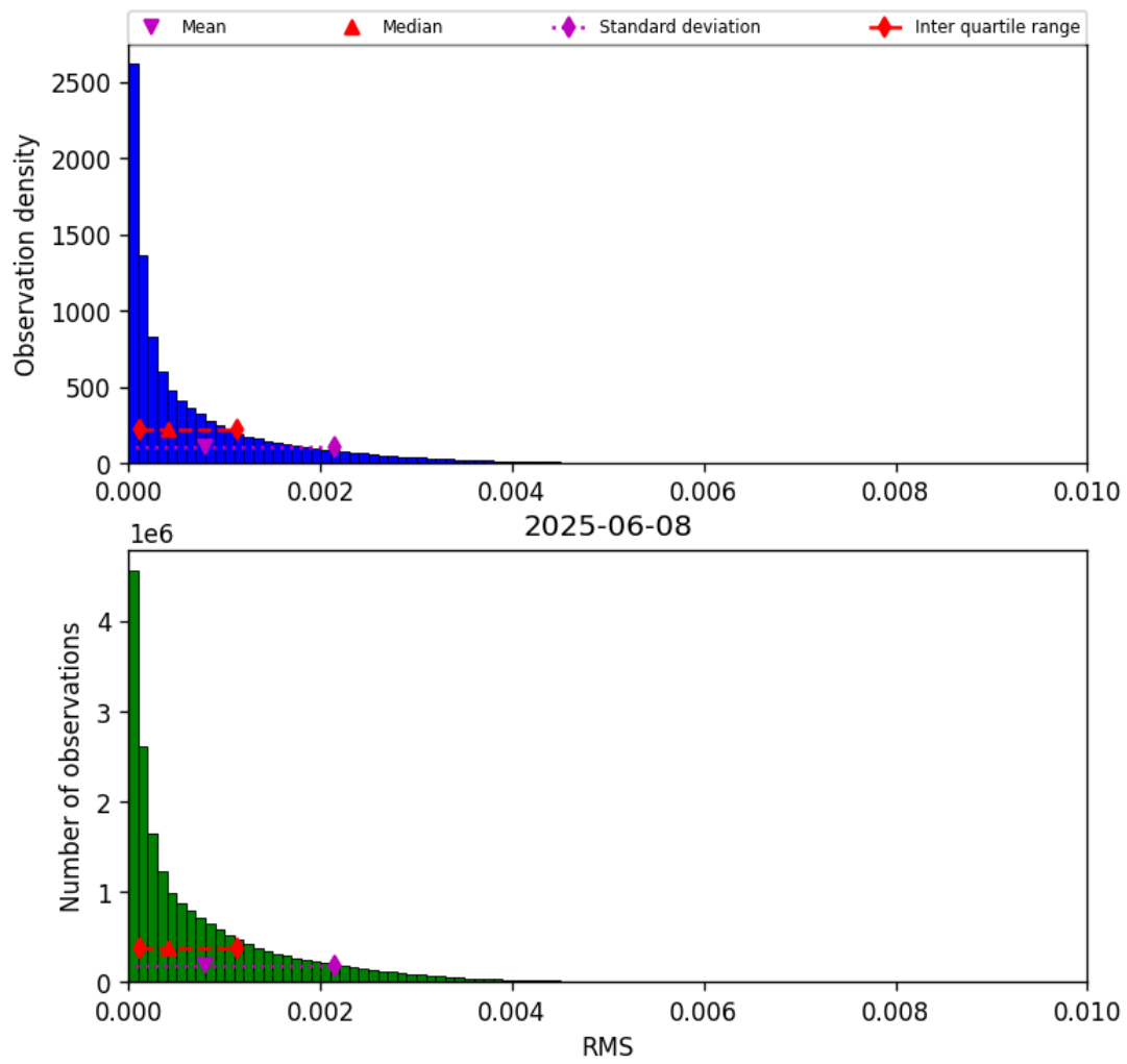
Figure 47: Histogram of “RMS” for 2025-06-07 to 2025-06-09
