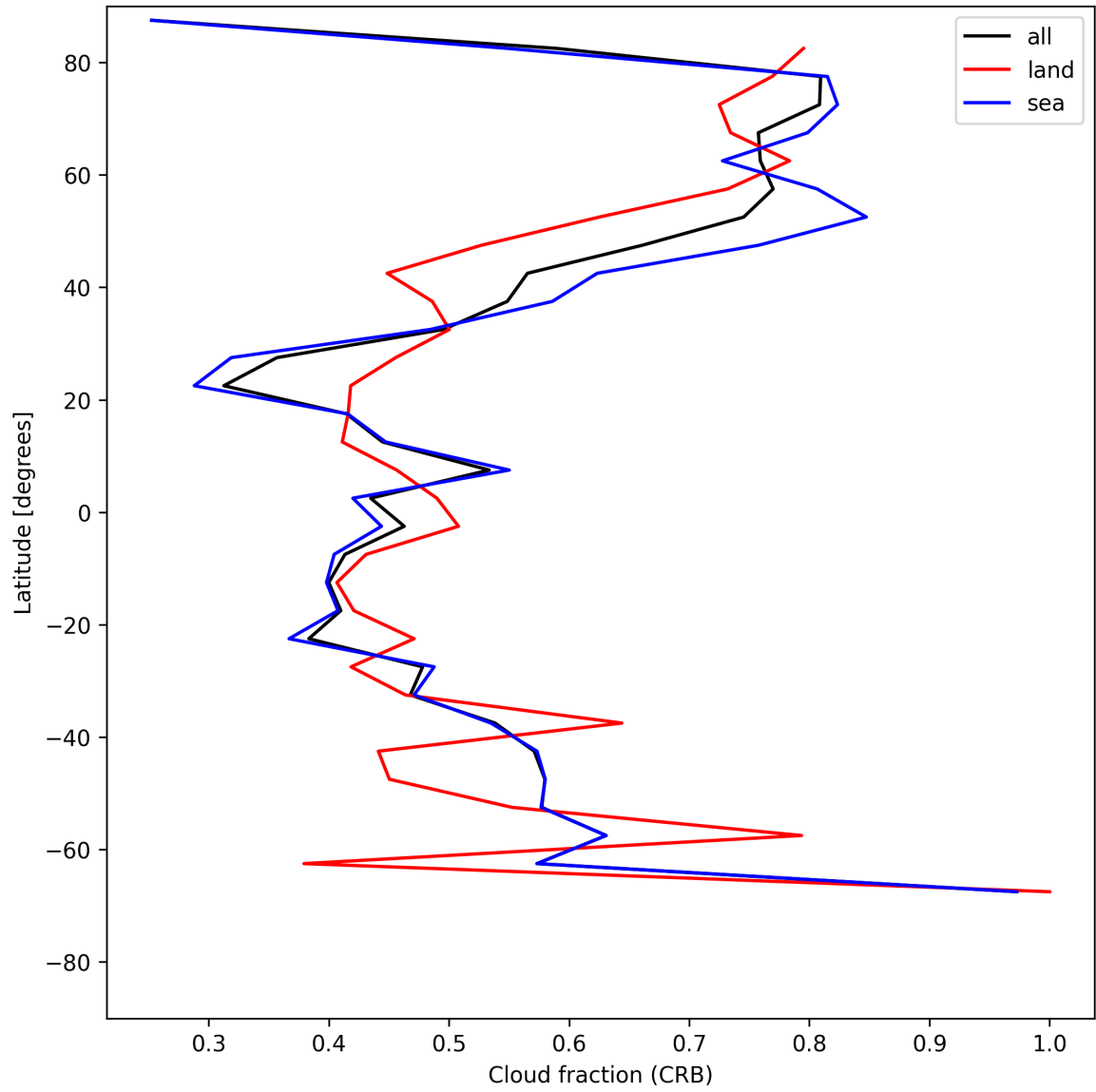
Figure 26: Zonal average of “Cloud fraction (CRB)” for 2025-06-07 to 2025-06-09.
