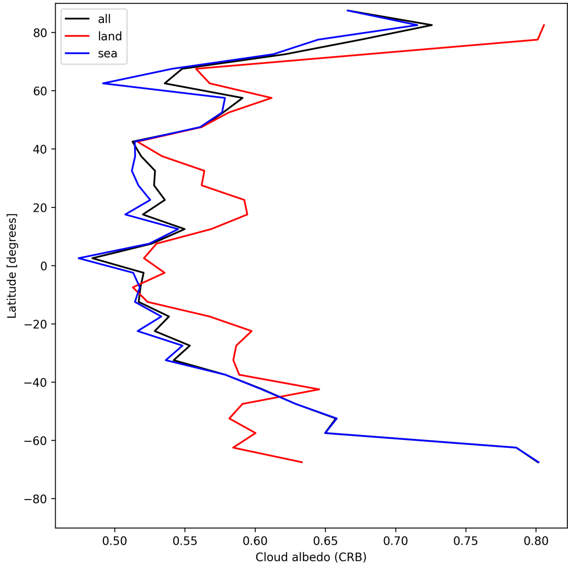
Figure 28: Zonal average of “Cloud albedo (CRB)” for 2025-06-07 to 2025-06-09.
