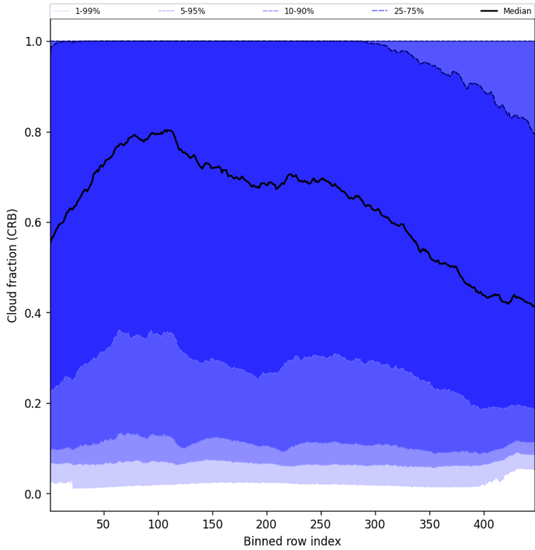
Figure 58: Along track statistics of “Cloud fraction (CRB)” for 2025-06-07 to 2025-06-09
