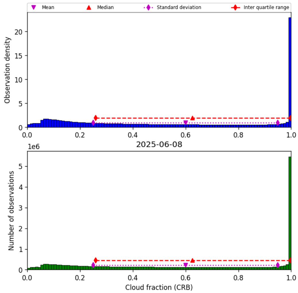
Figure 42: Histogram of “Cloud fraction (CRB)” for 2025-06-07 to 2025-06-09
