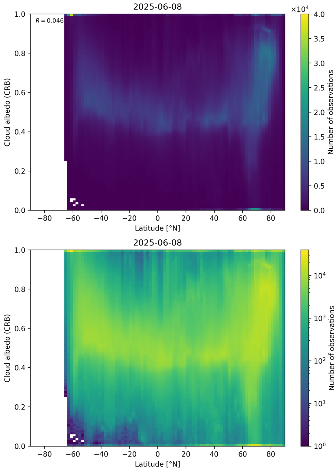
Figure 91: Scatter density plot of “Latitude” against “Cloud albedo (CRB)” for 2025-06-07 to 2025-06-09.
