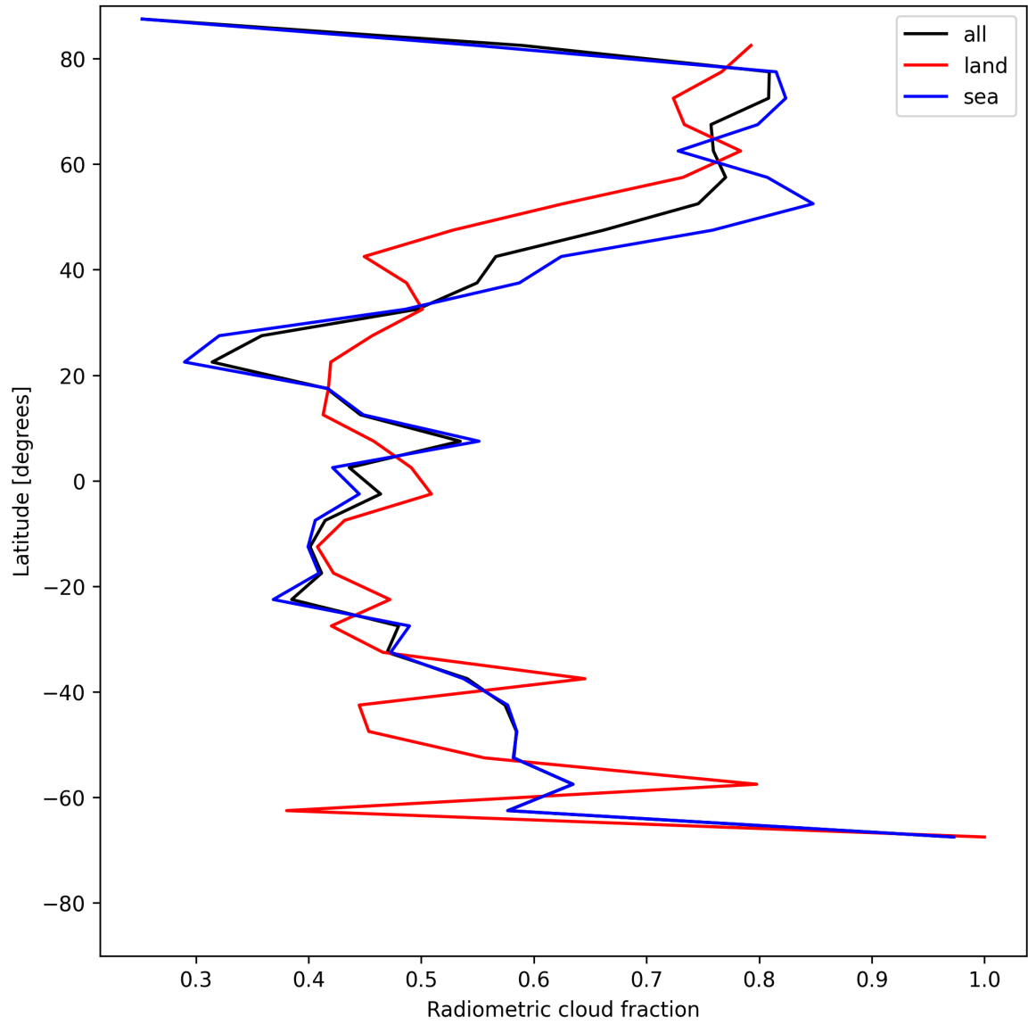
Figure 23: Zonal average of “Radiometric cloud fraction” for 2025-06-07 to 2025-06-09.
