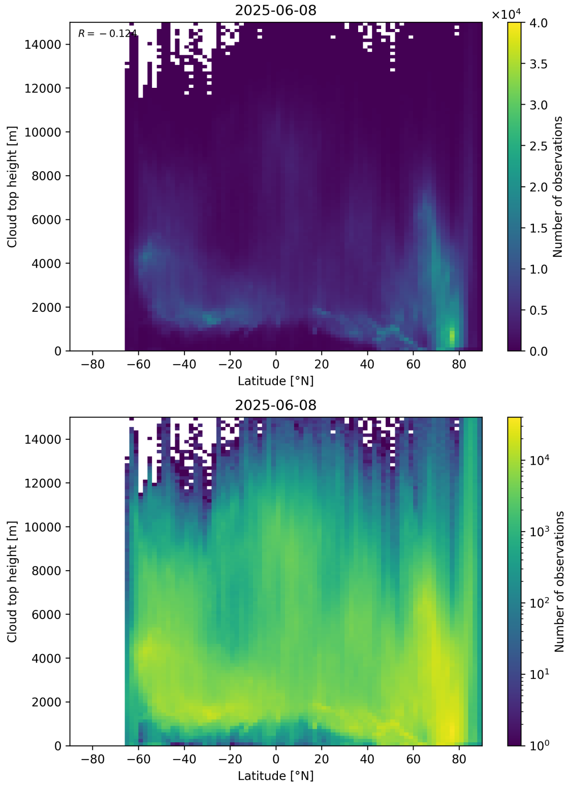
Figure 97: Scatter density plot of “Latitude” against “Cloud top height” for 2025-06-07 to 2025-06-09.
