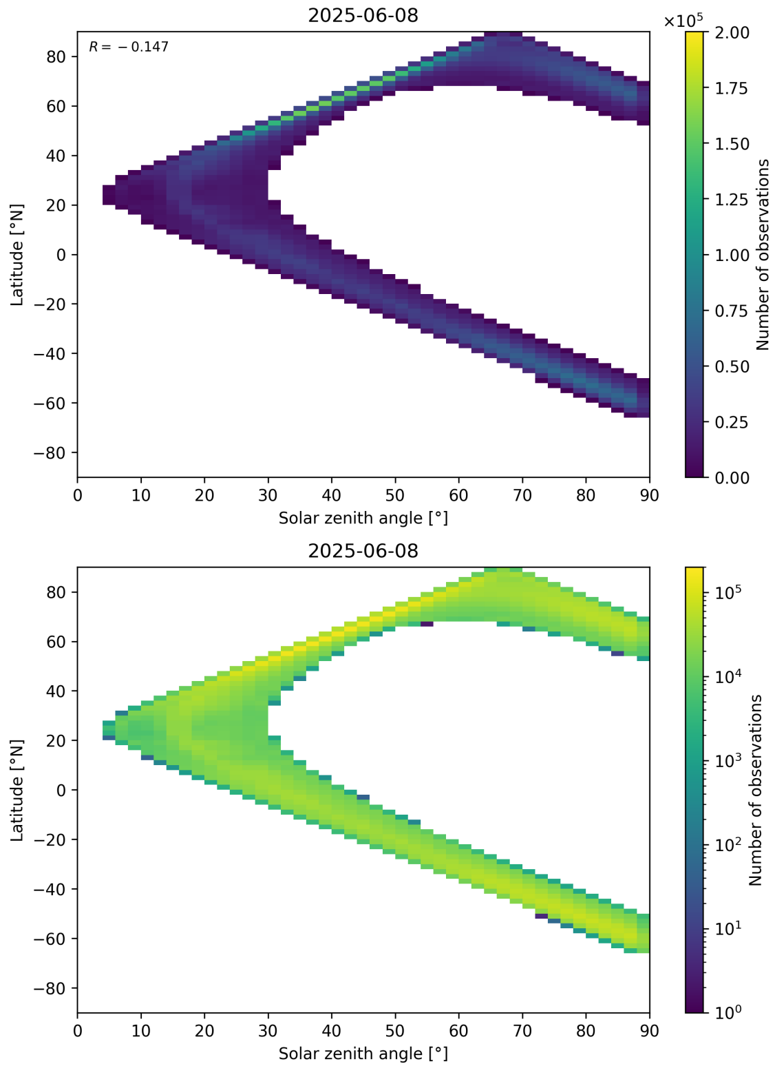
Figure 105: Scatter density plot of “Solar zenith angle” against “Latitude” for 2025-06-07 to 2025-06-09.
