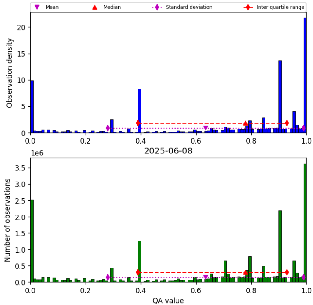
Figure 38: Histogram of “QA value” for 2025-06-07 to 2025-06-09
