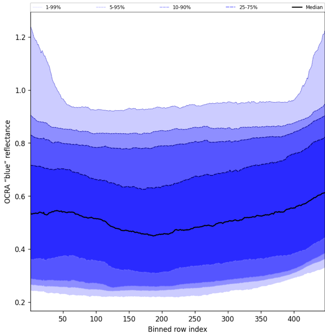
Figure 67: Along track statistics of “OCRA “blue” reflectance” for 2025-06-07 to 2025-06-09
