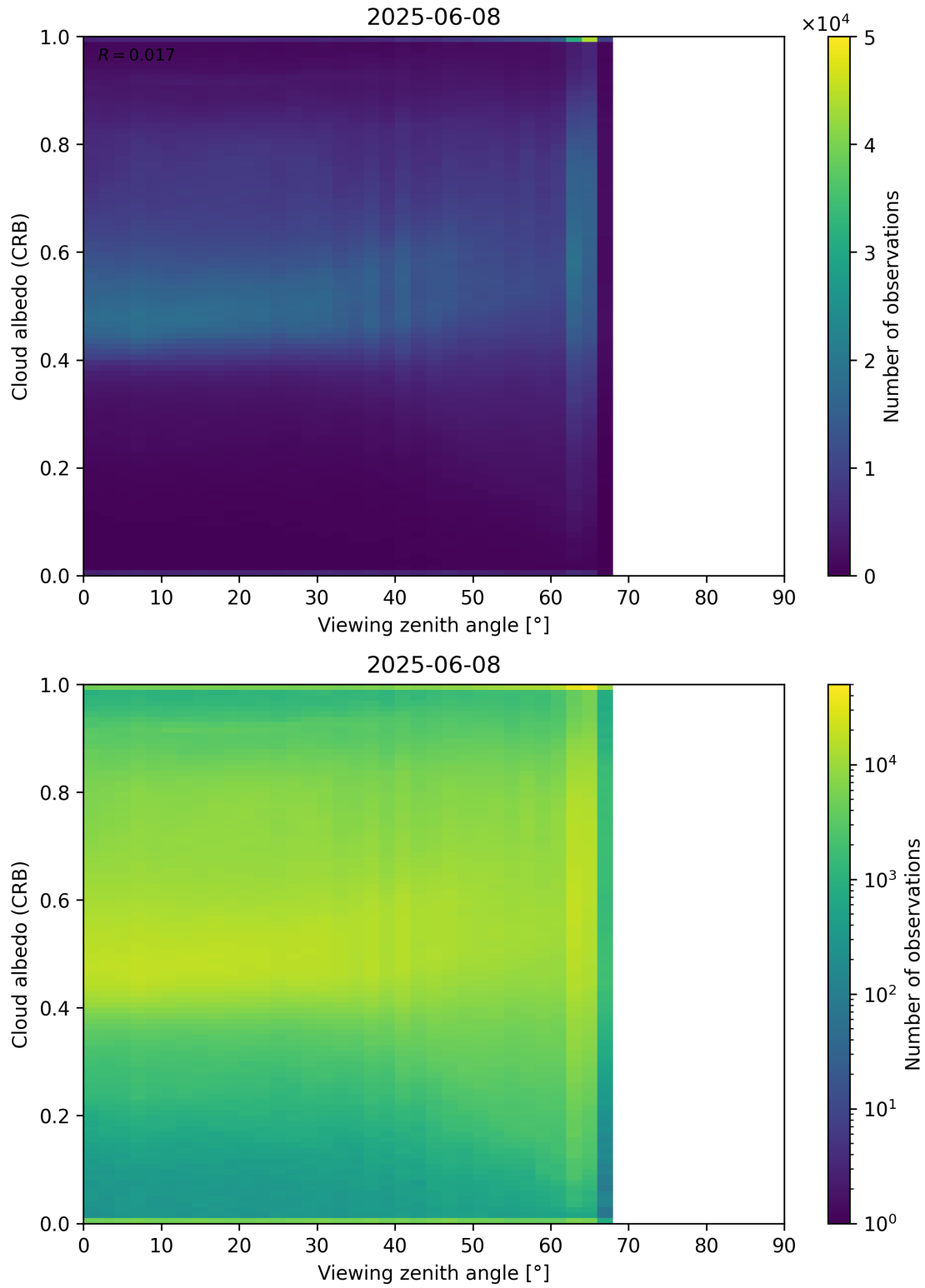
Figure 106: Scatter density plot of “Viewing zenith angle” against “Cloud albedo (CRB)” for 2025-06-07 to 2025-06-09.
