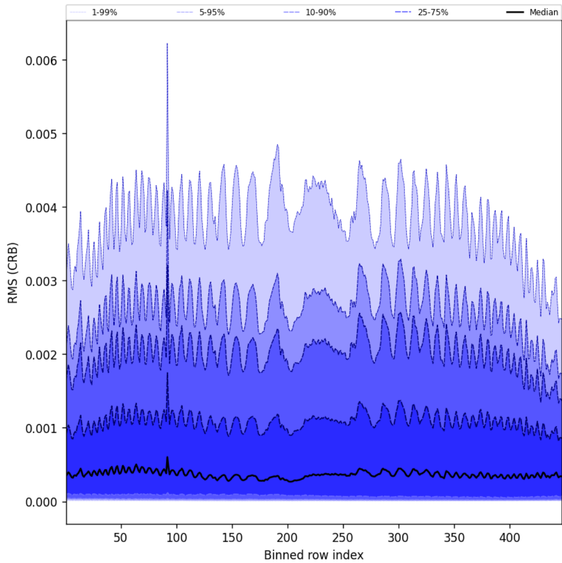
Figure 64: Along track statistics of “RMS (CRB)” for 2025-06-07 to 2025-06-09
