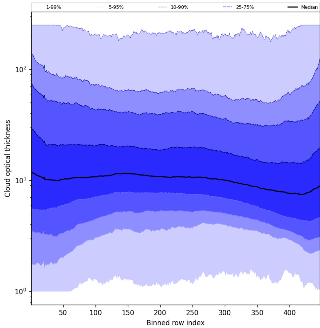
Figure 57: Along track statistics of “Cloud optical thickness” for 2025-06-07 to 2025-06-09
