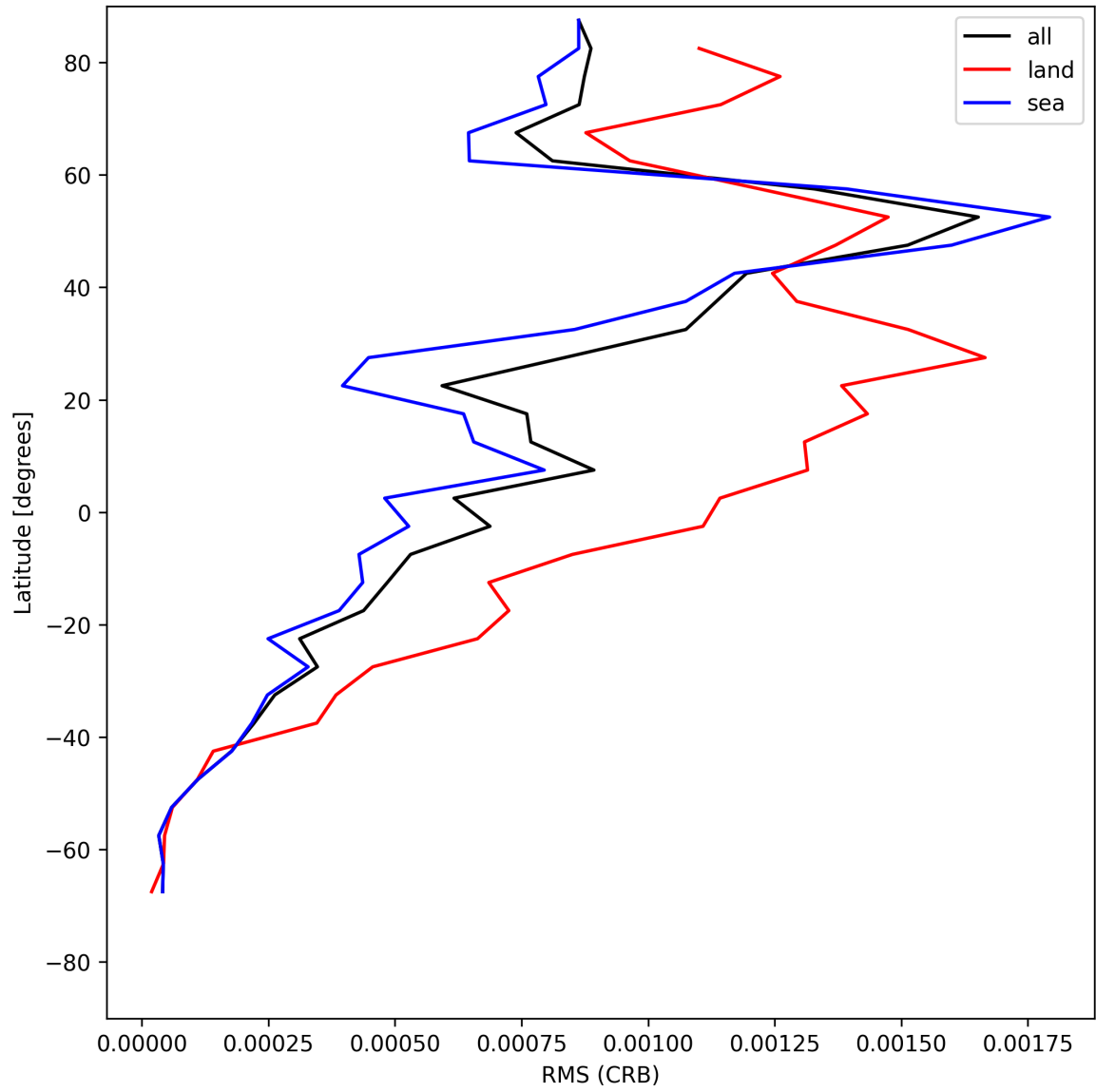
Figure 32: Zonal average of “RMS (CRB)” for 2025-06-07 to 2025-06-09.
