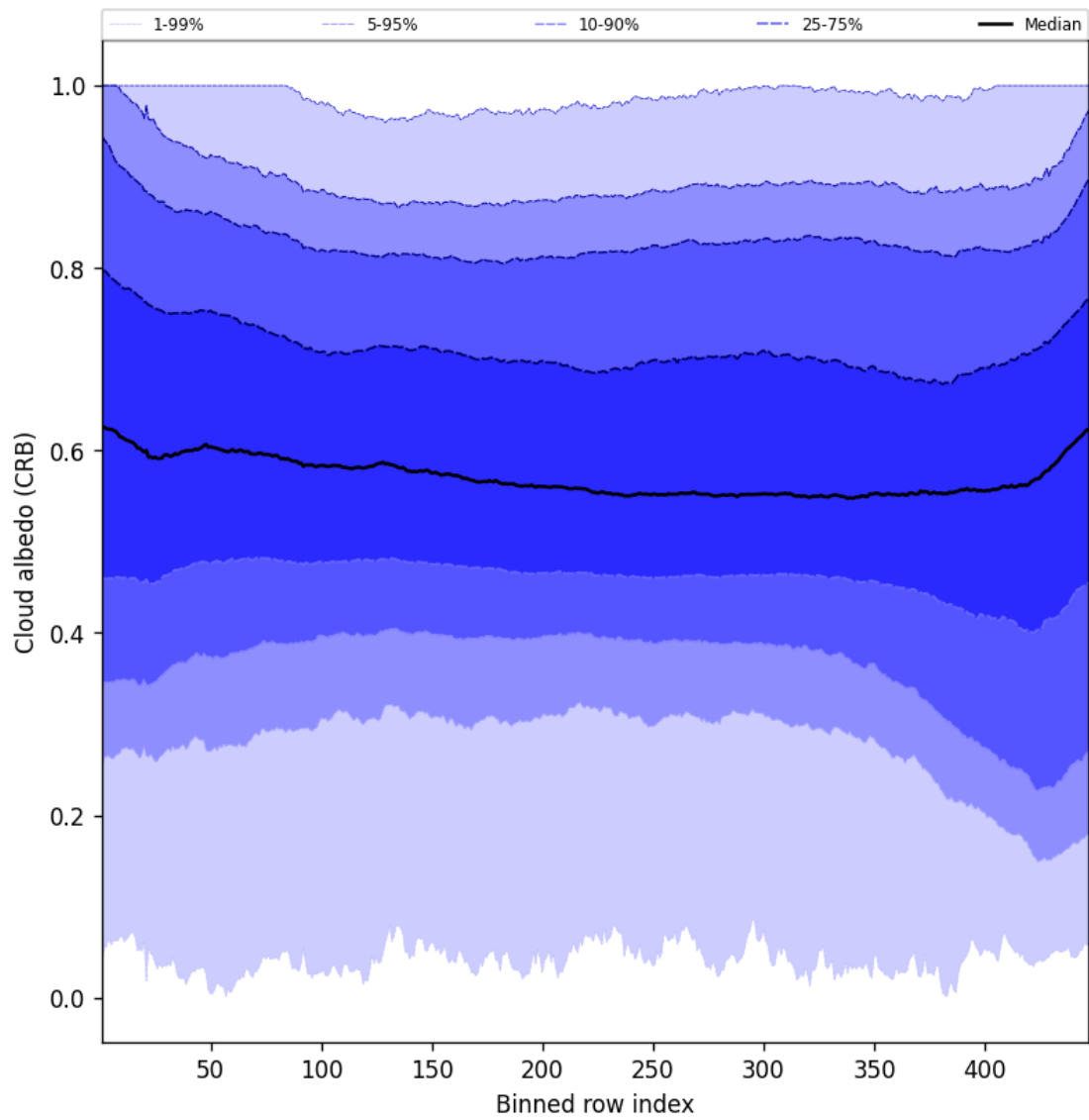
Figure 60: Along track statistics of “Cloud albedo (CRB)” for 2025-06-07 to 2025-06-09
