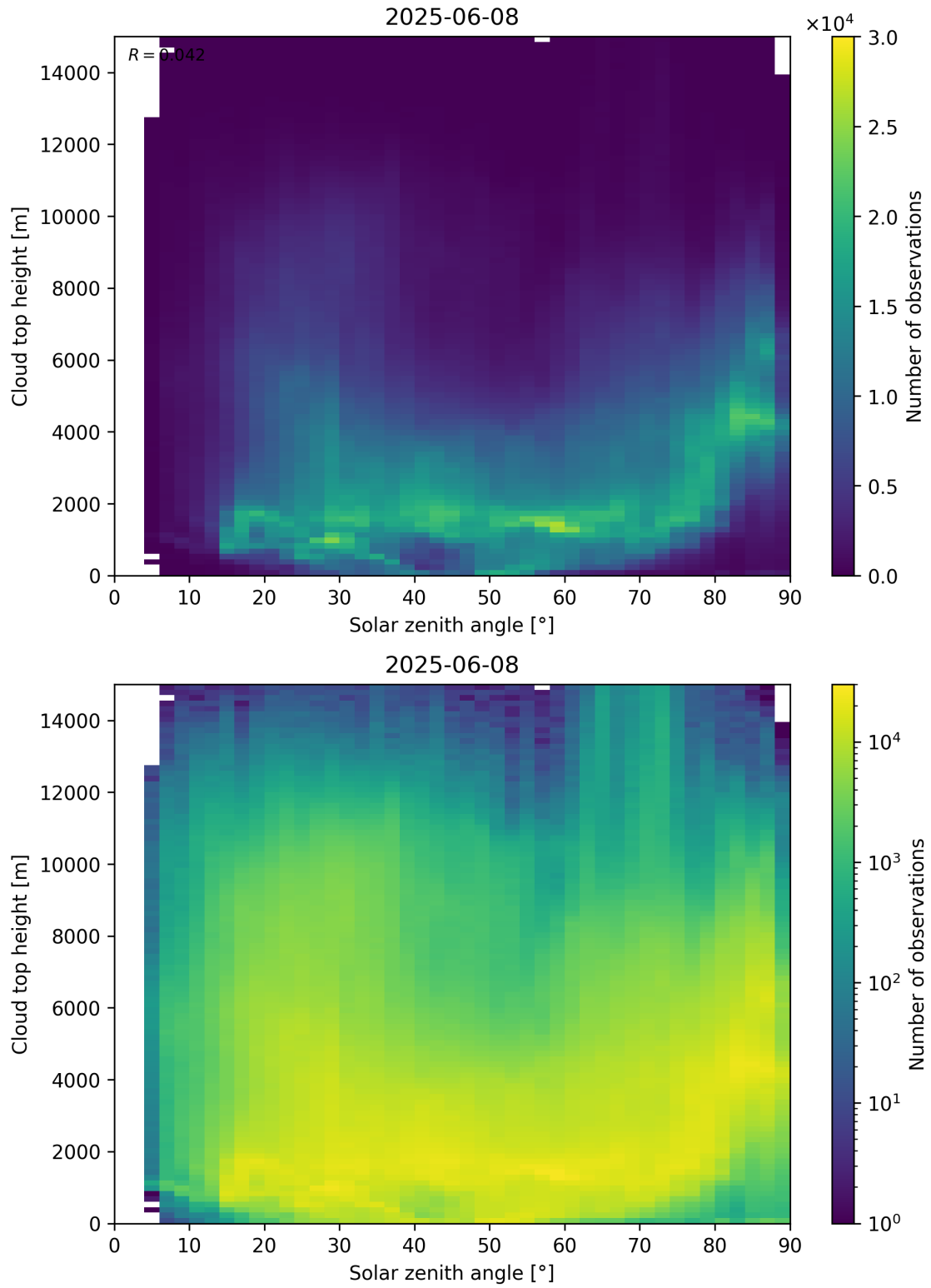
Figure 104: Scatter density plot of “Solar zenith angle” against “Cloud top height” for 2025-06-07 to 2025-06-09.
