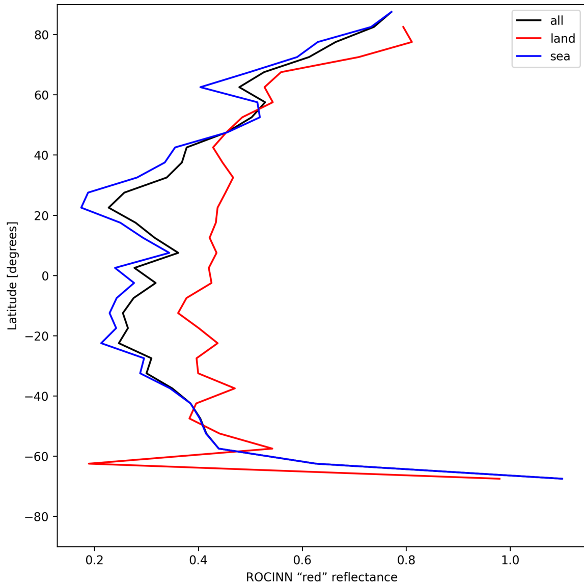
Figure 37: Zonal average of “ROCINN “red” reflectance” for 2025-06-07 to 2025-06-09.
