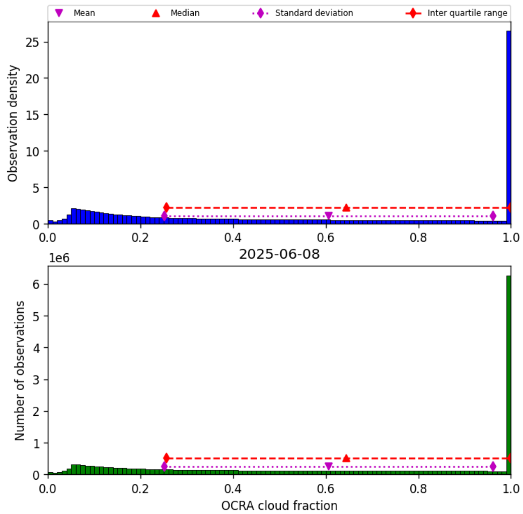
Figure 50: Histogram of “OCRA cloud fraction” for 2025-06-07 to 2025-06-09
