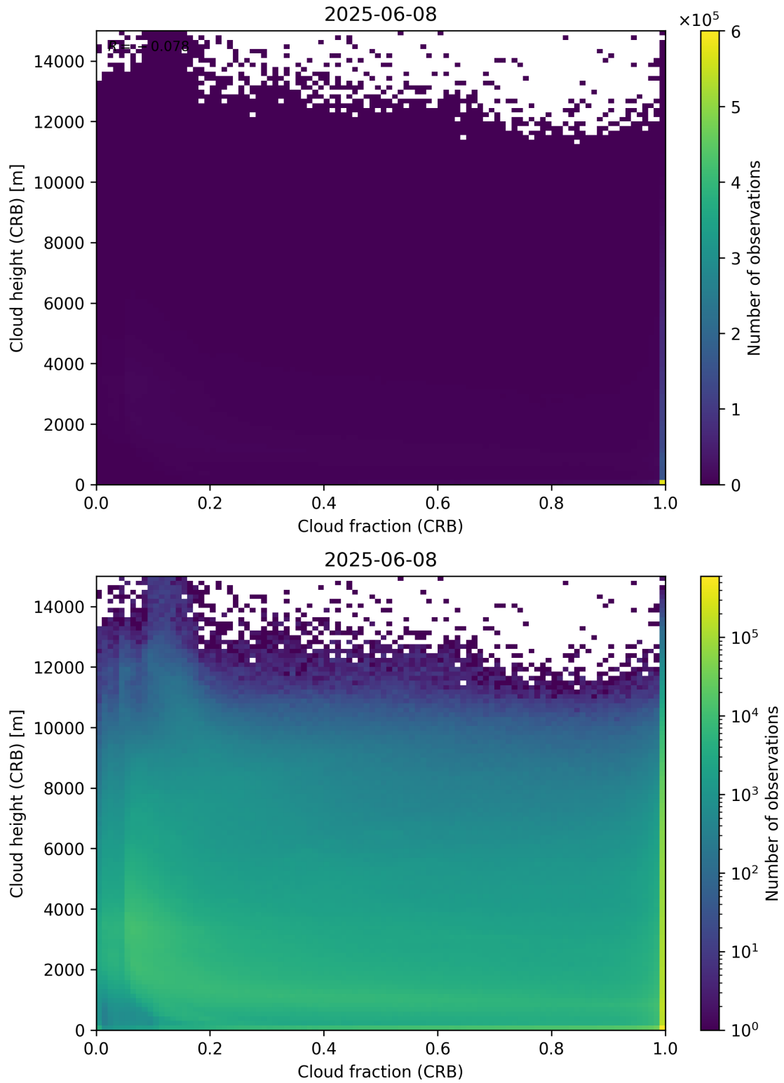
Figure 79: Scatter density plot of “Cloud fraction (CRB)” against “Cloud height (CRB)” for 2025-06-07 to 2025-06-09.
