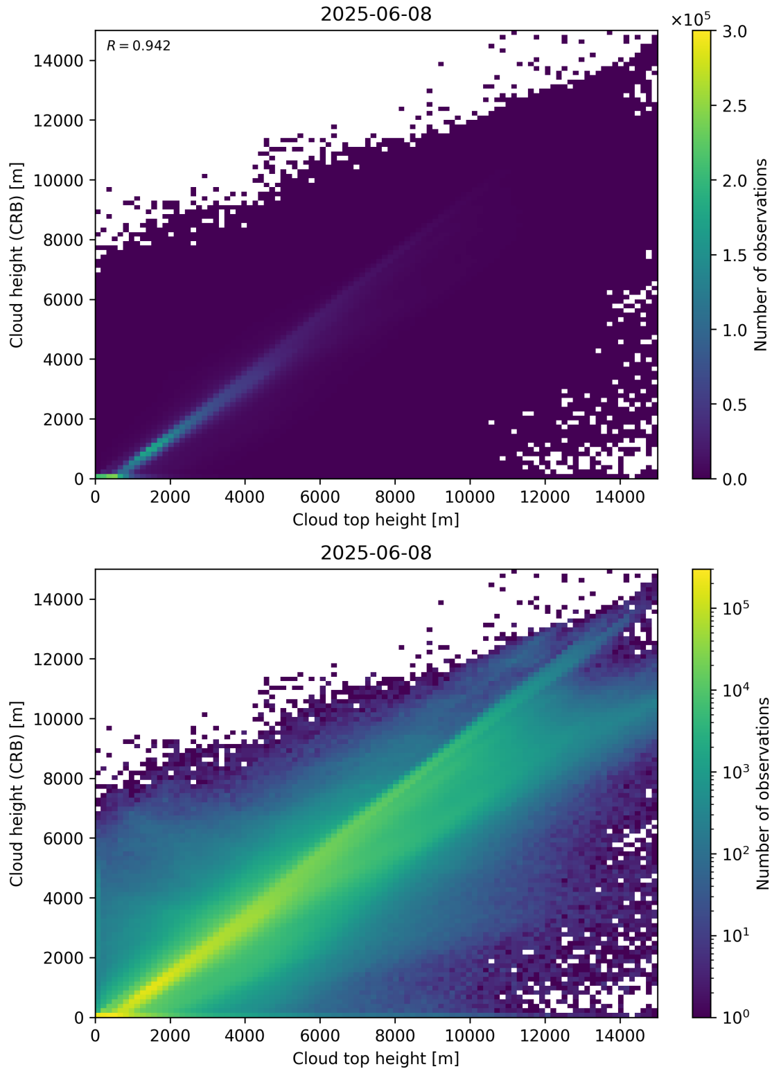
Figure 89: Scatter density plot of “Cloud top height” against “Cloud height (CRB)” for 2025-06-07 to 2025-06-09.
