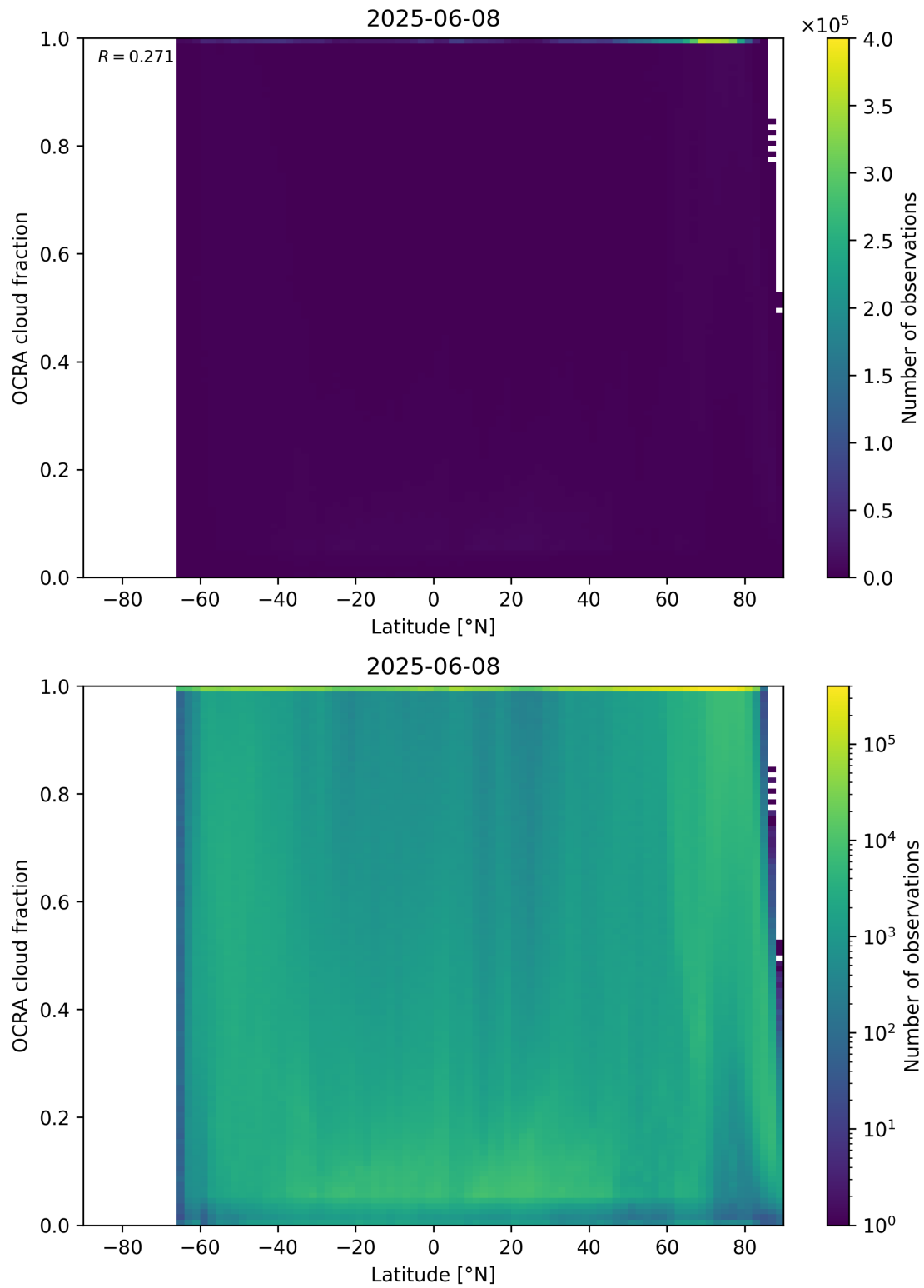
Figure 93: Scatter density plot of “Latitude” against “OCRA cloud fraction” for 2025-06-07 to 2025-06-09.
