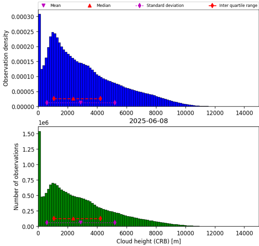
Figure 43: Histogram of “Cloud height (CRB)” for 2025-06-07 to 2025-06-09
