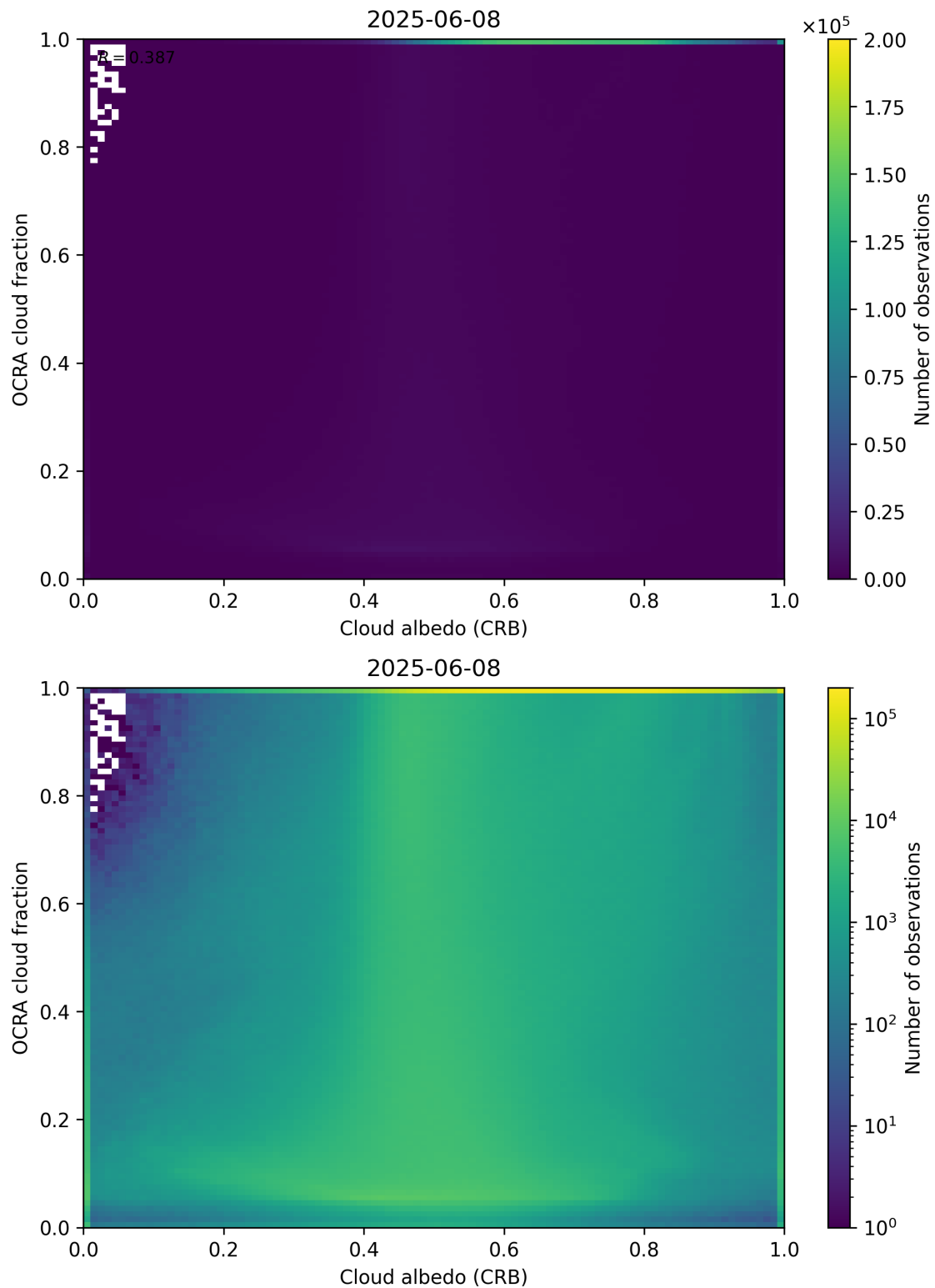
Figure 70: Scatter density plot of “Cloud albedo (CRB)” against “OCRA cloud fraction” for 2025-06-07 to 2025-06-09.
