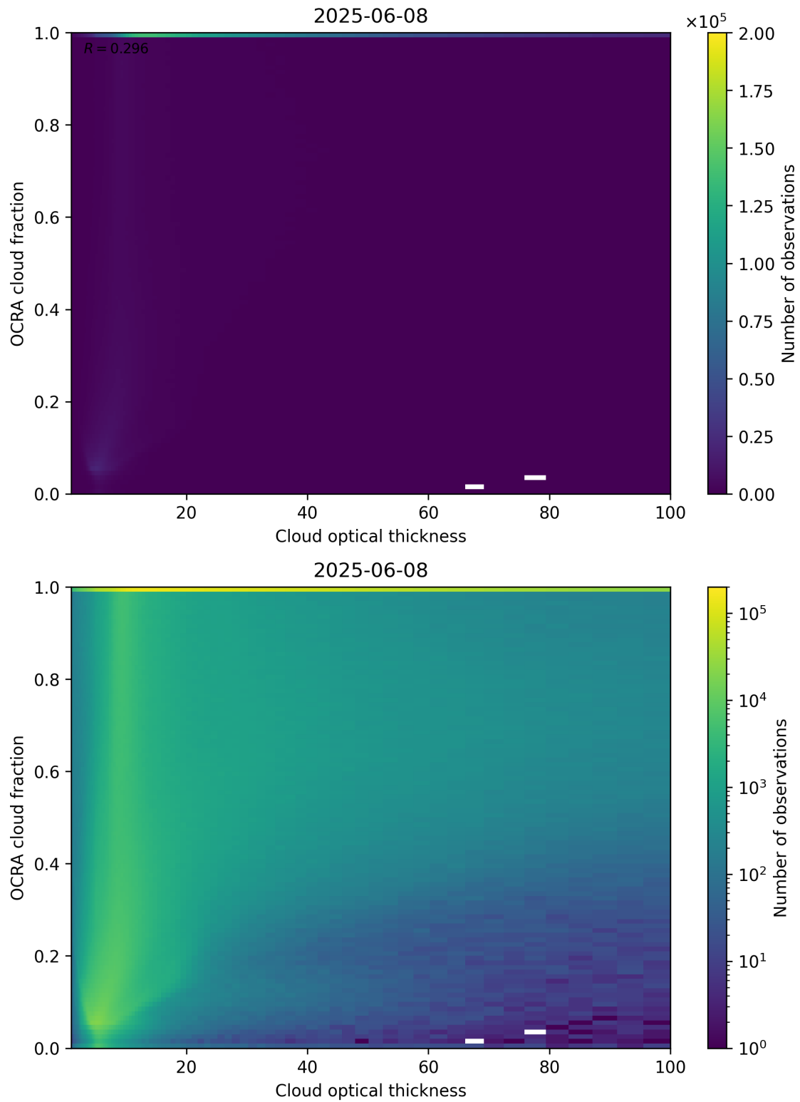
Figure 83: Scatter density plot of “Cloud optical thickness” against “OCRA cloud fraction” for 2025-06-07 to 2025-06-09.
