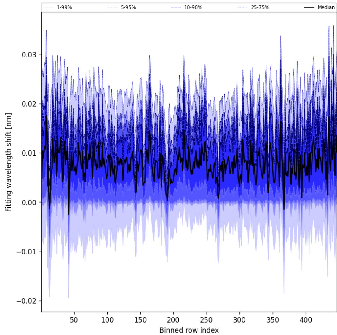
Figure 65: Along track statistics of “Fitting wavelength shift” for 2025-06-07 to 2025-06-09
