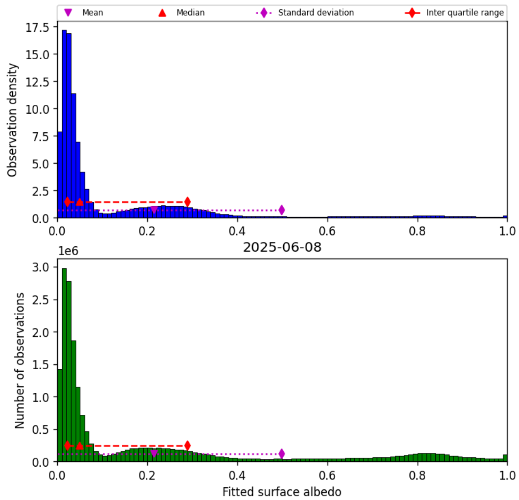
Figure 45: Histogram of “Fitted surface albedo” for 2025-06-07 to 2025-06-09
