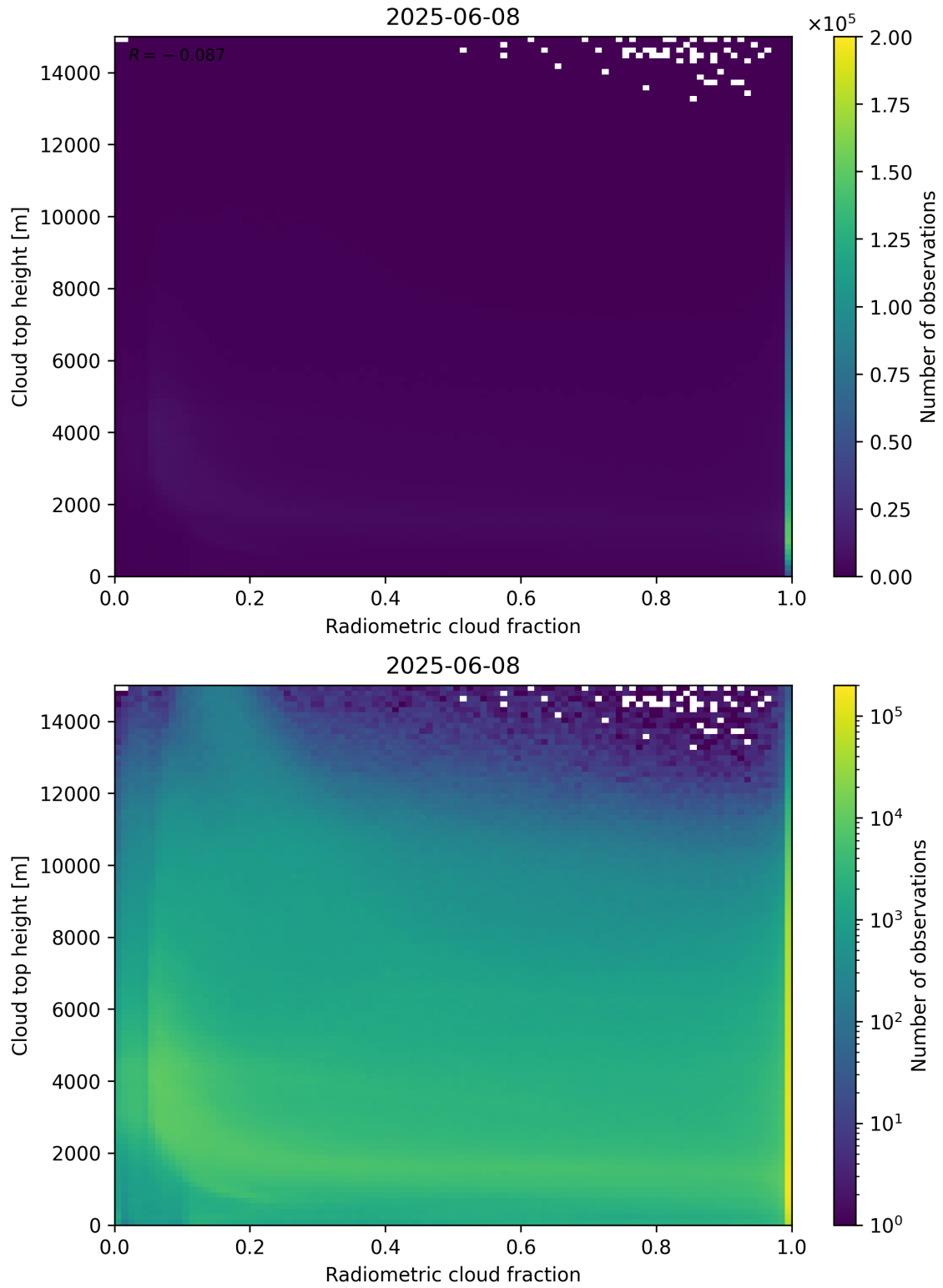
Figure 76: Scatter density plot of “Radiometric cloud fraction” against “Cloud top height” for 2025-06-07 to 2025-06-09.
