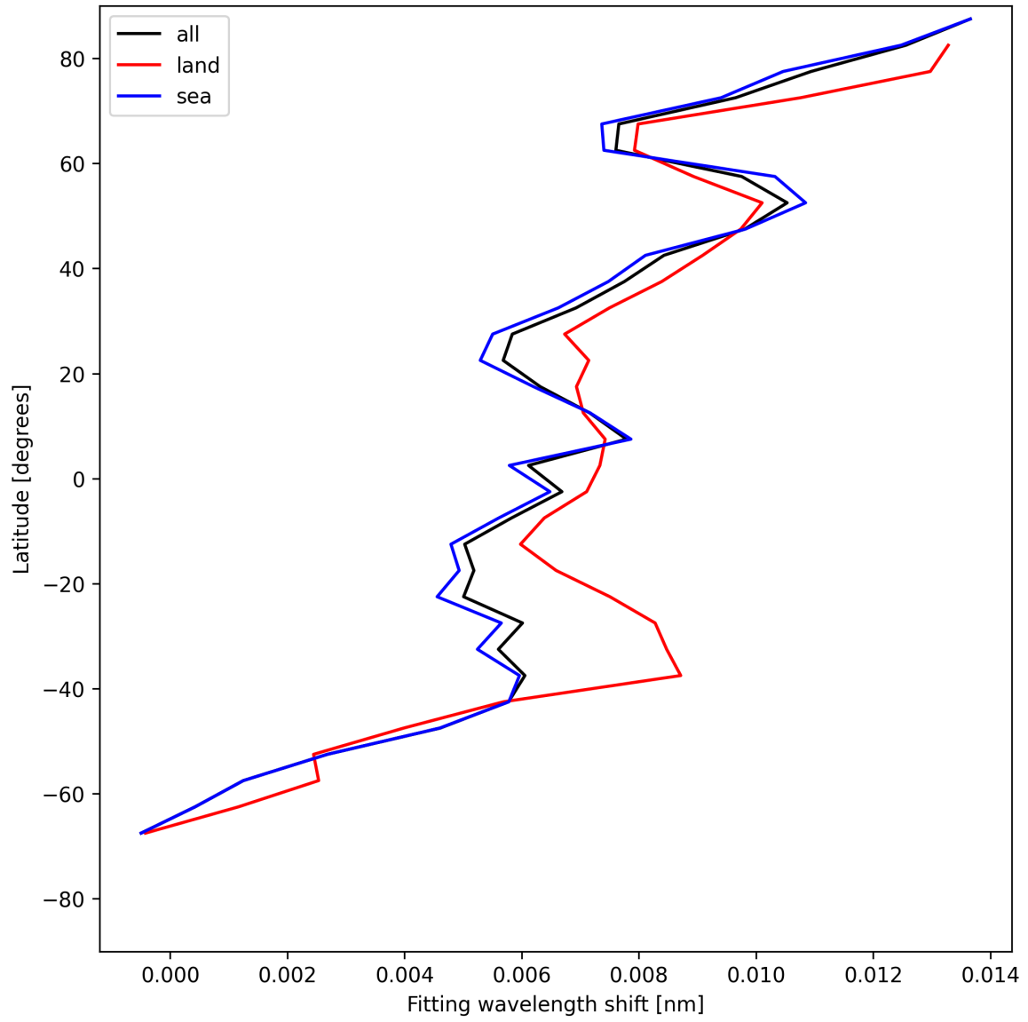
Figure 33: Zonal average of “Fitting wavelength shift” for 2025-06-07 to 2025-06-09.
