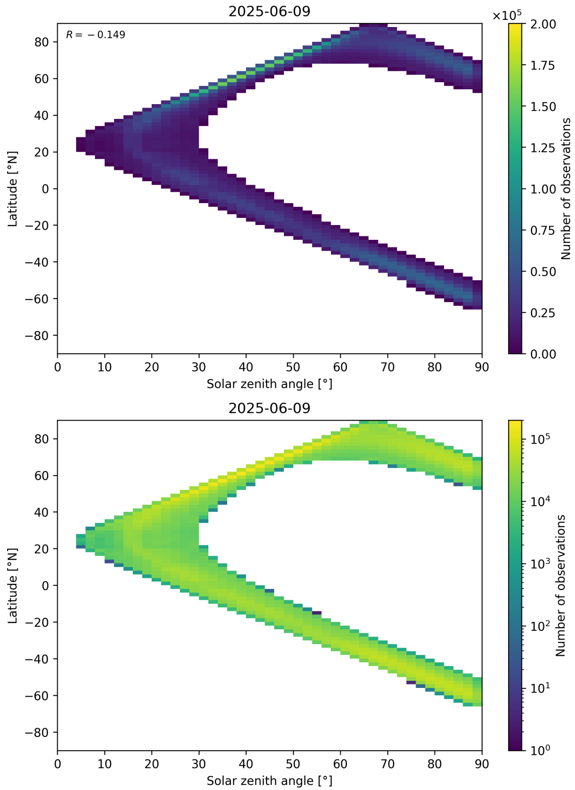
Figure 105: Scatter density plot of “Solar zenith angle” against “Latitude” for 2025-06-08 to 2025-06-10.
