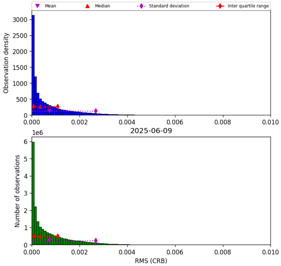
Figure 48: Histogram of “RMS (CRB)” for 2025-06-08 to 2025-06-10
