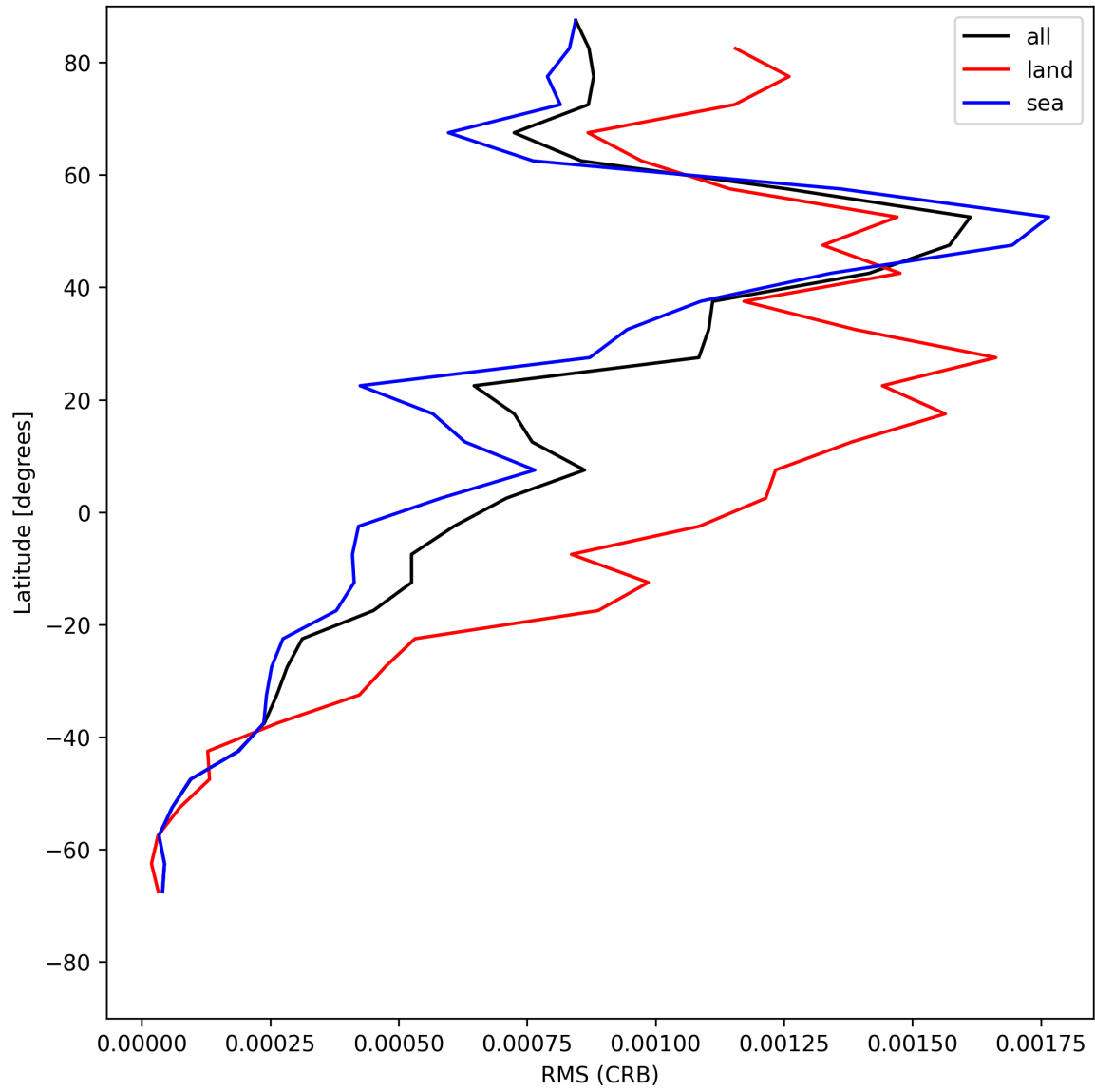
Figure 32: Zonal average of “RMS (CRB)” for 2025-06-08 to 2025-06-10.
