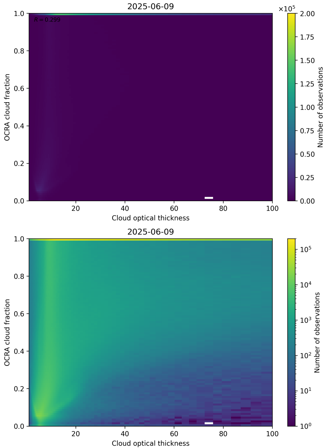
Figure 83: Scatter density plot of “Cloud optical thickness” against “OCRA cloud fraction” for 2025-06-08 to 2025-06-10.
