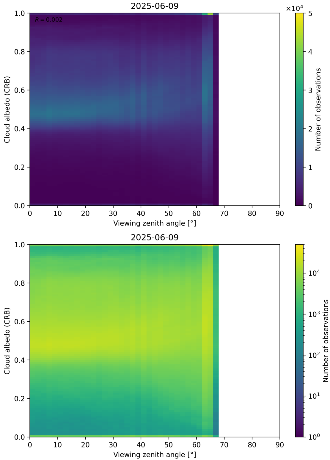
Figure 106: Scatter density plot of “Viewing zenith angle” against “Cloud albedo (CRB)” for 2025-06-08 to 2025-06-10.
