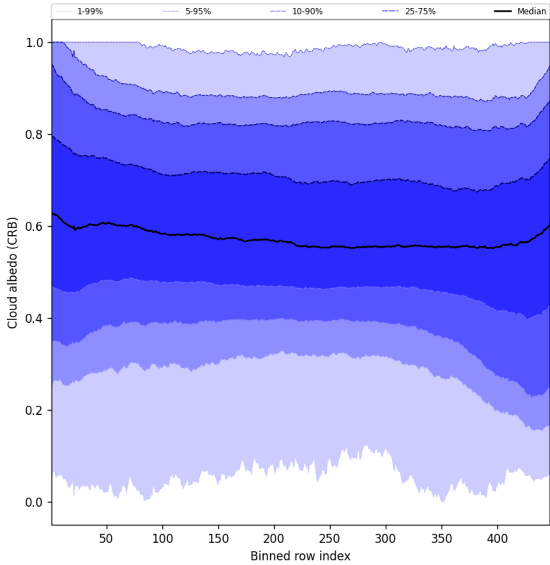
Figure 60: Along track statistics of “Cloud albedo (CRB)” for 2025-06-08 to 2025-06-10
