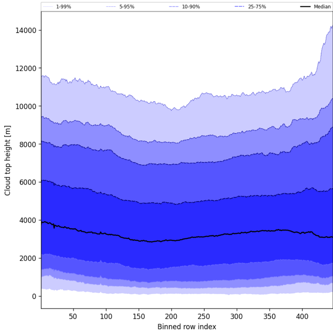
Figure 56: Along track statistics of “Cloud top height” for 2025-06-08 to 2025-06-10
