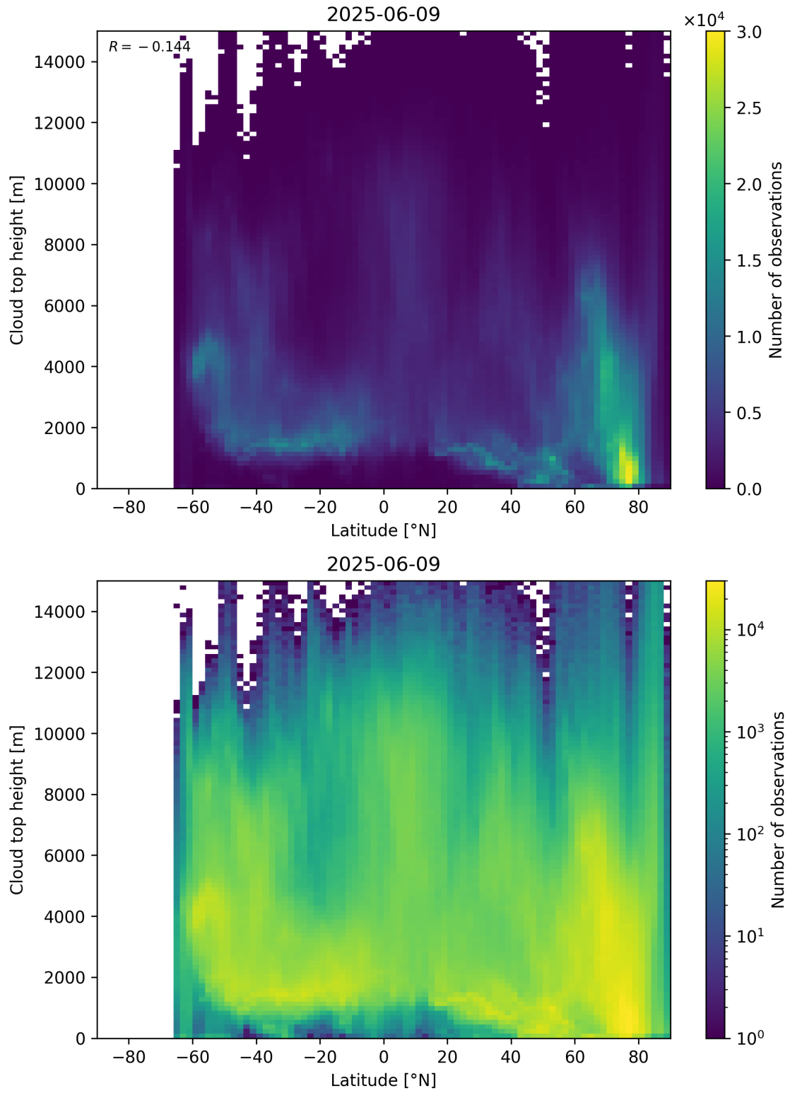
Figure 97: Scatter density plot of “Latitude” against “Cloud top height” for 2025-06-08 to 2025-06-10.
