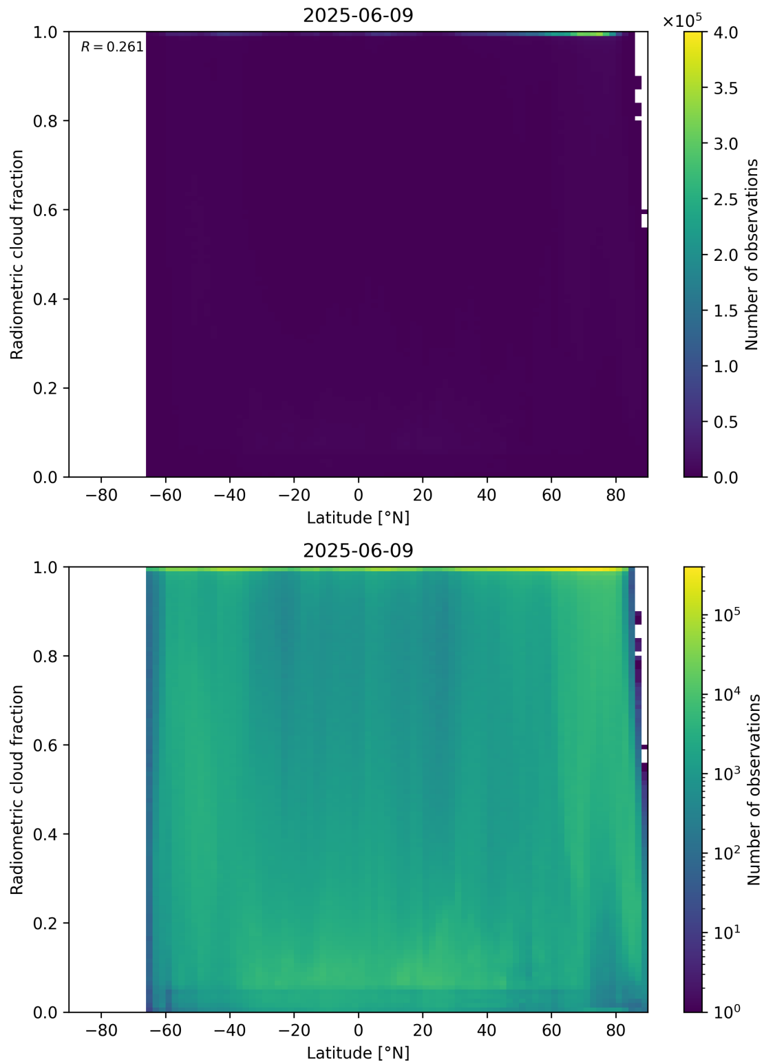
Figure 92: Scatter density plot of “Latitude” against “Radiometric cloud fraction” for 2025-06-08 to 2025-06-10.
