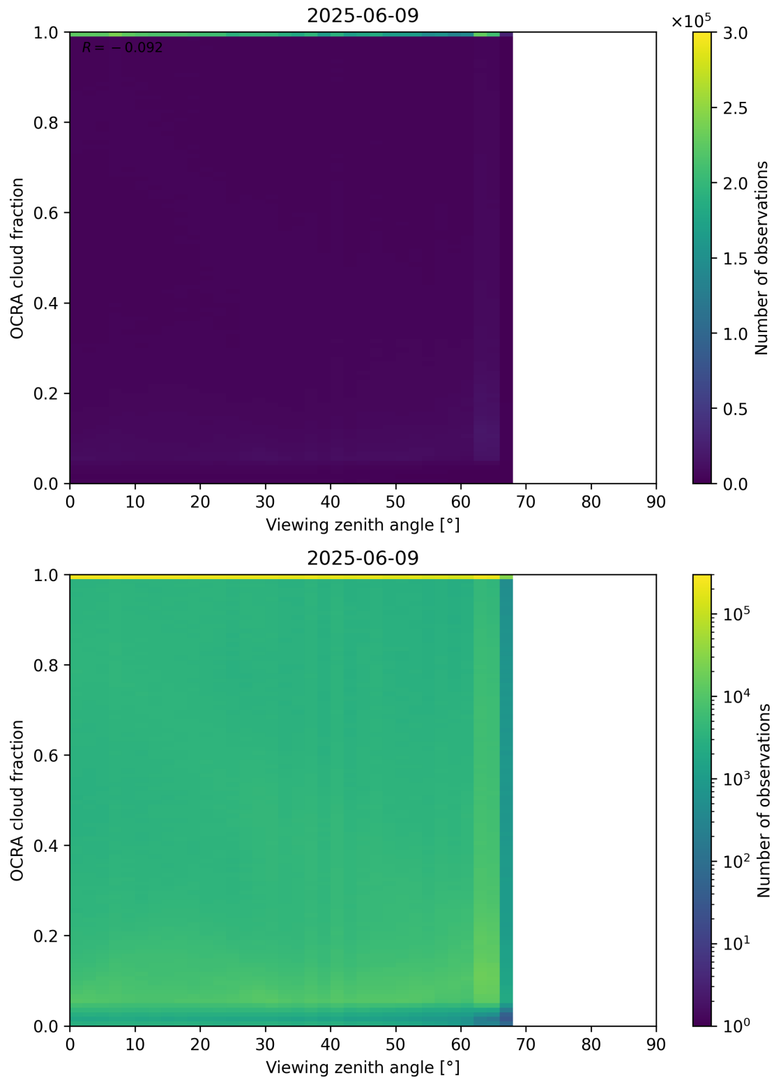
Figure 108: Scatter density plot of “Viewing zenith angle” against “OCRA cloud fraction” for 2025-06-08 to 2025-06-10.
