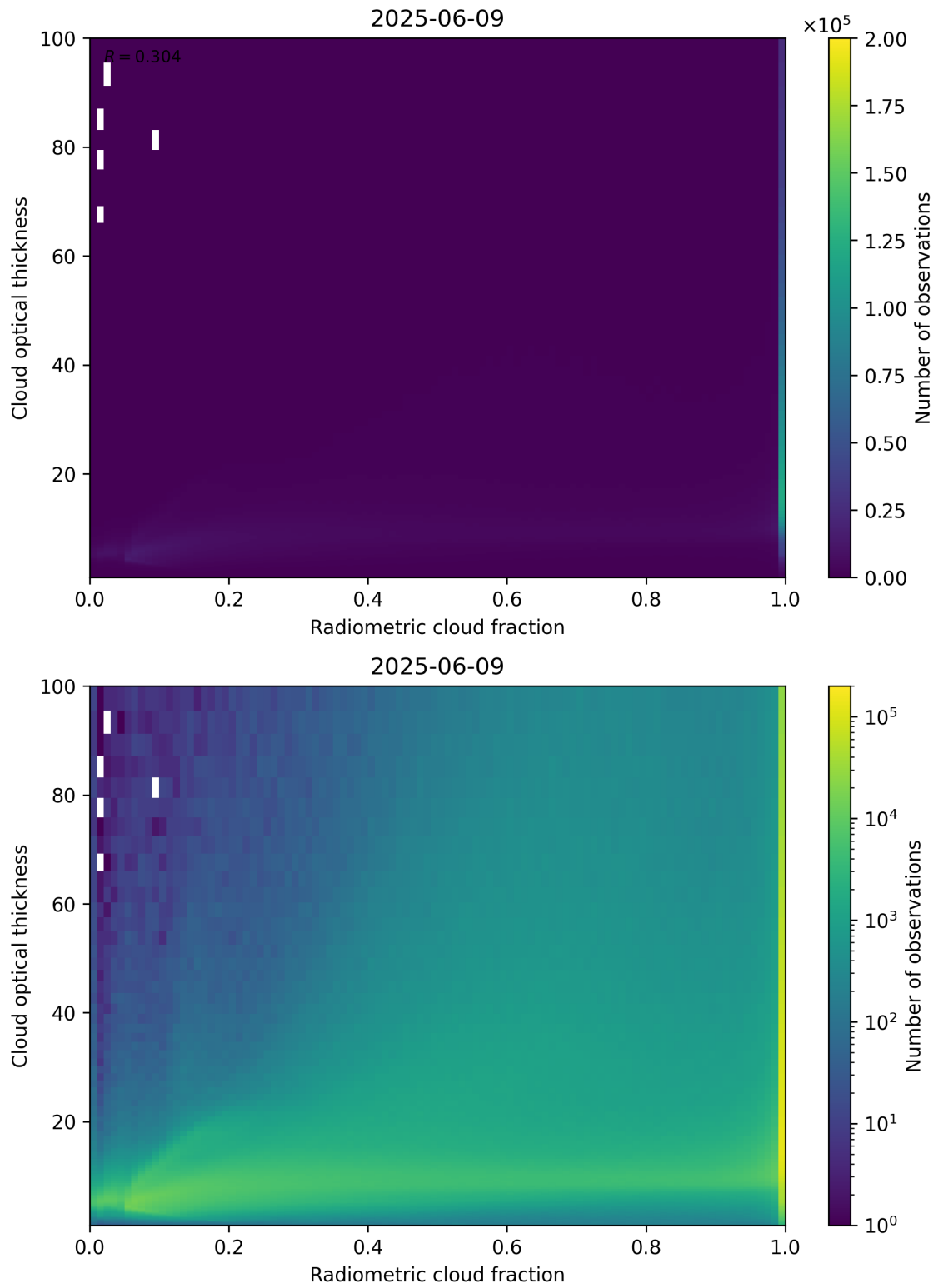
Figure 75: Scatter density plot of “Radiometric cloud fraction” against “Cloud optical thickness” for 2025-06-08 to 2025-06-10.
