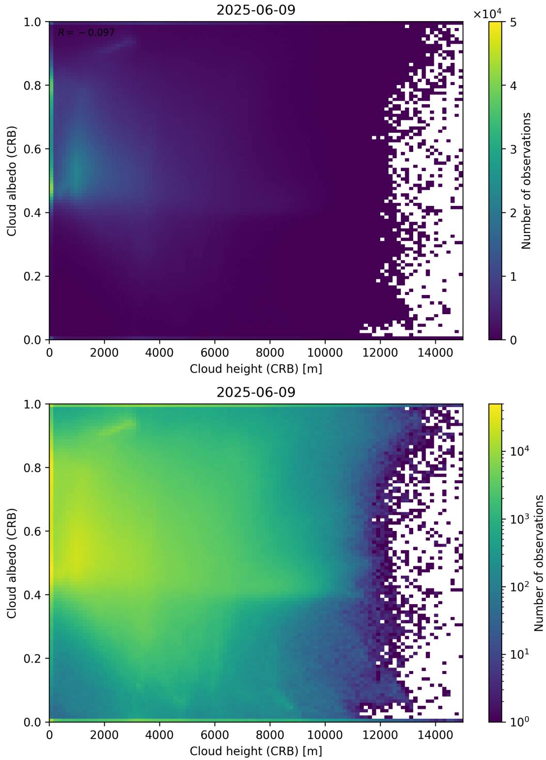
Figure 80: Scatter density plot of “Cloud height (CRB)” against “Cloud albedo (CRB)” for 2025-06-08 to 2025-06-10.
