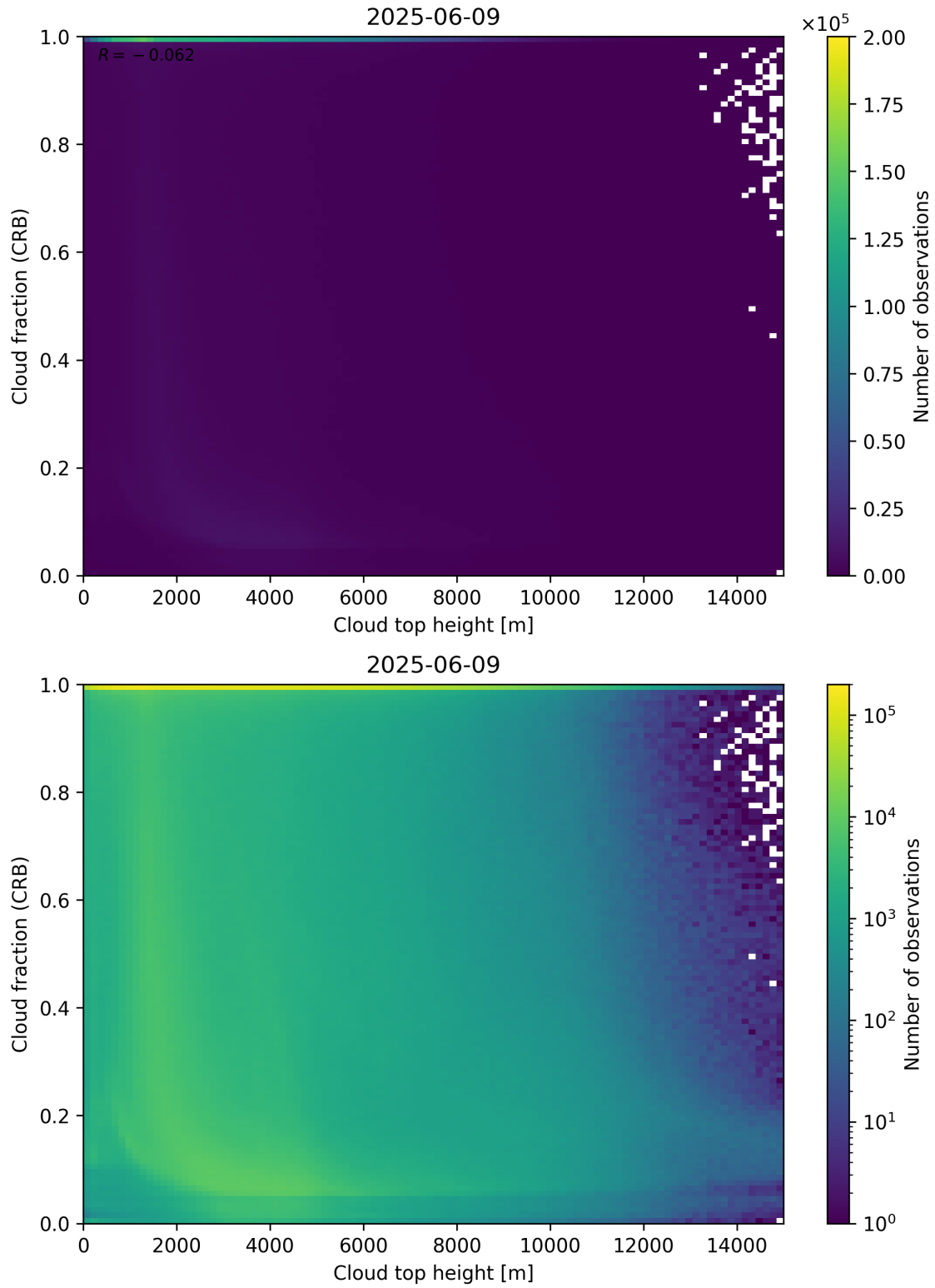
Figure 88: Scatter density plot of “Cloud top height” against “Cloud fraction (CRB)” for 2025-06-08 to 2025-06-10.
