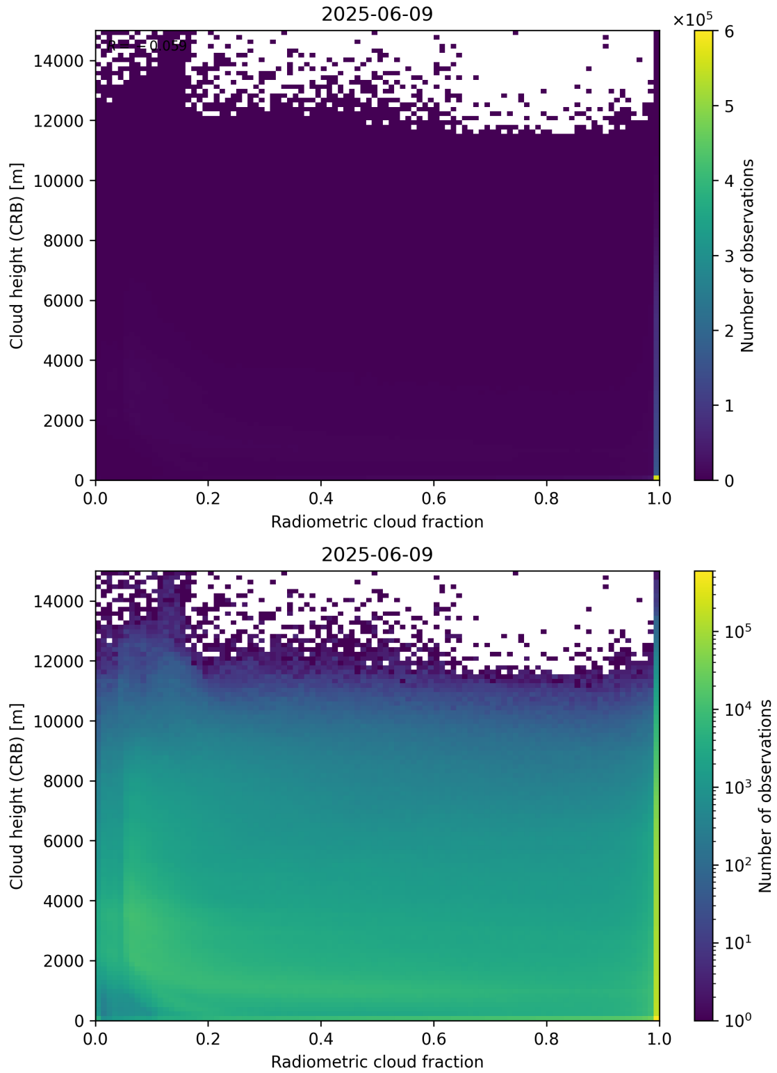
Figure 74: Scatter density plot of “Radiometric cloud fraction” against “Cloud height (CRB)” for 2025-06-08 to 2025-06-10.
