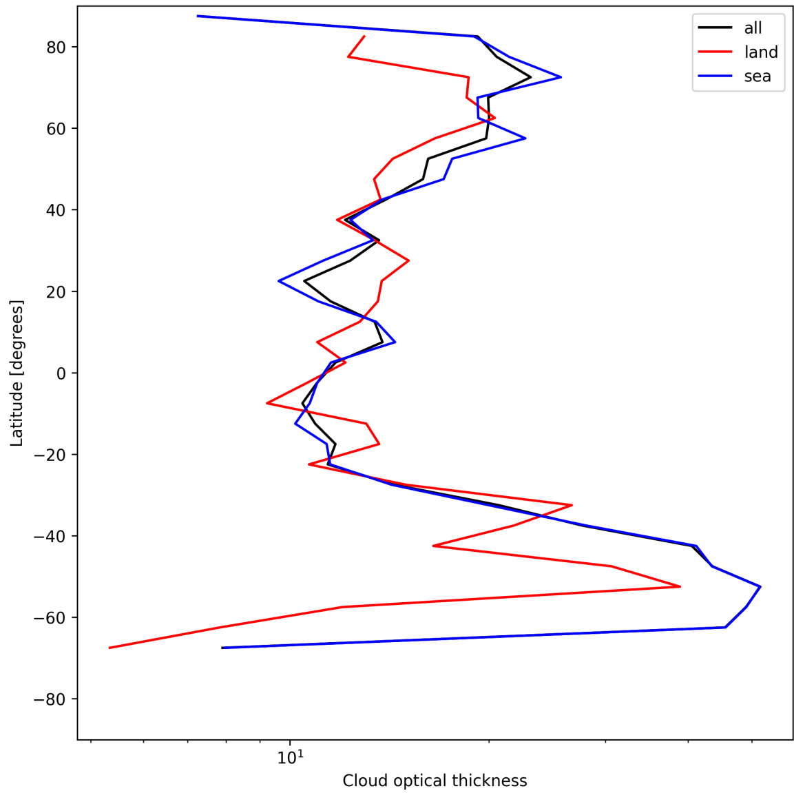
Figure 25: Zonal average of “Cloud optical thickness” for 2025-06-08 to 2025-06-10.
