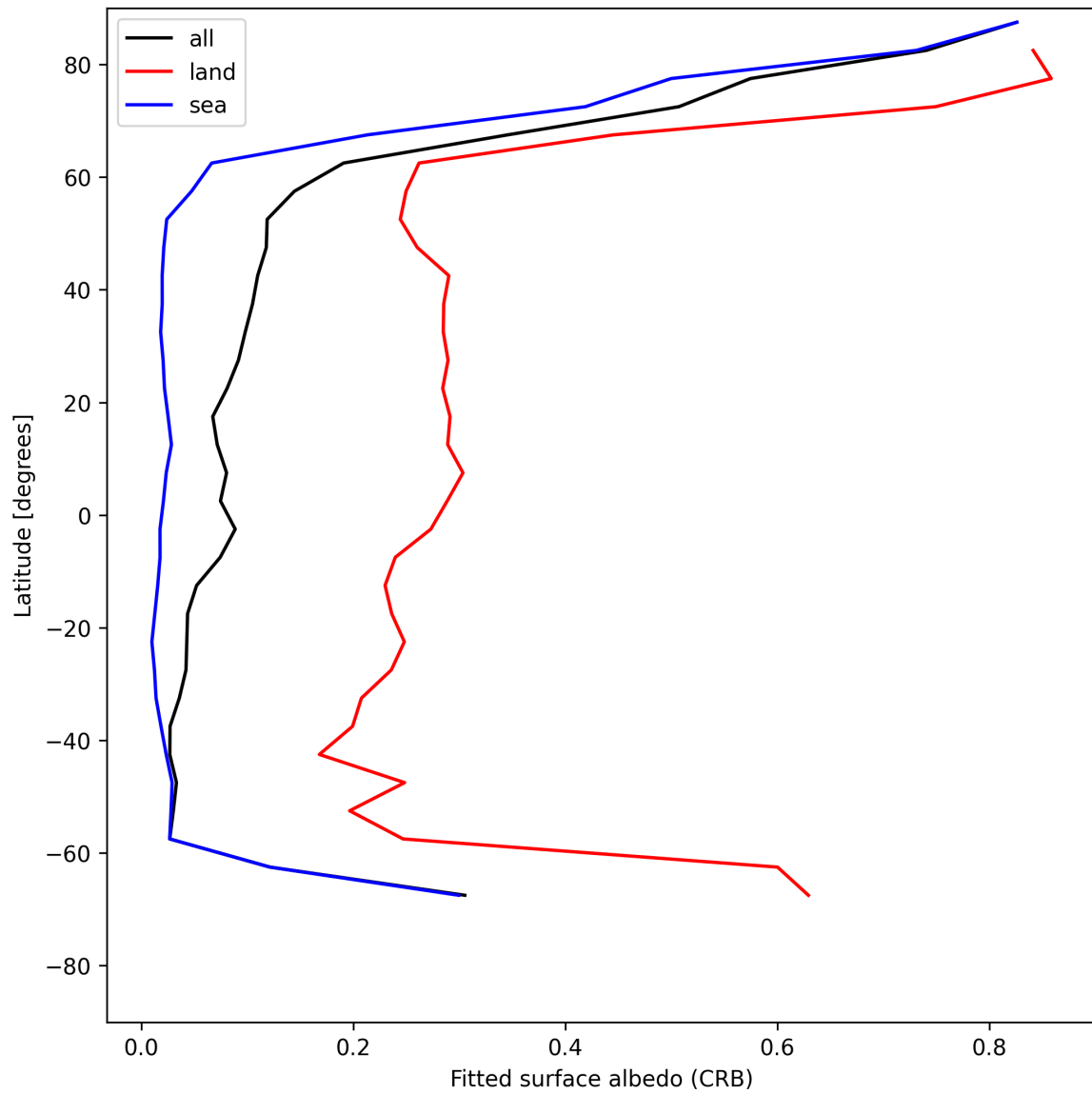
Figure 30: Zonal average of “Fitted surface albedo (CRB)” for 2025-06-08 to 2025-06-10.
