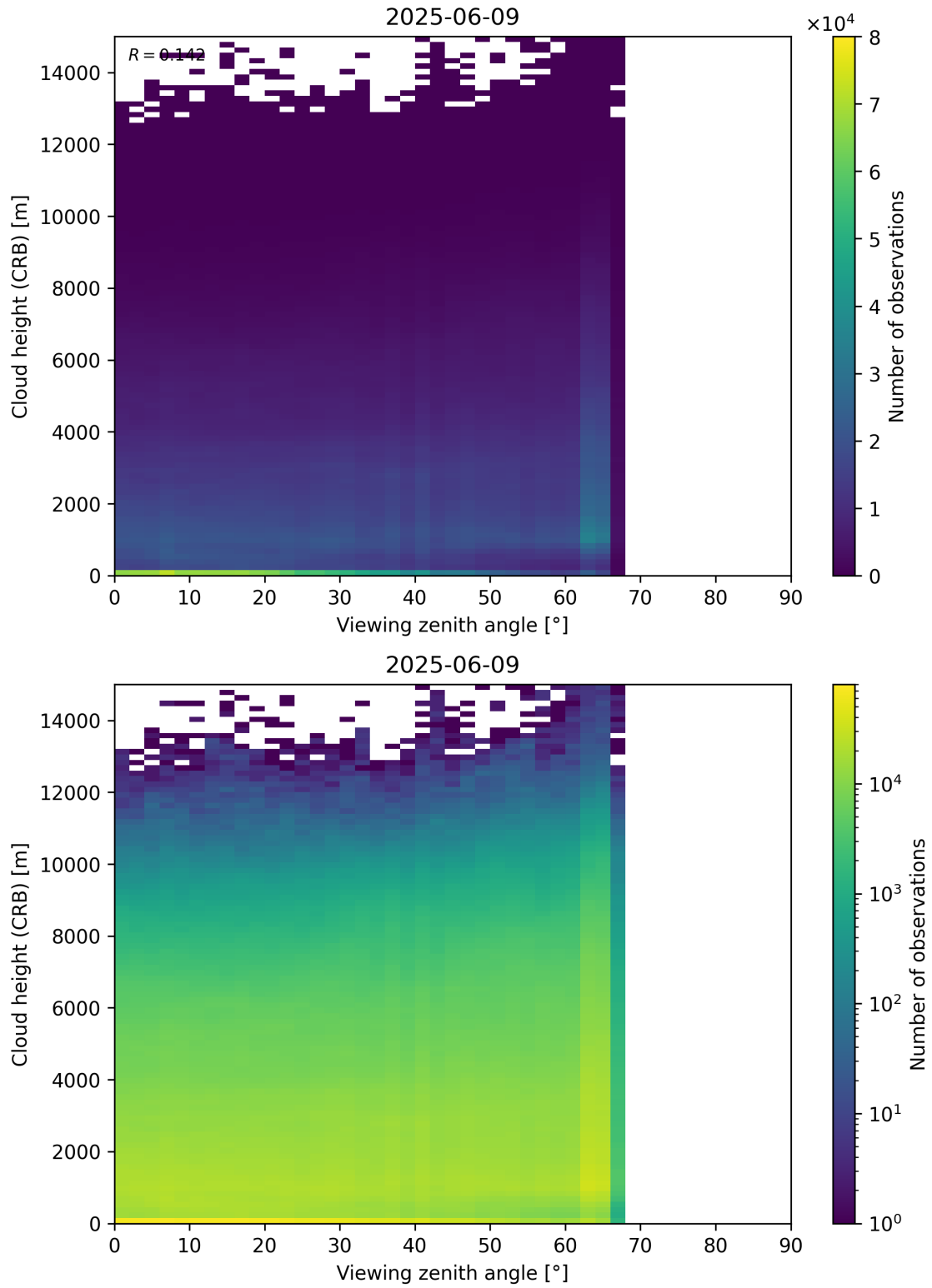
Figure 110: Scatter density plot of “Viewing zenith angle” against “Cloud height (CRB)” for 2025-06-08 to 2025-06-10.
