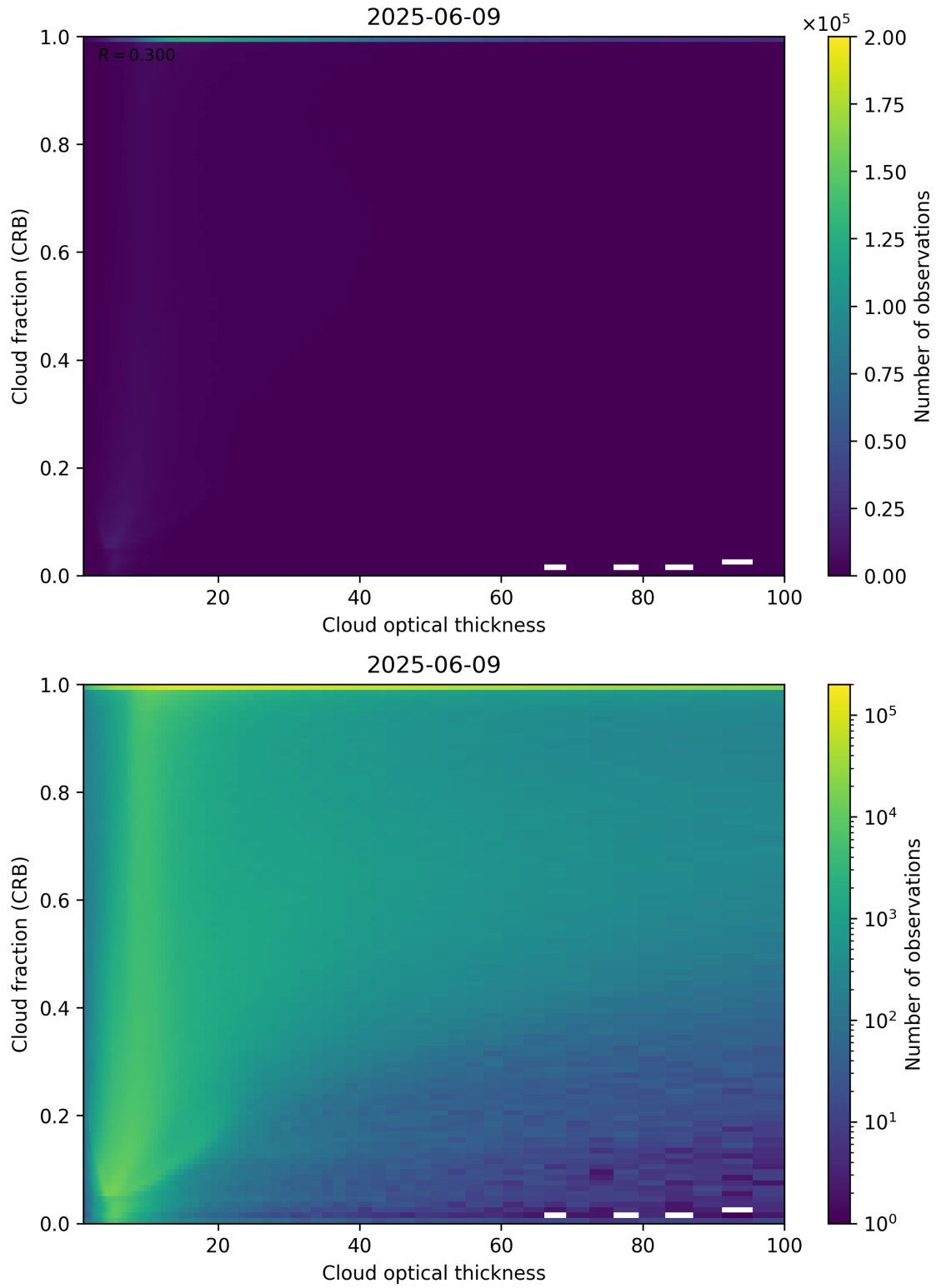
Figure 84: Scatter density plot of “Cloud optical thickness” against “Cloud fraction (CRB)” for 2025-06-08 to 2025-06-10.
