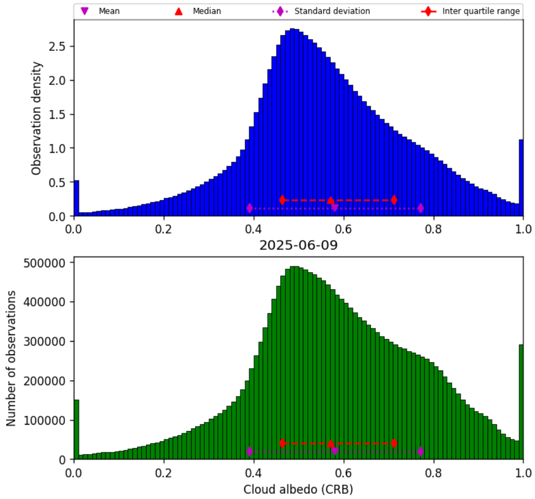
Figure 44: Histogram of “Cloud albedo (CRB)” for 2025-06-08 to 2025-06-10
