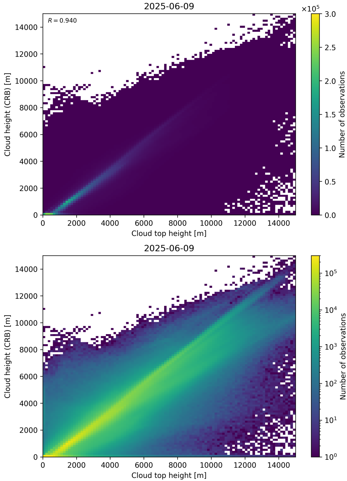
Figure 89: Scatter density plot of “Cloud top height” against “Cloud height (CRB)” for 2025-06-08 to 2025-06-10.
