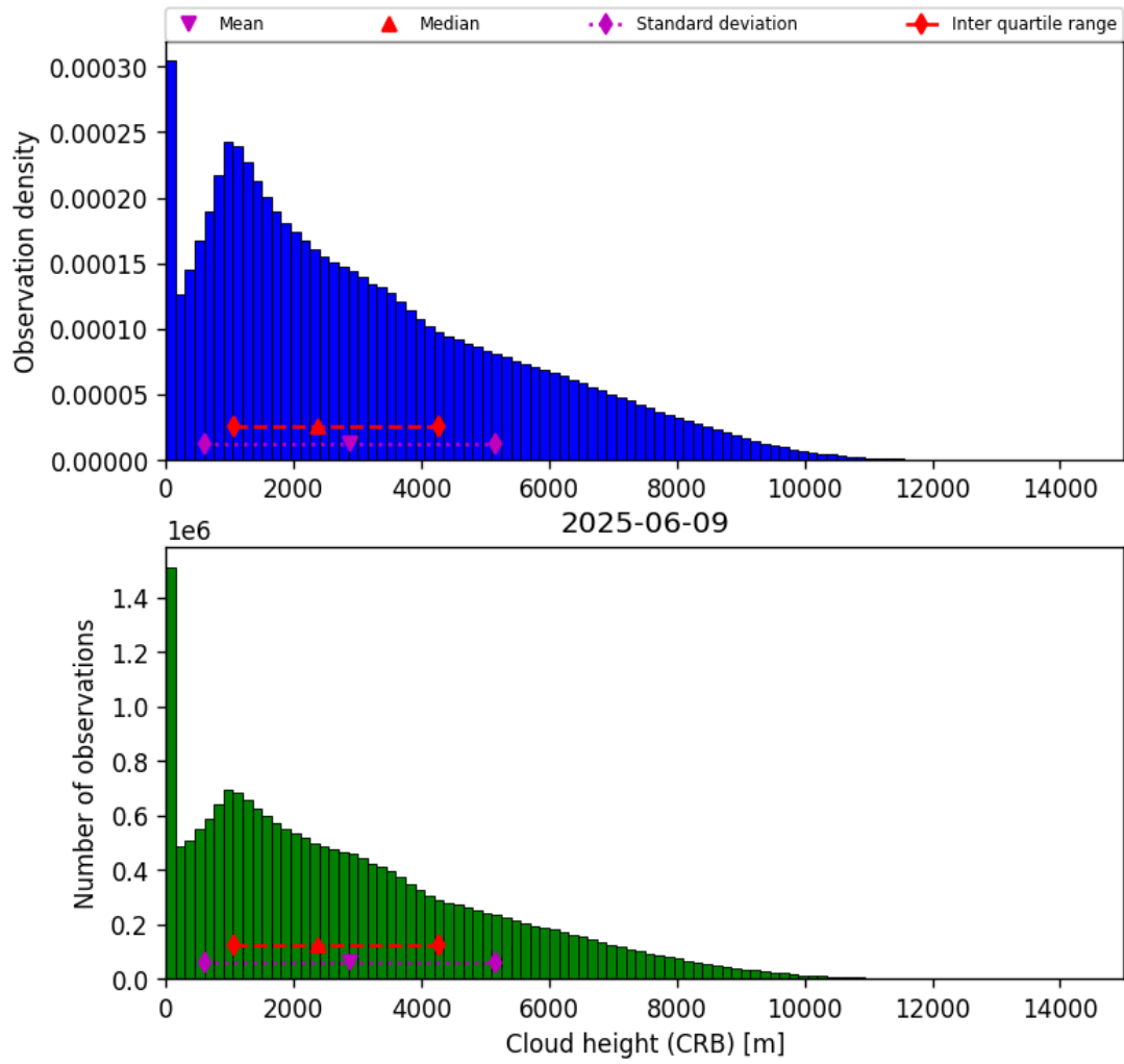
Figure 43: Histogram of “Cloud height (CRB)” for 2025-06-08 to 2025-06-10
