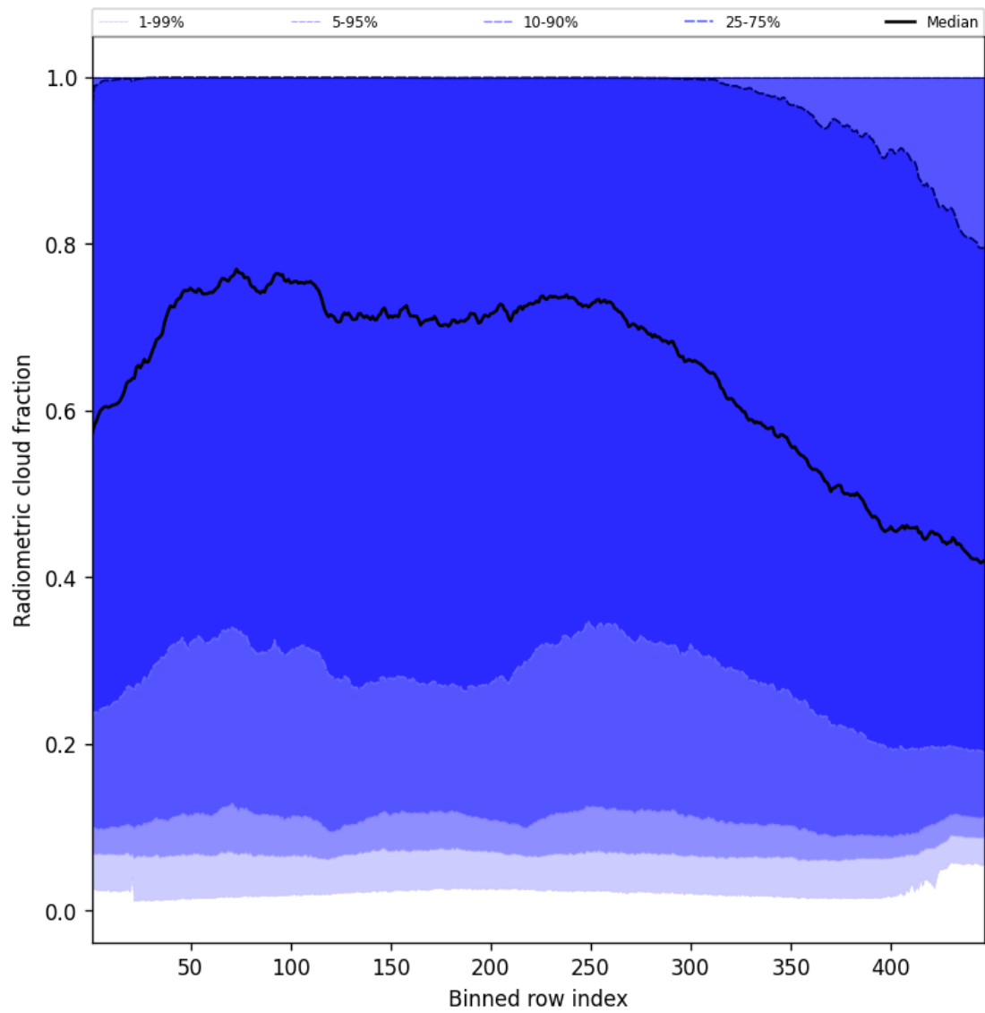
Figure 55: Along track statistics of “Radiometric cloud fraction” for 2025-06-08 to 2025-06-10
