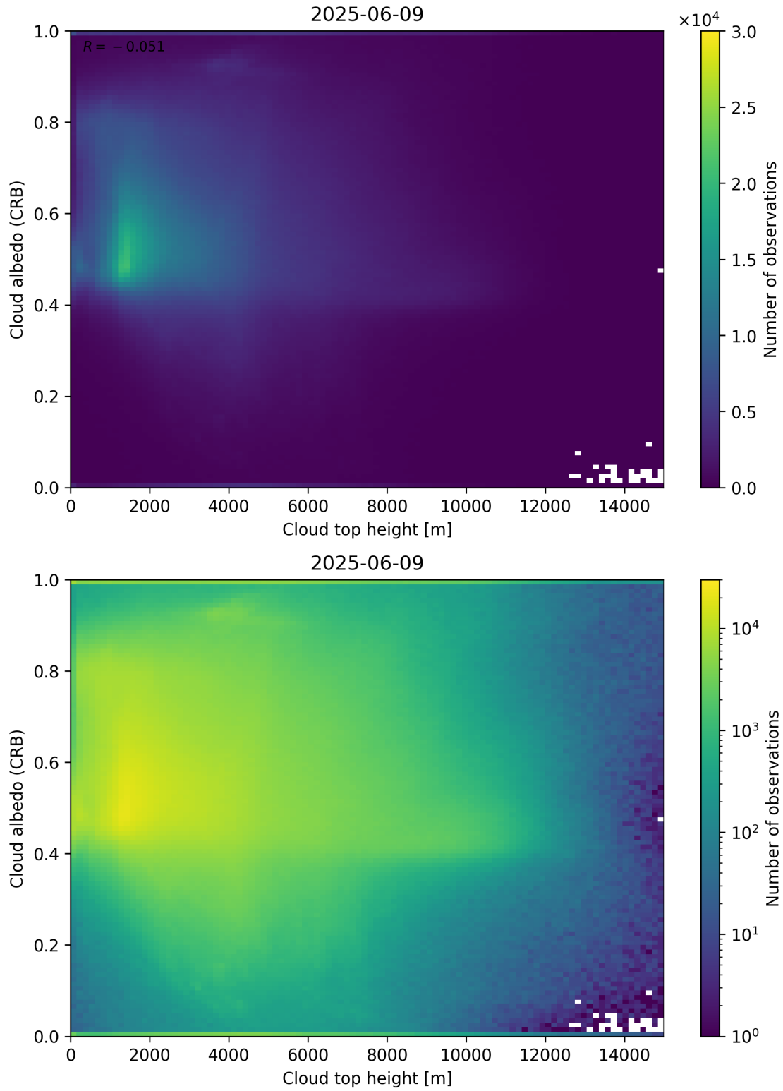
Figure 86: Scatter density plot of “Cloud top height” against “Cloud albedo (CRB)” for 2025-06-08 to 2025-06-10.
