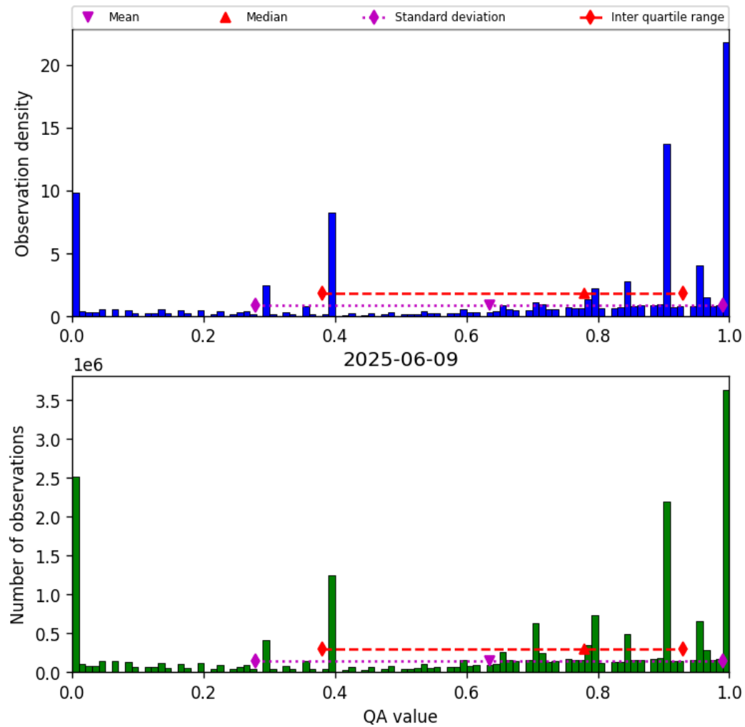
Figure 38: Histogram of “QA value” for 2025-06-08 to 2025-06-10
