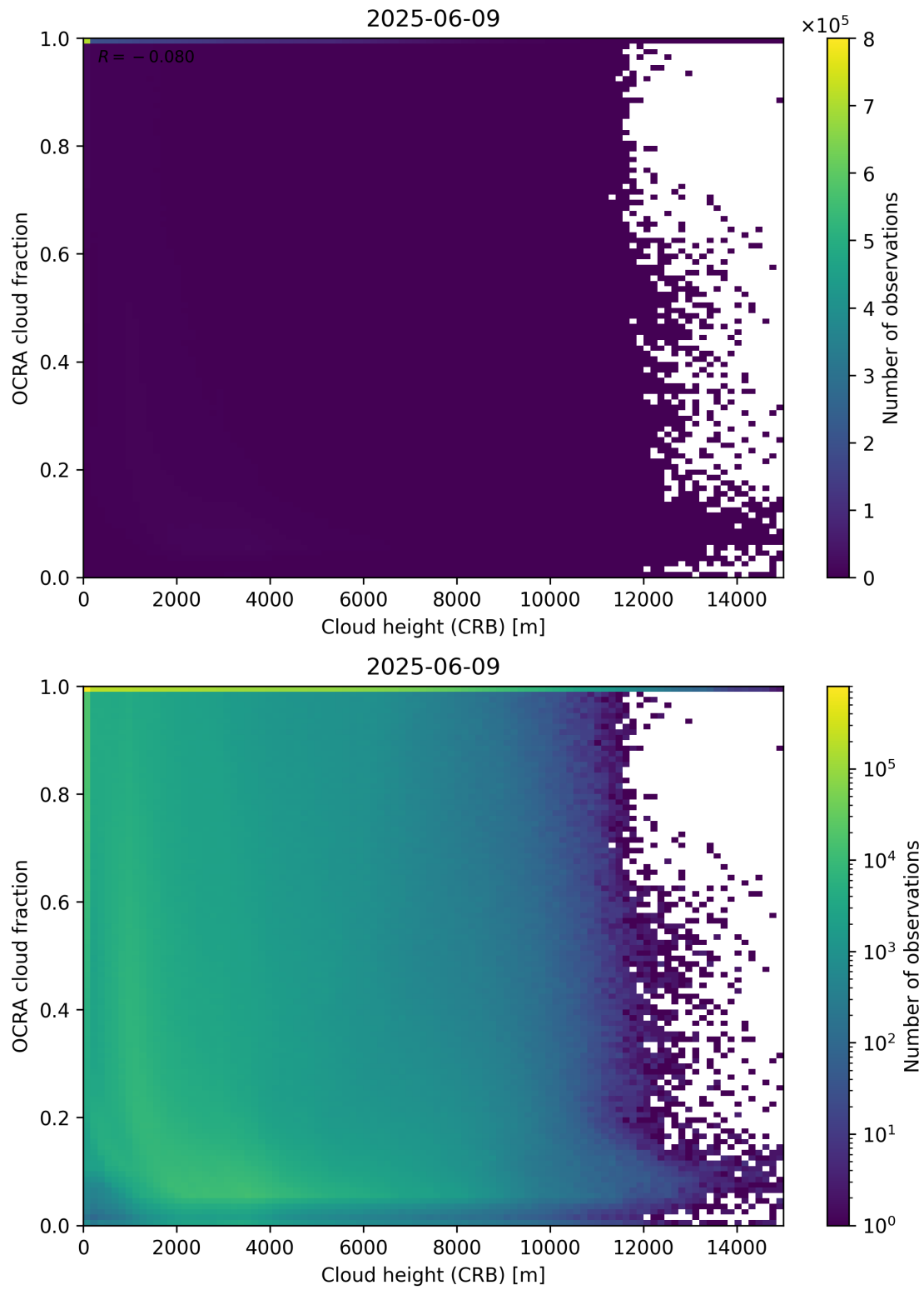
Figure 81: Scatter density plot of “Cloud height (CRB)” against “OCRA cloud fraction” for 2025-06-08 to 2025-06-10.
