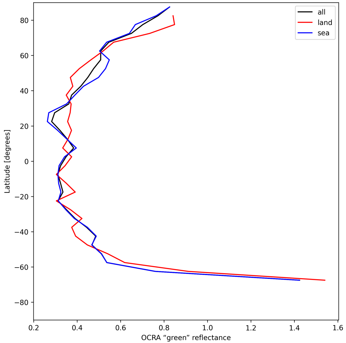
Figure 36: Zonal average of "OCRA "green" reflectance" for 2025-06-08 to 2025-06-10.
