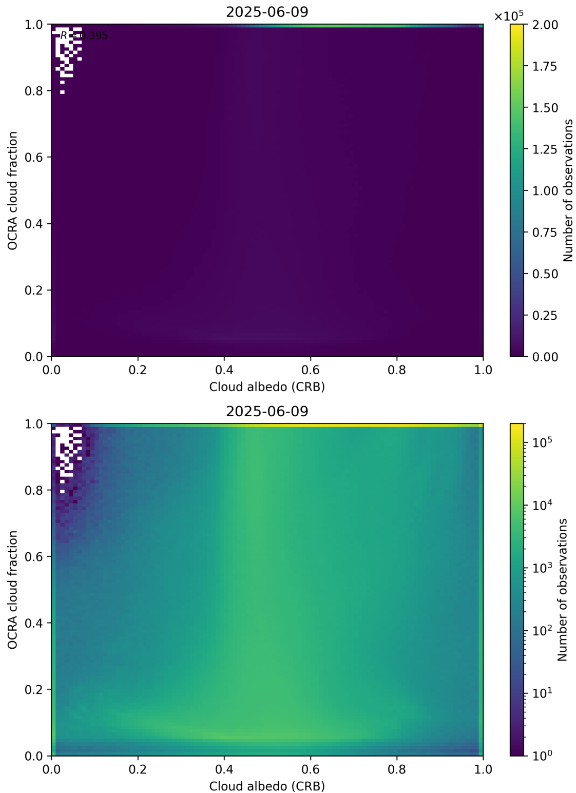
Figure 70: Scatter density plot of “Cloud albedo (CRB)” against “OCRA cloud fraction” for 2025-06-08 to 2025-06-10.
