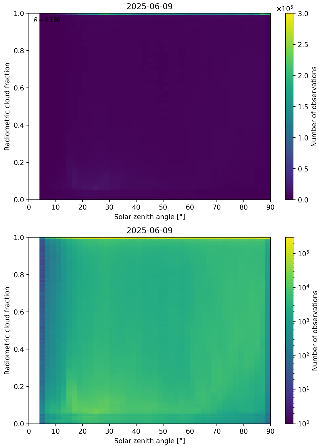
Figure 99: Scatter density plot of “Solar zenith angle” against “Radiometric cloud fraction” for 2025-06-08 to 2025-06-10.
