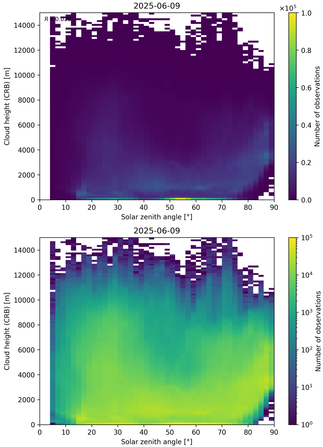
Figure 102: Scatter density plot of “Solar zenith angle” against “Cloud height (CRB)” for 2025-06-08 to 2025-06-10.
