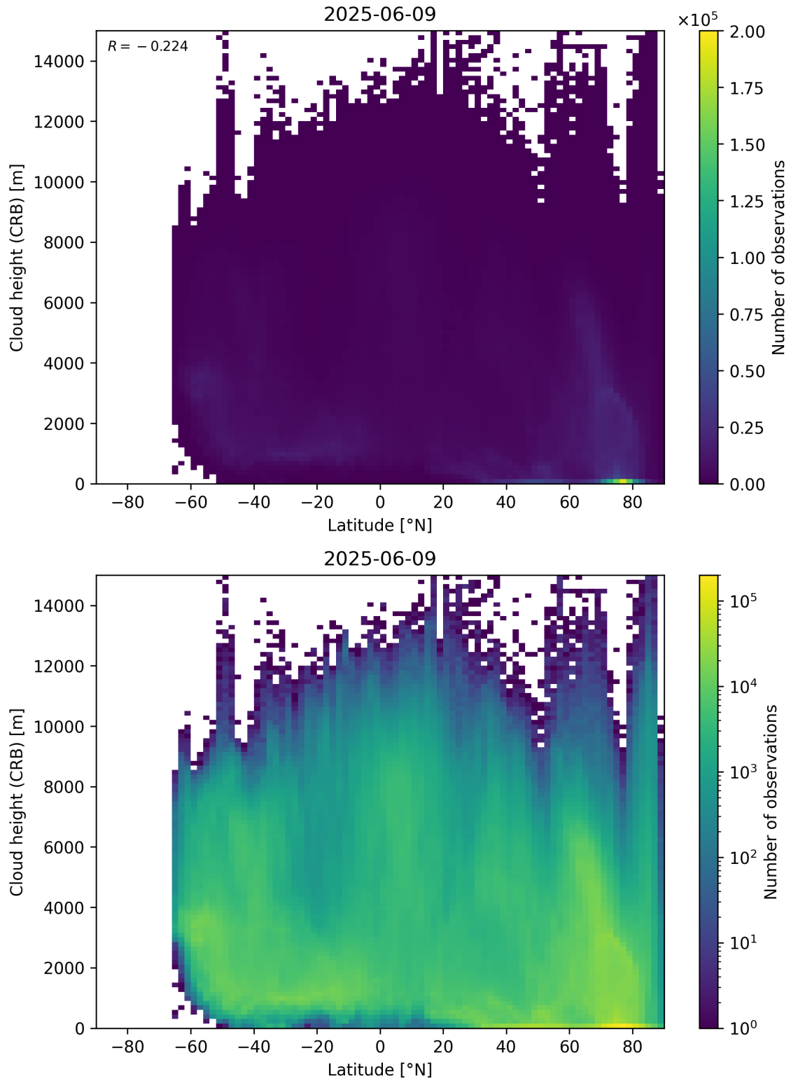
Figure 95: Scatter density plot of “Latitude” against “Cloud height (CRB)” for 2025-06-08 to 2025-06-10.
