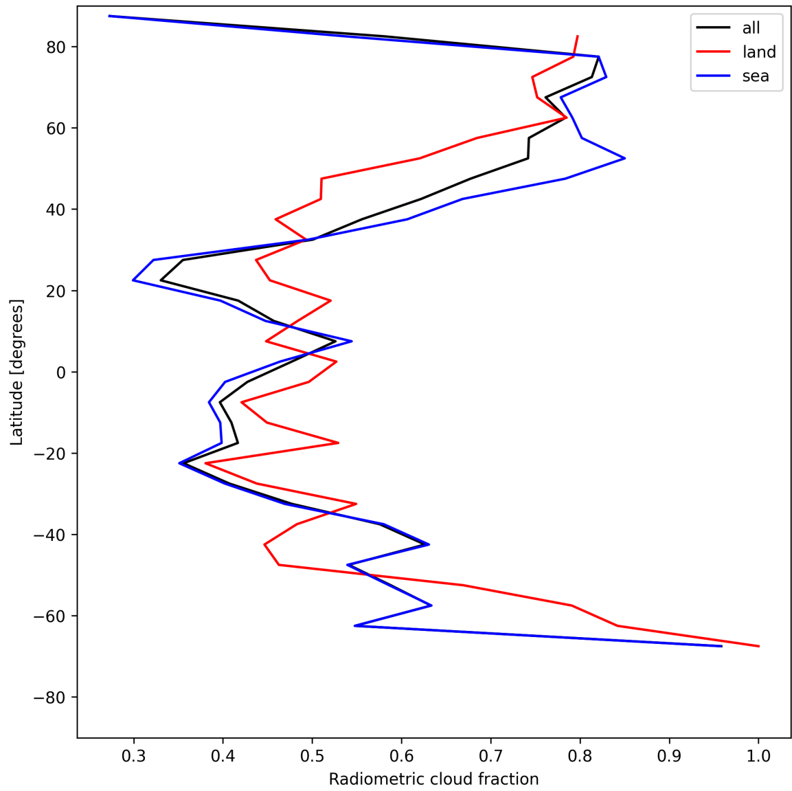
Figure 23: Zonal average of “Radiometric cloud fraction” for 2025-06-08 to 2025-06-10.
