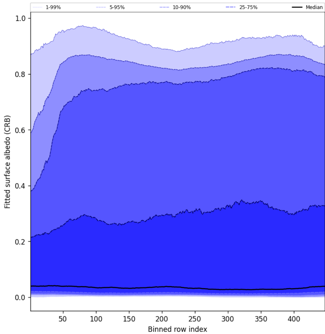
Figure 62: Along track statistics of “Fitted surface albedo (CRB)” for 2025-06-08 to 2025-06-10
