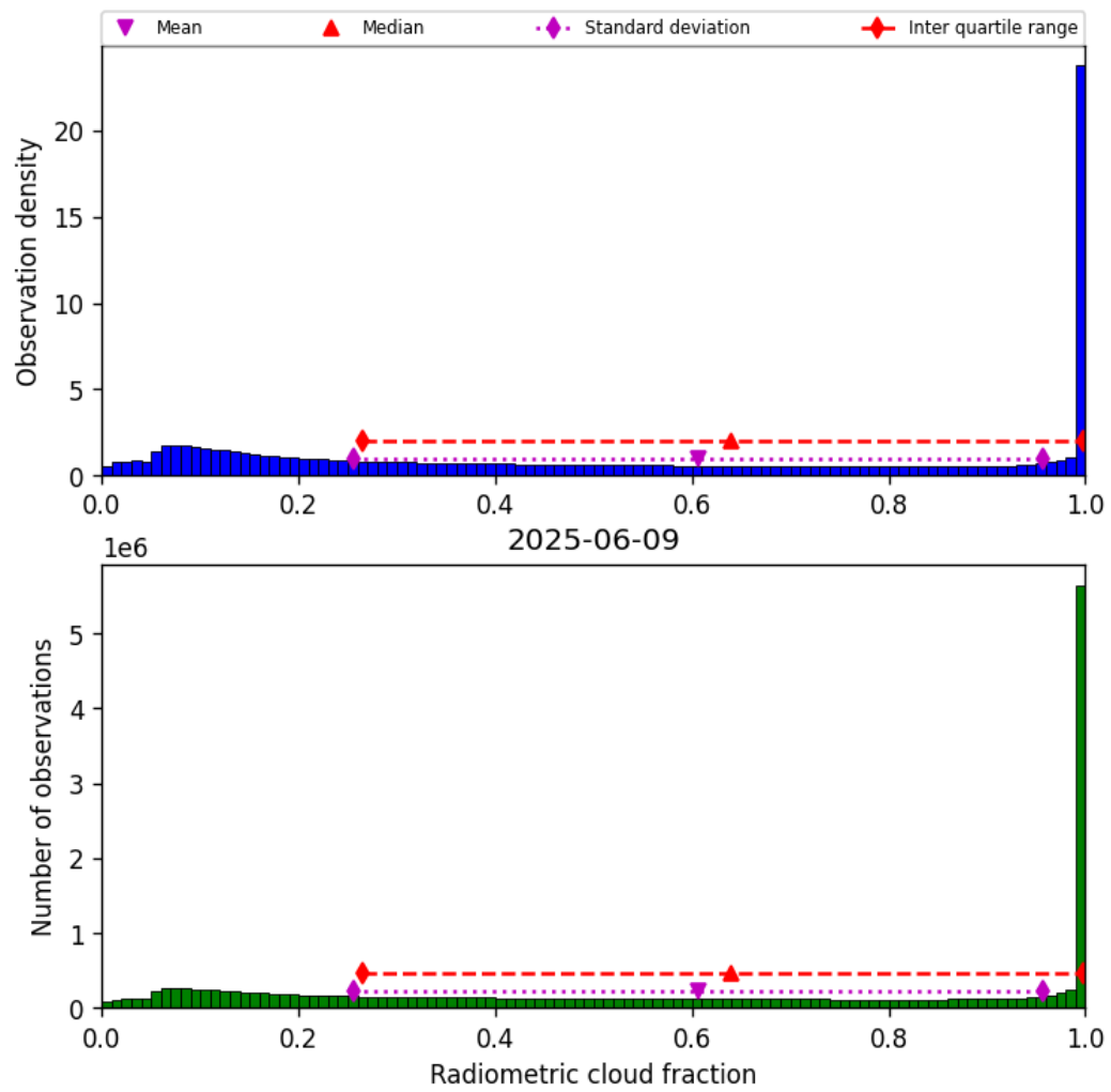
Figure 39: Histogram of “Radiometric cloud fraction” for 2025-06-08 to 2025-06-10
