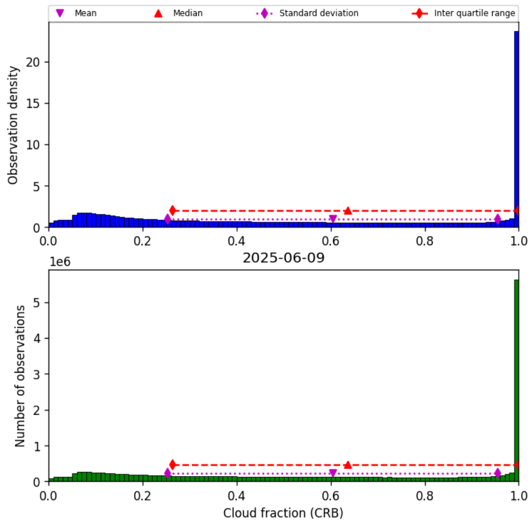
Figure 42: Histogram of “Cloud fraction (CRB)” for 2025-06-08 to 2025-06-10
