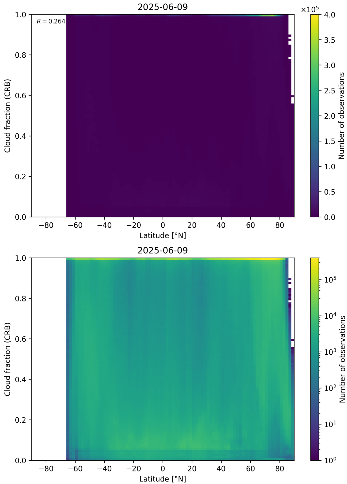
Figure 94: Scatter density plot of “Latitude” against “Cloud fraction (CRB)” for 2025-06-08 to 2025-06-10.
