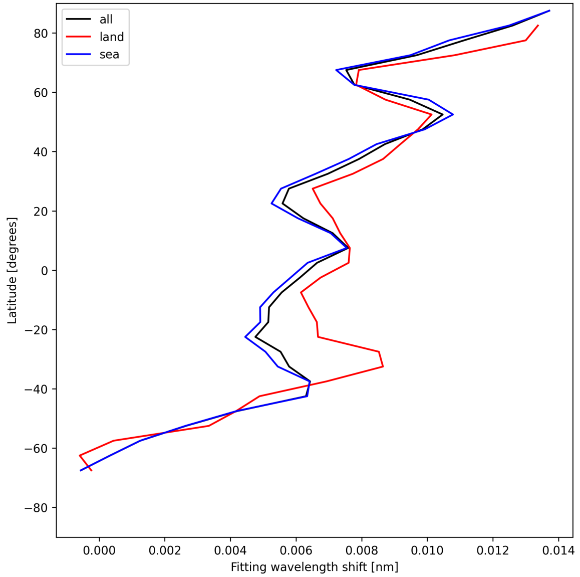
Figure 33: Zonal average of “Fitting wavelength shift” for 2025-06-08 to 2025-06-10.
