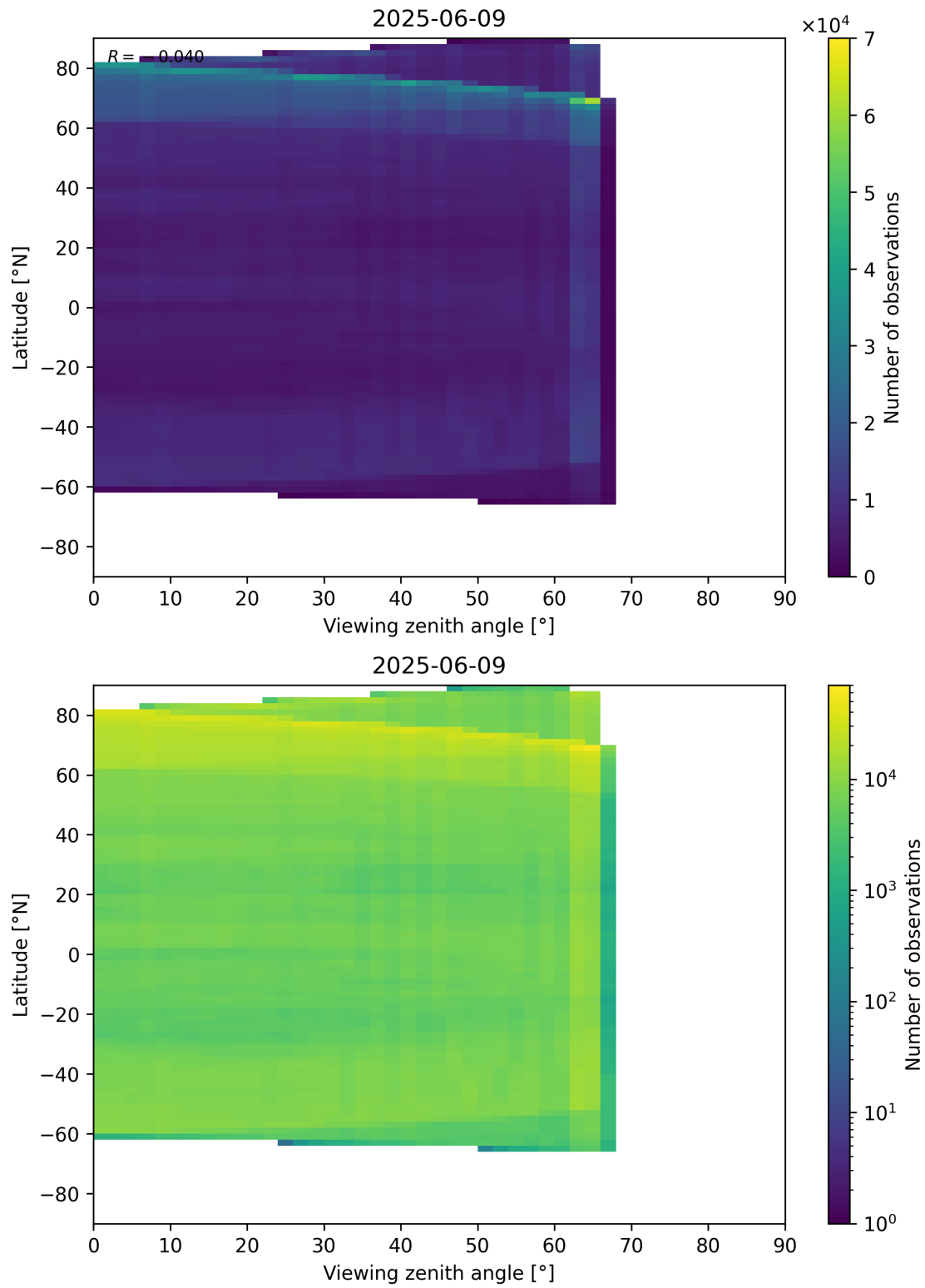
Figure 113: Scatter density plot of “Viewing zenith angle” against “Latitude” for 2025-06-08 to 2025-06-10.
