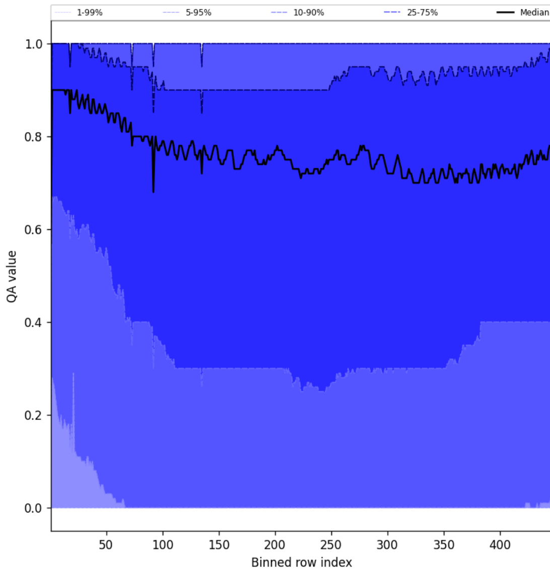
Figure 54: Along track statistics of “QA value” for 2025-06-08 to 2025-06-10
