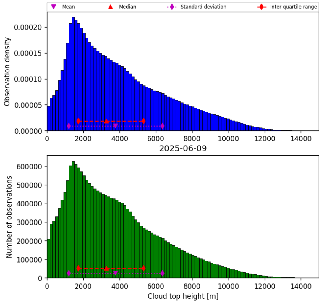
Figure 40: Histogram of “Cloud top height” for 2025-06-08 to 2025-06-10
