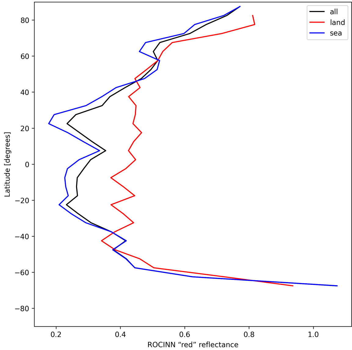
Figure 37: Zonal average of "ROCINN "red" reflectance" for 2025-06-08 to 2025-06-10.
