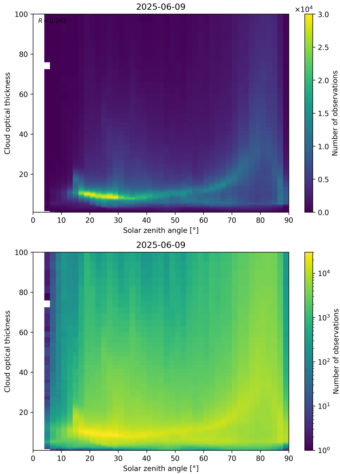
Figure 103: Scatter density plot of “Solar zenith angle” against “Cloud optical thickness” for 2025-06-08 to 2025-06-10.
