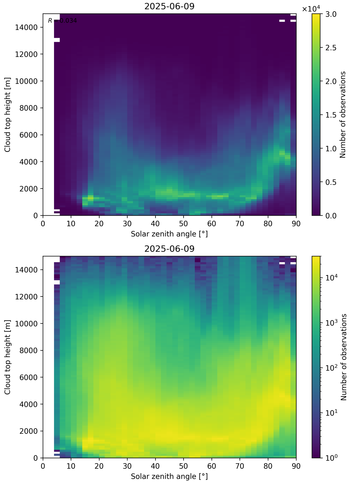
Figure 104: Scatter density plot of “Solar zenith angle” against “Cloud top height” for 2025-06-08 to 2025-06-10.
