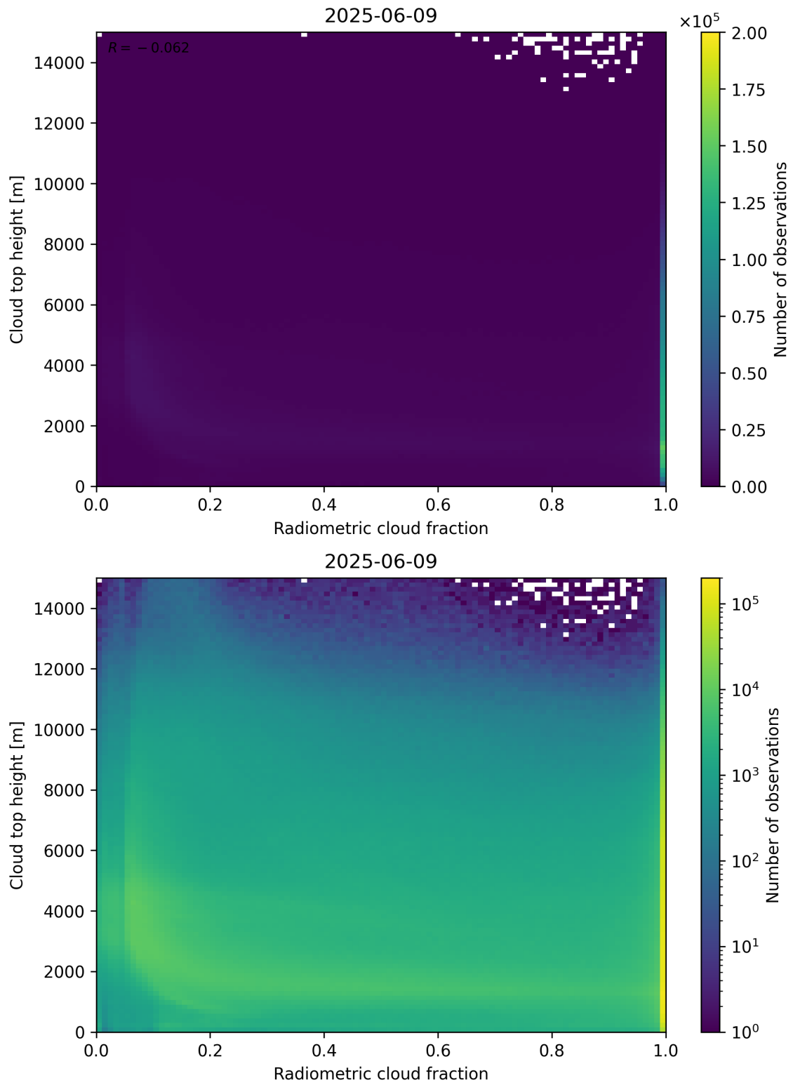
Figure 76: Scatter density plot of “Radiometric cloud fraction” against “Cloud top height” for 2025-06-08 to 2025-06-10.
