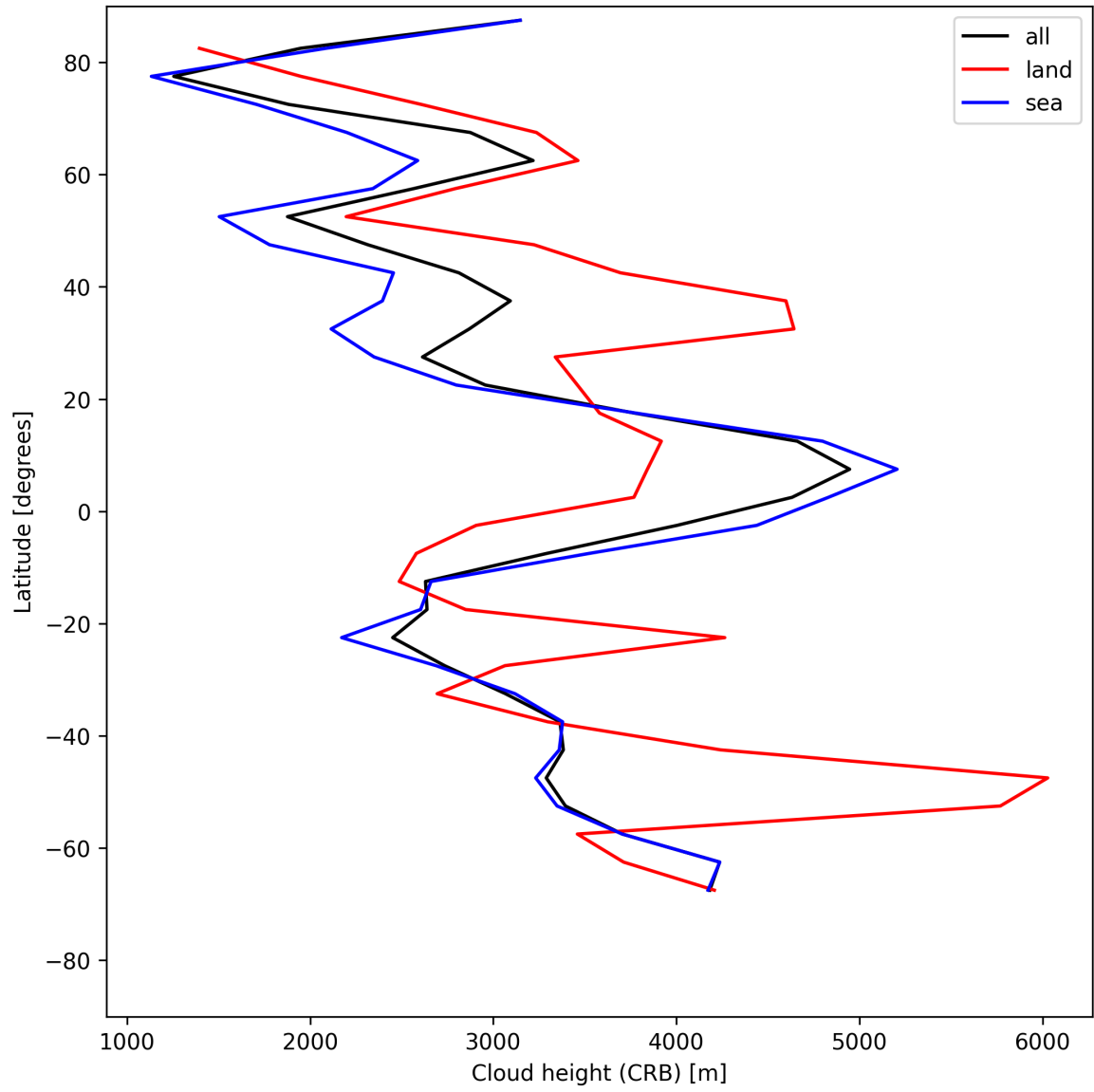
Figure 27: Zonal average of “Cloud height (CRB)” for 2025-06-08 to 2025-06-10.
