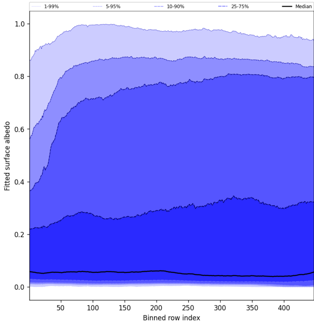
Figure 61: Along track statistics of “Fitted surface albedo” for 2025-06-08 to 2025-06-10
