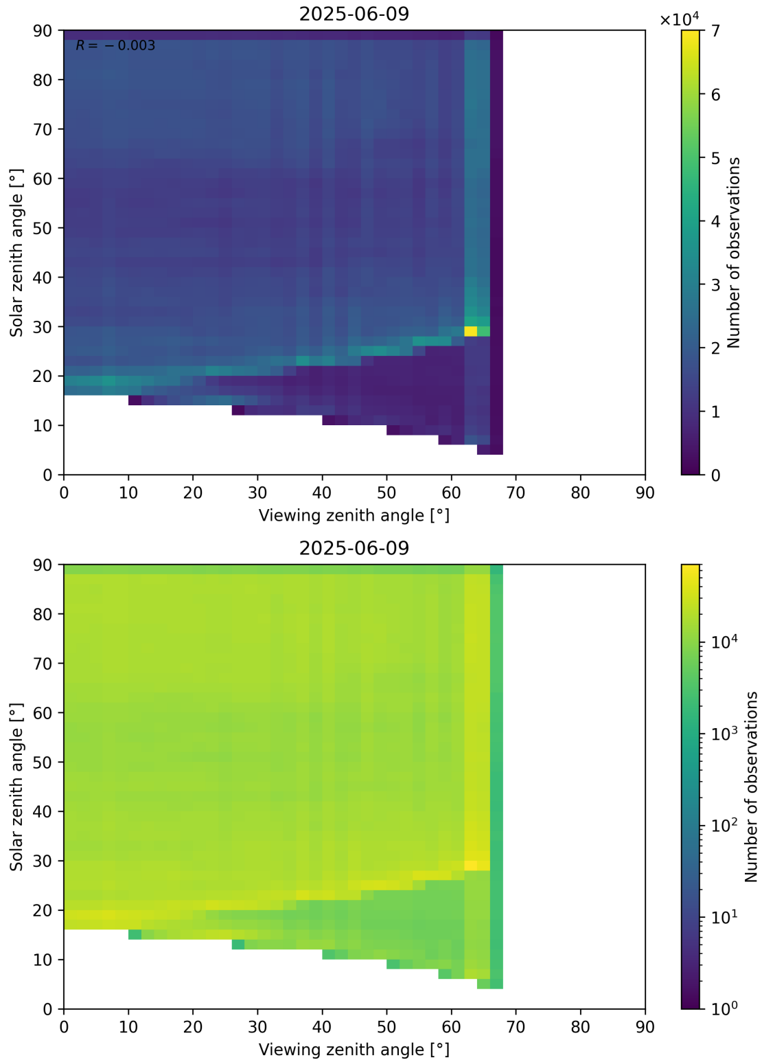
Figure 114: Scatter density plot of “Viewing zenith angle” against “Solar zenith angle” for 2025-06-08 to 2025-06-10.
