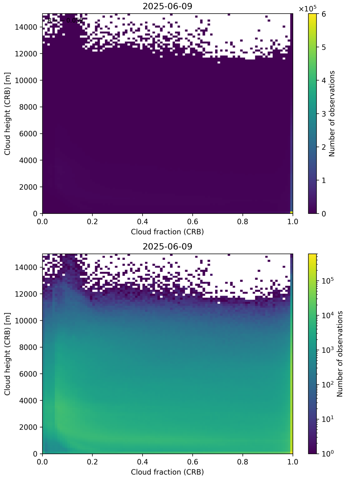
Figure 79: Scatter density plot of “Cloud fraction (CRB)” against “Cloud height (CRB)” for 2025-06-08 to 2025-06-10.
