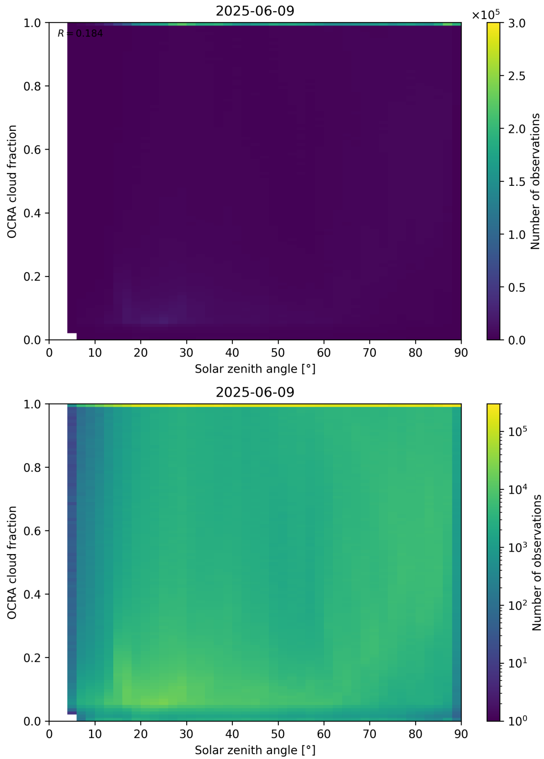
Figure 100: Scatter density plot of “Solar zenith angle” against “OCRA cloud fraction” for 2025-06-08 to 2025-06-10.
