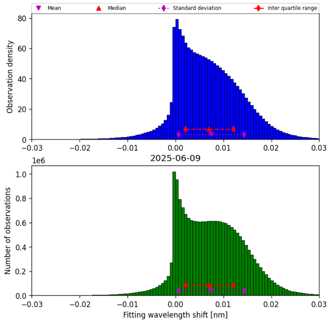
Figure 49: Histogram of “Fitting wavelength shift” for 2025-06-08 to 2025-06-10
