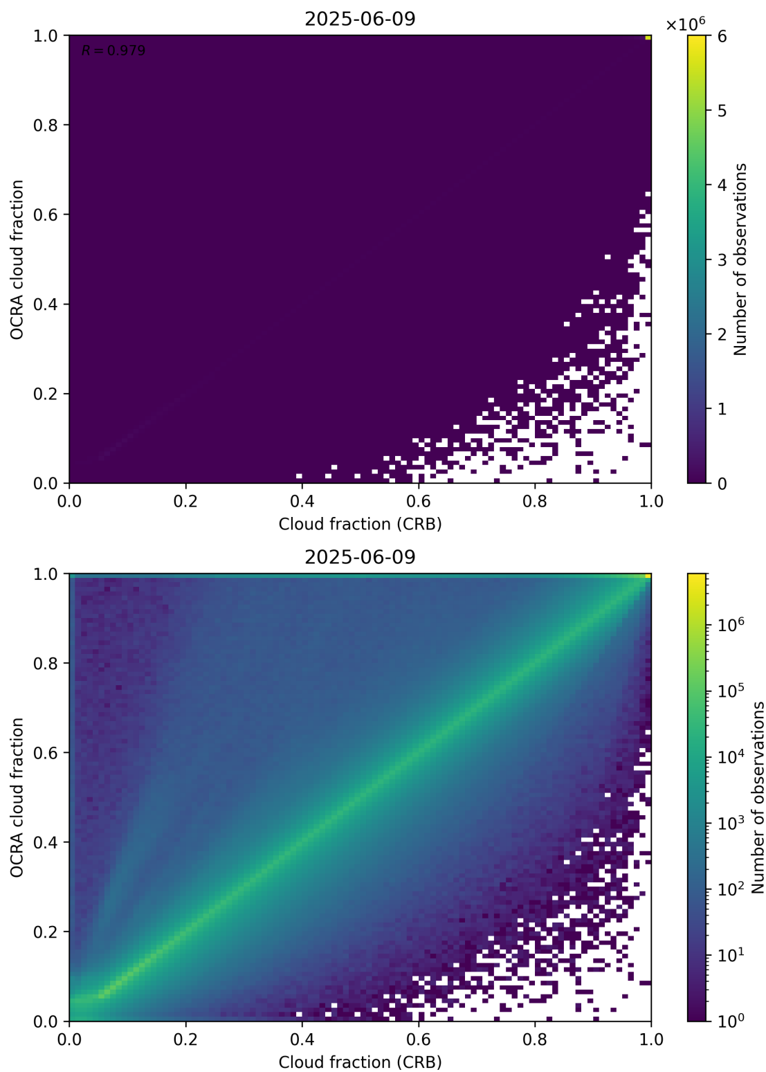
Figure 78: Scatter density plot of “Cloud fraction (CRB)” against “OCRA cloud fraction” for 2025-06-08 to 2025-06-10.
