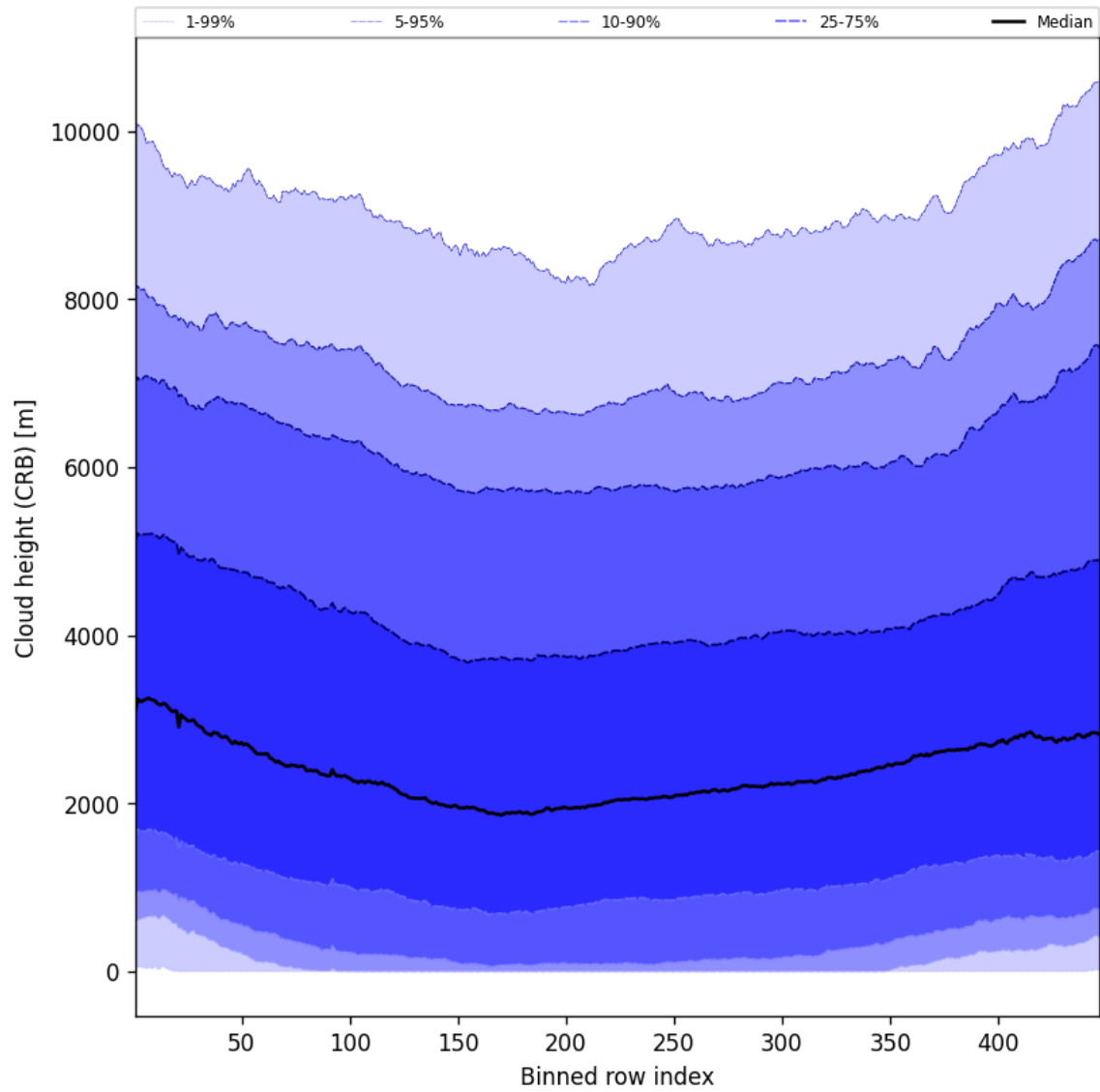
Figure 59: Along track statistics of “Cloud height (CRB)” for 2025-06-08 to 2025-06-10
