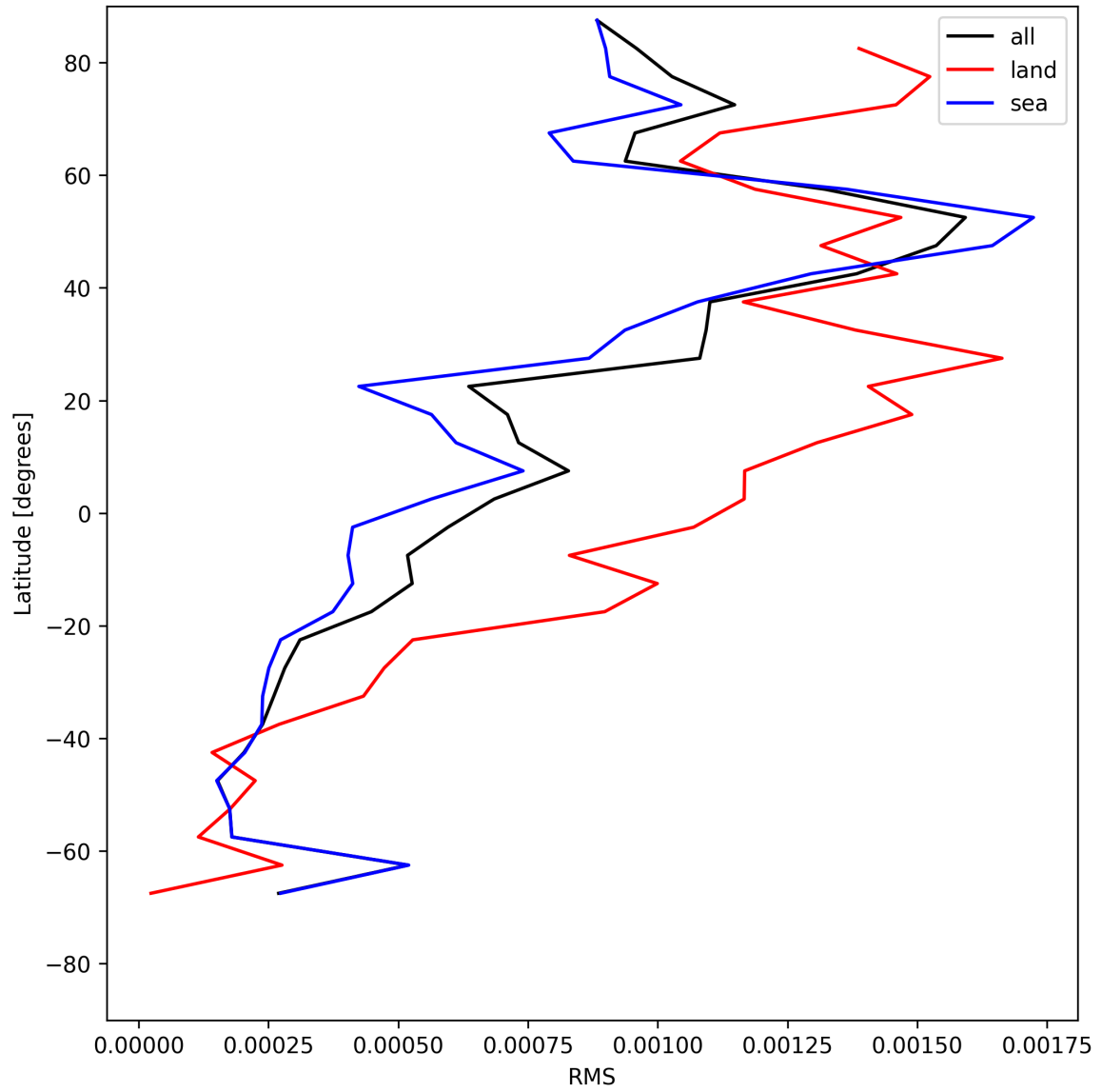
Figure 31: Zonal average of “RMS” for 2025-06-08 to 2025-06-10.
