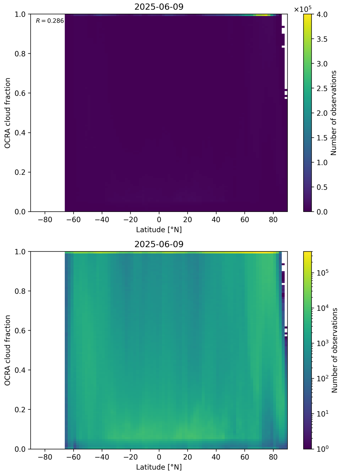
Figure 93: Scatter density plot of “Latitude” against “OCRA cloud fraction” for 2025-06-08 to 2025-06-10.
