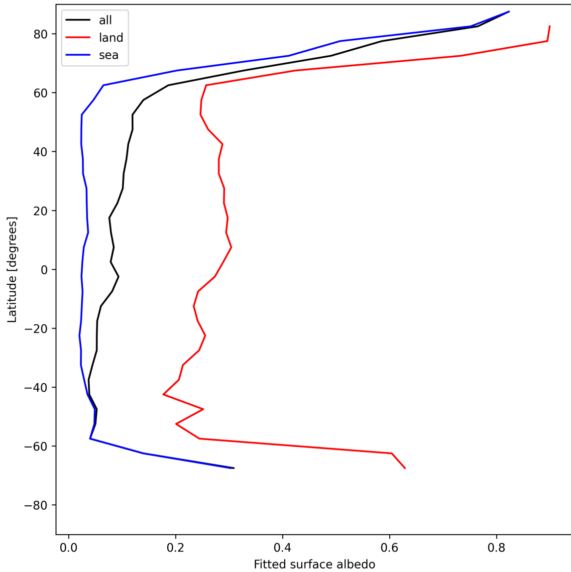
Figure 29: Zonal average of “Fitted surface albedo” for 2025-06-08 to 2025-06-10.
