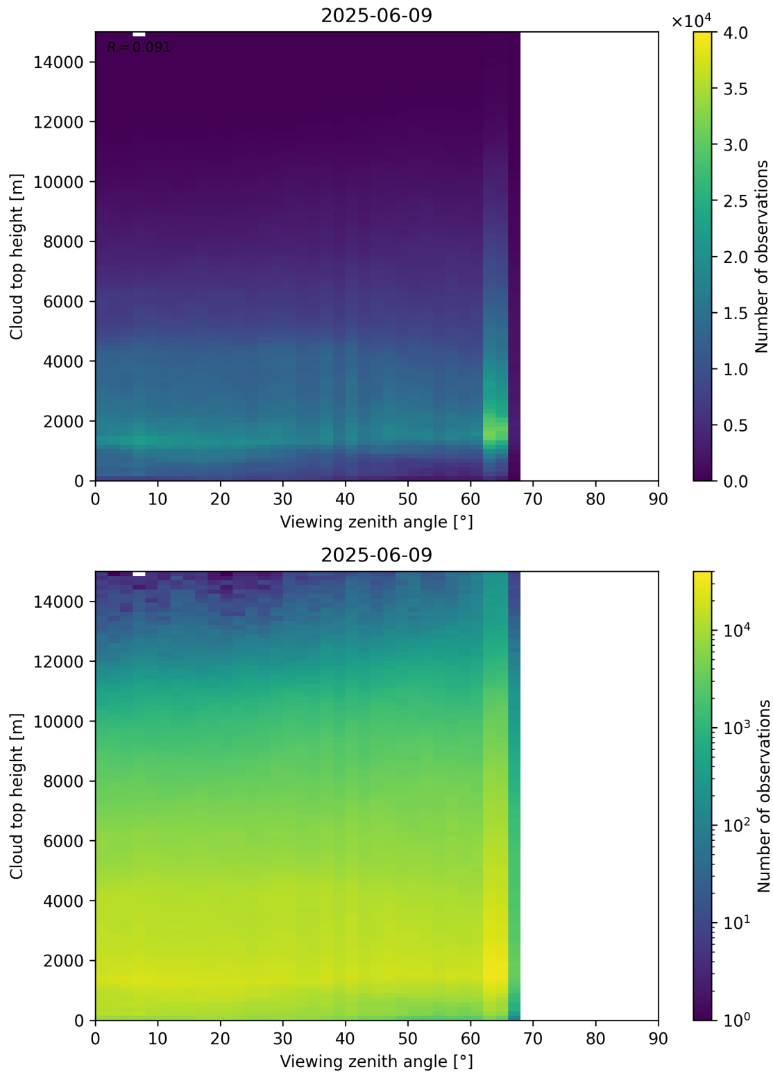
Figure 112: Scatter density plot of “Viewing zenith angle” against “Cloud top height” for 2025-06-08 to 2025-06-10.
