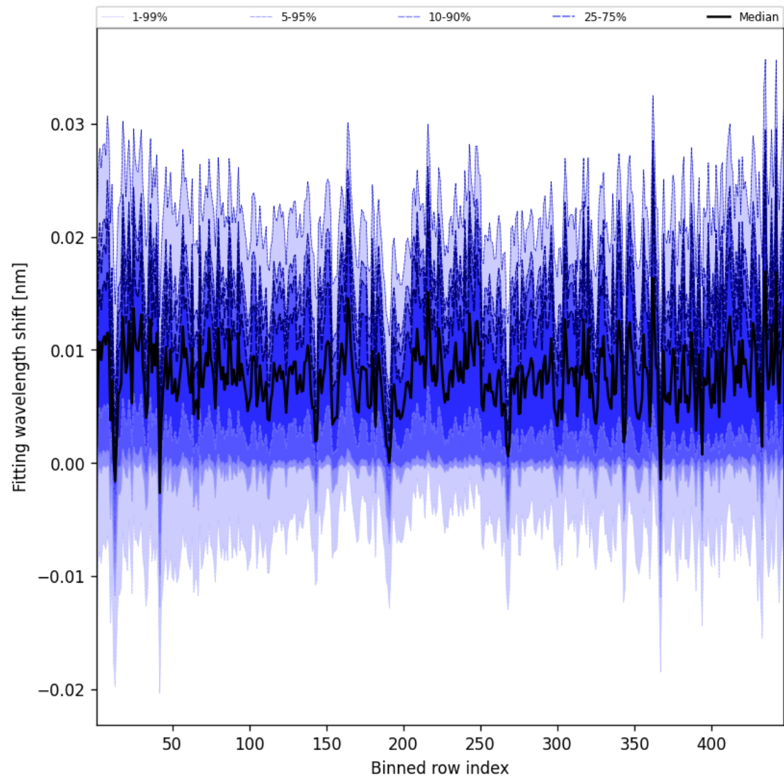
Figure 65: Along track statistics of “Fitting wavelength shift” for 2025-06-08 to 2025-06-10
