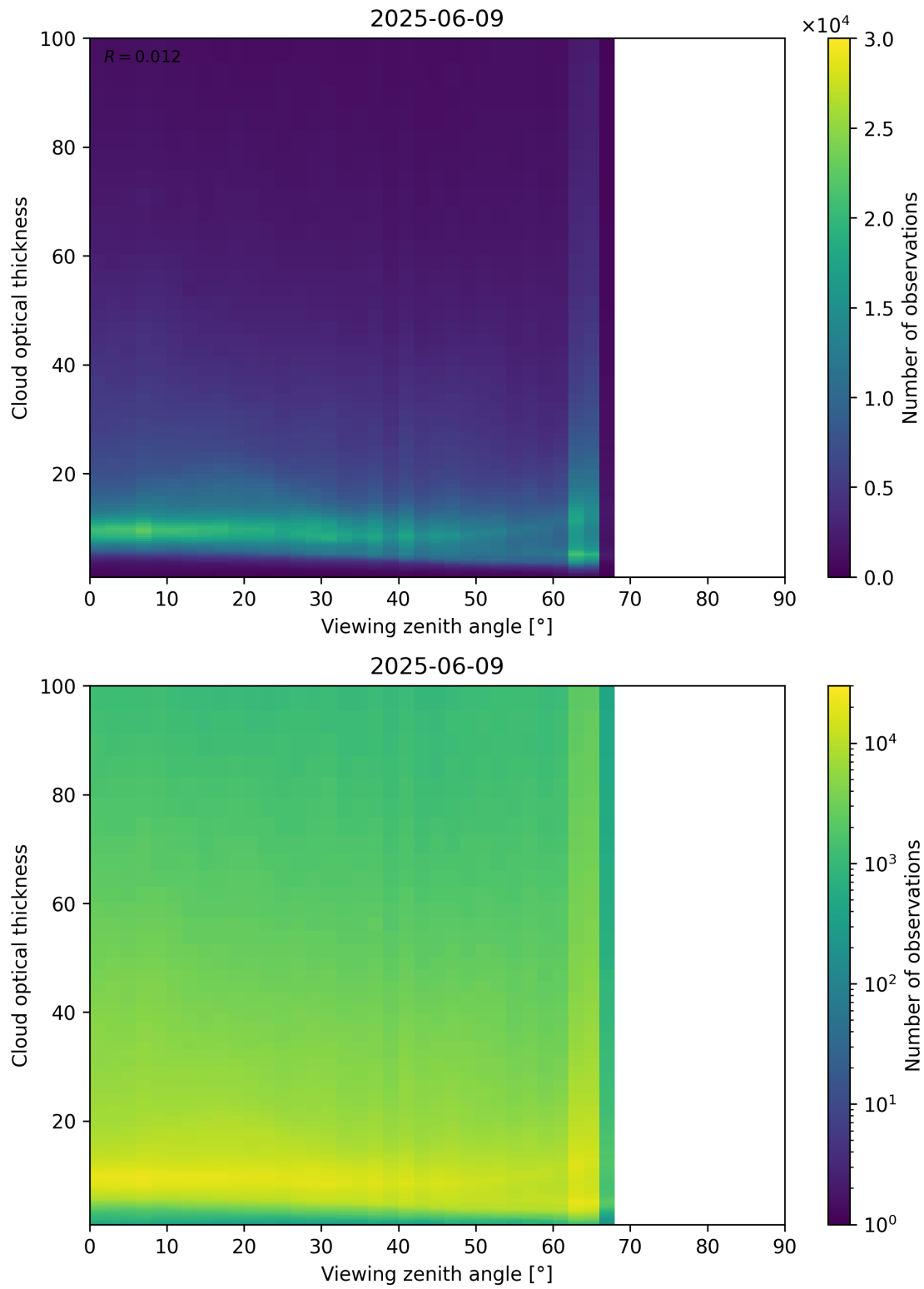
Figure 111: Scatter density plot of “Viewing zenith angle” against “Cloud optical thickness” for 2025-06-08 to 2025-06-10.
