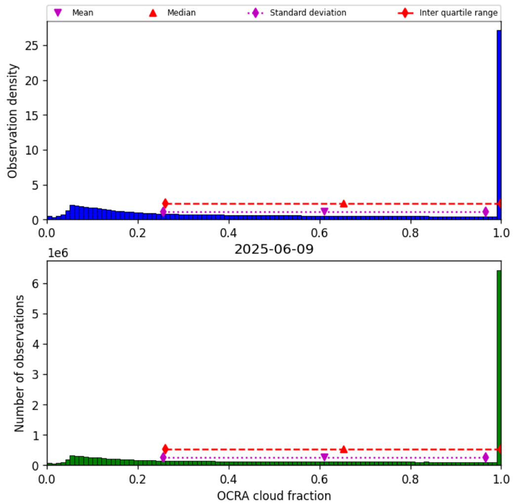
Figure 50: Histogram of “OCRA cloud fraction” for 2025-06-08 to 2025-06-10
