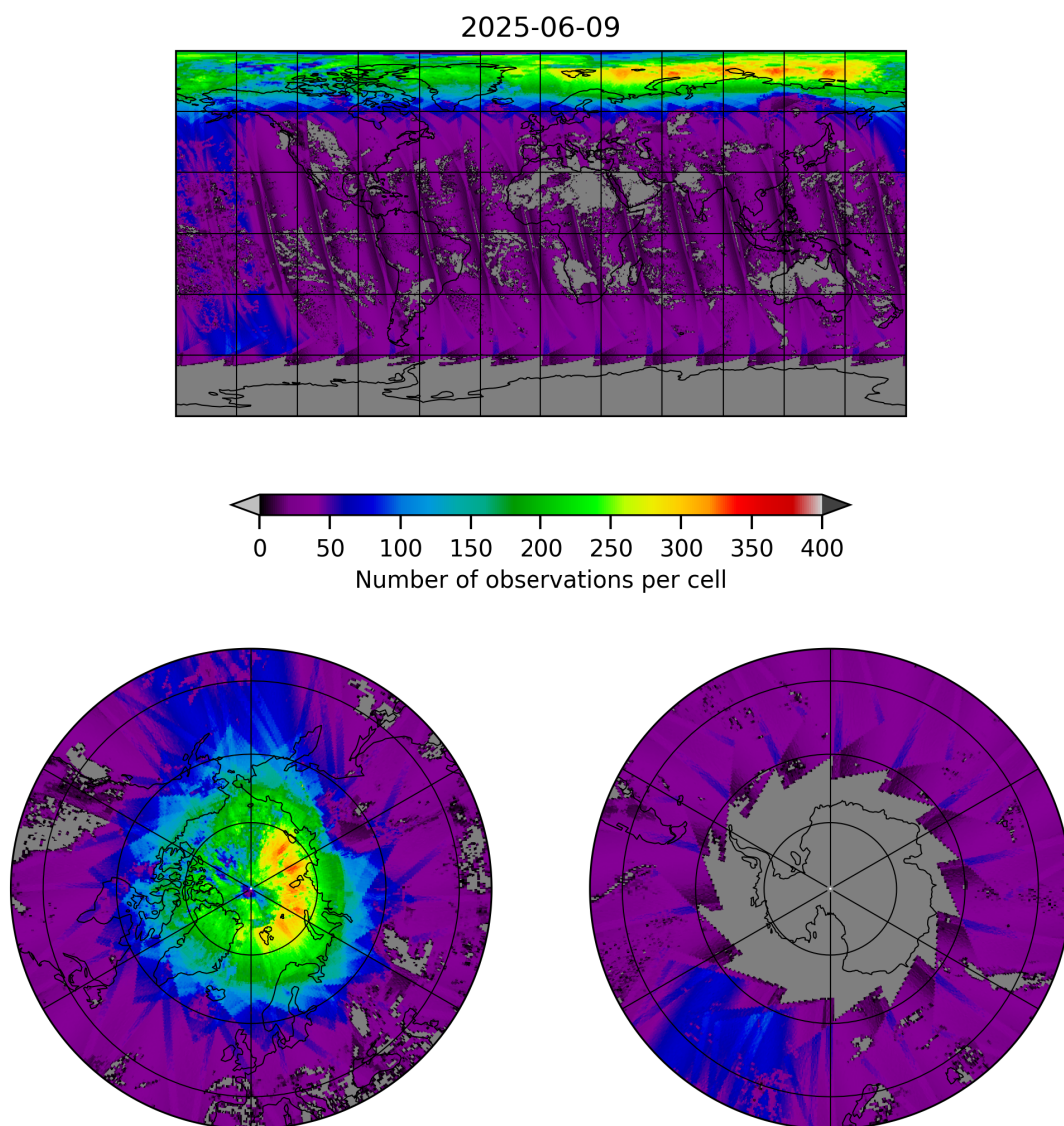
Figure 21: Map of the number of observations for 2025-06-08 to 2025-06-10
