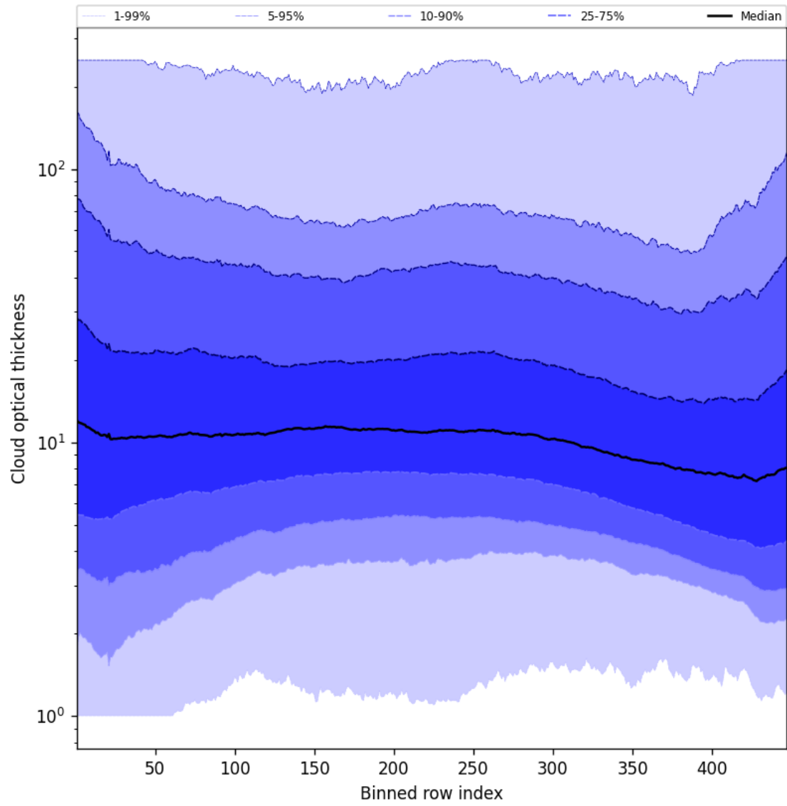
Figure 57: Along track statistics of “Cloud optical thickness” for 2025-06-08 to 2025-06-10
