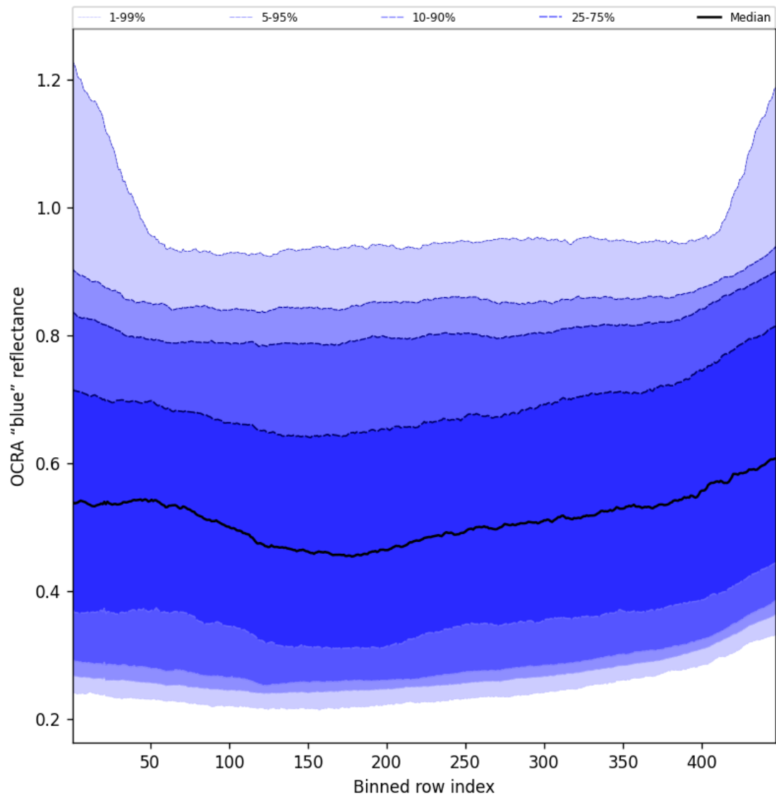
Figure 67: Along track statistics of “OCRA “blue” reflectance” for 2025-06-08 to 2025-06-10
