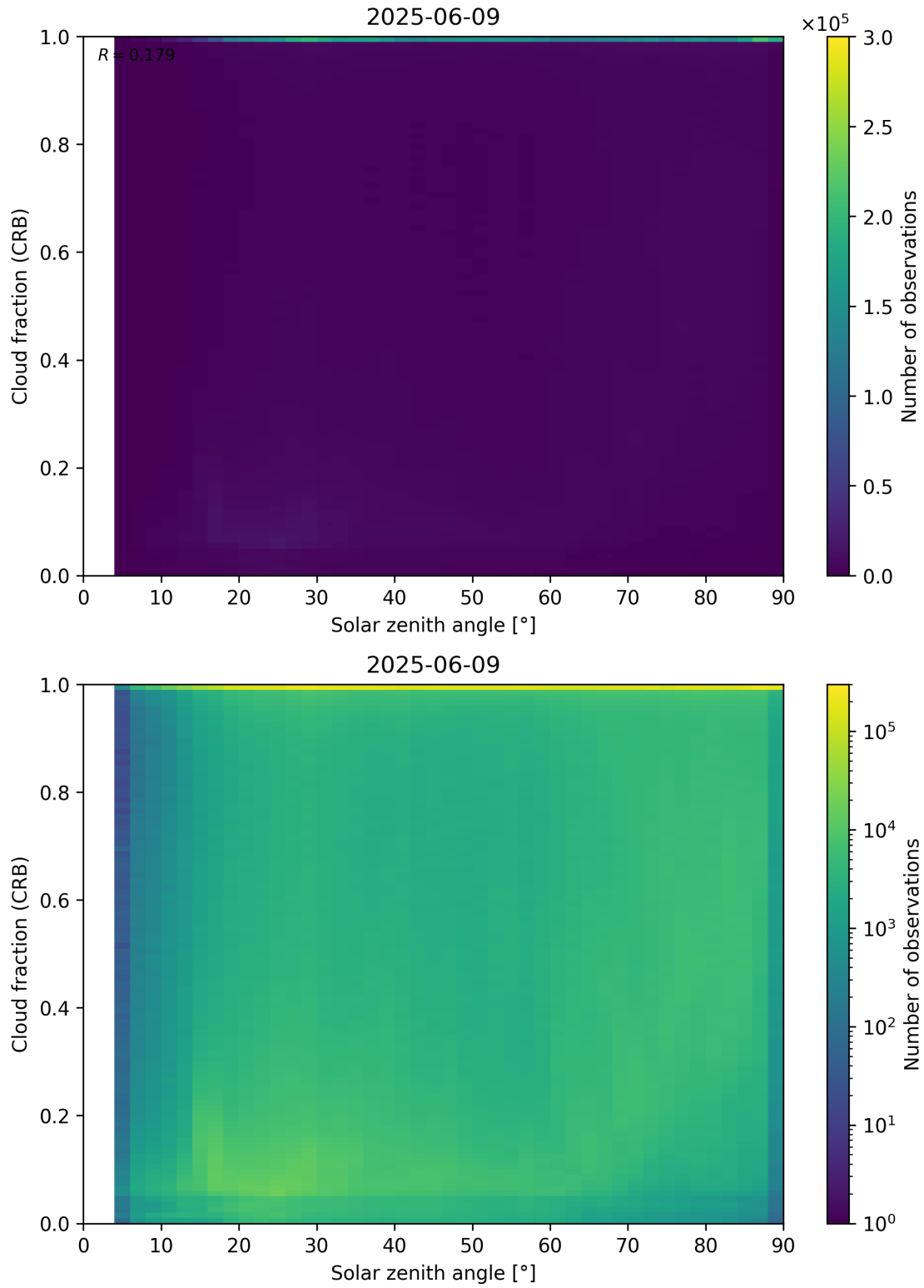
Figure 101: Scatter density plot of “Solar zenith angle” against “Cloud fraction (CRB)” for 2025-06-08 to 2025-06-10.
