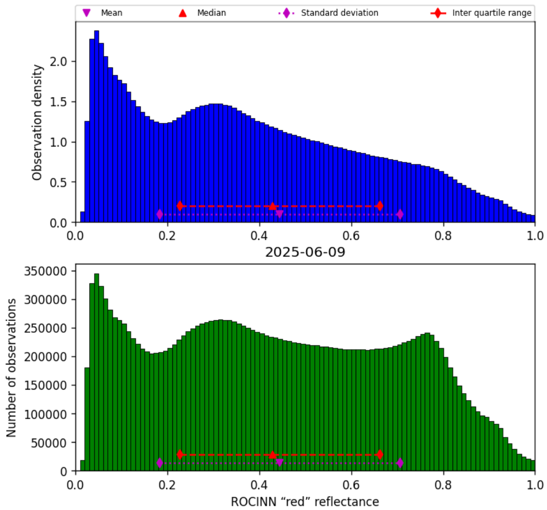
Figure 53: Histogram of “ROCINN “red” reflectance” for 2025-06-08 to 2025-06-10
