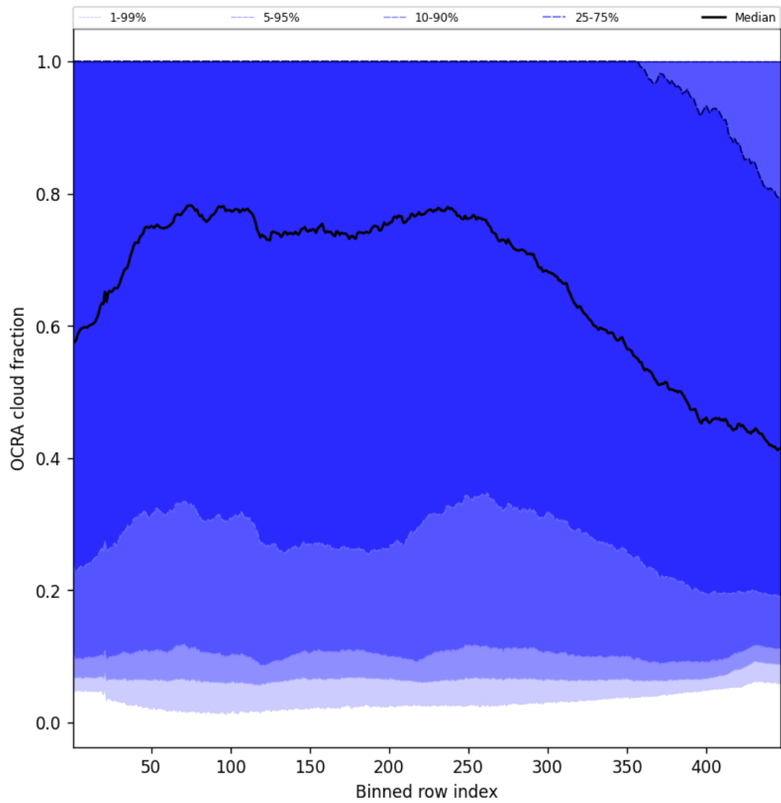
Figure 66: Along track statistics of “OCRA cloud fraction” for 2025-06-08 to 2025-06-10
