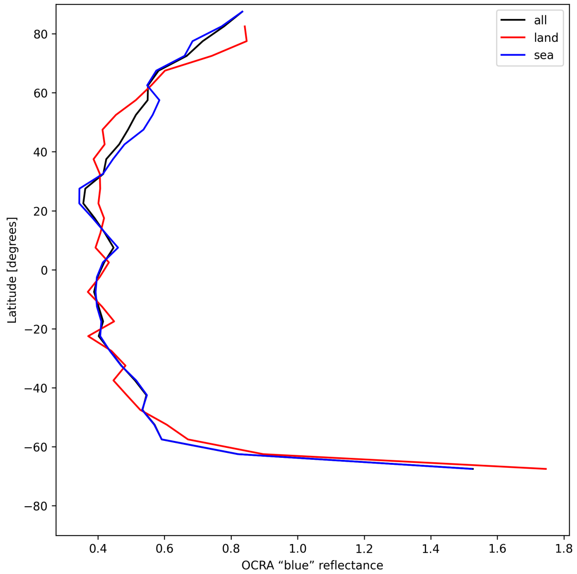
Figure 35: Zonal average of “OCRA “blue” reflectance” for 2025-06-08 to 2025-06-10.
