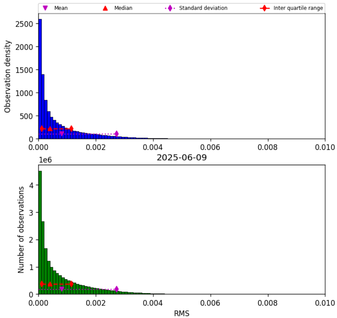
Figure 47: Histogram of “RMS” for 2025-06-08 to 2025-06-10
