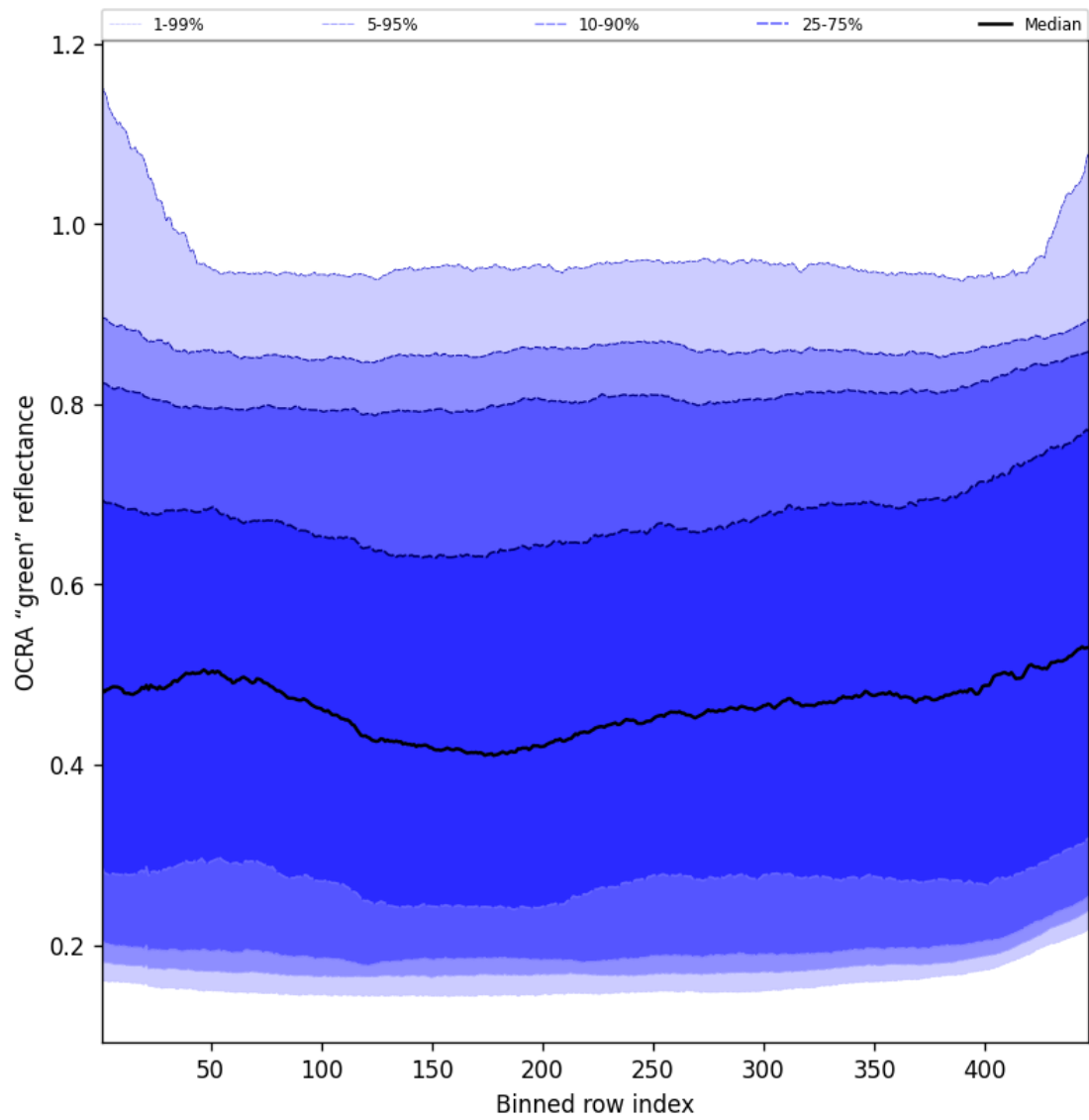
Figure 68: Along track statistics of “OCRA “green” reflectance” for 2025-06-08 to 2025-06-10
