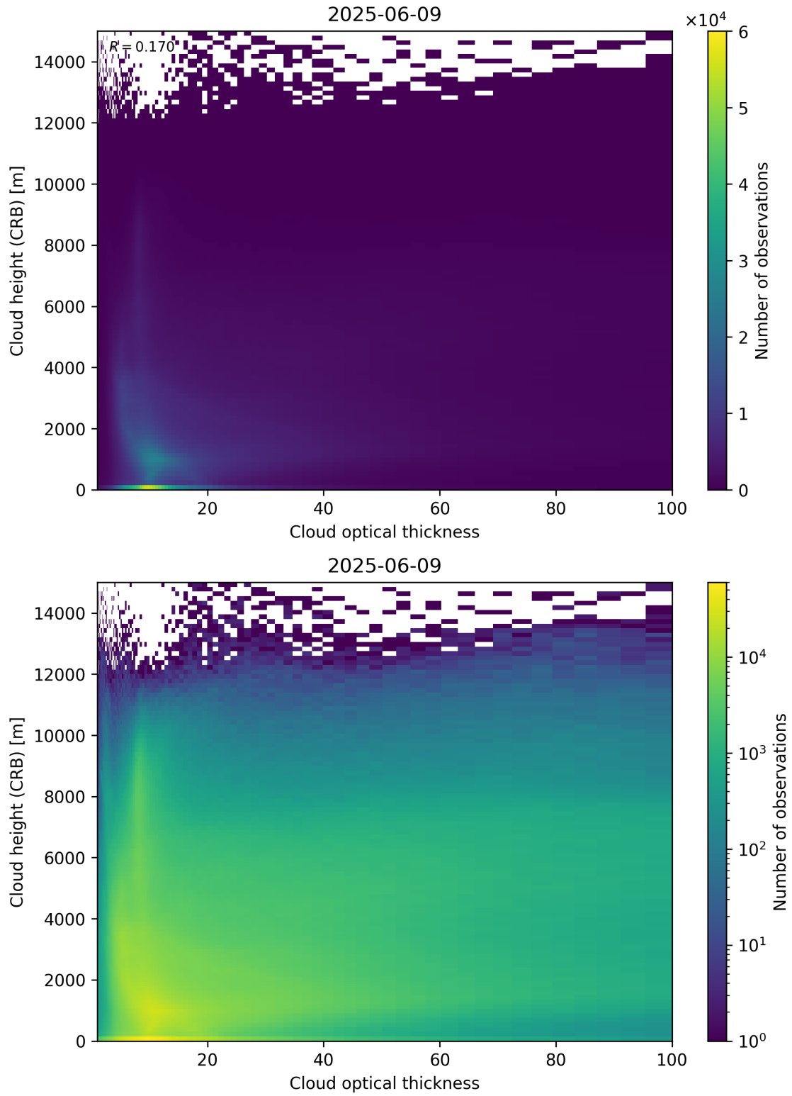
Figure 85: Scatter density plot of “Cloud optical thickness” against “Cloud height (CRB)” for 2025-06-08 to 2025-06-10.
