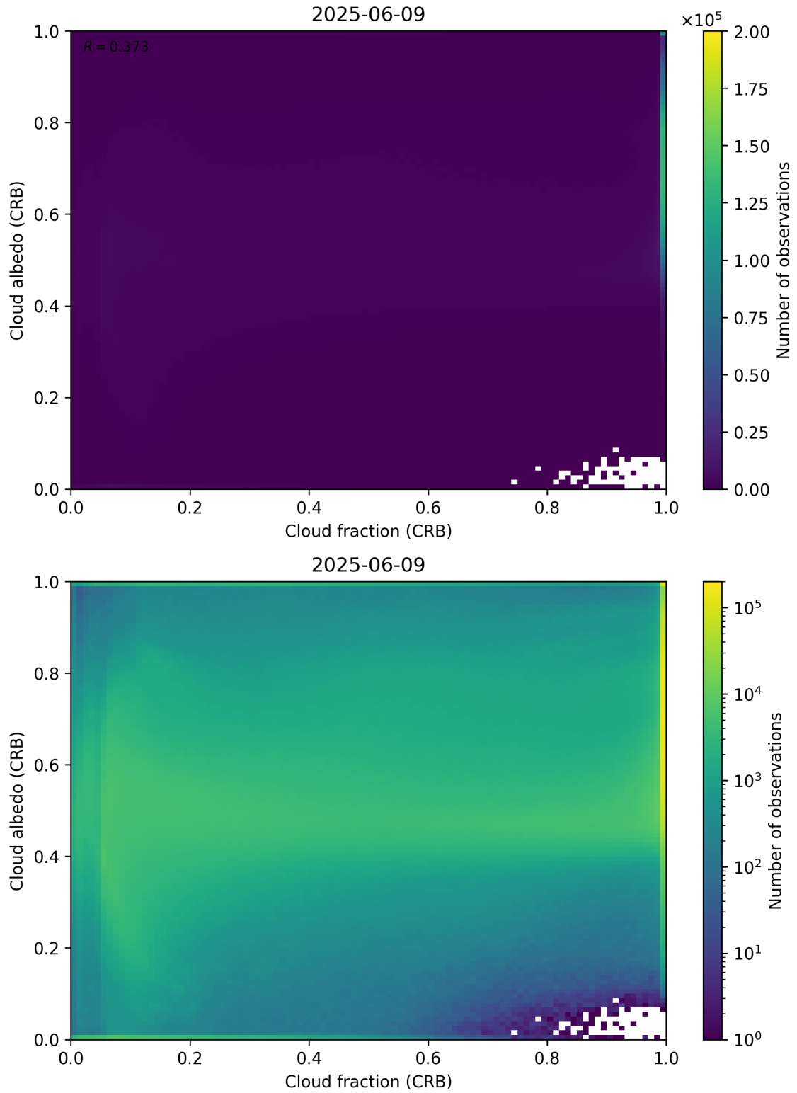
Figure 77: Scatter density plot of “Cloud fraction (CRB)” against “Cloud albedo (CRB)” for 2025-06-08 to 2025-06-10.
