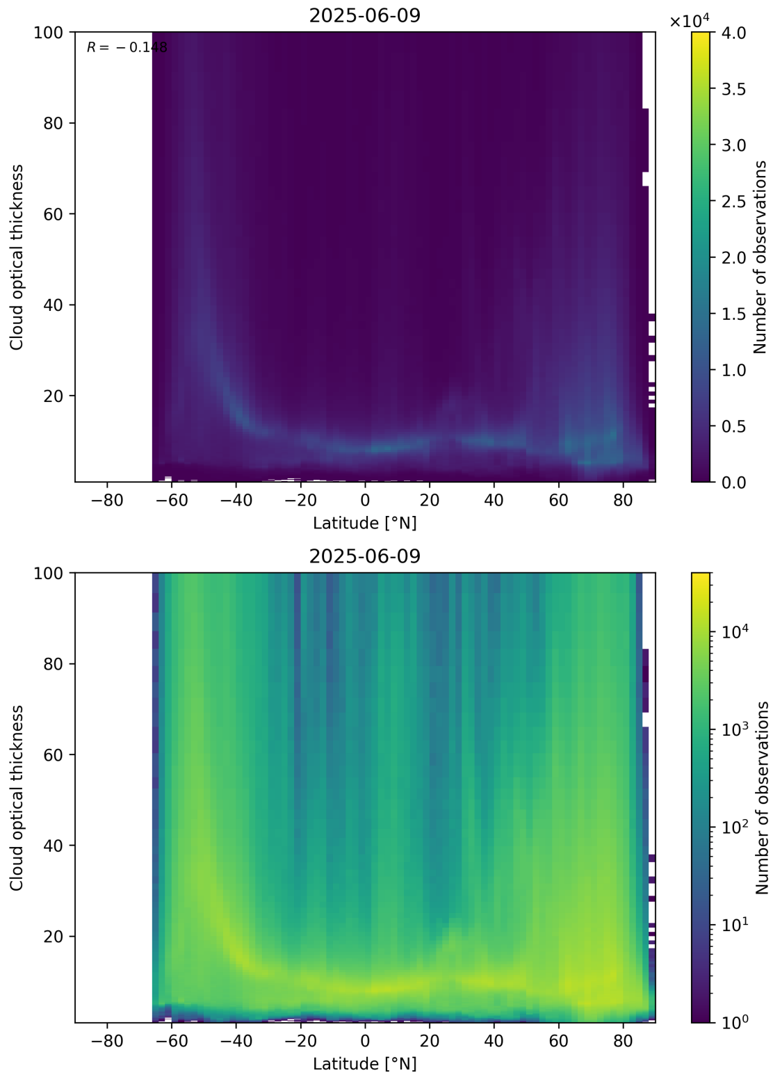
Figure 96: Scatter density plot of “Latitude” against “Cloud optical thickness” for 2025-06-08 to 2025-06-10.
