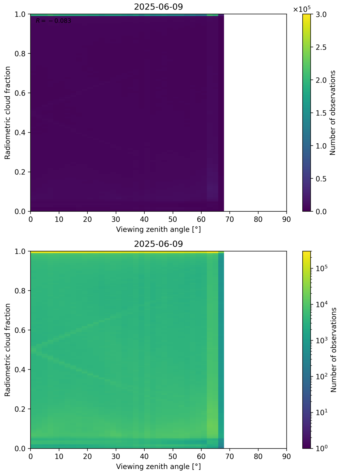
Figure 107: Scatter density plot of “Viewing zenith angle” against “Radiometric cloud fraction” for 2025-06-08 to 2025-06-10.
