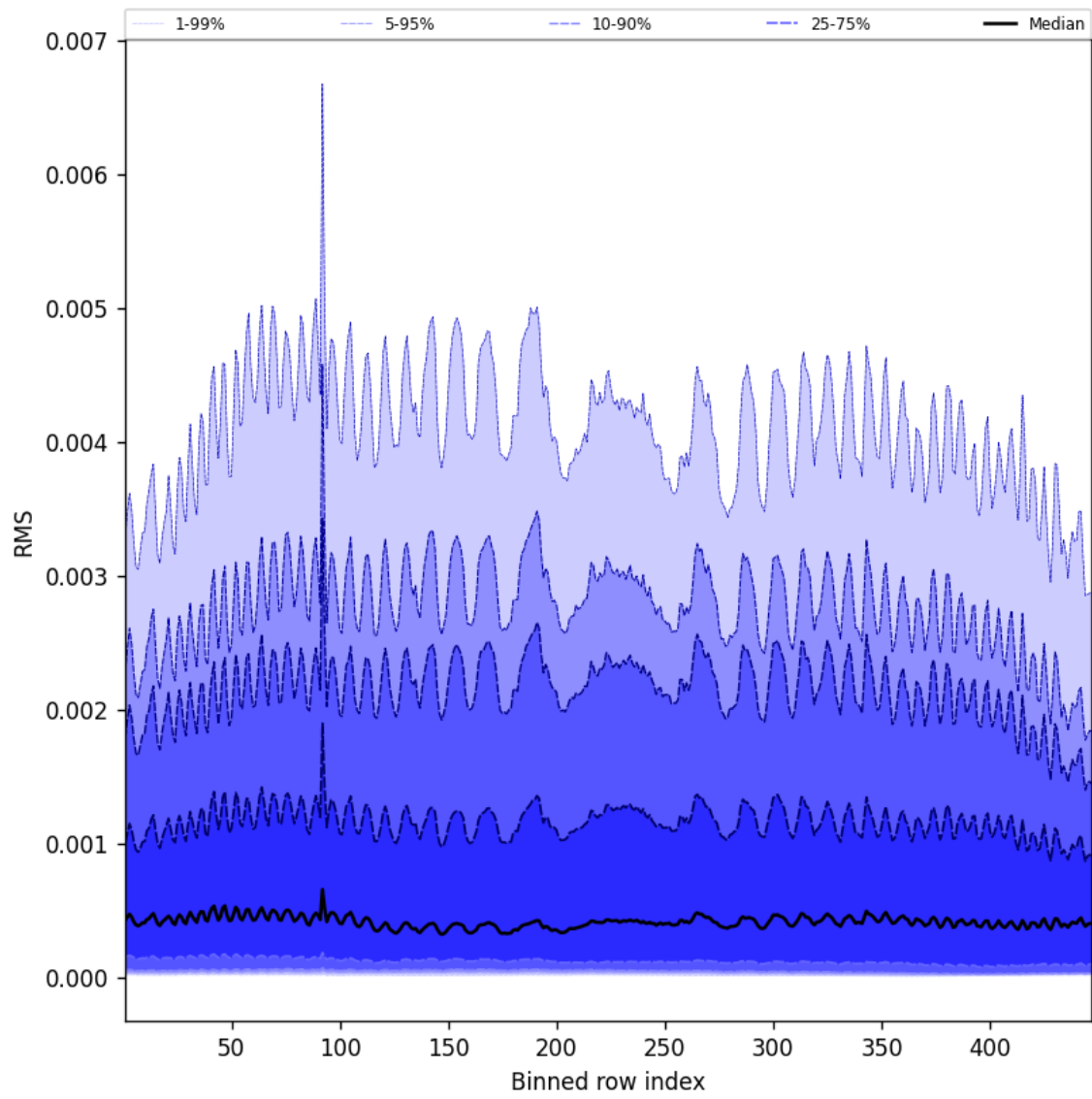
Figure 63: Along track statistics of “RMS” for 2025-06-08 to 2025-06-10
