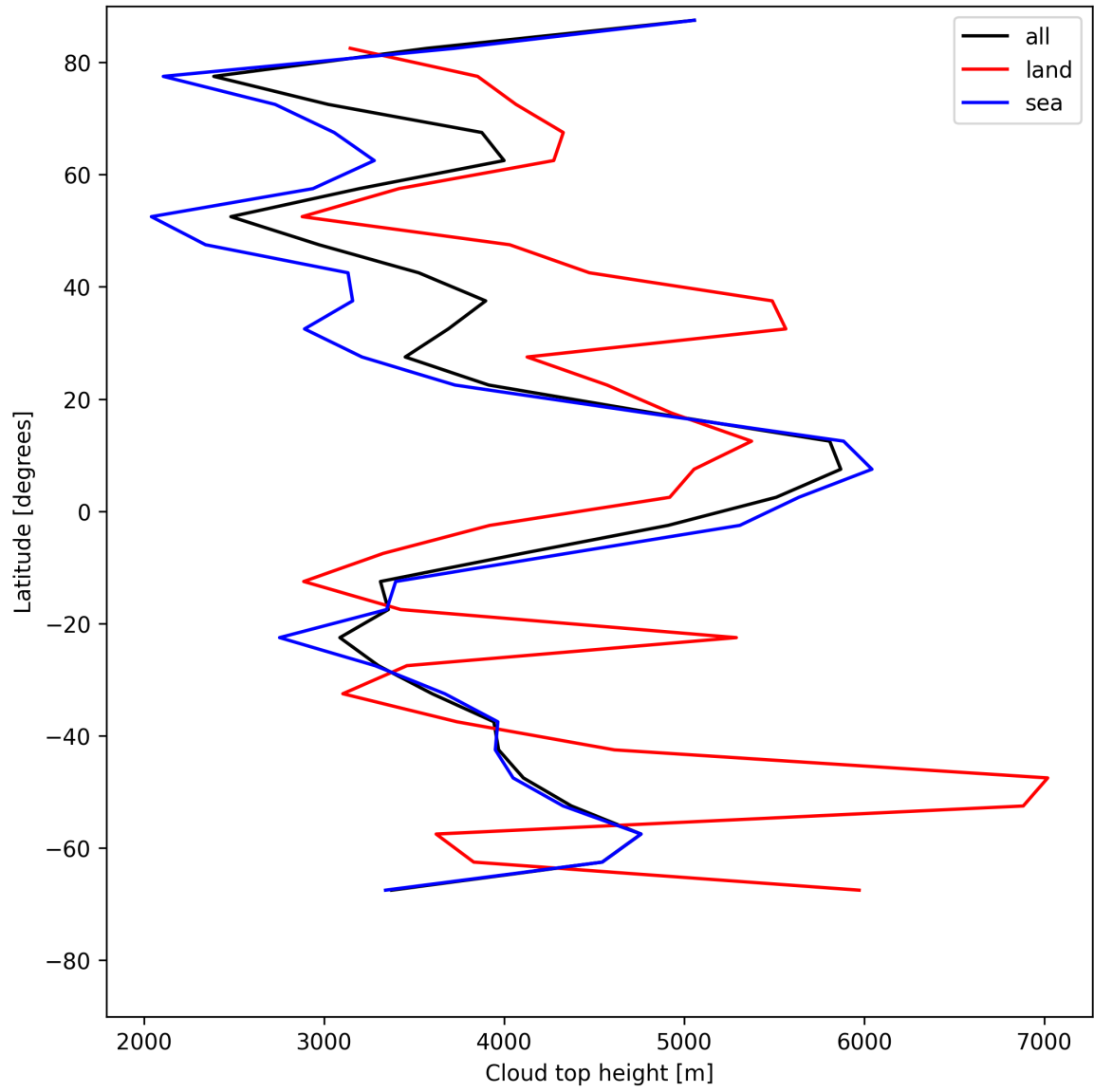
Figure 24: Zonal average of “Cloud top height” for 2025-06-08 to 2025-06-10.
