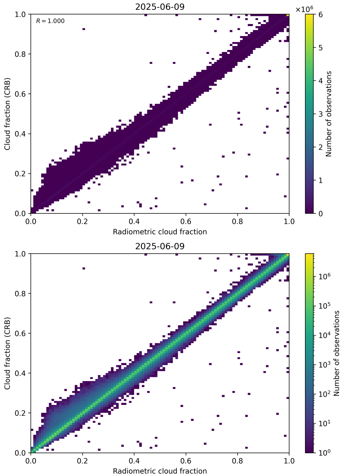
Figure 73: Scatter density plot of “Radiometric cloud fraction” against “Cloud fraction (CRB)” for 2025-06-08 to 2025-06-10.
