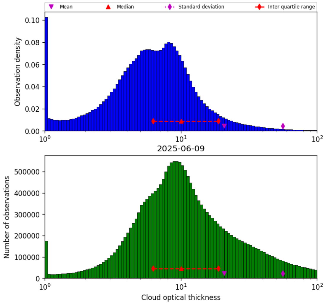
Figure 41: Histogram of “Cloud optical thickness” for 2025-06-08 to 2025-06-10
