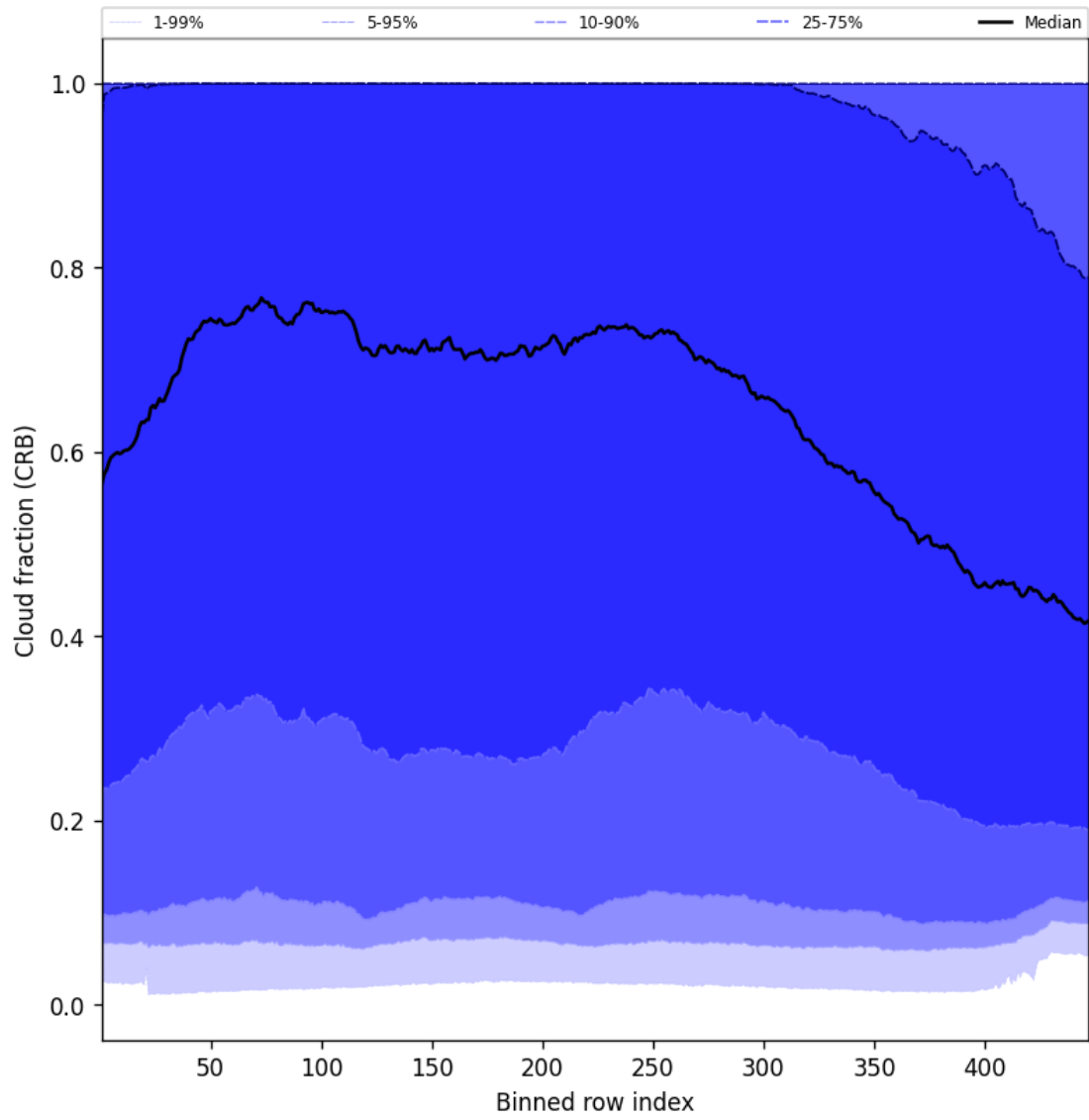
Figure 58: Along track statistics of “Cloud fraction (CRB)” for 2025-06-08 to 2025-06-10
