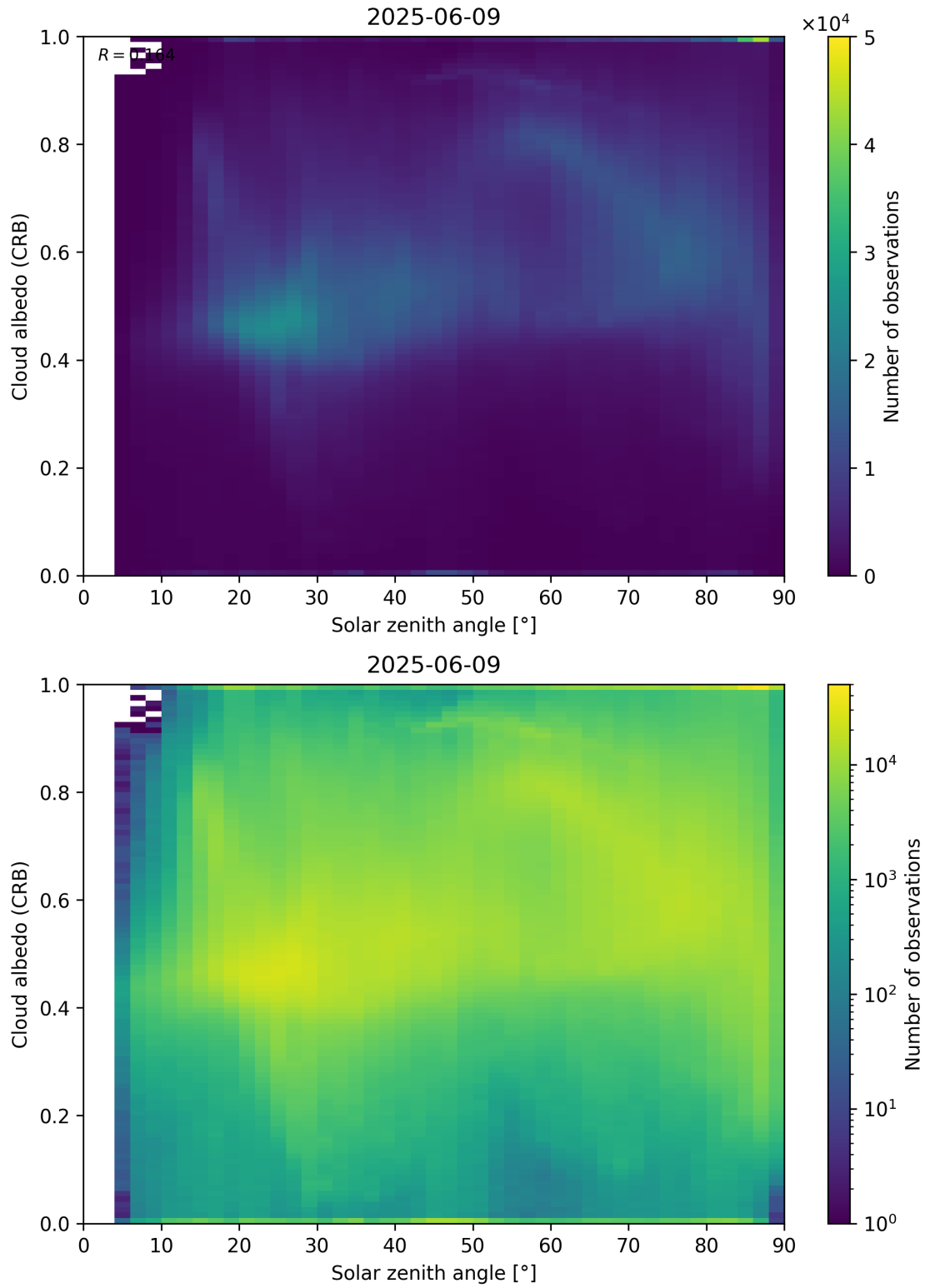
Figure 98: Scatter density plot of “Solar zenith angle” against “Cloud albedo (CRB)” for 2025-06-08 to 2025-06-10.
