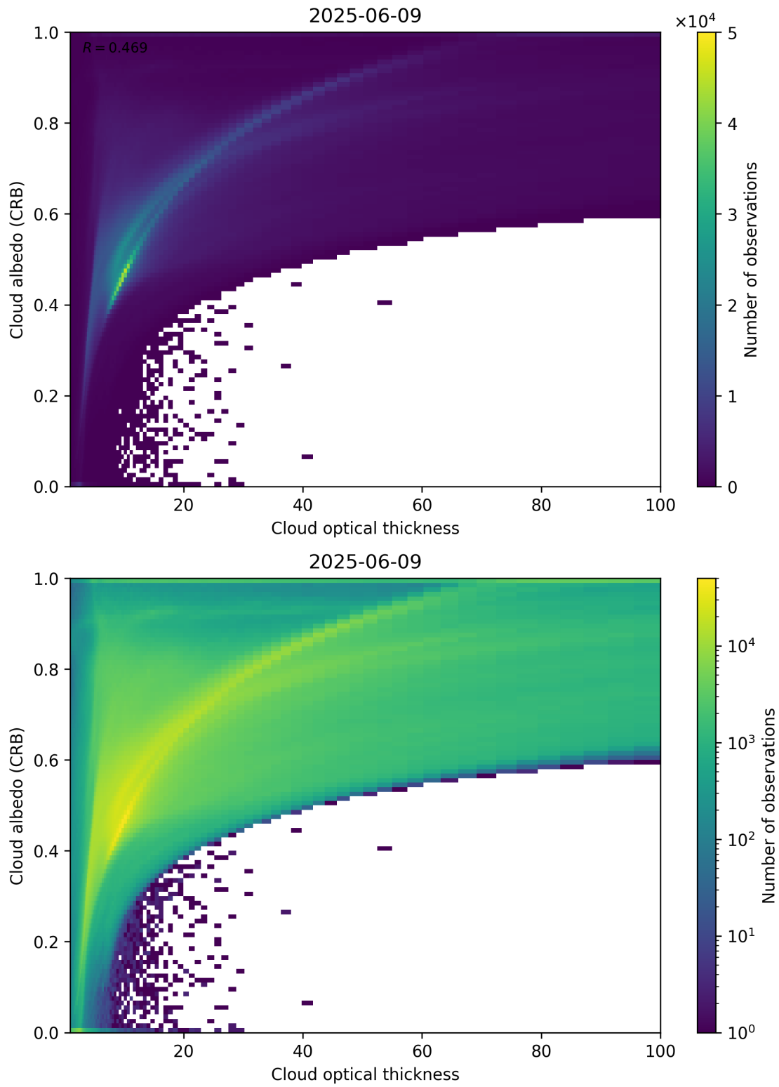
Figure 82: Scatter density plot of “Cloud optical thickness” against “Cloud albedo (CRB)” for 2025-06-08 to 2025-06-10.
