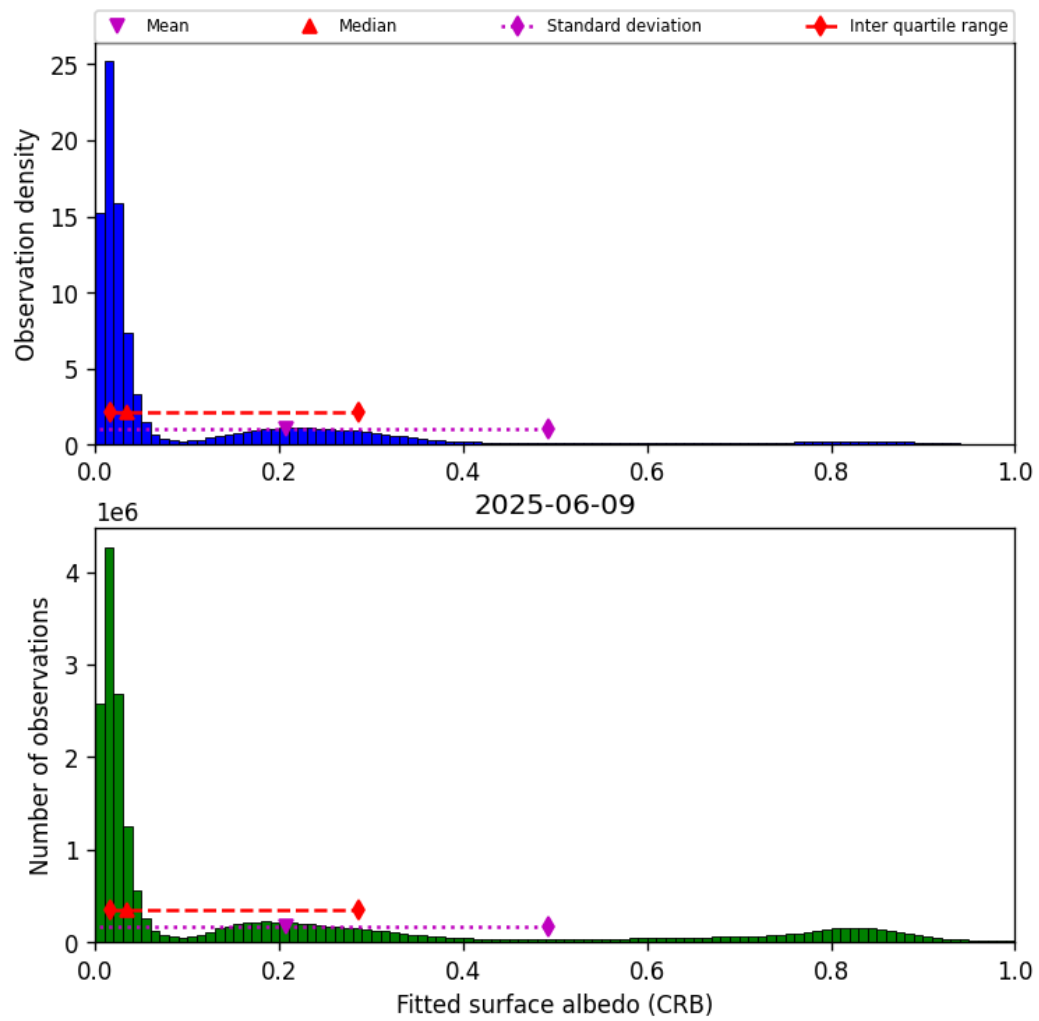
Figure 46: Histogram of “Fitted surface albedo (CRB)” for 2025-06-08 to 2025-06-10
