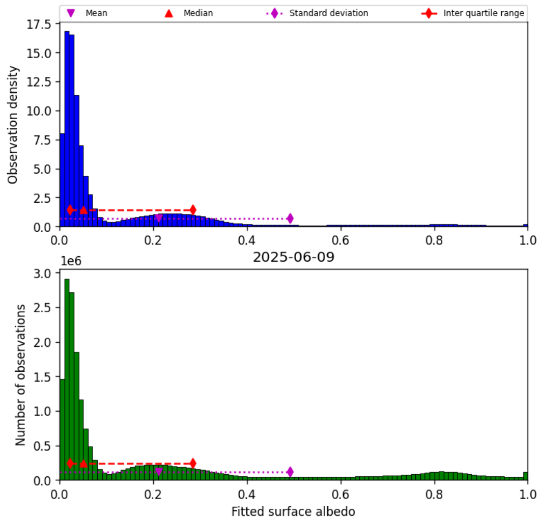
Figure 45: Histogram of “Fitted surface albedo” for 2025-06-08 to 2025-06-10
