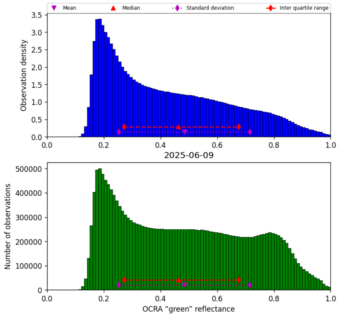
Figure 52: Histogram of “OCRA “green” reflectance” for 2025-06-08 to 2025-06-10
