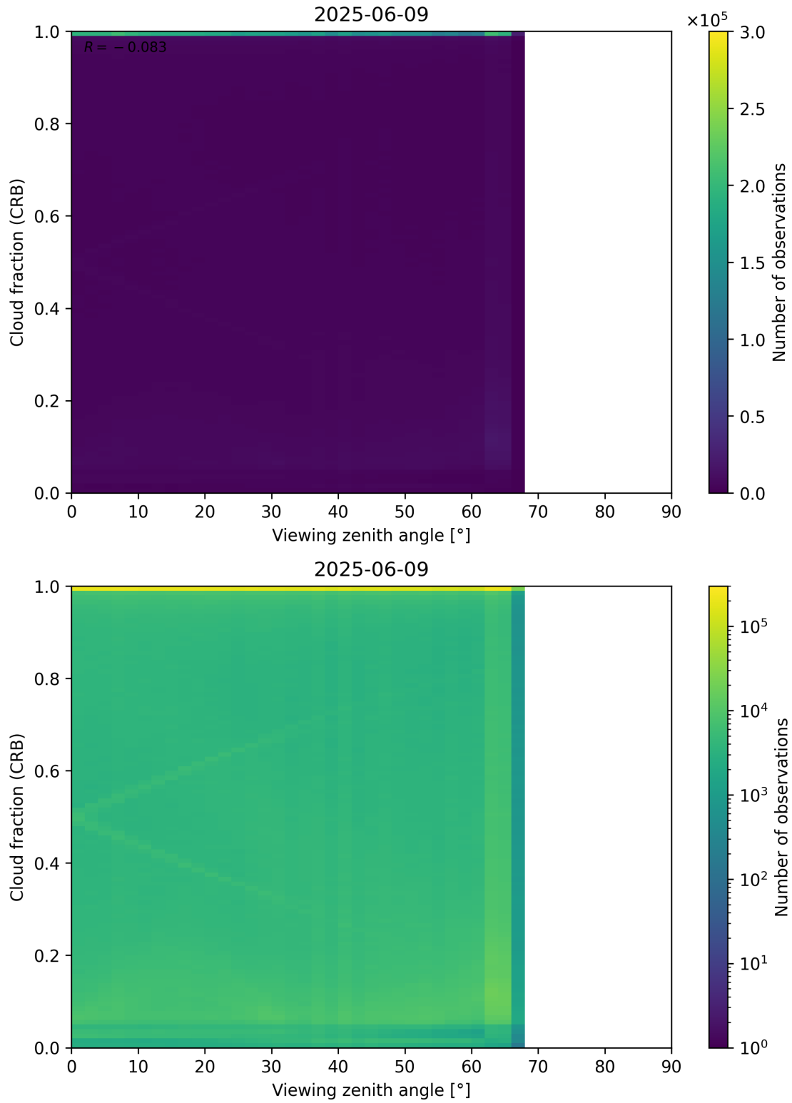
Figure 109: Scatter density plot of “Viewing zenith angle” against “Cloud fraction (CRB)” for 2025-06-08 to 2025-06-10.
