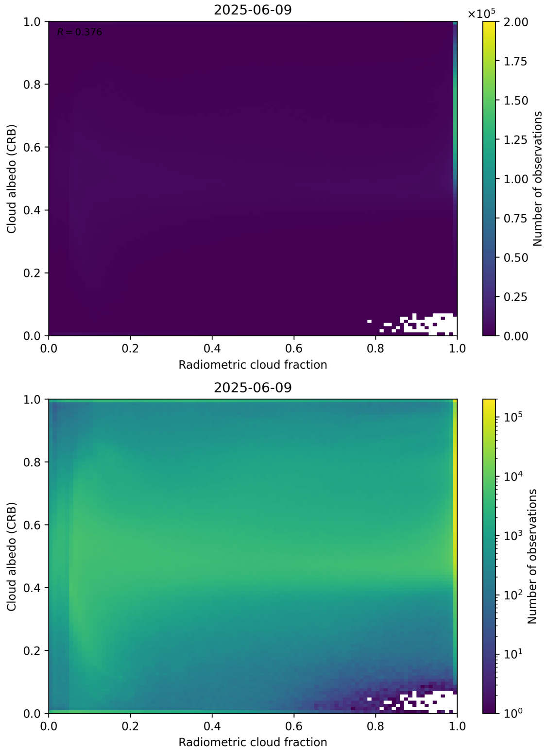
Figure 71: Scatter density plot of “Radiometric cloud fraction” against “Cloud albedo (CRB)” for 2025-06-08 to 2025-06-10.
