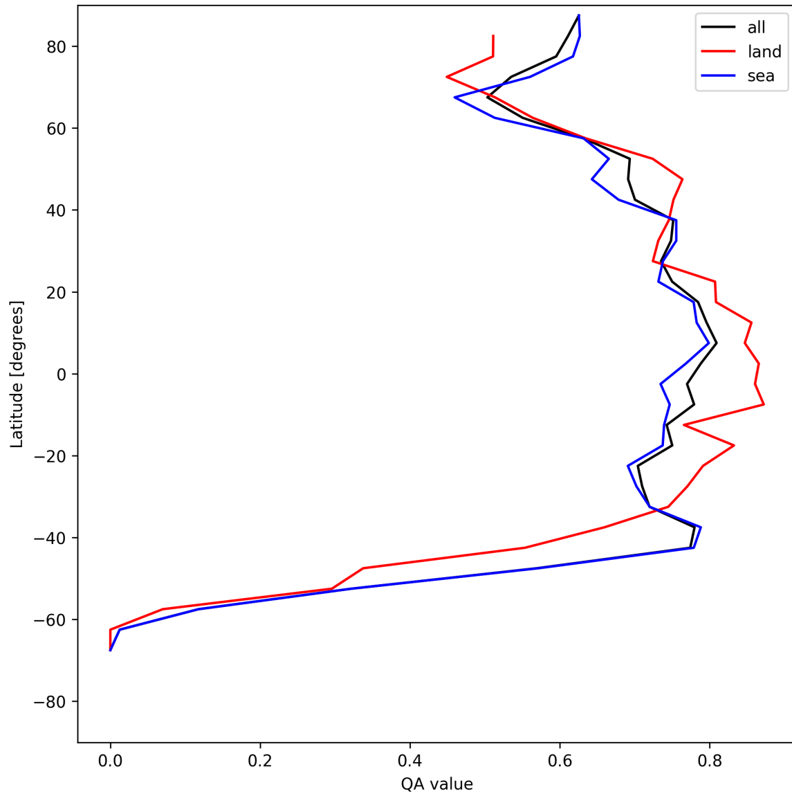
Figure 22: Zonal average of “QA value” for 2025-06-08 to 2025-06-10.
