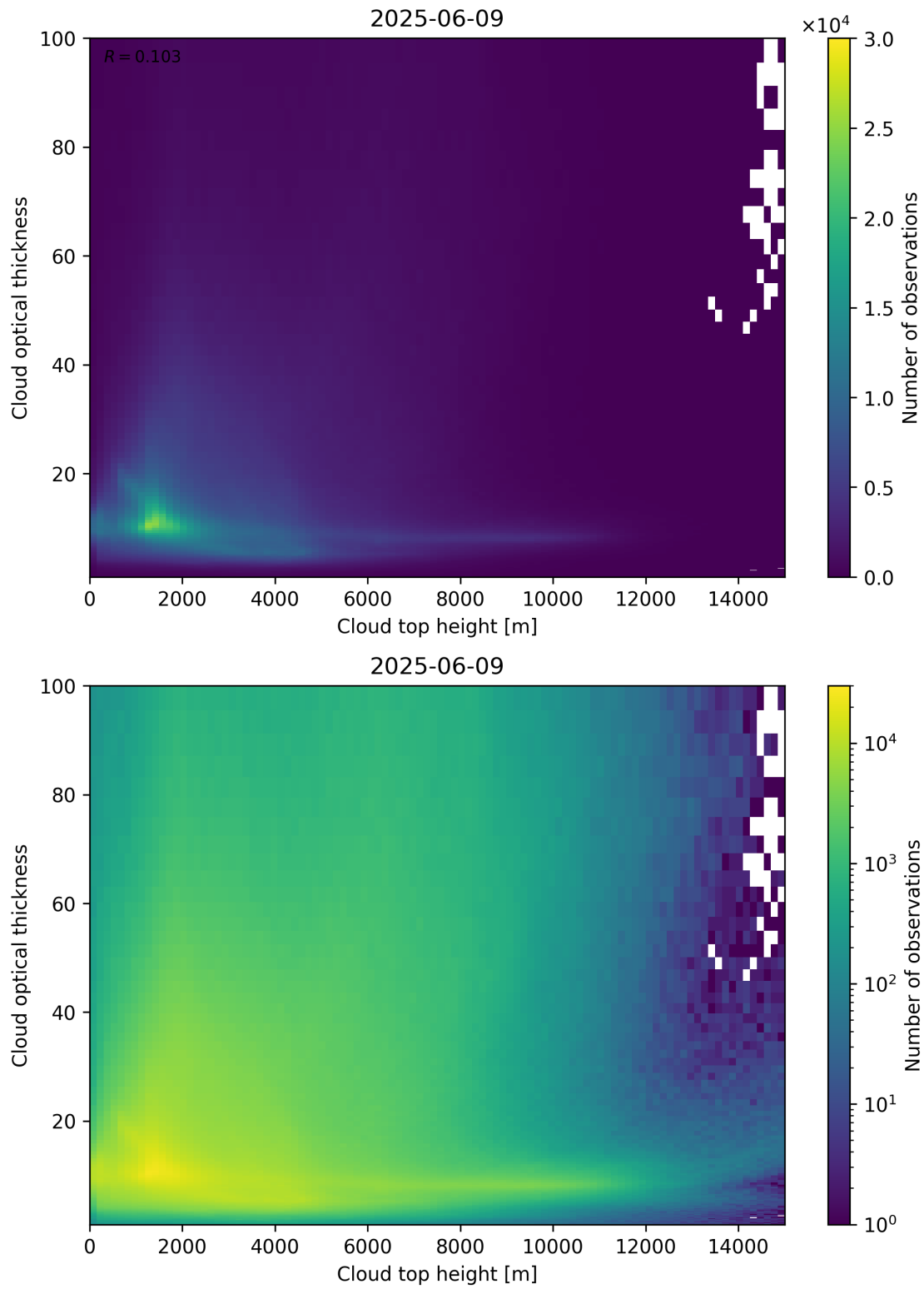
Figure 90: Scatter density plot of “Cloud top height” against “Cloud optical thickness” for 2025-06-08 to 2025-06-10.
