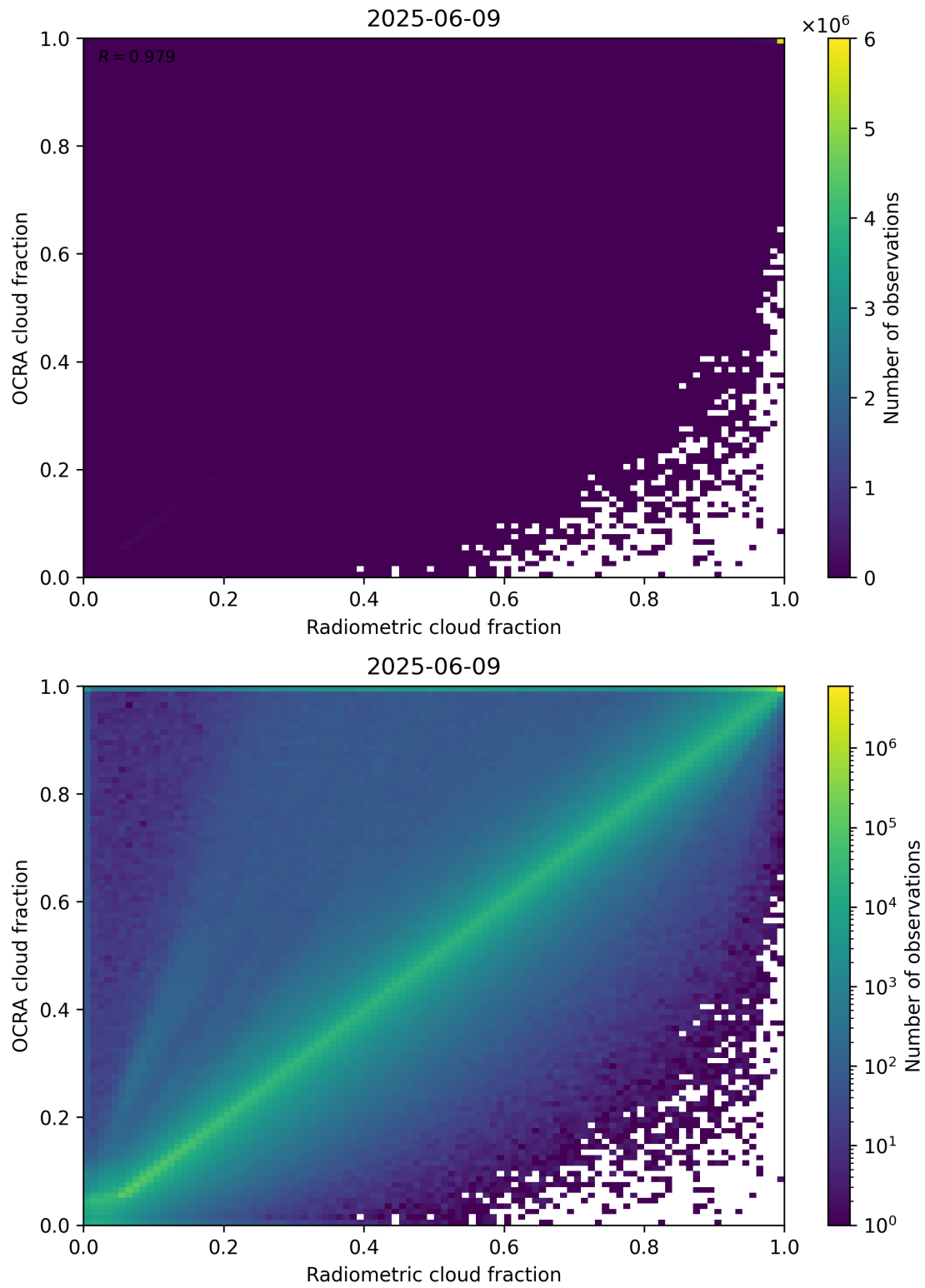
Figure 72: Scatter density plot of “Radiometric cloud fraction” against “OCRA cloud fraction” for 2025-06-08 to 2025-06-10.
