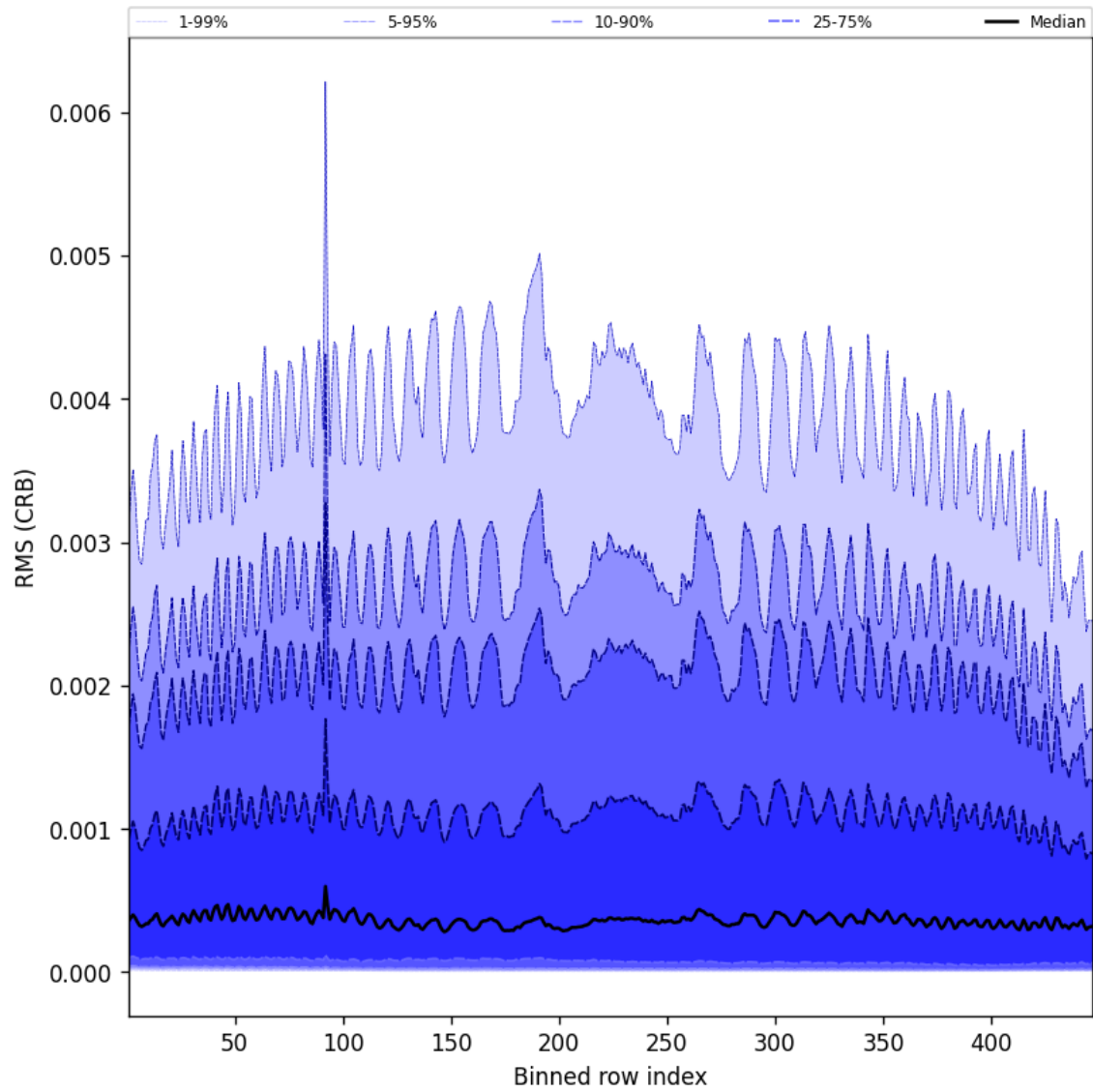
Figure 64: Along track statistics of “RMS (CRB)” for 2025-06-08 to 2025-06-10
