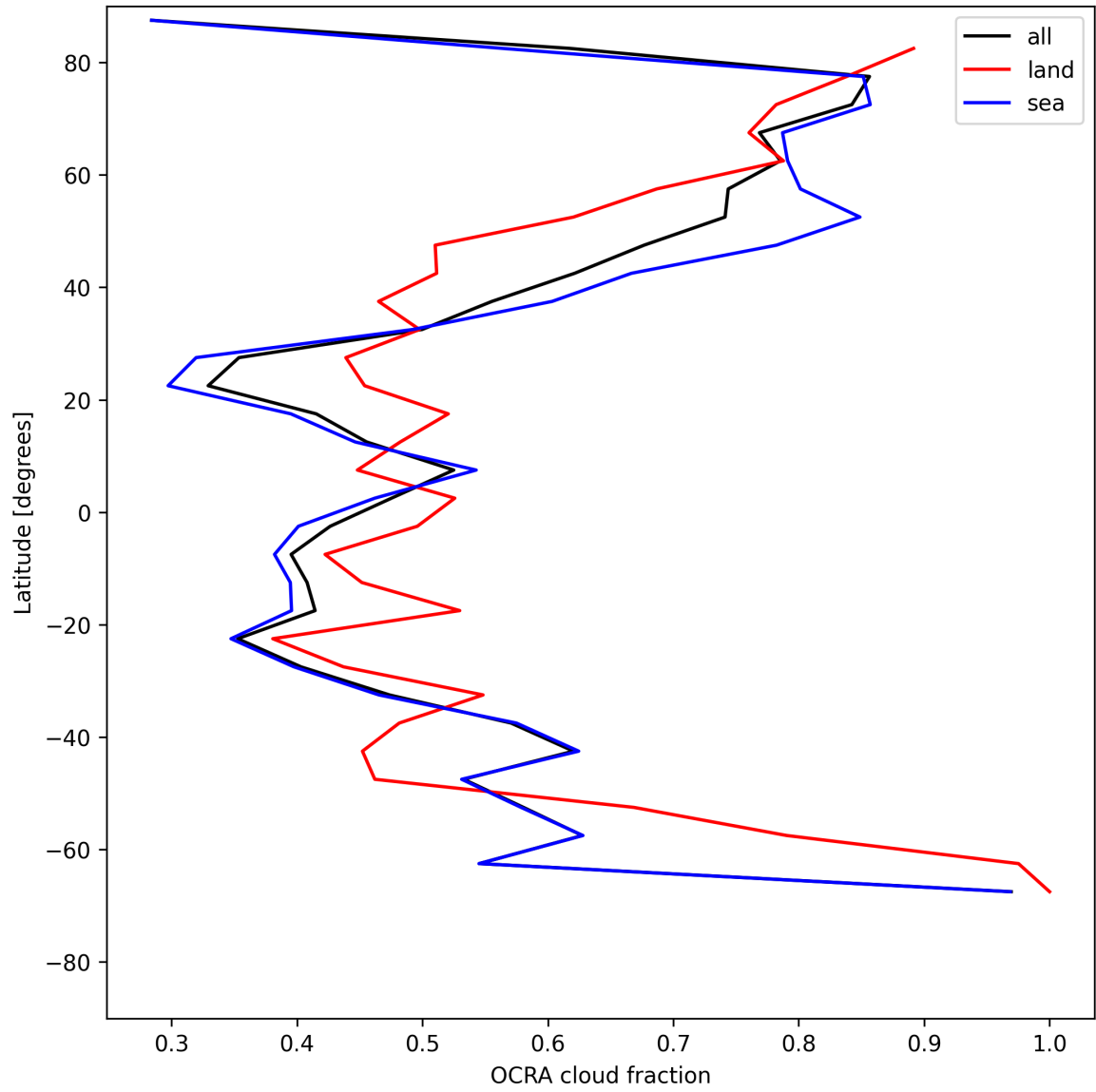
Figure 34: Zonal average of “OCRA cloud fraction” for 2025-06-08 to 2025-06-10.
