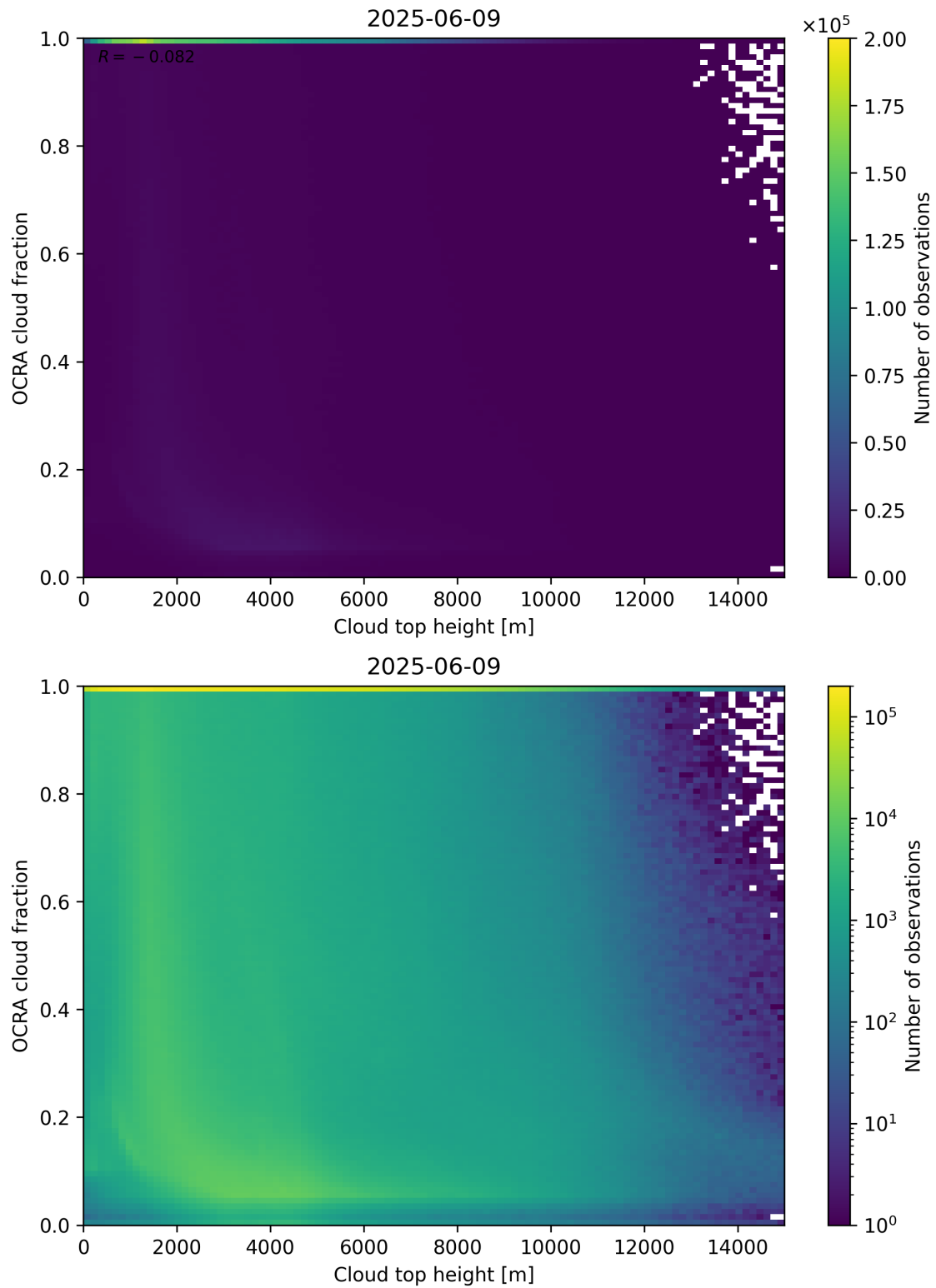
Figure 87: Scatter density plot of “Cloud top height” against “OCRA cloud fraction” for 2025-06-08 to 2025-06-10.
