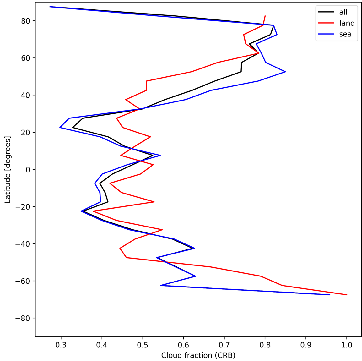
Figure 26: Zonal average of “Cloud fraction (CRB)” for 2025-06-08 to 2025-06-10.
