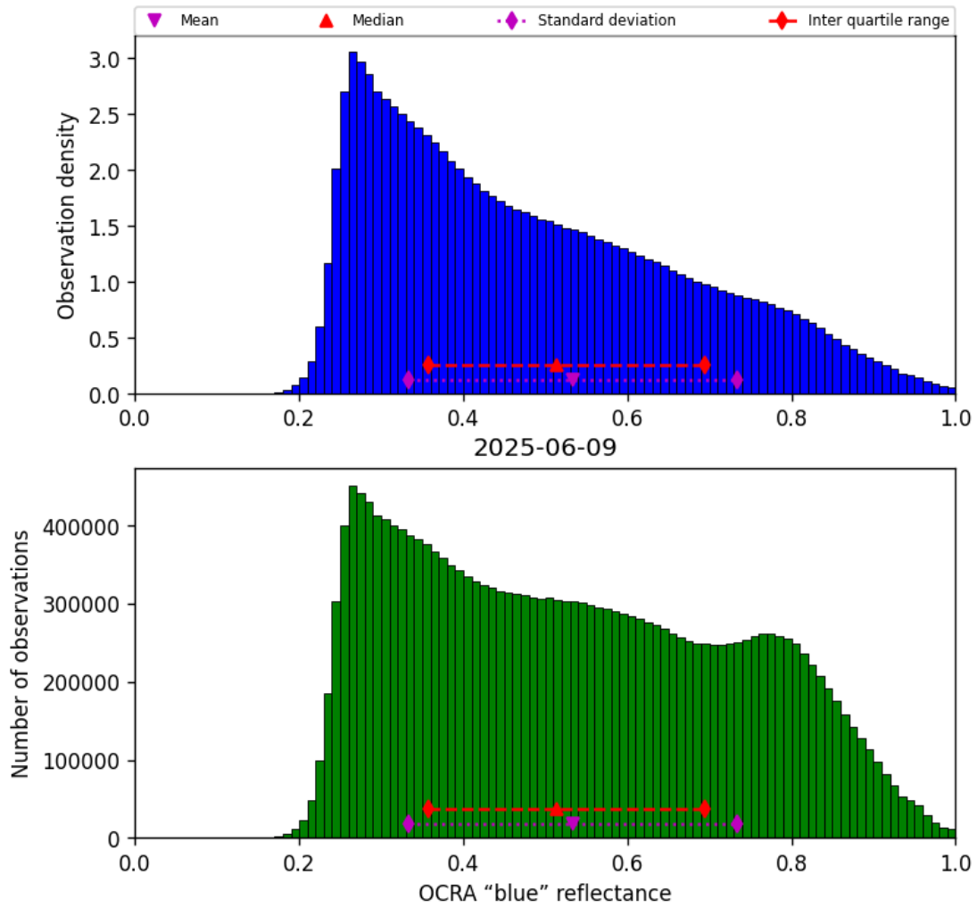
Figure 51: Histogram of “OCRA “blue” reflectance” for 2025-06-08 to 2025-06-10
