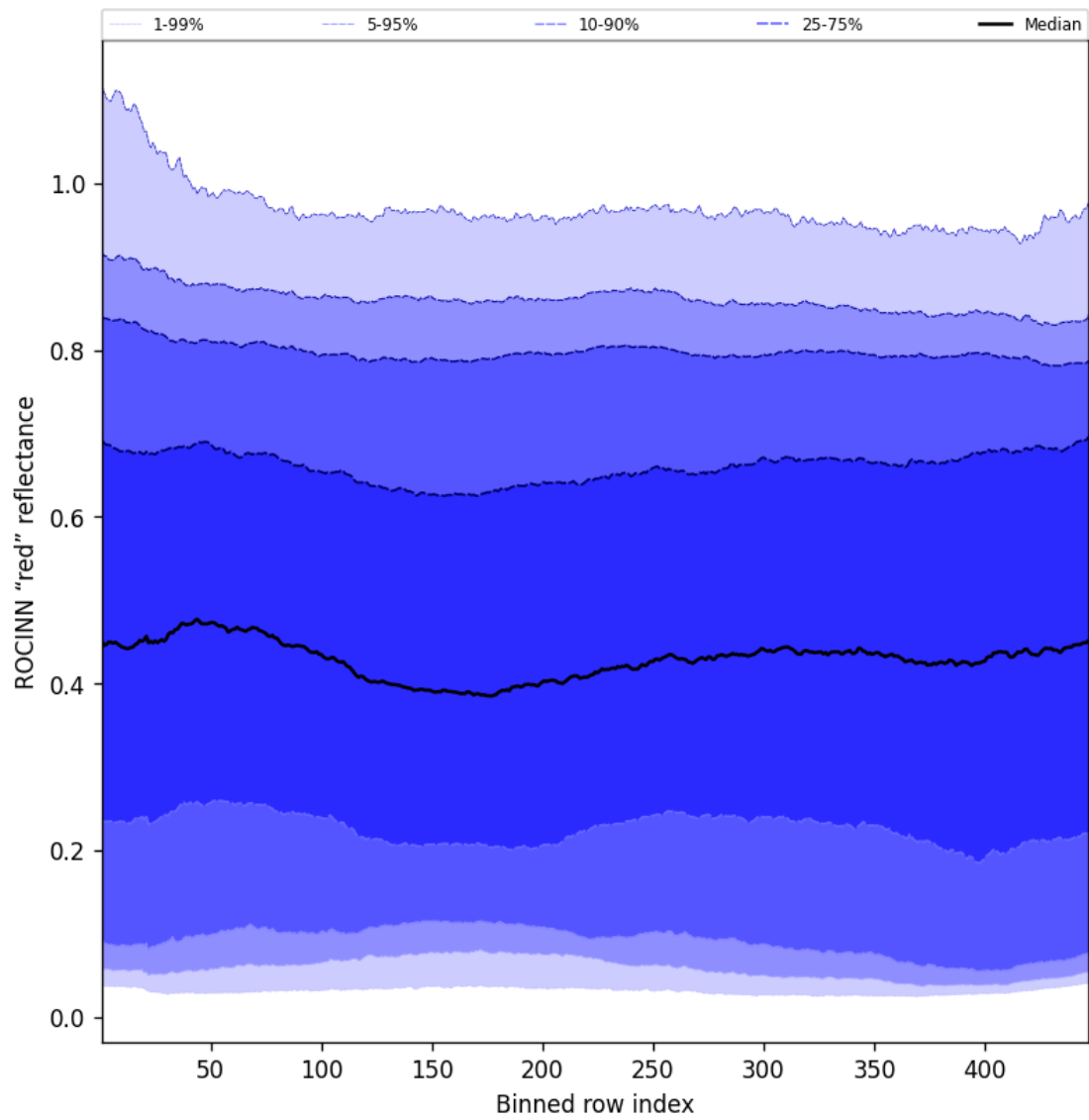
Figure 69: Along track statistics of “ROCINN “red” reflectance” for 2025-06-08 to 2025-06-10
