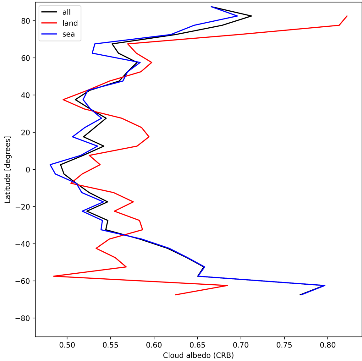
Figure 28: Zonal average of “Cloud albedo (CRB)” for 2025-06-08 to 2025-06-10.
