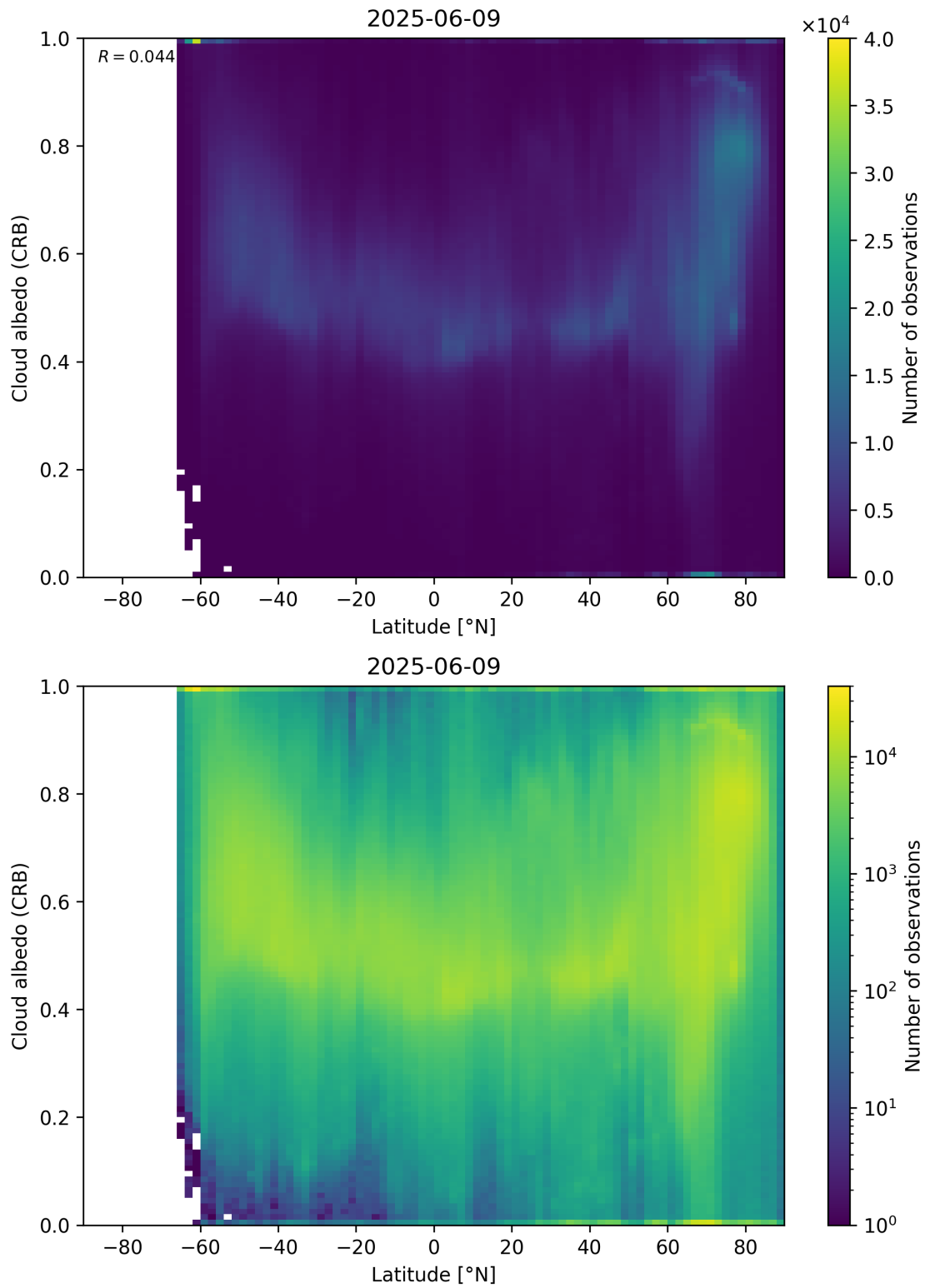
Figure 91: Scatter density plot of “Latitude” against “Cloud albedo (CRB)” for 2025-06-08 to 2025-06-10.
