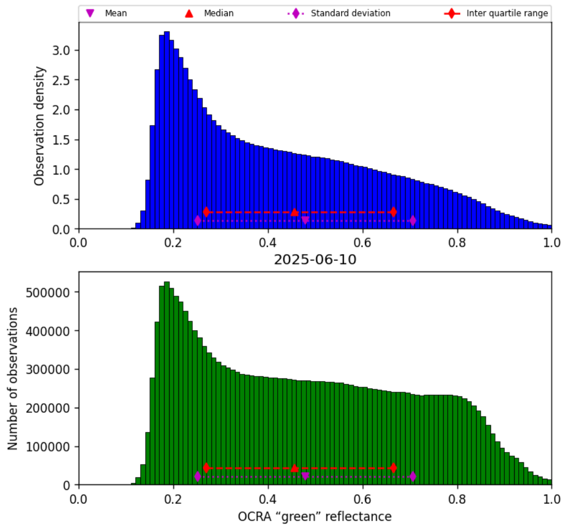
Figure 52: Histogram of “OCRA “green” reflectance” for 2025-06-09 to 2025-06-11
