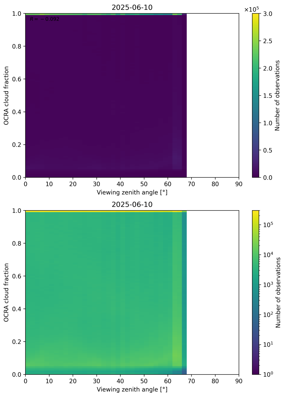
Figure 108: Scatter density plot of “Viewing zenith angle” against “OCRA cloud fraction” for 2025-06-09 to 2025-06-11.
