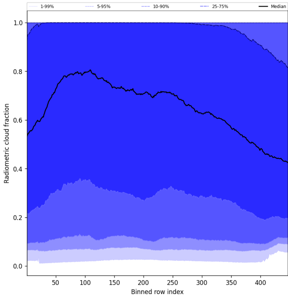
Figure 55: Along track statistics of “Radiometric cloud fraction” for 2025-06-09 to 2025-06-11
