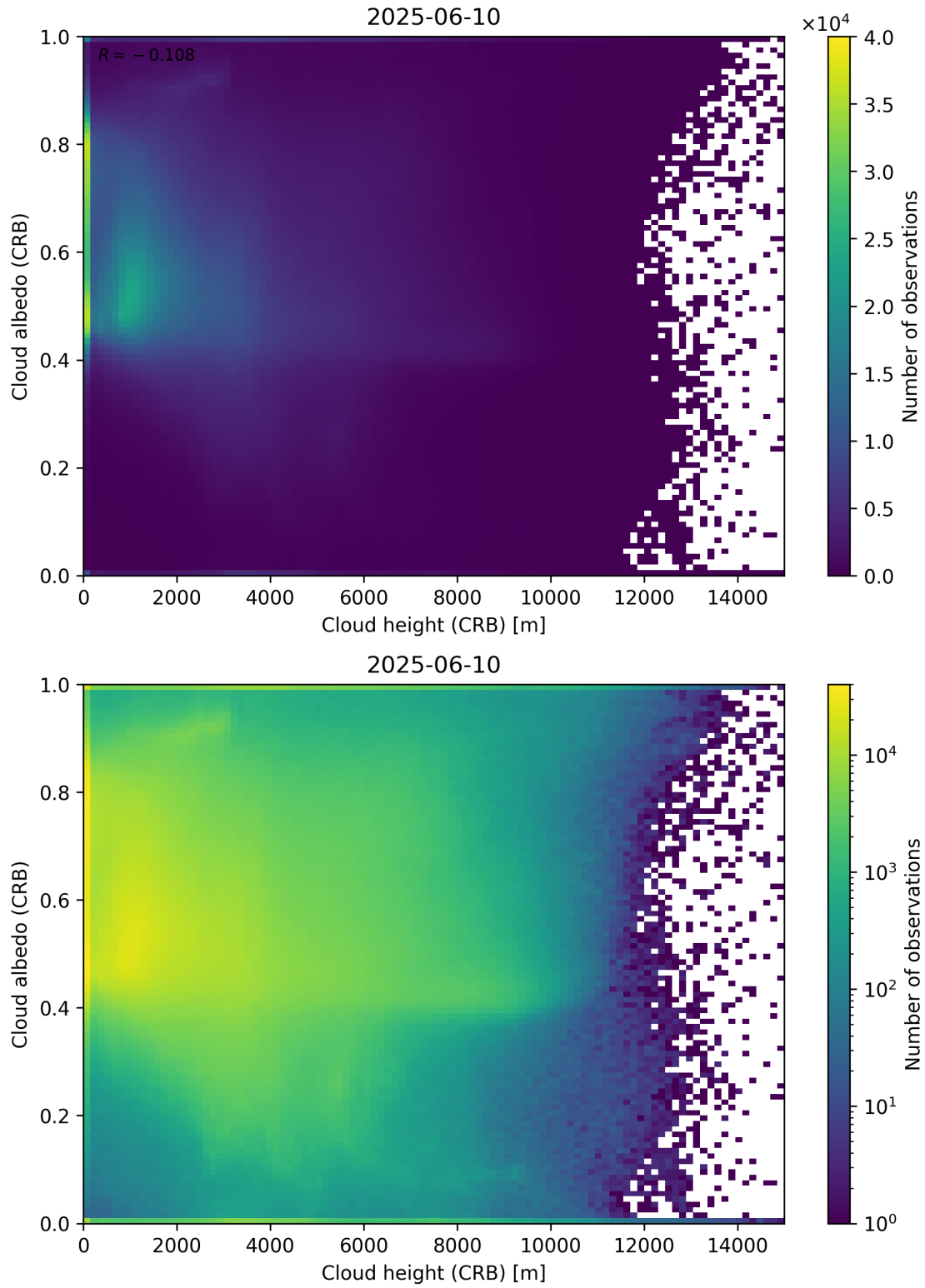
Figure 80: Scatter density plot of “Cloud height (CRB)” against “Cloud albedo (CRB)” for 2025-06-09 to 2025-06-11.
