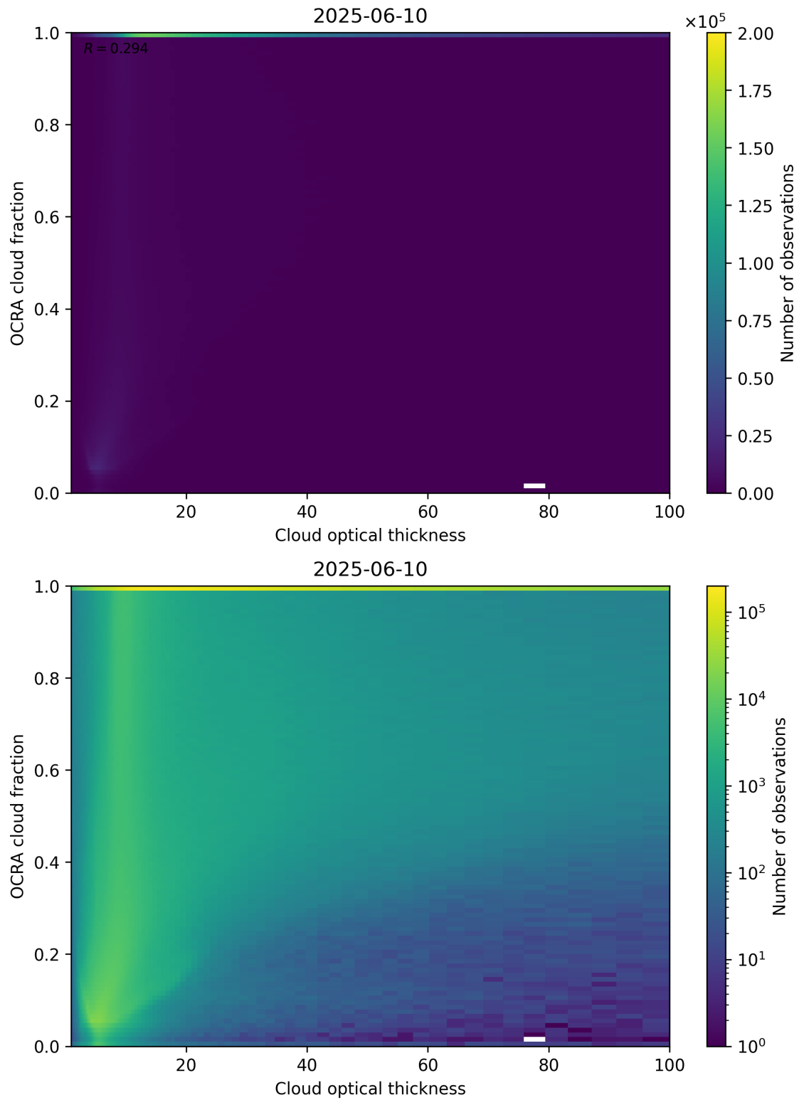
Figure 83: Scatter density plot of “Cloud optical thickness” against “OCRA cloud fraction” for 2025-06-09 to 2025-06-11.
