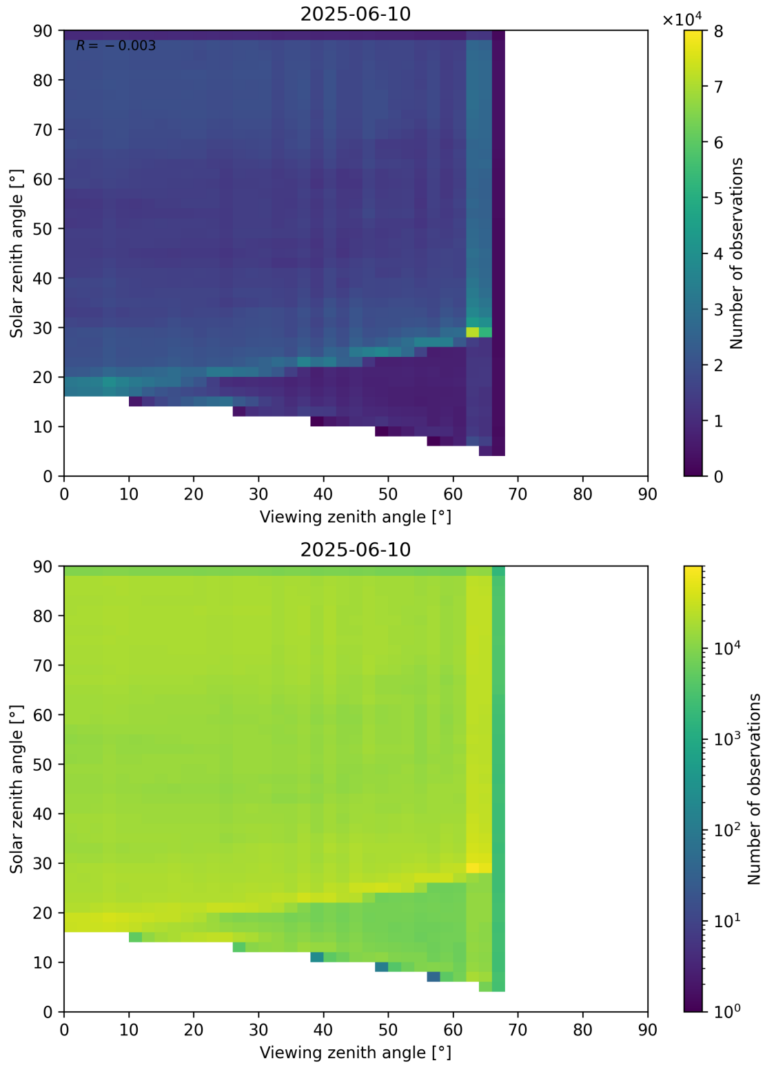
Figure 114: Scatter density plot of “Viewing zenith angle” against “Solar zenith angle” for 2025-06-09 to 2025-06-11.
