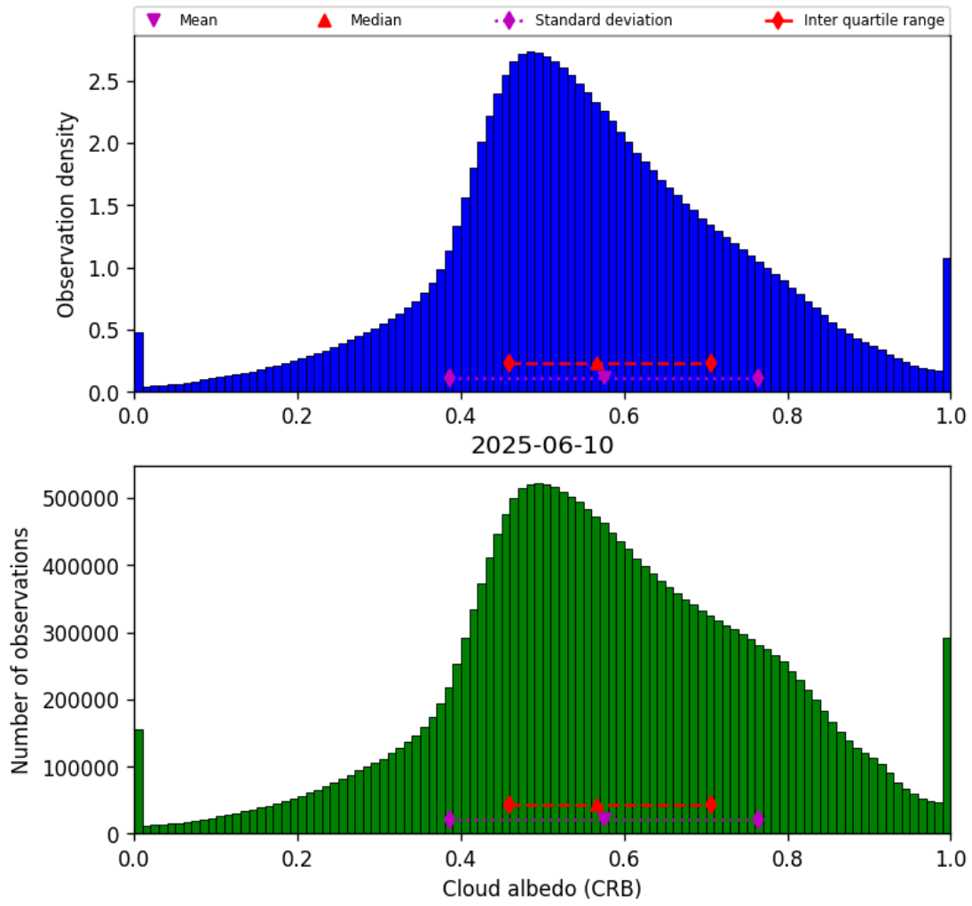
Figure 44: Histogram of “Cloud albedo (CRB)” for 2025-06-09 to 2025-06-11
