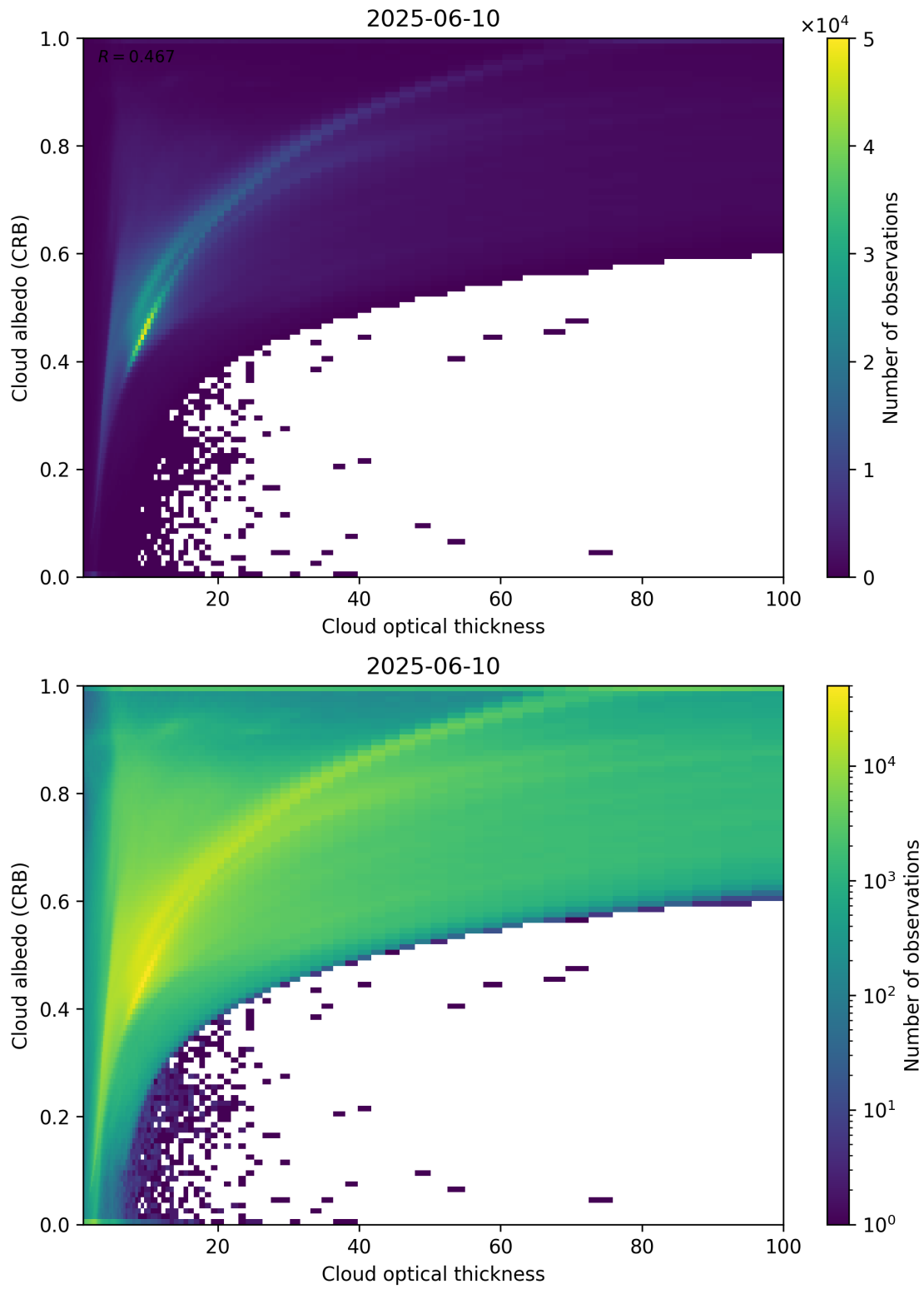
Figure 82: Scatter density plot of “Cloud optical thickness” against “Cloud albedo (CRB)” for 2025-06-09 to 2025-06-11.
