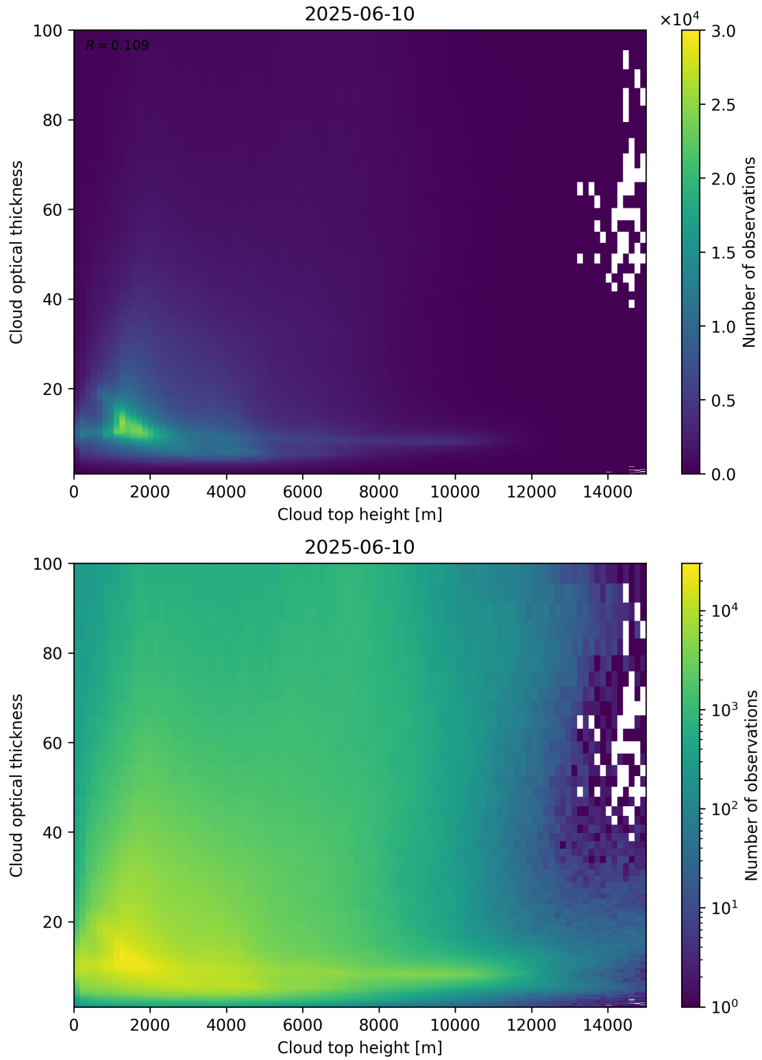
Figure 90: Scatter density plot of “Cloud top height” against “Cloud optical thickness” for 2025-06-09 to 2025-06-11.
