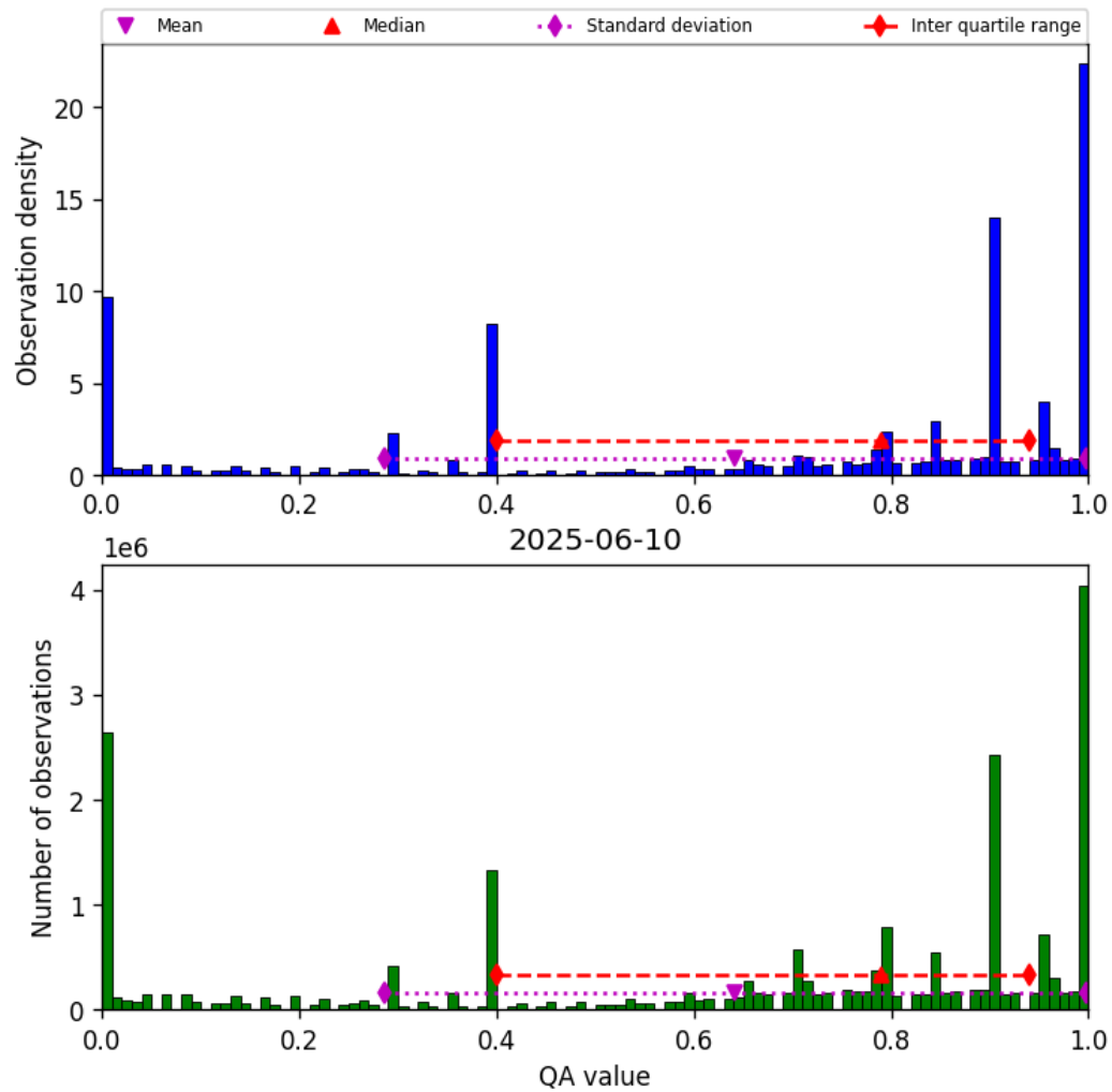
Figure 38: Histogram of “QA value” for 2025-06-09 to 2025-06-11
