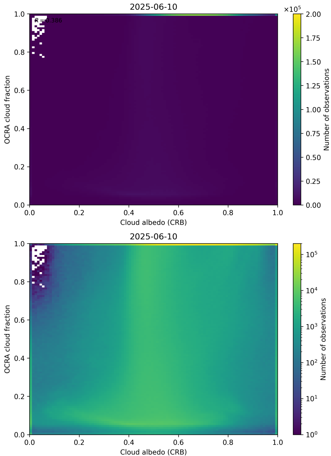
Figure 70: Scatter density plot of “Cloud albedo (CRB)” against “OCRA cloud fraction” for 2025-06-09 to 2025-06-11.
