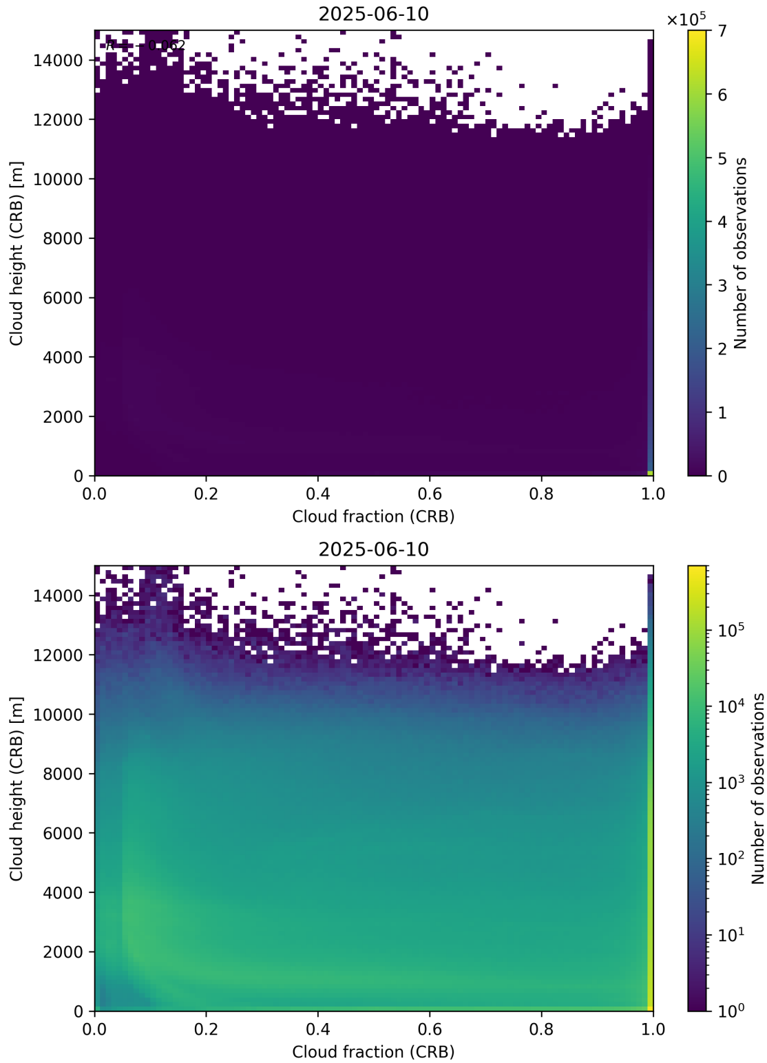
Figure 79: Scatter density plot of “Cloud fraction (CRB)” against “Cloud height (CRB)” for 2025-06-09 to 2025-06-11.
