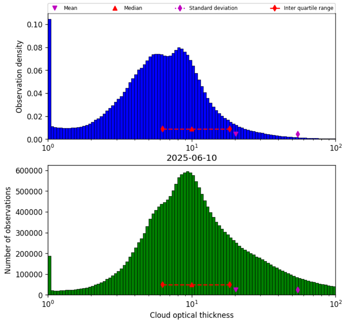
Figure 41: Histogram of “Cloud optical thickness” for 2025-06-09 to 2025-06-11
