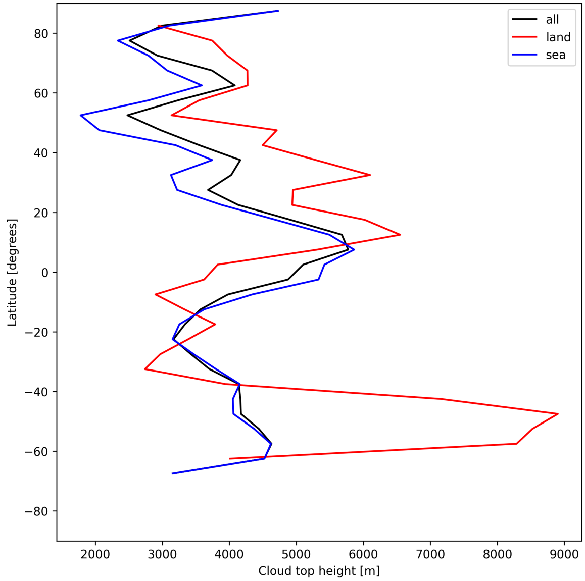
Figure 24: Zonal average of “Cloud top height” for 2025-06-09 to 2025-06-11.
