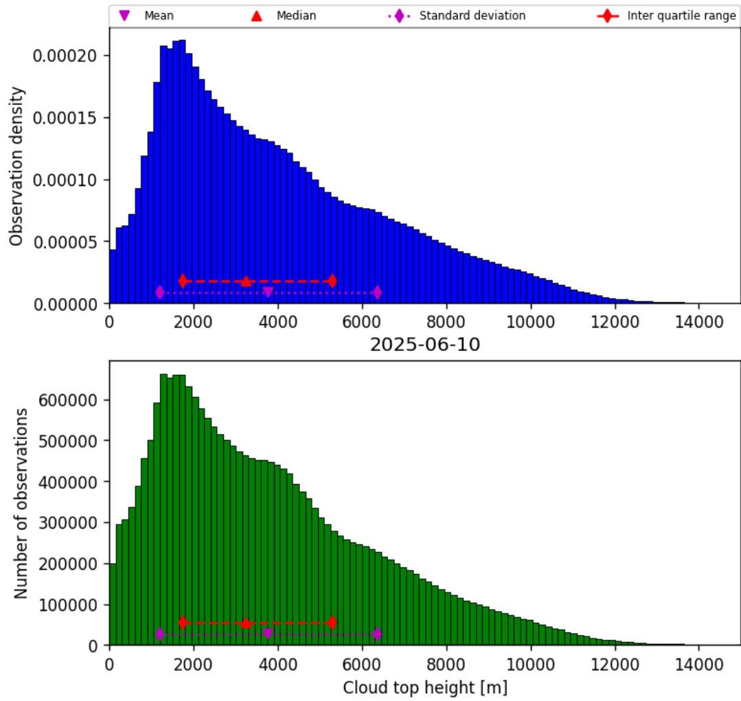
Figure 40: Histogram of “Cloud top height” for 2025-06-09 to 2025-06-11
