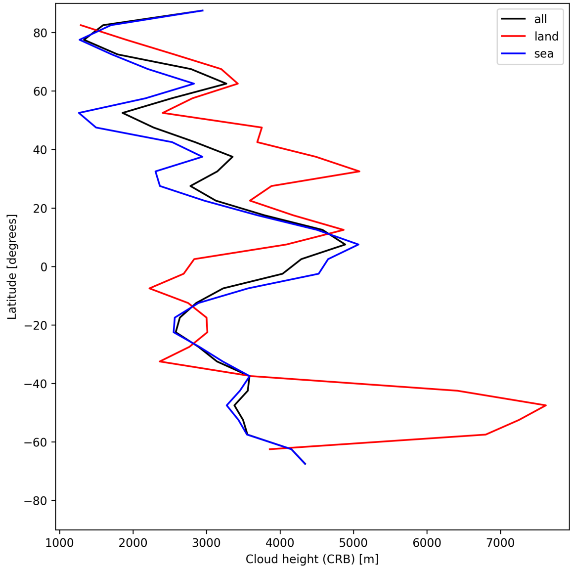
Figure 27: Zonal average of “Cloud height (CRB)” for 2025-06-09 to 2025-06-11.
