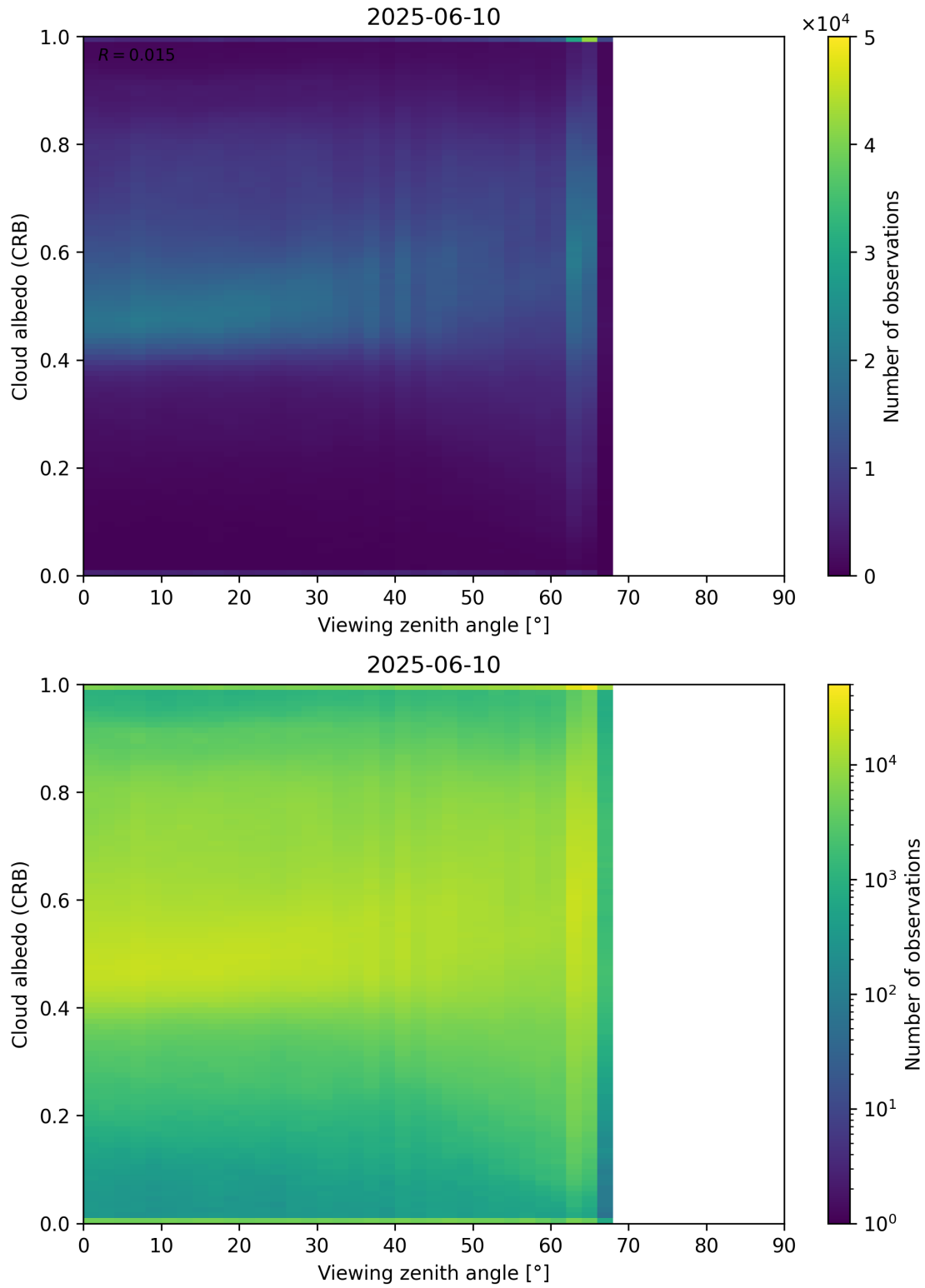
Figure 106: Scatter density plot of “Viewing zenith angle” against “Cloud albedo (CRB)” for 2025-06-09 to 2025-06-11.
