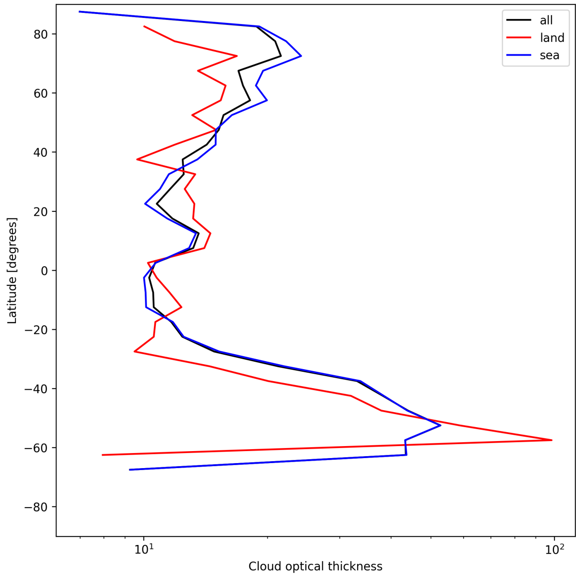
Figure 25: Zonal average of “Cloud optical thickness” for 2025-06-09 to 2025-06-11.
