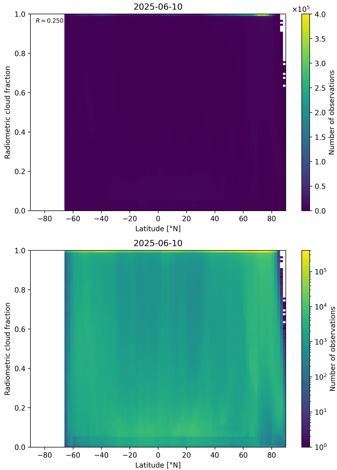
Figure 92: Scatter density plot of “Latitude” against “Radiometric cloud fraction” for 2025-06-09 to 2025-06-11.
