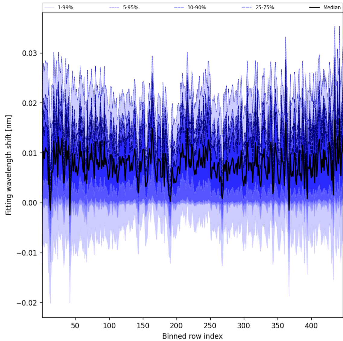
Figure 65: Along track statistics of “Fitting wavelength shift” for 2025-06-09 to 2025-06-11
