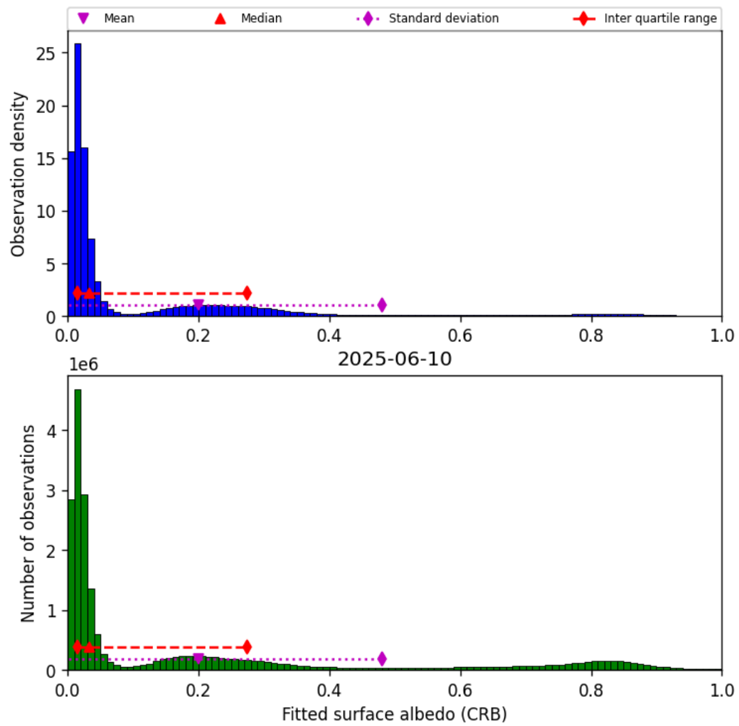
Figure 46: Histogram of “Fitted surface albedo (CRB)” for 2025-06-09 to 2025-06-11
