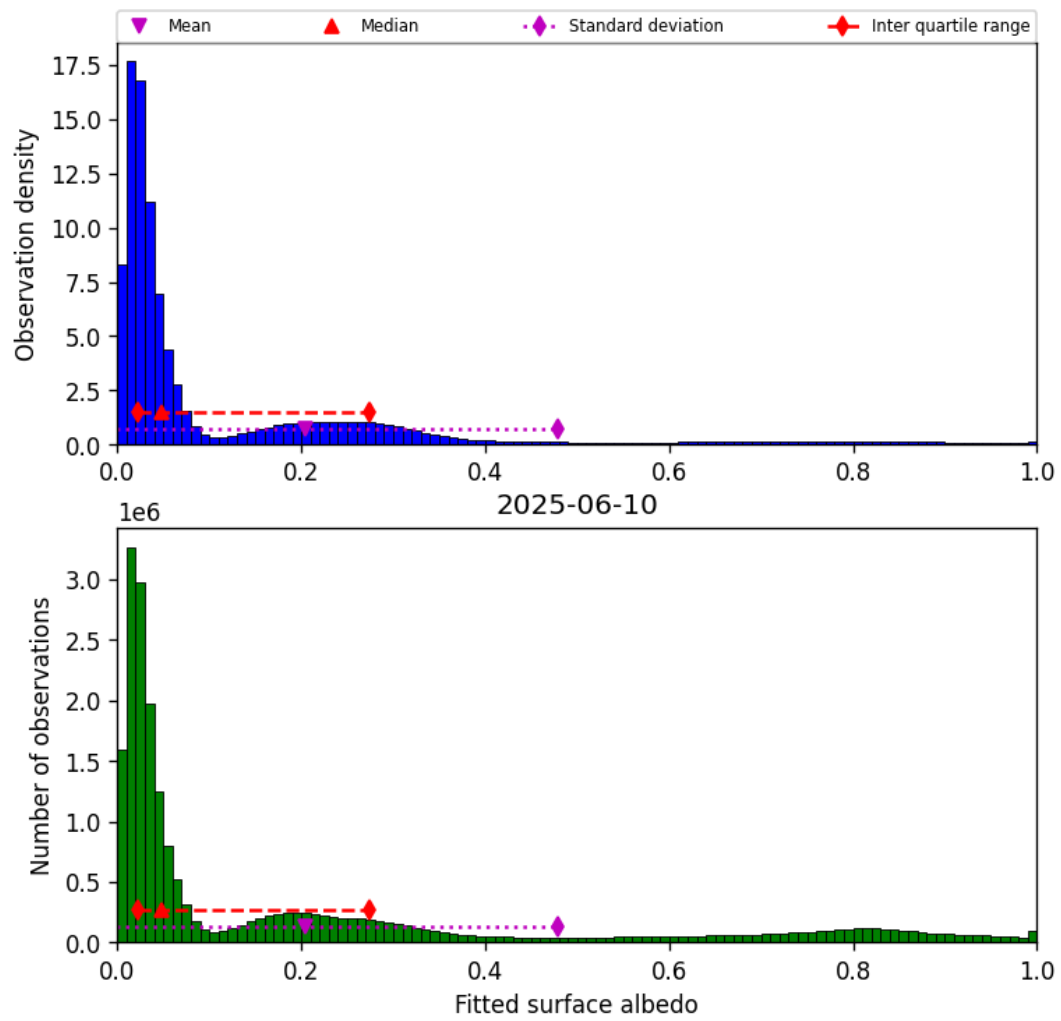
Figure 45: Histogram of “Fitted surface albedo” for 2025-06-09 to 2025-06-11
