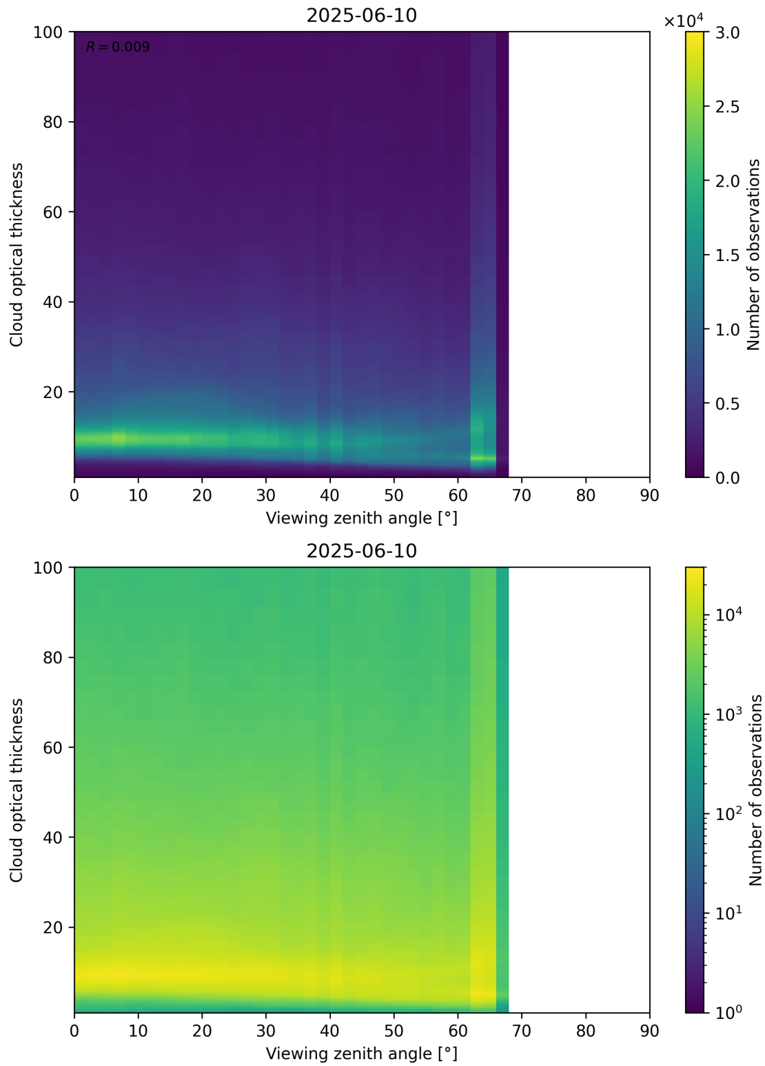
Figure 111: Scatter density plot of “Viewing zenith angle” against “Cloud optical thickness” for 2025-06-09 to 2025-06-11.
