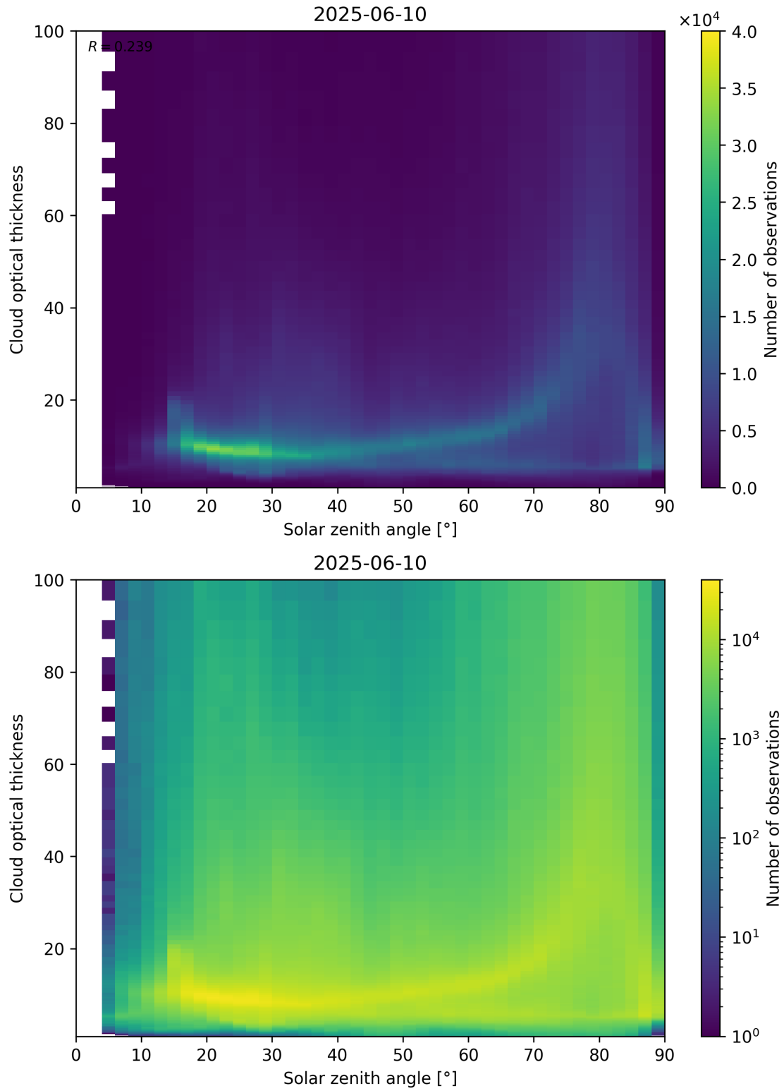
Figure 103: Scatter density plot of “Solar zenith angle” against “Cloud optical thickness” for 2025-06-09 to 2025-06-11.
