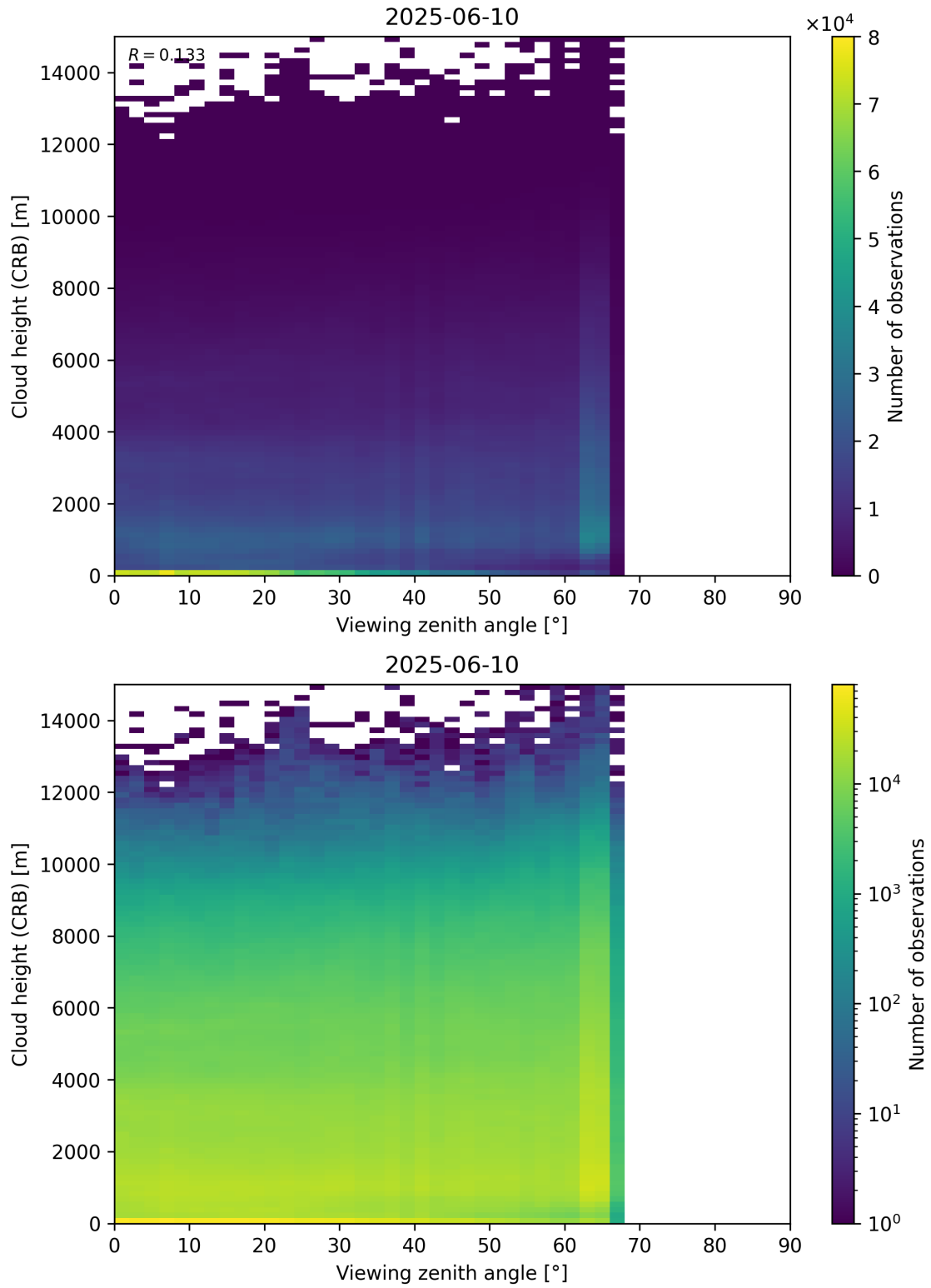
Figure 110: Scatter density plot of “Viewing zenith angle” against “Cloud height (CRB)” for 2025-06-09 to 2025-06-11.
