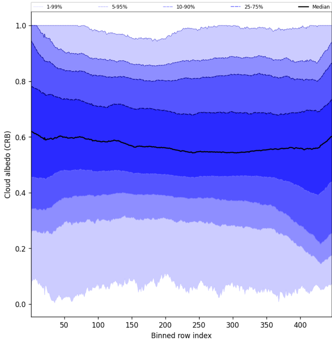
Figure 60: Along track statistics of “Cloud albedo (CRB)” for 2025-06-09 to 2025-06-11
