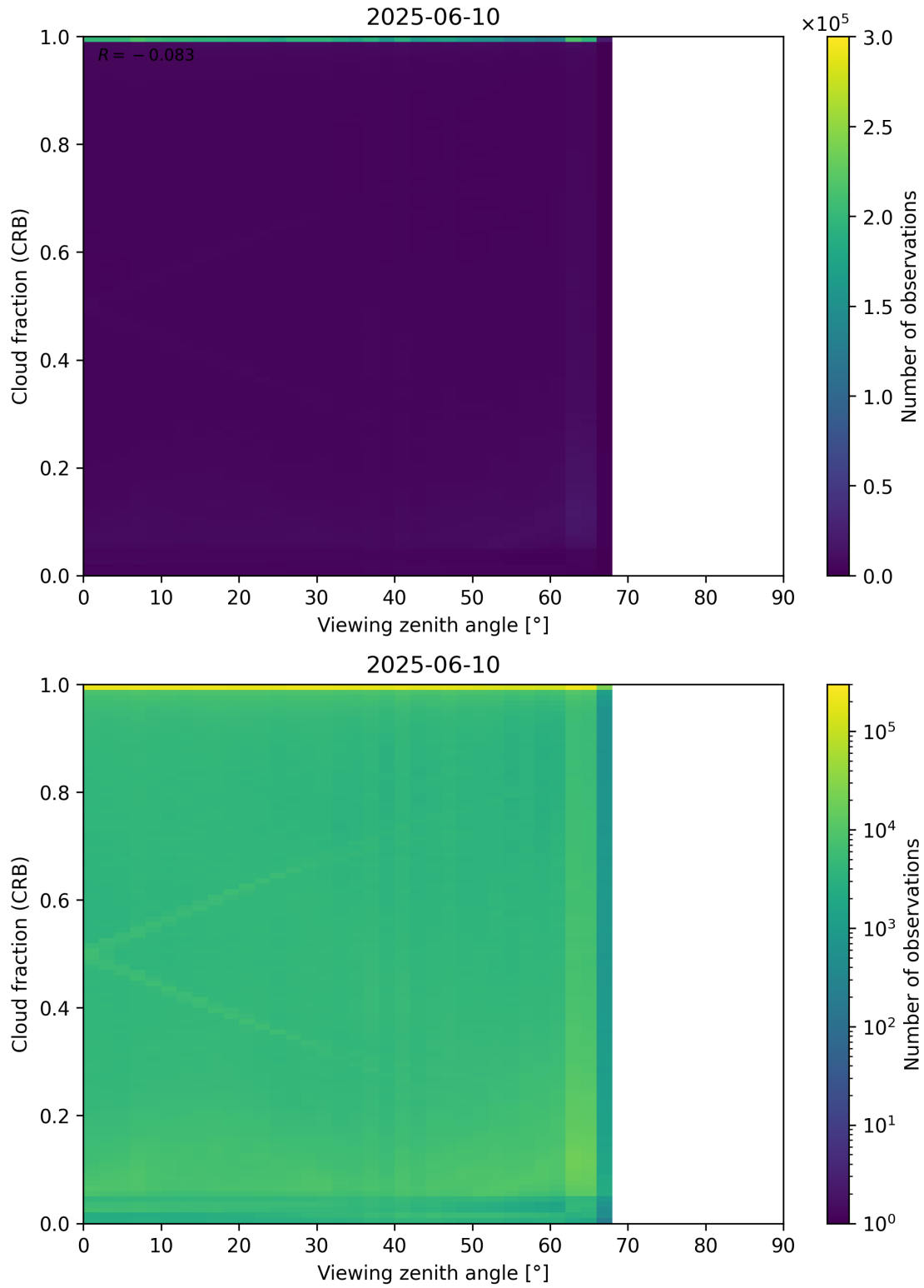
Figure 109: Scatter density plot of “Viewing zenith angle” against “Cloud fraction (CRB)” for 2025-06-09 to 2025-06-11.
