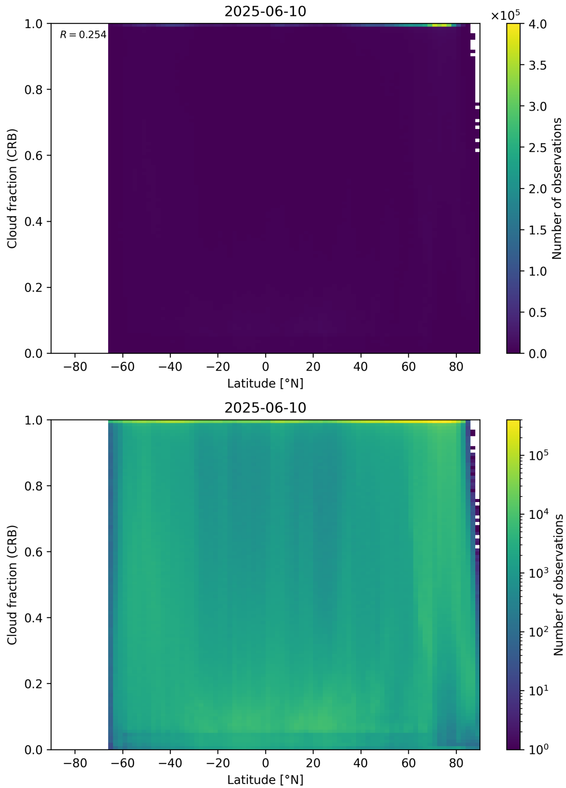
Figure 94: Scatter density plot of “Latitude” against “Cloud fraction (CRB)” for 2025-06-09 to 2025-06-11.
