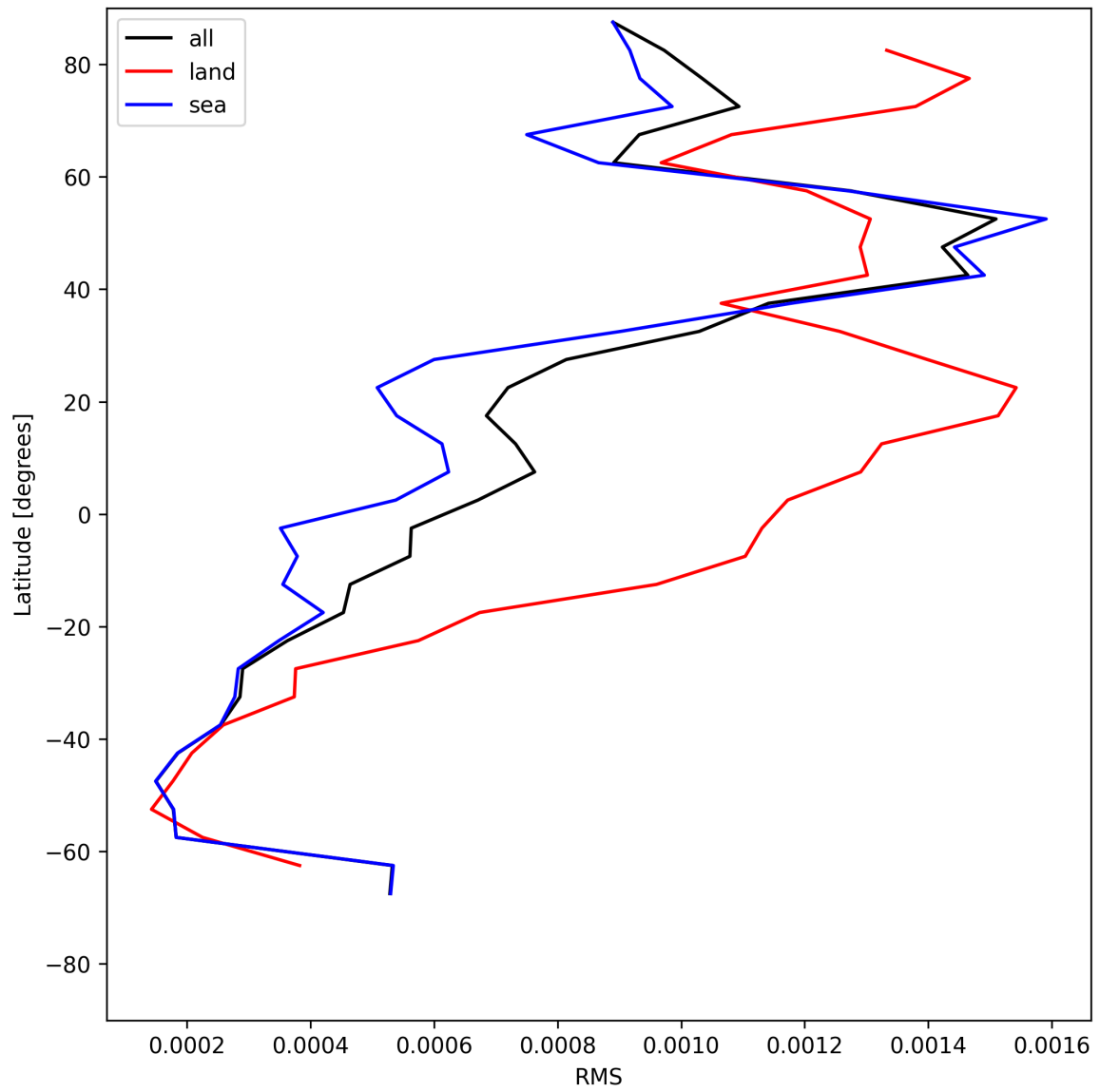
Figure 31: Zonal average of “RMS” for 2025-06-09 to 2025-06-11.
