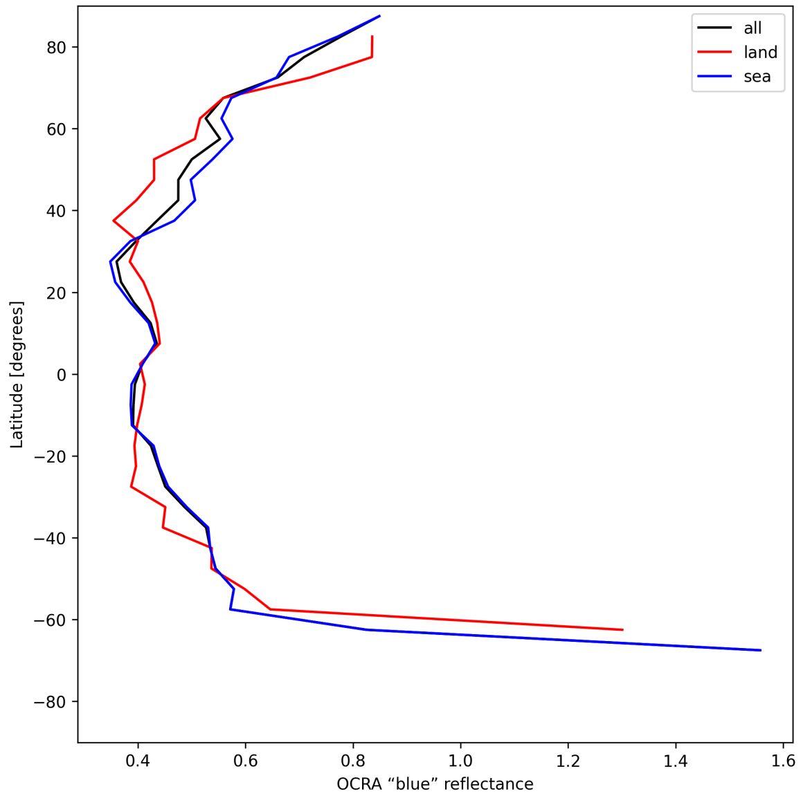
Figure 35: Zonal average of “OCRA “blue” reflectance” for 2025-06-09 to 2025-06-11.
