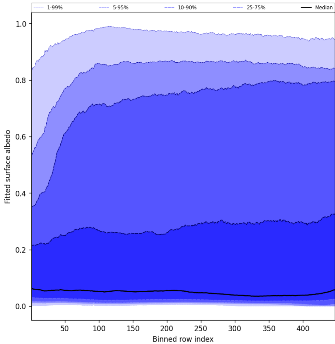
Figure 61: Along track statistics of “Fitted surface albedo” for 2025-06-09 to 2025-06-11
