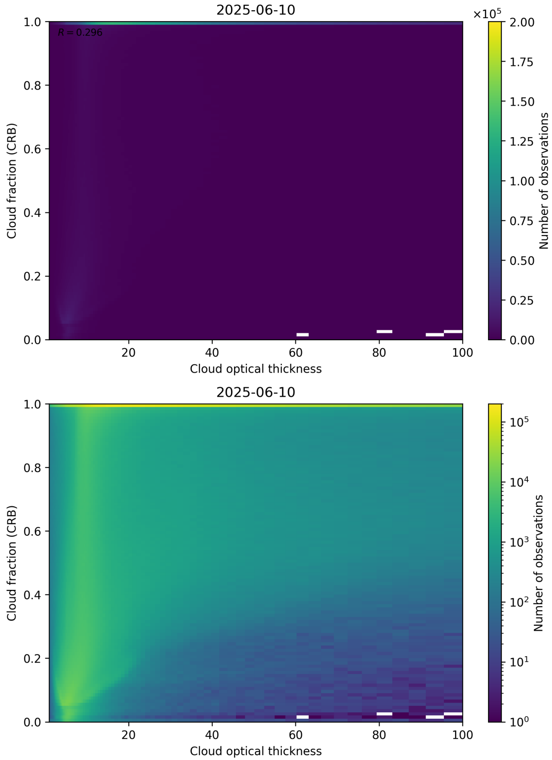
Figure 84: Scatter density plot of “Cloud optical thickness” against “Cloud fraction (CRB)” for 2025-06-09 to 2025-06-11.
