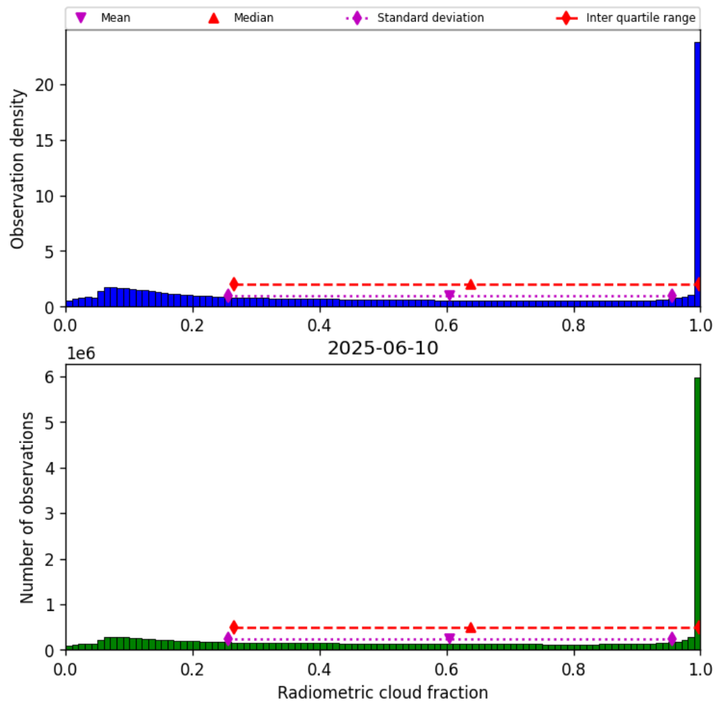
Figure 39: Histogram of “Radiometric cloud fraction” for 2025-06-09 to 2025-06-11
