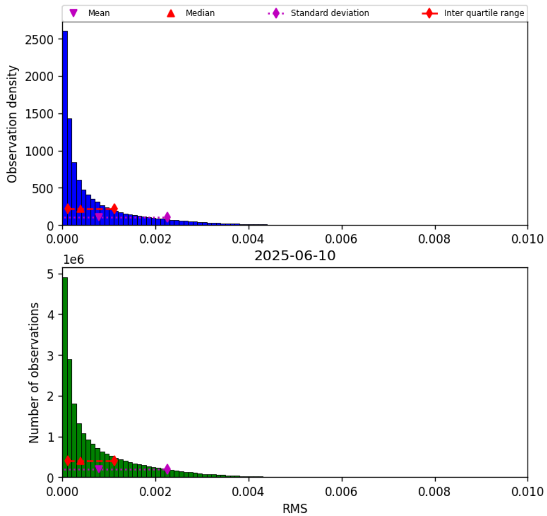
Figure 47: Histogram of “RMS” for 2025-06-09 to 2025-06-11
