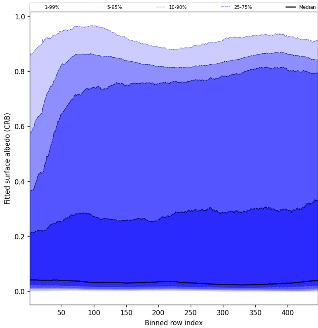
Figure 62: Along track statistics of “Fitted surface albedo (CRB)” for 2025-06-09 to 2025-06-11
