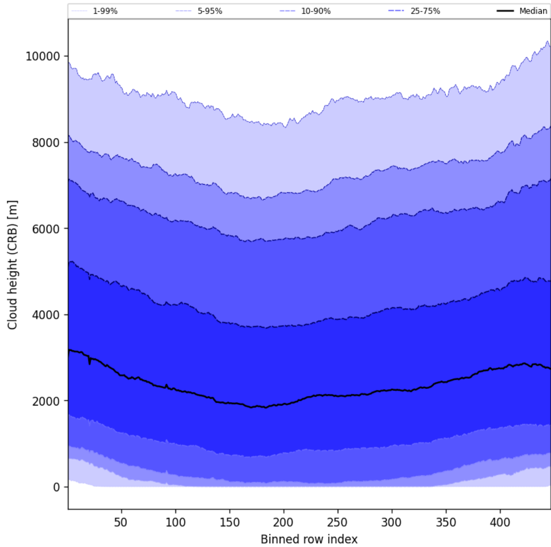
Figure 59: Along track statistics of “Cloud height (CRB)” for 2025-06-09 to 2025-06-11
