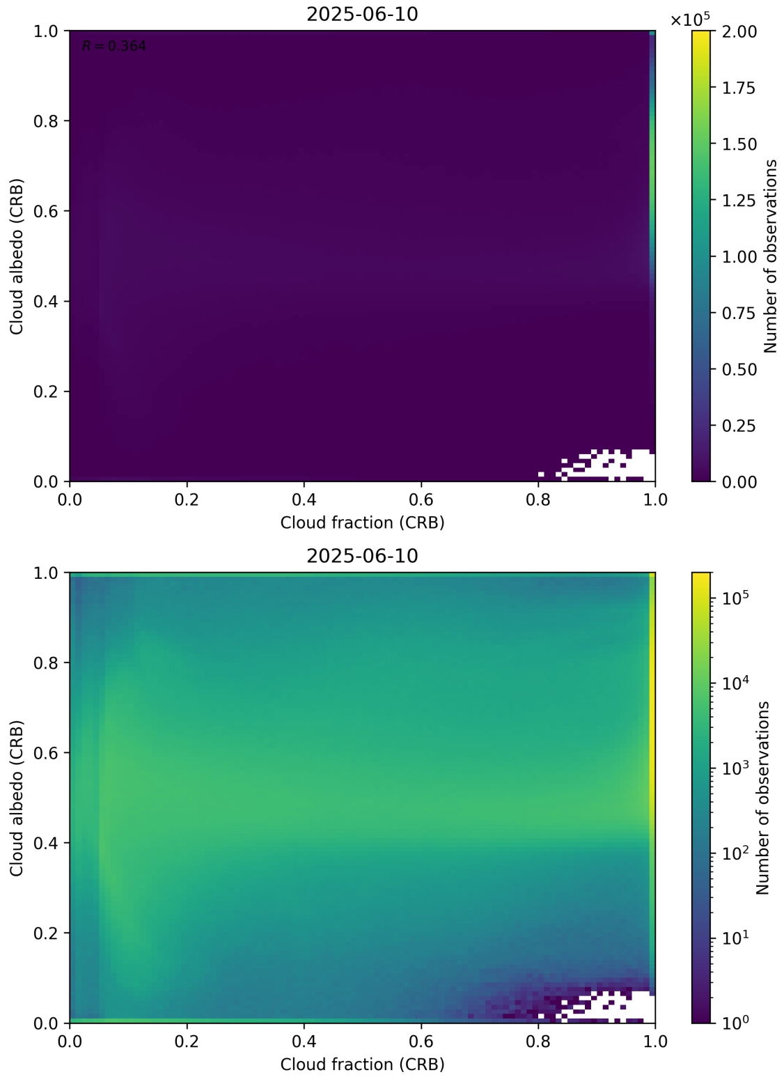
Figure 77: Scatter density plot of “Cloud fraction (CRB)” against “Cloud albedo (CRB)” for 2025-06-09 to 2025-06-11.
