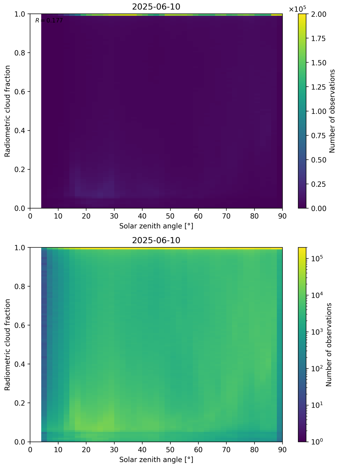
Figure 99: Scatter density plot of “Solar zenith angle” against “Radiometric cloud fraction” for 2025-06-09 to 2025-06-11.
