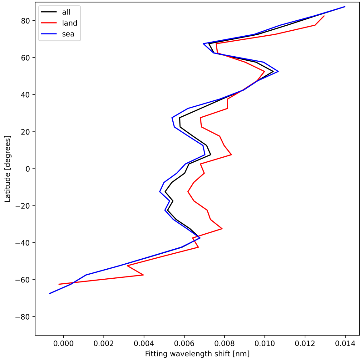
Figure 33: Zonal average of “Fitting wavelength shift” for 2025-06-09 to 2025-06-11.
