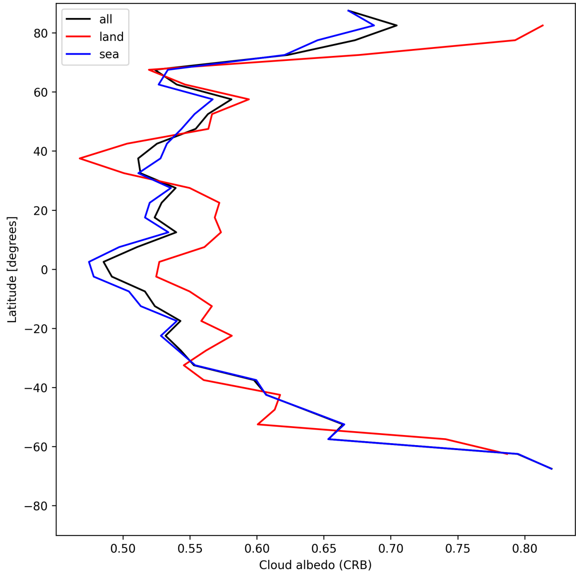
Figure 28: Zonal average of “Cloud albedo (CRB)” for 2025-06-09 to 2025-06-11.
