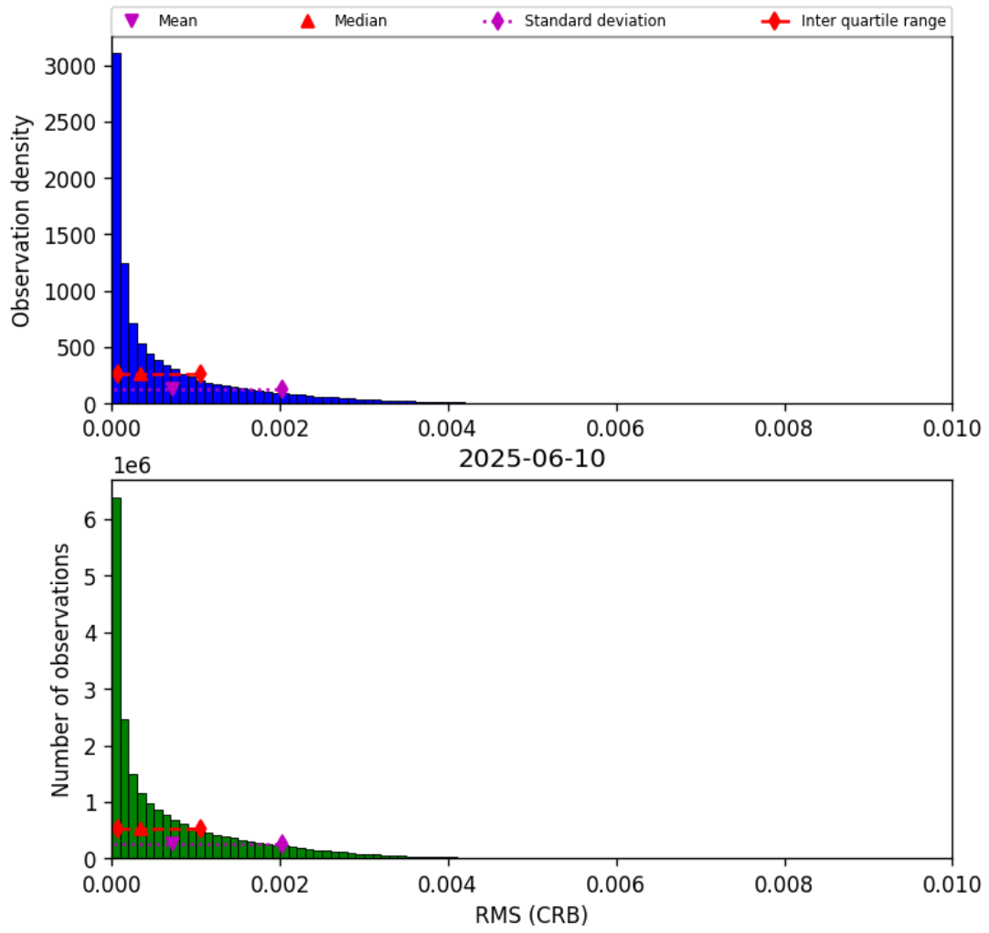
Figure 48: Histogram of “RMS (CRB)” for 2025-06-09 to 2025-06-11
