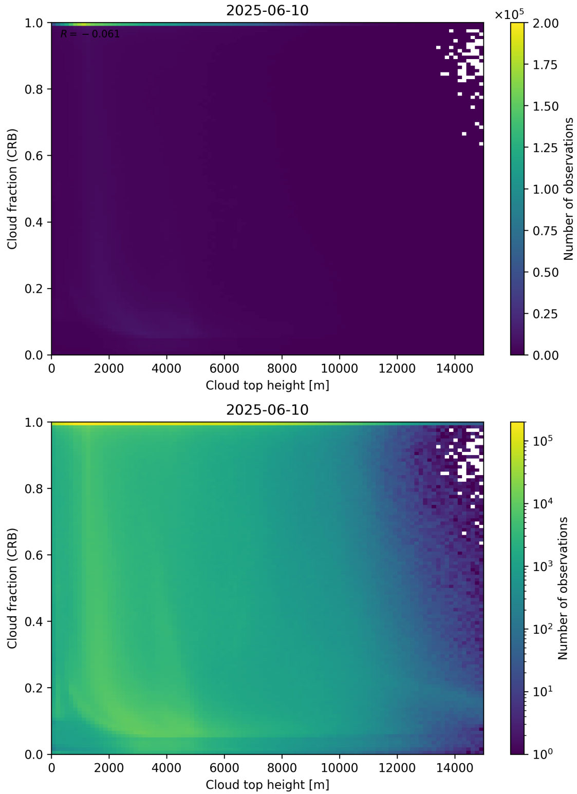
Figure 88: Scatter density plot of “Cloud top height” against “Cloud fraction (CRB)” for 2025-06-09 to 2025-06-11.
