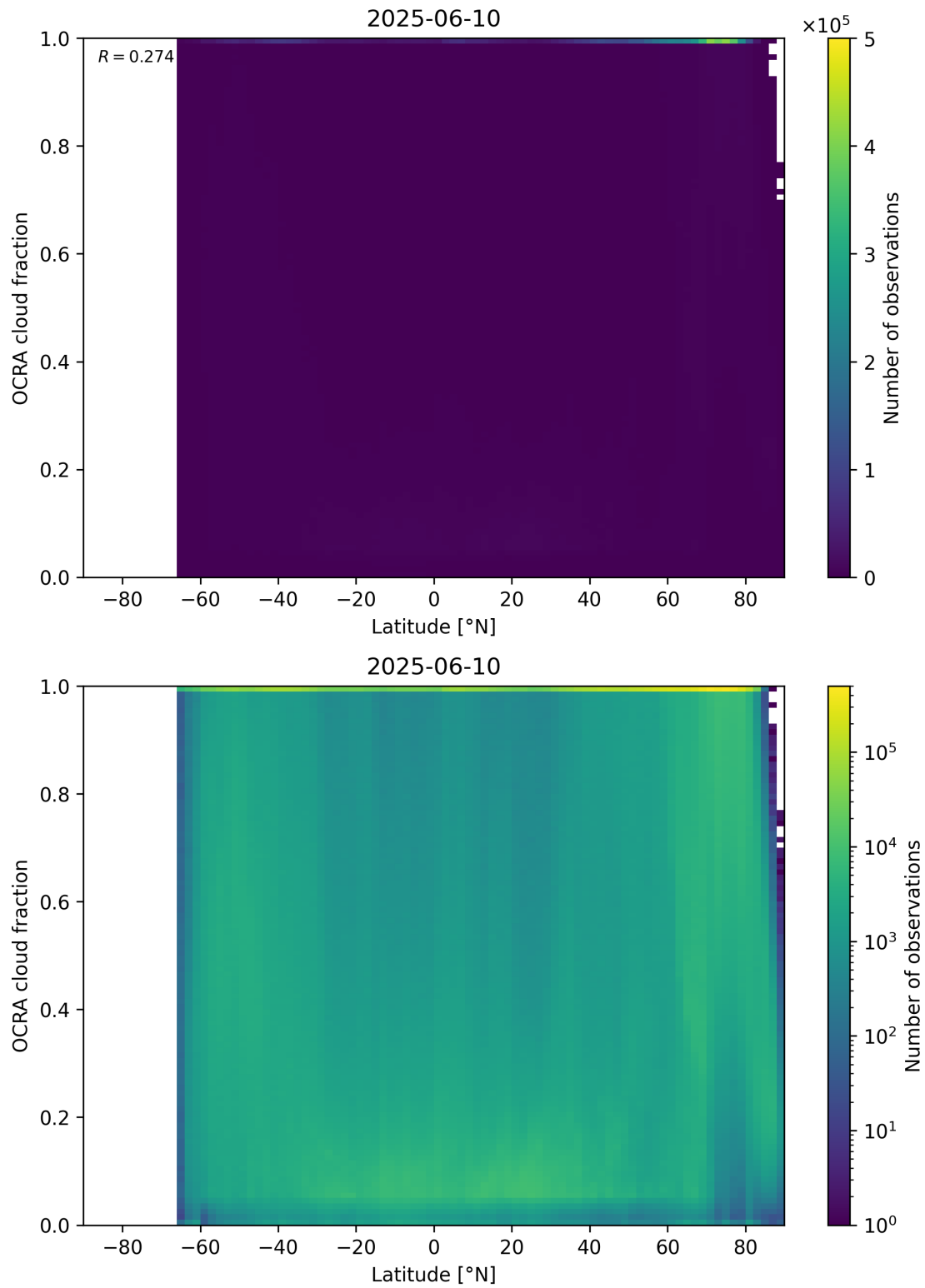
Figure 93: Scatter density plot of “Latitude” against “OCRA cloud fraction” for 2025-06-09 to 2025-06-11.
