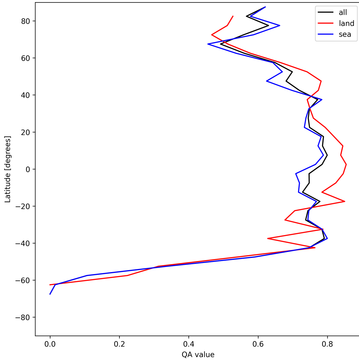
Figure 22: Zonal average of “QA value” for 2025-06-09 to 2025-06-11.
