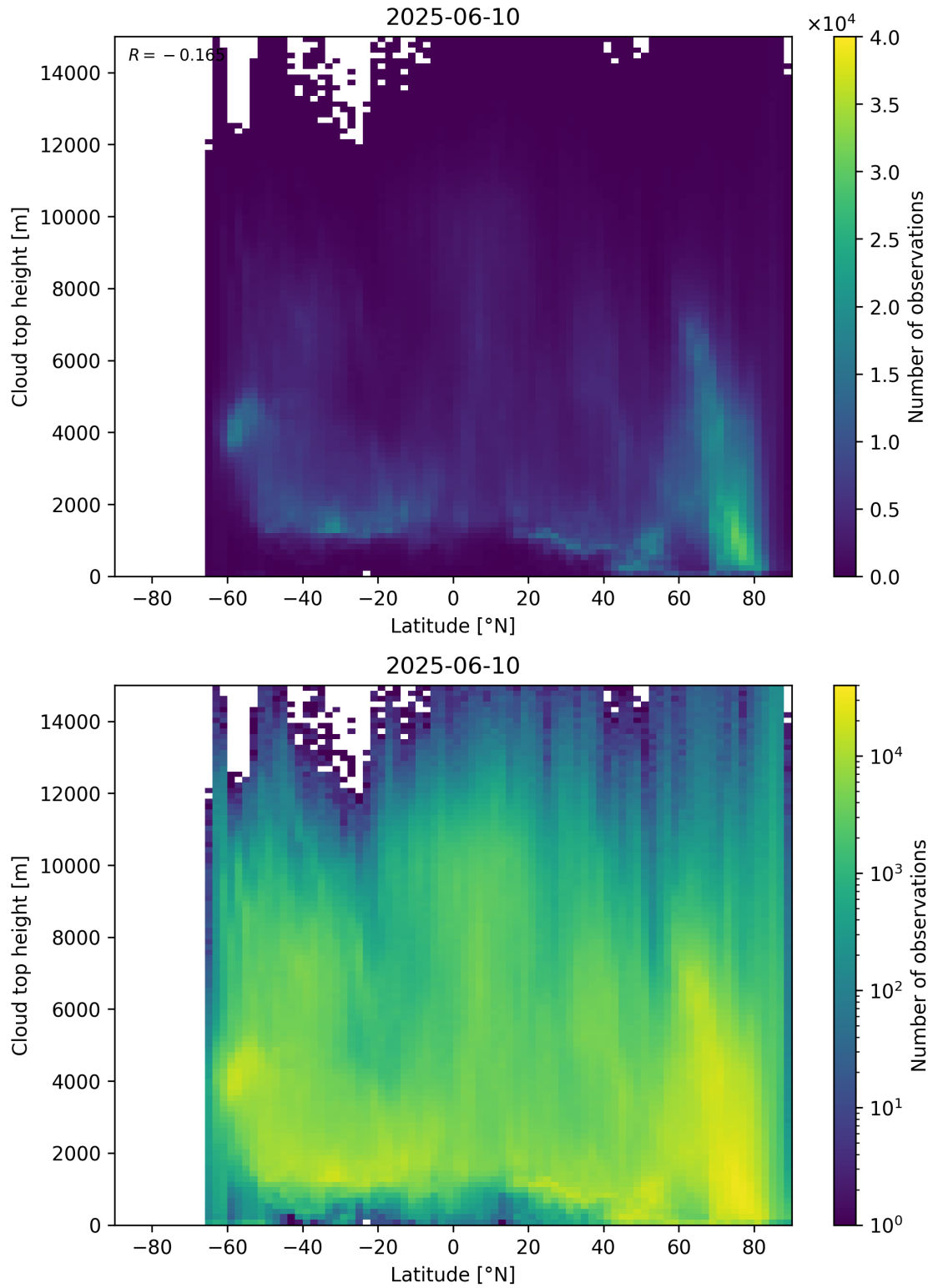
Figure 97: Scatter density plot of “Latitude” against “Cloud top height” for 2025-06-09 to 2025-06-11.
