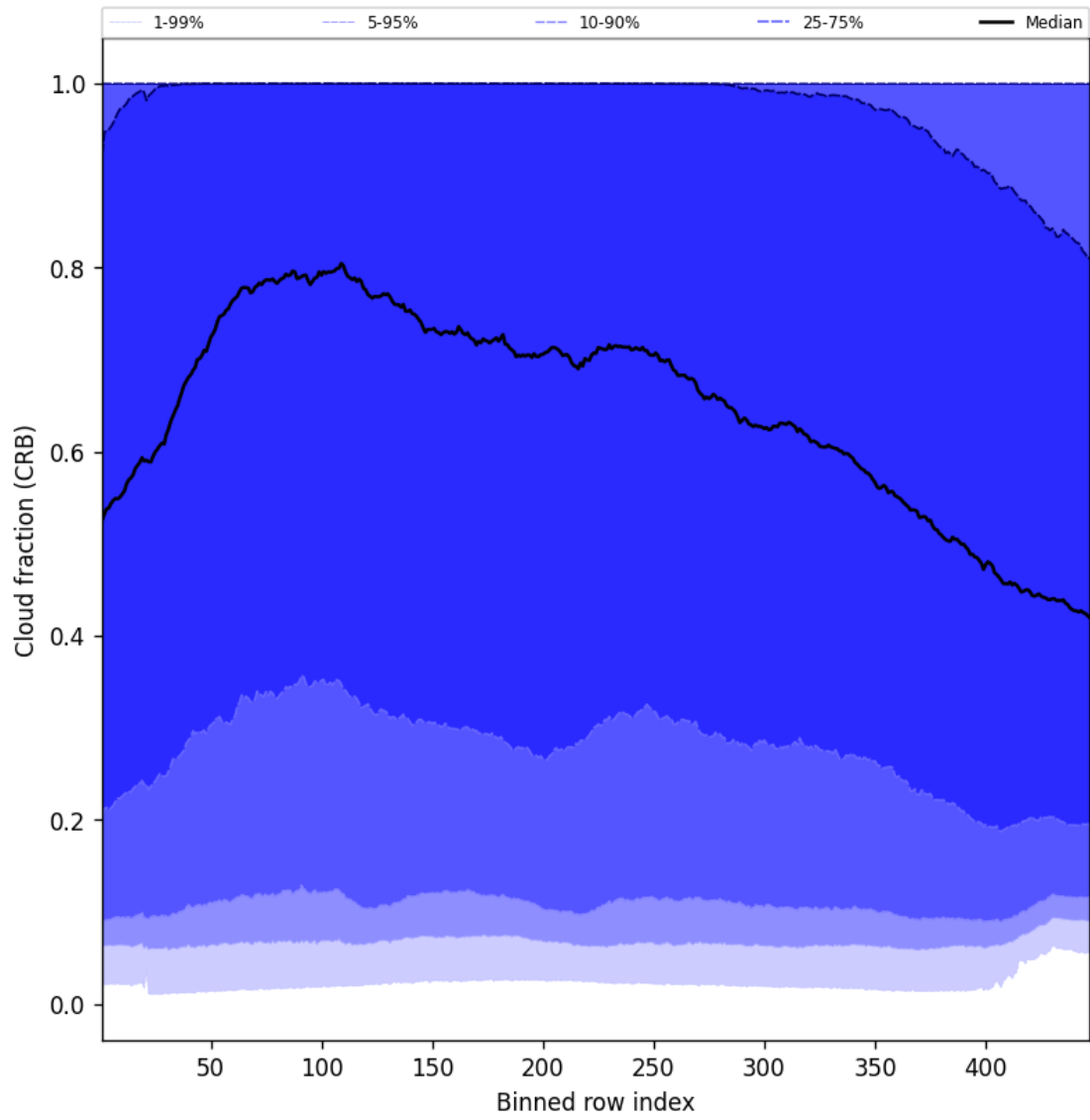
Figure 58: Along track statistics of “Cloud fraction (CRB)” for 2025-06-09 to 2025-06-11
