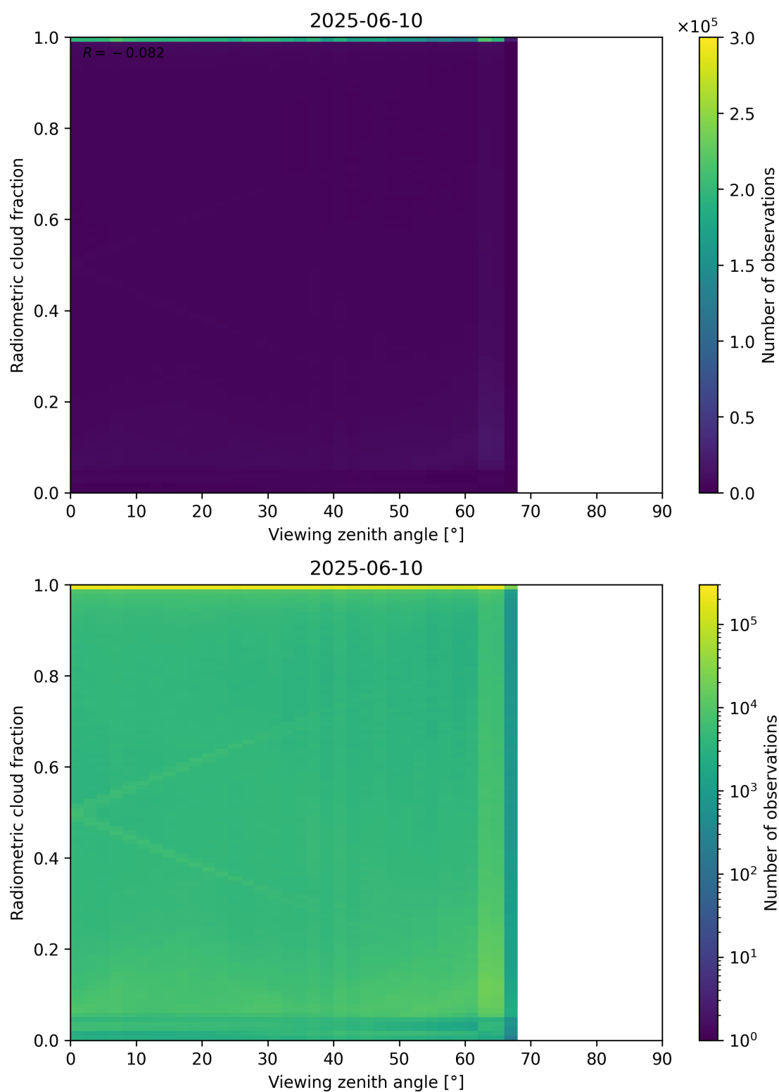
Figure 107: Scatter density plot of “Viewing zenith angle” against “Radiometric cloud fraction” for 2025-06-09 to 2025-06-11.
