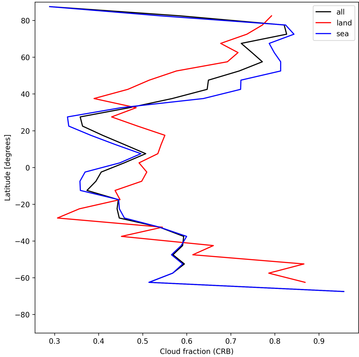
Figure 26: Zonal average of “Cloud fraction (CRB)” for 2025-06-09 to 2025-06-11.
