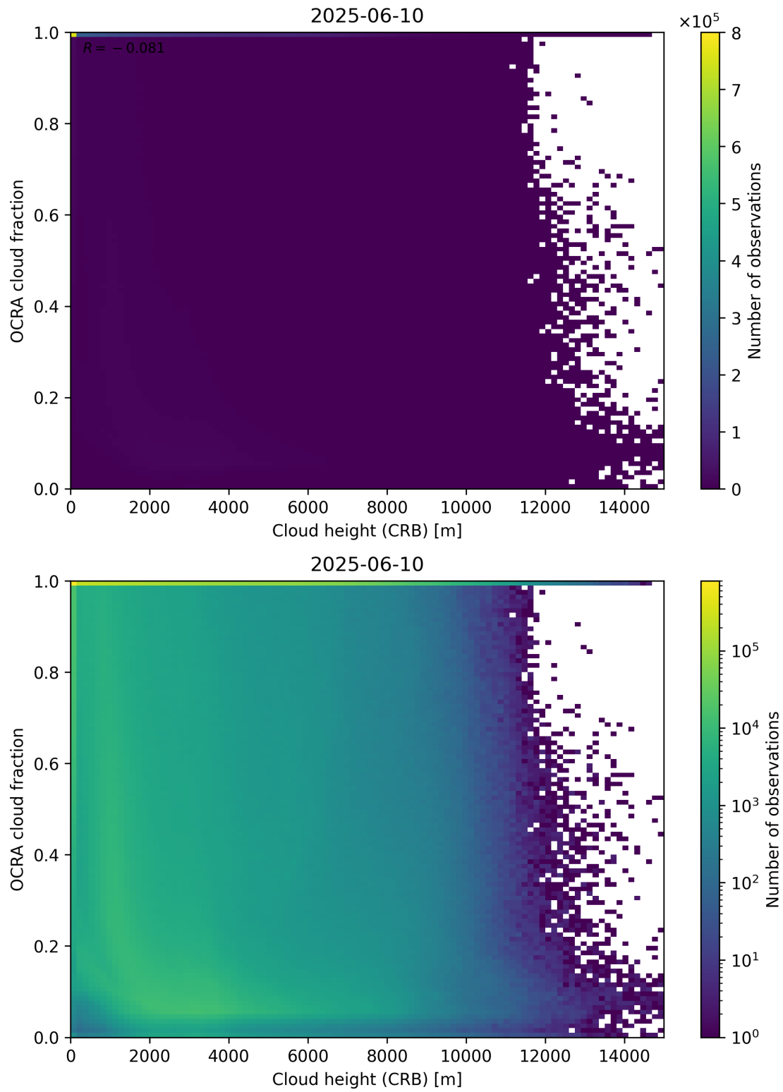
Figure 81: Scatter density plot of “Cloud height (CRB)” against “OCRA cloud fraction” for 2025-06-09 to 2025-06-11.
