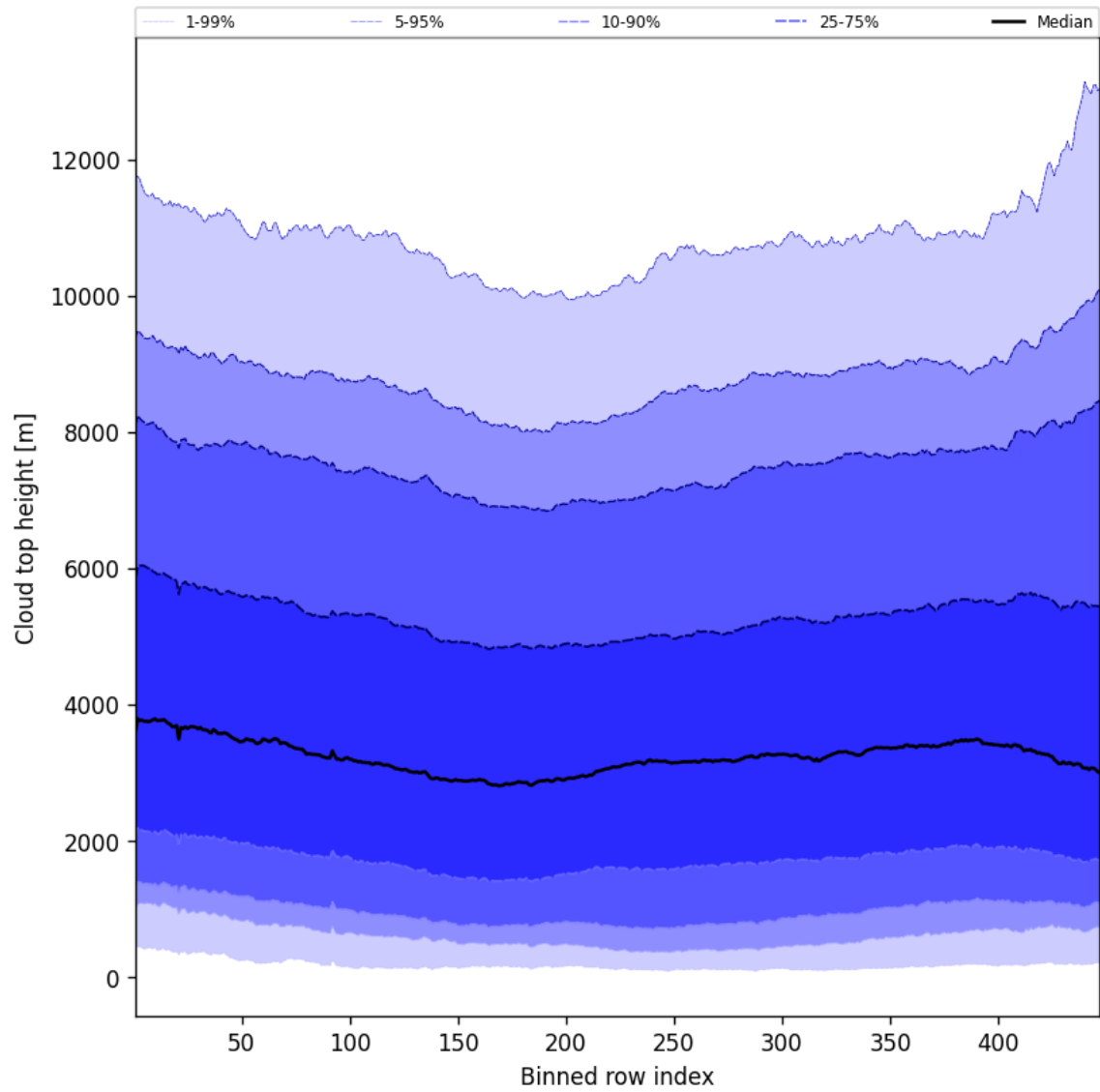
Figure 56: Along track statistics of “Cloud top height” for 2025-06-09 to 2025-06-11
