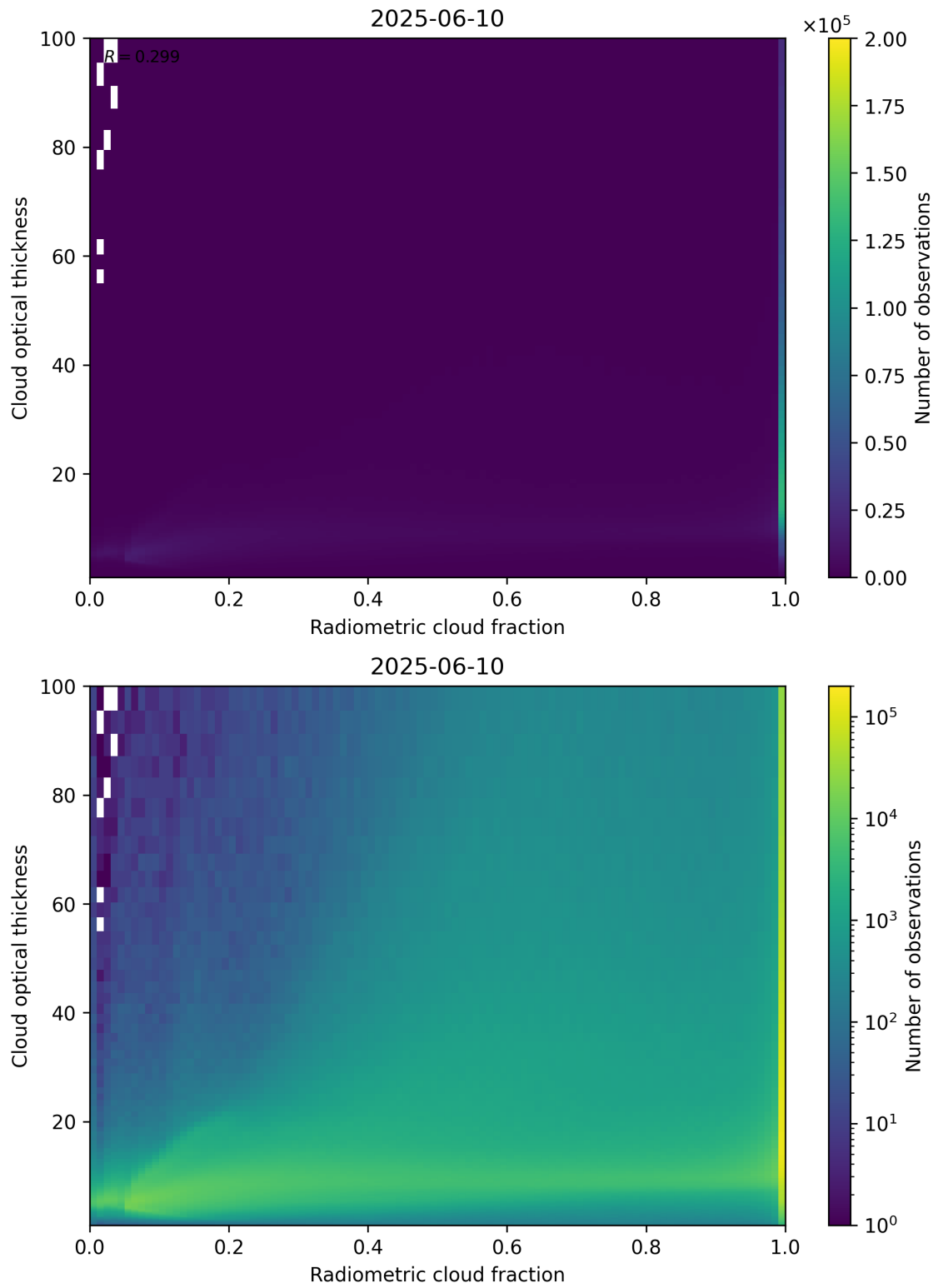
Figure 75: Scatter density plot of “Radiometric cloud fraction” against “Cloud optical thickness” for 2025-06-09 to 2025-06-11.
