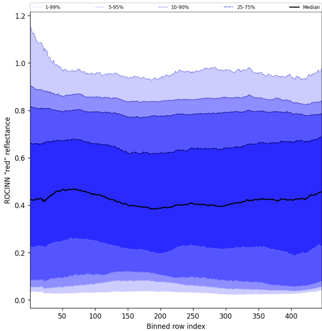
Figure 69: Along track statistics of “ROCINN “red” reflectance” for 2025-06-09 to 2025-06-11
