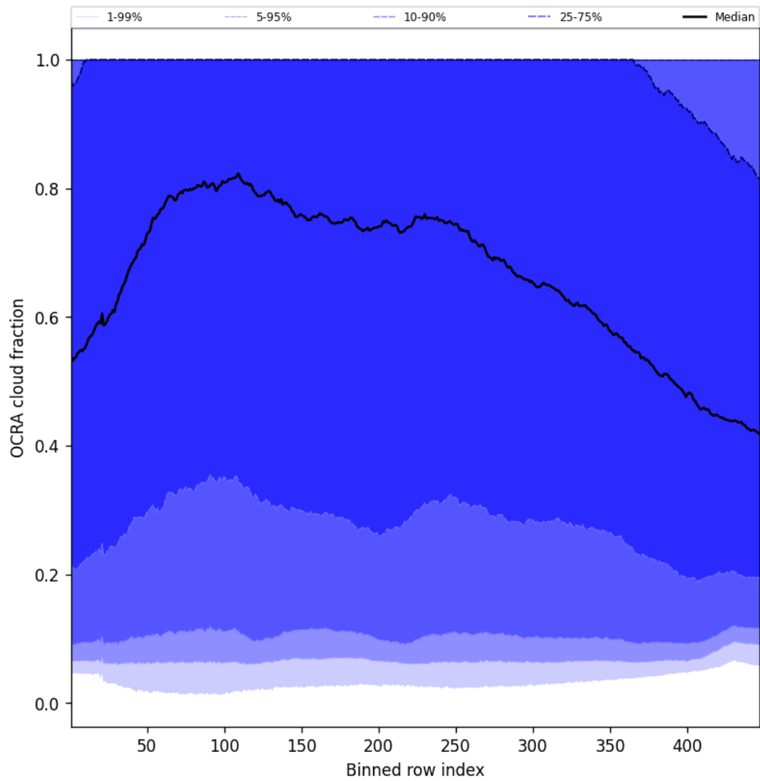
Figure 66: Along track statistics of “OCRA cloud fraction” for 2025-06-09 to 2025-06-11
