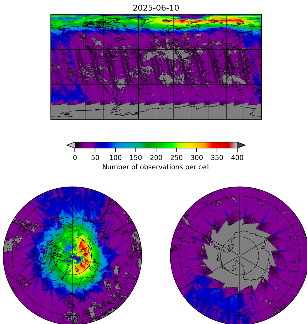
Figure 21: Map of the number of observations for 2025-06-09 to 2025-06-11
