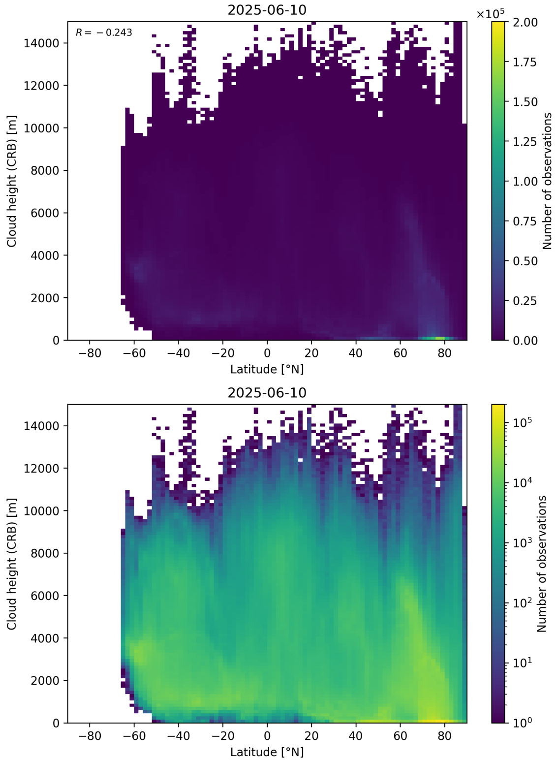
Figure 95: Scatter density plot of “Latitude” against “Cloud height (CRB)” for 2025-06-09 to 2025-06-11.
