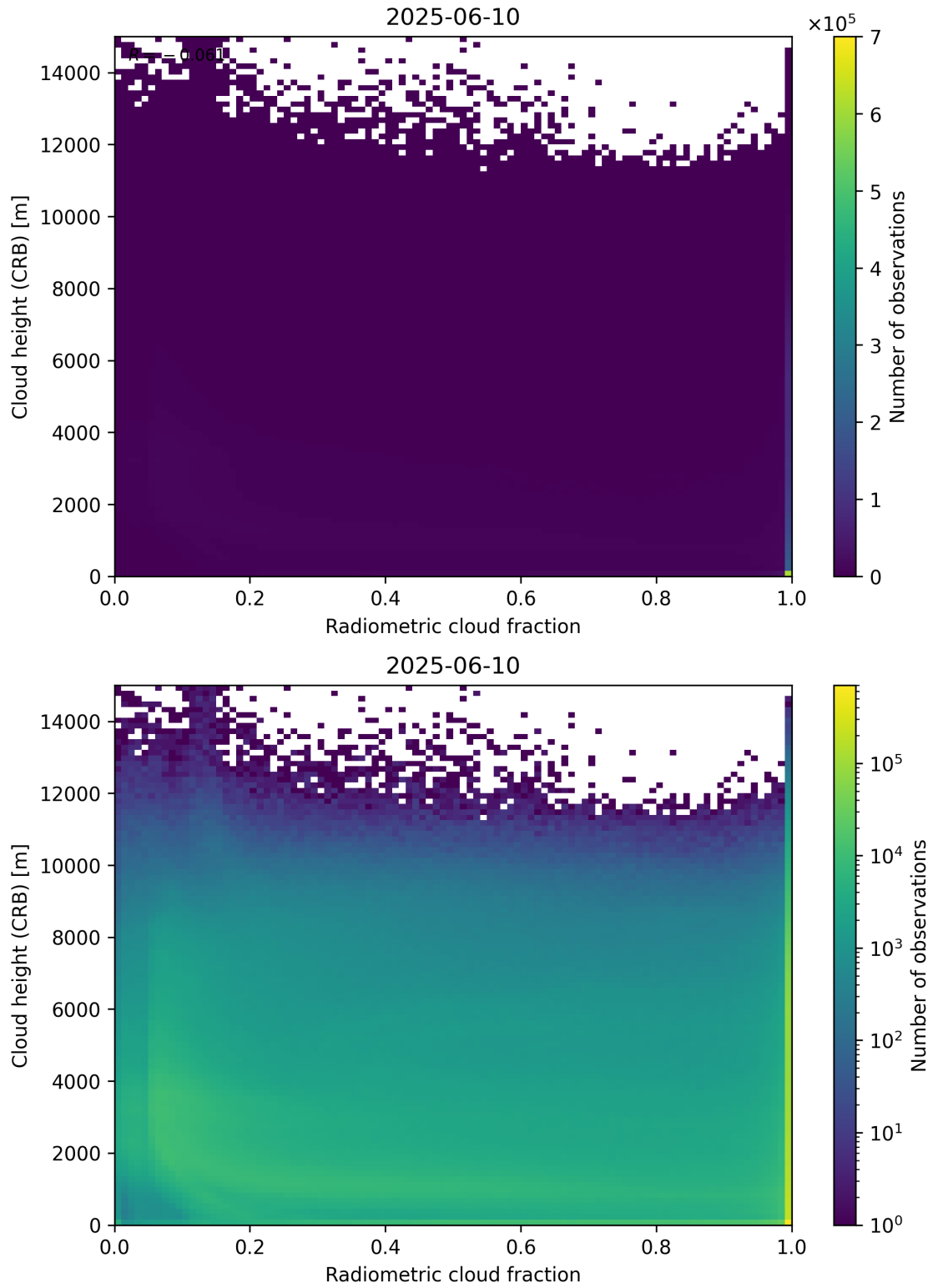
Figure 74: Scatter density plot of “Radiometric cloud fraction” against “Cloud height (CRB)” for 2025-06-09 to 2025-06-11.
