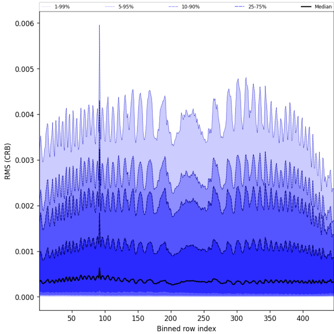
Figure 64: Along track statistics of “RMS (CRB)” for 2025-06-09 to 2025-06-11
