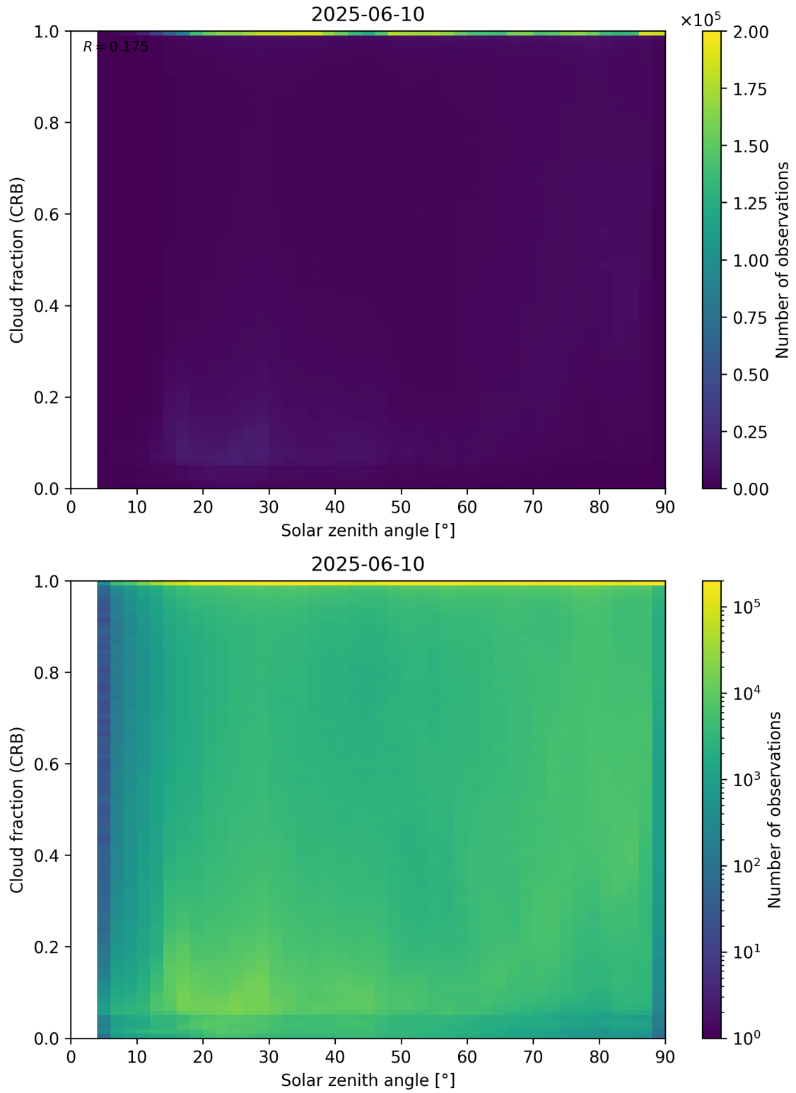
Figure 101: Scatter density plot of “Solar zenith angle” against “Cloud fraction (CRB)” for 2025-06-09 to 2025-06-11.
