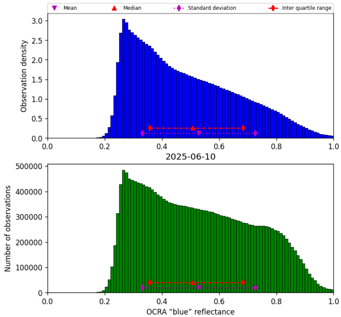
Figure 51: Histogram of “OCRA “blue” reflectance” for 2025-06-09 to 2025-06-11
