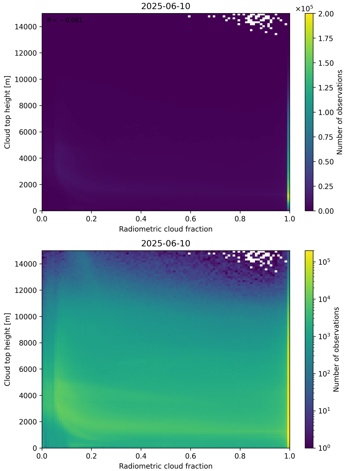
Figure 76: Scatter density plot of “Radiometric cloud fraction” against “Cloud top height” for 2025-06-09 to 2025-06-11.
