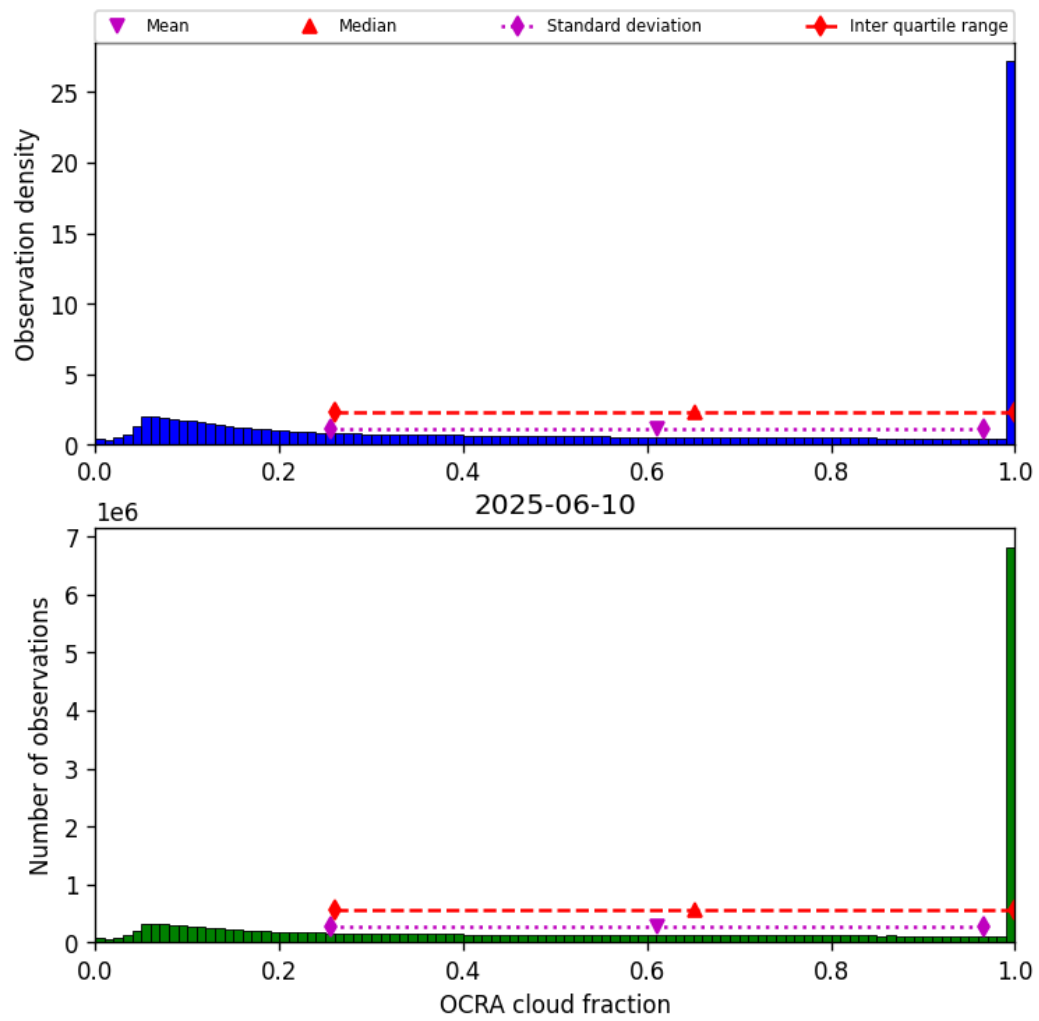
Figure 50: Histogram of “OCRA cloud fraction” for 2025-06-09 to 2025-06-11
