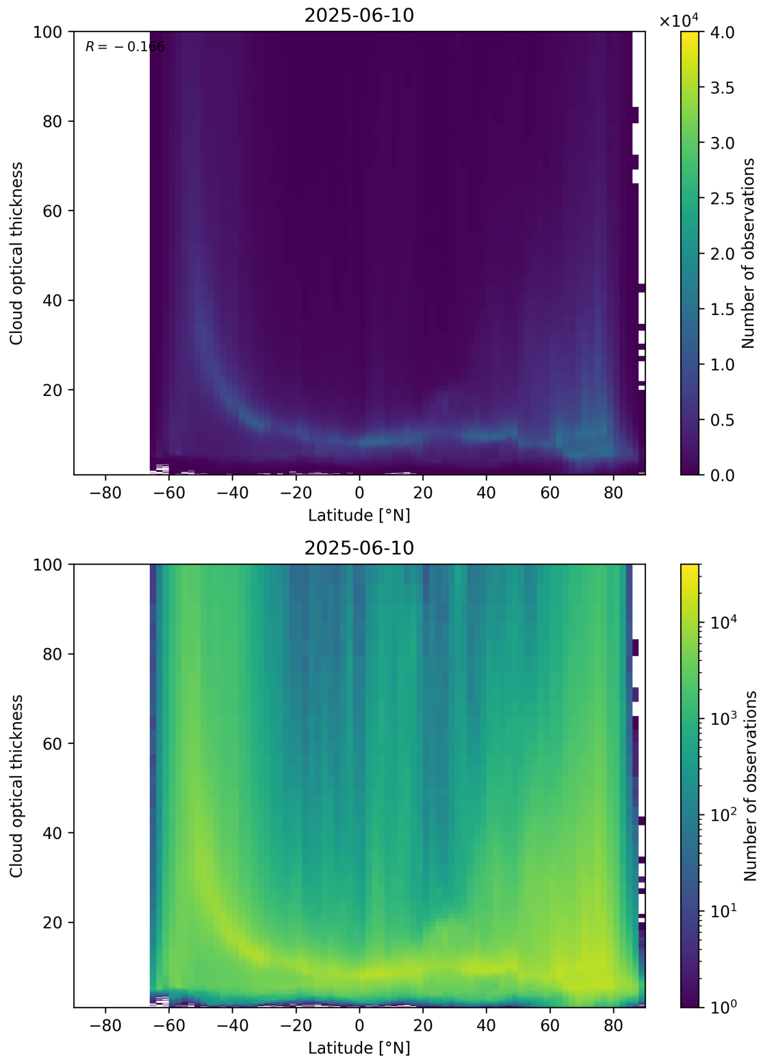
Figure 96: Scatter density plot of “Latitude” against “Cloud optical thickness” for 2025-06-09 to 2025-06-11.
