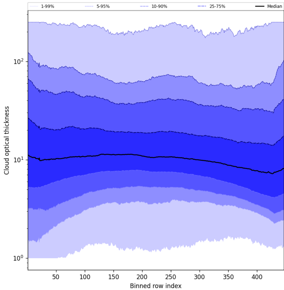
Figure 57: Along track statistics of “Cloud optical thickness” for 2025-06-09 to 2025-06-11
