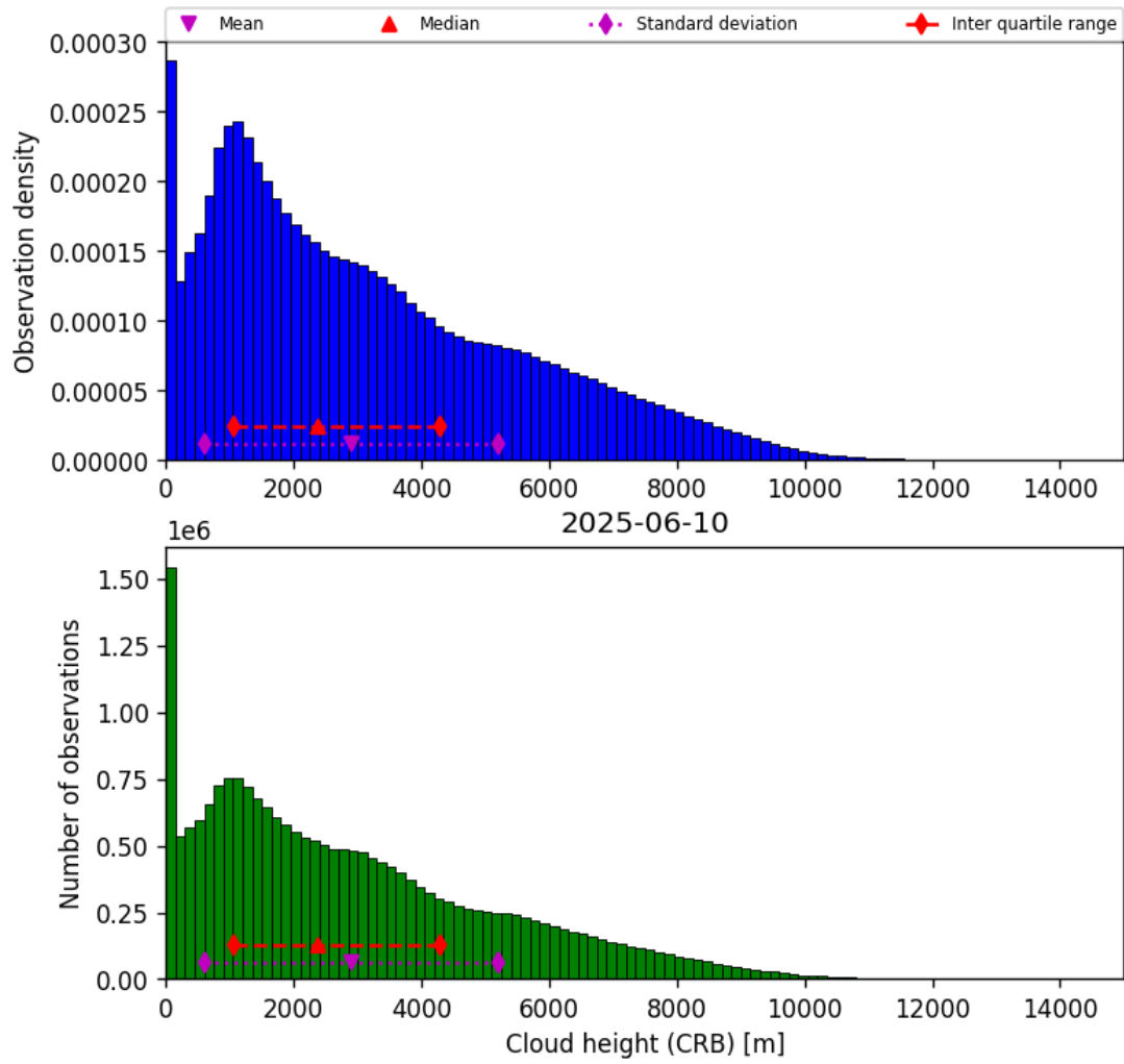
Figure 43: Histogram of “Cloud height (CRB)” for 2025-06-09 to 2025-06-11
