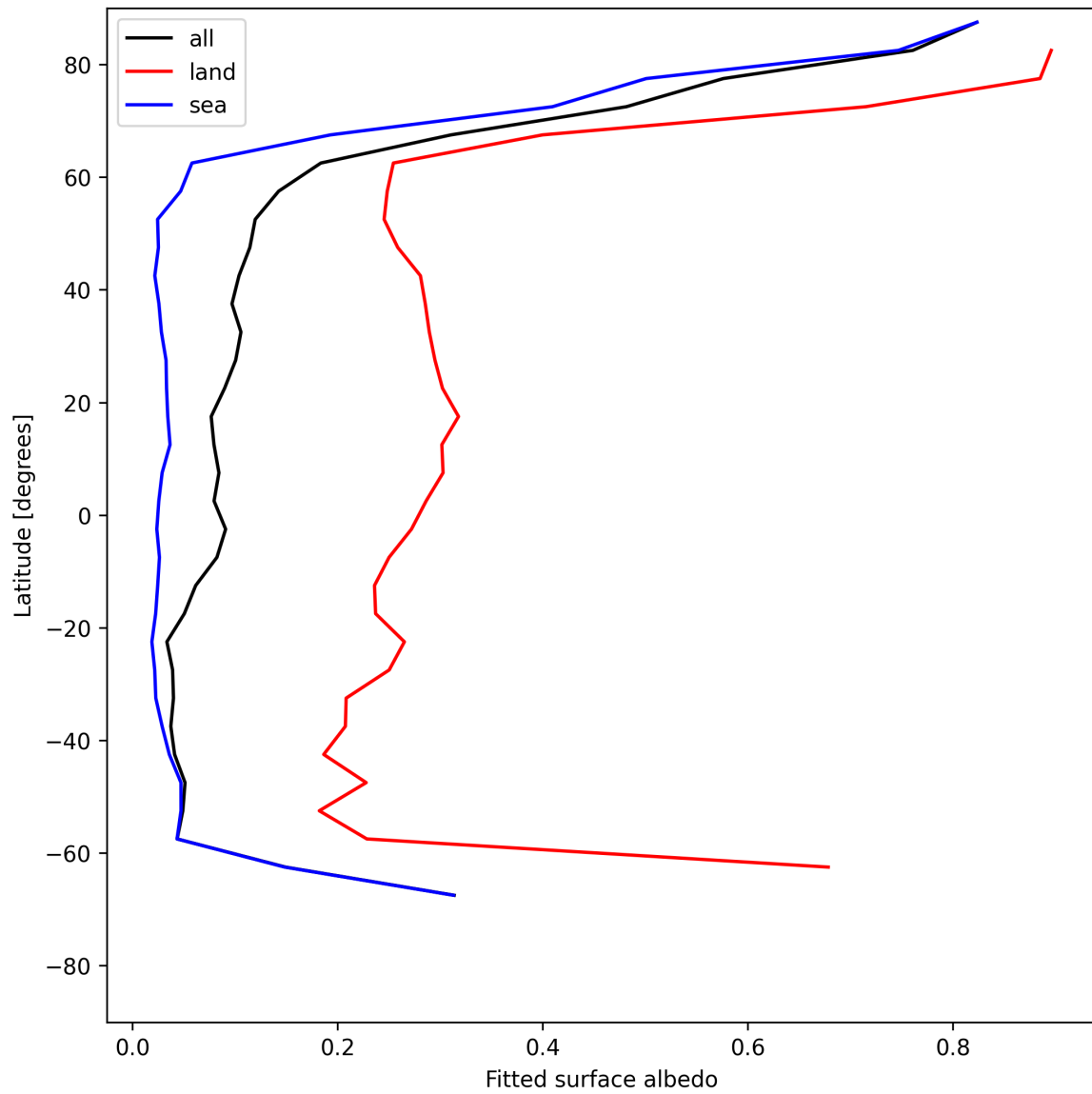
Figure 29: Zonal average of “Fitted surface albedo” for 2025-06-09 to 2025-06-11.
