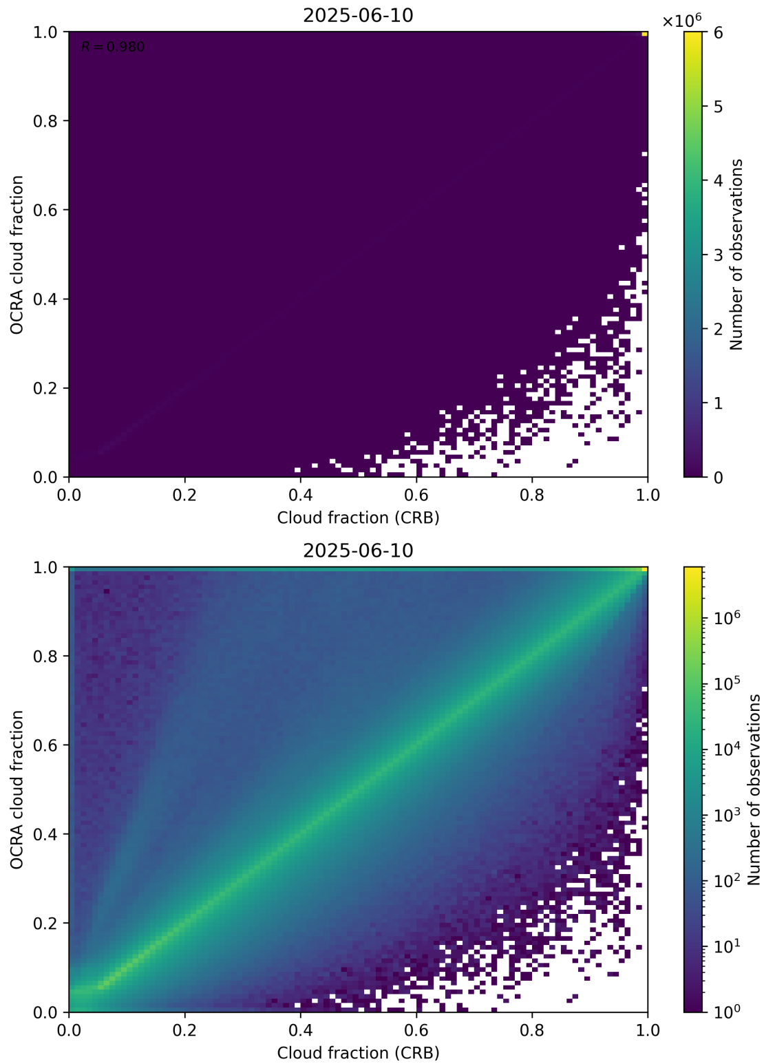
Figure 78: Scatter density plot of “Cloud fraction (CRB)” against “OCRA cloud fraction” for 2025-06-09 to 2025-06-11.
