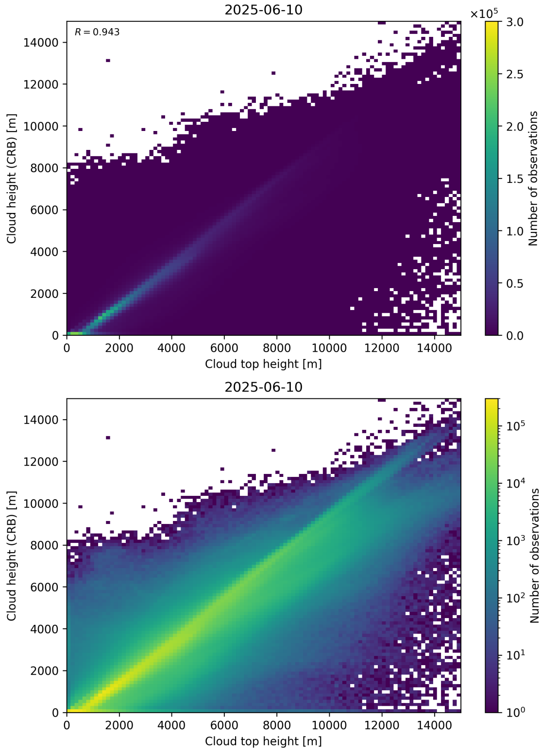
Figure 89: Scatter density plot of “Cloud top height” against “Cloud height (CRB)” for 2025-06-09 to 2025-06-11.
