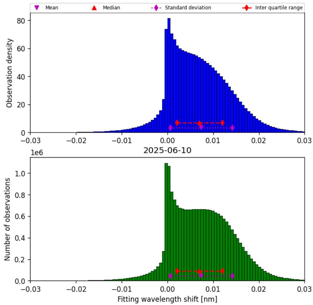
Figure 49: Histogram of “Fitting wavelength shift” for 2025-06-09 to 2025-06-11
