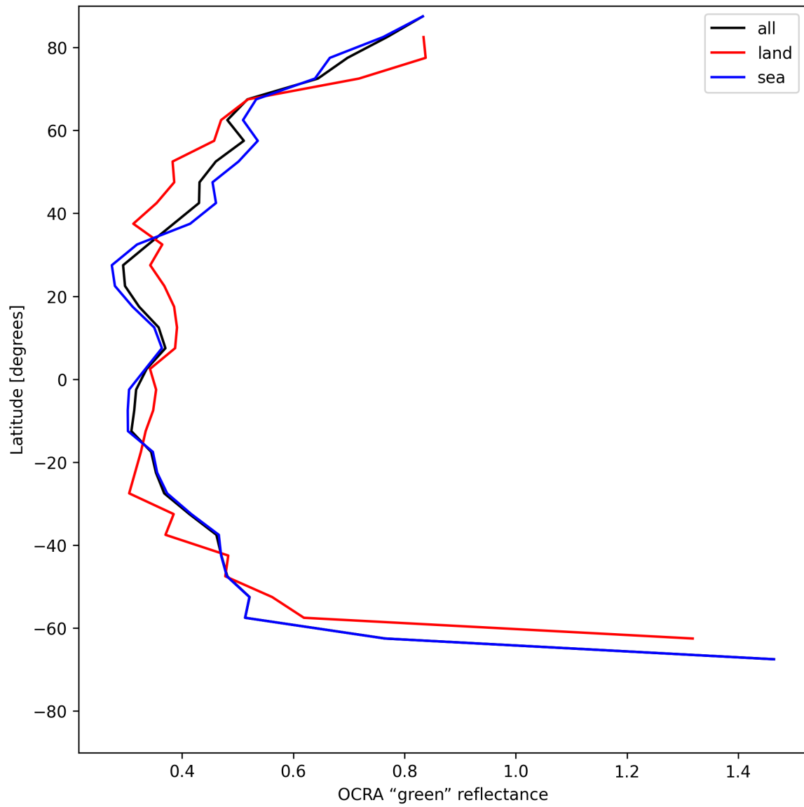
Figure 36: Zonal average of “OCRA “green” reflectance” for 2025-06-09 to 2025-06-11.
