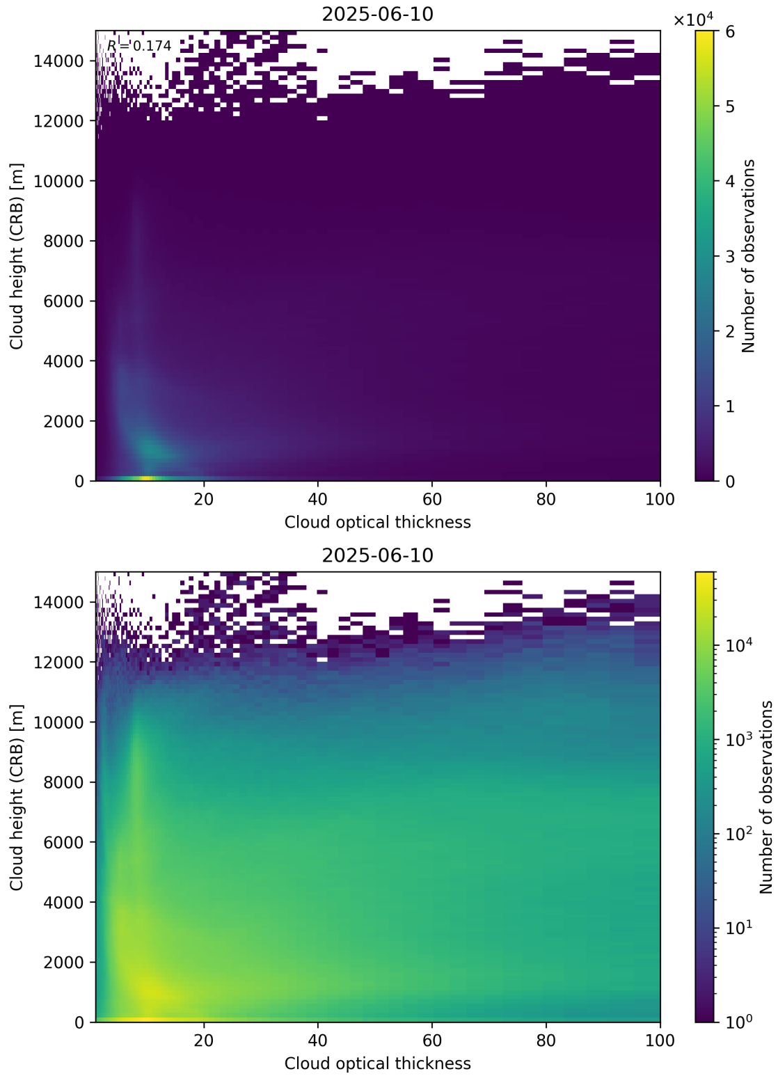
Figure 85: Scatter density plot of “Cloud optical thickness” against “Cloud height (CRB)” for 2025-06-09 to 2025-06-11.
