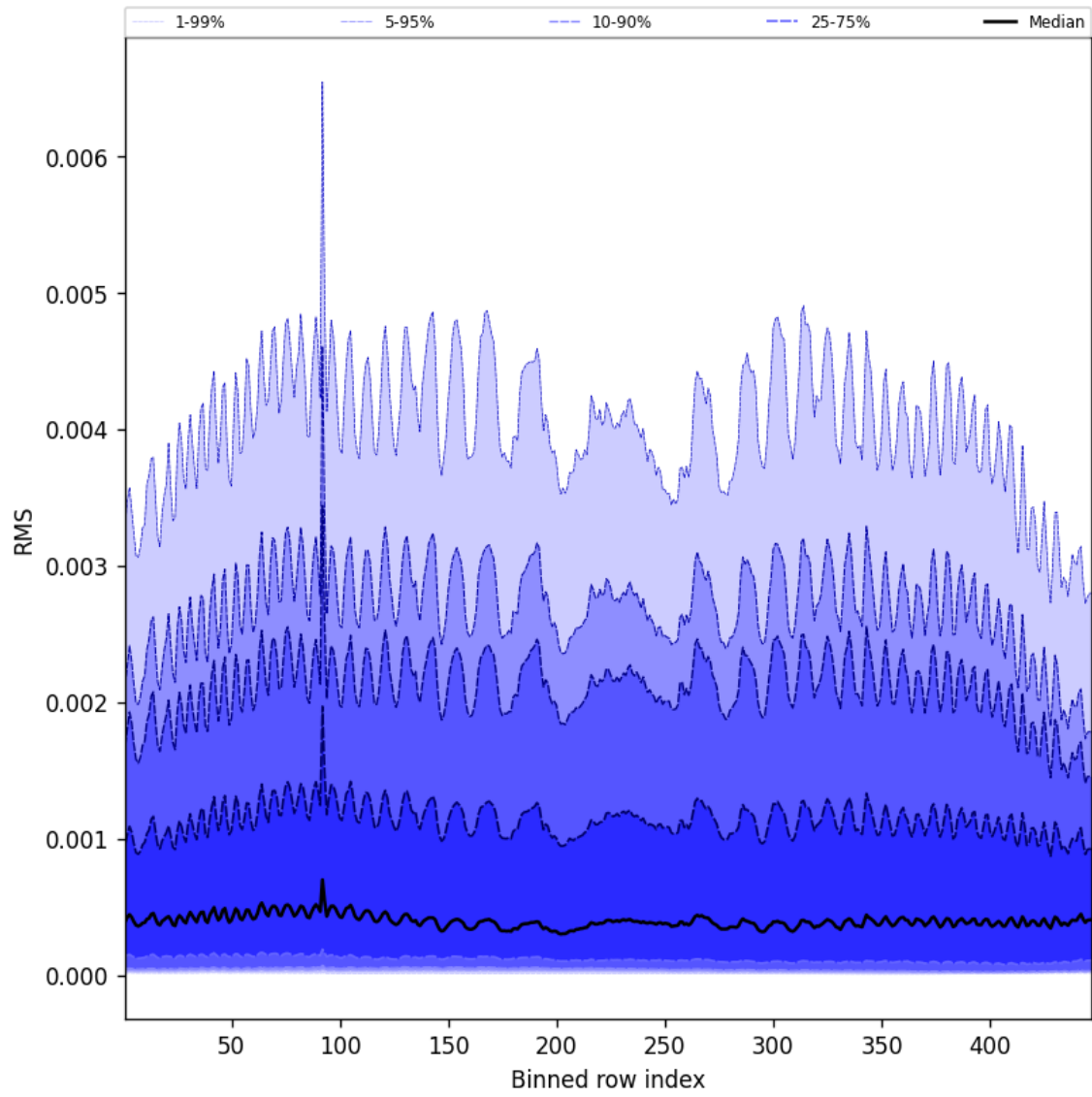
Figure 63: Along track statistics of “RMS” for 2025-06-09 to 2025-06-11
