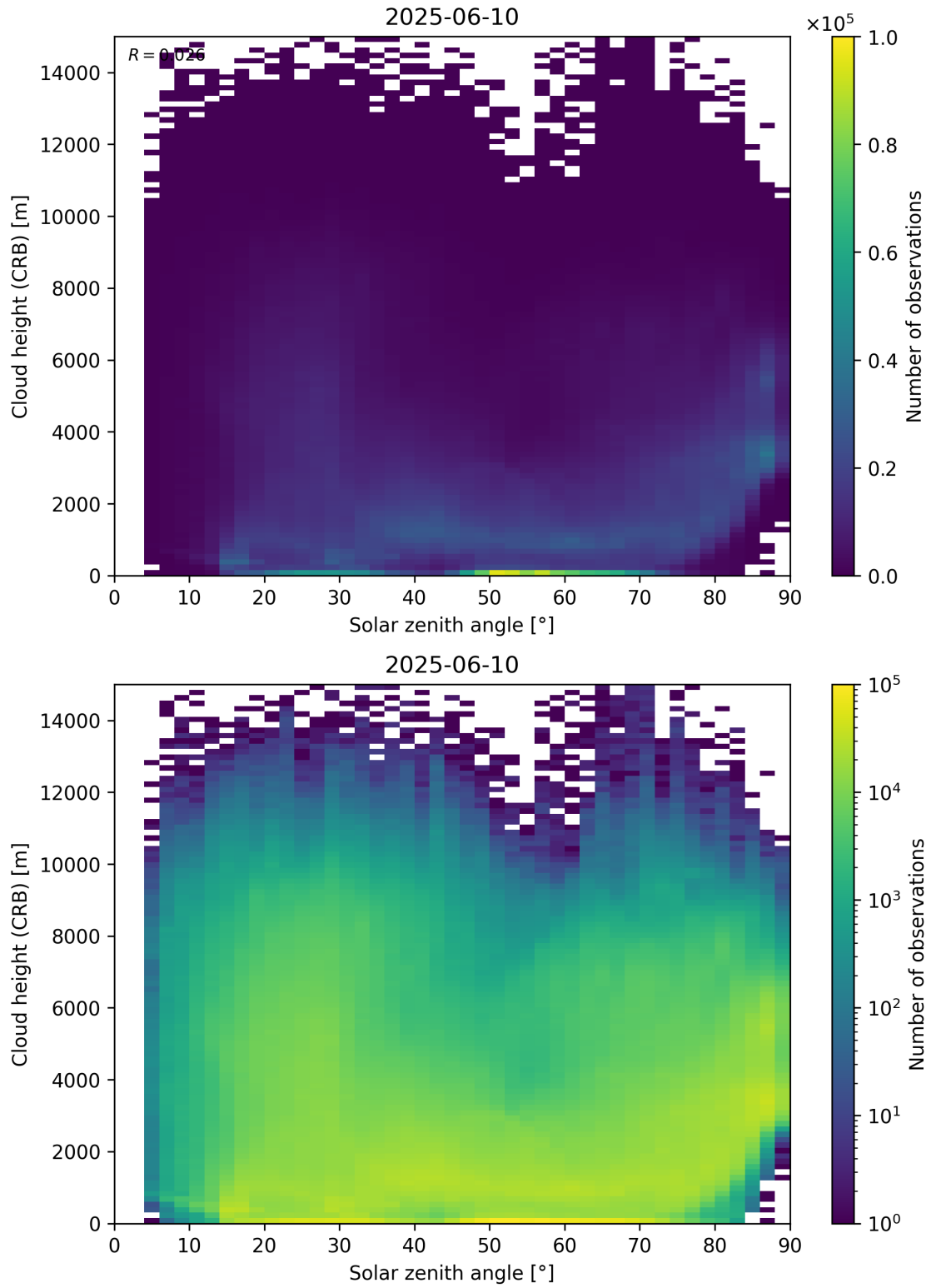
Figure 102: Scatter density plot of “Solar zenith angle” against “Cloud height (CRB)” for 2025-06-09 to 2025-06-11.
