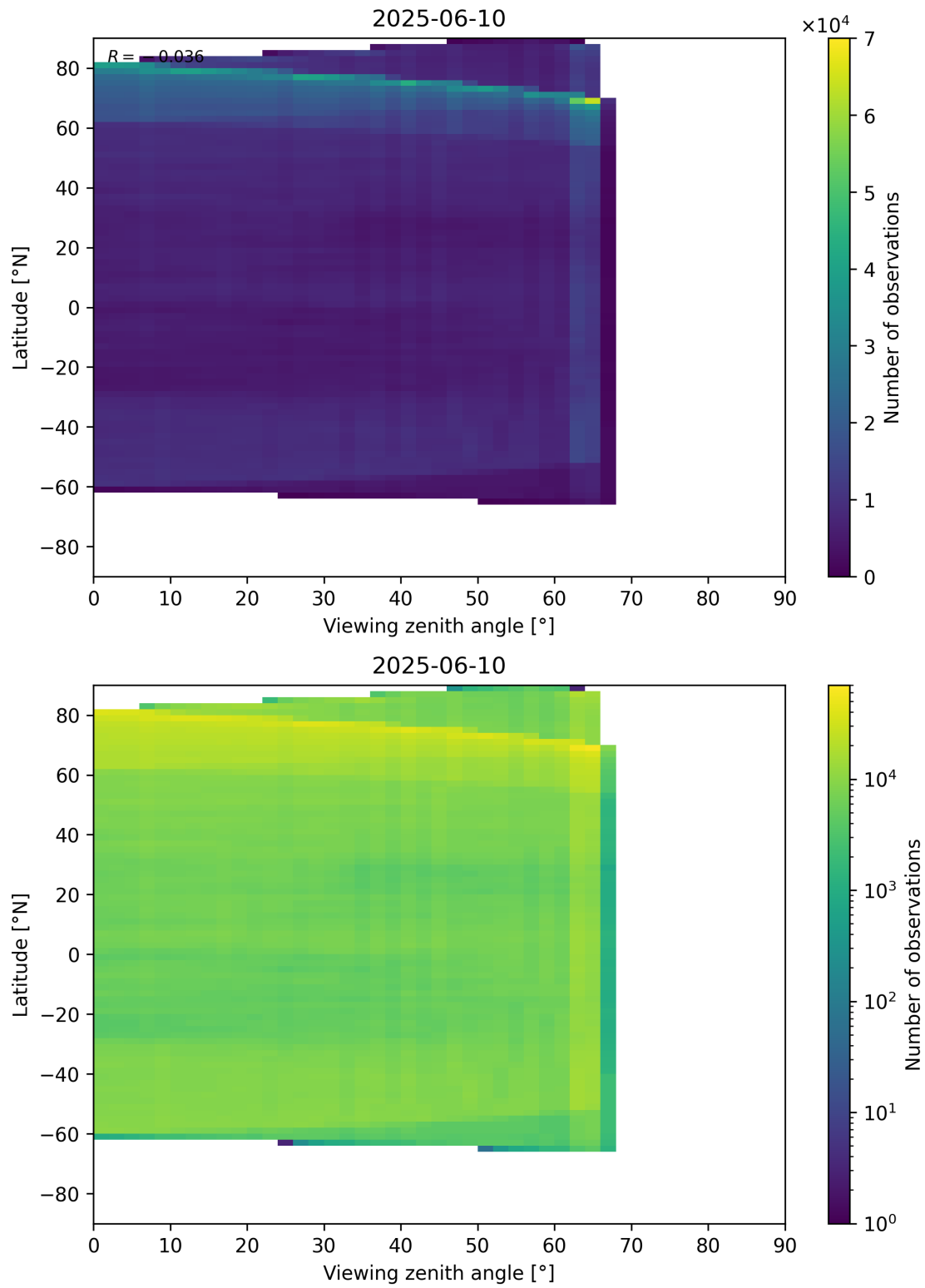
Figure 113: Scatter density plot of “Viewing zenith angle” against “Latitude” for 2025-06-09 to 2025-06-11.
