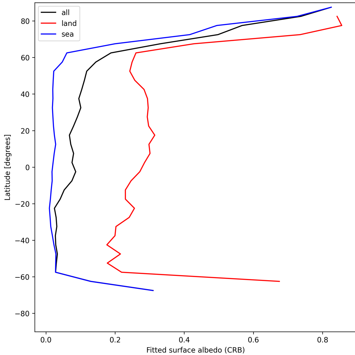
Figure 30: Zonal average of “Fitted surface albedo (CRB)” for 2025-06-09 to 2025-06-11.
