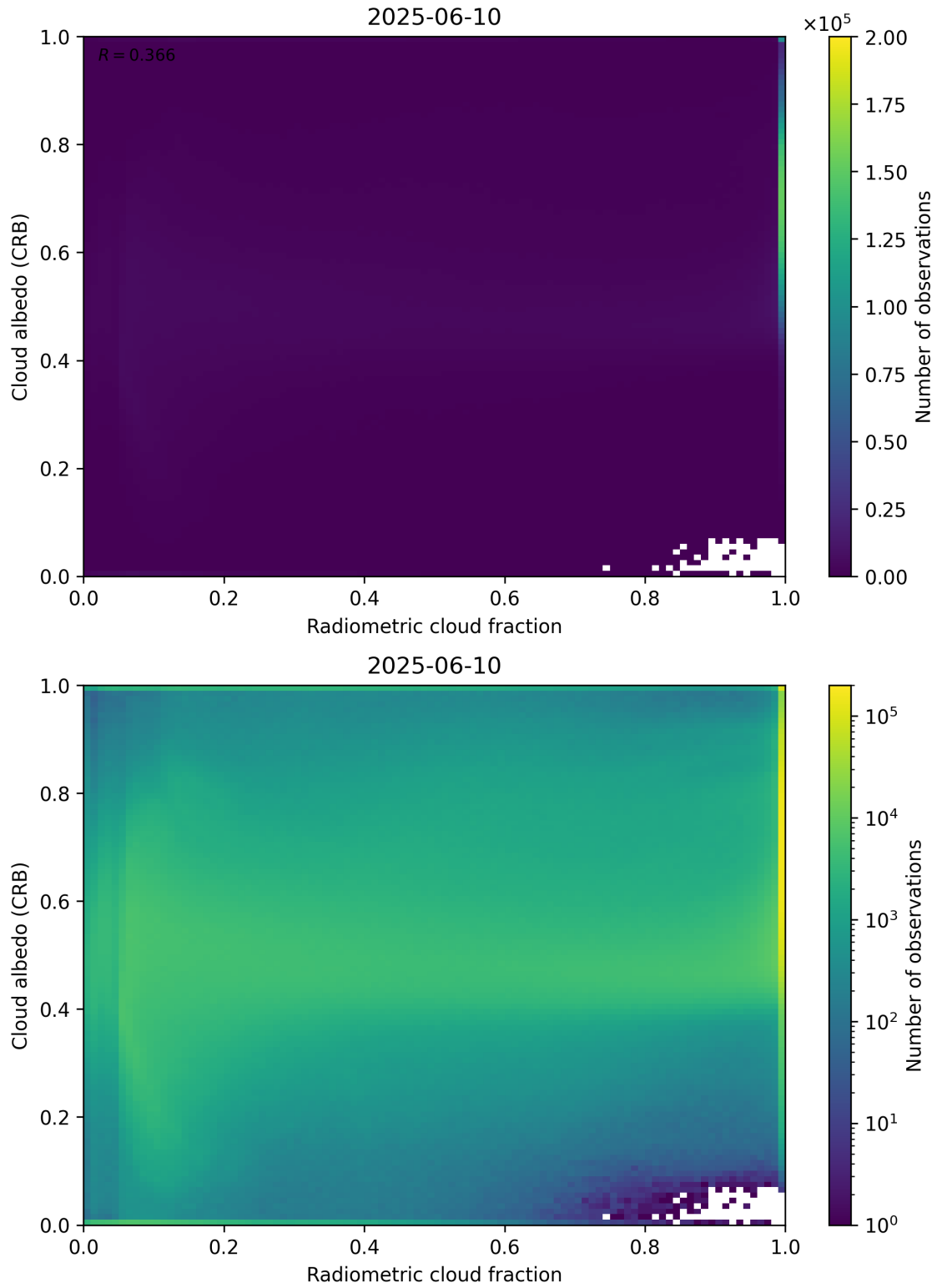
Figure 71: Scatter density plot of “Radiometric cloud fraction” against “Cloud albedo (CRB)” for 2025-06-09 to 2025-06-11.
