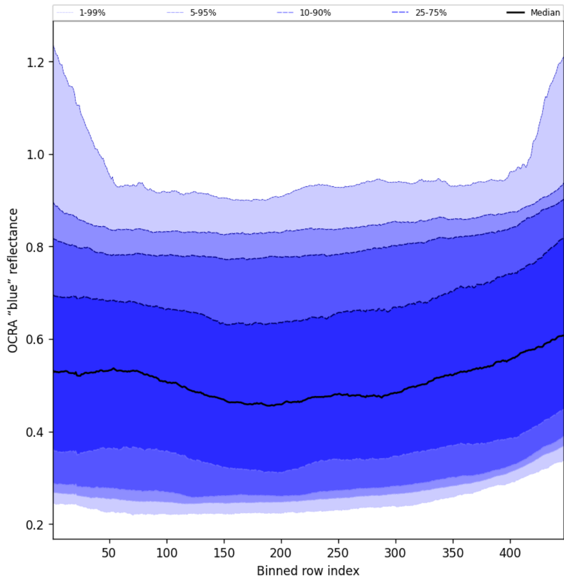
Figure 67: Along track statistics of “OCRA “blue” reflectance” for 2025-06-09 to 2025-06-11
