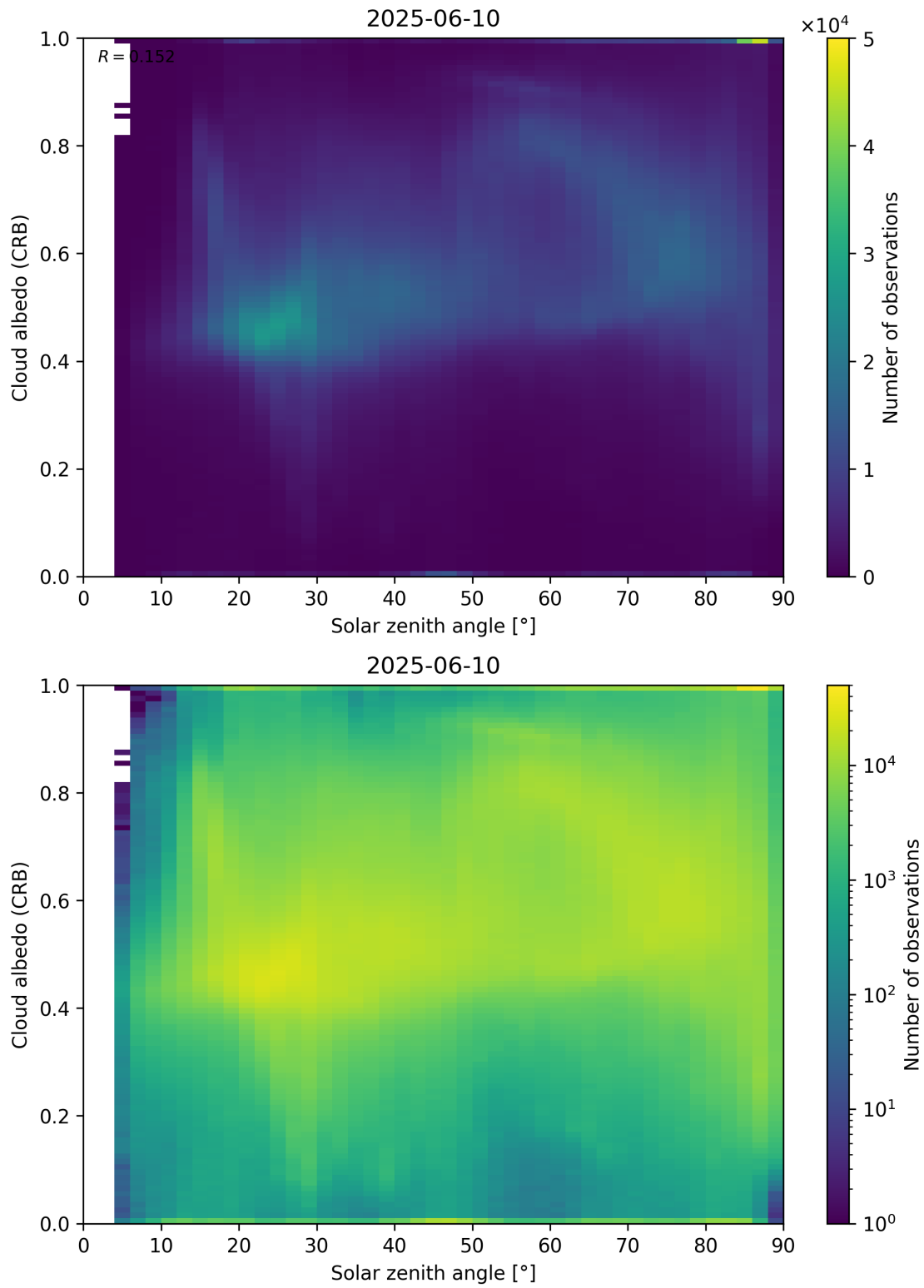
Figure 98: Scatter density plot of “Solar zenith angle” against “Cloud albedo (CRB)” for 2025-06-09 to 2025-06-11.
