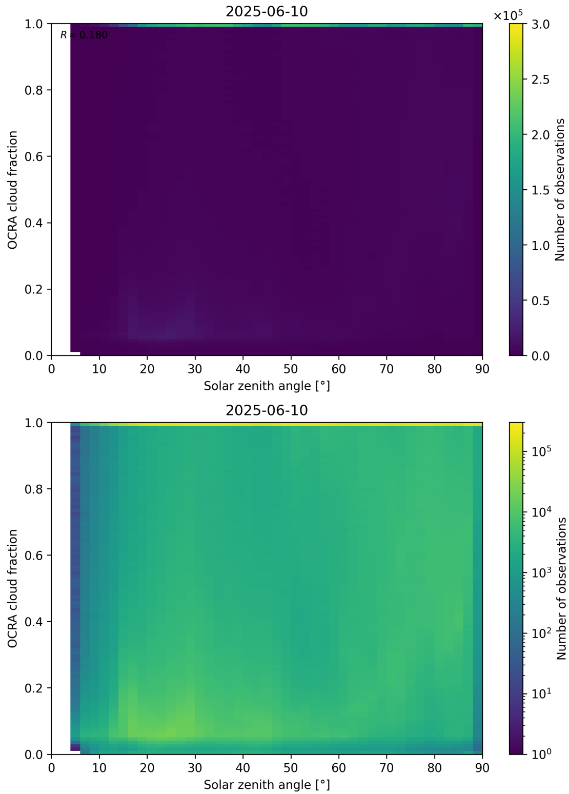
Figure 100: Scatter density plot of “Solar zenith angle” against “OCRA cloud fraction” for 2025-06-09 to 2025-06-11.
