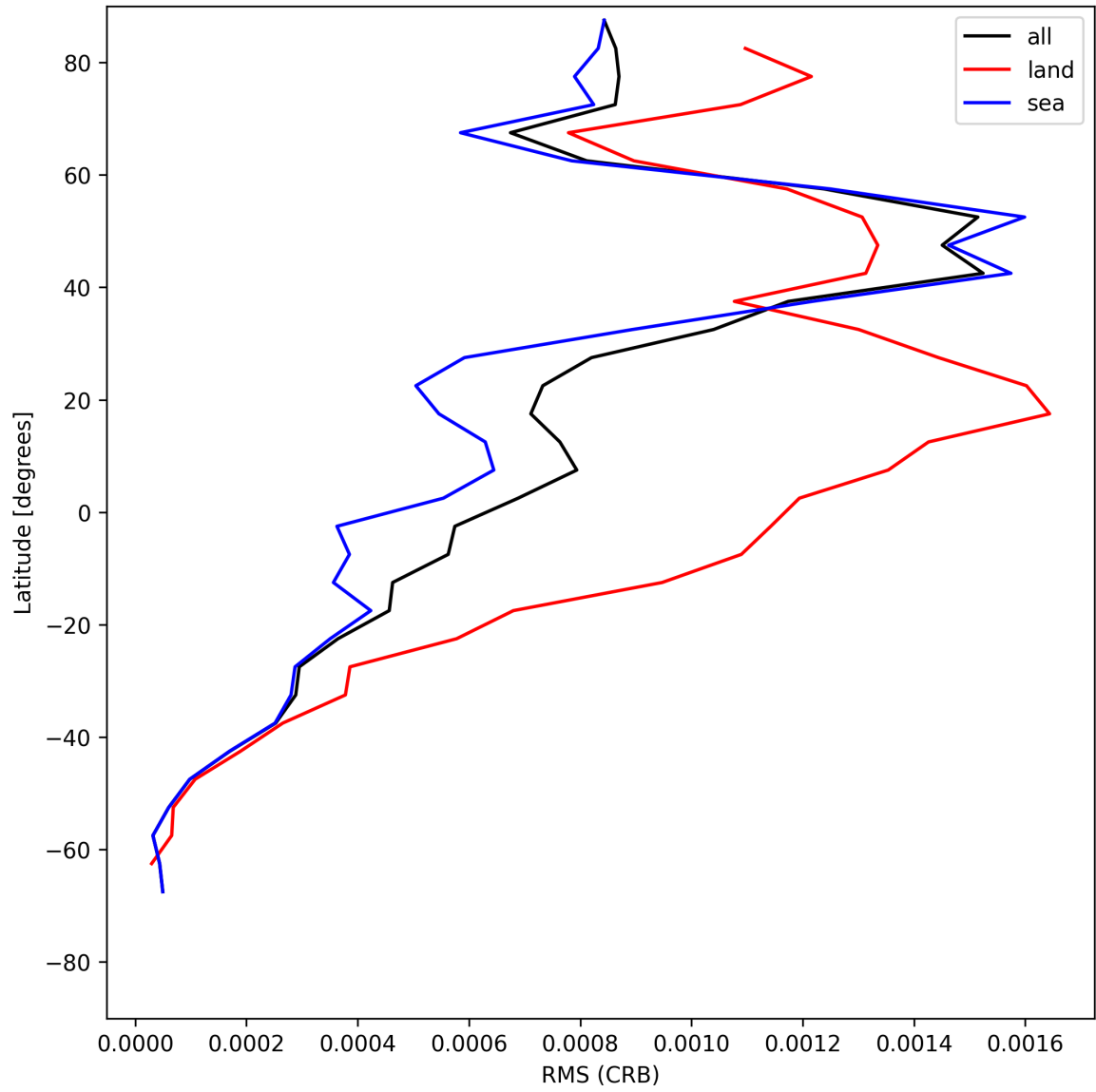
Figure 32: Zonal average of “RMS (CRB)” for 2025-06-09 to 2025-06-11.
