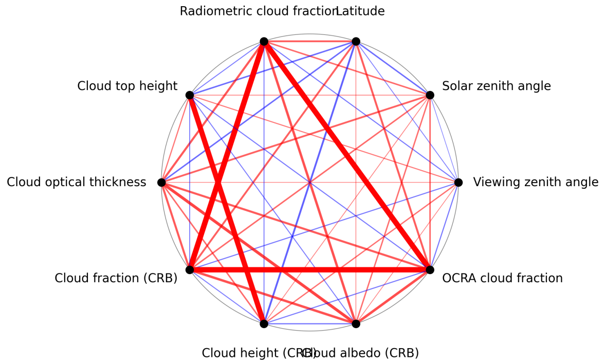
Figure 1: Map of correlation graph for 2025-06-09 to 2025-06-11.
