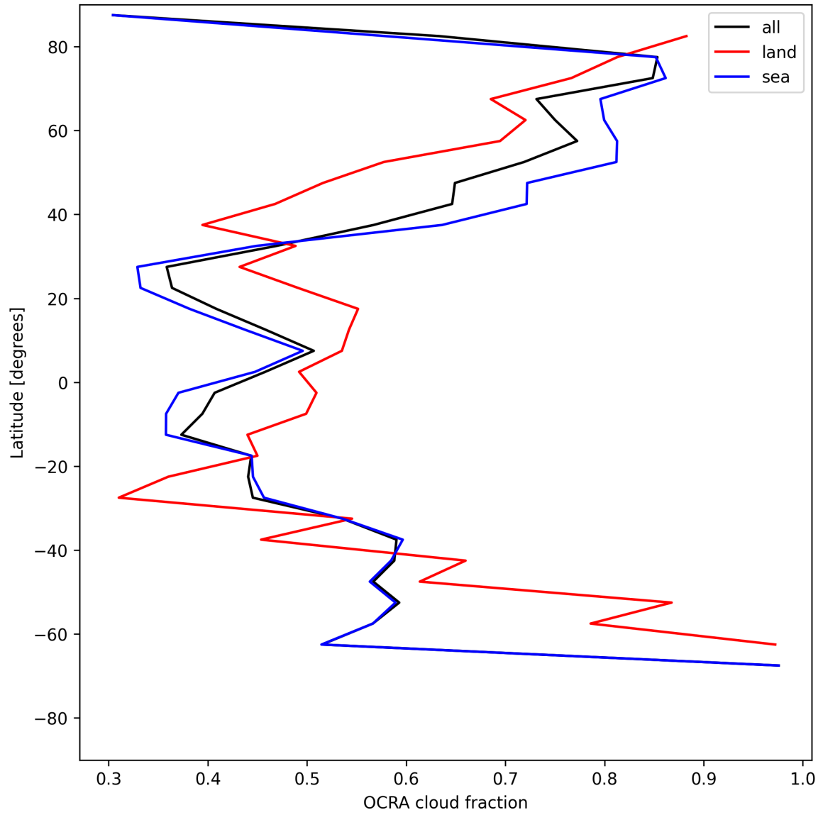
Figure 34: Zonal average of “OCRA cloud fraction” for 2025-06-09 to 2025-06-11.
