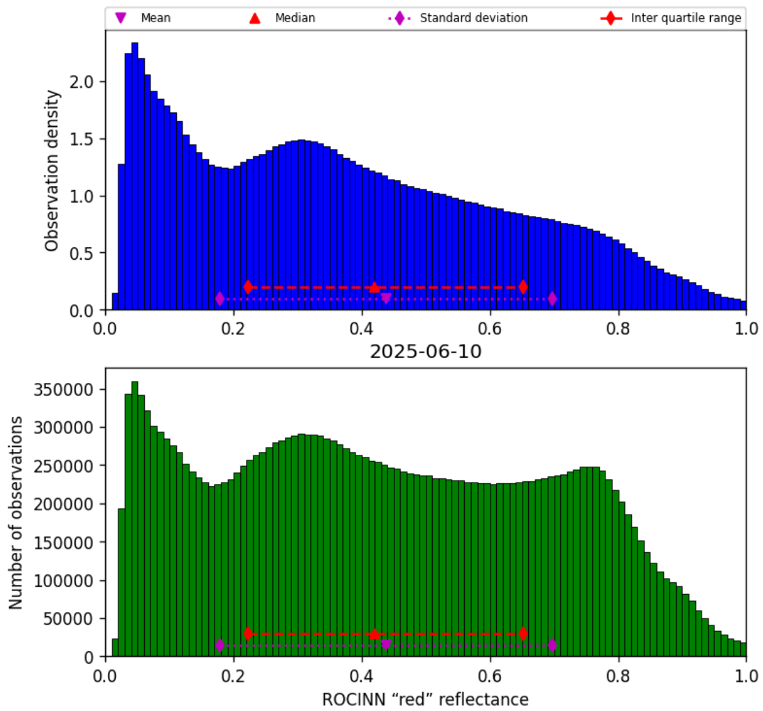
Figure 53: Histogram of “ROCINN “red” reflectance” for 2025-06-09 to 2025-06-11
