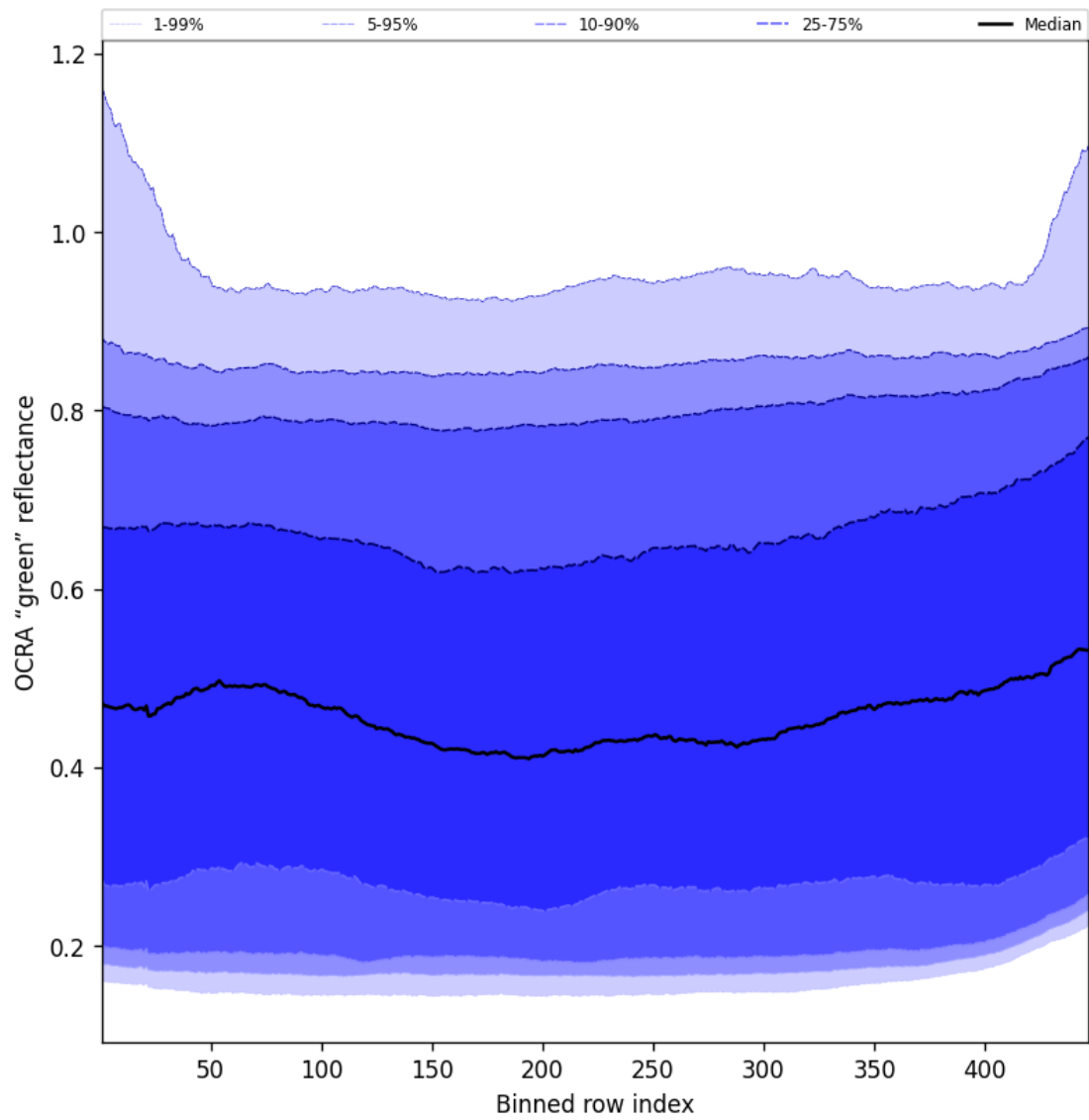
Figure 68: Along track statistics of "OCRA "green" reflectance" for 2025-06-09 to 2025-06-11
