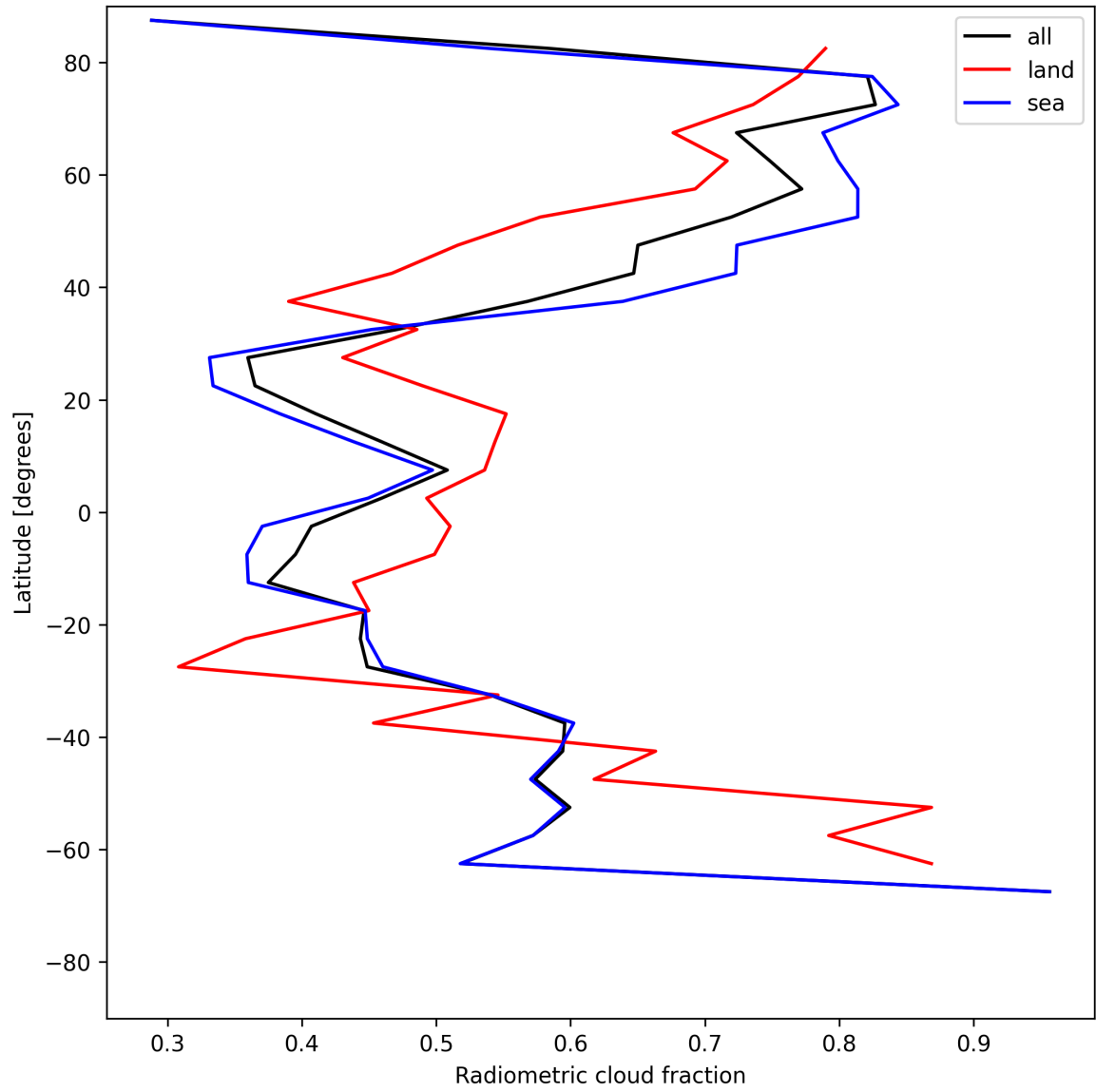
Figure 23: Zonal average of “Radiometric cloud fraction” for 2025-06-09 to 2025-06-11.
