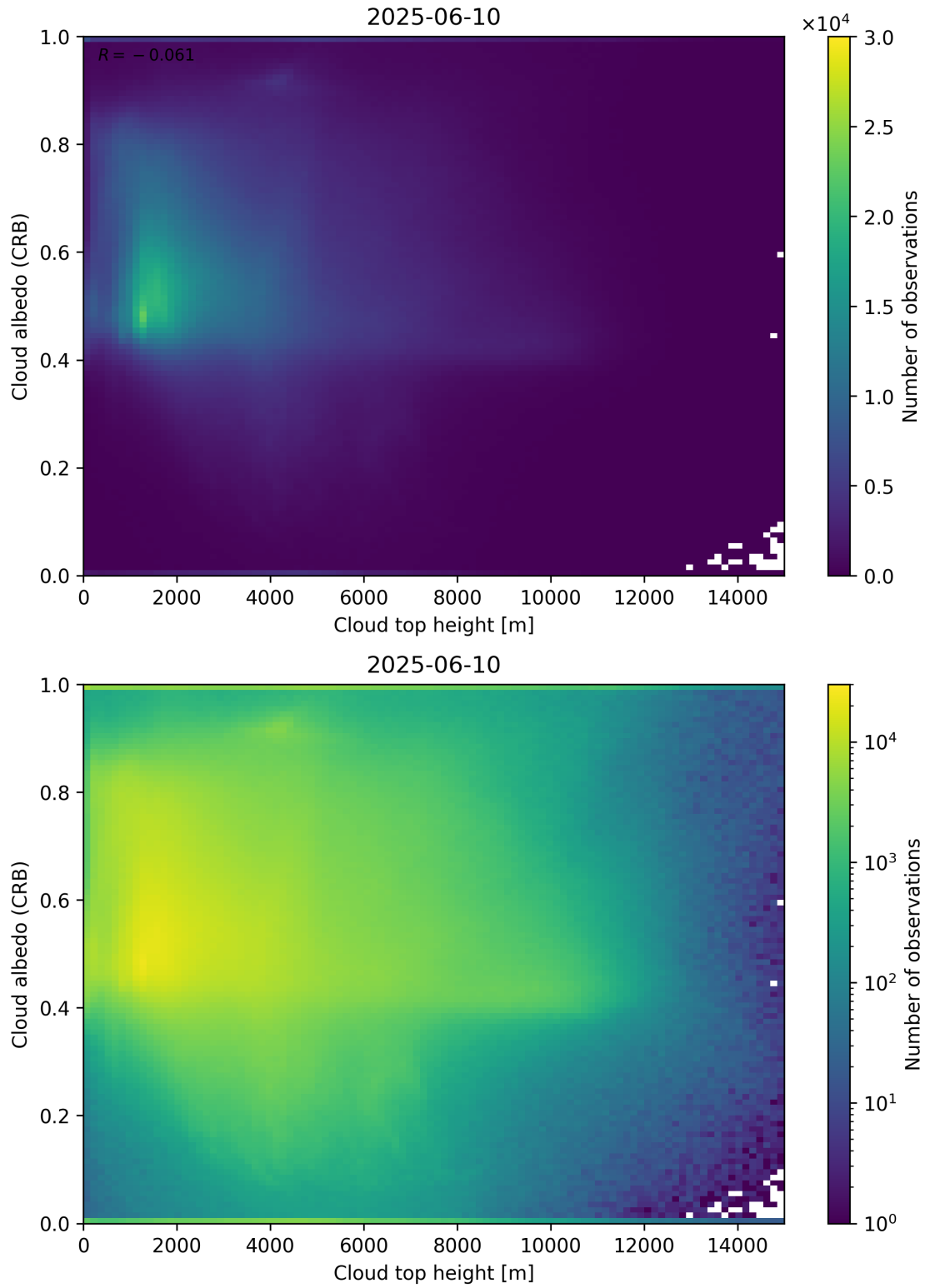
Figure 86: Scatter density plot of “Cloud top height” against “Cloud albedo (CRB)” for 2025-06-09 to 2025-06-11.
