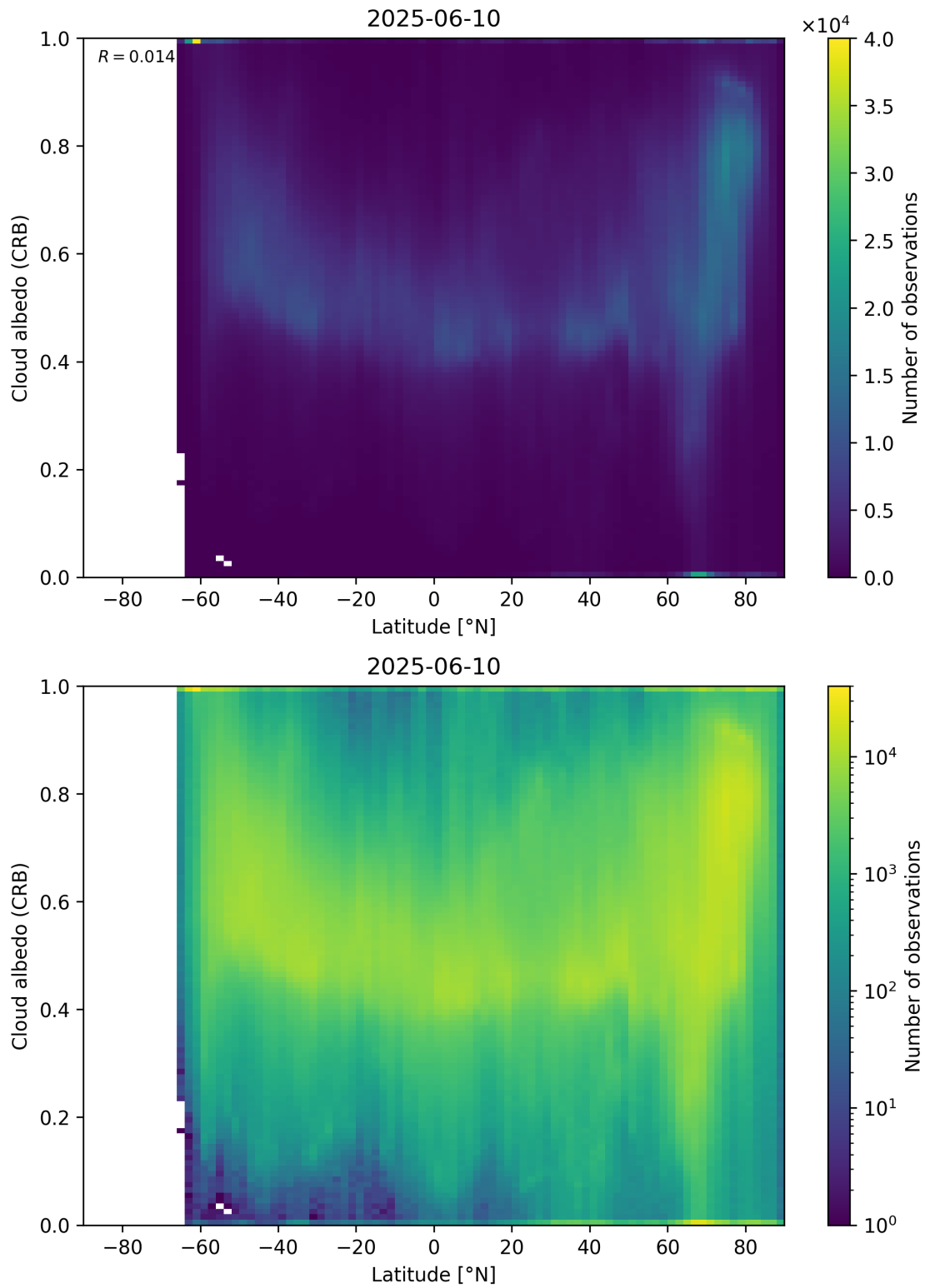
Figure 91: Scatter density plot of “Latitude” against “Cloud albedo (CRB)” for 2025-06-09 to 2025-06-11.
