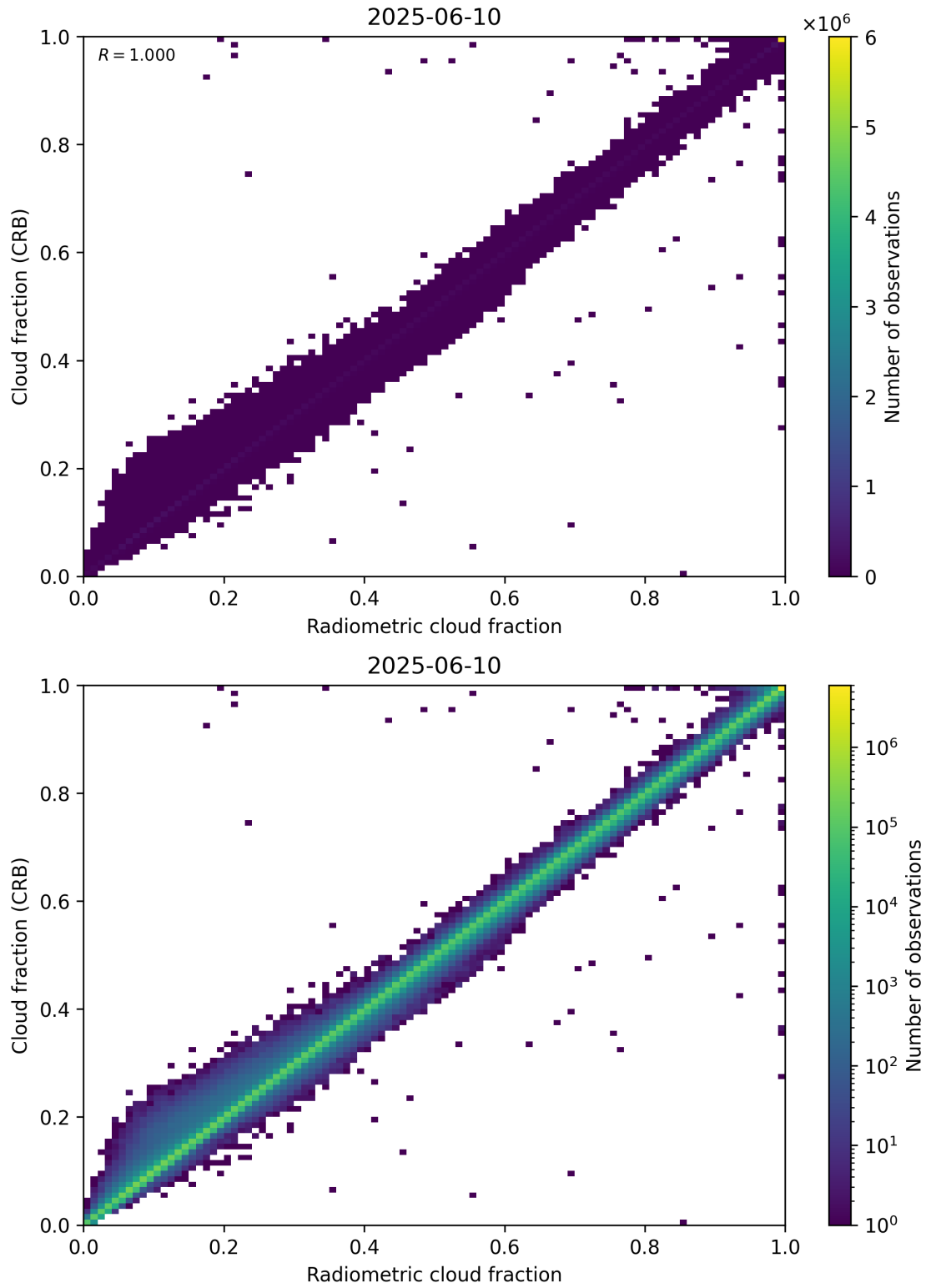
Figure 73: Scatter density plot of “Radiometric cloud fraction” against “Cloud fraction (CRB)” for 2025-06-09 to 2025-06-11.
