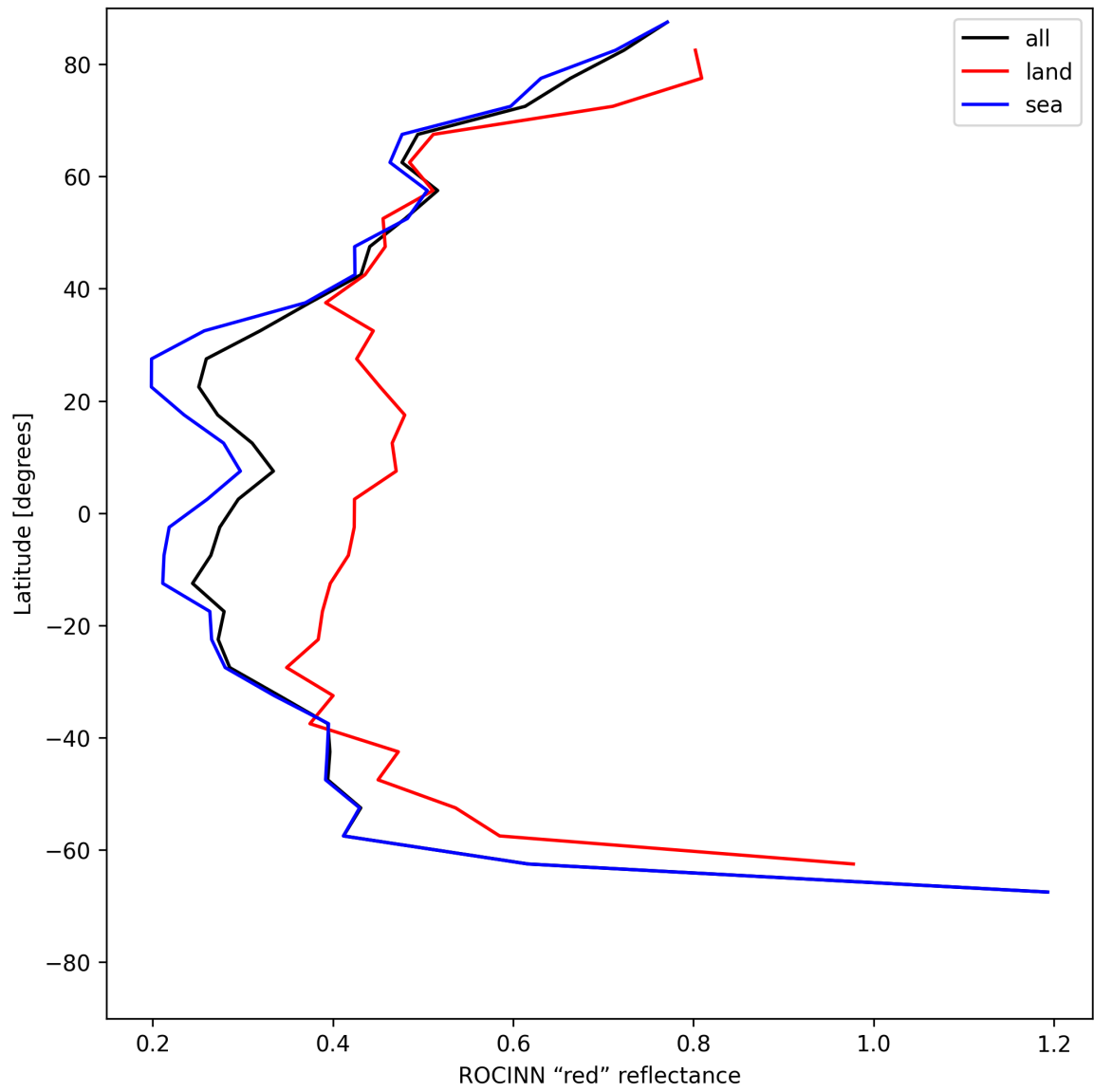
Figure 37: Zonal average of “ROCINN “red” reflectance” for 2025-06-09 to 2025-06-11.
