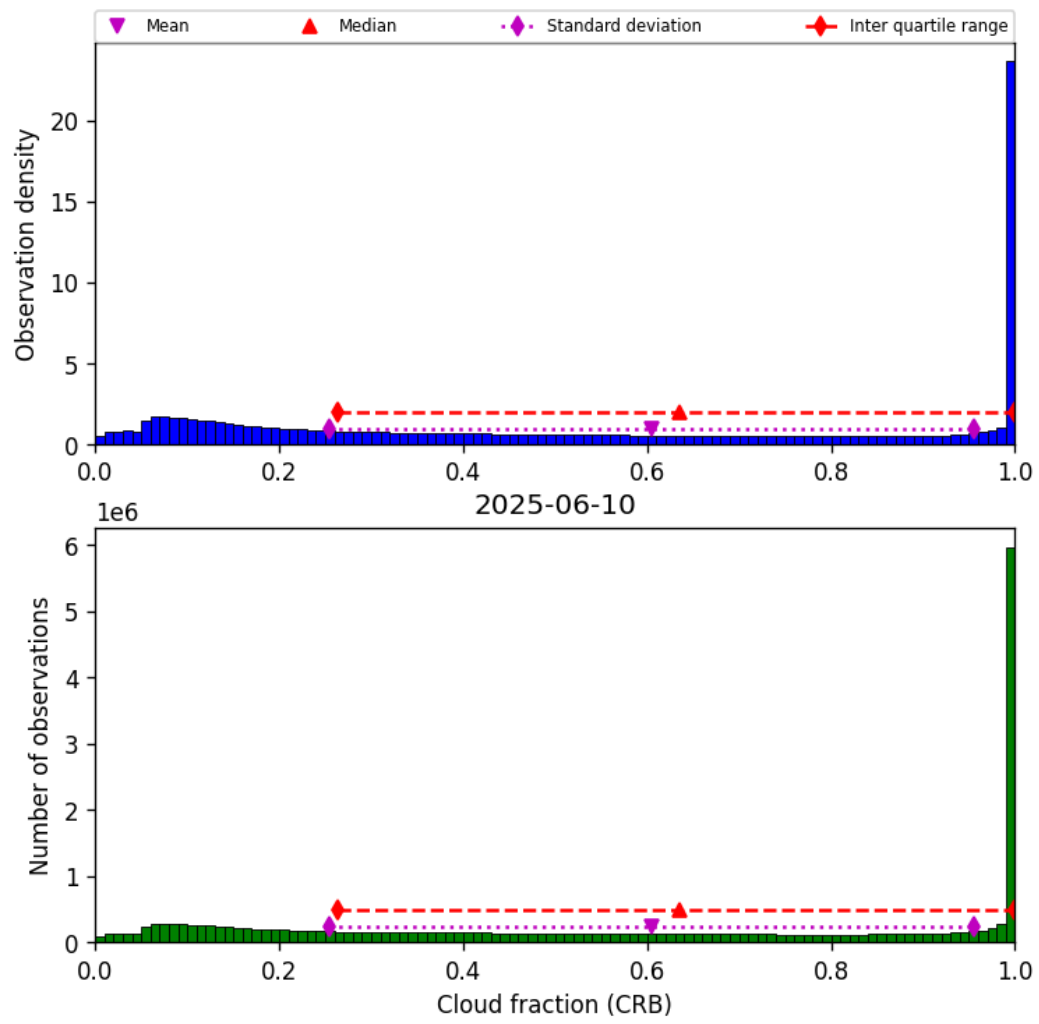
Figure 42: Histogram of “Cloud fraction (CRB)” for 2025-06-09 to 2025-06-11
