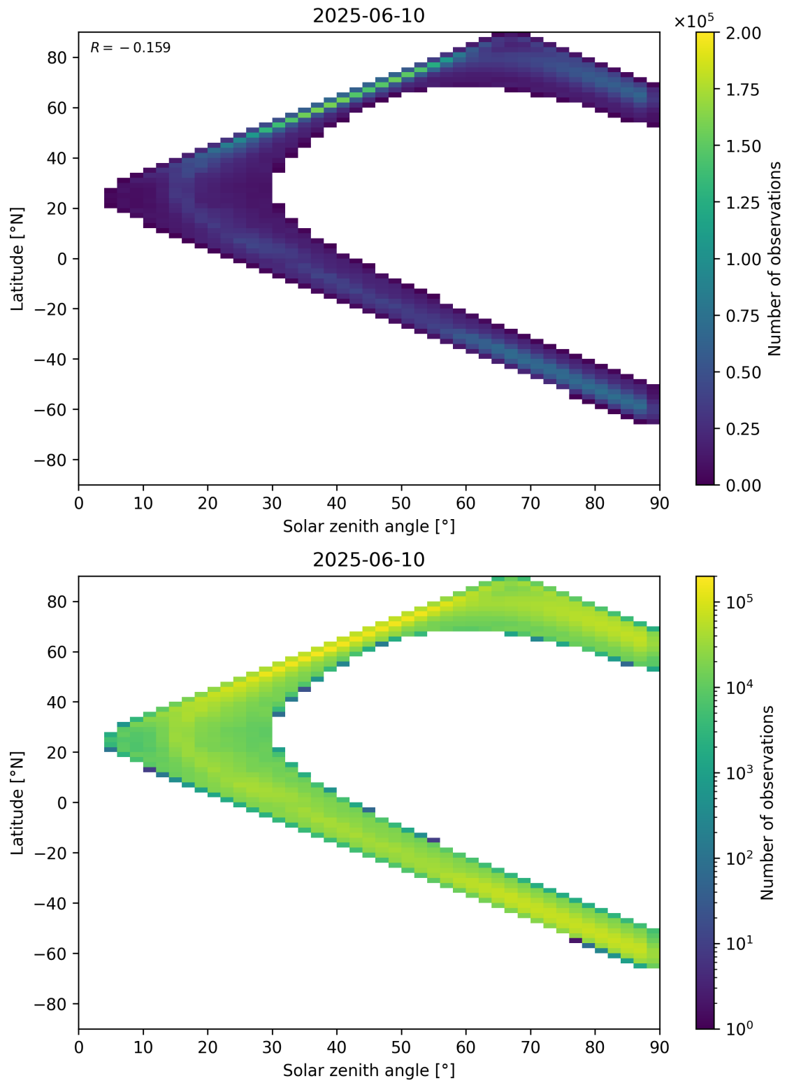
Figure 105: Scatter density plot of “Solar zenith angle” against “Latitude” for 2025-06-09 to 2025-06-11.
