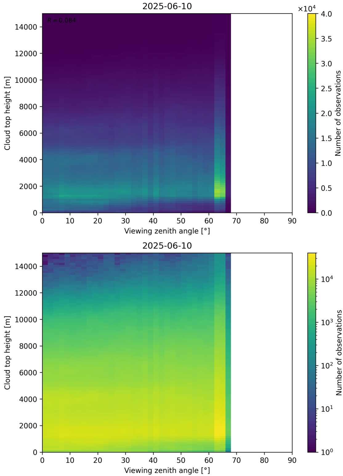
Figure 112: Scatter density plot of “Viewing zenith angle” against “Cloud top height” for 2025-06-09 to 2025-06-11.
