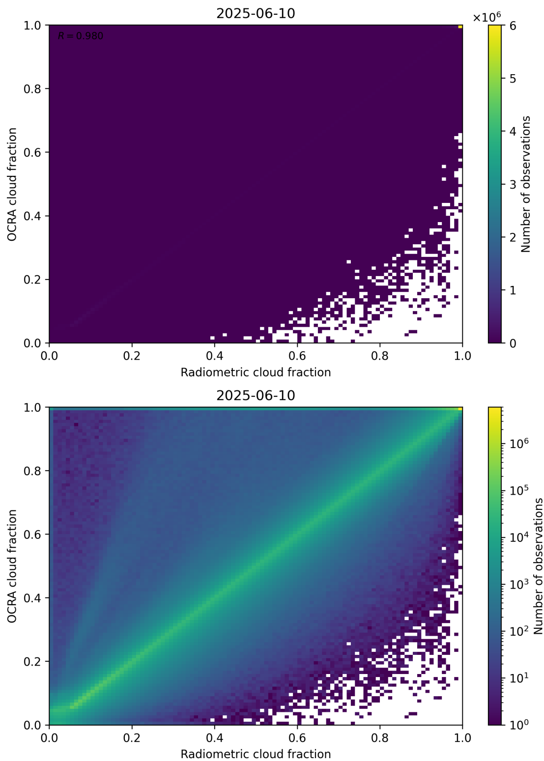
Figure 72: Scatter density plot of “Radiometric cloud fraction” against “OCRA cloud fraction” for 2025-06-09 to 2025-06-11.
