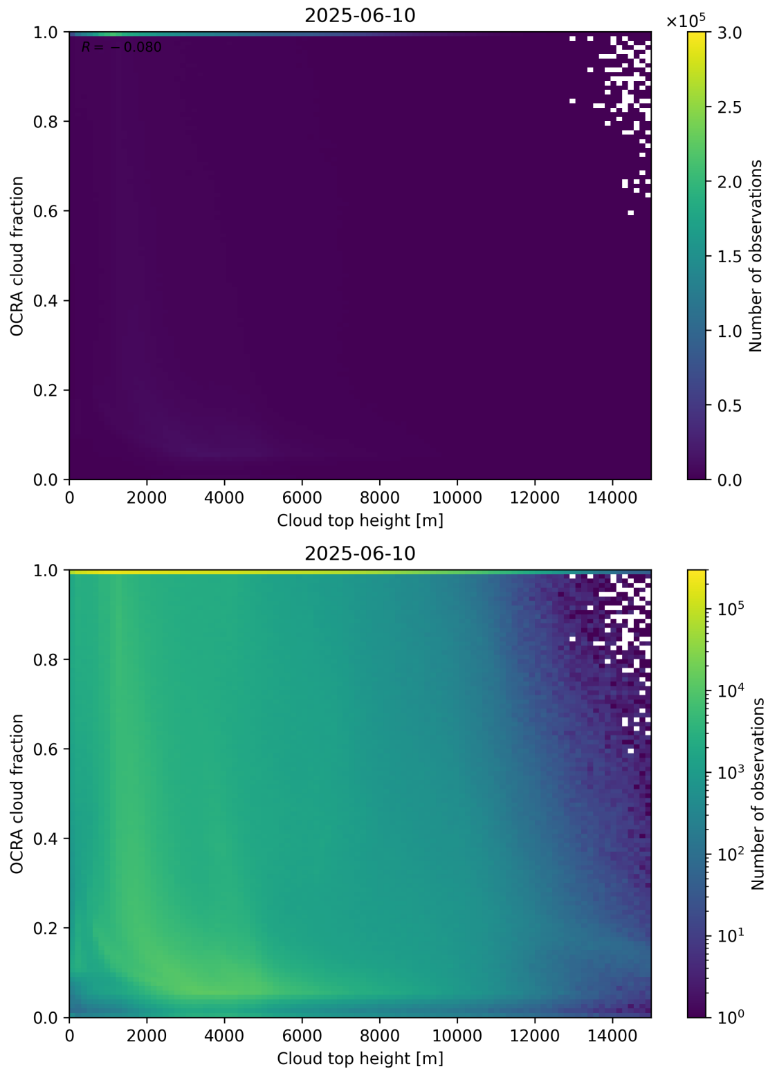
Figure 87: Scatter density plot of “Cloud top height” against “OCRA cloud fraction” for 2025-06-09 to 2025-06-11.
