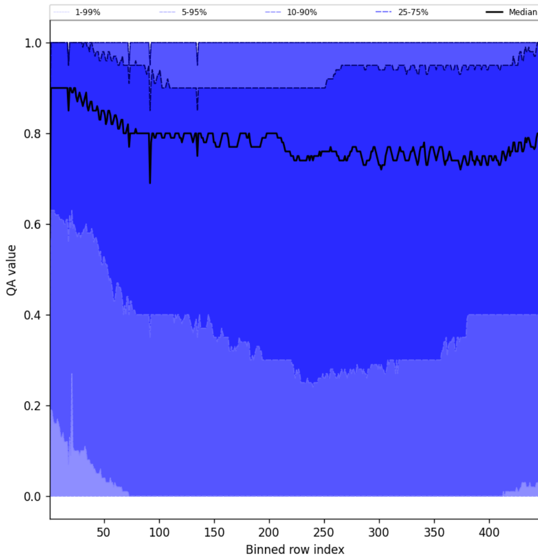
Figure 54: Along track statistics of “QA value” for 2025-06-09 to 2025-06-11
