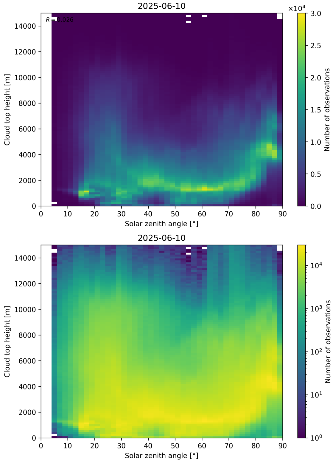
Figure 104: Scatter density plot of “Solar zenith angle” against “Cloud top height” for 2025-06-09 to 2025-06-11.
