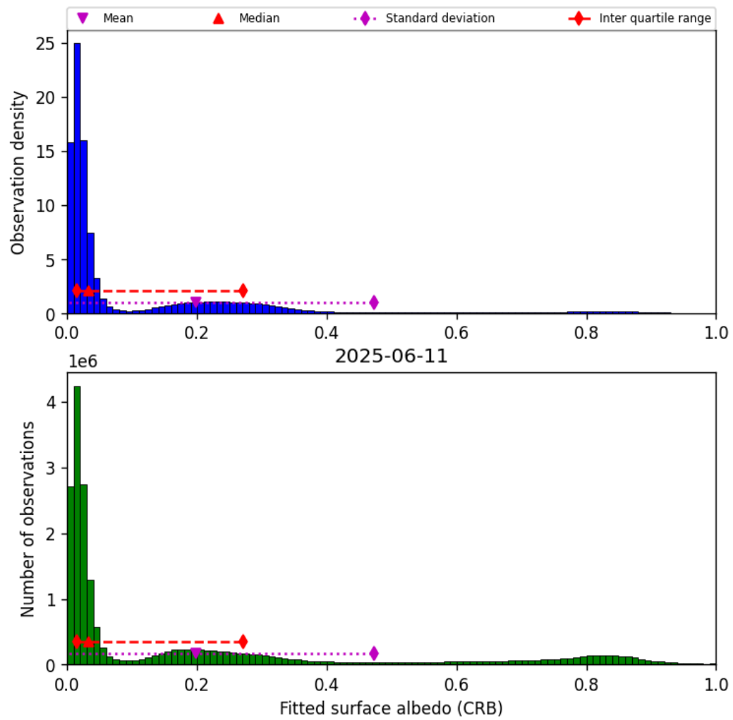
Figure 46: Histogram of “Fitted surface albedo (CRB)” for 2025-06-11 to 2025-06-12
