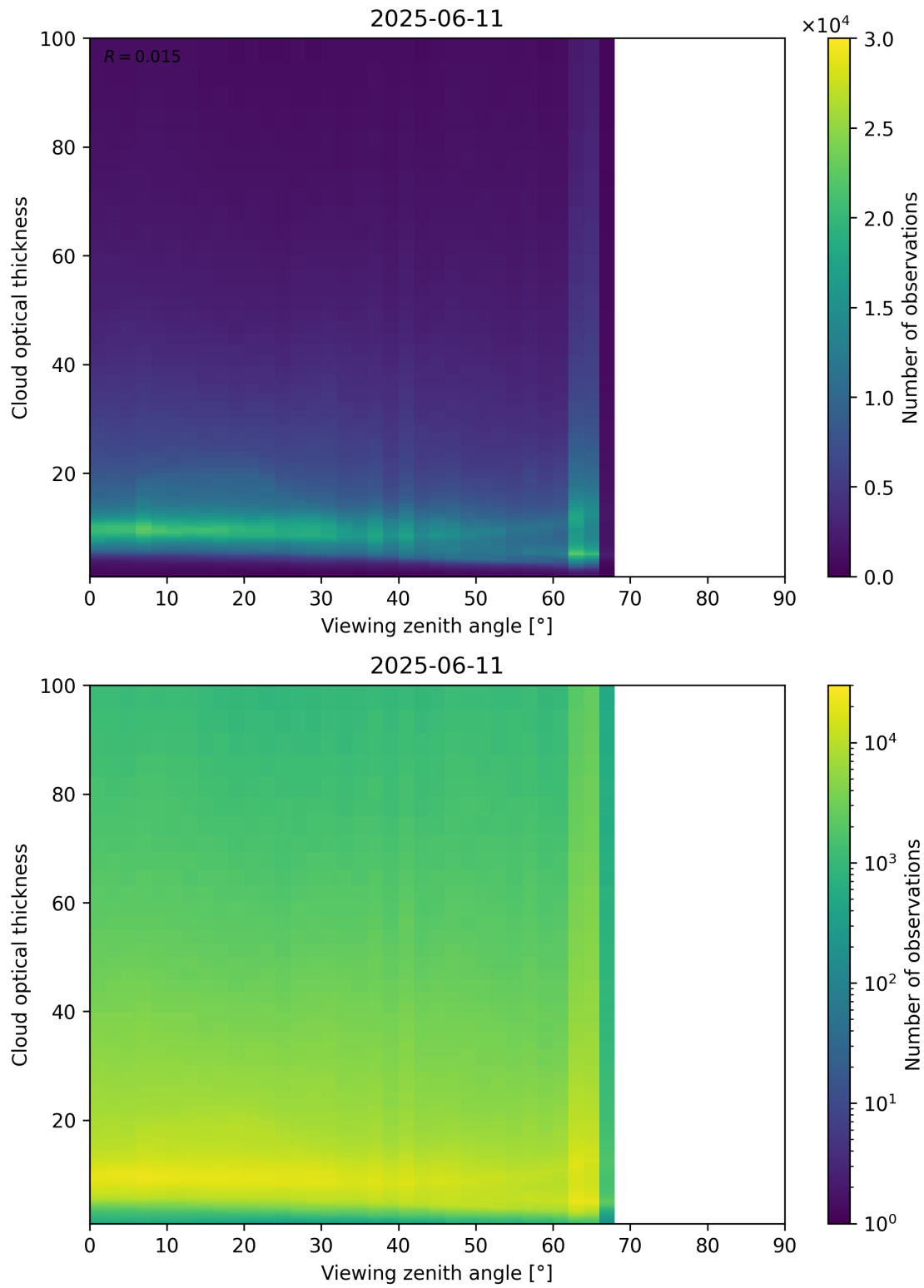
Figure 111: Scatter density plot of “Viewing zenith angle” against “Cloud optical thickness” for 2025-06-11 to 2025-06-12.
