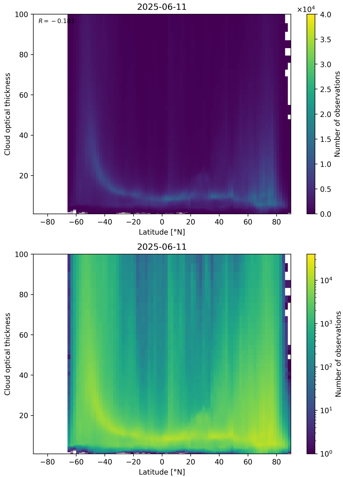
Figure 96: Scatter density plot of “Latitude” against “Cloud optical thickness” for 2025-06-11 to 2025-06-12.
