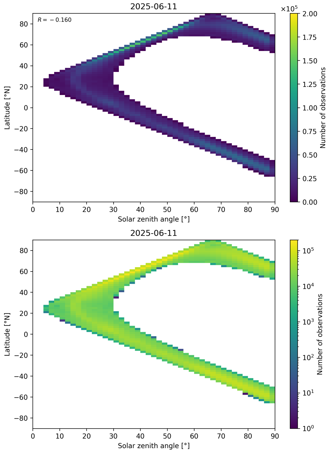
Figure 105: Scatter density plot of “Solar zenith angle” against “Latitude” for 2025-06-11 to 2025-06-12.
