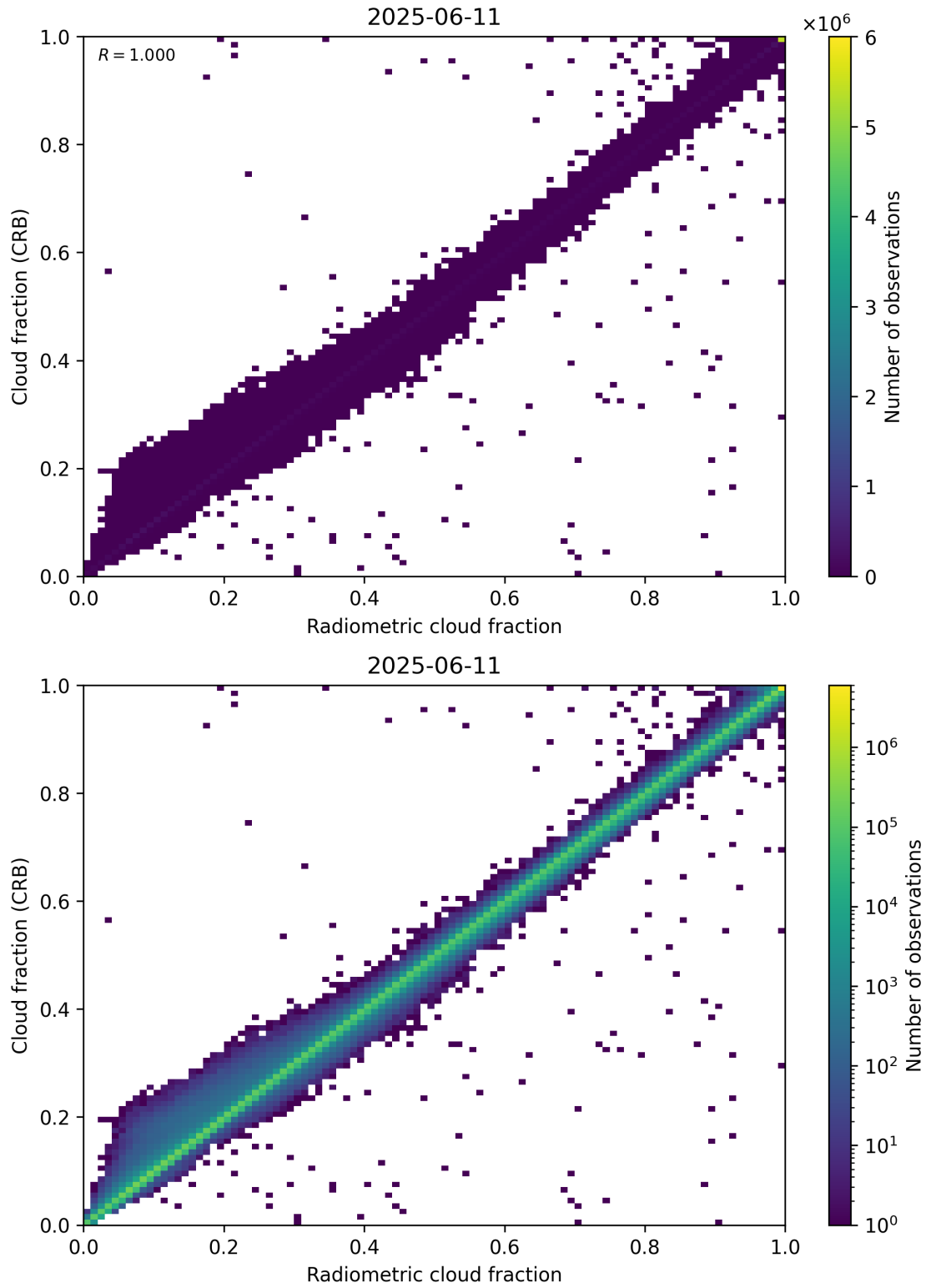
Figure 73: Scatter density plot of “Radiometric cloud fraction” against “Cloud fraction (CRB)” for 2025-06-11 to 2025-06-12.
