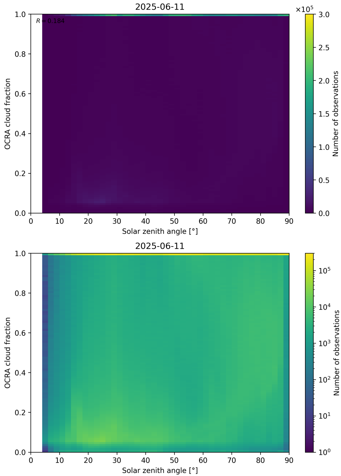
Figure 100: Scatter density plot of “Solar zenith angle” against “OCRA cloud fraction” for 2025-06-11 to 2025-06-12.
