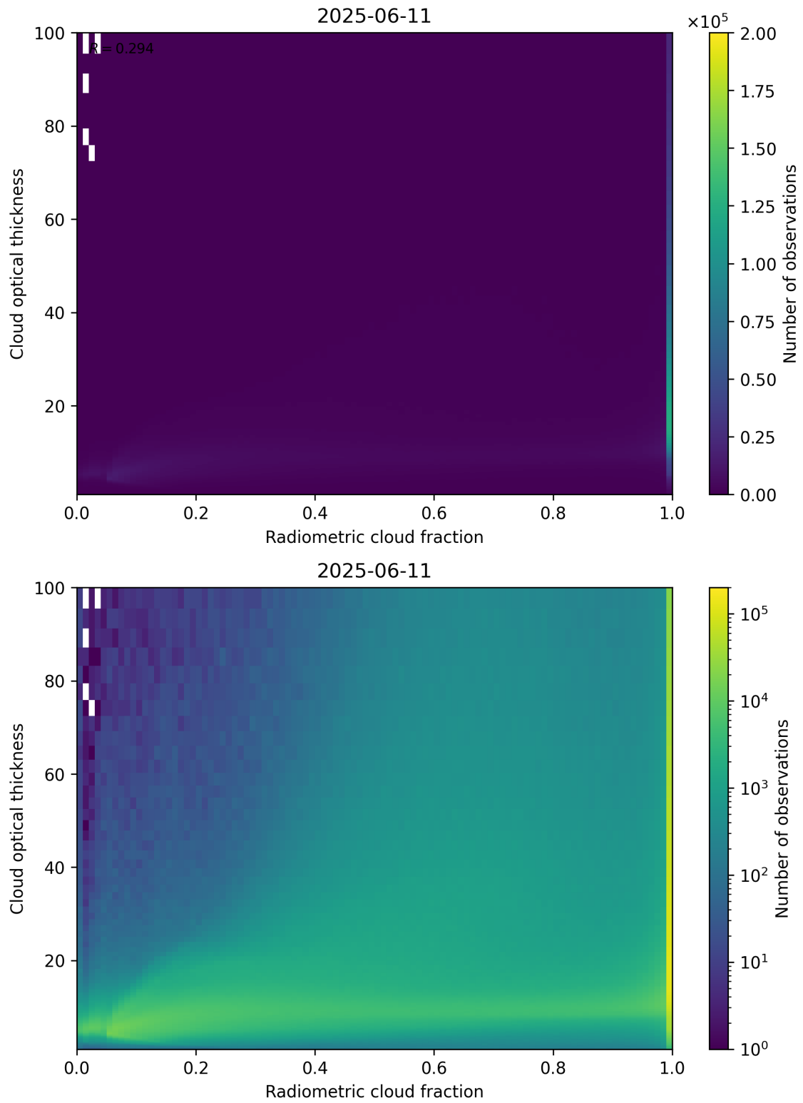
Figure 75: Scatter density plot of “Radiometric cloud fraction” against “Cloud optical thickness” for 2025-06-11 to 2025-06-12.
