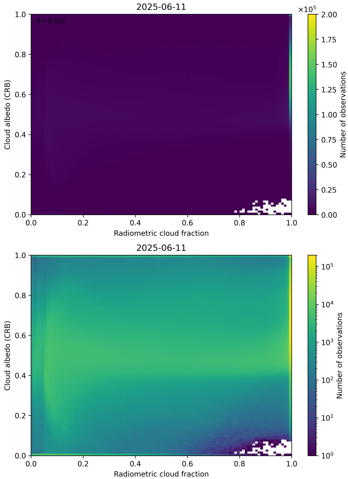
Figure 71: Scatter density plot of “Radiometric cloud fraction” against “Cloud albedo (CRB)” for 2025-06-11 to 2025-06-12.
