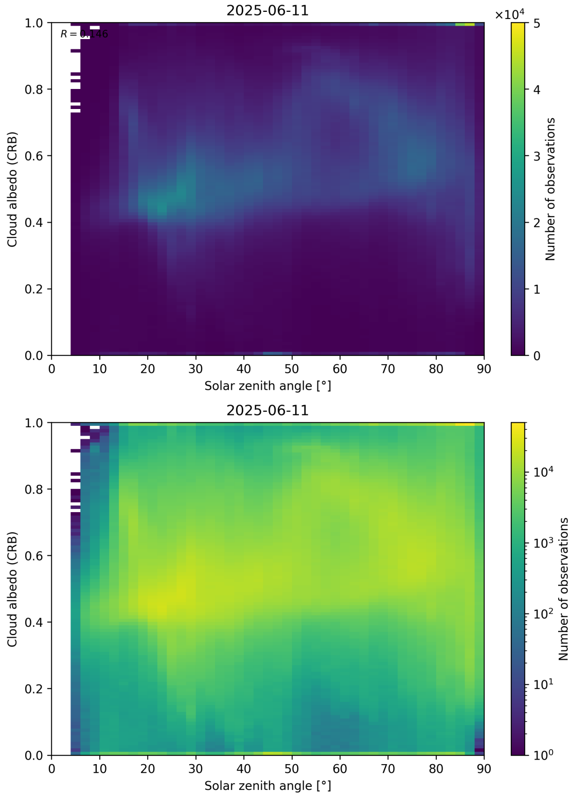
Figure 98: Scatter density plot of “Solar zenith angle” against “Cloud albedo (CRB)” for 2025-06-11 to 2025-06-12.
