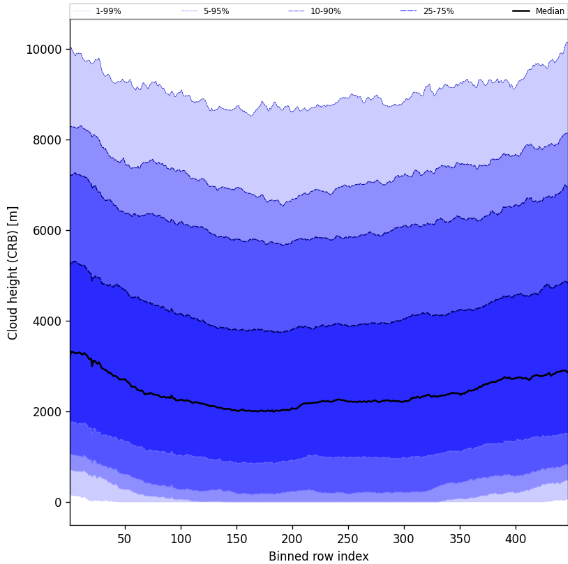
Figure 59: Along track statistics of “Cloud height (CRB)” for 2025-06-11 to 2025-06-12
