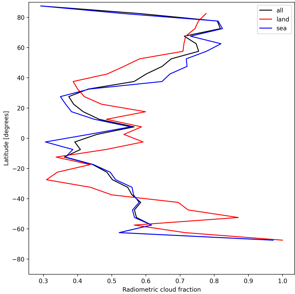
Figure 23: Zonal average of “Radiometric cloud fraction” for 2025-06-11 to 2025-06-12.
