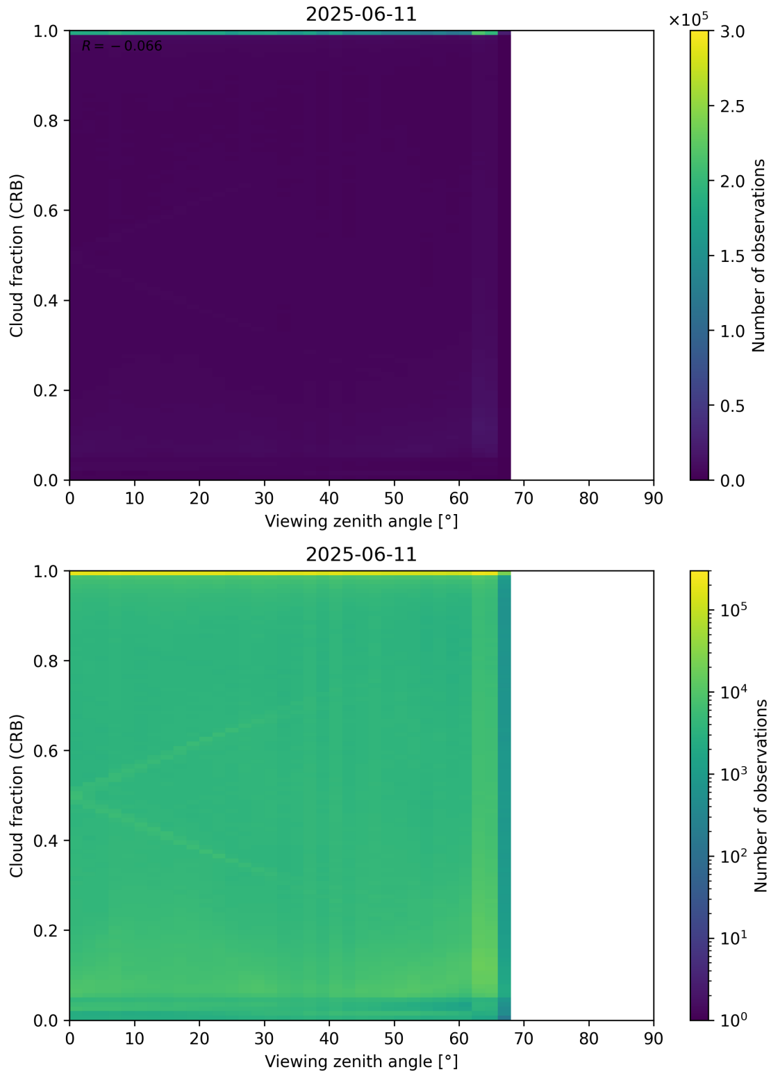
Figure 109: Scatter density plot of “Viewing zenith angle” against “Cloud fraction (CRB)” for 2025-06-11 to 2025-06-12.
