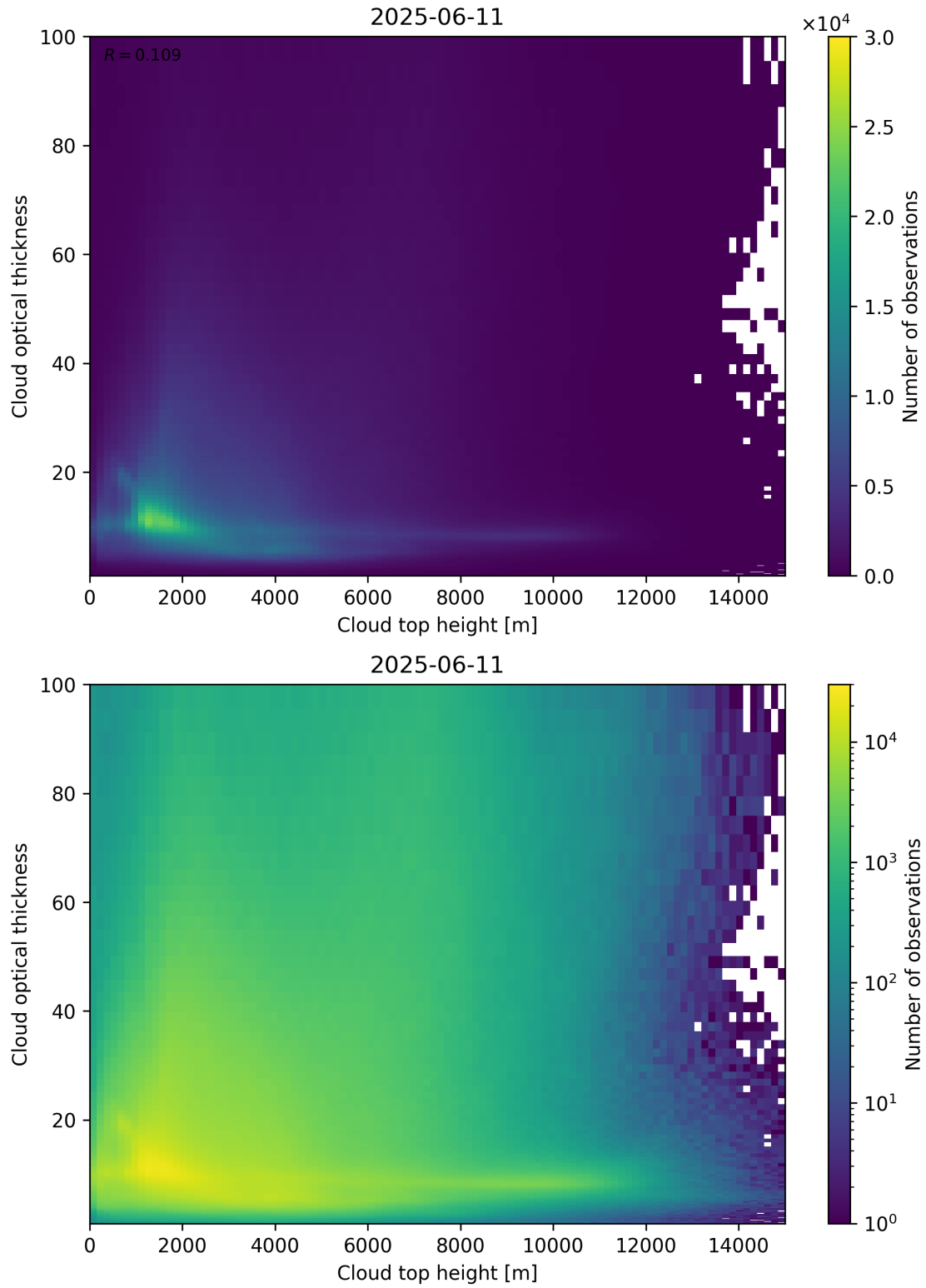
Figure 90: Scatter density plot of “Cloud top height” against “Cloud optical thickness” for 2025-06-11 to 2025-06-12.
