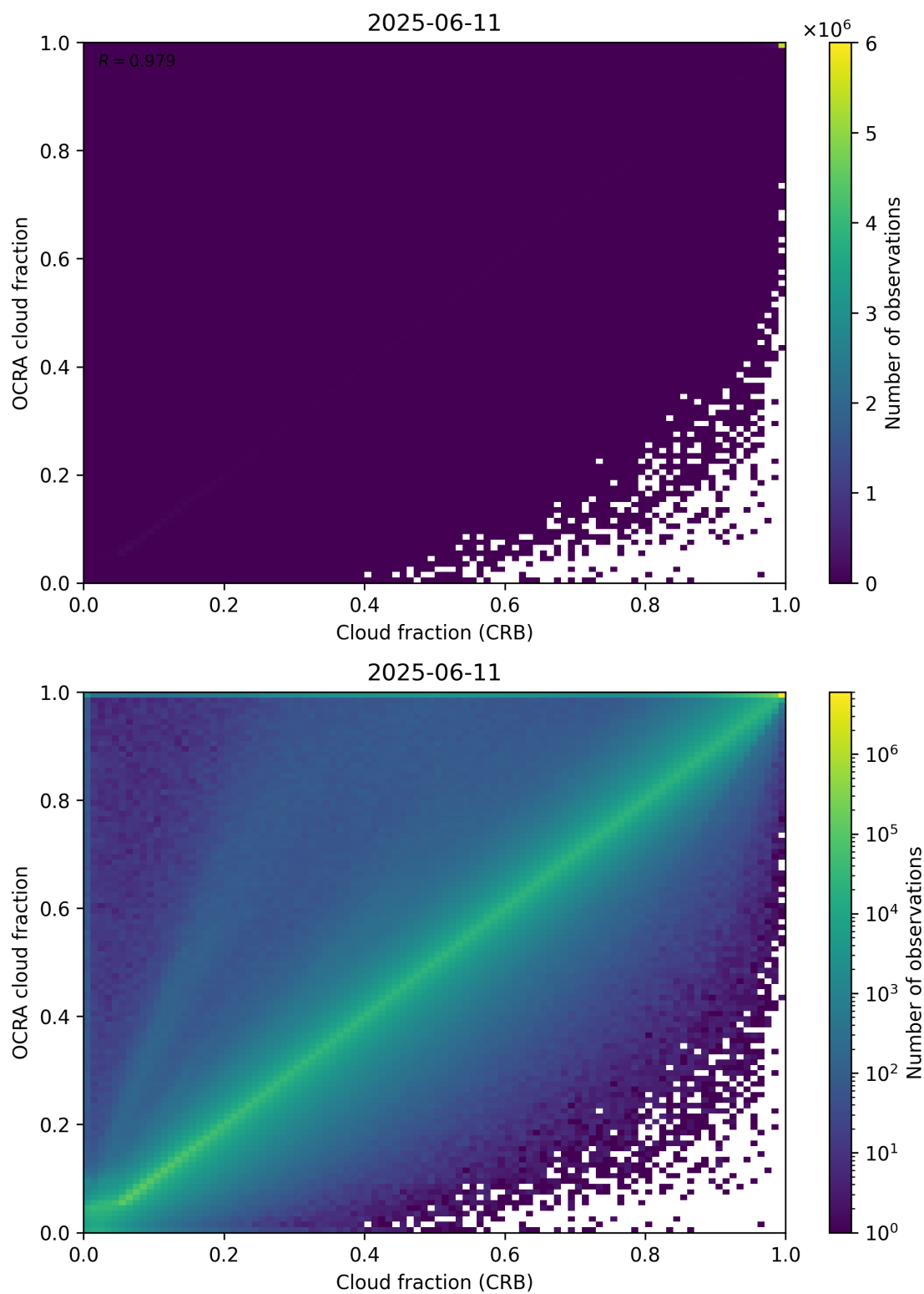
Figure 78: Scatter density plot of “Cloud fraction (CRB)” against “OCRA cloud fraction” for 2025-06-11 to 2025-06-12.
