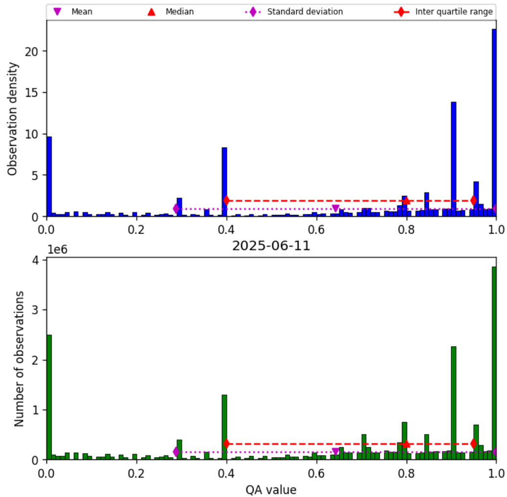
Figure 38: Histogram of “QA value” for 2025-06-11 to 2025-06-12
