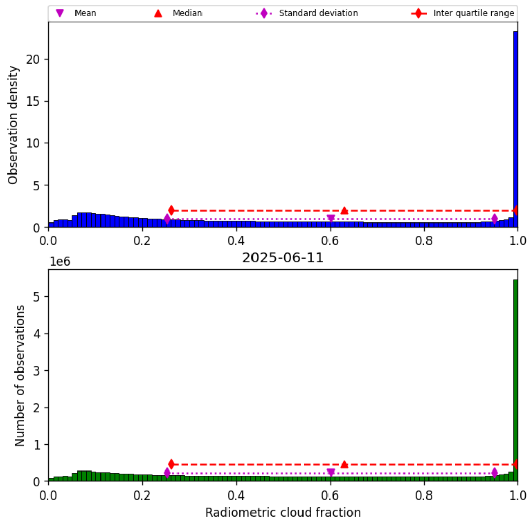
Figure 39: Histogram of “Radiometric cloud fraction” for 2025-06-11 to 2025-06-12
