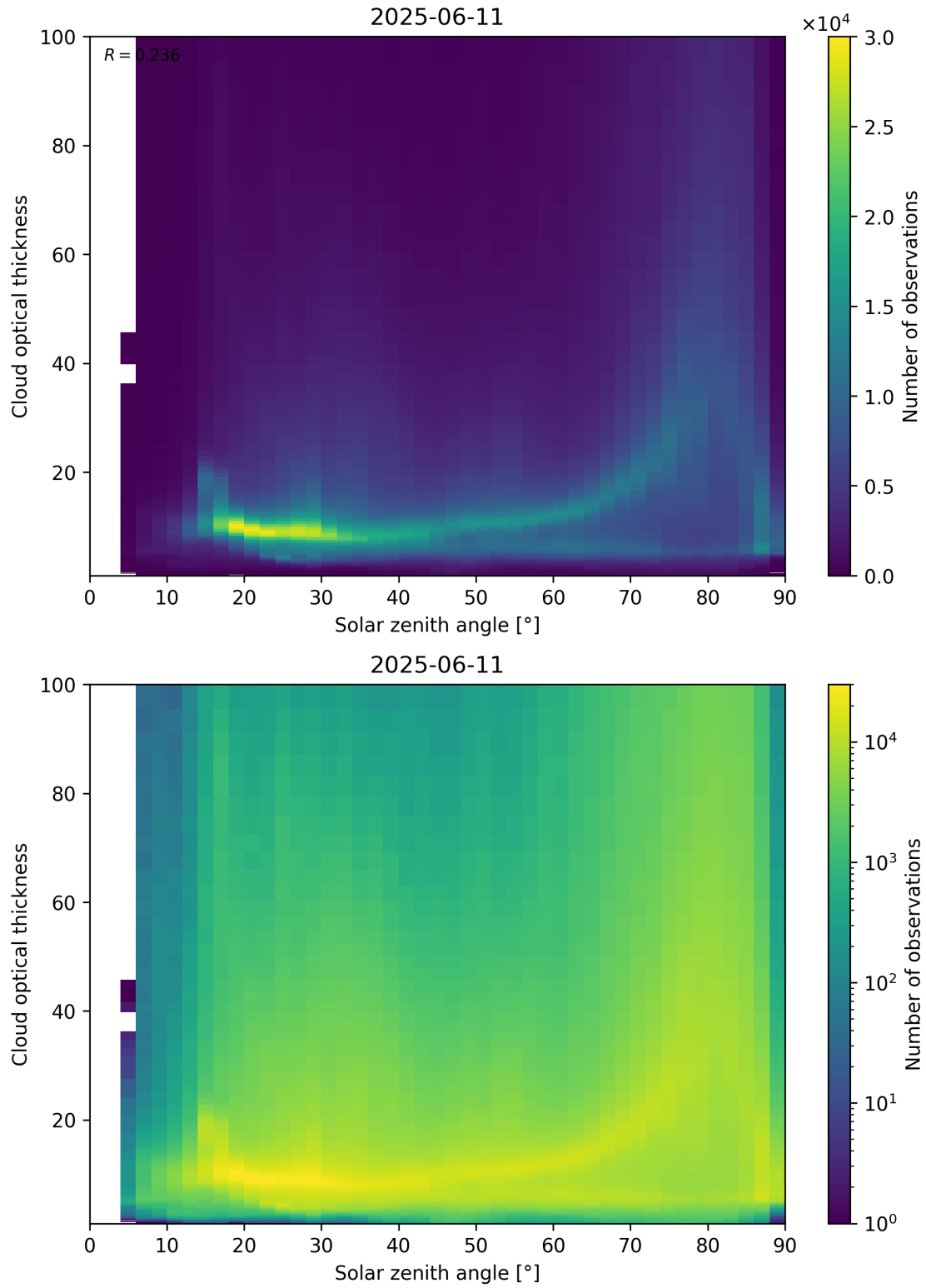
Figure 103: Scatter density plot of “Solar zenith angle” against “Cloud optical thickness” for 2025-06-11 to 2025-06-12.
