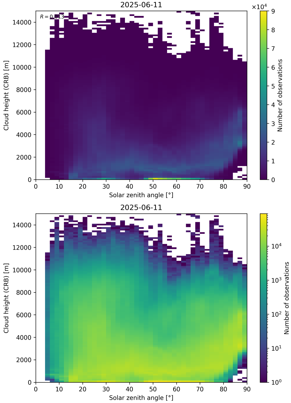
Figure 102: Scatter density plot of “Solar zenith angle” against “Cloud height (CRB)” for 2025-06-11 to 2025-06-12.
