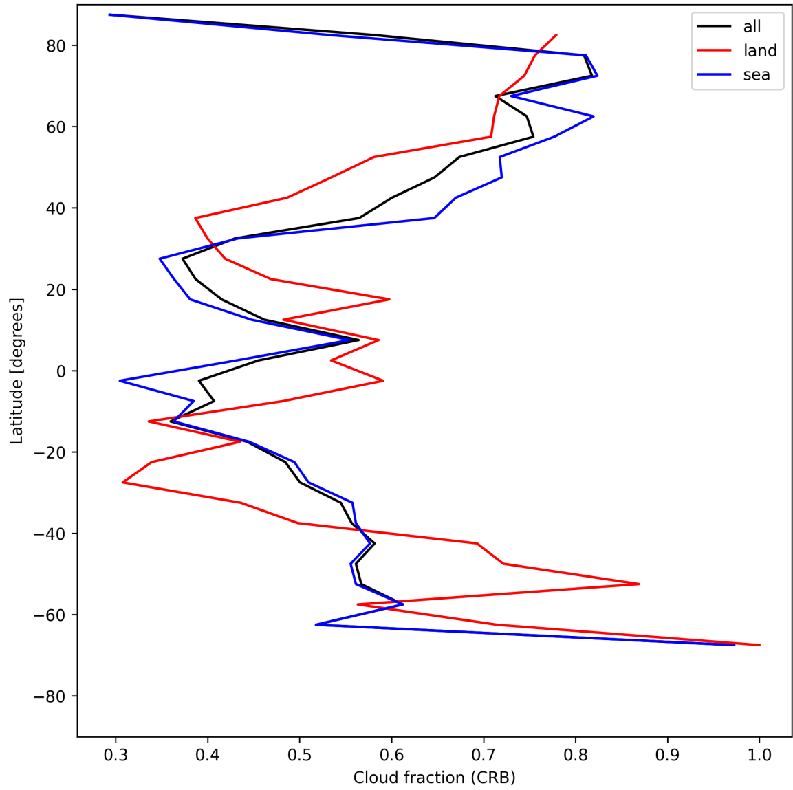
Figure 26: Zonal average of “Cloud fraction (CRB)” for 2025-06-11 to 2025-06-12.
