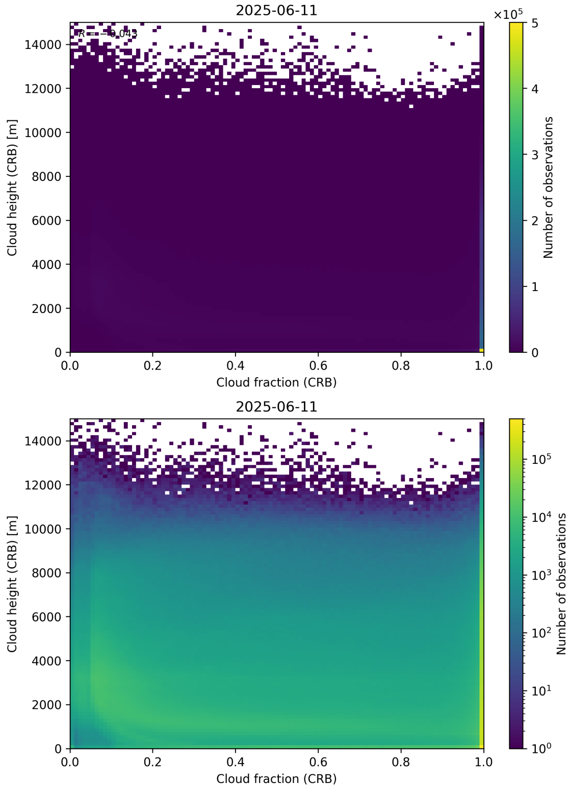
Figure 79: Scatter density plot of “Cloud fraction (CRB)” against “Cloud height (CRB)” for 2025-06-11 to 2025-06-12.
