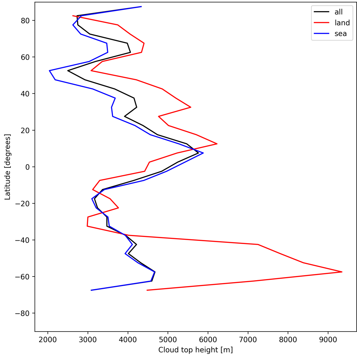
Figure 24: Zonal average of “Cloud top height” for 2025-06-11 to 2025-06-12.
