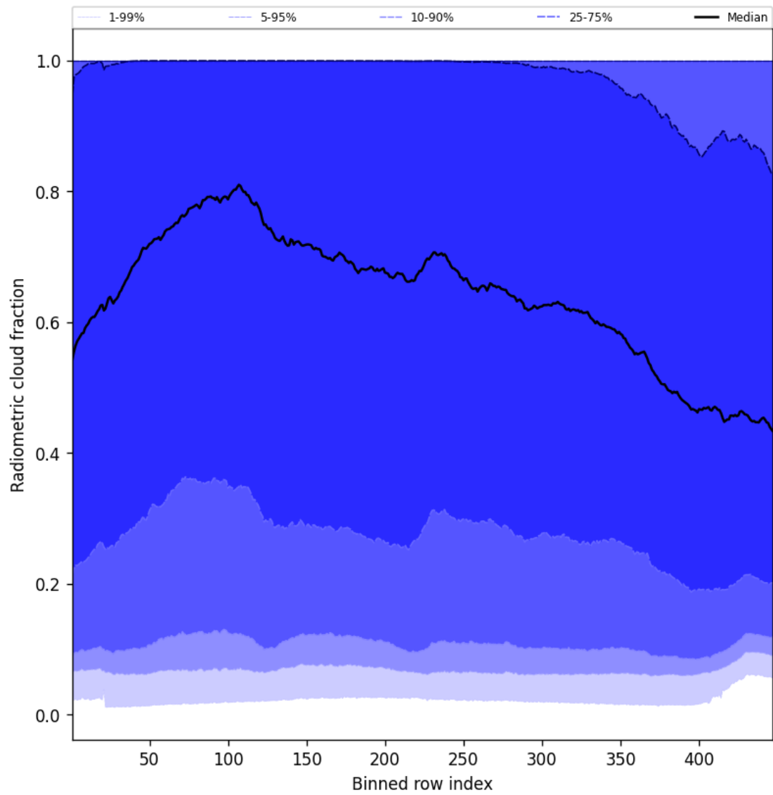
Figure 55: Along track statistics of “Radiometric cloud fraction” for 2025-06-11 to 2025-06-12
