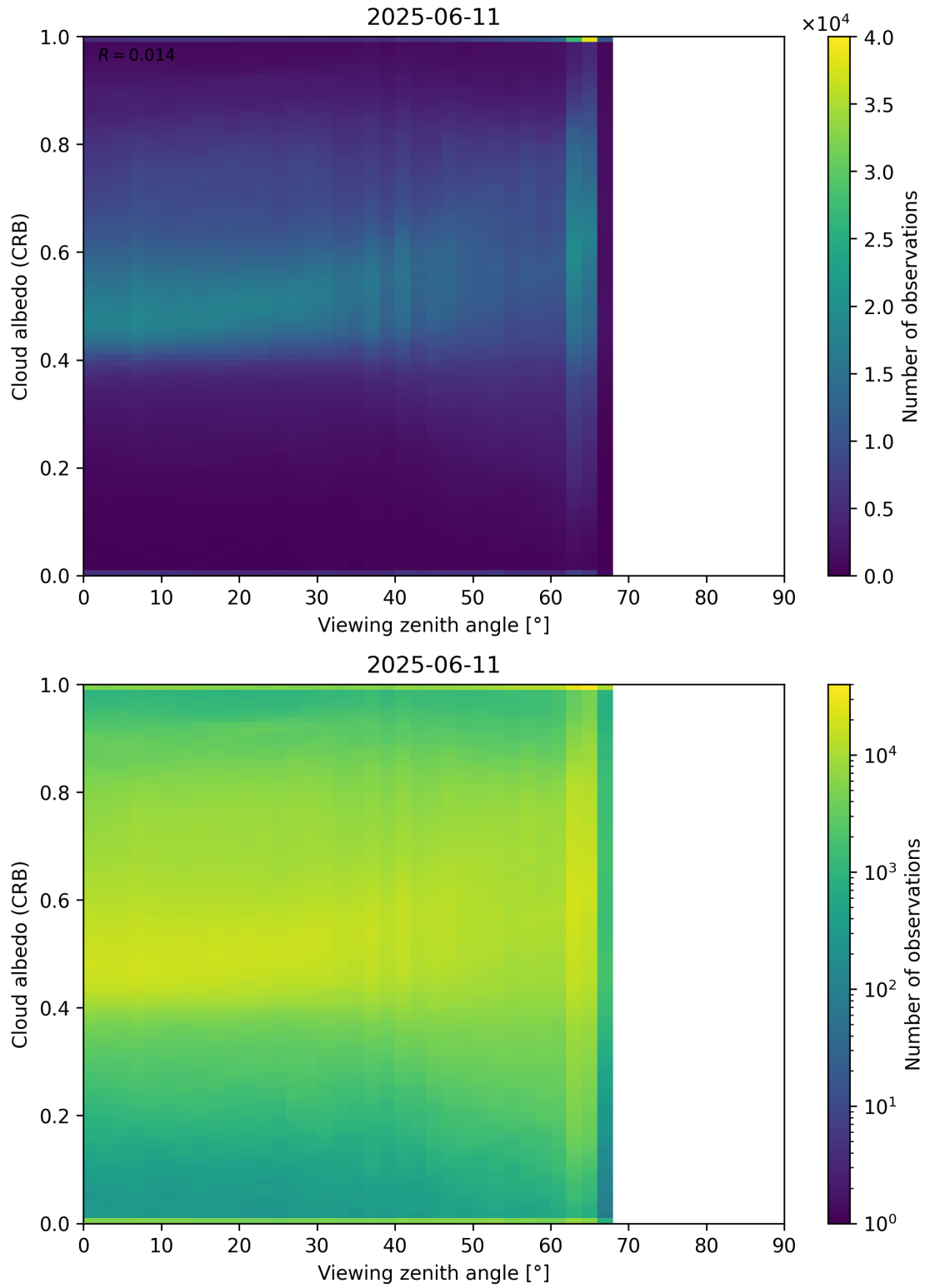
Figure 106: Scatter density plot of “Viewing zenith angle” against “Cloud albedo (CRB)” for 2025-06-11 to 2025-06-12.
