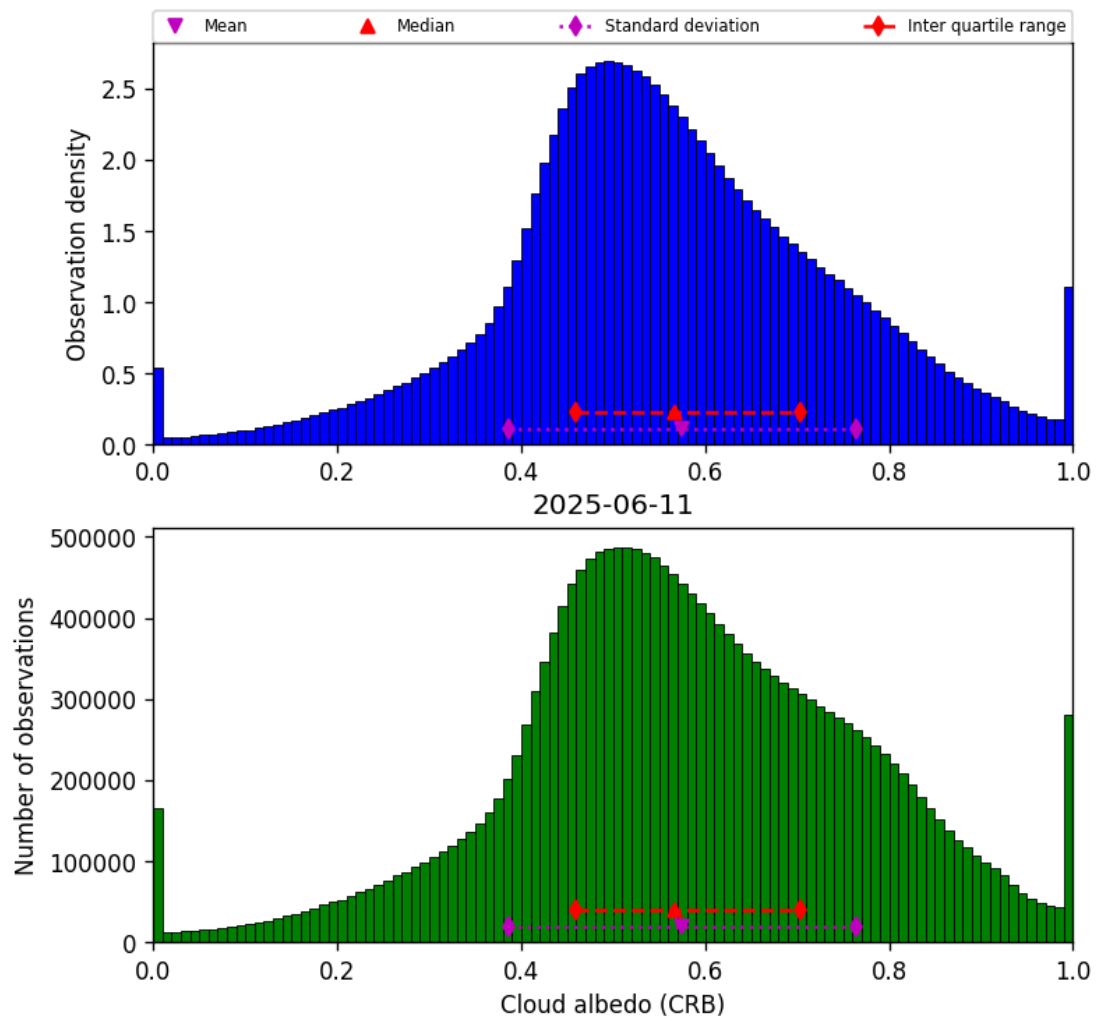
Figure 44: Histogram of “Cloud albedo (CRB)” for 2025-06-11 to 2025-06-12
