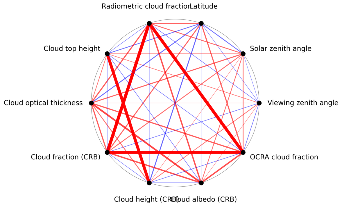
Figure 1: Map of correlation graph for 2025-06-11 to 2025-06-12.
