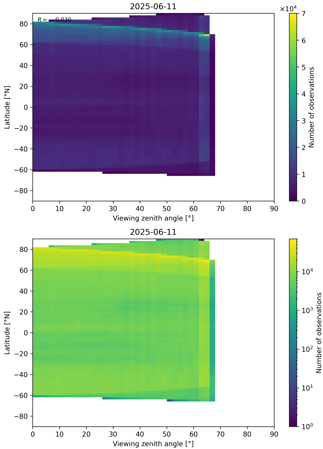
Figure 113: Scatter density plot of “Viewing zenith angle” against “Latitude” for 2025-06-11 to 2025-06-12.
