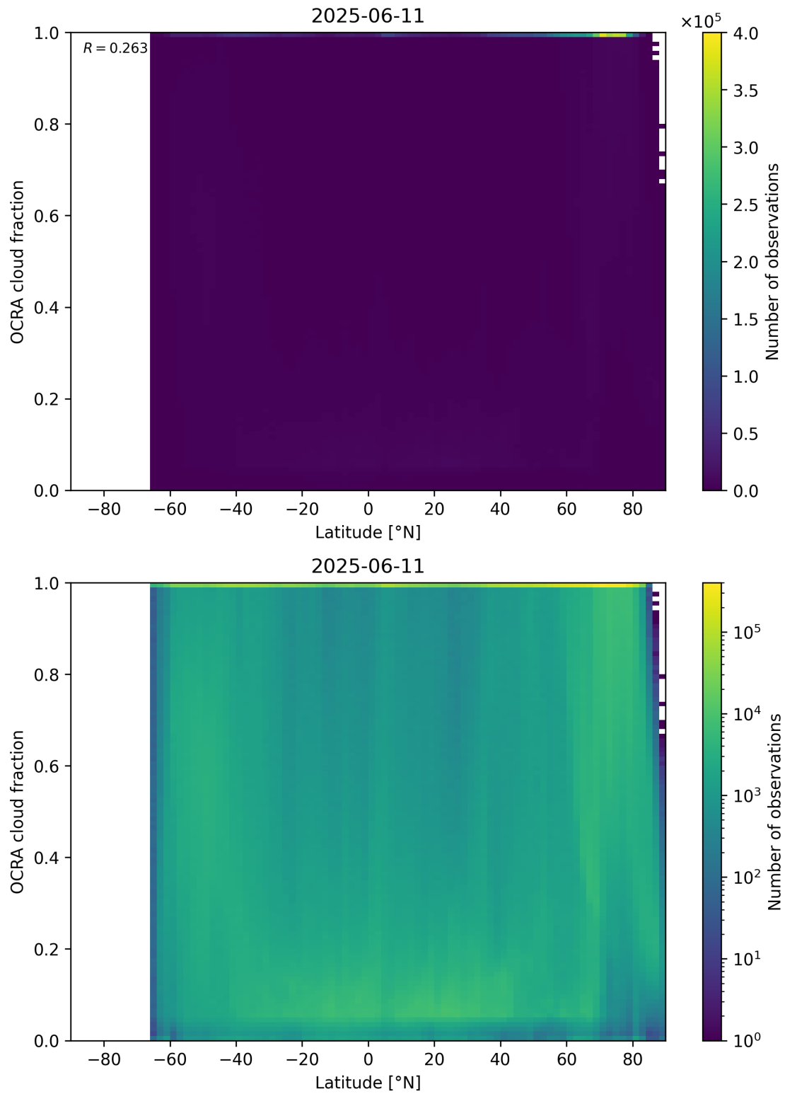
Figure 93: Scatter density plot of “Latitude” against “OCRA cloud fraction” for 2025-06-11 to 2025-06-12.
