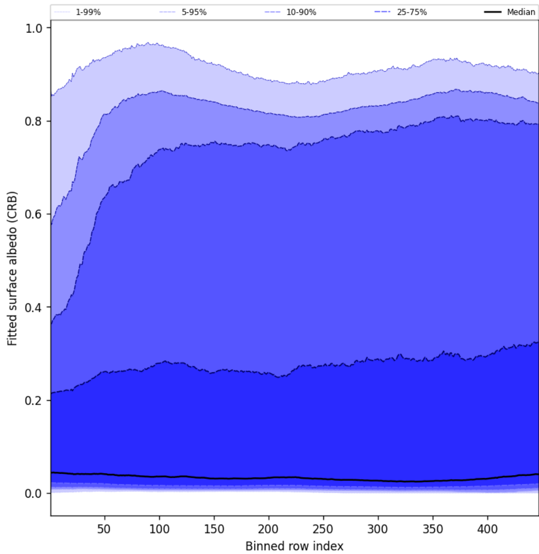
Figure 62: Along track statistics of “Fitted surface albedo (CRB)” for 2025-06-11 to 2025-06-12
