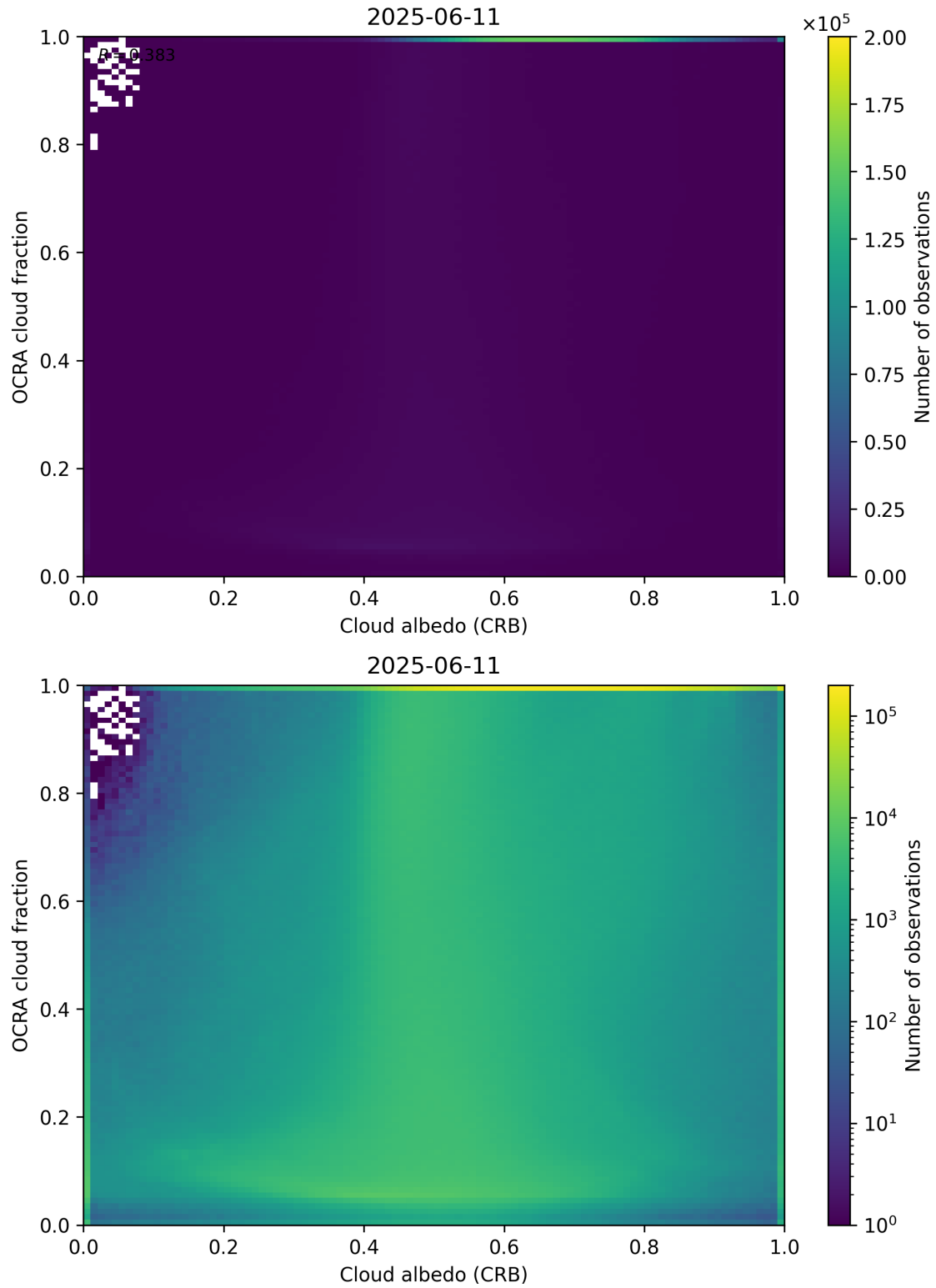
Figure 70: Scatter density plot of “Cloud albedo (CRB)” against “OCRA cloud fraction” for 2025-06-11 to 2025-06-12.
