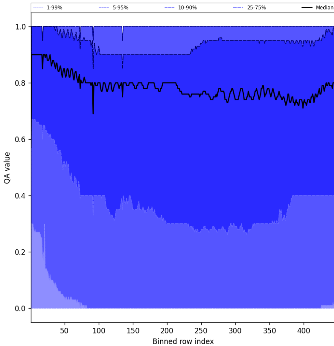
Figure 54: Along track statistics of “QA value” for 2025-06-11 to 2025-06-12
