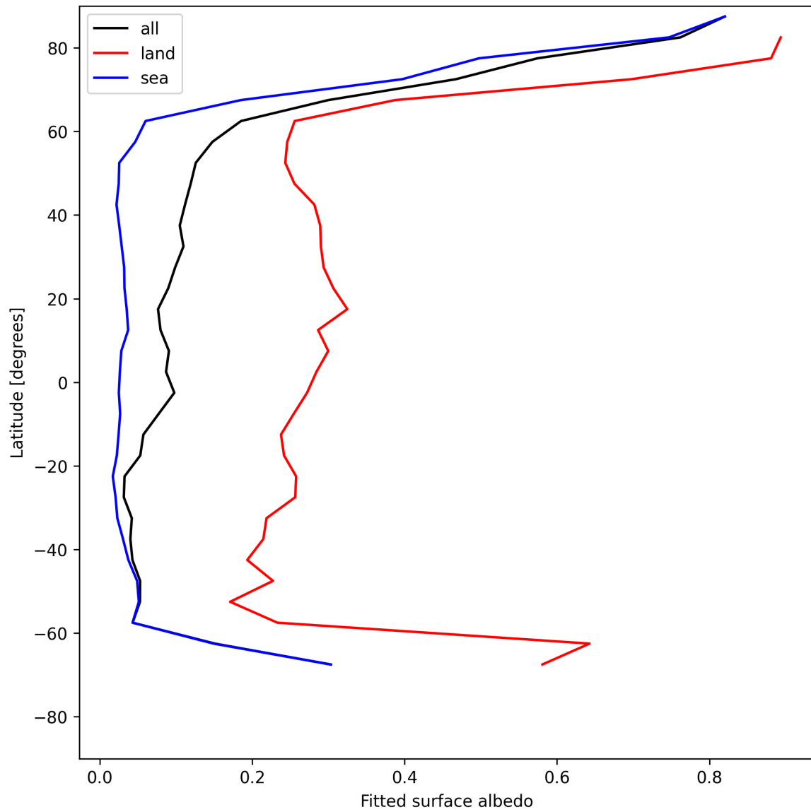
Figure 29: Zonal average of “Fitted surface albedo” for 2025-06-11 to 2025-06-12.
