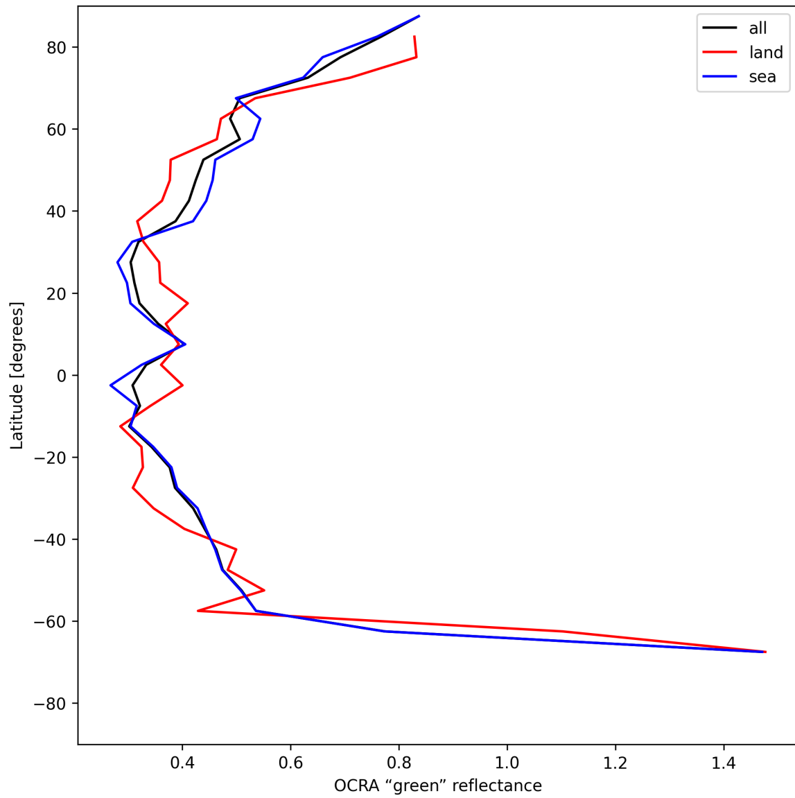
Figure 36: Zonal average of “OCRA “green” reflectance” for 2025-06-11 to 2025-06-12.
