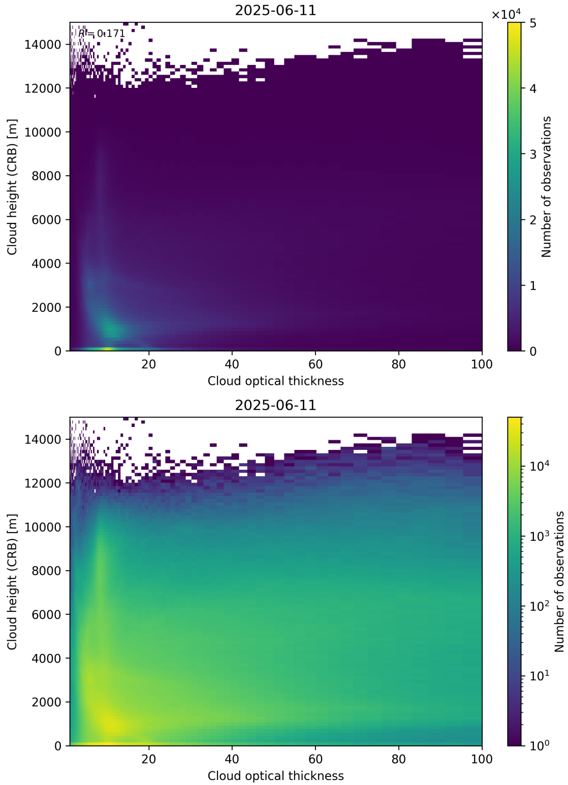
Figure 85: Scatter density plot of “Cloud optical thickness” against “Cloud height (CRB)” for 2025-06-11 to 2025-06-12.
