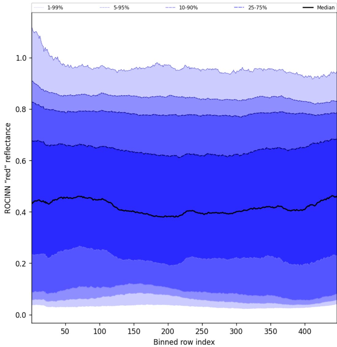
Figure 69: Along track statistics of “ROCINN “red” reflectance” for 2025-06-11 to 2025-06-12
