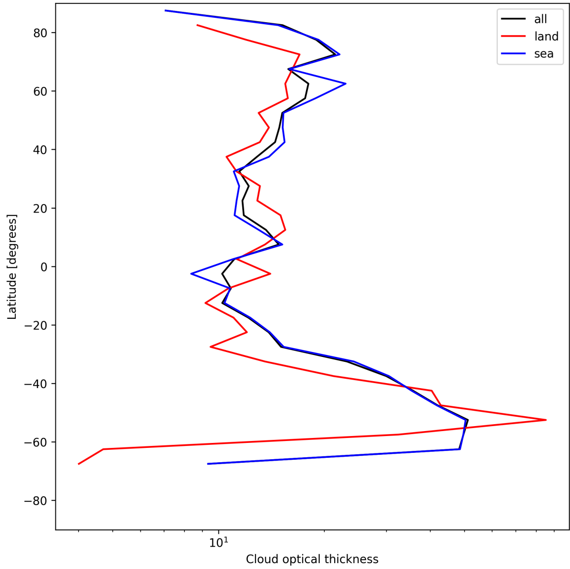
Figure 25: Zonal average of “Cloud optical thickness” for 2025-06-11 to 2025-06-12.
