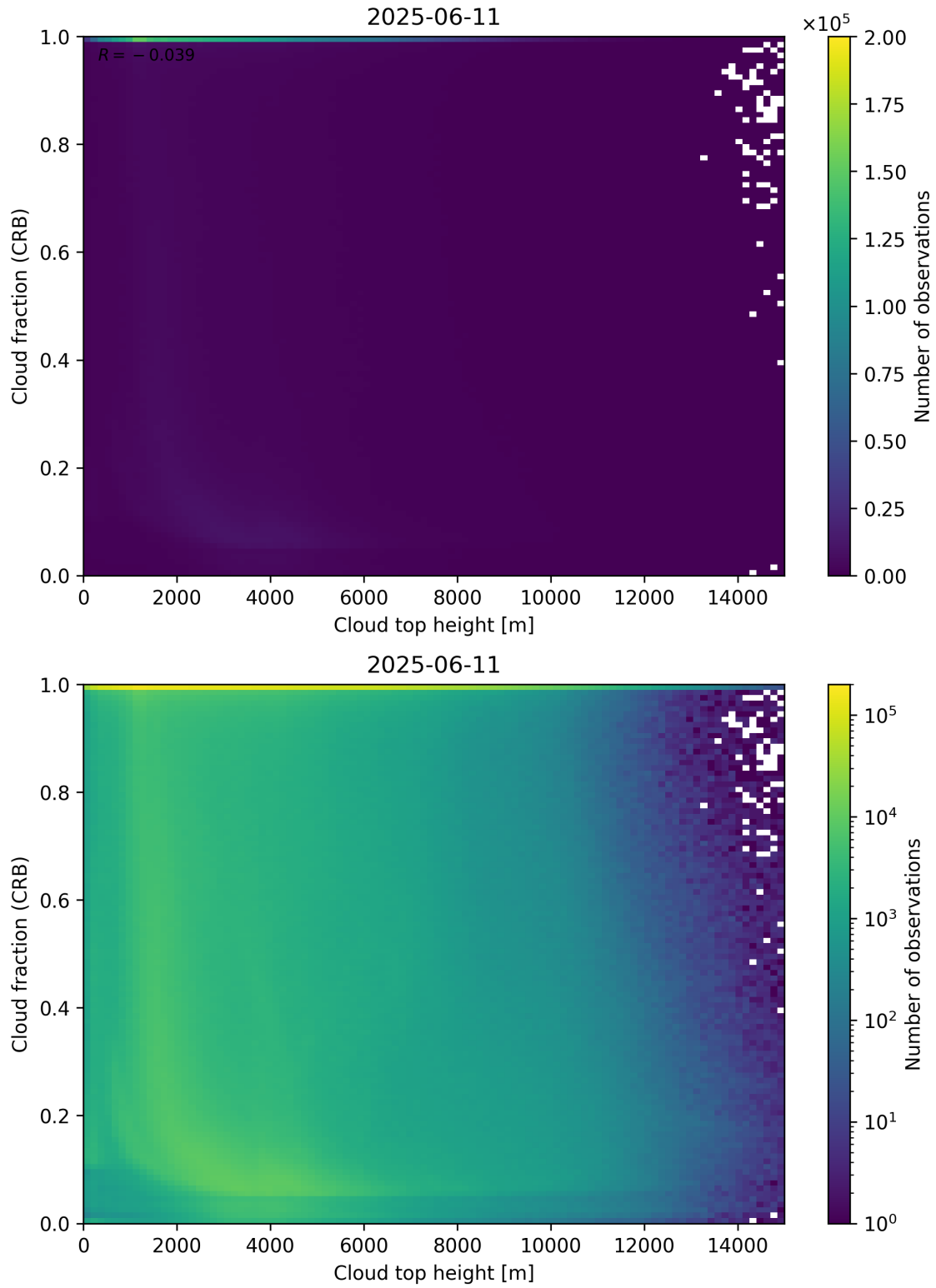
Figure 88: Scatter density plot of “Cloud top height” against “Cloud fraction (CRB)” for 2025-06-11 to 2025-06-12.
