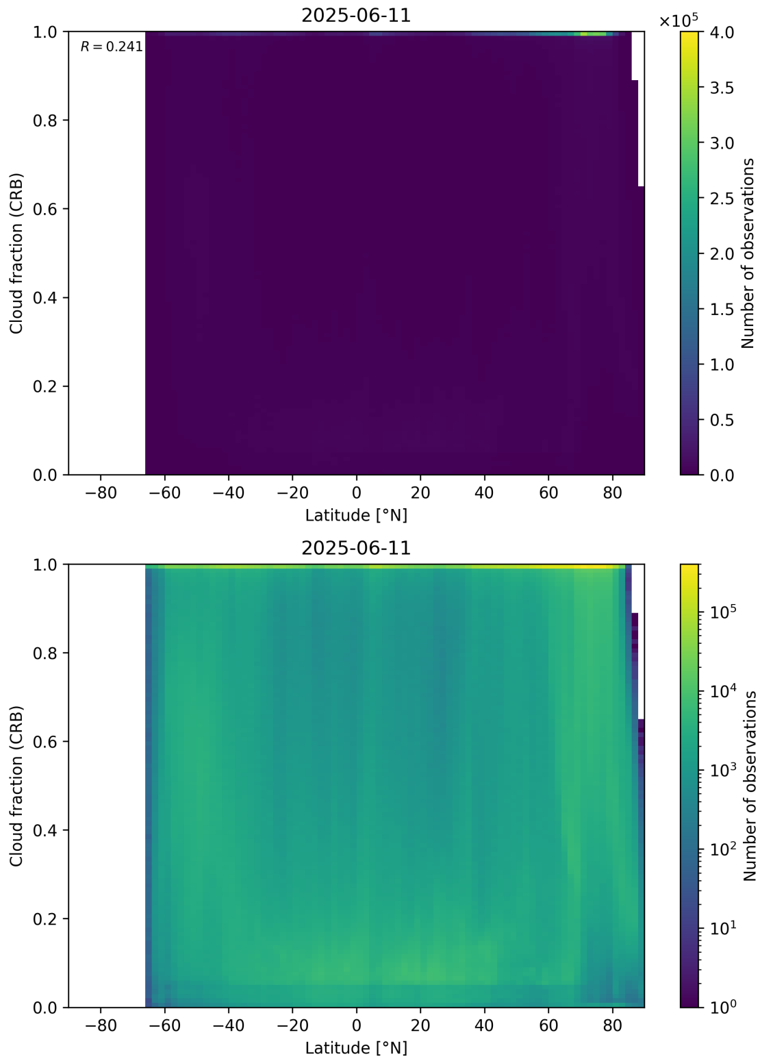
Figure 94: Scatter density plot of “Latitude” against “Cloud fraction (CRB)” for 2025-06-11 to 2025-06-12.
