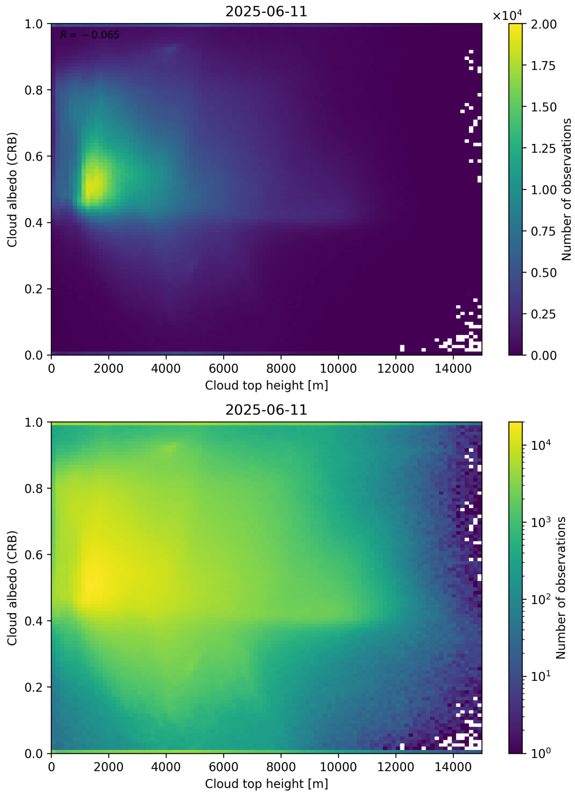
Figure 86: Scatter density plot of “Cloud top height” against “Cloud albedo (CRB)” for 2025-06-11 to 2025-06-12.
