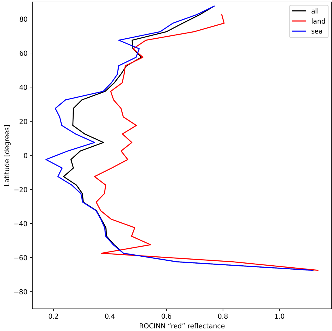
Figure 37: Zonal average of “ROCINN “red” reflectance” for 2025-06-11 to 2025-06-12.
