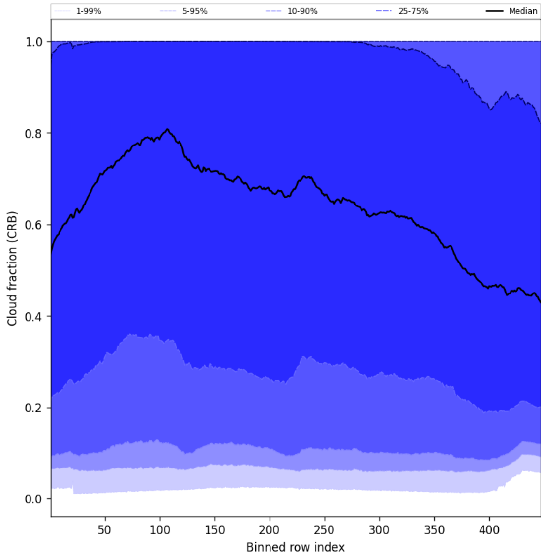
Figure 58: Along track statistics of “Cloud fraction (CRB)” for 2025-06-11 to 2025-06-12
