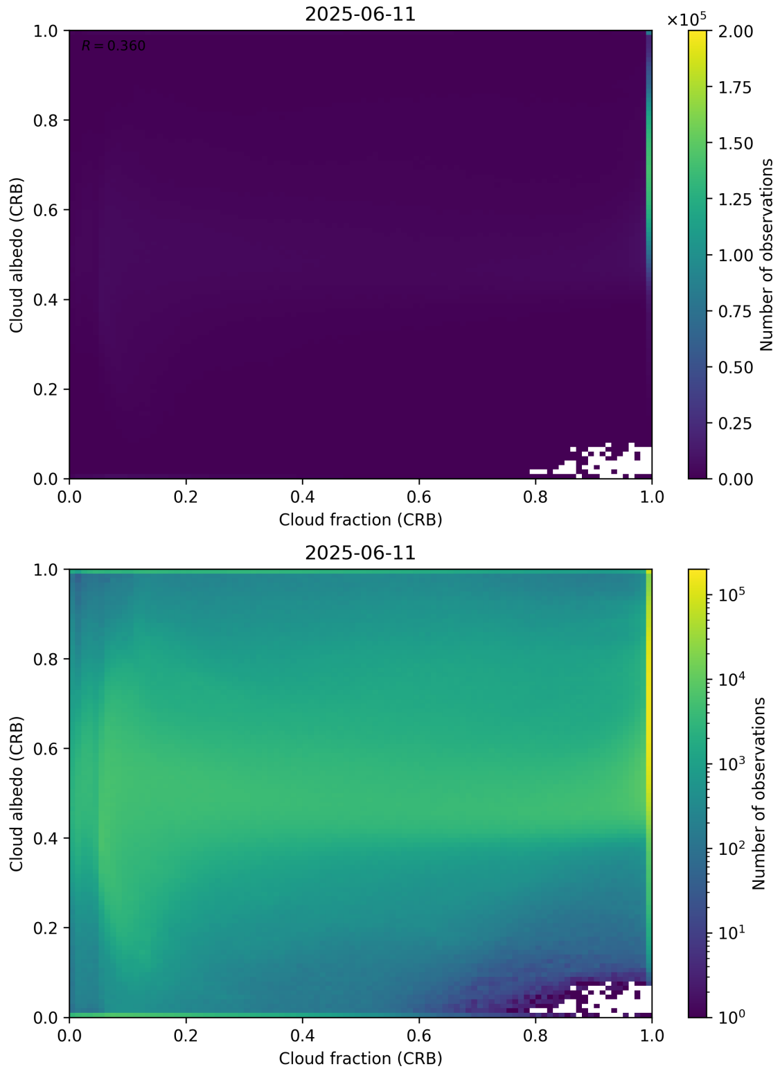
Figure 77: Scatter density plot of “Cloud fraction (CRB)” against “Cloud albedo (CRB)” for 2025-06-11 to 2025-06-12.
