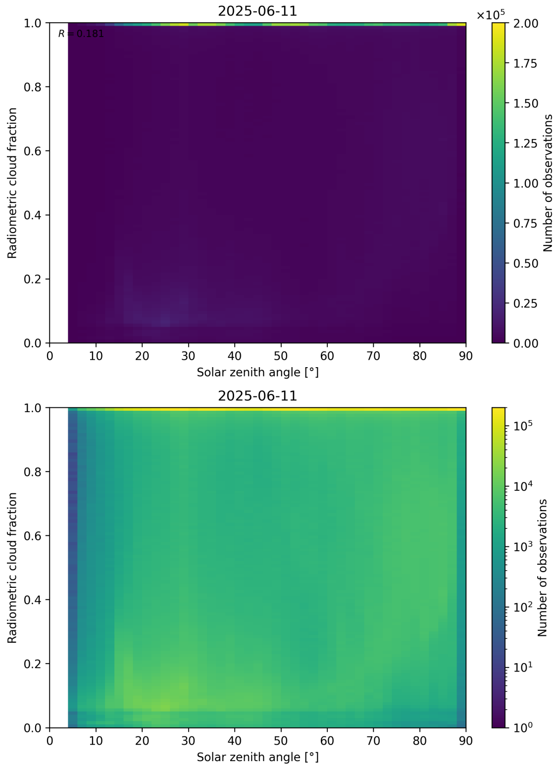
Figure 99: Scatter density plot of “Solar zenith angle” against “Radiometric cloud fraction” for 2025-06-11 to 2025-06-12.
