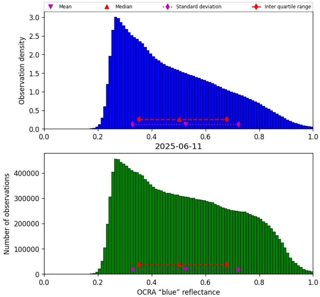
Figure 51: Histogram of “OCRA “blue” reflectance” for 2025-06-11 to 2025-06-12
