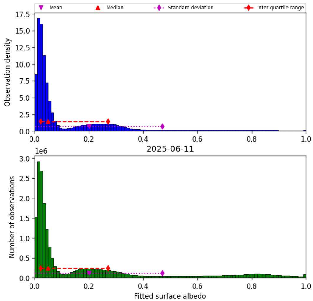
Figure 45: Histogram of “Fitted surface albedo” for 2025-06-11 to 2025-06-12
