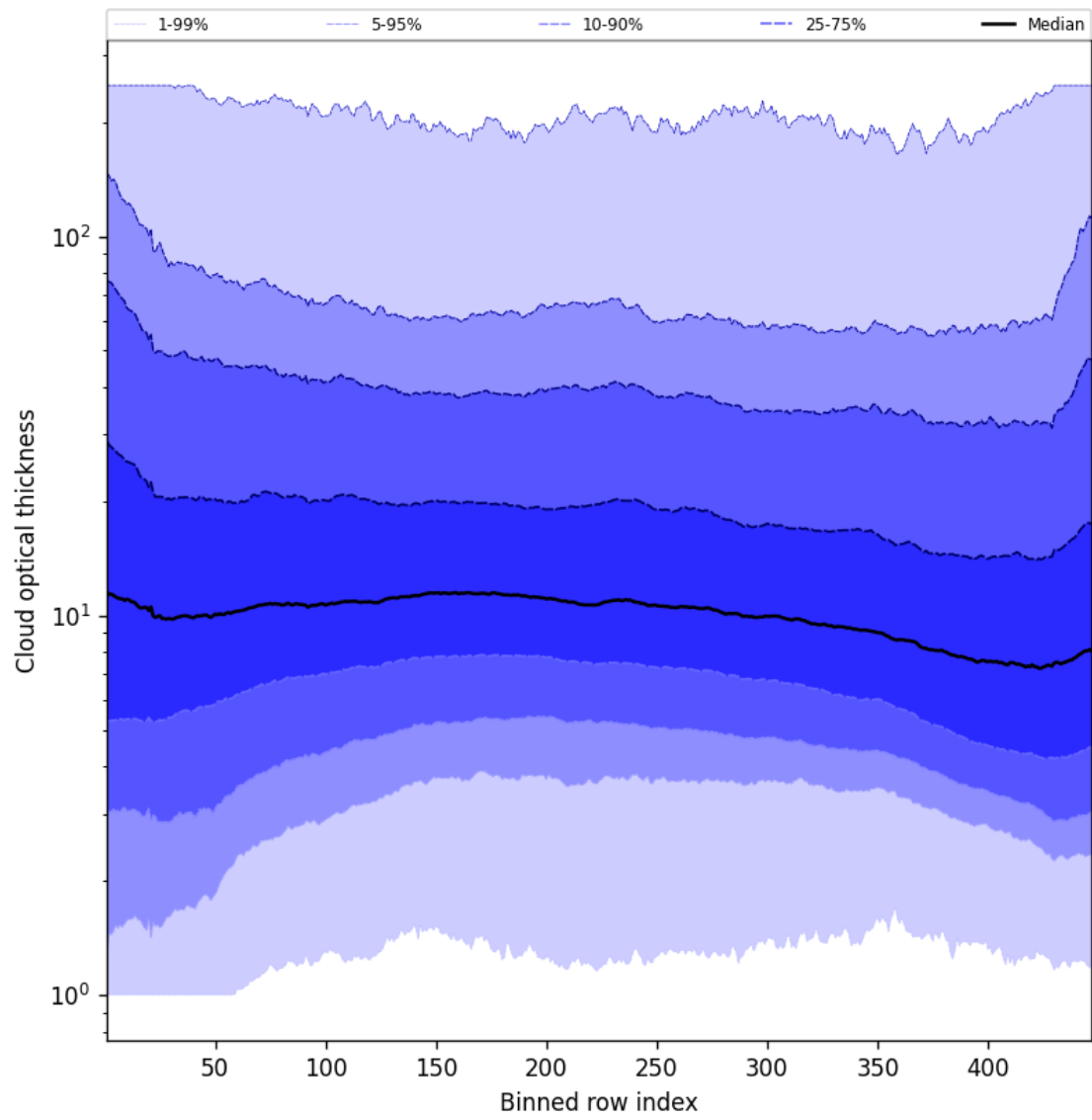
Figure 57: Along track statistics of “Cloud optical thickness” for 2025-06-11 to 2025-06-12
