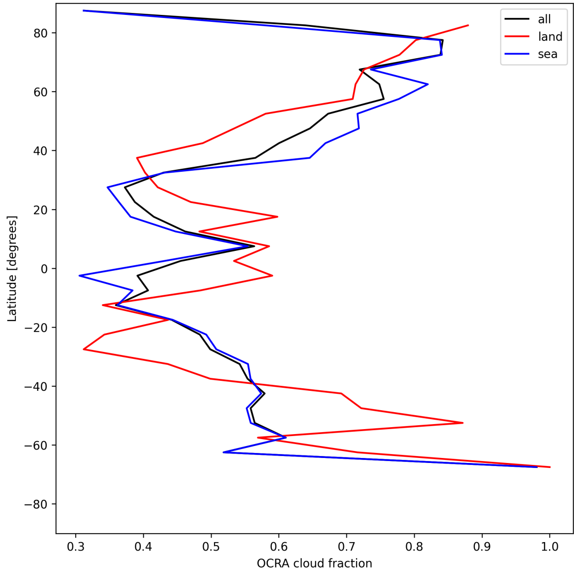
Figure 34: Zonal average of “OCRA cloud fraction” for 2025-06-11 to 2025-06-12.
