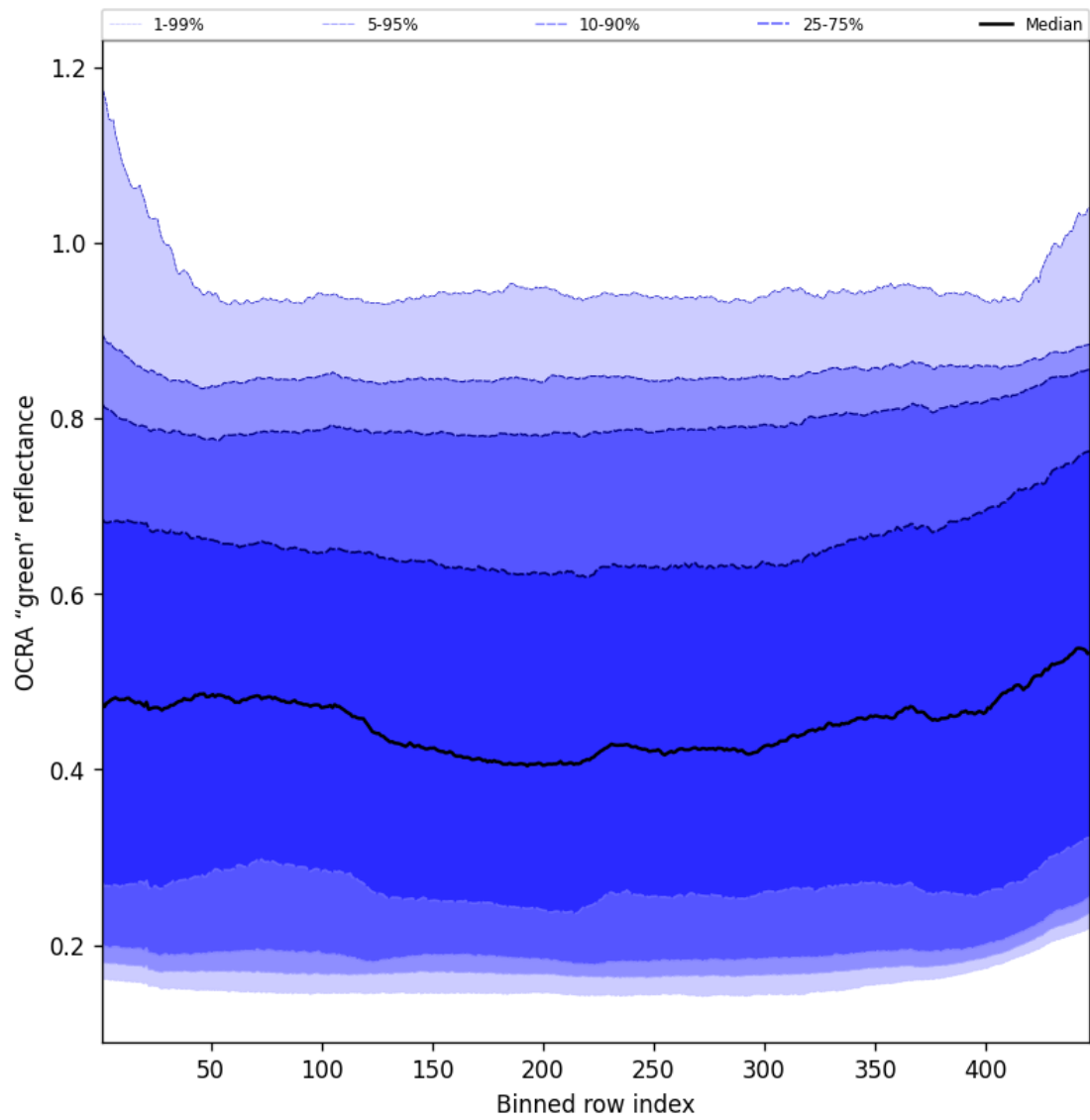
Figure 68: Along track statistics of “OCRA “green” reflectance” for 2025-06-11 to 2025-06-12
