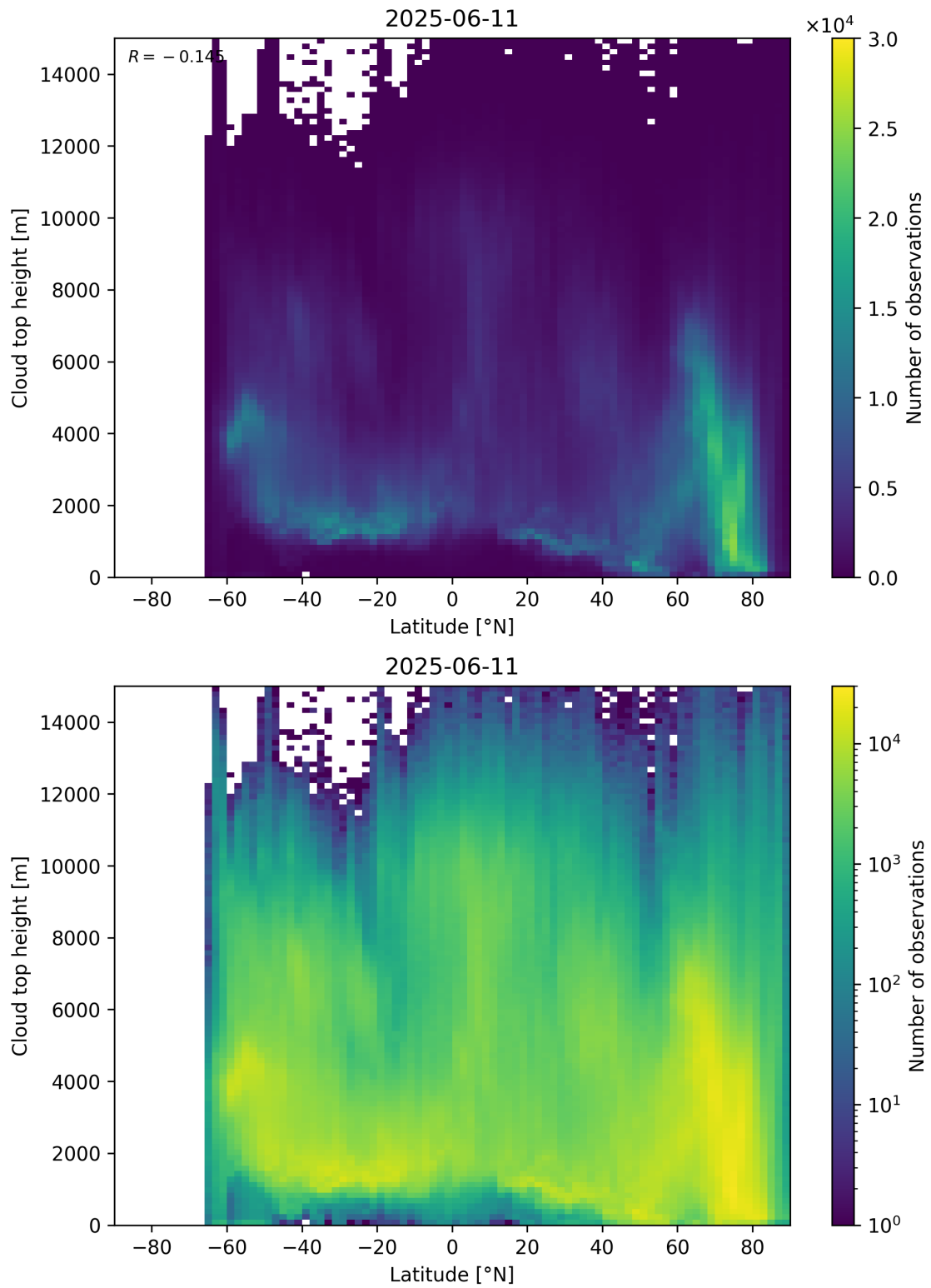
Figure 97: Scatter density plot of “Latitude” against “Cloud top height” for 2025-06-11 to 2025-06-12.
