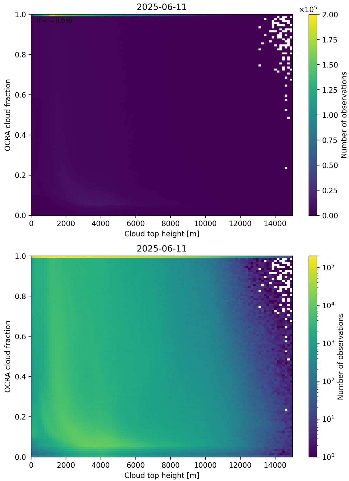
Figure 87: Scatter density plot of “Cloud top height” against “OCRA cloud fraction” for 2025-06-11 to 2025-06-12.
