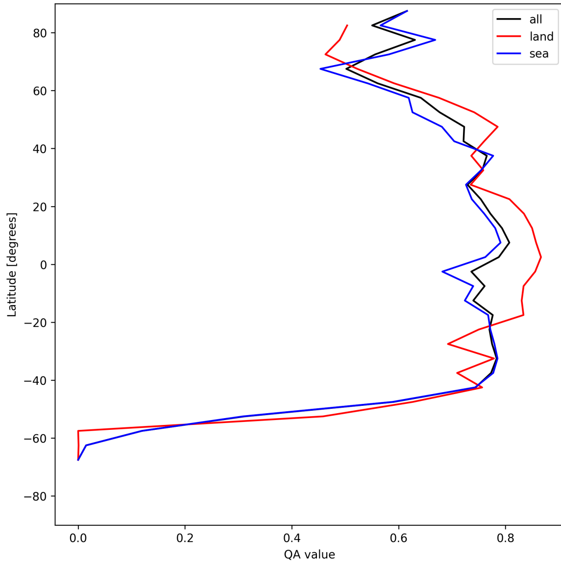
Figure 22: Zonal average of “QA value” for 2025-06-11 to 2025-06-12.
