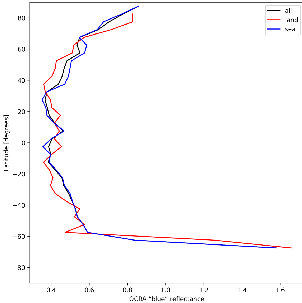
Figure 35: Zonal average of “OCRA “blue” reflectance” for 2025-06-11 to 2025-06-12.
