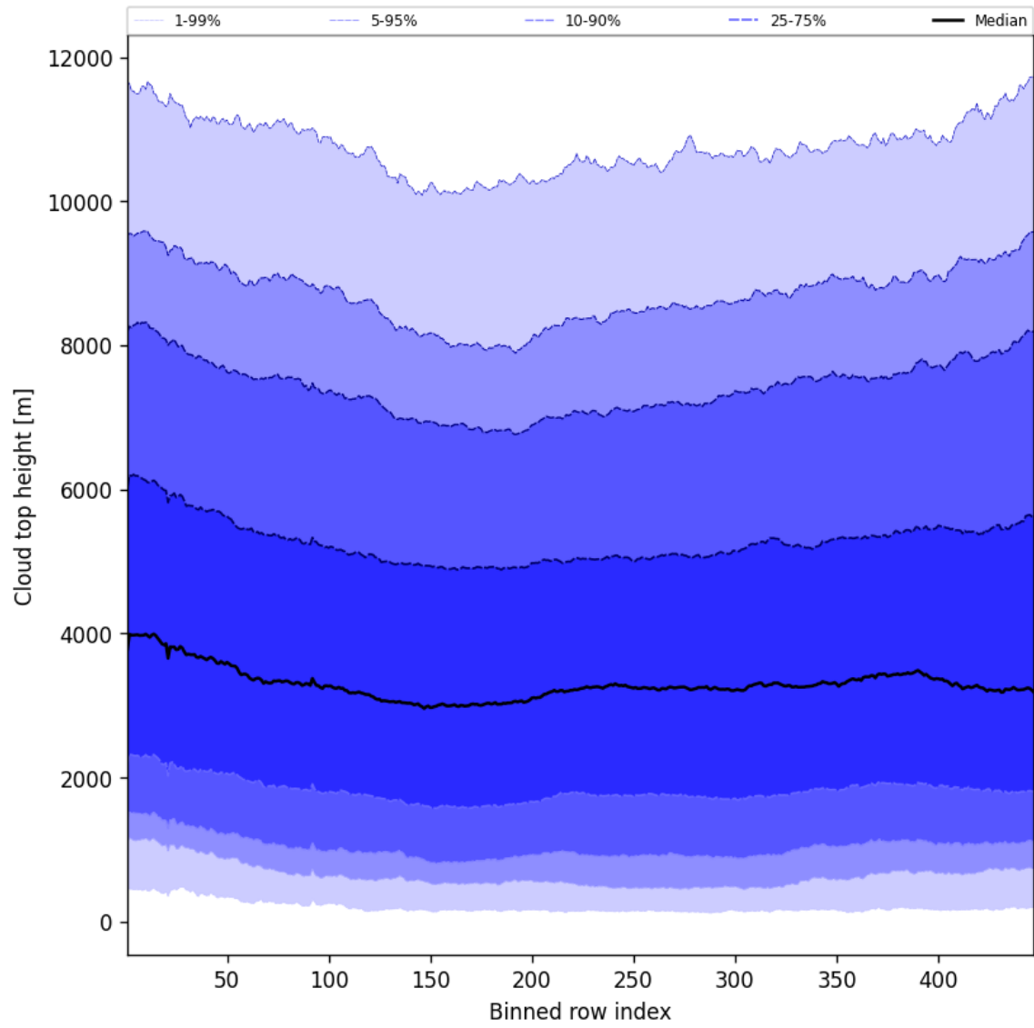
Figure 56: Along track statistics of “Cloud top height” for 2025-06-11 to 2025-06-12
