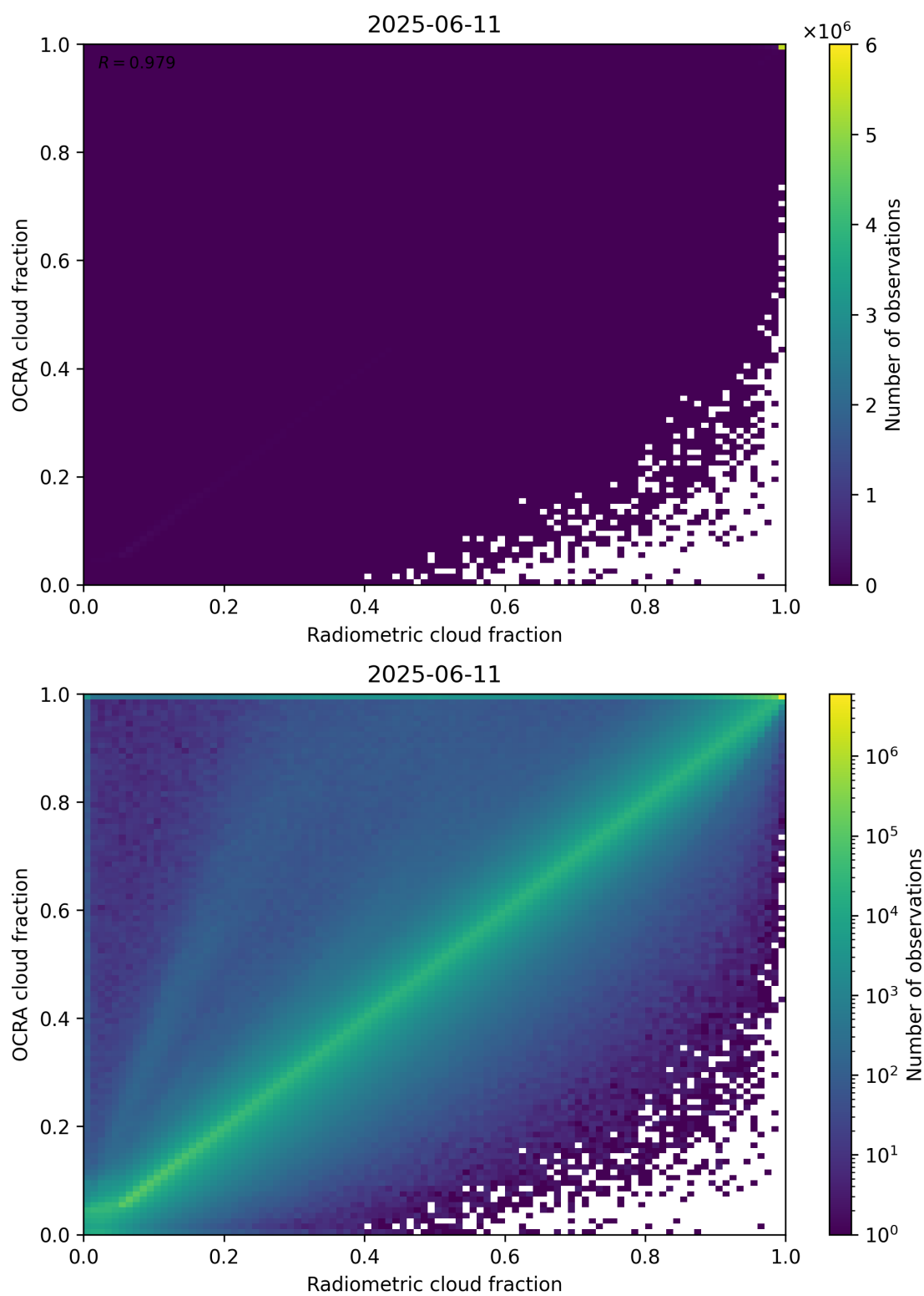
Figure 72: Scatter density plot of “Radiometric cloud fraction” against “OCRA cloud fraction” for 2025-06-11 to 2025-06-12.
