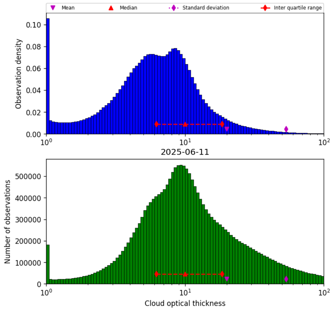
Figure 41: Histogram of “Cloud optical thickness” for 2025-06-11 to 2025-06-12
