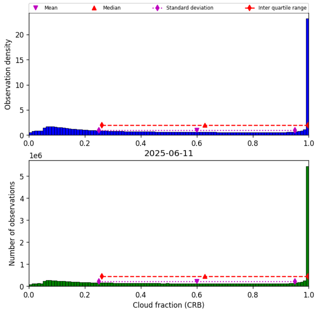
Figure 42: Histogram of "Cloud fraction (CRB)" for 2025-06-11 to 2025-06-12
