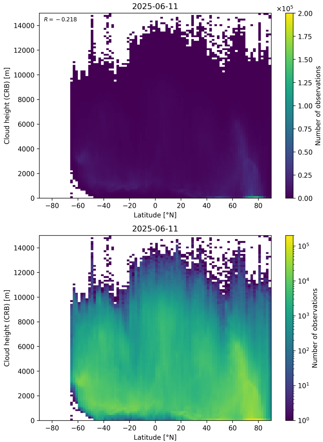
Figure 95: Scatter density plot of “Latitude” against “Cloud height (CRB)” for 2025-06-11 to 2025-06-12.
