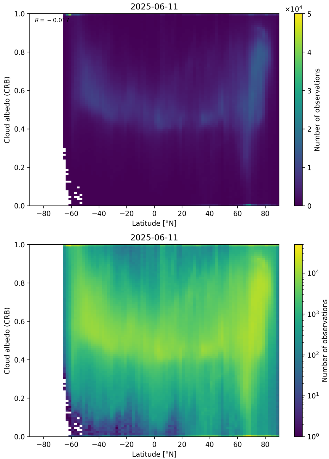
Figure 91: Scatter density plot of “Latitude” against “Cloud albedo (CRB)” for 2025-06-11 to 2025-06-12.
