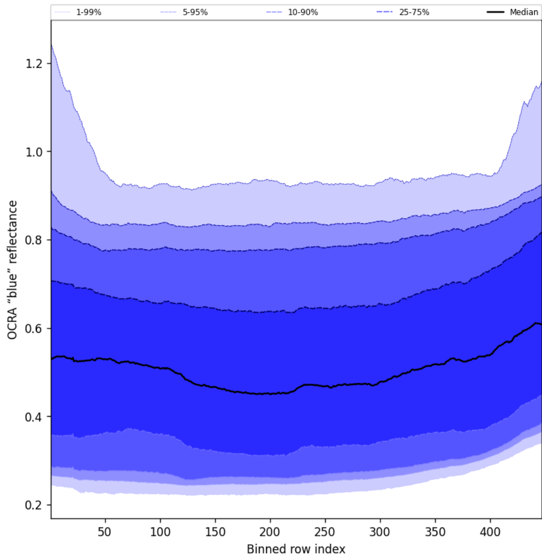
Figure 67: Along track statistics of “OCRA “blue” reflectance” for 2025-06-11 to 2025-06-12
