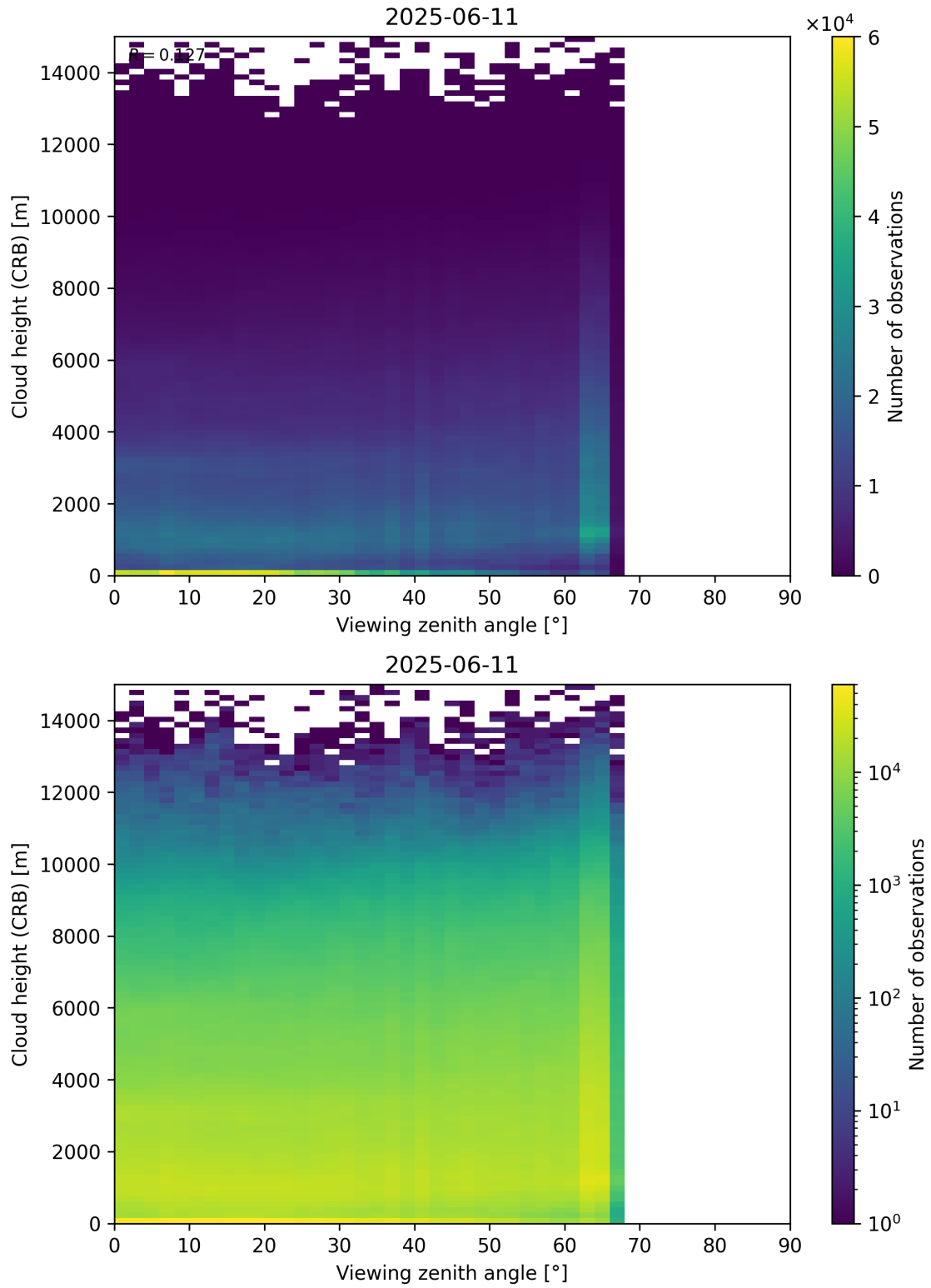
Figure 110: Scatter density plot of “Viewing zenith angle” against “Cloud height (CRB)” for 2025-06-11 to 2025-06-12.
