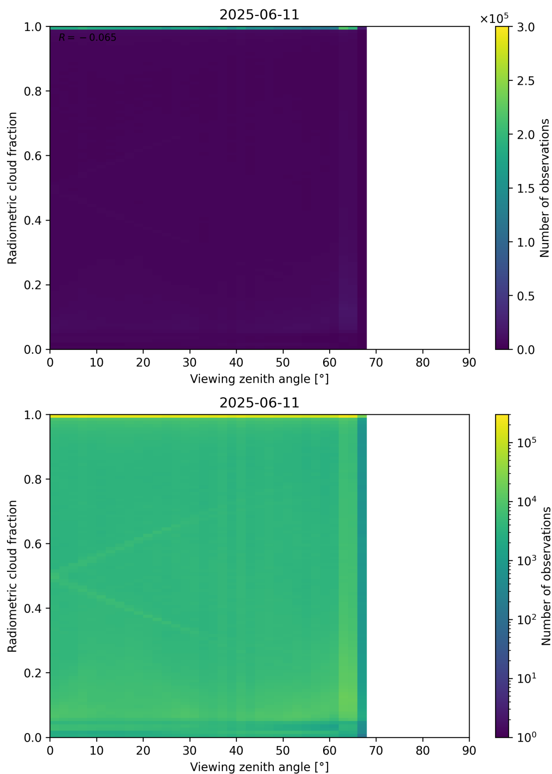
Figure 107: Scatter density plot of “Viewing zenith angle” against “Radiometric cloud fraction” for 2025-06-11 to 2025-06-12.
