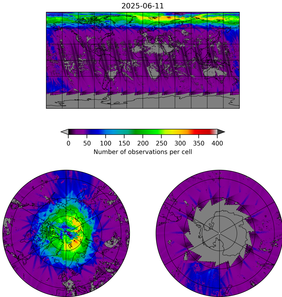
Figure 21: Map of the number of observations for 2025-06-11 to 2025-06-12
