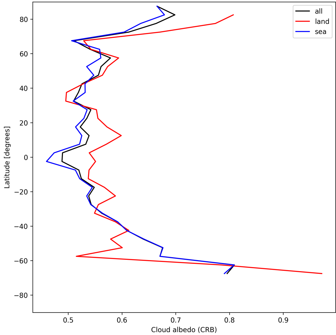
Figure 28: Zonal average of “Cloud albedo (CRB)” for 2025-06-11 to 2025-06-12.
