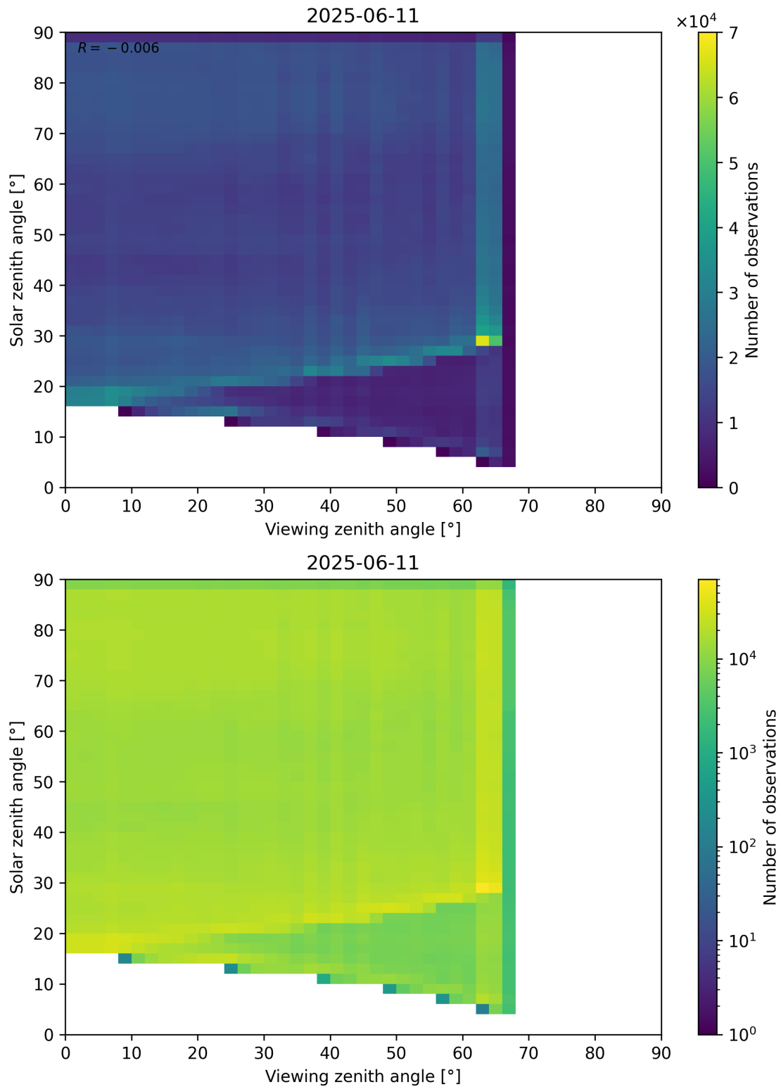
Figure 114: Scatter density plot of “Viewing zenith angle” against “Solar zenith angle” for 2025-06-11 to 2025-06-12.
