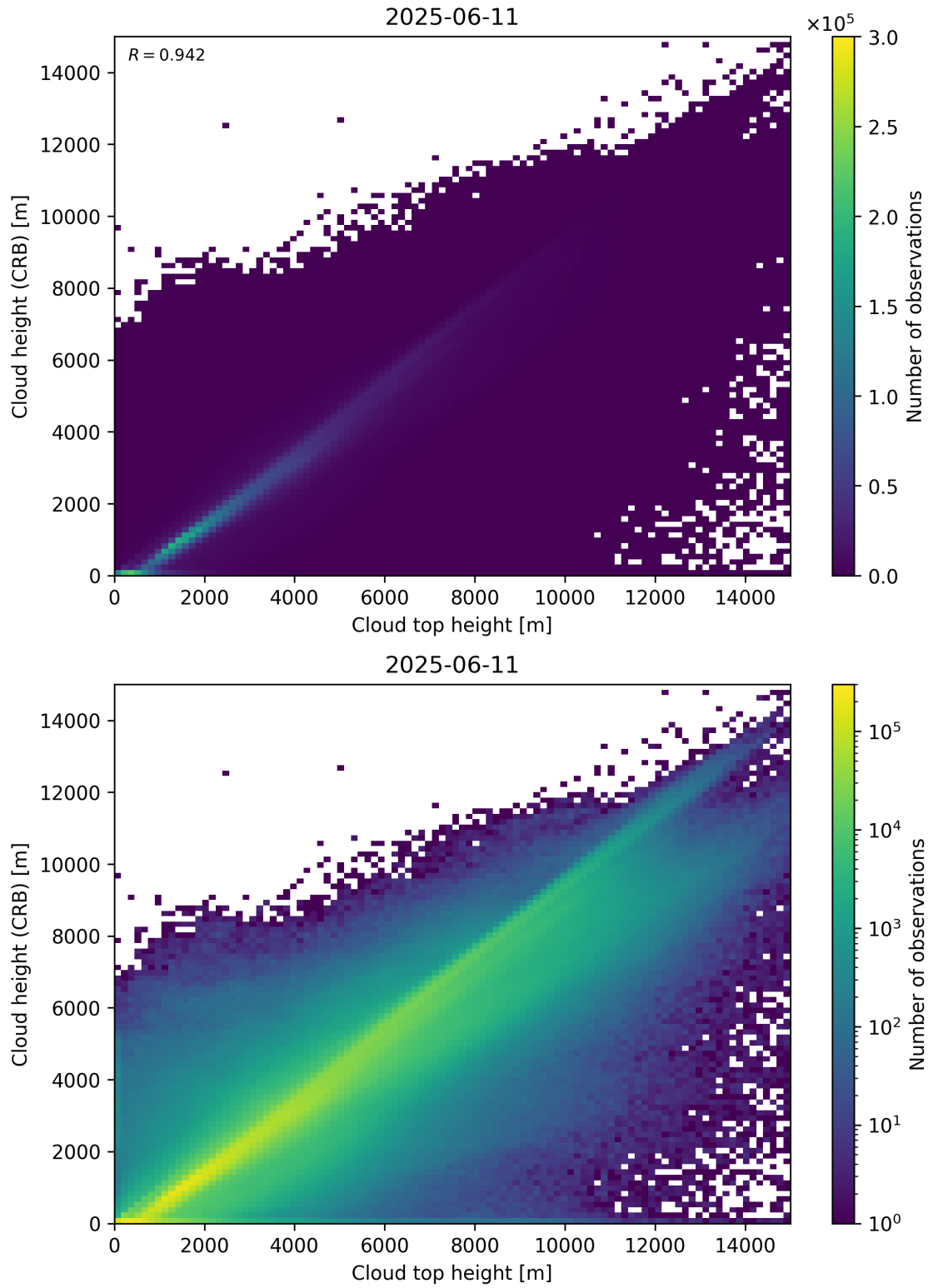
Figure 89: Scatter density plot of “Cloud top height” against “Cloud height (CRB)” for 2025-06-11 to 2025-06-12.
