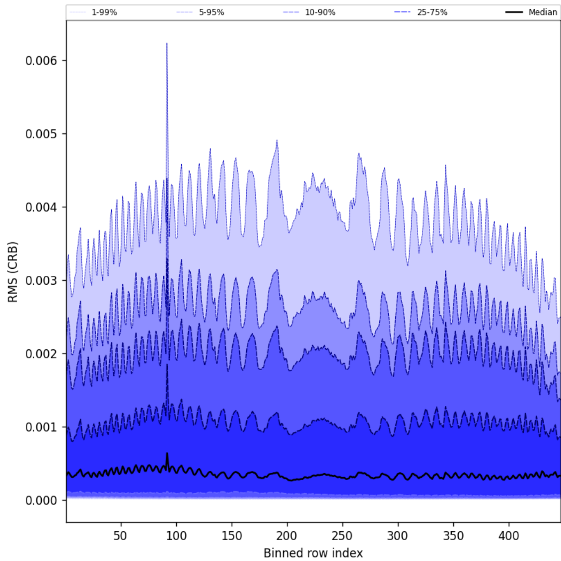
Figure 64: Along track statistics of “RMS (CRB)” for 2025-06-11 to 2025-06-12
