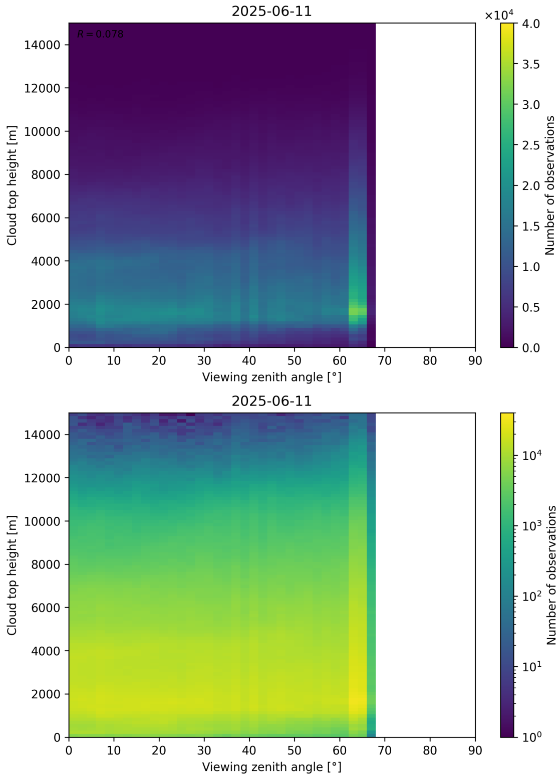
Figure 112: Scatter density plot of “Viewing zenith angle” against “Cloud top height” for 2025-06-11 to 2025-06-12.
