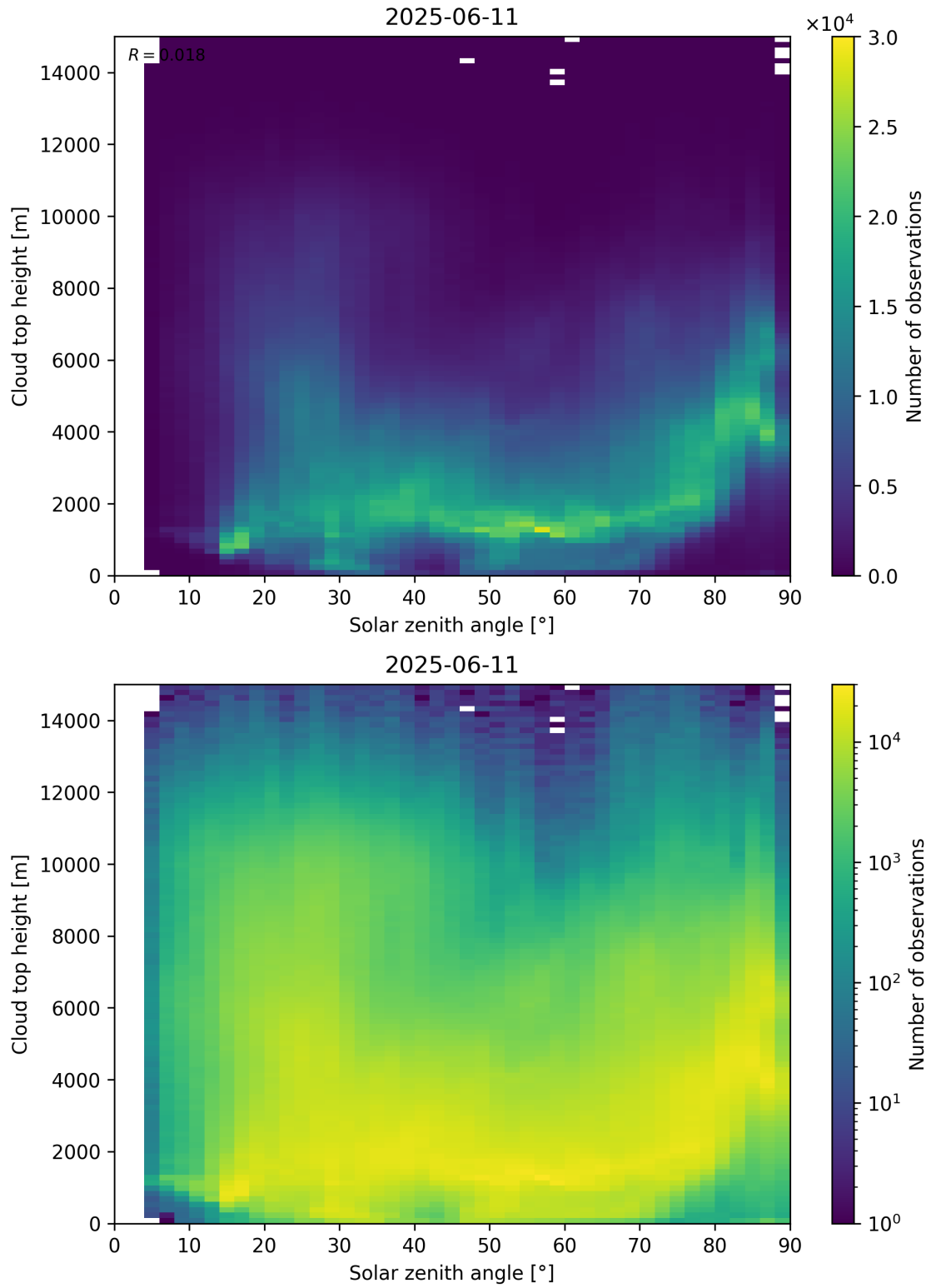
Figure 104: Scatter density plot of “Solar zenith angle” against “Cloud top height” for 2025-06-11 to 2025-06-12.
