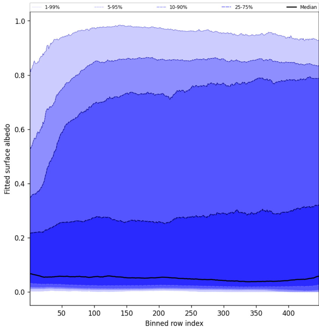
Figure 61: Along track statistics of “Fitted surface albedo” for 2025-06-11 to 2025-06-12
