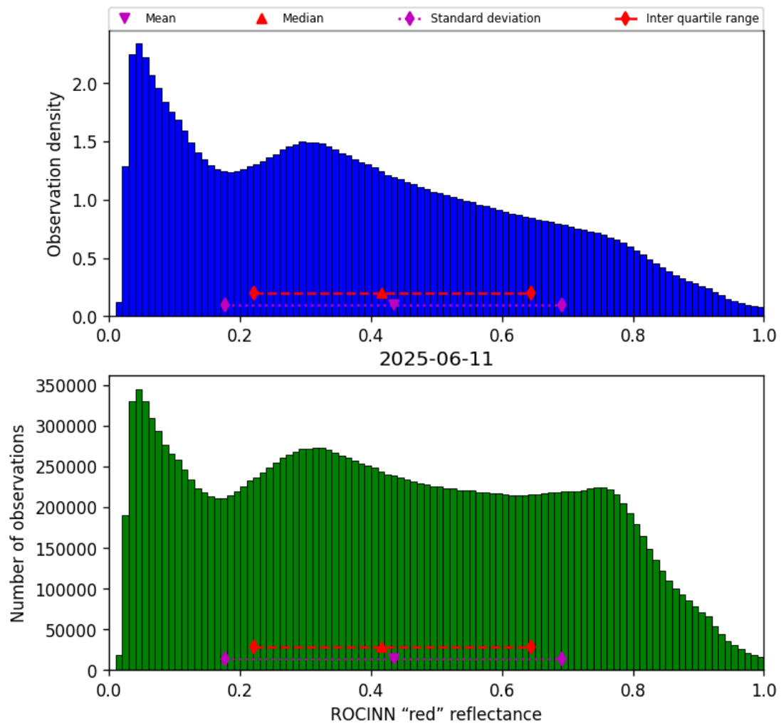
Figure 53: Histogram of “ROCINN “red” reflectance” for 2025-06-11 to 2025-06-12
