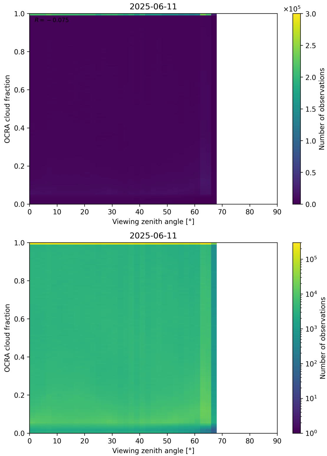
Figure 108: Scatter density plot of “Viewing zenith angle” against “OCRA cloud fraction” for 2025-06-11 to 2025-06-12.
