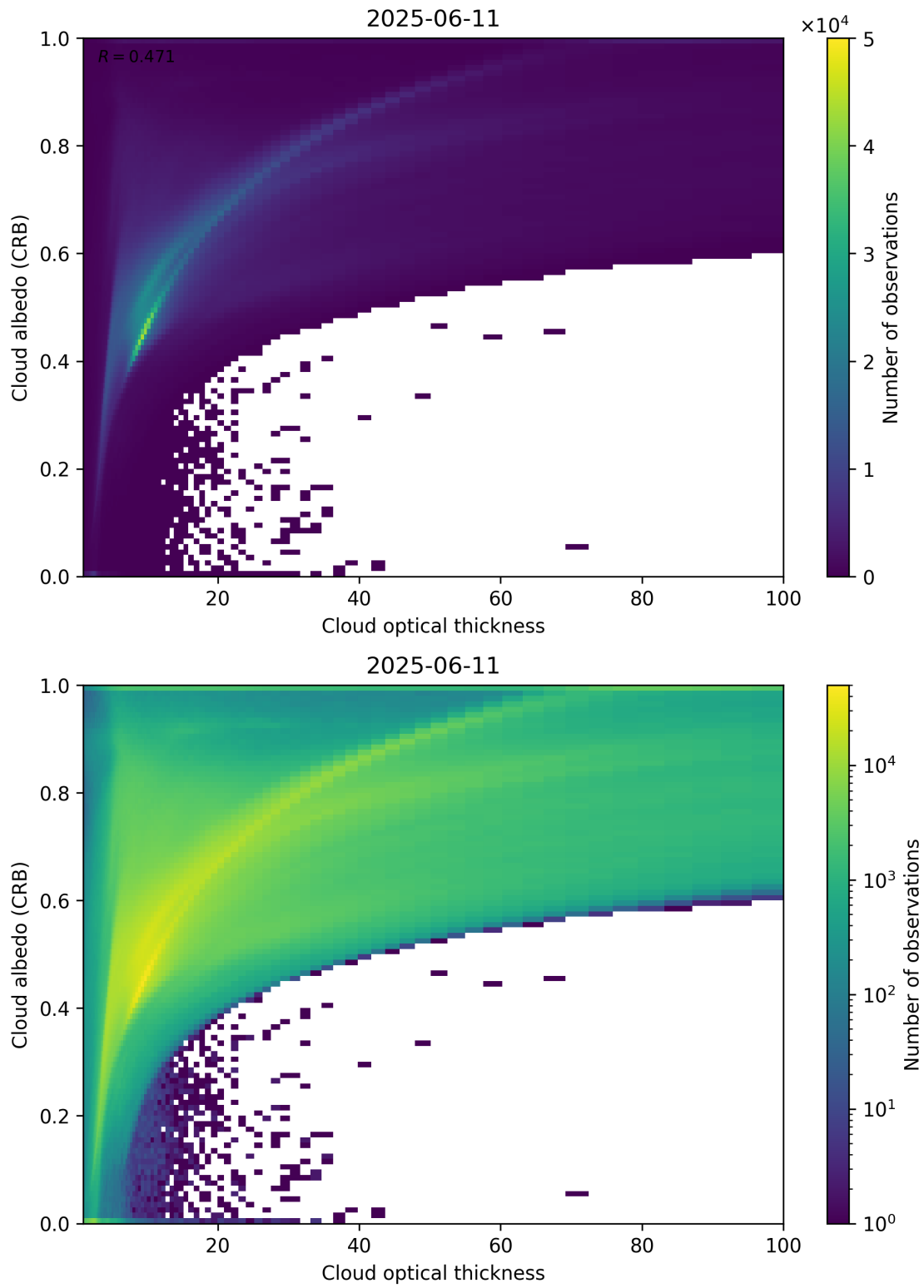
Figure 82: Scatter density plot of “Cloud optical thickness” against “Cloud albedo (CRB)” for 2025-06-11 to 2025-06-12.
