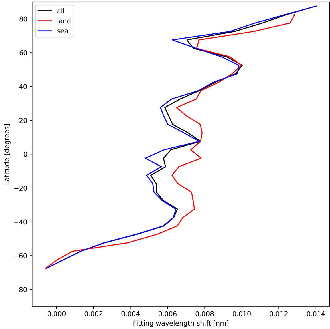
Figure 33: Zonal average of “Fitting wavelength shift” for 2025-06-11 to 2025-06-12.
