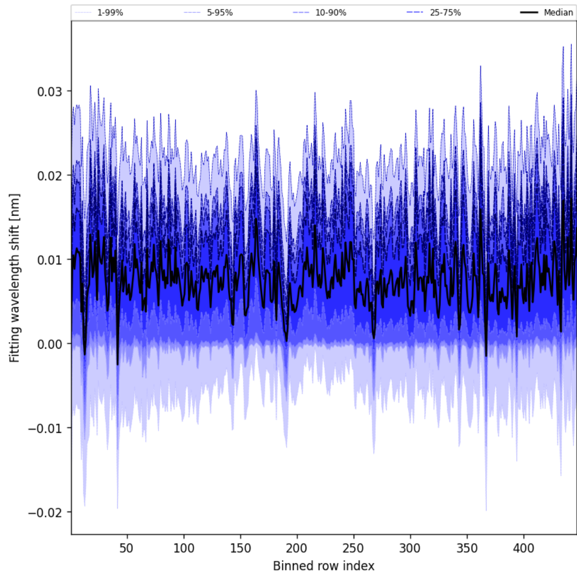
Figure 65: Along track statistics of “Fitting wavelength shift” for 2025-06-11 to 2025-06-12
