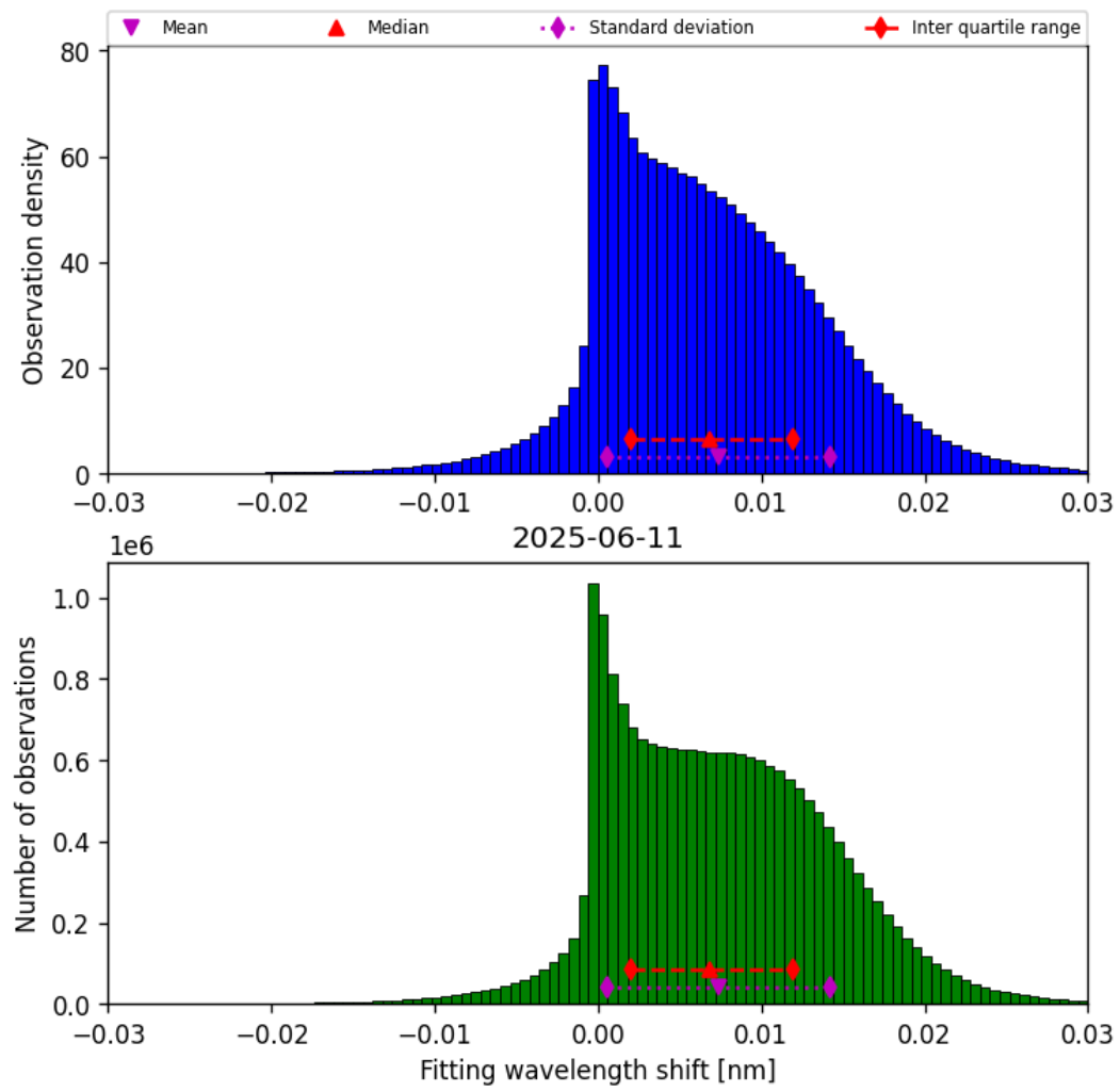
Figure 49: Histogram of “Fitting wavelength shift” for 2025-06-11 to 2025-06-12
