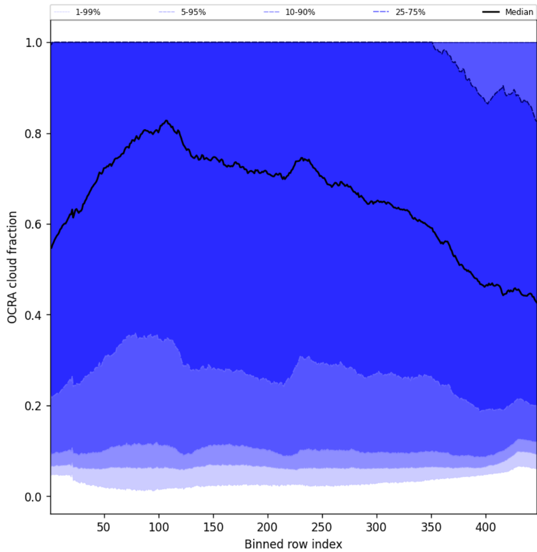
Figure 66: Along track statistics of “OCRA cloud fraction” for 2025-06-11 to 2025-06-12
