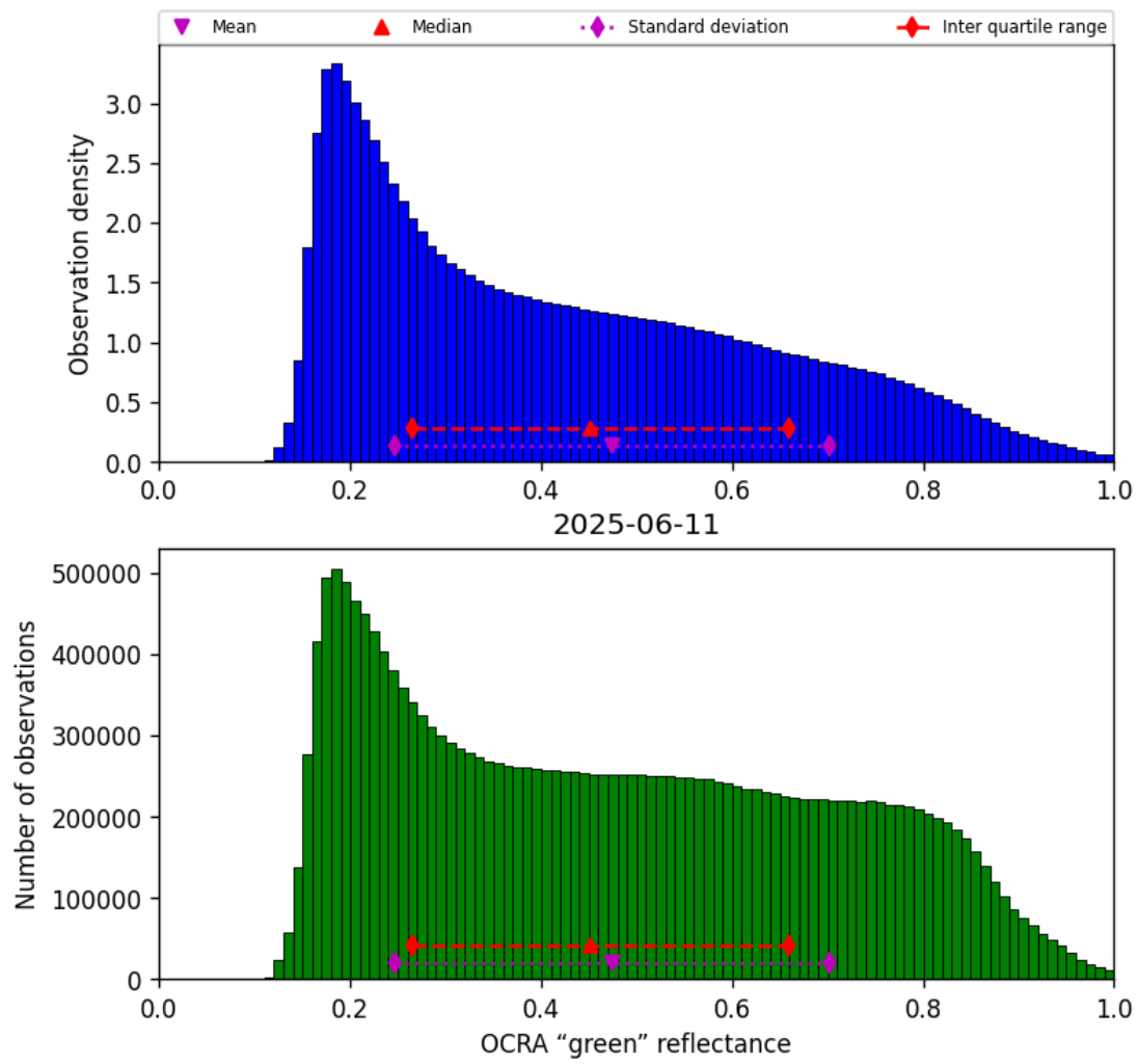
Figure 52: Histogram of “OCRA “green” reflectance” for 2025-06-11 to 2025-06-12
