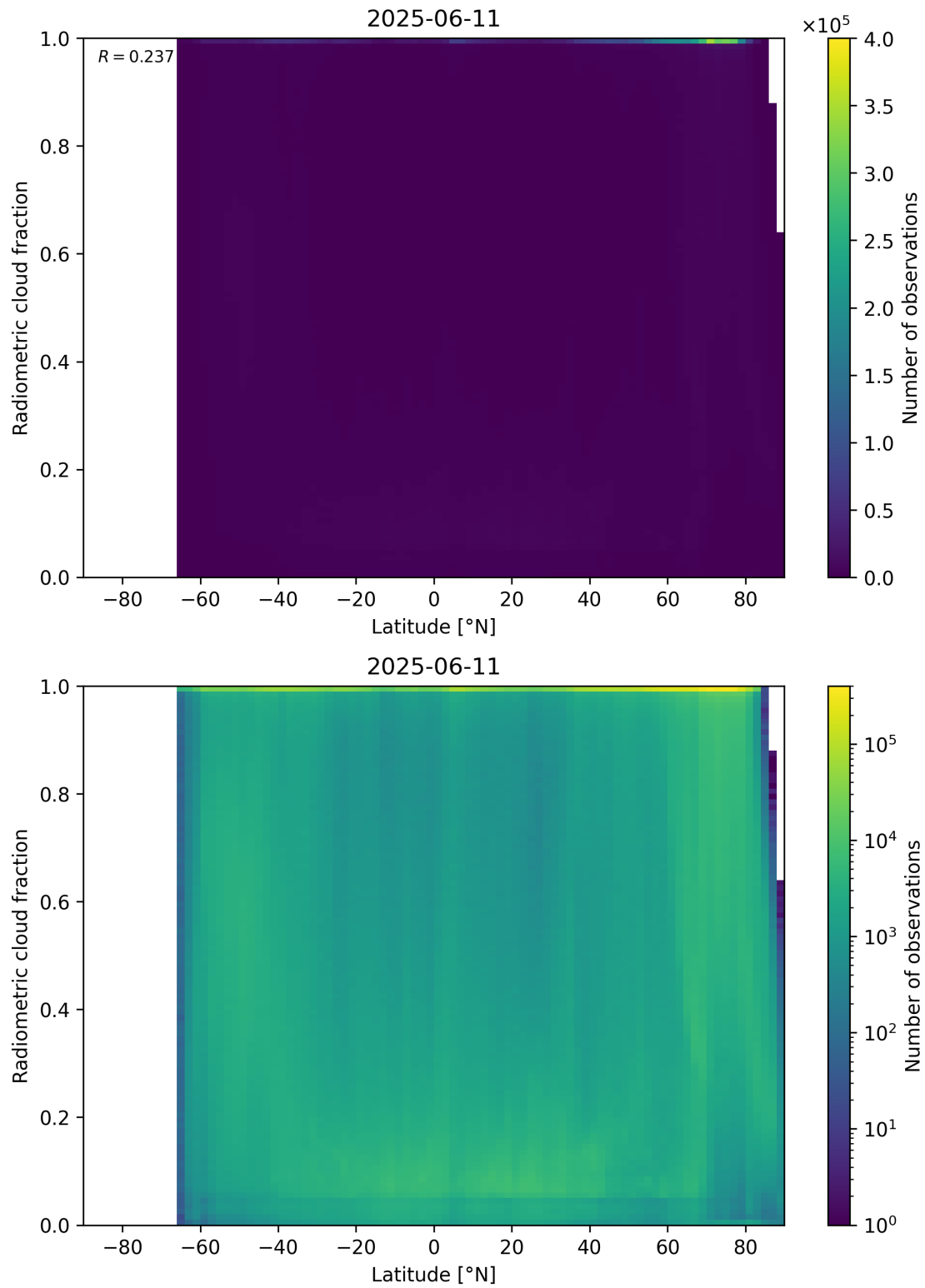
Figure 92: Scatter density plot of “Latitude” against “Radiometric cloud fraction” for 2025-06-11 to 2025-06-12.
