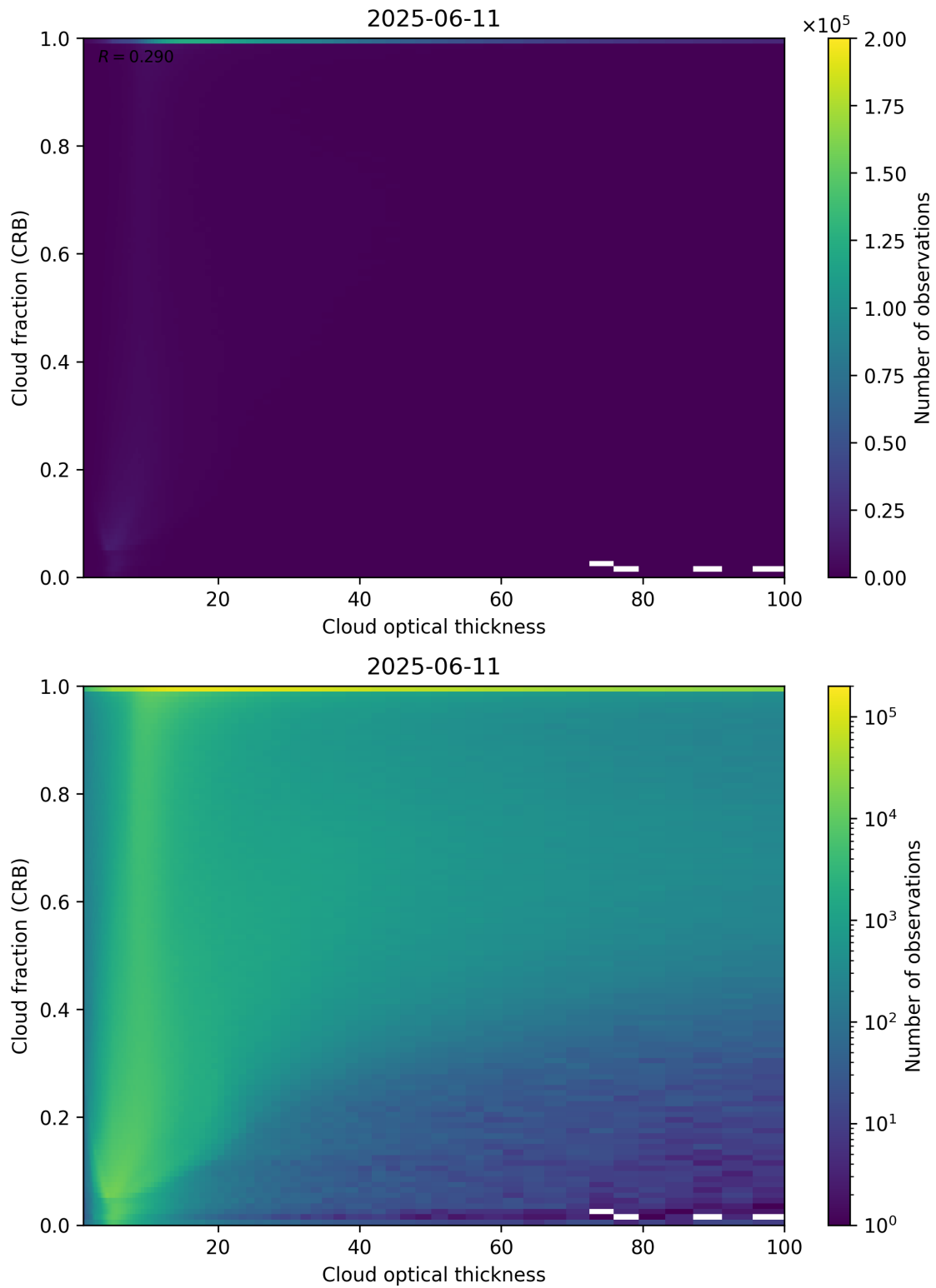
Figure 84: Scatter density plot of “Cloud optical thickness” against “Cloud fraction (CRB)” for 2025-06-11 to 2025-06-12.
