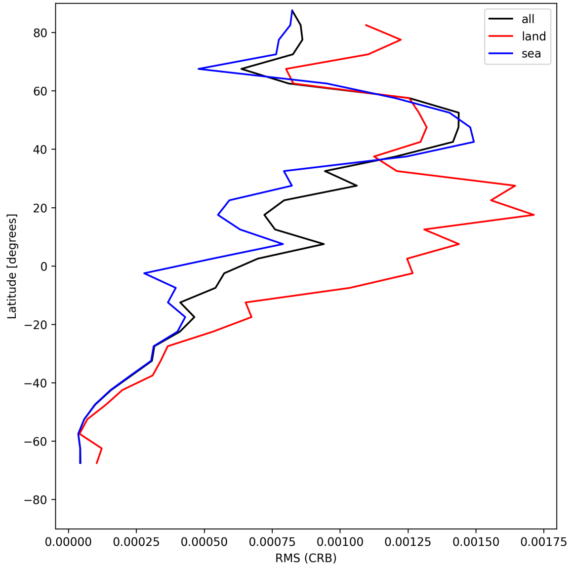
Figure 32: Zonal average of “RMS (CRB)” for 2025-06-11 to 2025-06-12.
