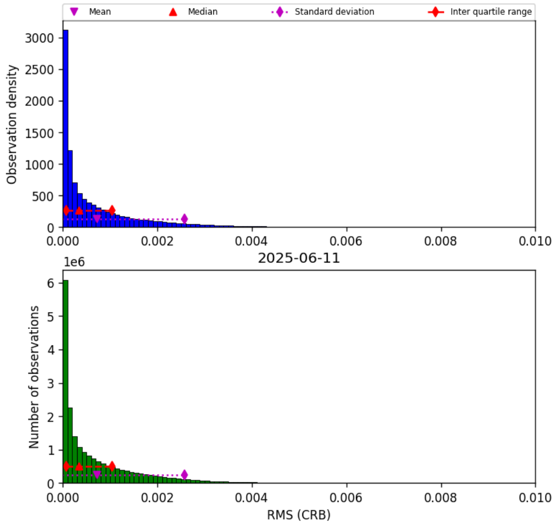
Figure 48: Histogram of “RMS (CRB)” for 2025-06-11 to 2025-06-12
