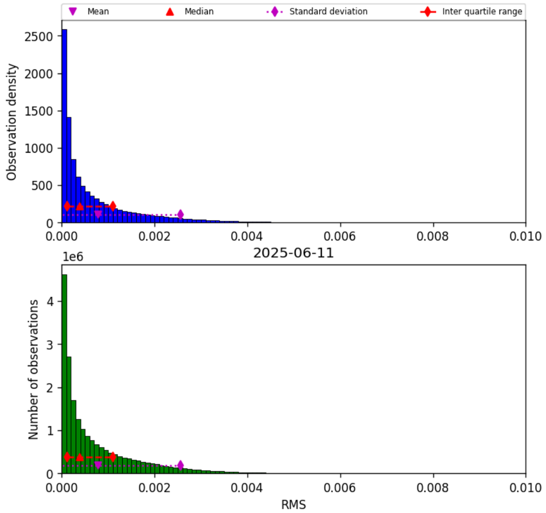
Figure 47: Histogram of “RMS” for 2025-06-11 to 2025-06-12
