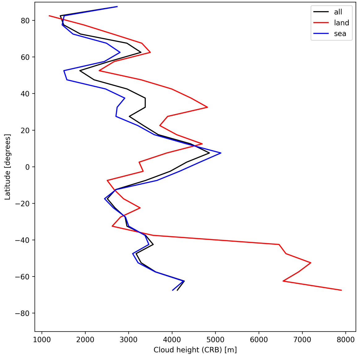
Figure 27: Zonal average of “Cloud height (CRB)” for 2025-06-11 to 2025-06-12.
