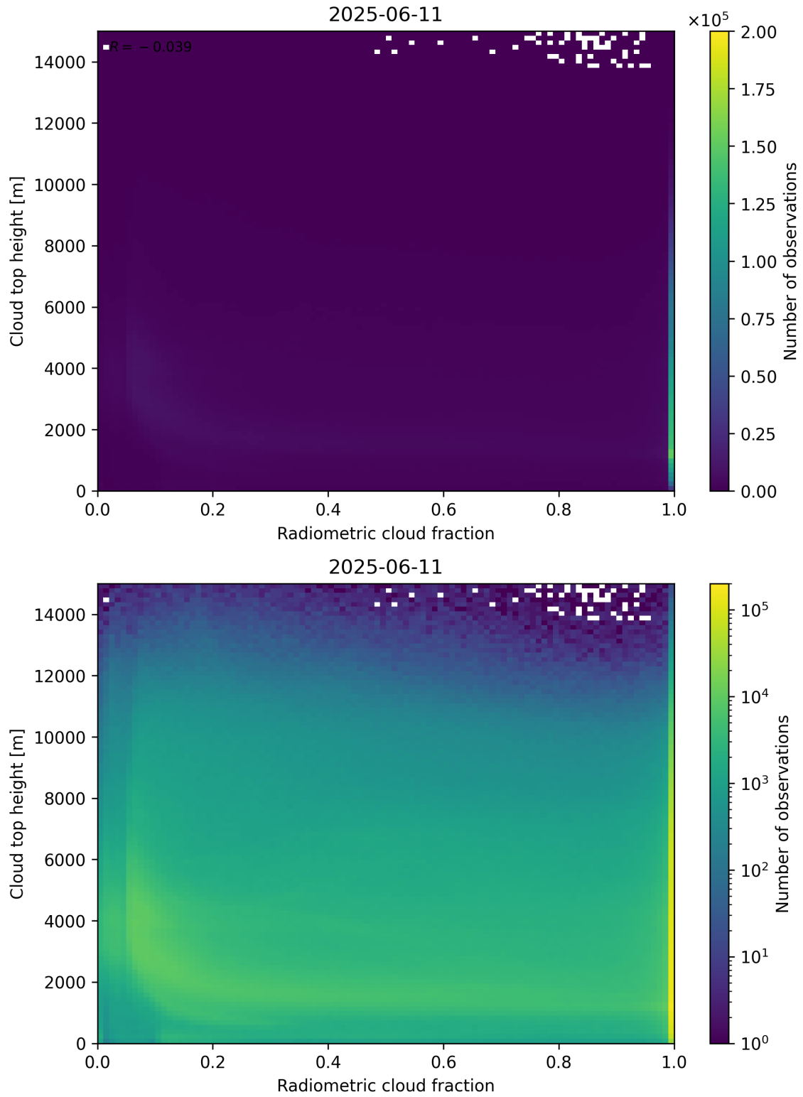
Figure 76: Scatter density plot of “Radiometric cloud fraction” against “Cloud top height” for 2025-06-11 to 2025-06-12.
