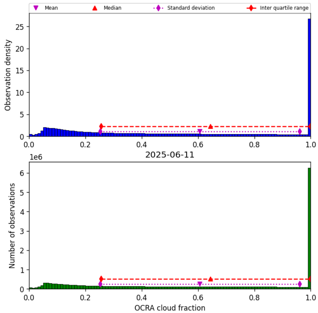
Figure 50: Histogram of “OCRA cloud fraction” for 2025-06-11 to 2025-06-12
