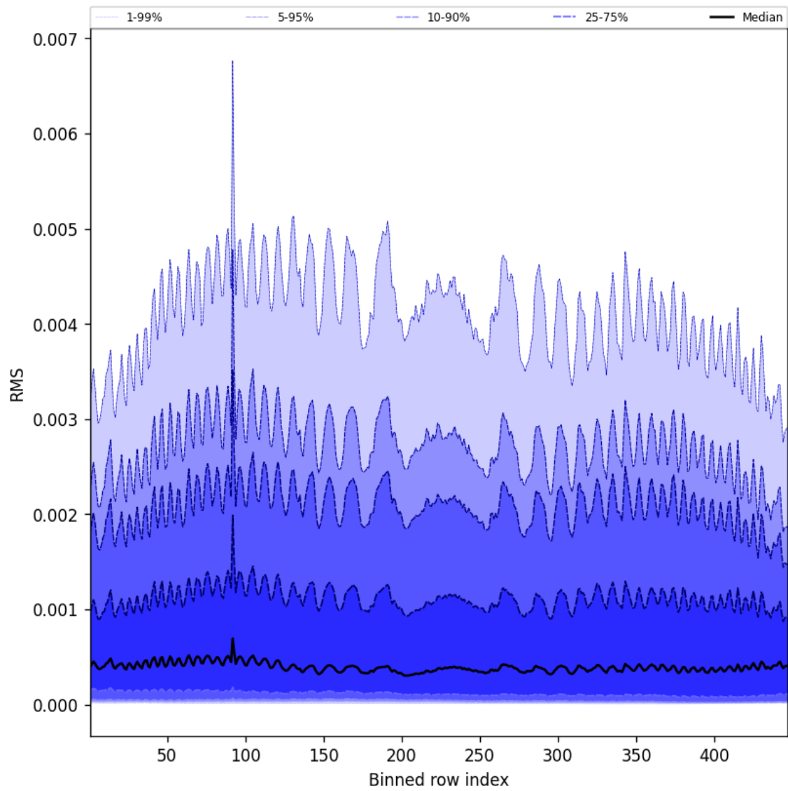
Figure 63: Along track statistics of “RMS” for 2025-06-11 to 2025-06-12
