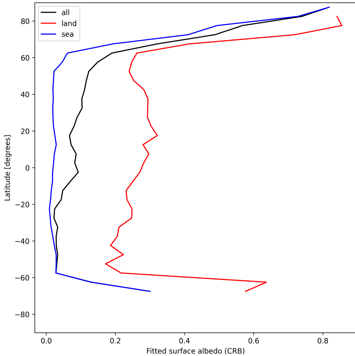
Figure 30: Zonal average of “Fitted surface albedo (CRB)” for 2025-06-11 to 2025-06-12.
