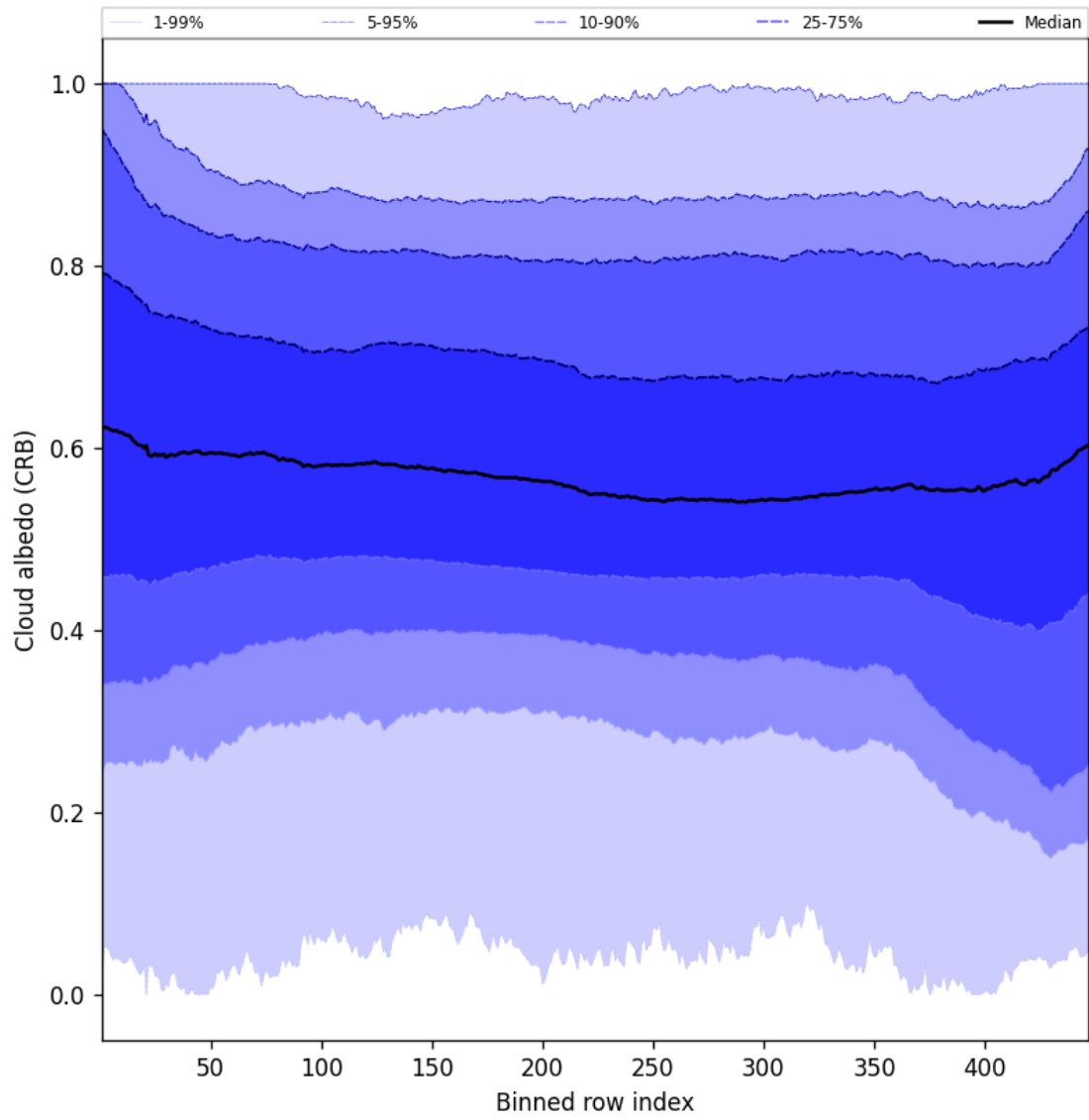
Figure 60: Along track statistics of “Cloud albedo (CRB)” for 2025-06-11 to 2025-06-12
