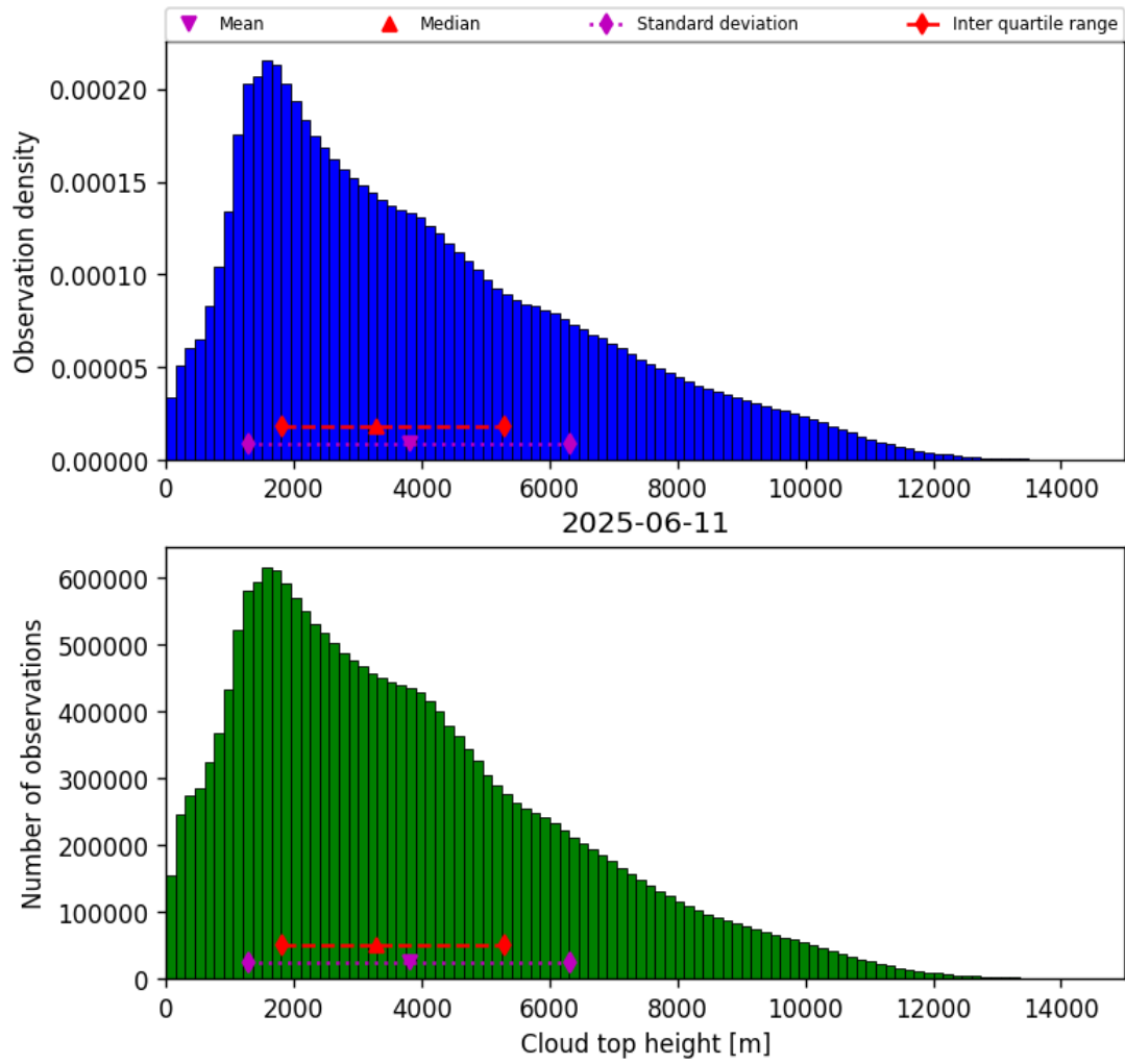
Figure 40: Histogram of “Cloud top height” for 2025-06-11 to 2025-06-12
