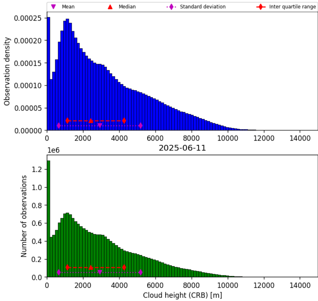
Figure 43: Histogram of “Cloud height (CRB)” for 2025-06-11 to 2025-06-12
