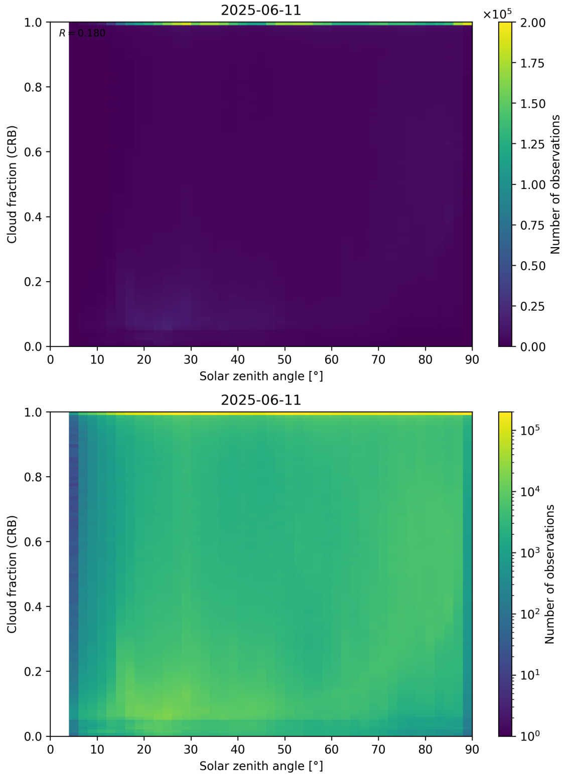
Figure 101: Scatter density plot of “Solar zenith angle” against “Cloud fraction (CRB)” for 2025-06-11 to 2025-06-12.
