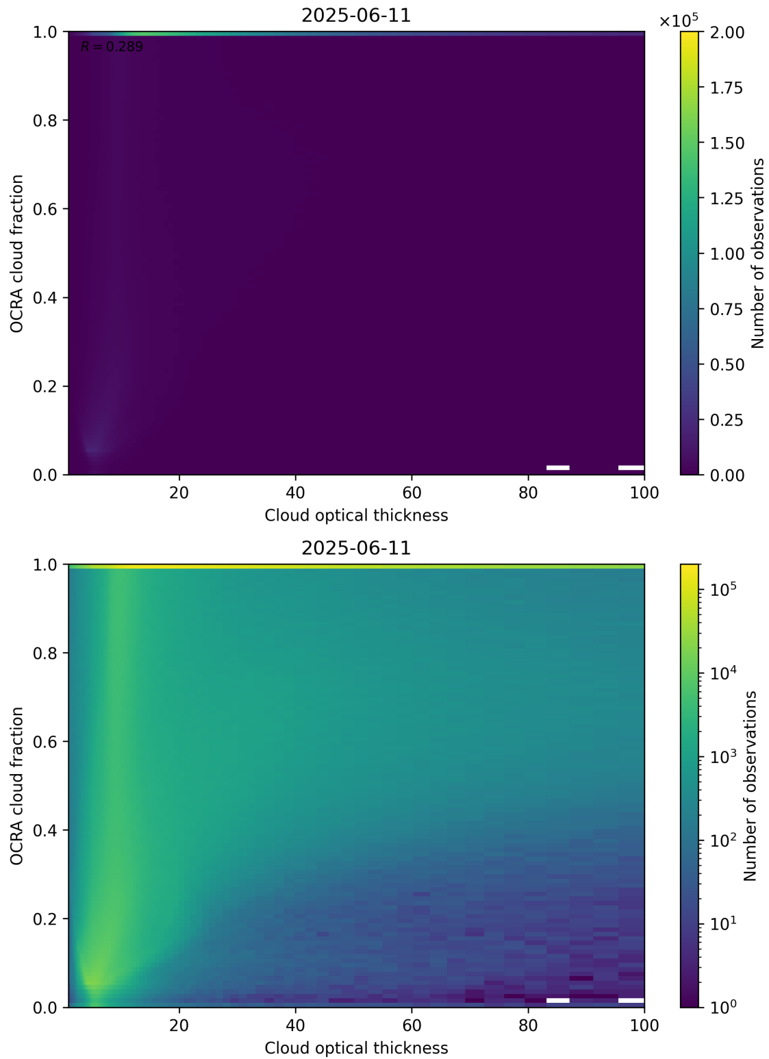
Figure 83: Scatter density plot of “Cloud optical thickness” against “OCRA cloud fraction” for 2025-06-11 to 2025-06-12.
