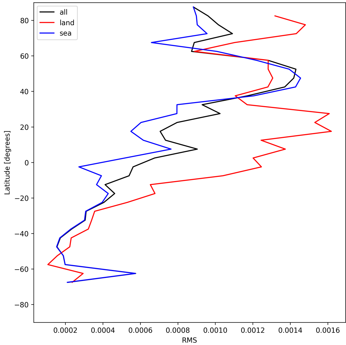
Figure 31: Zonal average of “RMS” for 2025-06-11 to 2025-06-12.
