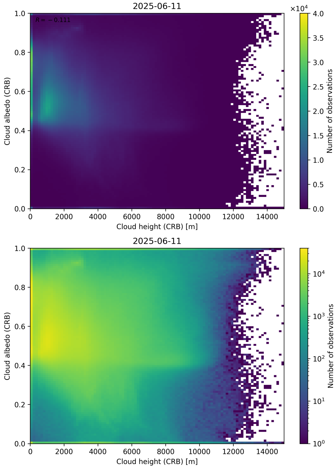
Figure 80: Scatter density plot of “Cloud height (CRB)” against “Cloud albedo (CRB)” for 2025-06-11 to 2025-06-12.
