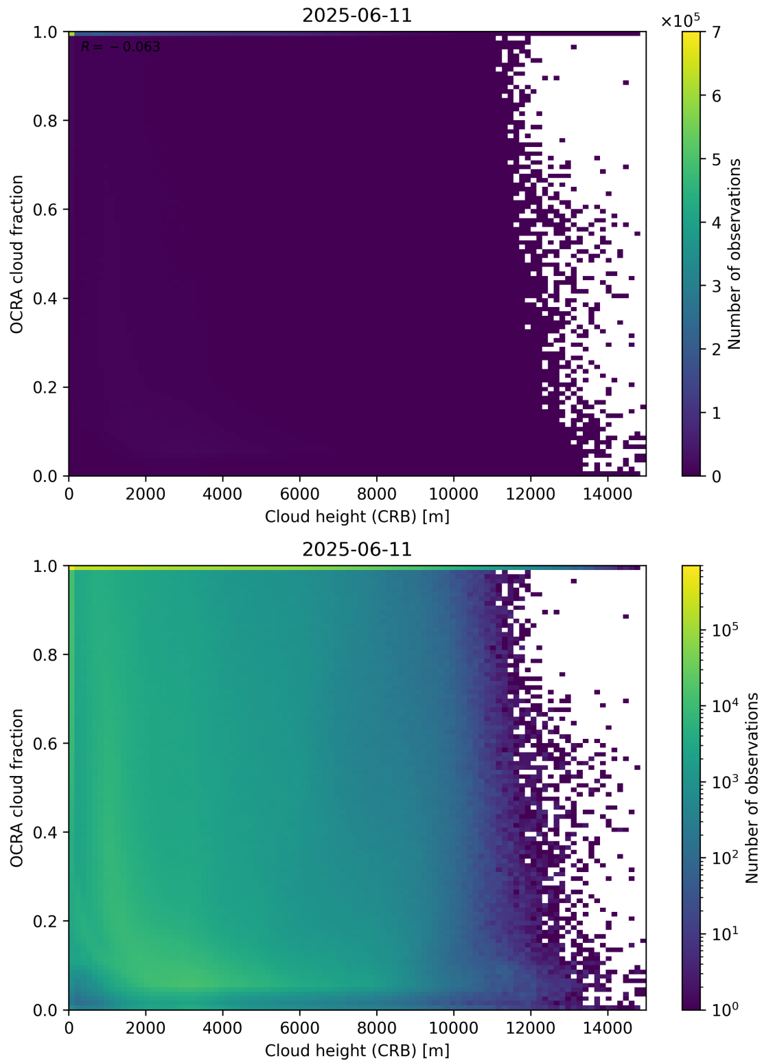
Figure 81: Scatter density plot of “Cloud height (CRB)” against “OCRA cloud fraction” for 2025-06-11 to 2025-06-12.
