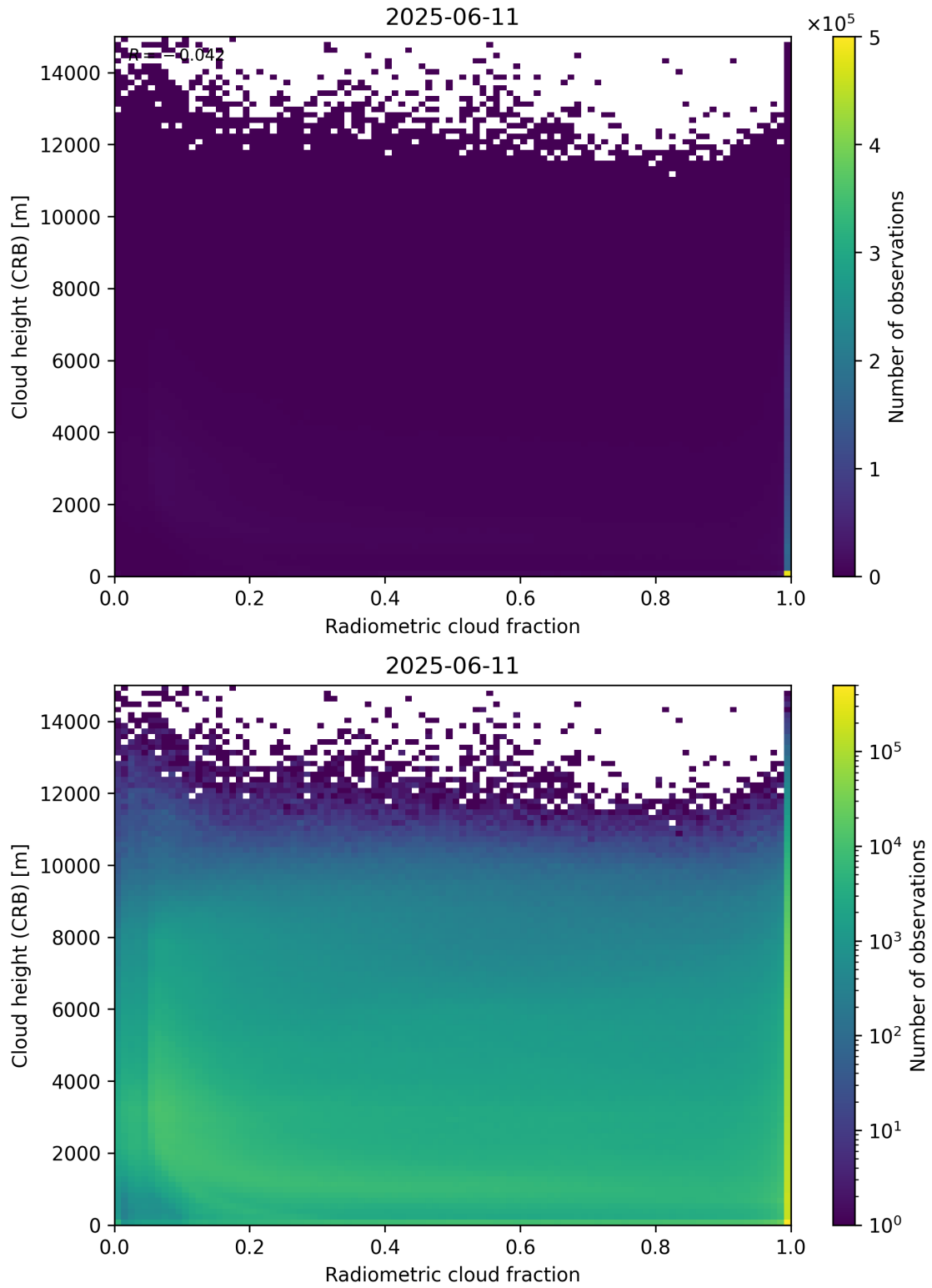
Figure 74: Scatter density plot of “Radiometric cloud fraction” against “Cloud height (CRB)” for 2025-06-11 to 2025-06-12.
