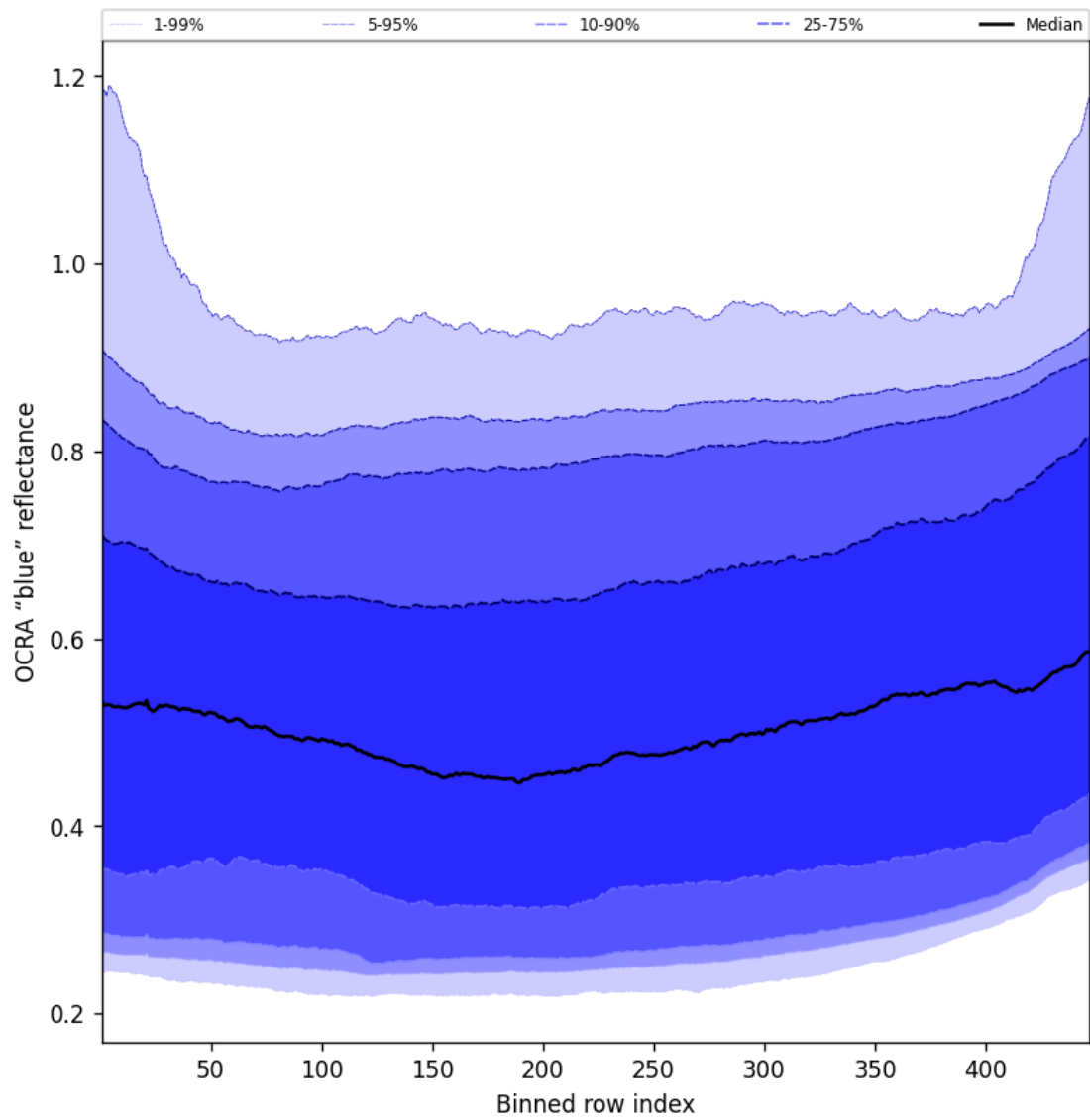
Figure 67: Along track statistics of “OCRA “blue” reflectance” for 2025-06-12 to 2025-06-14
