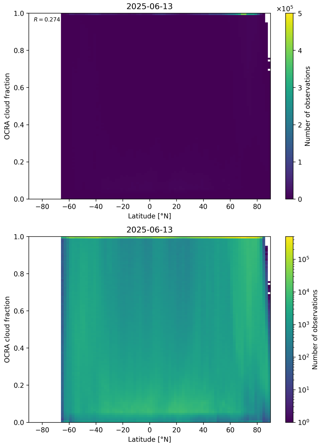
Figure 93: Scatter density plot of “Latitude” against “OCRA cloud fraction” for 2025-06-12 to 2025-06-14.
