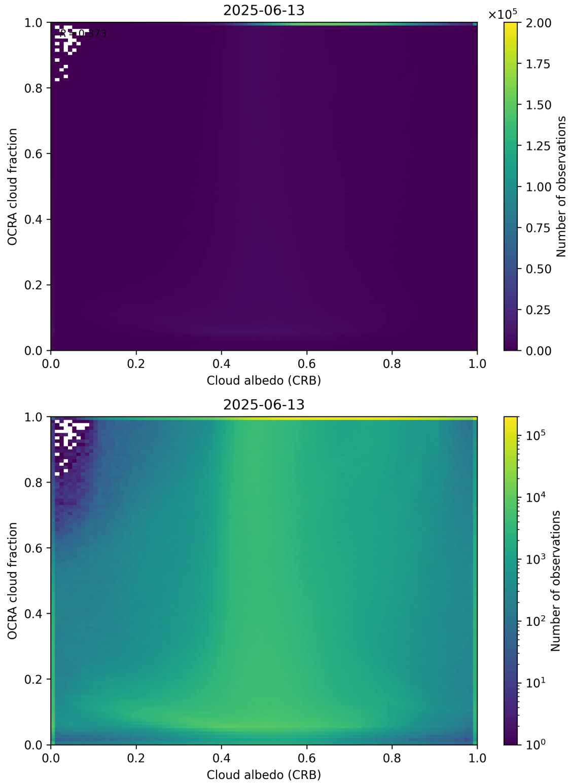
Figure 70: Scatter density plot of “Cloud albedo (CRB)” against “OCRA cloud fraction” for 2025-06-12 to 2025-06-14.
