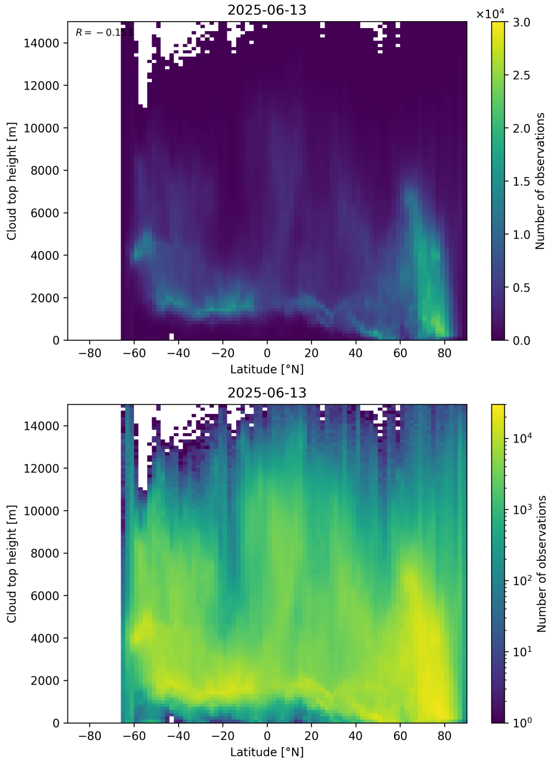
Figure 97: Scatter density plot of “Latitude” against “Cloud top height” for 2025-06-12 to 2025-06-14.
