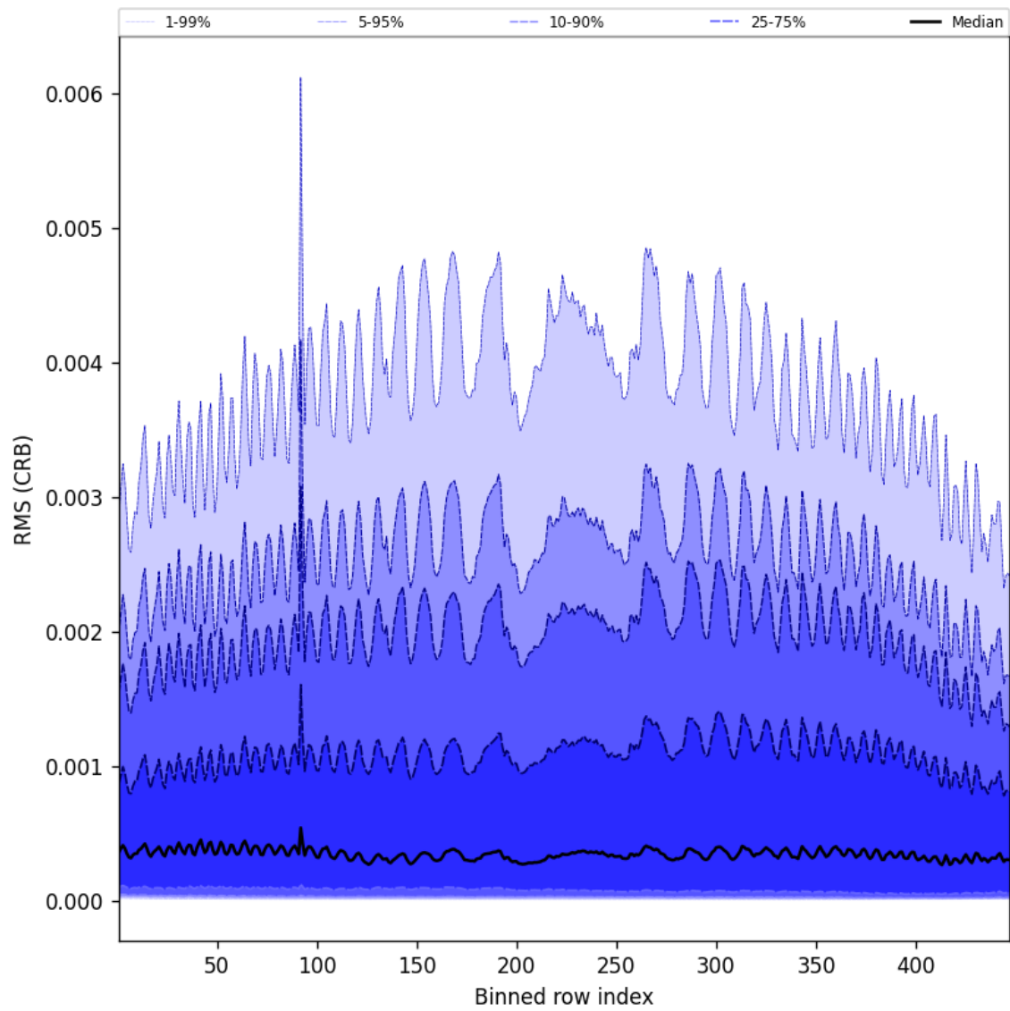
Figure 64: Along track statistics of “RMS (CRB)” for 2025-06-12 to 2025-06-14
