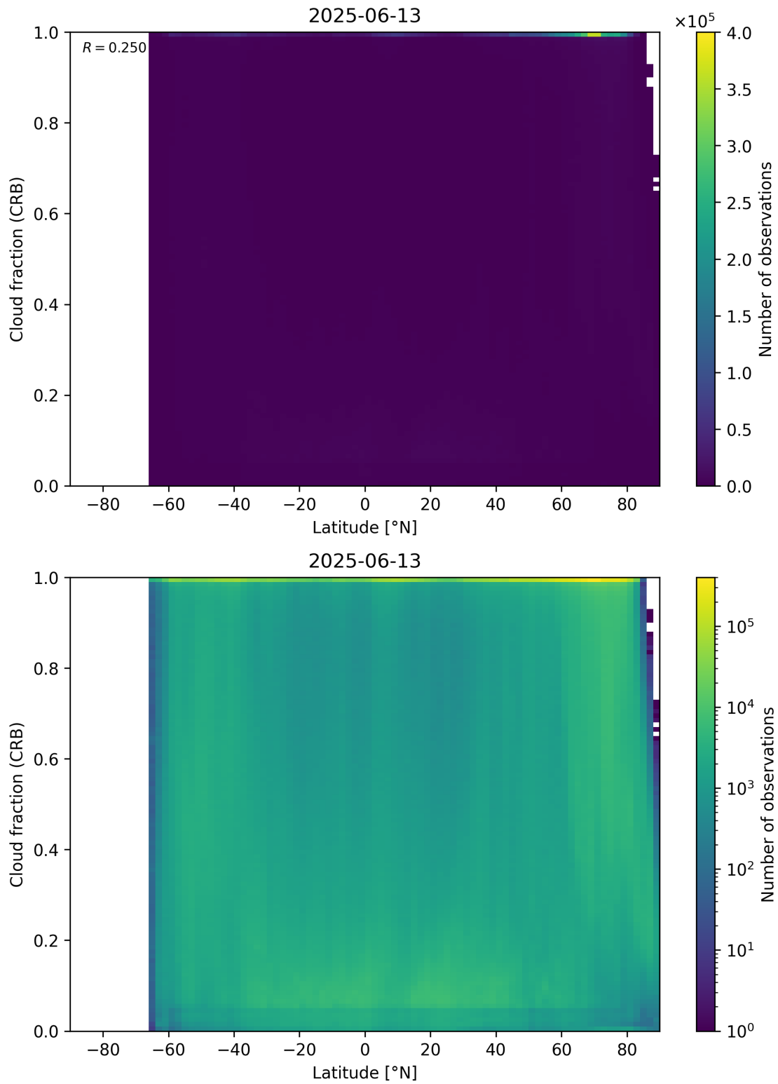
Figure 94: Scatter density plot of “Latitude” against “Cloud fraction (CRB)” for 2025-06-12 to 2025-06-14.
