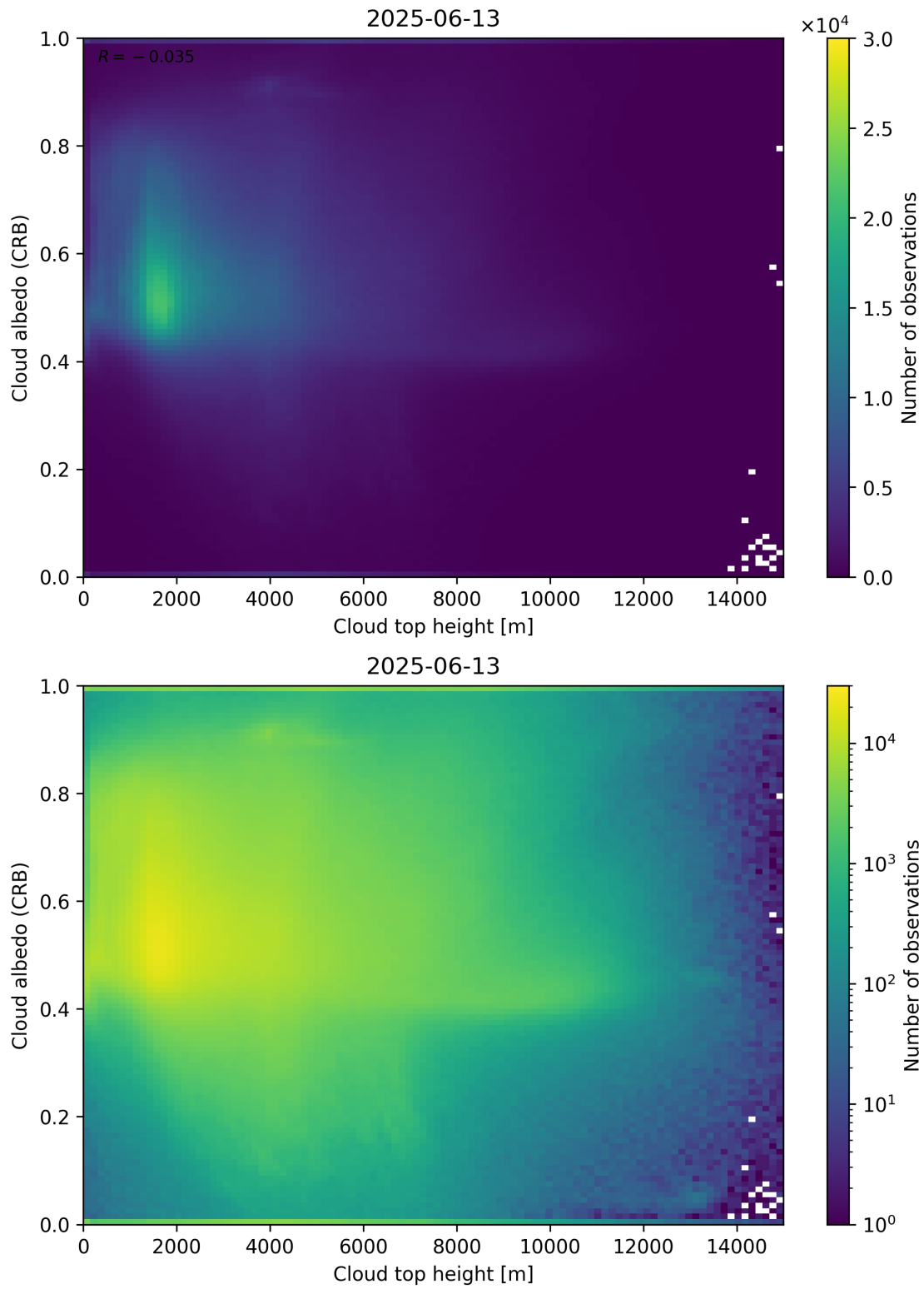
Figure 86: Scatter density plot of “Cloud top height” against “Cloud albedo (CRB)” for 2025-06-12 to 2025-06-14.
