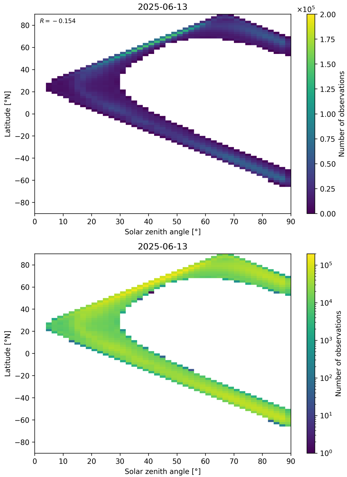
Figure 105: Scatter density plot of “Solar zenith angle” against “Latitude” for 2025-06-12 to 2025-06-14.
