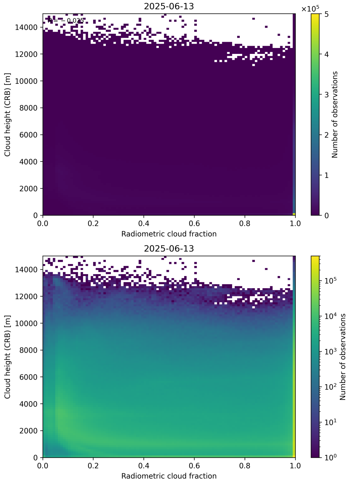
Figure 74: Scatter density plot of “Radiometric cloud fraction” against “Cloud height (CRB)” for 2025-06-12 to 2025-06-14.
