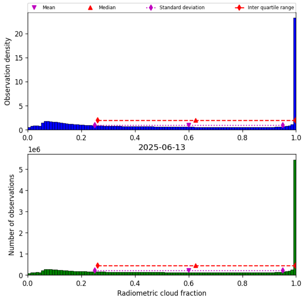
Figure 39: Histogram of “Radiometric cloud fraction” for 2025-06-12 to 2025-06-14
