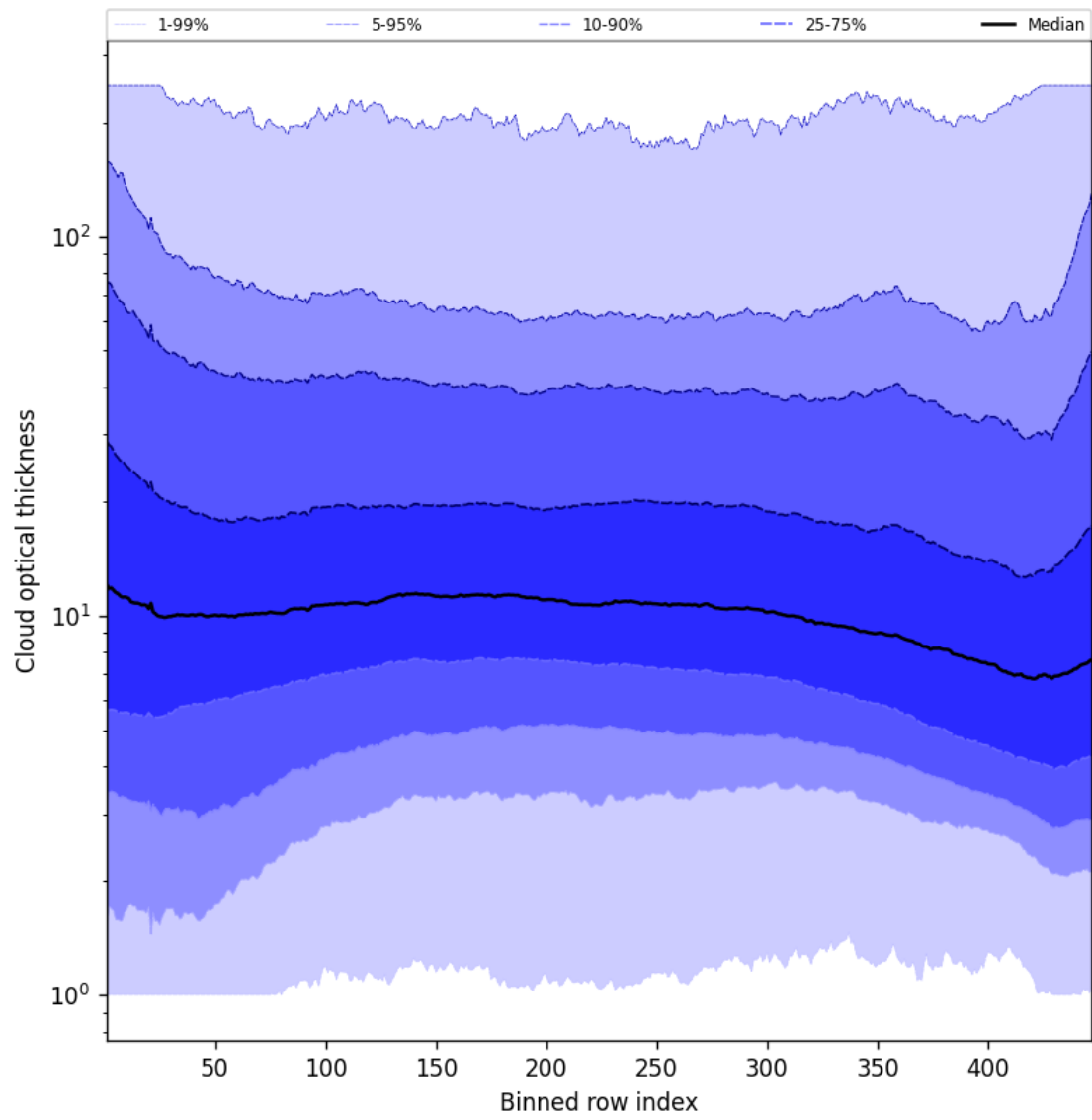
Figure 57: Along track statistics of “Cloud optical thickness” for 2025-06-12 to 2025-06-14
