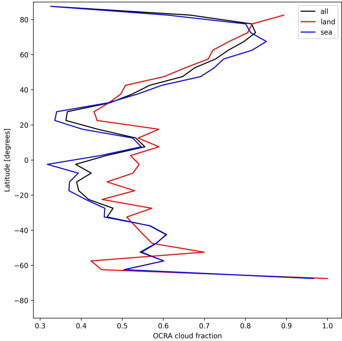
Figure 34: Zonal average of “OCRA cloud fraction” for 2025-06-12 to 2025-06-14.
