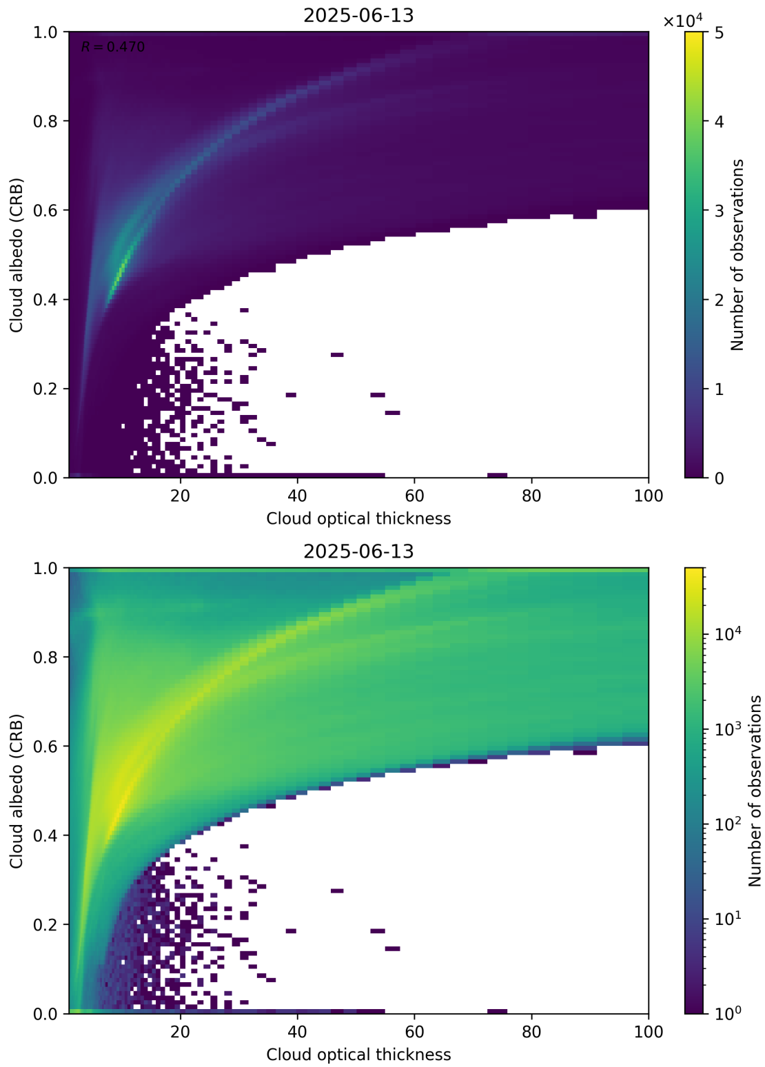
Figure 82: Scatter density plot of “Cloud optical thickness” against “Cloud albedo (CRB)” for 2025-06-12 to 2025-06-14.
