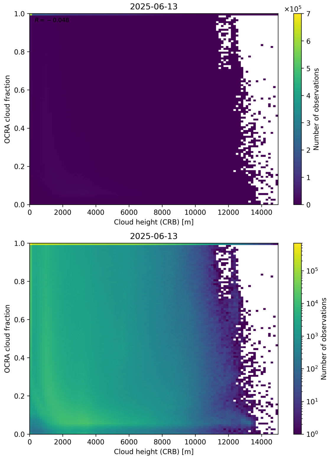
Figure 81: Scatter density plot of “Cloud height (CRB)” against “OCRA cloud fraction” for 2025-06-12 to 2025-06-14.
