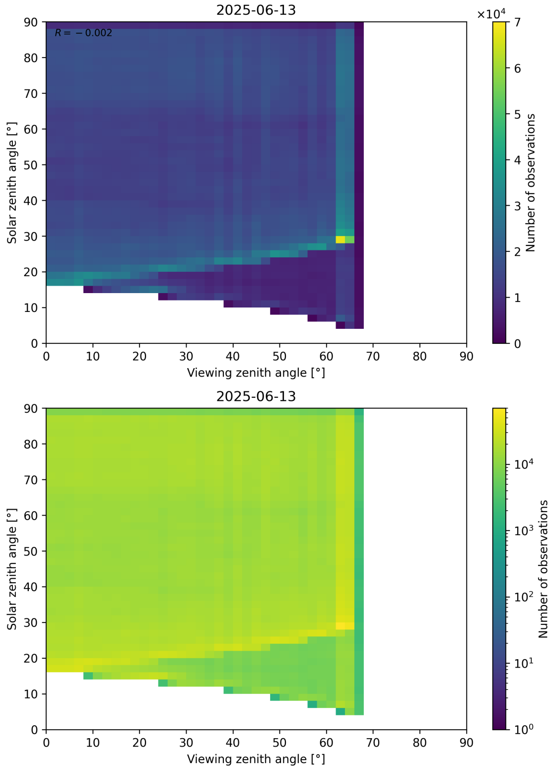
Figure 114: Scatter density plot of “Viewing zenith angle” against “Solar zenith angle” for 2025-06-12 to 2025-06-14.
