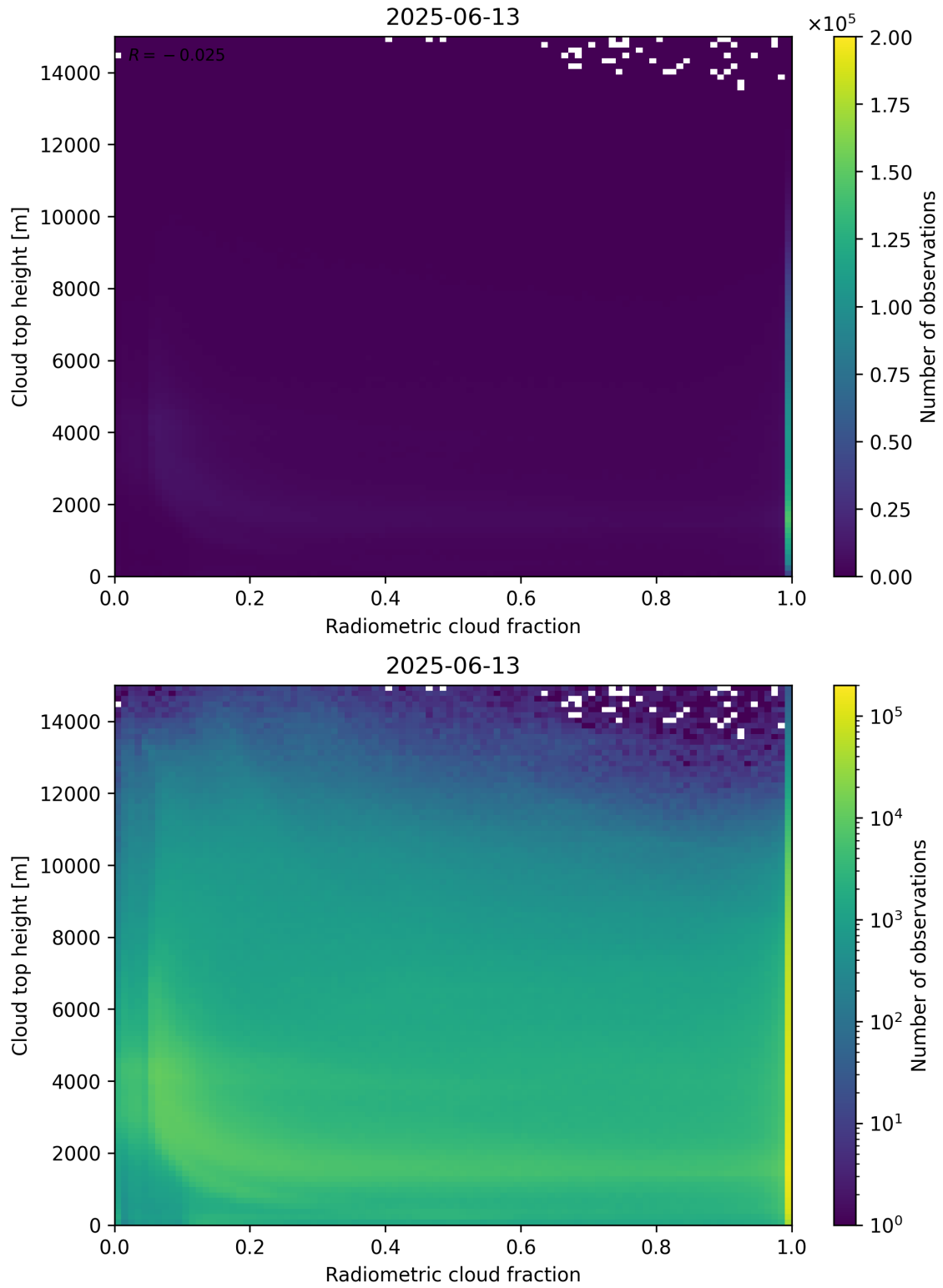
Figure 76: Scatter density plot of “Radiometric cloud fraction” against “Cloud top height” for 2025-06-12 to 2025-06-14.
