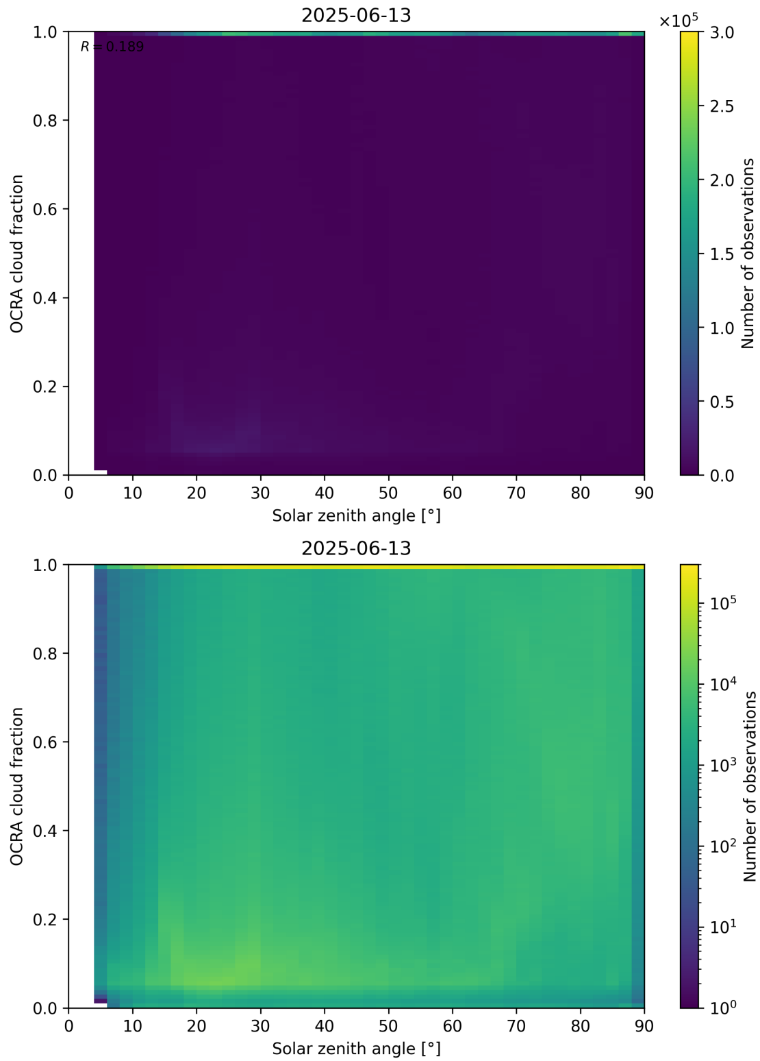
Figure 100: Scatter density plot of “Solar zenith angle” against “OCRA cloud fraction” for 2025-06-12 to 2025-06-14.
