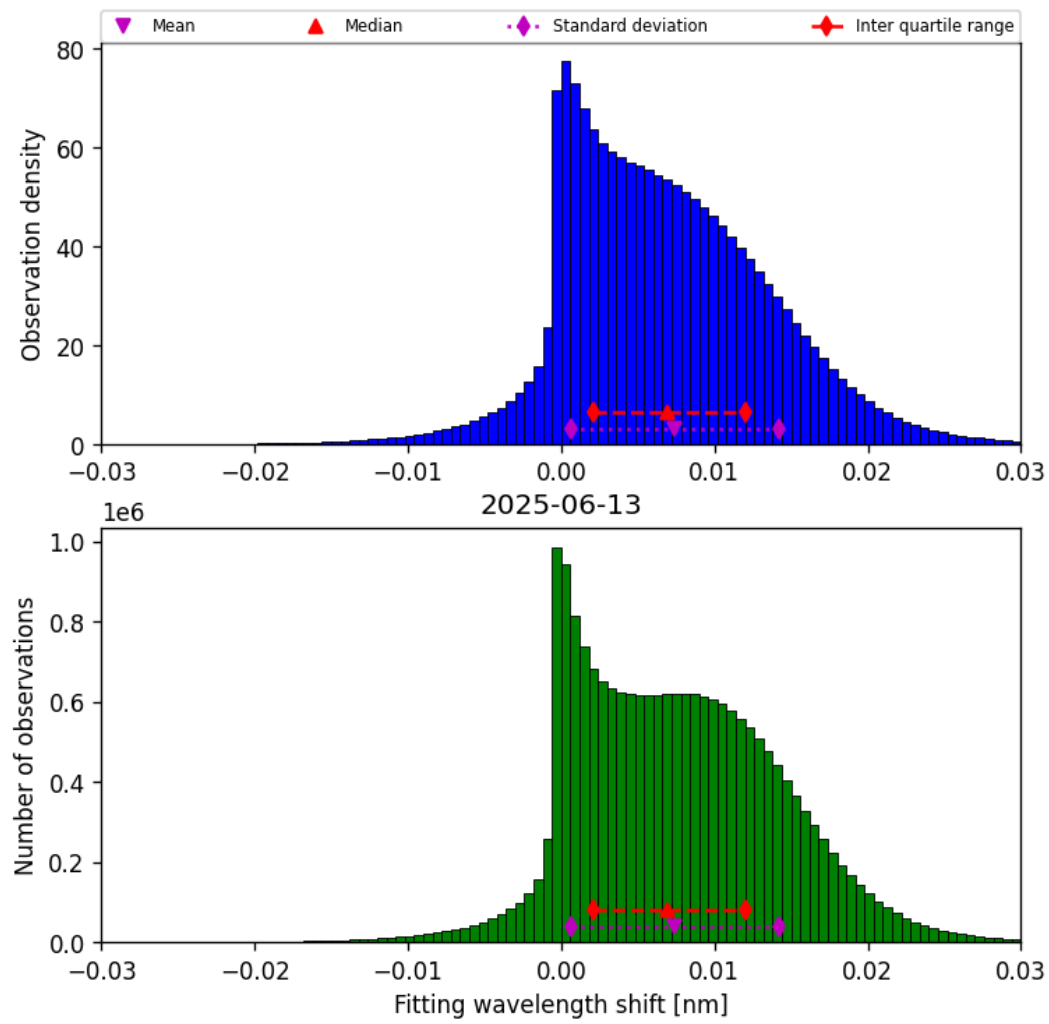
Figure 49: Histogram of “Fitting wavelength shift” for 2025-06-12 to 2025-06-14
