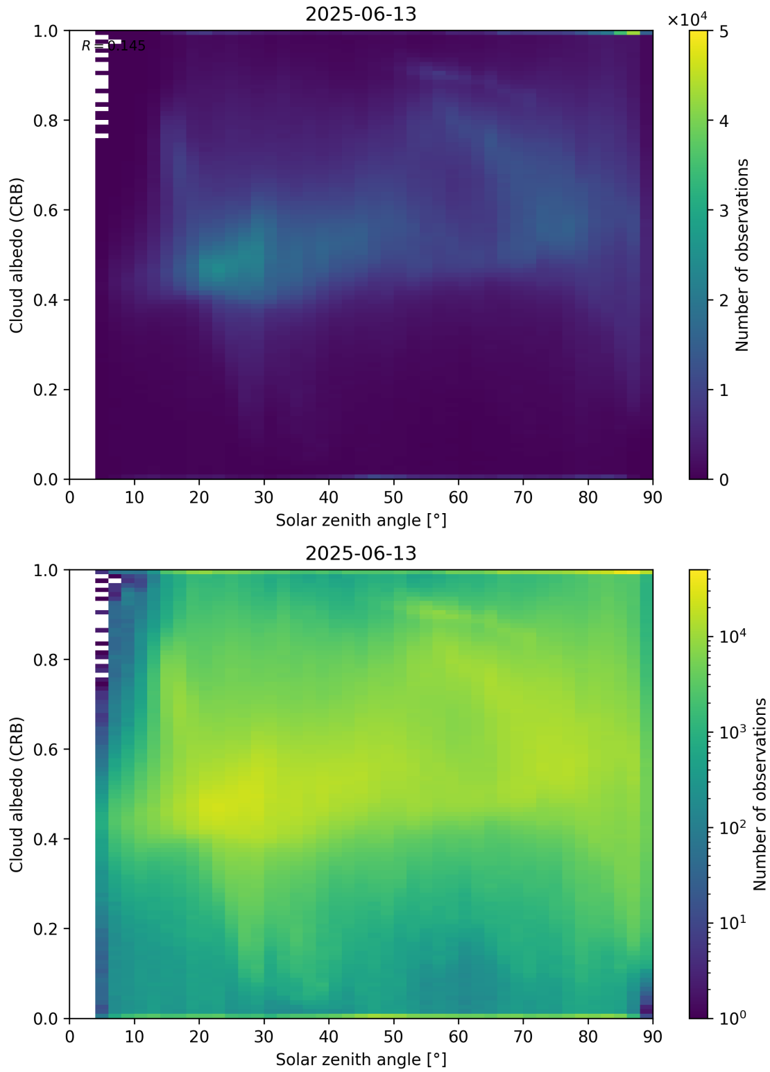
Figure 98: Scatter density plot of “Solar zenith angle” against “Cloud albedo (CRB)” for 2025-06-12 to 2025-06-14.
