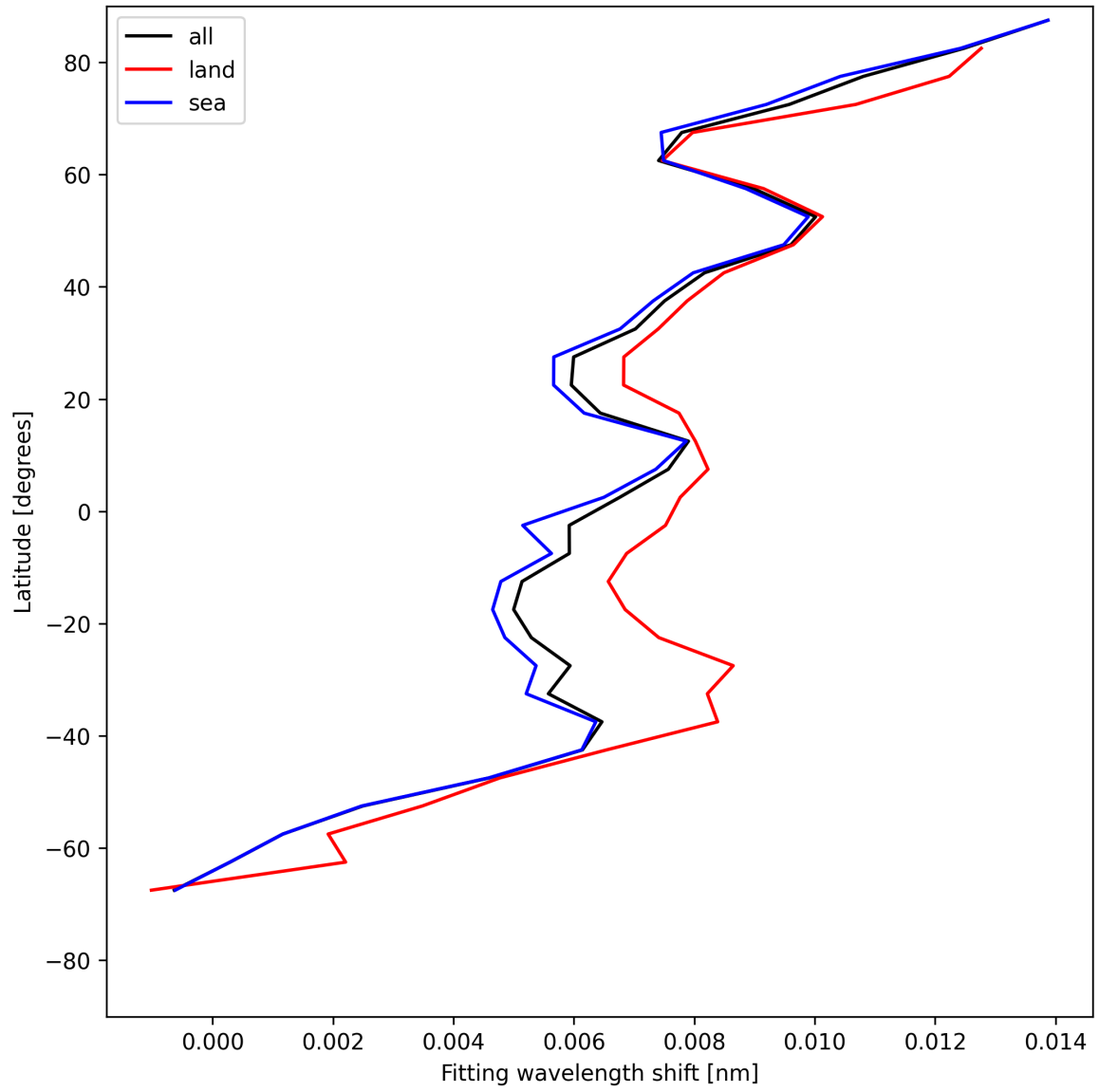
Figure 33: Zonal average of “Fitting wavelength shift” for 2025-06-12 to 2025-06-14.
