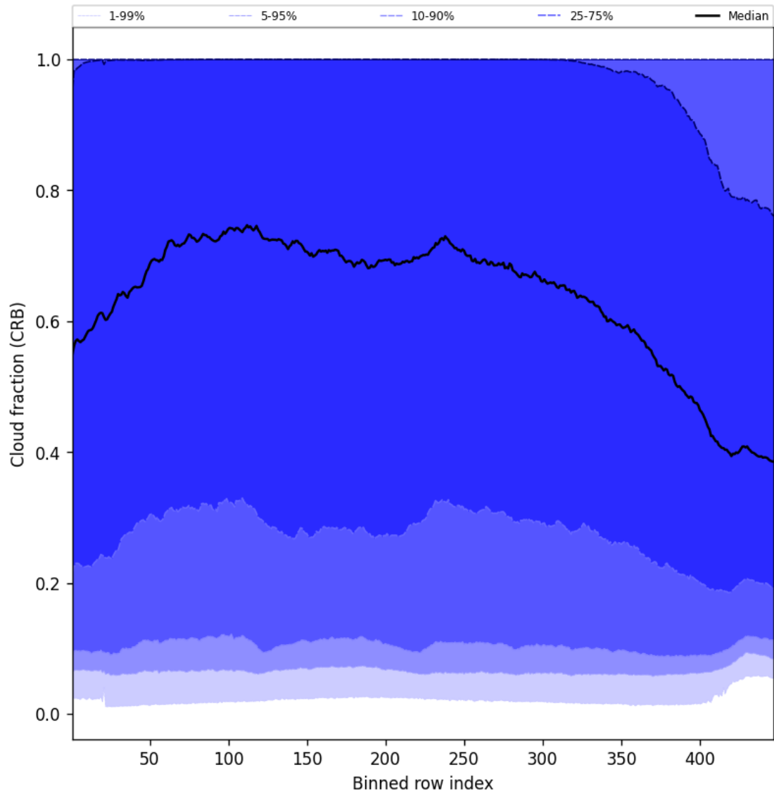
Figure 58: Along track statistics of “Cloud fraction (CRB)” for 2025-06-12 to 2025-06-14
