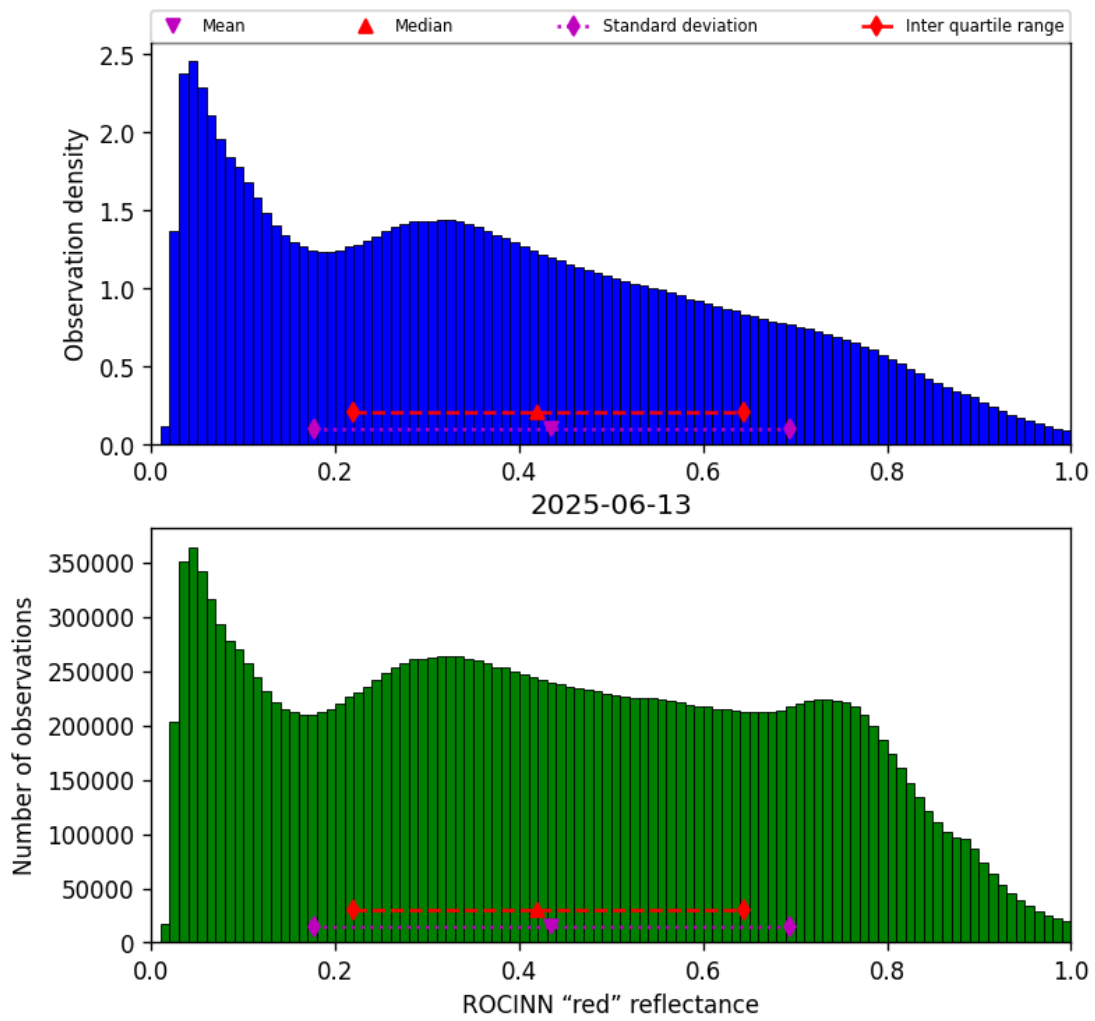
Figure 53: Histogram of "ROCINN "red" reflectance" for 2025-06-12 to 2025-06-14
