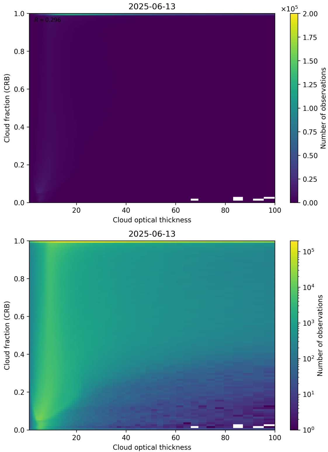
Figure 84: Scatter density plot of “Cloud optical thickness” against “Cloud fraction (CRB)” for 2025-06-12 to 2025-06-14.
