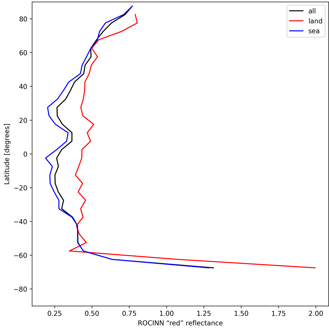
Figure 37: Zonal average of “ROCINN “red” reflectance” for 2025-06-12 to 2025-06-14.
