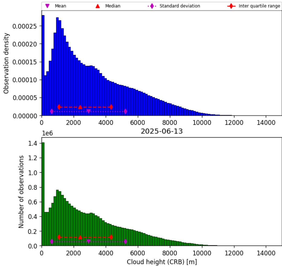
Figure 43: Histogram of “Cloud height (CRB)” for 2025-06-12 to 2025-06-14
