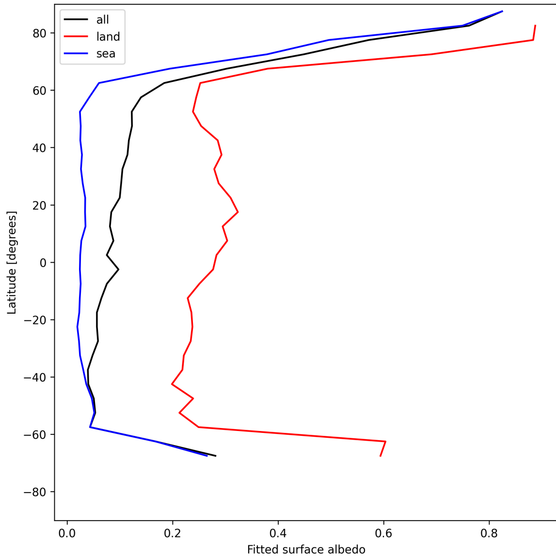
Figure 29: Zonal average of “Fitted surface albedo” for 2025-06-12 to 2025-06-14.
