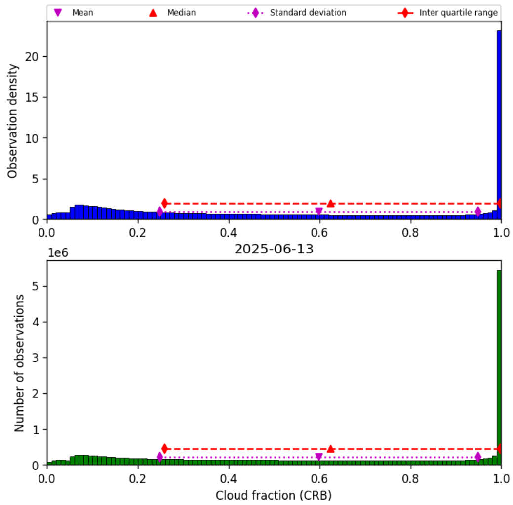
Figure 42: Histogram of “Cloud fraction (CRB)” for 2025-06-12 to 2025-06-14
