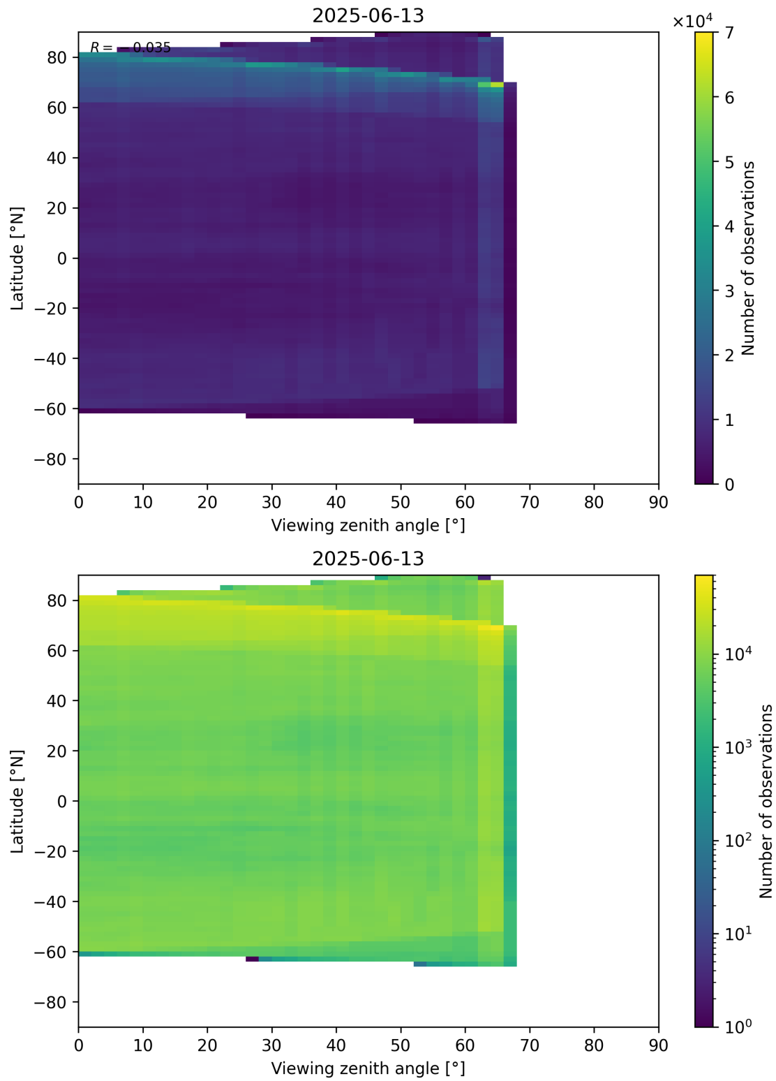
Figure 113: Scatter density plot of “Viewing zenith angle” against “Latitude” for 2025-06-12 to 2025-06-14.
