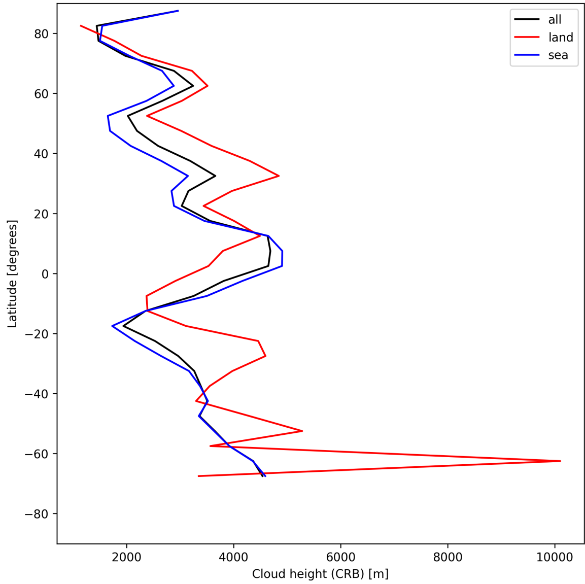
Figure 27: Zonal average of “Cloud height (CRB)” for 2025-06-12 to 2025-06-14.
