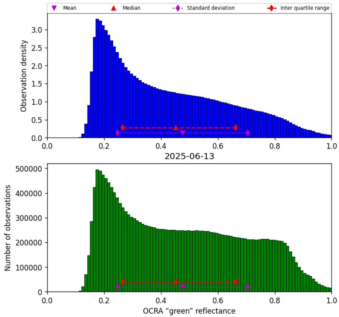
Figure 52: Histogram of “OCRA “green” reflectance” for 2025-06-12 to 2025-06-14
