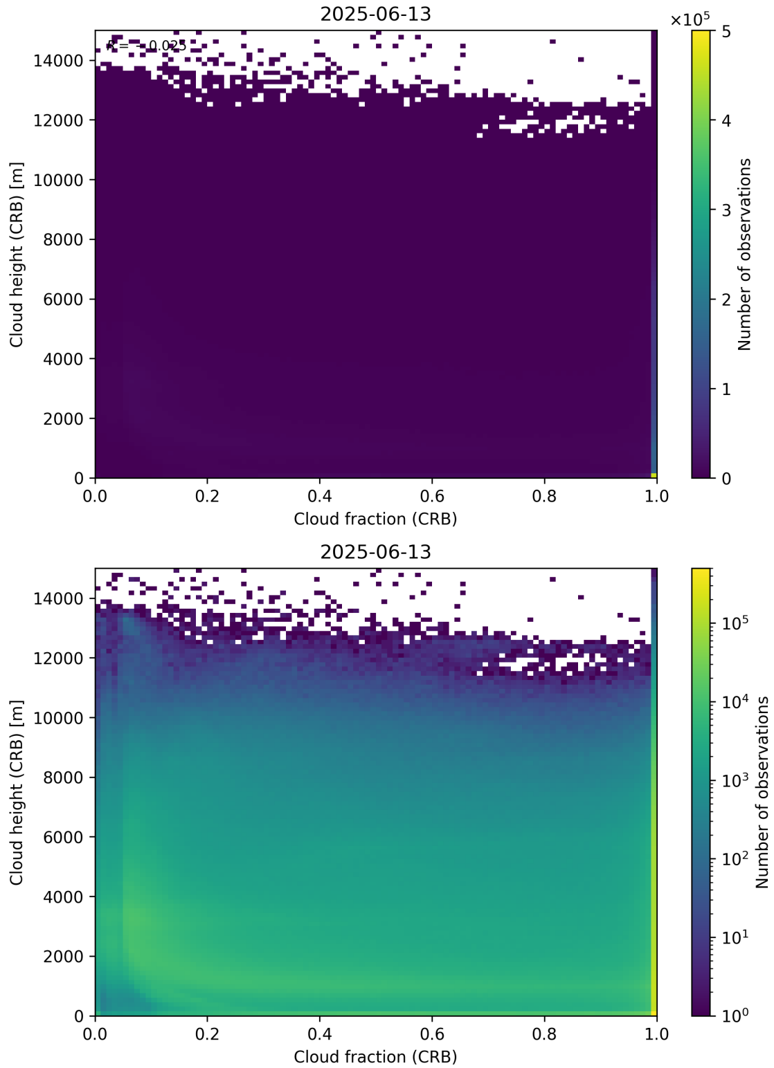
Figure 79: Scatter density plot of “Cloud fraction (CRB)” against “Cloud height (CRB)” for 2025-06-12 to 2025-06-14.
