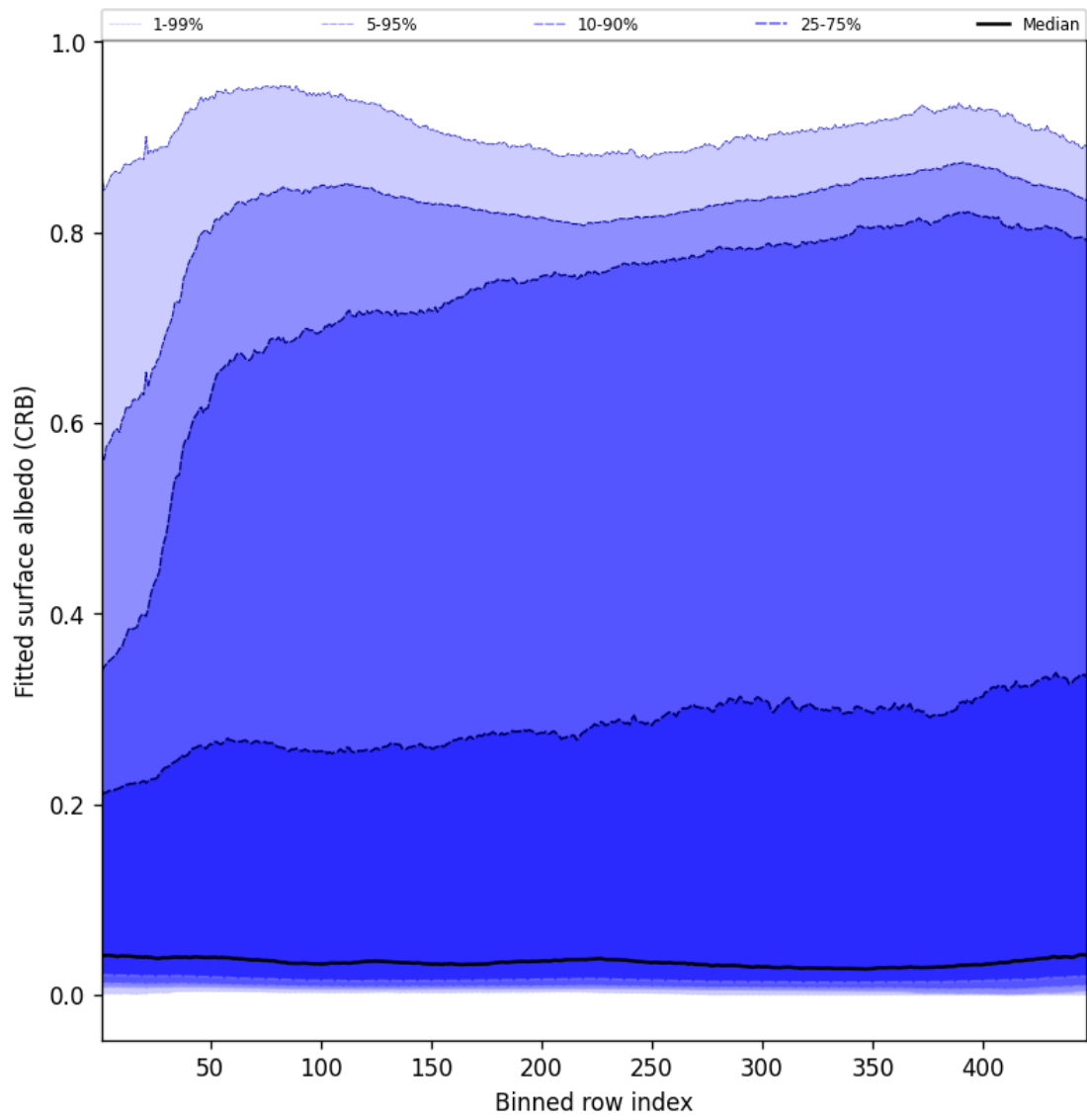
Figure 62: Along track statistics of “Fitted surface albedo (CRB)” for 2025-06-12 to 2025-06-14
