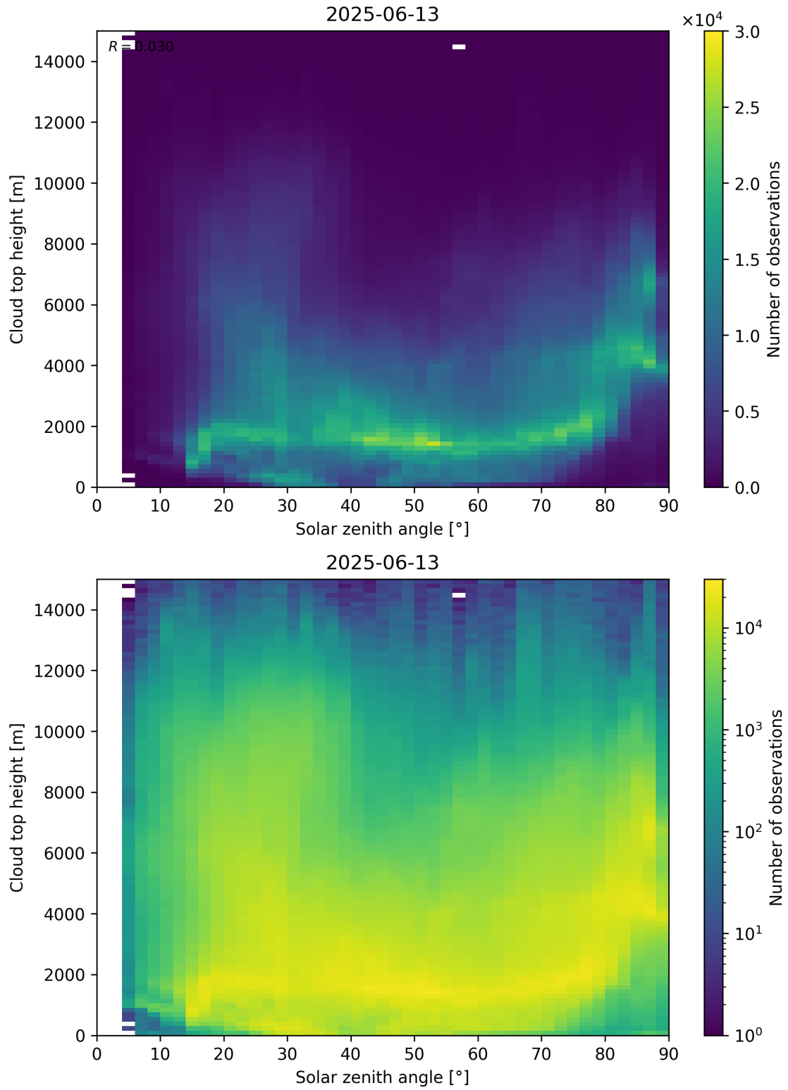
Figure 104: Scatter density plot of “Solar zenith angle” against “Cloud top height” for 2025-06-12 to 2025-06-14.
