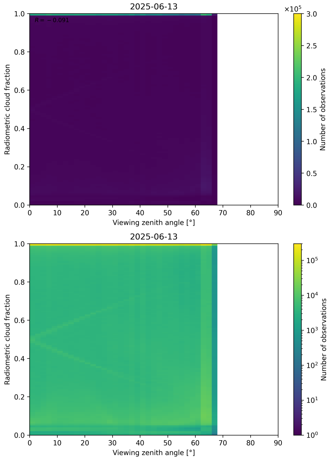
Figure 107: Scatter density plot of “Viewing zenith angle” against “Radiometric cloud fraction” for 2025-06-12 to 2025-06-14.
