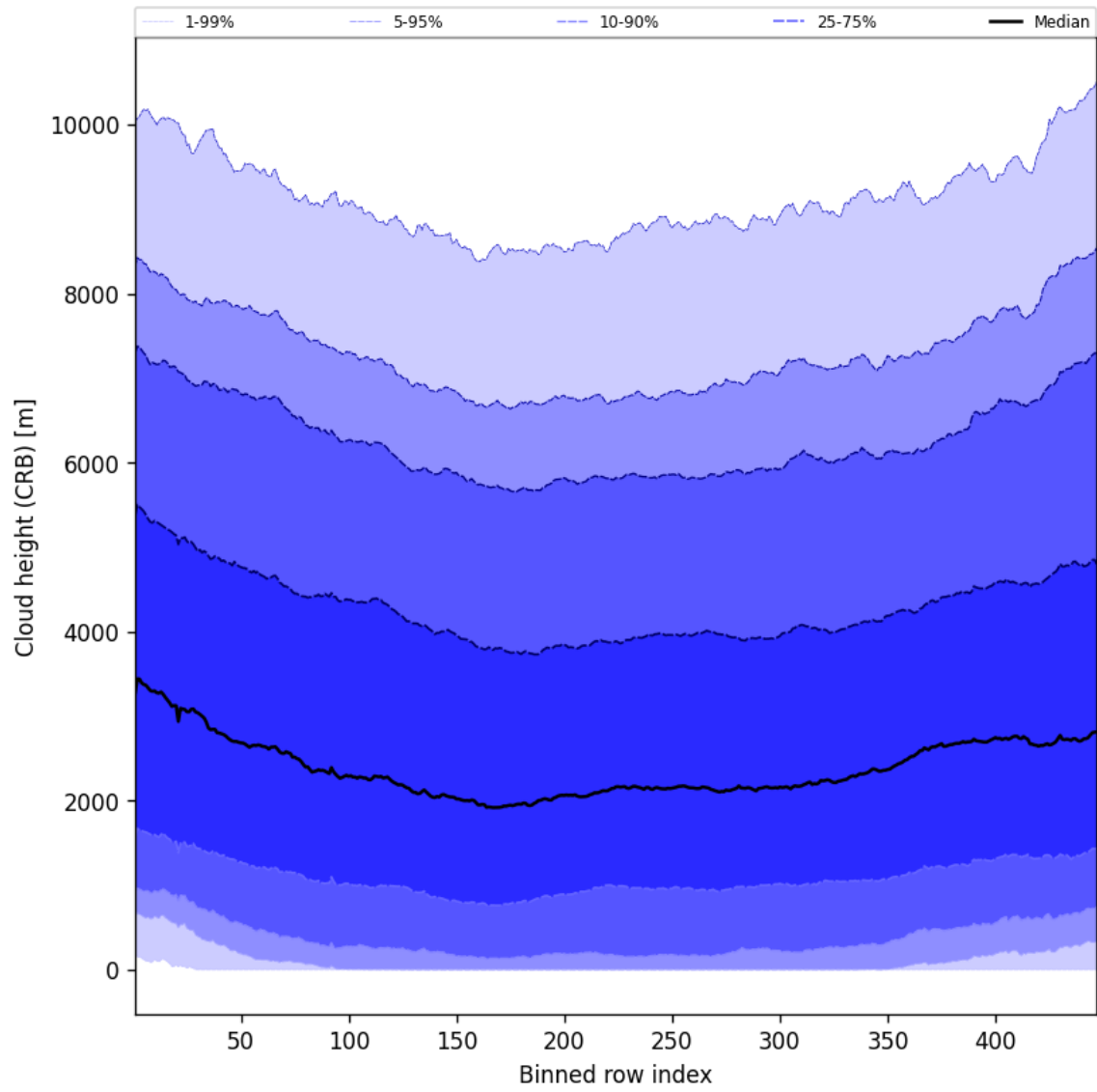
Figure 59: Along track statistics of “Cloud height (CRB)” for 2025-06-12 to 2025-06-14
