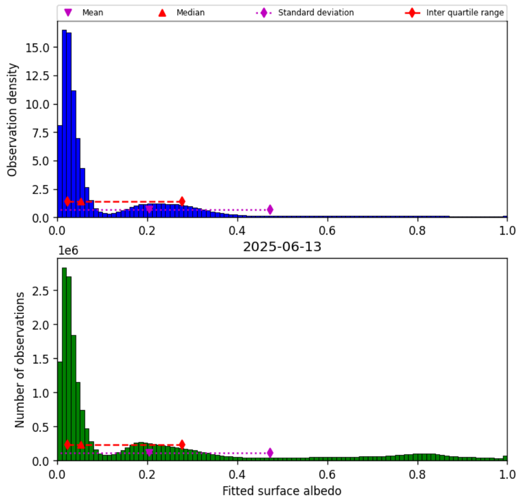
Figure 45: Histogram of “Fitted surface albedo” for 2025-06-12 to 2025-06-14
