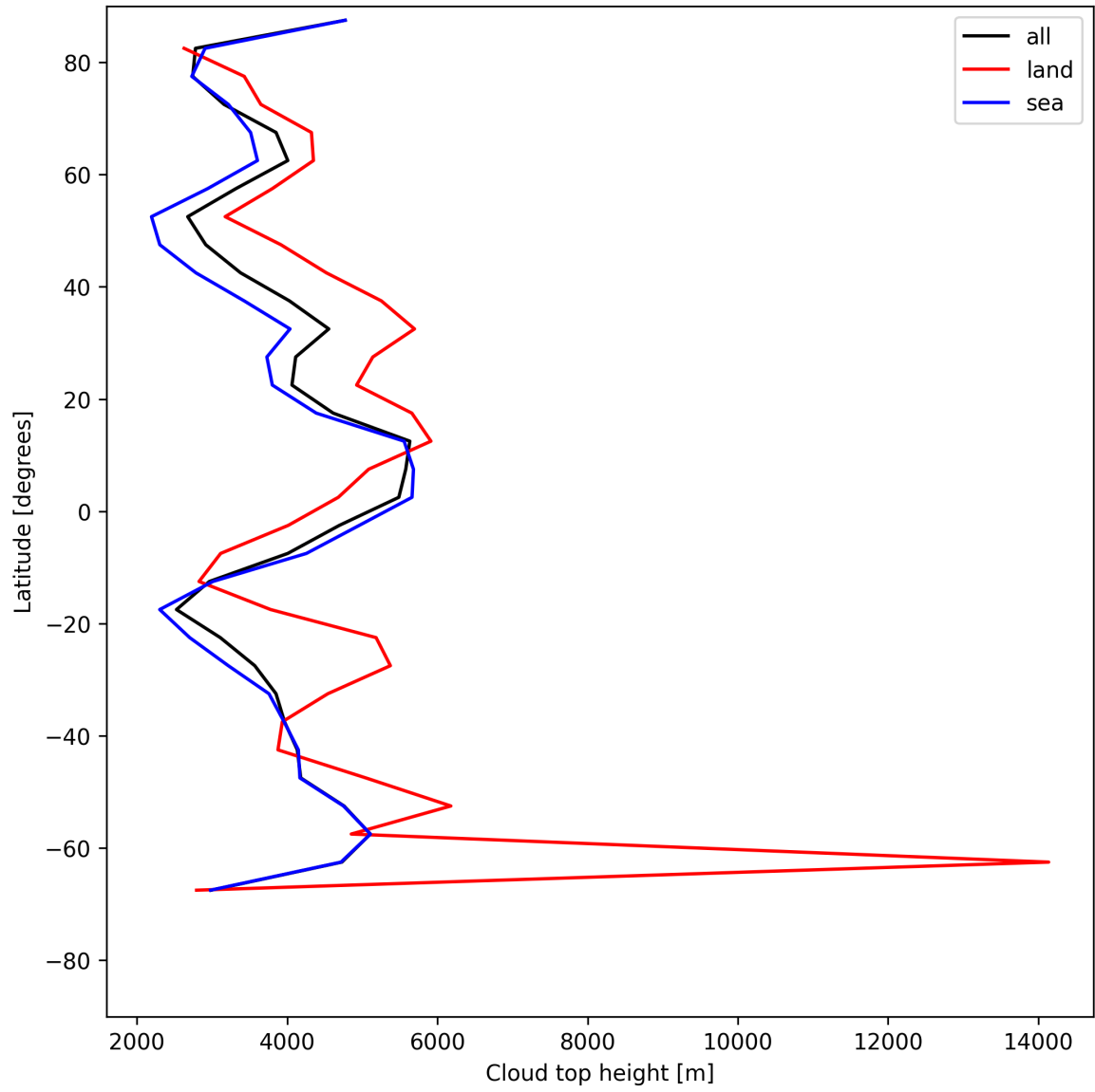
Figure 24: Zonal average of “Cloud top height” for 2025-06-12 to 2025-06-14.
