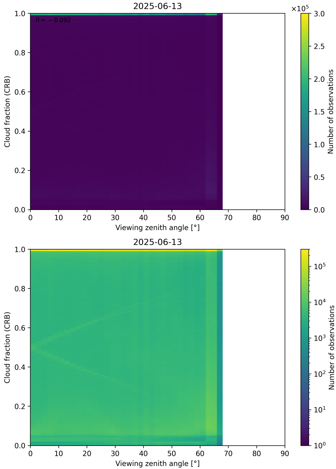
Figure 109: Scatter density plot of “Viewing zenith angle” against “Cloud fraction (CRB)” for 2025-06-12 to 2025-06-14.
