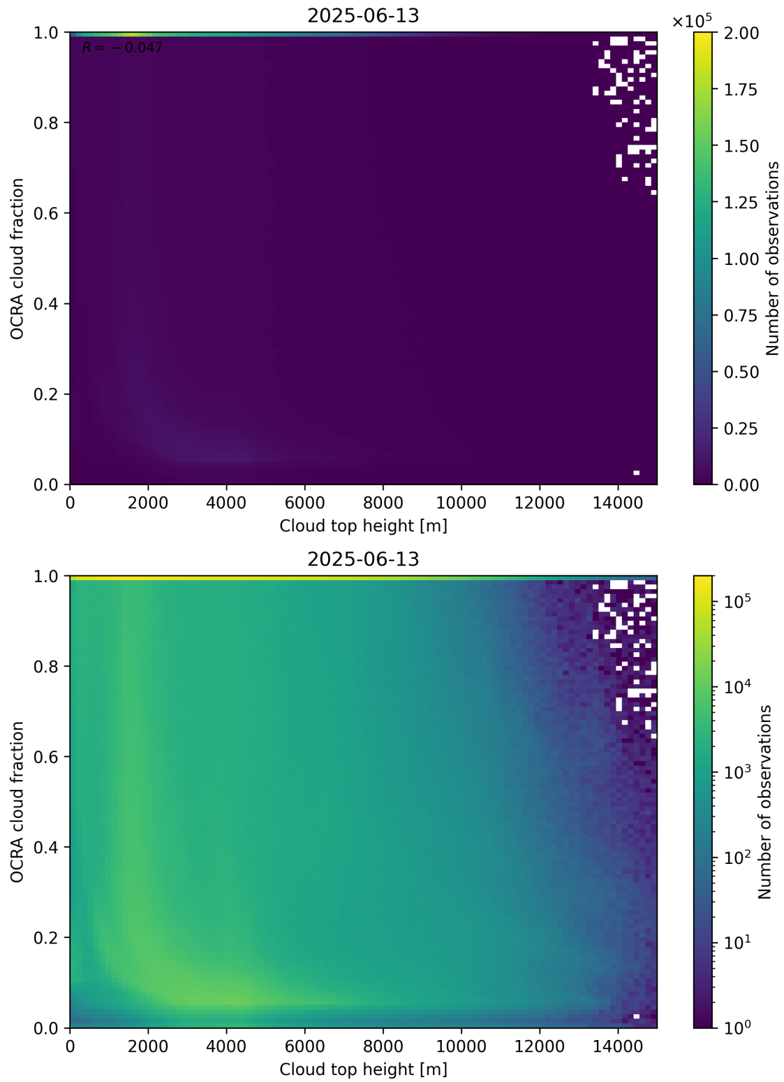
Figure 87: Scatter density plot of “Cloud top height” against “OCRA cloud fraction” for 2025-06-12 to 2025-06-14.
