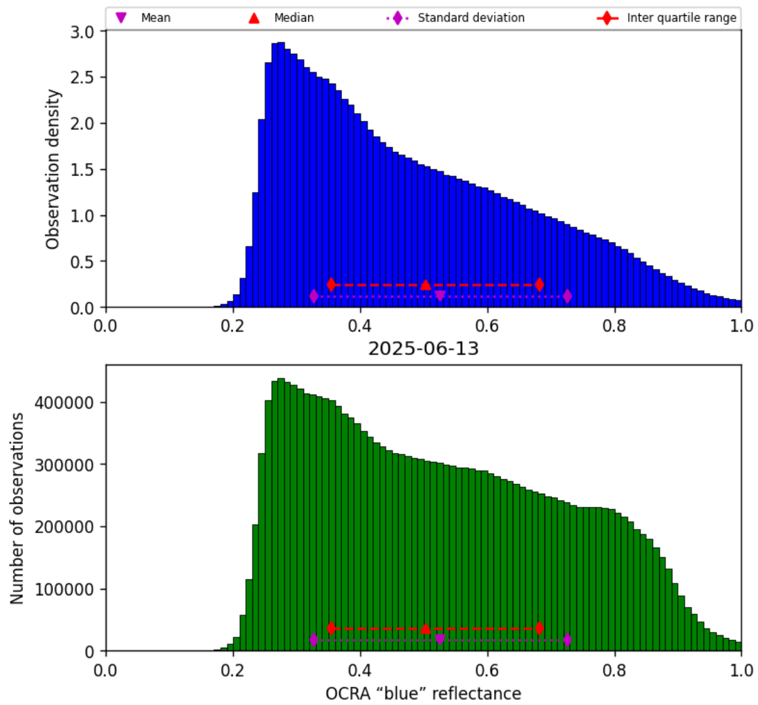
Figure 51: Histogram of “OCRA “blue” reflectance” for 2025-06-12 to 2025-06-14
