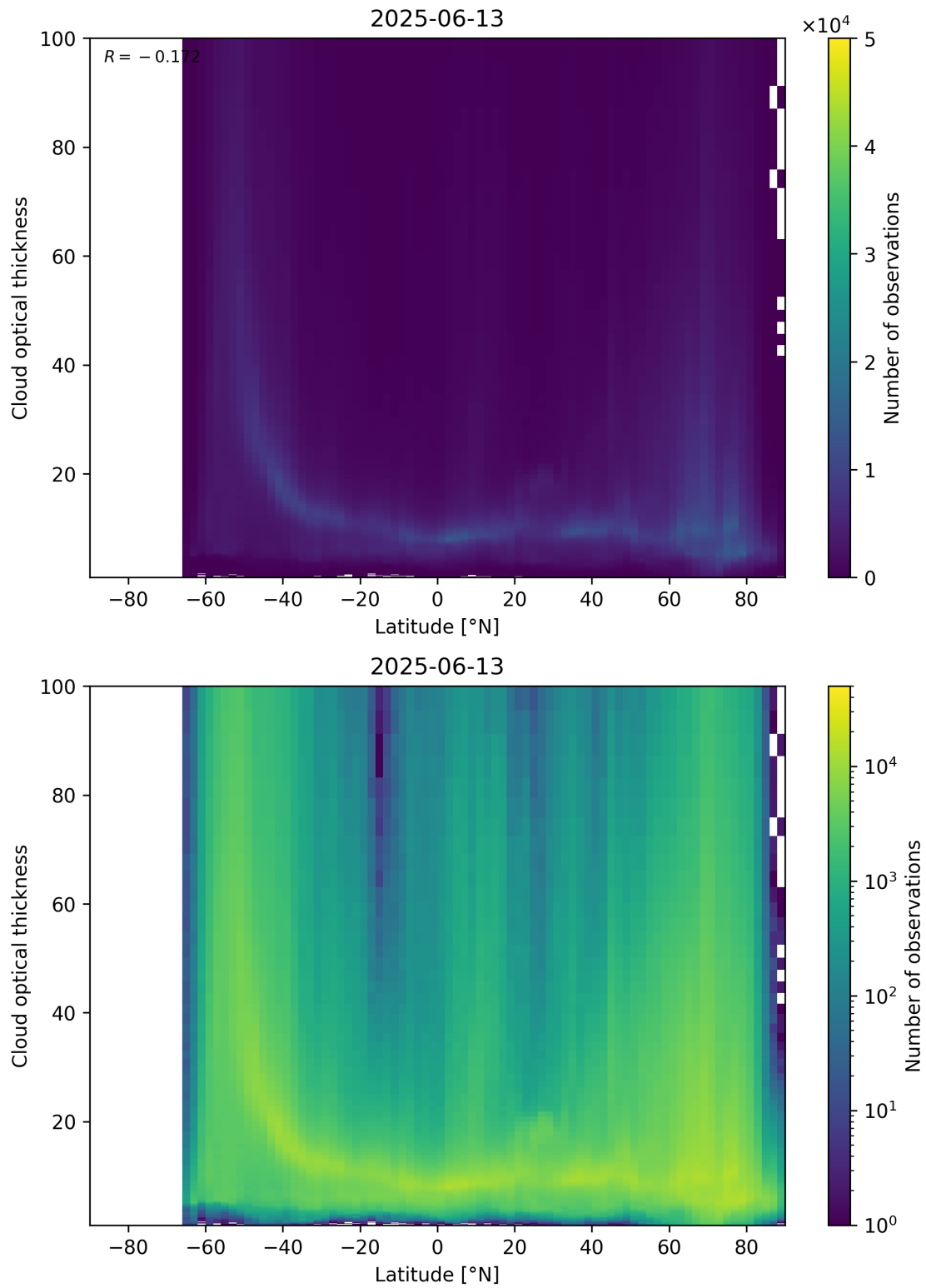
Figure 96: Scatter density plot of “Latitude” against “Cloud optical thickness” for 2025-06-12 to 2025-06-14.
