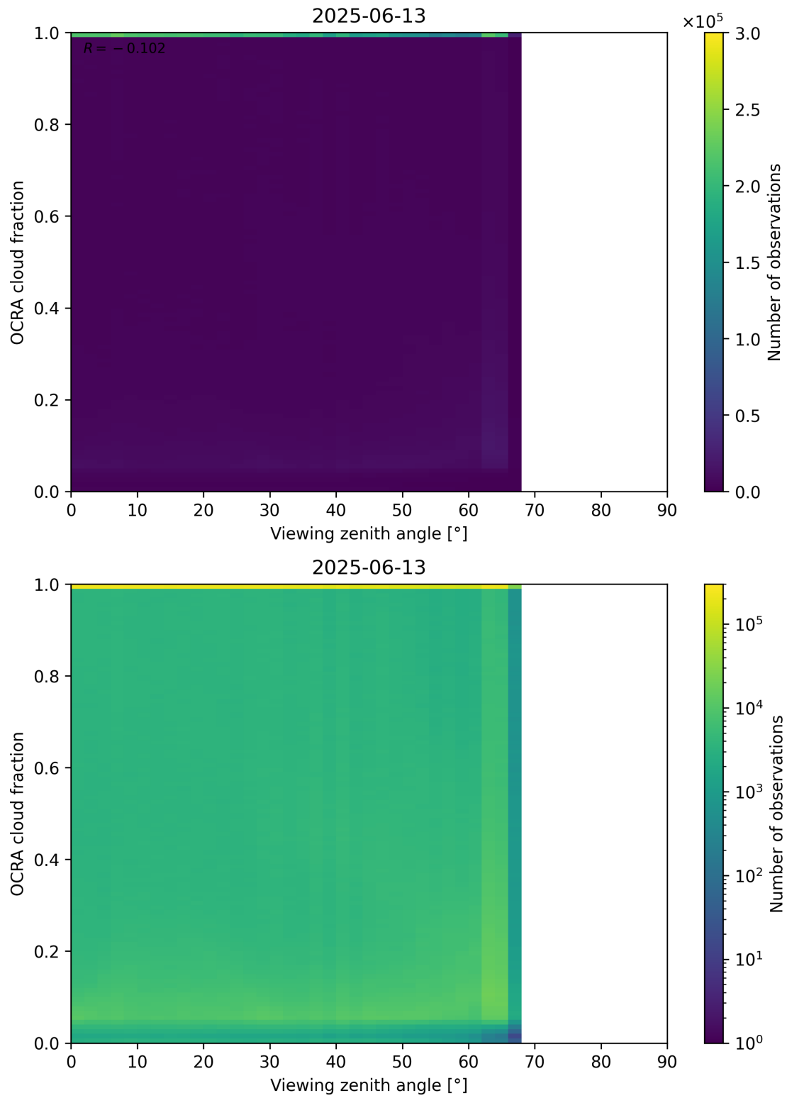
Figure 108: Scatter density plot of “Viewing zenith angle” against “OCRA cloud fraction” for 2025-06-12 to 2025-06-14.
