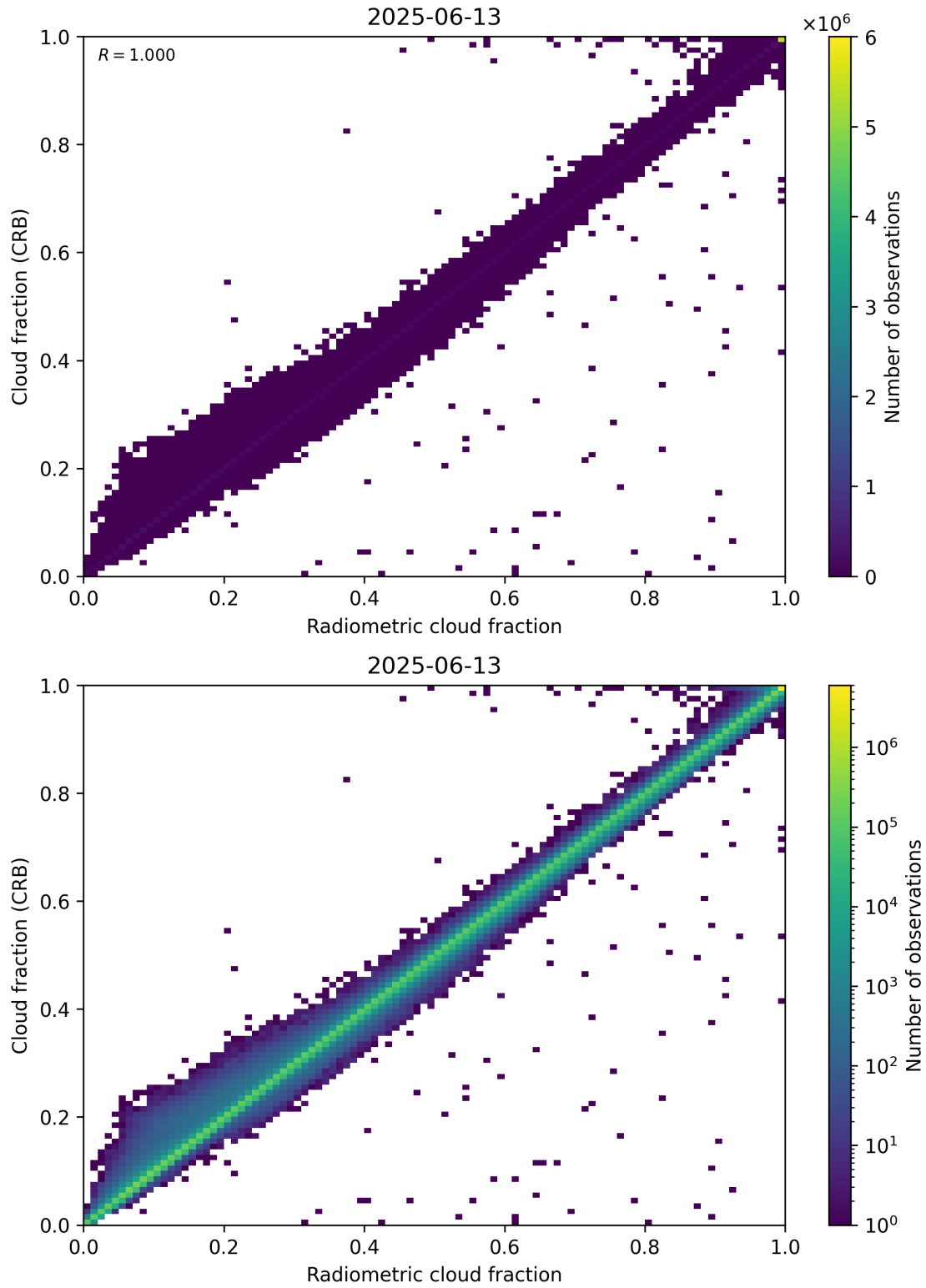
Figure 73: Scatter density plot of “Radiometric cloud fraction” against “Cloud fraction (CRB)” for 2025-06-12 to 2025-06-14.
