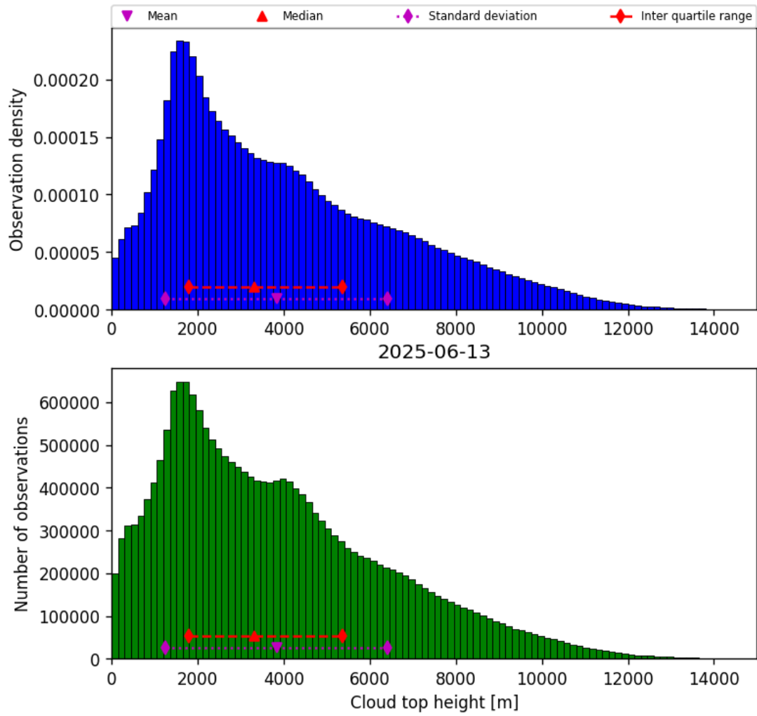
Figure 40: Histogram of “Cloud top height” for 2025-06-12 to 2025-06-14
