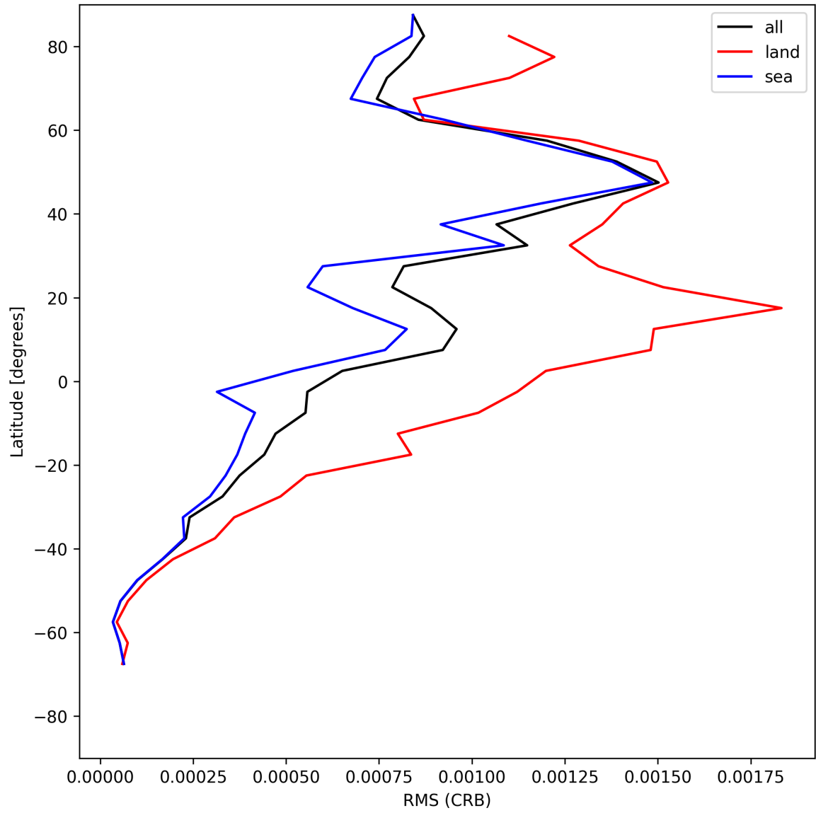
Figure 32: Zonal average of “RMS (CRB)” for 2025-06-12 to 2025-06-14.
