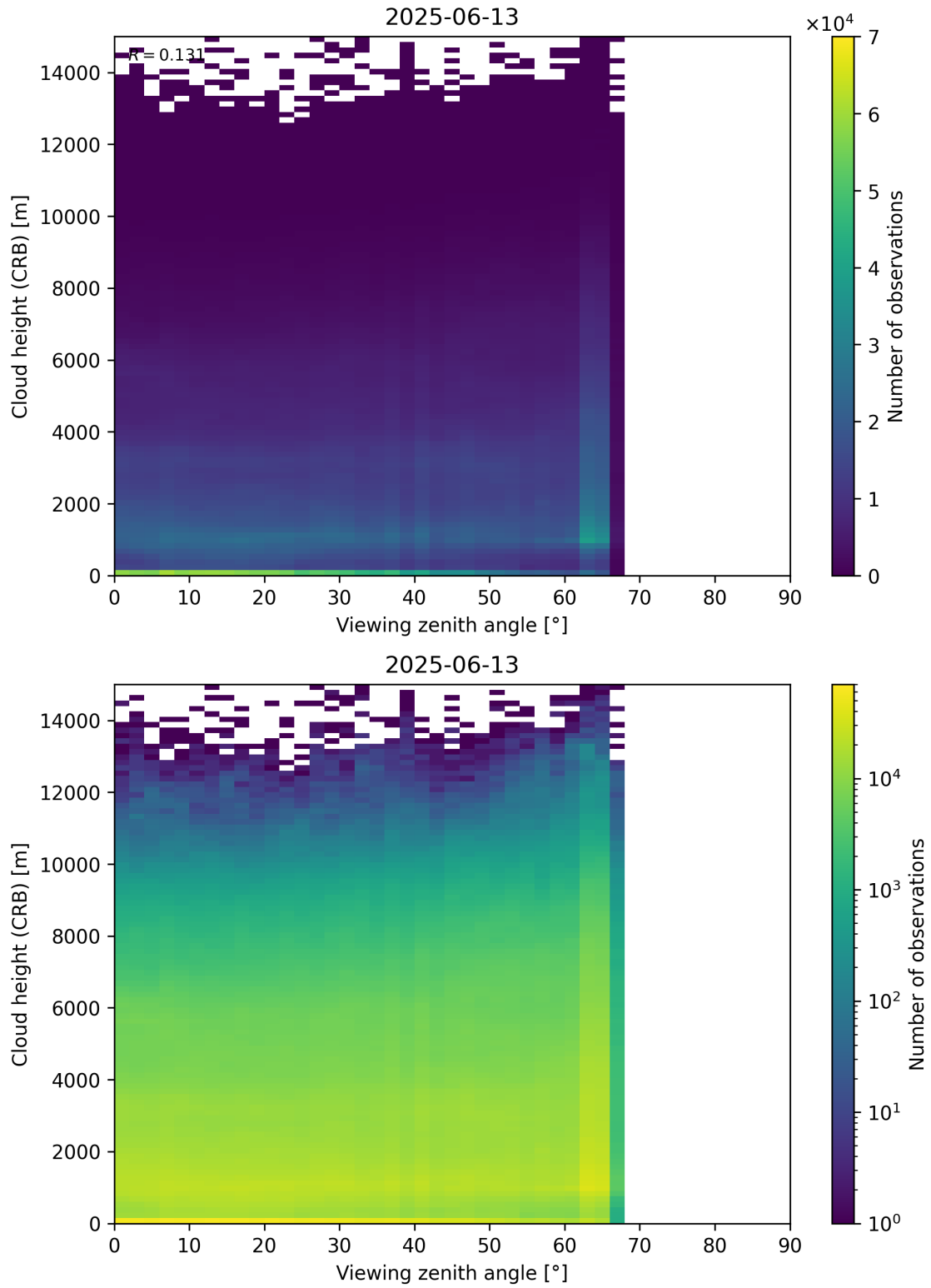
Figure 110: Scatter density plot of “Viewing zenith angle” against “Cloud height (CRB)” for 2025-06-12 to 2025-06-14.
