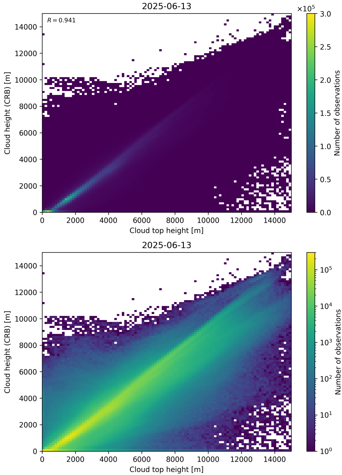
Figure 89: Scatter density plot of “Cloud top height” against “Cloud height (CRB)” for 2025-06-12 to 2025-06-14.
