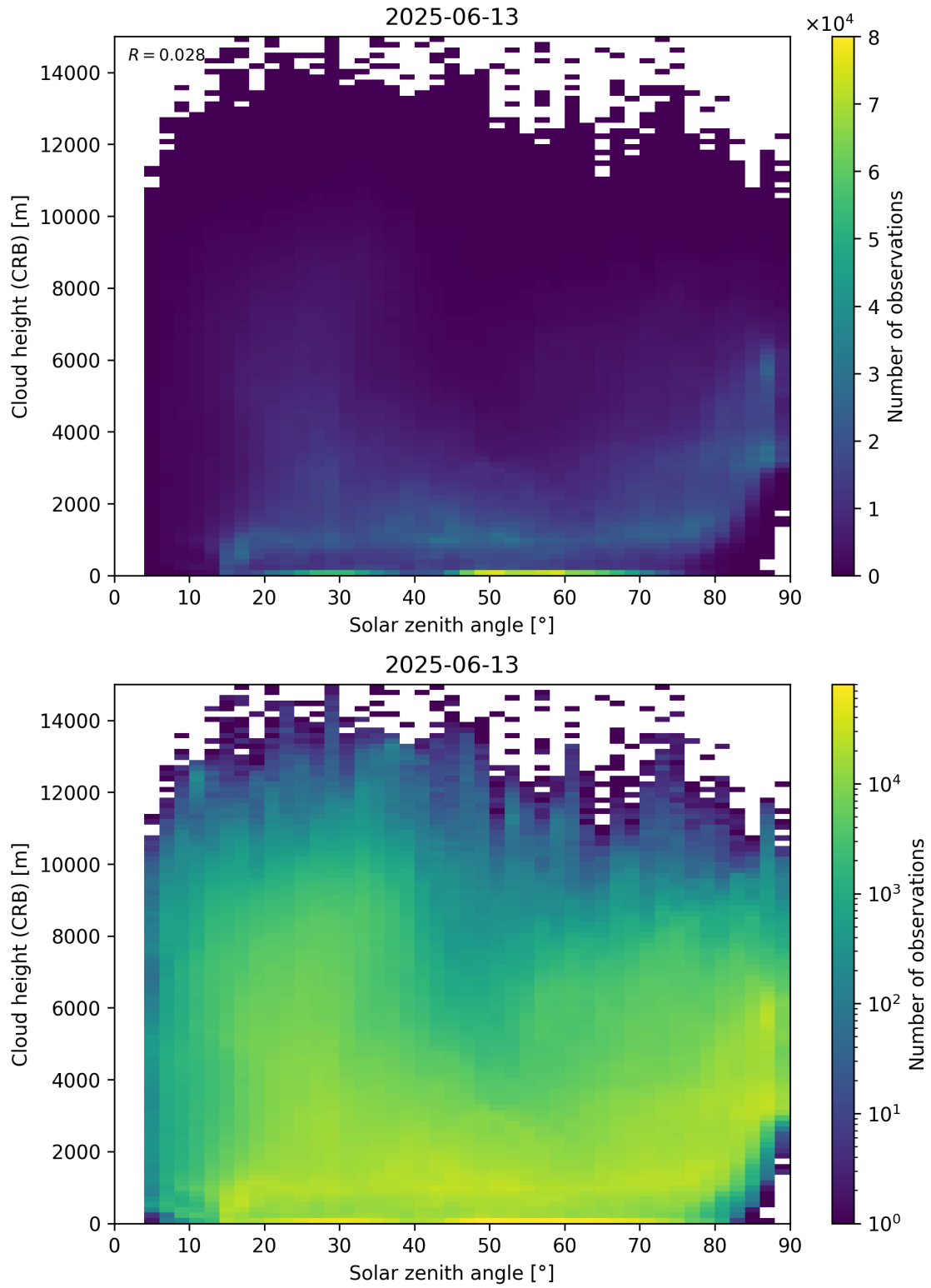
Figure 102: Scatter density plot of “Solar zenith angle” against “Cloud height (CRB)” for 2025-06-12 to 2025-06-14.
