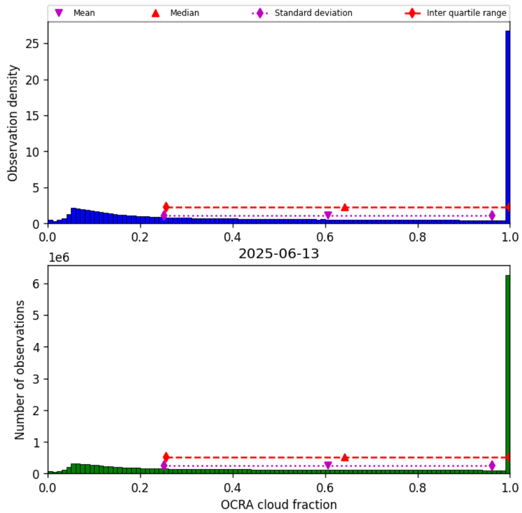
Figure 50: Histogram of “OCRA cloud fraction” for 2025-06-12 to 2025-06-14
