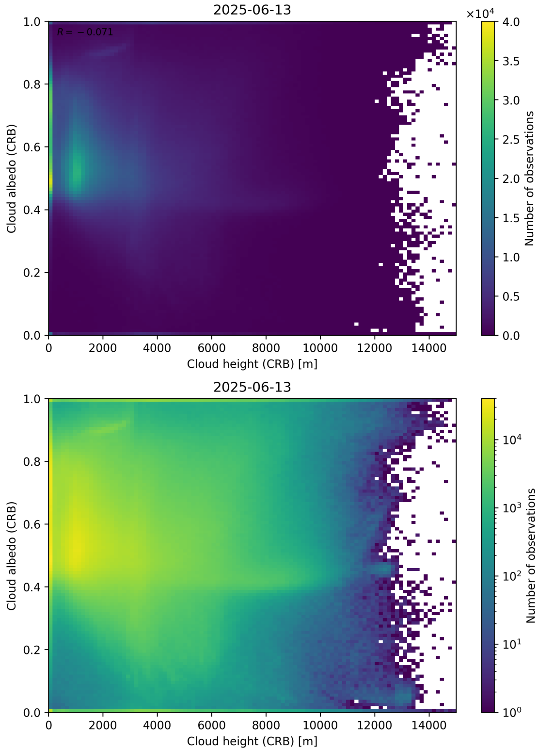
Figure 80: Scatter density plot of “Cloud height (CRB)” against “Cloud albedo (CRB)” for 2025-06-12 to 2025-06-14.
