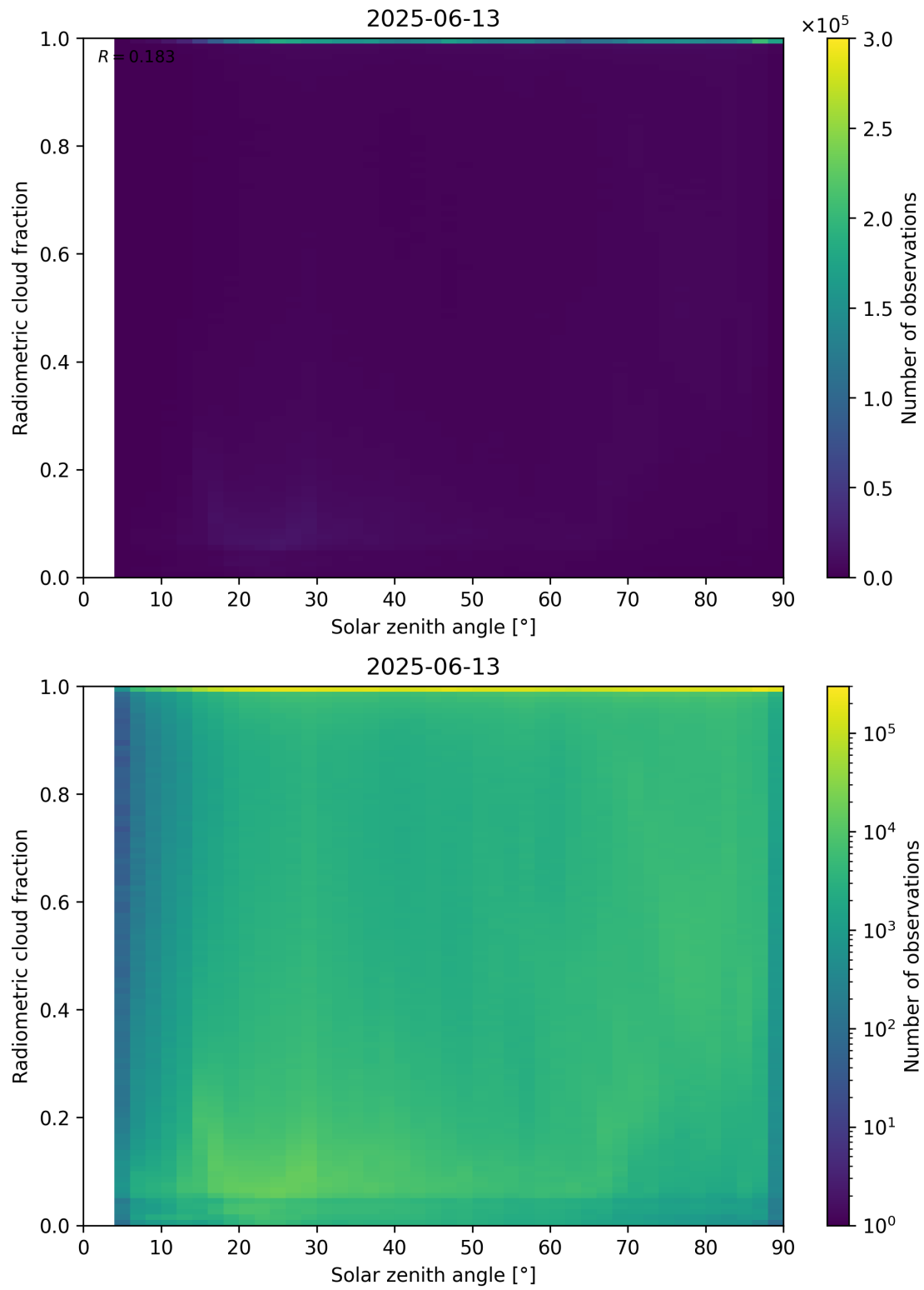
Figure 99: Scatter density plot of “Solar zenith angle” against “Radiometric cloud fraction” for 2025-06-12 to 2025-06-14.
