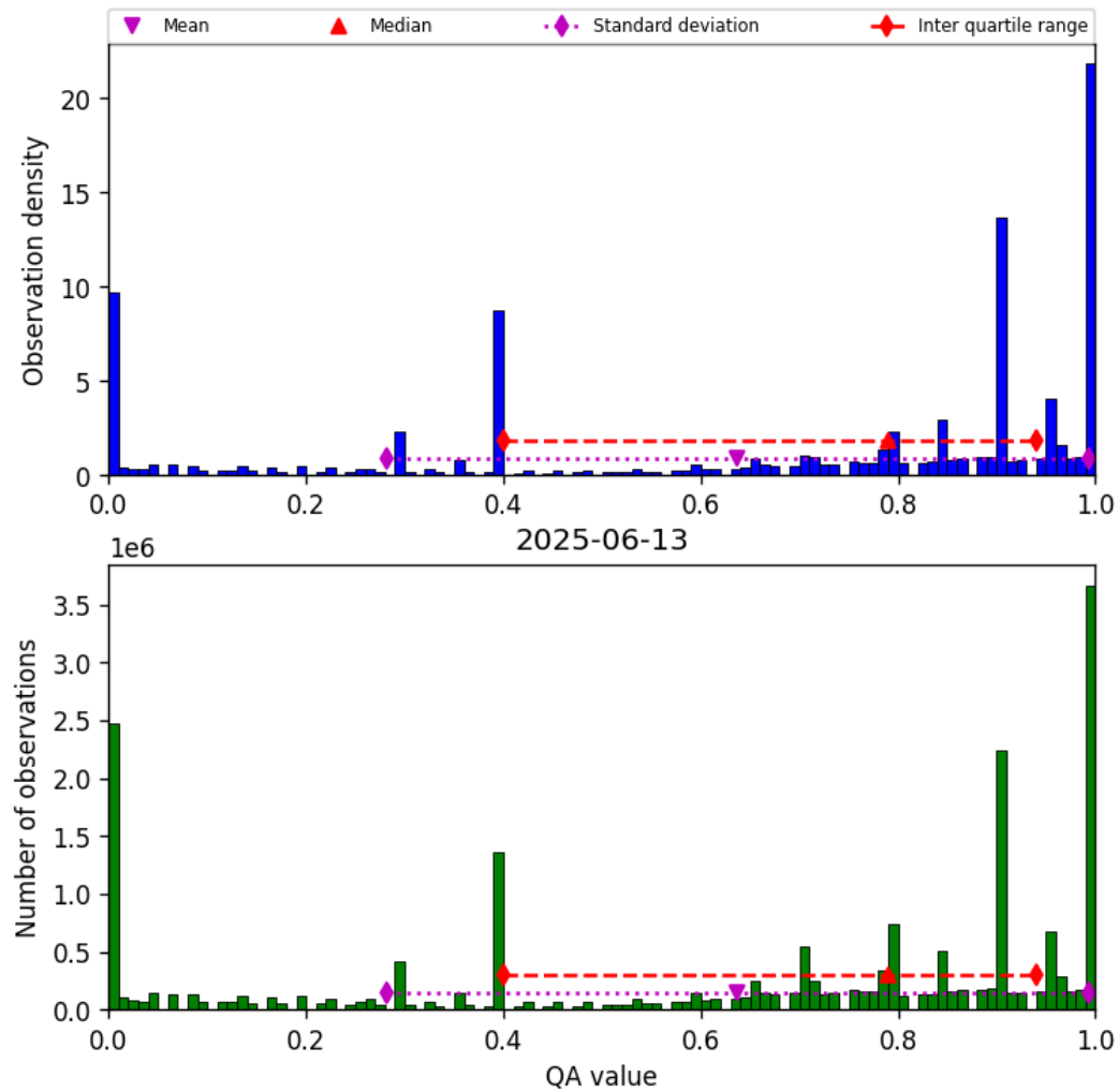
Figure 38: Histogram of “QA value” for 2025-06-12 to 2025-06-14
