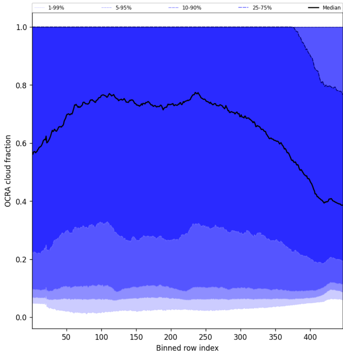
Figure 66: Along track statistics of “OCRA cloud fraction” for 2025-06-12 to 2025-06-14
