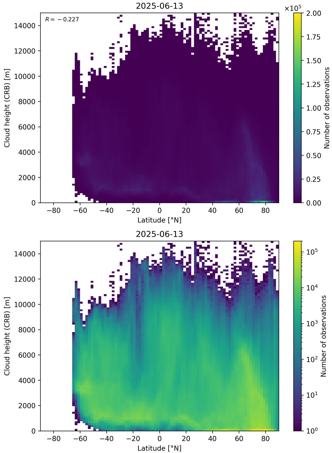
Figure 95: Scatter density plot of “Latitude” against “Cloud height (CRB)” for 2025-06-12 to 2025-06-14.
