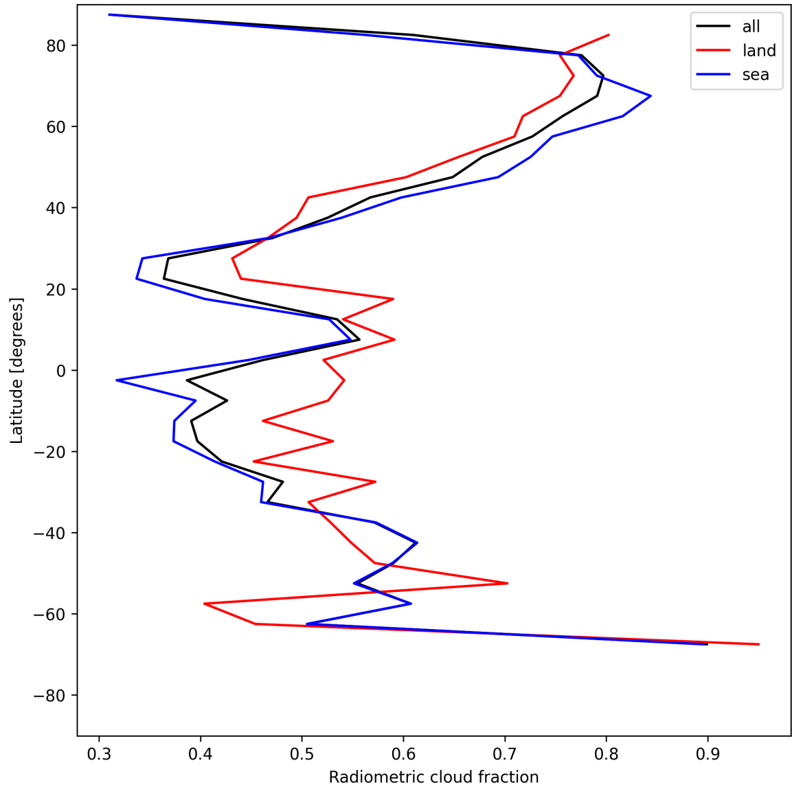
Figure 23: Zonal average of “Radiometric cloud fraction” for 2025-06-12 to 2025-06-14.
