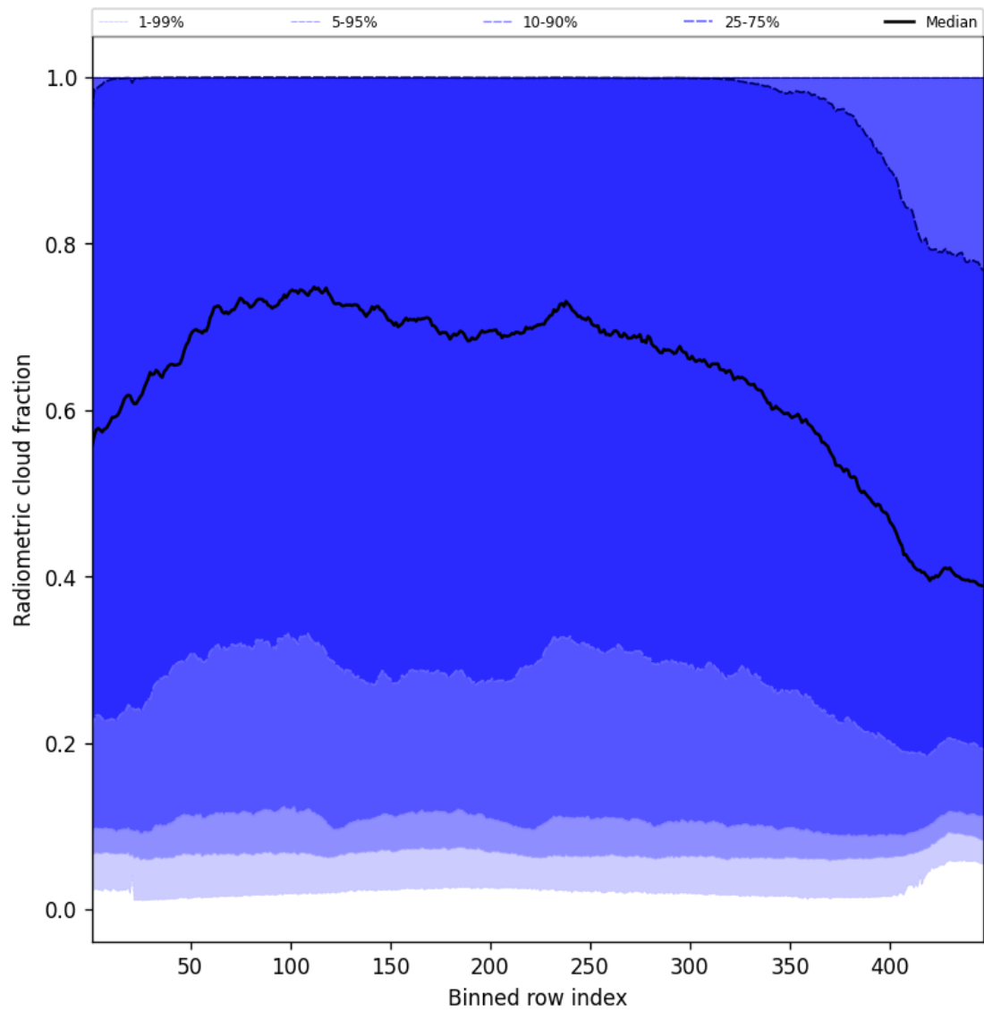
Figure 55: Along track statistics of “Radiometric cloud fraction” for 2025-06-12 to 2025-06-14
