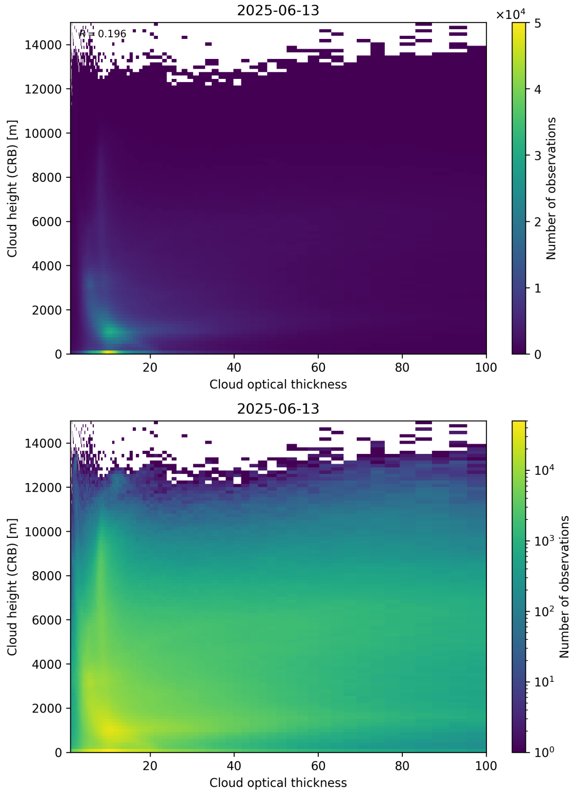
Figure 85: Scatter density plot of “Cloud optical thickness” against “Cloud height (CRB)” for 2025-06-12 to 2025-06-14.
