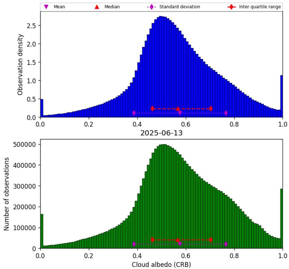
Figure 44: Histogram of “Cloud albedo (CRB)” for 2025-06-12 to 2025-06-14
