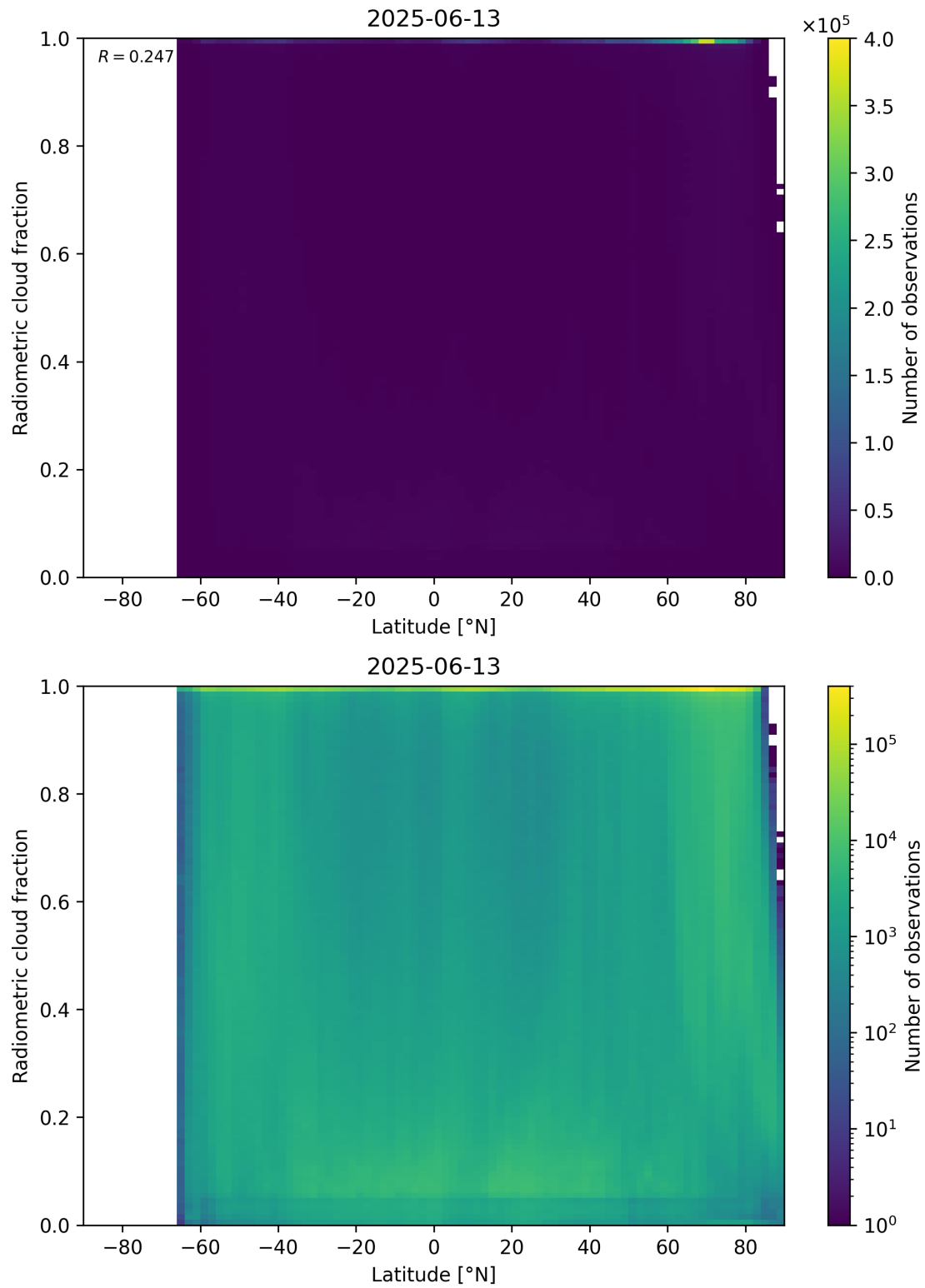
Figure 92: Scatter density plot of “Latitude” against “Radiometric cloud fraction” for 2025-06-12 to 2025-06-14.
