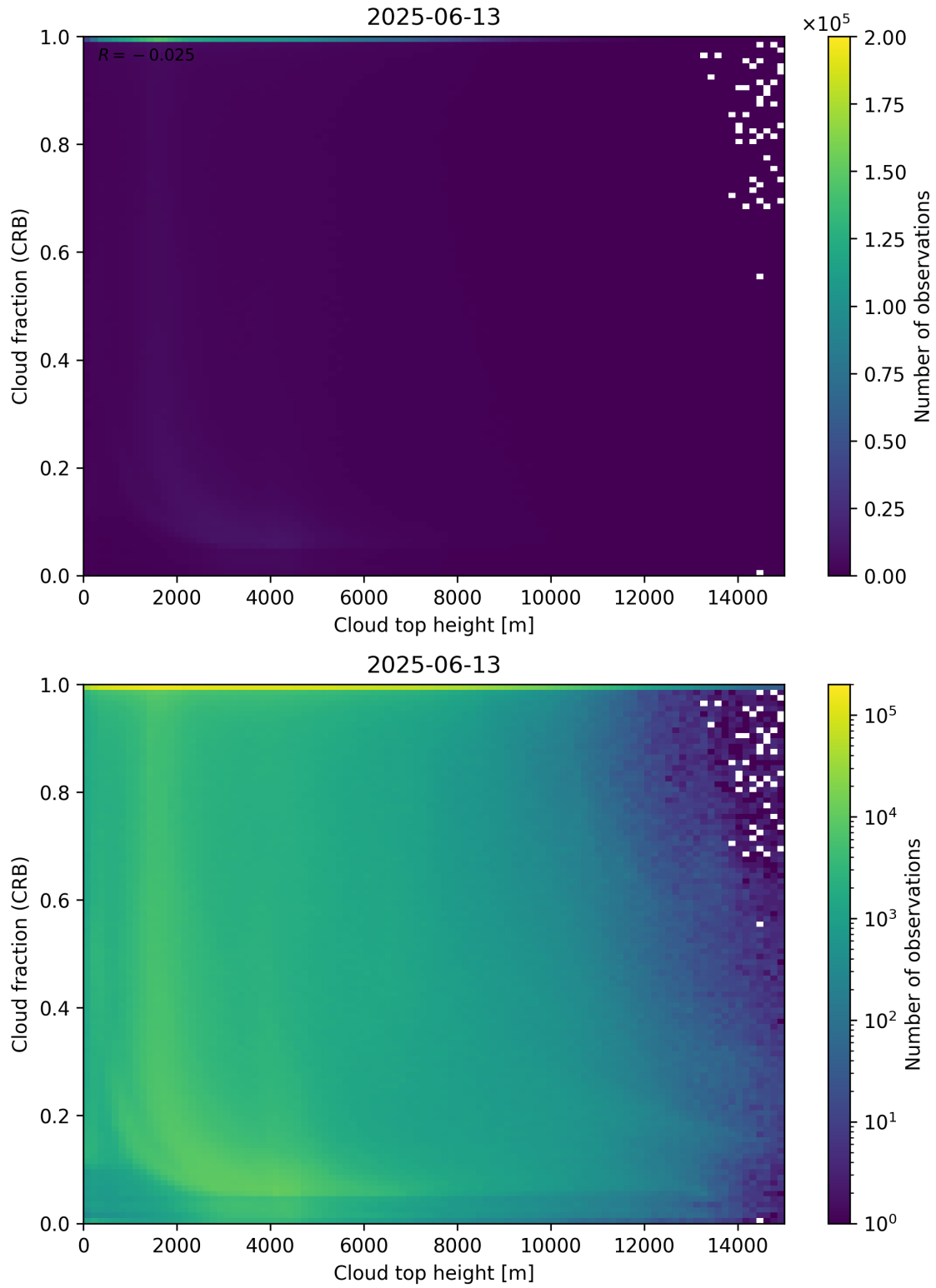
Figure 88: Scatter density plot of “Cloud top height” against “Cloud fraction (CRB)” for 2025-06-12 to 2025-06-14.
