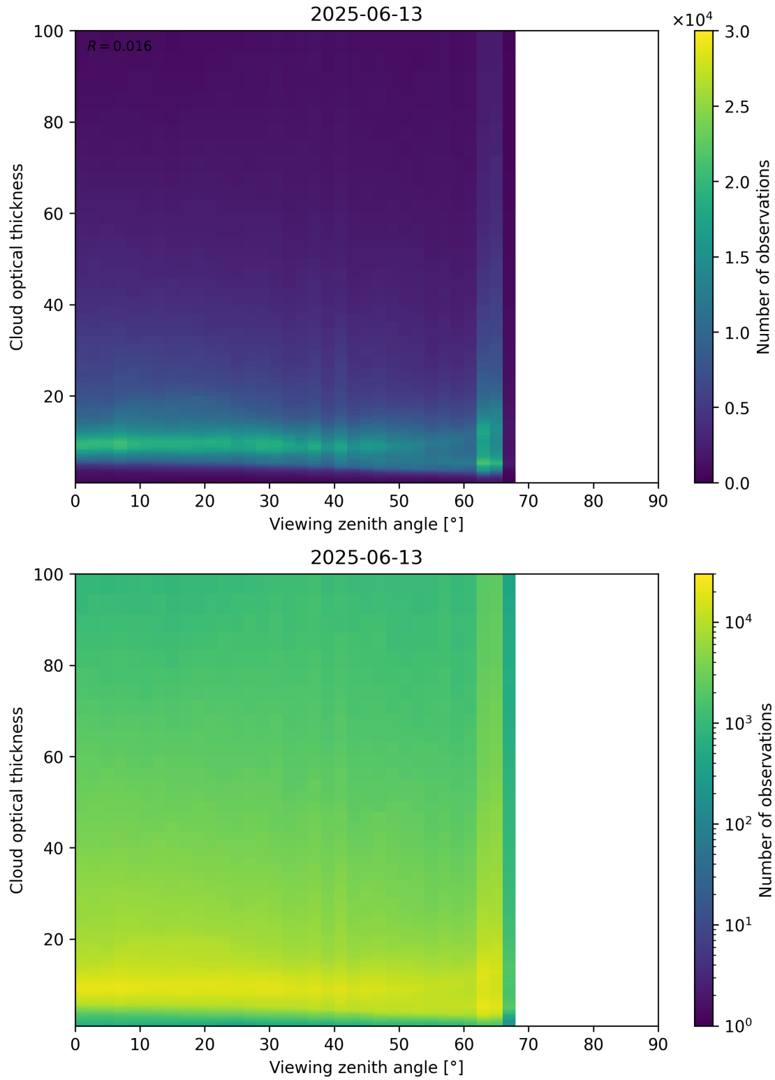
Figure 111: Scatter density plot of “Viewing zenith angle” against “Cloud optical thickness” for 2025-06-12 to 2025-06-14.
