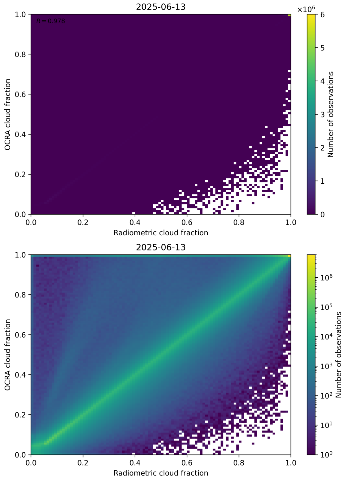
Figure 72: Scatter density plot of “Radiometric cloud fraction” against “OCRA cloud fraction” for 2025-06-12 to 2025-06-14.
