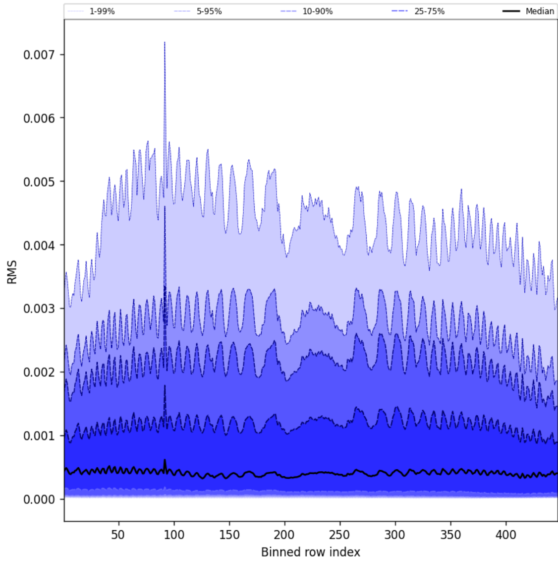
Figure 63: Along track statistics of “RMS” for 2025-06-12 to 2025-06-14
