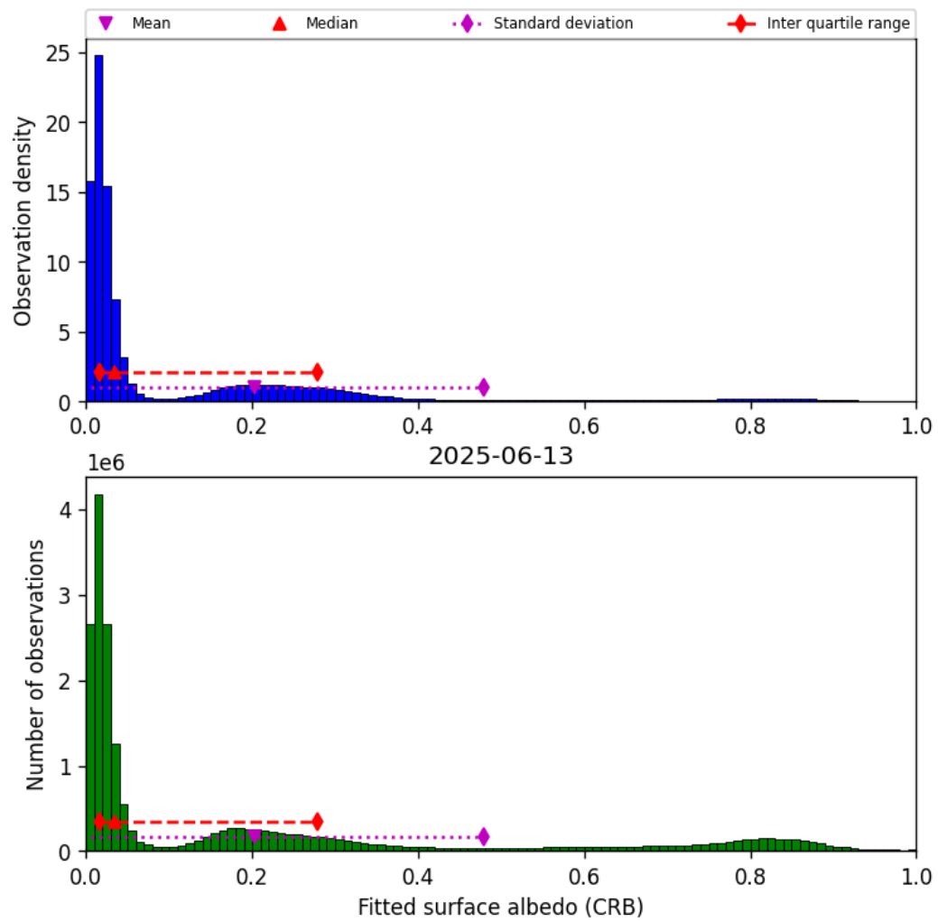
Figure 46: Histogram of “Fitted surface albedo (CRB)” for 2025-06-12 to 2025-06-14
