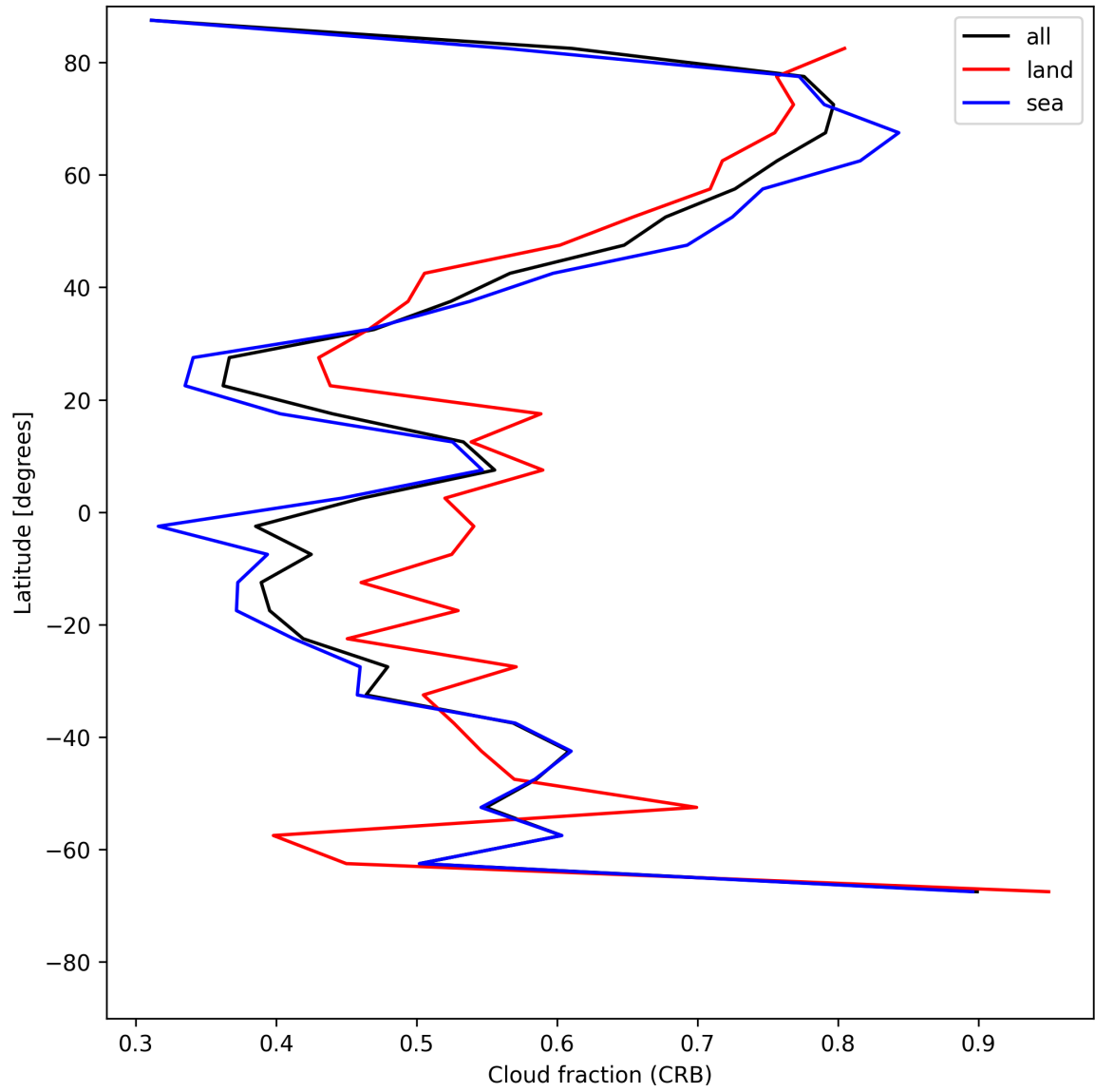
Figure 26: Zonal average of “Cloud fraction (CRB)” for 2025-06-12 to 2025-06-14.
