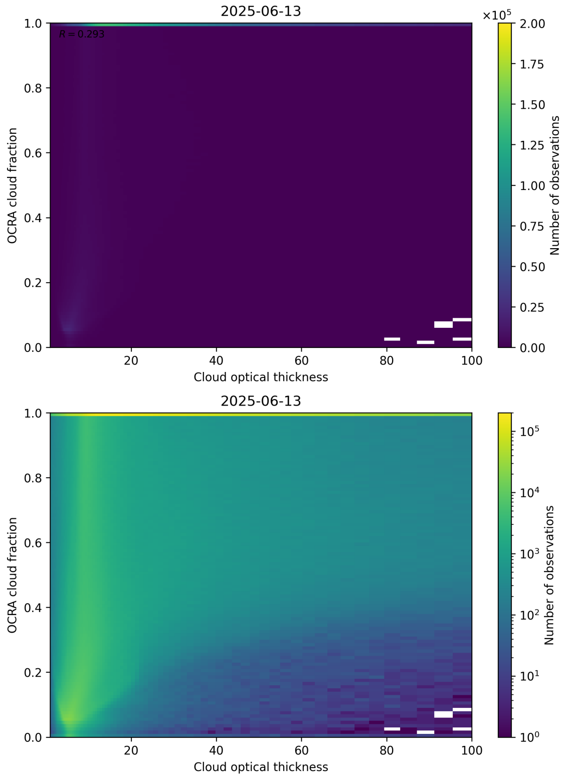
Figure 83: Scatter density plot of “Cloud optical thickness” against “OCRA cloud fraction” for 2025-06-12 to 2025-06-14.
