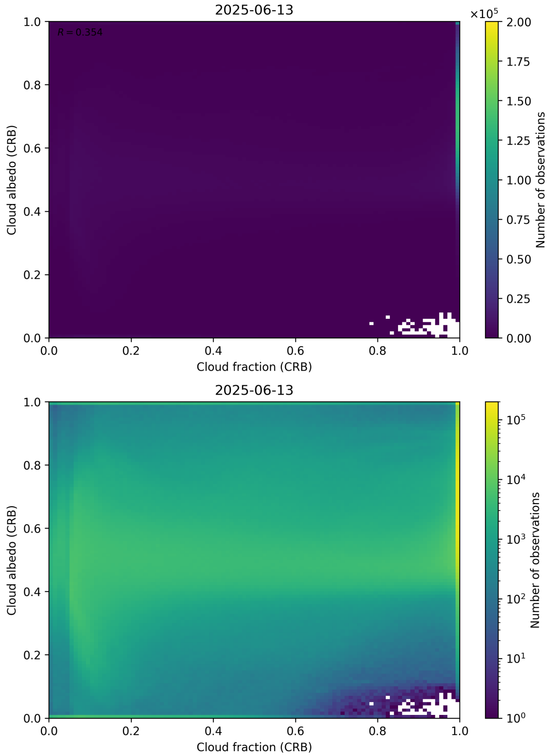
Figure 77: Scatter density plot of “Cloud fraction (CRB)” against “Cloud albedo (CRB)” for 2025-06-12 to 2025-06-14.
