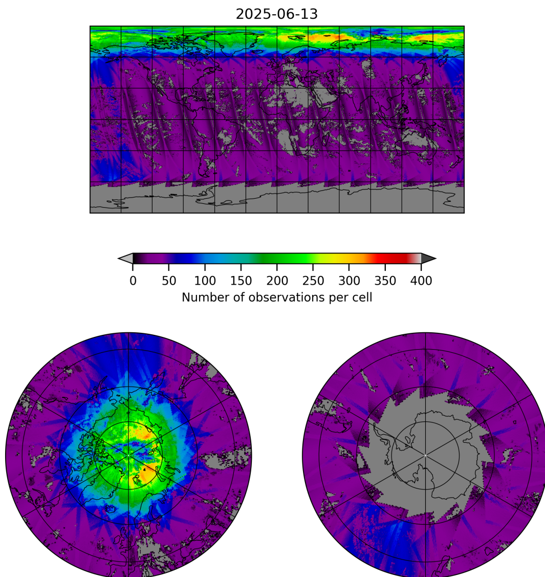
Figure 21: Map of the number of observations for 2025-06-12 to 2025-06-14
