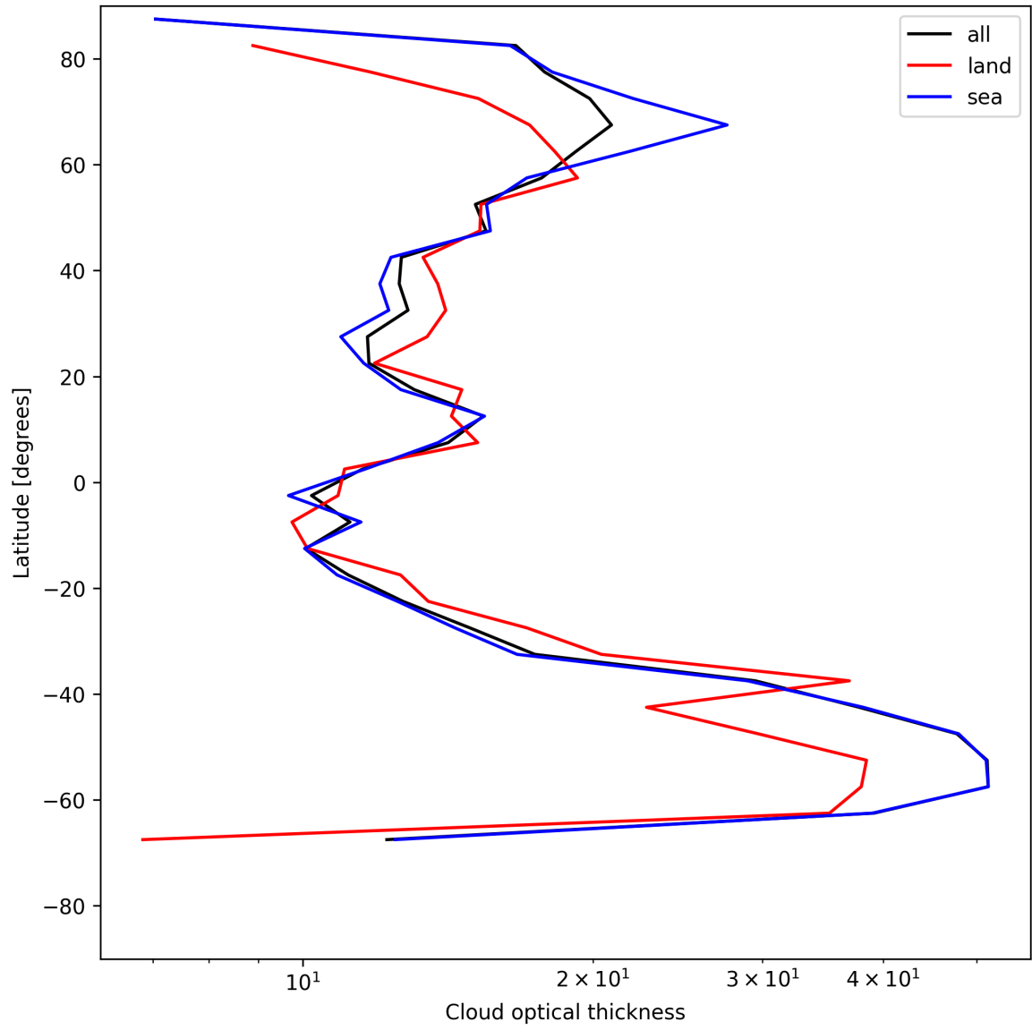
Figure 25: Zonal average of “Cloud optical thickness” for 2025-06-12 to 2025-06-14.
