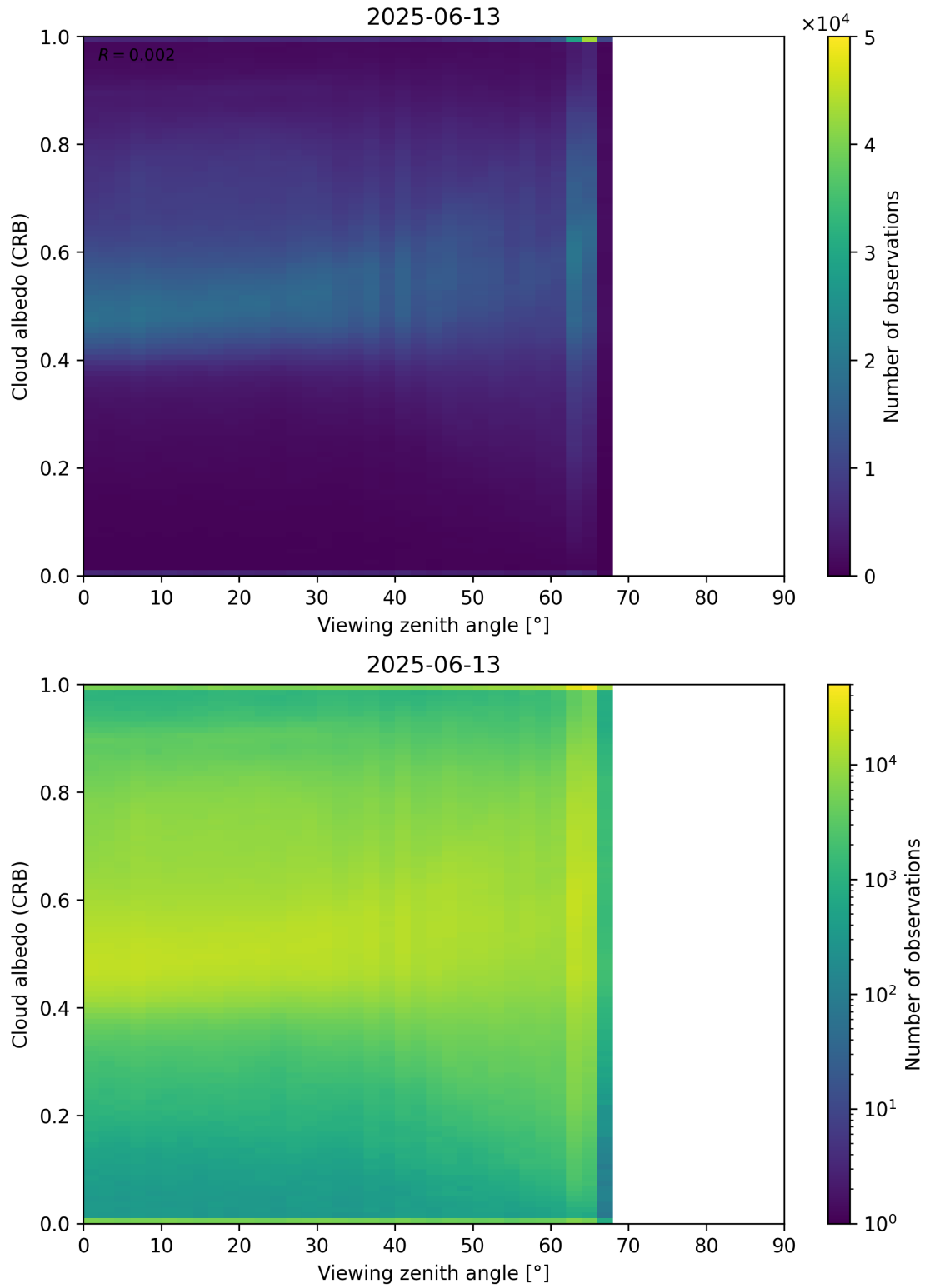
Figure 106: Scatter density plot of “Viewing zenith angle” against “Cloud albedo (CRB)” for 2025-06-12 to 2025-06-14.
