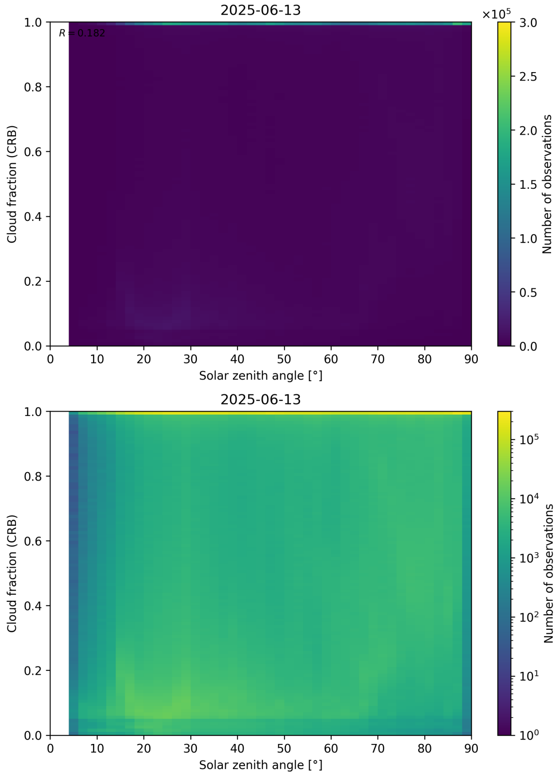
Figure 101: Scatter density plot of “Solar zenith angle” against “Cloud fraction (CRB)” for 2025-06-12 to 2025-06-14.
