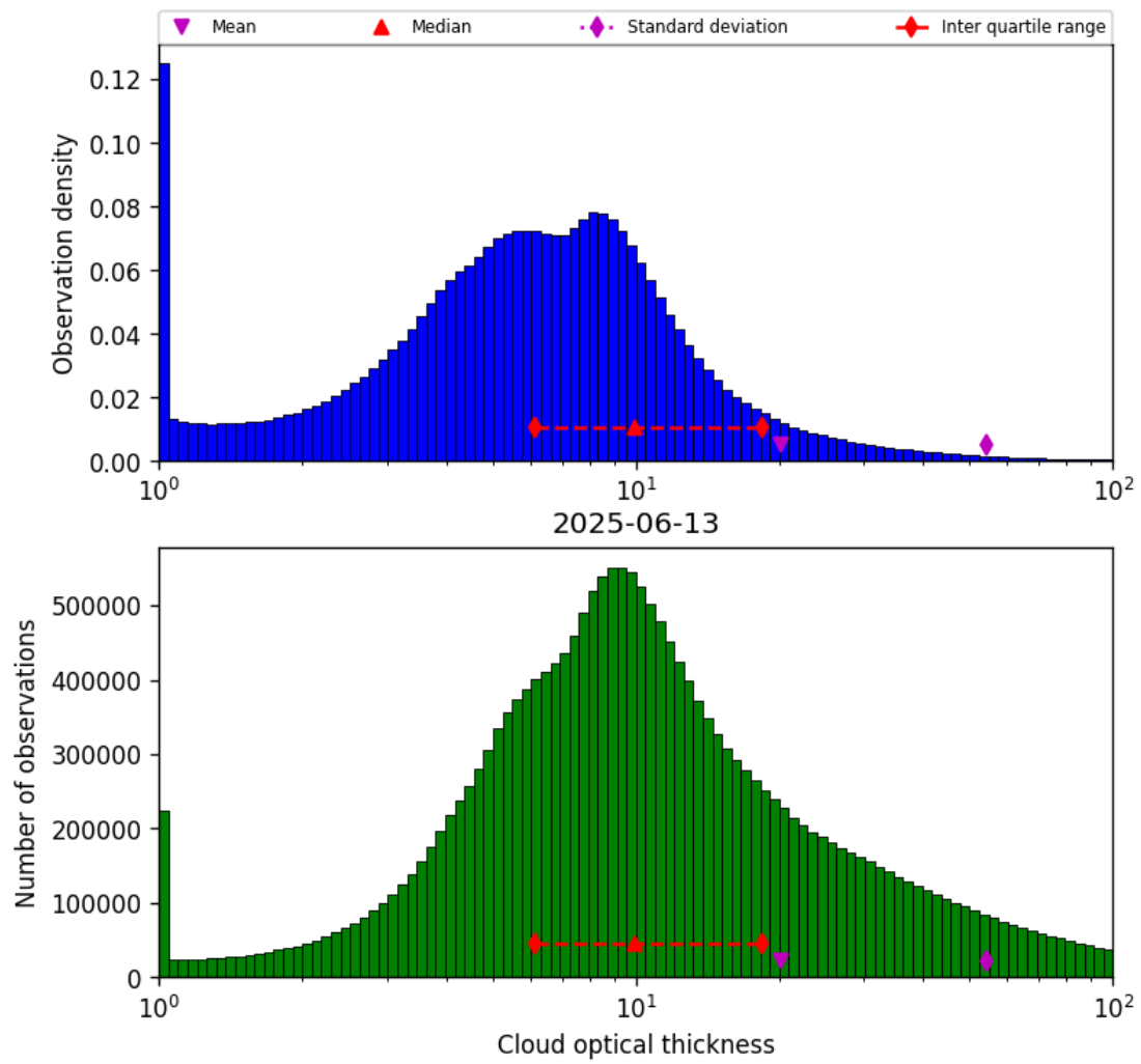
Figure 41: Histogram of “Cloud optical thickness” for 2025-06-12 to 2025-06-14
