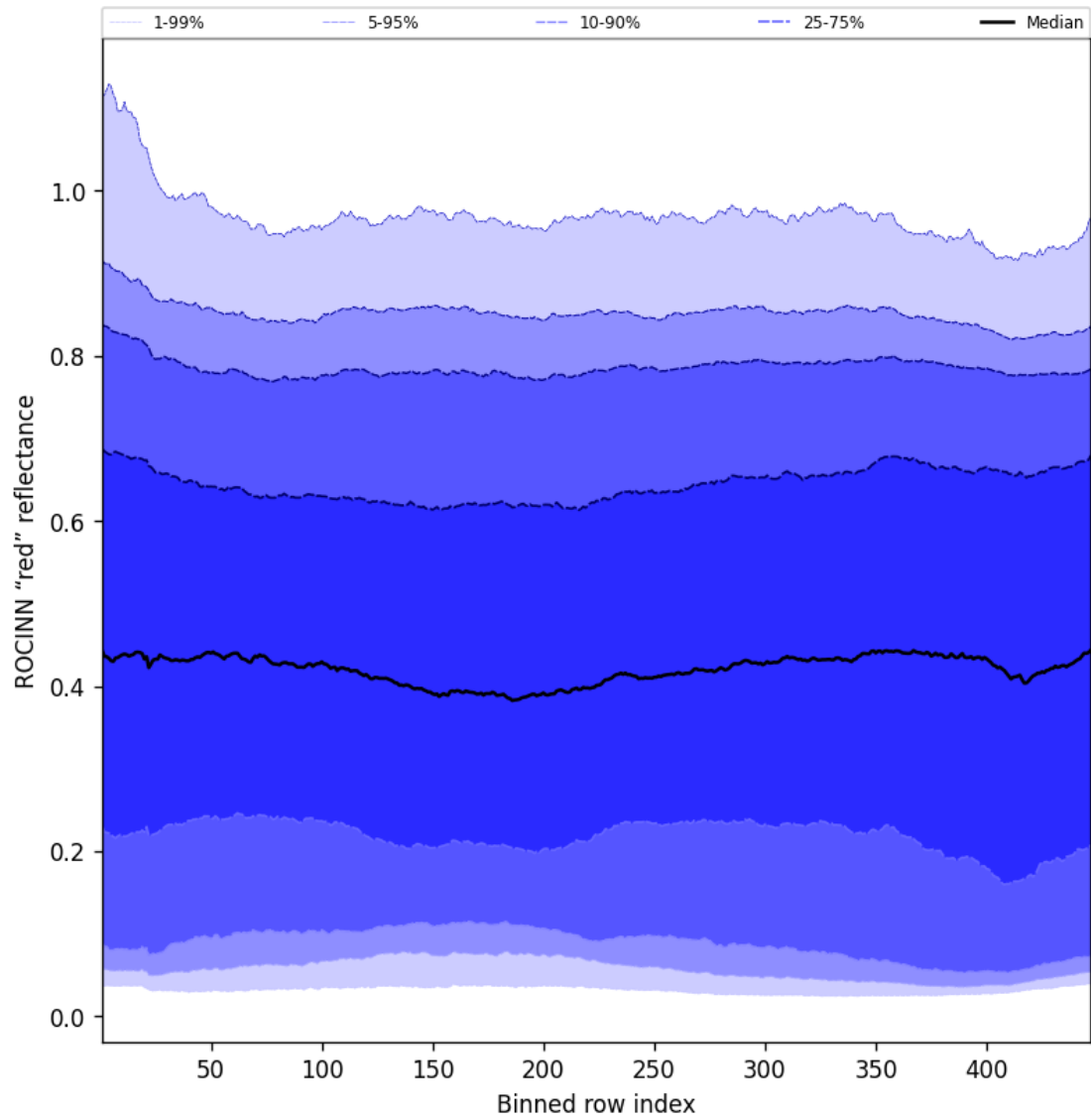
Figure 69: Along track statistics of "ROCINN "red" reflectance" for 2025-06-12 to 2025-06-14
