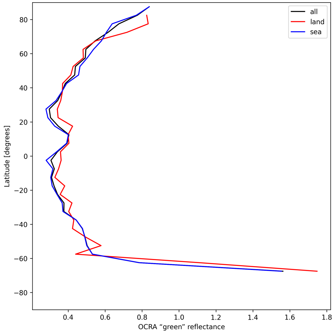
Figure 36: Zonal average of “OCRA “green” reflectance” for 2025-06-12 to 2025-06-14.
