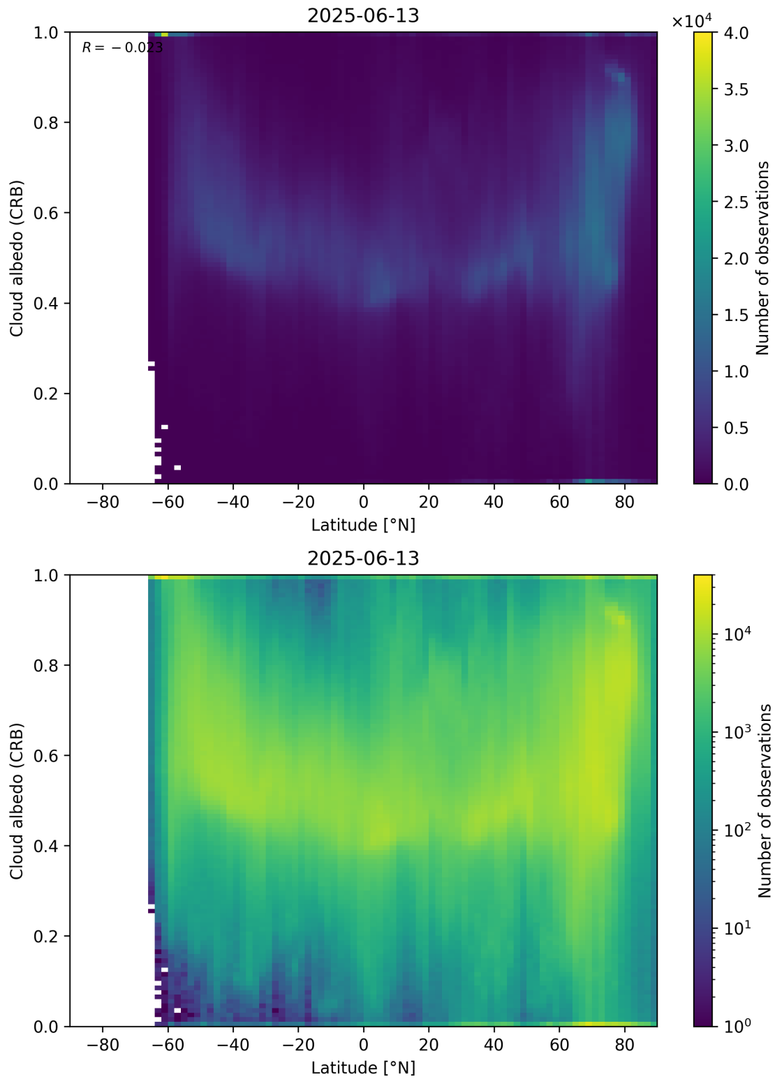
Figure 91: Scatter density plot of “Latitude” against “Cloud albedo (CRB)” for 2025-06-12 to 2025-06-14.
