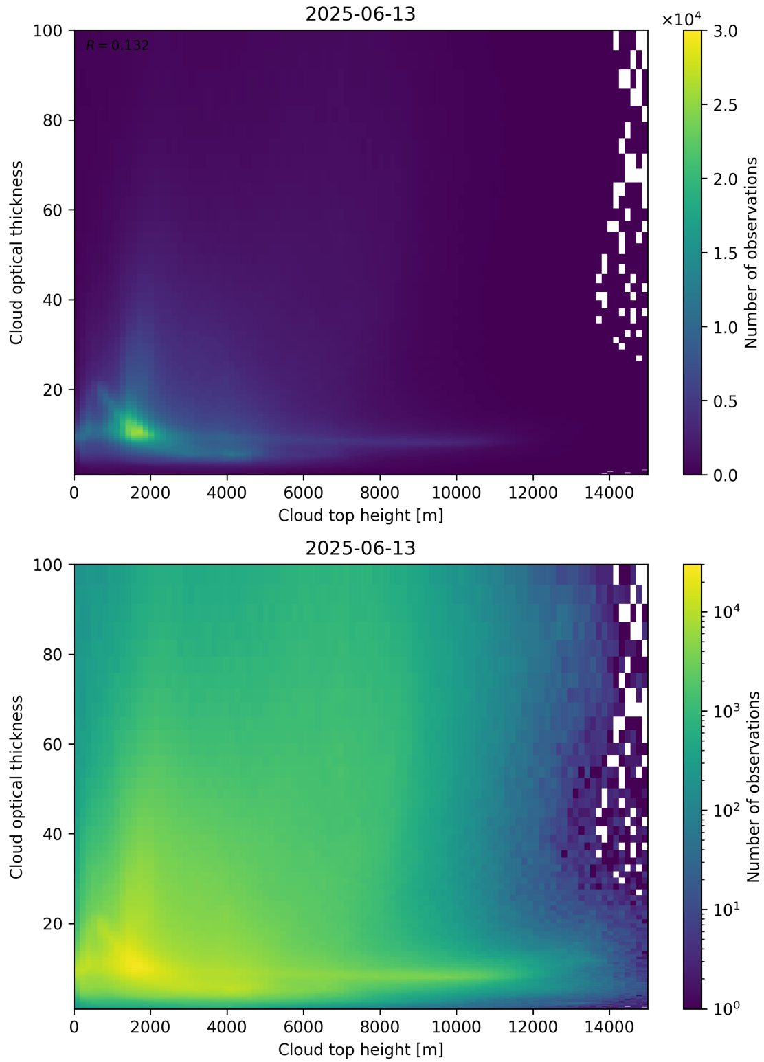
Figure 90: Scatter density plot of “Cloud top height” against “Cloud optical thickness” for 2025-06-12 to 2025-06-14.
