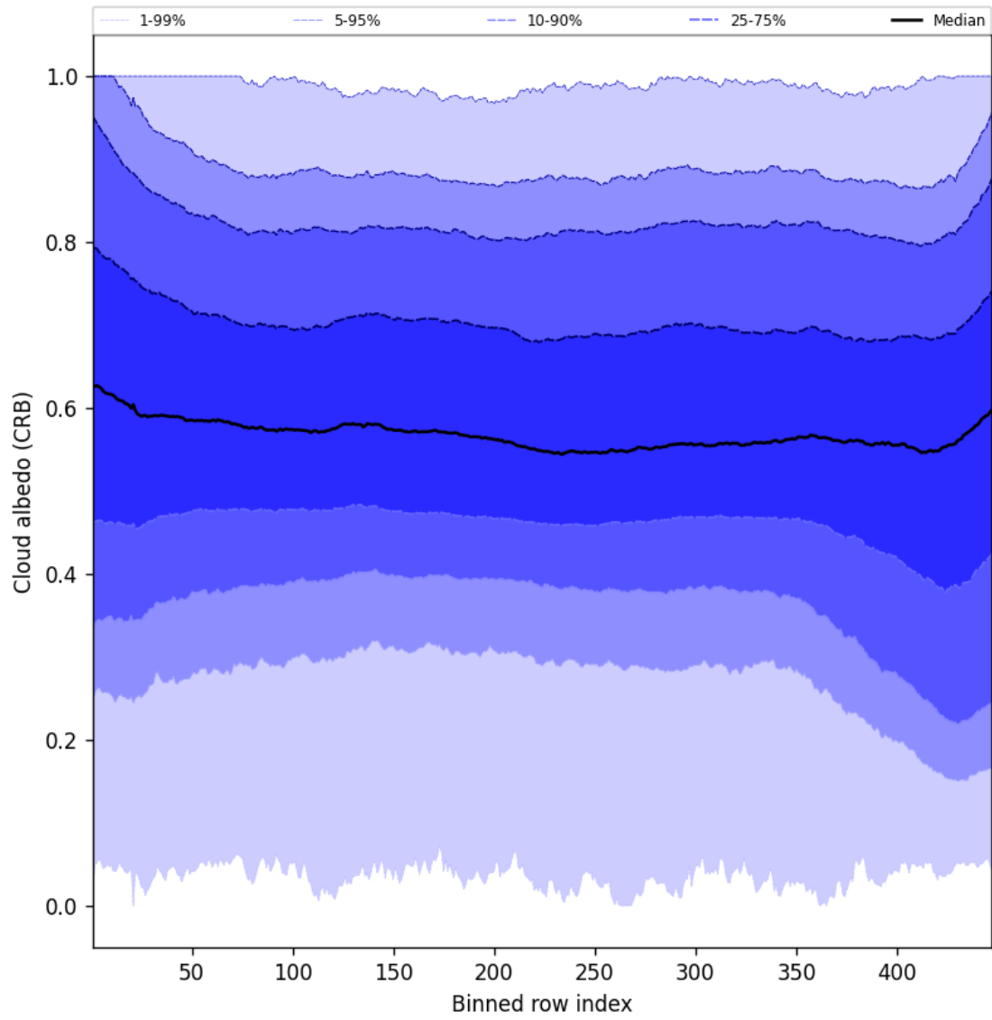
Figure 60: Along track statistics of “Cloud albedo (CRB)” for 2025-06-12 to 2025-06-14
