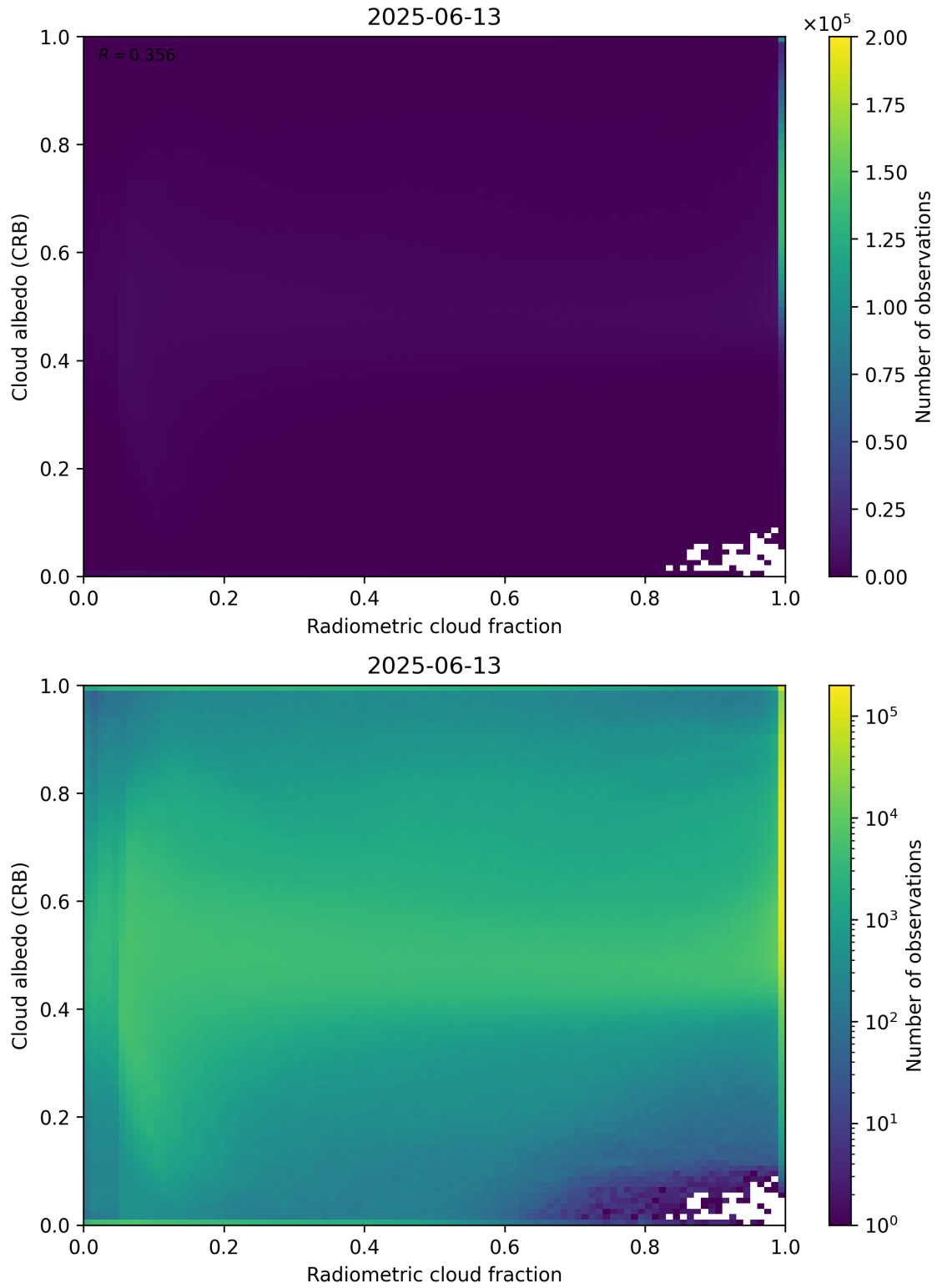
Figure 71: Scatter density plot of “Radiometric cloud fraction” against “Cloud albedo (CRB)” for 2025-06-12 to 2025-06-14.
