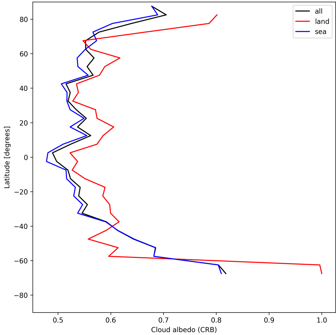
Figure 28: Zonal average of “Cloud albedo (CRB)” for 2025-06-12 to 2025-06-14.
