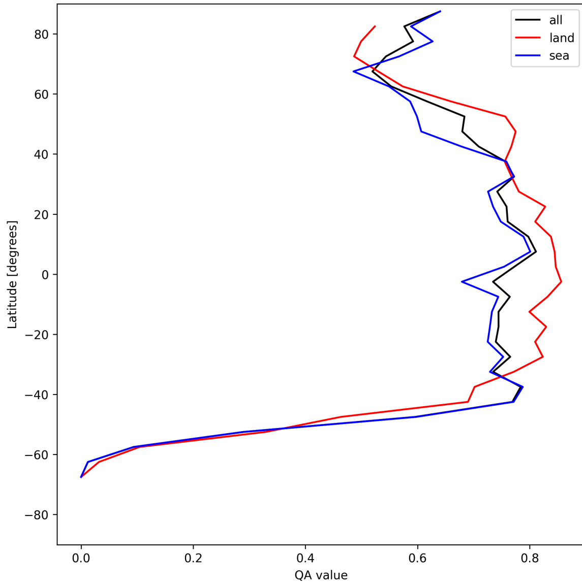
Figure 22: Zonal average of “QA value” for 2025-06-12 to 2025-06-14.
