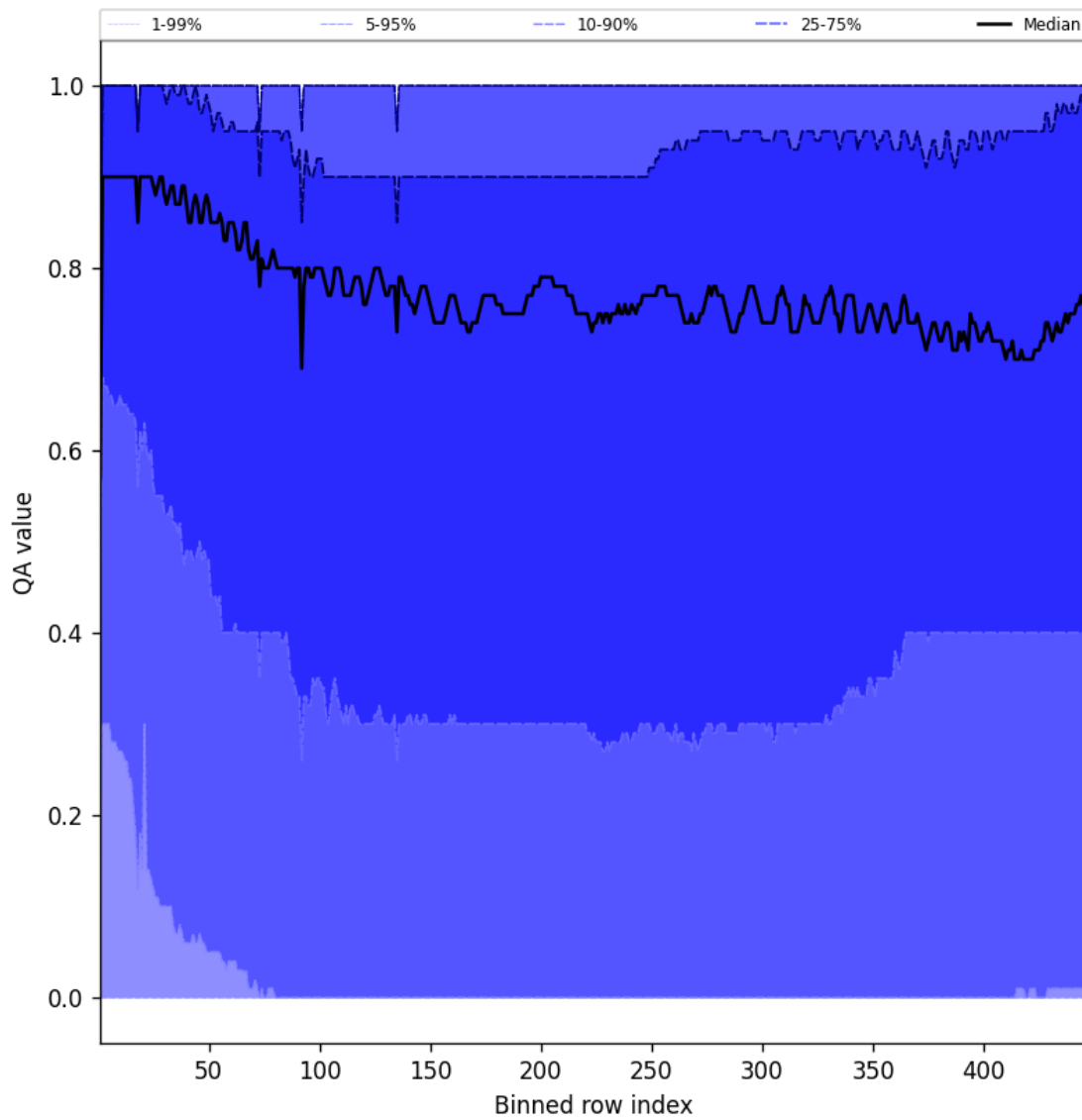
Figure 54: Along track statistics of “QA value” for 2025-06-12 to 2025-06-14
