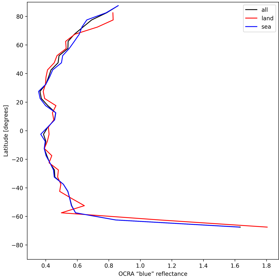
Figure 35: Zonal average of “OCRA “blue” reflectance” for 2025-06-12 to 2025-06-14.
