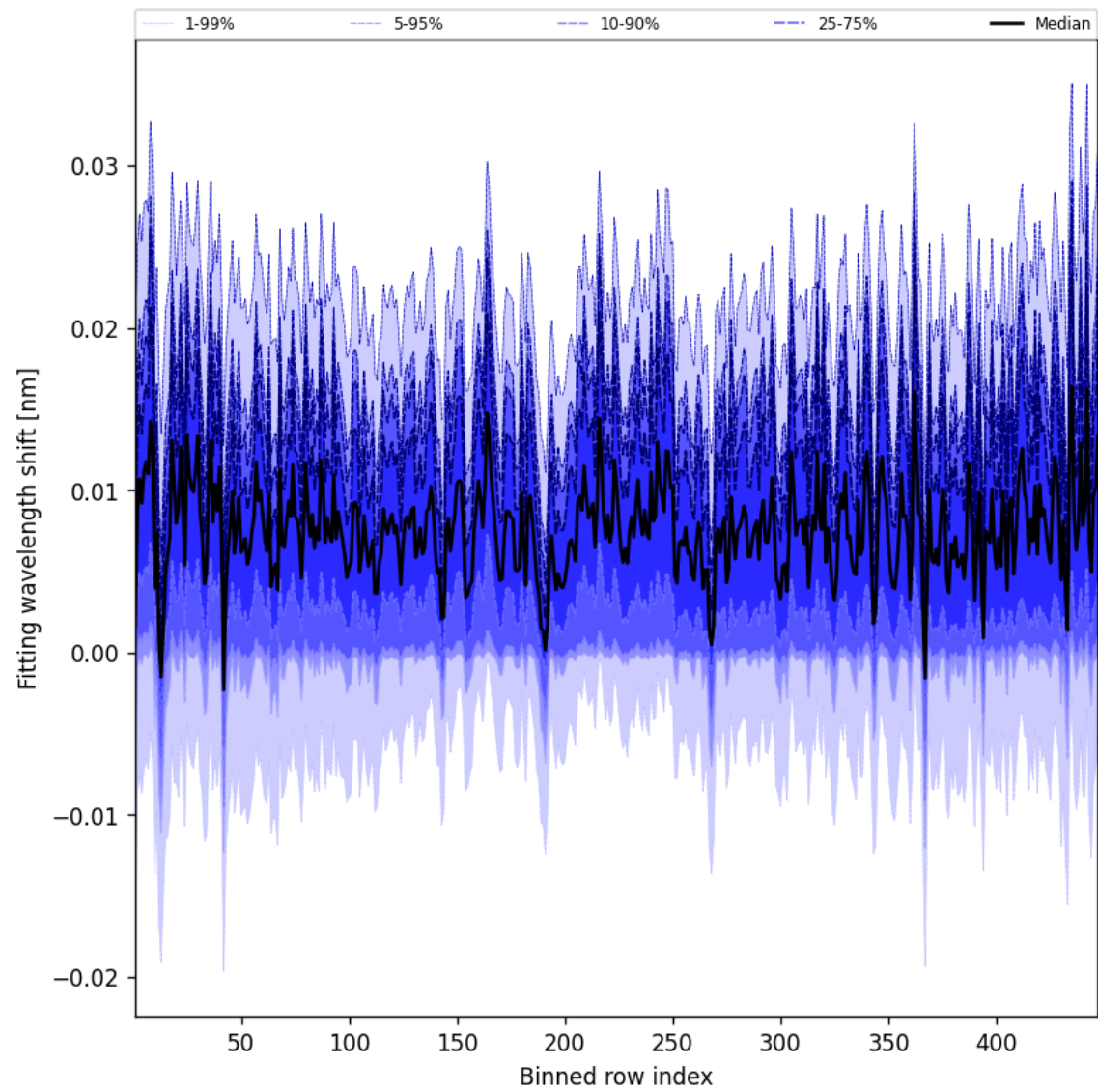
Figure 65: Along track statistics of “Fitting wavelength shift” for 2025-06-12 to 2025-06-14
