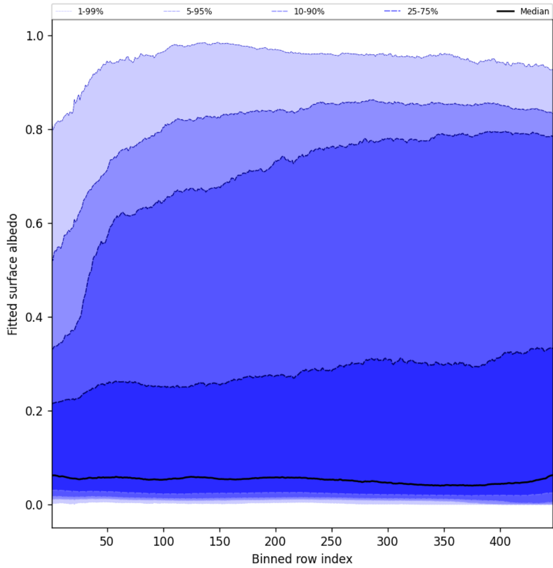
Figure 61: Along track statistics of “Fitted surface albedo” for 2025-06-12 to 2025-06-14
