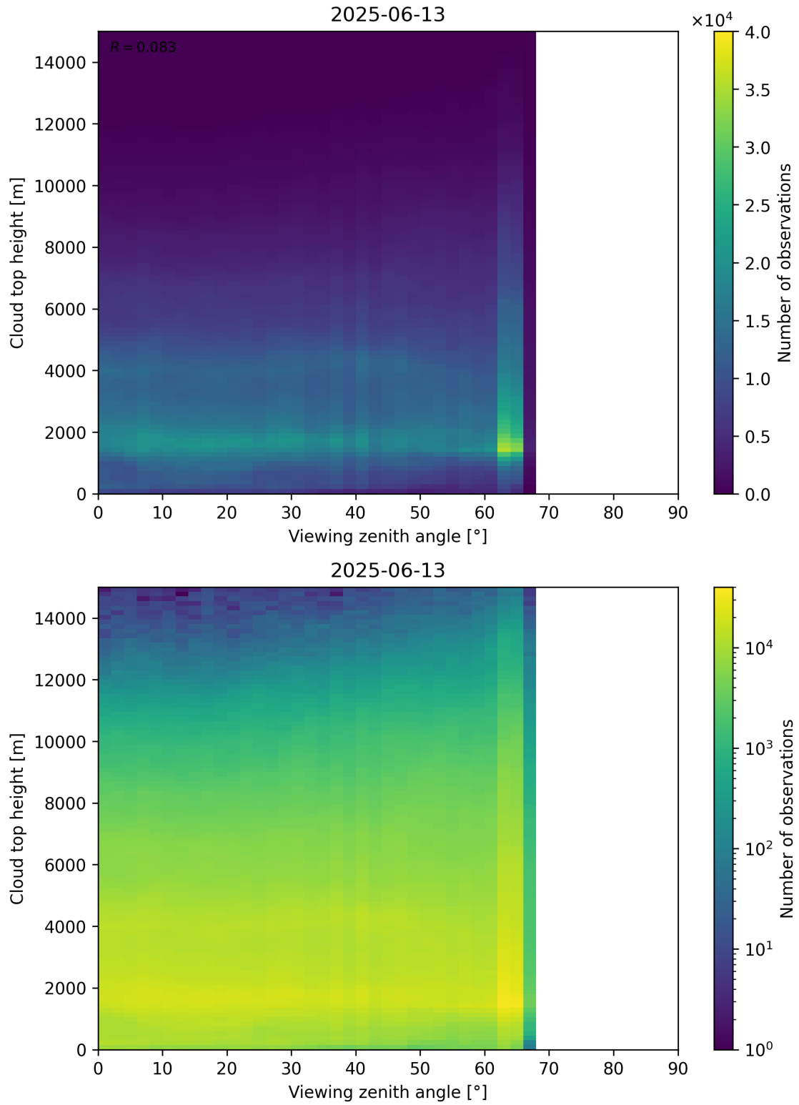
Figure 112: Scatter density plot of “Viewing zenith angle” against “Cloud top height” for 2025-06-12 to 2025-06-14.
