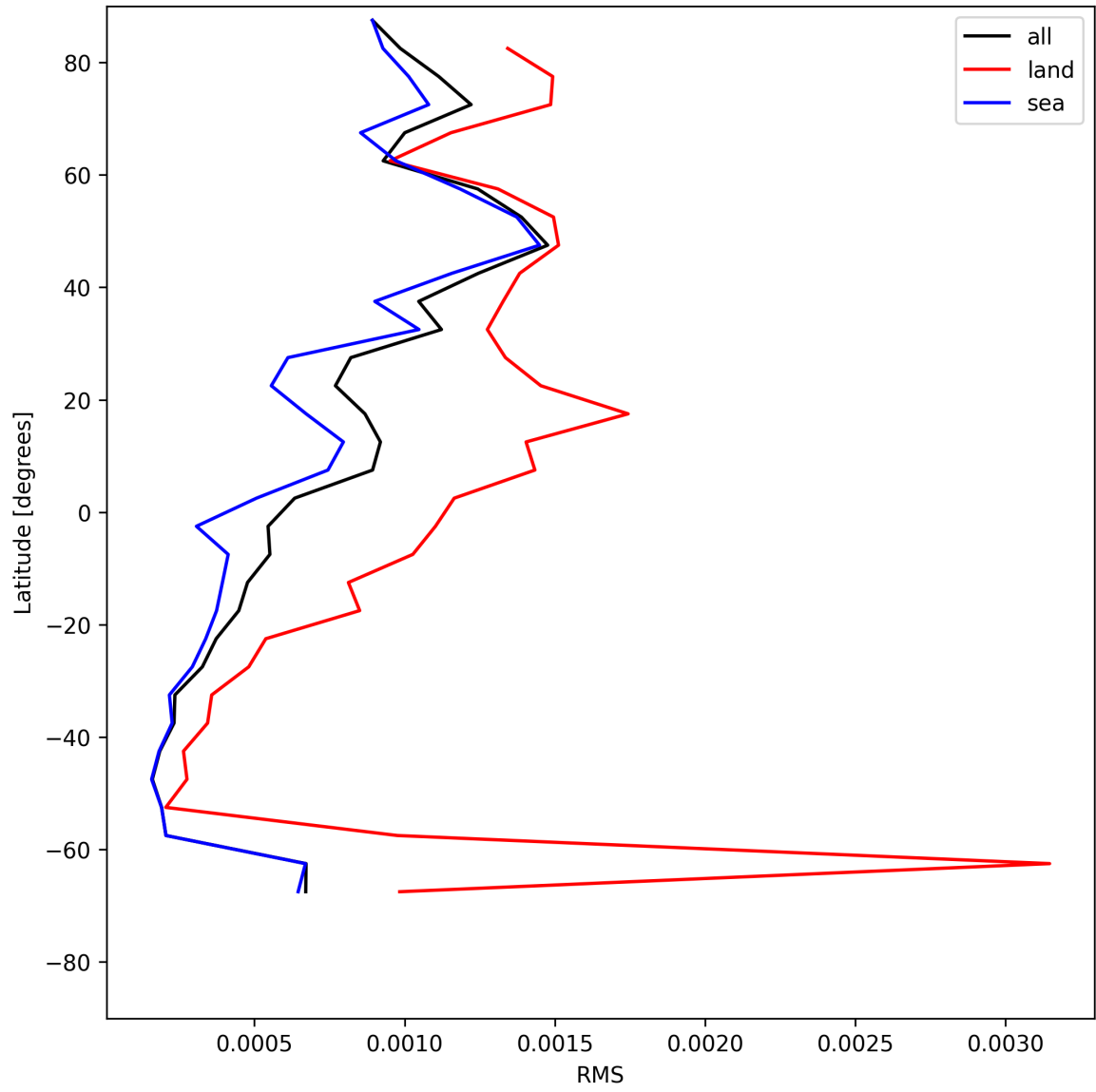
Figure 31: Zonal average of “RMS” for 2025-06-12 to 2025-06-14.
