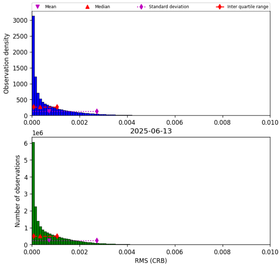
Figure 48: Histogram of “RMS (CRB)” for 2025-06-12 to 2025-06-14
