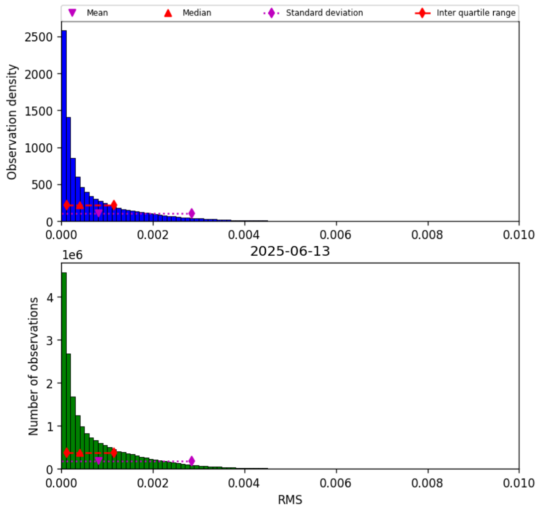
Figure 47: Histogram of “RMS” for 2025-06-12 to 2025-06-14
