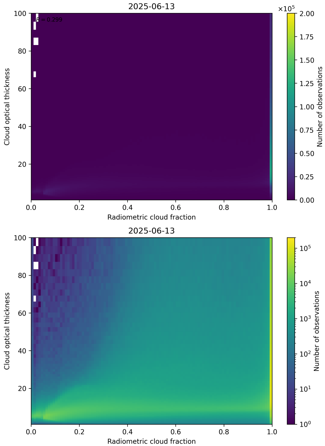
Figure 75: Scatter density plot of “Radiometric cloud fraction” against “Cloud optical thickness” for 2025-06-12 to 2025-06-14.
