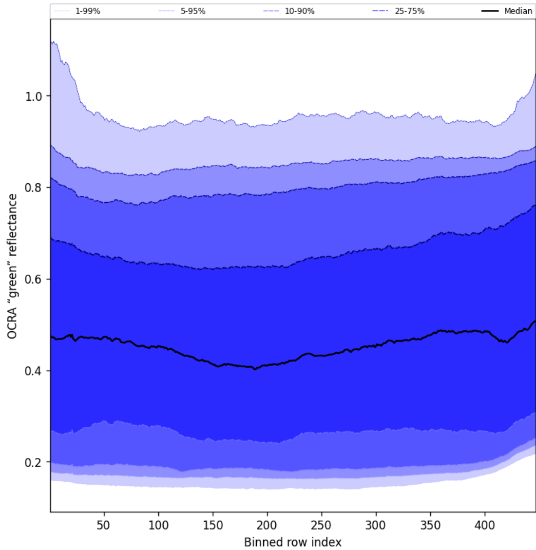
Figure 68: Along track statistics of "OCRA "green" reflectance" for 2025-06-12 to 2025-06-14
