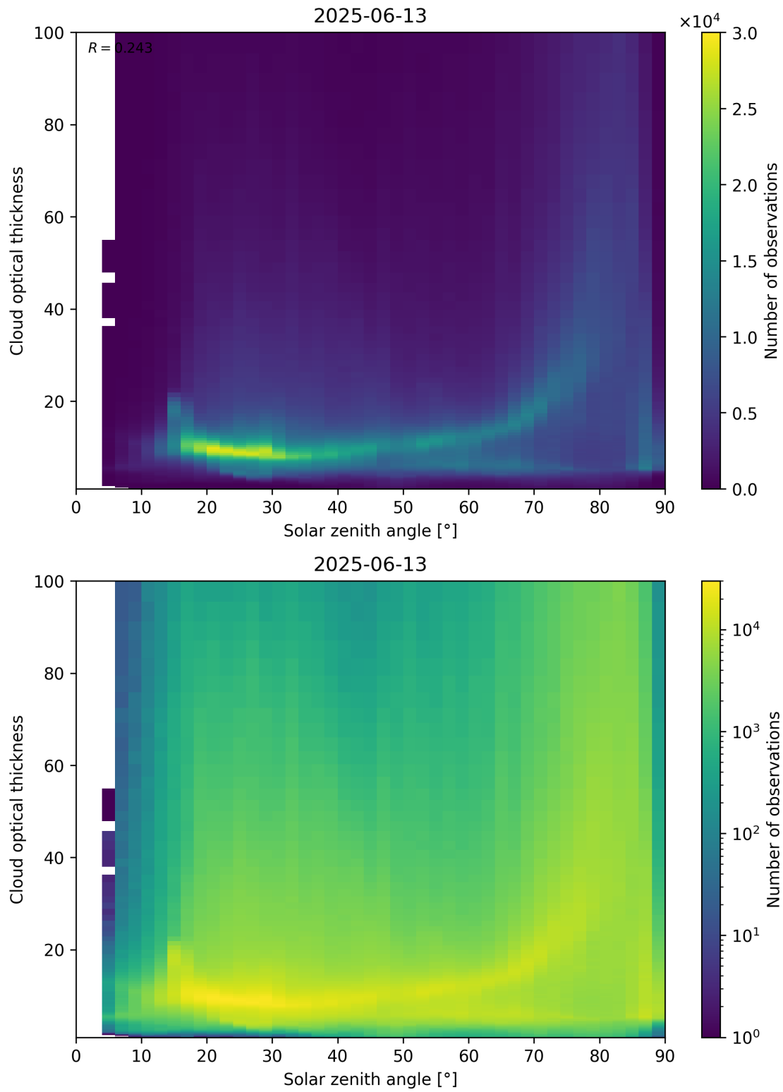
Figure 103: Scatter density plot of “Solar zenith angle” against “Cloud optical thickness” for 2025-06-12 to 2025-06-14.
