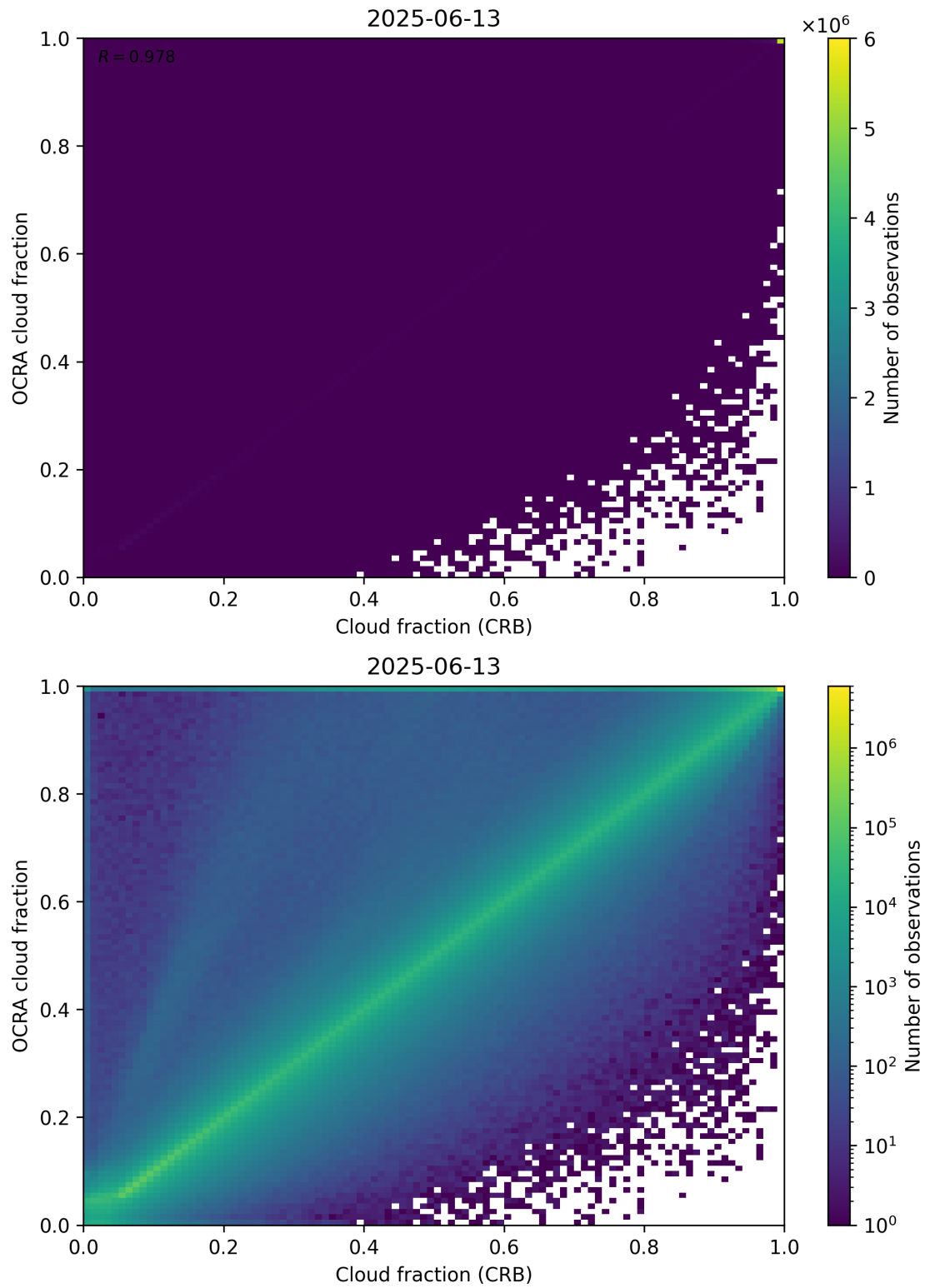
Figure 78: Scatter density plot of “Cloud fraction (CRB)” against “OCRA cloud fraction” for 2025-06-12 to 2025-06-14.
