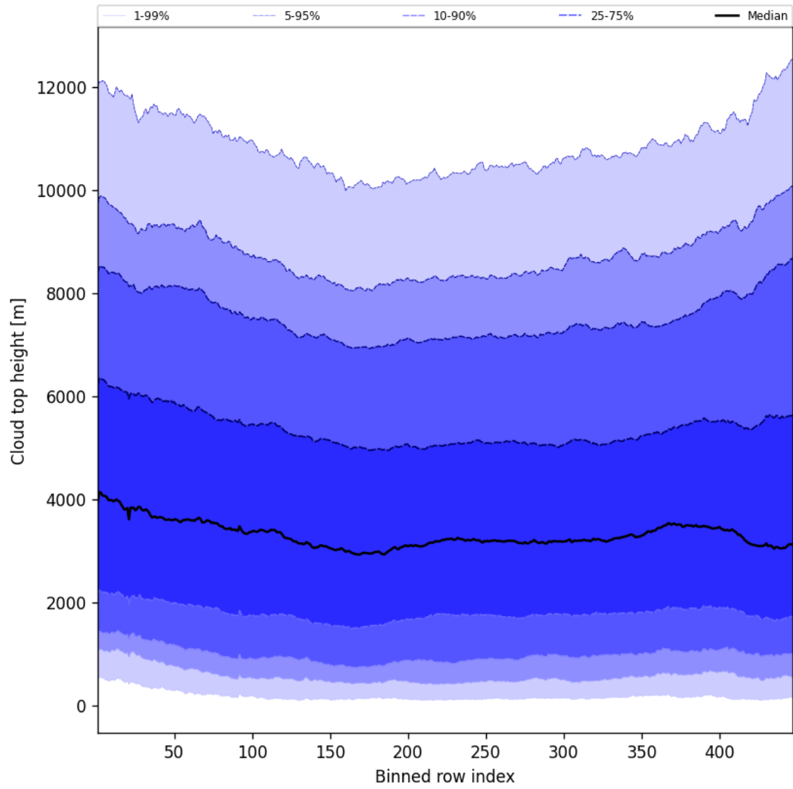
Figure 56: Along track statistics of “Cloud top height” for 2025-06-12 to 2025-06-14
