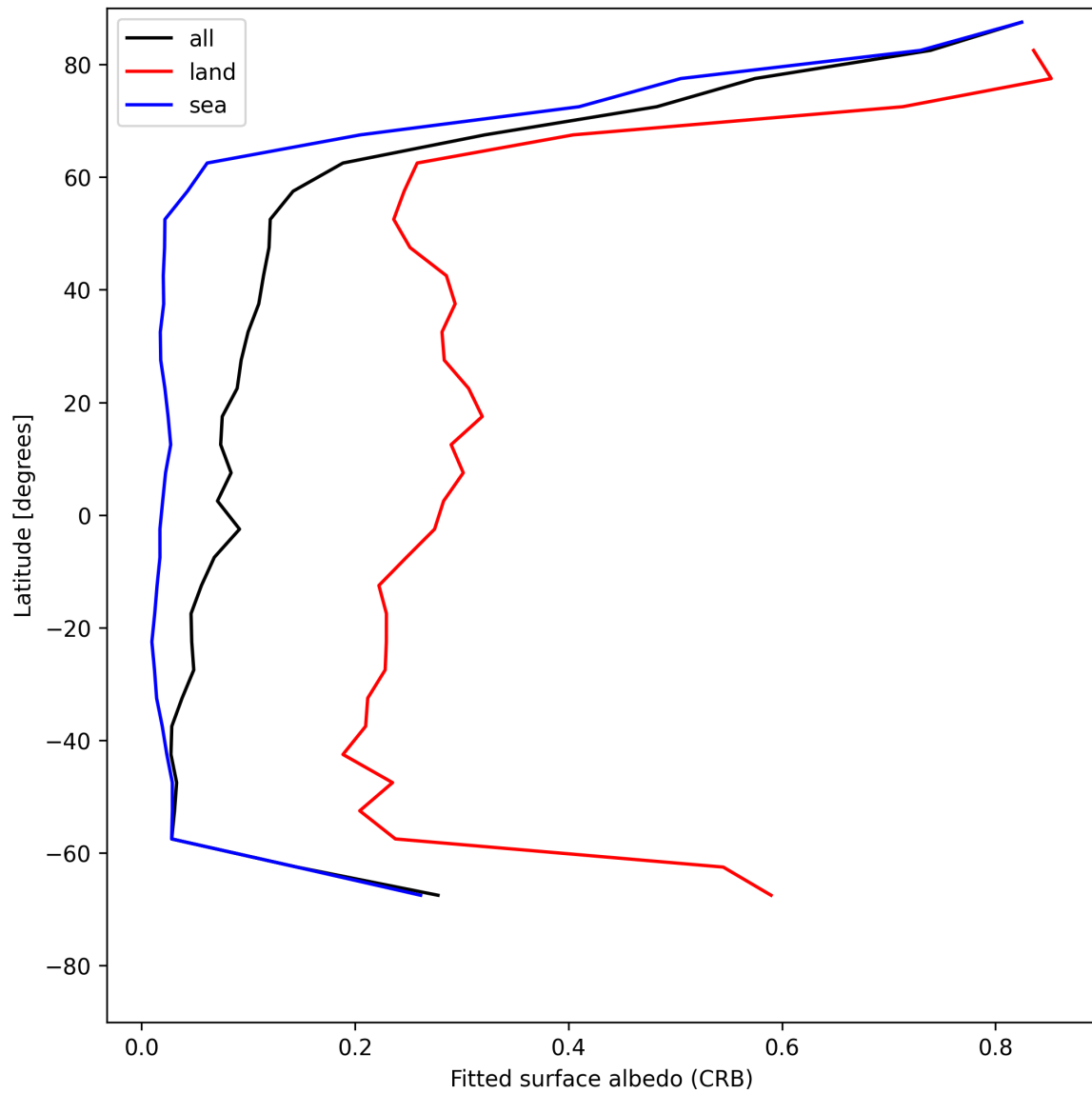
Figure 30: Zonal average of “Fitted surface albedo (CRB)” for 2025-06-12 to 2025-06-14.
