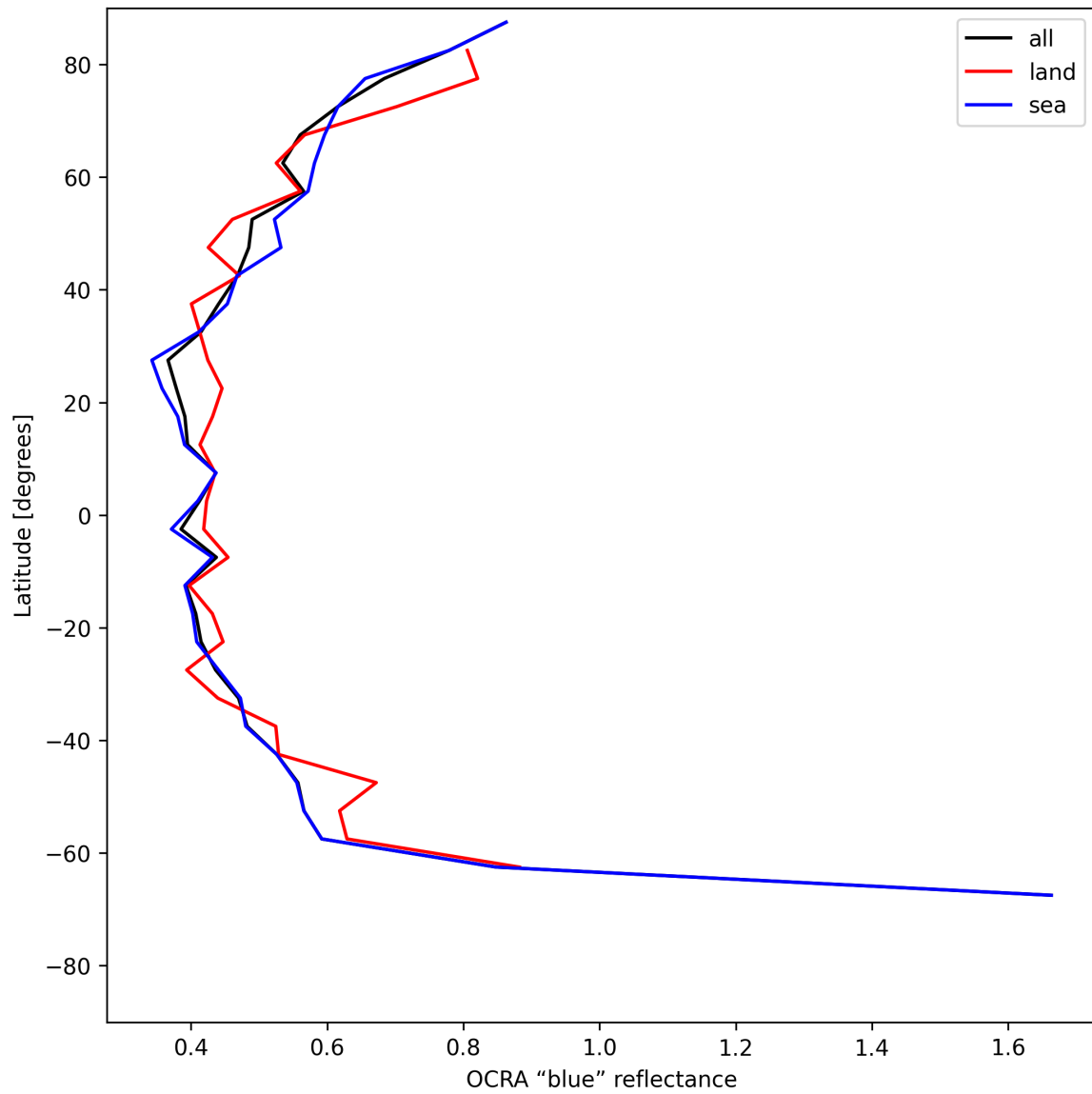
Figure 35: Zonal average of “OCRA “blue” reflectance” for 2025-06-14 to 2025-06-16.
