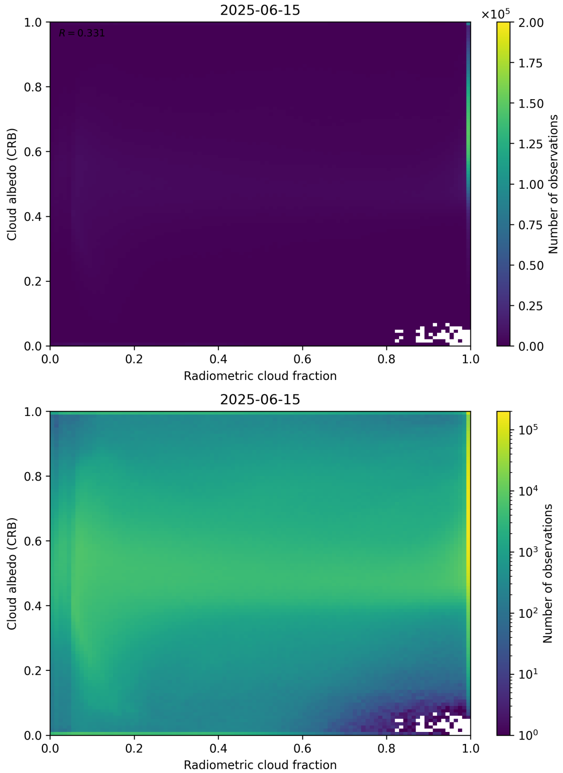
Figure 71: Scatter density plot of “Radiometric cloud fraction” against “Cloud albedo (CRB)” for 2025-06-14 to 2025-06-16.
