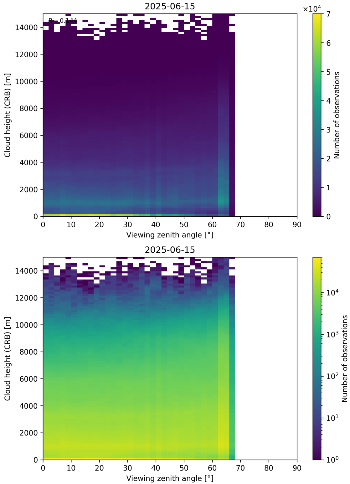
Figure 110: Scatter density plot of “Viewing zenith angle” against “Cloud height (CRB)” for 2025-06-14 to 2025-06-16.
