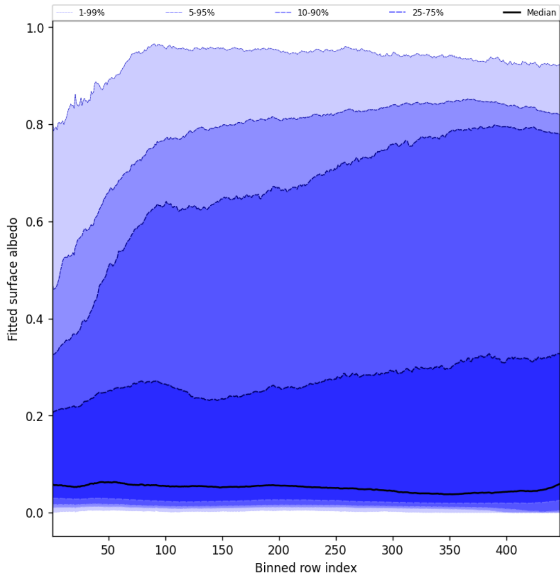
Figure 61: Along track statistics of “Fitted surface albedo” for 2025-06-14 to 2025-06-16
