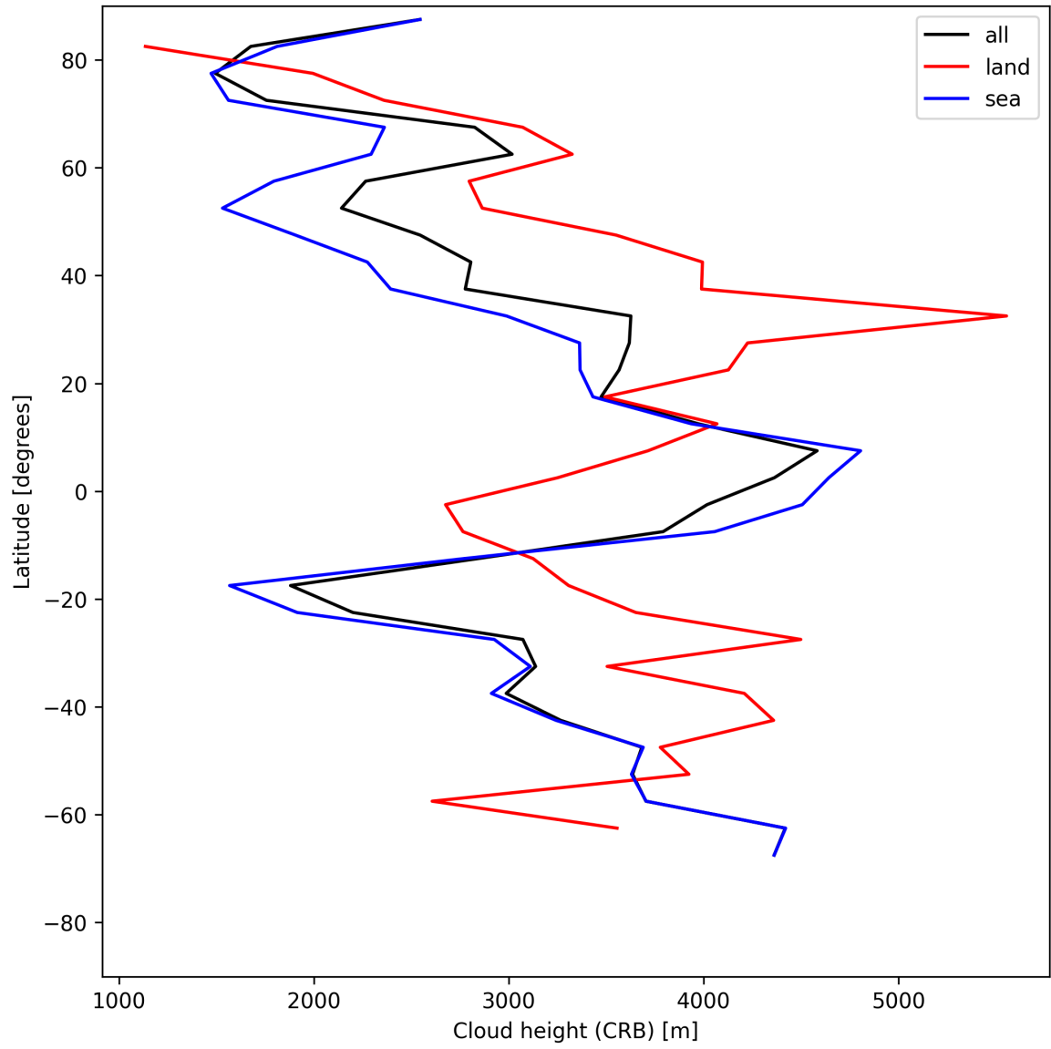
Figure 27: Zonal average of “Cloud height (CRB)” for 2025-06-14 to 2025-06-16.
