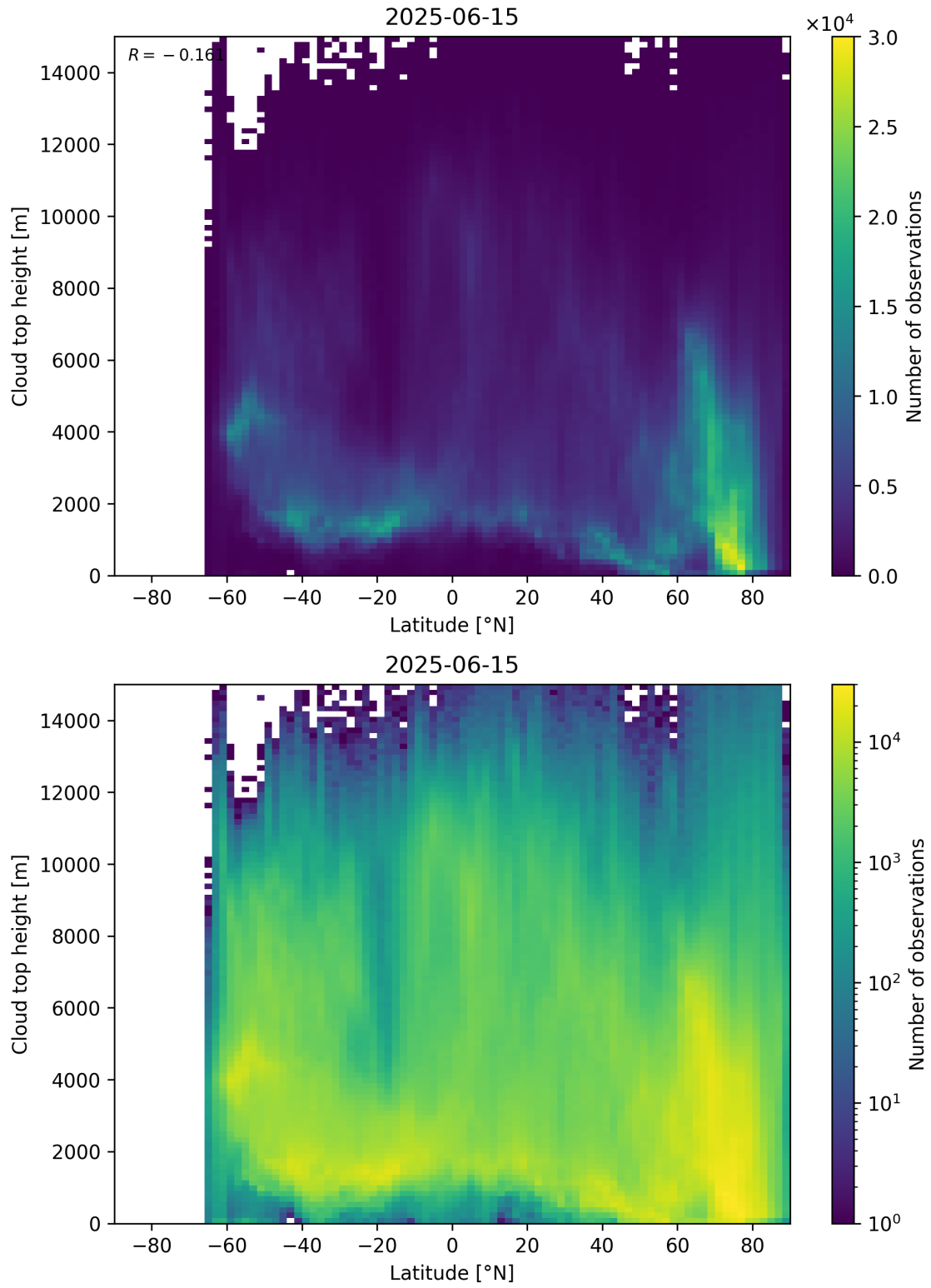
Figure 97: Scatter density plot of “Latitude” against “Cloud top height” for 2025-06-14 to 2025-06-16.
