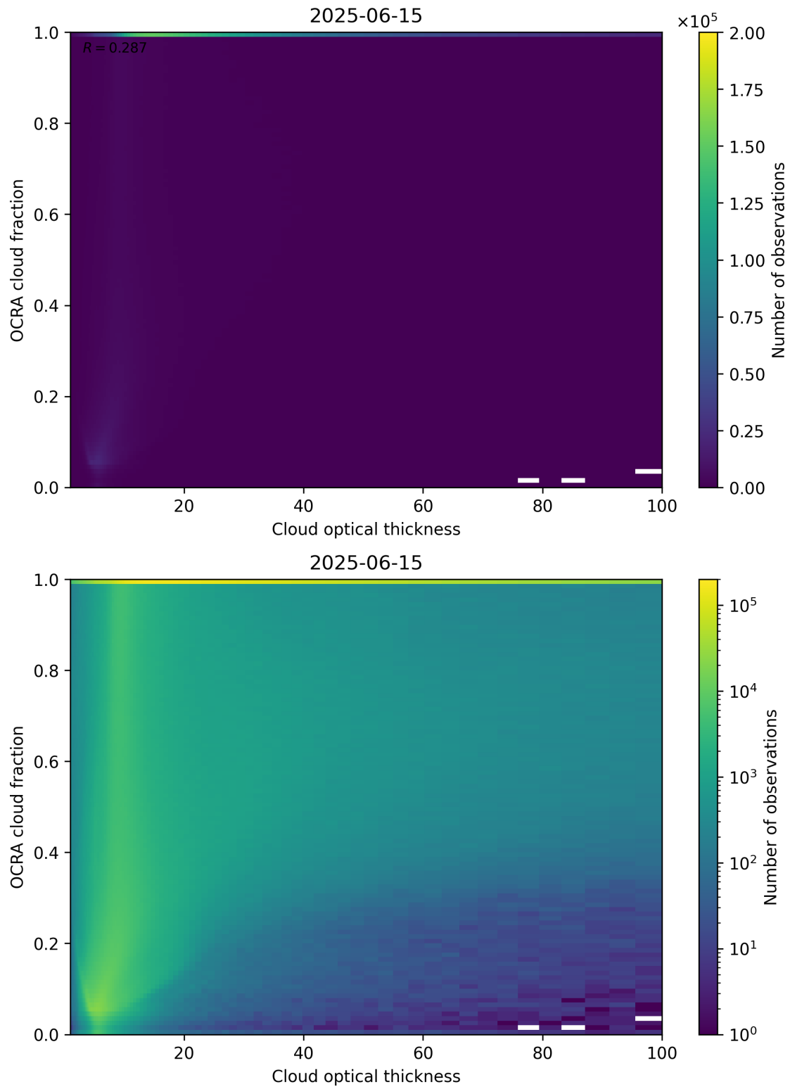
Figure 83: Scatter density plot of “Cloud optical thickness” against “OCRA cloud fraction” for 2025-06-14 to 2025-06-16.
