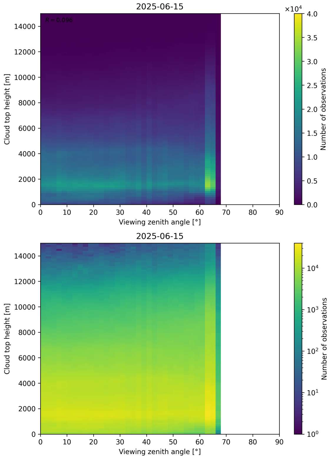
Figure 112: Scatter density plot of “Viewing zenith angle” against “Cloud top height” for 2025-06-14 to 2025-06-16.
