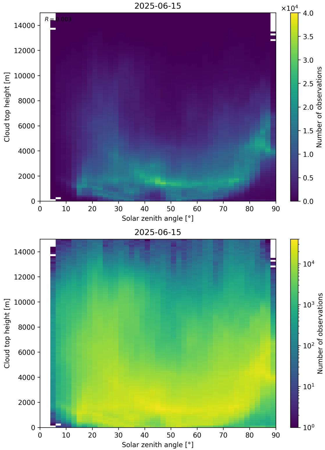
Figure 104: Scatter density plot of “Solar zenith angle” against “Cloud top height” for 2025-06-14 to 2025-06-16.
