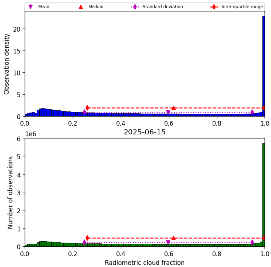
Figure 39: Histogram of “Radiometric cloud fraction” for 2025-06-14 to 2025-06-16
