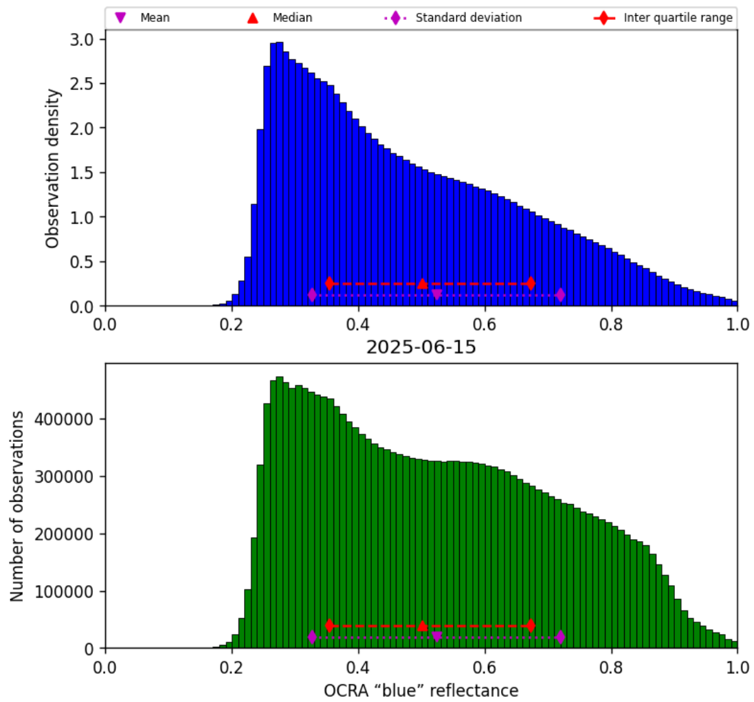
Figure 51: Histogram of “OCRA “blue” reflectance” for 2025-06-14 to 2025-06-16
