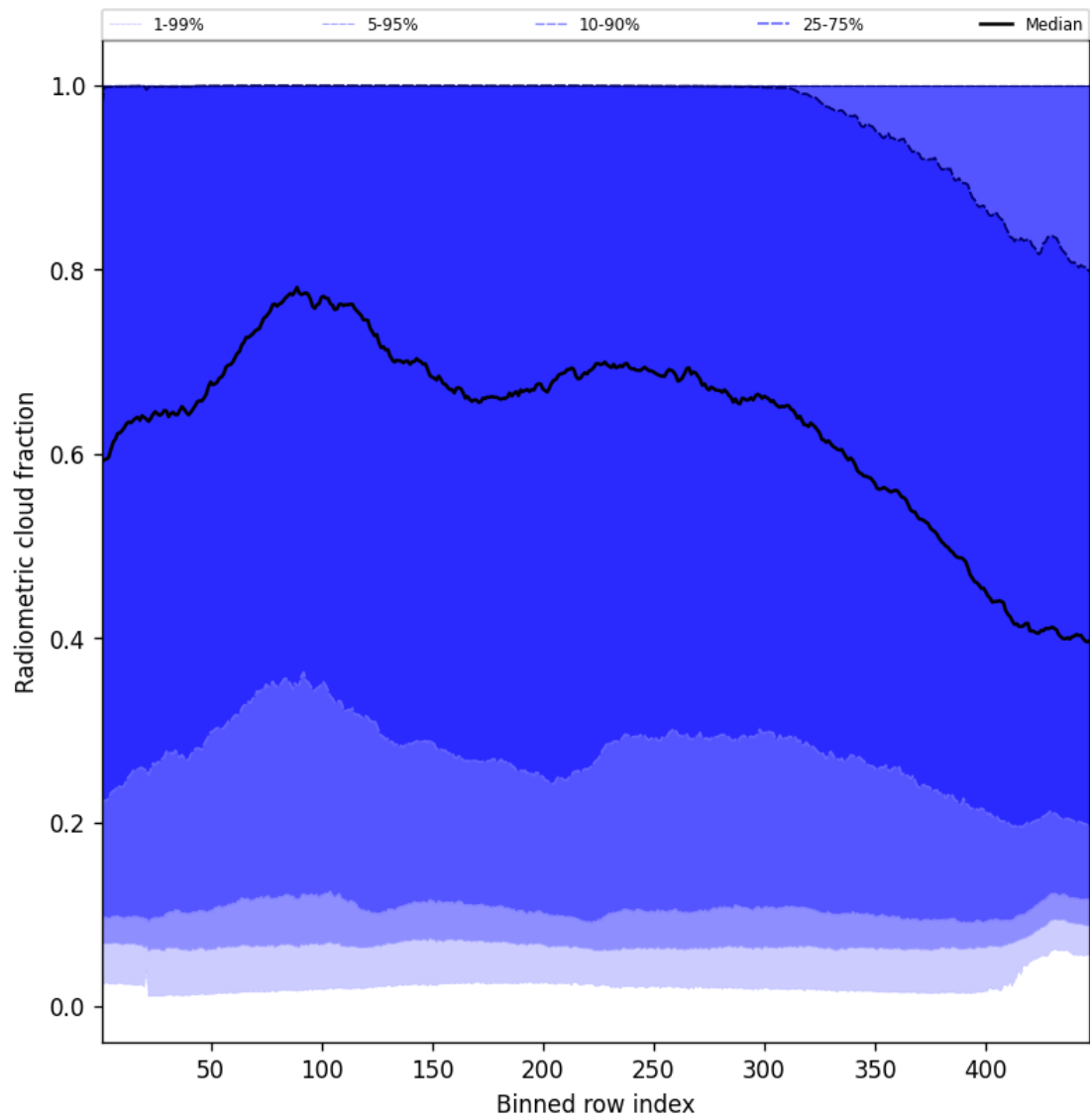
Figure 55: Along track statistics of “Radiometric cloud fraction” for 2025-06-14 to 2025-06-16
