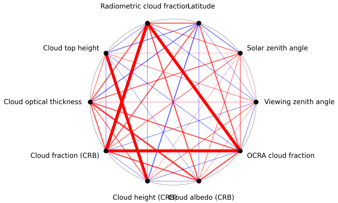
Figure 1: Map of correlation graph for 2025-06-14 to 2025-06-16.
