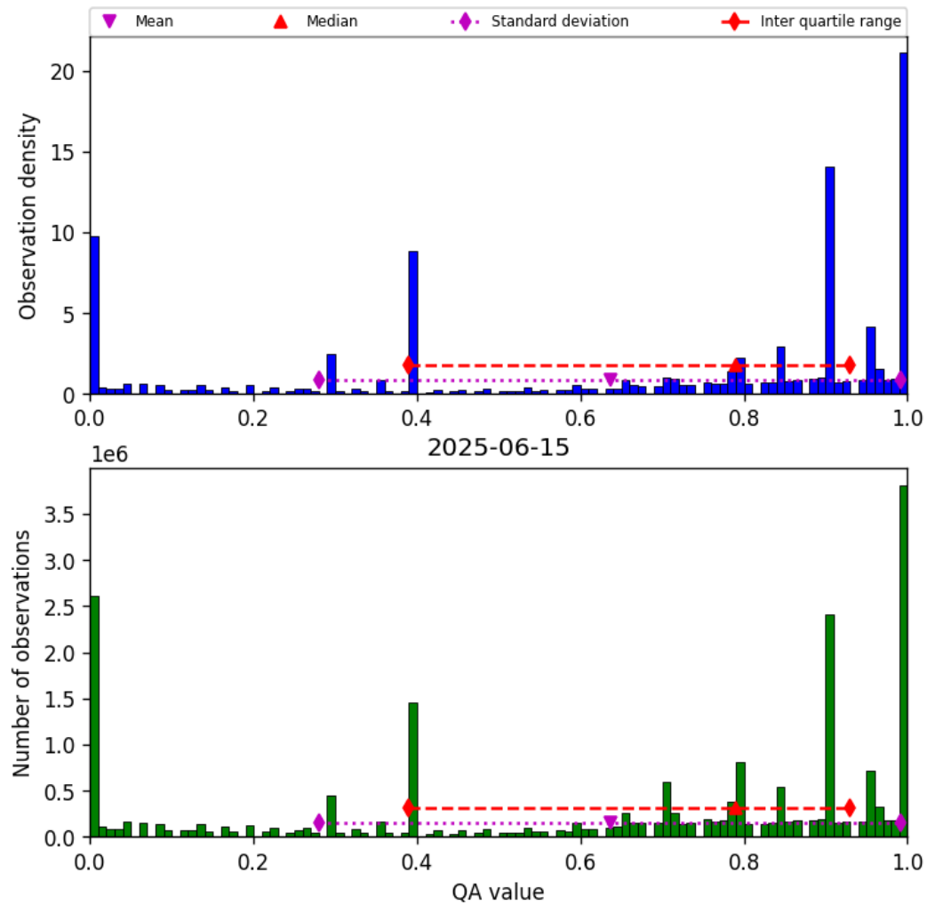
Figure 38: Histogram of “QA value” for 2025-06-14 to 2025-06-16
