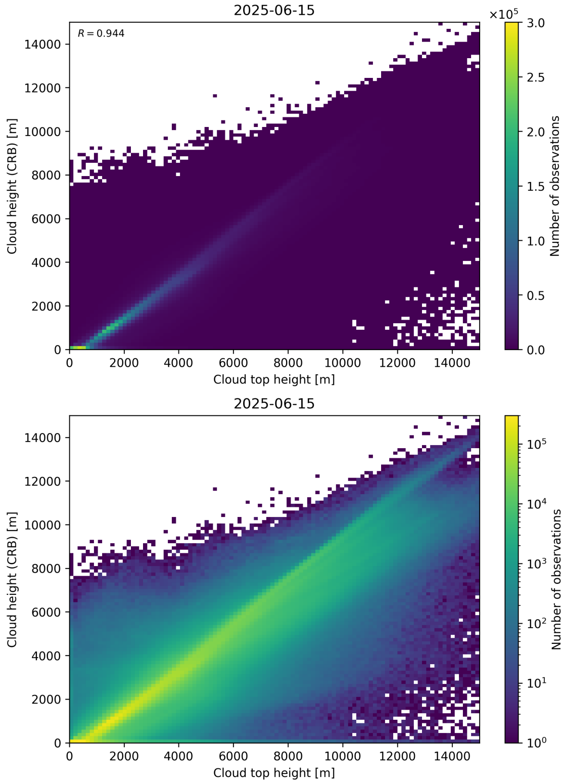
Figure 89: Scatter density plot of “Cloud top height” against “Cloud height (CRB)” for 2025-06-14 to 2025-06-16.
