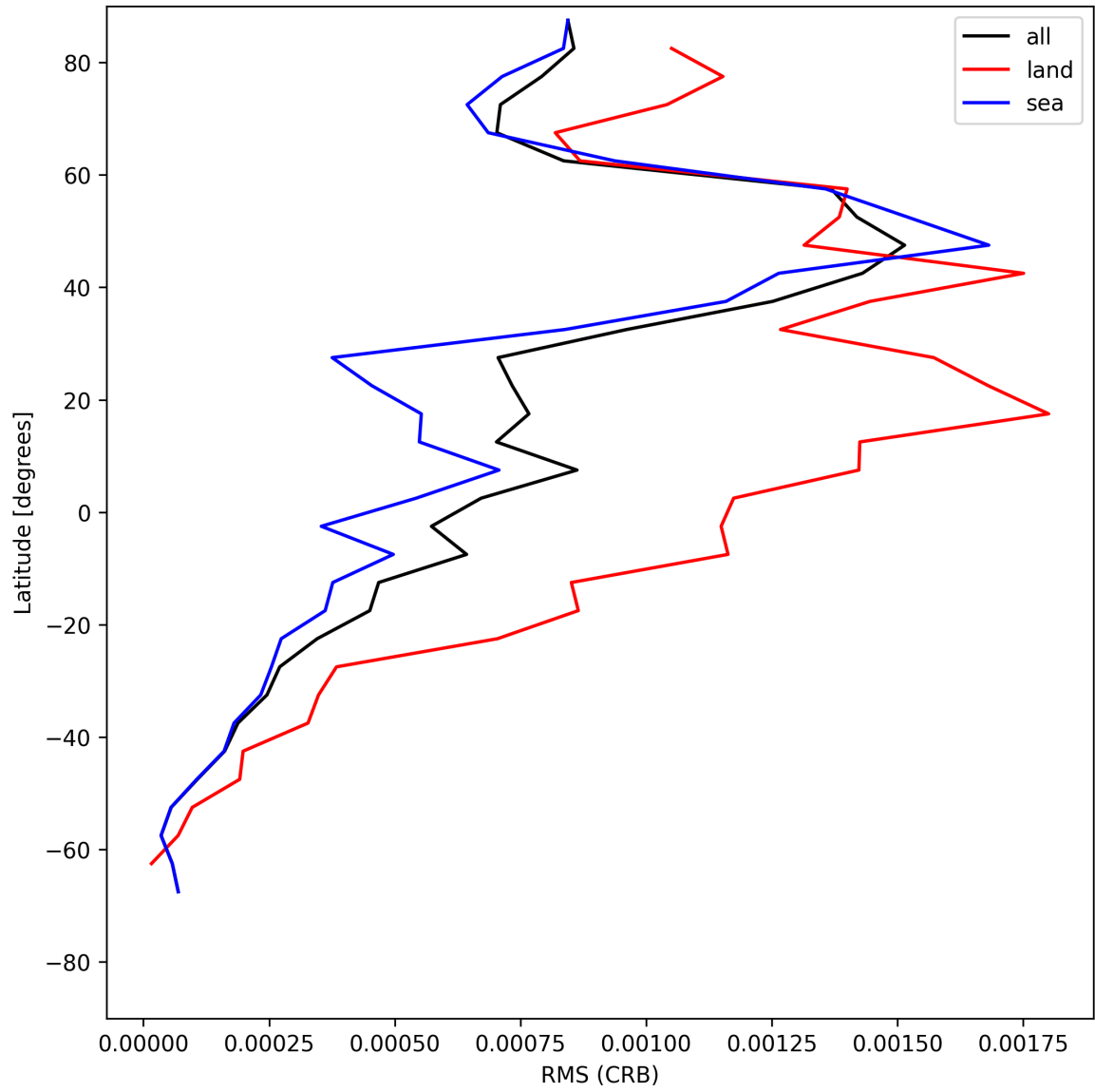
Figure 32: Zonal average of “RMS (CRB)” for 2025-06-14 to 2025-06-16.
