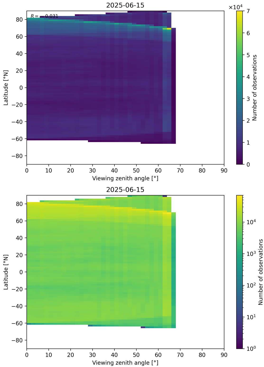
Figure 113: Scatter density plot of “Viewing zenith angle” against “Latitude” for 2025-06-14 to 2025-06-16.
