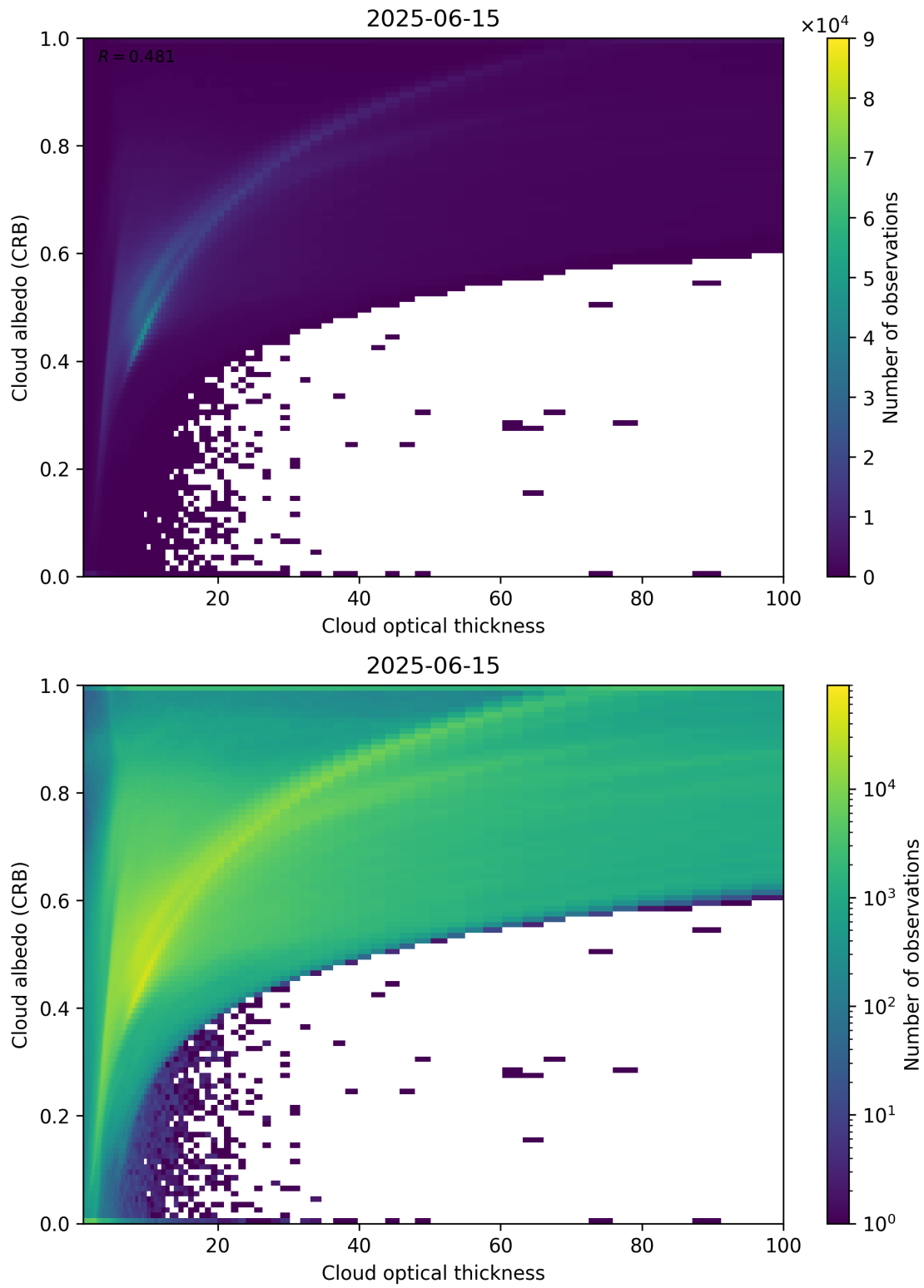
Figure 82: Scatter density plot of “Cloud optical thickness” against “Cloud albedo (CRB)” for 2025-06-14 to 2025-06-16.
