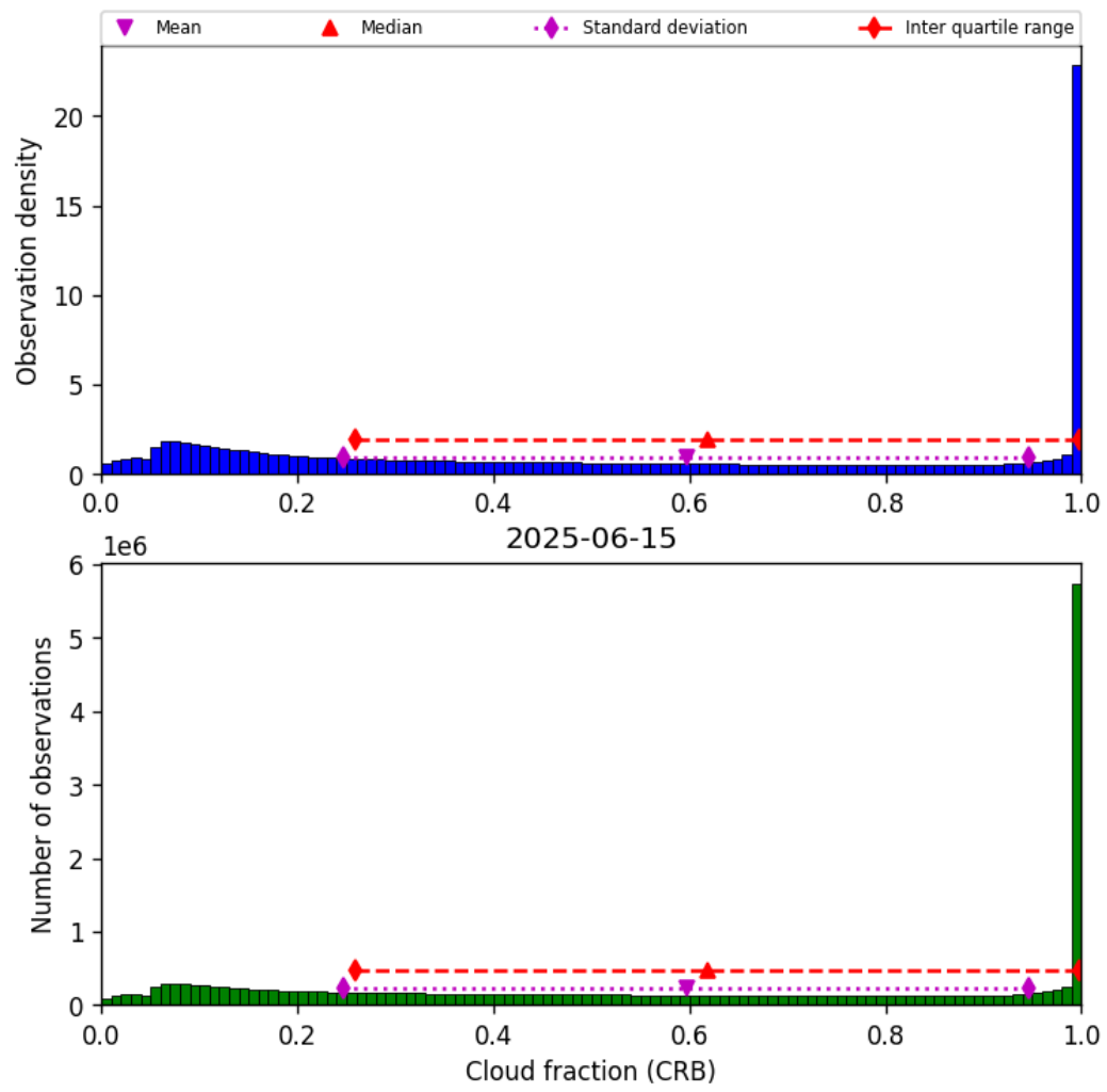
Figure 42: Histogram of “Cloud fraction (CRB)” for 2025-06-14 to 2025-06-16
