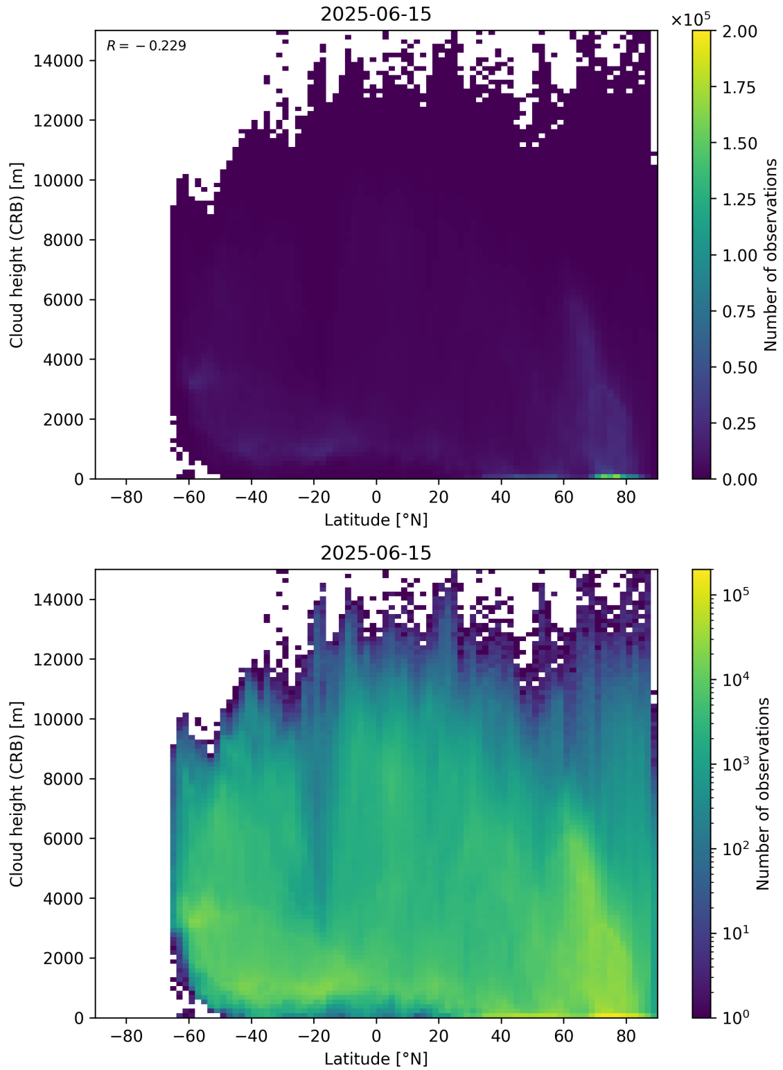
Figure 95: Scatter density plot of “Latitude” against “Cloud height (CRB)” for 2025-06-14 to 2025-06-16.
