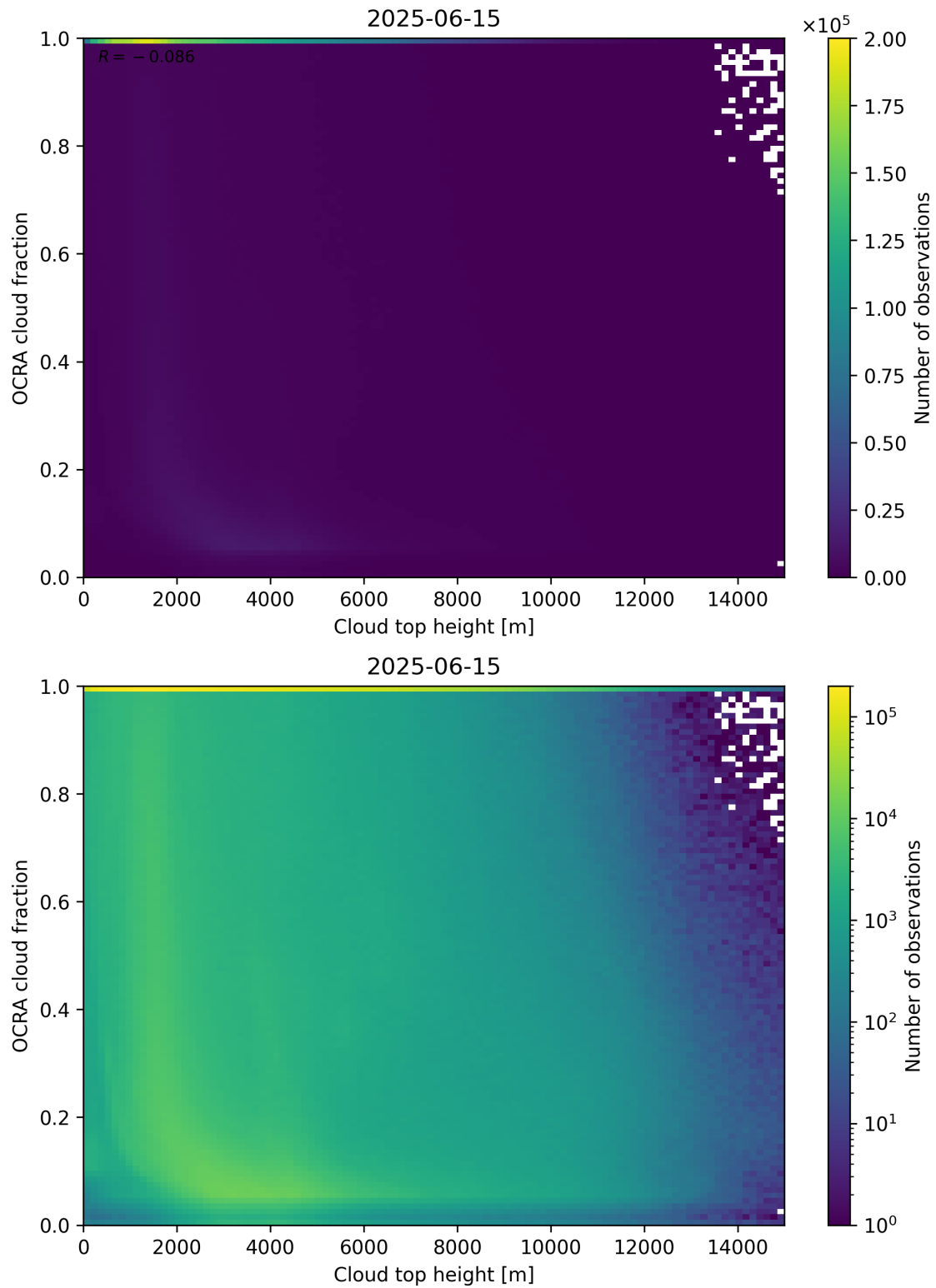
Figure 87: Scatter density plot of “Cloud top height” against “OCRA cloud fraction” for 2025-06-14 to 2025-06-16.
