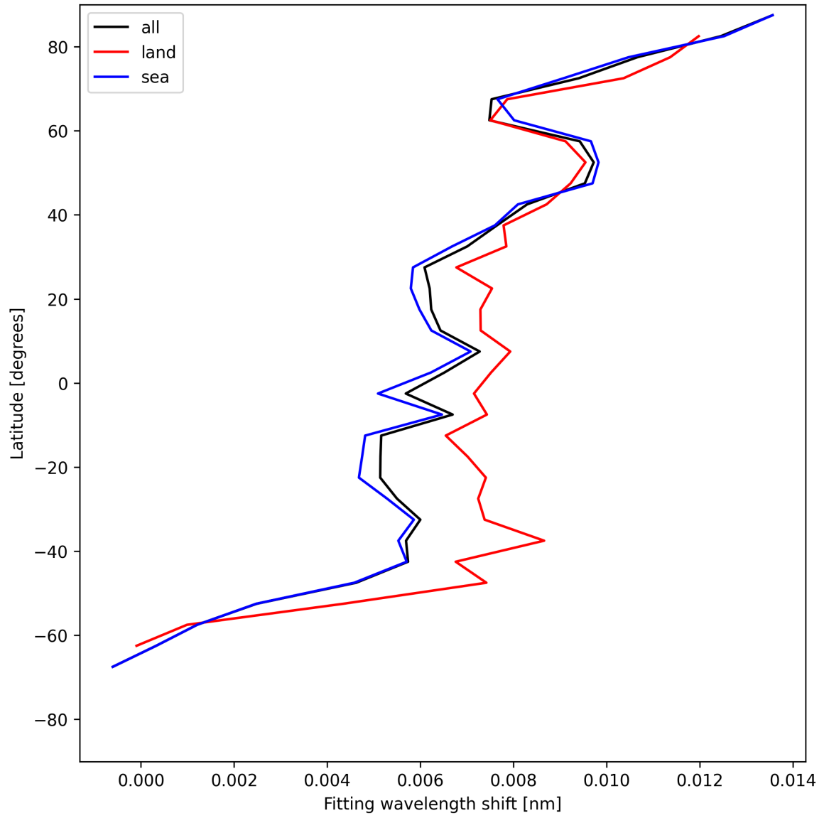
Figure 33: Zonal average of “Fitting wavelength shift” for 2025-06-14 to 2025-06-16.
