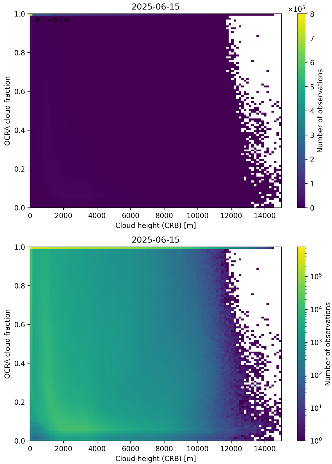
Figure 81: Scatter density plot of “Cloud height (CRB)” against “OCRA cloud fraction” for 2025-06-14 to 2025-06-16.
