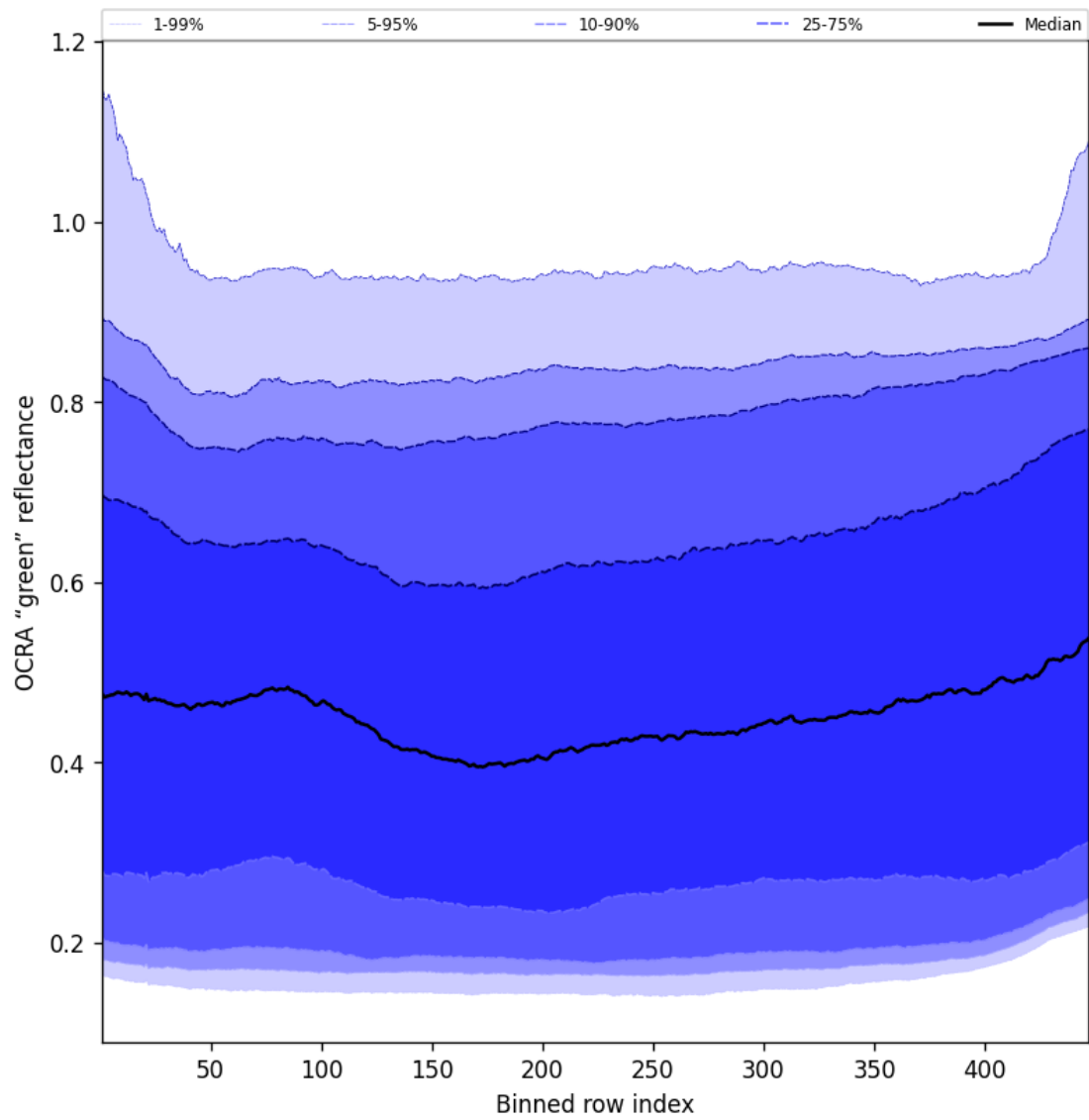
Figure 68: Along track statistics of “OCRA “green” reflectance” for 2025-06-14 to 2025-06-16
