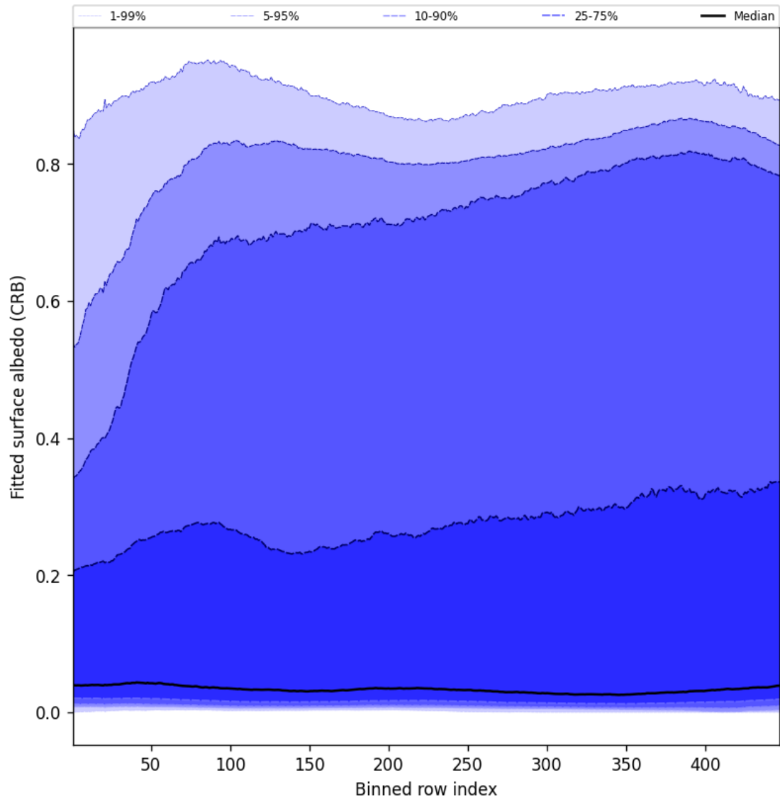
Figure 62: Along track statistics of “Fitted surface albedo (CRB)” for 2025-06-14 to 2025-06-16
