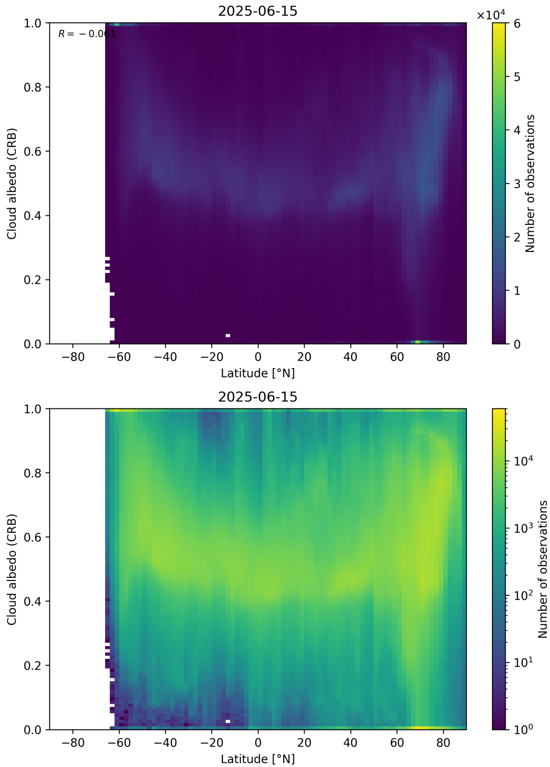
Figure 91: Scatter density plot of “Latitude” against “Cloud albedo (CRB)” for 2025-06-14 to 2025-06-16.
