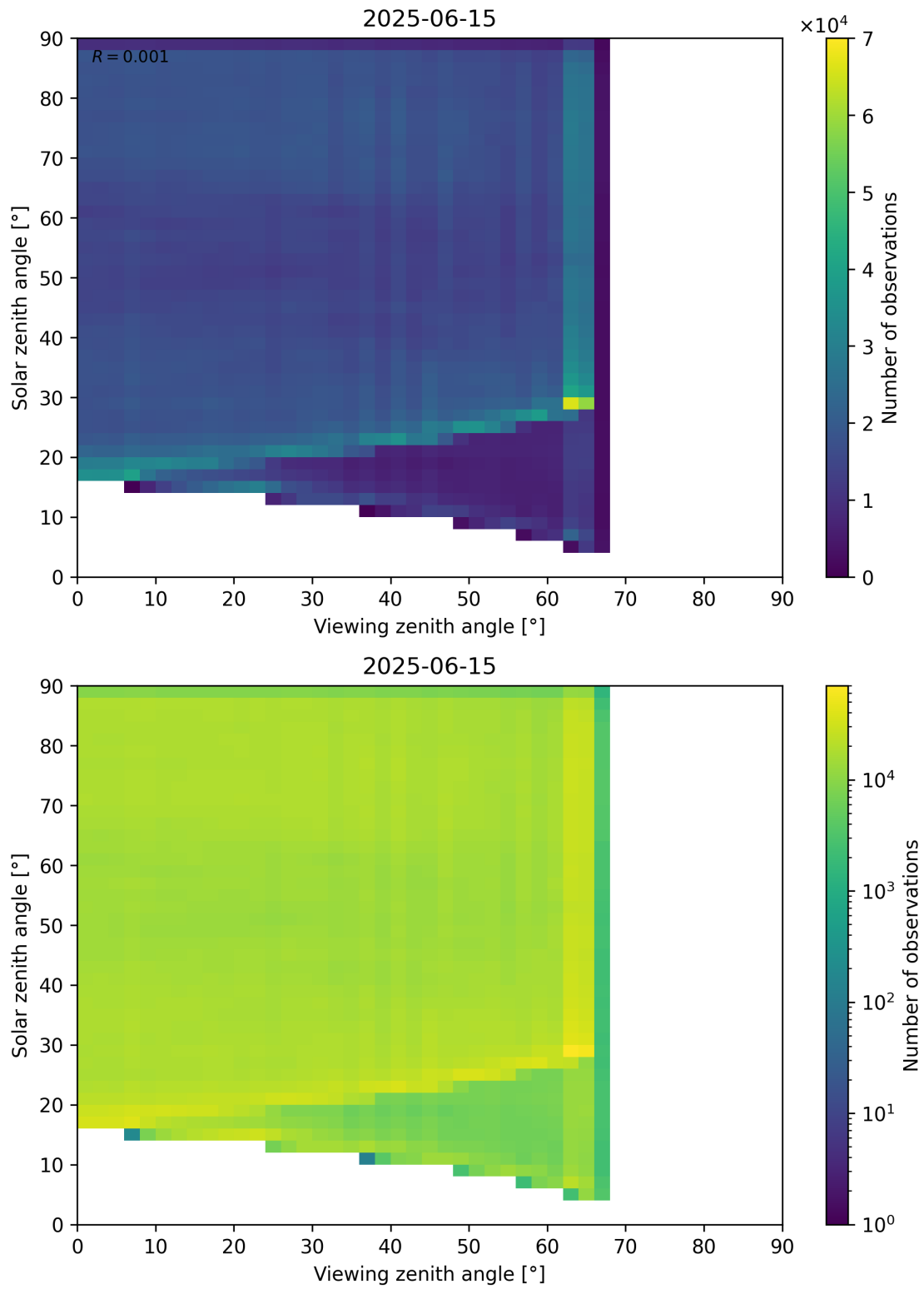
Figure 114: Scatter density plot of “Viewing zenith angle” against “Solar zenith angle” for 2025-06-14 to 2025-06-16.
