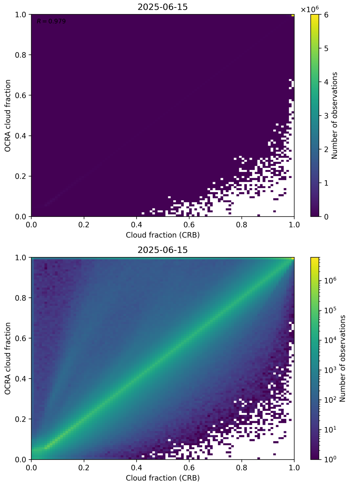
Figure 78: Scatter density plot of “Cloud fraction (CRB)” against “OCRA cloud fraction” for 2025-06-14 to 2025-06-16.
