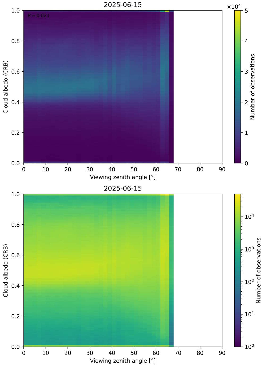
Figure 106: Scatter density plot of “Viewing zenith angle” against “Cloud albedo (CRB)” for 2025-06-14 to 2025-06-16.
