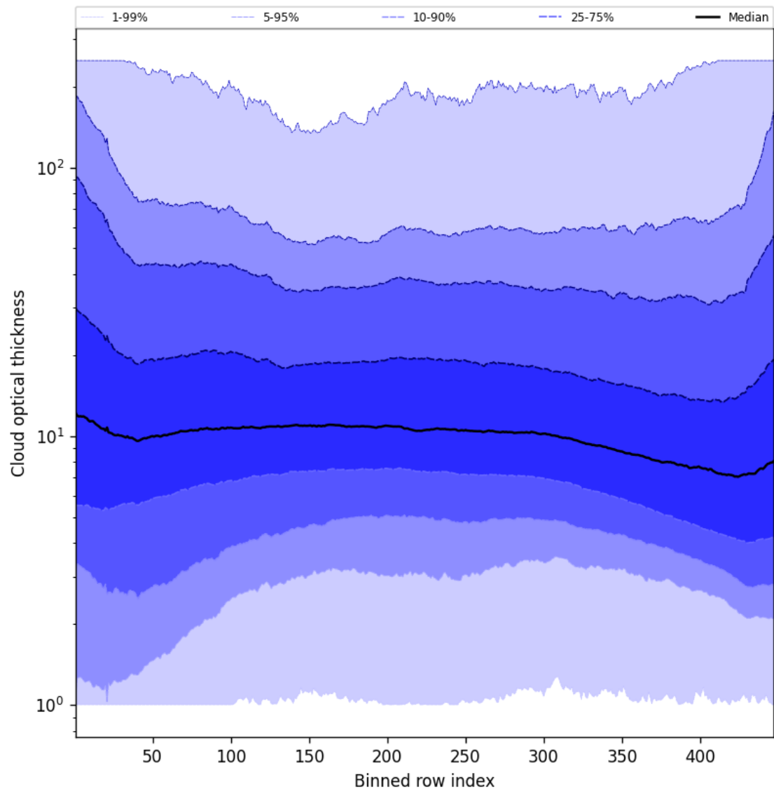
Figure 57: Along track statistics of “Cloud optical thickness” for 2025-06-14 to 2025-06-16
