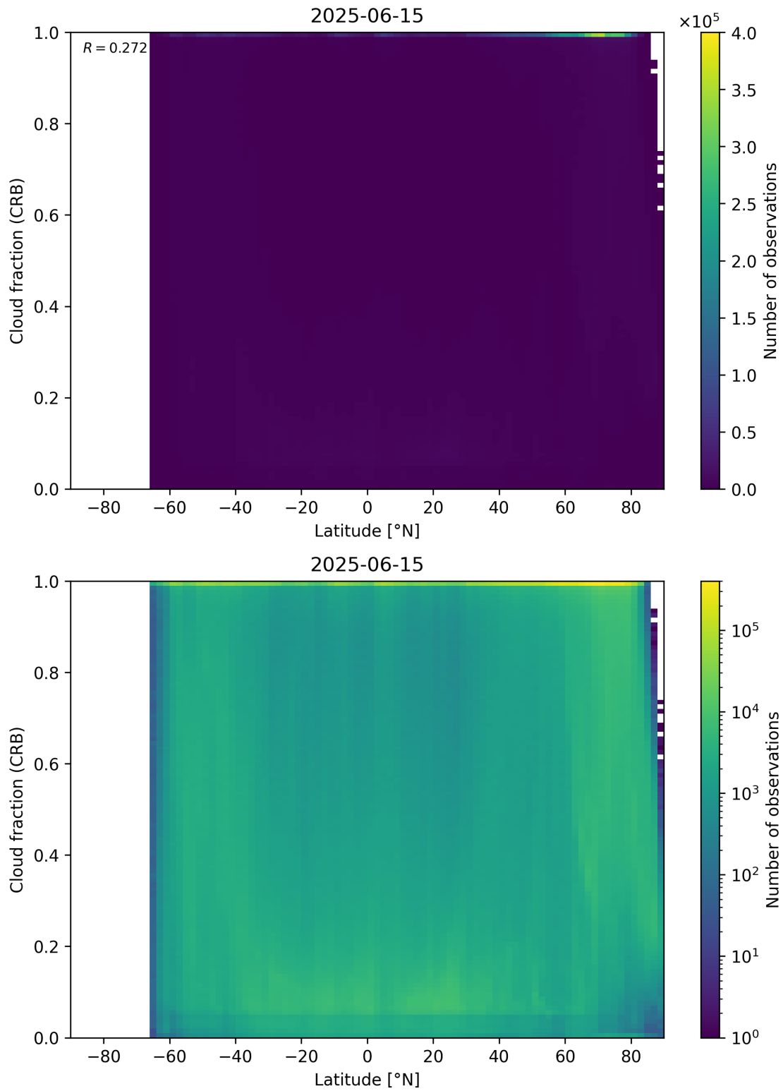
Figure 94: Scatter density plot of “Latitude” against “Cloud fraction (CRB)” for 2025-06-14 to 2025-06-16.
