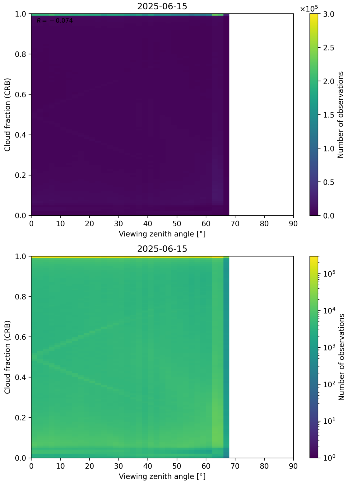
Figure 109: Scatter density plot of “Viewing zenith angle” against “Cloud fraction (CRB)” for 2025-06-14 to 2025-06-16.
