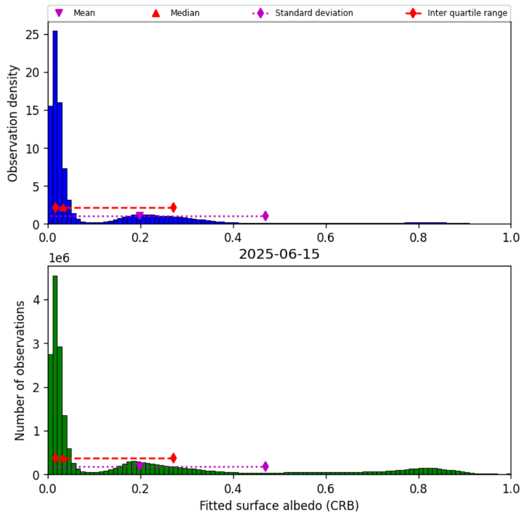
Figure 46: Histogram of “Fitted surface albedo (CRB)” for 2025-06-14 to 2025-06-16
