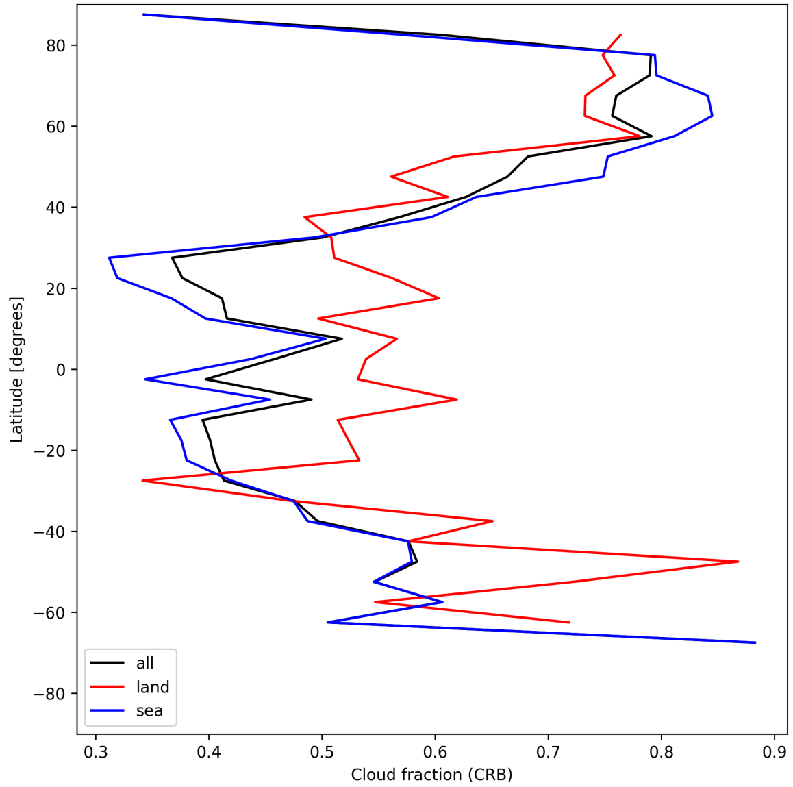
Figure 26: Zonal average of “Cloud fraction (CRB)” for 2025-06-14 to 2025-06-16.
