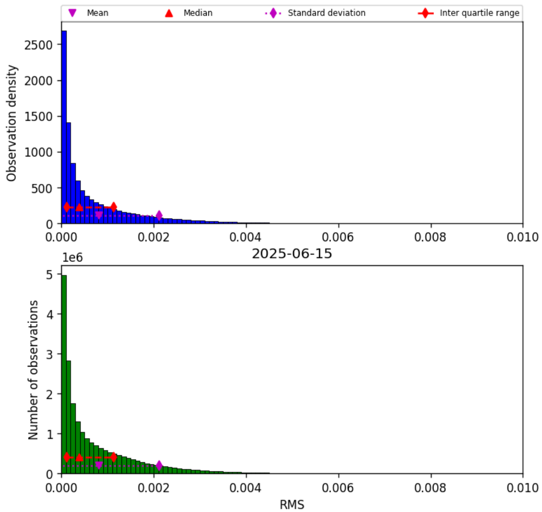
Figure 47: Histogram of “RMS” for 2025-06-14 to 2025-06-16
