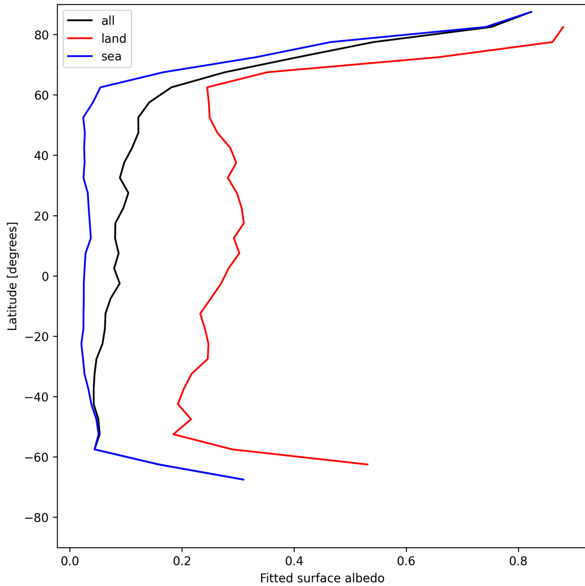
Figure 29: Zonal average of “Fitted surface albedo” for 2025-06-14 to 2025-06-16.
