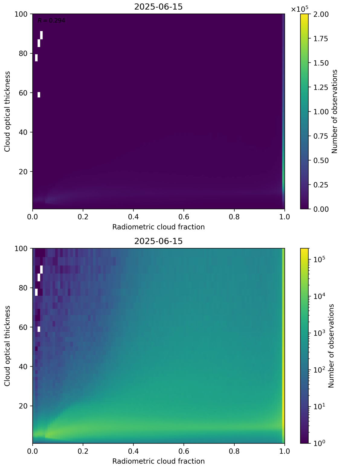
Figure 75: Scatter density plot of “Radiometric cloud fraction” against “Cloud optical thickness” for 2025-06-14 to 2025-06-16.
