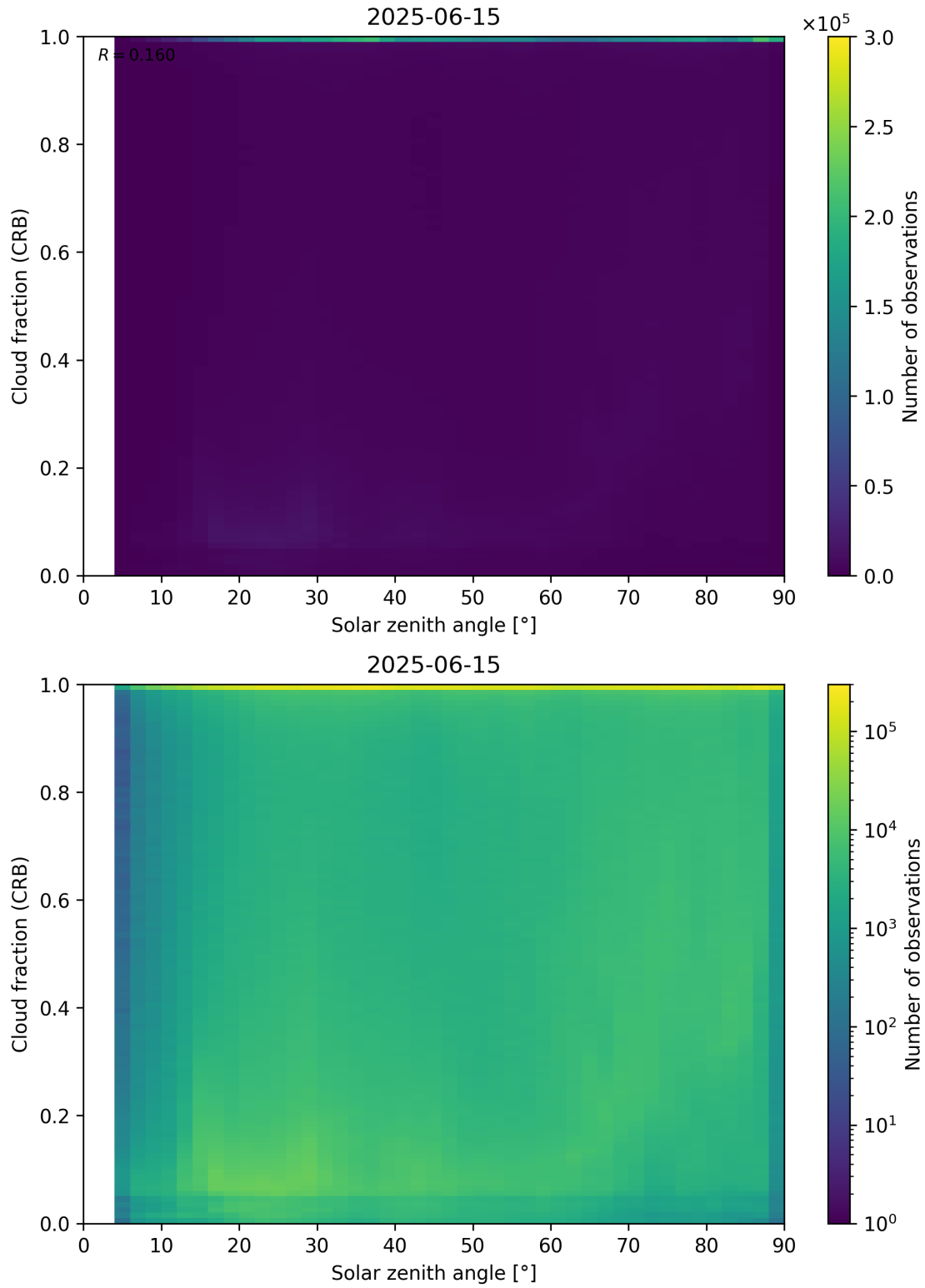
Figure 101: Scatter density plot of “Solar zenith angle” against “Cloud fraction (CRB)” for 2025-06-14 to 2025-06-16.
