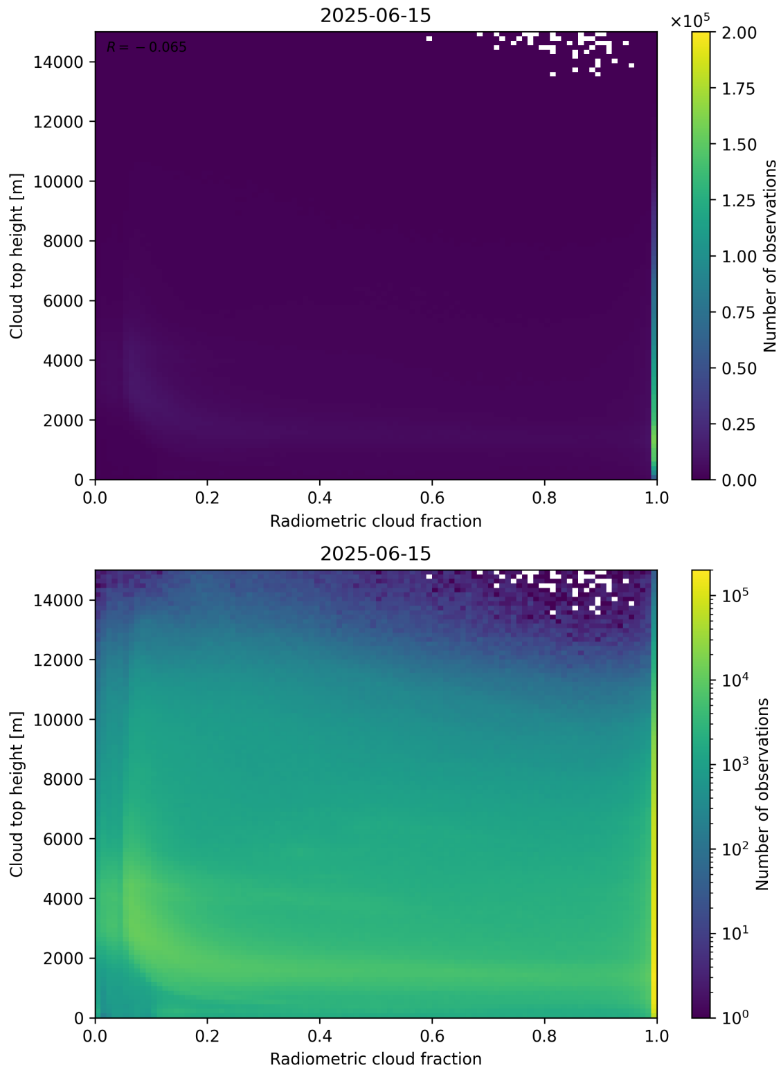
Figure 76: Scatter density plot of “Radiometric cloud fraction” against “Cloud top height” for 2025-06-14 to 2025-06-16.
