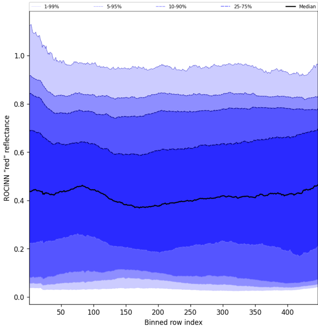
Figure 69: Along track statistics of "ROCINN "red" reflectance" for 2025-06-14 to 2025-06-16
