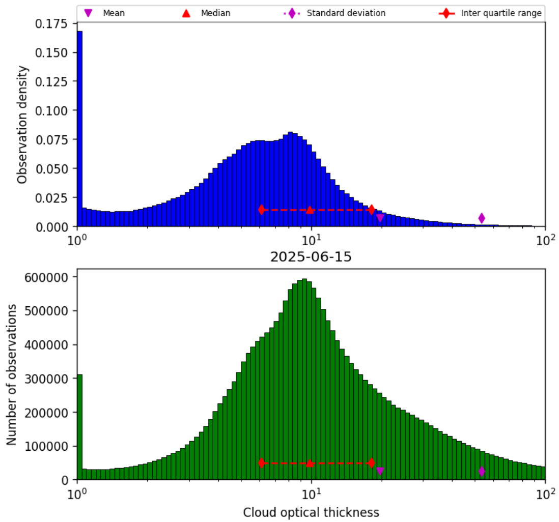
Figure 41: Histogram of “Cloud optical thickness” for 2025-06-14 to 2025-06-16
