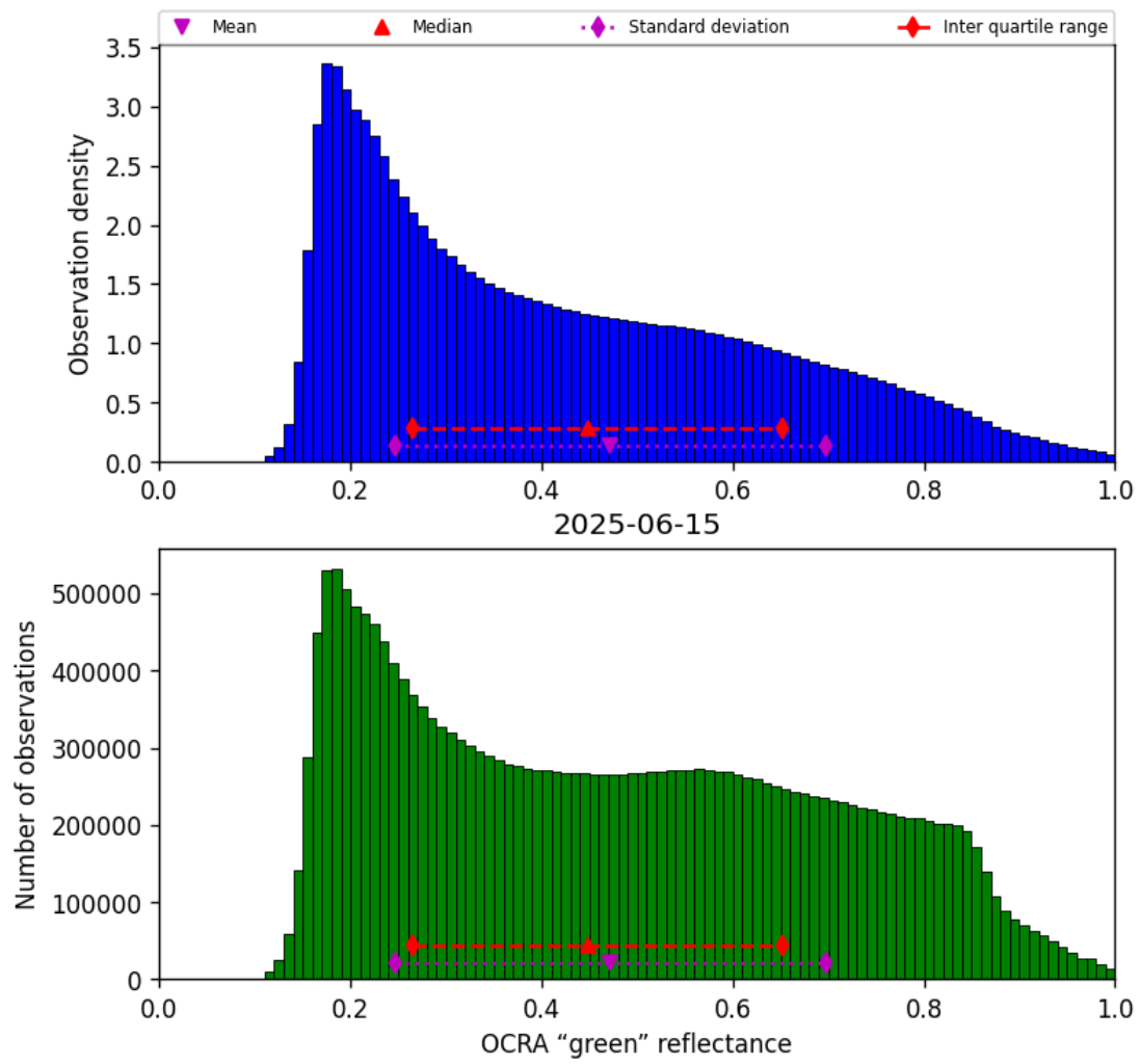
Figure 52: Histogram of “OCRA “green” reflectance” for 2025-06-14 to 2025-06-16
