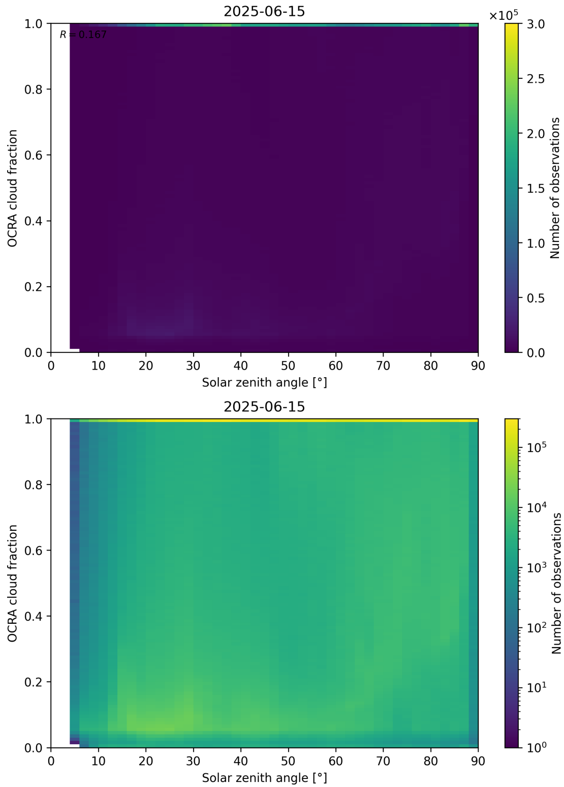
Figure 100: Scatter density plot of “Solar zenith angle” against “OCRA cloud fraction” for 2025-06-14 to 2025-06-16.
