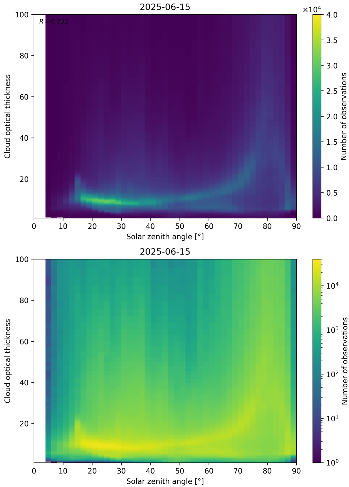
Figure 103: Scatter density plot of “Solar zenith angle” against “Cloud optical thickness” for 2025-06-14 to 2025-06-16.
