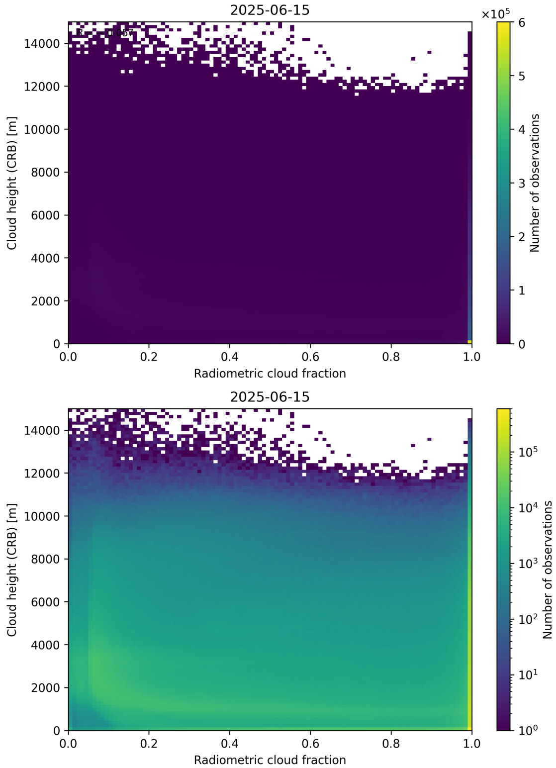
Figure 74: Scatter density plot of “Radiometric cloud fraction” against “Cloud height (CRB)” for 2025-06-14 to 2025-06-16.
