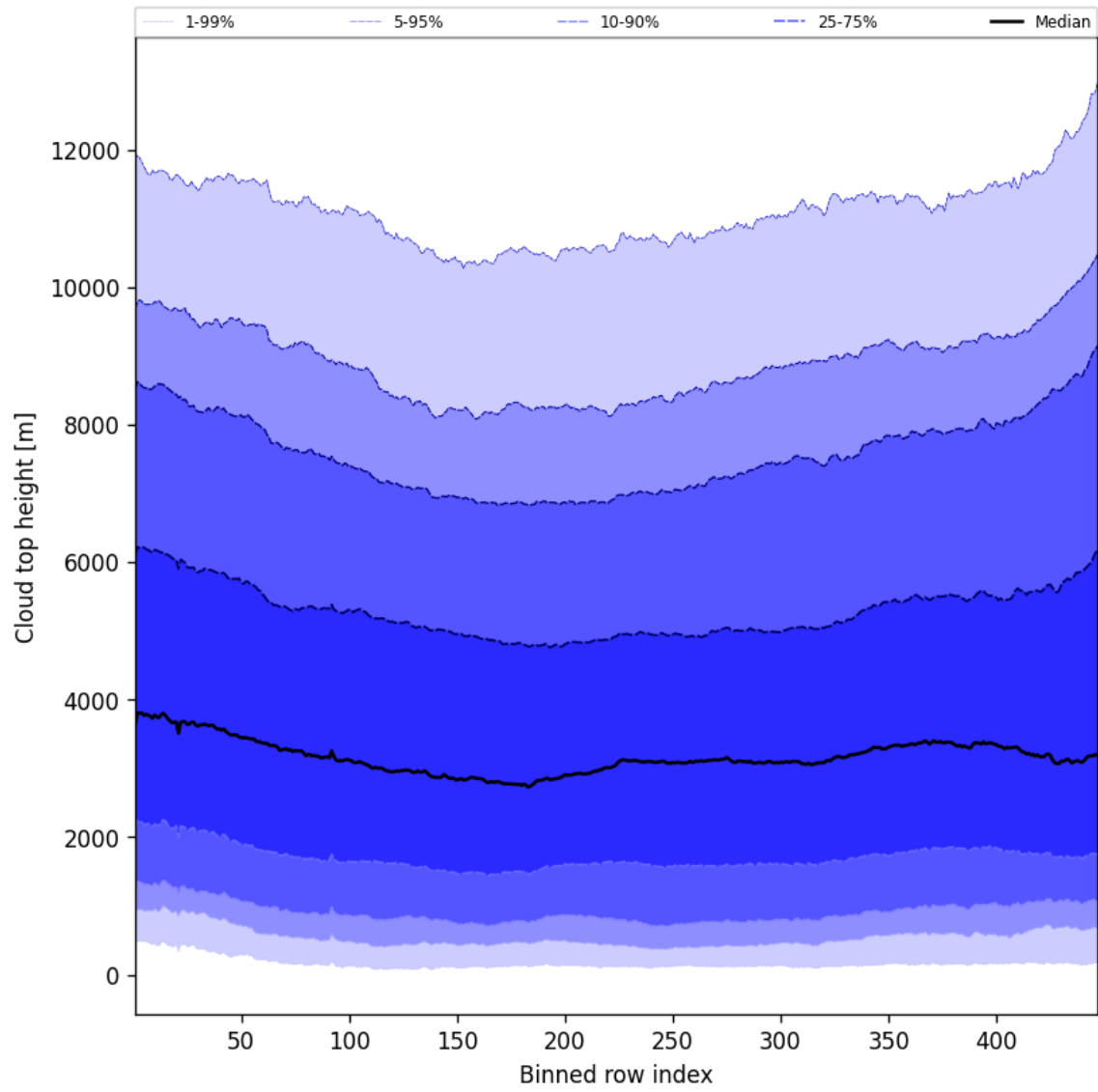
Figure 56: Along track statistics of “Cloud top height” for 2025-06-14 to 2025-06-16
