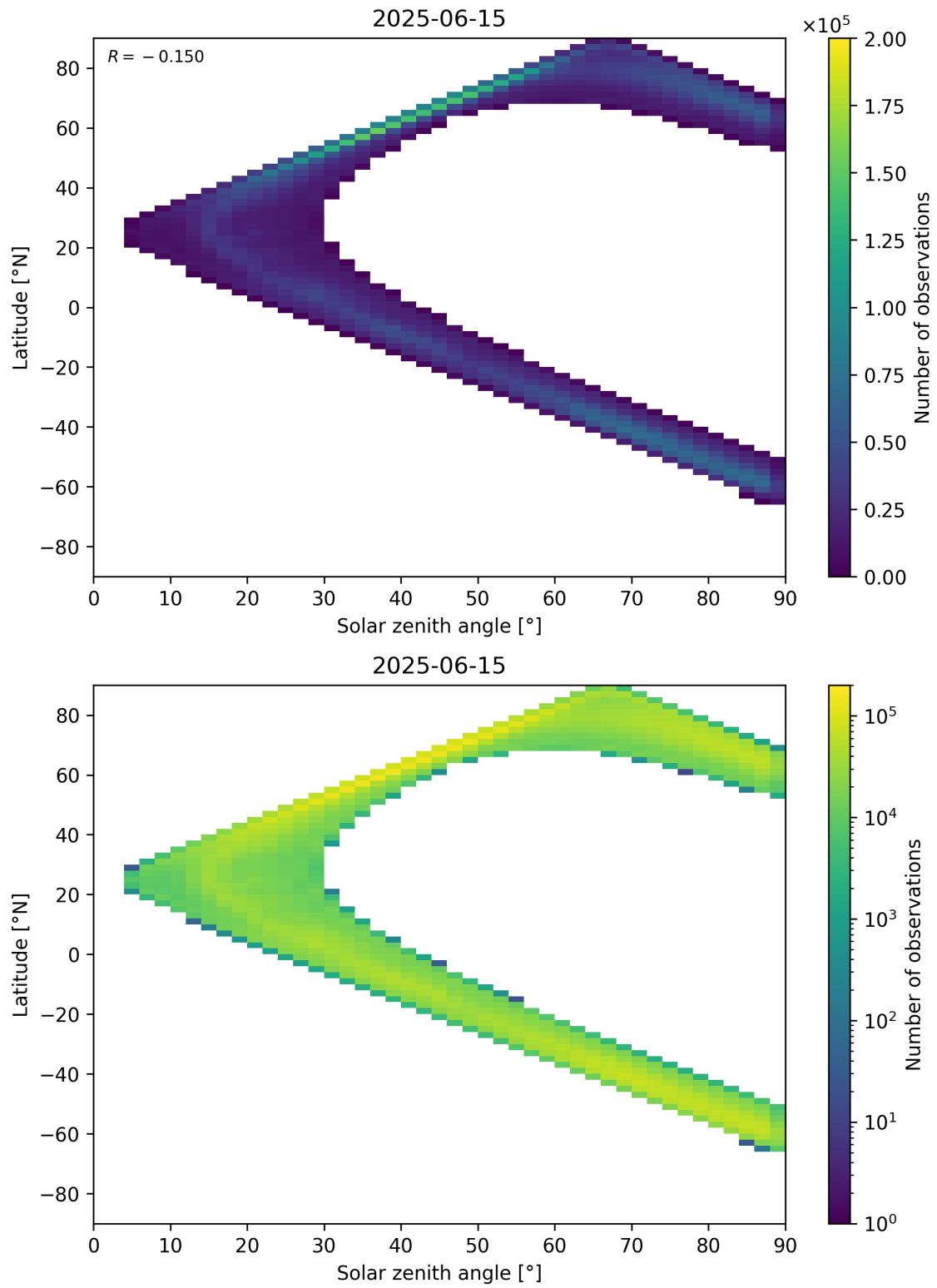
Figure 105: Scatter density plot of “Solar zenith angle” against “Latitude” for 2025-06-14 to 2025-06-16.
