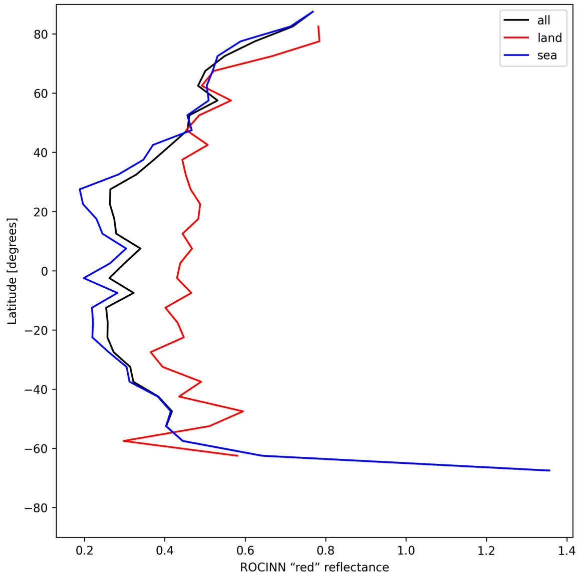
Figure 37: Zonal average of “ROCINN “red” reflectance” for 2025-06-14 to 2025-06-16.
