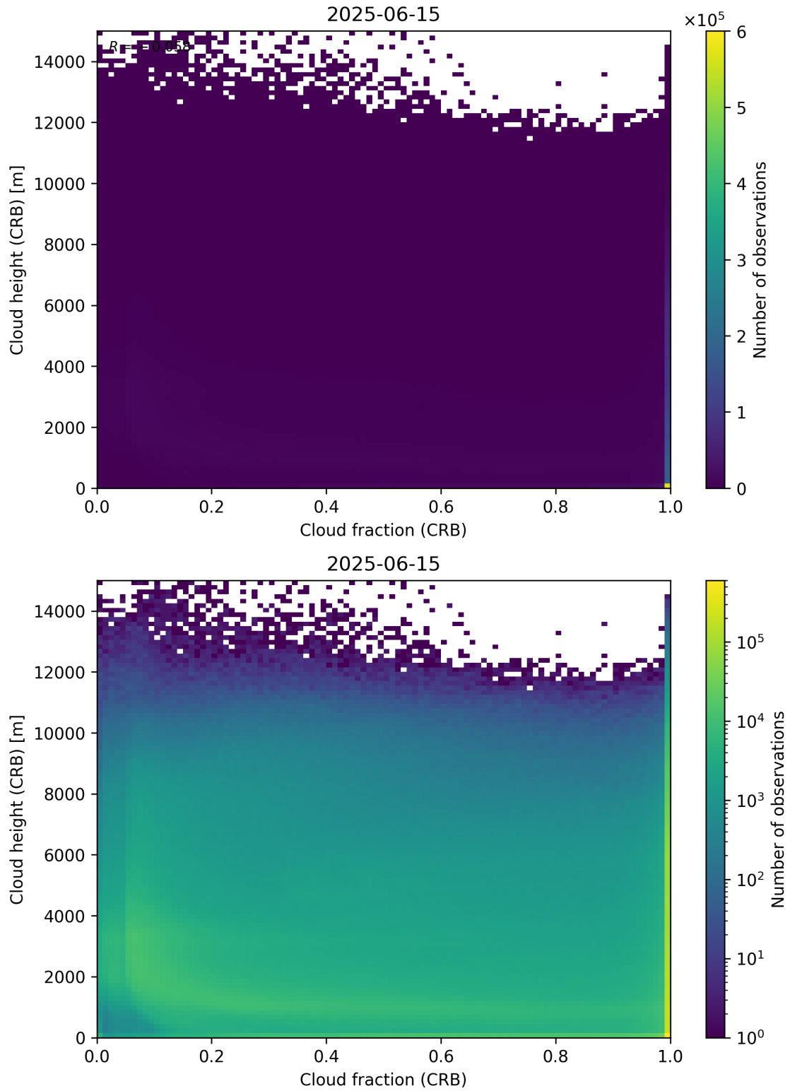
Figure 79: Scatter density plot of “Cloud fraction (CRB)” against “Cloud height (CRB)” for 2025-06-14 to 2025-06-16.
