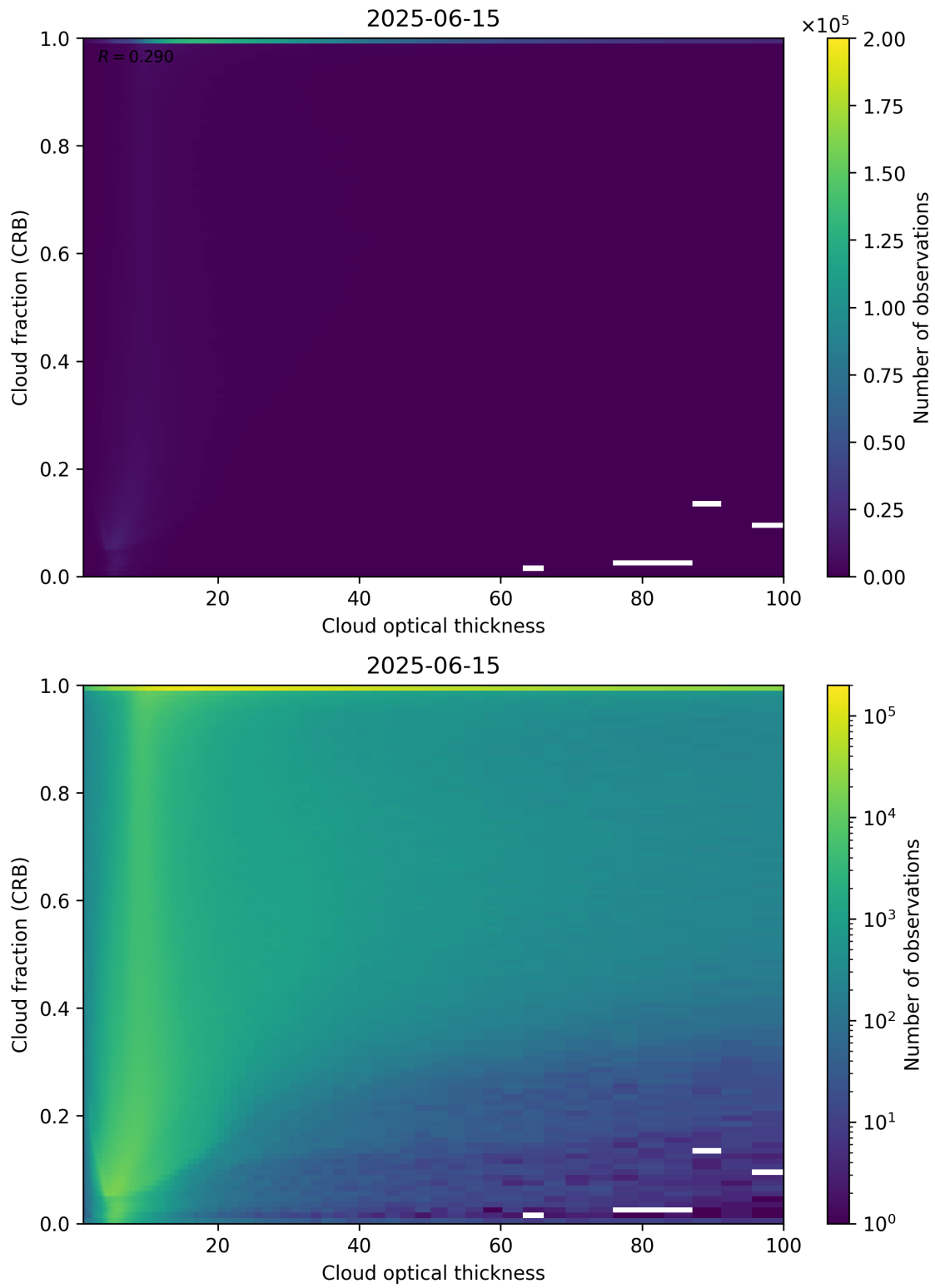
Figure 84: Scatter density plot of “Cloud optical thickness” against “Cloud fraction (CRB)” for 2025-06-14 to 2025-06-16.
