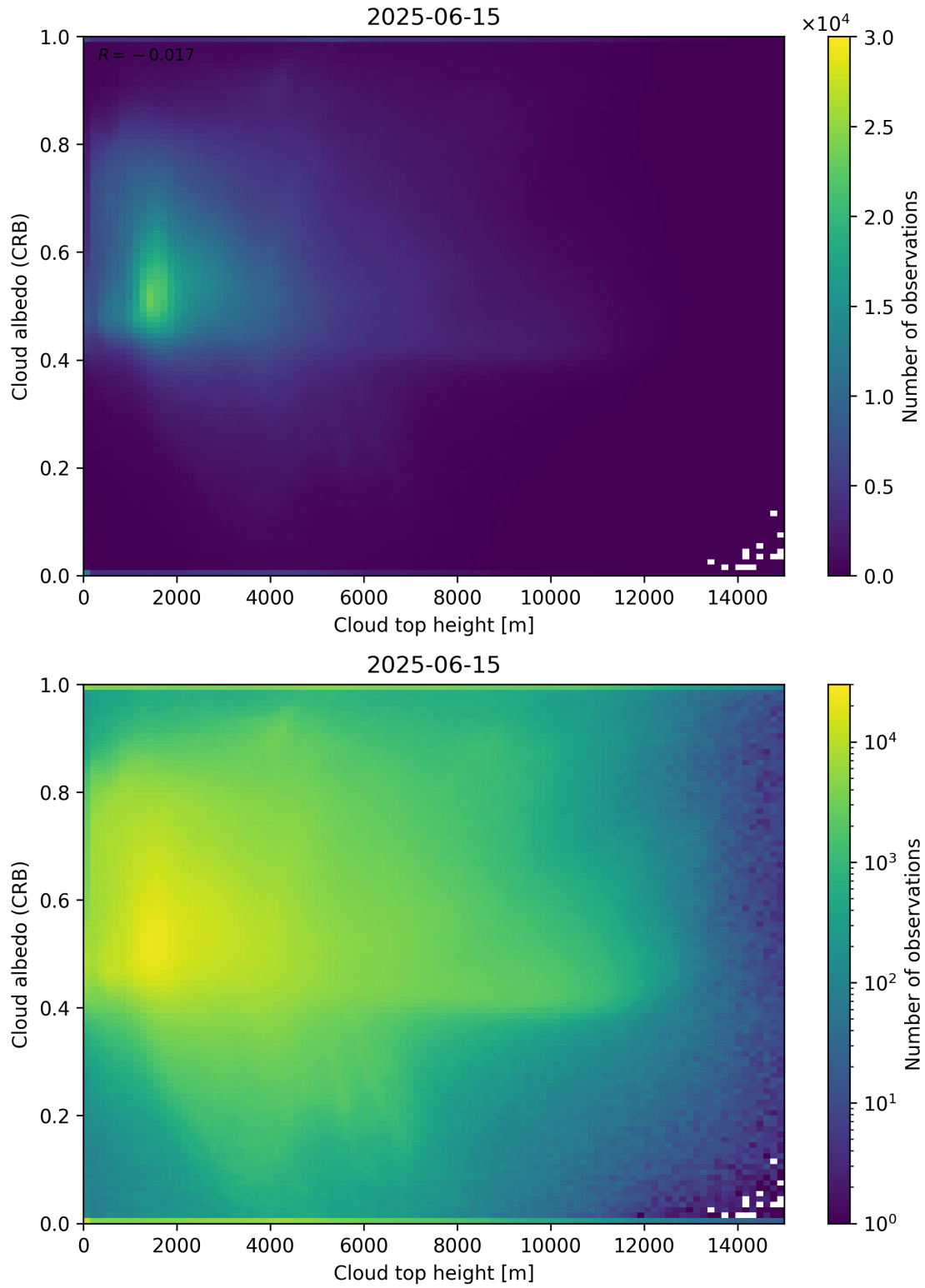
Figure 86: Scatter density plot of “Cloud top height” against “Cloud albedo (CRB)” for 2025-06-14 to 2025-06-16.
