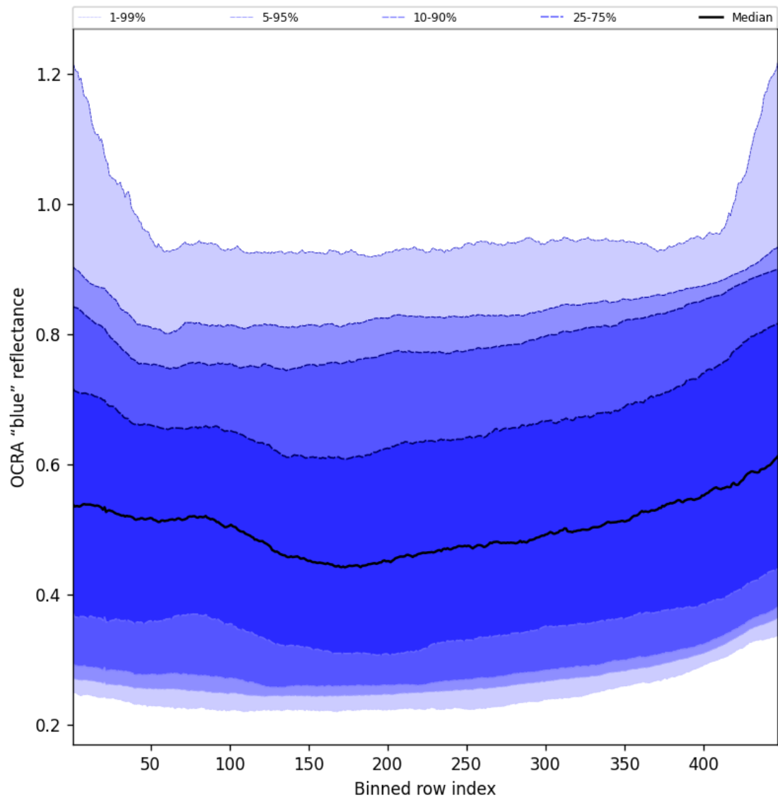
Figure 67: Along track statistics of “OCRA “blue” reflectance” for 2025-06-14 to 2025-06-16
