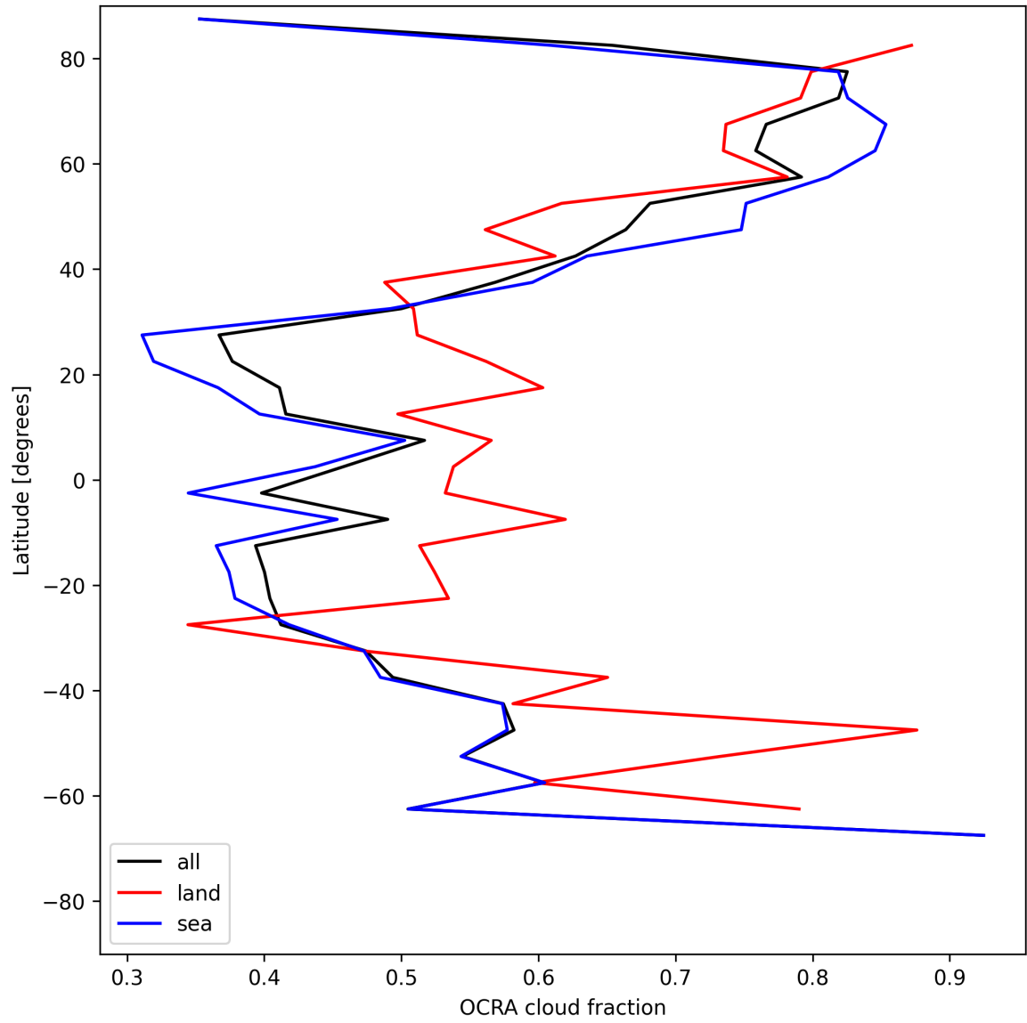
Figure 34: Zonal average of “OCRA cloud fraction” for 2025-06-14 to 2025-06-16.
