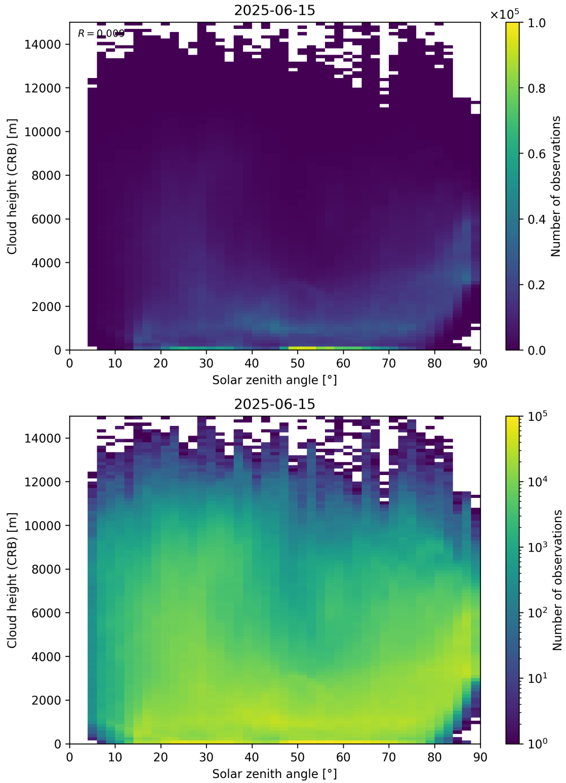
Figure 102: Scatter density plot of “Solar zenith angle” against “Cloud height (CRB)” for 2025-06-14 to 2025-06-16.
