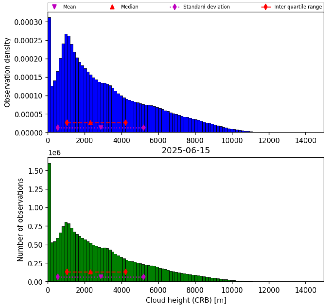
Figure 43: Histogram of “Cloud height (CRB)” for 2025-06-14 to 2025-06-16
