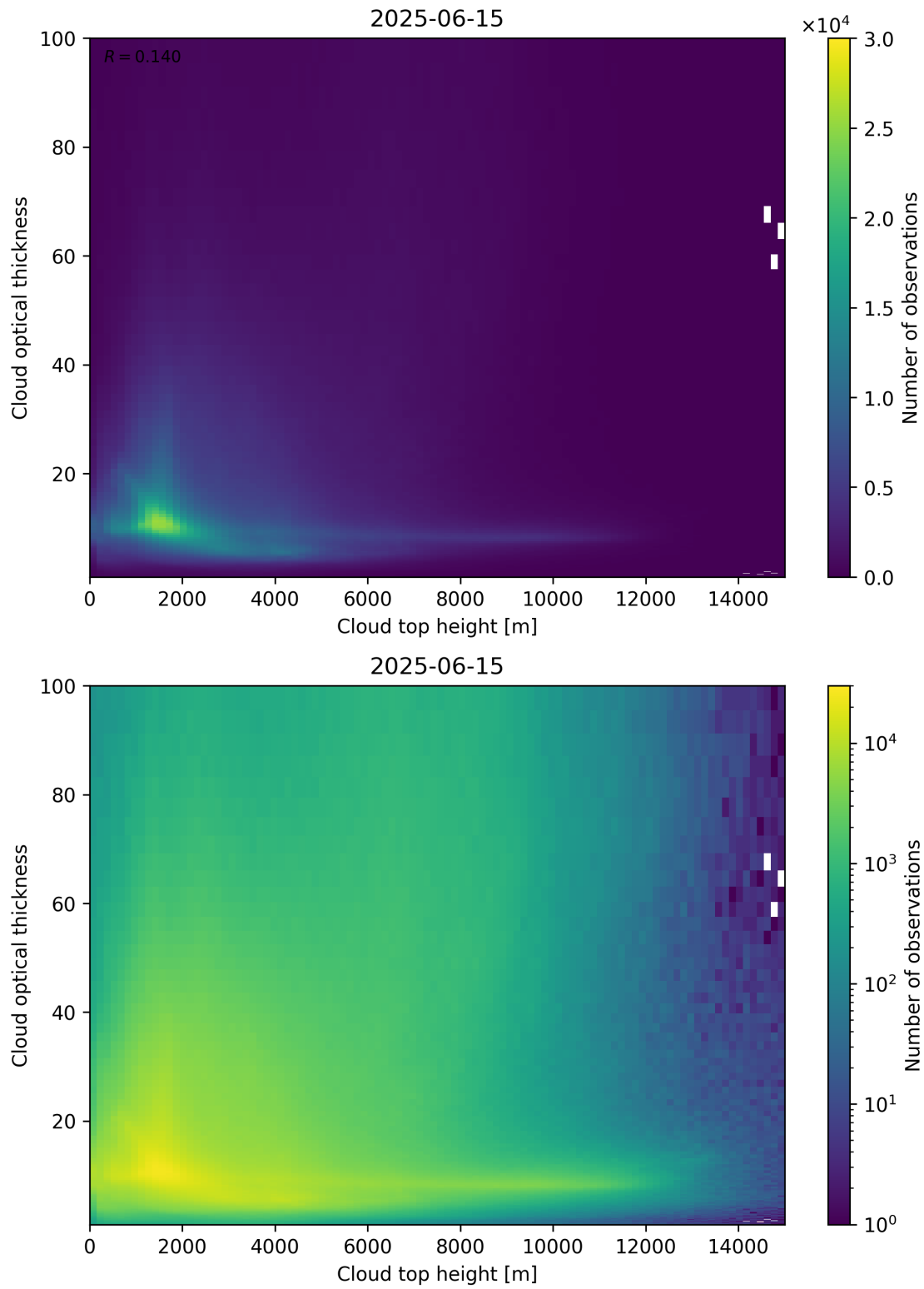
Figure 90: Scatter density plot of “Cloud top height” against “Cloud optical thickness” for 2025-06-14 to 2025-06-16.
