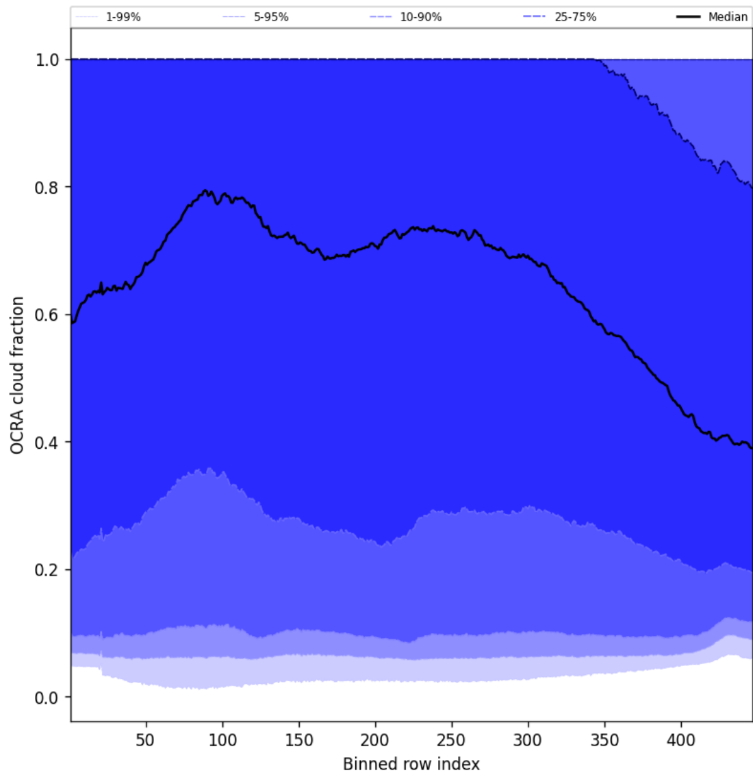
Figure 66: Along track statistics of “OCRA cloud fraction” for 2025-06-14 to 2025-06-16
