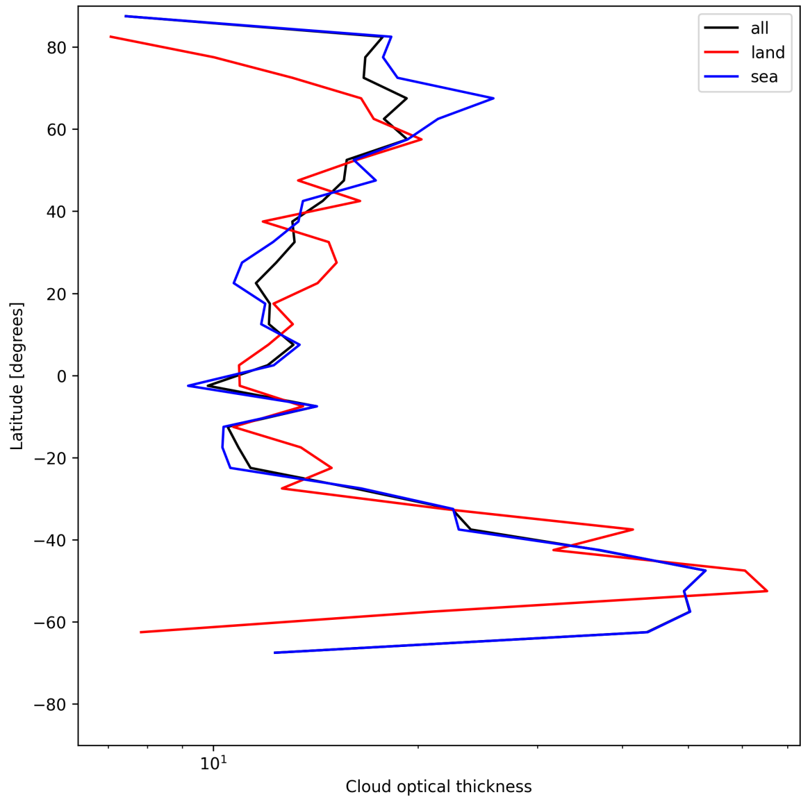
Figure 25: Zonal average of “Cloud optical thickness” for 2025-06-14 to 2025-06-16.
