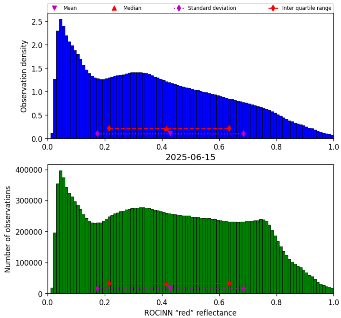
Figure 53: Histogram of “ROCINN “red” reflectance” for 2025-06-14 to 2025-06-16
