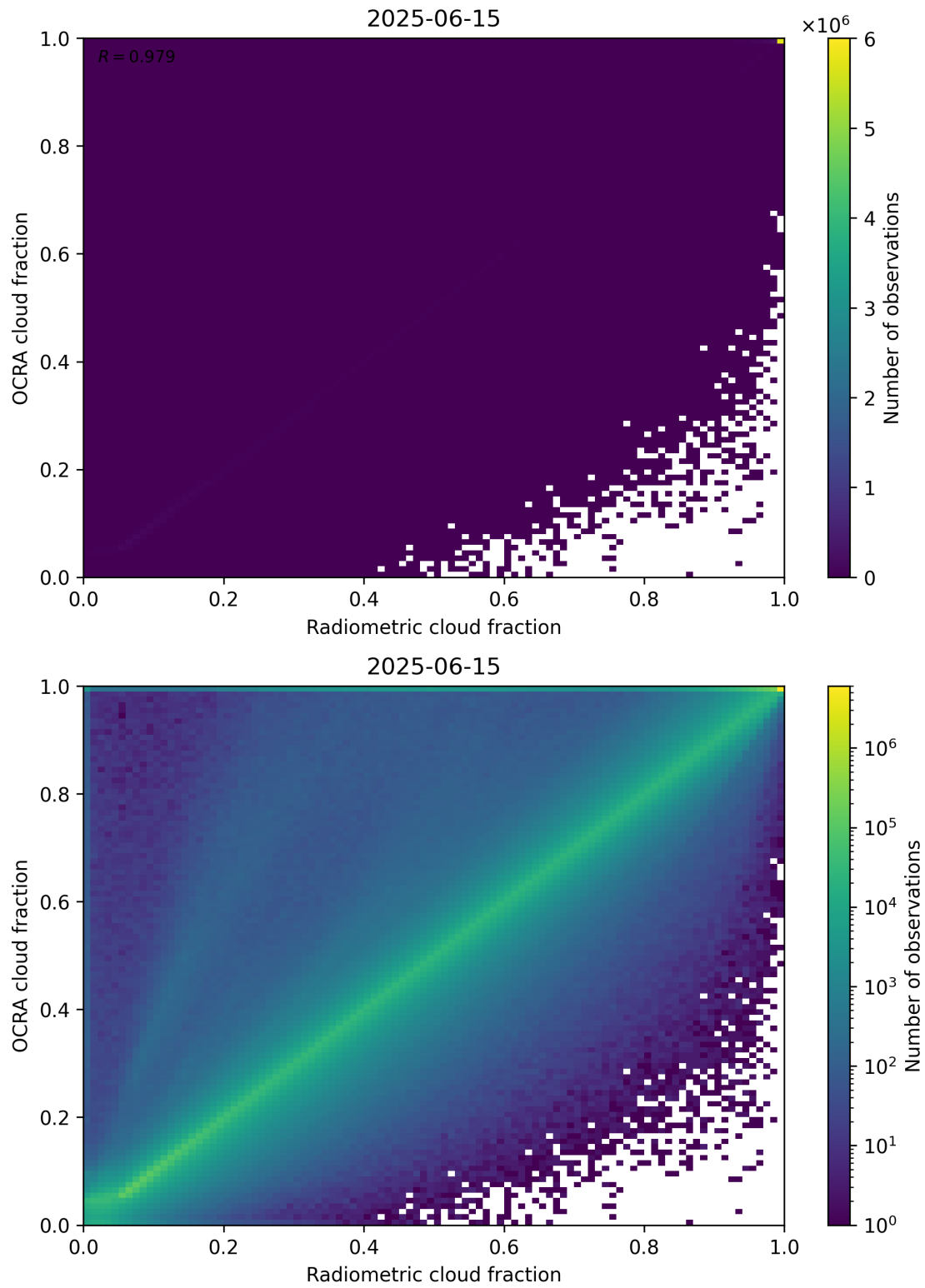
Figure 72: Scatter density plot of “Radiometric cloud fraction” against “OCRA cloud fraction” for 2025-06-14 to 2025-06-16.
