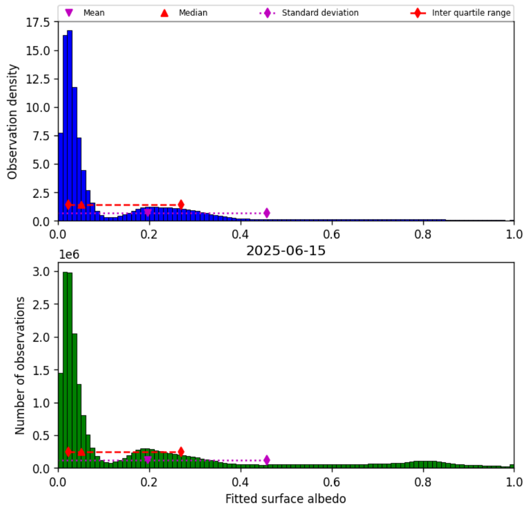
Figure 45: Histogram of “Fitted surface albedo” for 2025-06-14 to 2025-06-16
