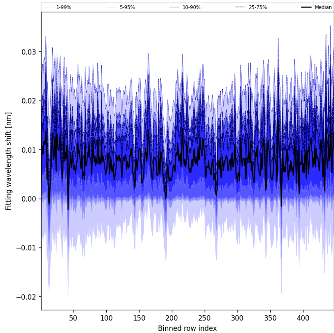
Figure 65: Along track statistics of “Fitting wavelength shift” for 2025-06-14 to 2025-06-16
