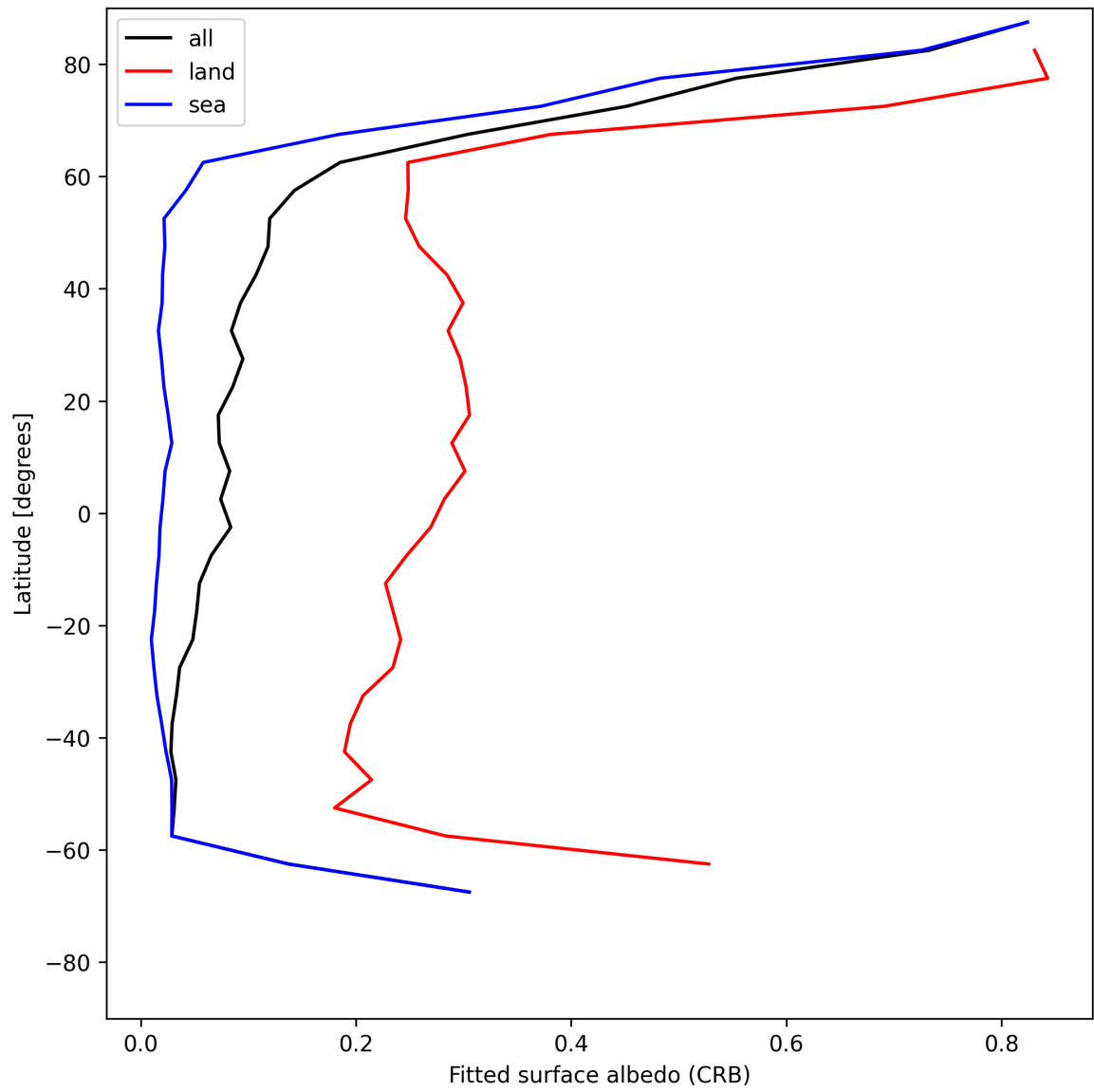
Figure 30: Zonal average of “Fitted surface albedo (CRB)” for 2025-06-14 to 2025-06-16.
