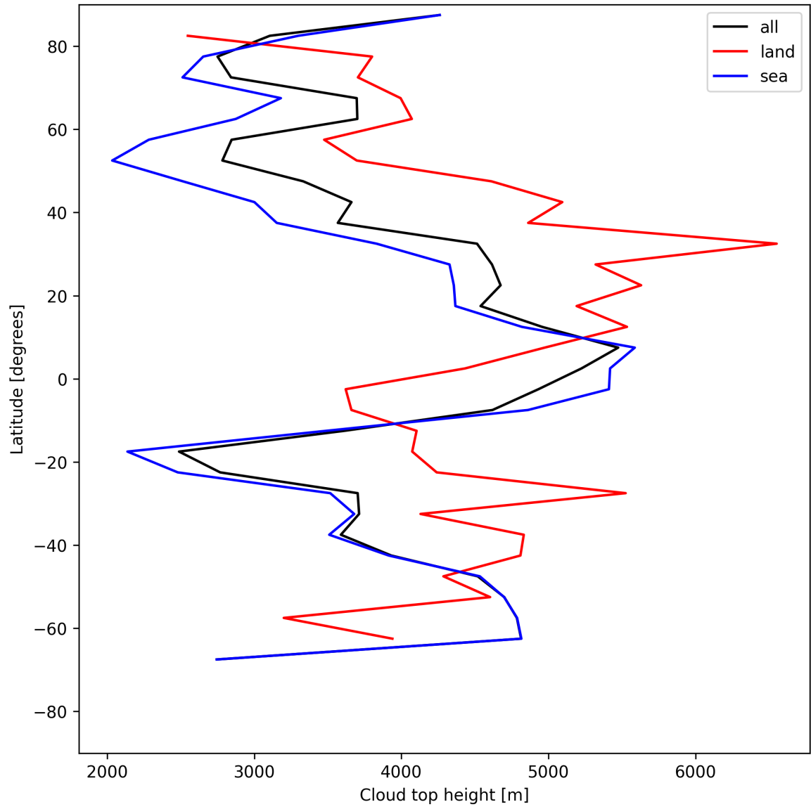
Figure 24: Zonal average of “Cloud top height” for 2025-06-14 to 2025-06-16.
