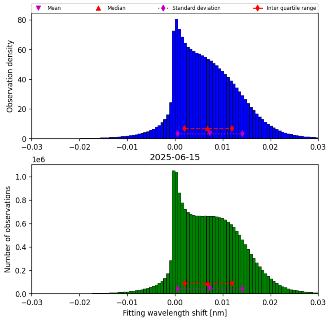
Figure 49: Histogram of “Fitting wavelength shift” for 2025-06-14 to 2025-06-16
