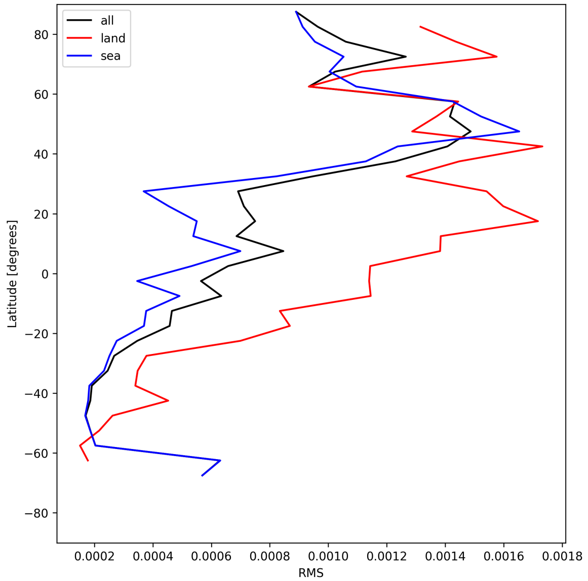
Figure 31: Zonal average of “RMS” for 2025-06-14 to 2025-06-16.
