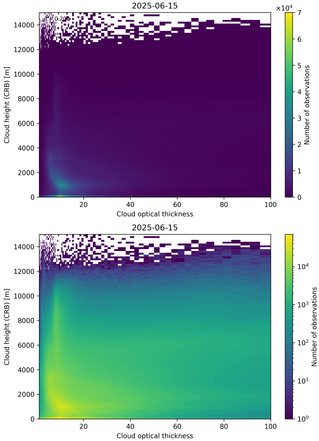
Figure 85: Scatter density plot of “Cloud optical thickness” against “Cloud height (CRB)” for 2025-06-14 to 2025-06-16.
