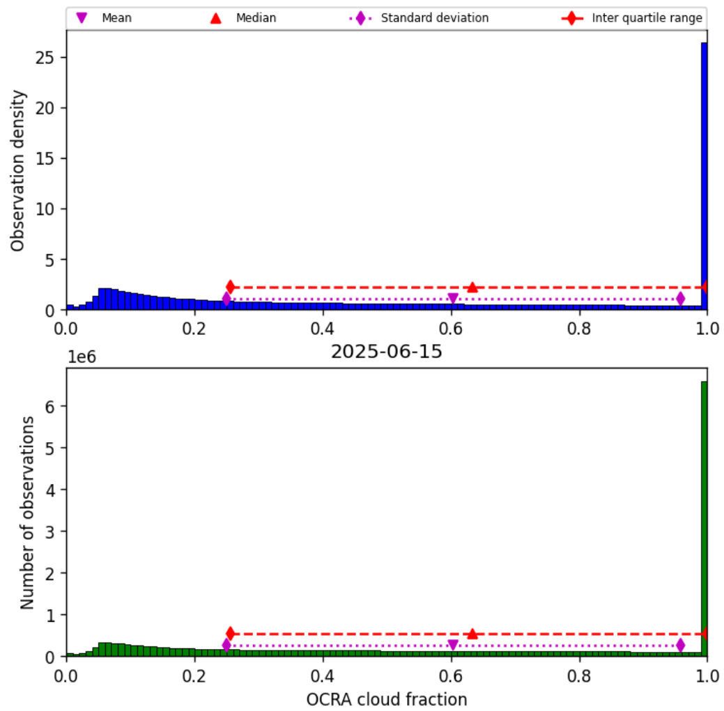
Figure 50: Histogram of “OCRA cloud fraction” for 2025-06-14 to 2025-06-16
