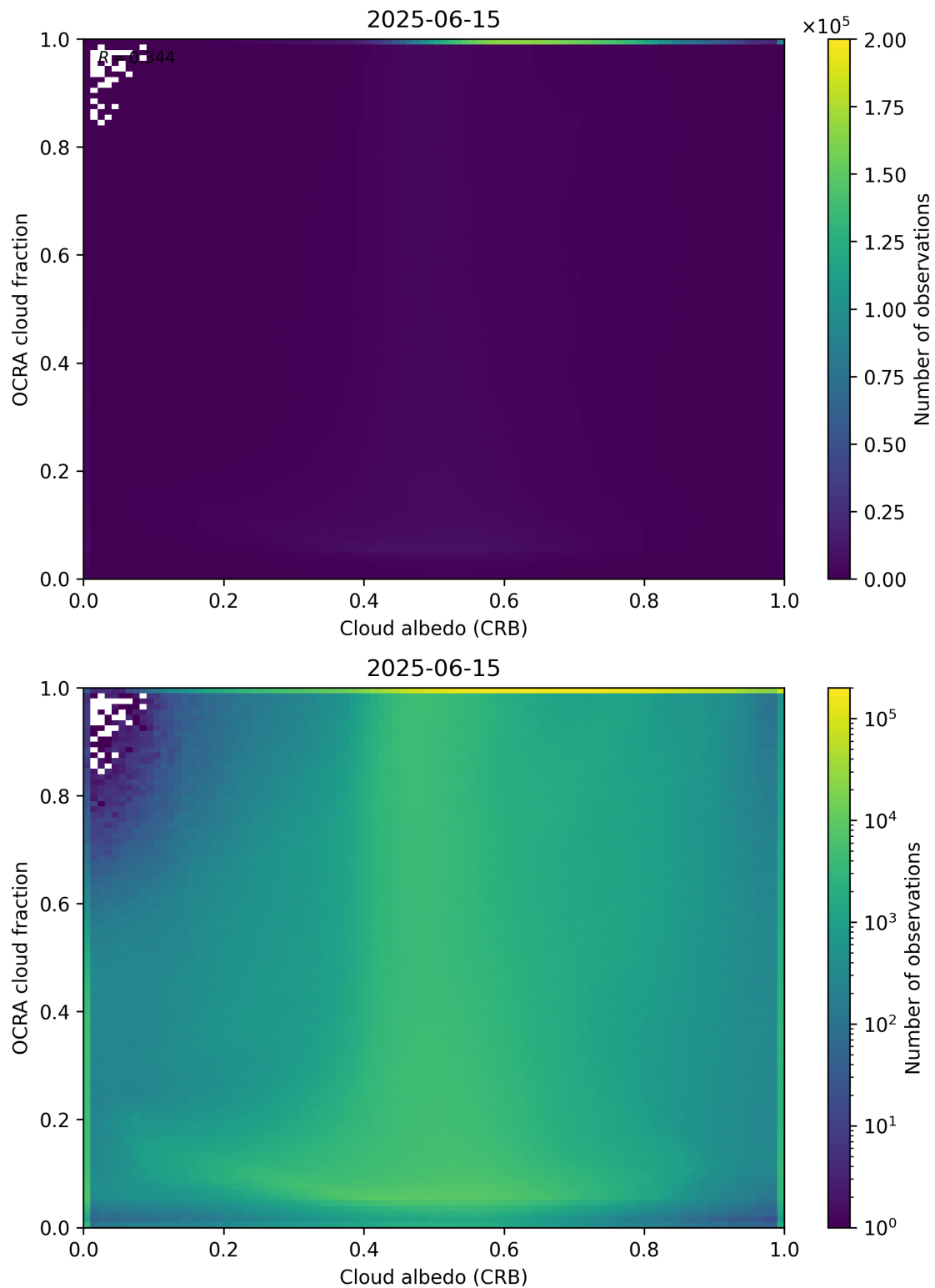
Figure 70: Scatter density plot of “Cloud albedo (CRB)” against “OCRA cloud fraction” for 2025-06-14 to 2025-06-16.
