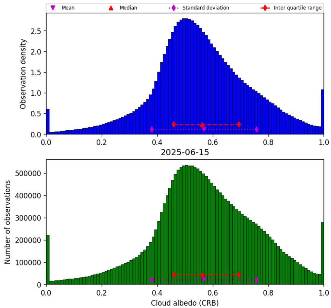
Figure 44: Histogram of “Cloud albedo (CRB)” for 2025-06-14 to 2025-06-16
