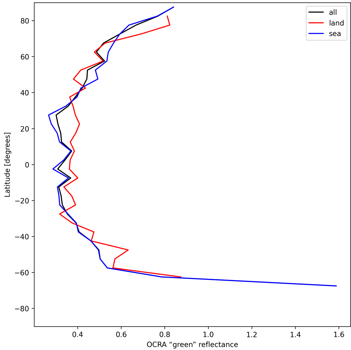
Figure 36: Zonal average of “OCRA “green” reflectance” for 2025-06-14 to 2025-06-16.
