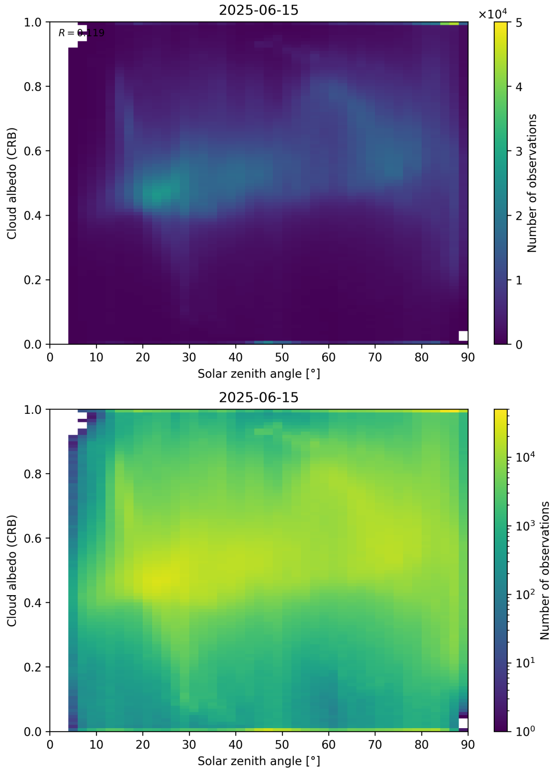
Figure 98: Scatter density plot of “Solar zenith angle” against “Cloud albedo (CRB)” for 2025-06-14 to 2025-06-16.
