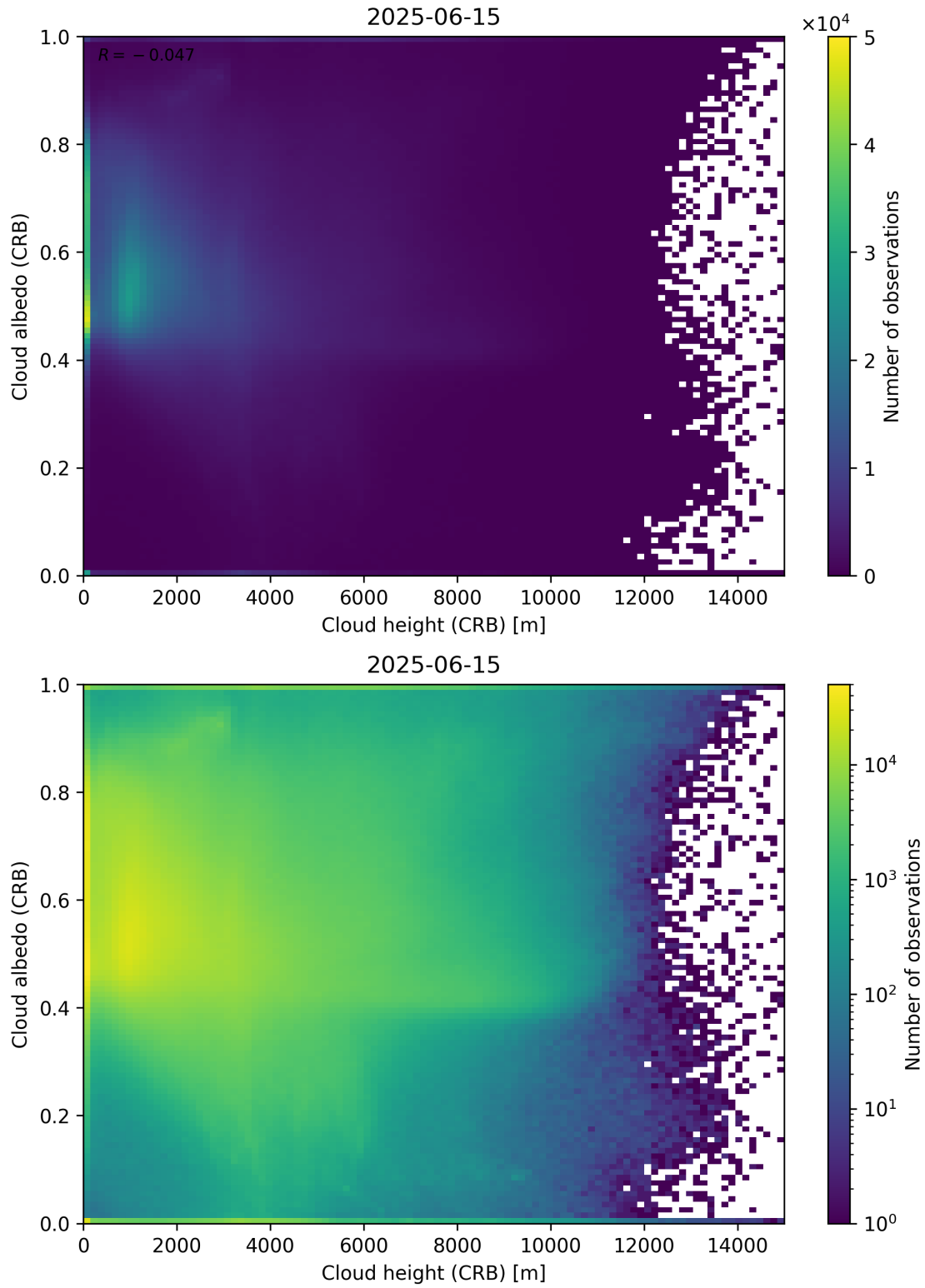
Figure 80: Scatter density plot of “Cloud height (CRB)” against “Cloud albedo (CRB)” for 2025-06-14 to 2025-06-16.
