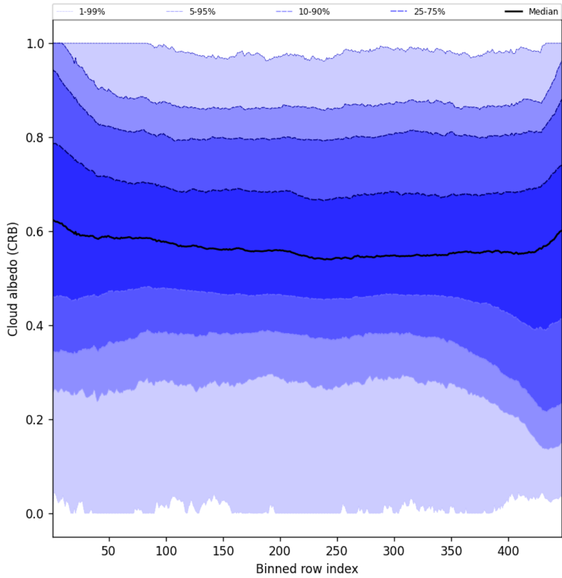
Figure 60: Along track statistics of “Cloud albedo (CRB)” for 2025-06-14 to 2025-06-16
