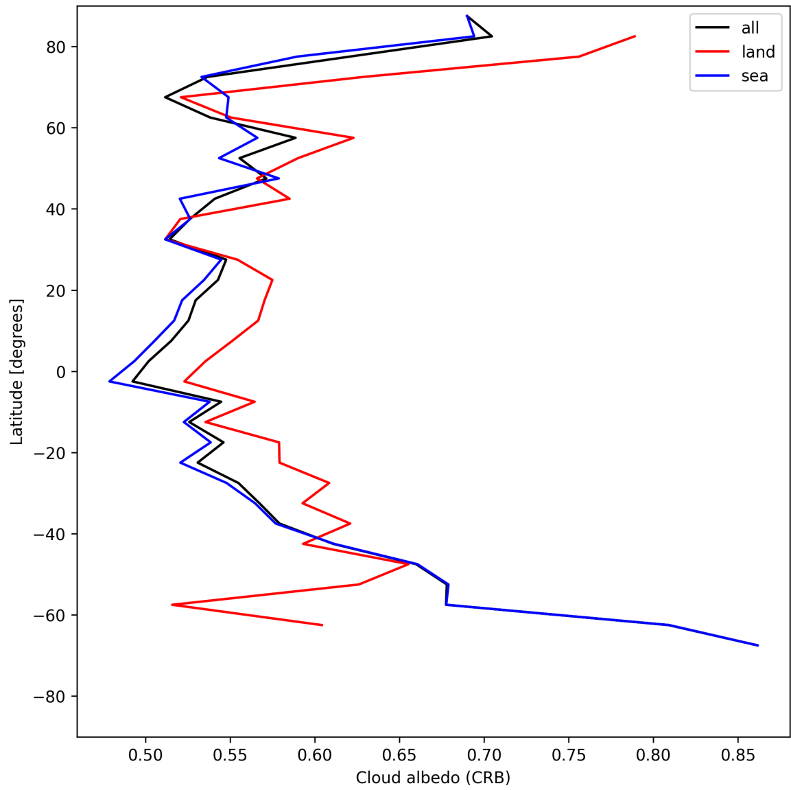
Figure 28: Zonal average of “Cloud albedo (CRB)” for 2025-06-14 to 2025-06-16.
