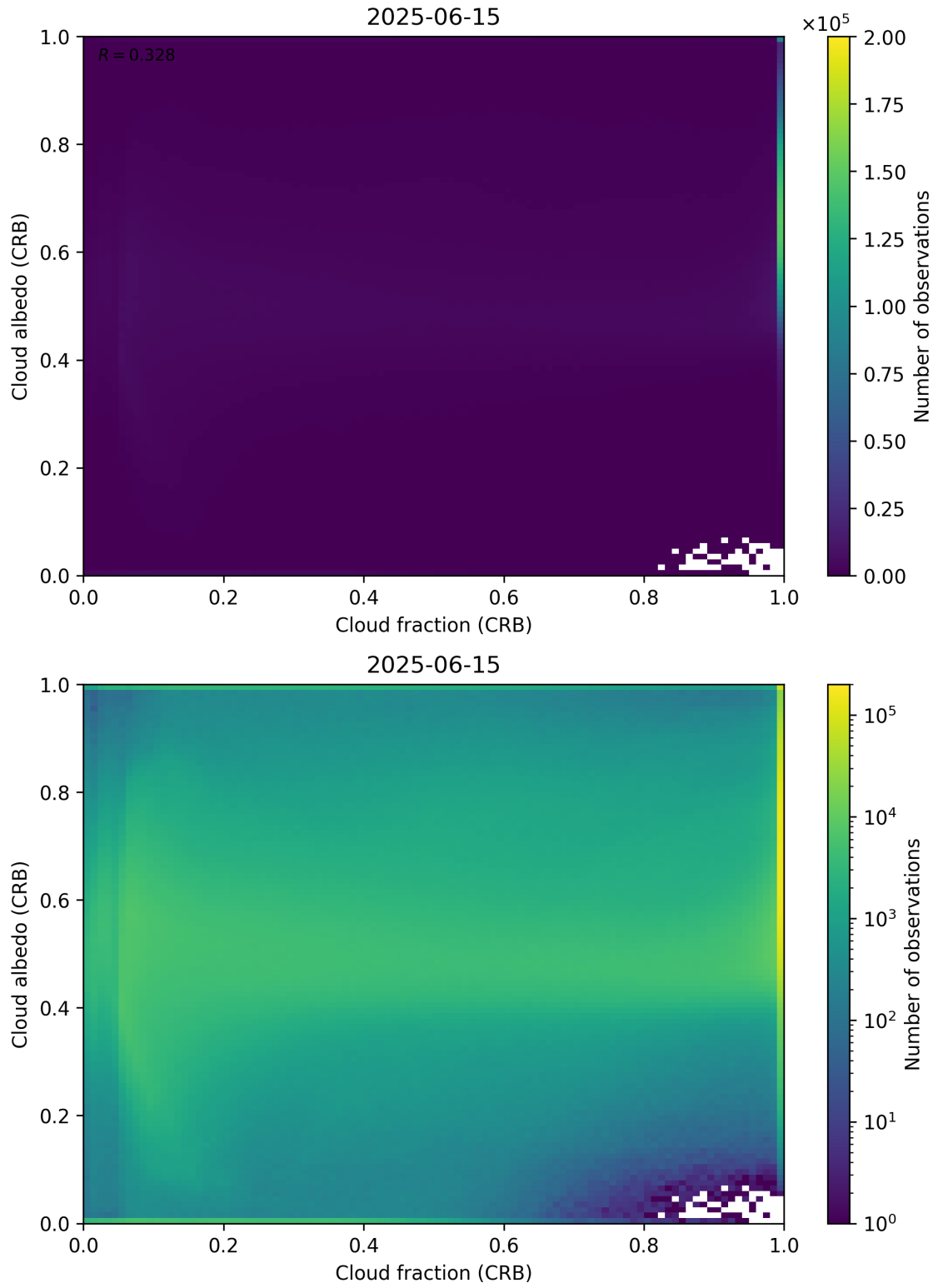
Figure 77: Scatter density plot of “Cloud fraction (CRB)” against “Cloud albedo (CRB)” for 2025-06-14 to 2025-06-16.
