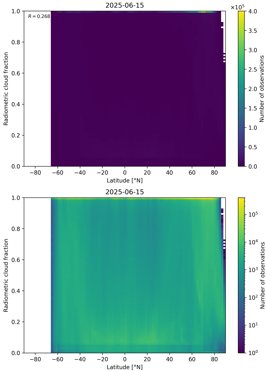
Figure 92: Scatter density plot of “Latitude” against “Radiometric cloud fraction” for 2025-06-14 to 2025-06-16.
