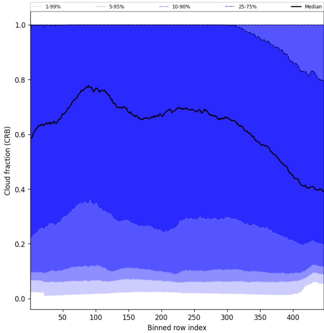
Figure 58: Along track statistics of “Cloud fraction (CRB)” for 2025-06-14 to 2025-06-16
