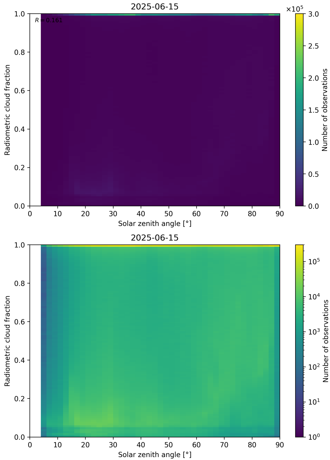
Figure 99: Scatter density plot of “Solar zenith angle” against “Radiometric cloud fraction” for 2025-06-14 to 2025-06-16.
