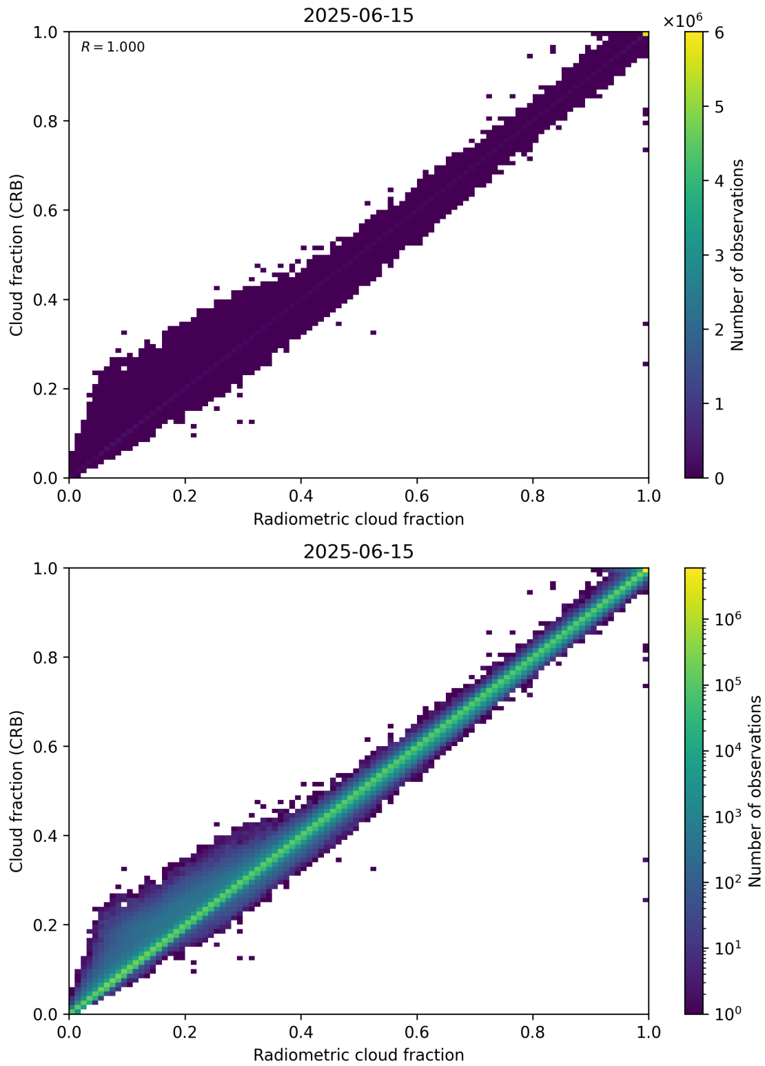
Figure 73: Scatter density plot of “Radiometric cloud fraction” against “Cloud fraction (CRB)” for 2025-06-14 to 2025-06-16.
