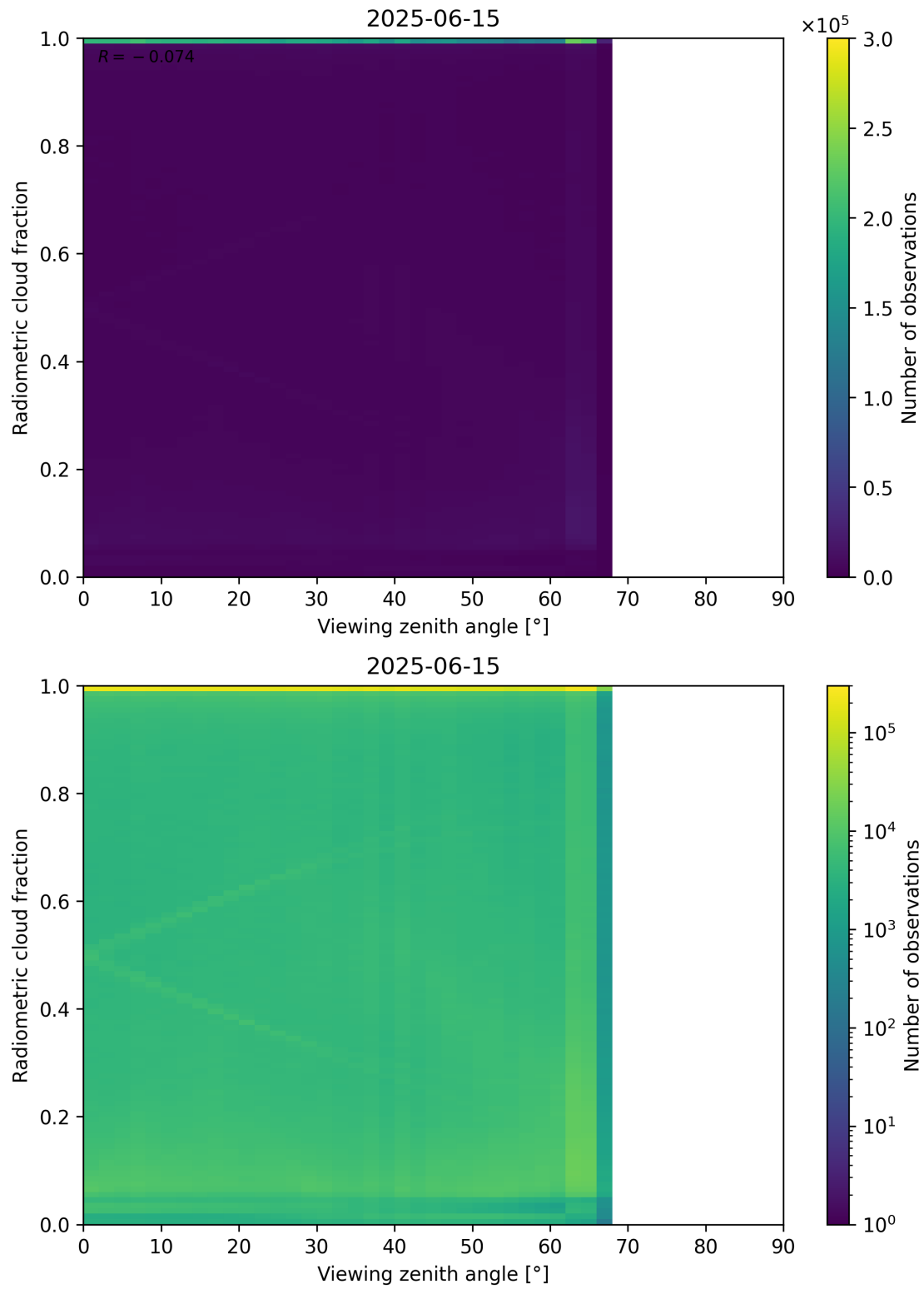
Figure 107: Scatter density plot of “Viewing zenith angle” against “Radiometric cloud fraction” for 2025-06-14 to 2025-06-16.
