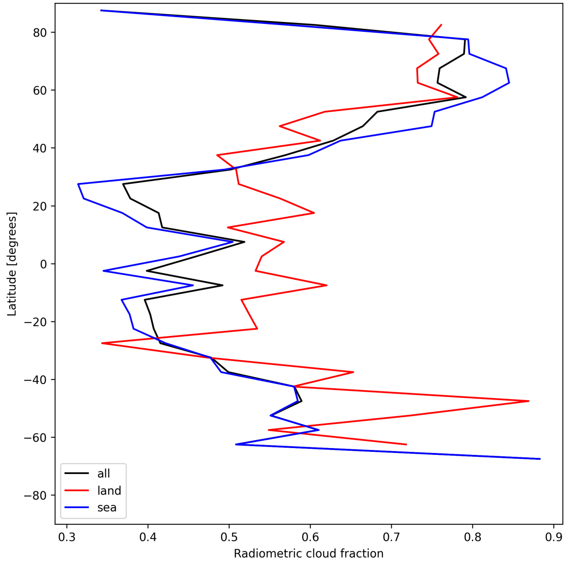
Figure 23: Zonal average of “Radiometric cloud fraction” for 2025-06-14 to 2025-06-16.
