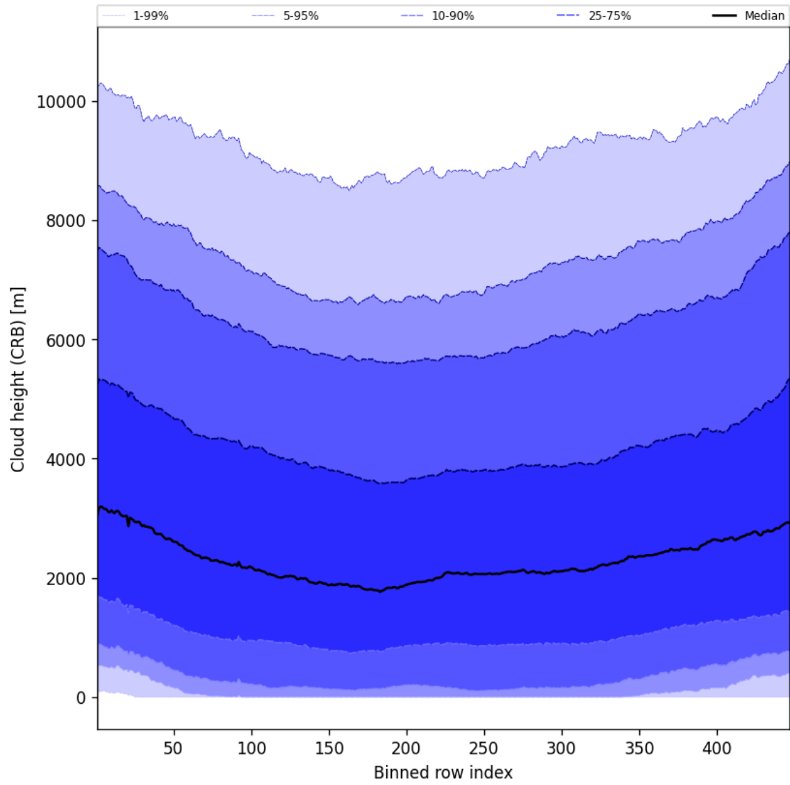
Figure 59: Along track statistics of “Cloud height (CRB)” for 2025-06-14 to 2025-06-16
