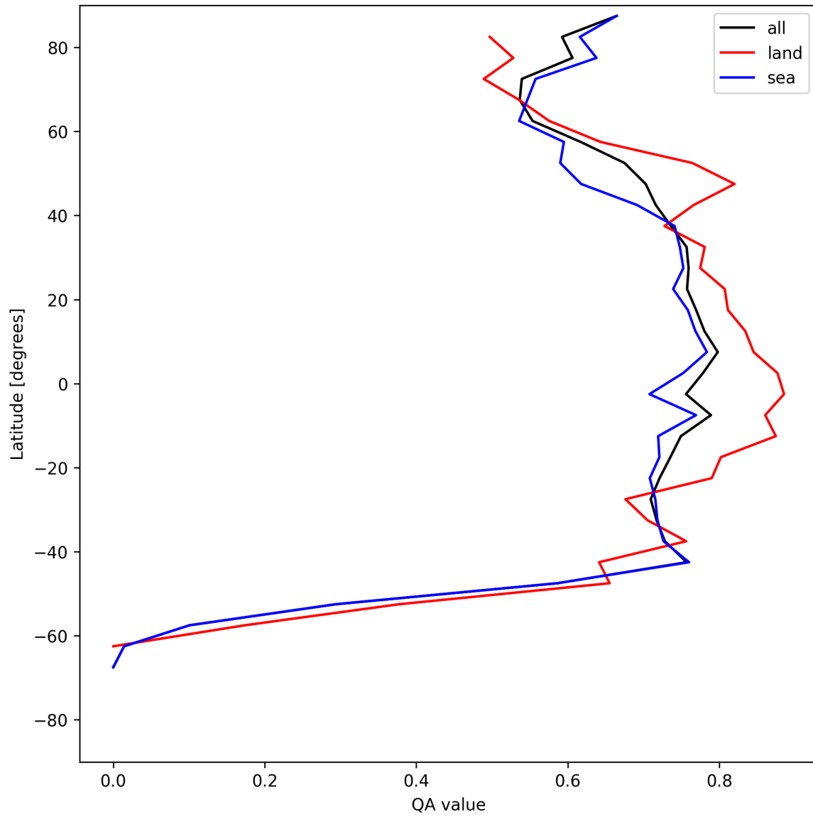
Figure 22: Zonal average of “QA value” for 2025-06-14 to 2025-06-16.
