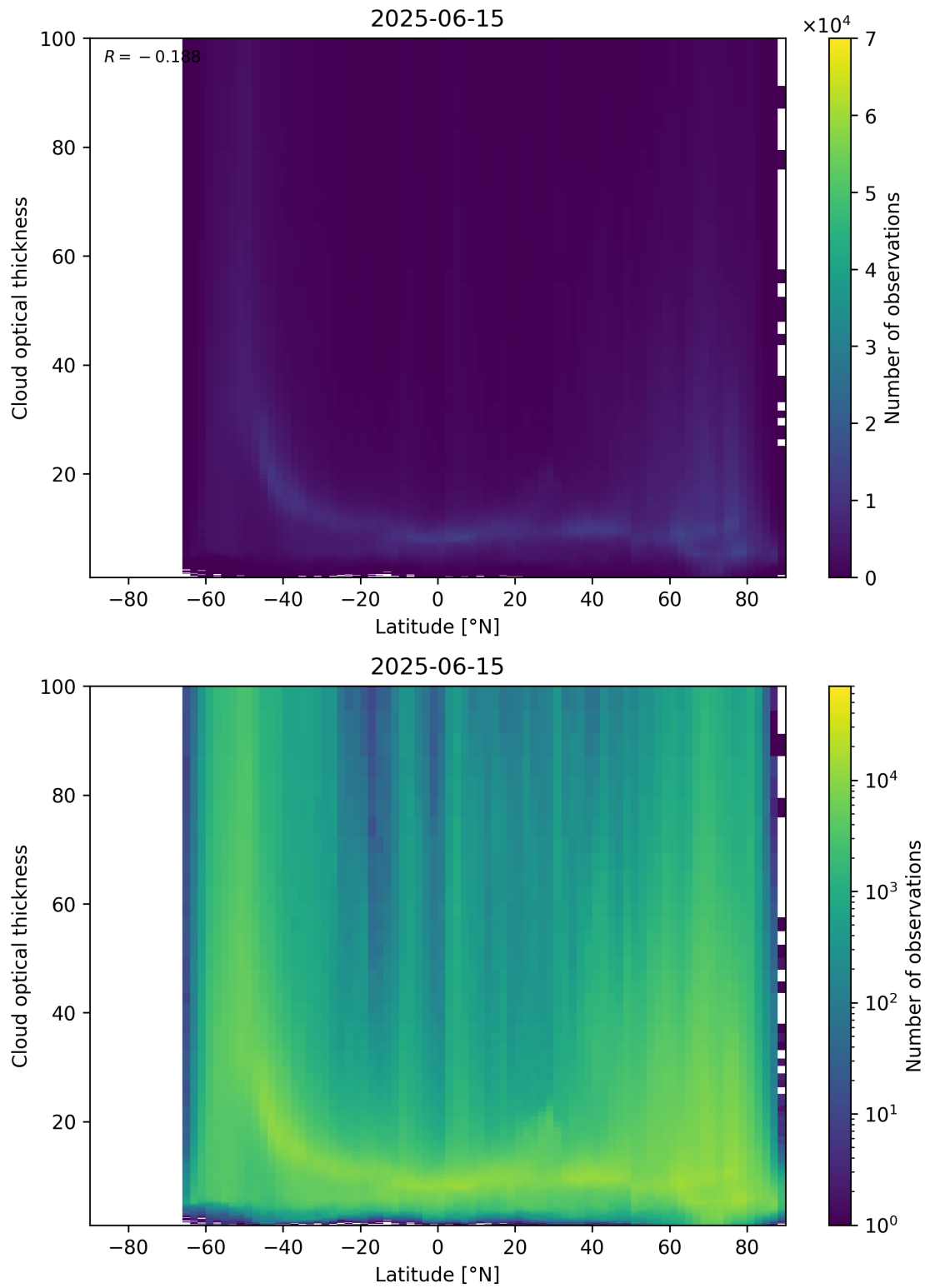
Figure 96: Scatter density plot of “Latitude” against “Cloud optical thickness” for 2025-06-14 to 2025-06-16.
