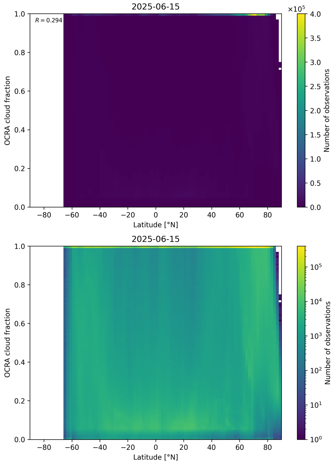
Figure 93: Scatter density plot of “Latitude” against “OCRA cloud fraction” for 2025-06-14 to 2025-06-16.
