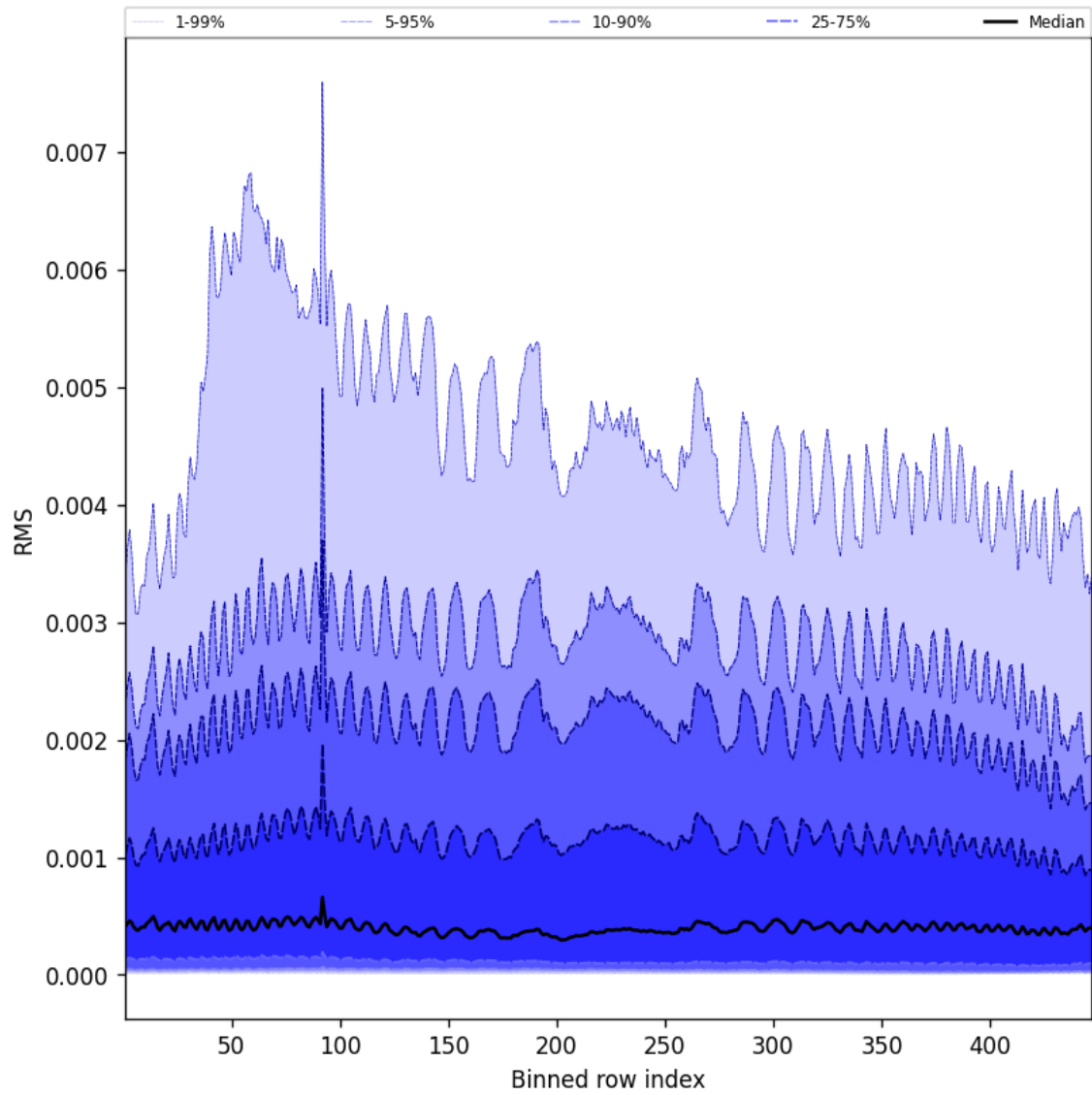
Figure 63: Along track statistics of “RMS” for 2025-06-14 to 2025-06-16
