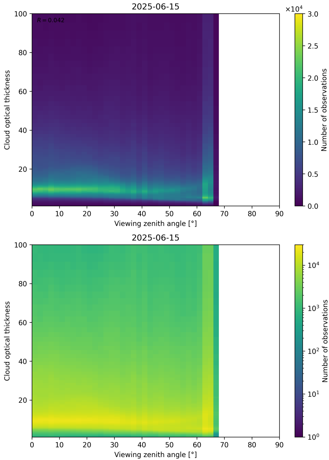
Figure 111: Scatter density plot of “Viewing zenith angle” against “Cloud optical thickness” for 2025-06-14 to 2025-06-16.
