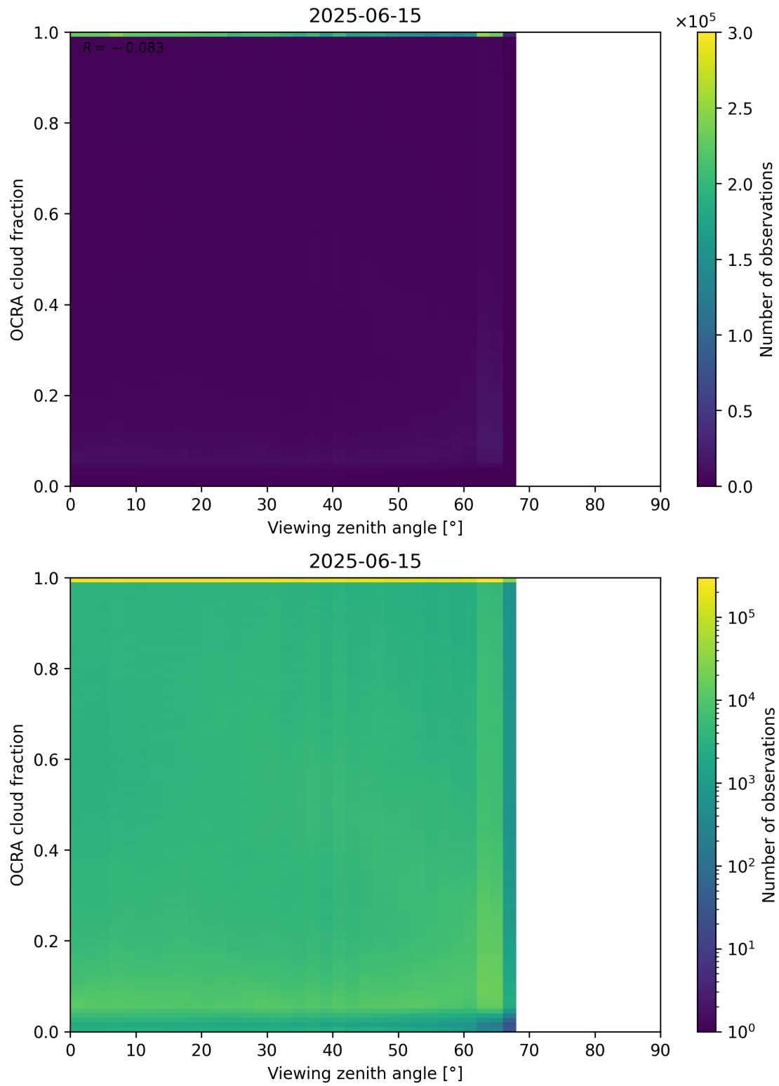
Figure 108: Scatter density plot of “Viewing zenith angle” against “OCRA cloud fraction” for 2025-06-14 to 2025-06-16.
