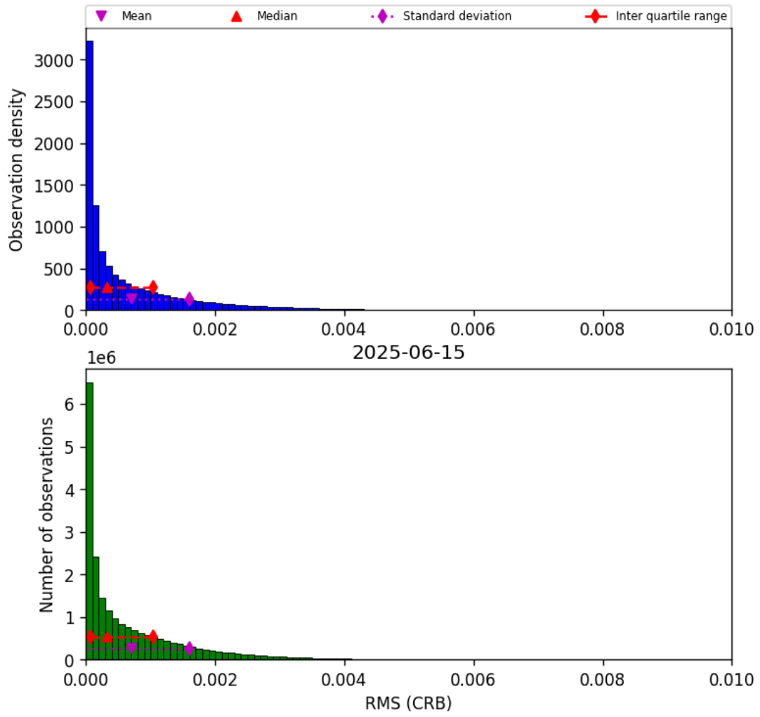
Figure 48: Histogram of “RMS (CRB)” for 2025-06-14 to 2025-06-16
