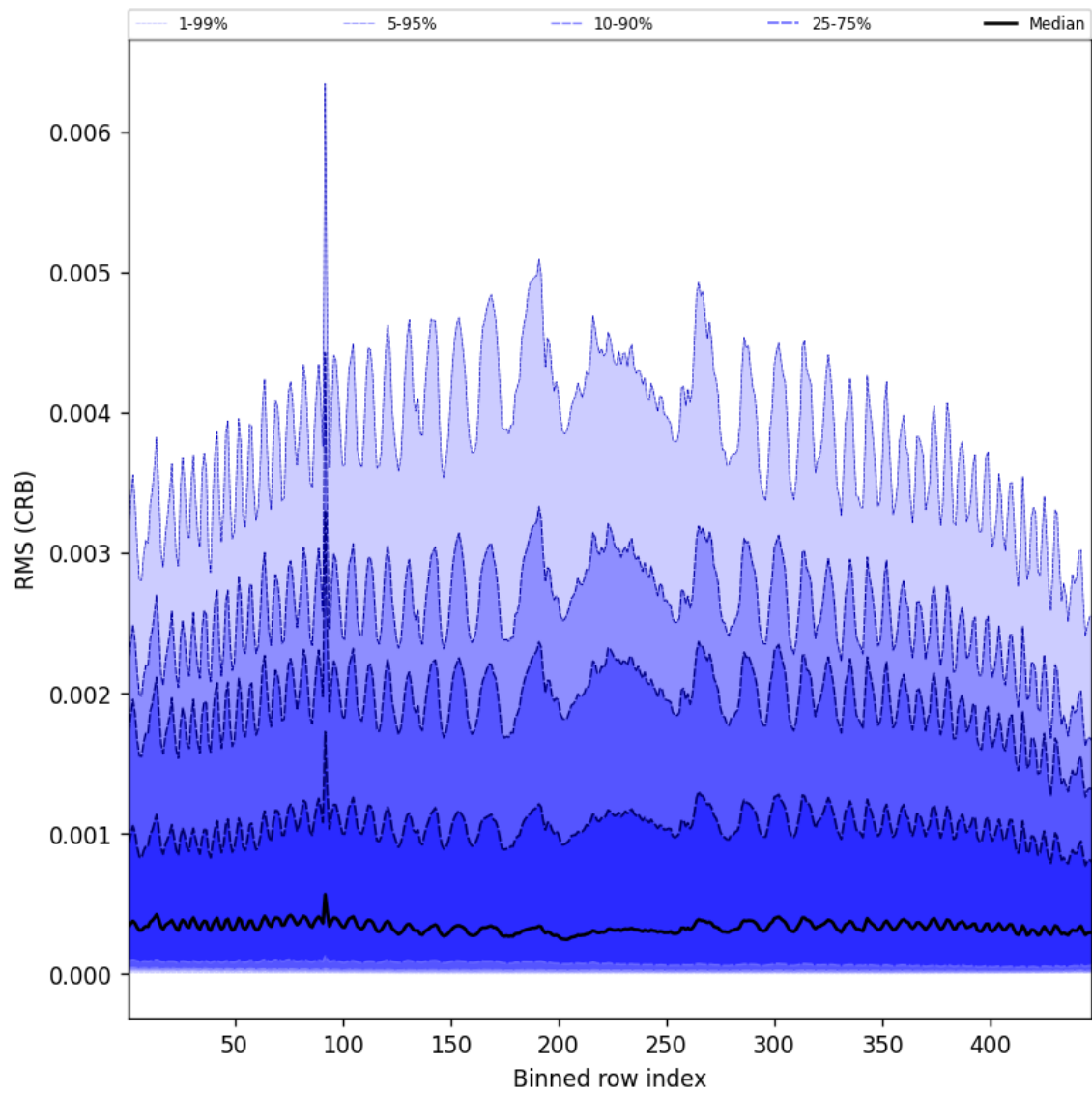
Figure 64: Along track statistics of “RMS (CRB)” for 2025-06-14 to 2025-06-16
