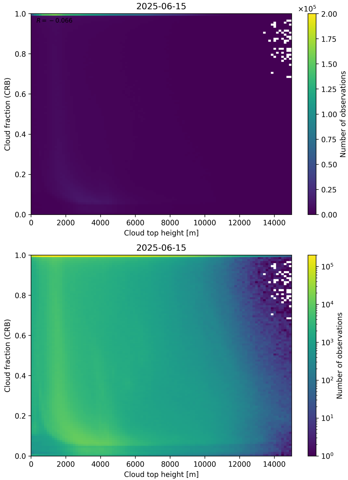
Figure 88: Scatter density plot of “Cloud top height” against “Cloud fraction (CRB)” for 2025-06-14 to 2025-06-16.
