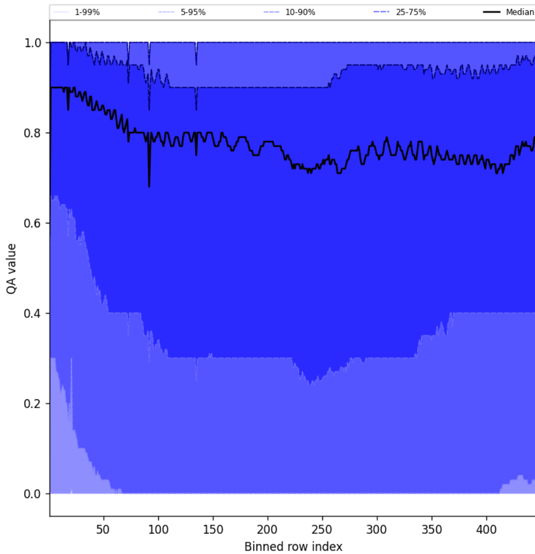
Figure 54: Along track statistics of “QA value” for 2025-06-14 to 2025-06-16
