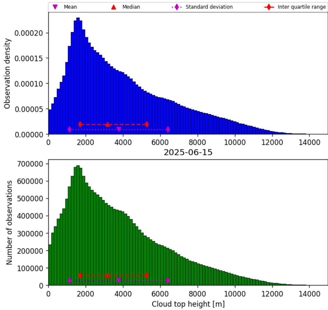
Figure 40: Histogram of “Cloud top height” for 2025-06-14 to 2025-06-16
