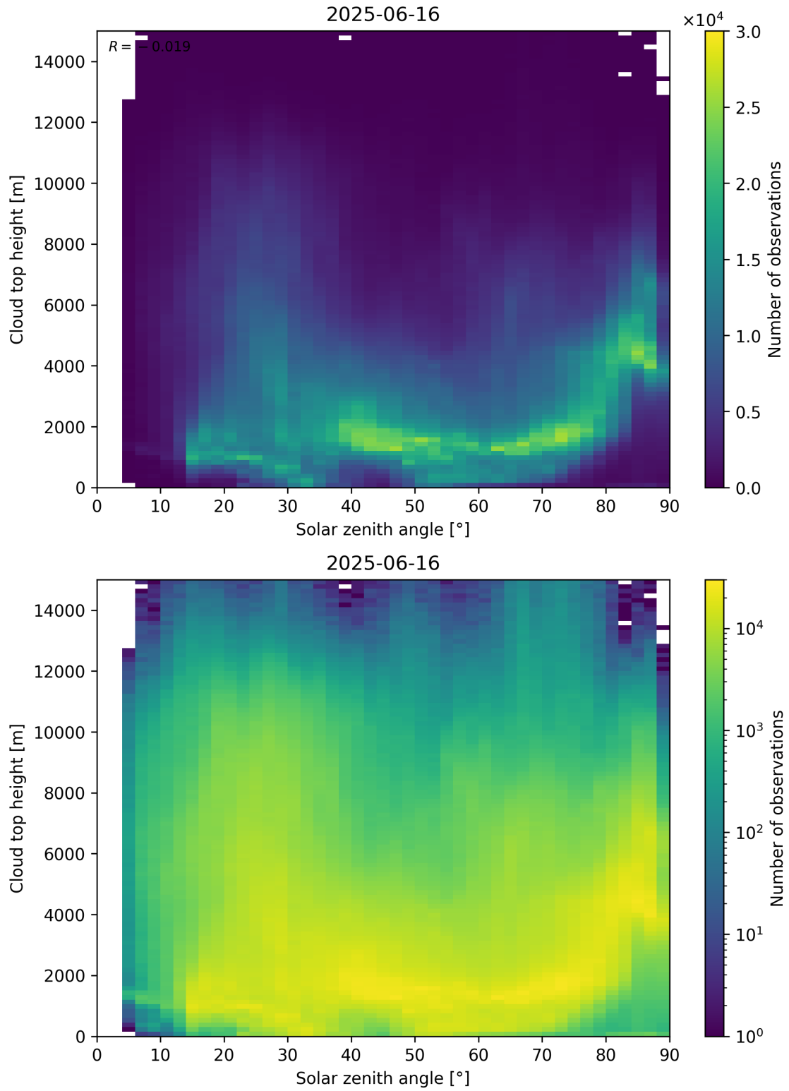
Figure 104: Scatter density plot of “Solar zenith angle” against “Cloud top height” for 2025-06-16 to 2025-06-17.
