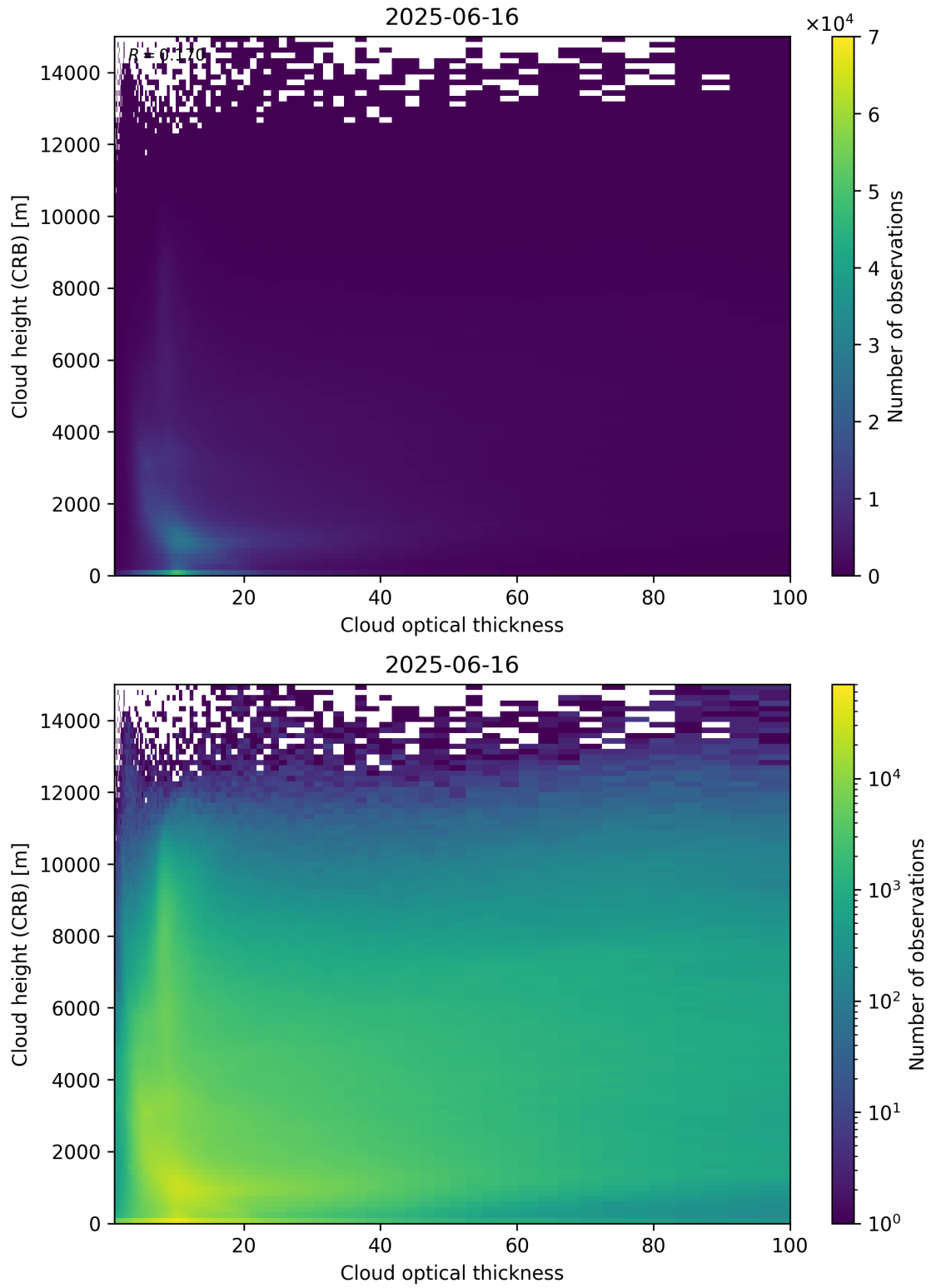
Figure 85: Scatter density plot of “Cloud optical thickness” against “Cloud height (CRB)” for 2025-06-16 to 2025-06-17.
