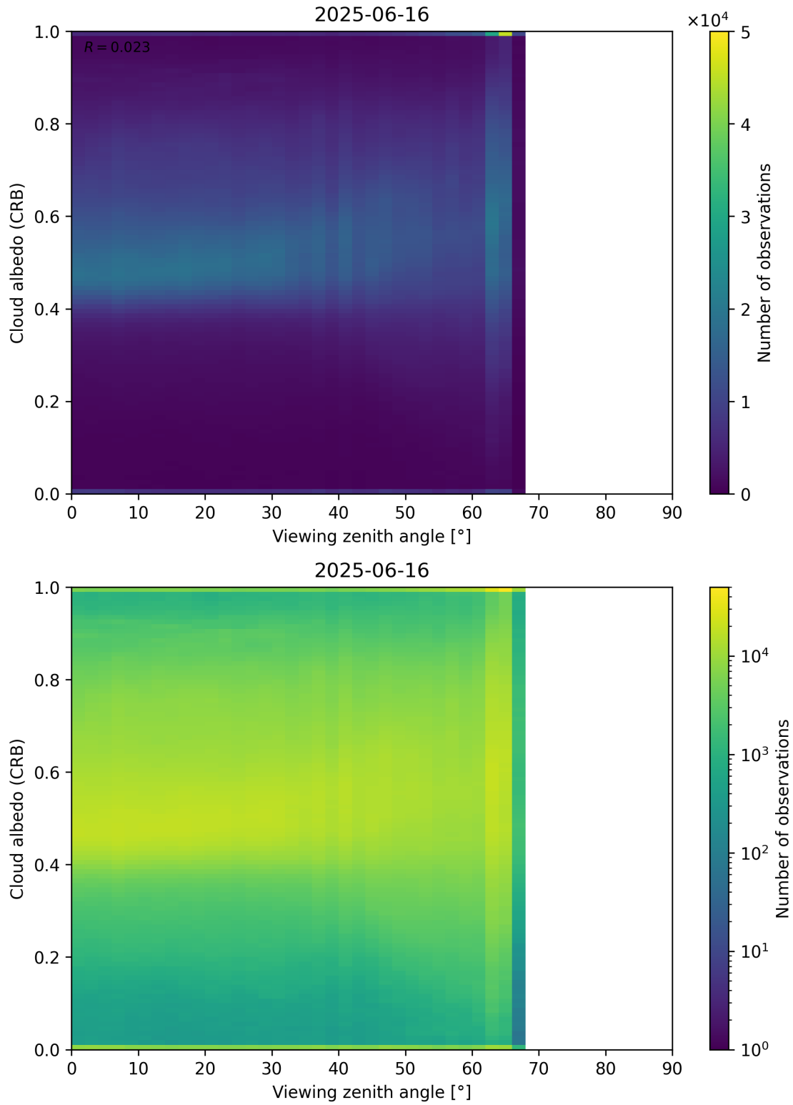
Figure 106: Scatter density plot of “Viewing zenith angle” against “Cloud albedo (CRB)” for 2025-06-16 to 2025-06-17.
