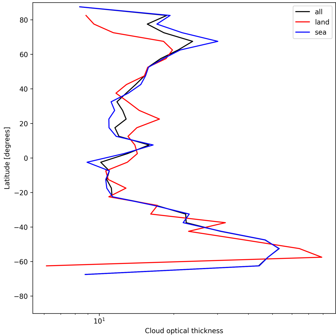
Figure 25: Zonal average of “Cloud optical thickness” for 2025-06-16 to 2025-06-17.
