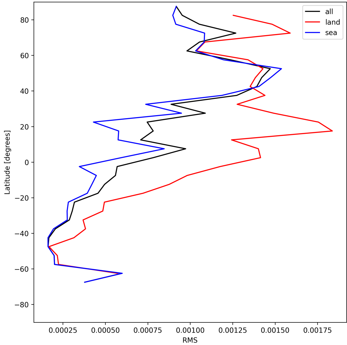
Figure 31: Zonal average of “RMS” for 2025-06-16 to 2025-06-17.
