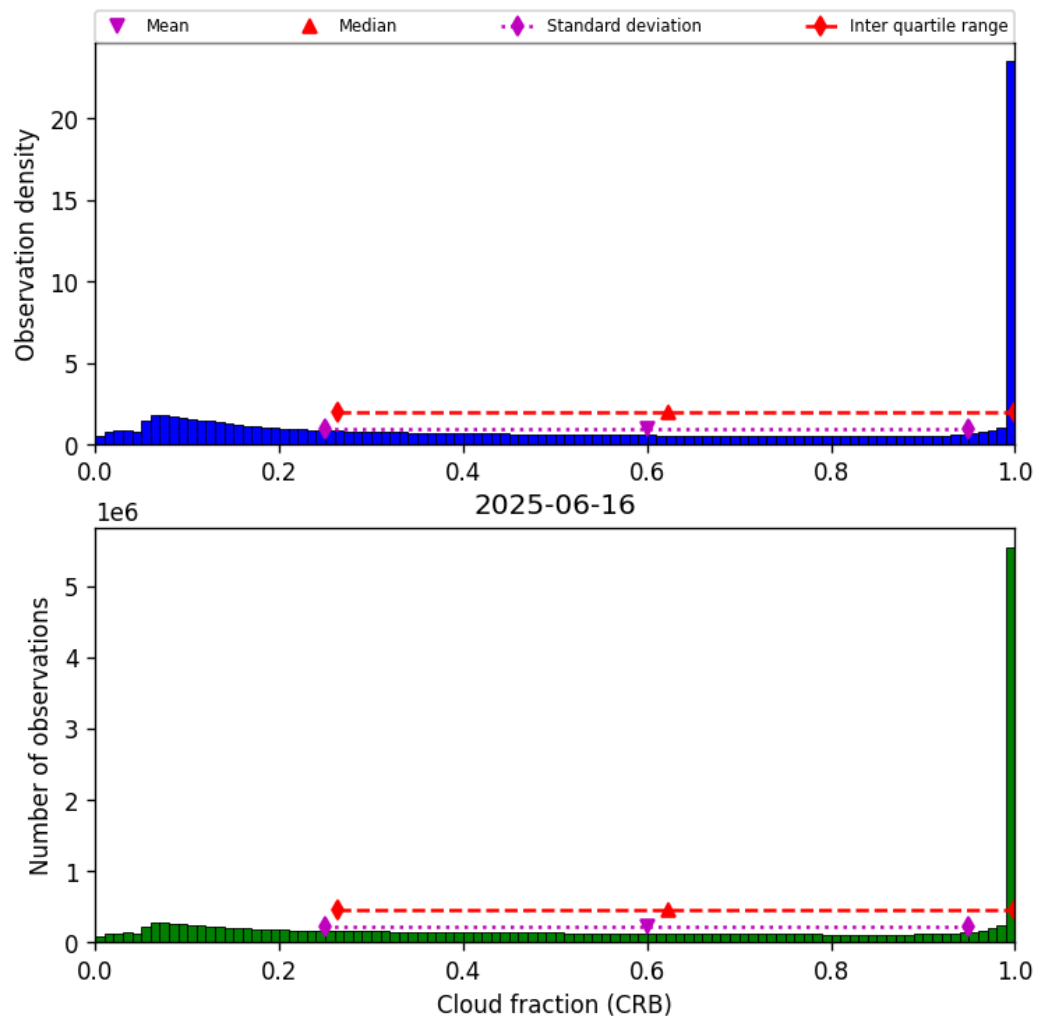
Figure 42: Histogram of “Cloud fraction (CRB)” for 2025-06-16 to 2025-06-17
