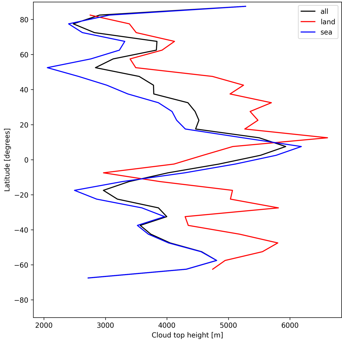
Figure 24: Zonal average of “Cloud top height” for 2025-06-16 to 2025-06-17.
