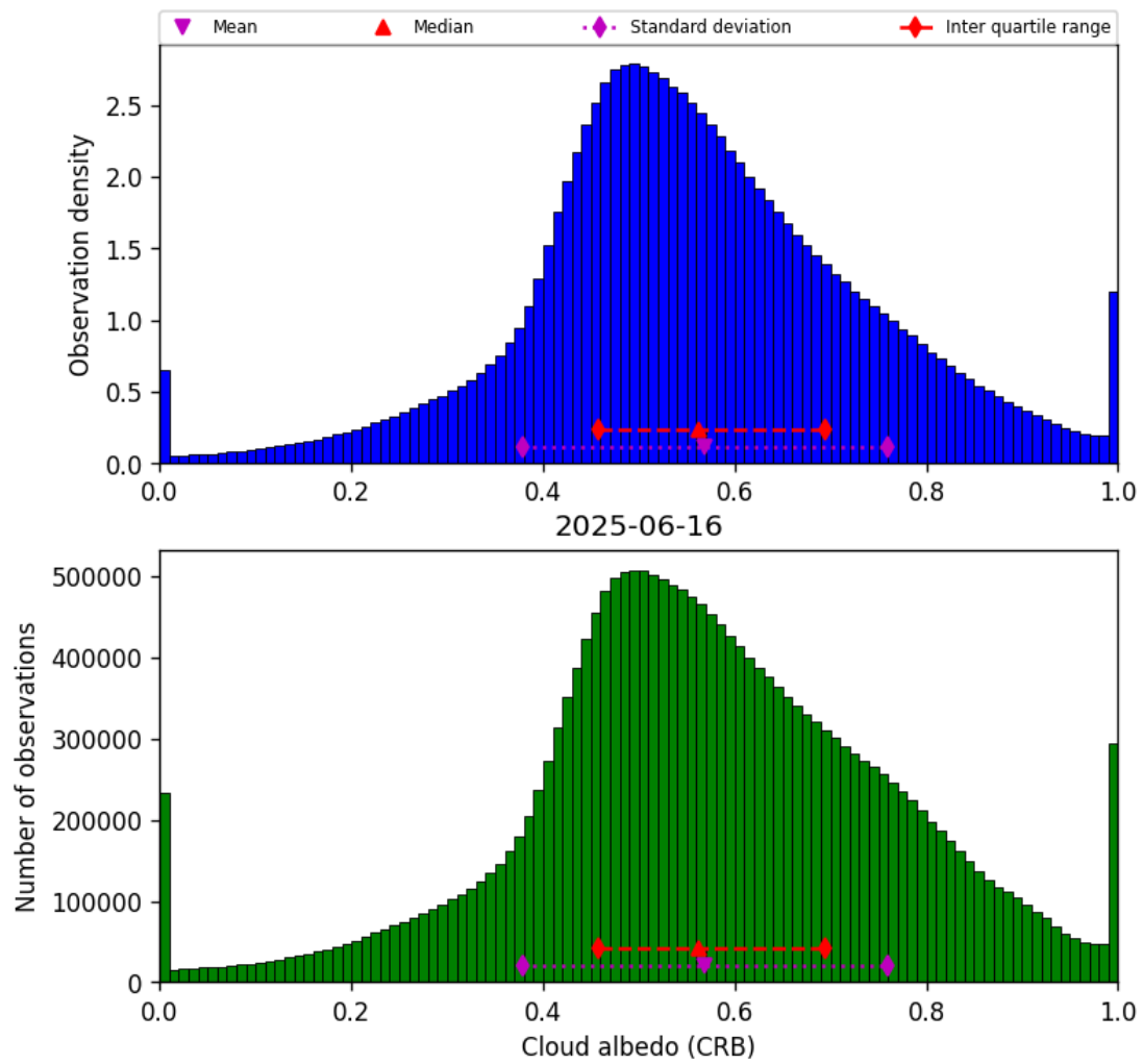
Figure 44: Histogram of “Cloud albedo (CRB)” for 2025-06-16 to 2025-06-17
