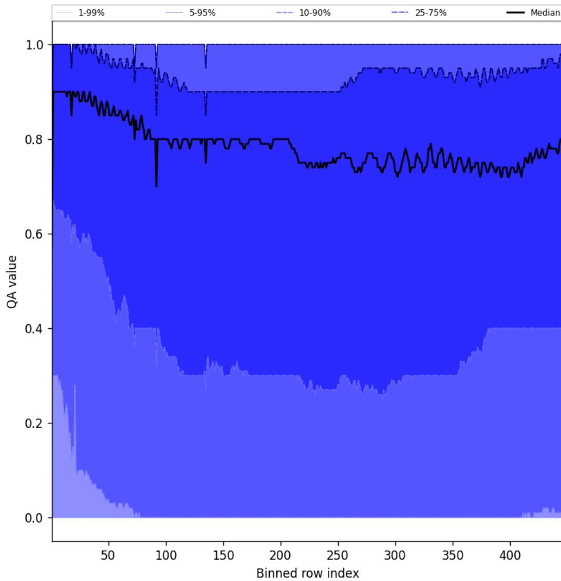
Figure 54: Along track statistics of “QA value” for 2025-06-16 to 2025-06-17
