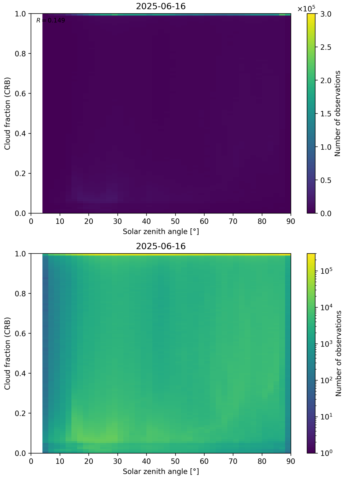
Figure 101: Scatter density plot of “Solar zenith angle” against “Cloud fraction (CRB)” for 2025-06-16 to 2025-06-17.
