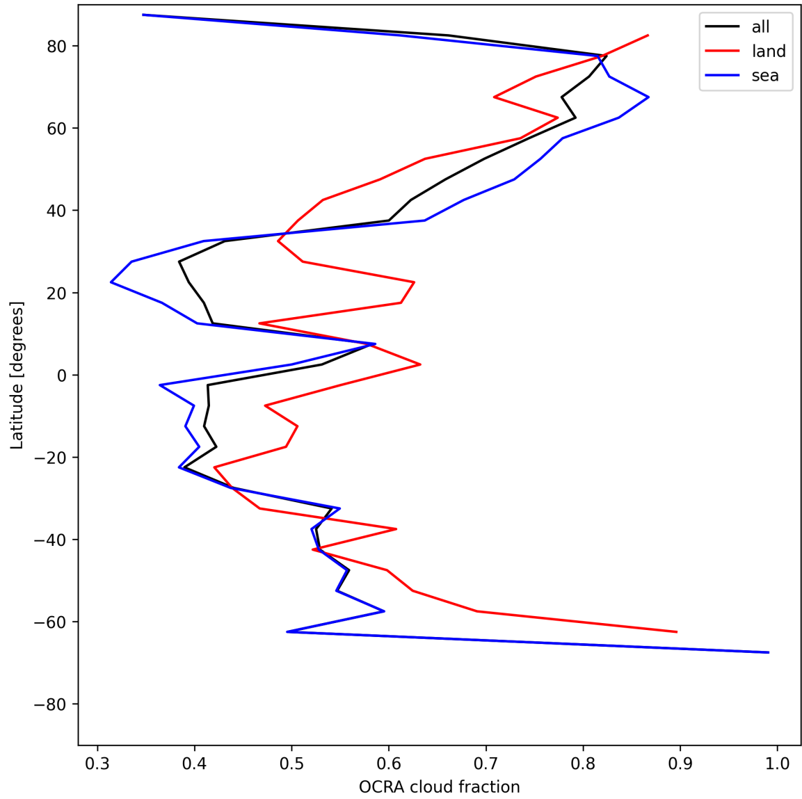
Figure 34: Zonal average of “OCRA cloud fraction” for 2025-06-16 to 2025-06-17.
