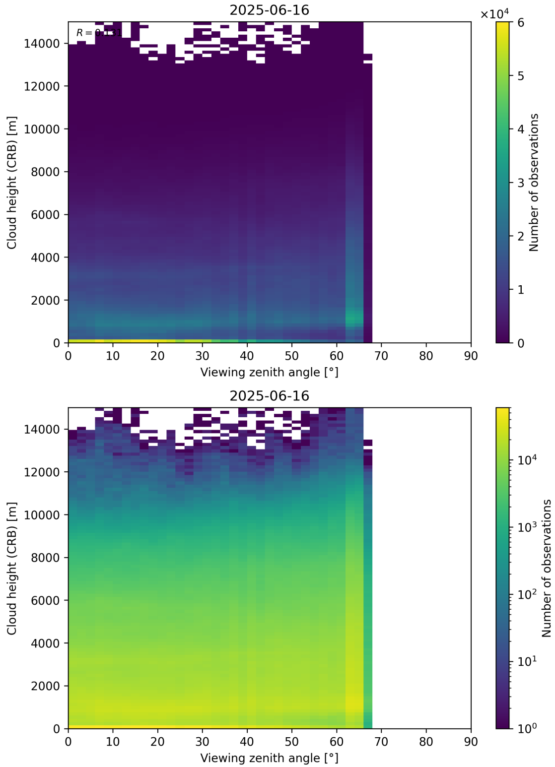
Figure 110: Scatter density plot of “Viewing zenith angle” against “Cloud height (CRB)” for 2025-06-16 to 2025-06-17.
