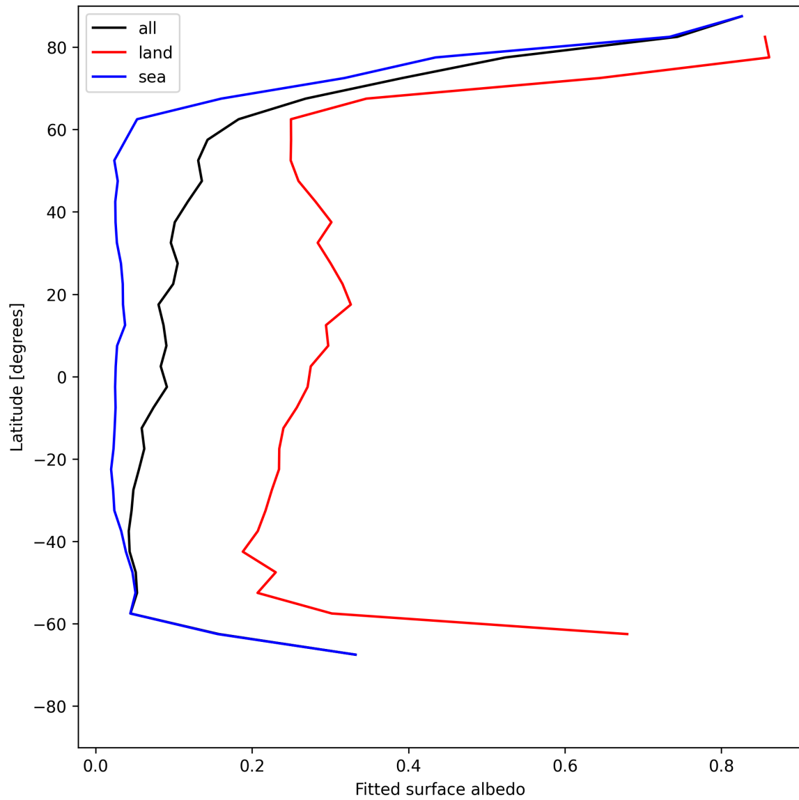
Figure 29: Zonal average of “Fitted surface albedo” for 2025-06-16 to 2025-06-17.
