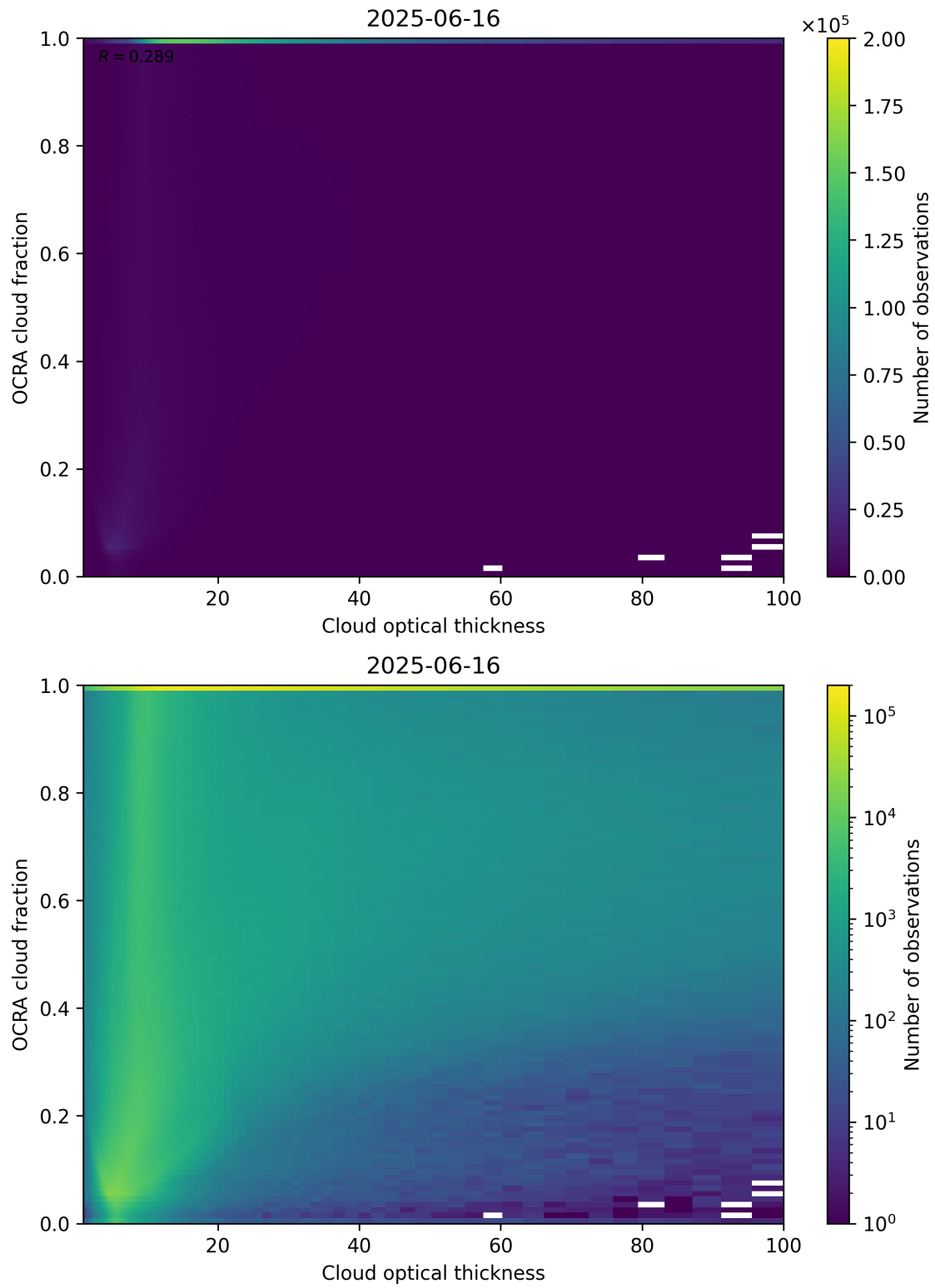
Figure 83: Scatter density plot of “Cloud optical thickness” against “OCRA cloud fraction” for 2025-06-16 to 2025-06-17.
