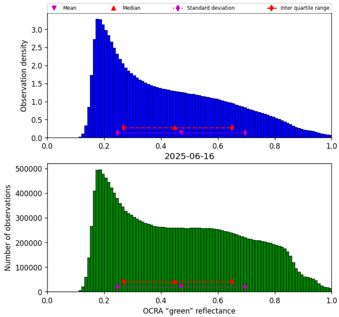
Figure 52: Histogram of “OCRA “green” reflectance” for 2025-06-16 to 2025-06-17
