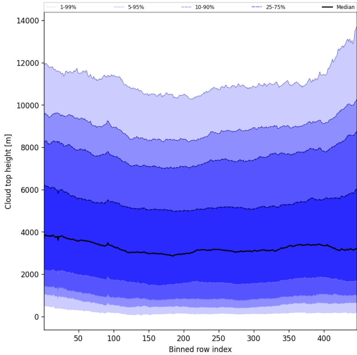
Figure 56: Along track statistics of “Cloud top height” for 2025-06-16 to 2025-06-17
