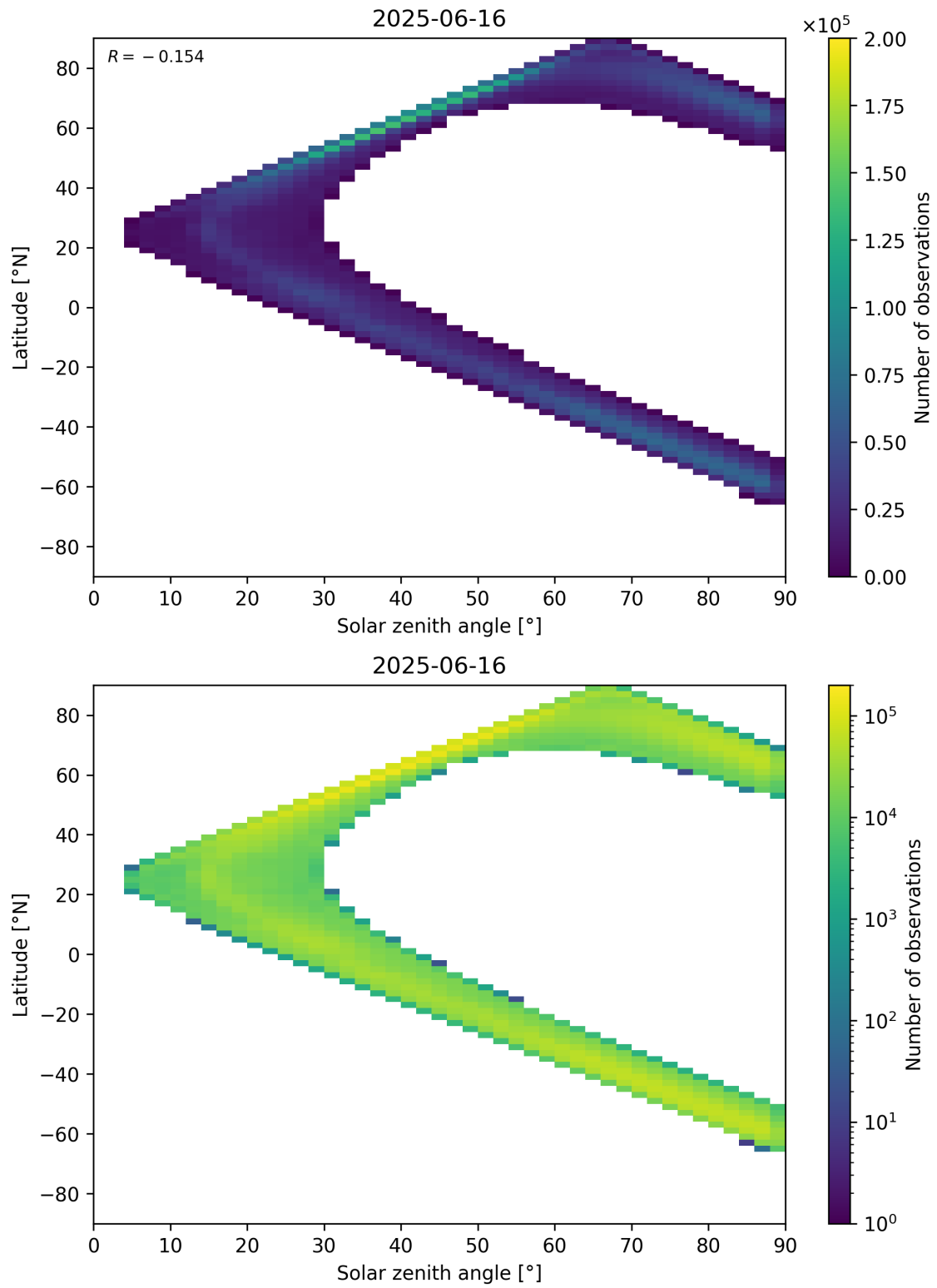
Figure 105: Scatter density plot of “Solar zenith angle” against “Latitude” for 2025-06-16 to 2025-06-17.
