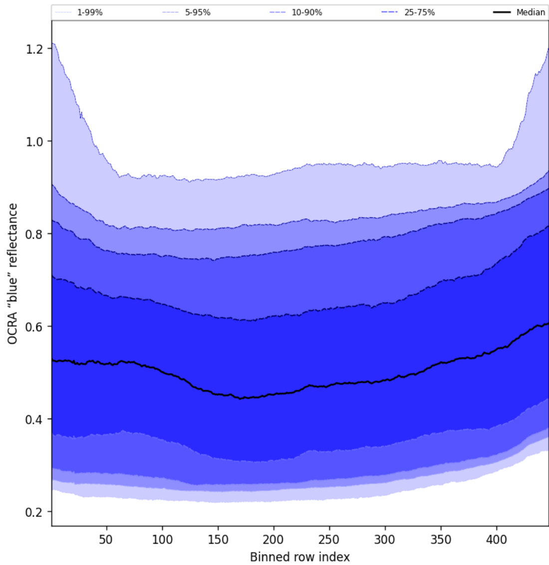
Figure 67: Along track statistics of “OCRA “blue” reflectance” for 2025-06-16 to 2025-06-17
