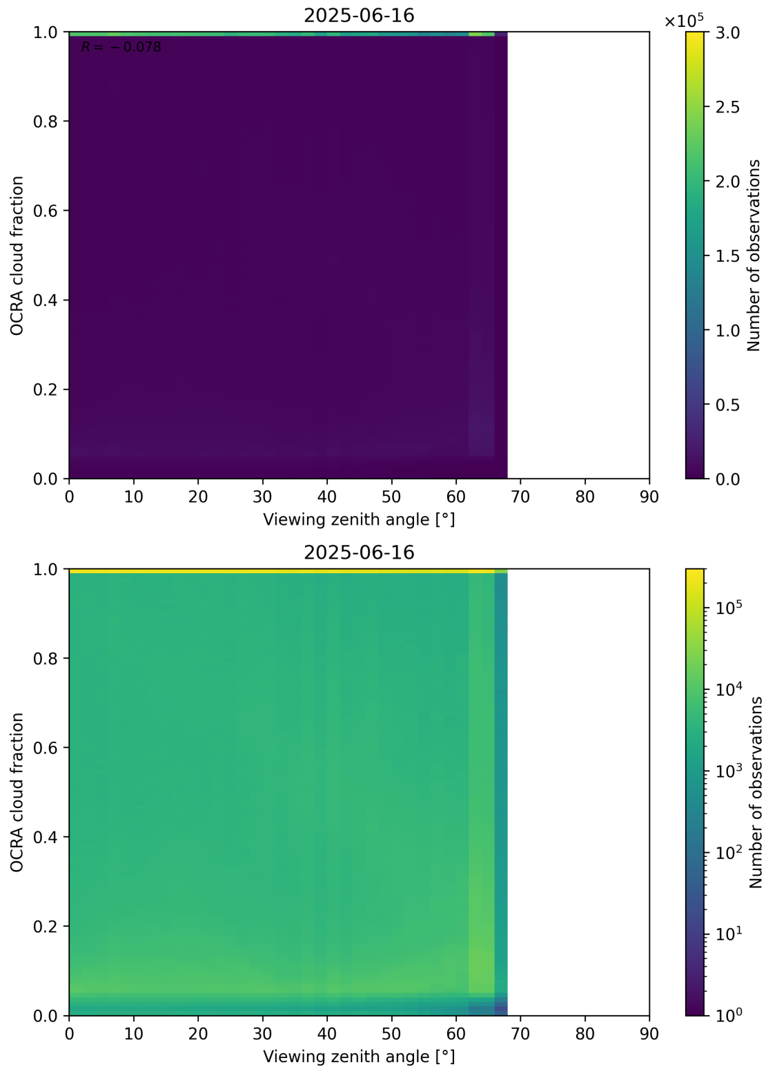
Figure 108: Scatter density plot of “Viewing zenith angle” against “OCRA cloud fraction” for 2025-06-16 to 2025-06-17.
