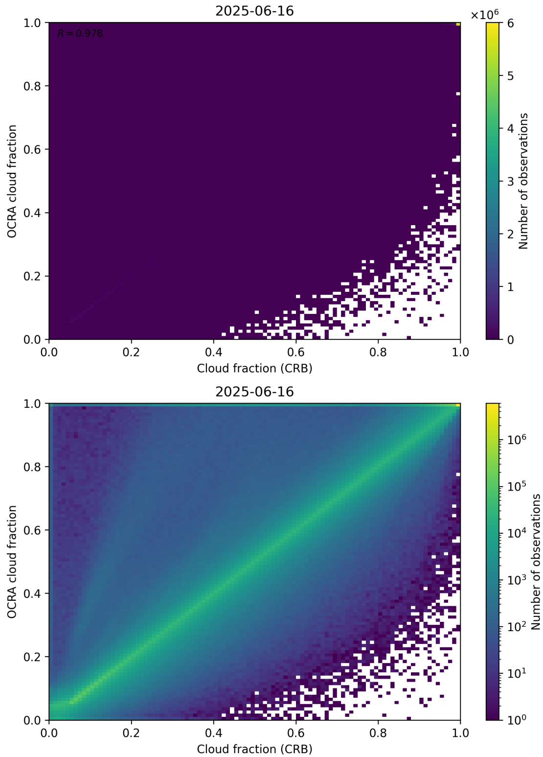
Figure 78: Scatter density plot of “Cloud fraction (CRB)” against “OCRA cloud fraction” for 2025-06-16 to 2025-06-17.
