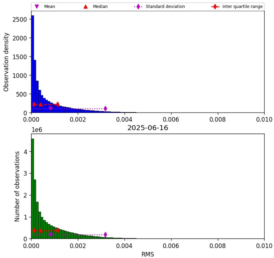
Figure 47: Histogram of “RMS” for 2025-06-16 to 2025-06-17
