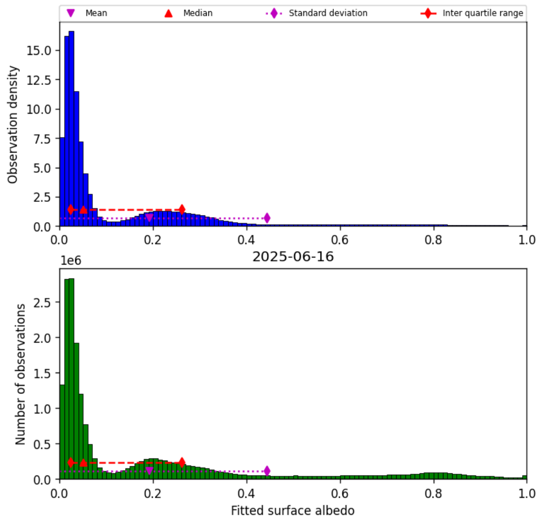
Figure 45: Histogram of “Fitted surface albedo” for 2025-06-16 to 2025-06-17
