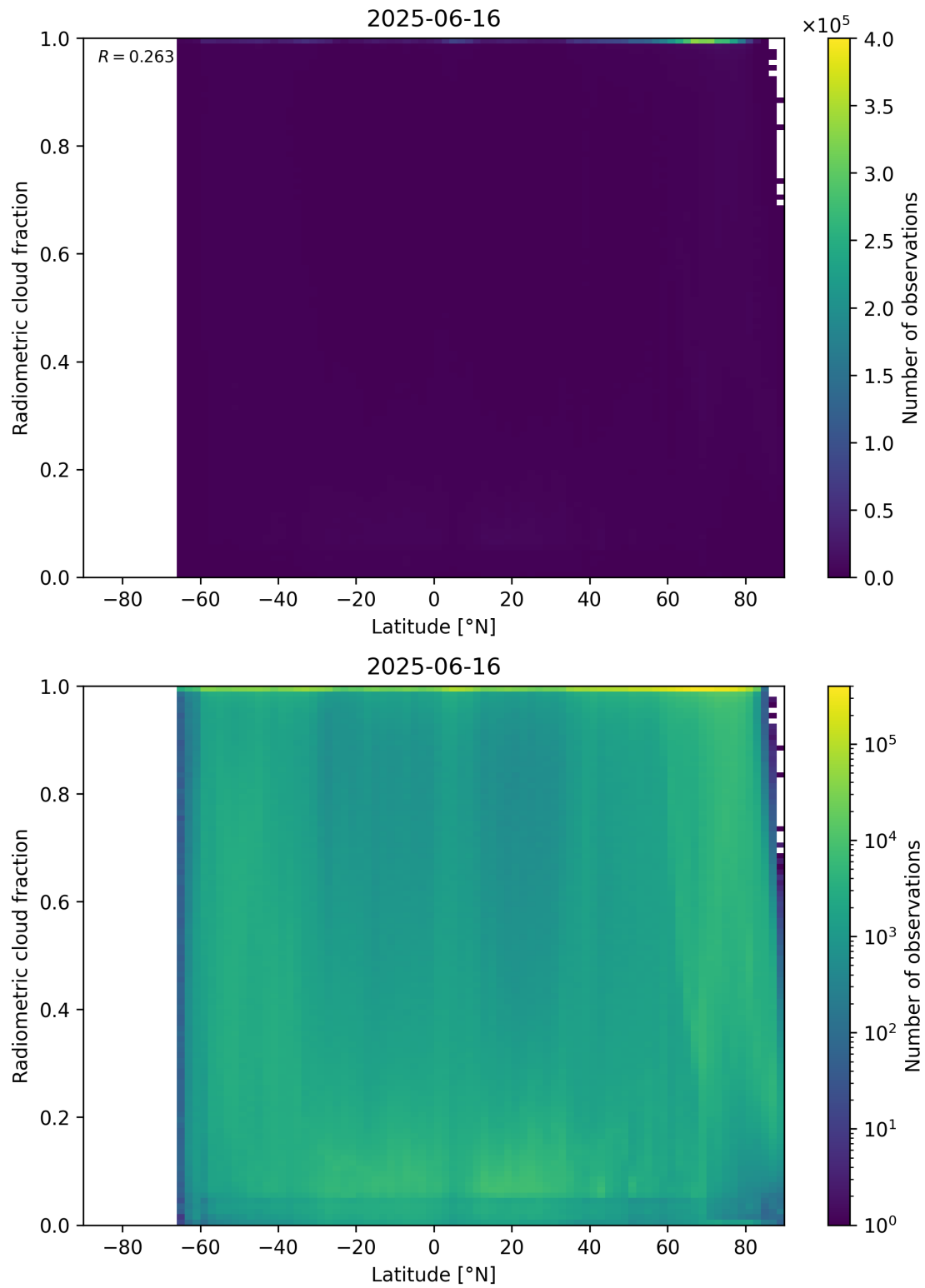
Figure 92: Scatter density plot of “Latitude” against “Radiometric cloud fraction” for 2025-06-16 to 2025-06-17.
