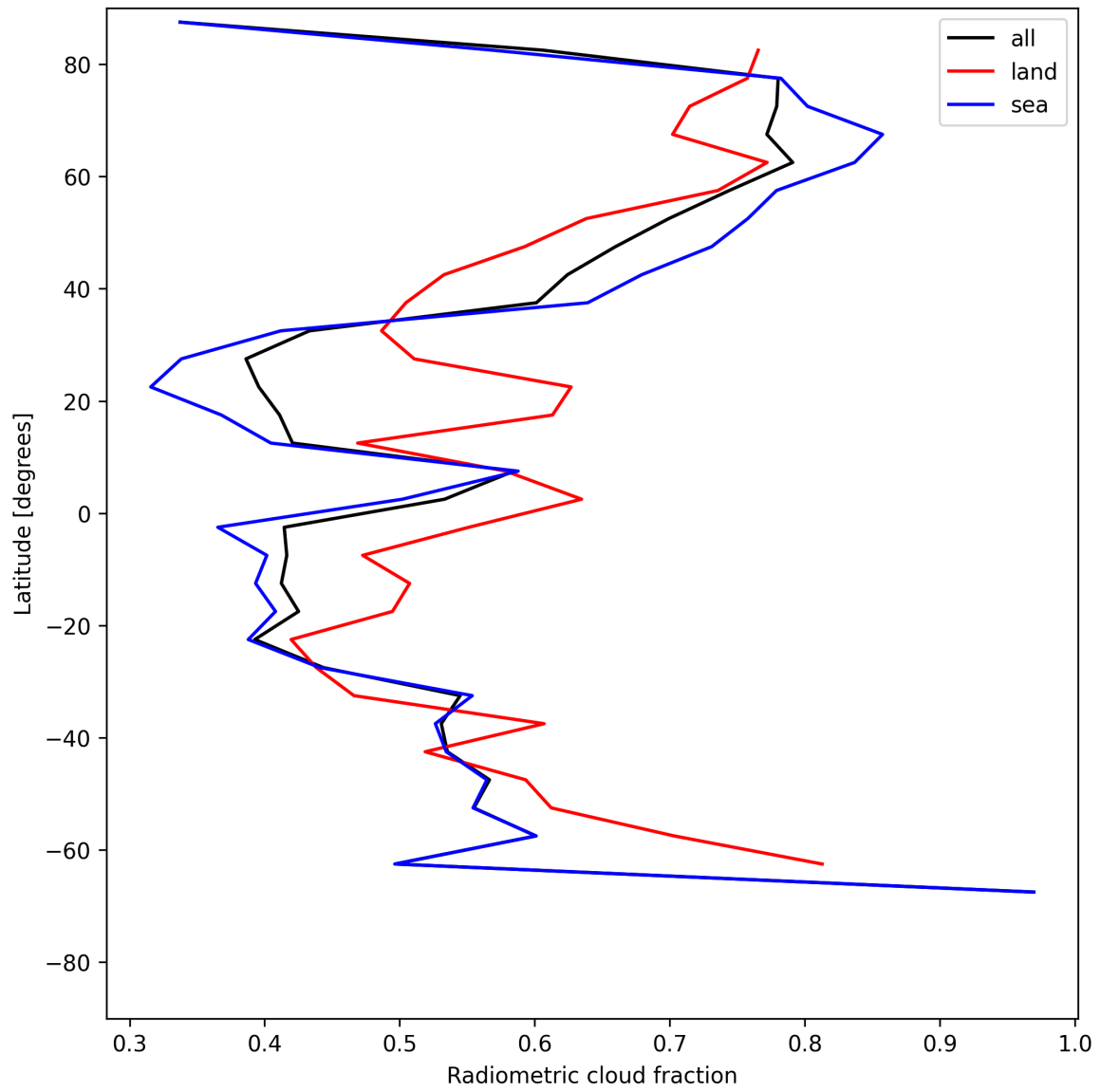
Figure 23: Zonal average of “Radiometric cloud fraction” for 2025-06-16 to 2025-06-17.
