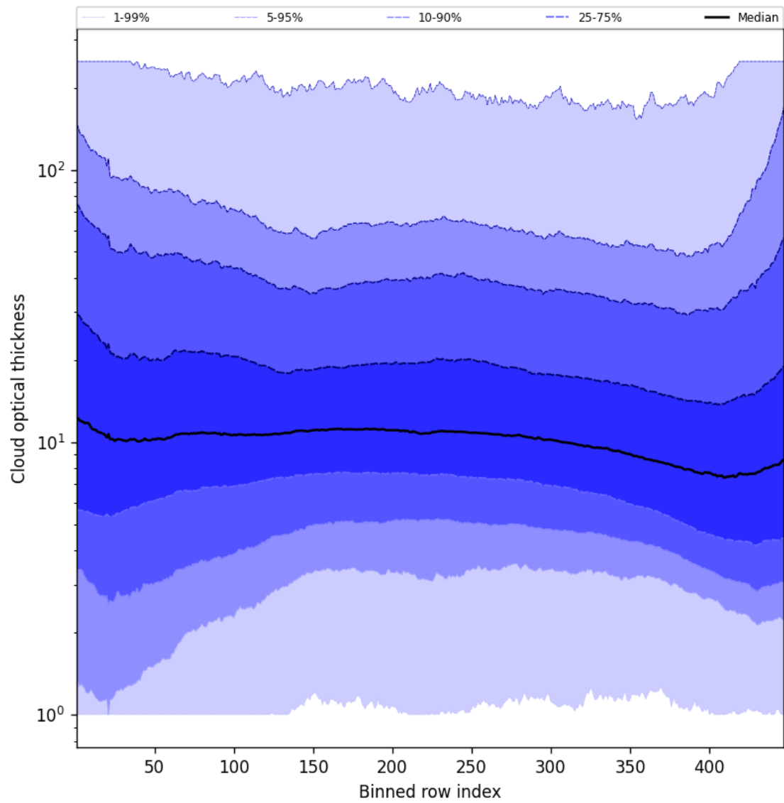
Figure 57: Along track statistics of “Cloud optical thickness” for 2025-06-16 to 2025-06-17
