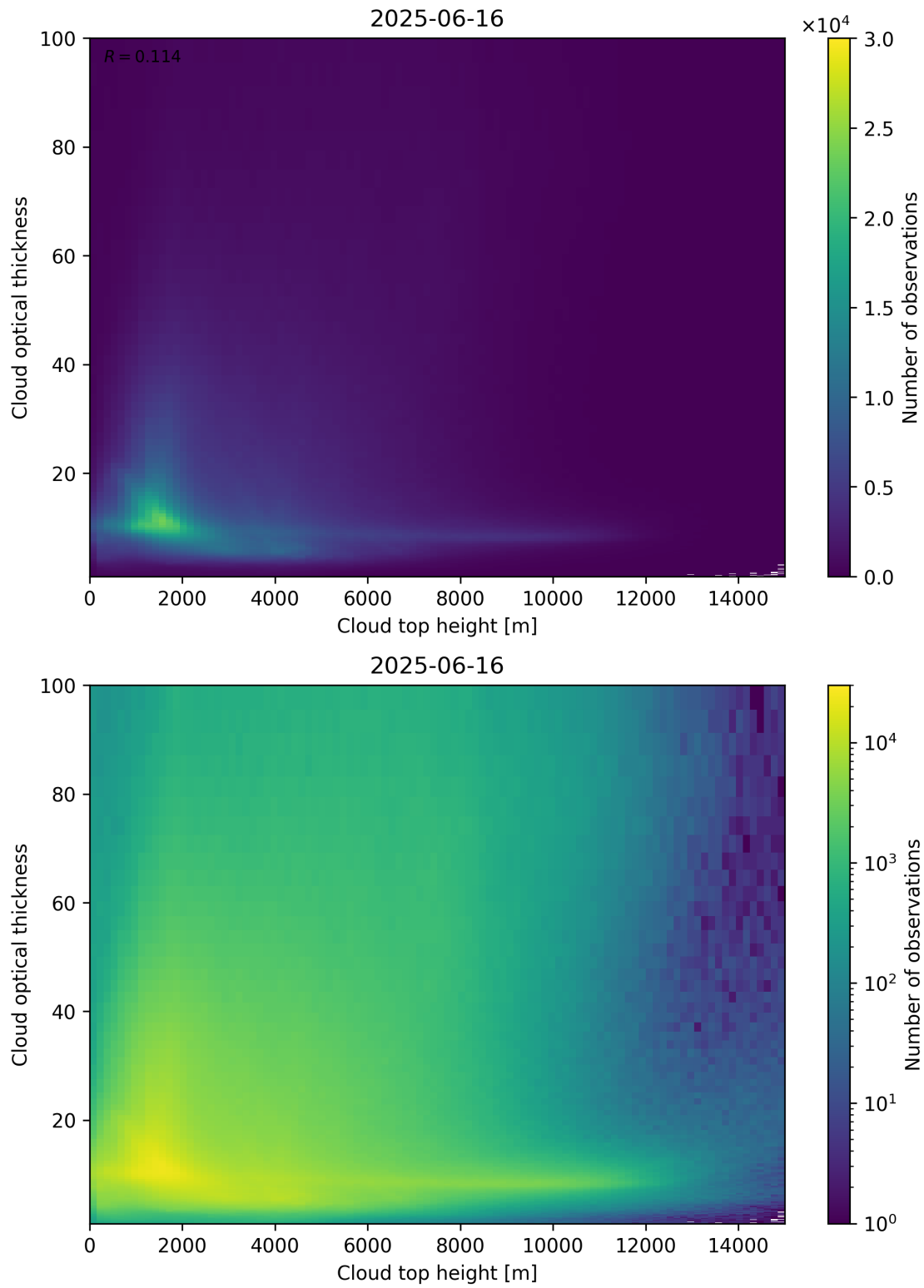
Figure 90: Scatter density plot of “Cloud top height” against “Cloud optical thickness” for 2025-06-16 to 2025-06-17.
