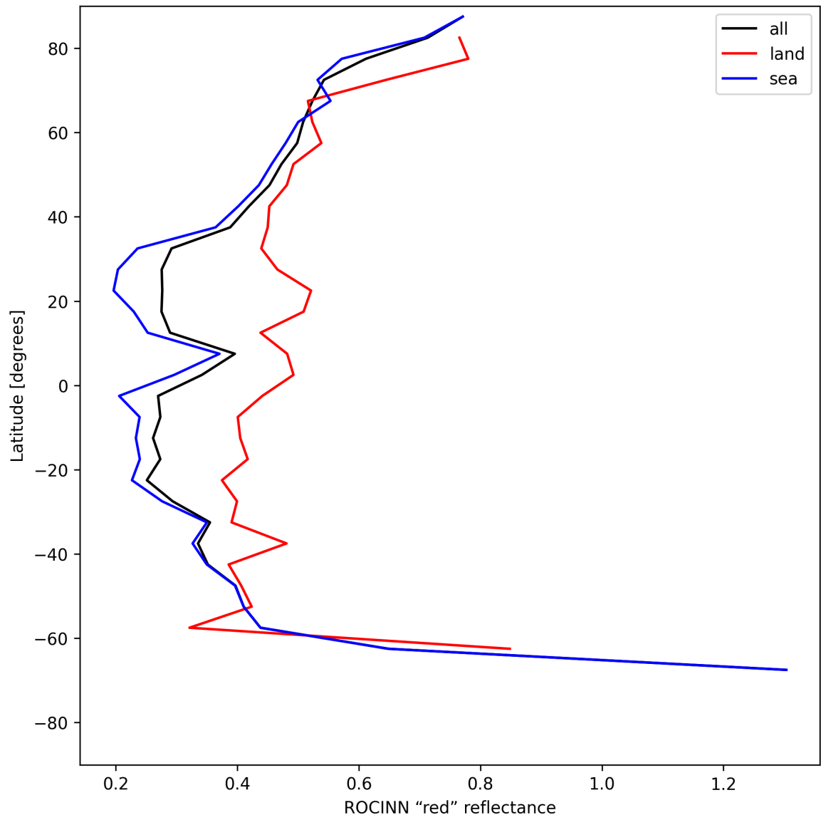
Figure 37: Zonal average of “ROCINN “red” reflectance” for 2025-06-16 to 2025-06-17.
