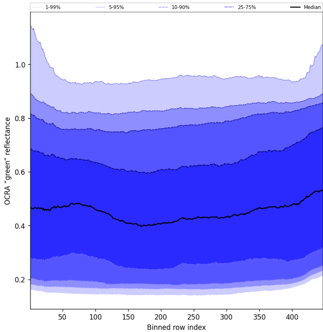
Figure 68: Along track statistics of “OCRA “green” reflectance” for 2025-06-16 to 2025-06-17
