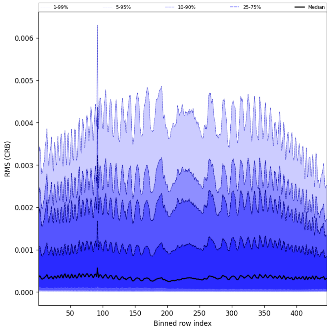
Figure 64: Along track statistics of “RMS (CRB)” for 2025-06-16 to 2025-06-17
