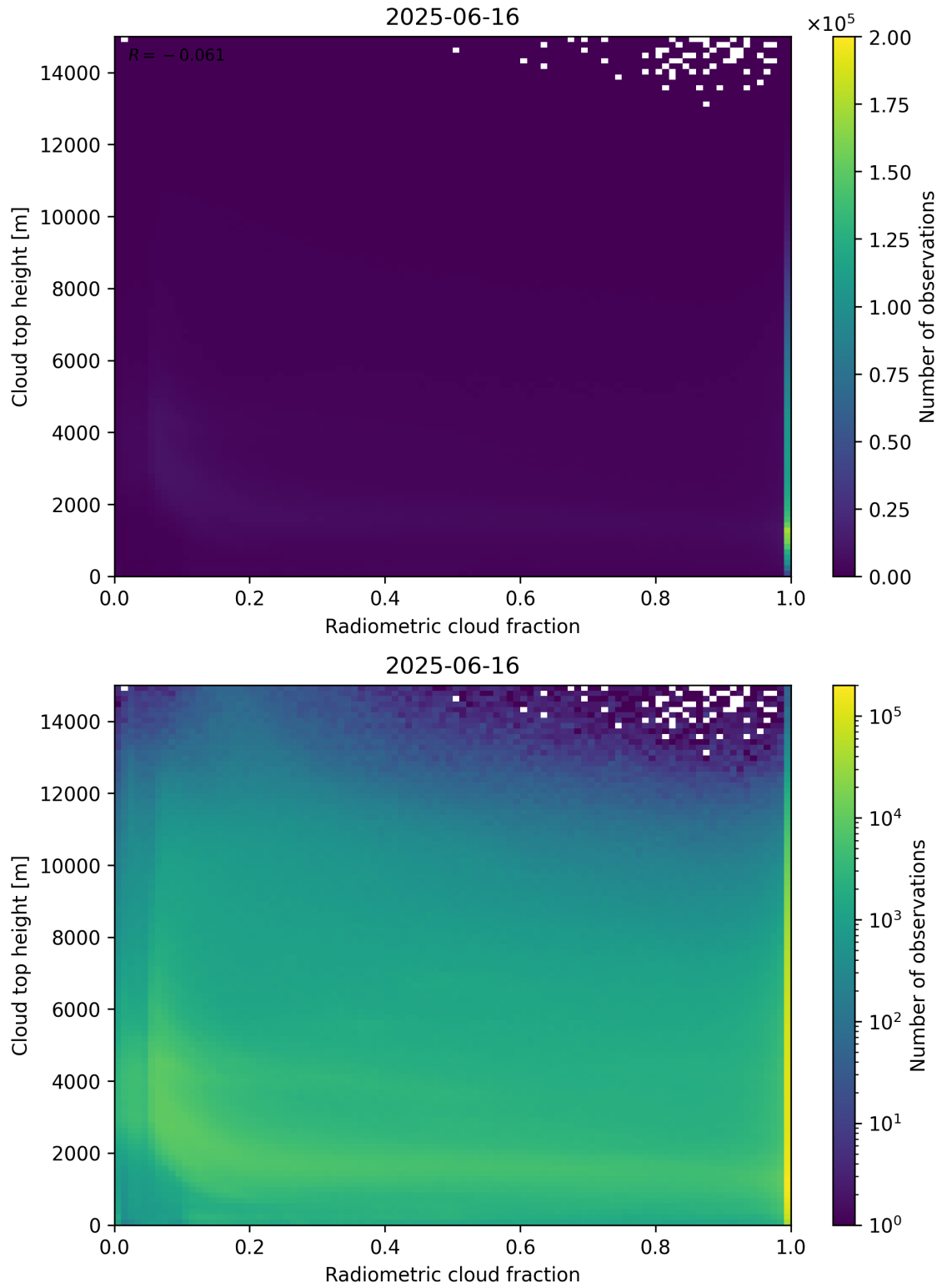
Figure 76: Scatter density plot of “Radiometric cloud fraction” against “Cloud top height” for 2025-06-16 to 2025-06-17.
