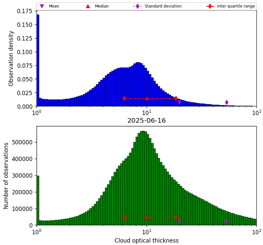
Figure 41: Histogram of “Cloud optical thickness” for 2025-06-16 to 2025-06-17
