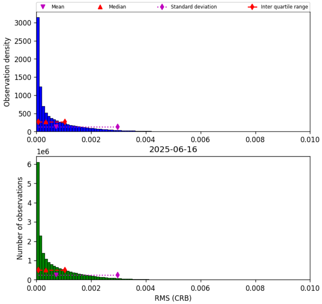
Figure 48: Histogram of “RMS (CRB)” for 2025-06-16 to 2025-06-17
