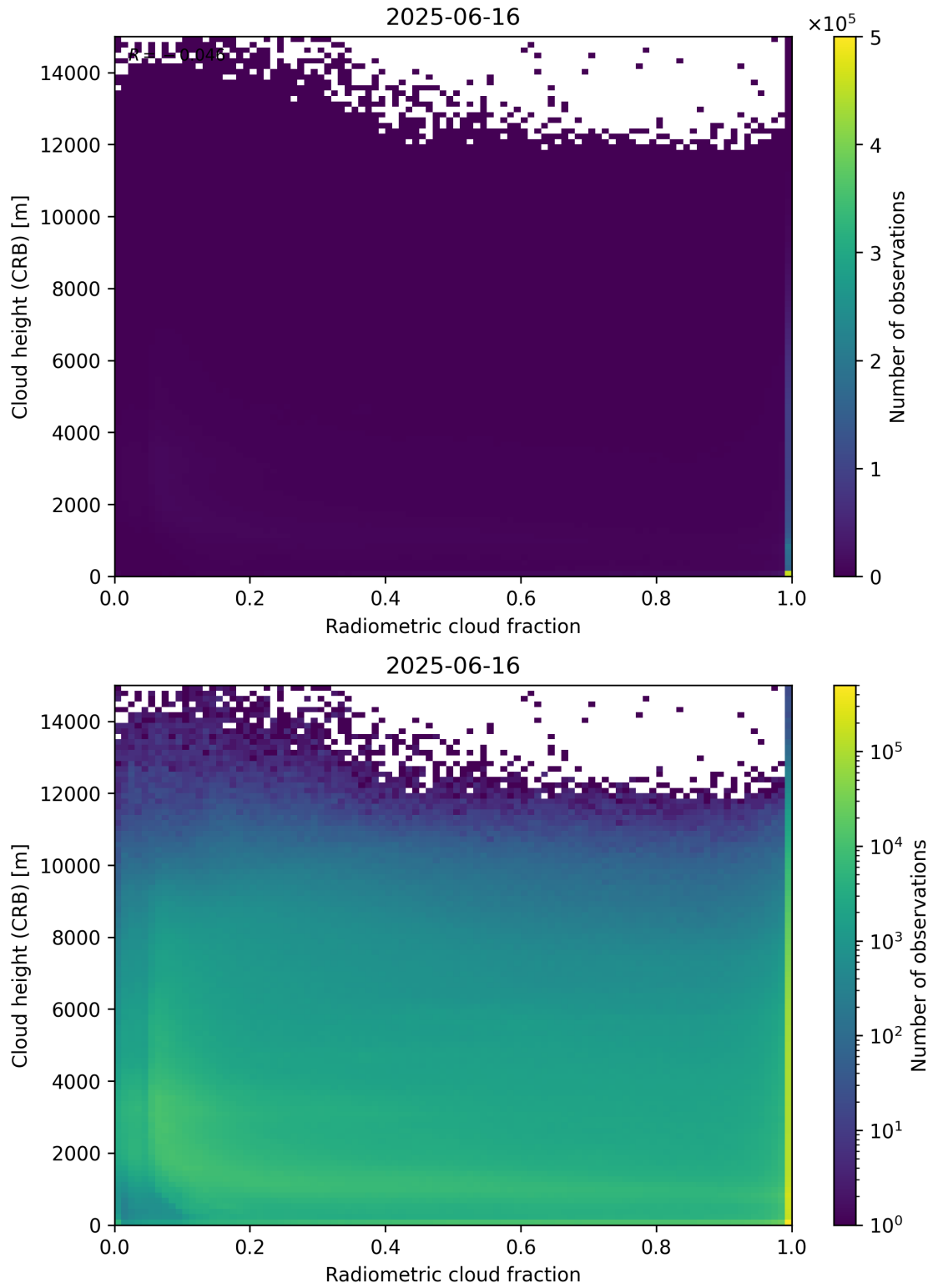
Figure 74: Scatter density plot of “Radiometric cloud fraction” against “Cloud height (CRB)” for 2025-06-16 to 2025-06-17.
