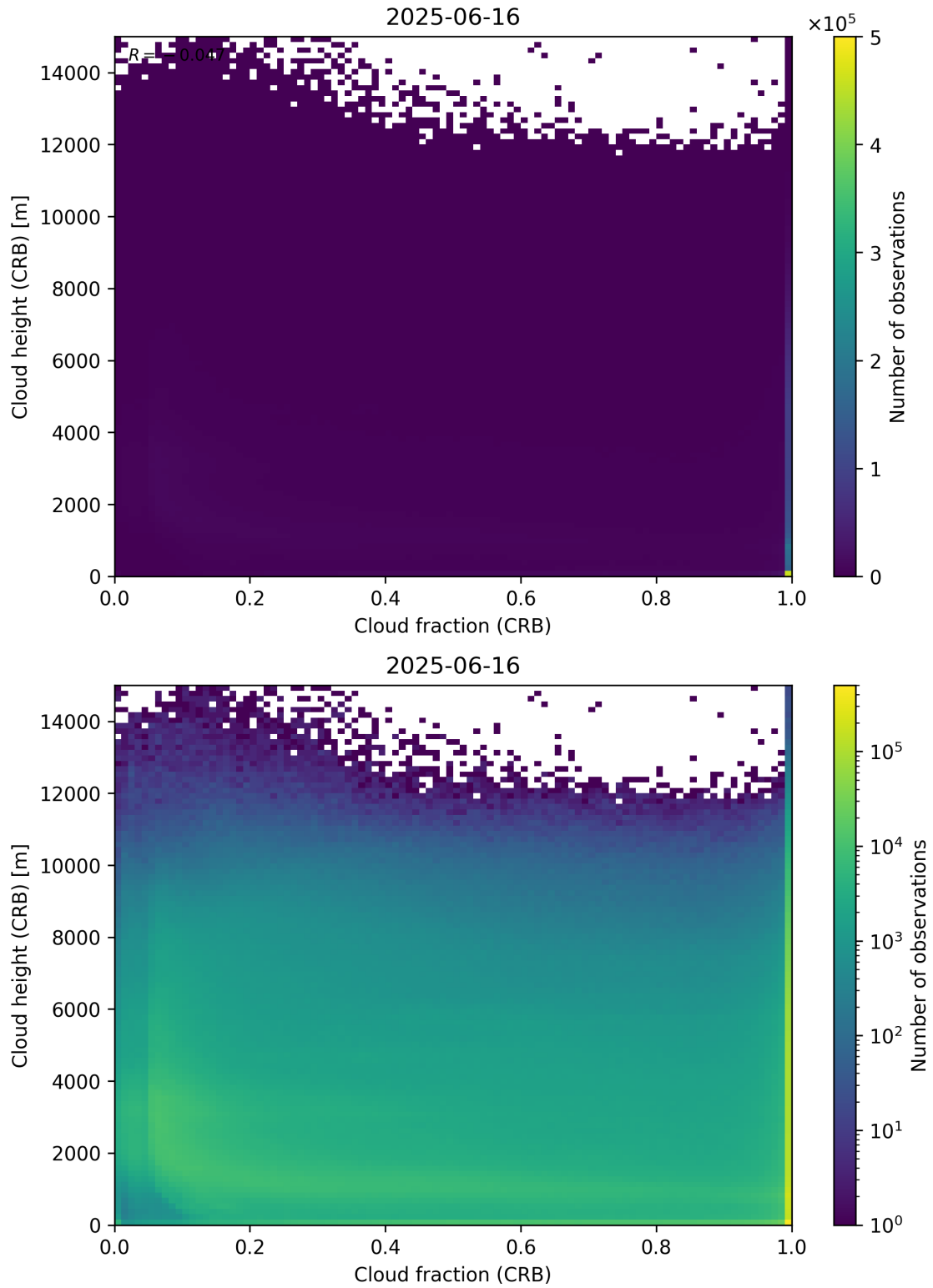
Figure 79: Scatter density plot of “Cloud fraction (CRB)” against “Cloud height (CRB)” for 2025-06-16 to 2025-06-17.
