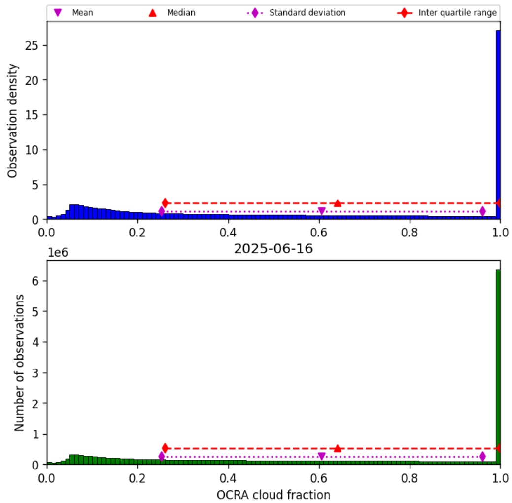
Figure 50: Histogram of “OCRA cloud fraction” for 2025-06-16 to 2025-06-17
