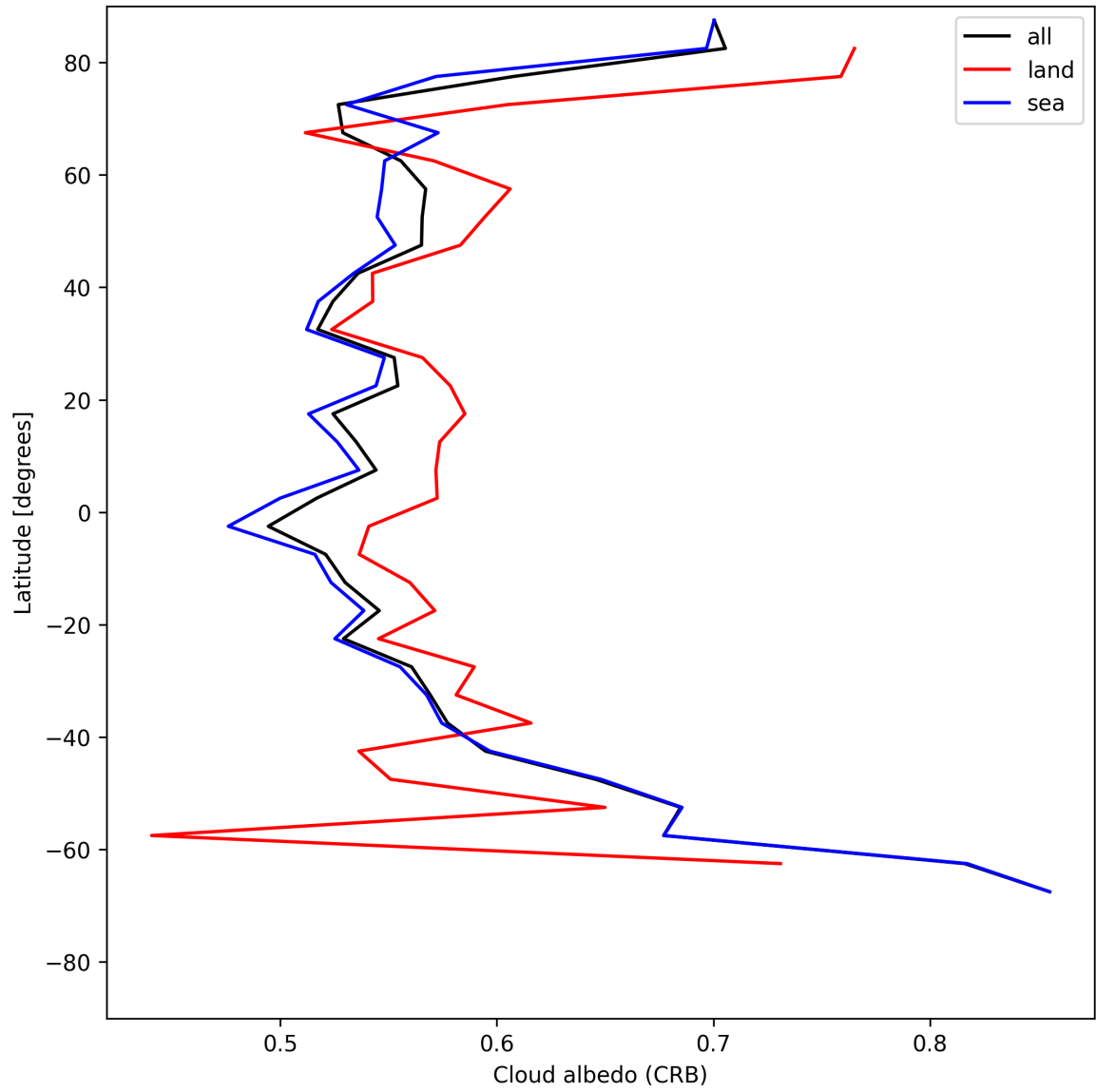
Figure 28: Zonal average of “Cloud albedo (CRB)” for 2025-06-16 to 2025-06-17.
