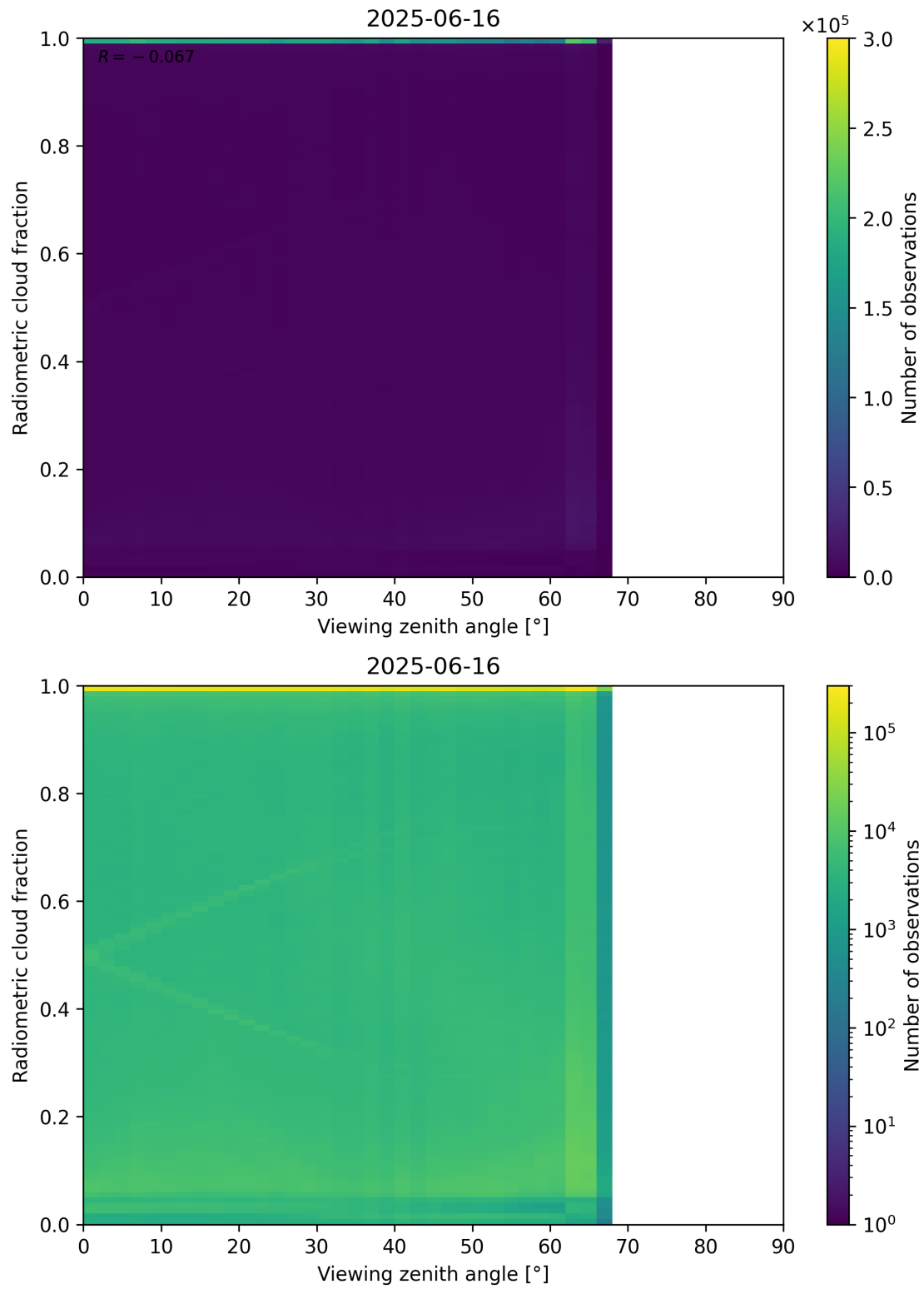
Figure 107: Scatter density plot of “Viewing zenith angle” against “Radiometric cloud fraction” for 2025-06-16 to 2025-06-17.
