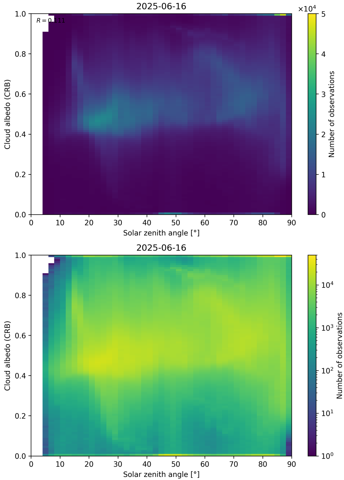
Figure 98: Scatter density plot of “Solar zenith angle” against “Cloud albedo (CRB)” for 2025-06-16 to 2025-06-17.
