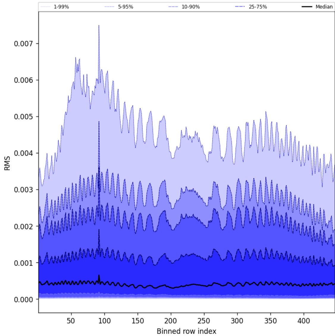
Figure 63: Along track statistics of “RMS” for 2025-06-16 to 2025-06-17
