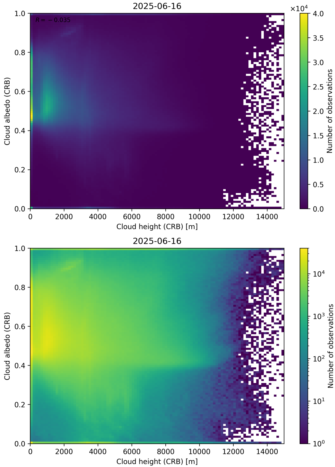
Figure 80: Scatter density plot of “Cloud height (CRB)” against “Cloud albedo (CRB)” for 2025-06-16 to 2025-06-17.
