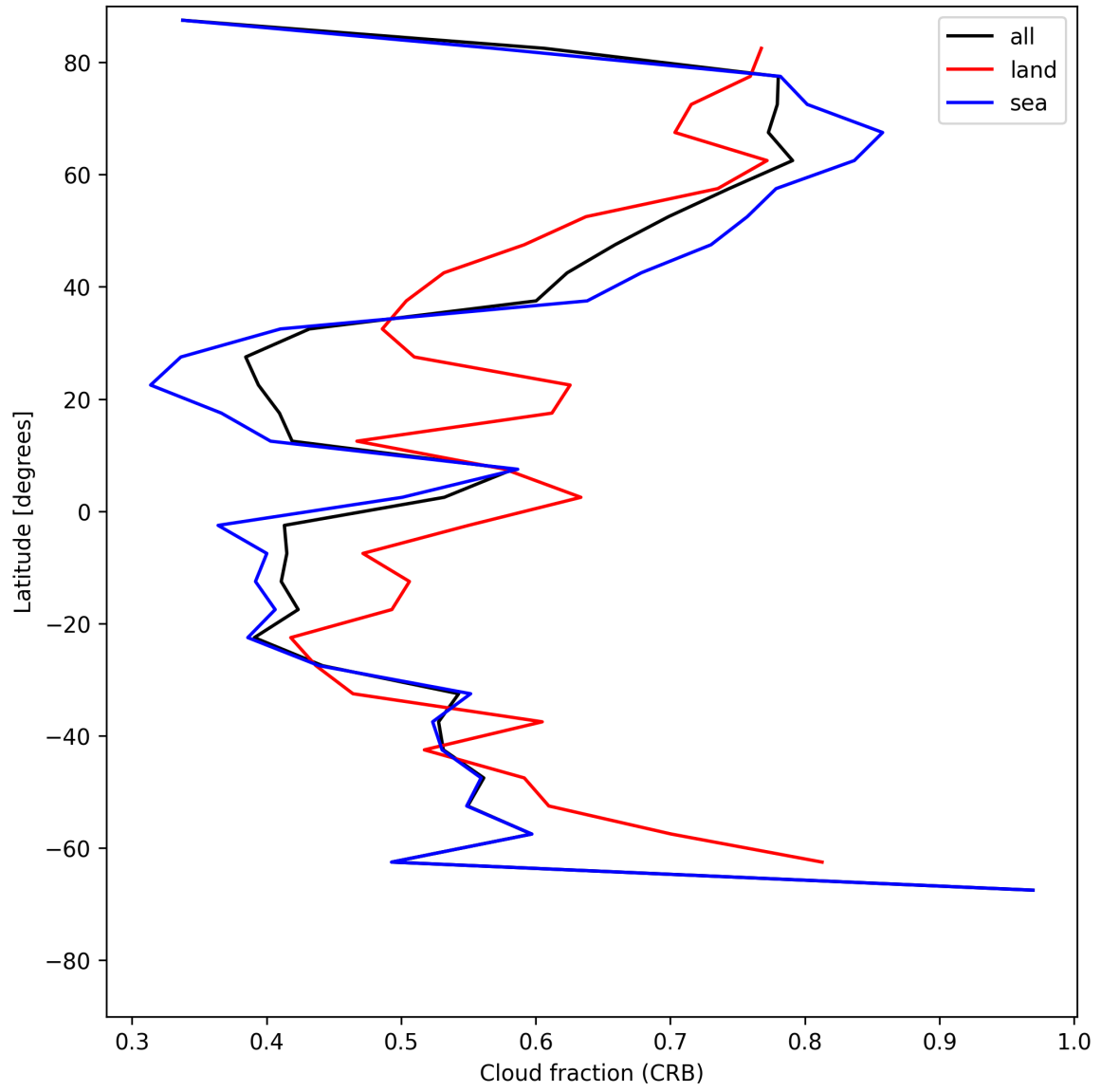
Figure 26: Zonal average of “Cloud fraction (CRB)” for 2025-06-16 to 2025-06-17.
