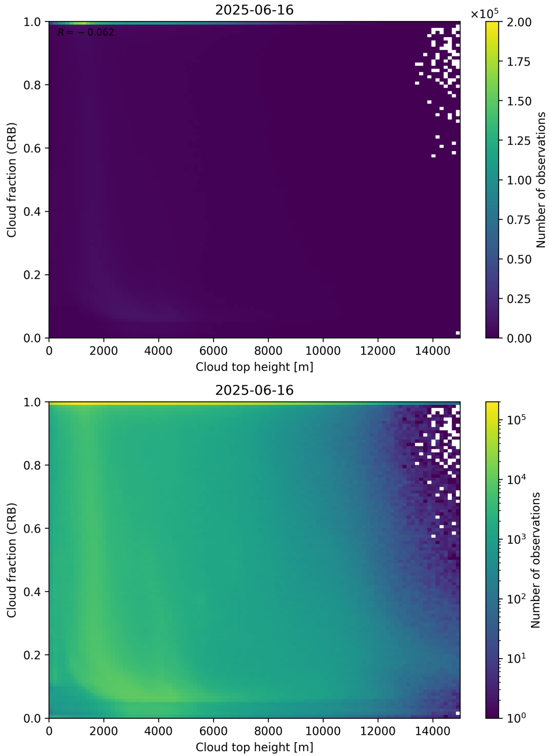
Figure 88: Scatter density plot of “Cloud top height” against “Cloud fraction (CRB)” for 2025-06-16 to 2025-06-17.
