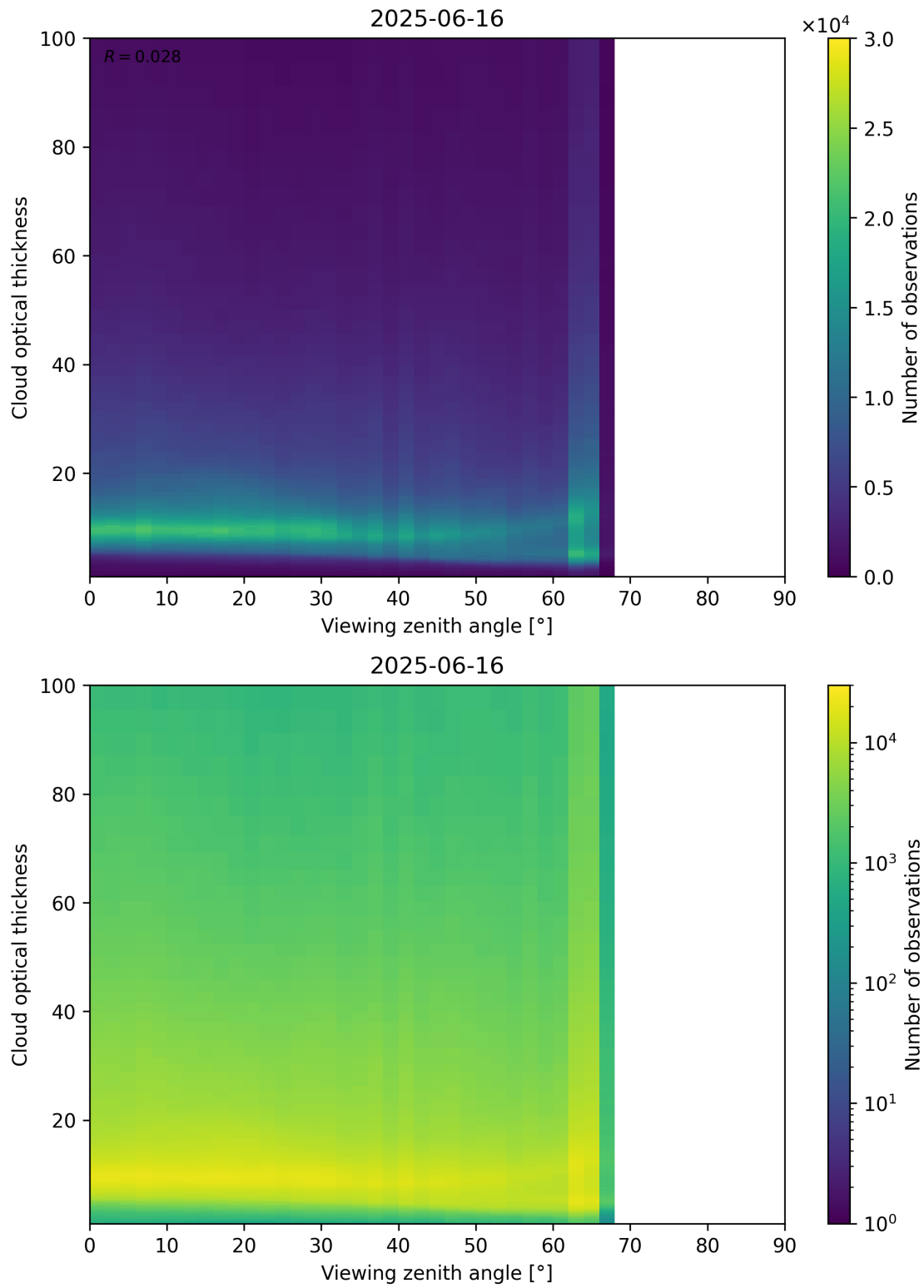
Figure 111: Scatter density plot of “Viewing zenith angle” against “Cloud optical thickness” for 2025-06-16 to 2025-06-17.
