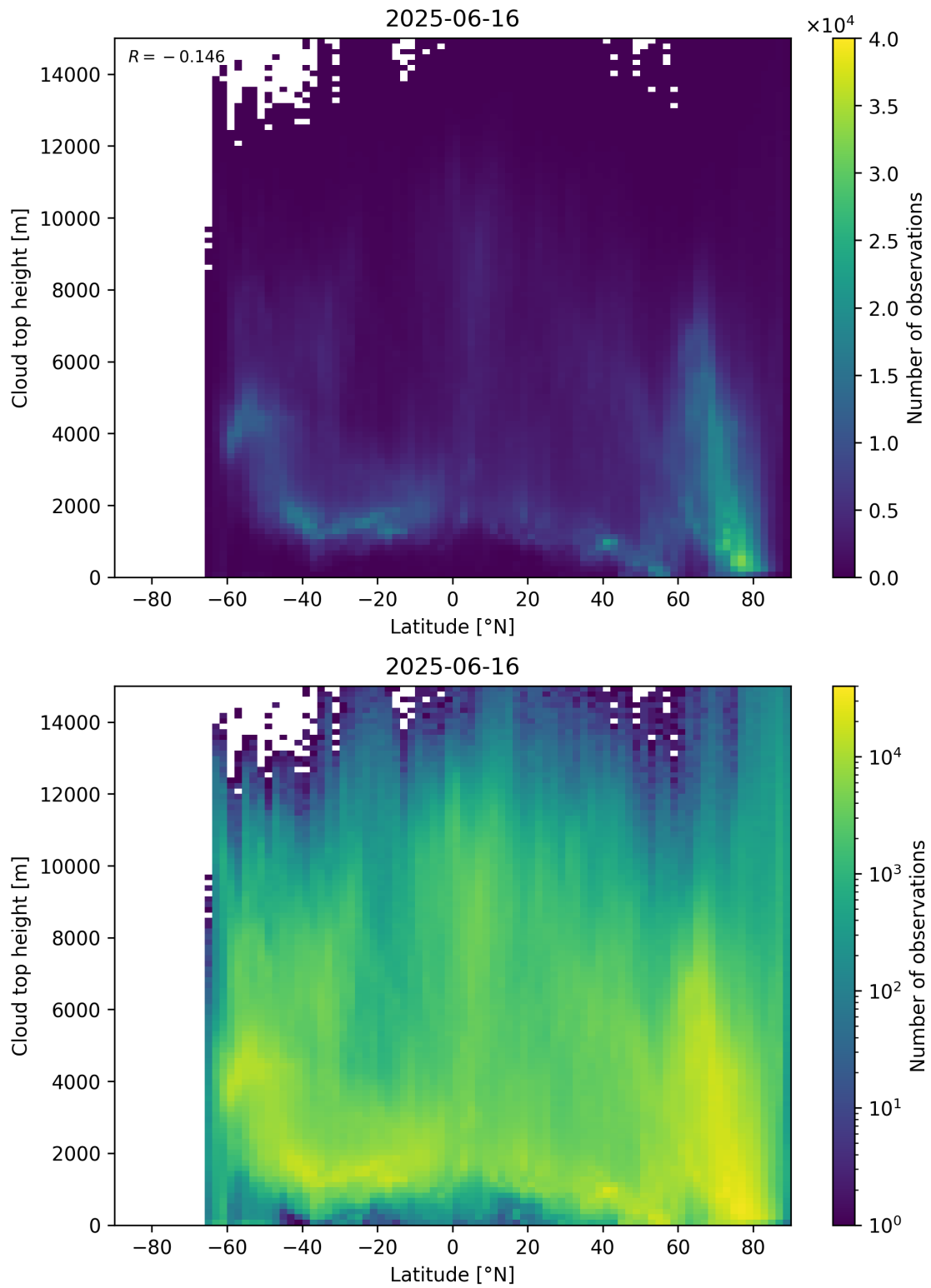
Figure 97: Scatter density plot of “Latitude” against “Cloud top height” for 2025-06-16 to 2025-06-17.
