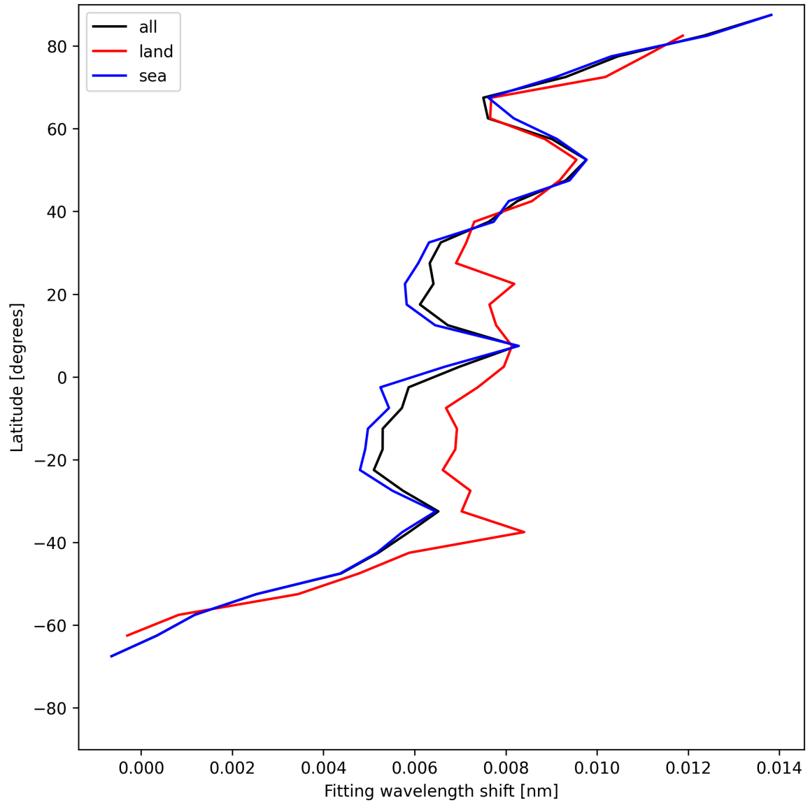
Figure 33: Zonal average of “Fitting wavelength shift” for 2025-06-16 to 2025-06-17.
