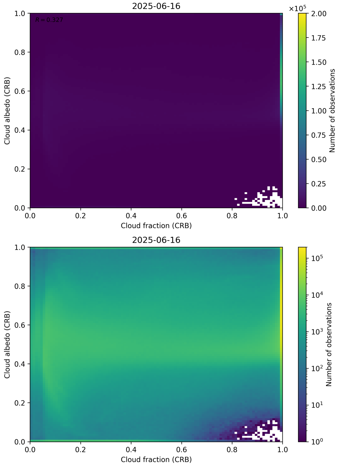
Figure 77: Scatter density plot of “Cloud fraction (CRB)” against “Cloud albedo (CRB)” for 2025-06-16 to 2025-06-17.
