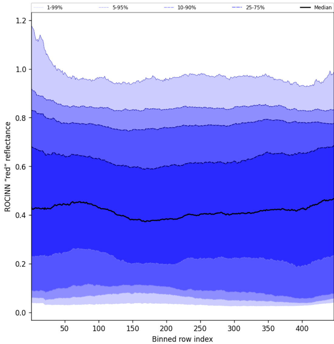
Figure 69: Along track statistics of “ROCINN “red” reflectance” for 2025-06-16 to 2025-06-17
