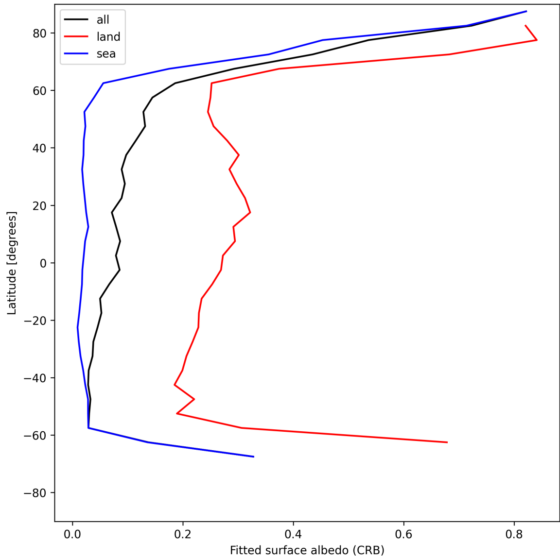
Figure 30: Zonal average of “Fitted surface albedo (CRB)” for 2025-06-16 to 2025-06-17.
