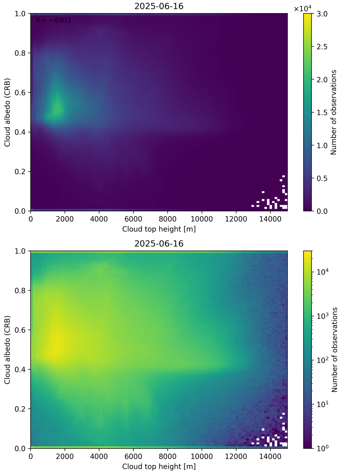
Figure 86: Scatter density plot of “Cloud top height” against “Cloud albedo (CRB)” for 2025-06-16 to 2025-06-17.
