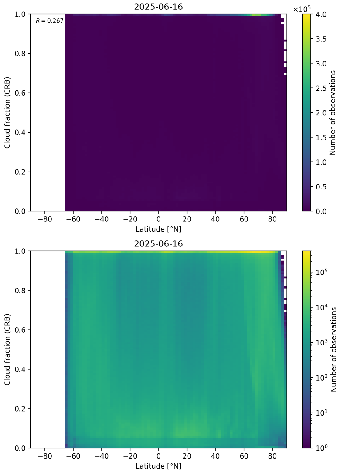
Figure 94: Scatter density plot of “Latitude” against “Cloud fraction (CRB)” for 2025-06-16 to 2025-06-17.
