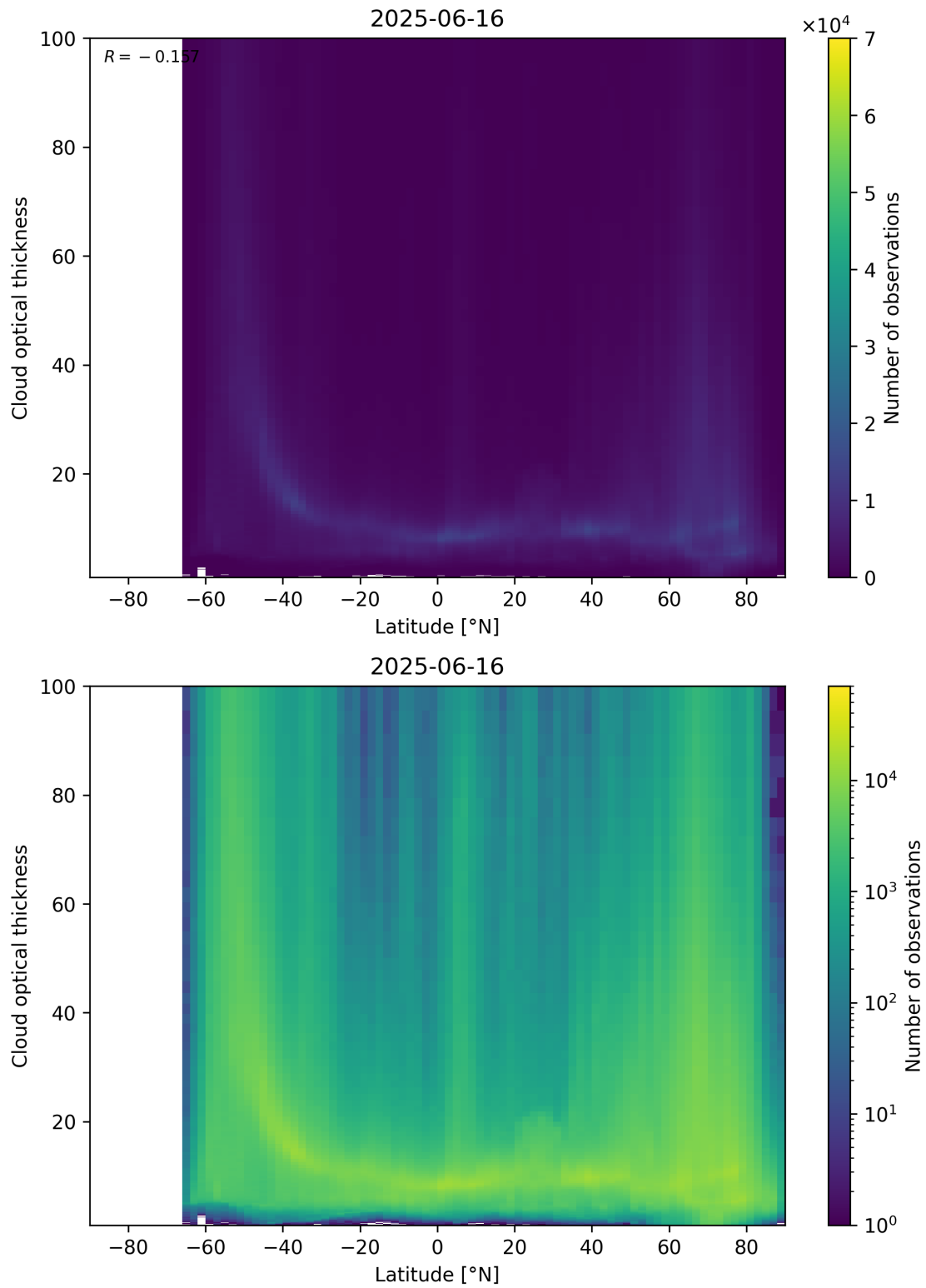
Figure 96: Scatter density plot of “Latitude” against “Cloud optical thickness” for 2025-06-16 to 2025-06-17.
