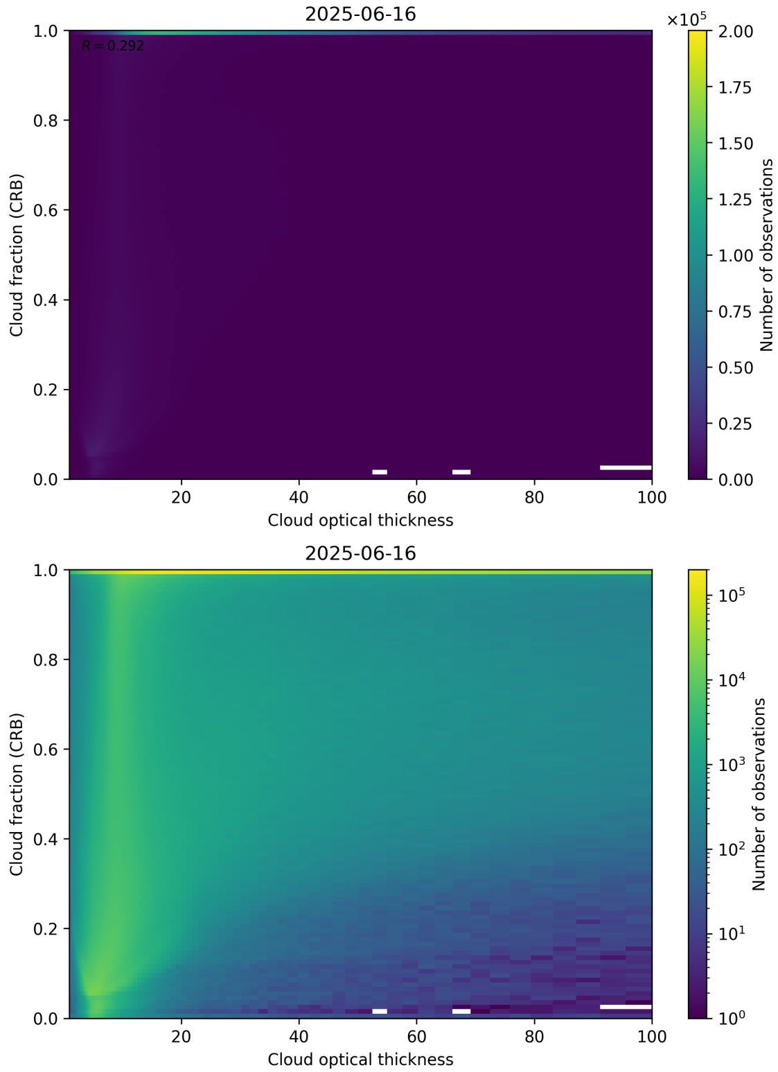
Figure 84: Scatter density plot of “Cloud optical thickness” against “Cloud fraction (CRB)” for 2025-06-16 to 2025-06-17.
