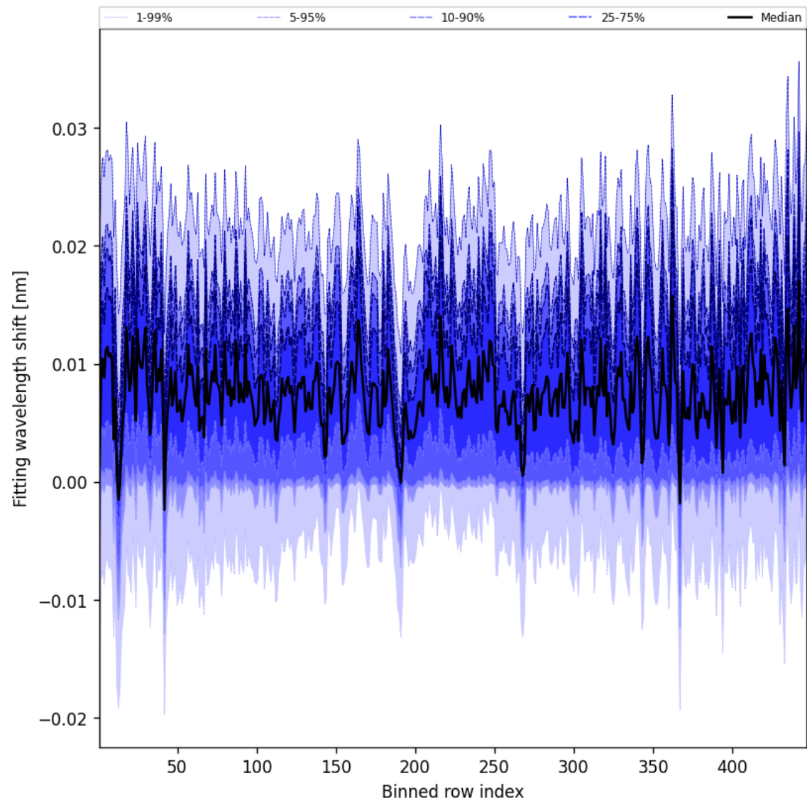
Figure 65: Along track statistics of “Fitting wavelength shift” for 2025-06-16 to 2025-06-17
