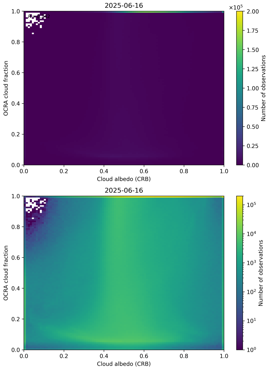
Figure 70: Scatter density plot of “Cloud albedo (CRB)” against “OCRA cloud fraction” for 2025-06-16 to 2025-06-17.
