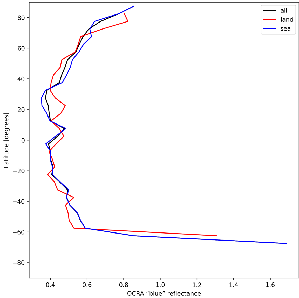
Figure 35: Zonal average of “OCRA “blue” reflectance” for 2025-06-16 to 2025-06-17.
