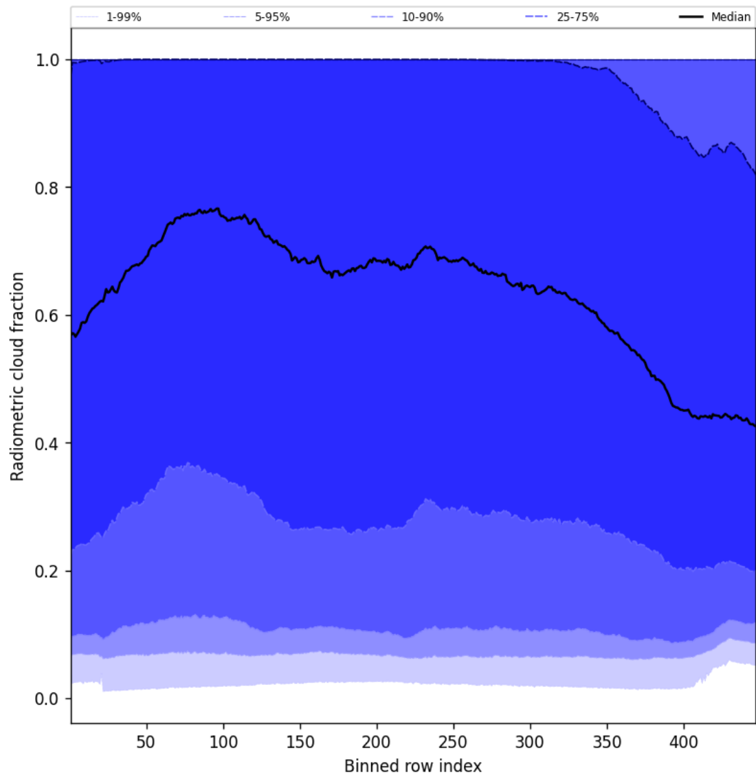
Figure 55: Along track statistics of “Radiometric cloud fraction” for 2025-06-16 to 2025-06-17
