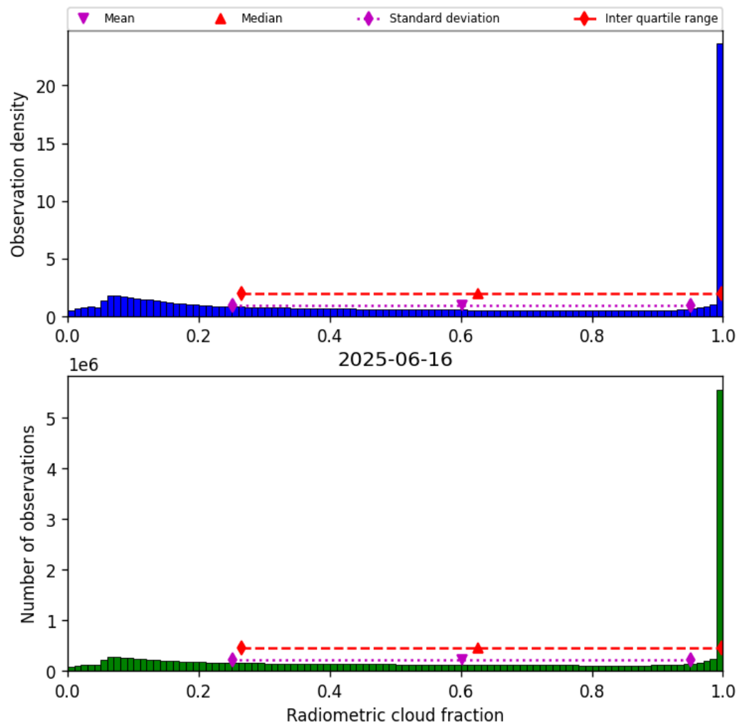
Figure 39: Histogram of “Radiometric cloud fraction” for 2025-06-16 to 2025-06-17
