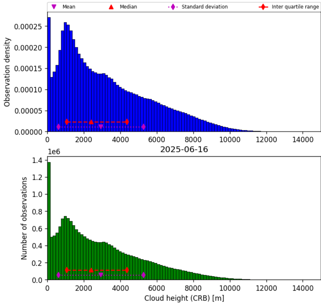
Figure 43: Histogram of “Cloud height (CRB)” for 2025-06-16 to 2025-06-17
