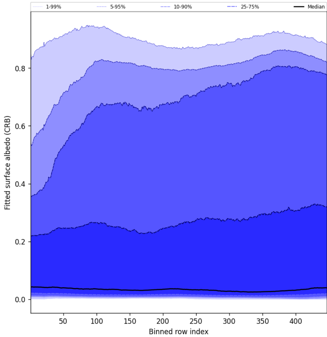
Figure 62: Along track statistics of “Fitted surface albedo (CRB)” for 2025-06-16 to 2025-06-17
