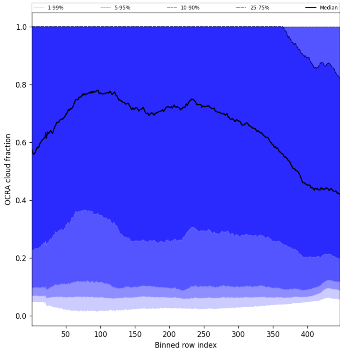
Figure 66: Along track statistics of “OCRA cloud fraction” for 2025-06-16 to 2025-06-17
