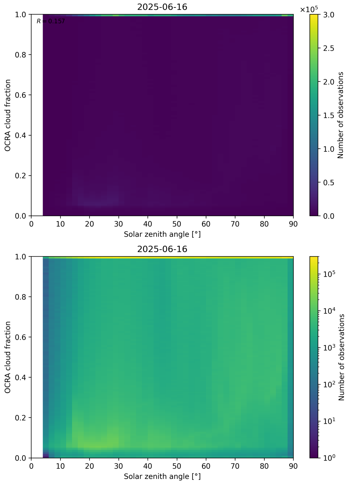
Figure 100: Scatter density plot of “Solar zenith angle” against “OCRA cloud fraction” for 2025-06-16 to 2025-06-17.
