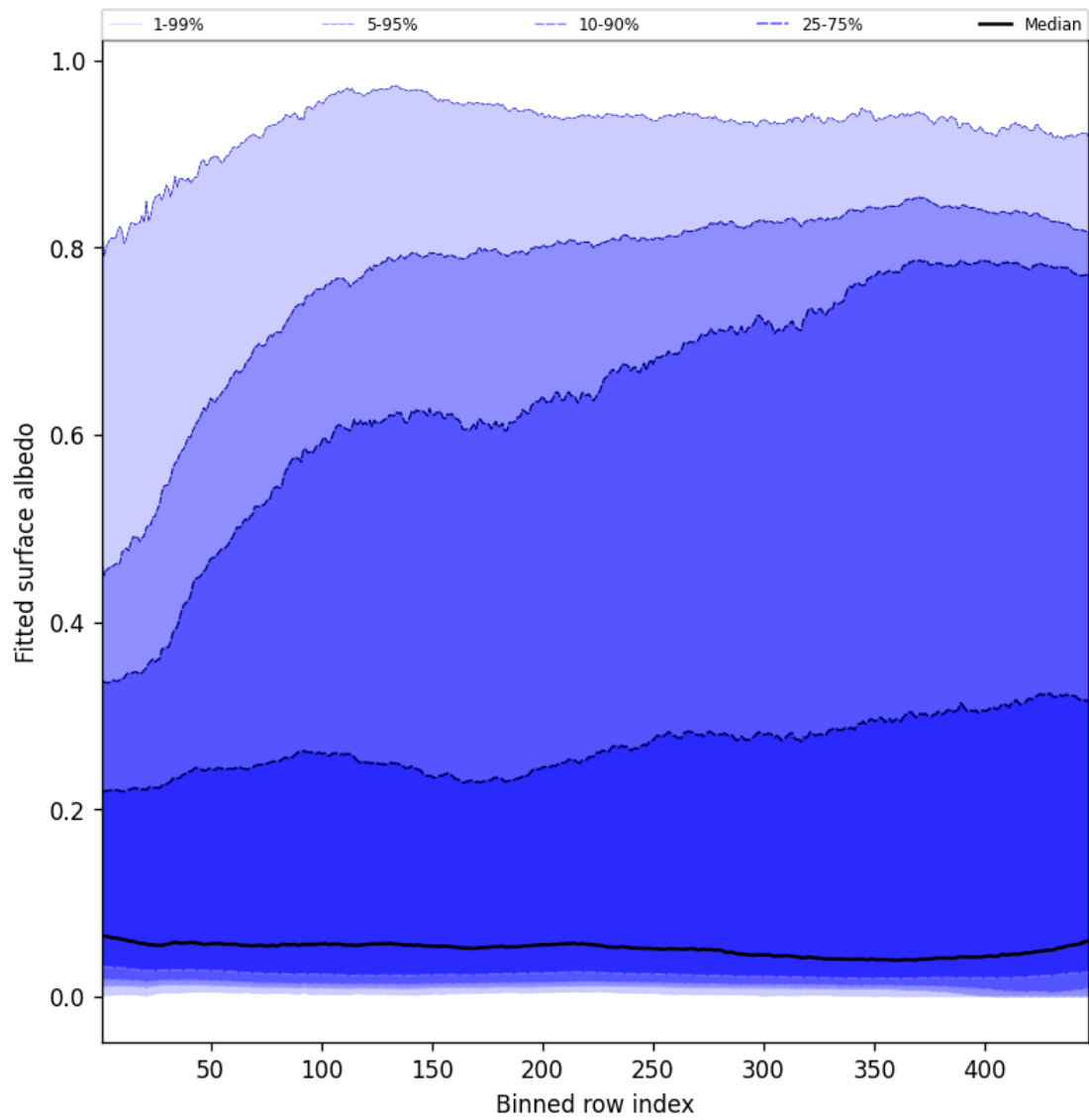
Figure 61: Along track statistics of “Fitted surface albedo” for 2025-06-16 to 2025-06-17
