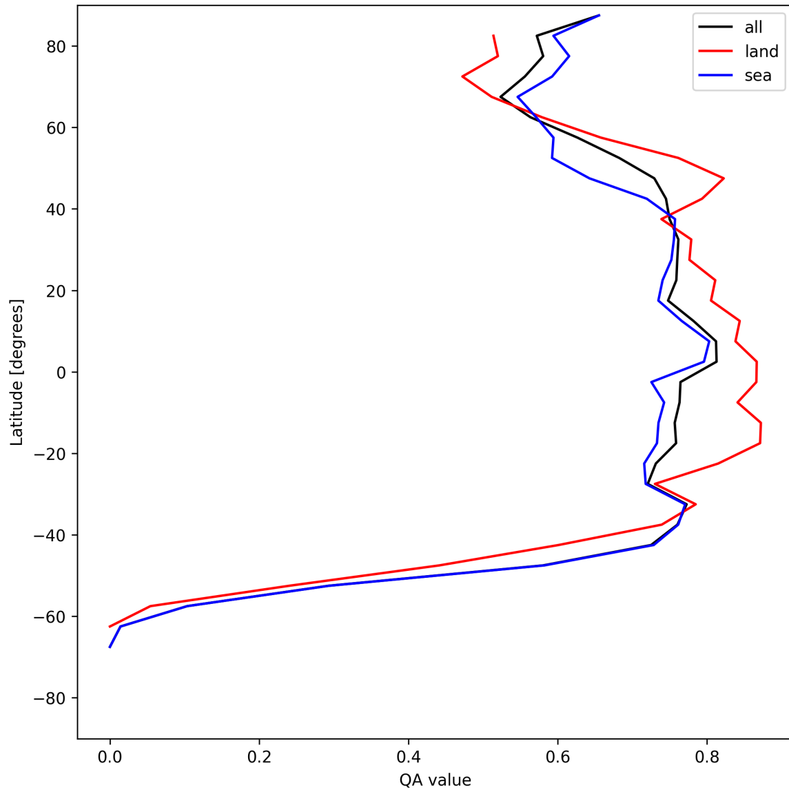
Figure 22: Zonal average of “QA value” for 2025-06-16 to 2025-06-17.
