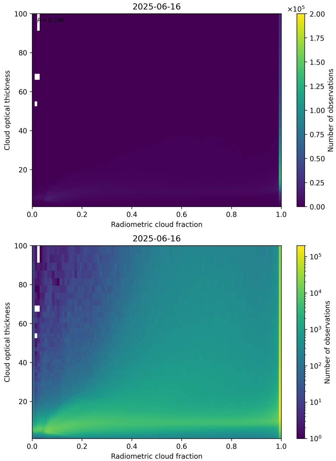
Figure 75: Scatter density plot of “Radiometric cloud fraction” against “Cloud optical thickness” for 2025-06-16 to 2025-06-17.
