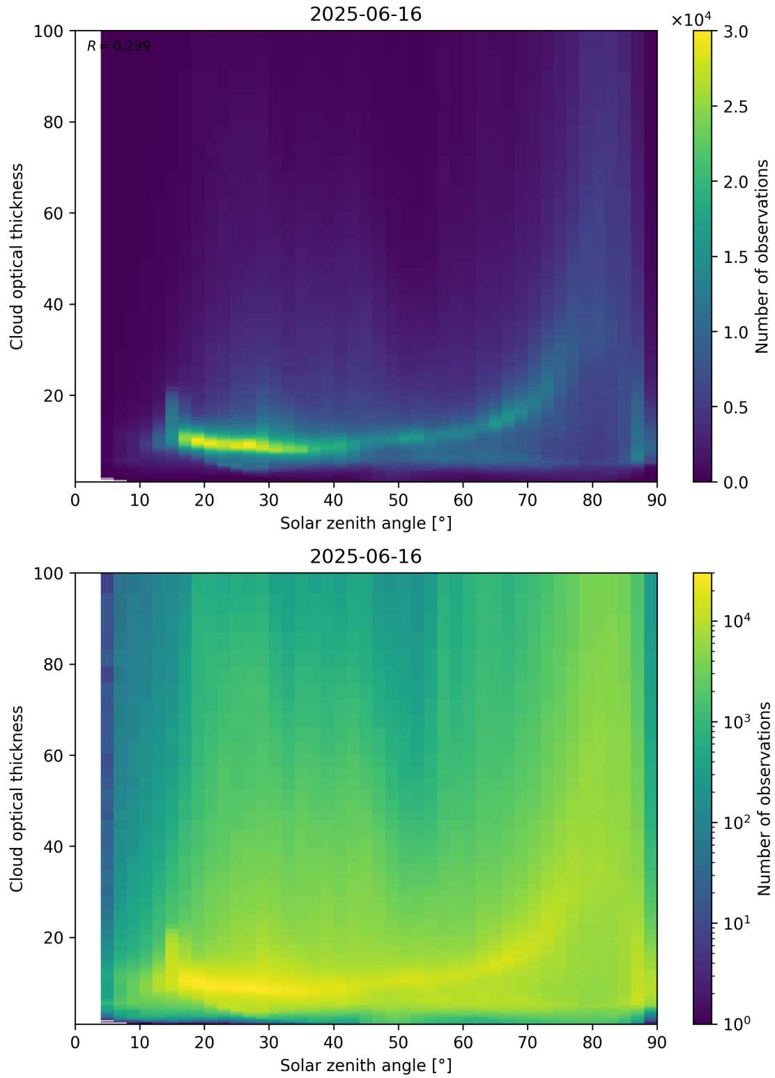
Figure 103: Scatter density plot of “Solar zenith angle” against “Cloud optical thickness” for 2025-06-16 to 2025-06-17.
