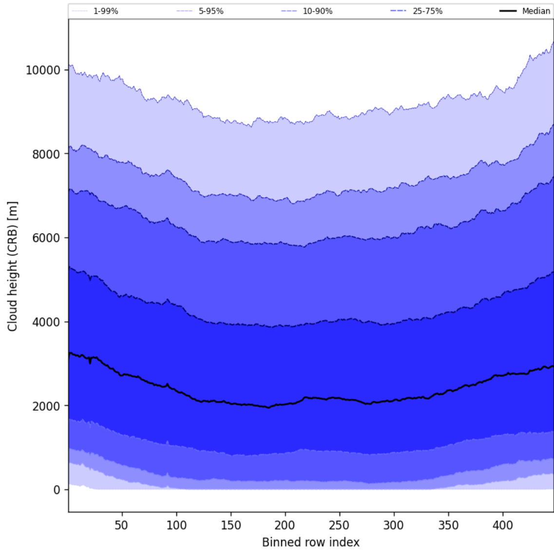
Figure 59: Along track statistics of “Cloud height (CRB)” for 2025-06-16 to 2025-06-17
