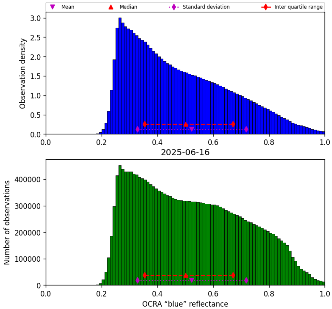
Figure 51: Histogram of “OCRA “blue” reflectance” for 2025-06-16 to 2025-06-17
