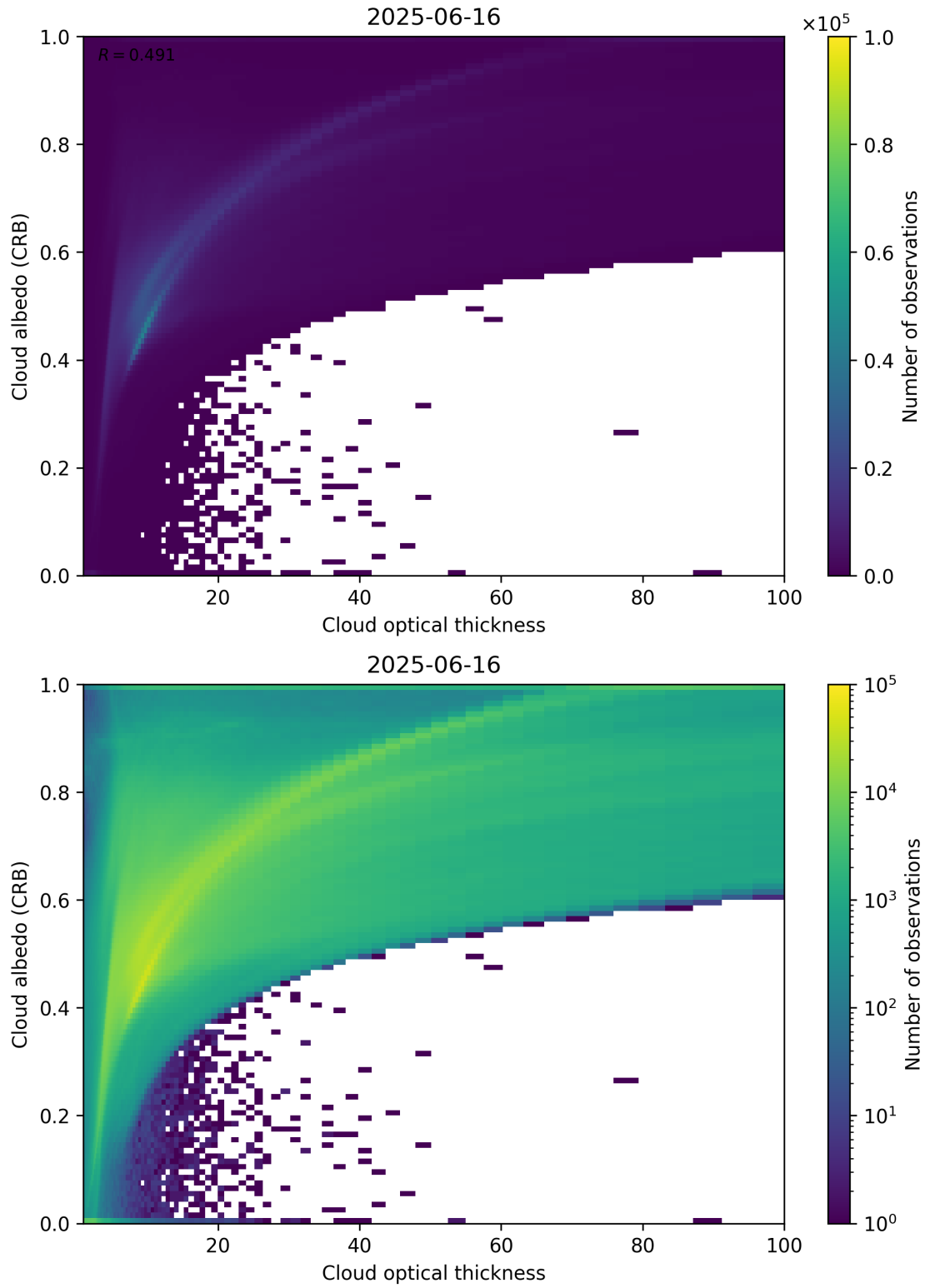
Figure 82: Scatter density plot of “Cloud optical thickness” against “Cloud albedo (CRB)” for 2025-06-16 to 2025-06-17.
