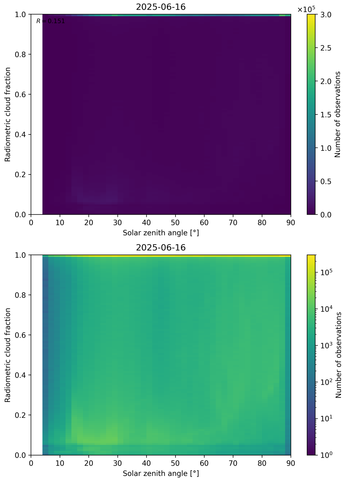
Figure 99: Scatter density plot of “Solar zenith angle” against “Radiometric cloud fraction” for 2025-06-16 to 2025-06-17.
