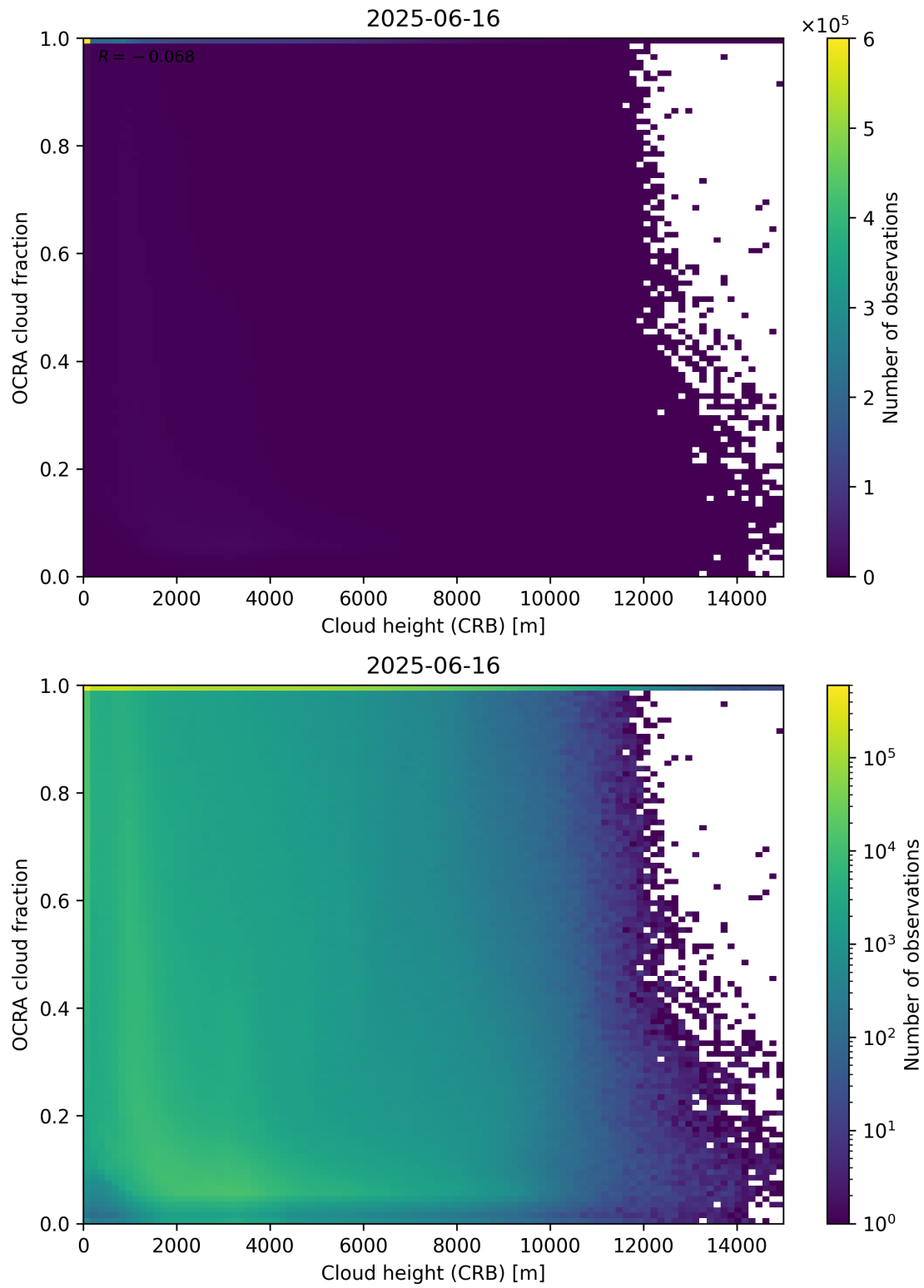
Figure 81: Scatter density plot of “Cloud height (CRB)” against “OCRA cloud fraction” for 2025-06-16 to 2025-06-17.
