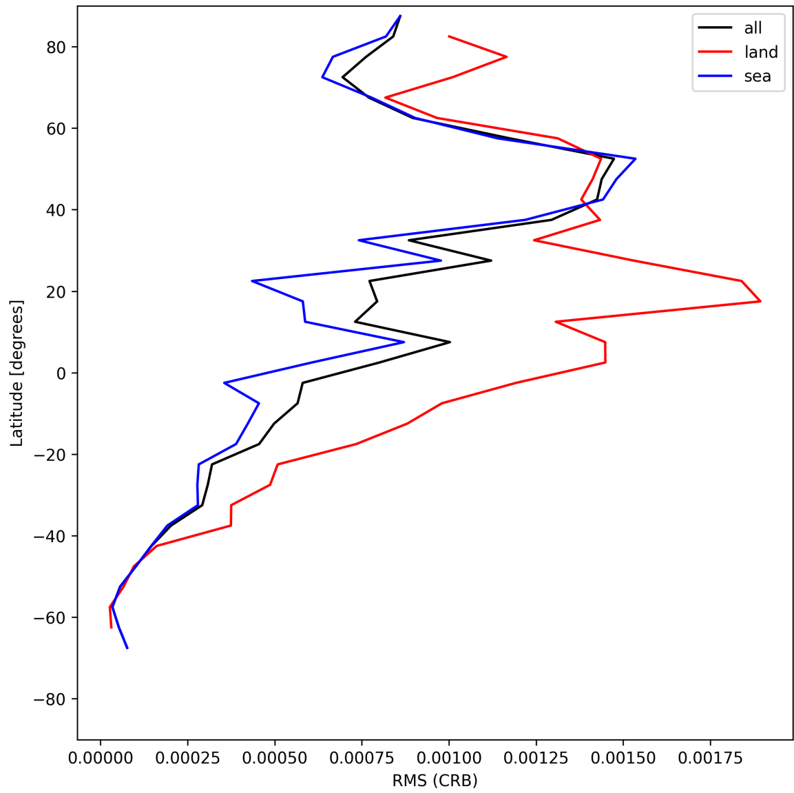
Figure 32: Zonal average of “RMS (CRB)” for 2025-06-16 to 2025-06-17.
