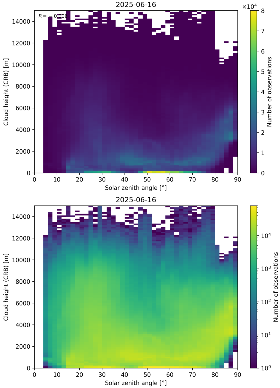
Figure 102: Scatter density plot of “Solar zenith angle” against “Cloud height (CRB)” for 2025-06-16 to 2025-06-17.
