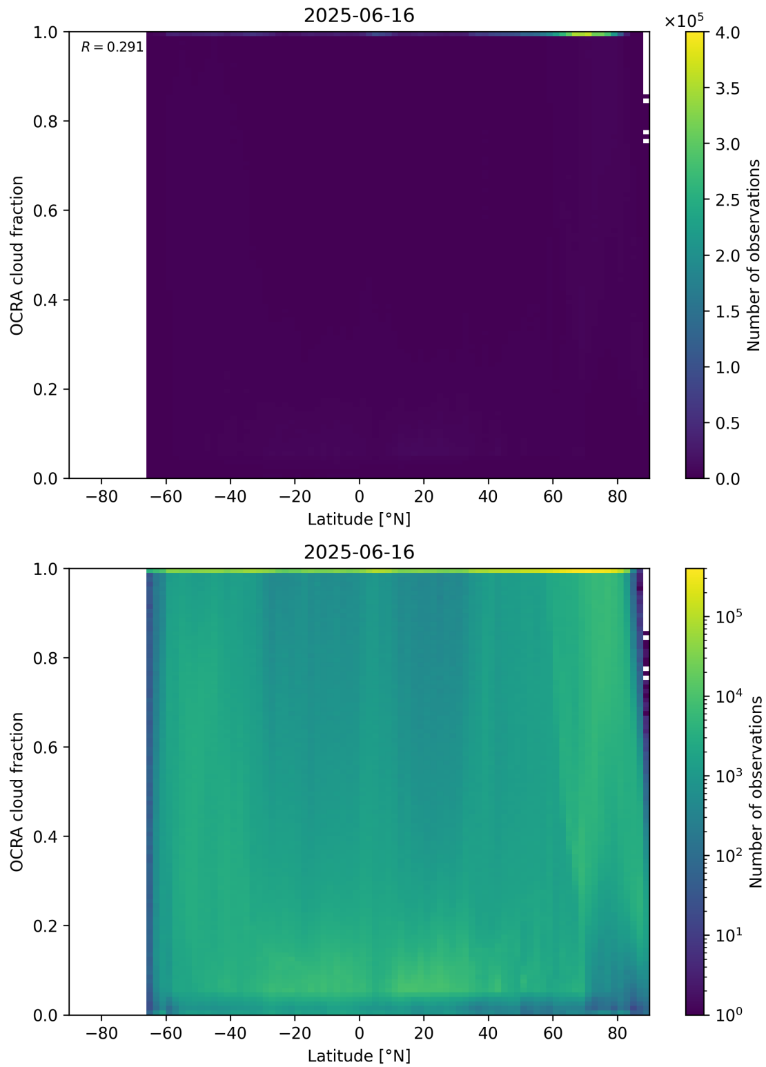
Figure 93: Scatter density plot of “Latitude” against “OCRA cloud fraction” for 2025-06-16 to 2025-06-17.
