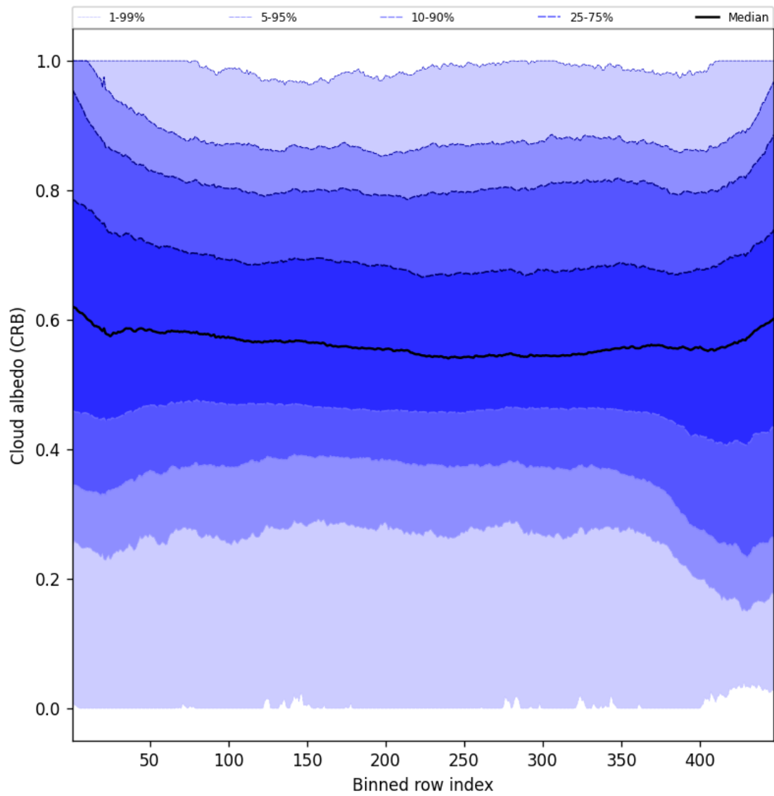
Figure 60: Along track statistics of “Cloud albedo (CRB)” for 2025-06-16 to 2025-06-17
