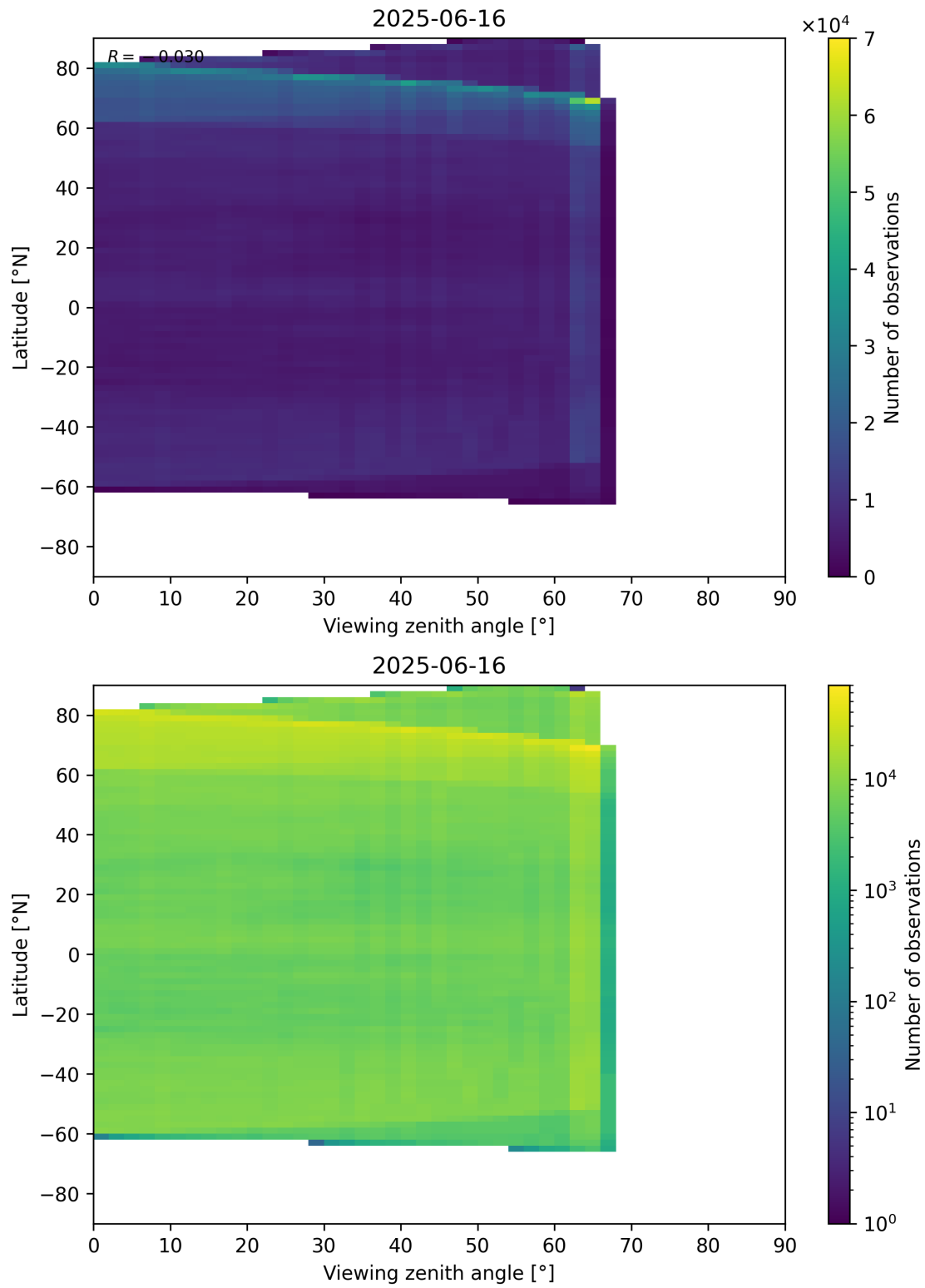
Figure 113: Scatter density plot of “Viewing zenith angle” against “Latitude” for 2025-06-16 to 2025-06-17.
