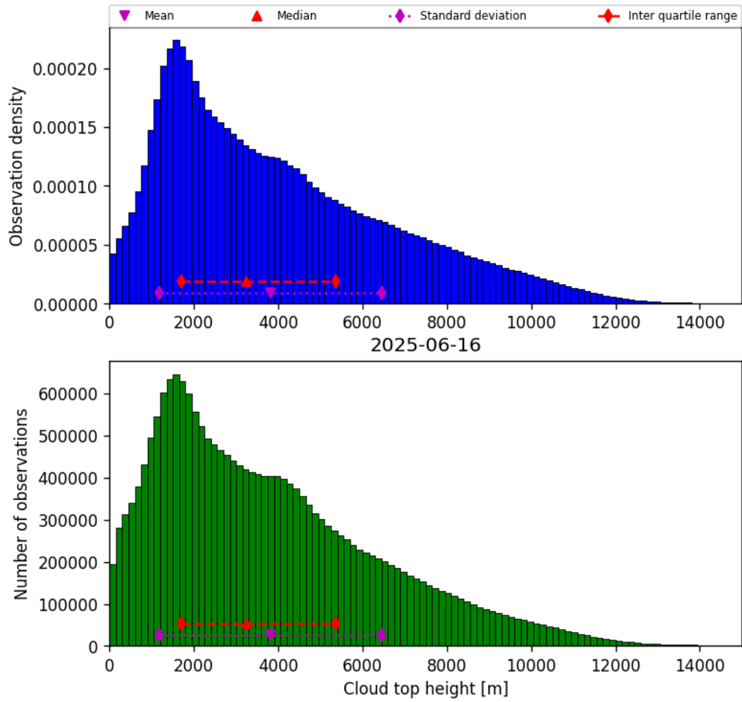
Figure 40: Histogram of “Cloud top height” for 2025-06-16 to 2025-06-17
