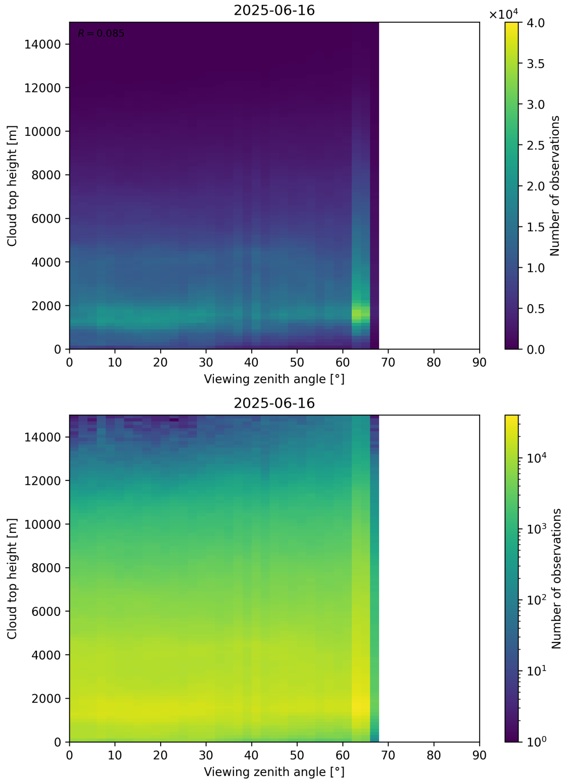
Figure 112: Scatter density plot of “Viewing zenith angle” against “Cloud top height” for 2025-06-16 to 2025-06-17.
