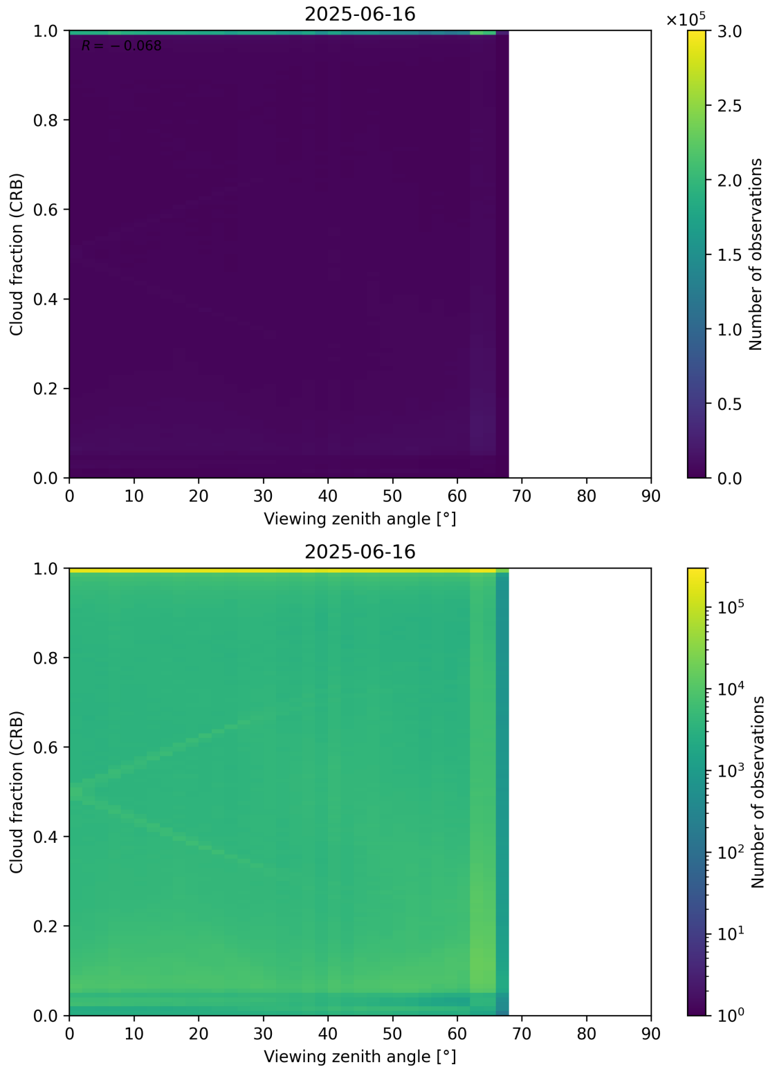
Figure 109: Scatter density plot of “Viewing zenith angle” against “Cloud fraction (CRB)” for 2025-06-16 to 2025-06-17.
