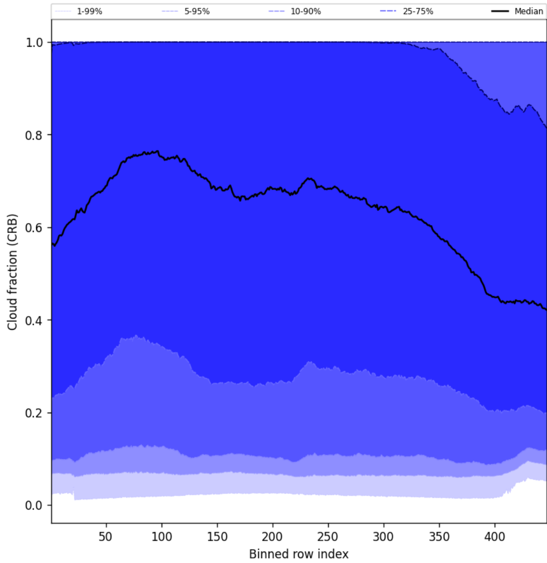
Figure 58: Along track statistics of “Cloud fraction (CRB)” for 2025-06-16 to 2025-06-17
