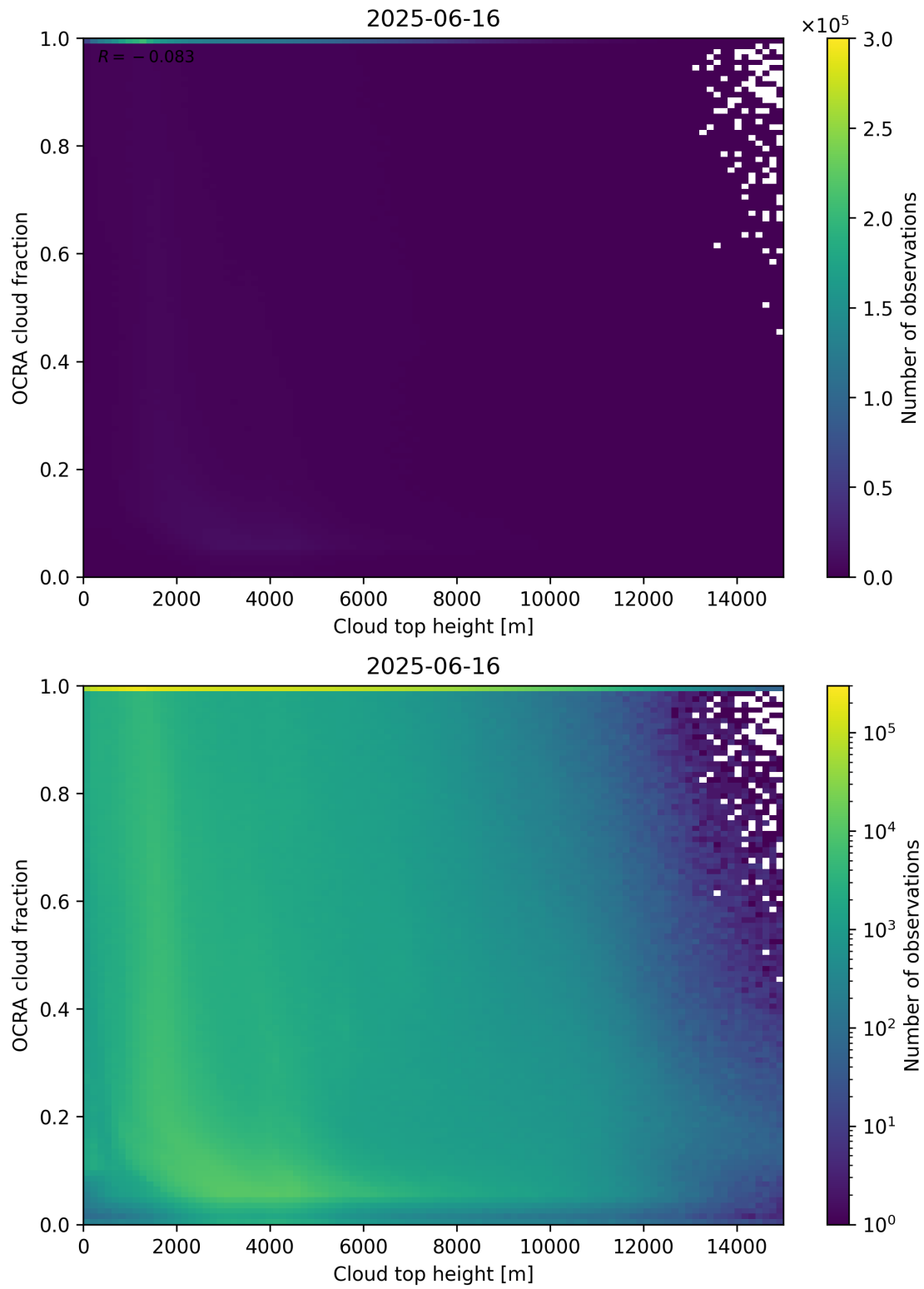
Figure 87: Scatter density plot of “Cloud top height” against “OCRA cloud fraction” for 2025-06-16 to 2025-06-17.
