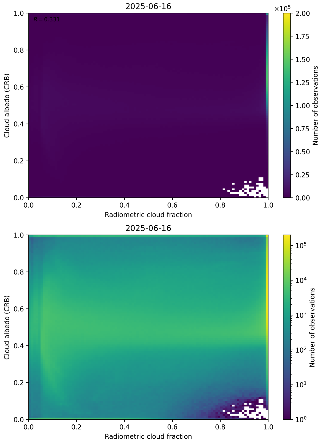
Figure 71: Scatter density plot of “Radiometric cloud fraction” against “Cloud albedo (CRB)” for 2025-06-16 to 2025-06-17.
