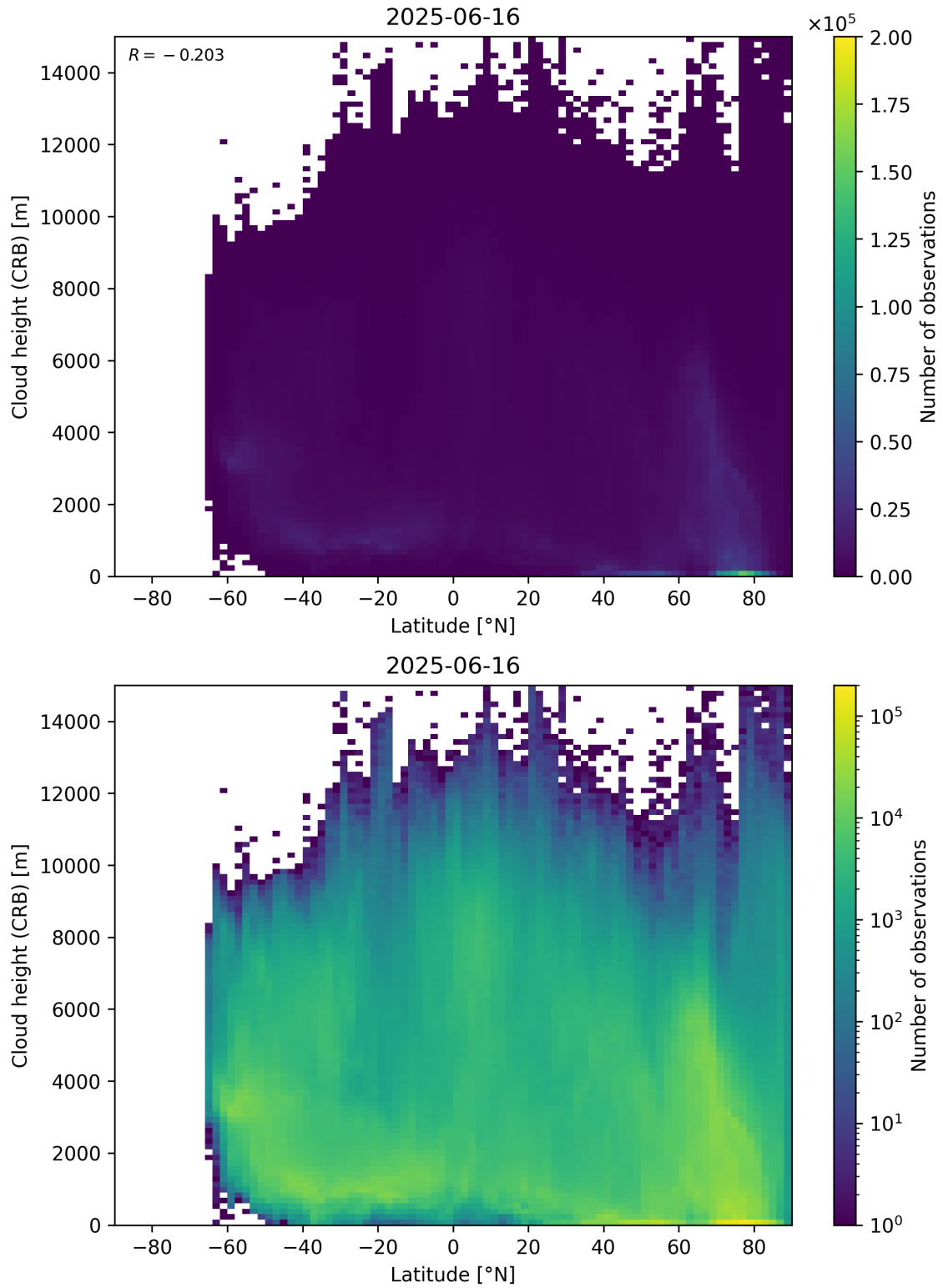
Figure 95: Scatter density plot of “Latitude” against “Cloud height (CRB)” for 2025-06-16 to 2025-06-17.
