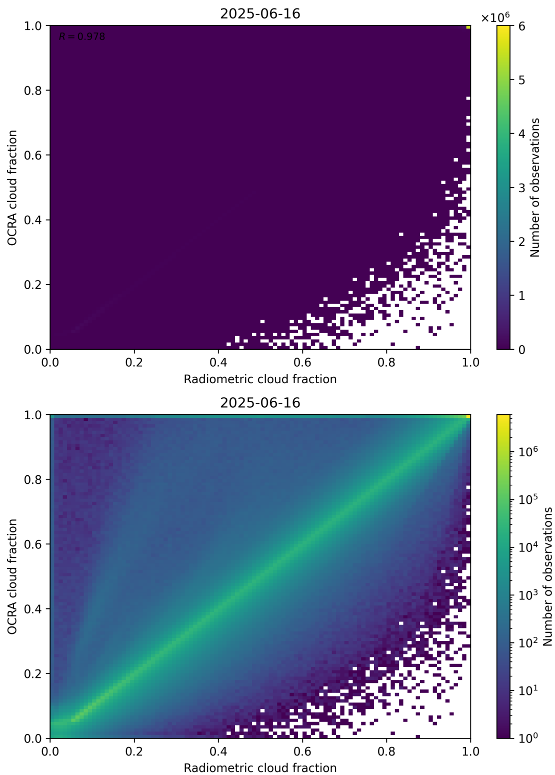
Figure 72: Scatter density plot of “Radiometric cloud fraction” against “OCRA cloud fraction” for 2025-06-16 to 2025-06-17.
