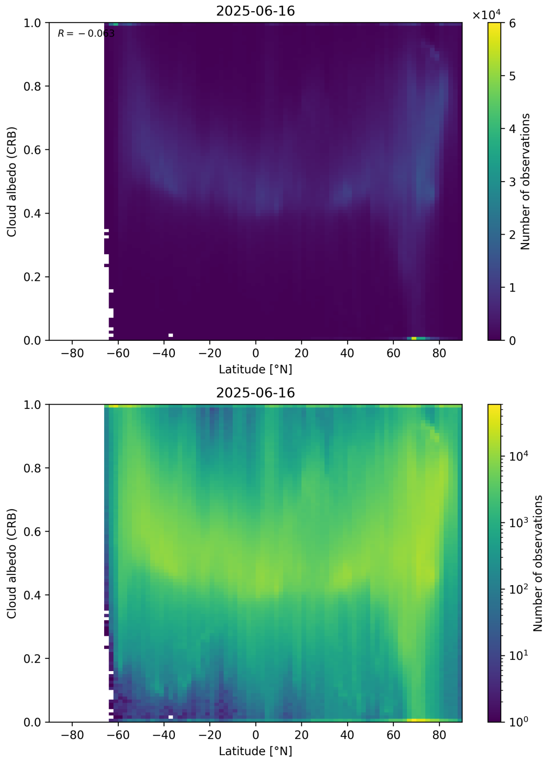
Figure 91: Scatter density plot of “Latitude” against “Cloud albedo (CRB)” for 2025-06-16 to 2025-06-17.
