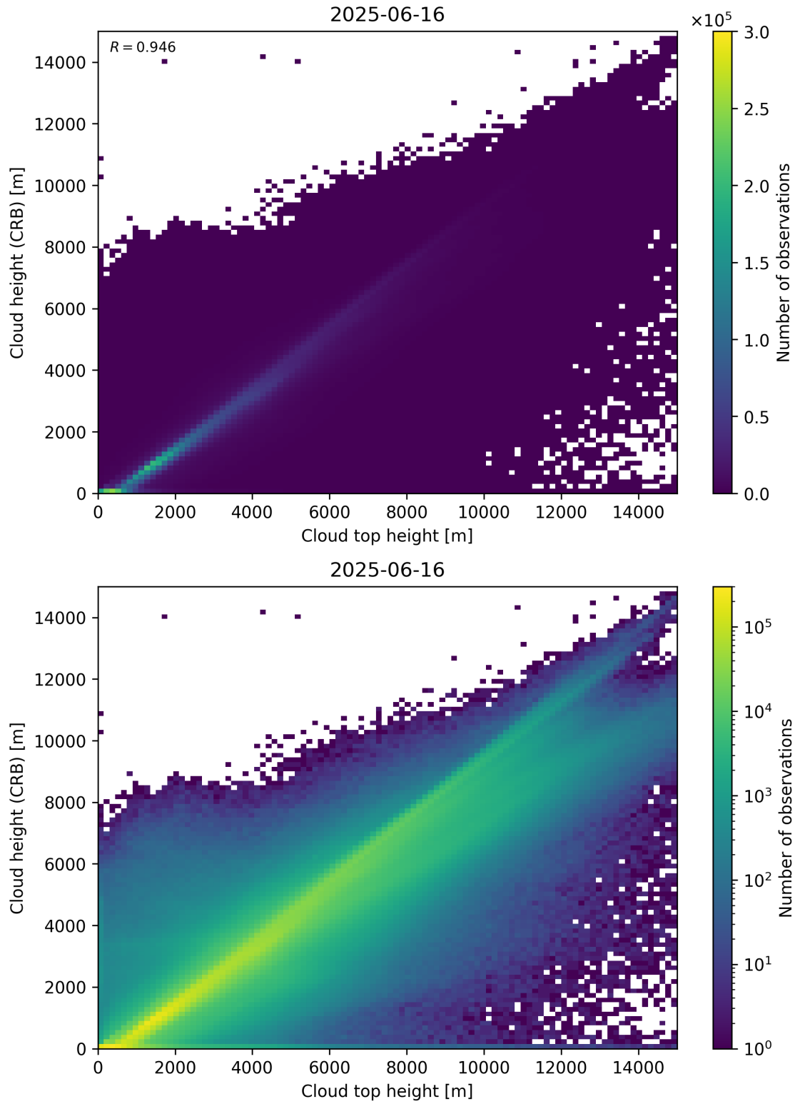
Figure 89: Scatter density plot of “Cloud top height” against “Cloud height (CRB)” for 2025-06-16 to 2025-06-17.
