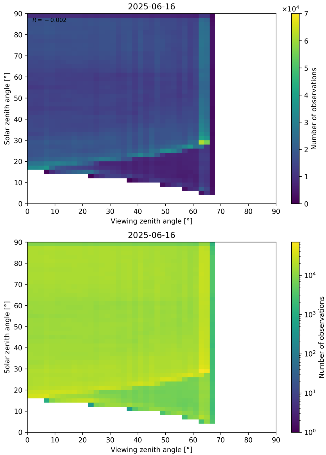
Figure 114: Scatter density plot of “Viewing zenith angle” against “Solar zenith angle” for 2025-06-16 to 2025-06-17.
