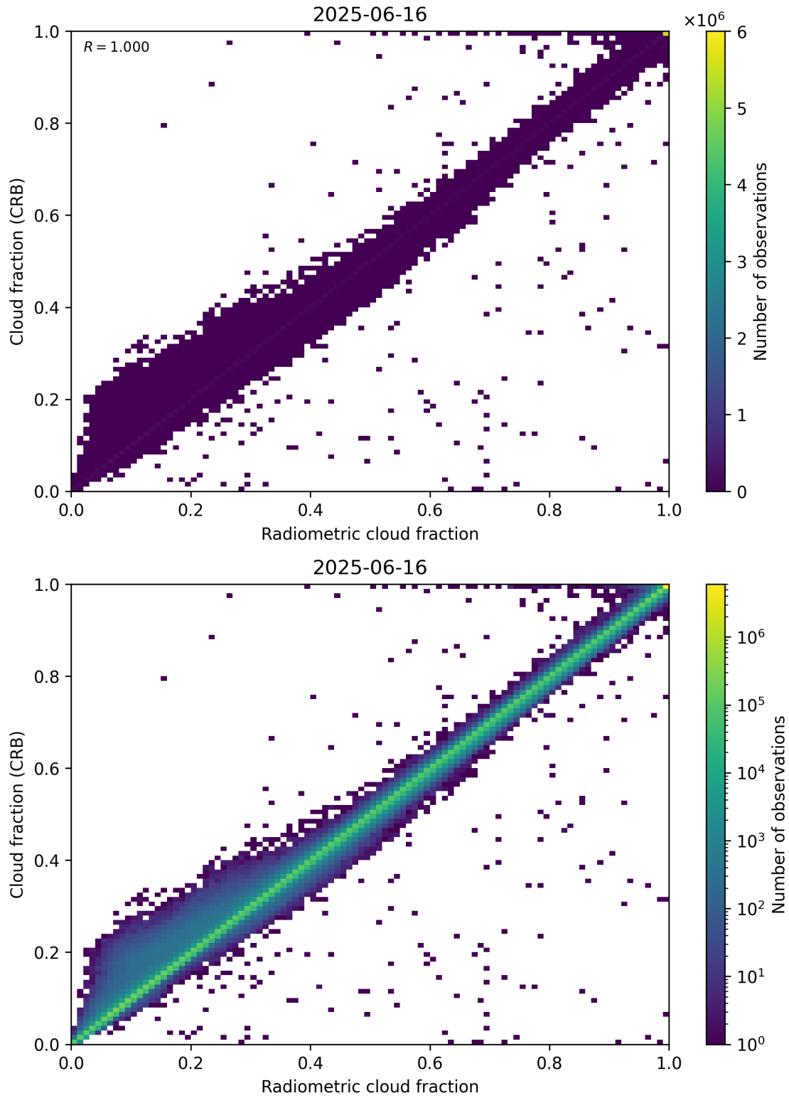
Figure 73: Scatter density plot of “Radiometric cloud fraction” against “Cloud fraction (CRB)” for 2025-06-16 to 2025-06-17.
