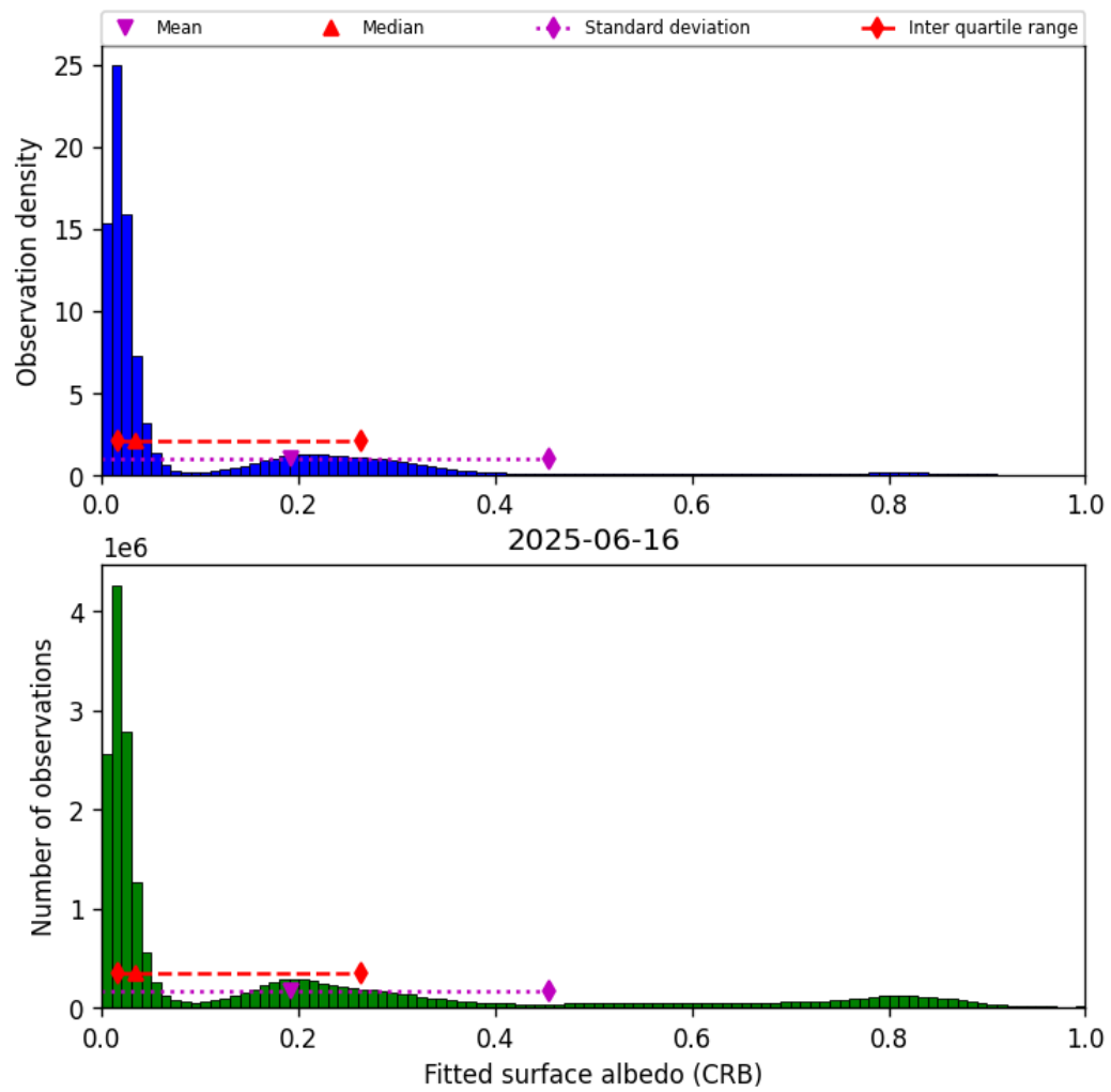
Figure 46: Histogram of “Fitted surface albedo (CRB)” for 2025-06-16 to 2025-06-17
