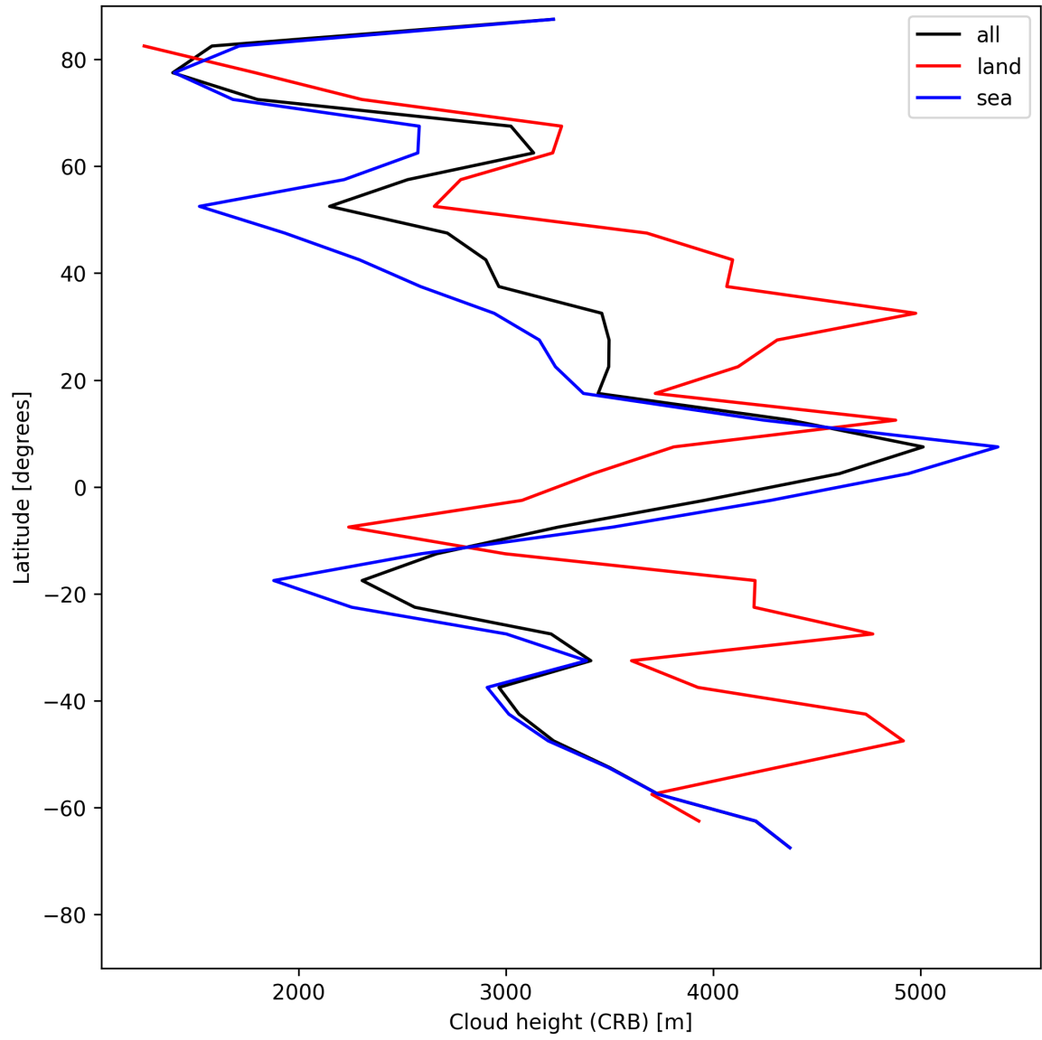
Figure 27: Zonal average of “Cloud height (CRB)” for 2025-06-16 to 2025-06-17.
