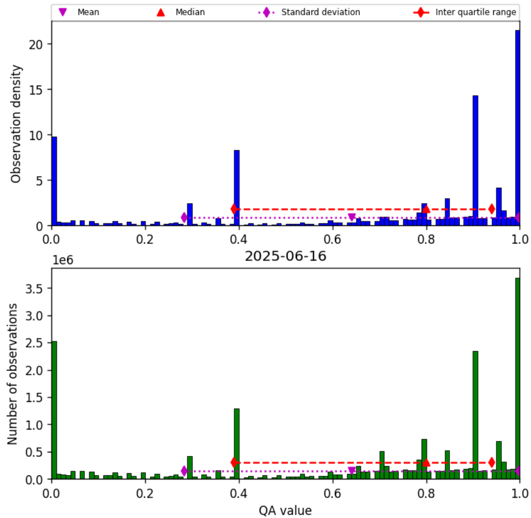
Figure 38: Histogram of “QA value” for 2025-06-16 to 2025-06-17
