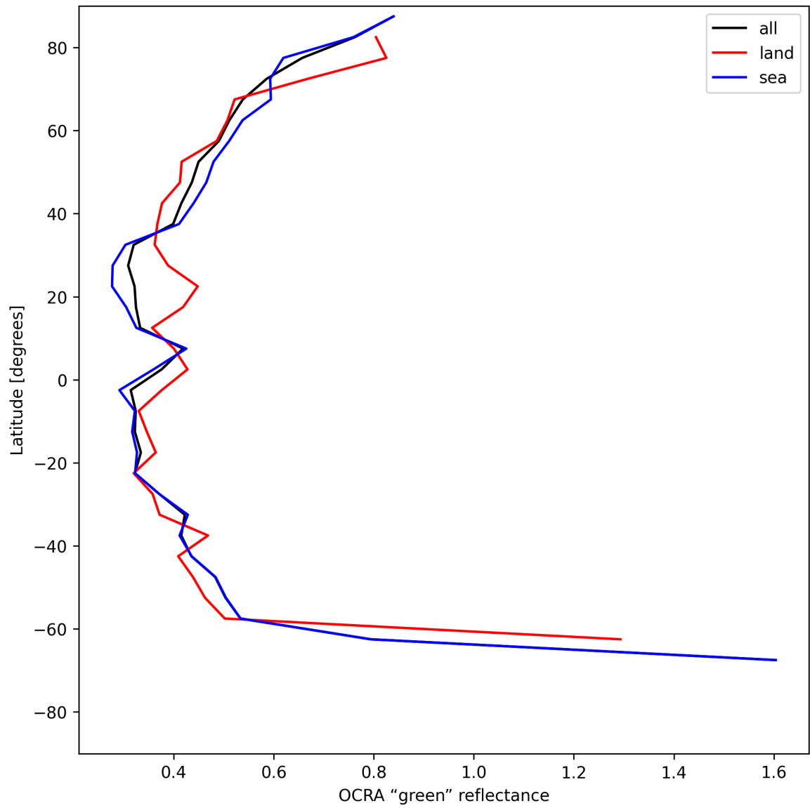
Figure 36: Zonal average of “OCRA “green” reflectance” for 2025-06-16 to 2025-06-17.
