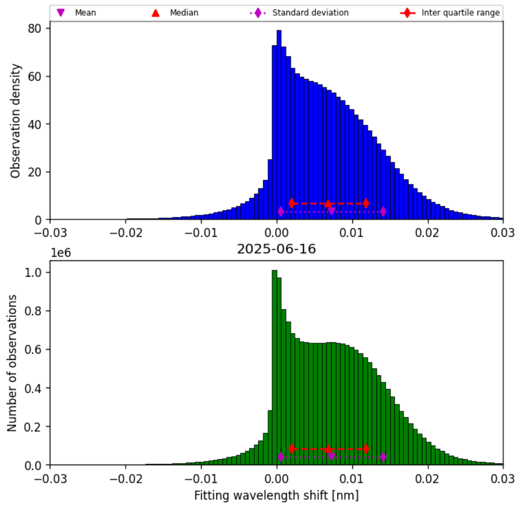
Figure 49: Histogram of “Fitting wavelength shift” for 2025-06-16 to 2025-06-17
