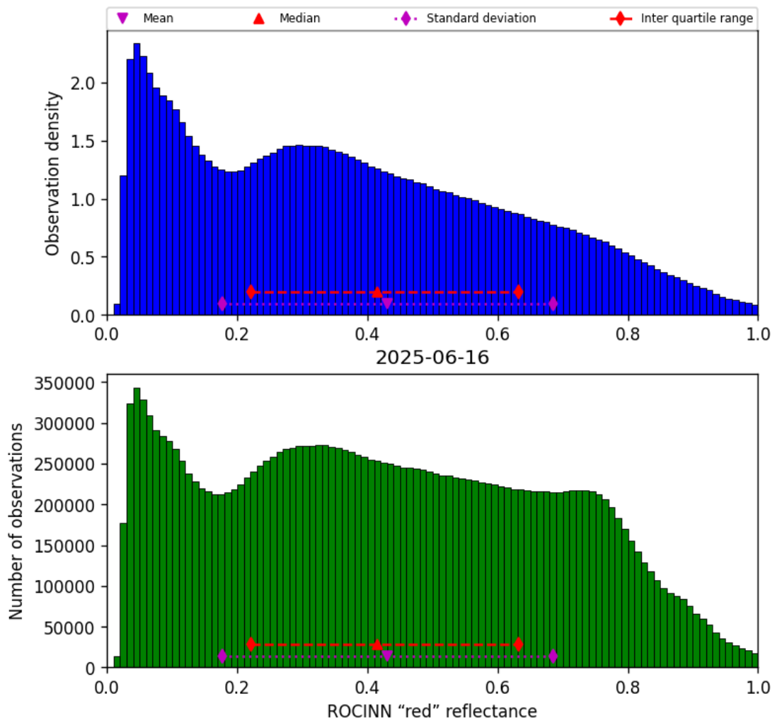
Figure 53: Histogram of “ROCINN “red” reflectance” for 2025-06-16 to 2025-06-17
