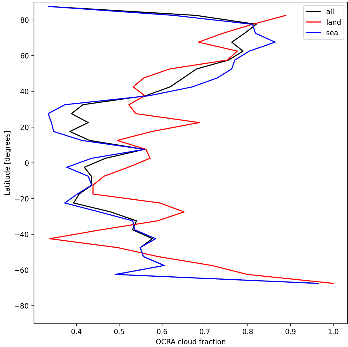
Figure 34: Zonal average of “OCRA cloud fraction” for 2025-06-17 to 2025-06-18.
