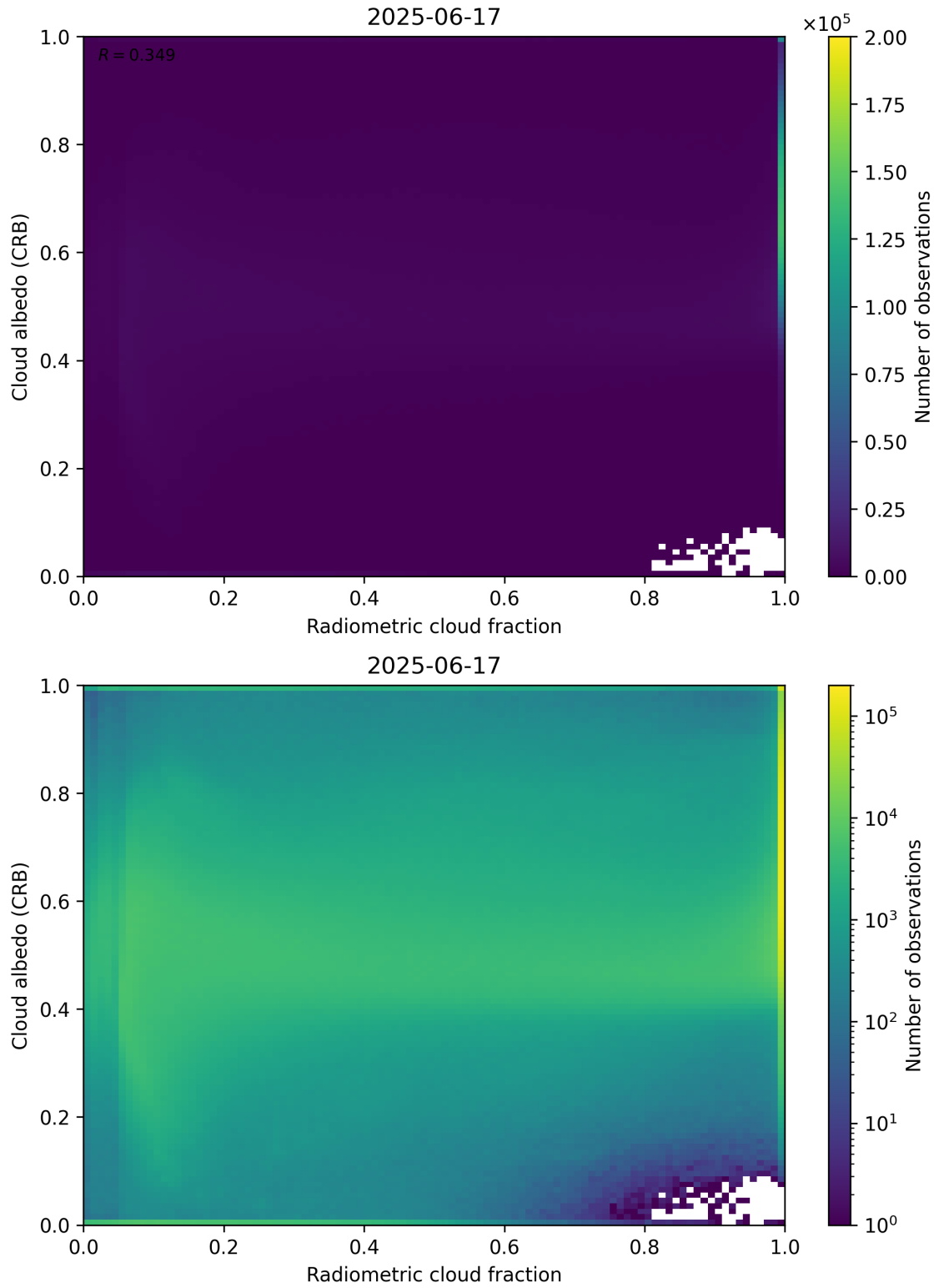
Figure 71: Scatter density plot of “Radiometric cloud fraction” against “Cloud albedo (CRB)” for 2025-06-17 to 2025-06-18.
