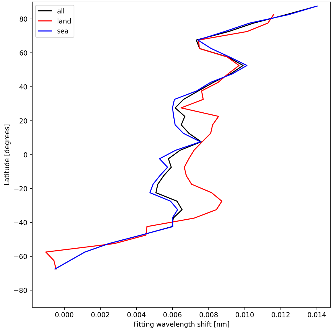
Figure 33: Zonal average of “Fitting wavelength shift” for 2025-06-17 to 2025-06-18.
