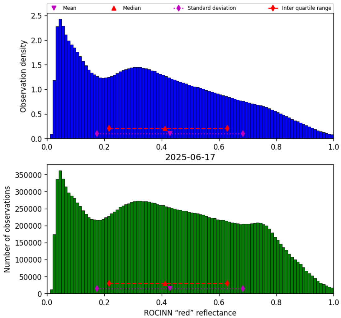
Figure 53: Histogram of “ROCINN “red” reflectance” for 2025-06-17 to 2025-06-18
