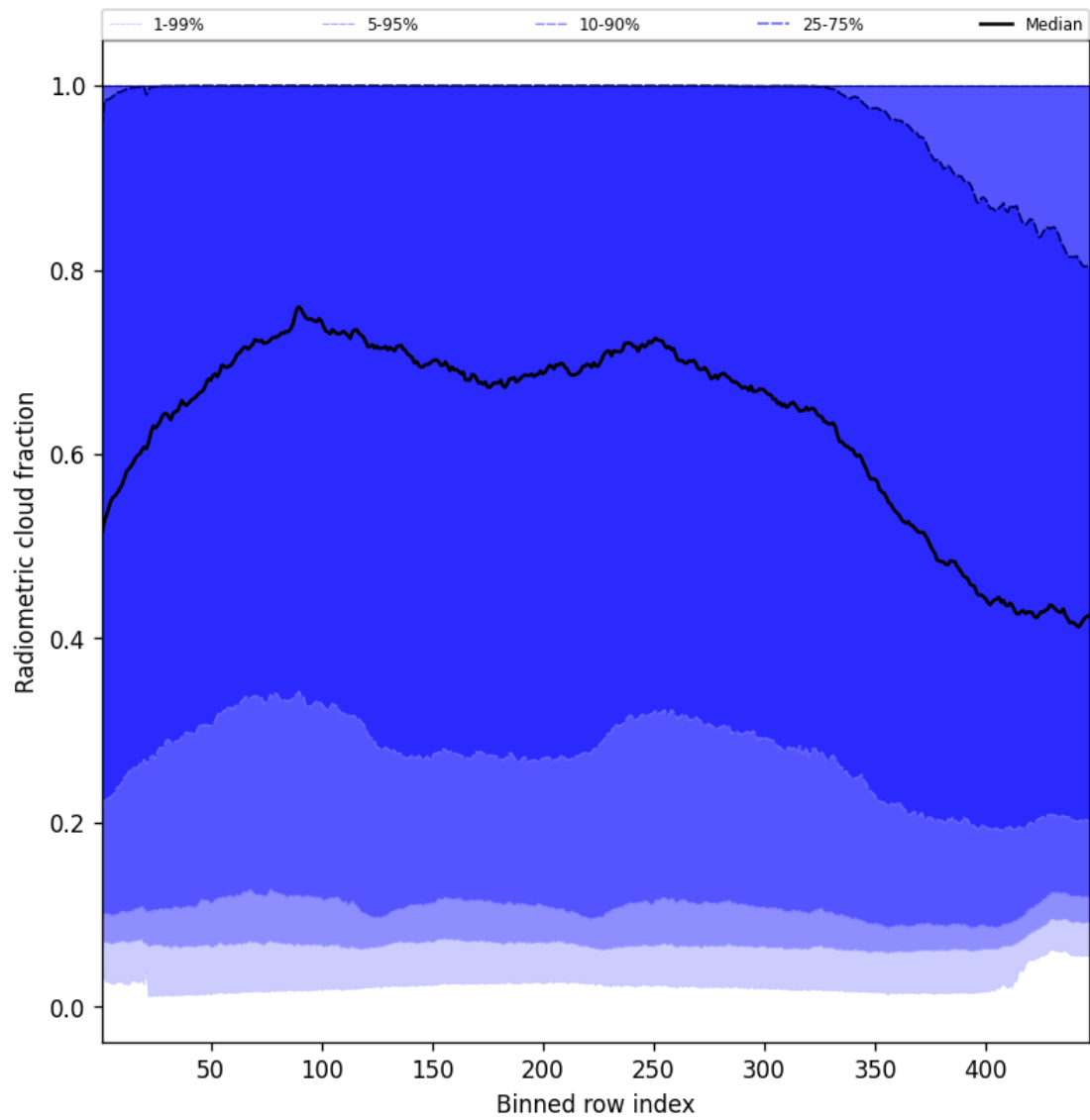
Figure 55: Along track statistics of “Radiometric cloud fraction” for 2025-06-17 to 2025-06-18
