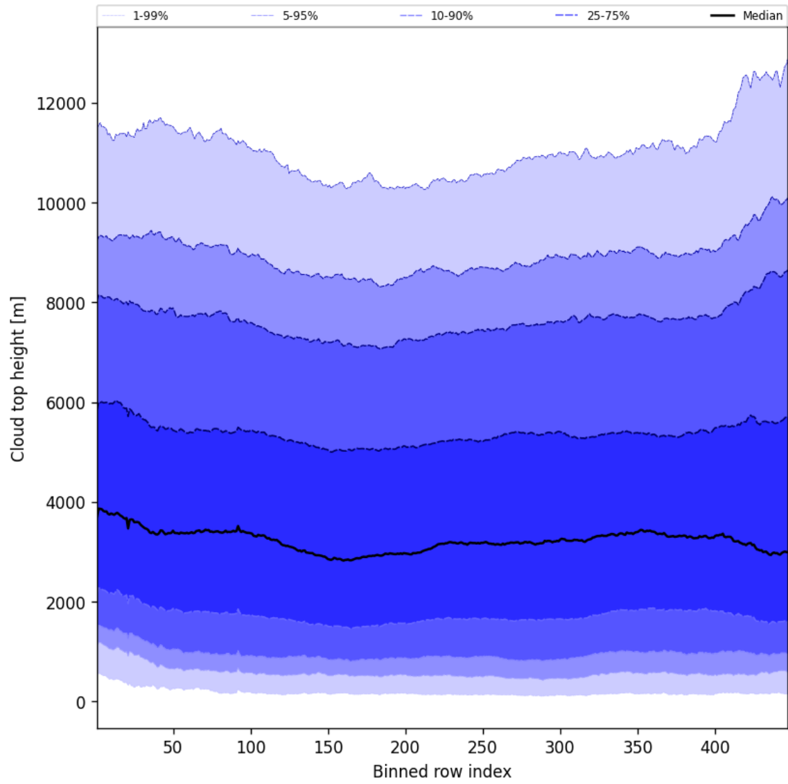
Figure 56: Along track statistics of “Cloud top height” for 2025-06-17 to 2025-06-18
