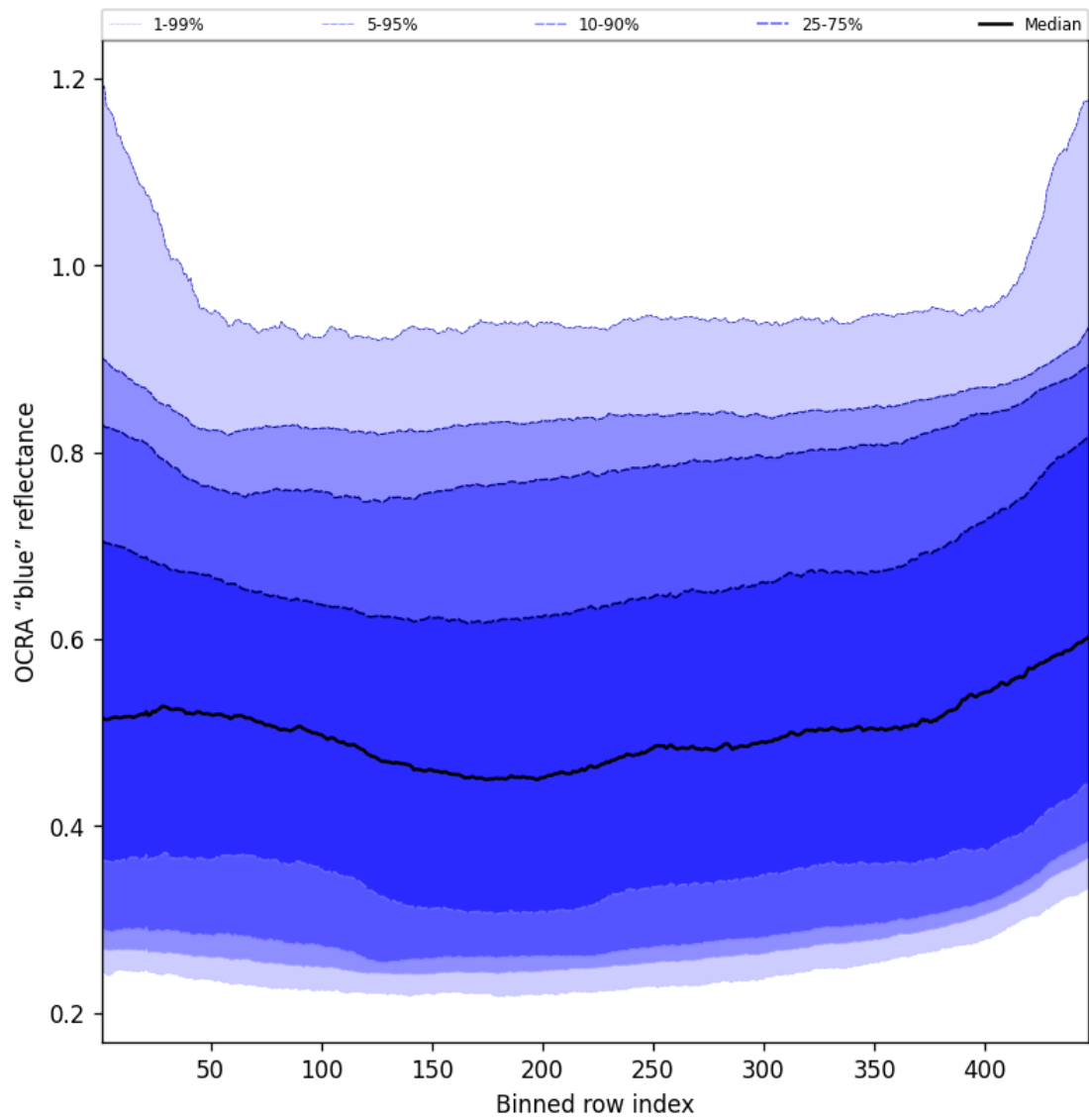
Figure 67: Along track statistics of "OCRA "blue" reflectance" for 2025-06-17 to 2025-06-18
