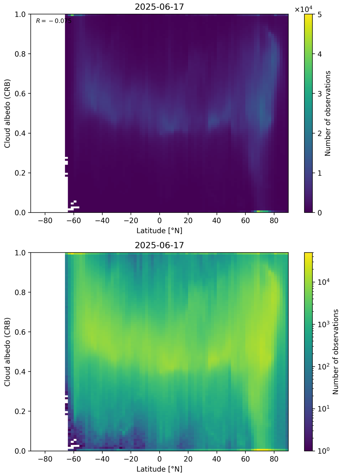
Figure 91: Scatter density plot of “Latitude” against “Cloud albedo (CRB)” for 2025-06-17 to 2025-06-18.
