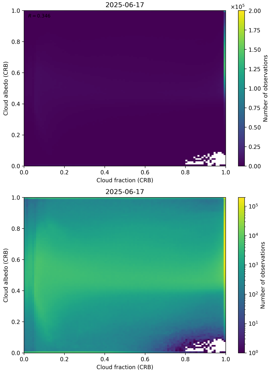
Figure 77: Scatter density plot of “Cloud fraction (CRB)” against “Cloud albedo (CRB)” for 2025-06-17 to 2025-06-18.
