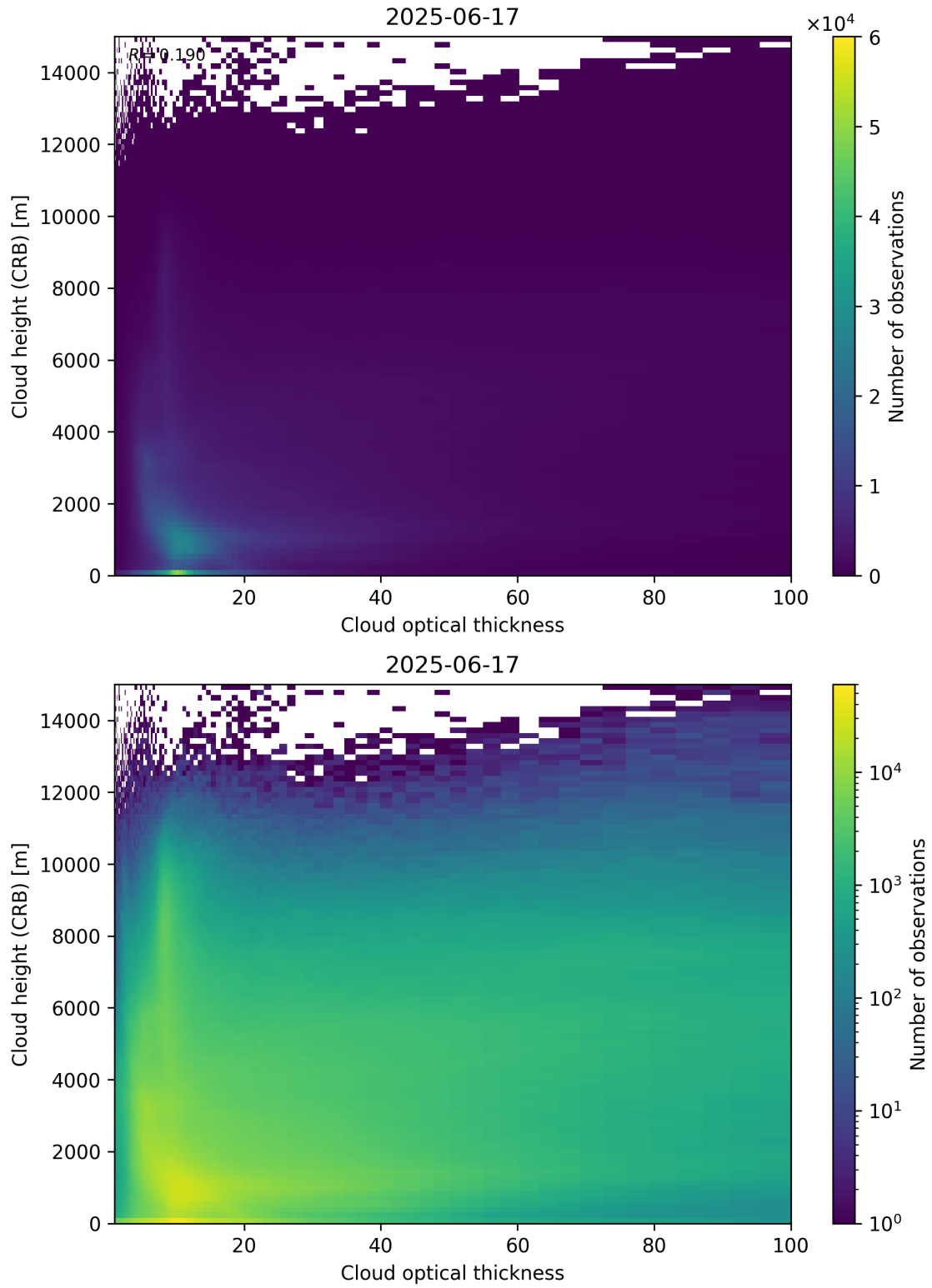
Figure 85: Scatter density plot of “Cloud optical thickness” against “Cloud height (CRB)” for 2025-06-17 to 2025-06-18.
