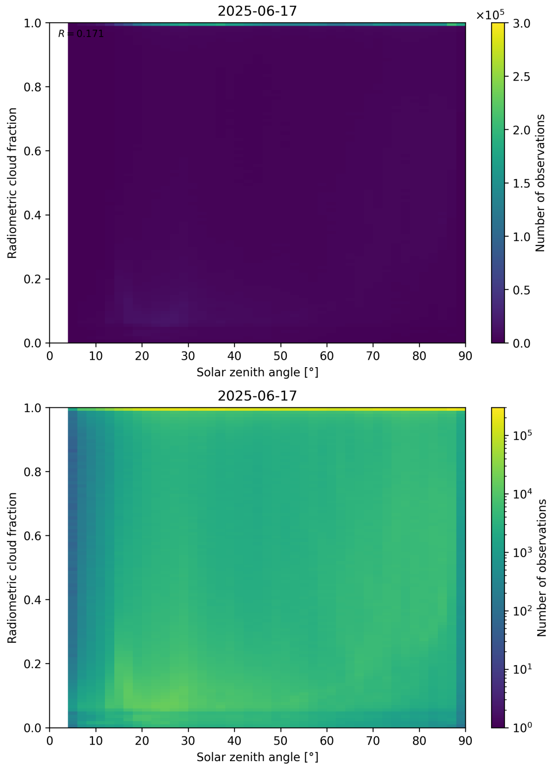
Figure 99: Scatter density plot of “Solar zenith angle” against “Radiometric cloud fraction” for 2025-06-17 to 2025-06-18.
