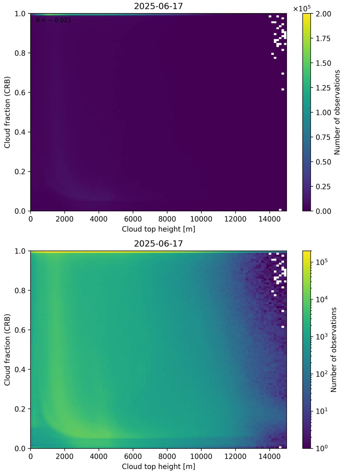
Figure 88: Scatter density plot of “Cloud top height” against “Cloud fraction (CRB)” for 2025-06-17 to 2025-06-18.
