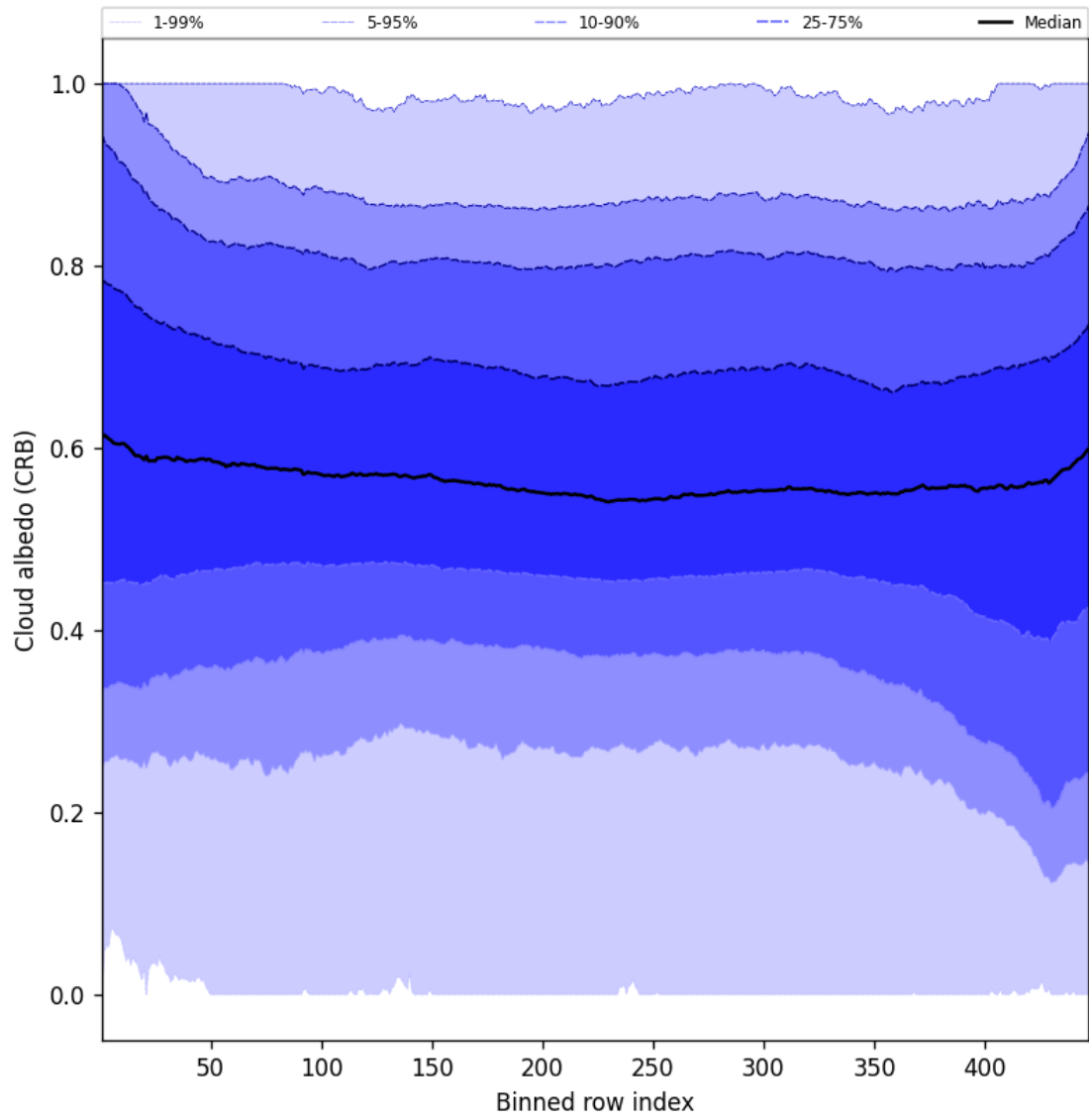
Figure 60: Along track statistics of “Cloud albedo (CRB)” for 2025-06-17 to 2025-06-18
