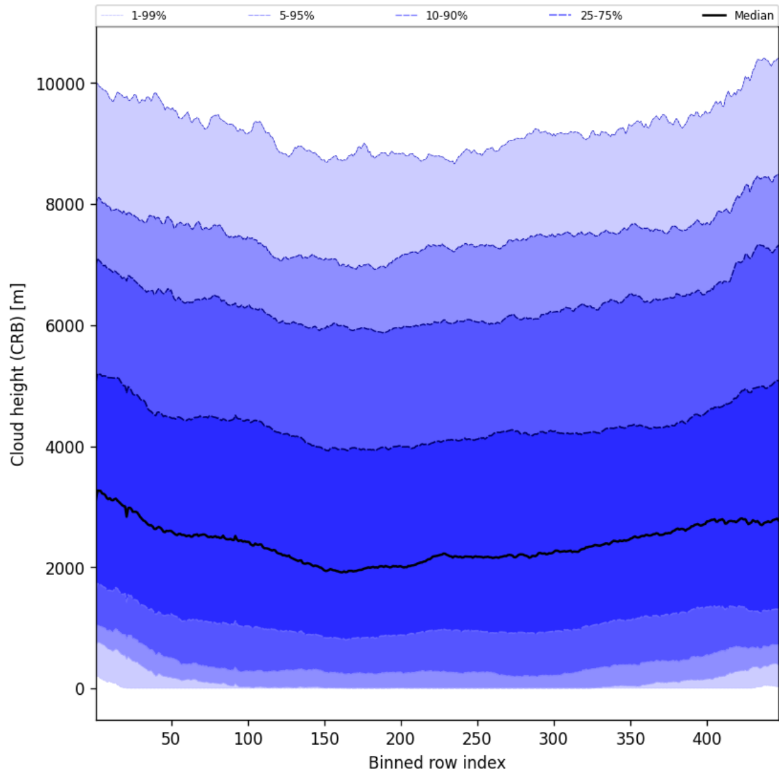
Figure 59: Along track statistics of “Cloud height (CRB)” for 2025-06-17 to 2025-06-18
