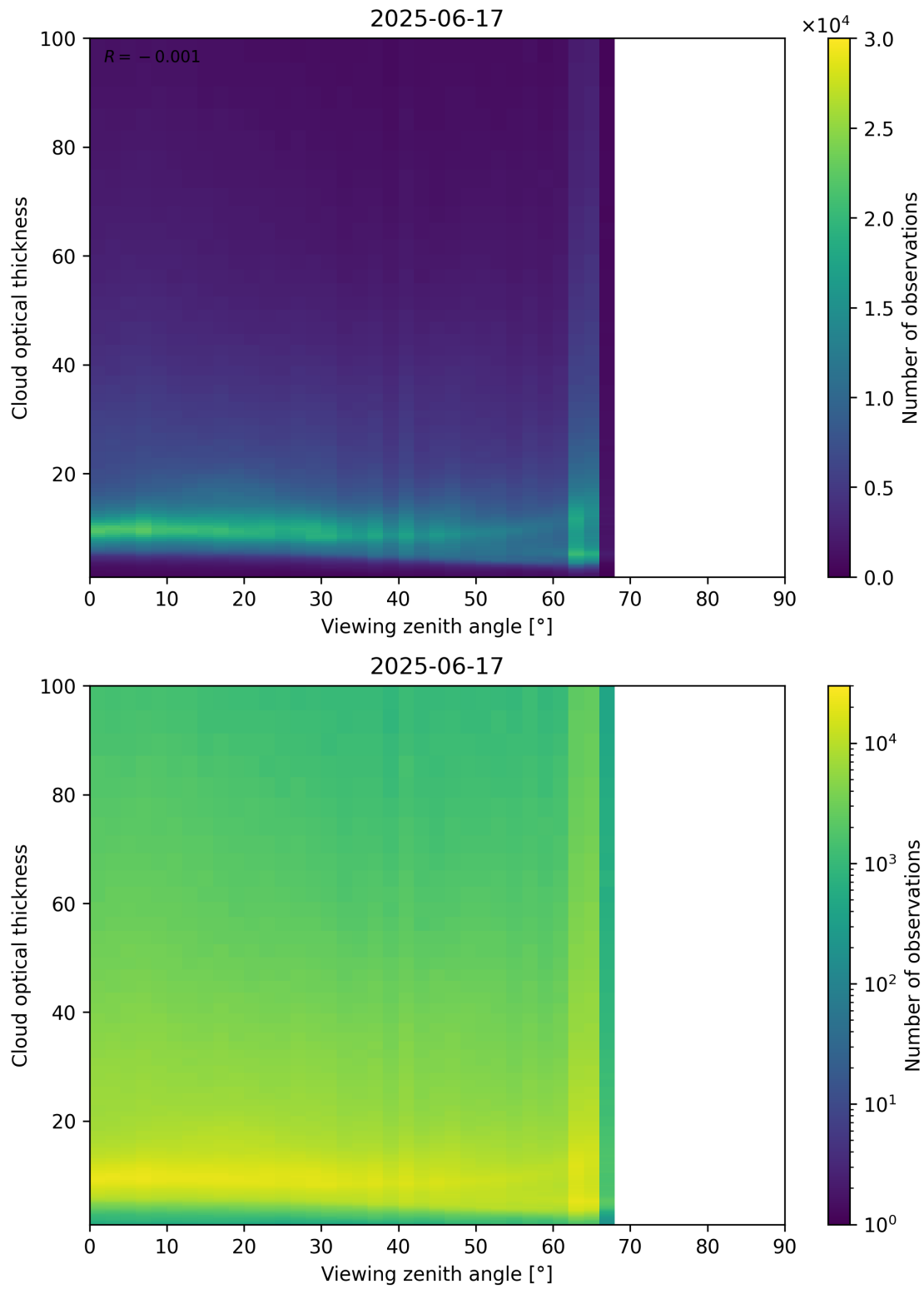
Figure 111: Scatter density plot of “Viewing zenith angle” against “Cloud optical thickness” for 2025-06-17 to 2025-06-18.
