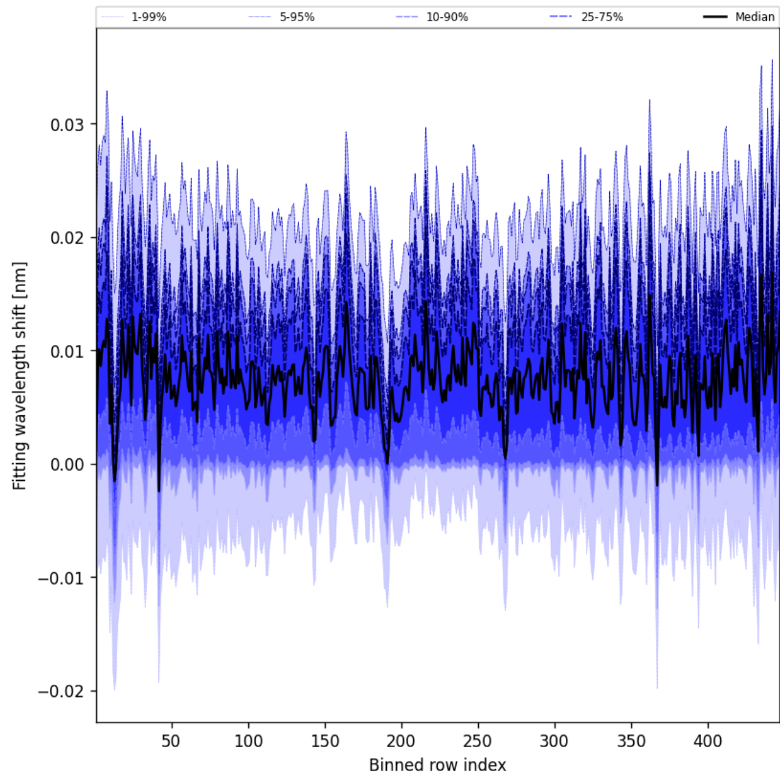
Figure 65: Along track statistics of “Fitting wavelength shift” for 2025-06-17 to 2025-06-18
