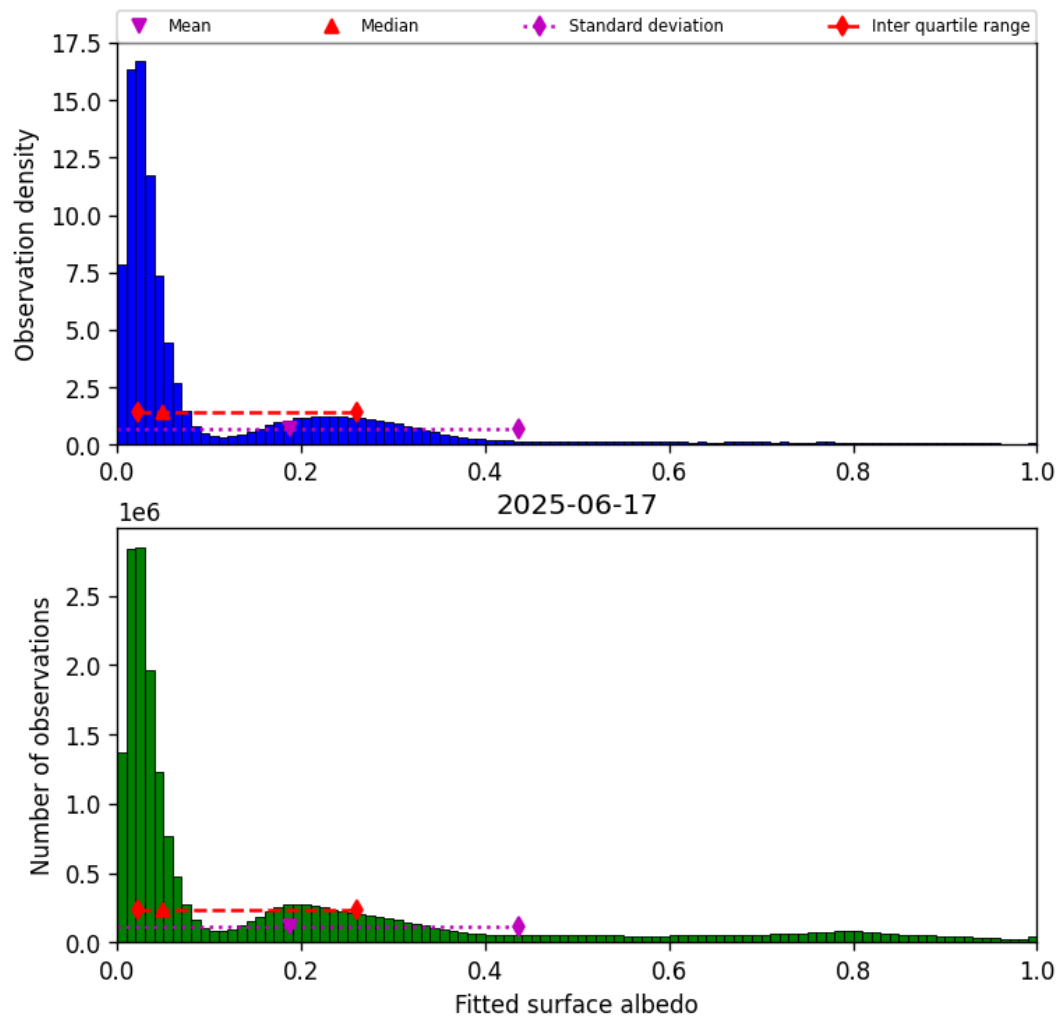
Figure 45: Histogram of “Fitted surface albedo” for 2025-06-17 to 2025-06-18
