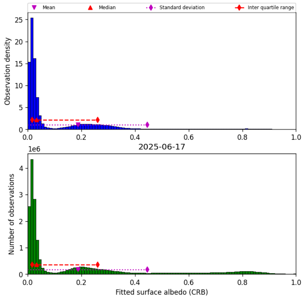
Figure 46: Histogram of “Fitted surface albedo (CRB)” for 2025-06-17 to 2025-06-18
