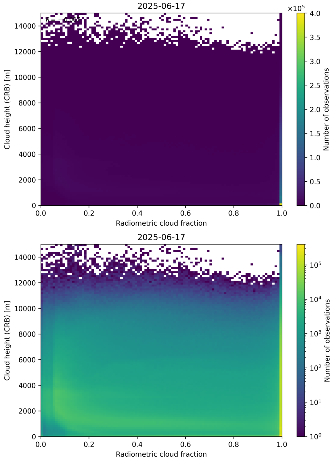
Figure 74: Scatter density plot of “Radiometric cloud fraction” against “Cloud height (CRB)” for 2025-06-17 to 2025-06-18.
