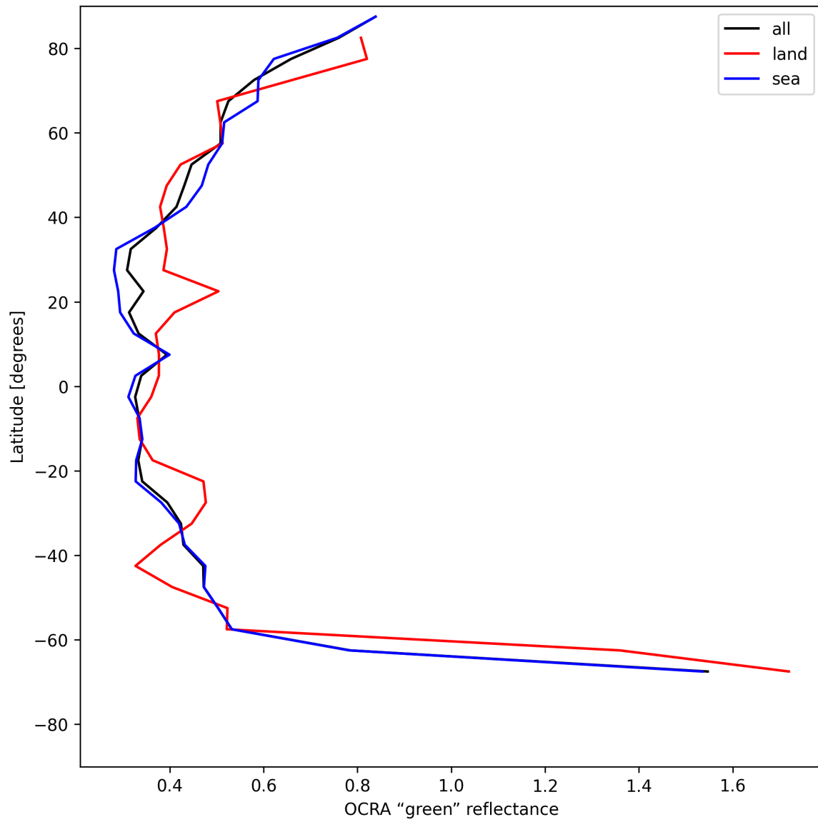
Figure 36: Zonal average of “OCRA “green” reflectance” for 2025-06-17 to 2025-06-18.
