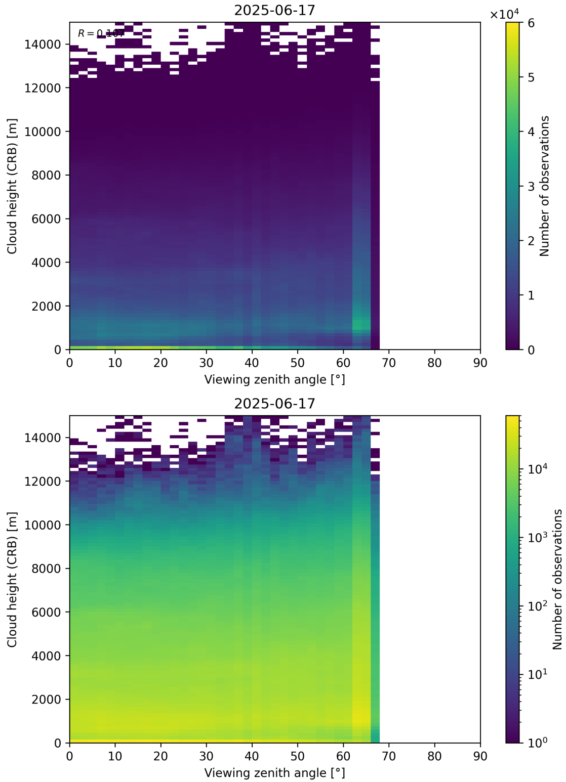
Figure 110: Scatter density plot of “Viewing zenith angle” against “Cloud height (CRB)” for 2025-06-17 to 2025-06-18.
