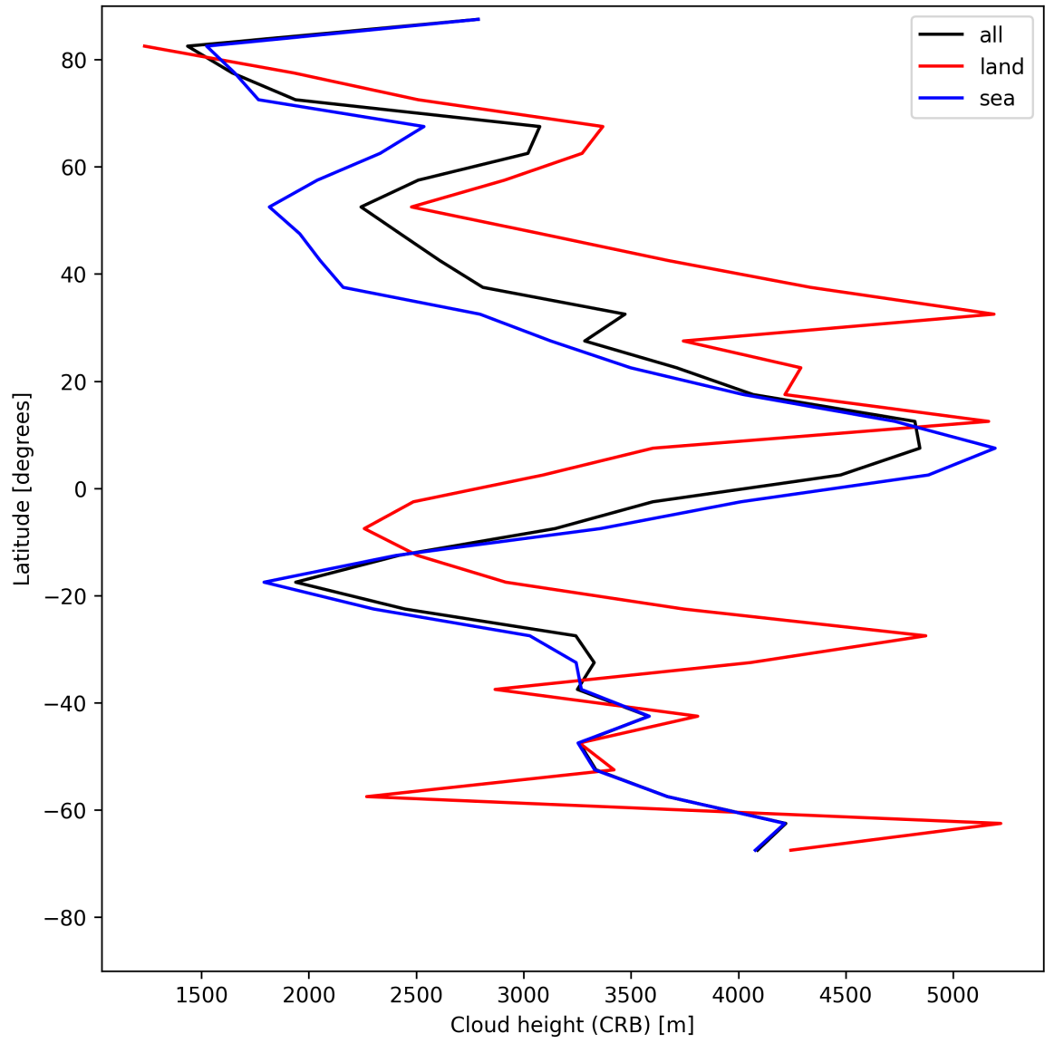
Figure 27: Zonal average of “Cloud height (CRB)” for 2025-06-17 to 2025-06-18.
