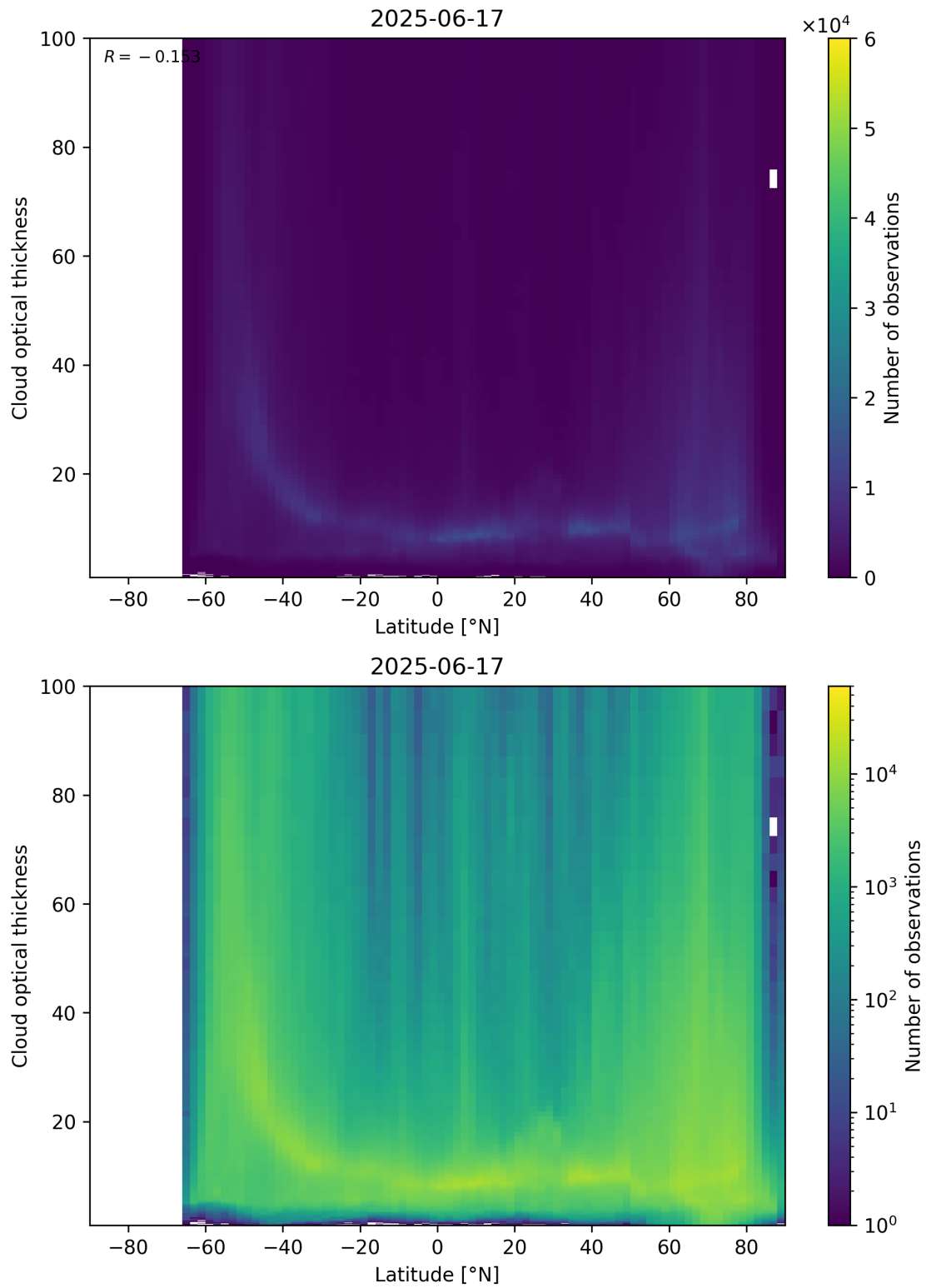
Figure 96: Scatter density plot of “Latitude” against “Cloud optical thickness” for 2025-06-17 to 2025-06-18.
