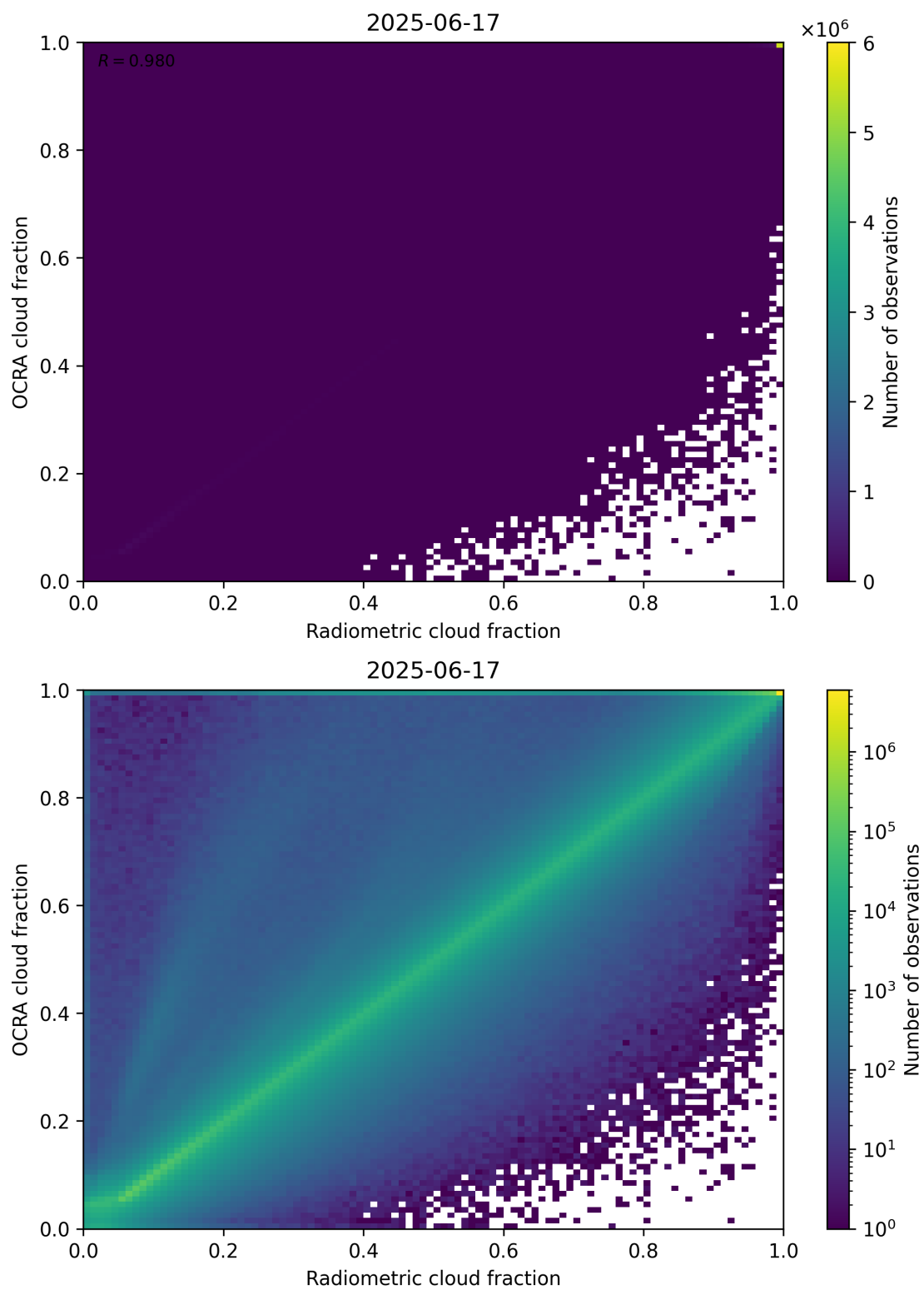
Figure 72: Scatter density plot of “Radiometric cloud fraction” against “OCRA cloud fraction” for 2025-06-17 to 2025-06-18.
