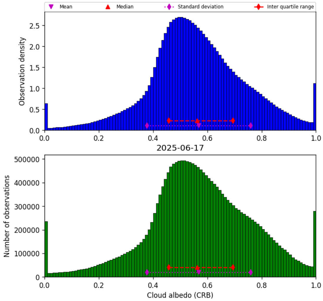
Figure 44: Histogram of “Cloud albedo (CRB)” for 2025-06-17 to 2025-06-18
