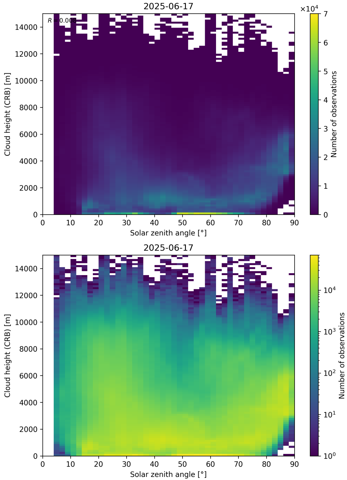
Figure 102: Scatter density plot of “Solar zenith angle” against “Cloud height (CRB)” for 2025-06-17 to 2025-06-18.
