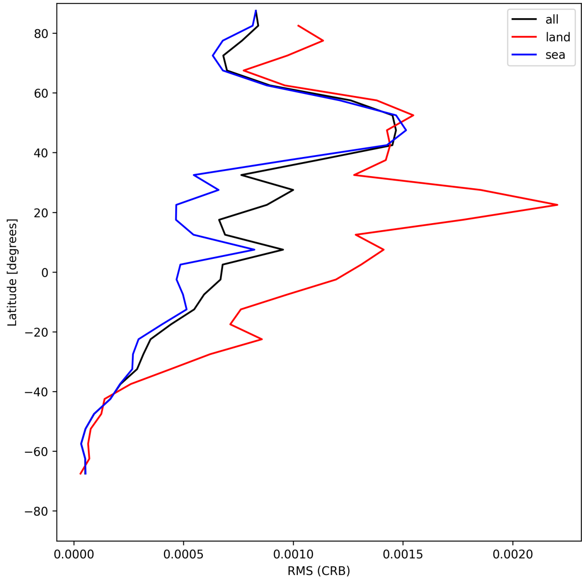
Figure 32: Zonal average of “RMS (CRB)” for 2025-06-17 to 2025-06-18.
