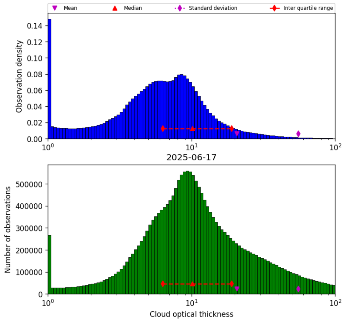
Figure 41: Histogram of “Cloud optical thickness” for 2025-06-17 to 2025-06-18
