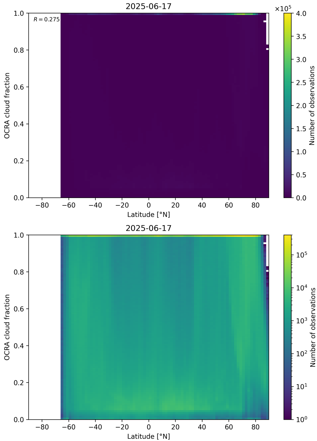
Figure 93: Scatter density plot of “Latitude” against “OCRA cloud fraction” for 2025-06-17 to 2025-06-18.
