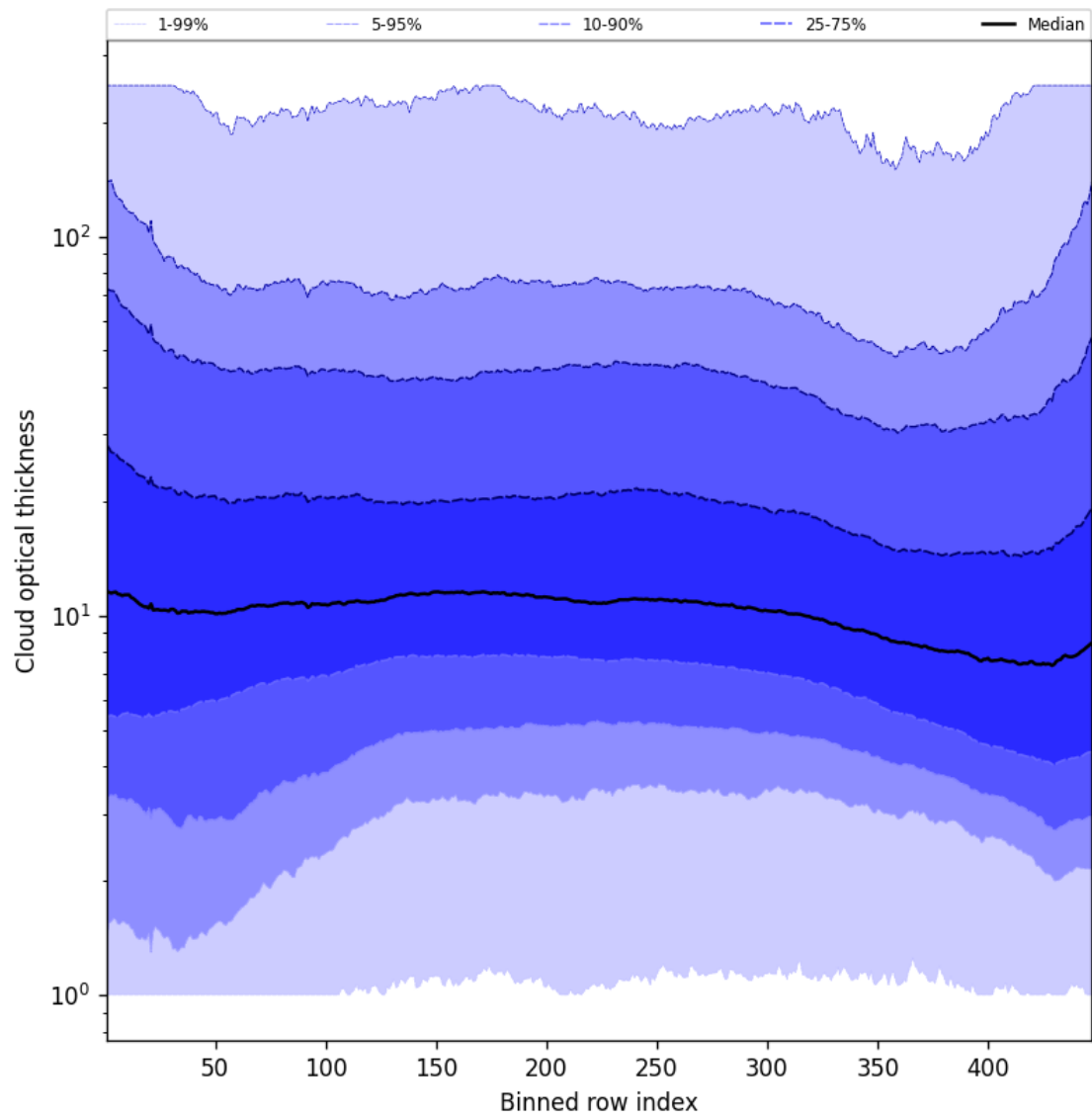
Figure 57: Along track statistics of “Cloud optical thickness” for 2025-06-17 to 2025-06-18
