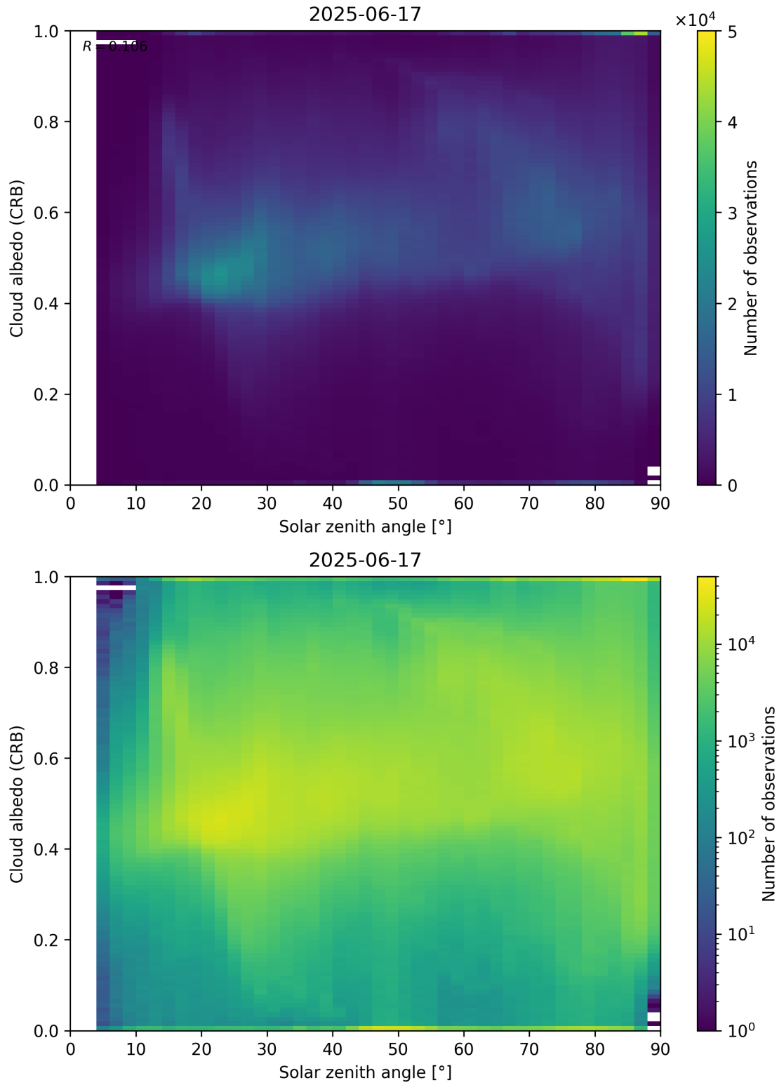
Figure 98: Scatter density plot of “Solar zenith angle” against “Cloud albedo (CRB)” for 2025-06-17 to 2025-06-18.
