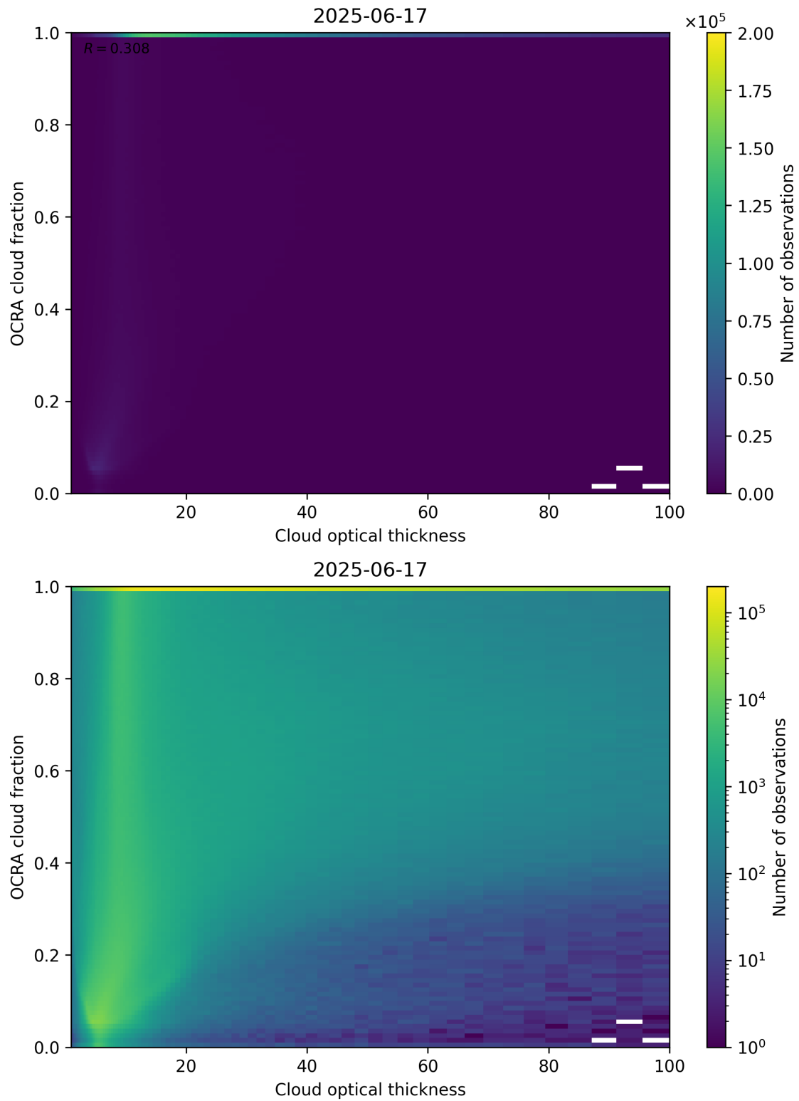
Figure 83: Scatter density plot of “Cloud optical thickness” against “OCRA cloud fraction” for 2025-06-17 to 2025-06-18.
