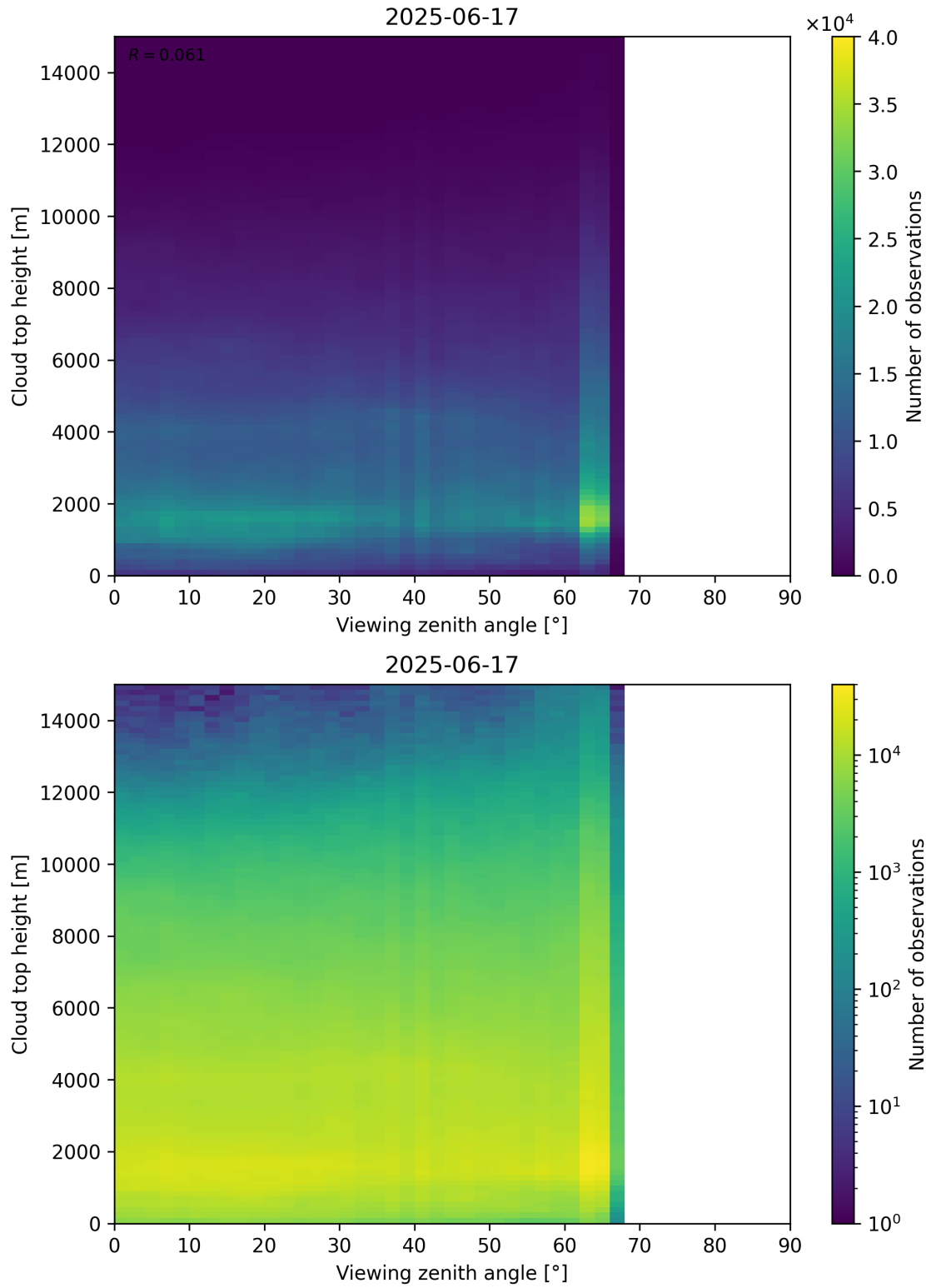
Figure 112: Scatter density plot of “Viewing zenith angle” against “Cloud top height” for 2025-06-17 to 2025-06-18.
