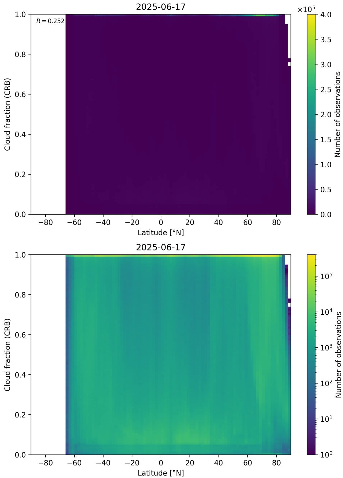
Figure 94: Scatter density plot of “Latitude” against “Cloud fraction (CRB)” for 2025-06-17 to 2025-06-18.
