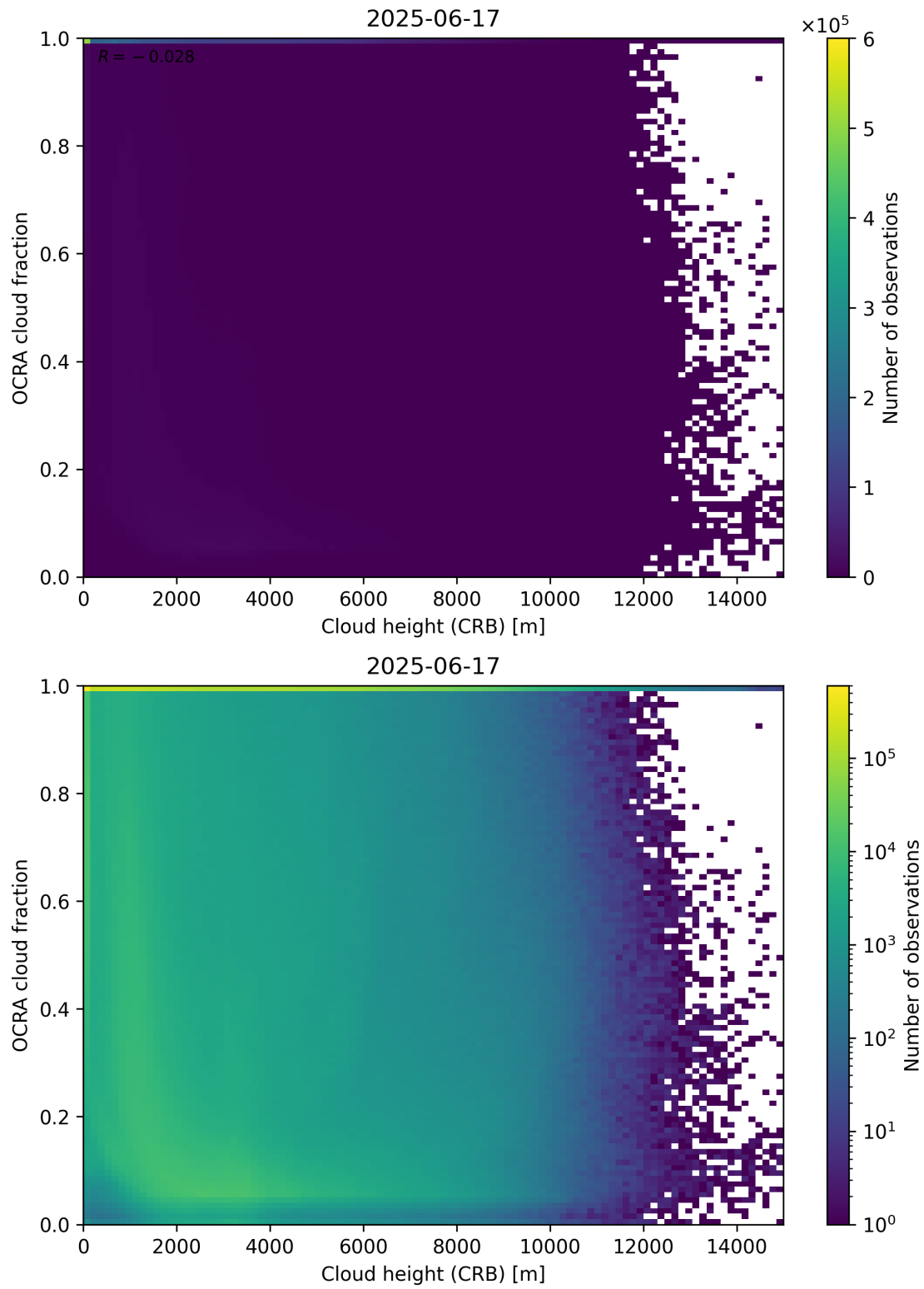
Figure 81: Scatter density plot of “Cloud height (CRB)” against “OCRA cloud fraction” for 2025-06-17 to 2025-06-18.
