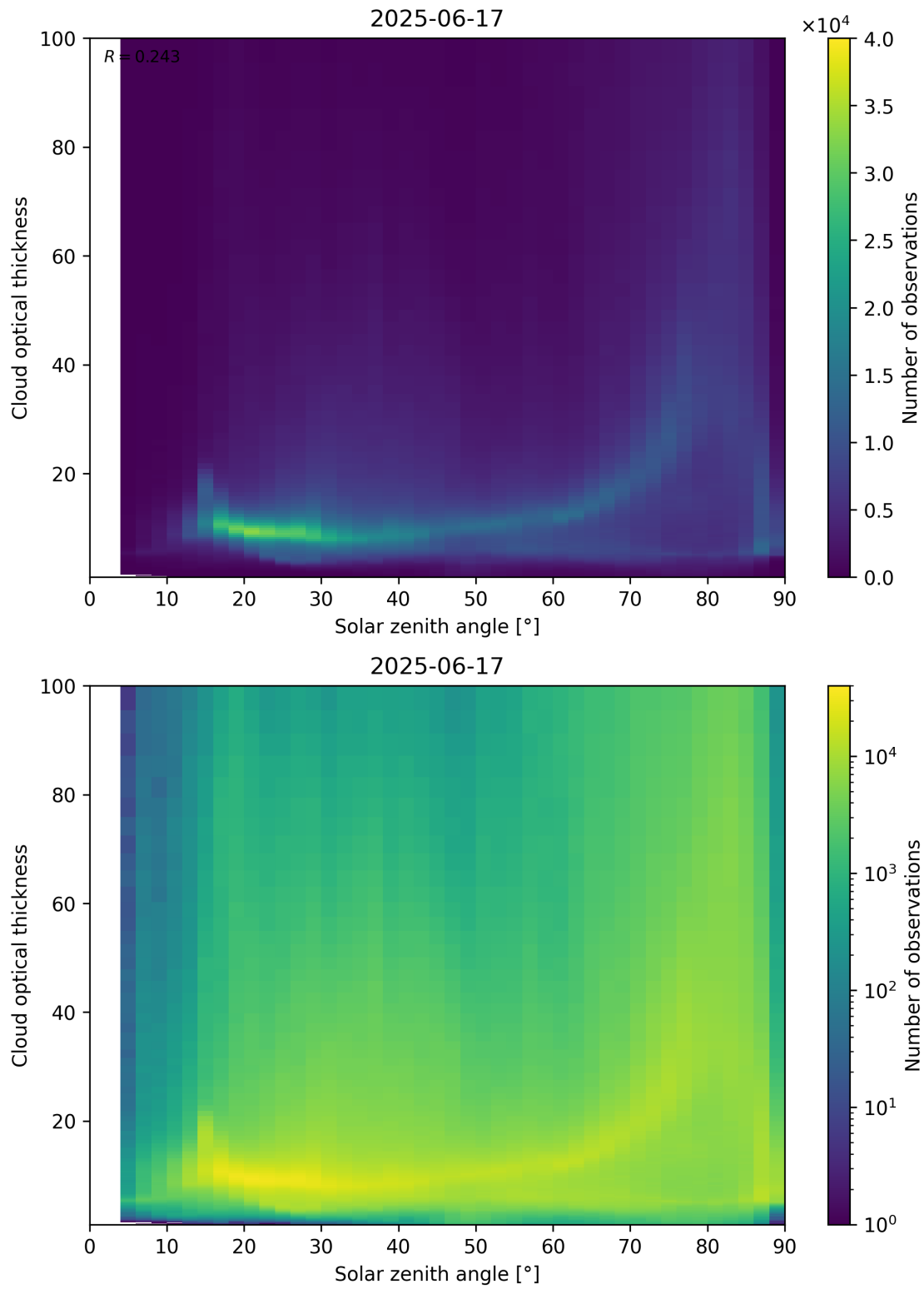
Figure 103: Scatter density plot of “Solar zenith angle” against “Cloud optical thickness” for 2025-06-17 to 2025-06-18.
