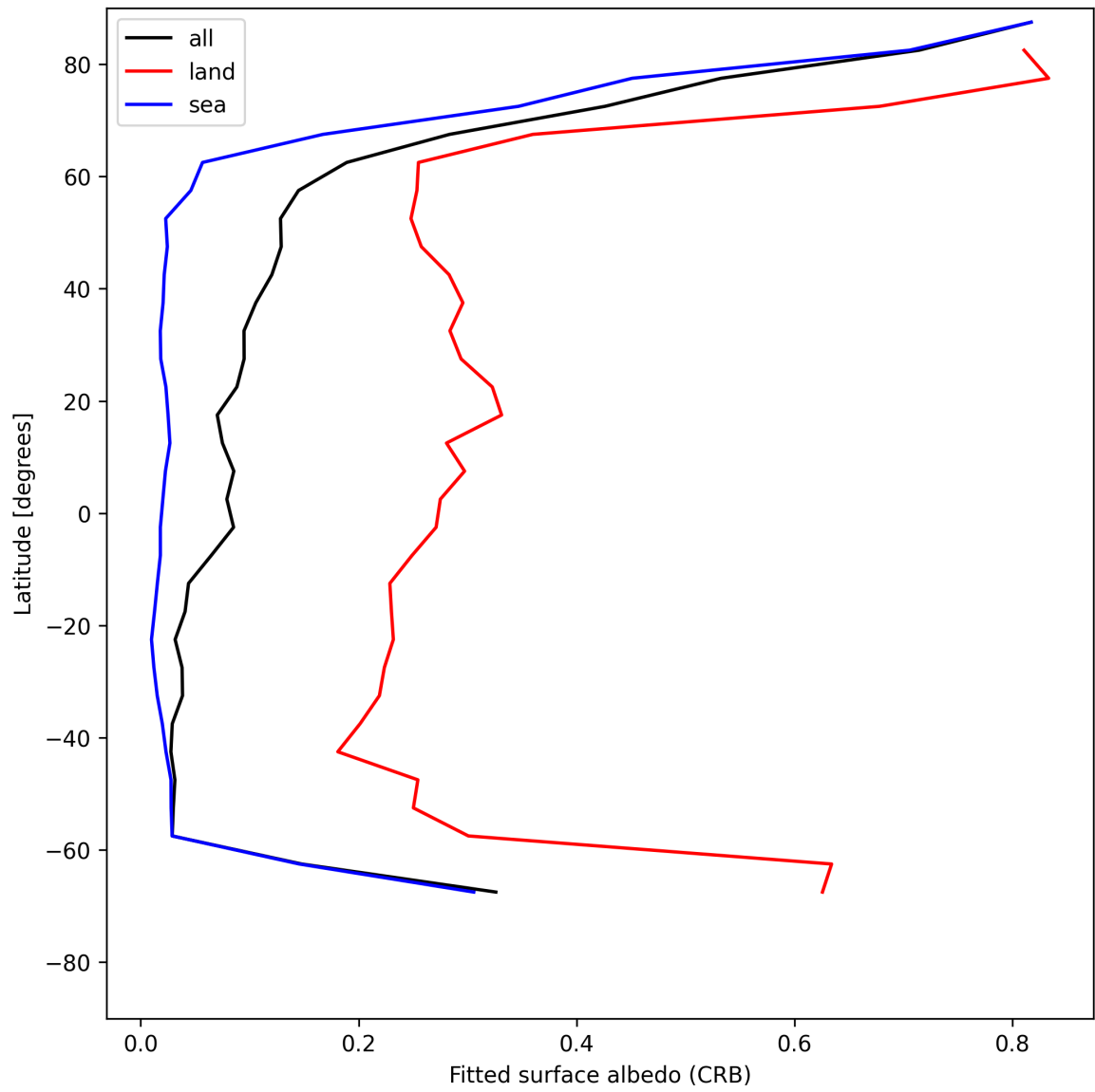
Figure 30: Zonal average of “Fitted surface albedo (CRB)” for 2025-06-17 to 2025-06-18.
