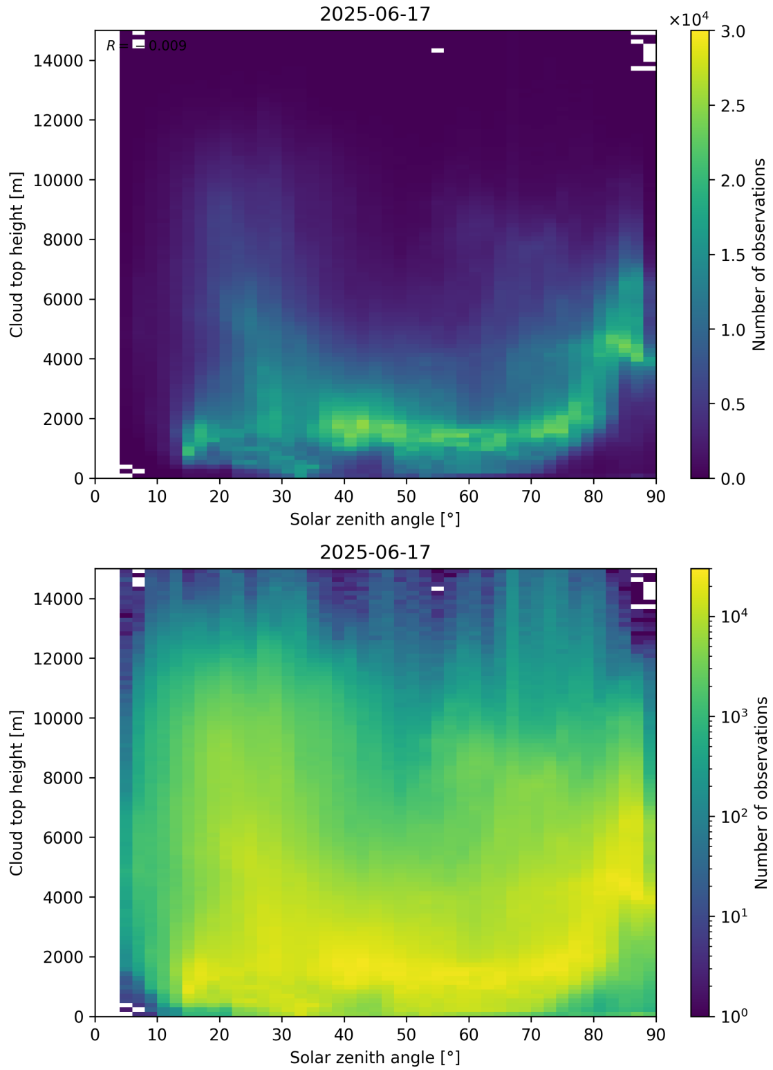
Figure 104: Scatter density plot of “Solar zenith angle” against “Cloud top height” for 2025-06-17 to 2025-06-18.
