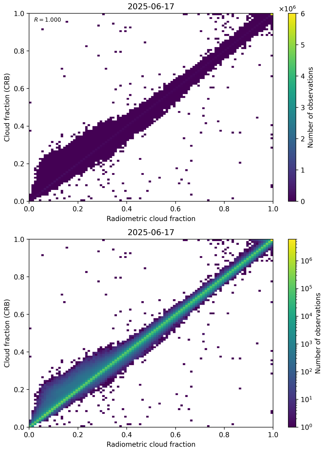
Figure 73: Scatter density plot of “Radiometric cloud fraction” against “Cloud fraction (CRB)” for 2025-06-17 to 2025-06-18.
