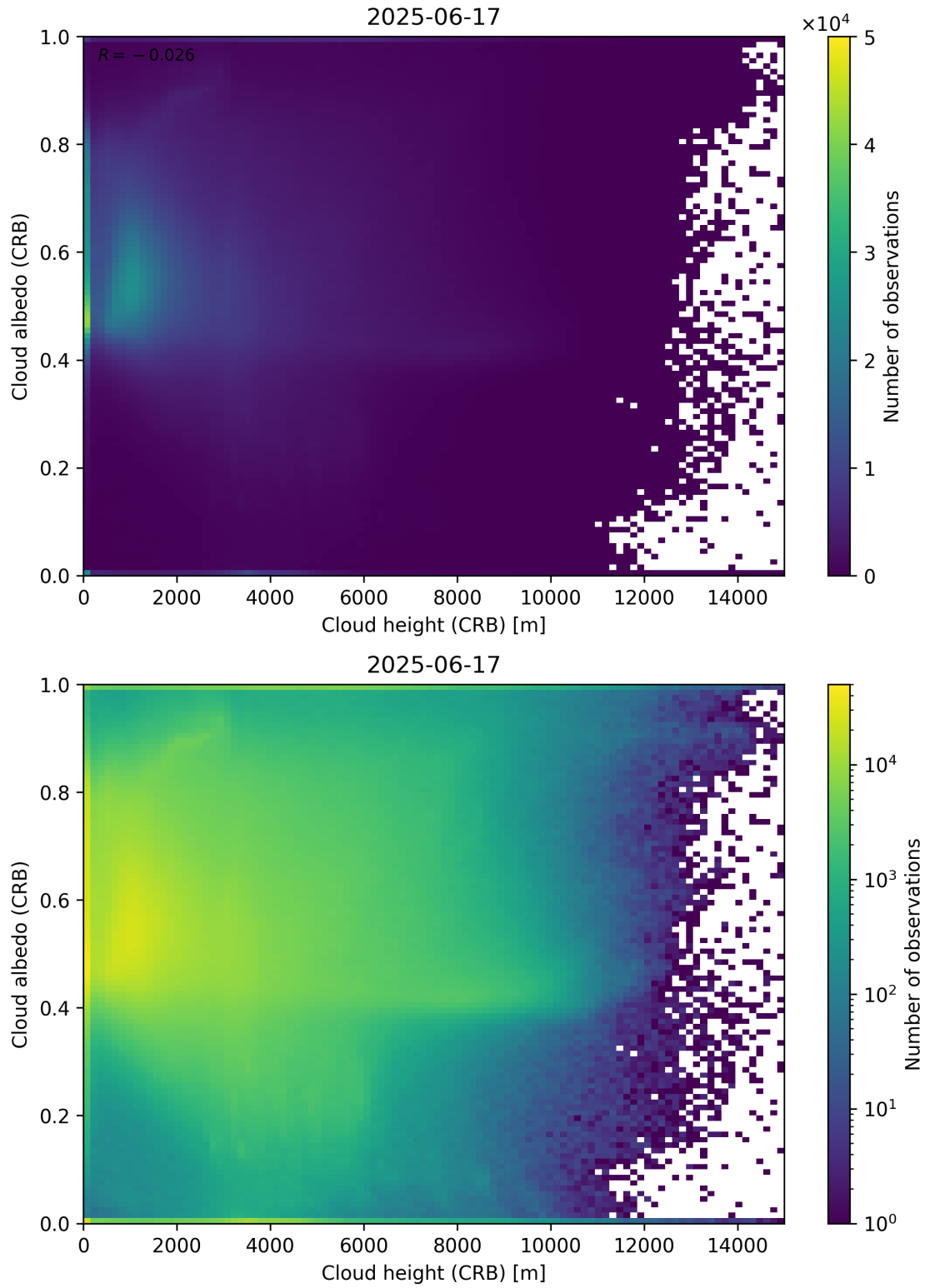
Figure 80: Scatter density plot of “Cloud height (CRB)” against “Cloud albedo (CRB)” for 2025-06-17 to 2025-06-18.
