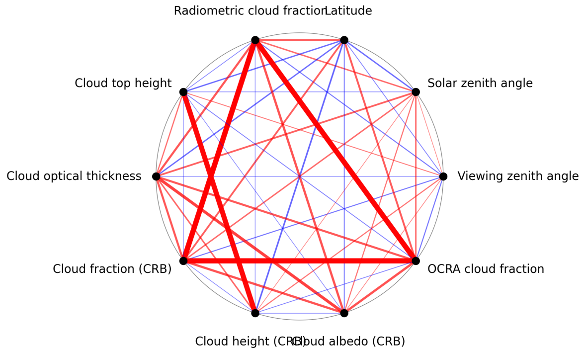
Figure 1: Map of correlation graph for 2025-06-17 to 2025-06-18.
