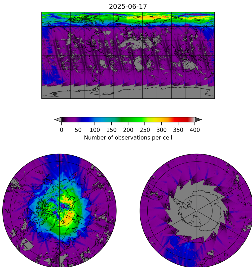
Figure 21: Map of the number of observations for 2025-06-17 to 2025-06-18
