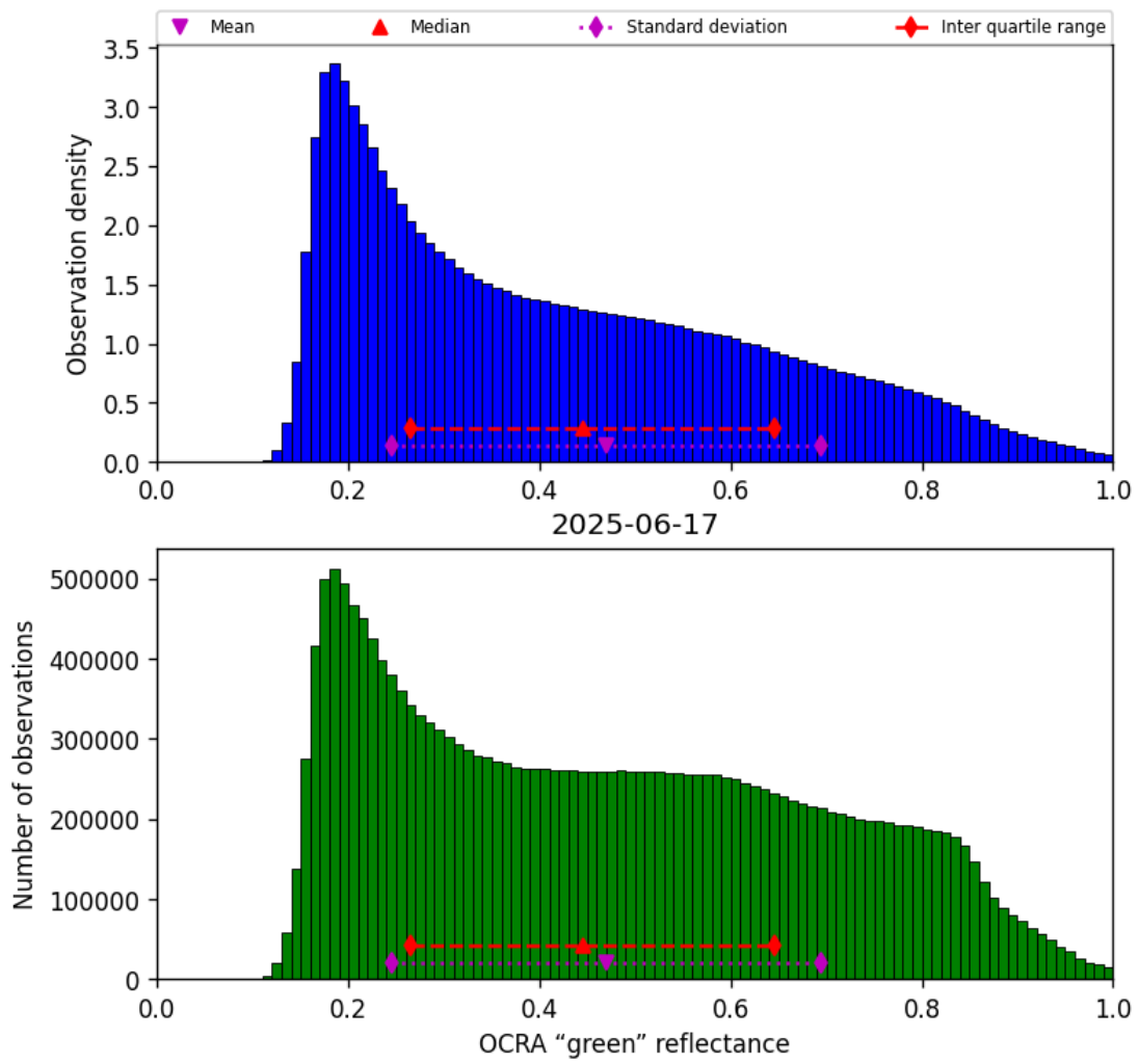
Figure 52: Histogram of “OCRA “green” reflectance” for 2025-06-17 to 2025-06-18
