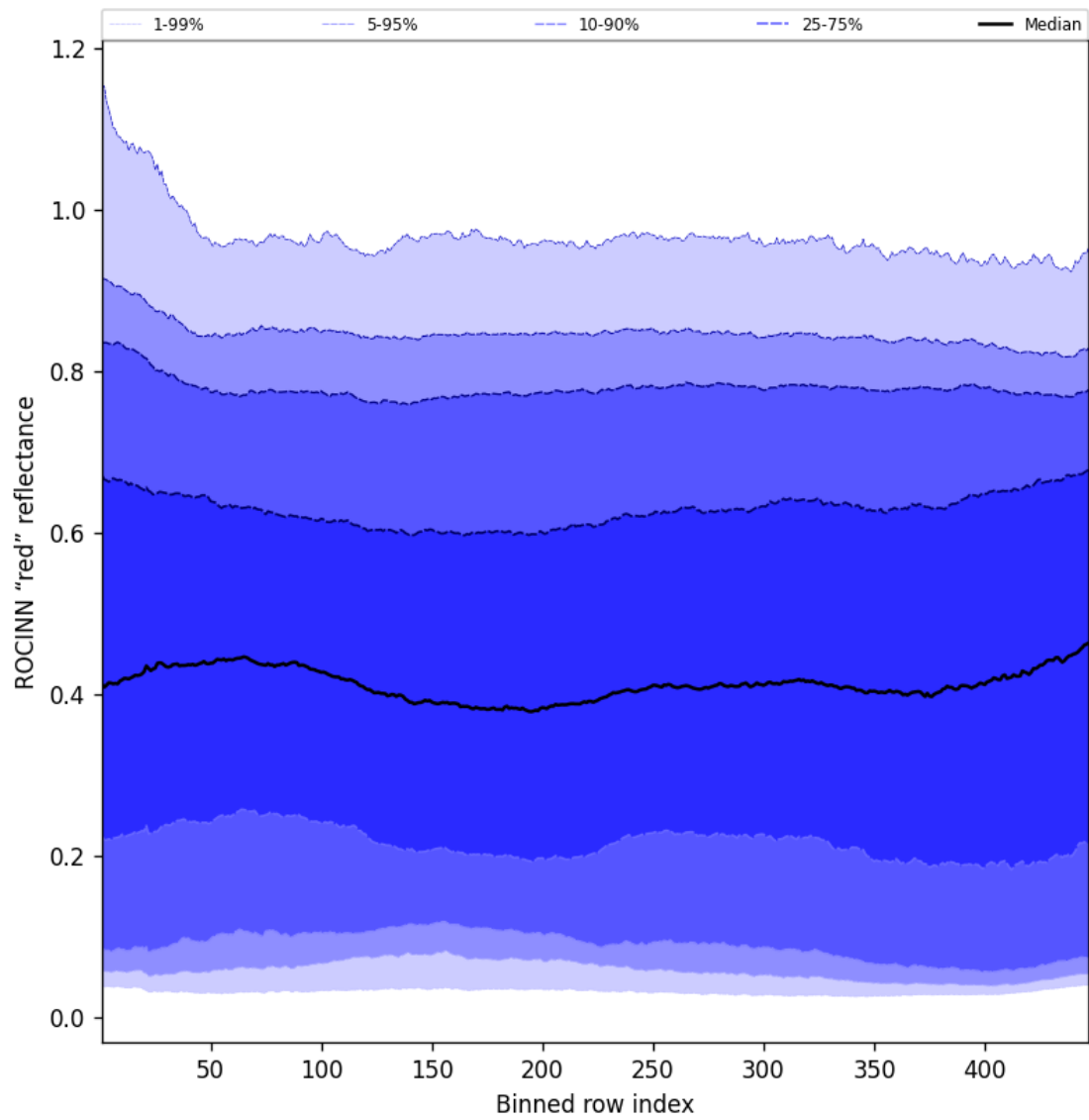
Figure 69: Along track statistics of “ROCINN “red” reflectance” for 2025-06-17 to 2025-06-18
