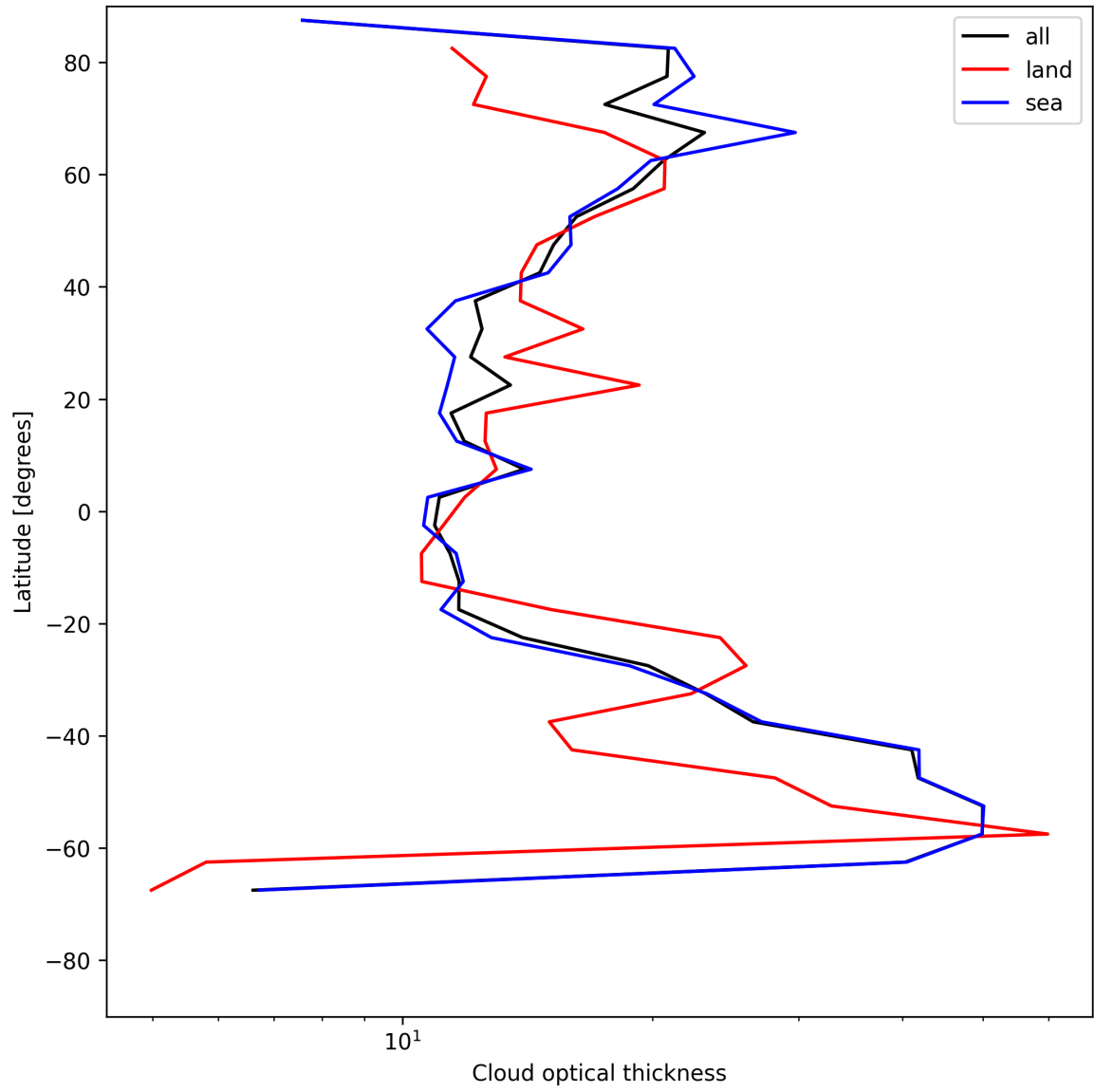
Figure 25: Zonal average of “Cloud optical thickness” for 2025-06-17 to 2025-06-18.
