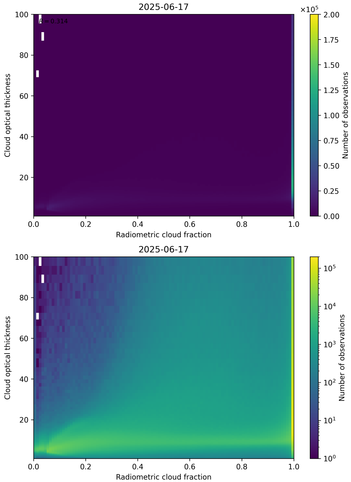
Figure 75: Scatter density plot of “Radiometric cloud fraction” against “Cloud optical thickness” for 2025-06-17 to 2025-06-18.
