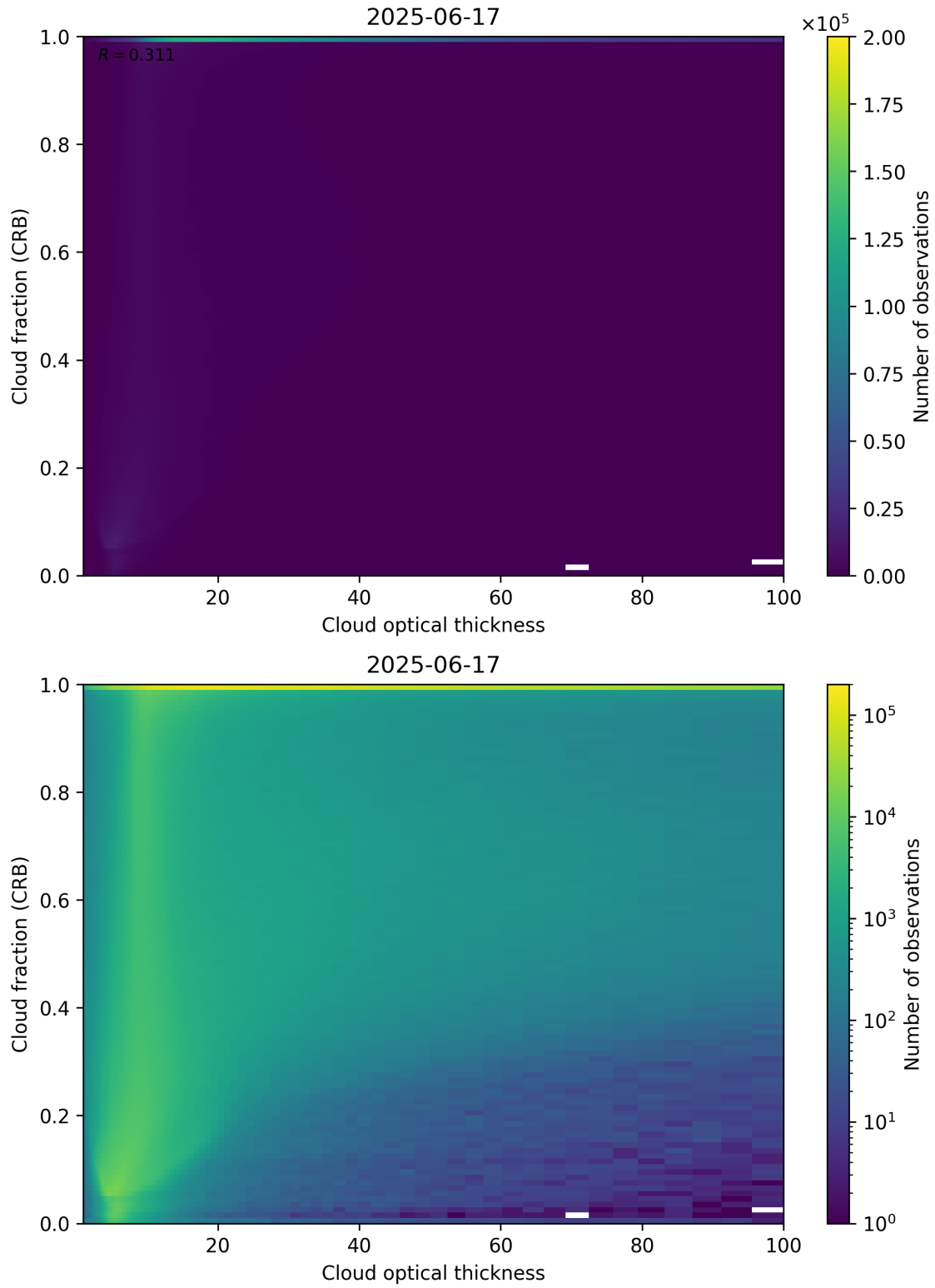
Figure 84: Scatter density plot of “Cloud optical thickness” against “Cloud fraction (CRB)” for 2025-06-17 to 2025-06-18.
