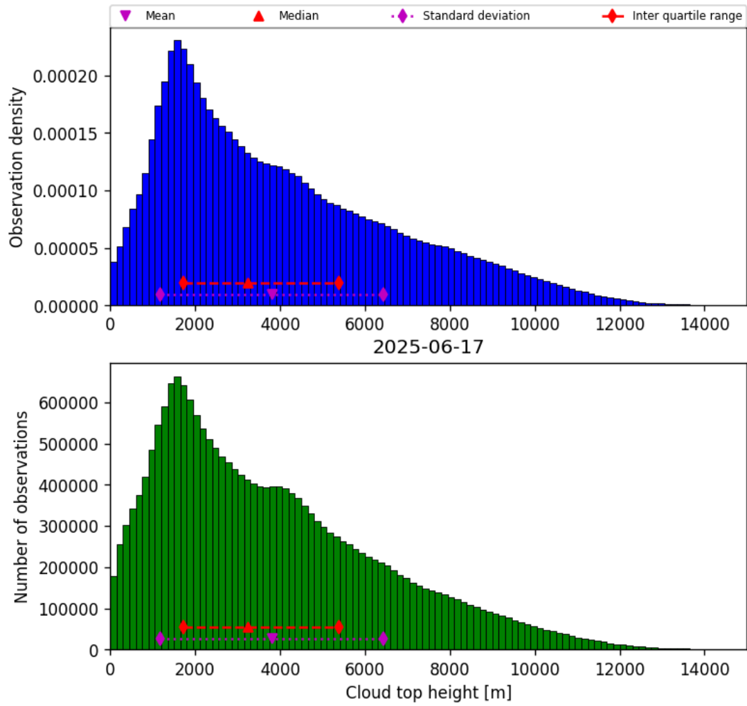
Figure 40: Histogram of “Cloud top height” for 2025-06-17 to 2025-06-18
