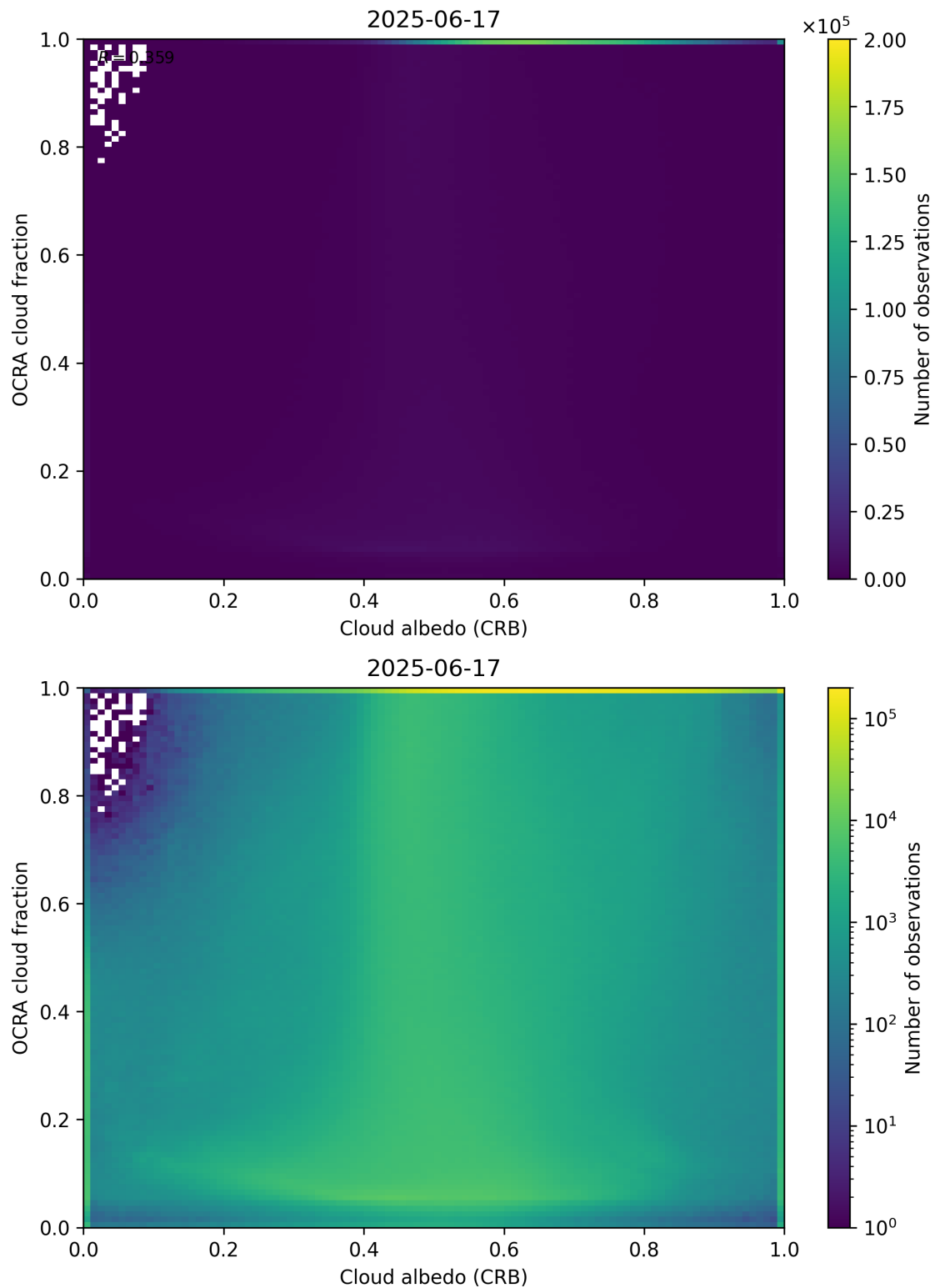
Figure 70: Scatter density plot of “Cloud albedo (CRB)” against “OCRA cloud fraction” for 2025-06-17 to 2025-06-18.
