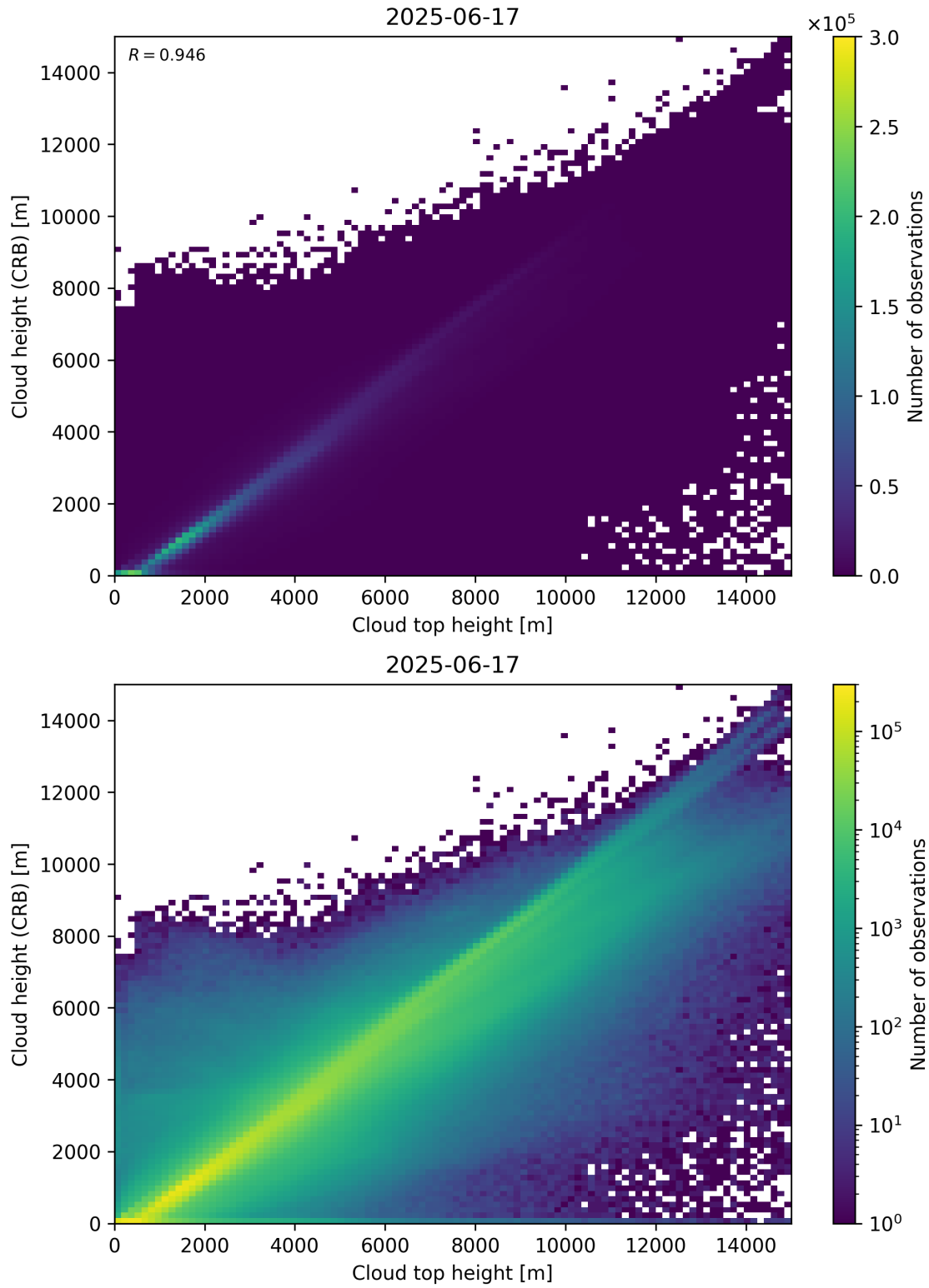
Figure 89: Scatter density plot of “Cloud top height” against “Cloud height (CRB)” for 2025-06-17 to 2025-06-18.
