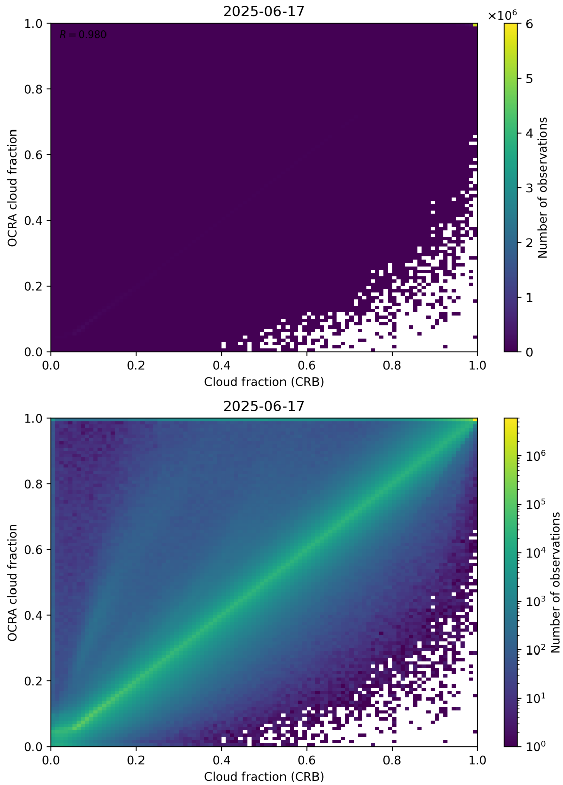
Figure 78: Scatter density plot of “Cloud fraction (CRB)” against “OCRA cloud fraction” for 2025-06-17 to 2025-06-18.
