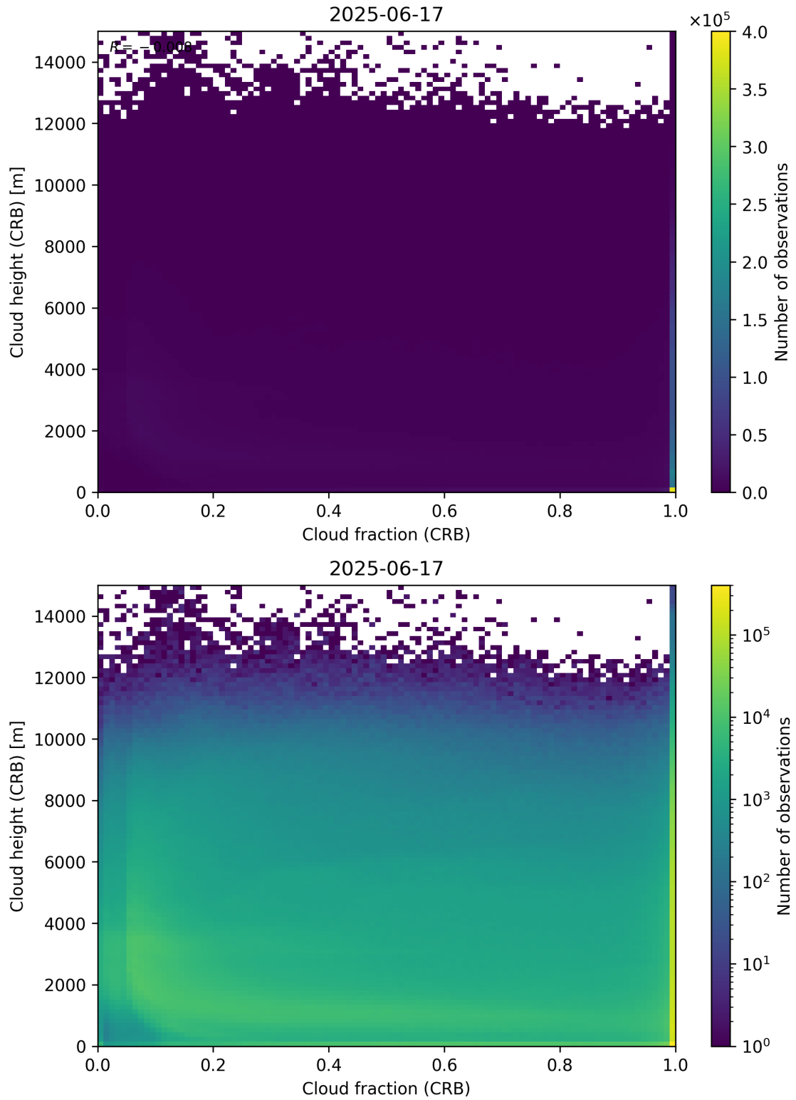
Figure 79: Scatter density plot of “Cloud fraction (CRB)” against “Cloud height (CRB)” for 2025-06-17 to 2025-06-18.
