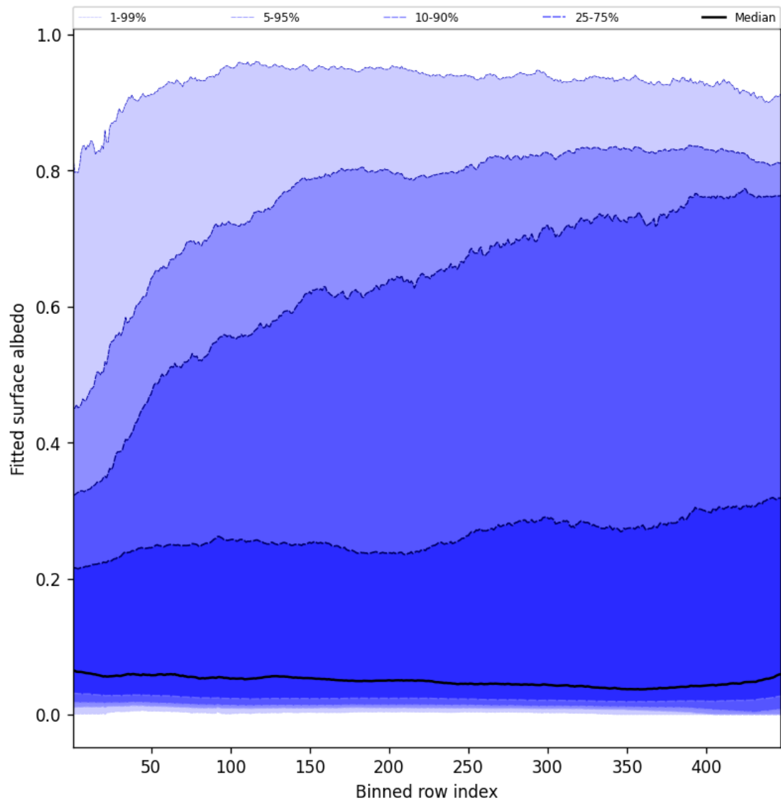
Figure 61: Along track statistics of “Fitted surface albedo” for 2025-06-17 to 2025-06-18
