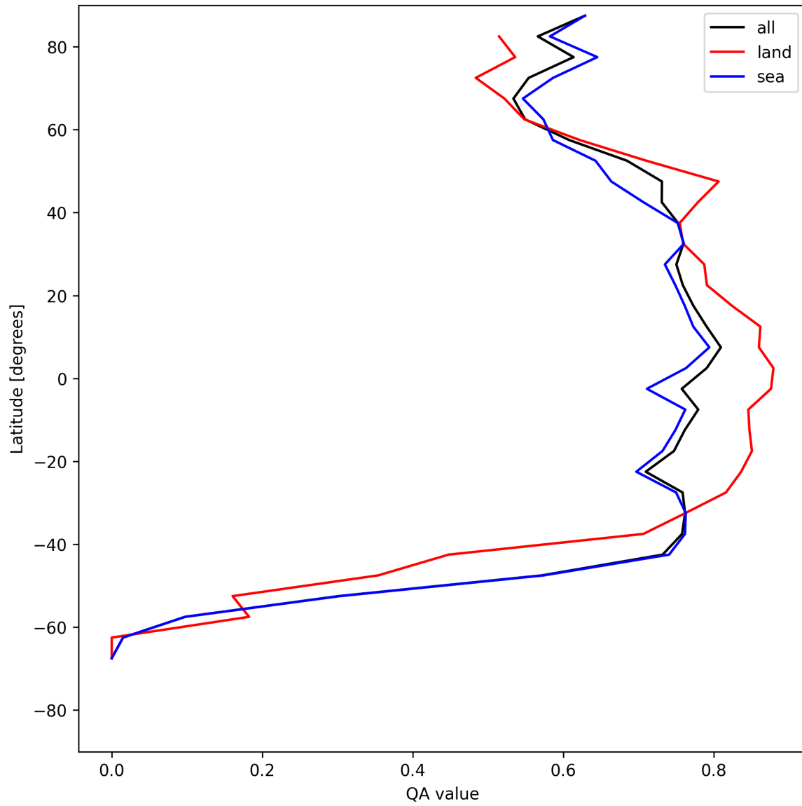
Figure 22: Zonal average of “QA value” for 2025-06-17 to 2025-06-18.
