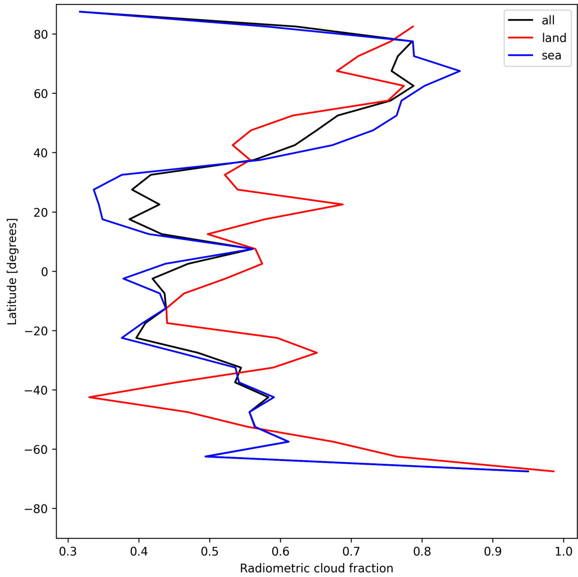
Figure 23: Zonal average of “Radiometric cloud fraction” for 2025-06-17 to 2025-06-18.
