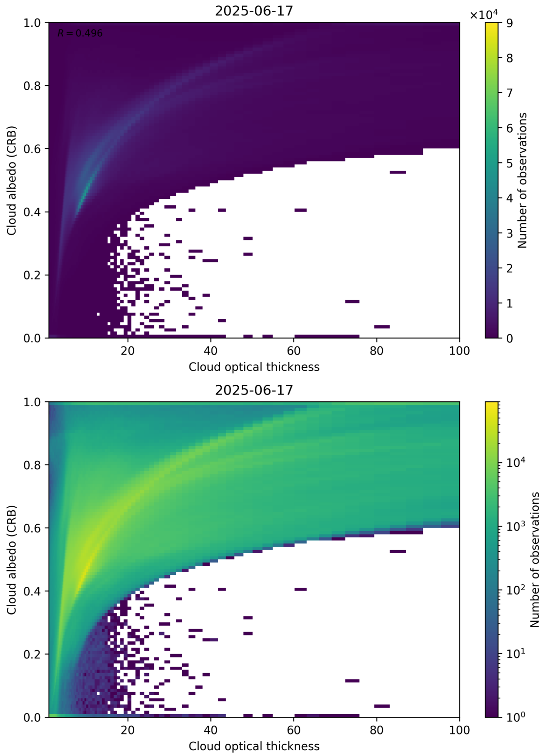
Figure 82: Scatter density plot of “Cloud optical thickness” against “Cloud albedo (CRB)” for 2025-06-17 to 2025-06-18.
