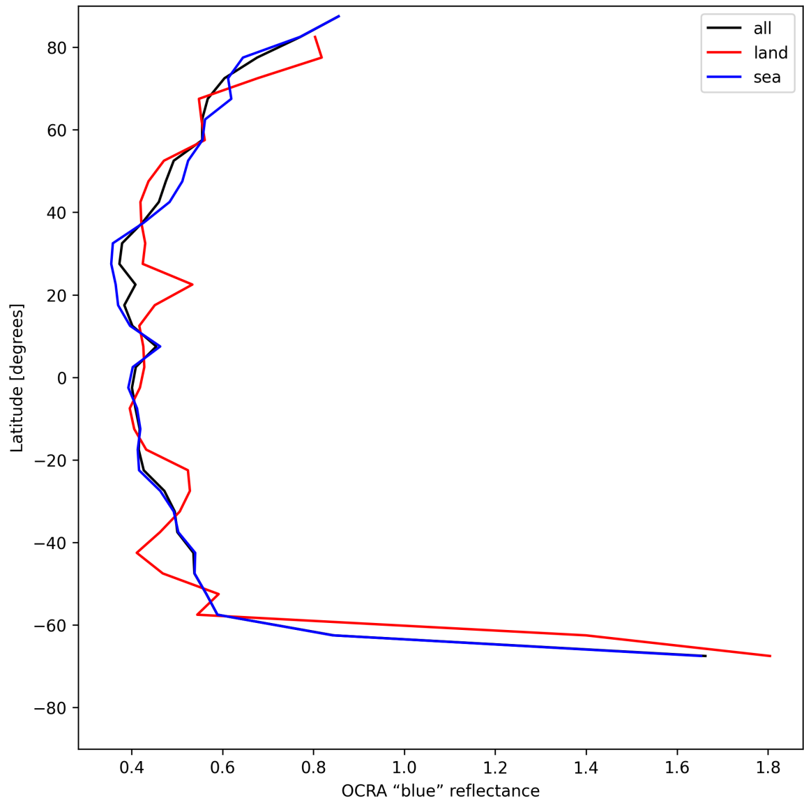
Figure 35: Zonal average of “OCRA “blue” reflectance” for 2025-06-17 to 2025-06-18.
