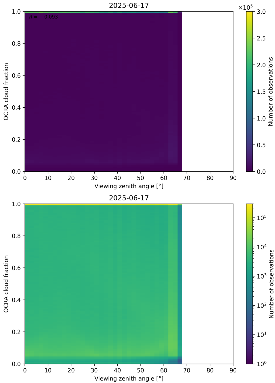
Figure 108: Scatter density plot of “Viewing zenith angle” against “OCRA cloud fraction” for 2025-06-17 to 2025-06-18.
