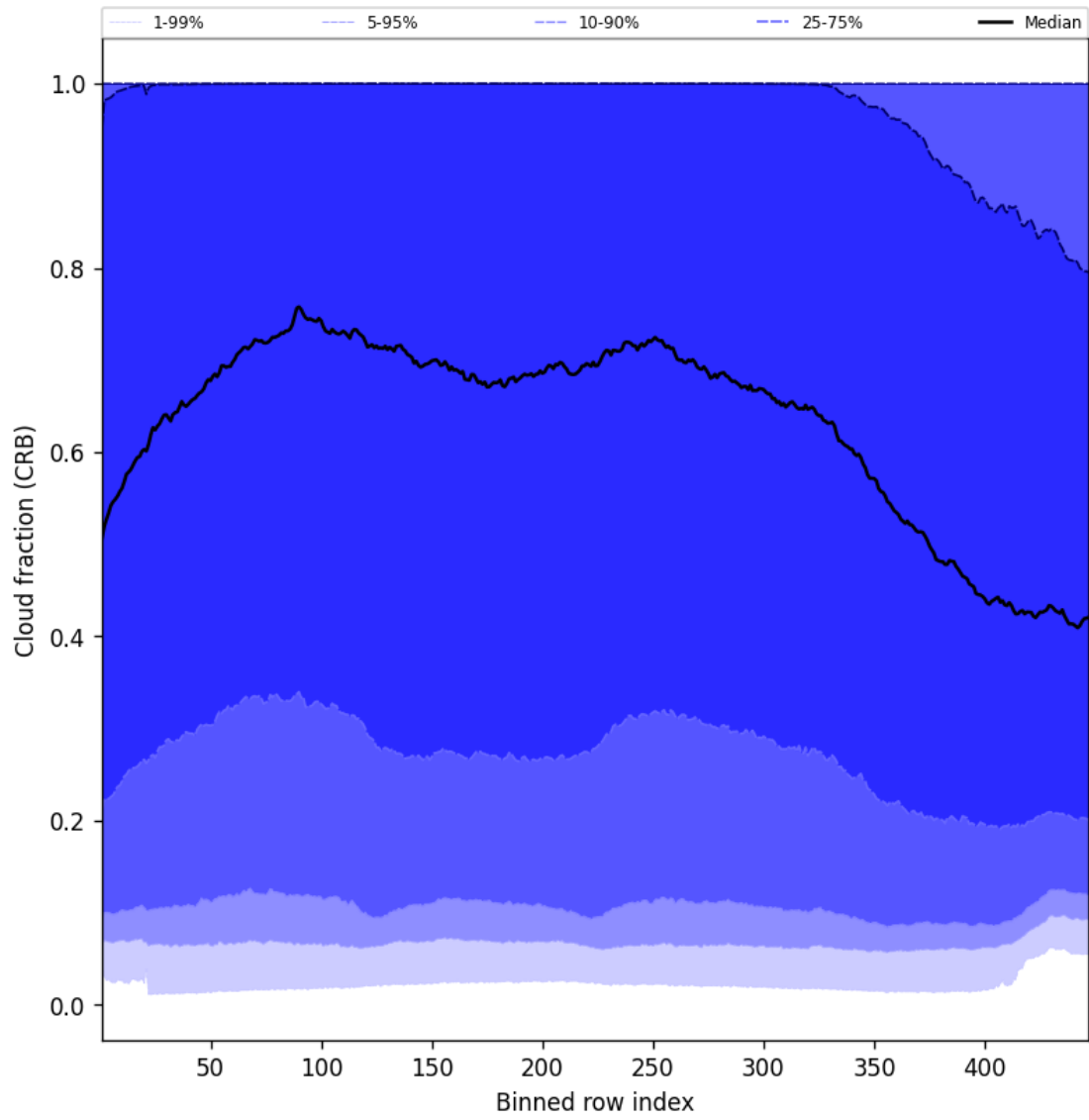
Figure 58: Along track statistics of “Cloud fraction (CRB)” for 2025-06-17 to 2025-06-18
