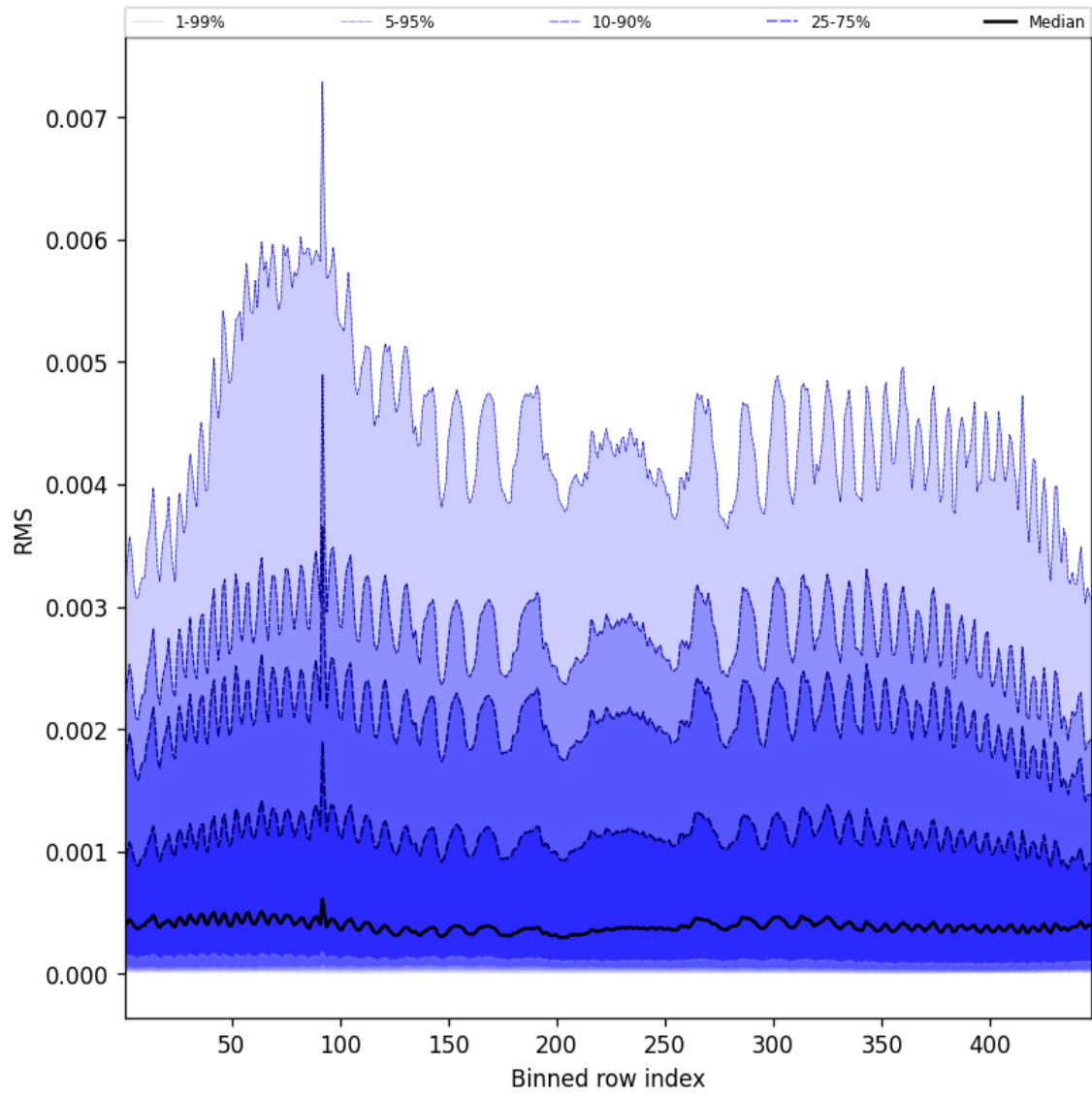
Figure 63: Along track statistics of “RMS” for 2025-06-17 to 2025-06-18
