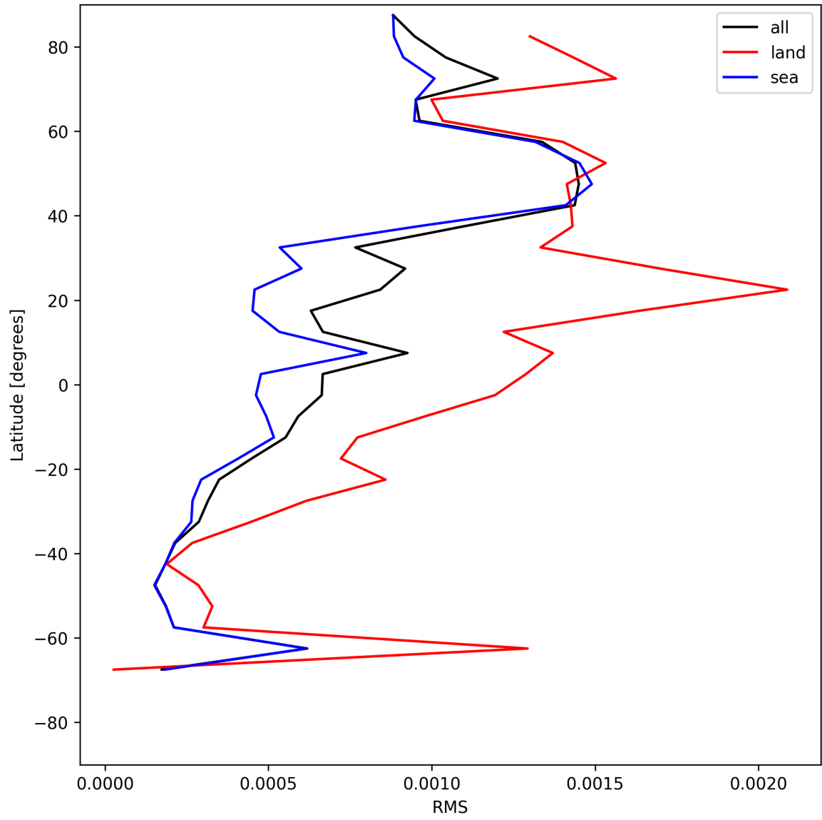
Figure 31: Zonal average of “RMS” for 2025-06-17 to 2025-06-18.
