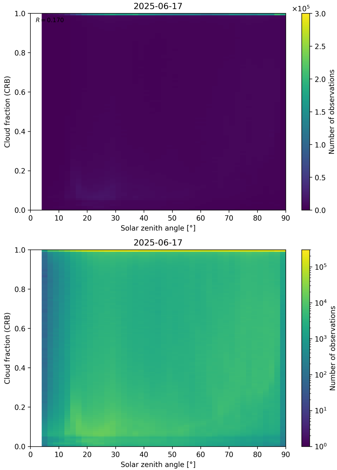
Figure 101: Scatter density plot of “Solar zenith angle” against “Cloud fraction (CRB)” for 2025-06-17 to 2025-06-18.
