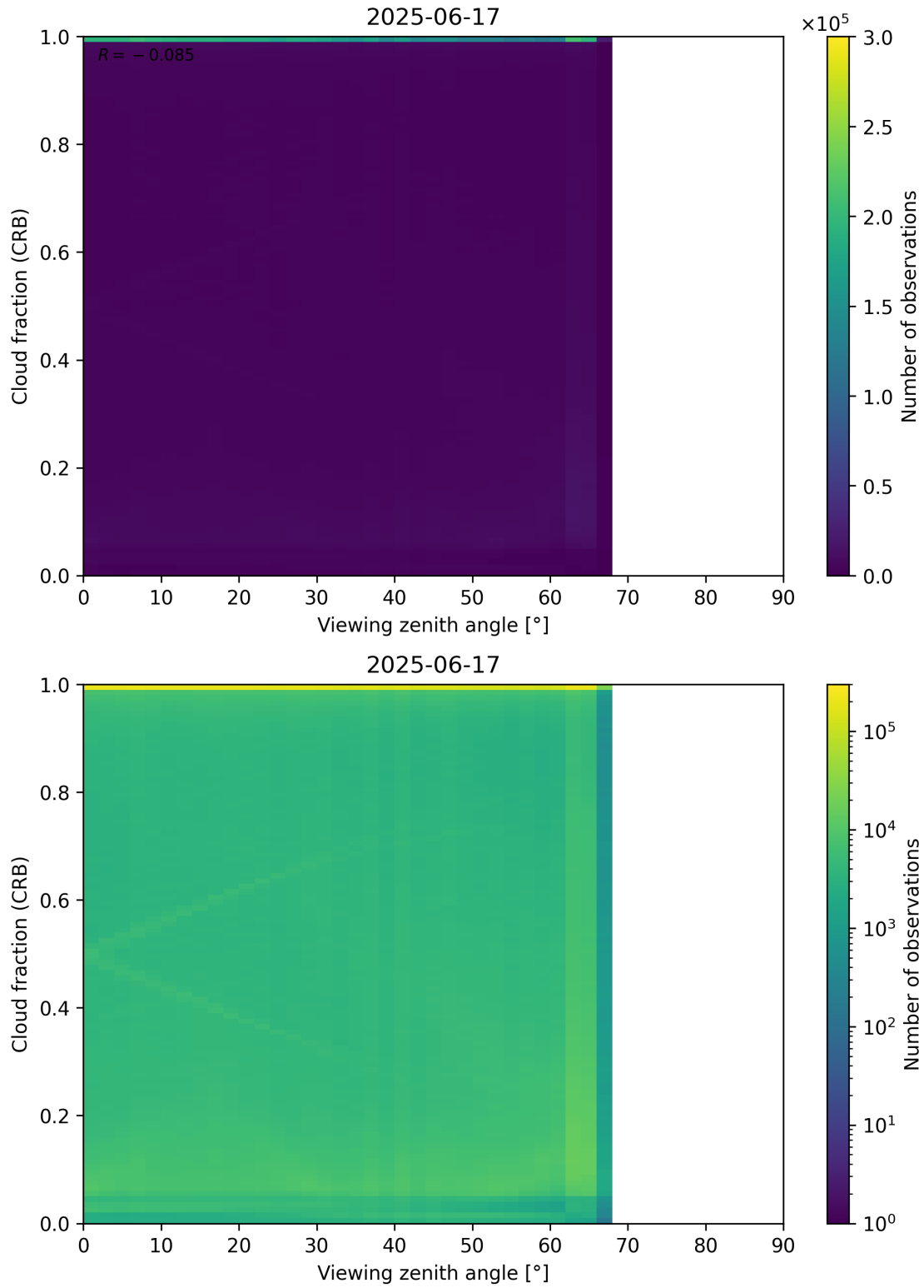
Figure 109: Scatter density plot of “Viewing zenith angle” against “Cloud fraction (CRB)” for 2025-06-17 to 2025-06-18.
