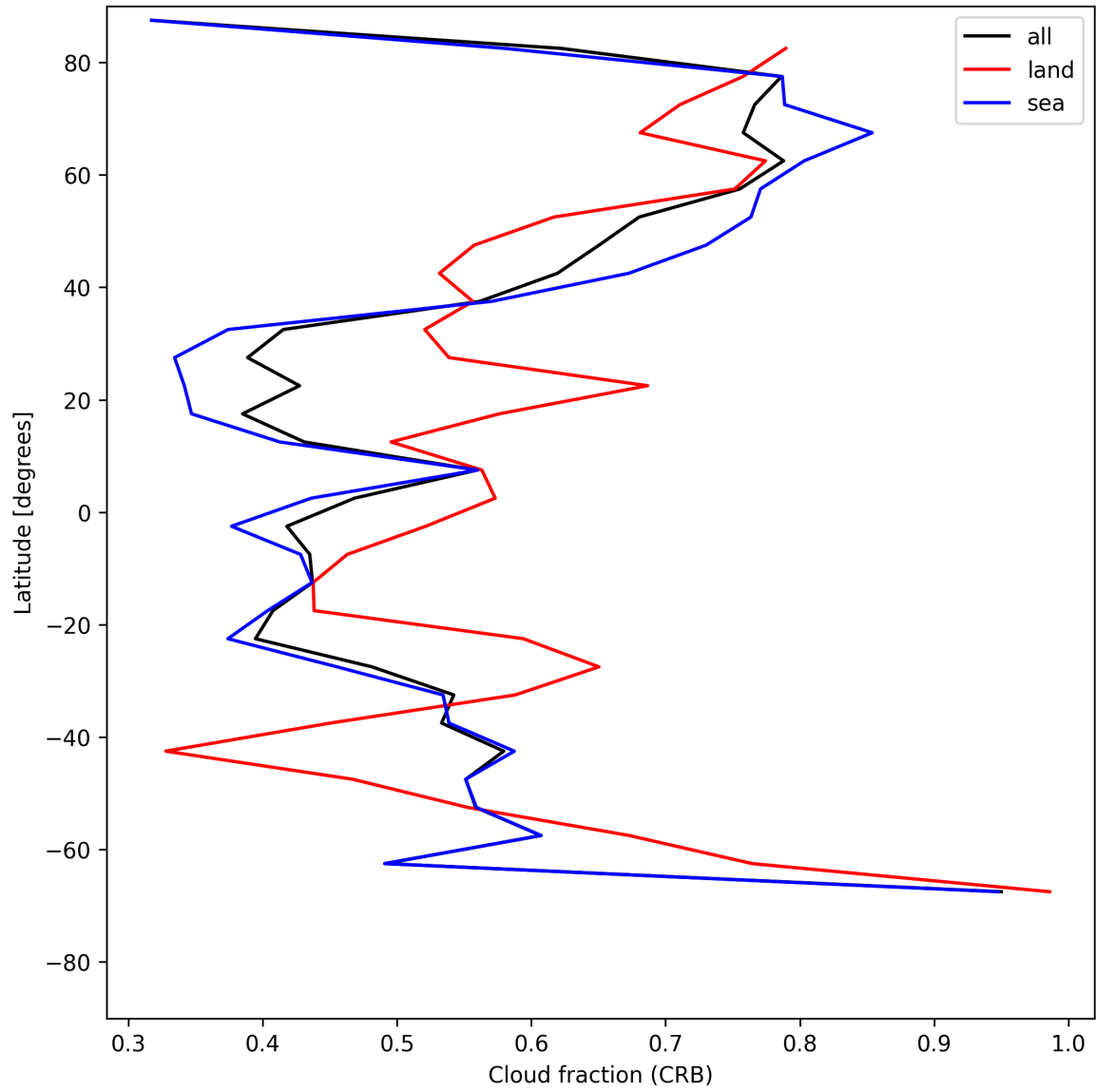
Figure 26: Zonal average of “Cloud fraction (CRB)” for 2025-06-17 to 2025-06-18.
