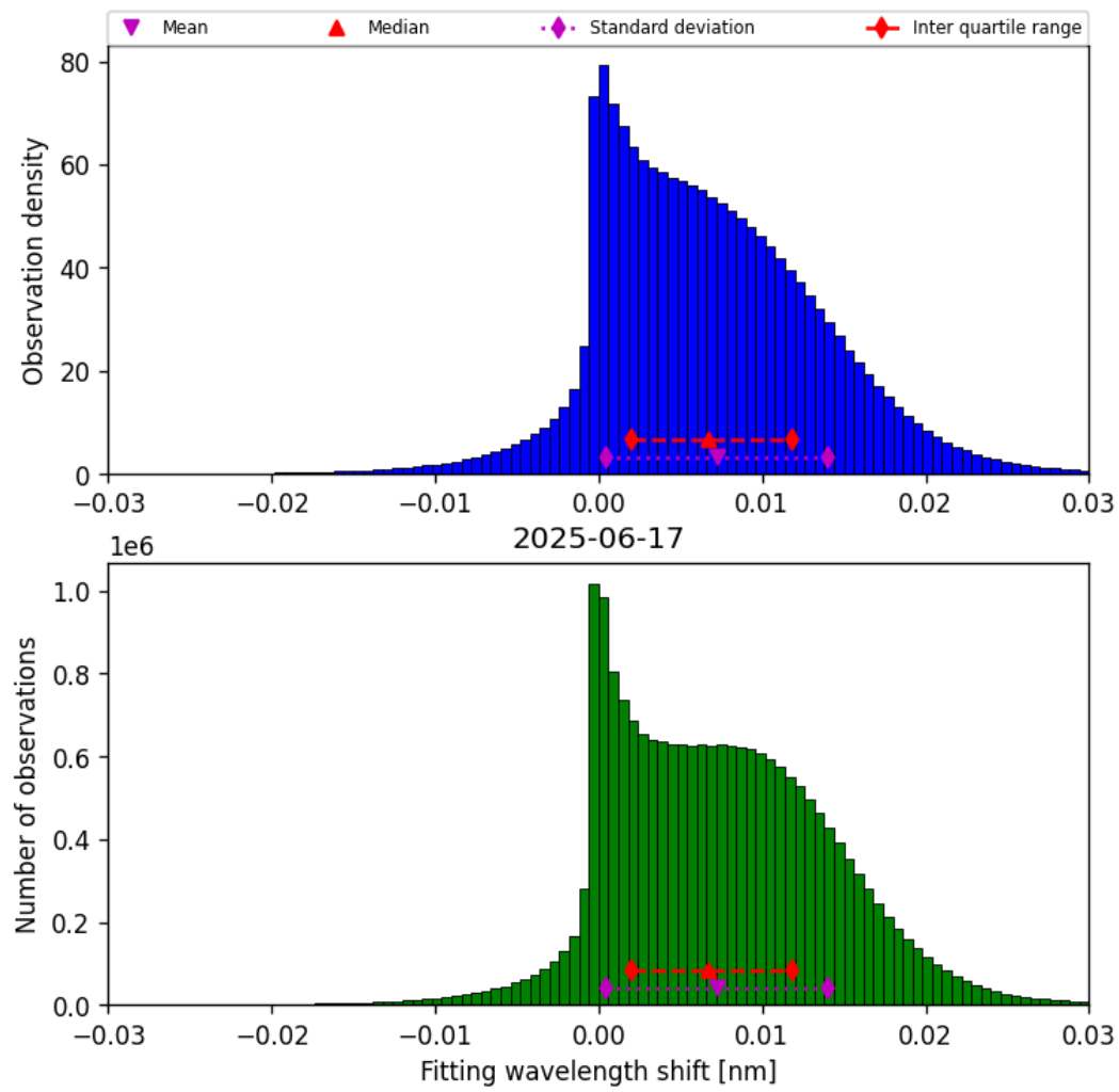
Figure 49: Histogram of “Fitting wavelength shift” for 2025-06-17 to 2025-06-18
