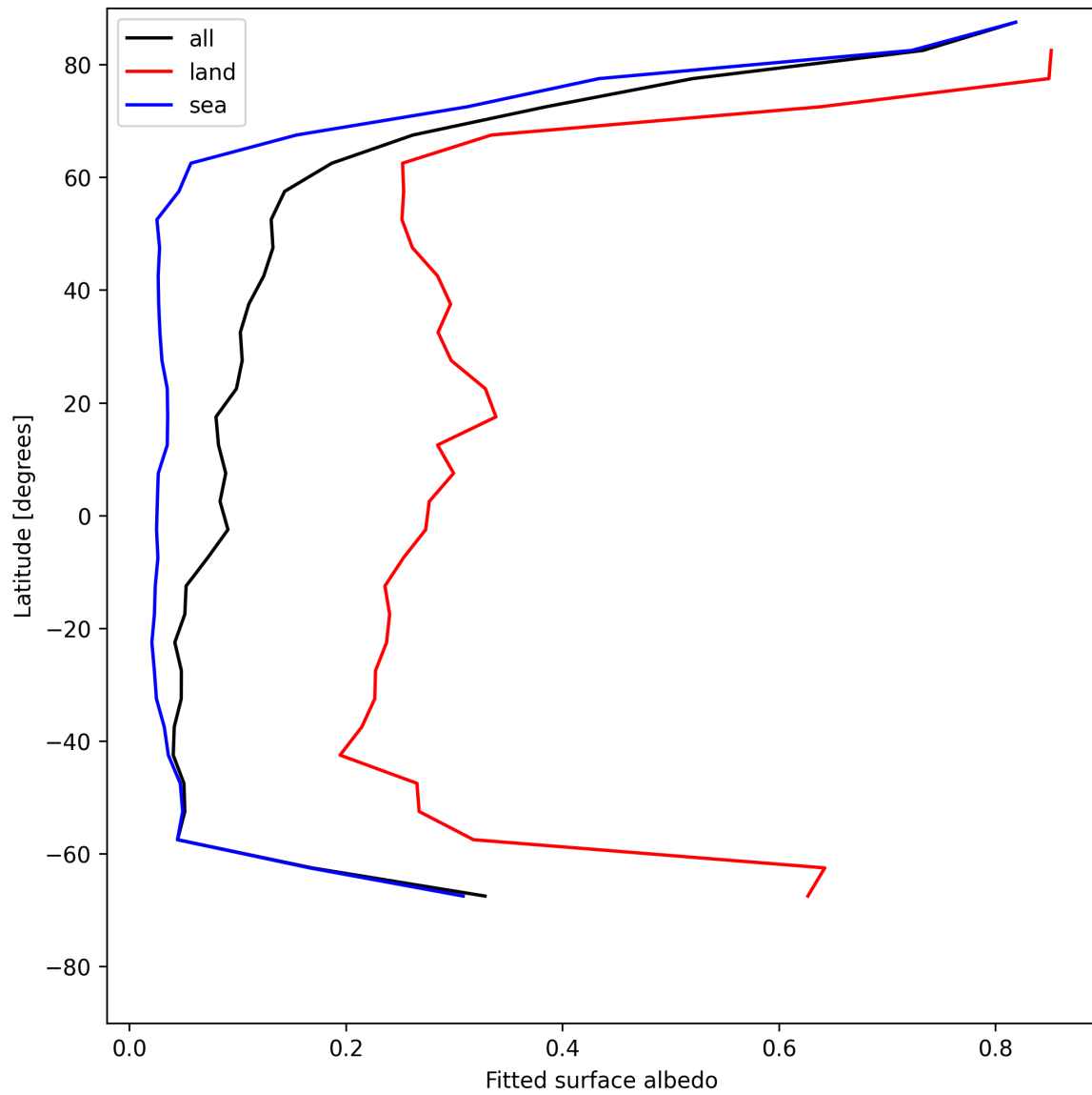
Figure 29: Zonal average of “Fitted surface albedo” for 2025-06-17 to 2025-06-18.
