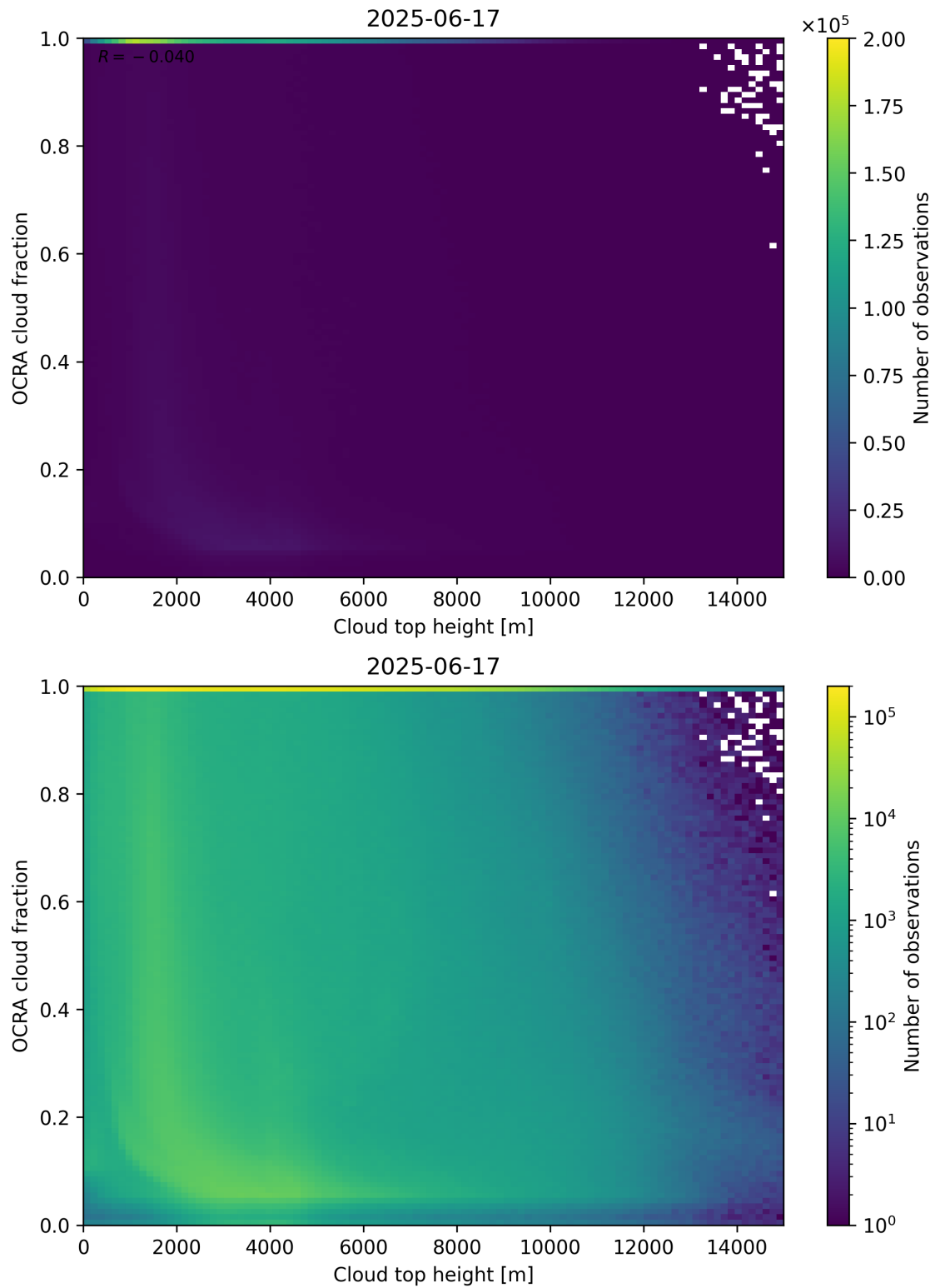
Figure 87: Scatter density plot of “Cloud top height” against “OCRA cloud fraction” for 2025-06-17 to 2025-06-18.
