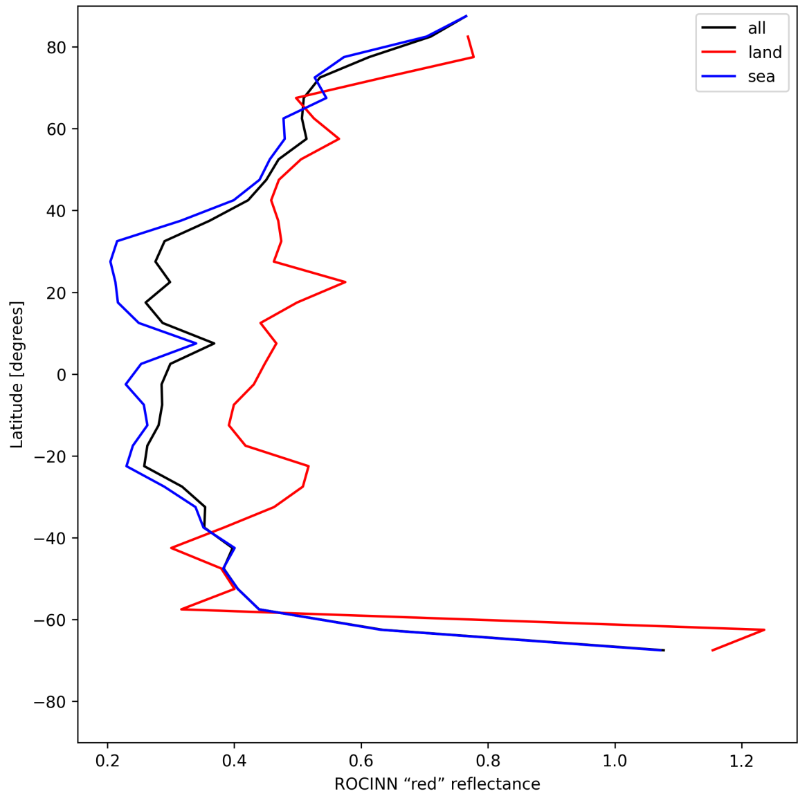
Figure 37: Zonal average of “ROCINN “red” reflectance” for 2025-06-17 to 2025-06-18.
