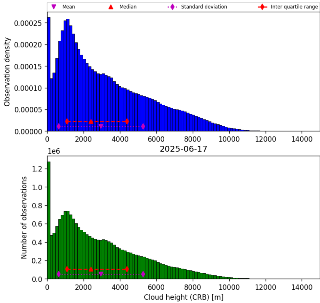
Figure 43: Histogram of “Cloud height (CRB)” for 2025-06-17 to 2025-06-18
