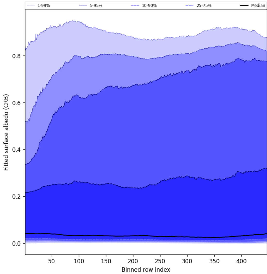
Figure 62: Along track statistics of “Fitted surface albedo (CRB)” for 2025-06-17 to 2025-06-18
