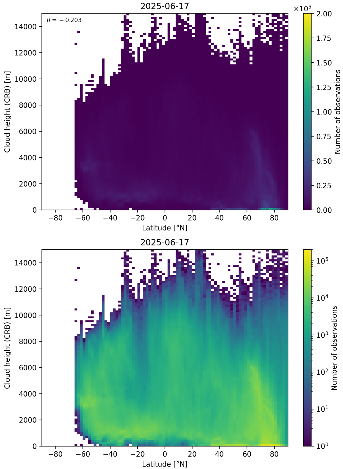
Figure 95: Scatter density plot of “Latitude” against “Cloud height (CRB)” for 2025-06-17 to 2025-06-18.
