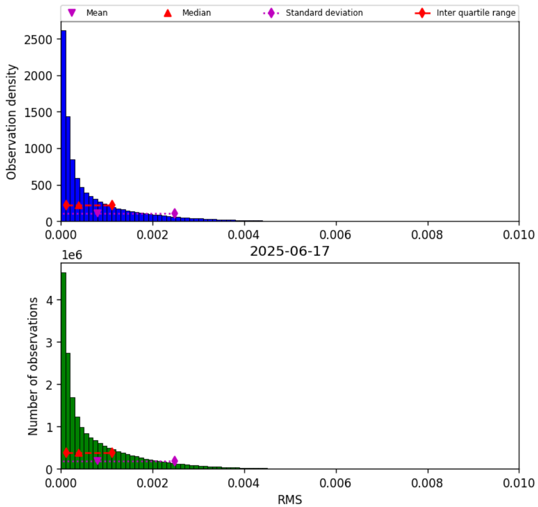
Figure 47: Histogram of “RMS” for 2025-06-17 to 2025-06-18
