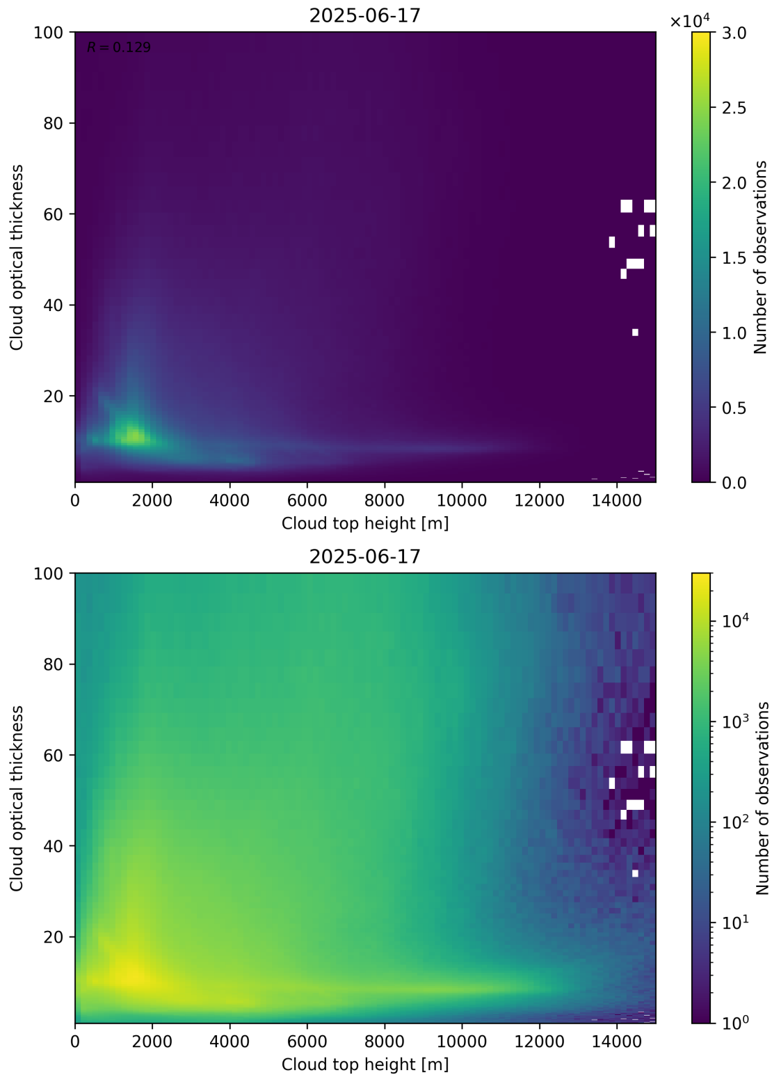
Figure 90: Scatter density plot of “Cloud top height” against “Cloud optical thickness” for 2025-06-17 to 2025-06-18.
