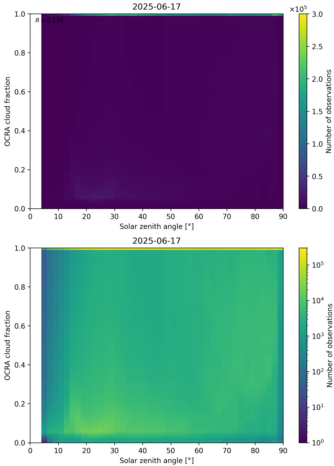
Figure 100: Scatter density plot of “Solar zenith angle” against “OCRA cloud fraction” for 2025-06-17 to 2025-06-18.
