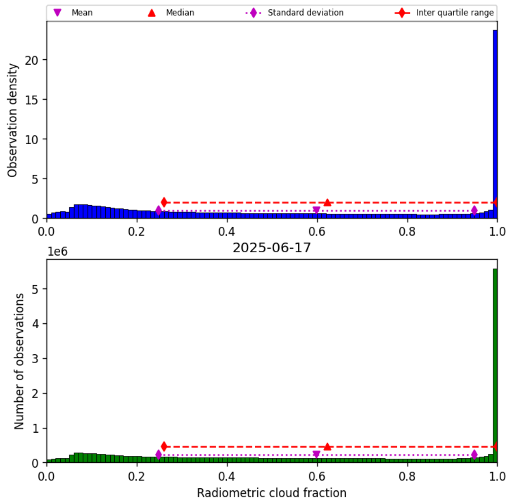
Figure 39: Histogram of “Radiometric cloud fraction” for 2025-06-17 to 2025-06-18
