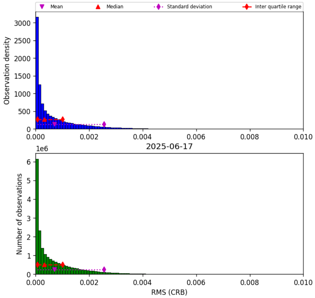
Figure 48: Histogram of “RMS (CRB)” for 2025-06-17 to 2025-06-18
