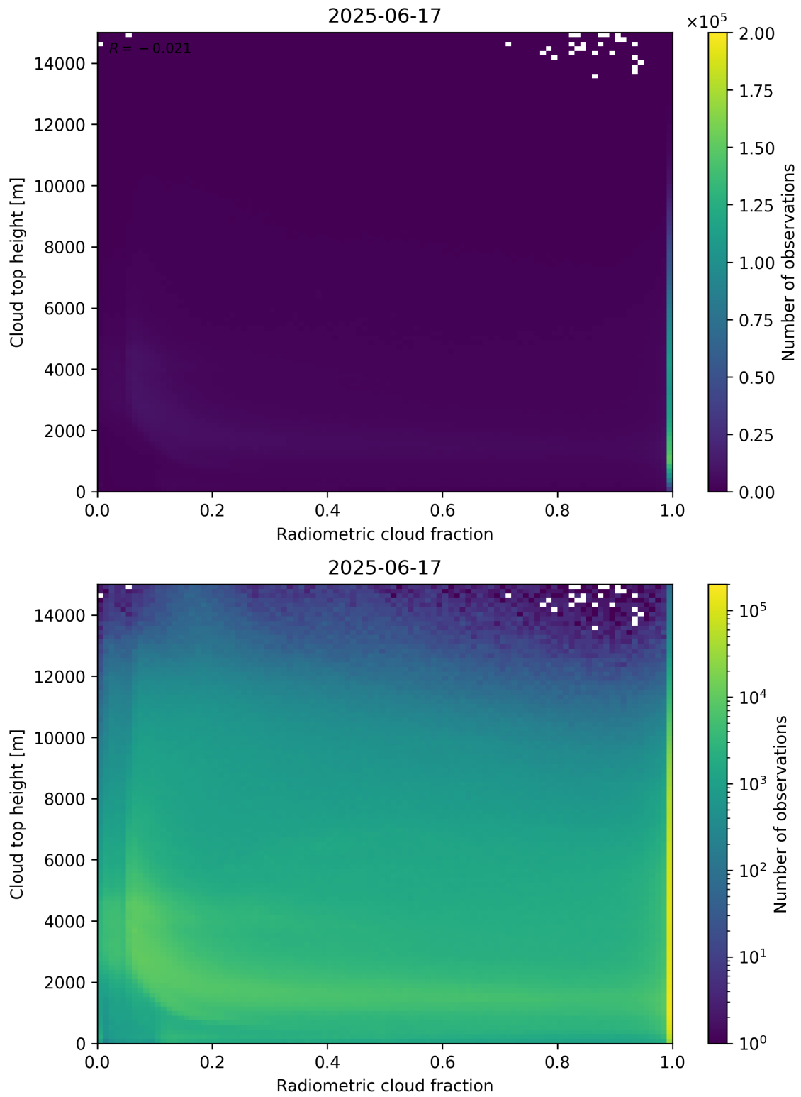
Figure 76: Scatter density plot of “Radiometric cloud fraction” against “Cloud top height” for 2025-06-17 to 2025-06-18.
