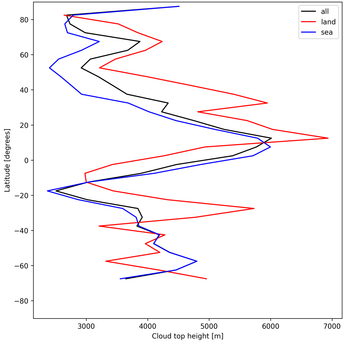
Figure 24: Zonal average of “Cloud top height” for 2025-06-17 to 2025-06-18.
