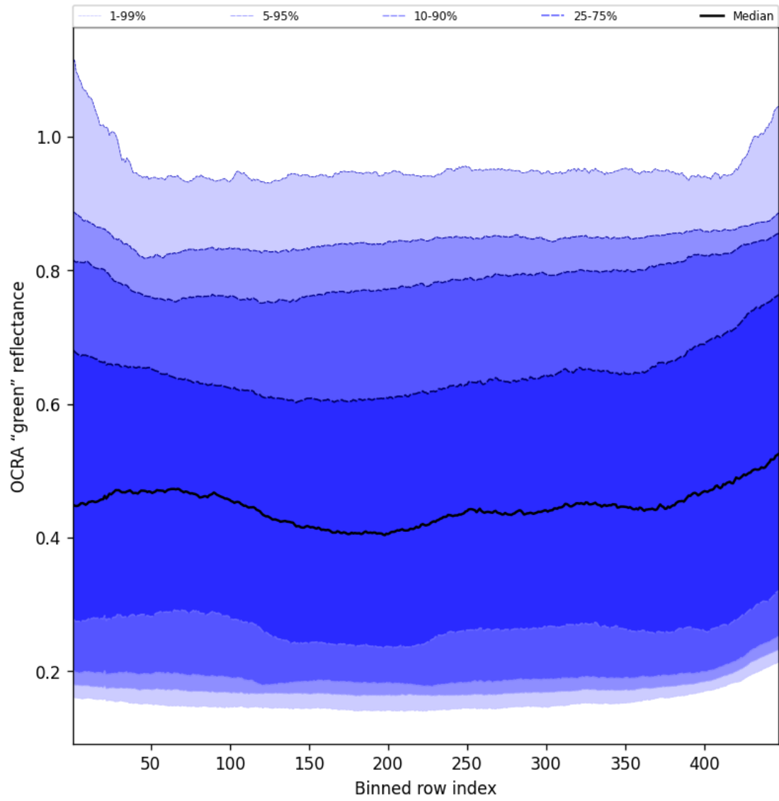
Figure 68: Along track statistics of "OCRA "green" reflectance" for 2025-06-17 to 2025-06-18
