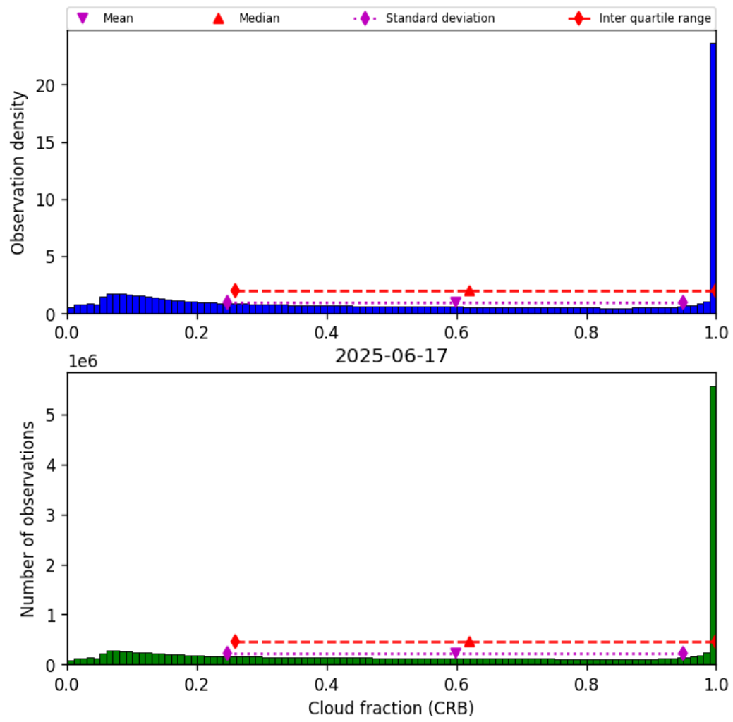
Figure 42: Histogram of “Cloud fraction (CRB)” for 2025-06-17 to 2025-06-18
