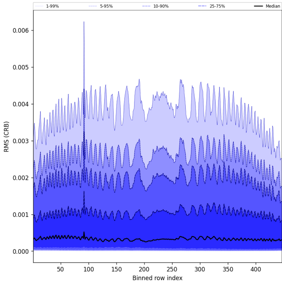
Figure 64: Along track statistics of “RMS (CRB)” for 2025-06-17 to 2025-06-18
