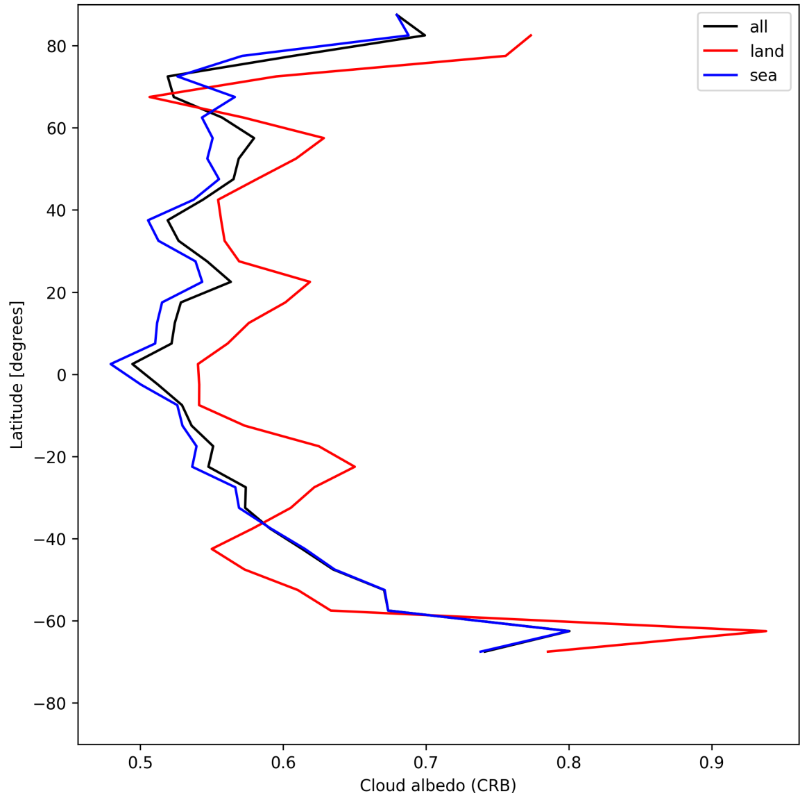
Figure 28: Zonal average of “Cloud albedo (CRB)” for 2025-06-17 to 2025-06-18.
