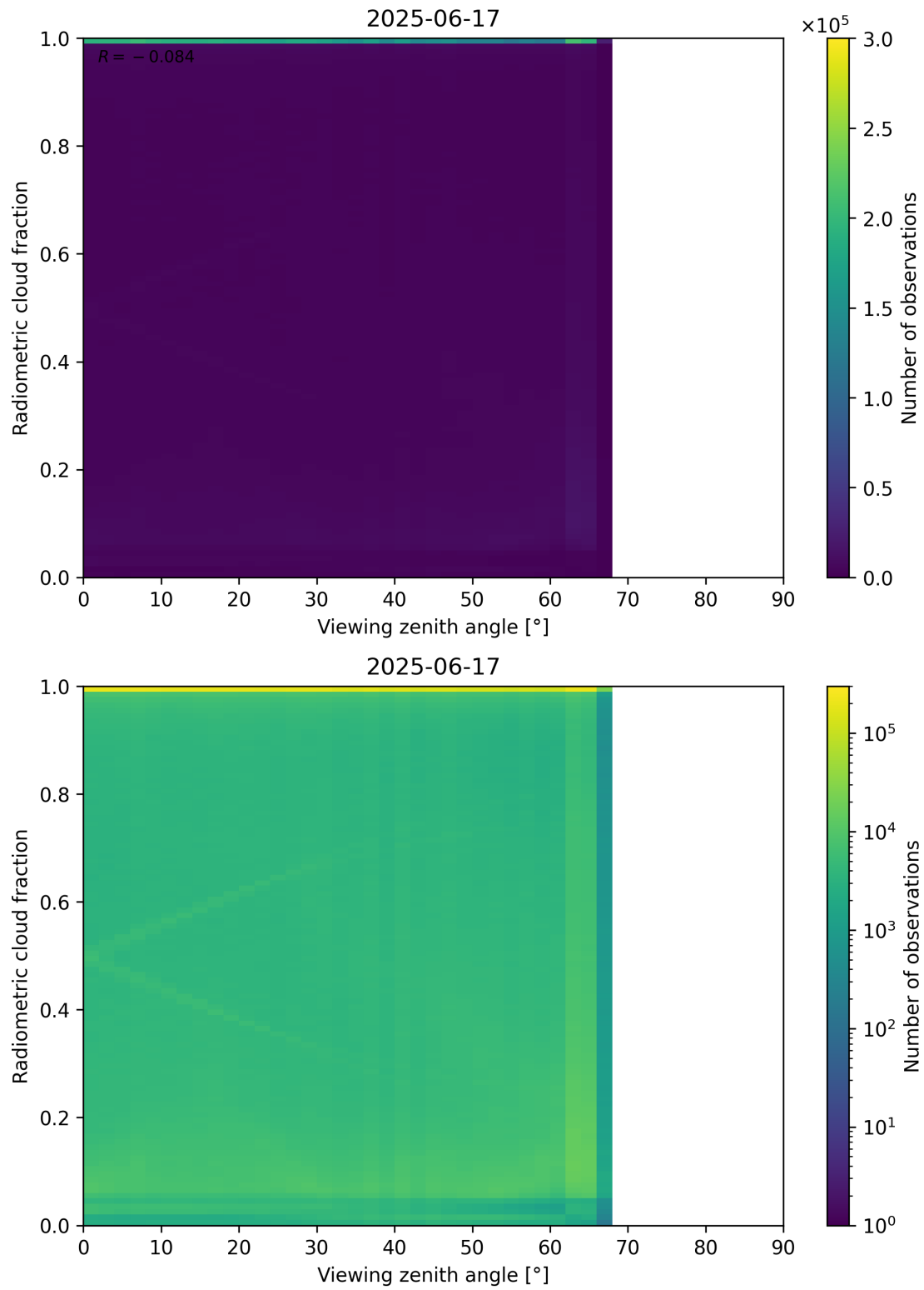
Figure 107: Scatter density plot of “Viewing zenith angle” against “Radiometric cloud fraction” for 2025-06-17 to 2025-06-18.
