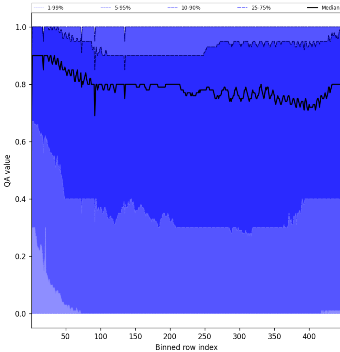
Figure 54: Along track statistics of “QA value” for 2025-06-17 to 2025-06-18
