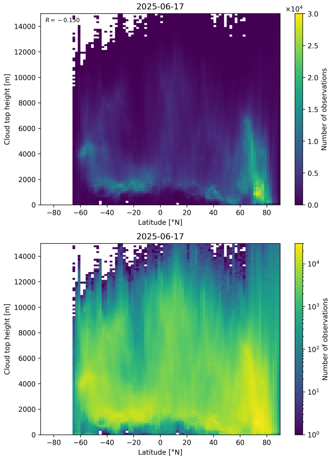
Figure 97: Scatter density plot of “Latitude” against “Cloud top height” for 2025-06-17 to 2025-06-18.
