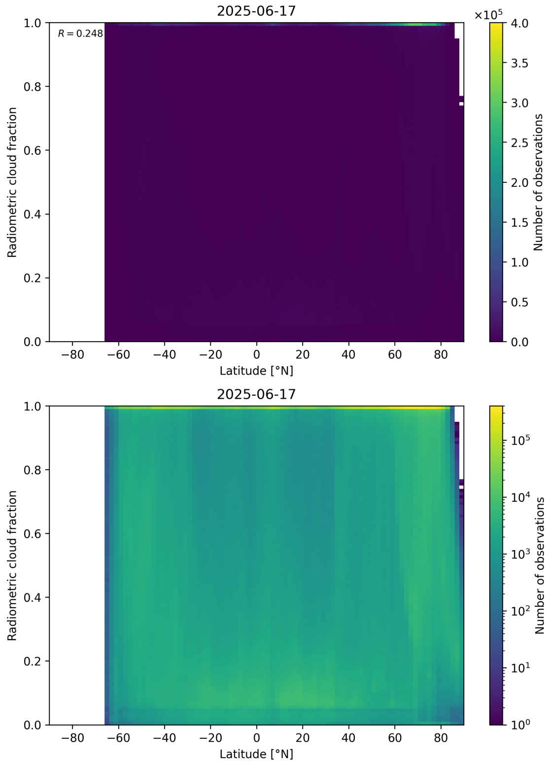
Figure 92: Scatter density plot of “Latitude” against “Radiometric cloud fraction” for 2025-06-17 to 2025-06-18.
