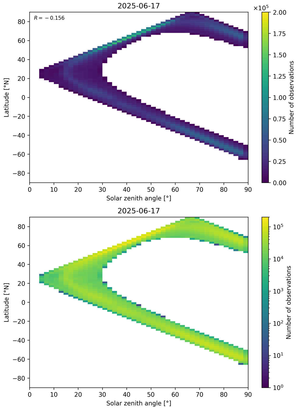
Figure 105: Scatter density plot of “Solar zenith angle” against “Latitude” for 2025-06-17 to 2025-06-18.
