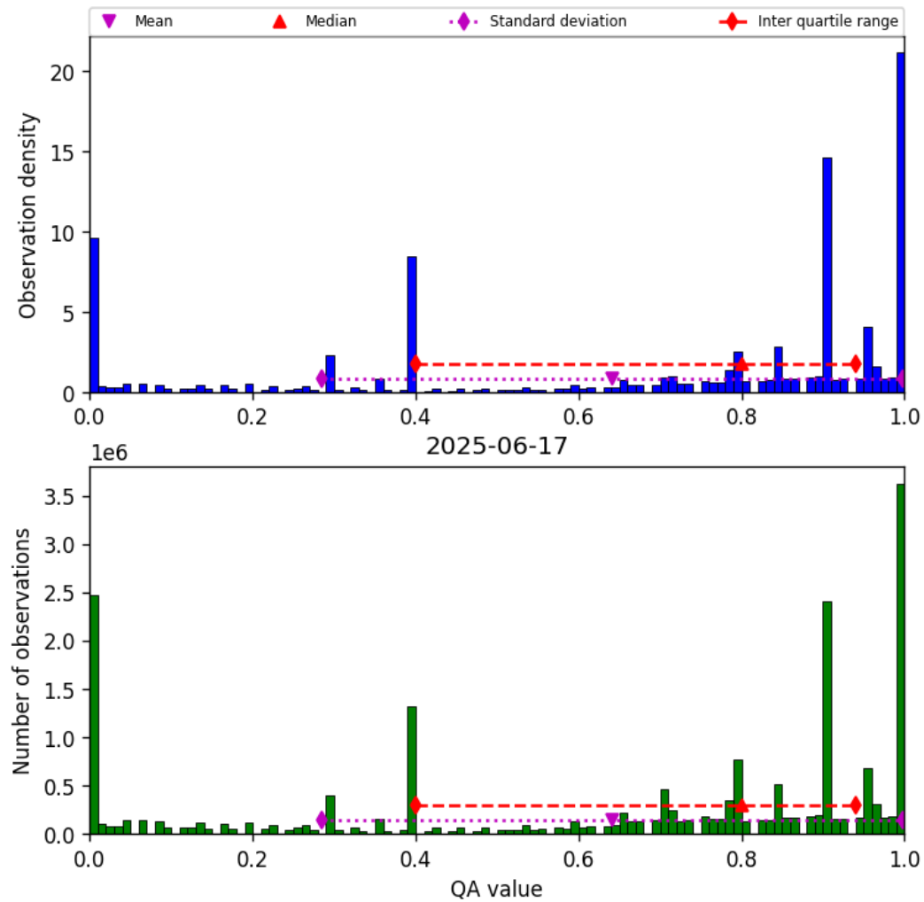
Figure 38: Histogram of “QA value” for 2025-06-17 to 2025-06-18
