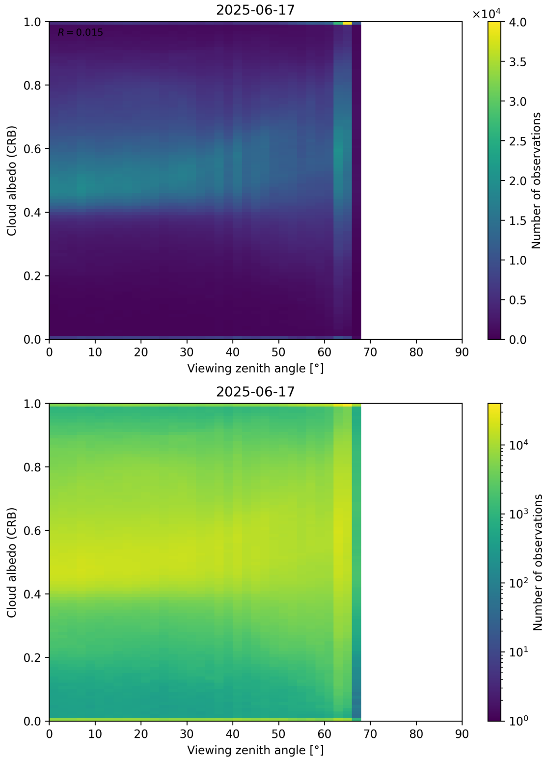
Figure 106: Scatter density plot of “Viewing zenith angle” against “Cloud albedo (CRB)” for 2025-06-17 to 2025-06-18.
