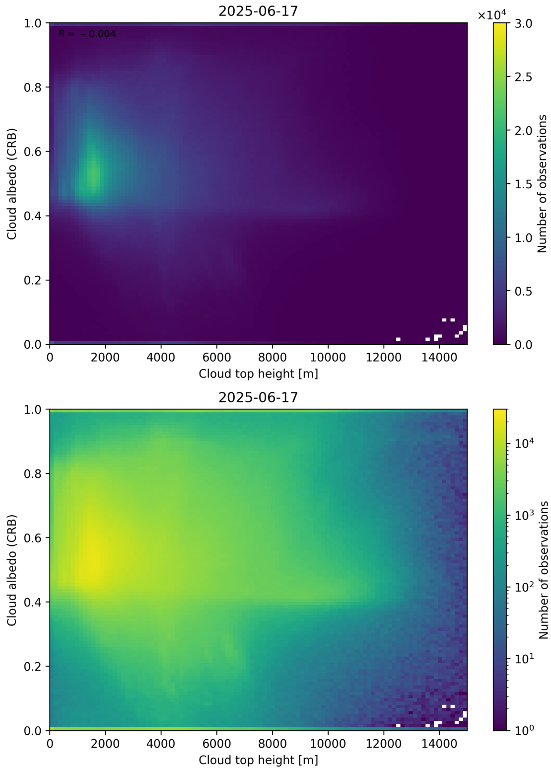
Figure 86: Scatter density plot of “Cloud top height” against “Cloud albedo (CRB)” for 2025-06-17 to 2025-06-18.
