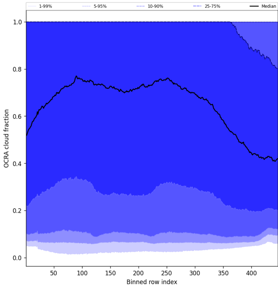
Figure 66: Along track statistics of “OCRA cloud fraction” for 2025-06-17 to 2025-06-18
