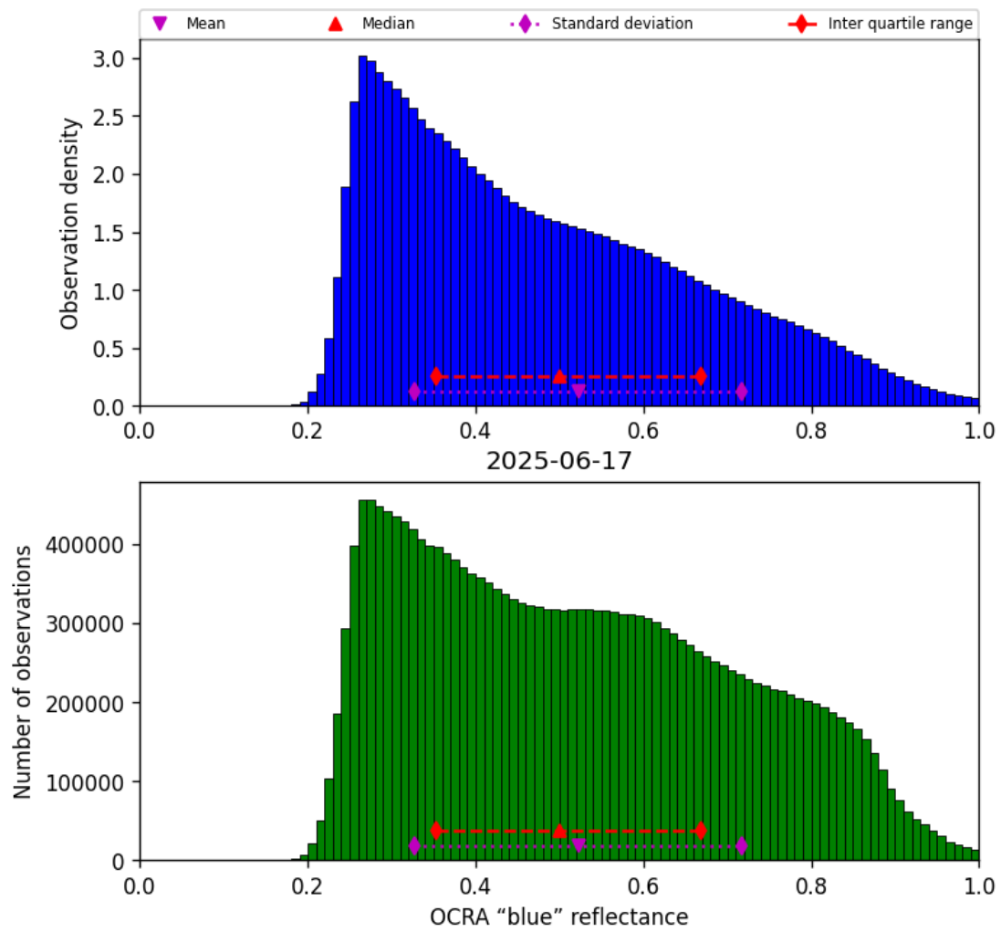
Figure 51: Histogram of “OCRA “blue” reflectance” for 2025-06-17 to 2025-06-18
