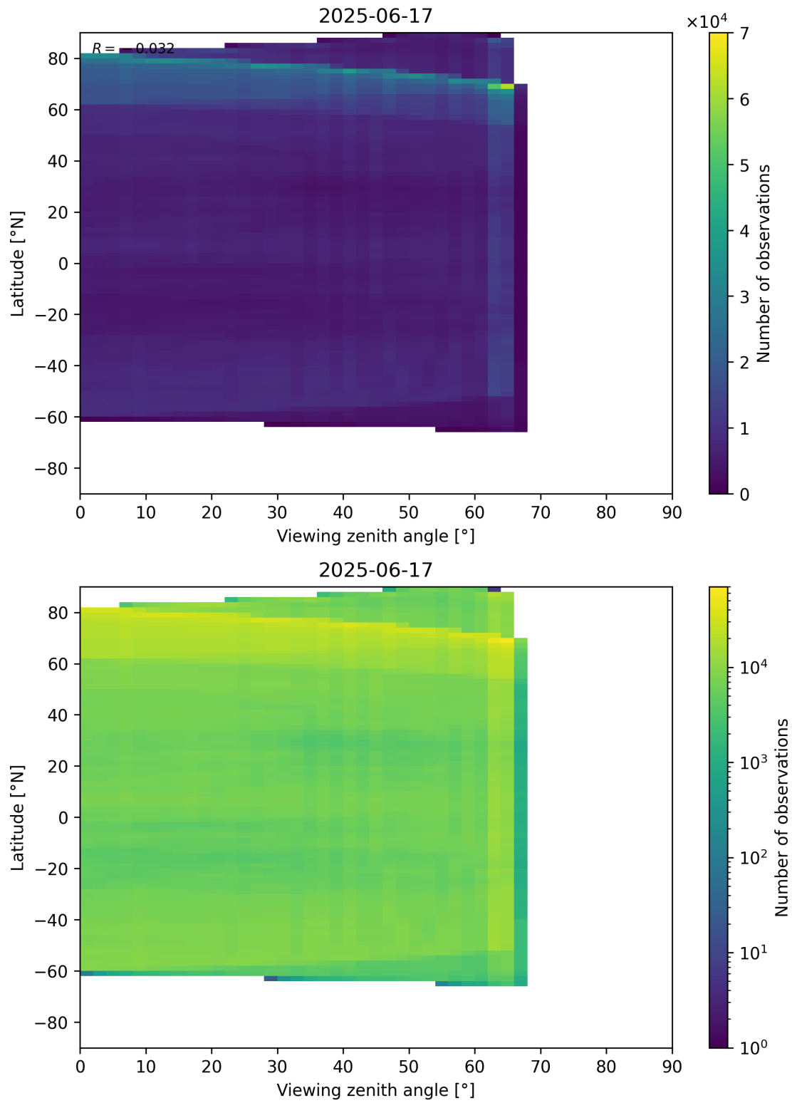
Figure 113: Scatter density plot of “Viewing zenith angle” against “Latitude” for 2025-06-17 to 2025-06-18.
