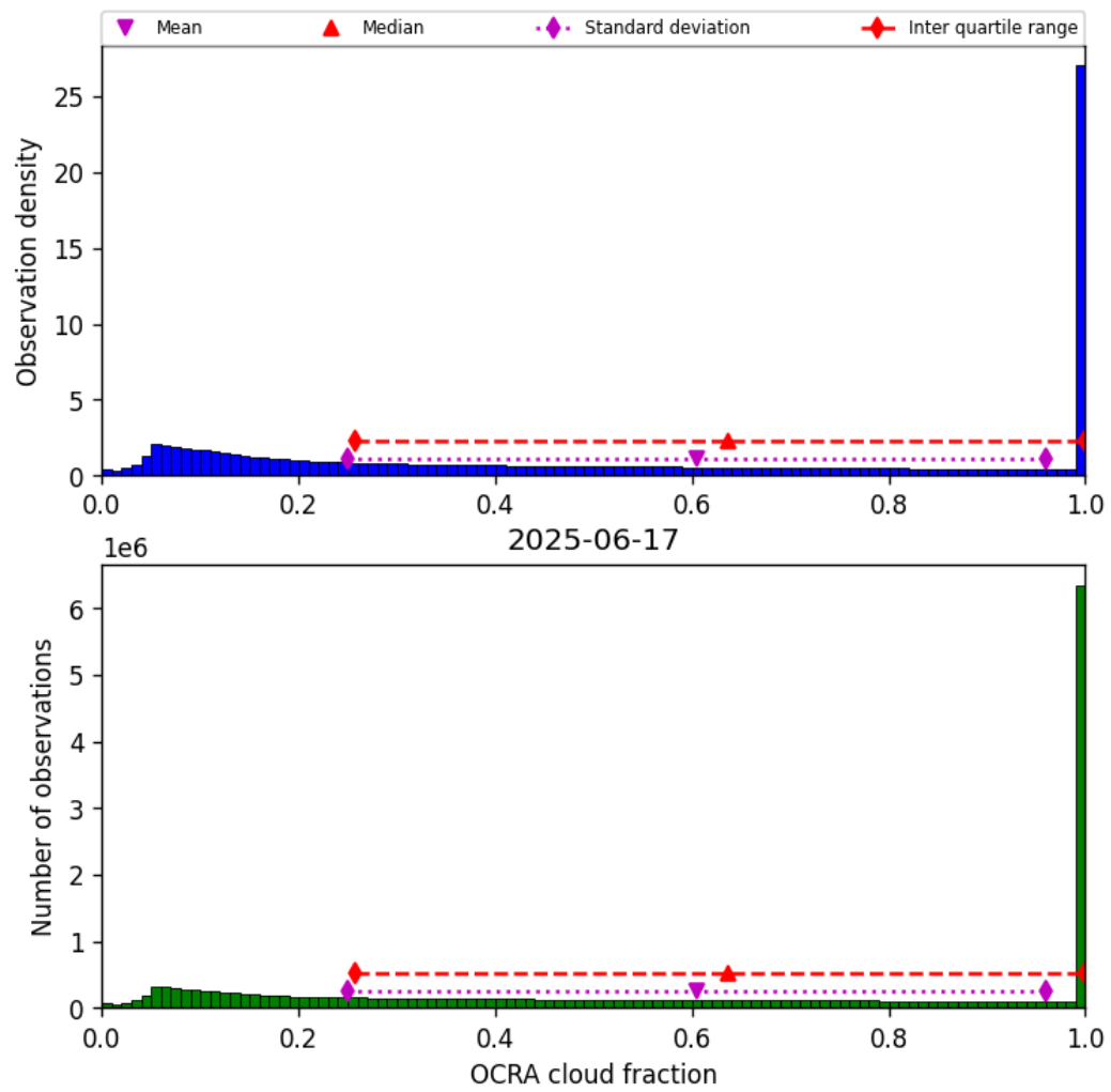
Figure 50: Histogram of “OCRA cloud fraction” for 2025-06-17 to 2025-06-18
