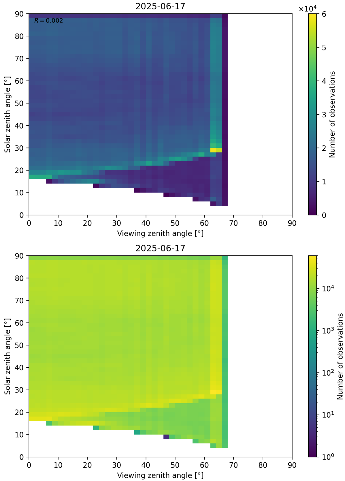
Figure 114: Scatter density plot of “Viewing zenith angle” against “Solar zenith angle” for 2025-06-17 to 2025-06-18.
