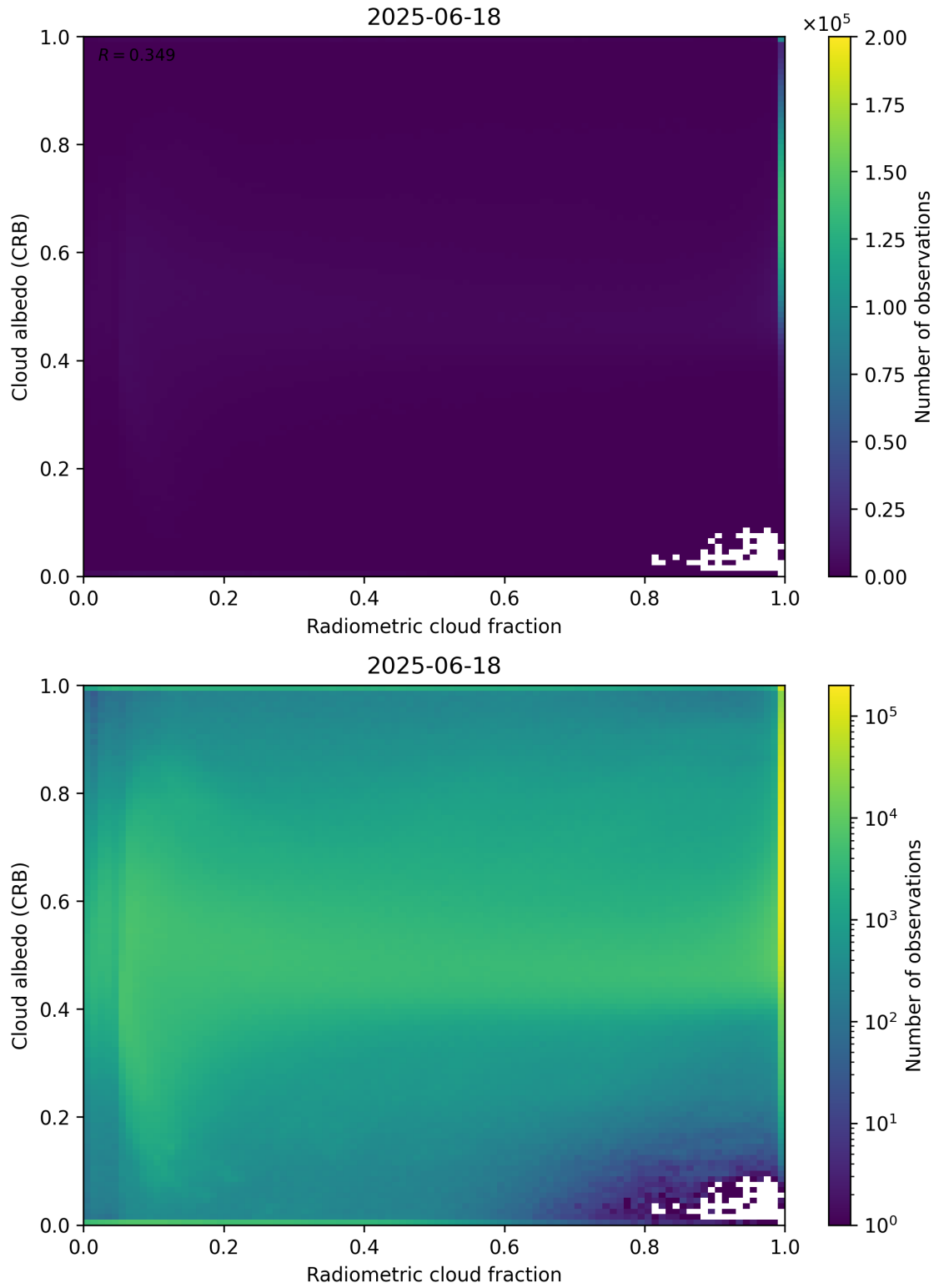
Figure 71: Scatter density plot of “Radiometric cloud fraction” against “Cloud albedo (CRB)” for 2025-06-17 to 2025-06-19.
