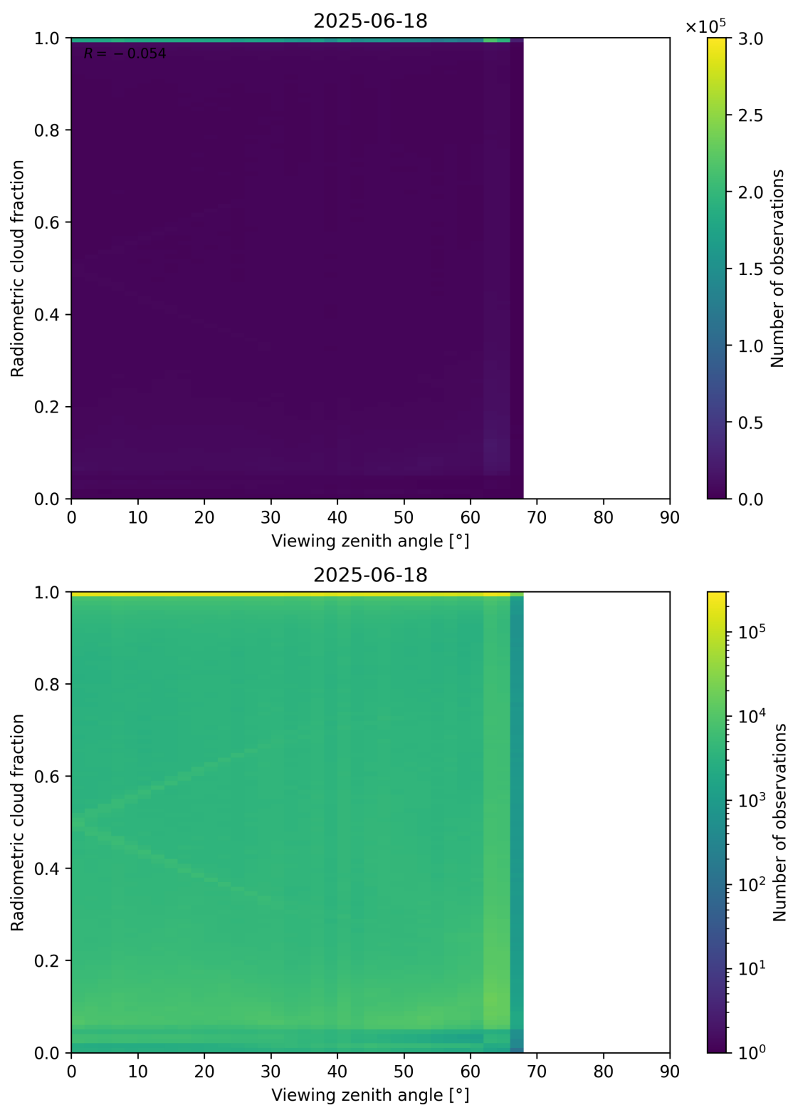
Figure 107: Scatter density plot of “Viewing zenith angle” against “Radiometric cloud fraction” for 2025-06-17 to 2025-06-19.
