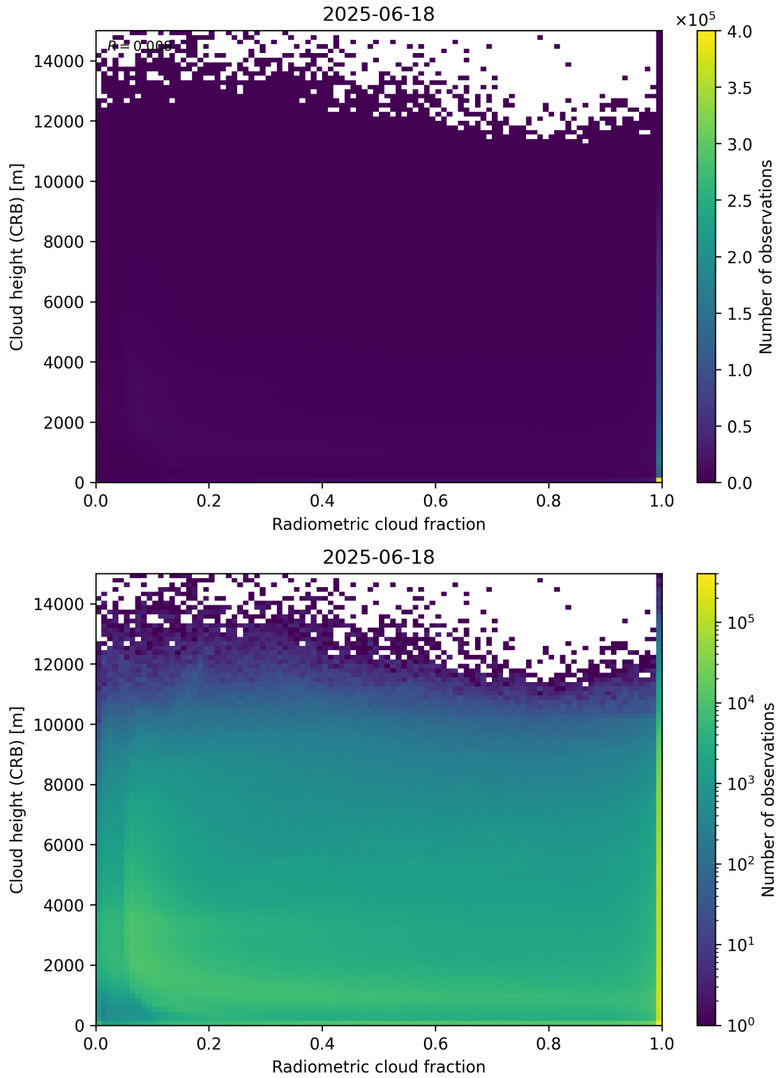
Figure 74: Scatter density plot of “Radiometric cloud fraction” against “Cloud height (CRB)” for 2025-06-17 to 2025-06-19.
