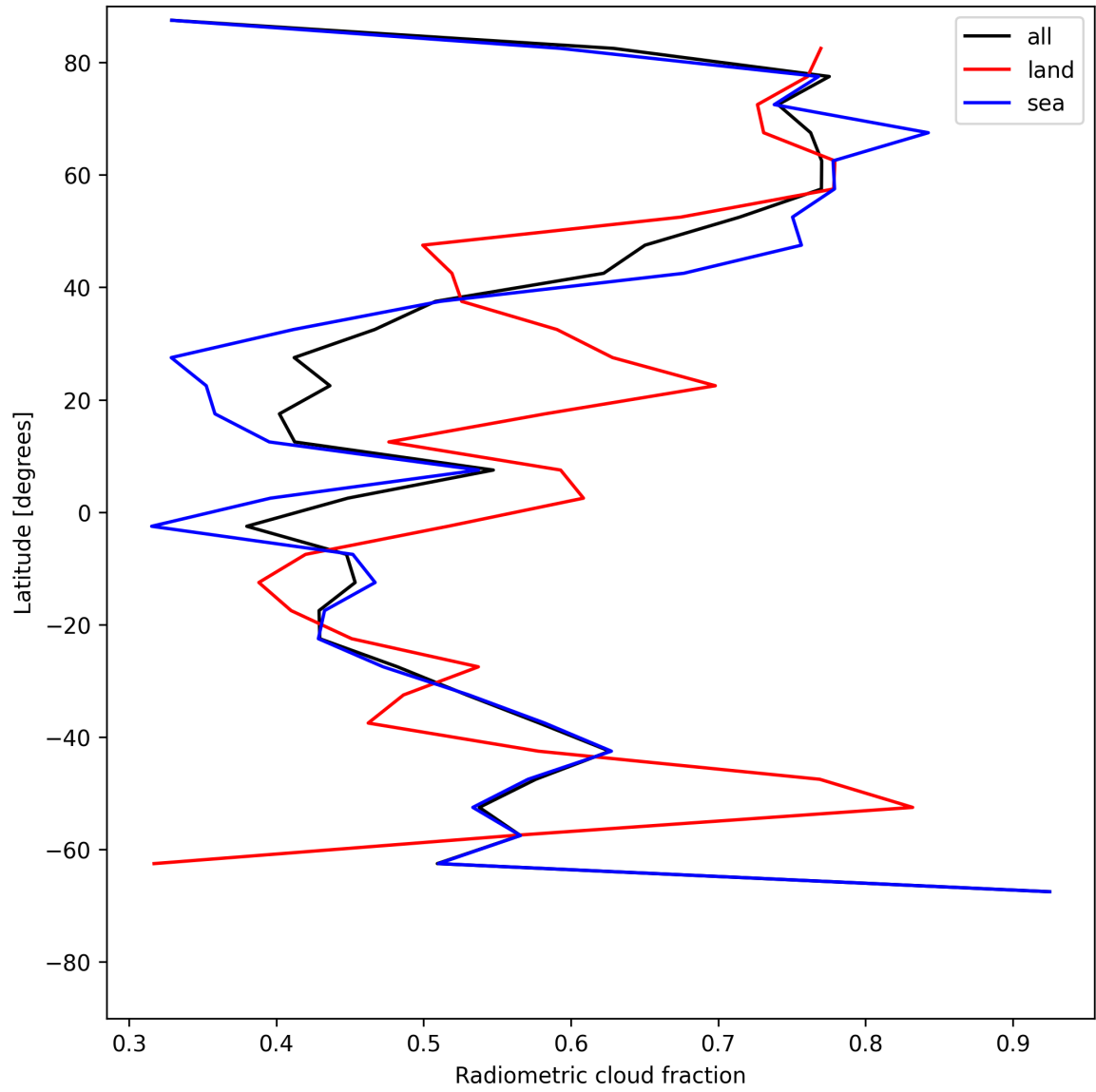
Figure 23: Zonal average of “Radiometric cloud fraction” for 2025-06-17 to 2025-06-19.
