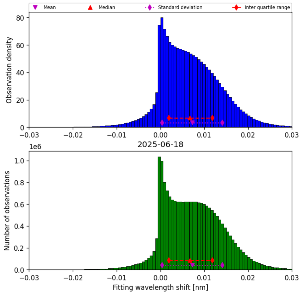
Figure 49: Histogram of “Fitting wavelength shift” for 2025-06-17 to 2025-06-19
