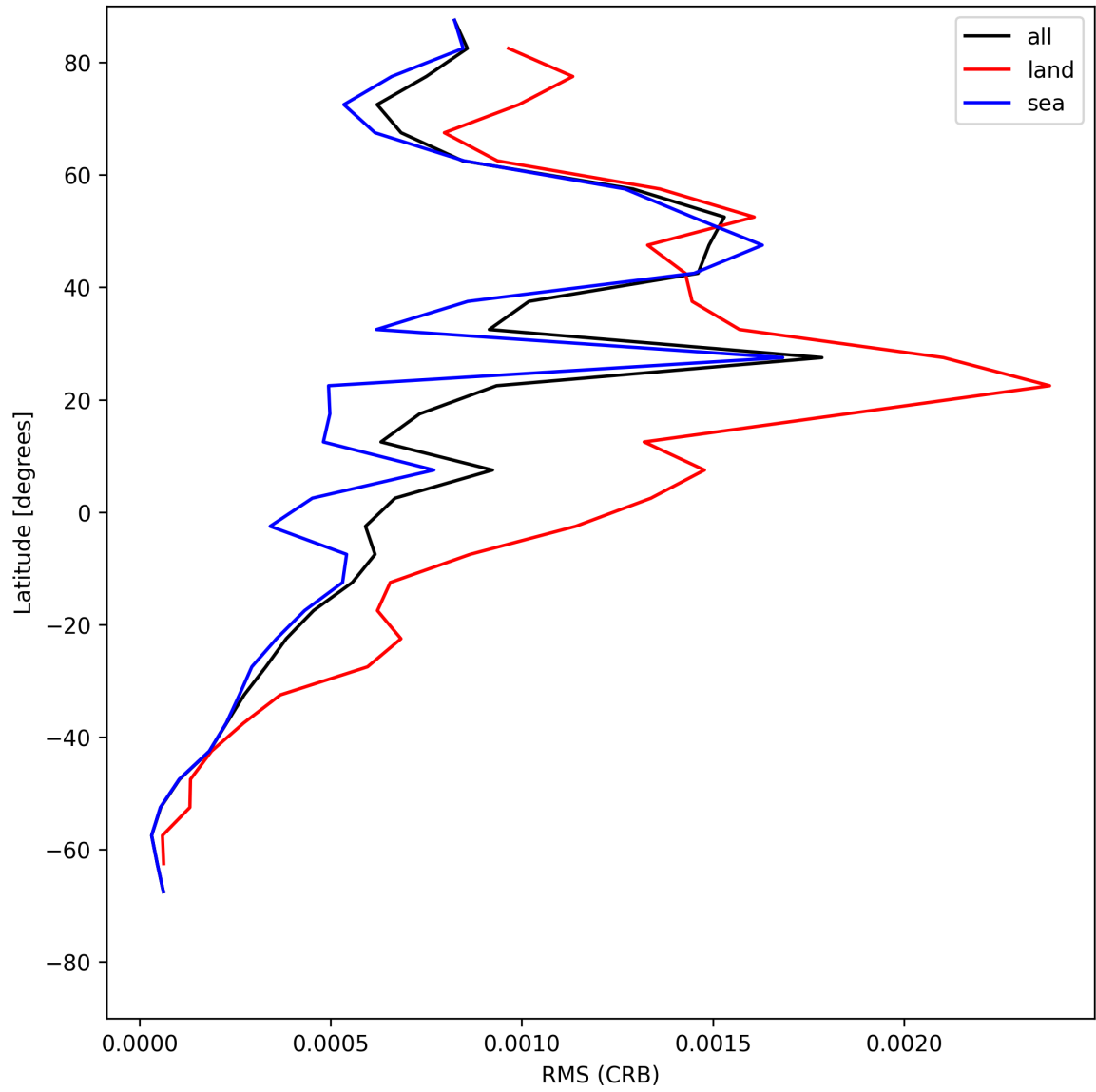
Figure 32: Zonal average of “RMS (CRB)” for 2025-06-17 to 2025-06-19.
