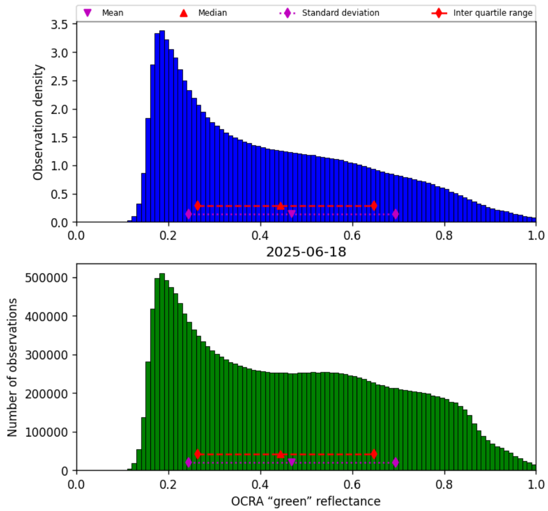
Figure 52: Histogram of “OCRA “green” reflectance” for 2025-06-17 to 2025-06-19
