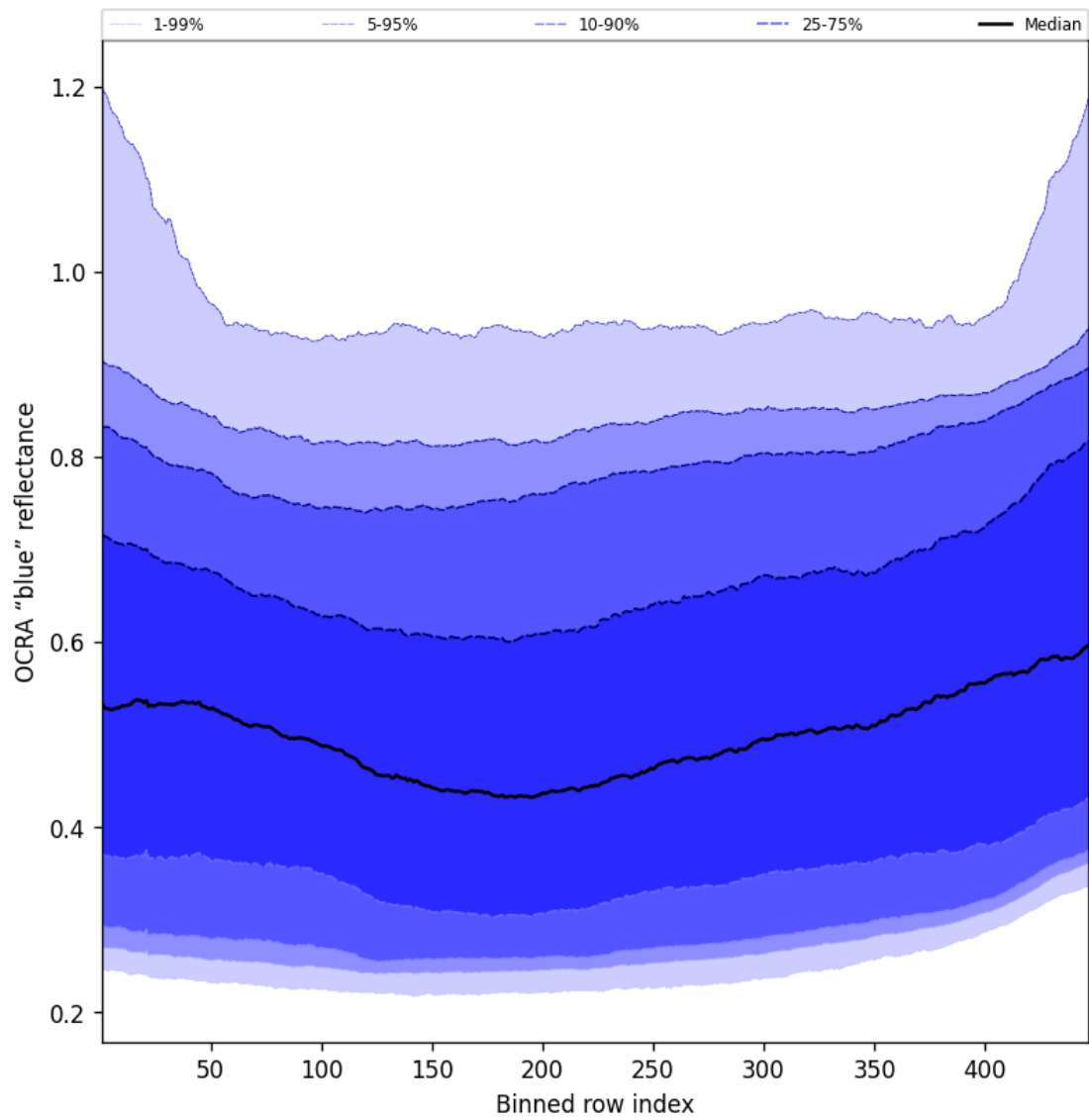
Figure 67: Along track statistics of “OCRA “blue” reflectance” for 2025-06-17 to 2025-06-19
