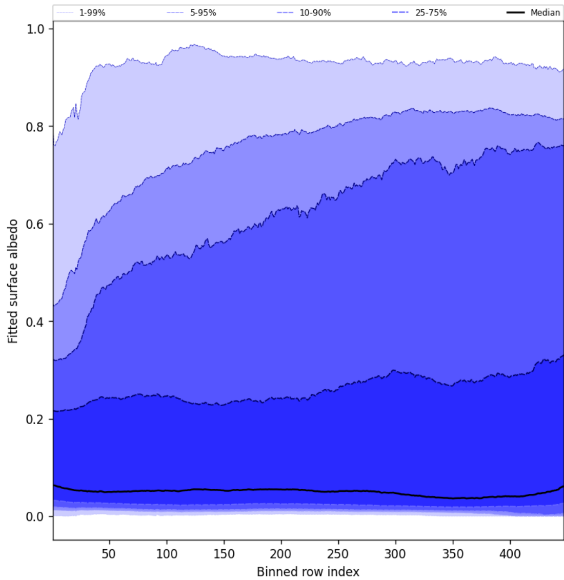
Figure 61: Along track statistics of “Fitted surface albedo” for 2025-06-17 to 2025-06-19
