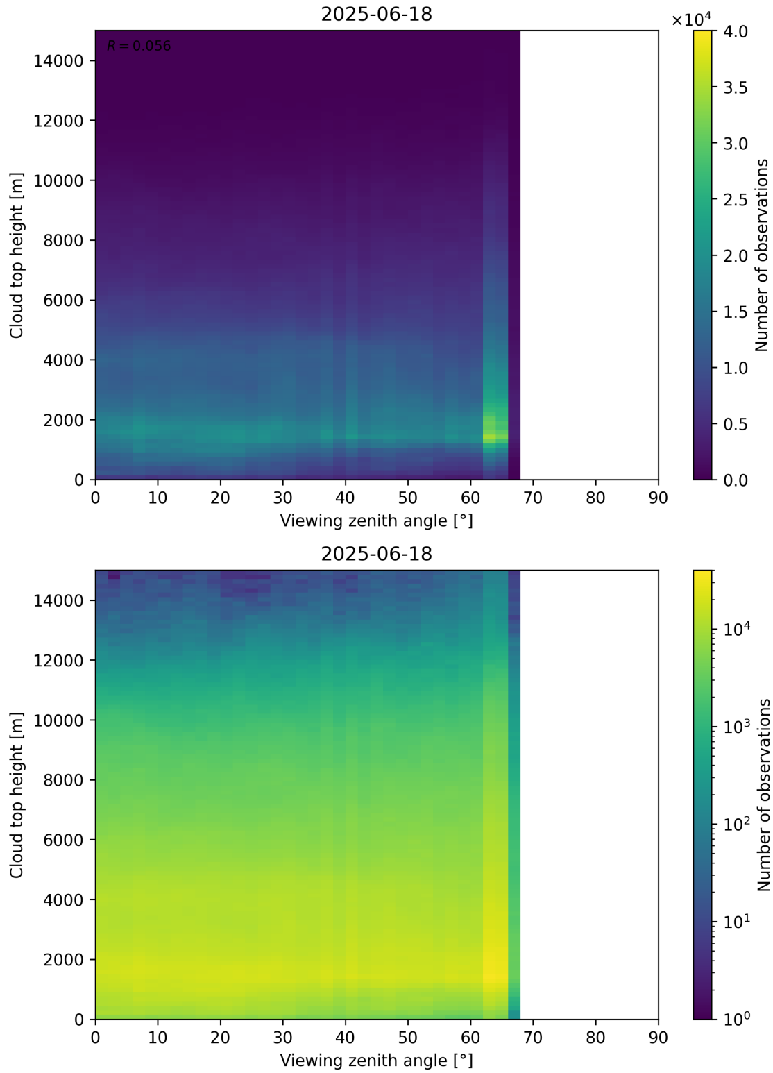
Figure 112: Scatter density plot of “Viewing zenith angle” against “Cloud top height” for 2025-06-17 to 2025-06-19.
