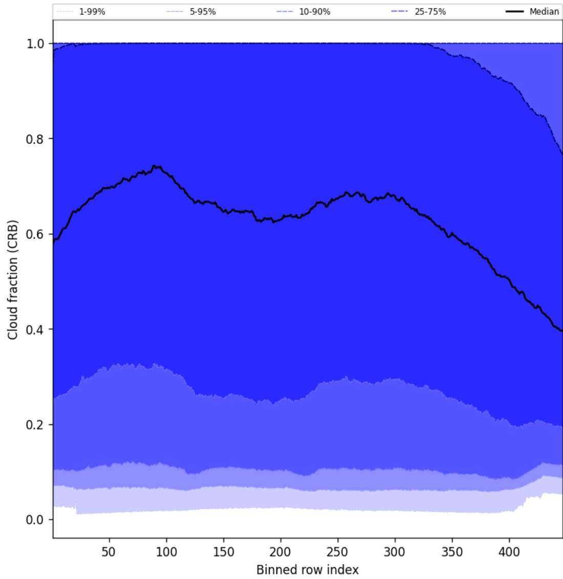
Figure 58: Along track statistics of “Cloud fraction (CRB)” for 2025-06-17 to 2025-06-19
