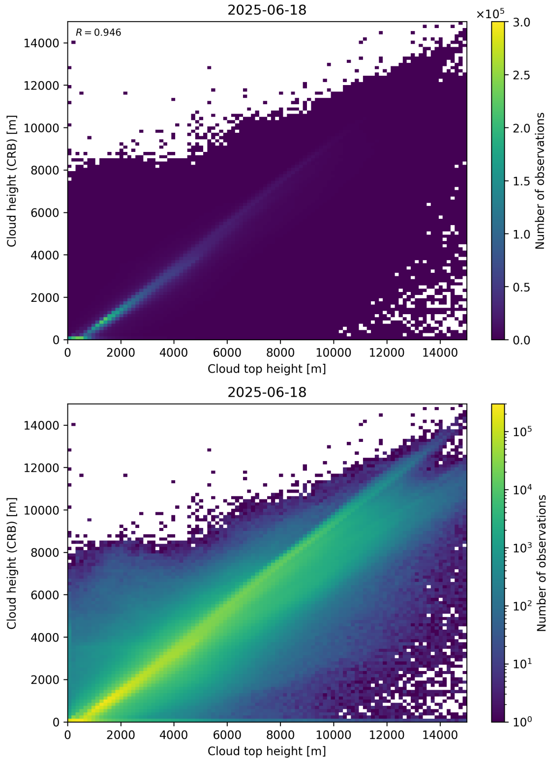
Figure 89: Scatter density plot of “Cloud top height” against “Cloud height (CRB)” for 2025-06-17 to 2025-06-19.
