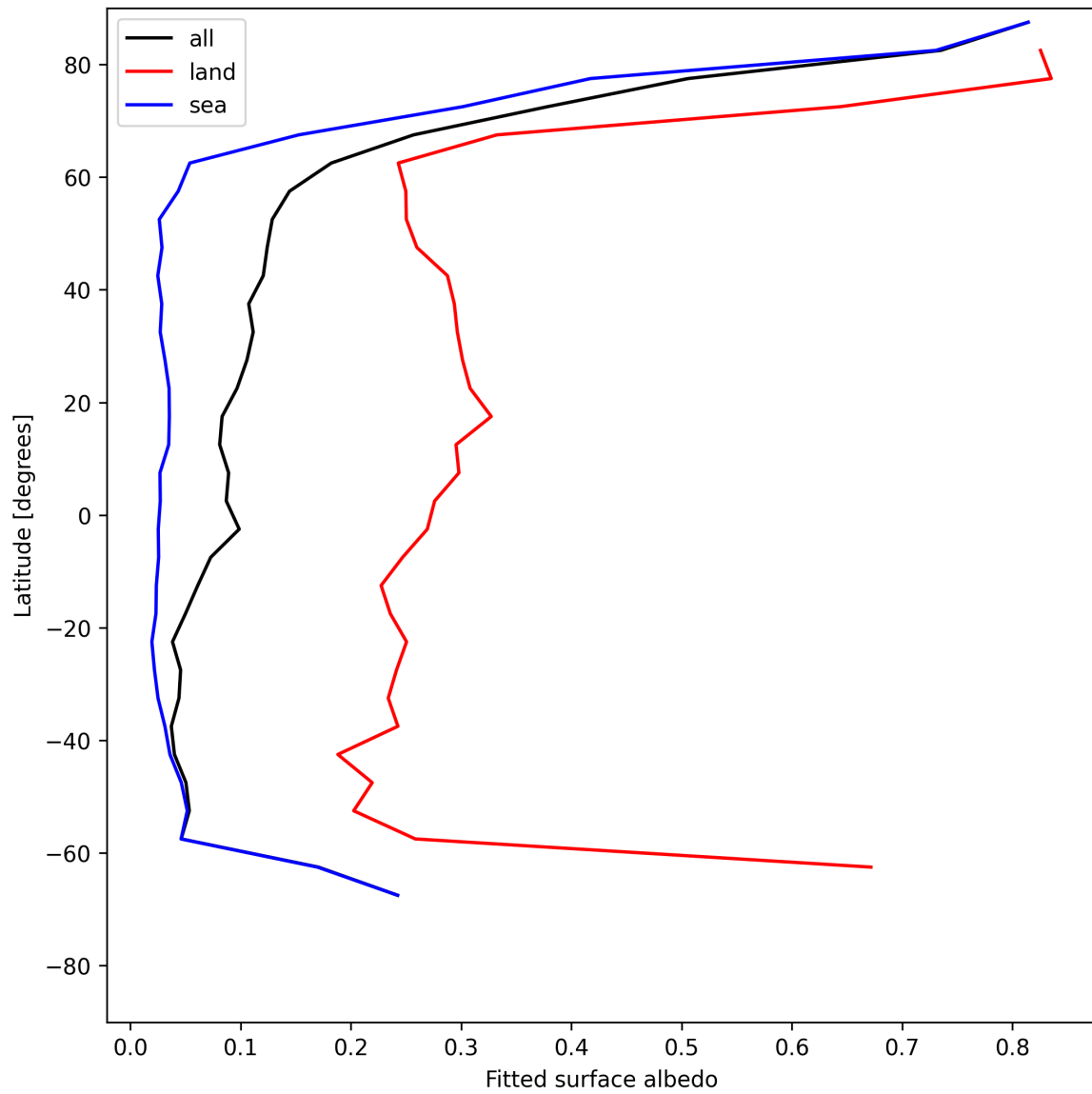
Figure 29: Zonal average of “Fitted surface albedo” for 2025-06-17 to 2025-06-19.
