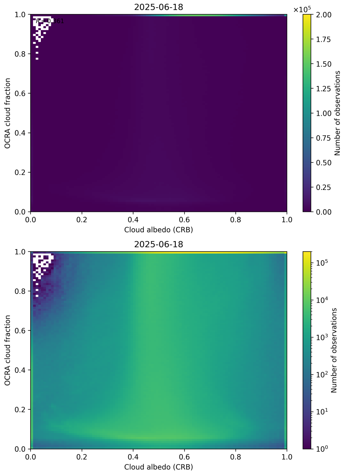
Figure 70: Scatter density plot of “Cloud albedo (CRB)” against “OCRA cloud fraction” for 2025-06-17 to 2025-06-19.
