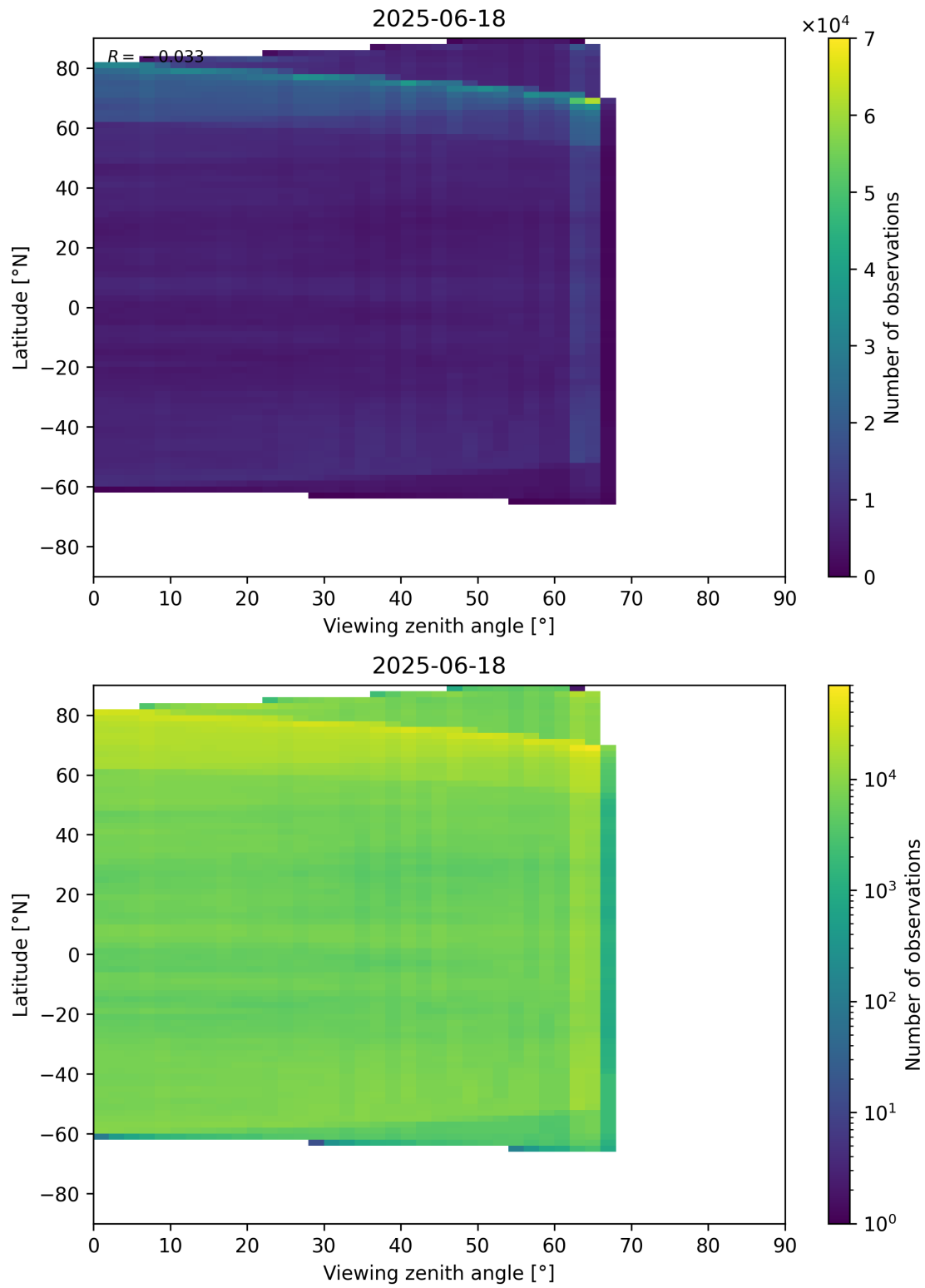
Figure 113: Scatter density plot of “Viewing zenith angle” against “Latitude” for 2025-06-17 to 2025-06-19.
