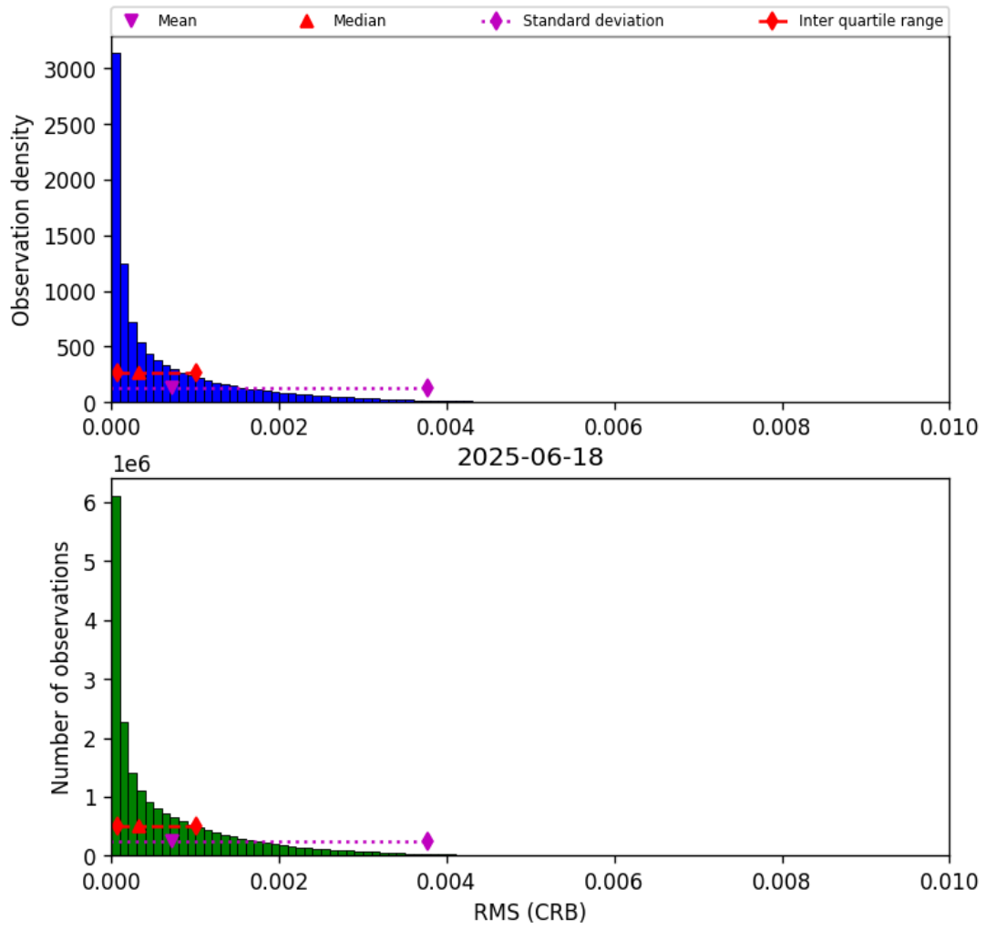
Figure 48: Histogram of “RMS (CRB)” for 2025-06-17 to 2025-06-19
