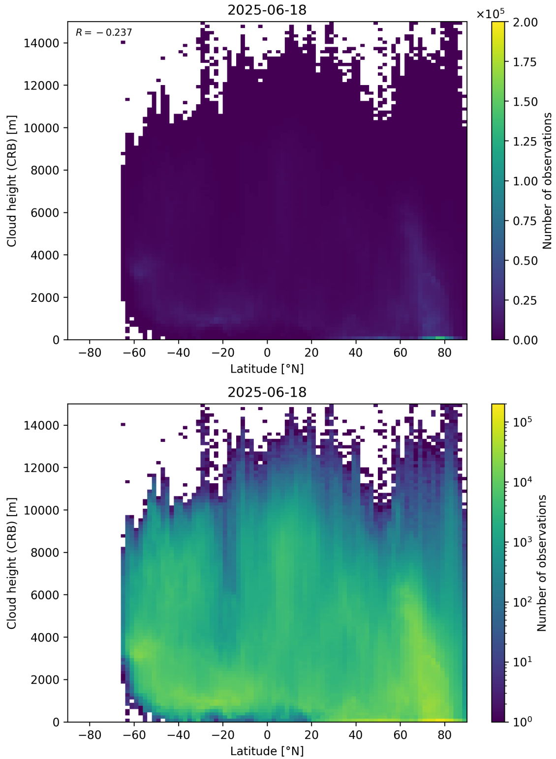
Figure 95: Scatter density plot of “Latitude” against “Cloud height (CRB)” for 2025-06-17 to 2025-06-19.
