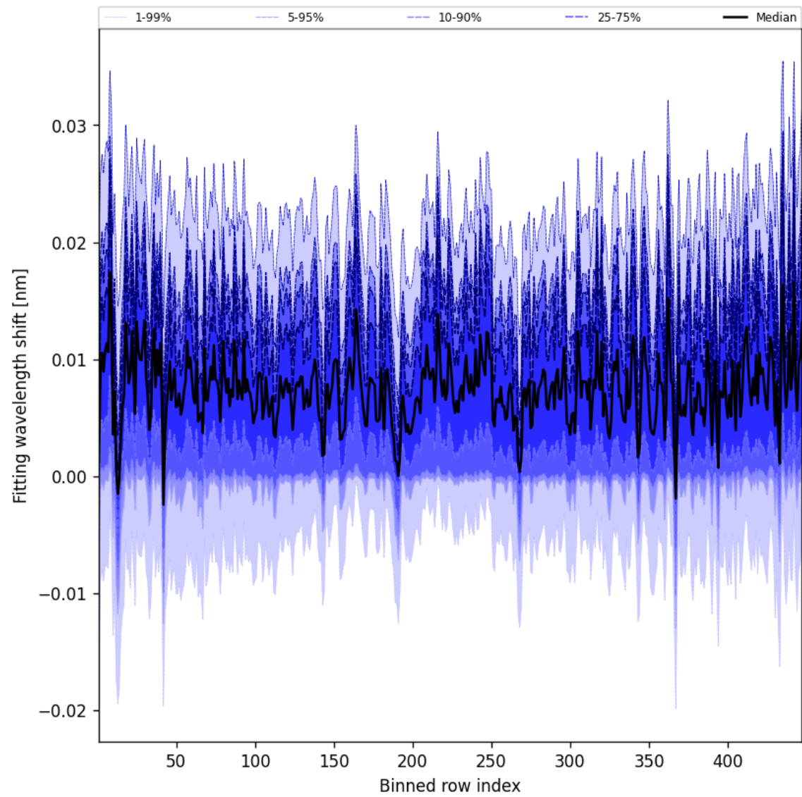
Figure 65: Along track statistics of “Fitting wavelength shift” for 2025-06-17 to 2025-06-19
