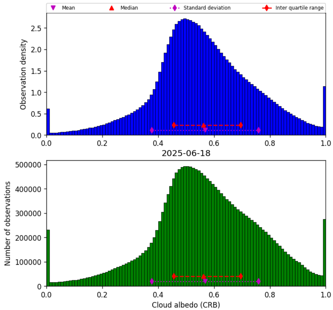
Figure 44: Histogram of “Cloud albedo (CRB)” for 2025-06-17 to 2025-06-19
