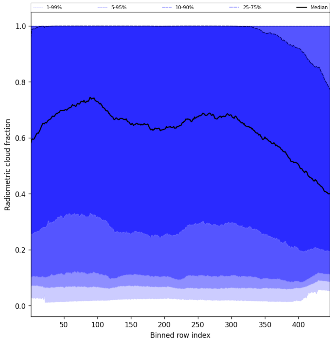
Figure 55: Along track statistics of “Radiometric cloud fraction” for 2025-06-17 to 2025-06-19
