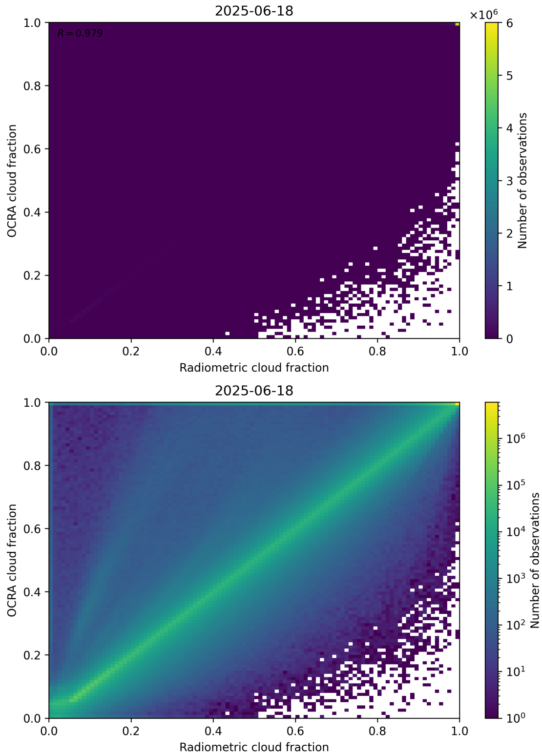
Figure 72: Scatter density plot of “Radiometric cloud fraction” against “OCRA cloud fraction” for 2025-06-17 to 2025-06-19.
