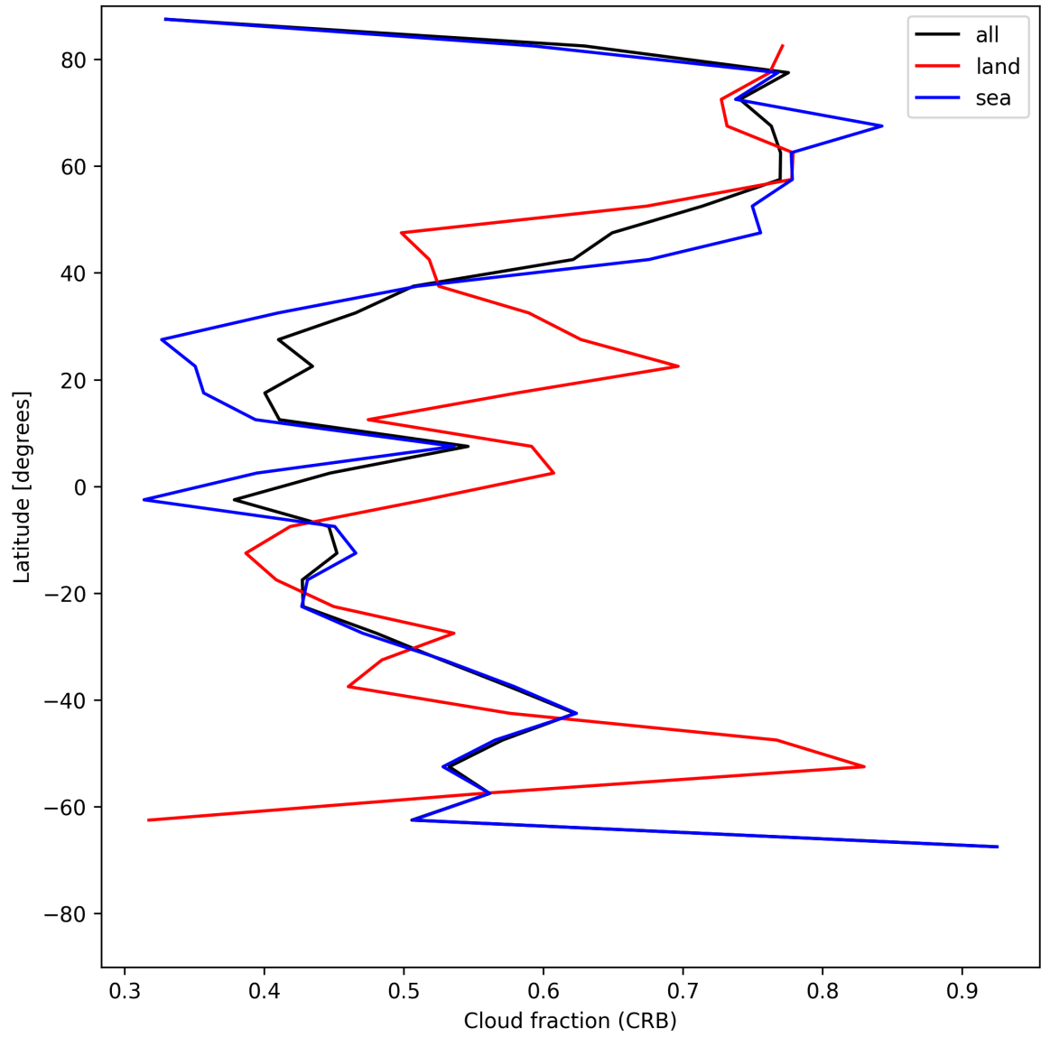
Figure 26: Zonal average of “Cloud fraction (CRB)” for 2025-06-17 to 2025-06-19.
