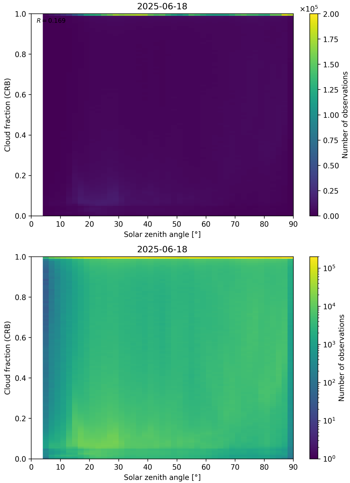
Figure 101: Scatter density plot of “Solar zenith angle” against “Cloud fraction (CRB)” for 2025-06-17 to 2025-06-19.
