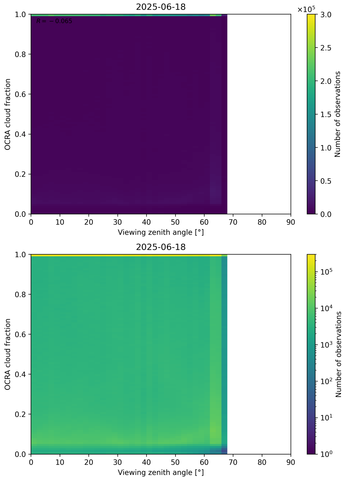
Figure 108: Scatter density plot of “Viewing zenith angle” against “OCRA cloud fraction” for 2025-06-17 to 2025-06-19.
