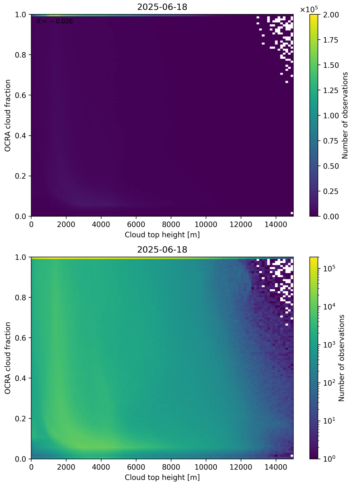
Figure 87: Scatter density plot of “Cloud top height” against “OCRA cloud fraction” for 2025-06-17 to 2025-06-19.
