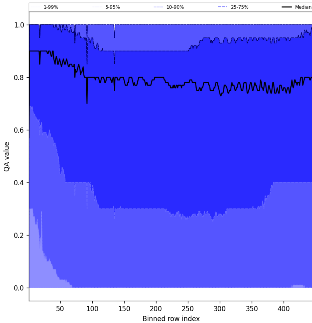
Figure 54: Along track statistics of “QA value” for 2025-06-17 to 2025-06-19
