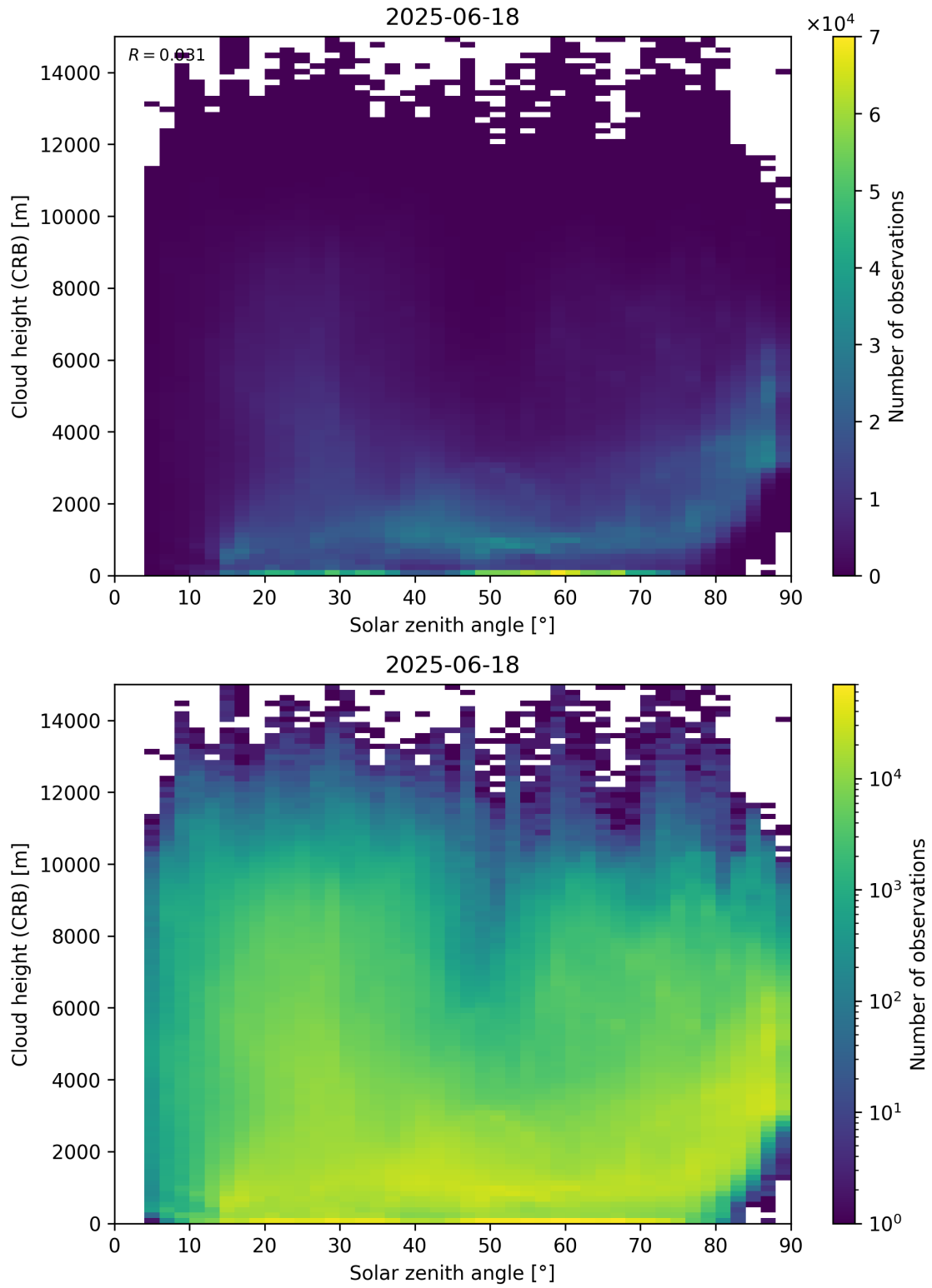
Figure 102: Scatter density plot of “Solar zenith angle” against “Cloud height (CRB)” for 2025-06-17 to 2025-06-19.
