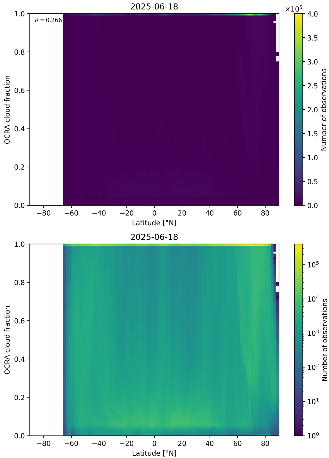
Figure 93: Scatter density plot of “Latitude” against “OCRA cloud fraction” for 2025-06-17 to 2025-06-19.
