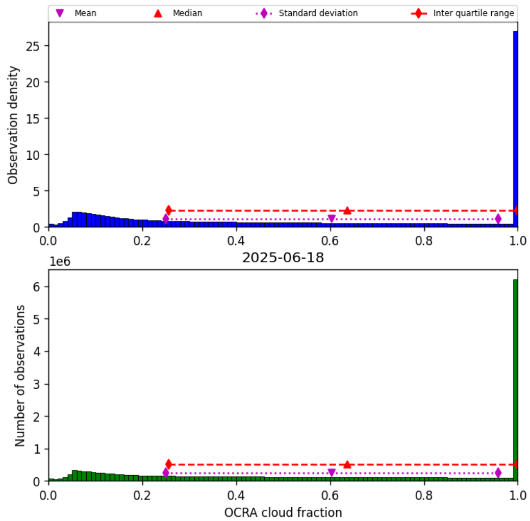
Figure 50: Histogram of “OCRA cloud fraction” for 2025-06-17 to 2025-06-19
