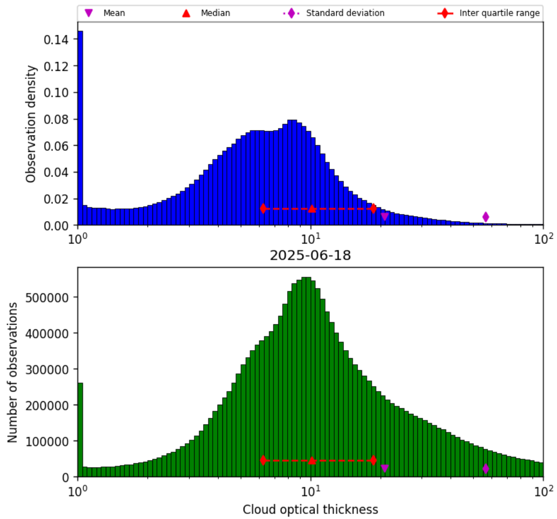
Figure 41: Histogram of “Cloud optical thickness” for 2025-06-17 to 2025-06-19
