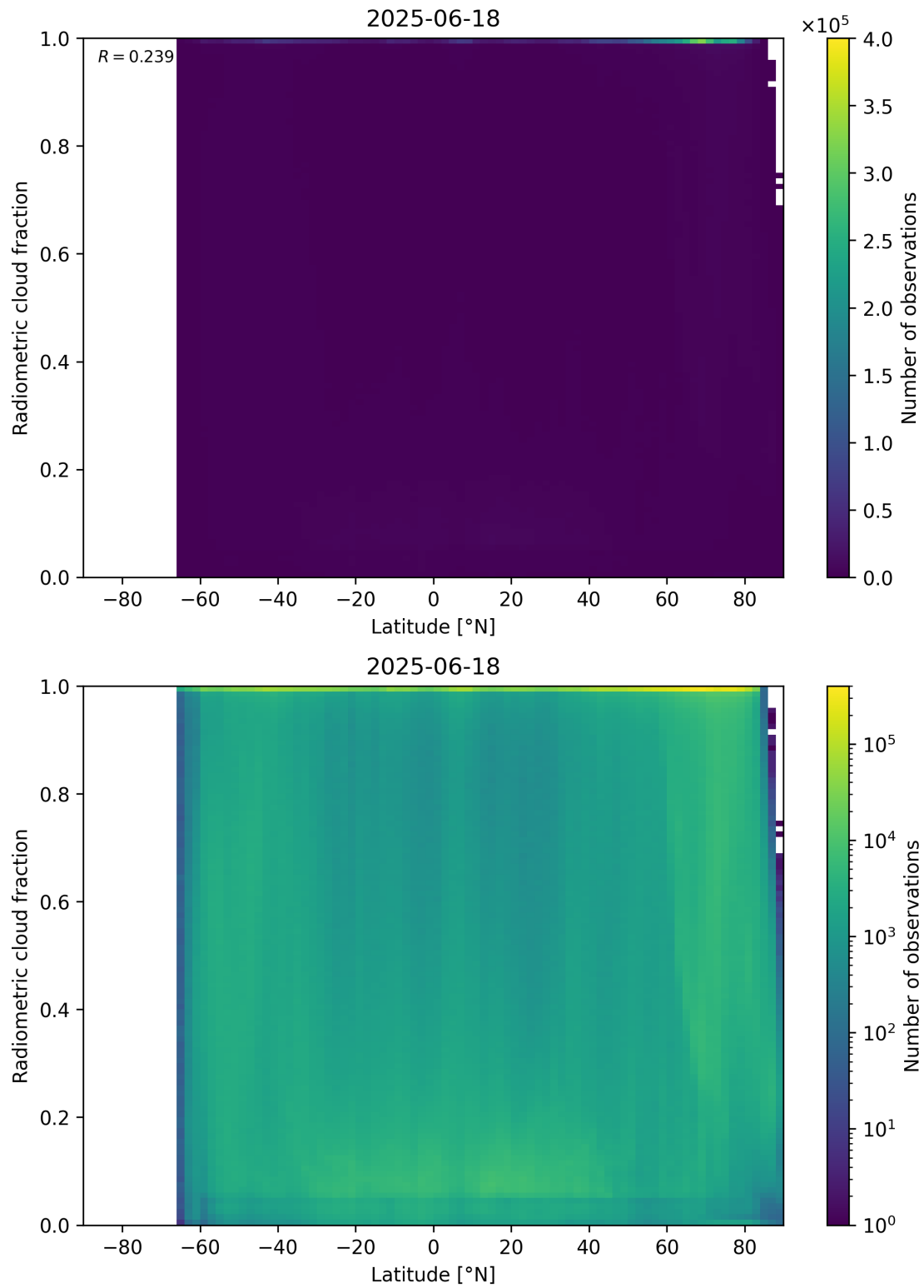
Figure 92: Scatter density plot of “Latitude” against “Radiometric cloud fraction” for 2025-06-17 to 2025-06-19.
