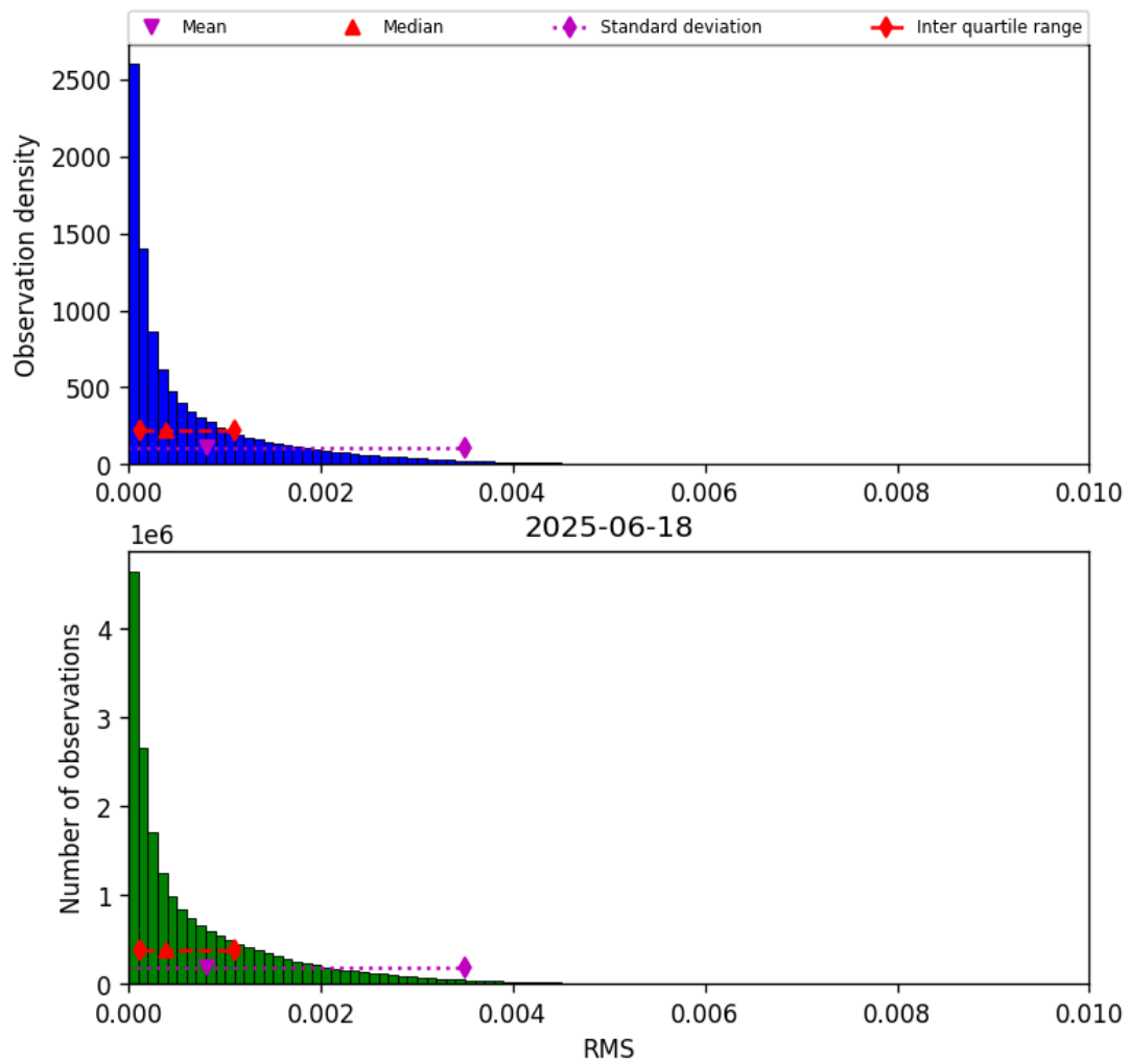
Figure 47: Histogram of “RMS” for 2025-06-17 to 2025-06-19
