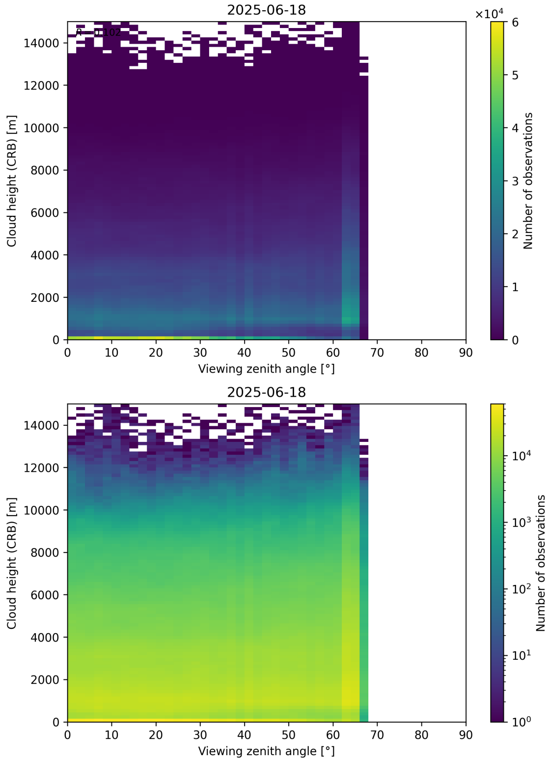
Figure 110: Scatter density plot of “Viewing zenith angle” against “Cloud height (CRB)” for 2025-06-17 to 2025-06-19.
