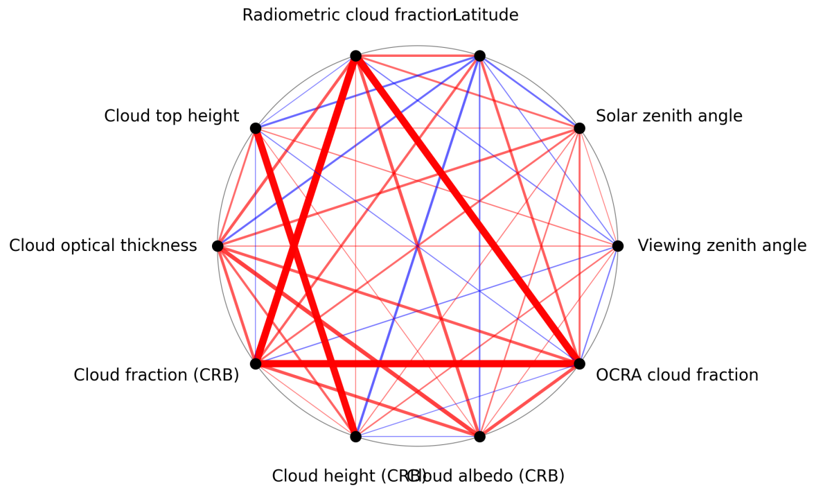
Figure 1: Map of correlation graph for 2025-06-17 to 2025-06-19.
