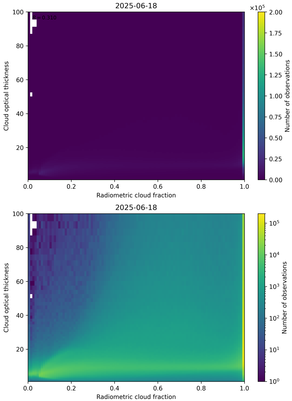
Figure 75: Scatter density plot of “Radiometric cloud fraction” against “Cloud optical thickness” for 2025-06-17 to 2025-06-19.
