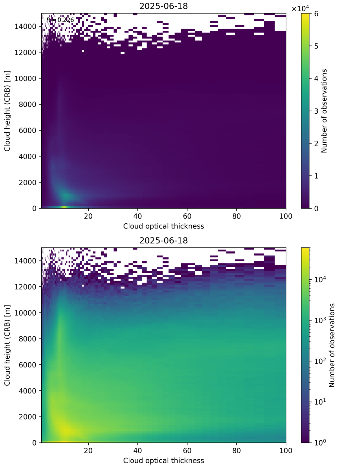
Figure 85: Scatter density plot of “Cloud optical thickness” against “Cloud height (CRB)” for 2025-06-17 to 2025-06-19.
