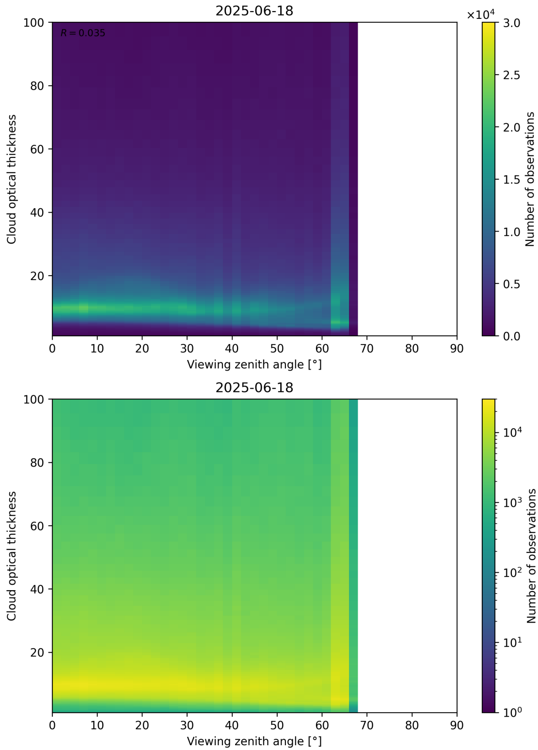
Figure 111: Scatter density plot of “Viewing zenith angle” against “Cloud optical thickness” for 2025-06-17 to 2025-06-19.
