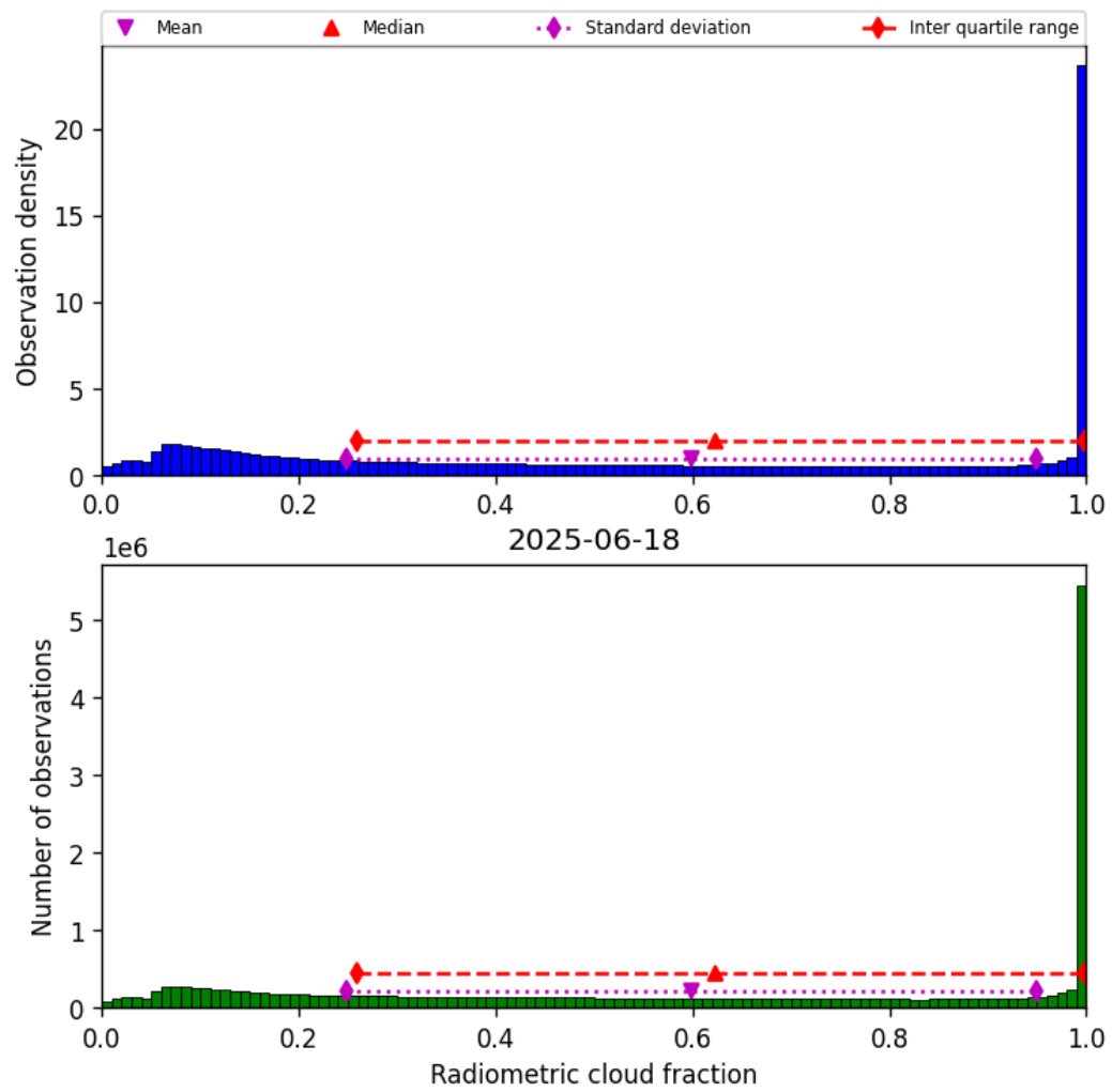
Figure 39: Histogram of “Radiometric cloud fraction” for 2025-06-17 to 2025-06-19
