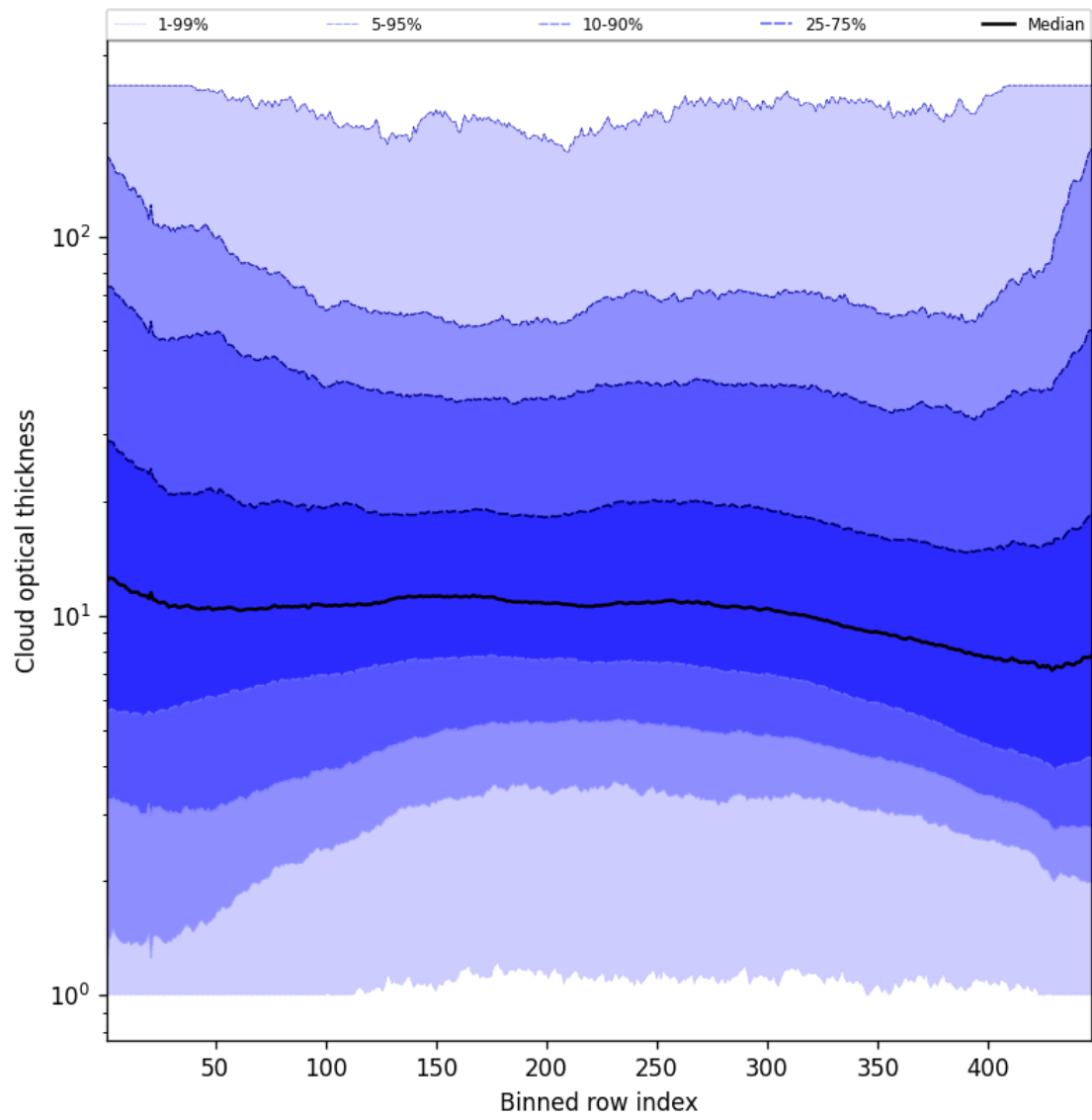
Figure 57: Along track statistics of “Cloud optical thickness” for 2025-06-17 to 2025-06-19
