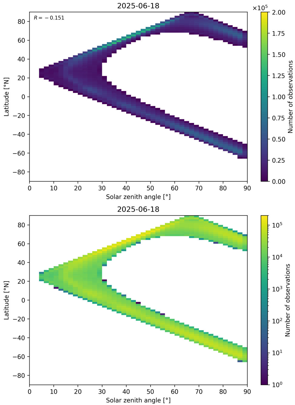
Figure 105: Scatter density plot of “Solar zenith angle” against “Latitude” for 2025-06-17 to 2025-06-19.
