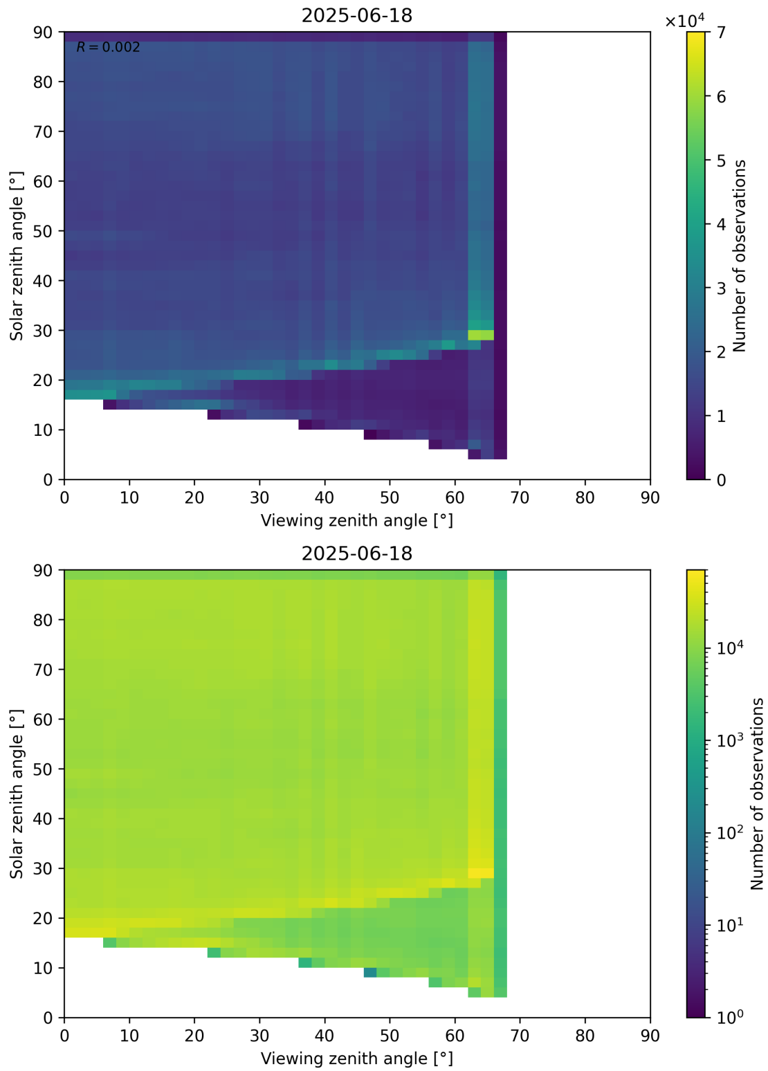
Figure 114: Scatter density plot of “Viewing zenith angle” against “Solar zenith angle” for 2025-06-17 to 2025-06-19.
