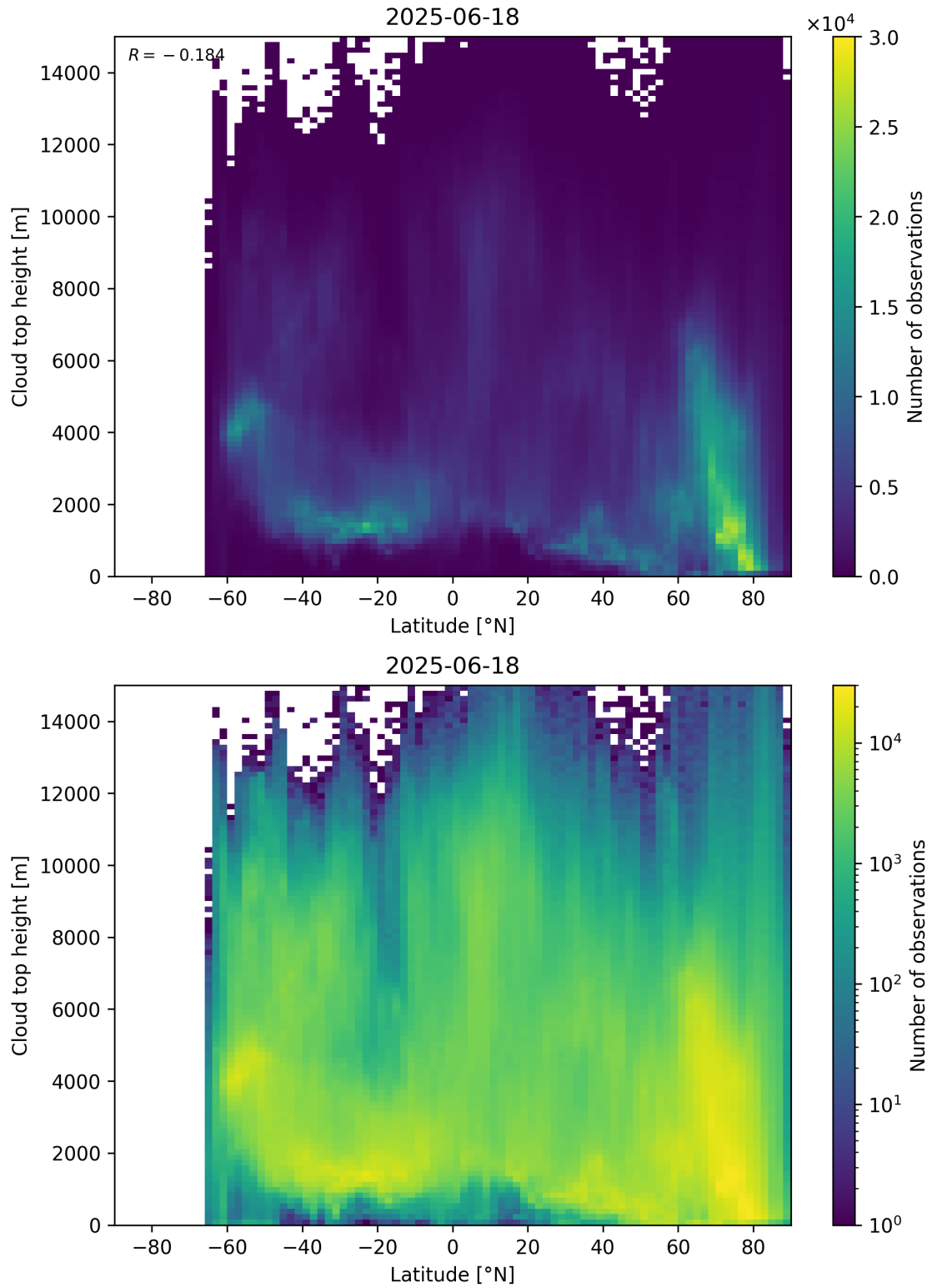
Figure 97: Scatter density plot of “Latitude” against “Cloud top height” for 2025-06-17 to 2025-06-19.
