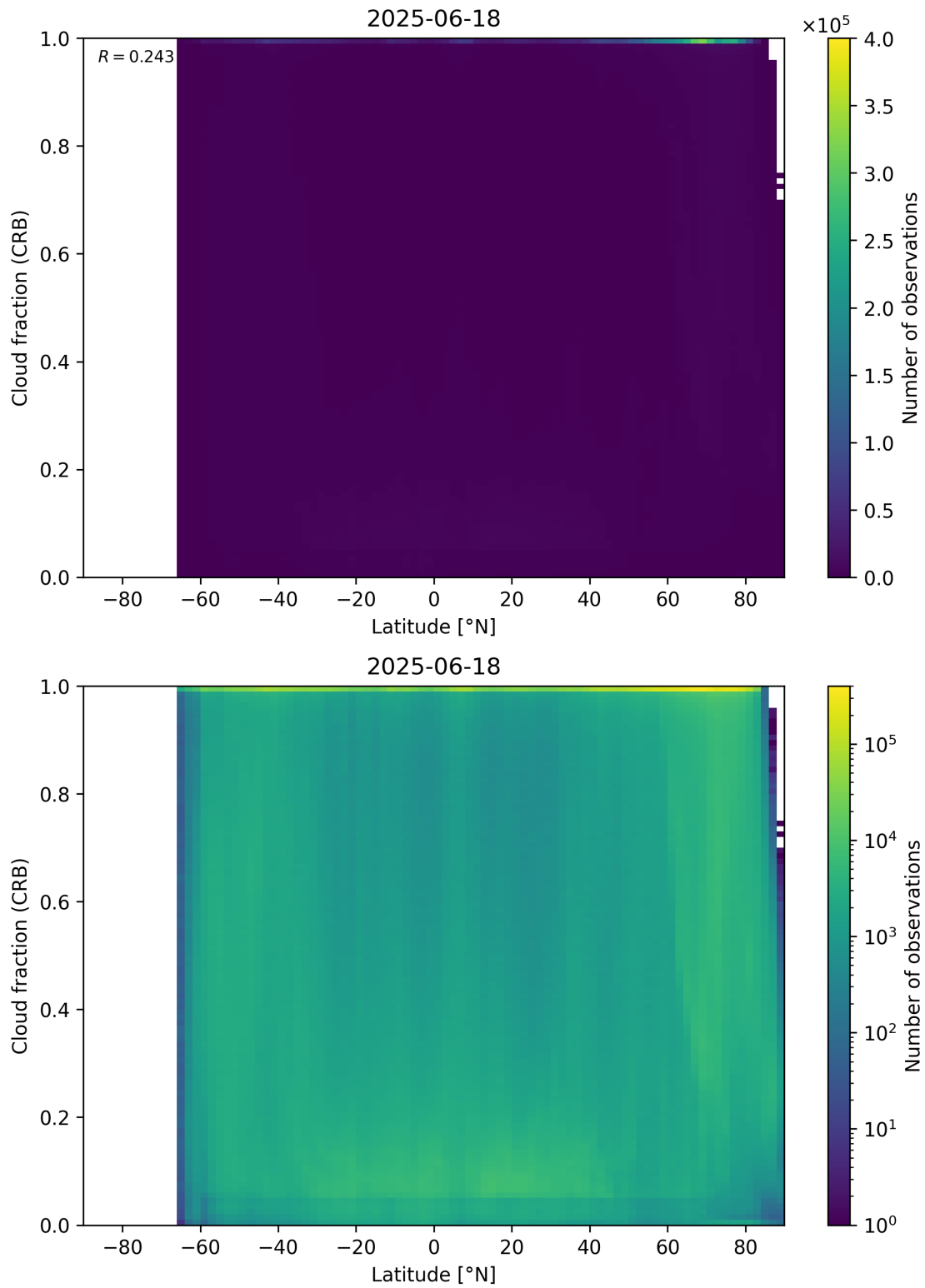
Figure 94: Scatter density plot of “Latitude” against “Cloud fraction (CRB)” for 2025-06-17 to 2025-06-19.
