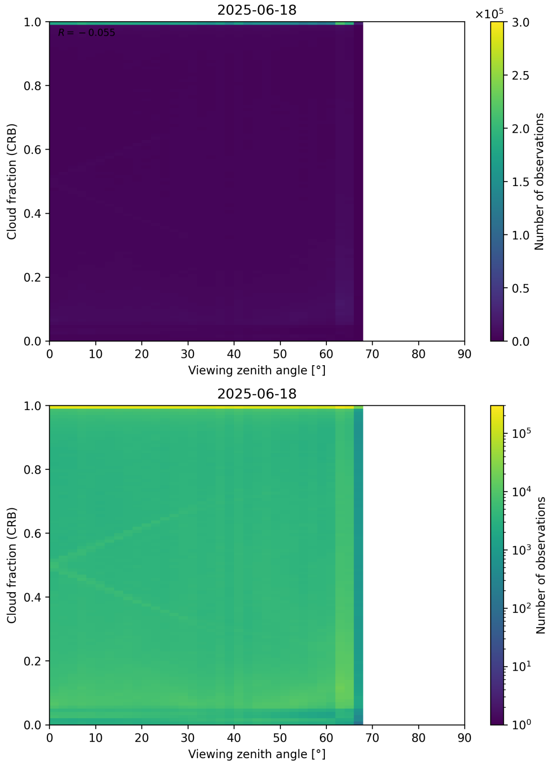
Figure 109: Scatter density plot of “Viewing zenith angle” against “Cloud fraction (CRB)” for 2025-06-17 to 2025-06-19.
