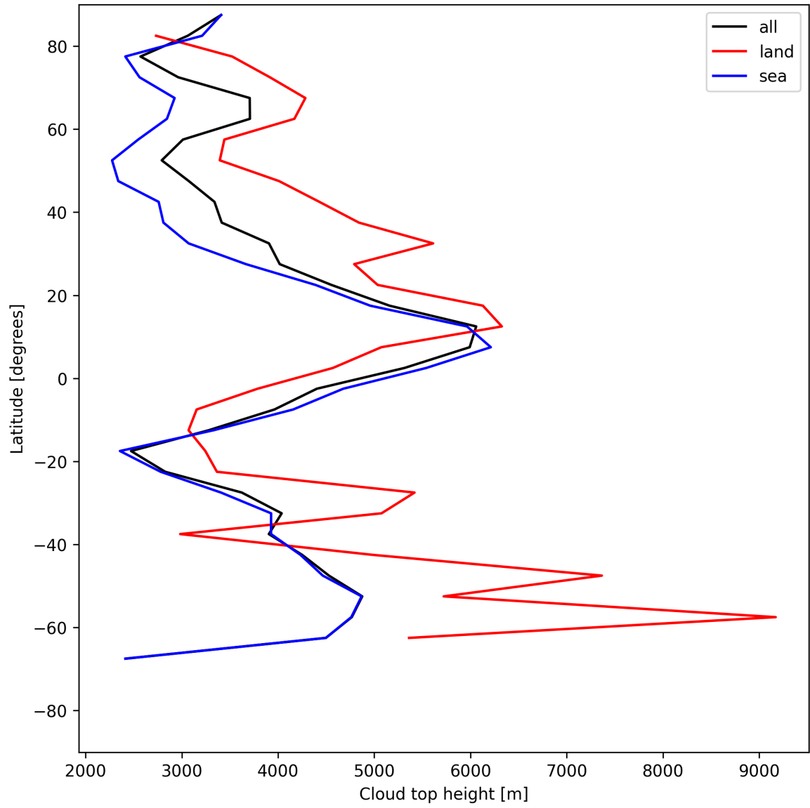
Figure 24: Zonal average of “Cloud top height” for 2025-06-17 to 2025-06-19.
