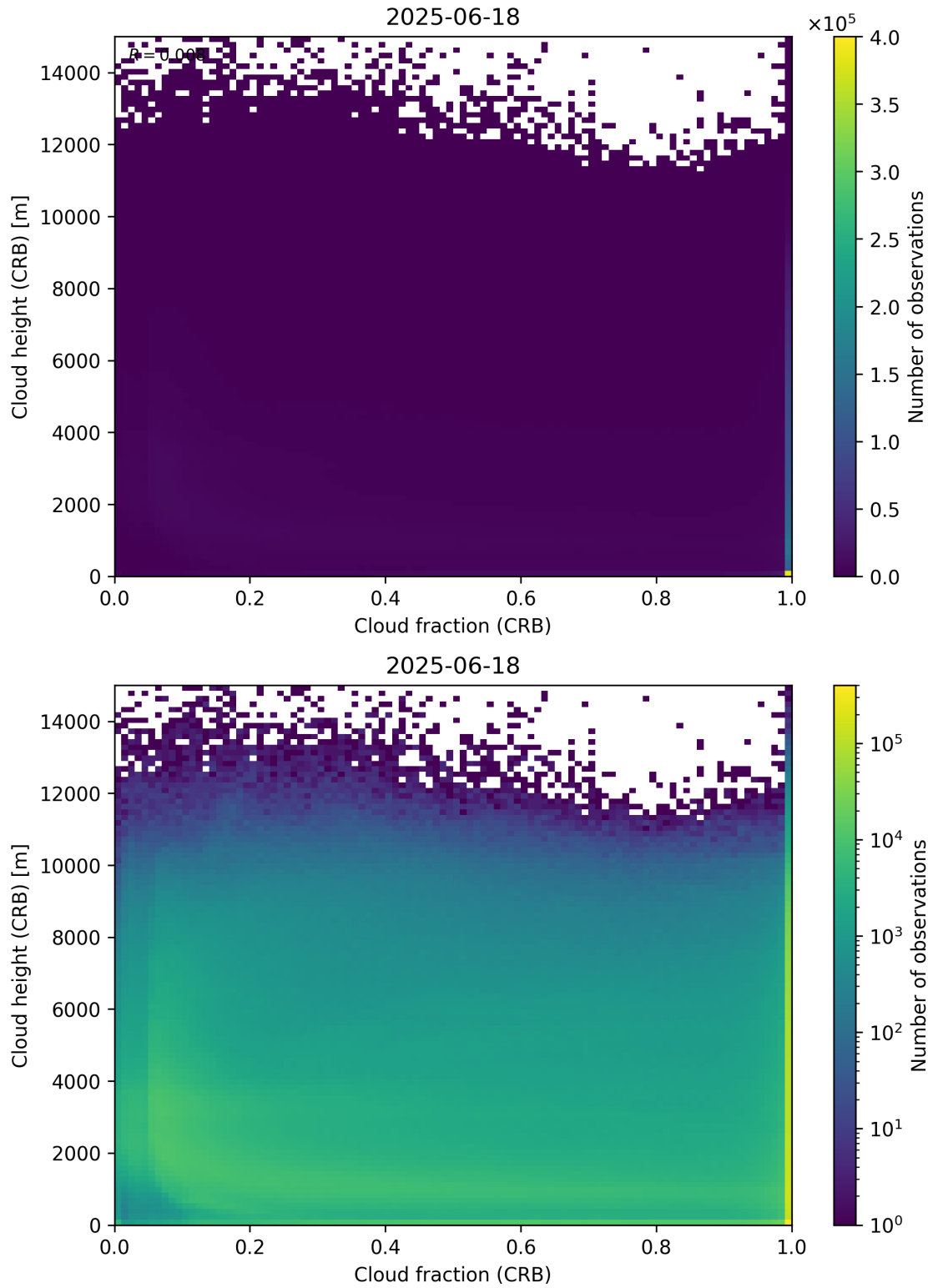
Figure 79: Scatter density plot of “Cloud fraction (CRB)” against “Cloud height (CRB)” for 2025-06-17 to 2025-06-19.
