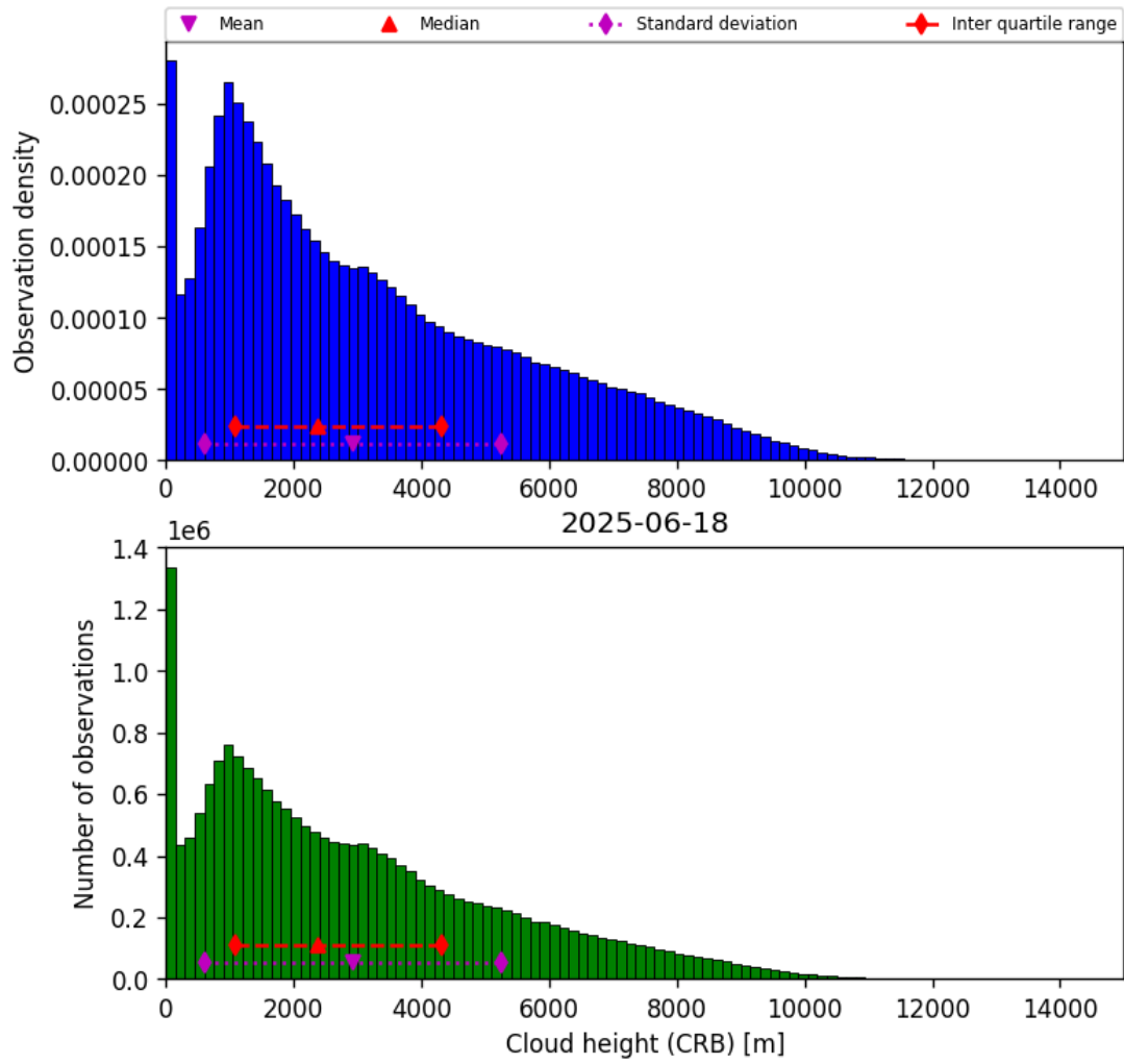
Figure 43: Histogram of “Cloud height (CRB)” for 2025-06-17 to 2025-06-19
