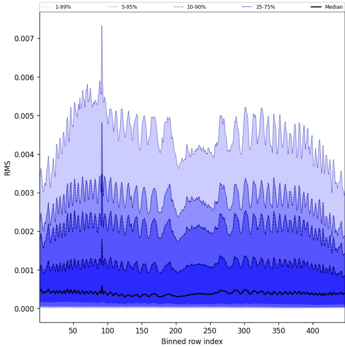
Figure 63: Along track statistics of “RMS” for 2025-06-17 to 2025-06-19
