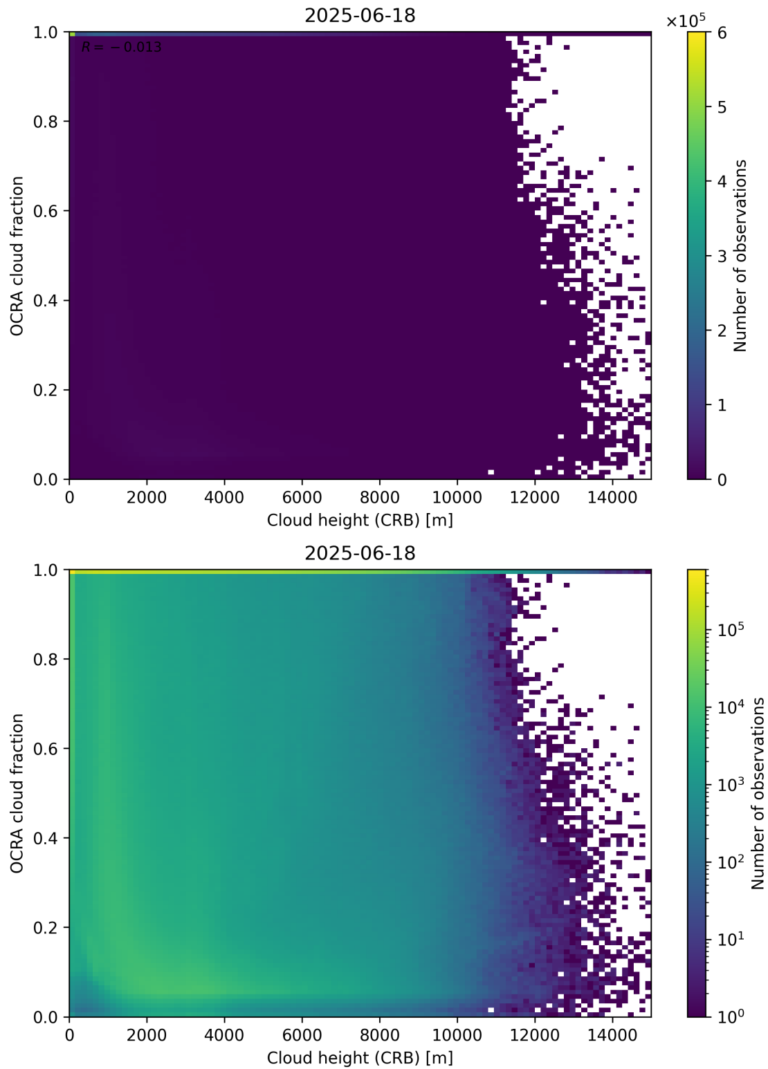
Figure 81: Scatter density plot of “Cloud height (CRB)” against “OCRA cloud fraction” for 2025-06-17 to 2025-06-19.
