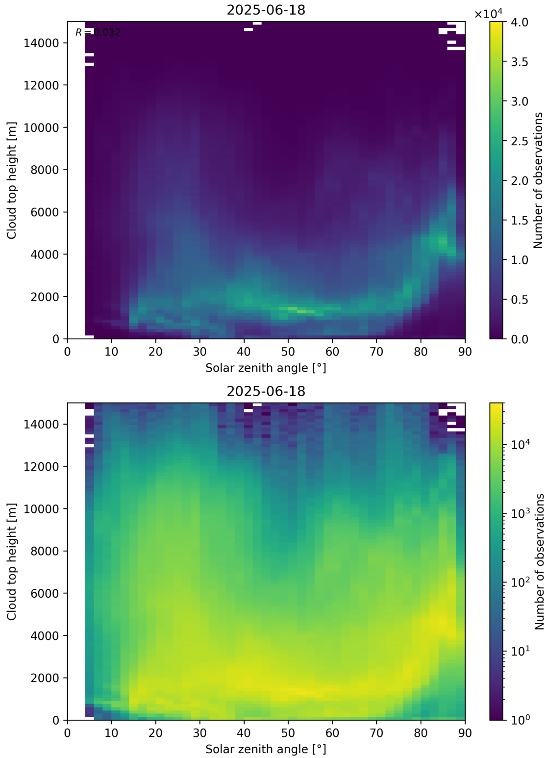
Figure 104: Scatter density plot of “Solar zenith angle” against “Cloud top height” for 2025-06-17 to 2025-06-19.
