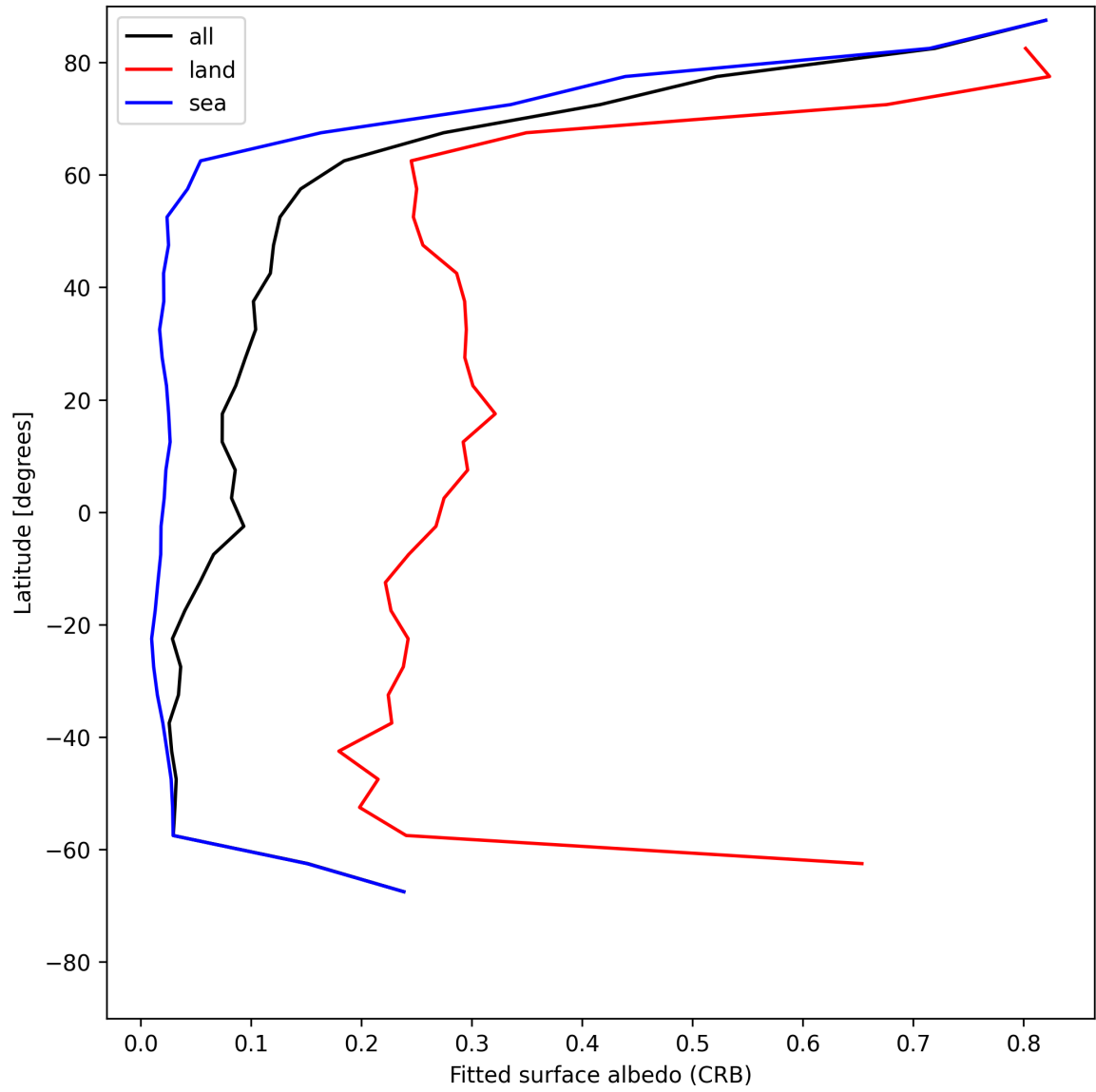
Figure 30: Zonal average of “Fitted surface albedo (CRB)” for 2025-06-17 to 2025-06-19.
