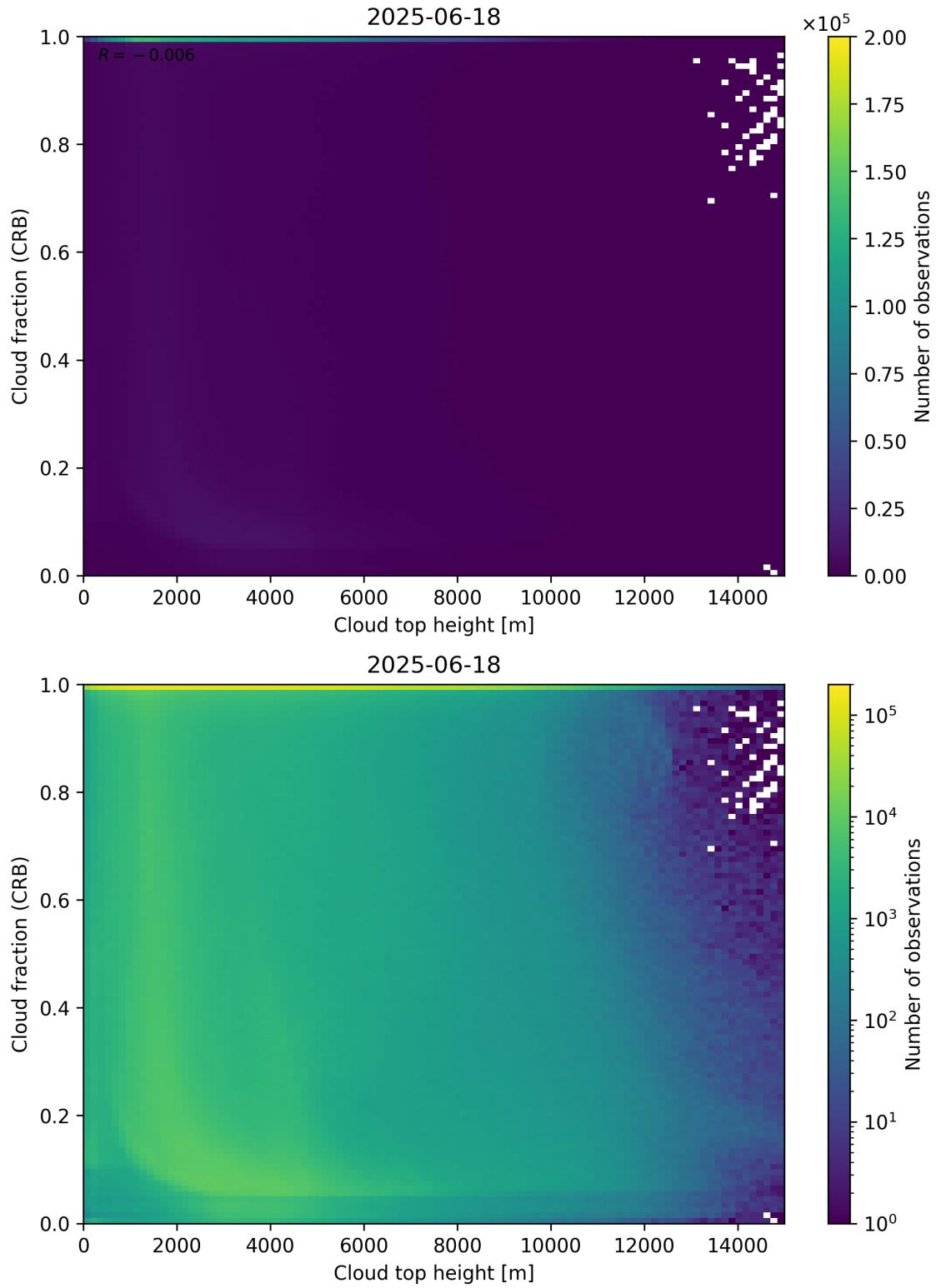
Figure 88: Scatter density plot of “Cloud top height” against “Cloud fraction (CRB)” for 2025-06-17 to 2025-06-19.
