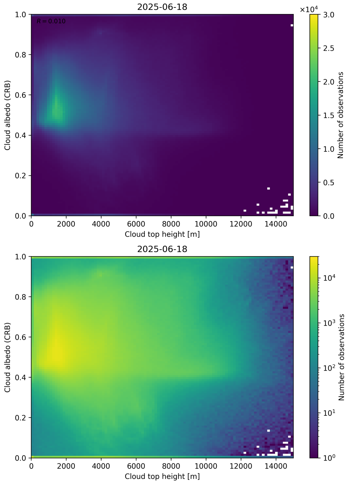
Figure 86: Scatter density plot of “Cloud top height” against “Cloud albedo (CRB)” for 2025-06-17 to 2025-06-19.
