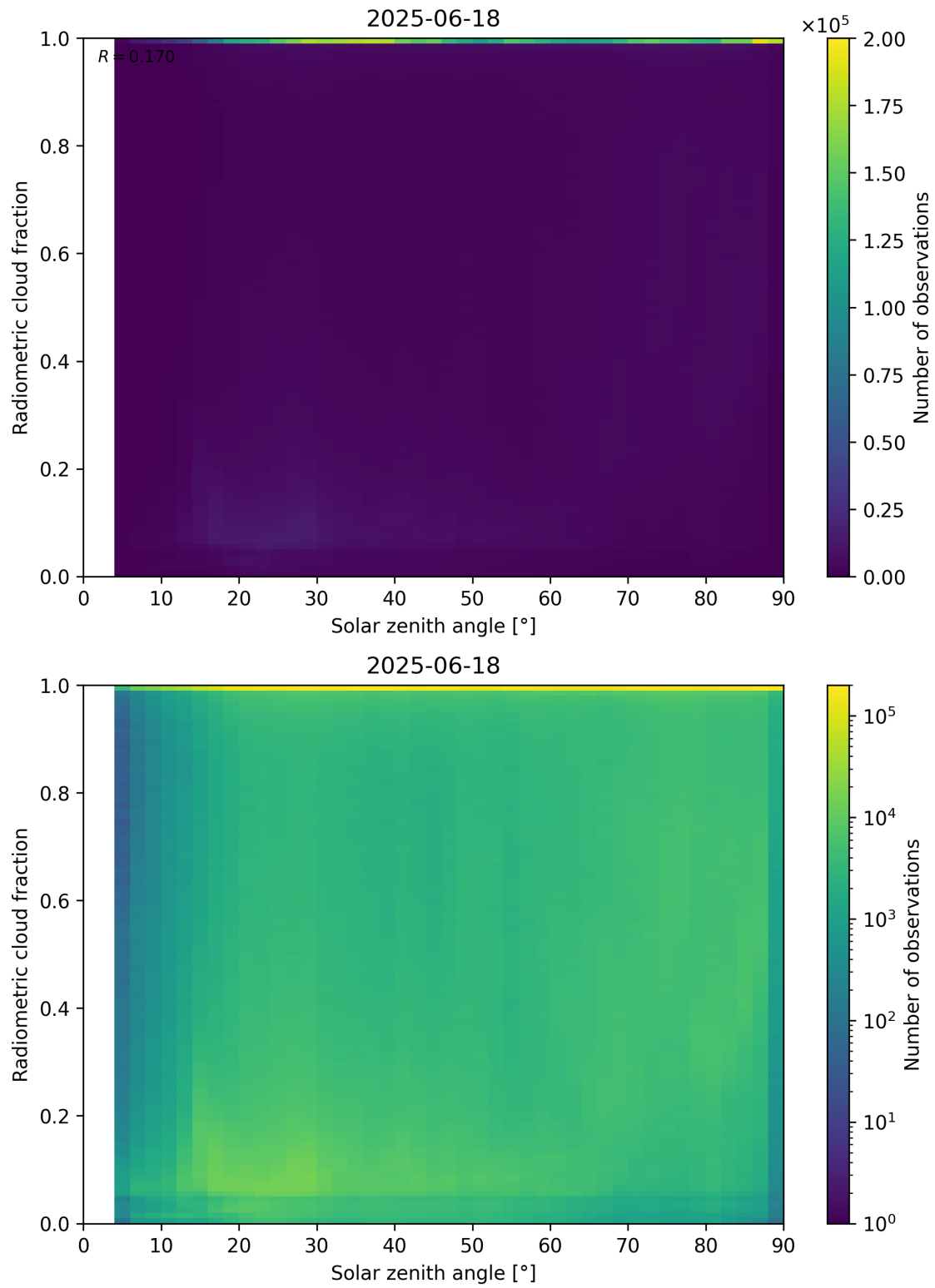
Figure 99: Scatter density plot of “Solar zenith angle” against “Radiometric cloud fraction” for 2025-06-17 to 2025-06-19.
