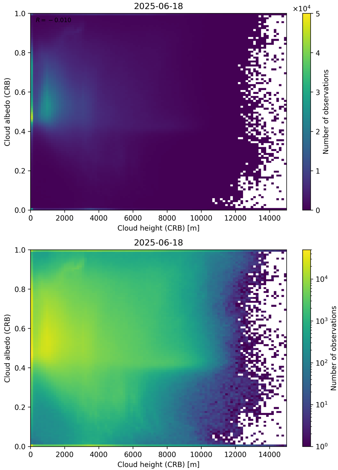
Figure 80: Scatter density plot of “Cloud height (CRB)” against “Cloud albedo (CRB)” for 2025-06-17 to 2025-06-19.
