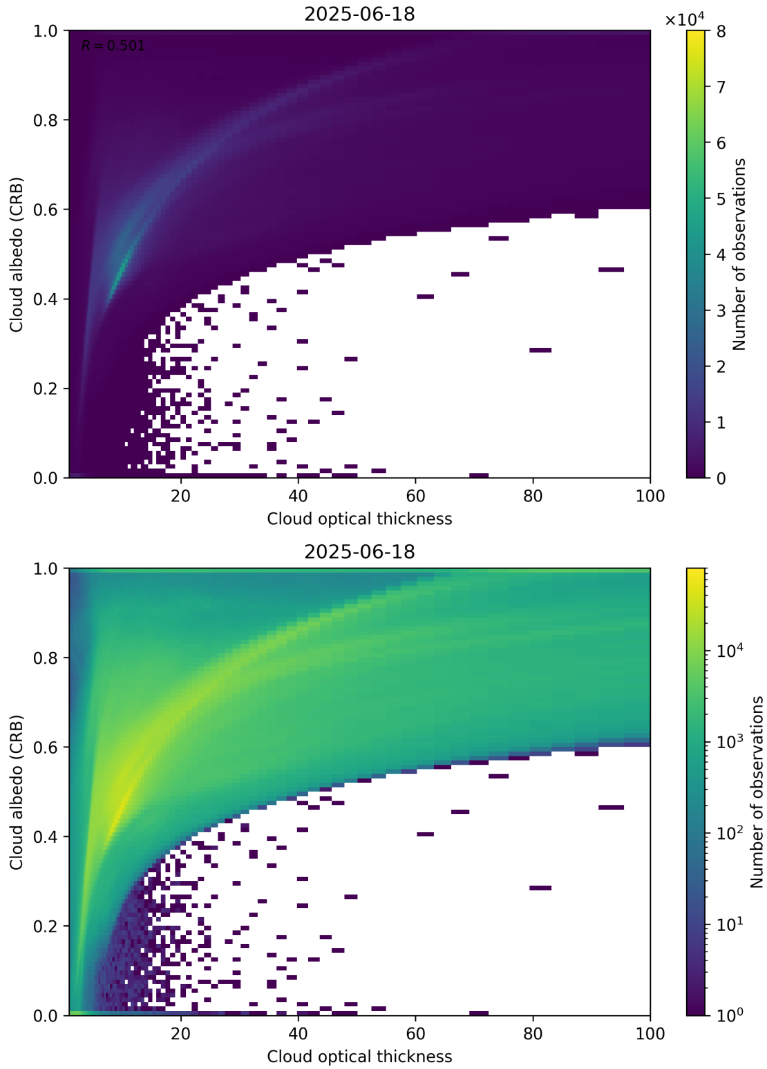
Figure 82: Scatter density plot of “Cloud optical thickness” against “Cloud albedo (CRB)” for 2025-06-17 to 2025-06-19.
