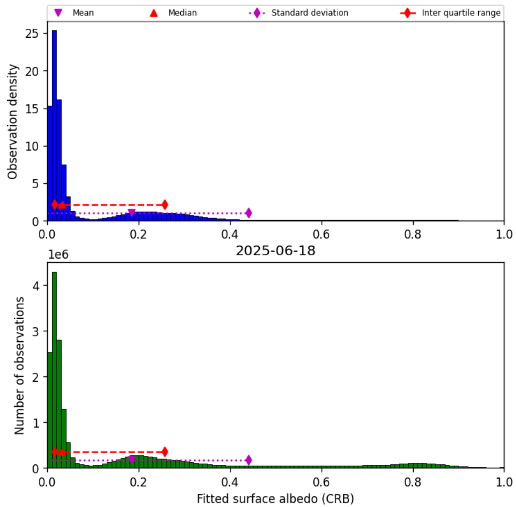
Figure 46: Histogram of “Fitted surface albedo (CRB)” for 2025-06-17 to 2025-06-19
