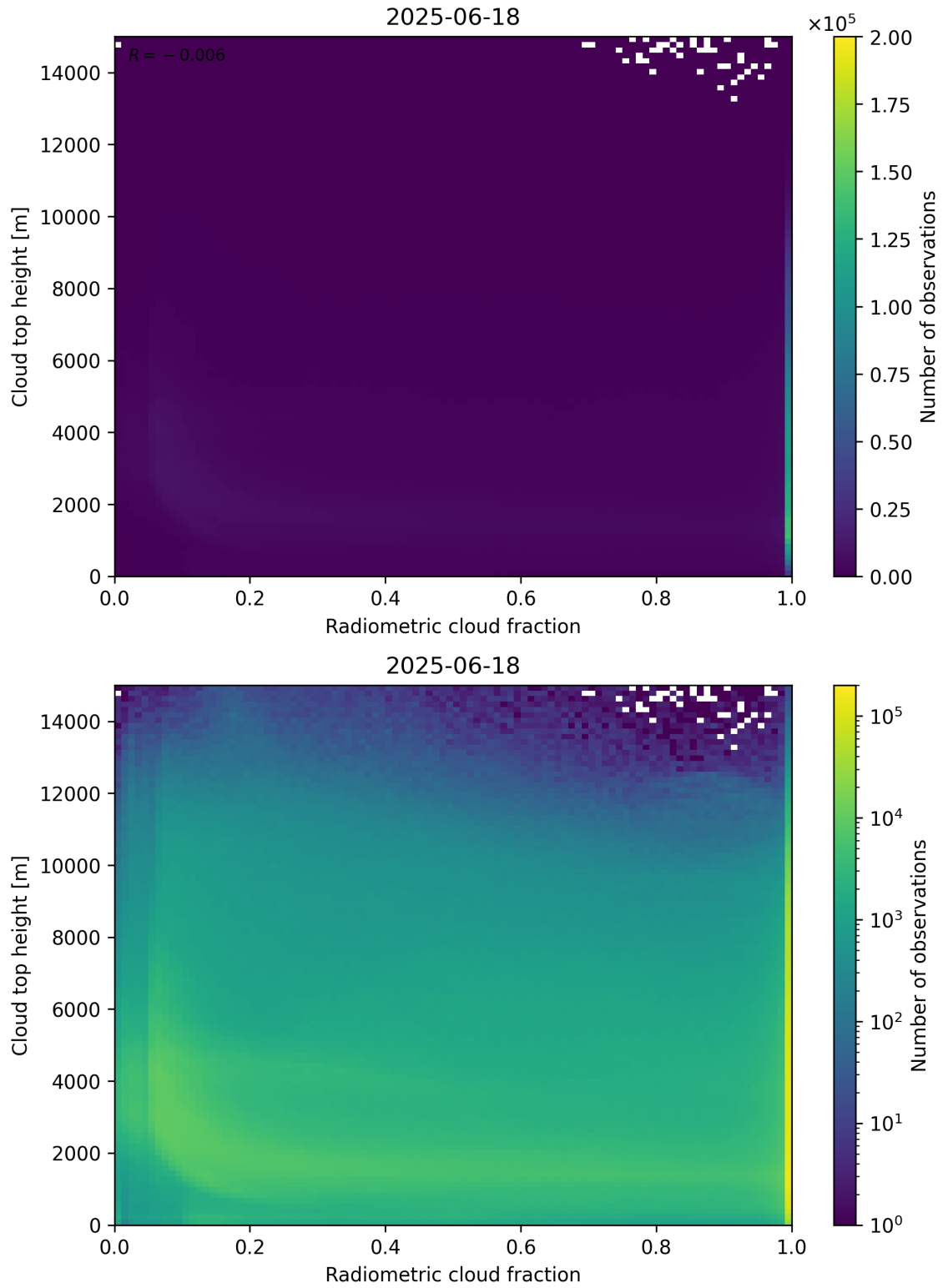
Figure 76: Scatter density plot of “Radiometric cloud fraction” against “Cloud top height” for 2025-06-17 to 2025-06-19.
