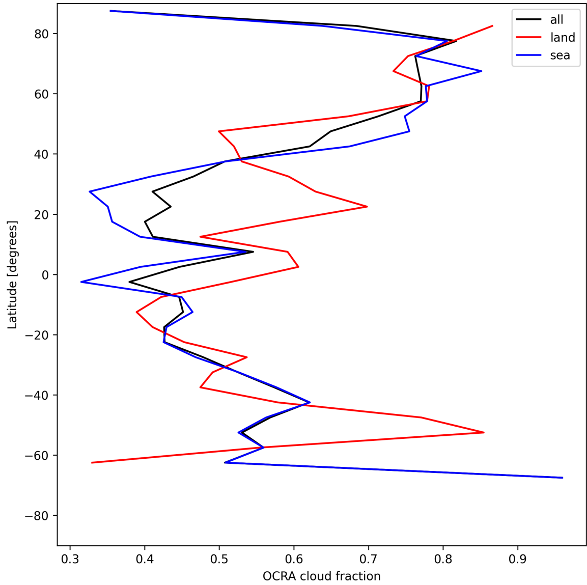
Figure 34: Zonal average of “OCRA cloud fraction” for 2025-06-17 to 2025-06-19.
