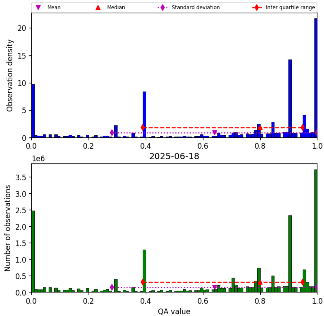
Figure 38: Histogram of “QA value” for 2025-06-17 to 2025-06-19
