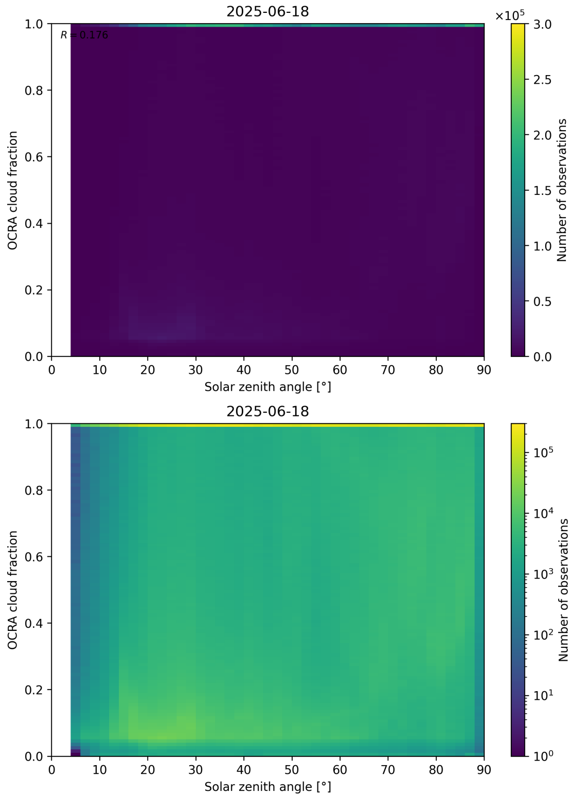
Figure 100: Scatter density plot of “Solar zenith angle” against “OCRA cloud fraction” for 2025-06-17 to 2025-06-19.
