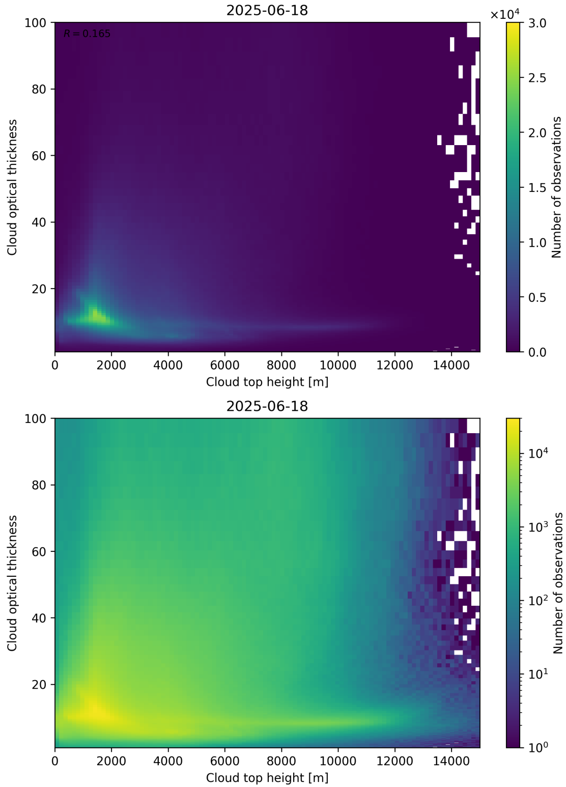
Figure 90: Scatter density plot of “Cloud top height” against “Cloud optical thickness” for 2025-06-17 to 2025-06-19.
