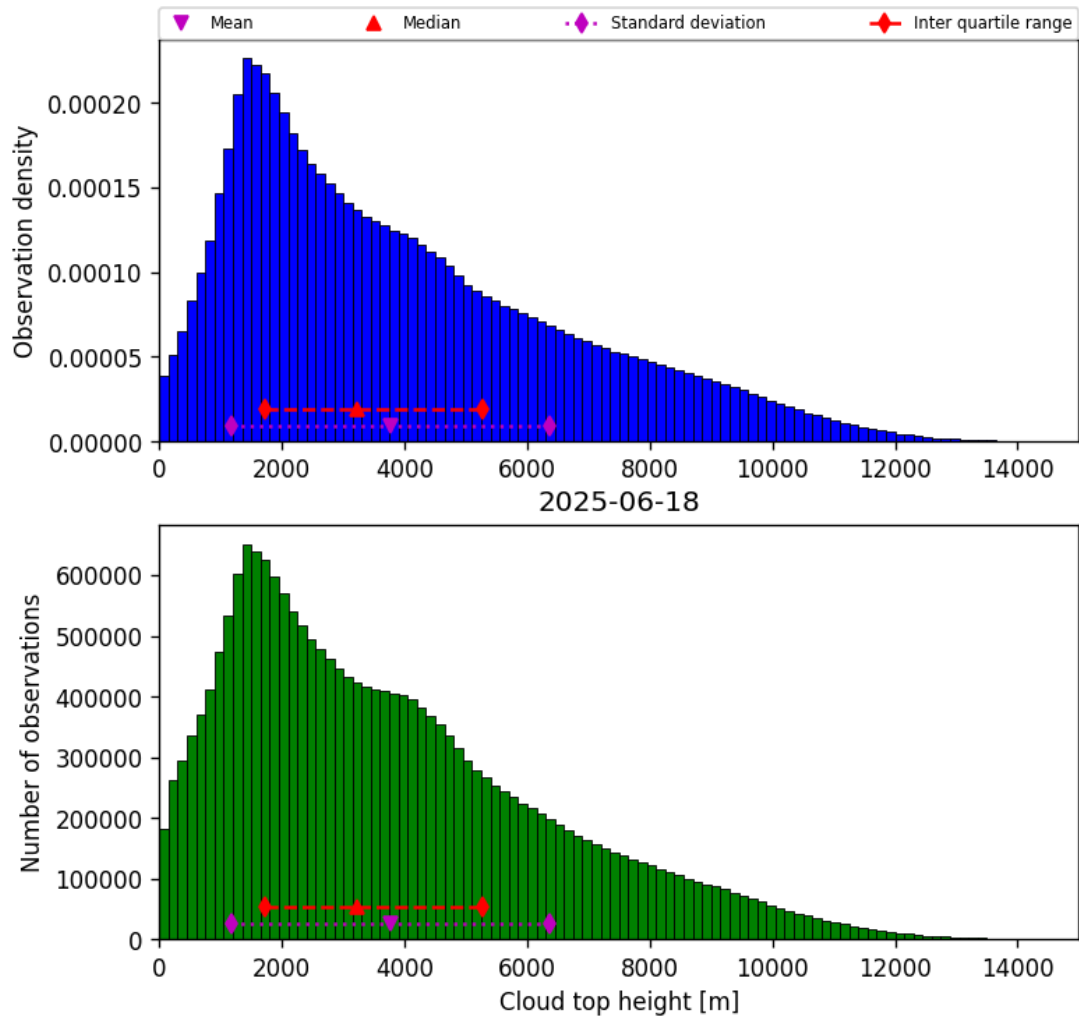
Figure 40: Histogram of “Cloud top height” for 2025-06-17 to 2025-06-19
