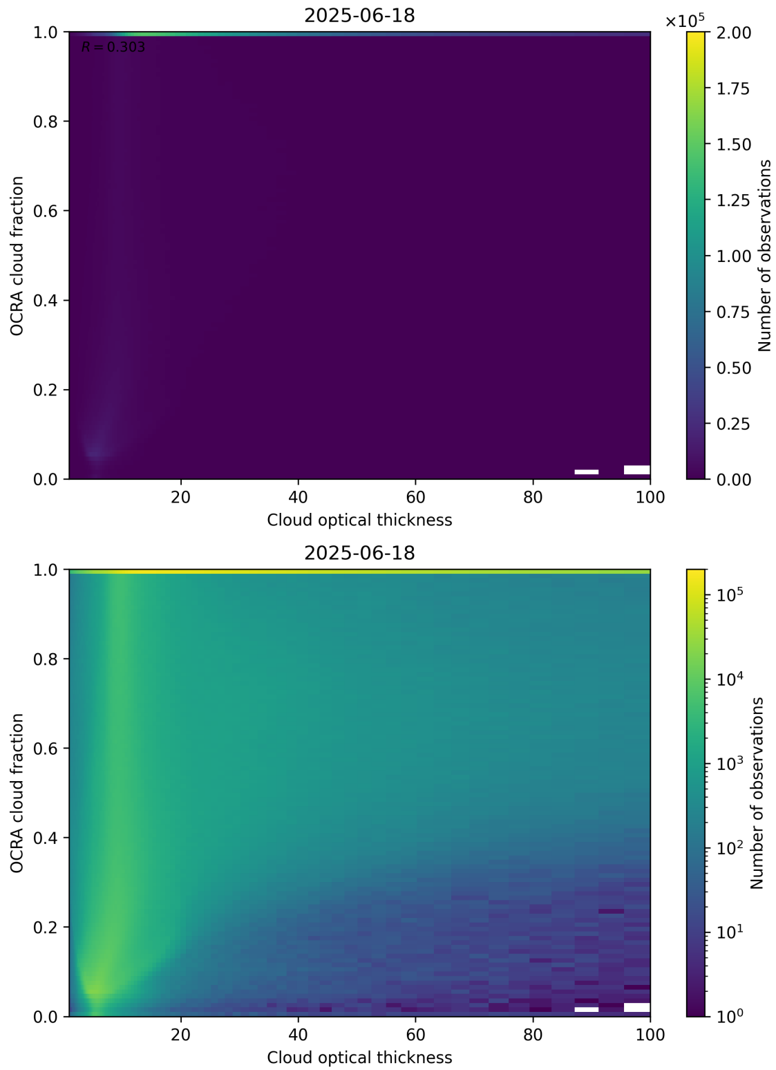
Figure 83: Scatter density plot of “Cloud optical thickness” against “OCRA cloud fraction” for 2025-06-17 to 2025-06-19.
