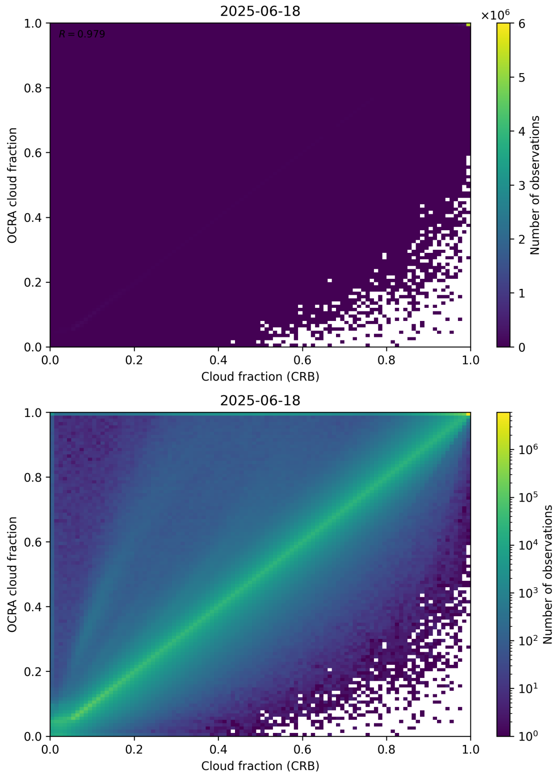
Figure 78: Scatter density plot of “Cloud fraction (CRB)” against “OCRA cloud fraction” for 2025-06-17 to 2025-06-19.
