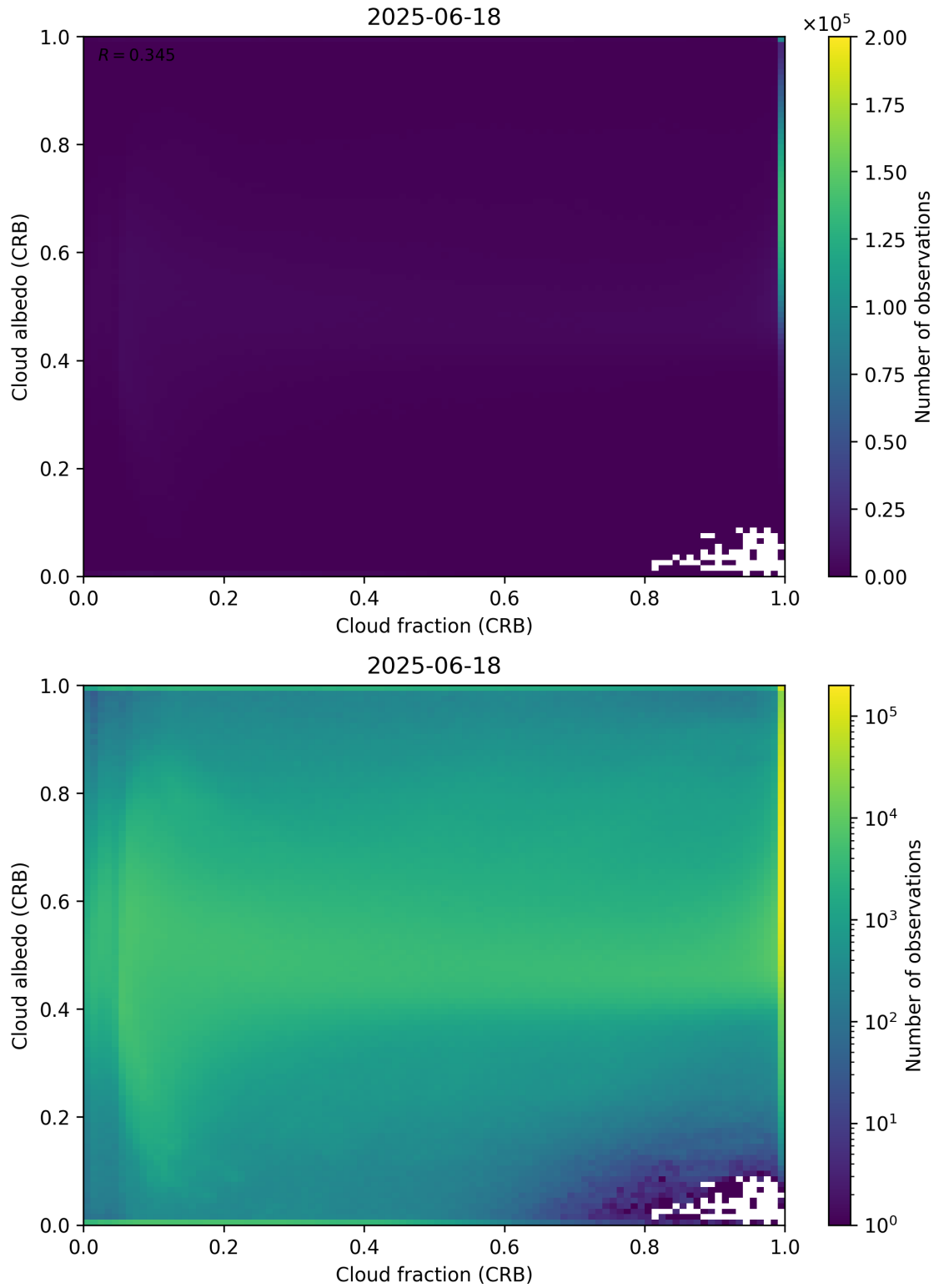
Figure 77: Scatter density plot of “Cloud fraction (CRB)” against “Cloud albedo (CRB)” for 2025-06-17 to 2025-06-19.
