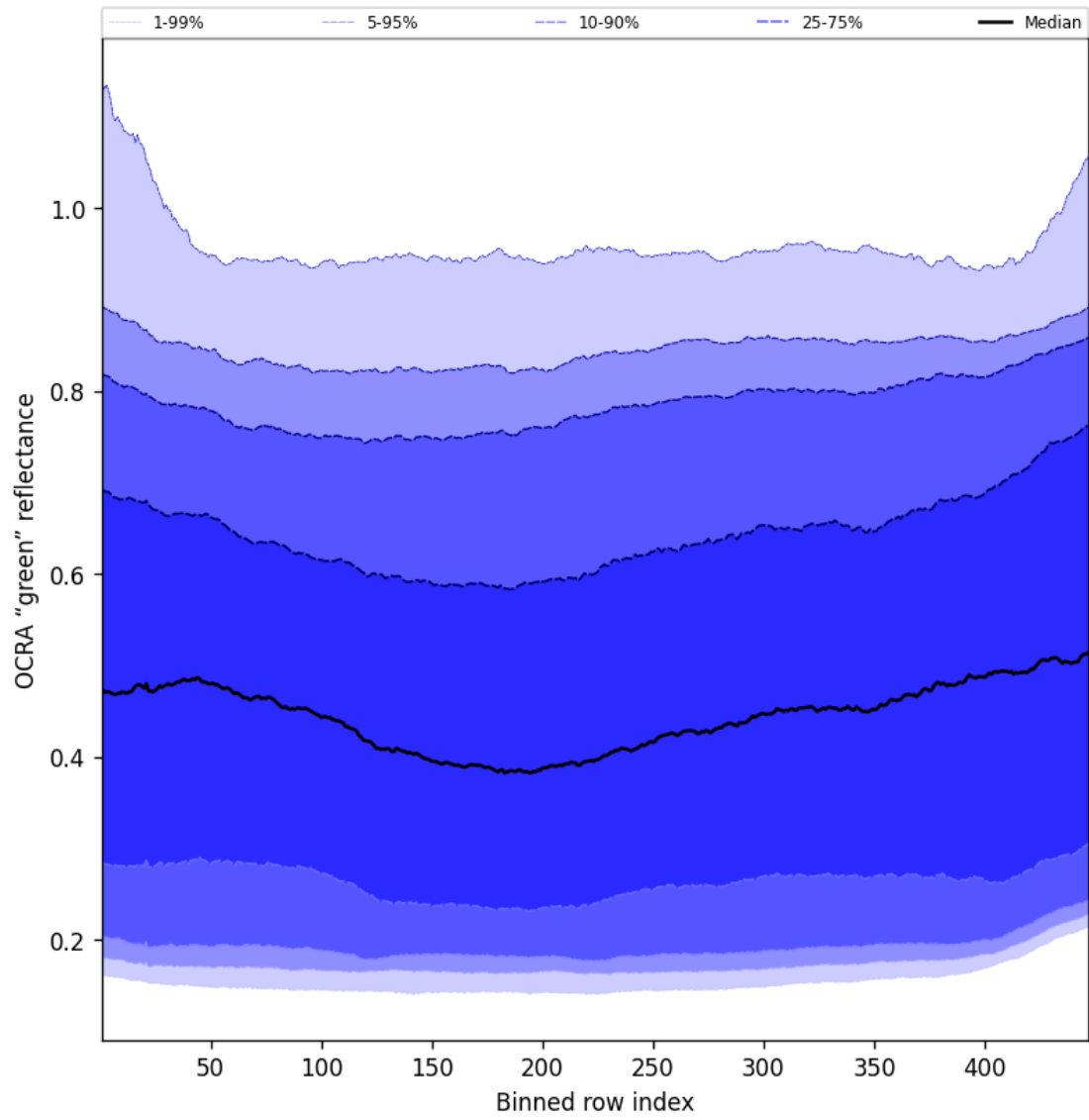
Figure 68: Along track statistics of “OCRA “green” reflectance” for 2025-06-17 to 2025-06-19
