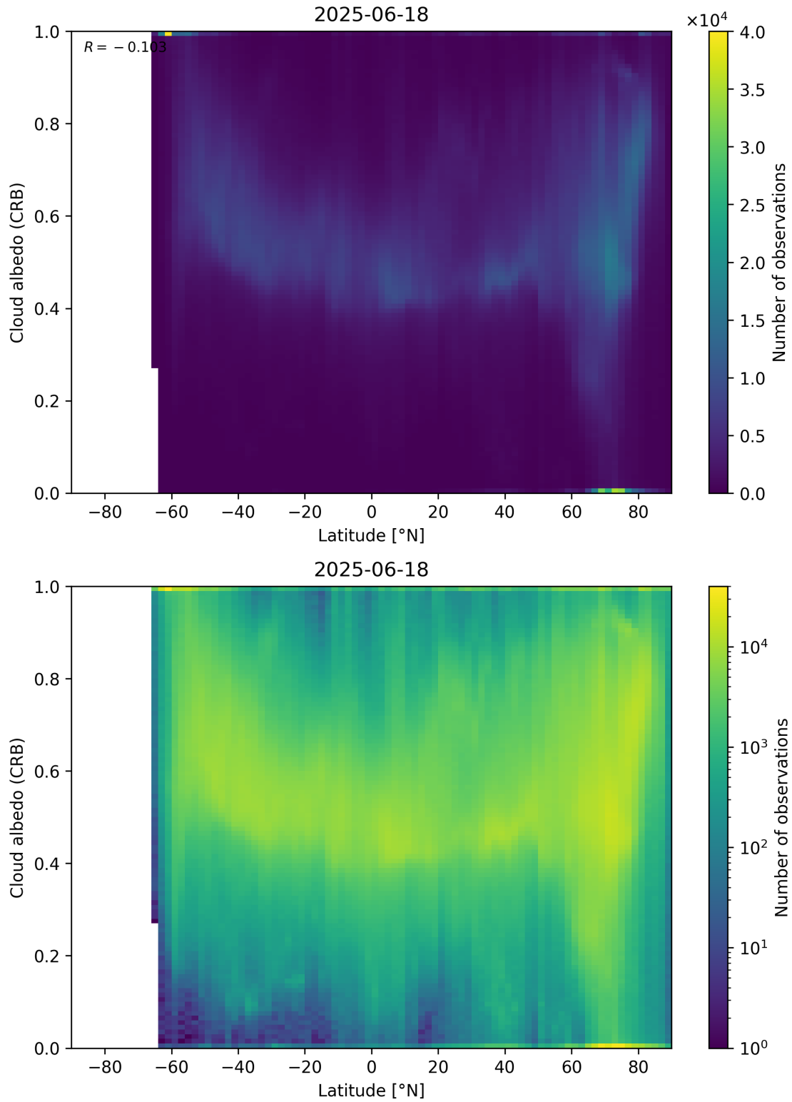
Figure 91: Scatter density plot of “Latitude” against “Cloud albedo (CRB)” for 2025-06-17 to 2025-06-19.
