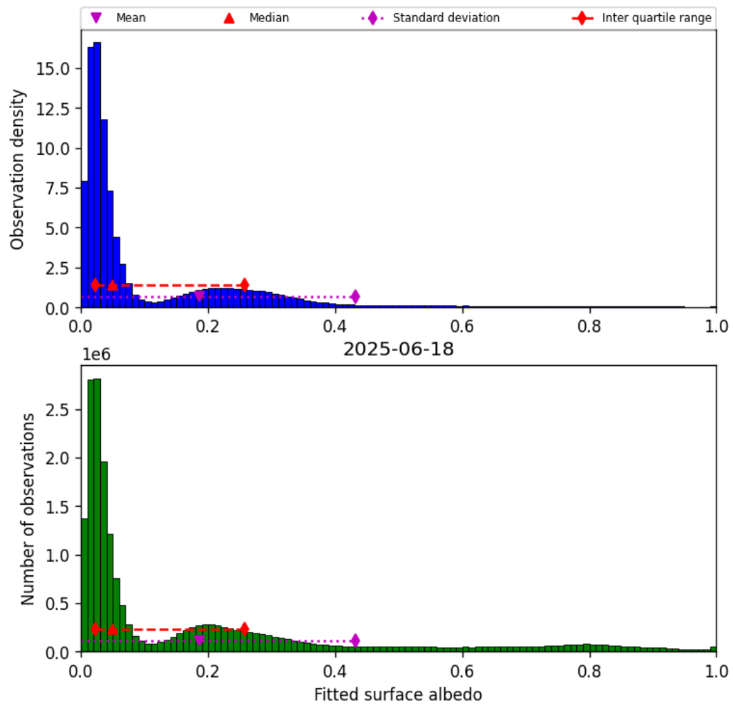
Figure 45: Histogram of “Fitted surface albedo” for 2025-06-17 to 2025-06-19
