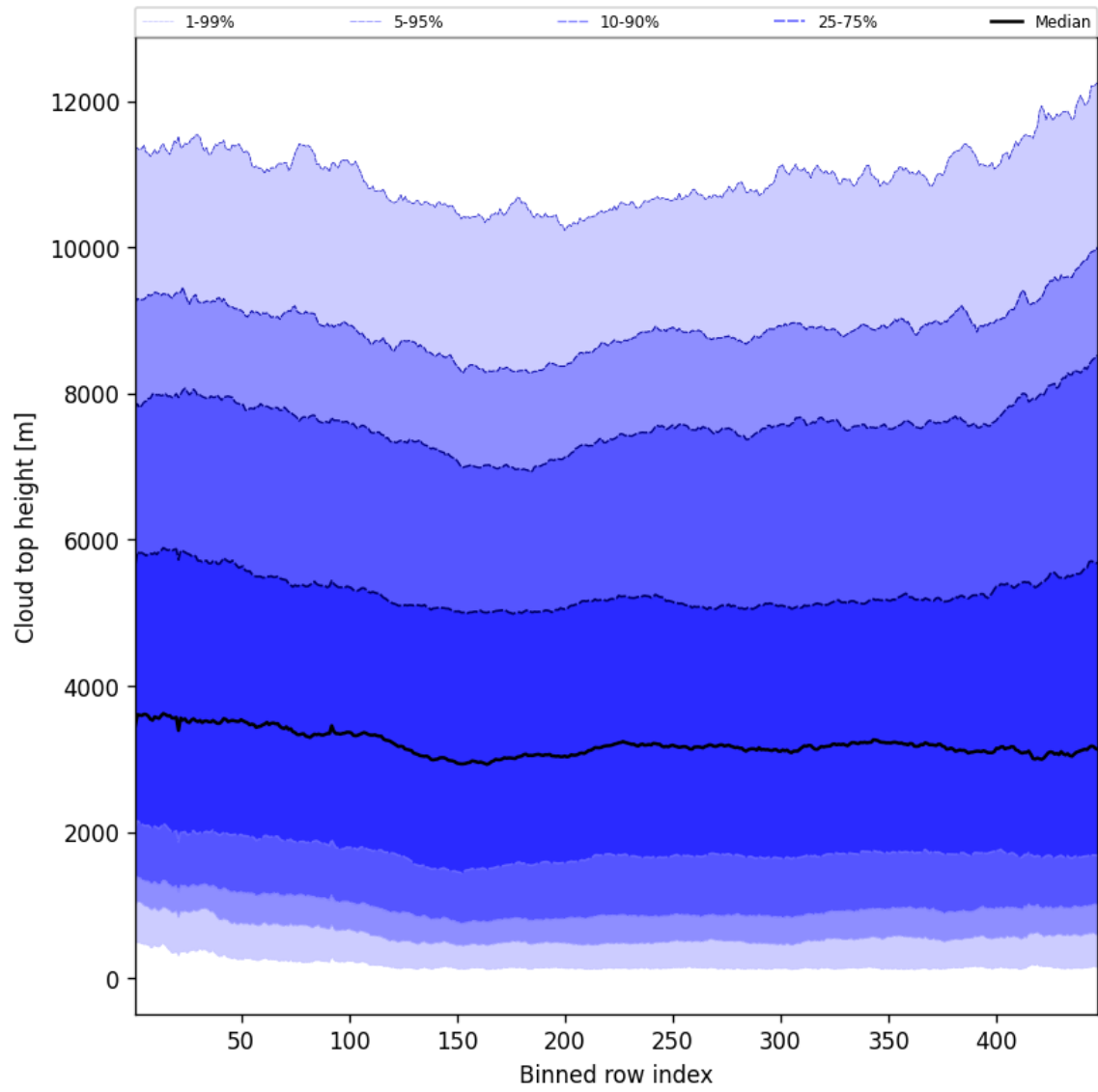
Figure 56: Along track statistics of “Cloud top height” for 2025-06-17 to 2025-06-19
