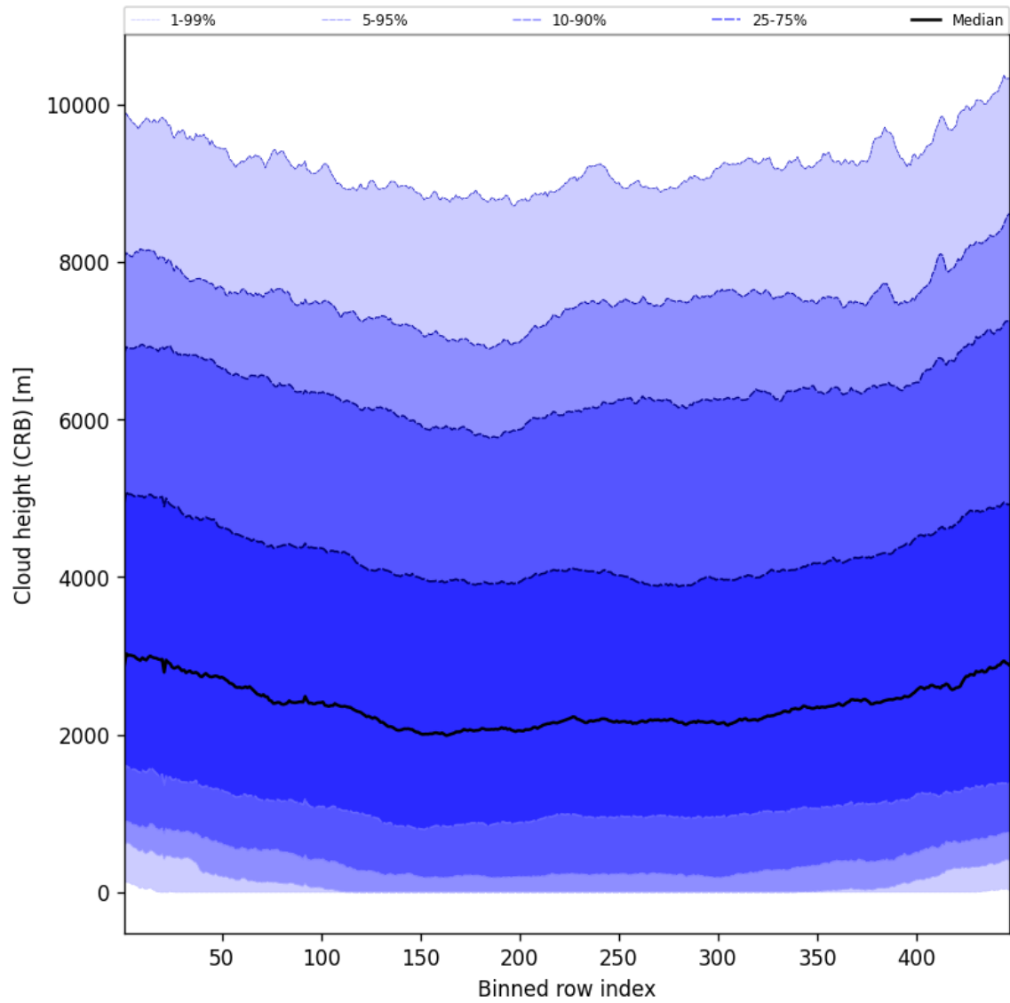
Figure 59: Along track statistics of “Cloud height (CRB)” for 2025-06-17 to 2025-06-19
