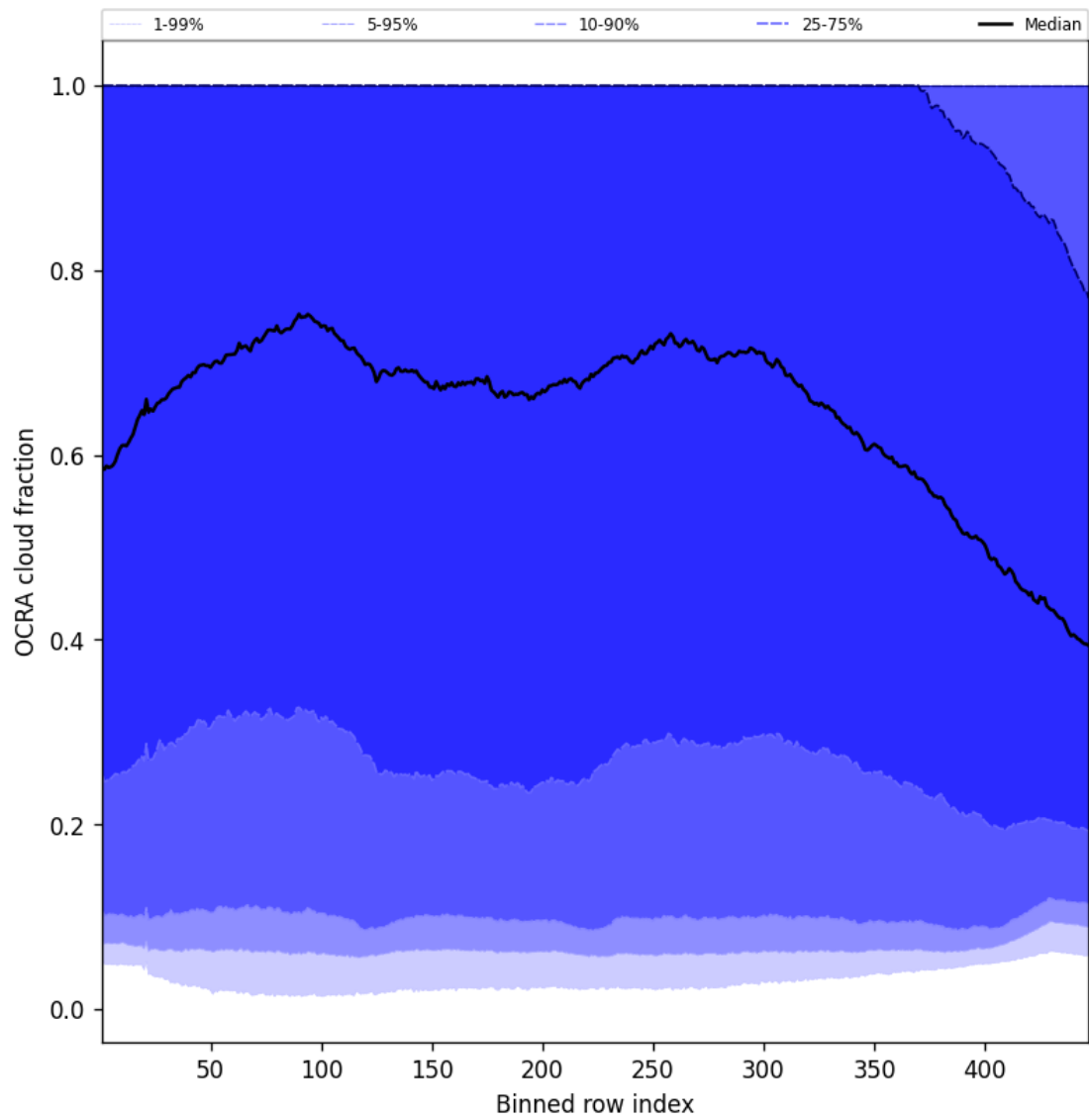
Figure 66: Along track statistics of “OCRA cloud fraction” for 2025-06-17 to 2025-06-19
