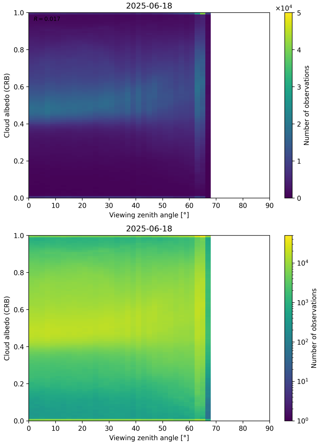
Figure 106: Scatter density plot of “Viewing zenith angle” against “Cloud albedo (CRB)” for 2025-06-17 to 2025-06-19.
