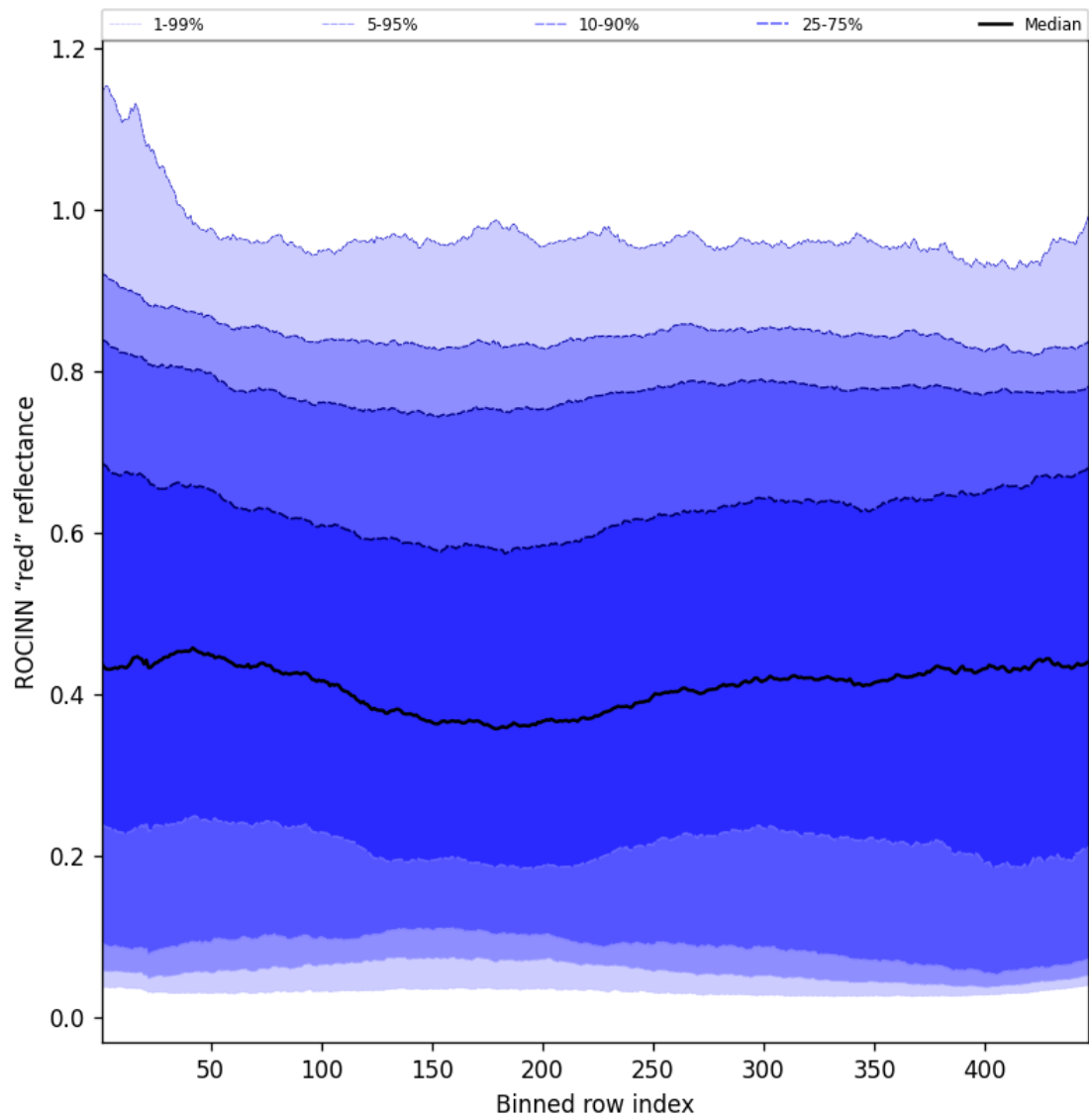
Figure 69: Along track statistics of "ROCINN "red" reflectance" for 2025-06-17 to 2025-06-19
