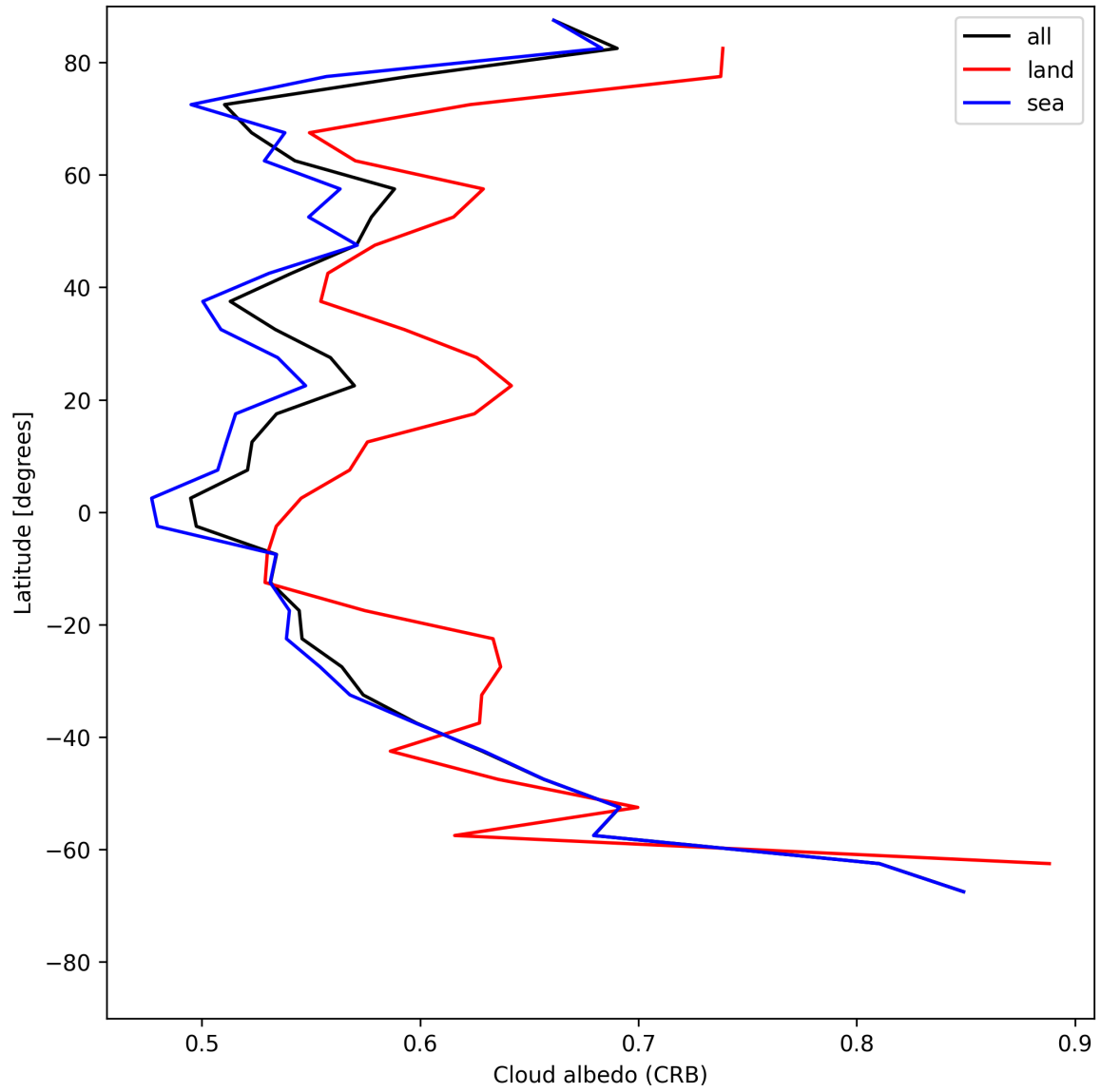
Figure 28: Zonal average of “Cloud albedo (CRB)” for 2025-06-17 to 2025-06-19.
