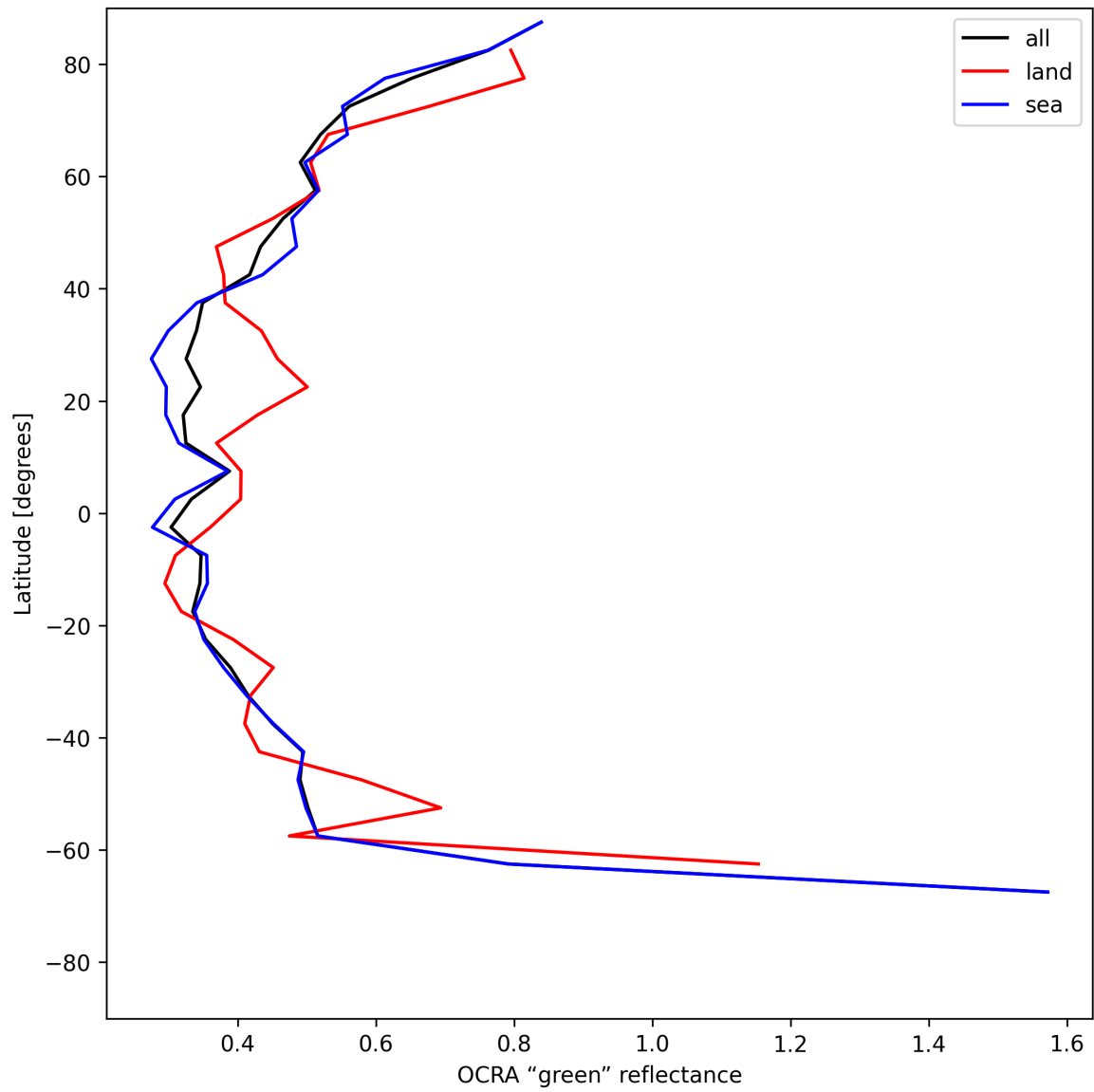
Figure 36: Zonal average of “OCRA “green” reflectance” for 2025-06-17 to 2025-06-19.
