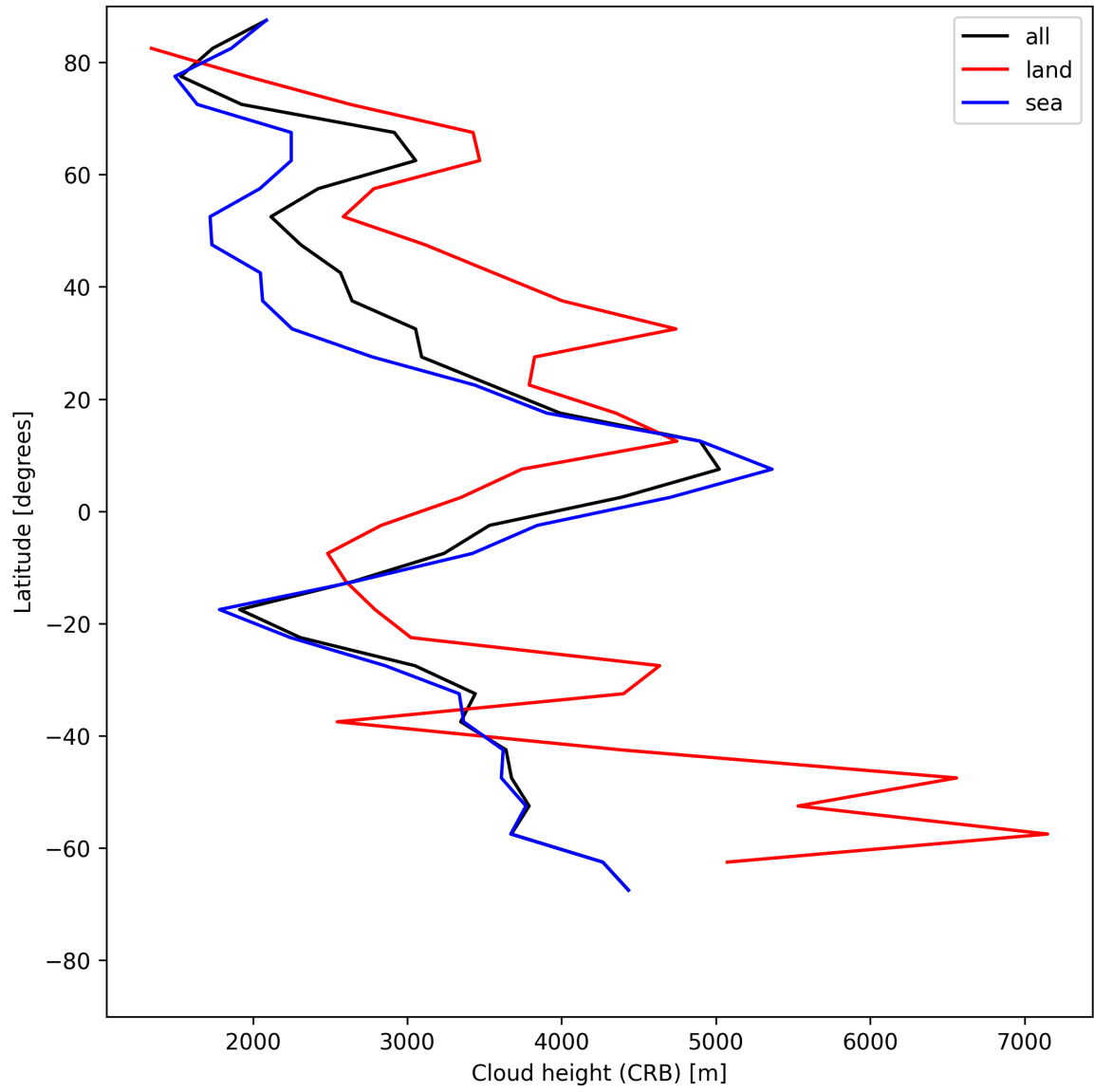
Figure 27: Zonal average of “Cloud height (CRB)” for 2025-06-17 to 2025-06-19.
