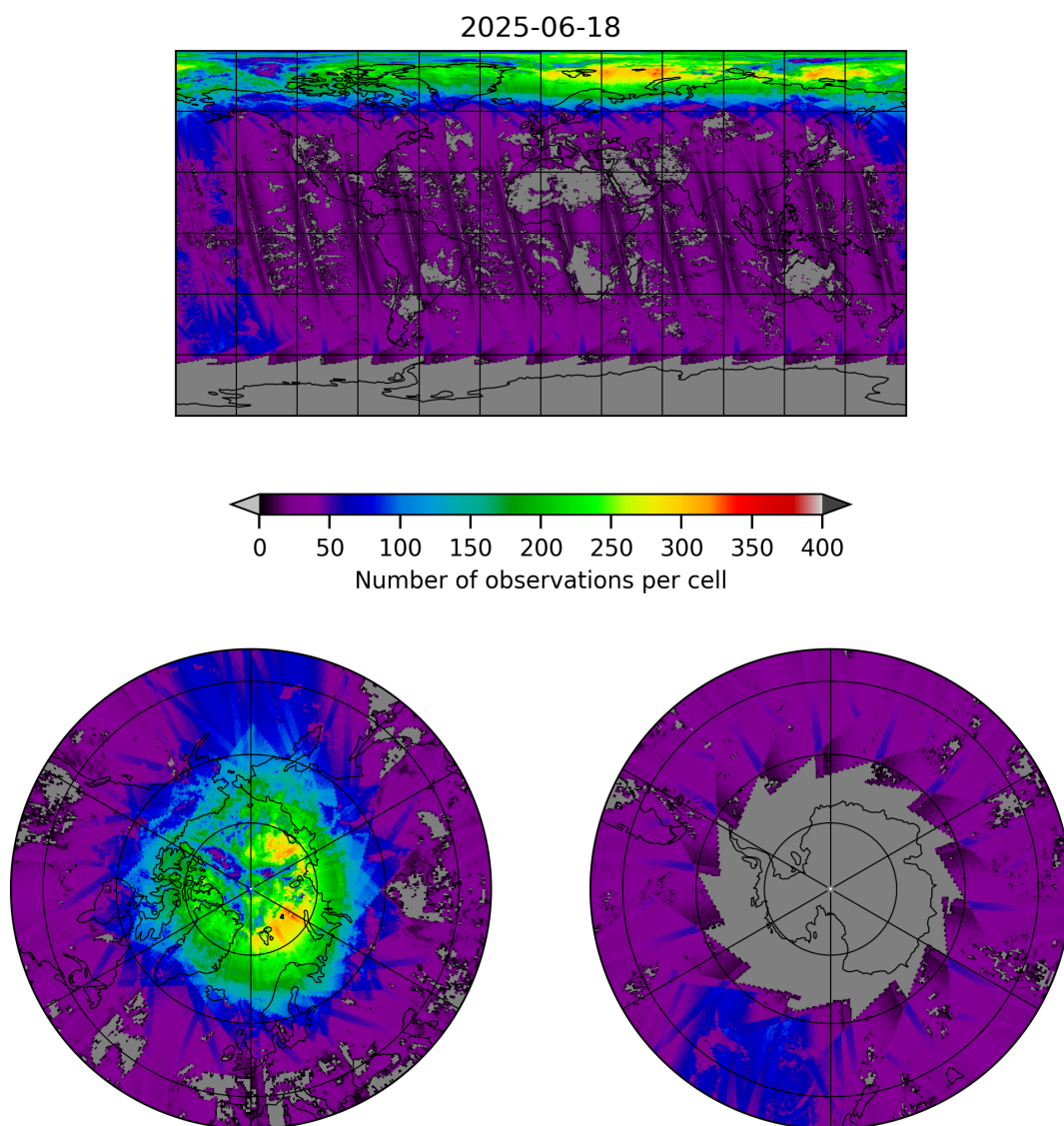
Figure 21: Map of the number of observations for 2025-06-17 to 2025-06-19
