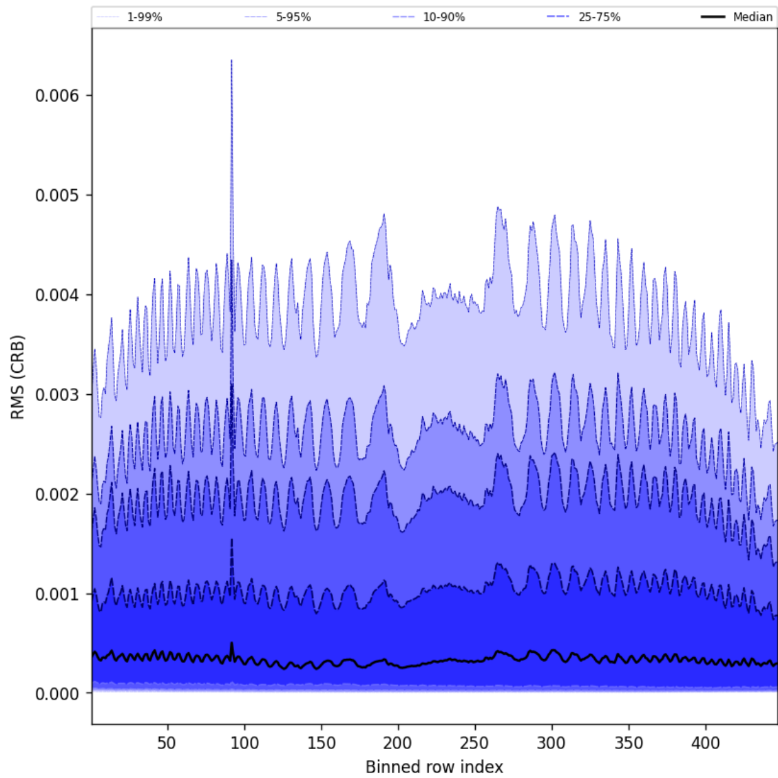
Figure 64: Along track statistics of “RMS (CRB)” for 2025-06-17 to 2025-06-19
