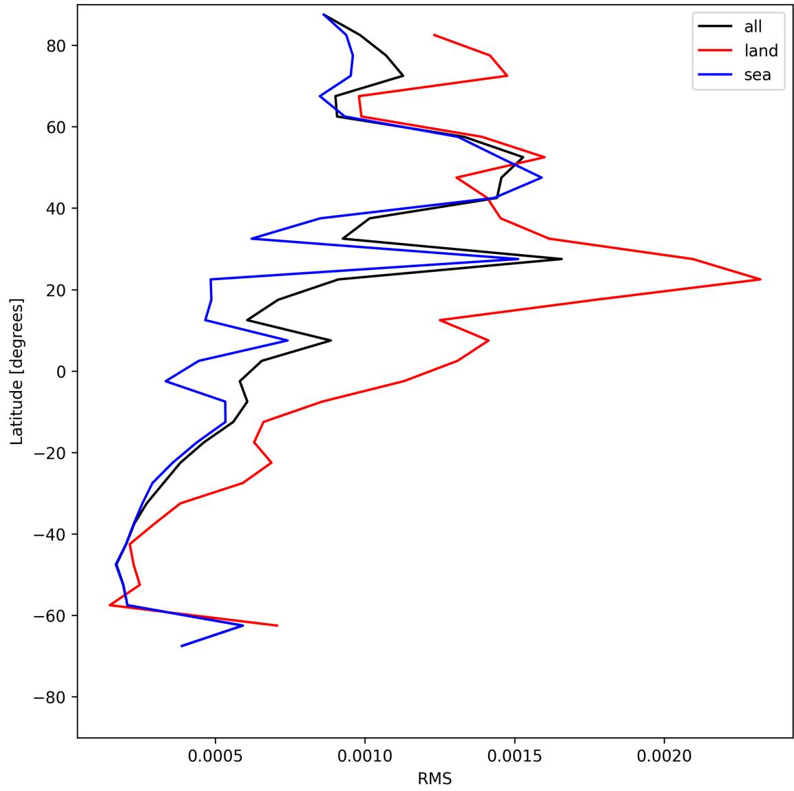
Figure 31: Zonal average of “RMS” for 2025-06-17 to 2025-06-19.
