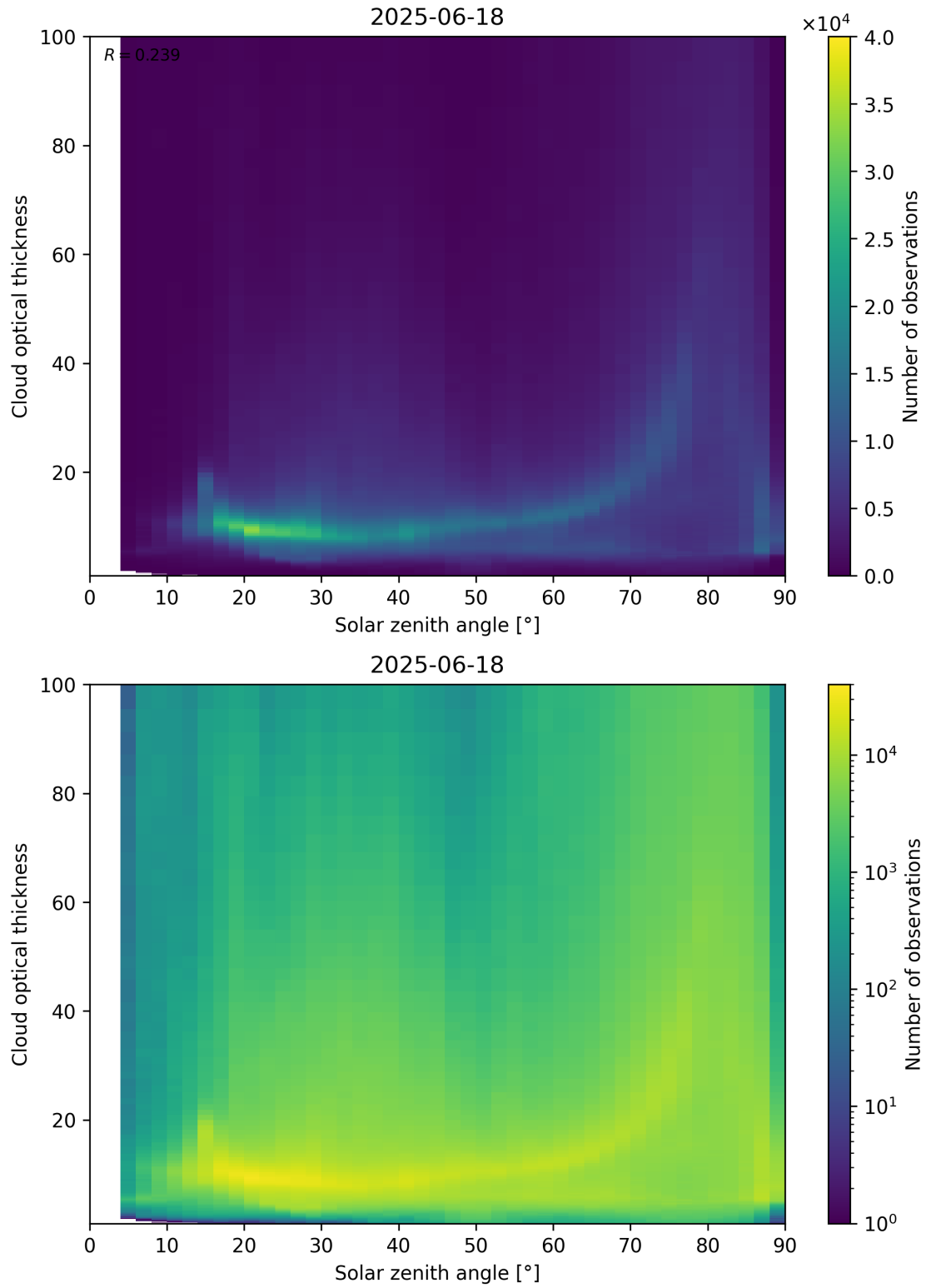
Figure 103: Scatter density plot of “Solar zenith angle” against “Cloud optical thickness” for 2025-06-17 to 2025-06-19.
