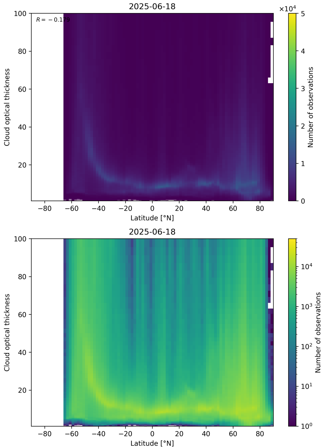
Figure 96: Scatter density plot of “Latitude” against “Cloud optical thickness” for 2025-06-17 to 2025-06-19.
