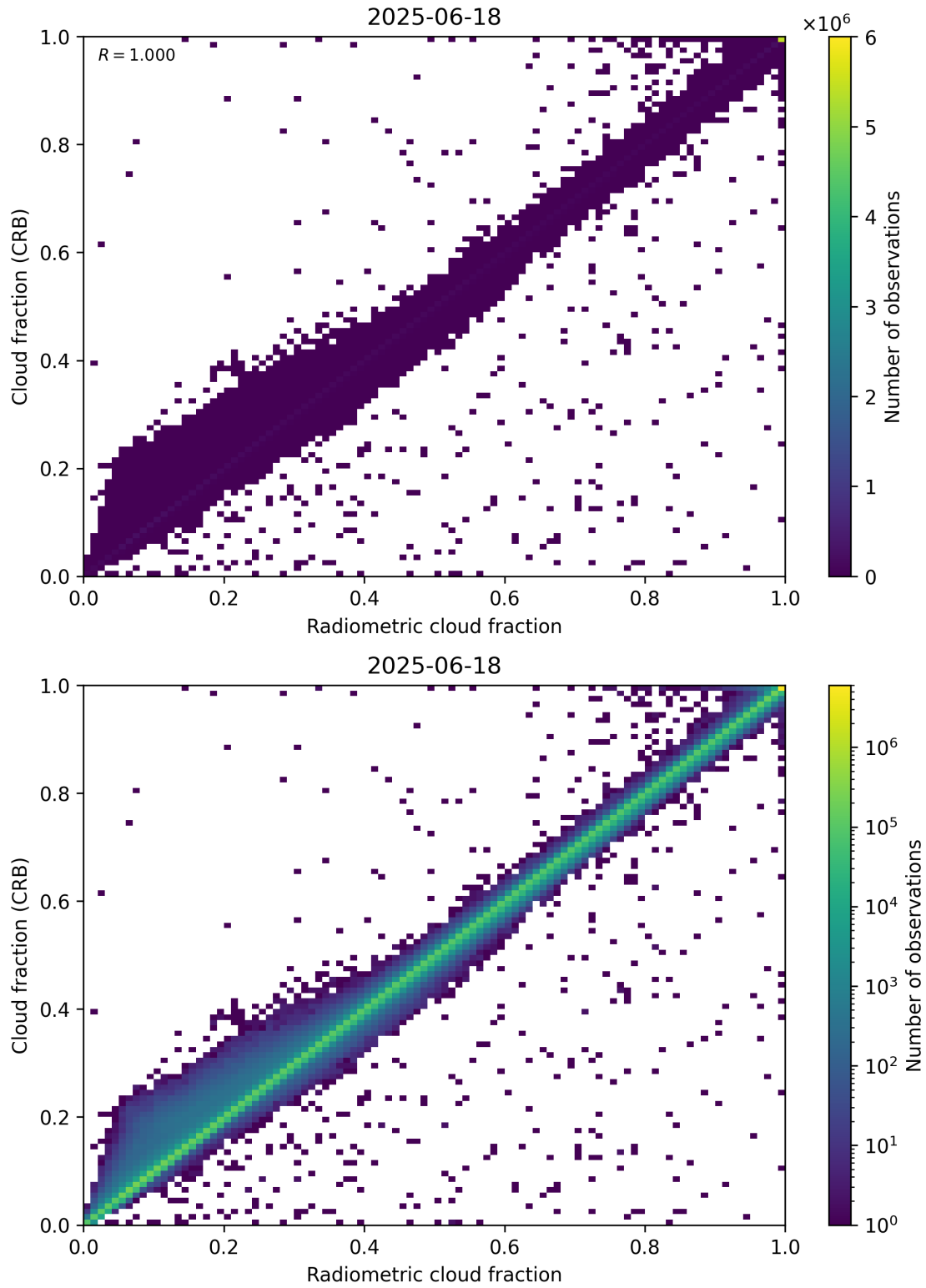
Figure 73: Scatter density plot of “Radiometric cloud fraction” against “Cloud fraction (CRB)” for 2025-06-17 to 2025-06-19.
