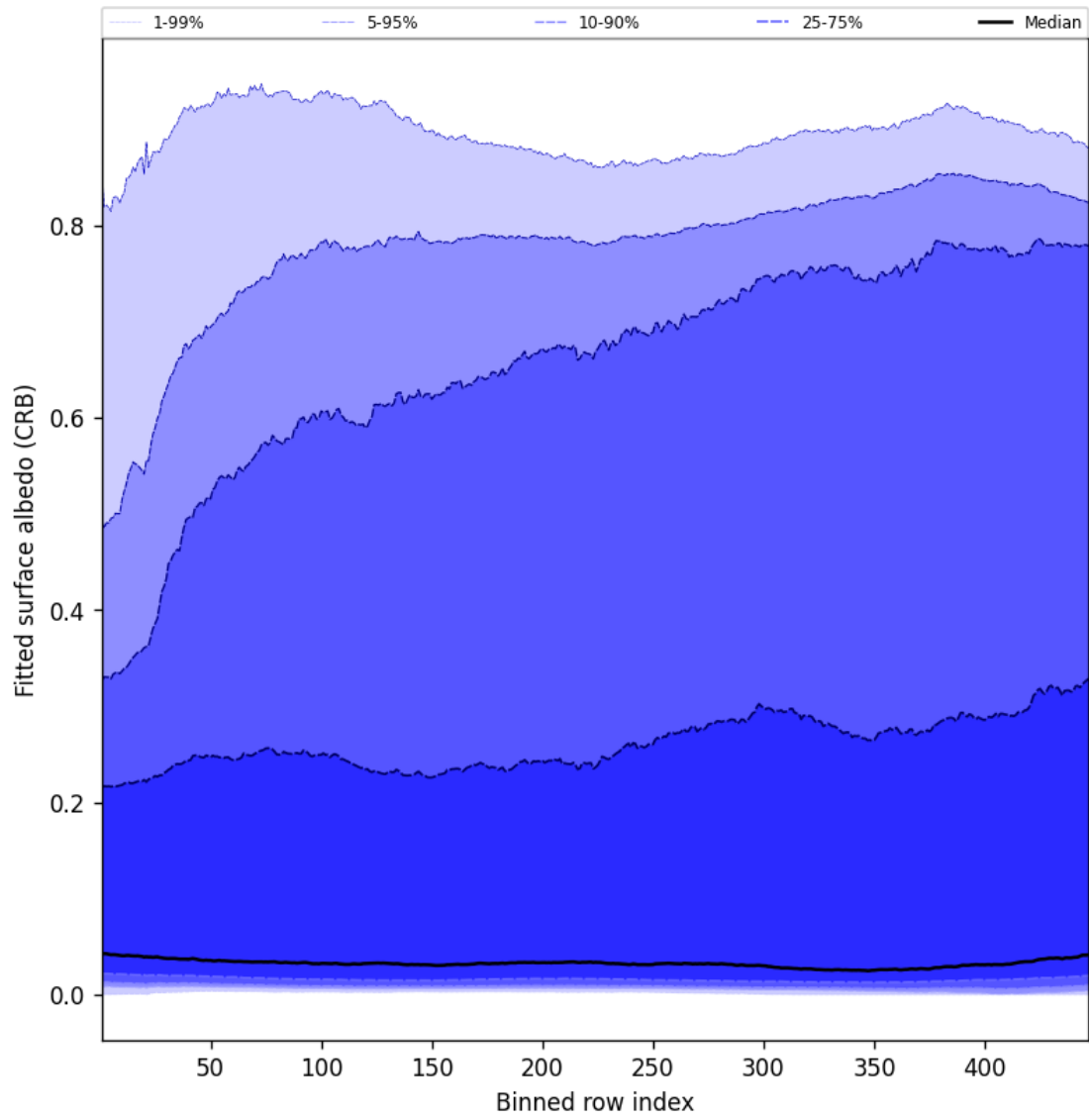
Figure 62: Along track statistics of “Fitted surface albedo (CRB)” for 2025-06-17 to 2025-06-19
