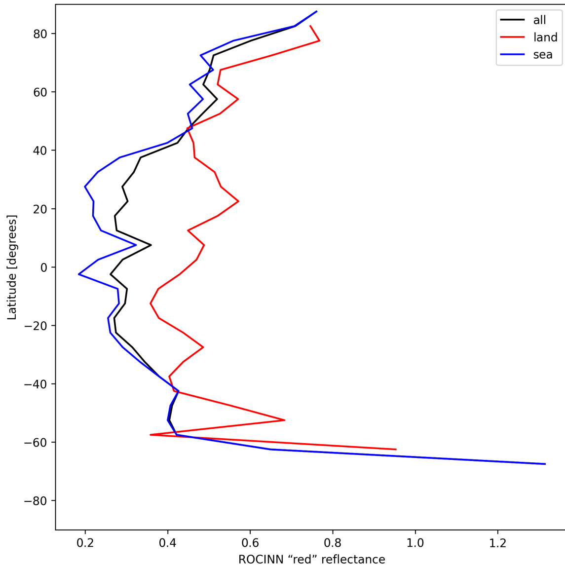
Figure 37: Zonal average of “ROCINN “red” reflectance” for 2025-06-17 to 2025-06-19.
