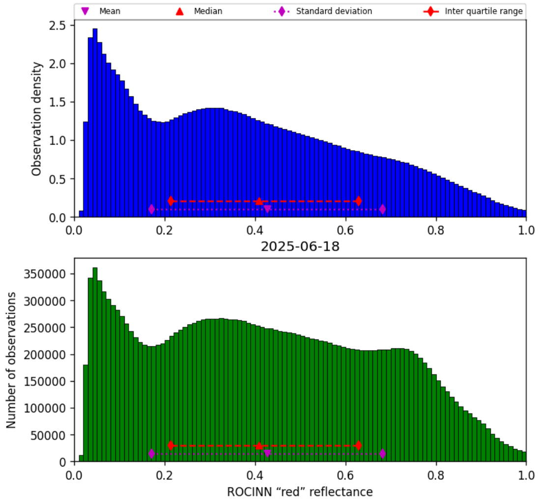
Figure 53: Histogram of “ROCINN “red” reflectance” for 2025-06-17 to 2025-06-19
