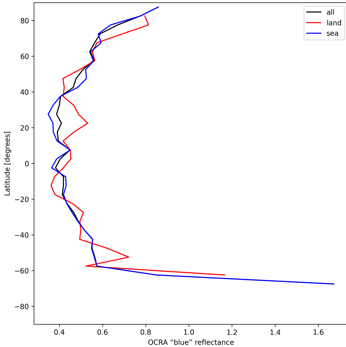
Figure 35: Zonal average of “OCRA “blue” reflectance” for 2025-06-17 to 2025-06-19.
