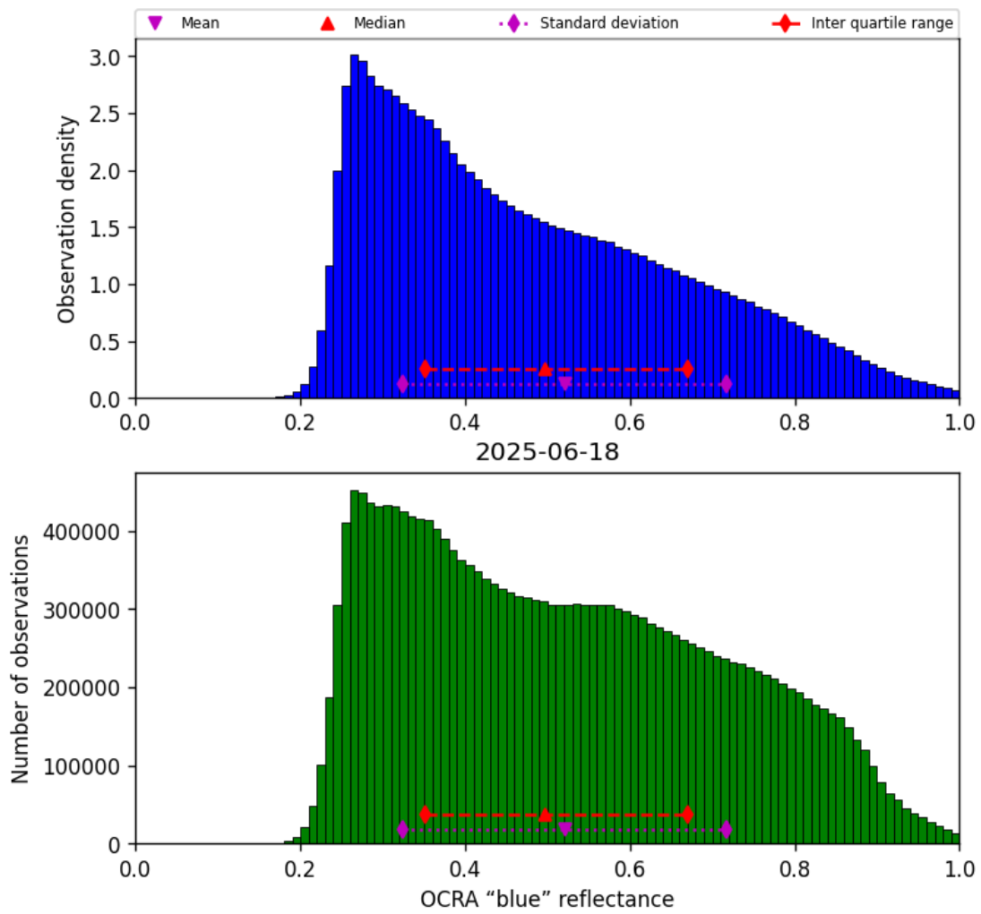
Figure 51: Histogram of “OCRA “blue” reflectance” for 2025-06-17 to 2025-06-19
