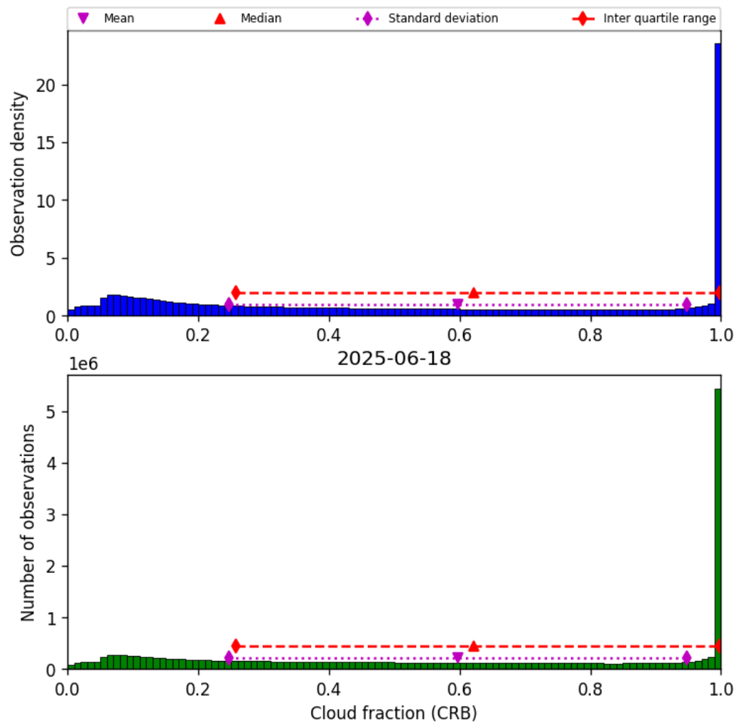
Figure 42: Histogram of “Cloud fraction (CRB)” for 2025-06-17 to 2025-06-19
