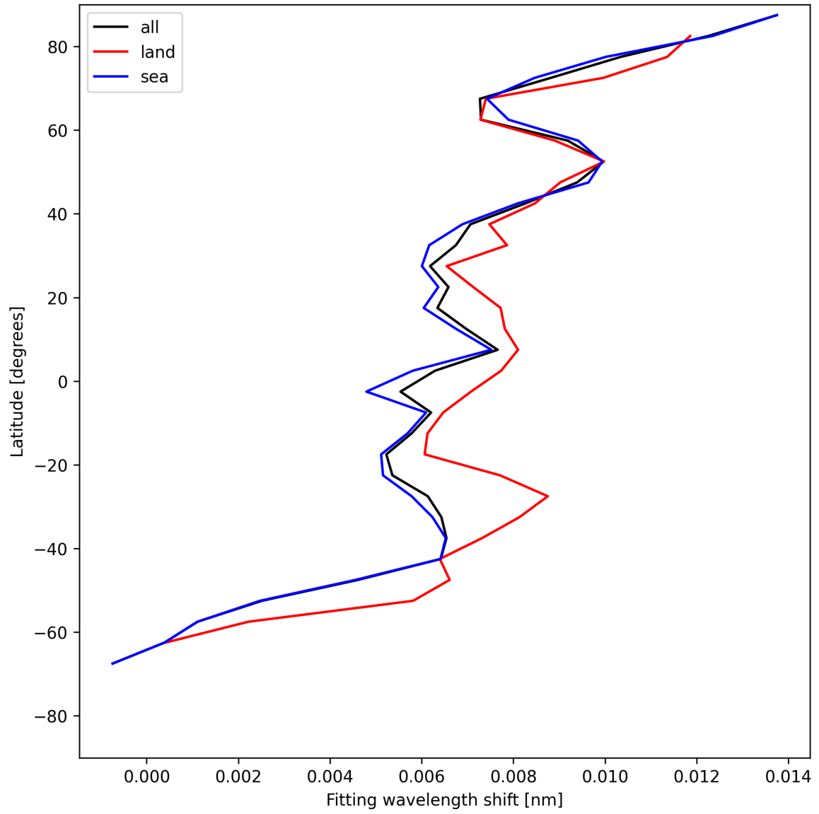
Figure 33: Zonal average of “Fitting wavelength shift” for 2025-06-17 to 2025-06-19.
