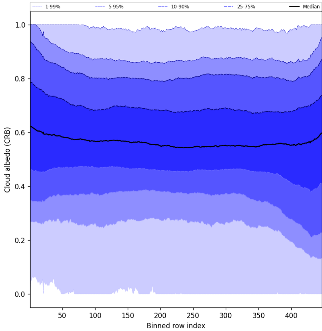
Figure 60: Along track statistics of “Cloud albedo (CRB)” for 2025-06-17 to 2025-06-19
