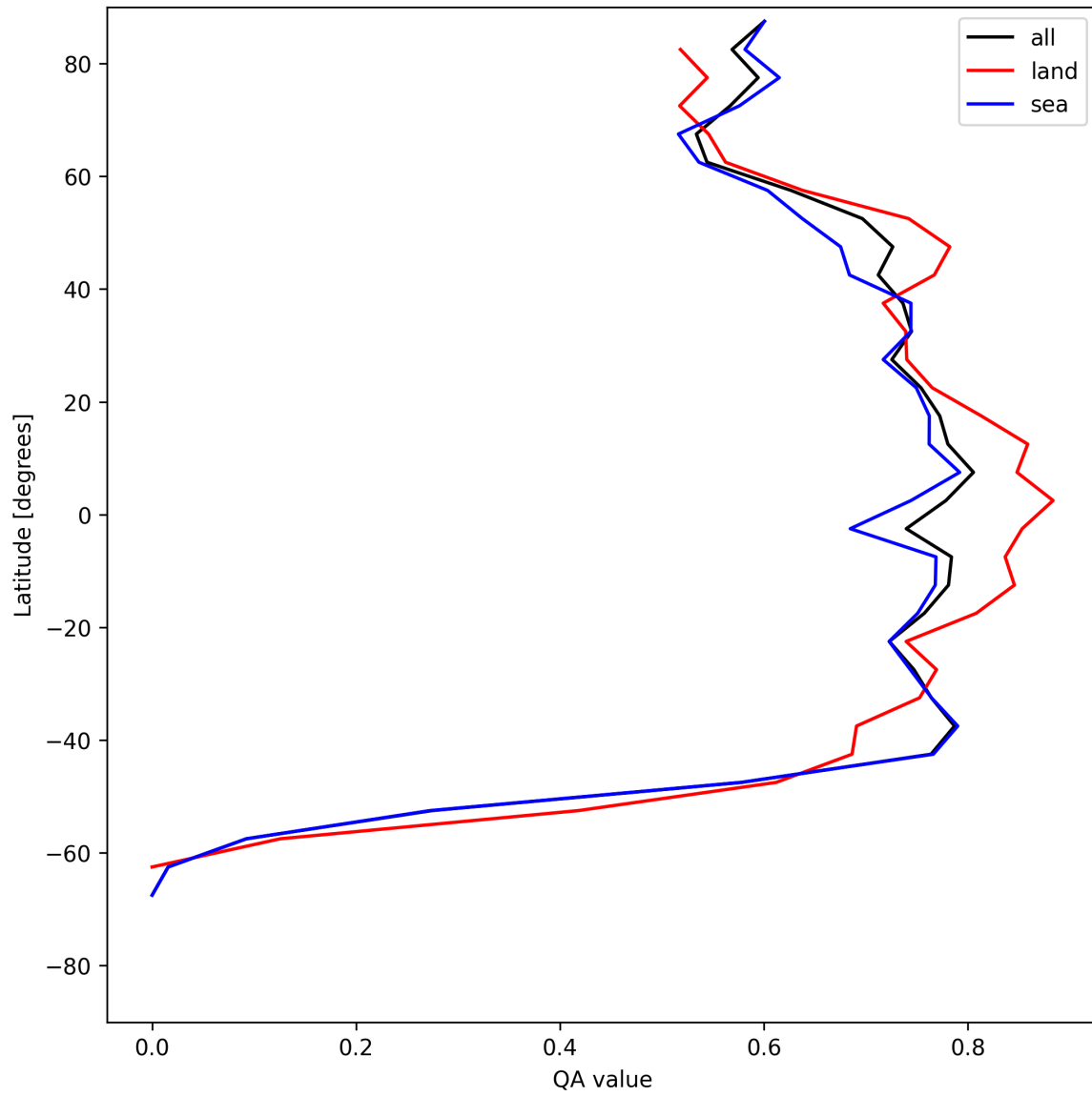
Figure 22: Zonal average of “QA value” for 2025-06-17 to 2025-06-19.
