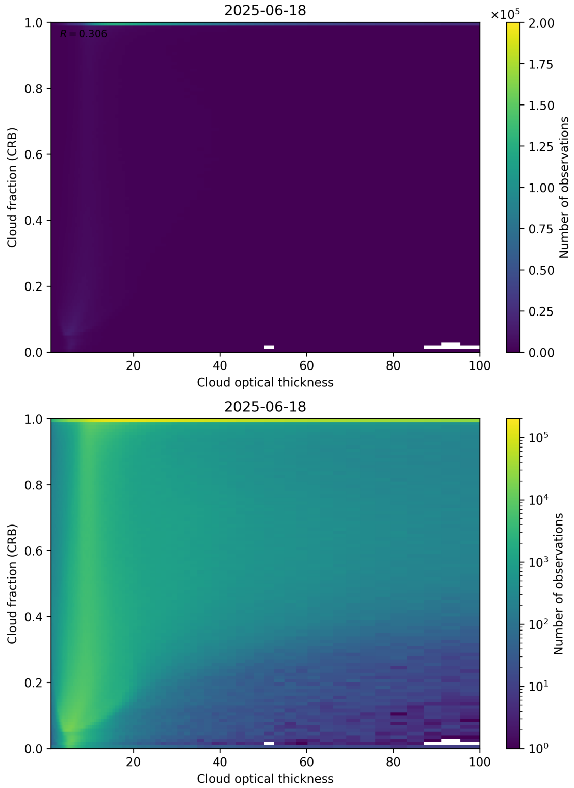
Figure 84: Scatter density plot of “Cloud optical thickness” against “Cloud fraction (CRB)” for 2025-06-17 to 2025-06-19.
