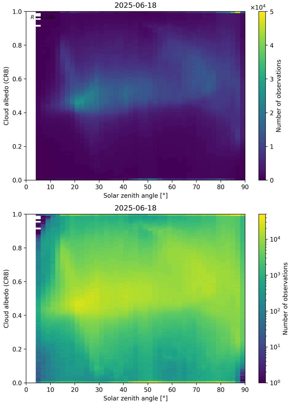
Figure 98: Scatter density plot of “Solar zenith angle” against “Cloud albedo (CRB)” for 2025-06-17 to 2025-06-19.
