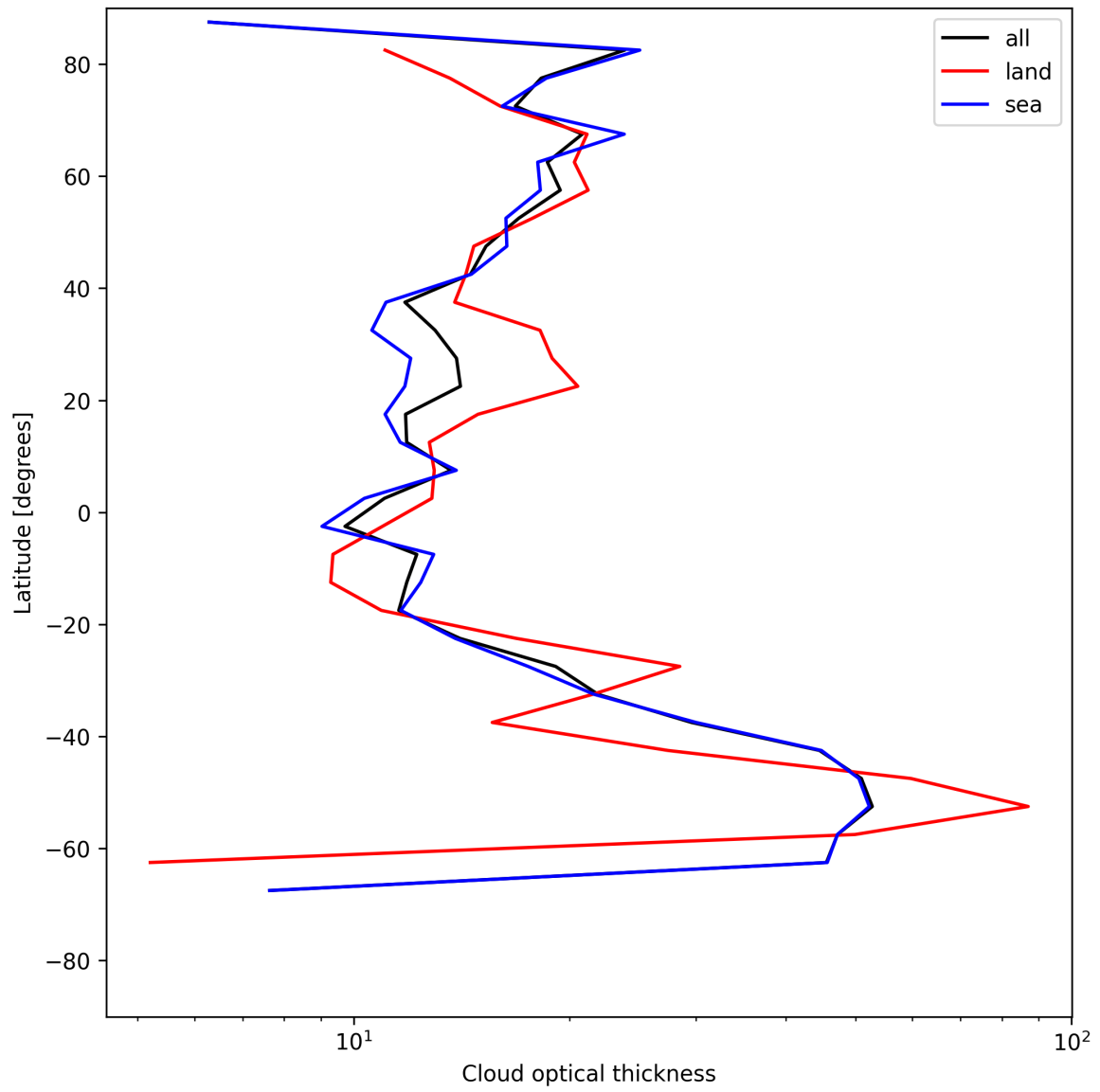
Figure 25: Zonal average of “Cloud optical thickness” for 2025-06-17 to 2025-06-19.
