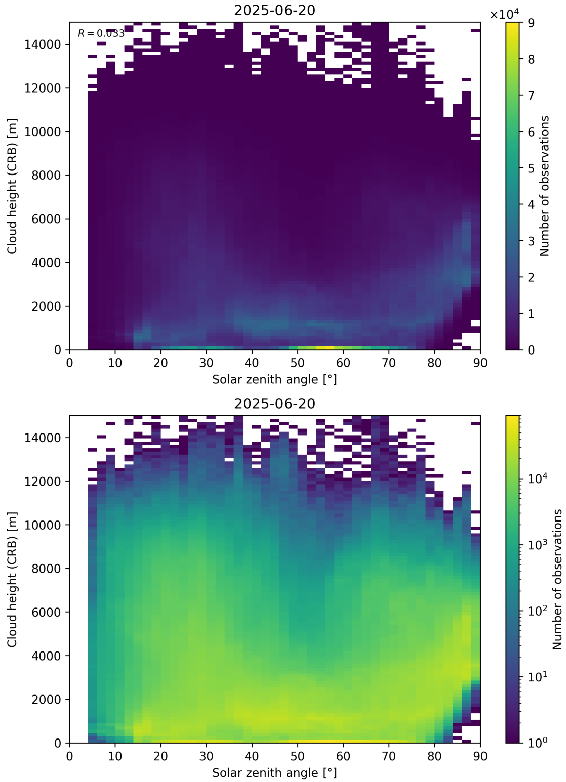
Figure 102: Scatter density plot of “Solar zenith angle” against “Cloud height (CRB)” for 2025-06-19 to 2025-06-21.
