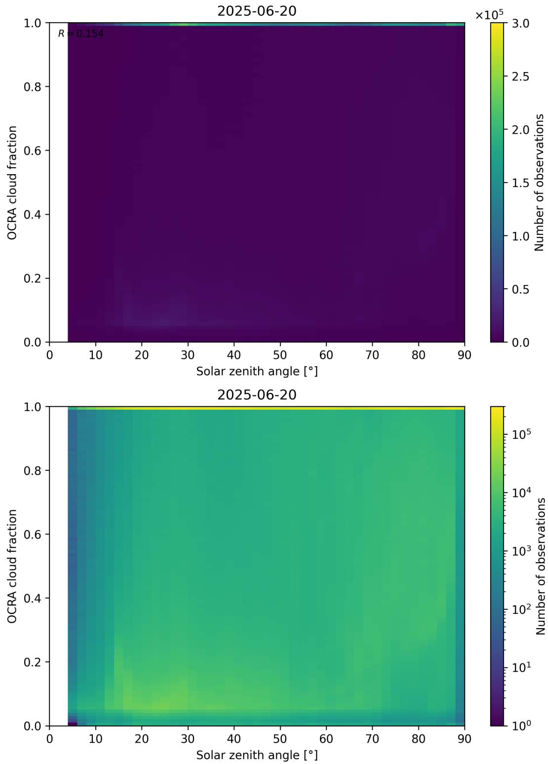
Figure 100: Scatter density plot of “Solar zenith angle” against “OCRA cloud fraction” for 2025-06-19 to 2025-06-21.
