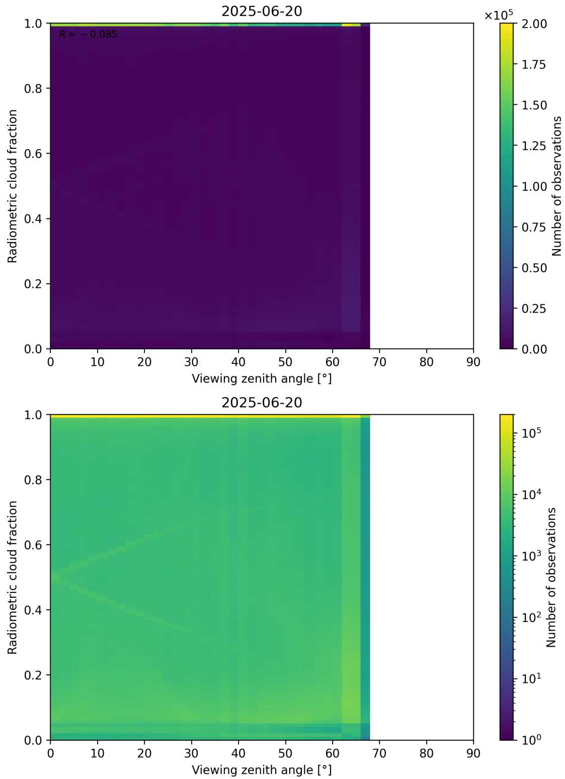
Figure 107: Scatter density plot of “Viewing zenith angle” against “Radiometric cloud fraction” for 2025-06-19 to 2025-06-21.
