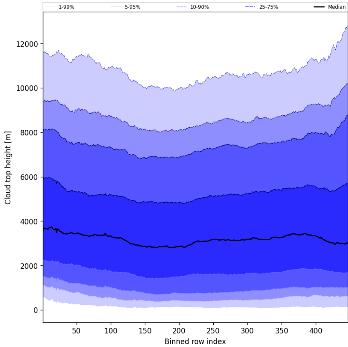
Figure 56: Along track statistics of “Cloud top height” for 2025-06-19 to 2025-06-21
