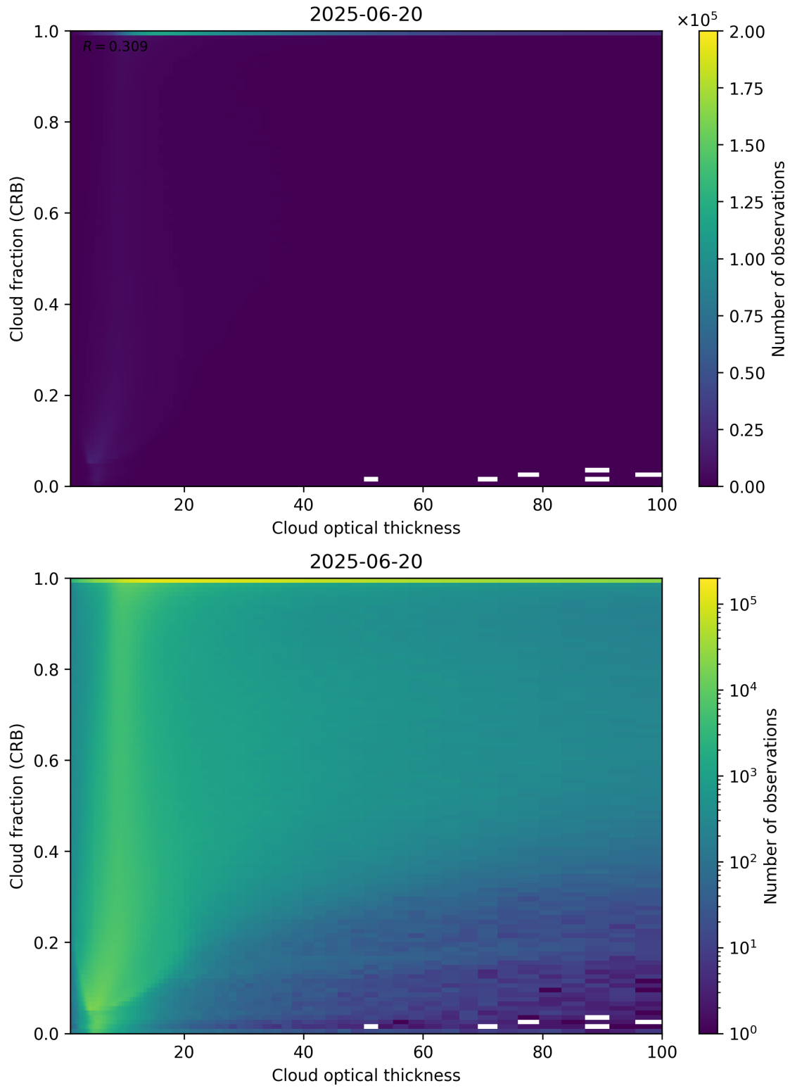
Figure 84: Scatter density plot of “Cloud optical thickness” against “Cloud fraction (CRB)” for 2025-06-19 to 2025-06-21.
