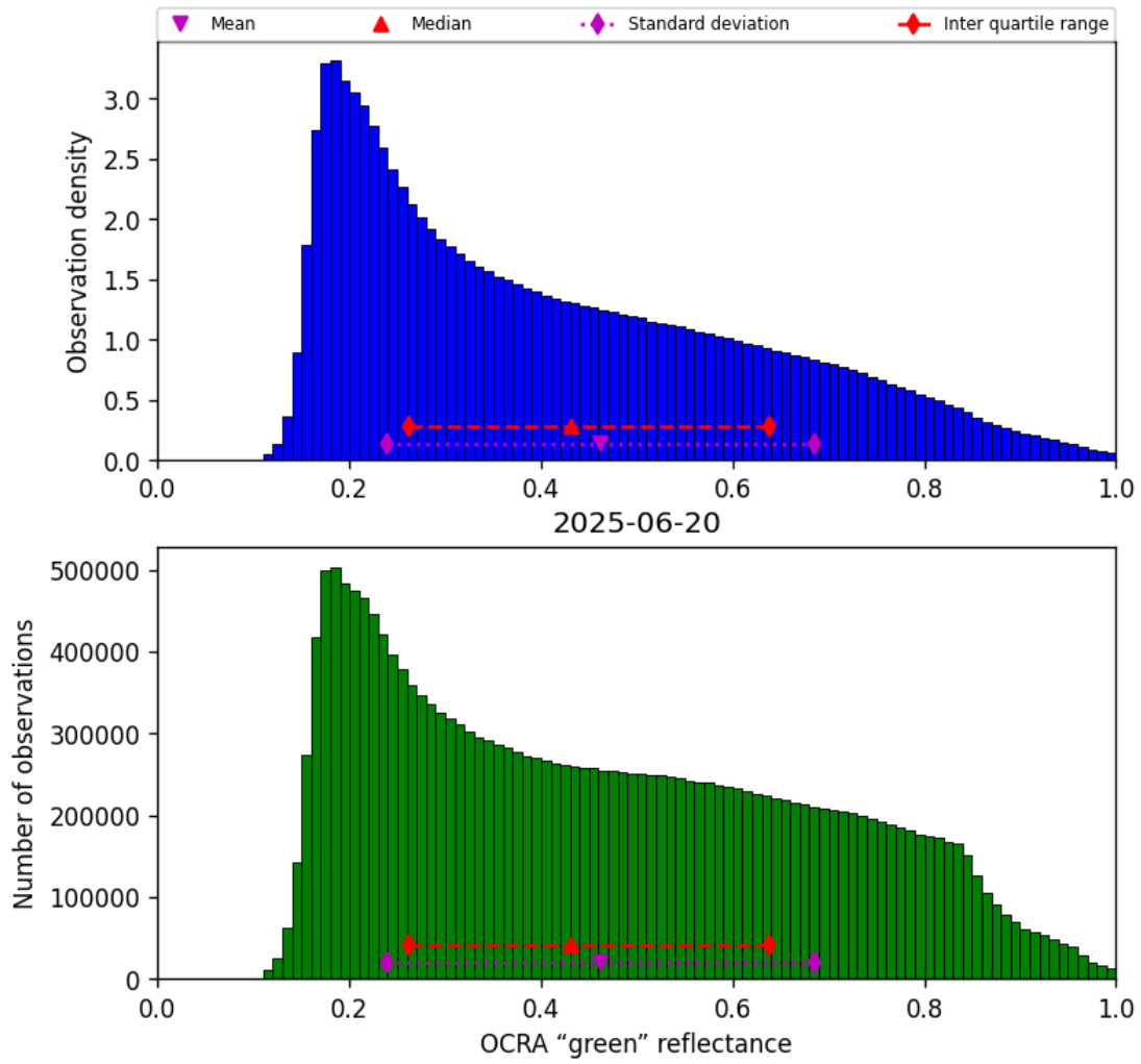
Figure 52: Histogram of “OCRA “green” reflectance” for 2025-06-19 to 2025-06-21
