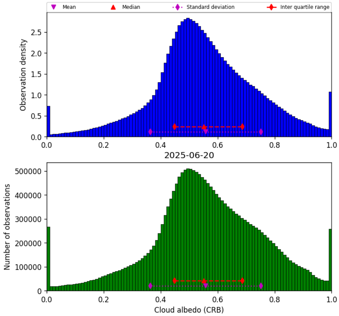
Figure 44: Histogram of “Cloud albedo (CRB)” for 2025-06-19 to 2025-06-21
