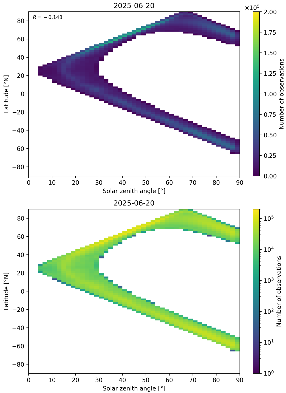
Figure 105: Scatter density plot of “Solar zenith angle” against “Latitude” for 2025-06-19 to 2025-06-21.
