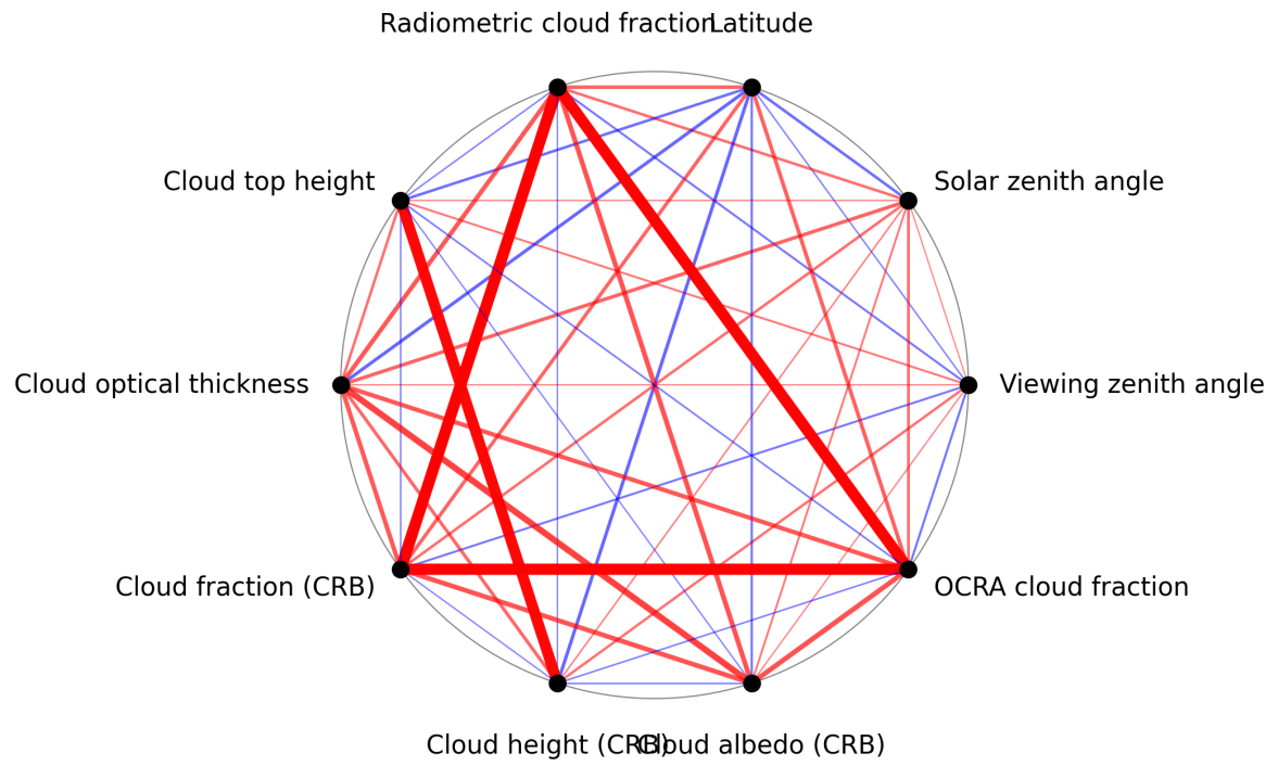
Figure 1: Map of correlation graph for 2025-06-19 to 2025-06-21.
