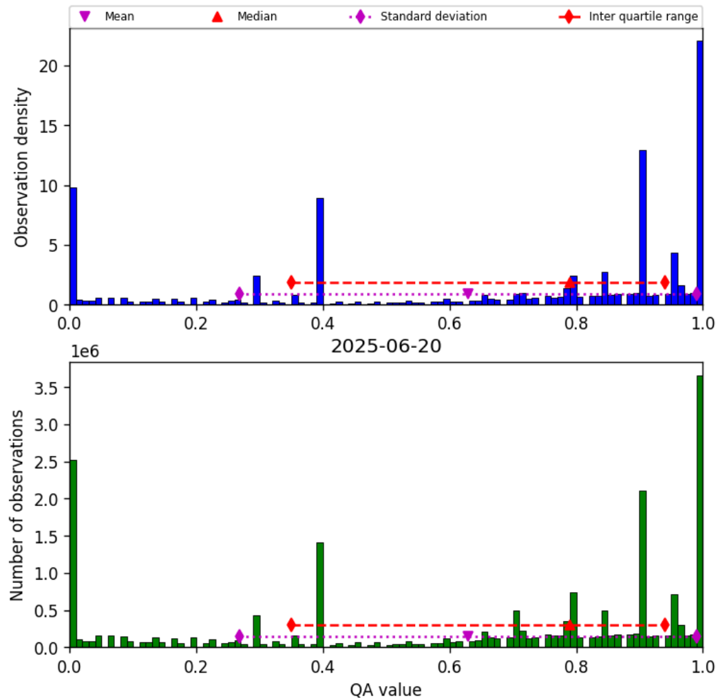
Figure 38: Histogram of “QA value” for 2025-06-19 to 2025-06-21
