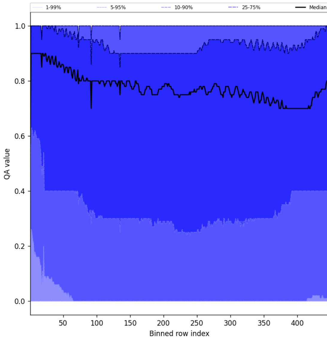
Figure 54: Along track statistics of “QA value” for 2025-06-19 to 2025-06-21
