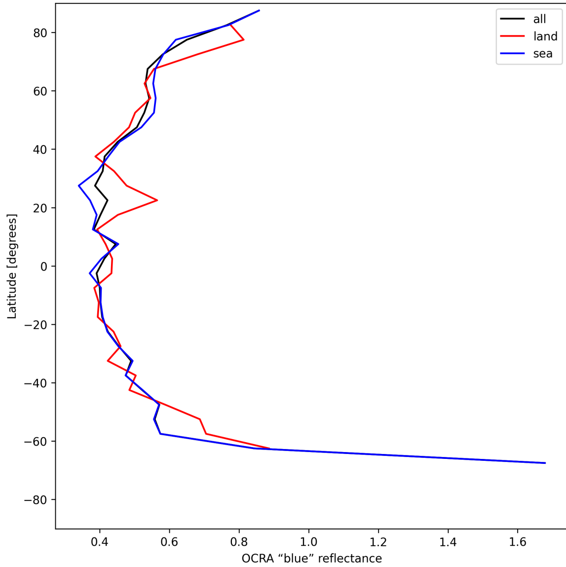
Figure 35: Zonal average of “OCRA “blue” reflectance” for 2025-06-19 to 2025-06-21.
