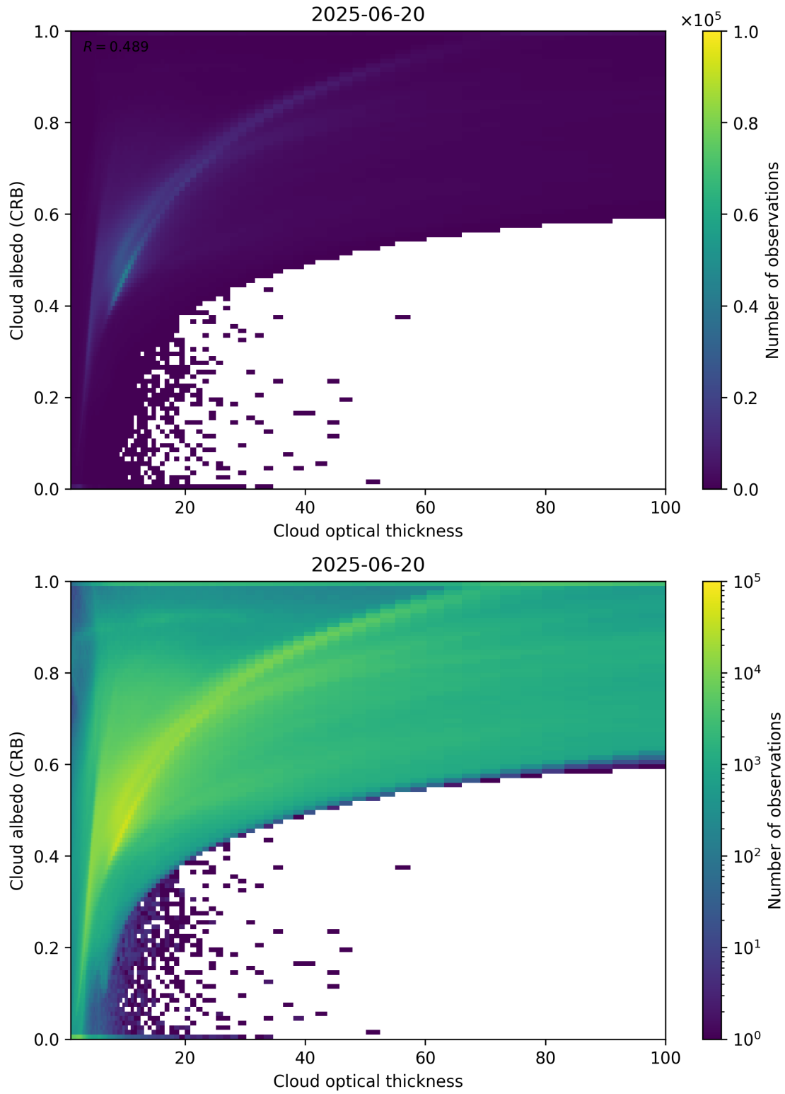
Figure 82: Scatter density plot of “Cloud optical thickness” against “Cloud albedo (CRB)” for 2025-06-19 to 2025-06-21.
