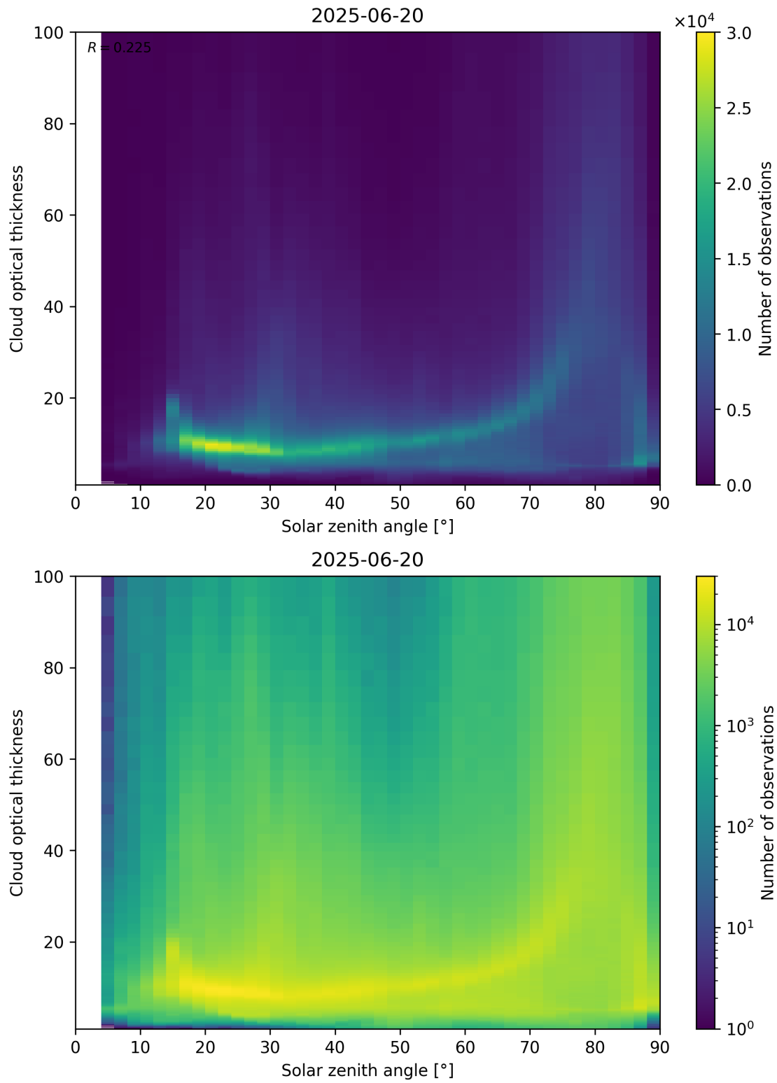
Figure 103: Scatter density plot of “Solar zenith angle” against “Cloud optical thickness” for 2025-06-19 to 2025-06-21.
