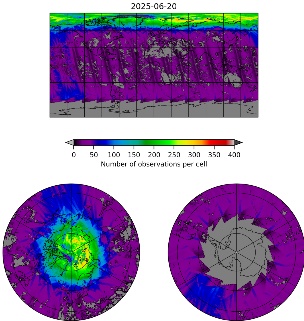
Figure 21: Map of the number of observations for 2025-06-19 to 2025-06-21
