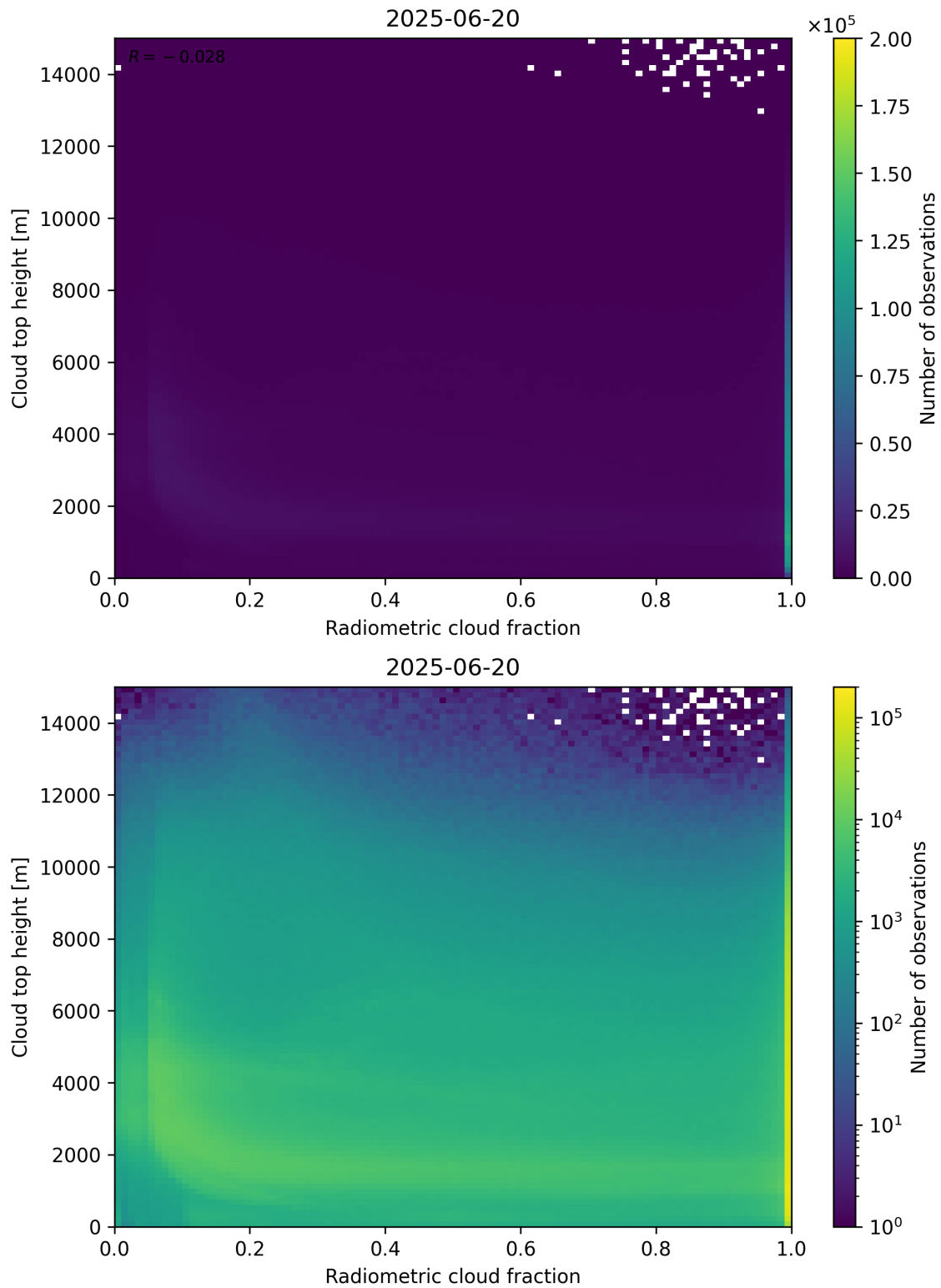
Figure 76: Scatter density plot of “Radiometric cloud fraction” against “Cloud top height” for 2025-06-19 to 2025-06-21.
