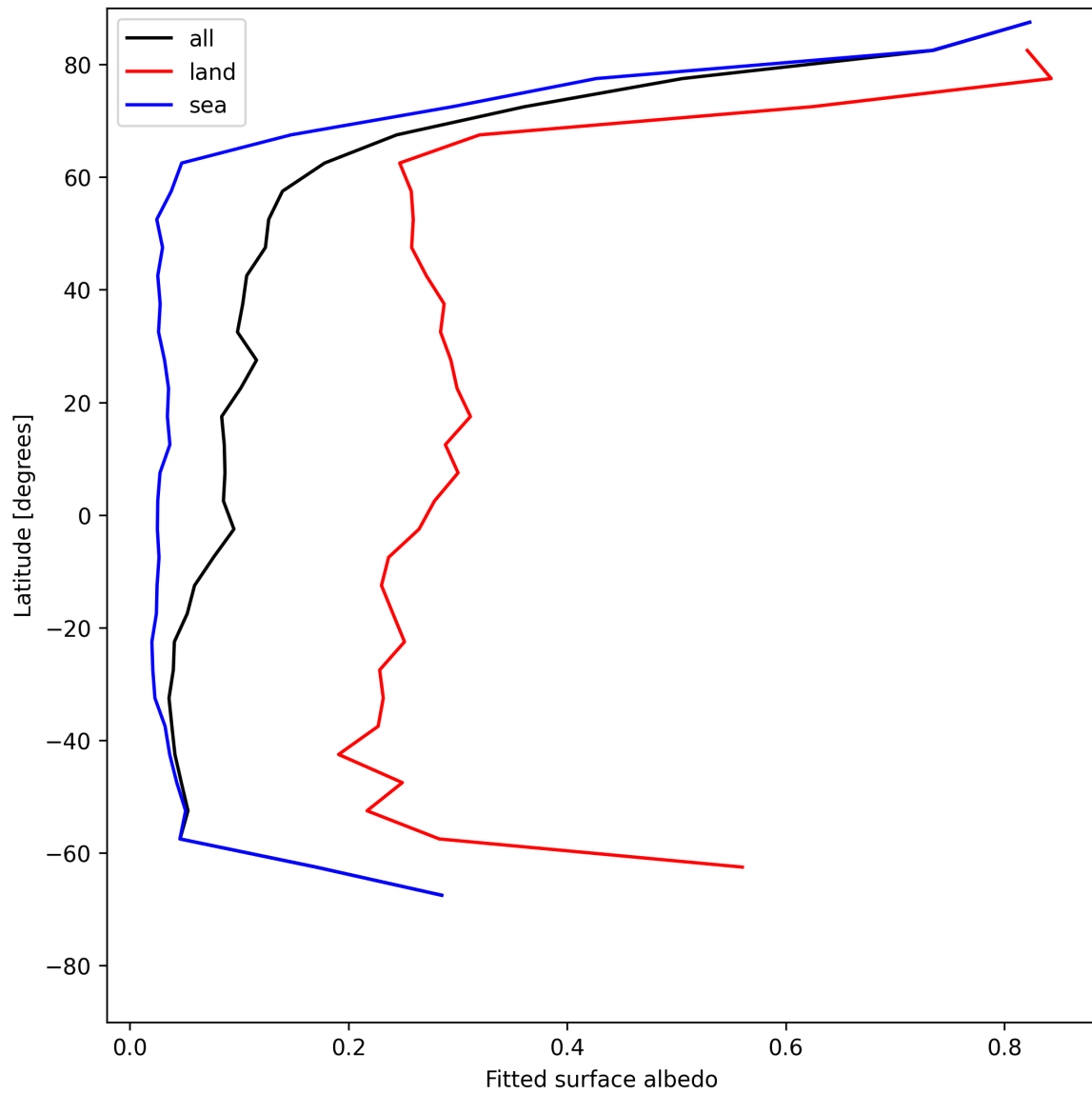
Figure 29: Zonal average of “Fitted surface albedo” for 2025-06-19 to 2025-06-21.
