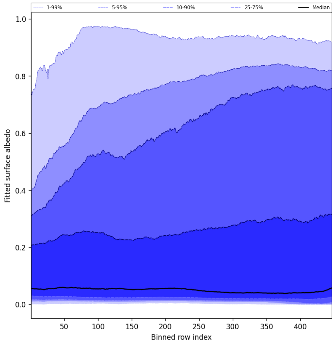
Figure 61: Along track statistics of “Fitted surface albedo” for 2025-06-19 to 2025-06-21
