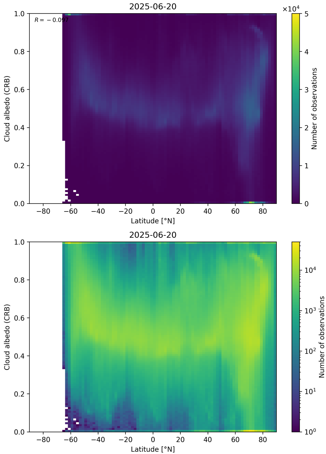
Figure 91: Scatter density plot of “Latitude” against “Cloud albedo (CRB)” for 2025-06-19 to 2025-06-21.
