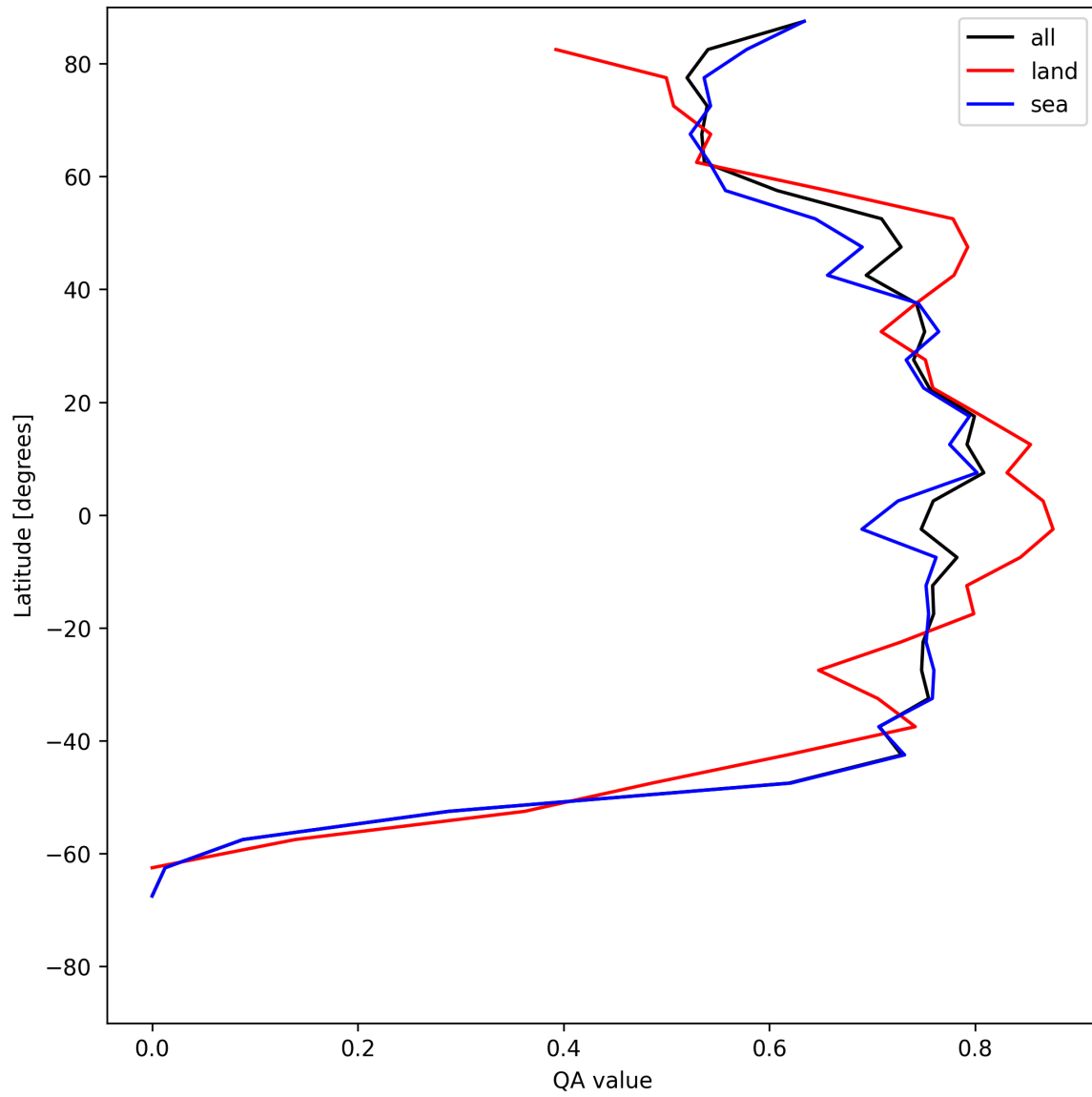
Figure 22: Zonal average of “QA value” for 2025-06-19 to 2025-06-21.
