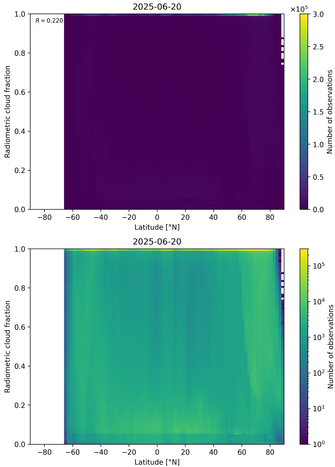
Figure 92: Scatter density plot of “Latitude” against “Radiometric cloud fraction” for 2025-06-19 to 2025-06-21.
