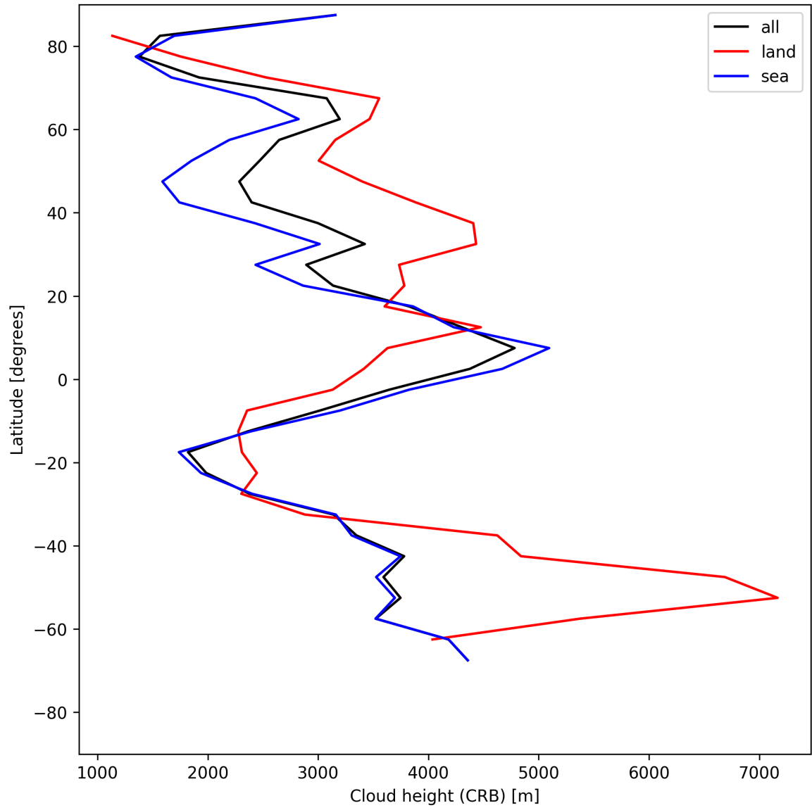
Figure 27: Zonal average of “Cloud height (CRB)” for 2025-06-19 to 2025-06-21.
