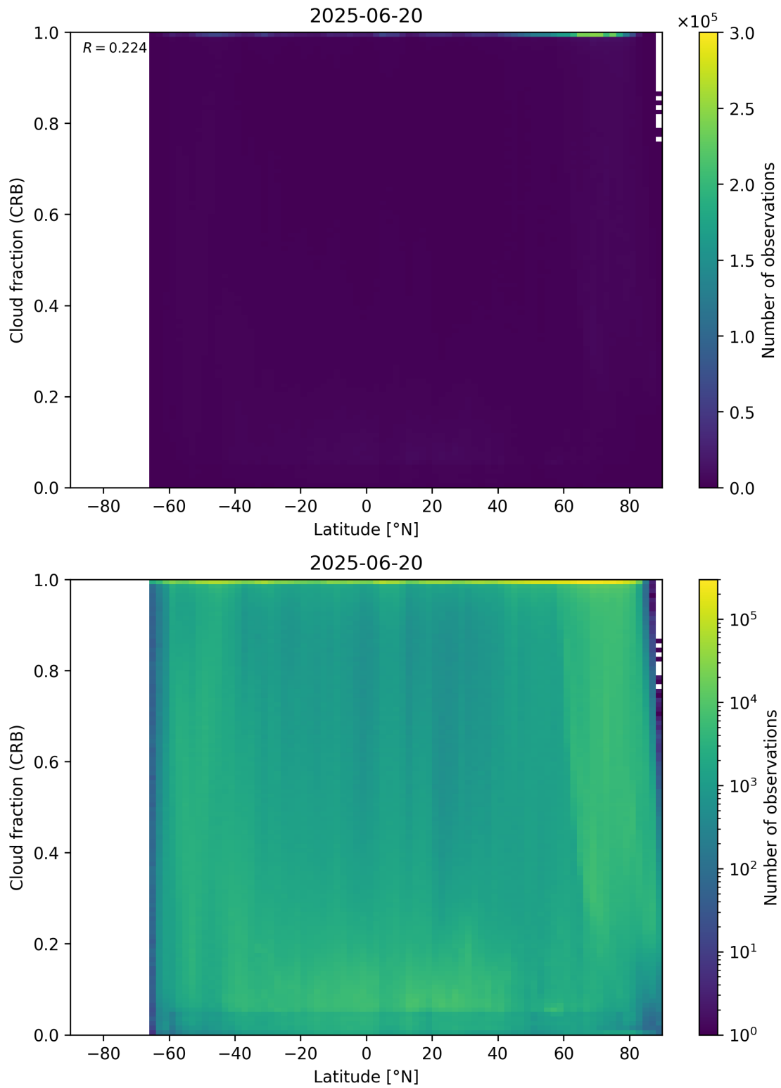
Figure 94: Scatter density plot of “Latitude” against “Cloud fraction (CRB)” for 2025-06-19 to 2025-06-21.
