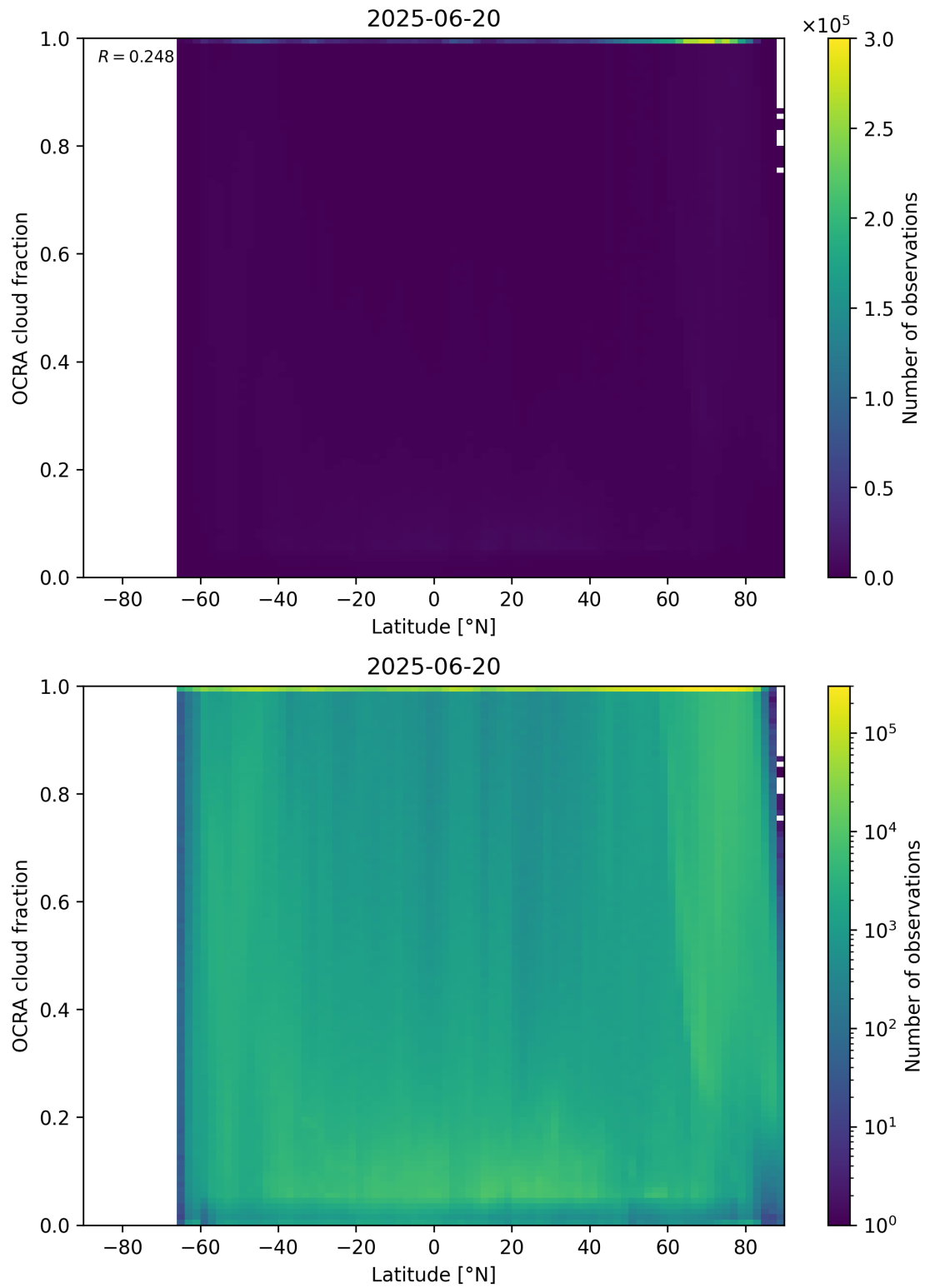
Figure 93: Scatter density plot of “Latitude” against “OCRA cloud fraction” for 2025-06-19 to 2025-06-21.
