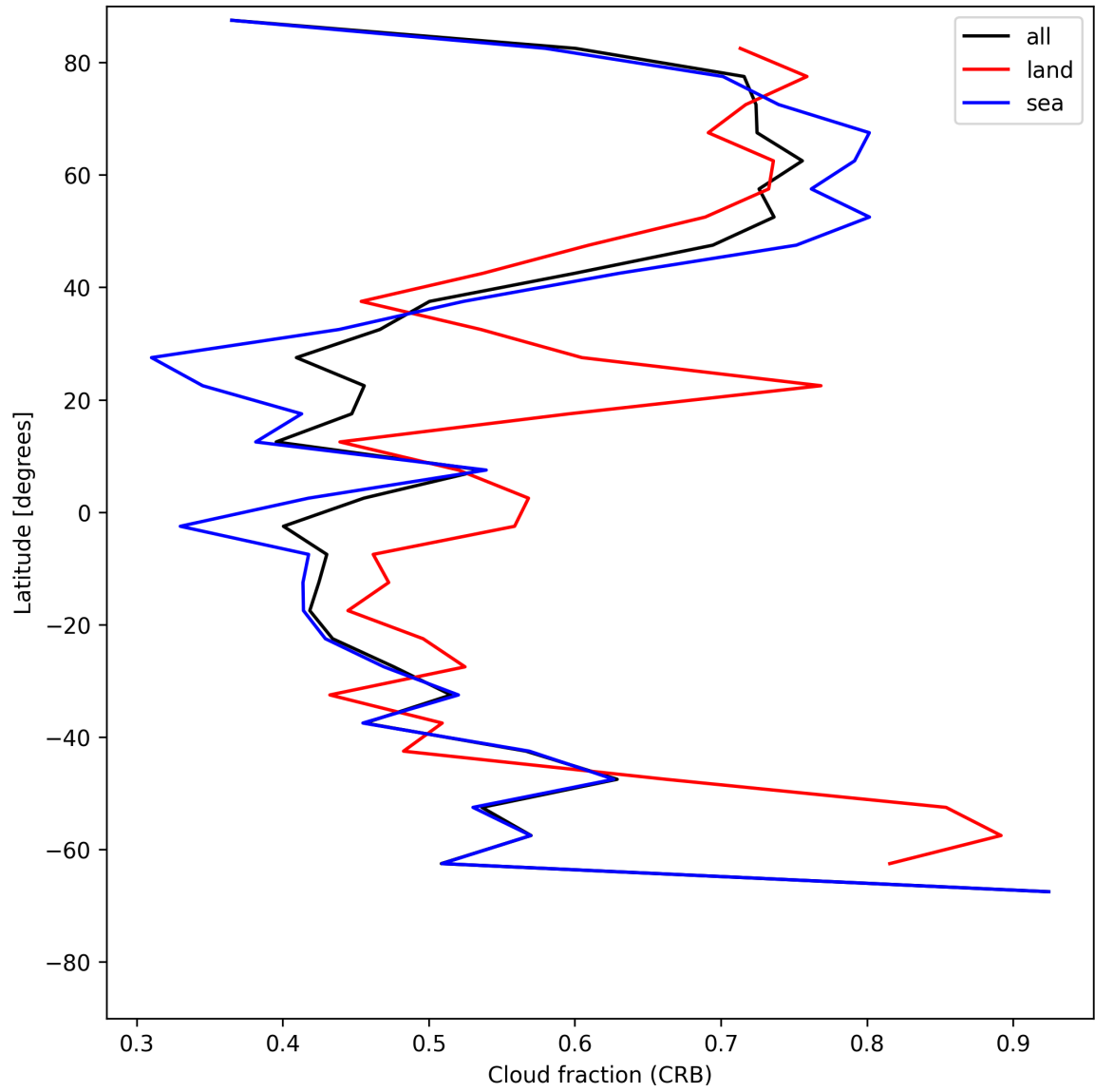
Figure 26: Zonal average of “Cloud fraction (CRB)” for 2025-06-19 to 2025-06-21.
