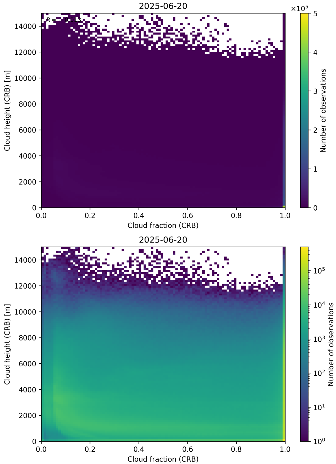
Figure 79: Scatter density plot of “Cloud fraction (CRB)” against “Cloud height (CRB)” for 2025-06-19 to 2025-06-21.
