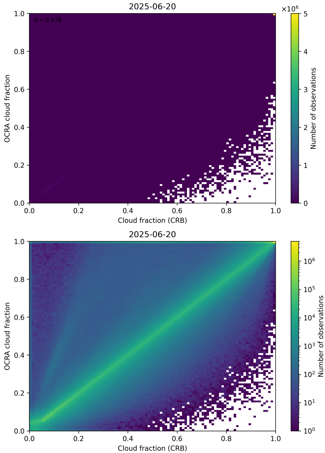
Figure 78: Scatter density plot of “Cloud fraction (CRB)” against “OCRA cloud fraction” for 2025-06-19 to 2025-06-21.
