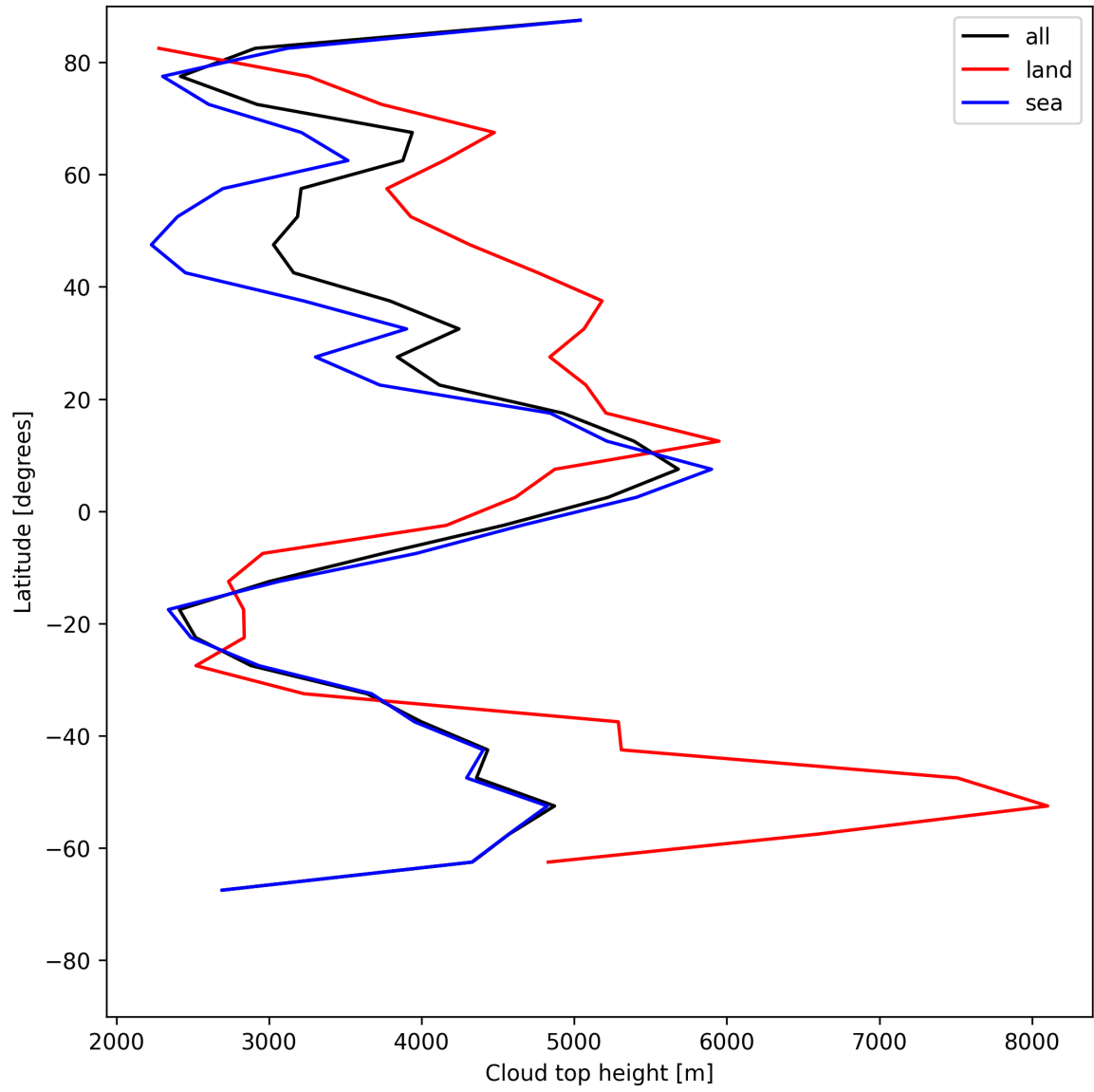
Figure 24: Zonal average of “Cloud top height” for 2025-06-19 to 2025-06-21.
