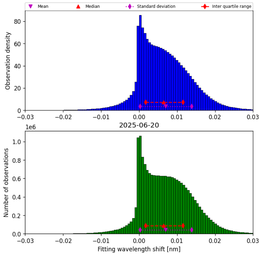
Figure 49: Histogram of “Fitting wavelength shift” for 2025-06-19 to 2025-06-21
