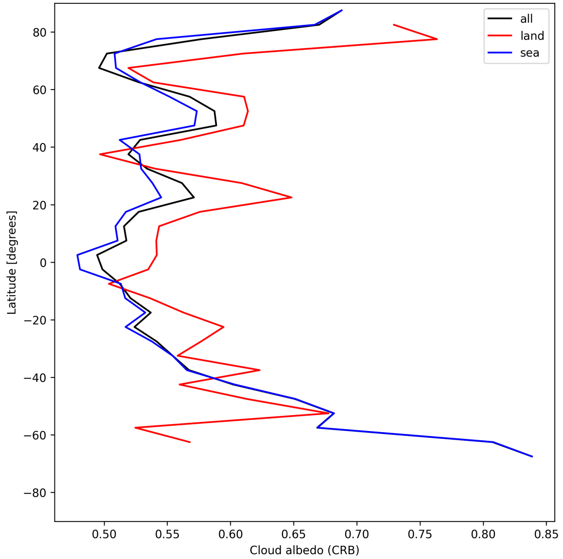
Figure 28: Zonal average of “Cloud albedo (CRB)” for 2025-06-19 to 2025-06-21.
