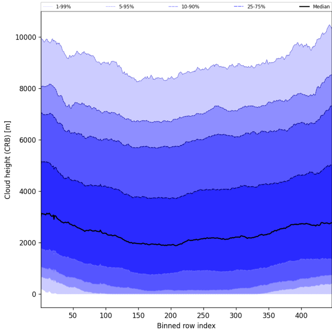
Figure 59: Along track statistics of “Cloud height (CRB)” for 2025-06-19 to 2025-06-21
