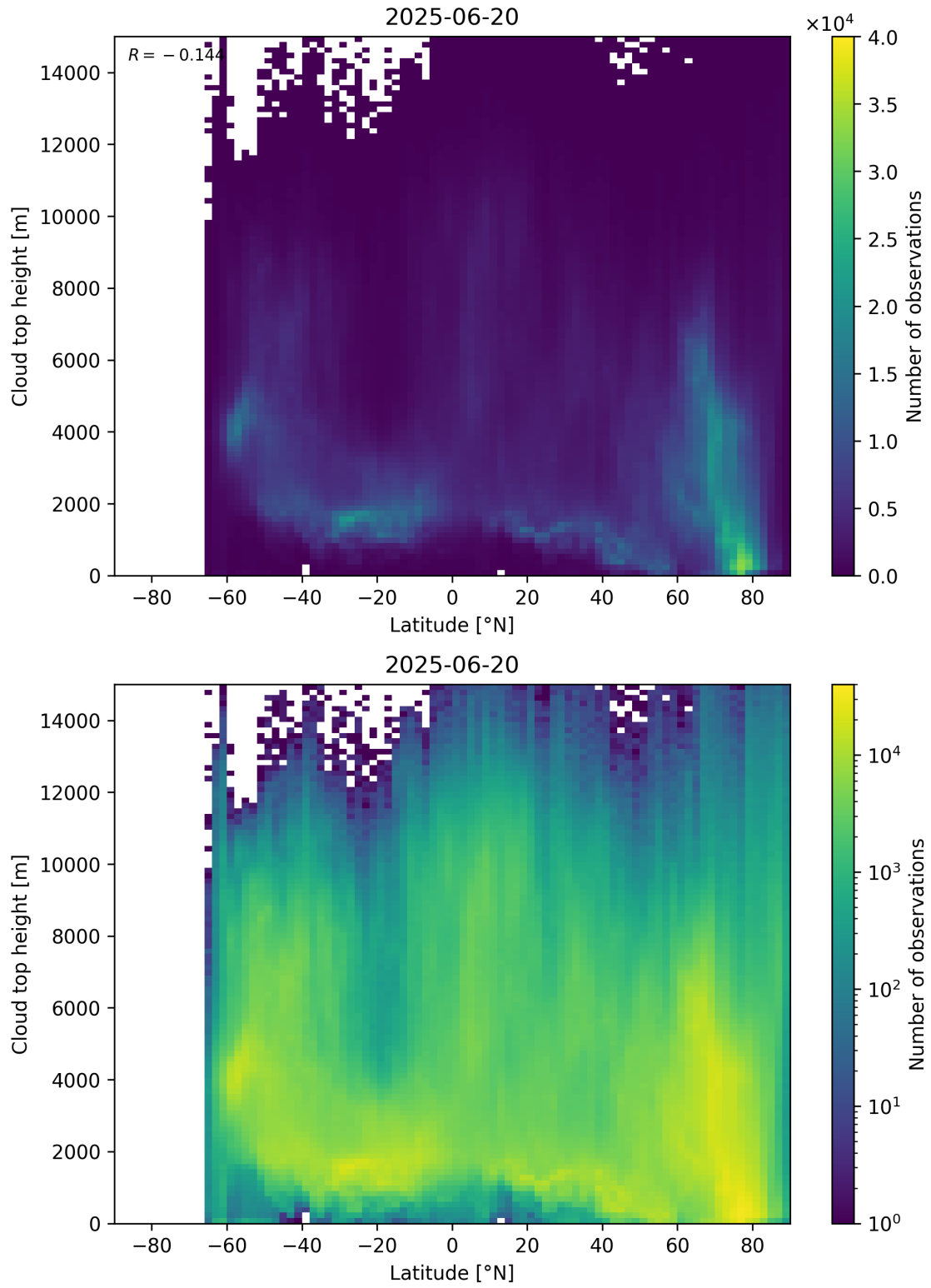
Figure 97: Scatter density plot of “Latitude” against “Cloud top height” for 2025-06-19 to 2025-06-21.
