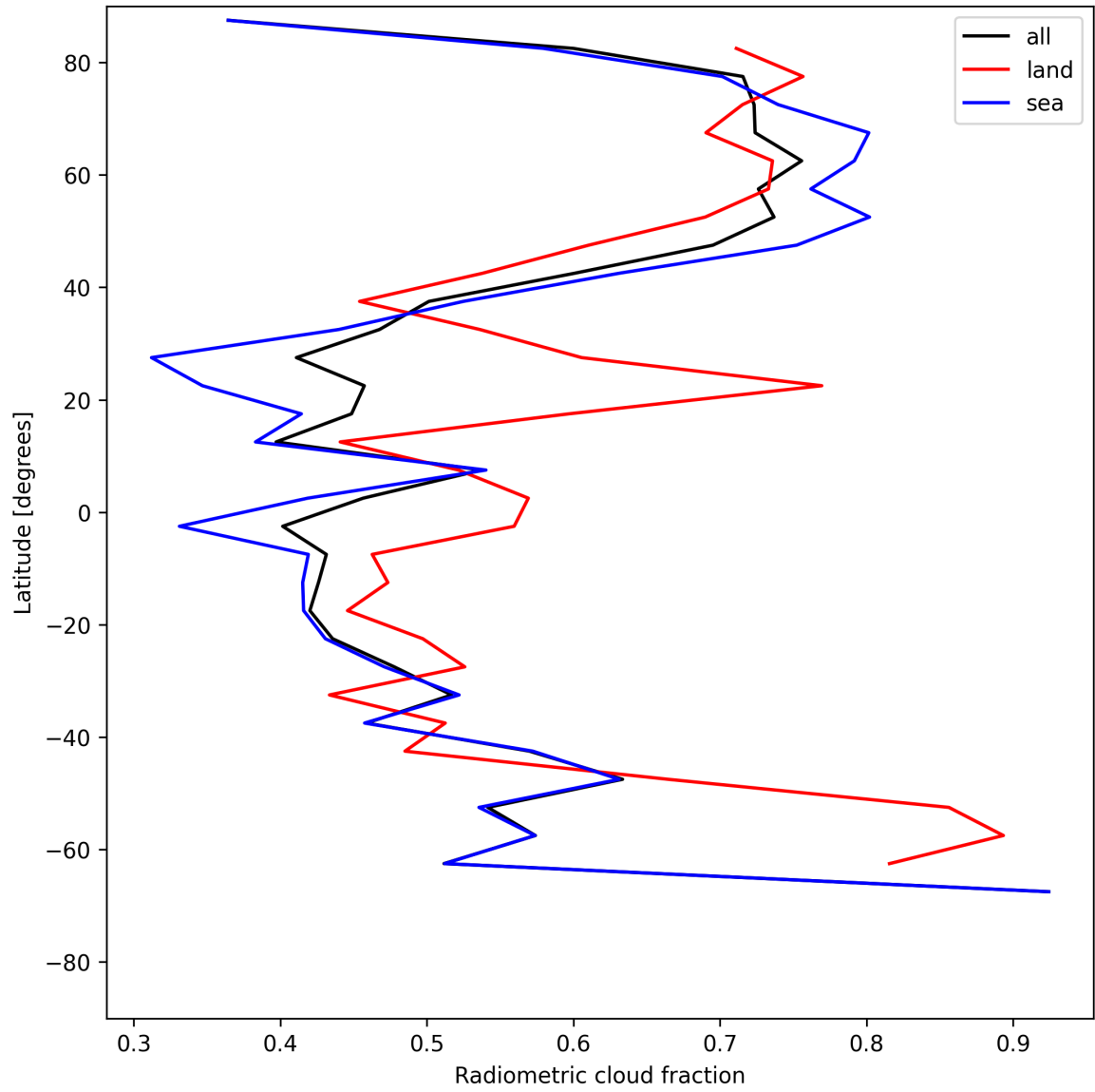
Figure 23: Zonal average of “Radiometric cloud fraction” for 2025-06-19 to 2025-06-21.
