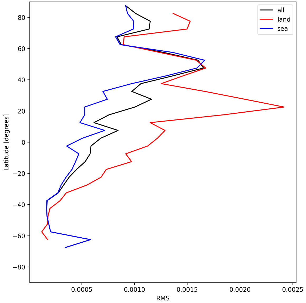
Figure 31: Zonal average of “RMS” for 2025-06-19 to 2025-06-21.
