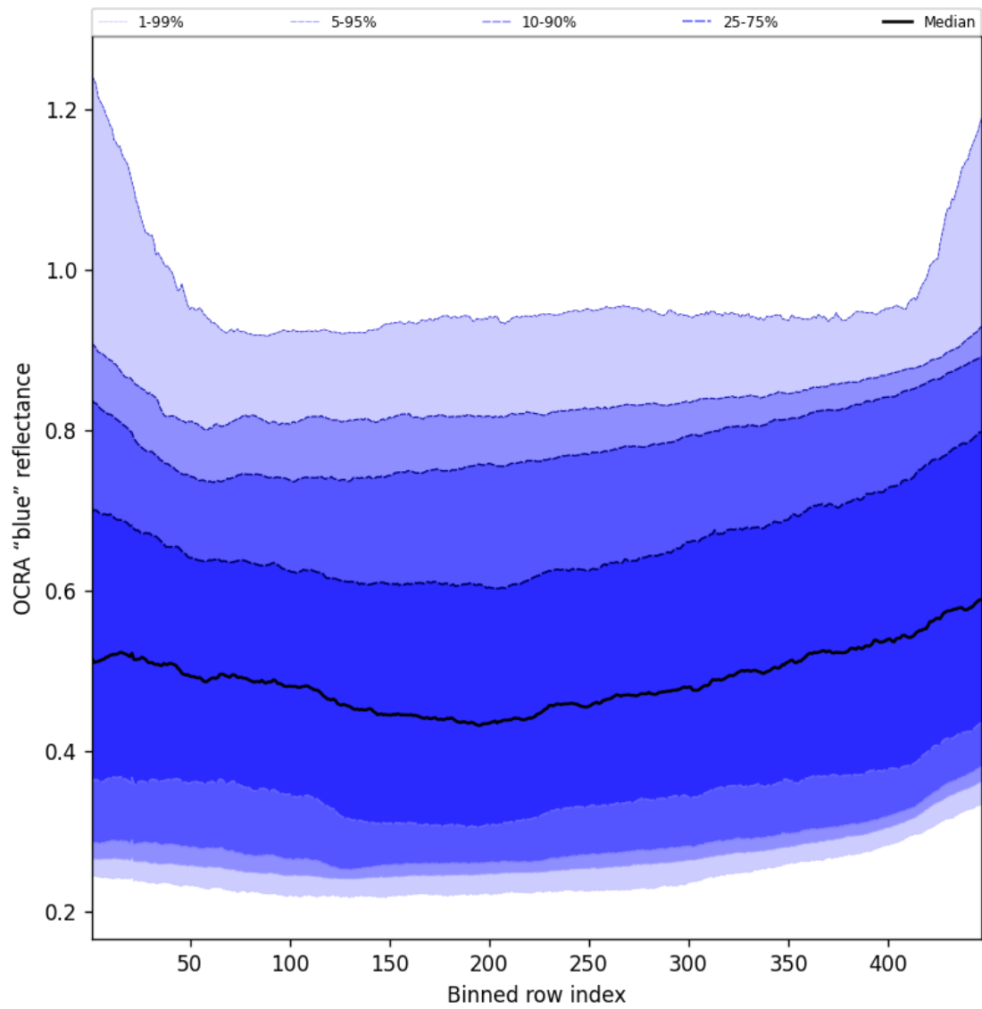
Figure 67: Along track statistics of “OCRA “blue” reflectance” for 2025-06-19 to 2025-06-21
