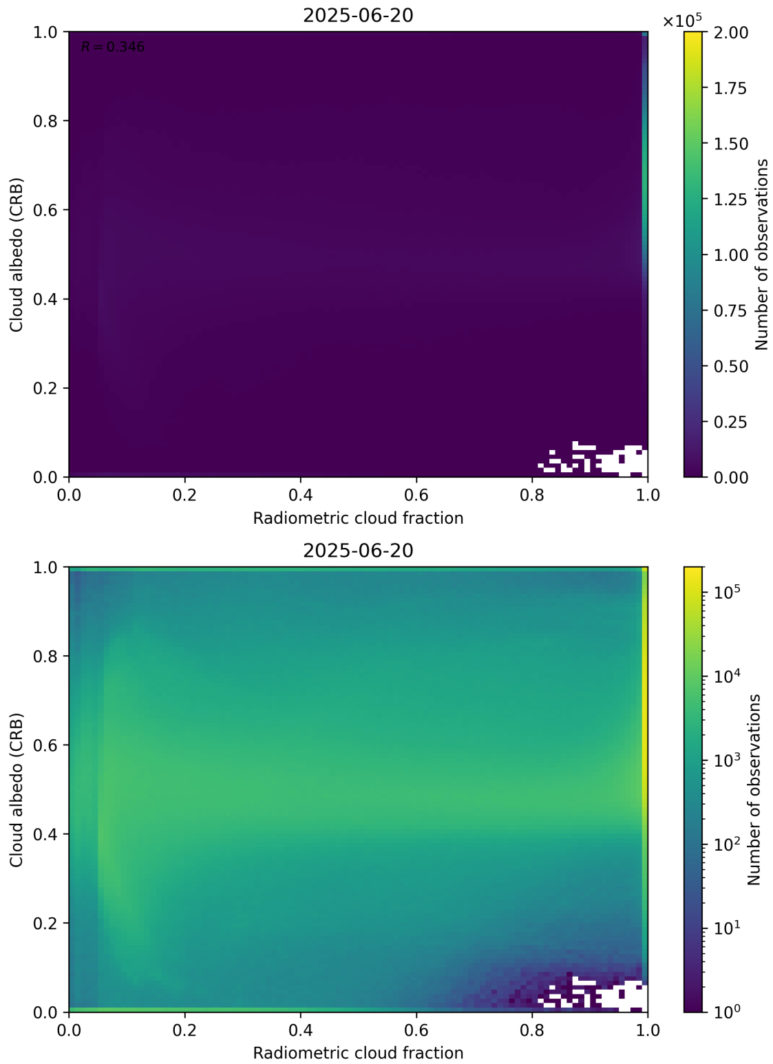
Figure 71: Scatter density plot of “Radiometric cloud fraction” against “Cloud albedo (CRB)” for 2025-06-19 to 2025-06-21.
