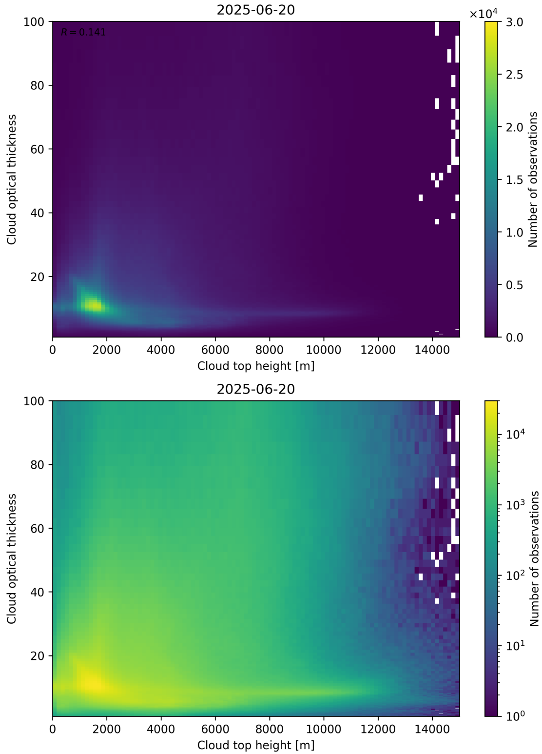
Figure 90: Scatter density plot of “Cloud top height” against “Cloud optical thickness” for 2025-06-19 to 2025-06-21.
