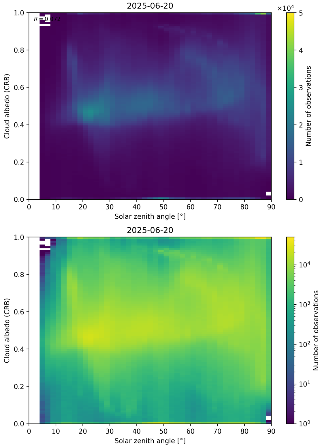
Figure 98: Scatter density plot of “Solar zenith angle” against “Cloud albedo (CRB)” for 2025-06-19 to 2025-06-21.
