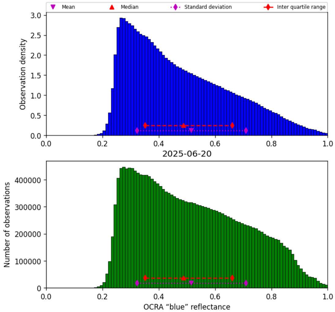
Figure 51: Histogram of “OCRA “blue” reflectance” for 2025-06-19 to 2025-06-21
