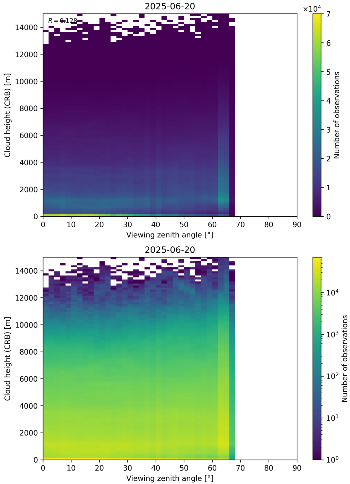
Figure 110: Scatter density plot of “Viewing zenith angle” against “Cloud height (CRB)” for 2025-06-19 to 2025-06-21.
