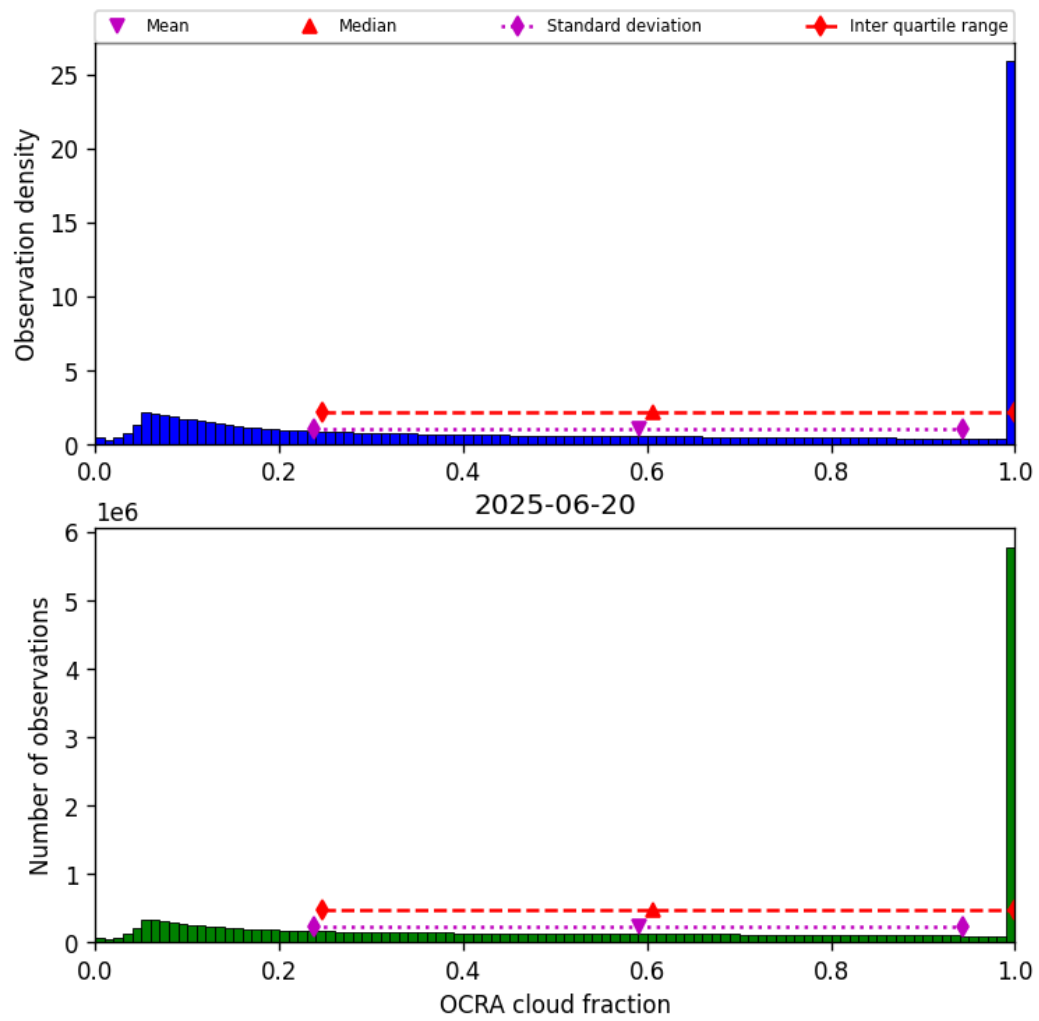
Figure 50: Histogram of “OCRA cloud fraction” for 2025-06-19 to 2025-06-21
