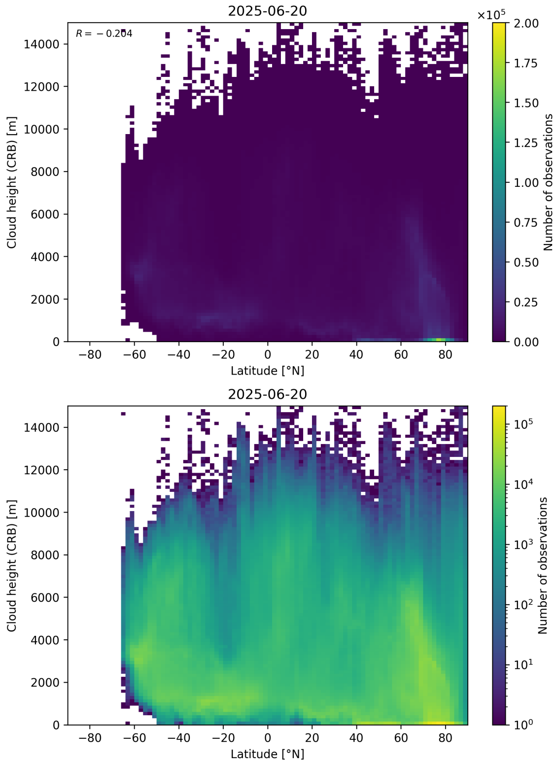
Figure 95: Scatter density plot of “Latitude” against “Cloud height (CRB)” for 2025-06-19 to 2025-06-21.
