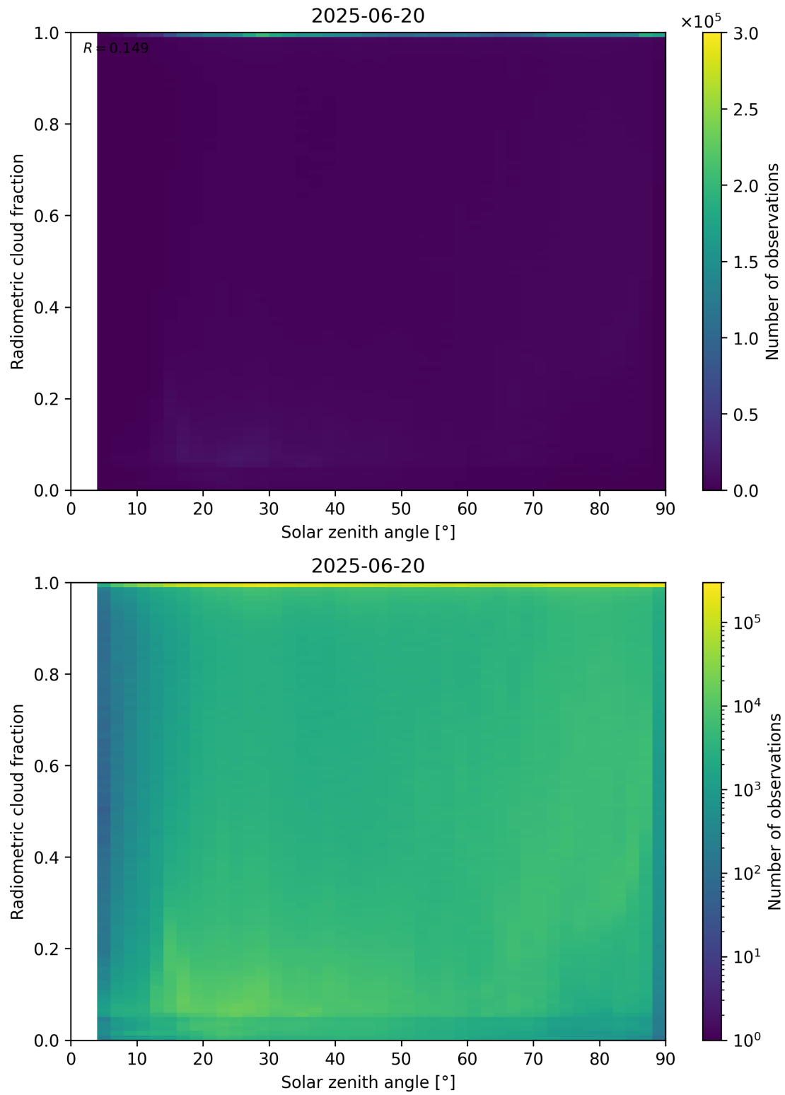
Figure 99: Scatter density plot of “Solar zenith angle” against “Radiometric cloud fraction” for 2025-06-19 to 2025-06-21.
