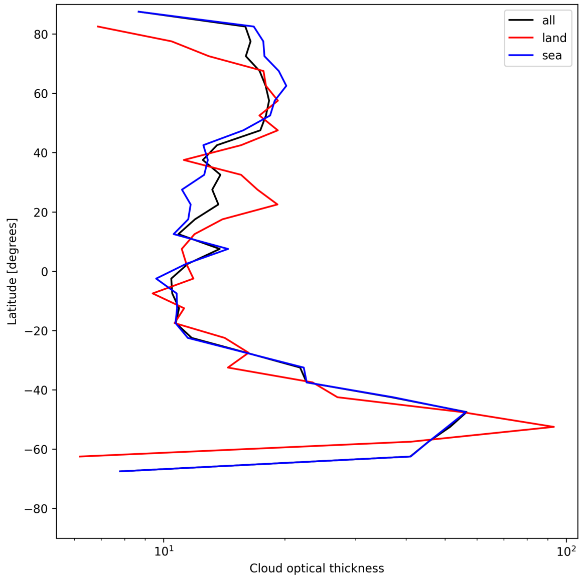
Figure 25: Zonal average of “Cloud optical thickness” for 2025-06-19 to 2025-06-21.
