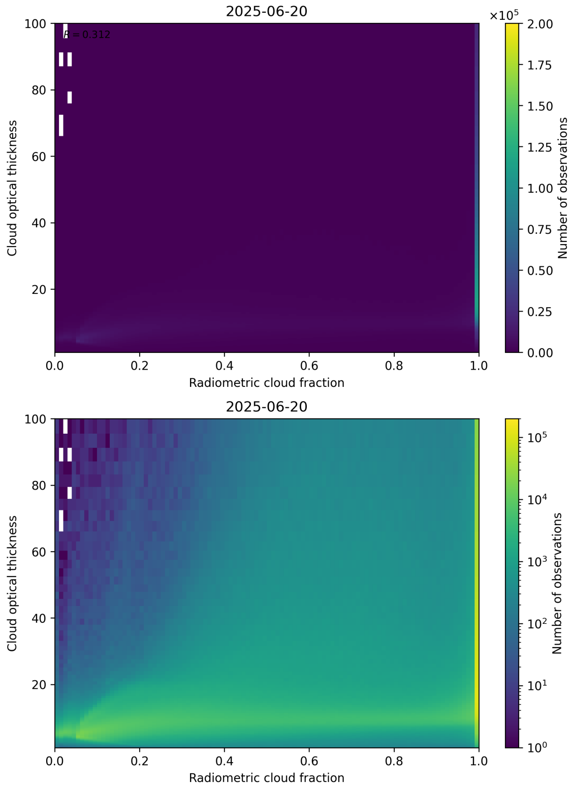
Figure 75: Scatter density plot of “Radiometric cloud fraction” against “Cloud optical thickness” for 2025-06-19 to 2025-06-21.
