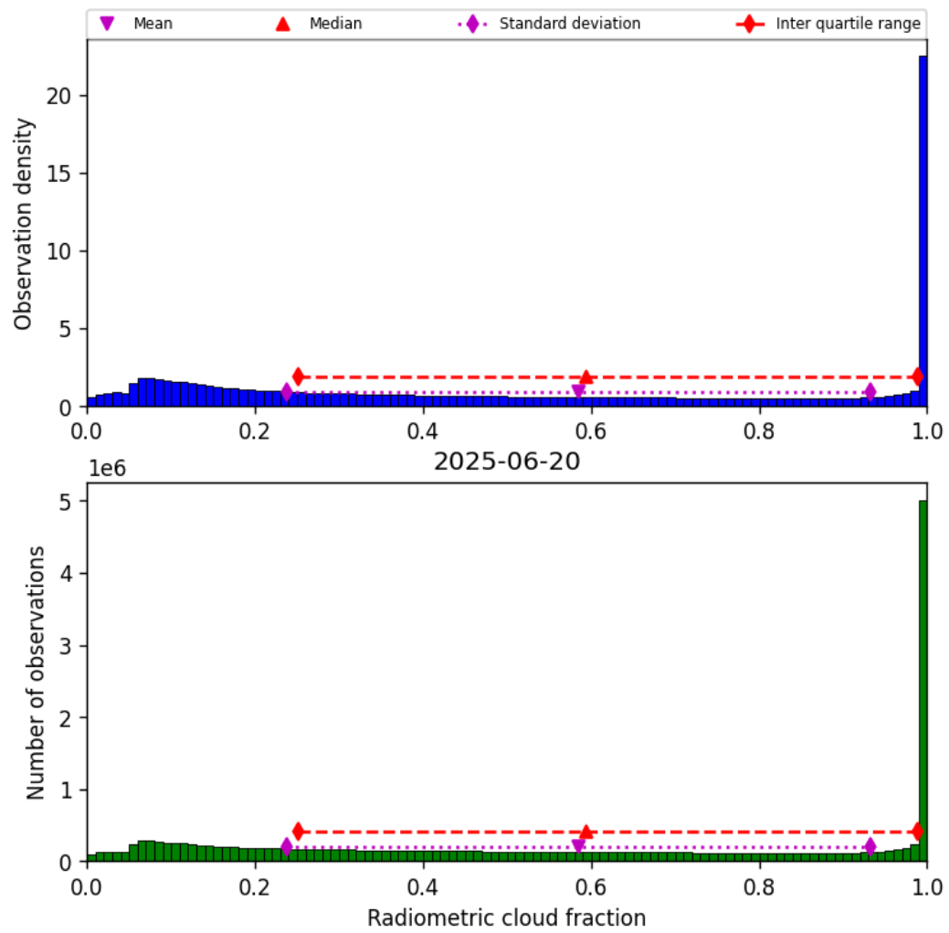
Figure 39: Histogram of “Radiometric cloud fraction” for 2025-06-19 to 2025-06-21
