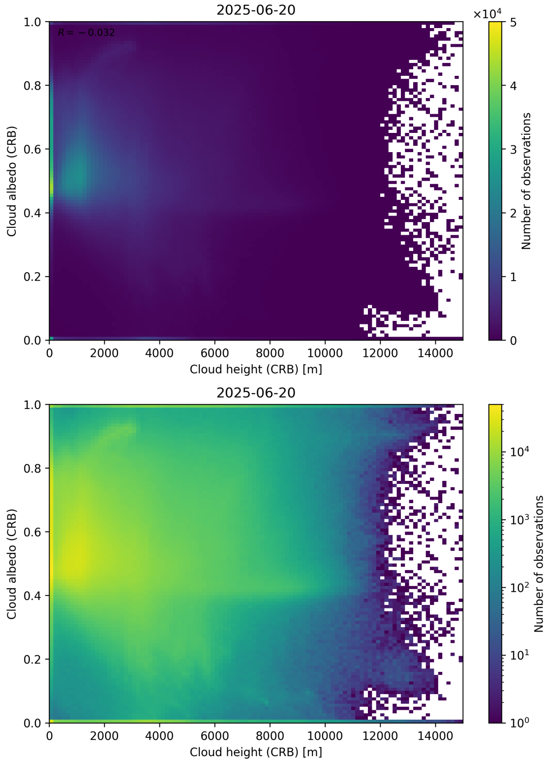
Figure 80: Scatter density plot of “Cloud height (CRB)” against “Cloud albedo (CRB)” for 2025-06-19 to 2025-06-21.
