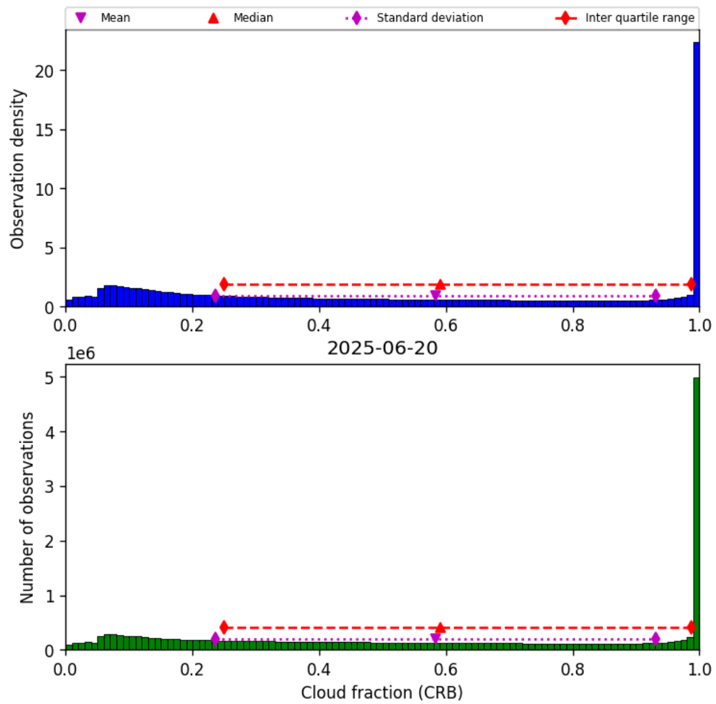
Figure 42: Histogram of “Cloud fraction (CRB)” for 2025-06-19 to 2025-06-21
