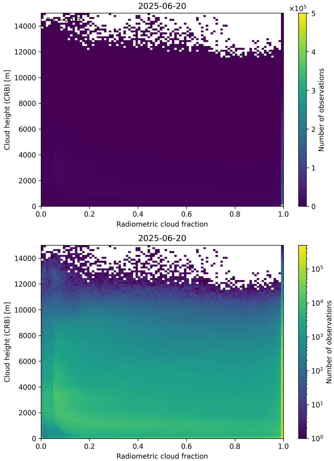
Figure 74: Scatter density plot of “Radiometric cloud fraction” against “Cloud height (CRB)” for 2025-06-19 to 2025-06-21.
