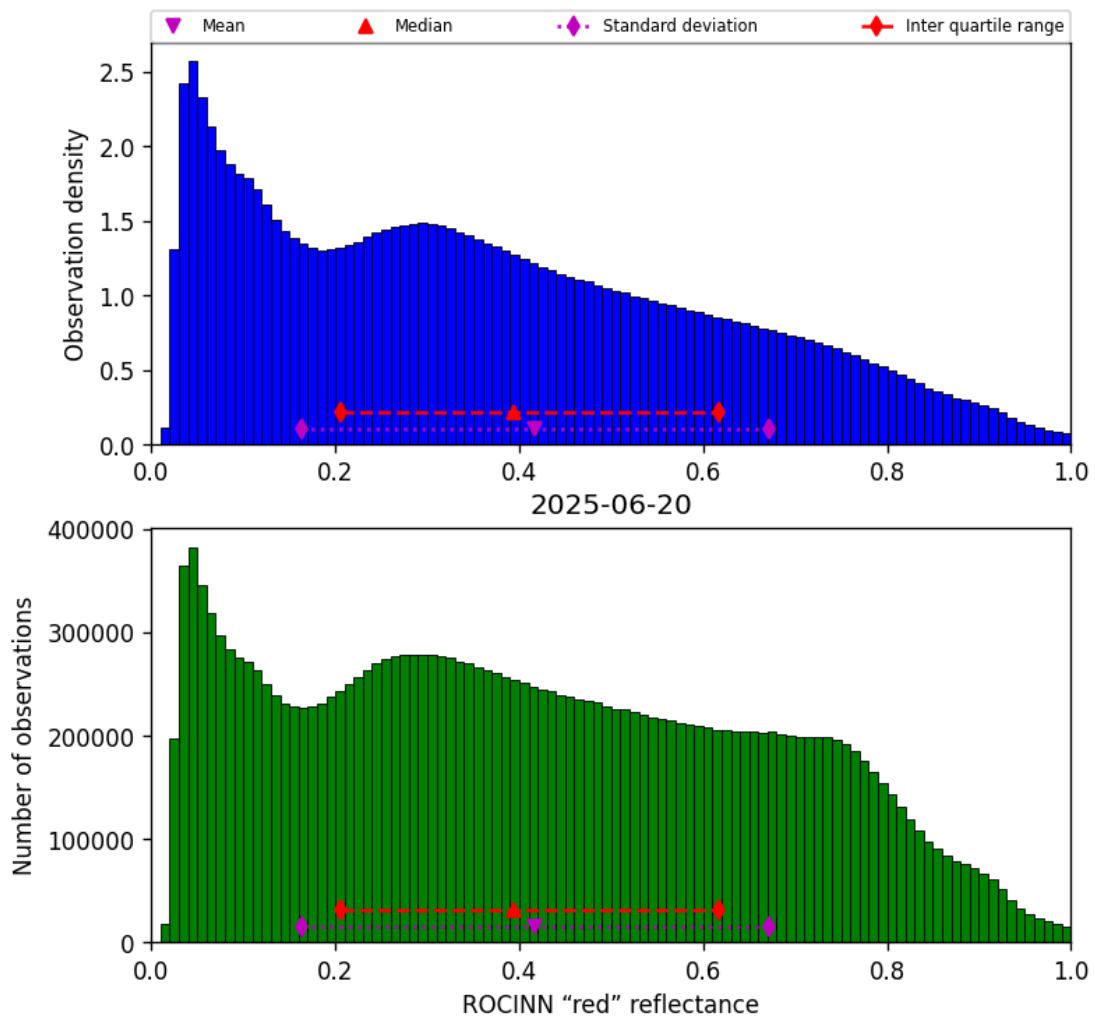
Figure 53: Histogram of “ROCINN “red” reflectance” for 2025-06-19 to 2025-06-21
