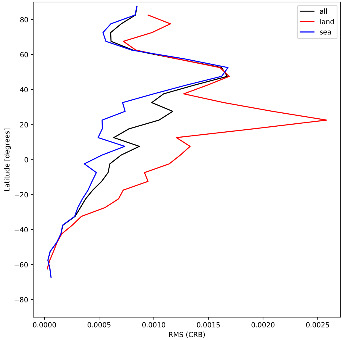
Figure 32: Zonal average of “RMS (CRB)” for 2025-06-19 to 2025-06-21.
