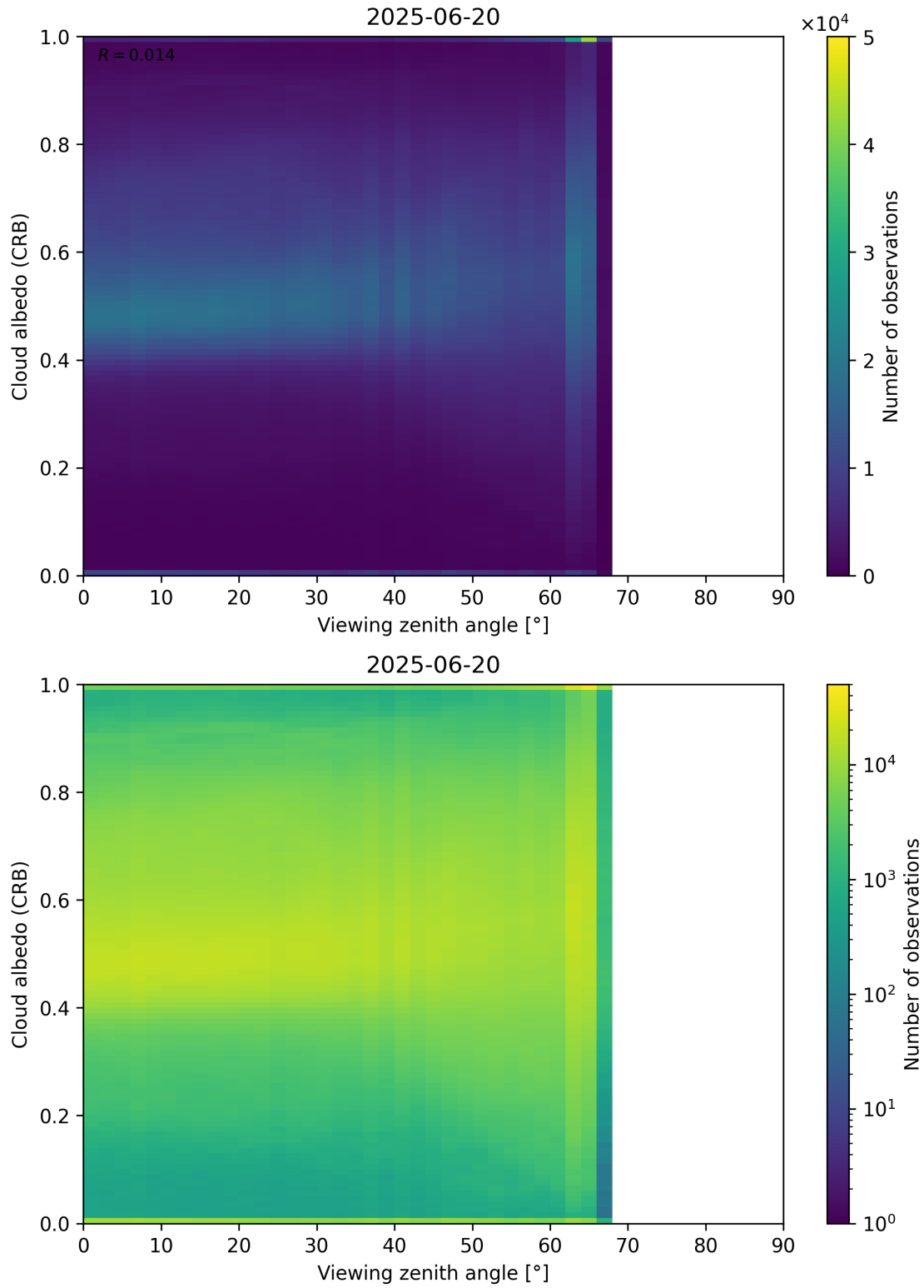
Figure 106: Scatter density plot of “Viewing zenith angle” against “Cloud albedo (CRB)” for 2025-06-19 to 2025-06-21.
