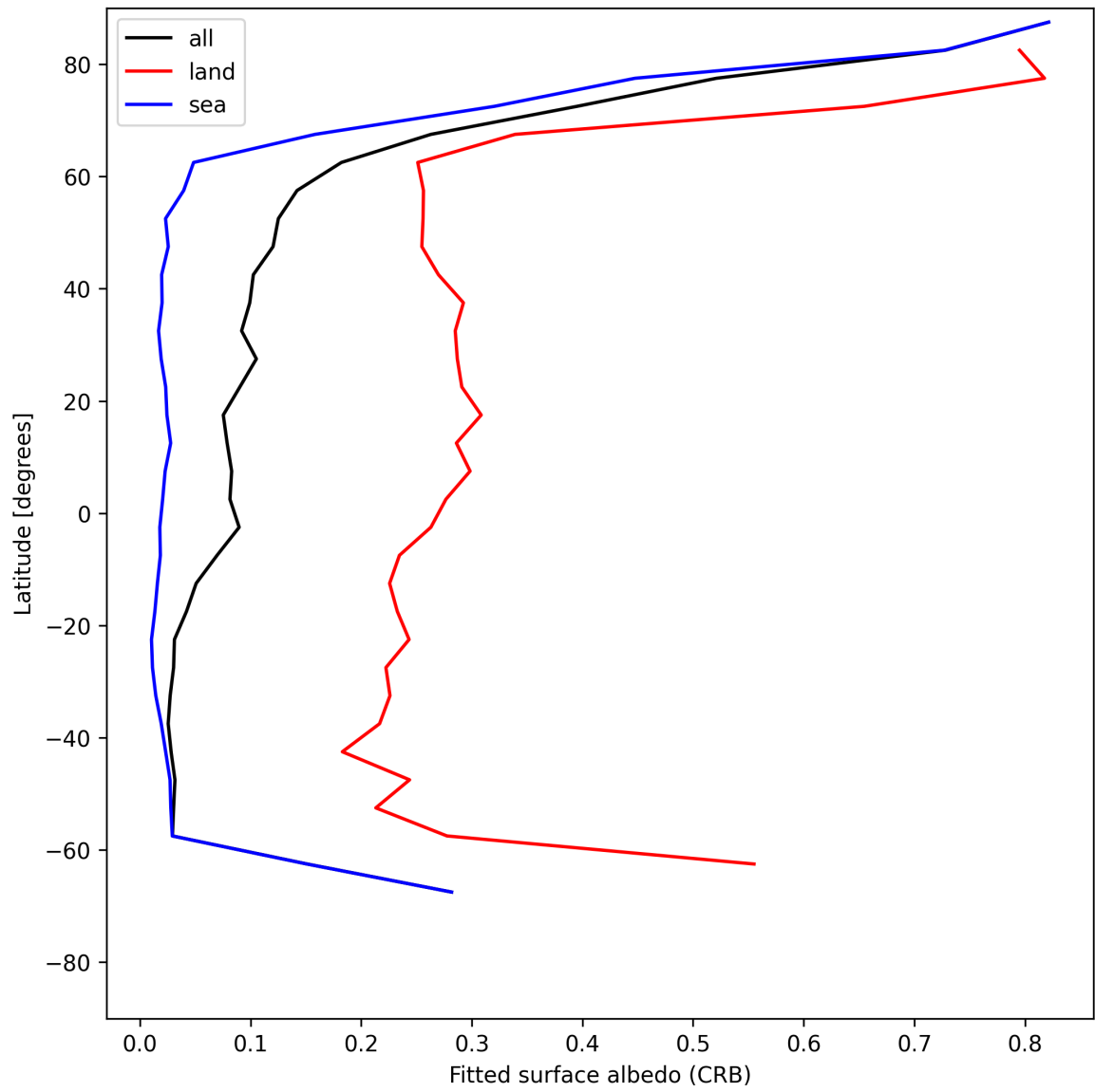
Figure 30: Zonal average of “Fitted surface albedo (CRB)” for 2025-06-19 to 2025-06-21.
