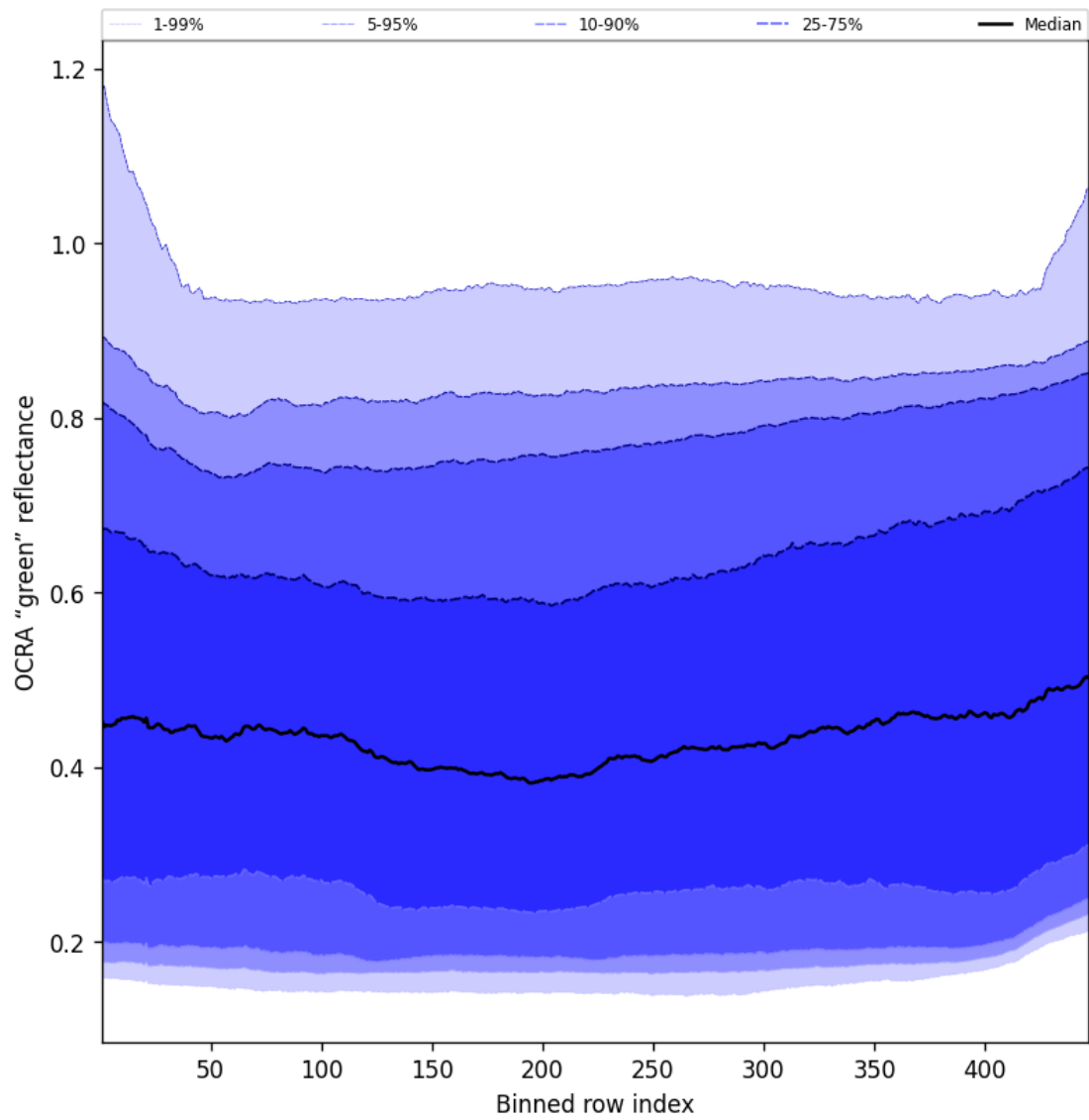
Figure 68: Along track statistics of "OCRA "green" reflectance" for 2025-06-19 to 2025-06-21
