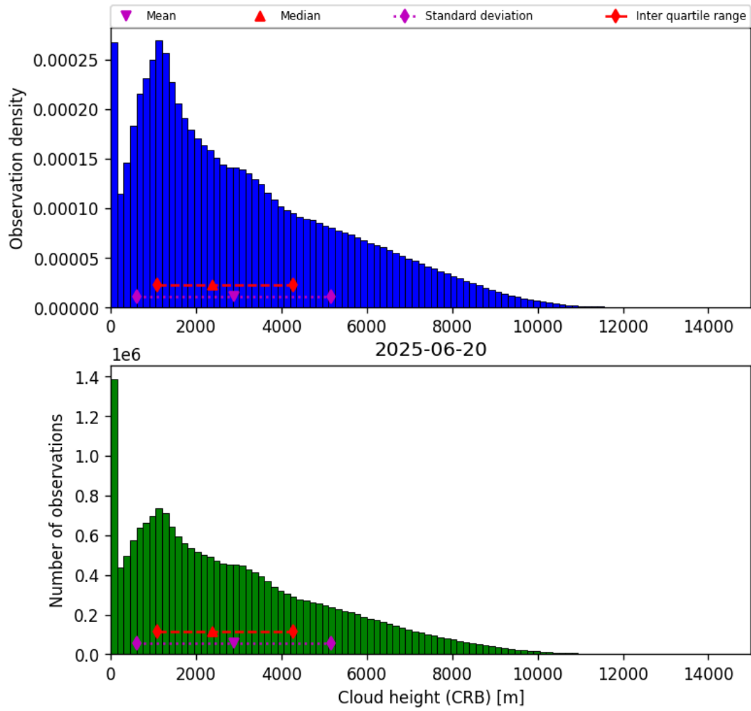
Figure 43: Histogram of “Cloud height (CRB)” for 2025-06-19 to 2025-06-21
