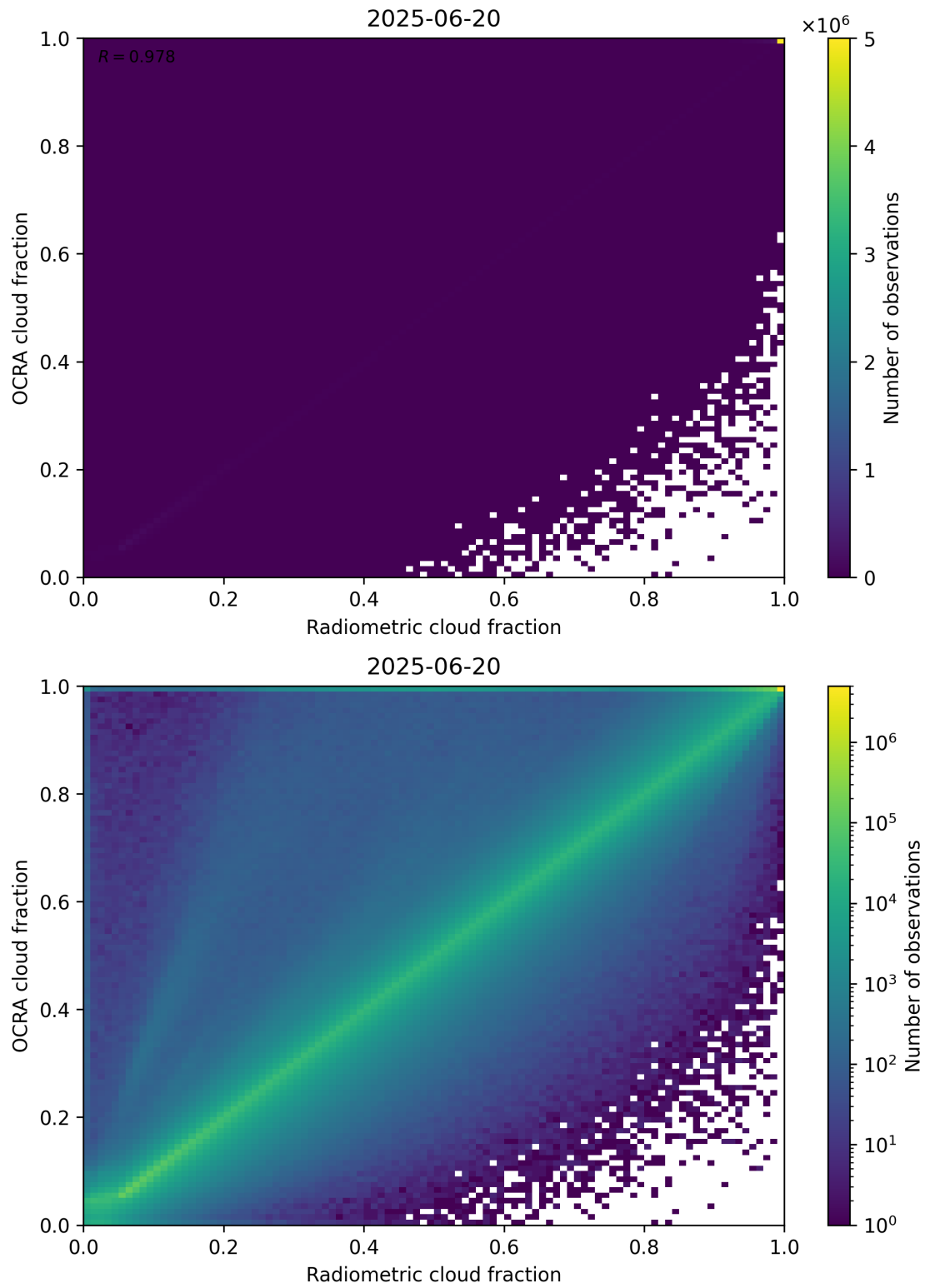
Figure 72: Scatter density plot of “Radiometric cloud fraction” against “OCRA cloud fraction” for 2025-06-19 to 2025-06-21.
