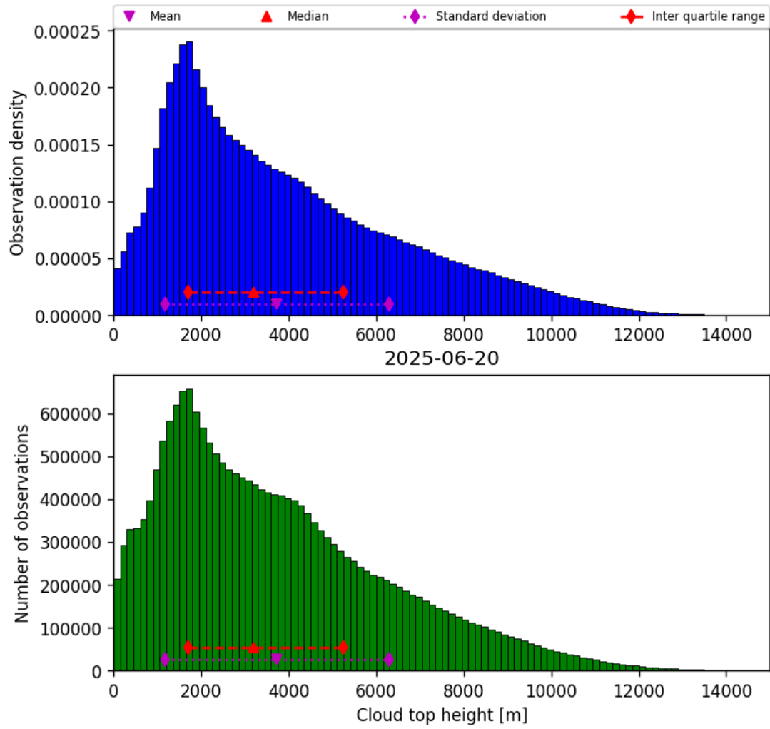
Figure 40: Histogram of “Cloud top height” for 2025-06-19 to 2025-06-21
