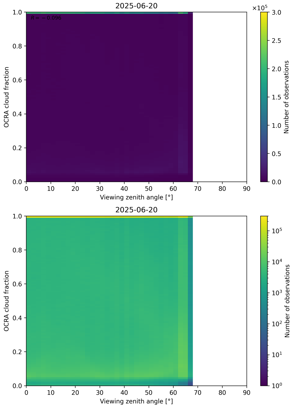
Figure 108: Scatter density plot of “Viewing zenith angle” against “OCRA cloud fraction” for 2025-06-19 to 2025-06-21.
