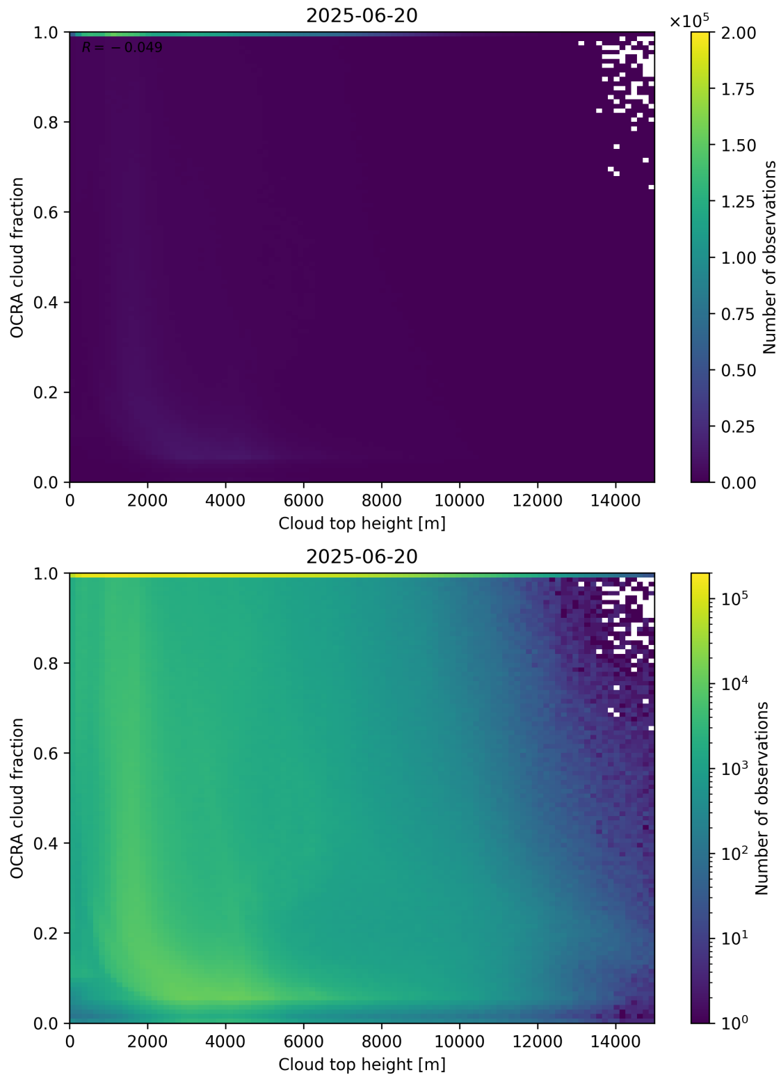
Figure 87: Scatter density plot of “Cloud top height” against “OCRA cloud fraction” for 2025-06-19 to 2025-06-21.
