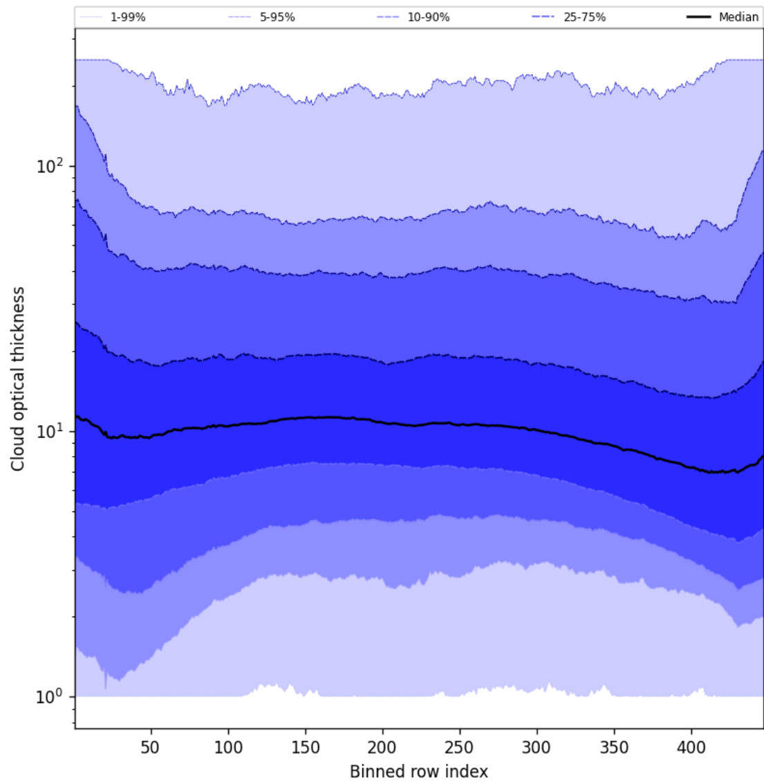
Figure 57: Along track statistics of “Cloud optical thickness” for 2025-06-19 to 2025-06-21
