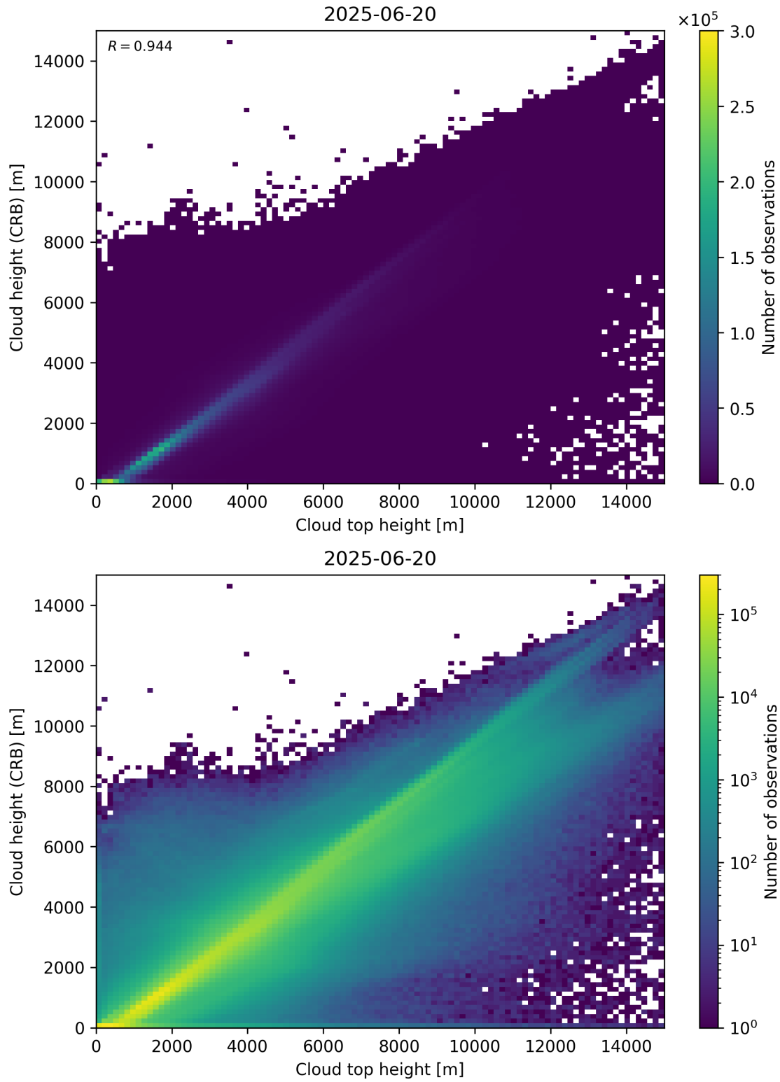
Figure 89: Scatter density plot of “Cloud top height” against “Cloud height (CRB)” for 2025-06-19 to 2025-06-21.
