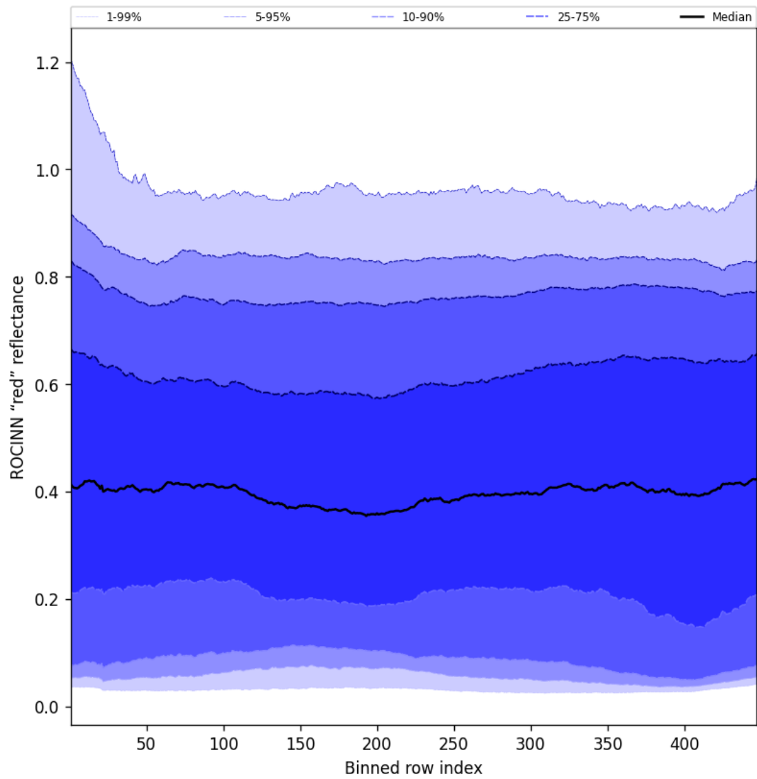
Figure 69: Along track statistics of "ROCINN "red" reflectance" for 2025-06-19 to 2025-06-21
