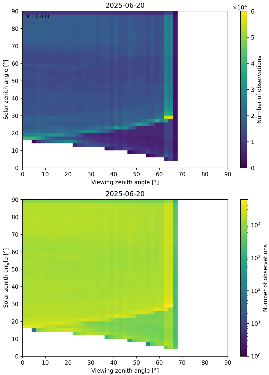
Figure 114: Scatter density plot of “Viewing zenith angle” against “Solar zenith angle” for 2025-06-19 to 2025-06-21.
