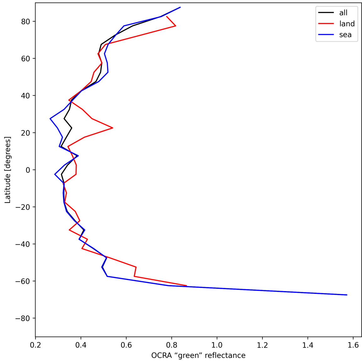
Figure 36: Zonal average of “OCRA “green” reflectance” for 2025-06-19 to 2025-06-21.
