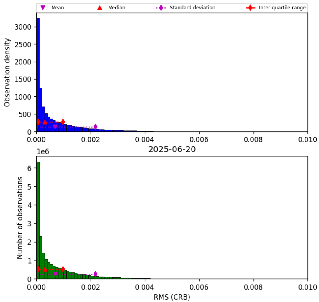
Figure 48: Histogram of “RMS (CRB)” for 2025-06-19 to 2025-06-21
