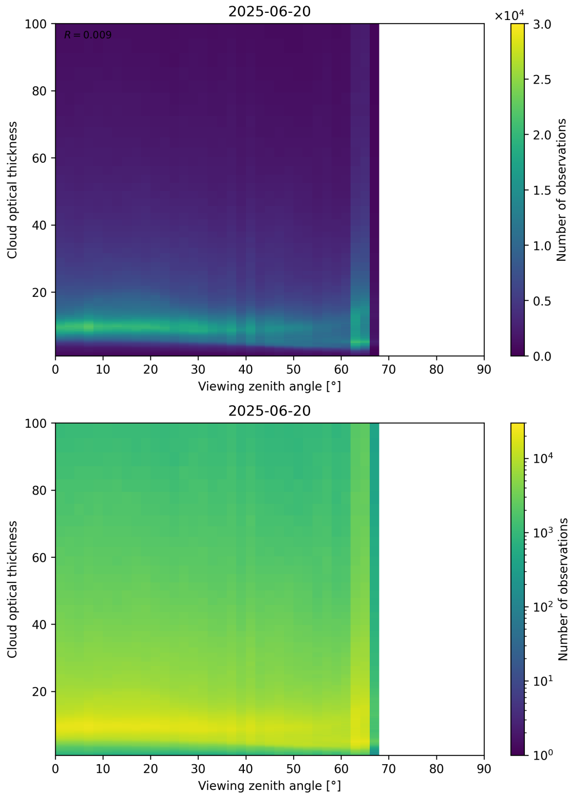
Figure 111: Scatter density plot of “Viewing zenith angle” against “Cloud optical thickness” for 2025-06-19 to 2025-06-21.
