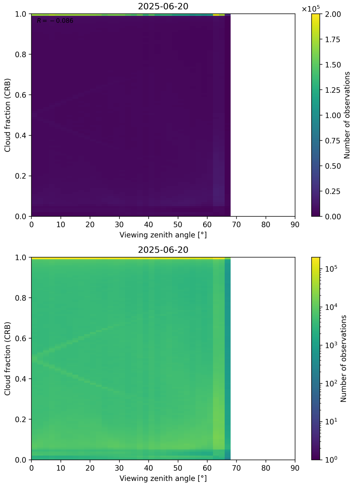
Figure 109: Scatter density plot of “Viewing zenith angle” against “Cloud fraction (CRB)” for 2025-06-19 to 2025-06-21.
