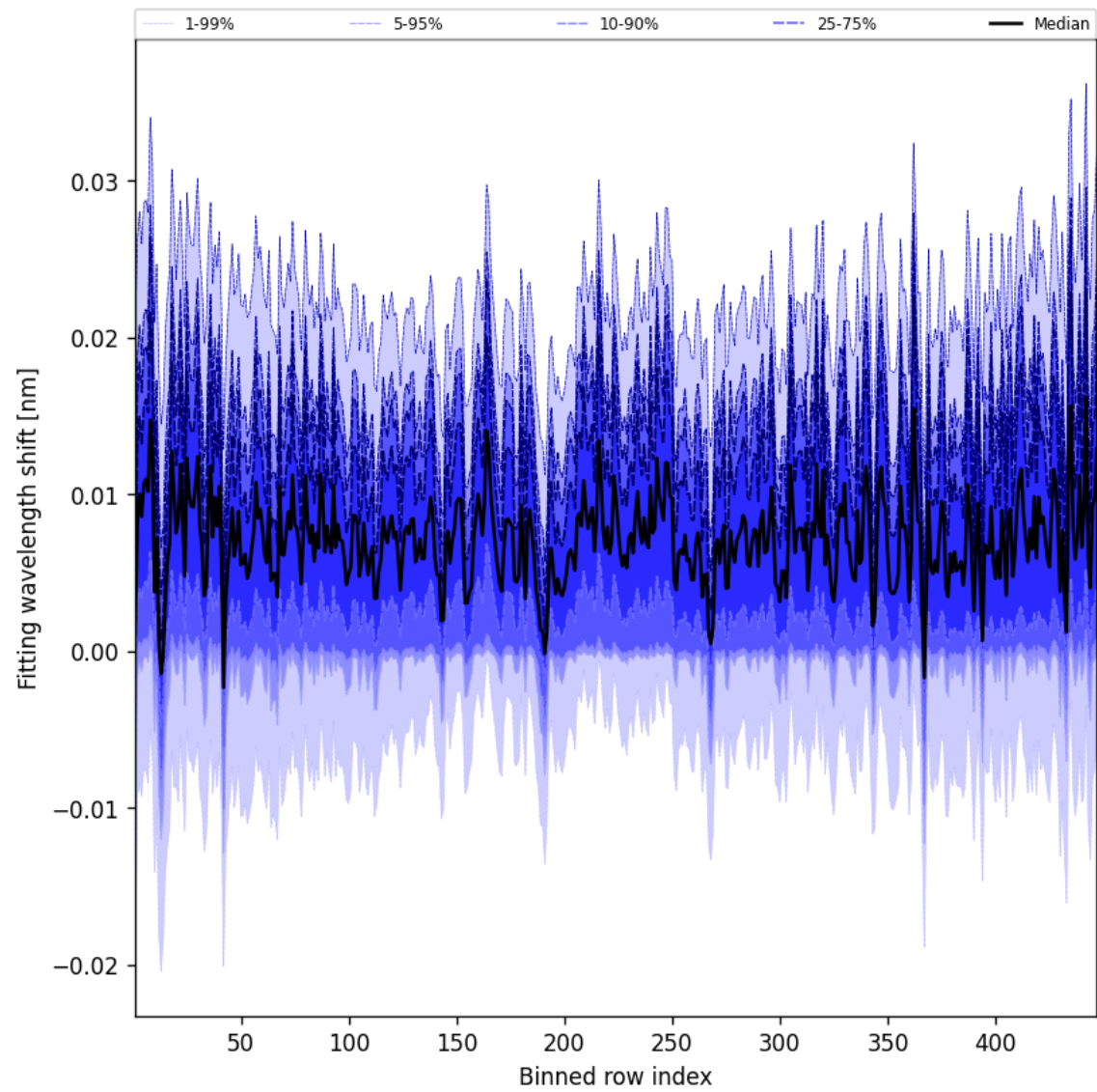
Figure 65: Along track statistics of “Fitting wavelength shift” for 2025-06-19 to 2025-06-21
