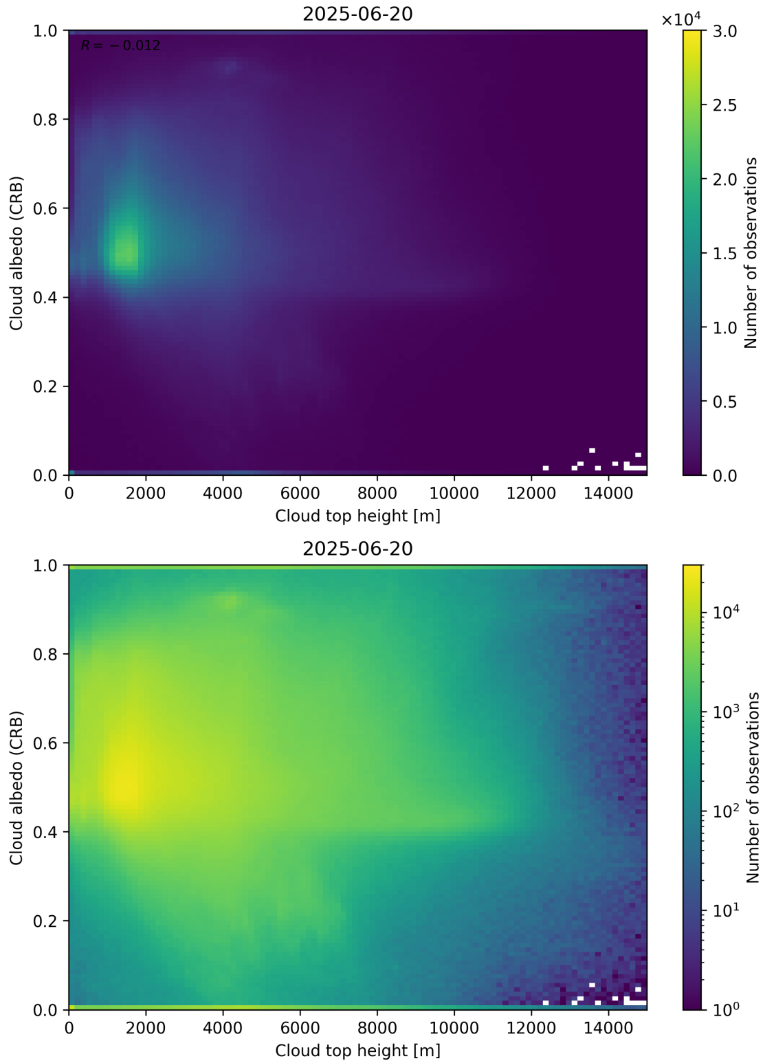
Figure 86: Scatter density plot of “Cloud top height” against “Cloud albedo (CRB)” for 2025-06-19 to 2025-06-21.
