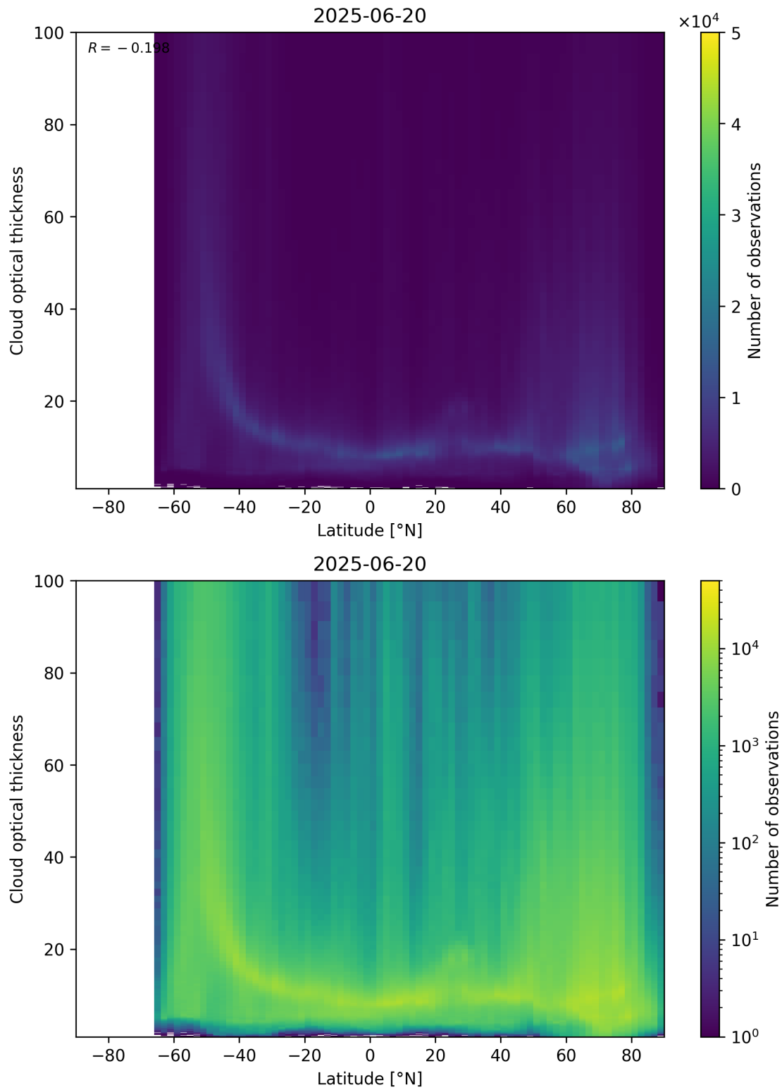
Figure 96: Scatter density plot of “Latitude” against “Cloud optical thickness” for 2025-06-19 to 2025-06-21.
