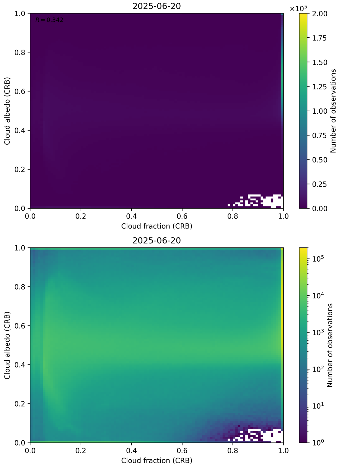
Figure 77: Scatter density plot of “Cloud fraction (CRB)” against “Cloud albedo (CRB)” for 2025-06-19 to 2025-06-21.
