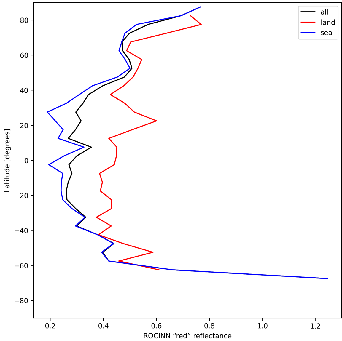
Figure 37: Zonal average of "ROCINN "red" reflectance" for 2025-06-19 to 2025-06-21.
