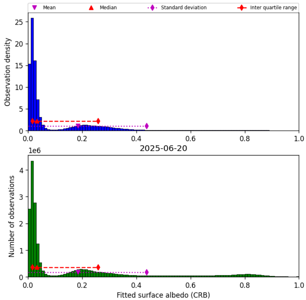
Figure 46: Histogram of “Fitted surface albedo (CRB)” for 2025-06-19 to 2025-06-21
