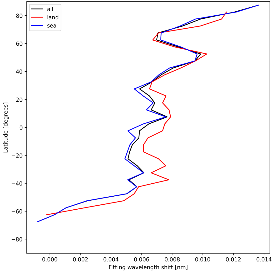
Figure 33: Zonal average of “Fitting wavelength shift” for 2025-06-19 to 2025-06-21.
