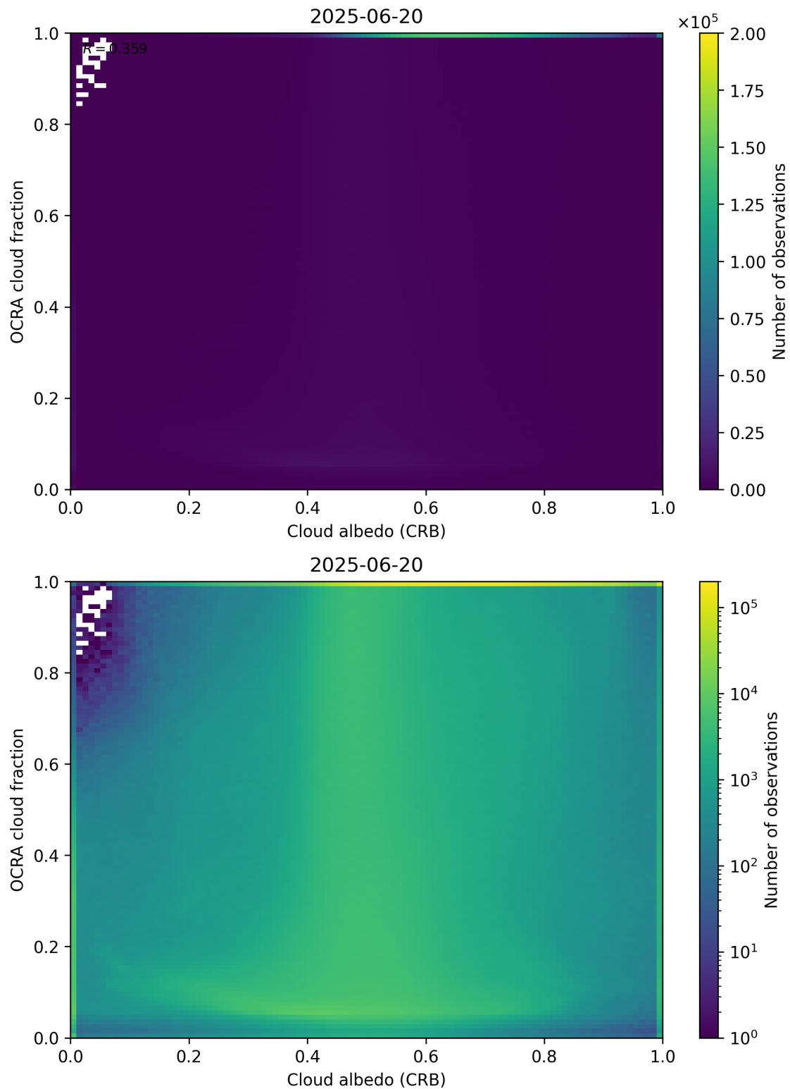
Figure 70: Scatter density plot of “Cloud albedo (CRB)” against “OCRA cloud fraction” for 2025-06-19 to 2025-06-21.
