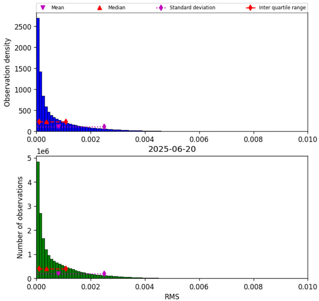
Figure 47: Histogram of “RMS” for 2025-06-19 to 2025-06-21
