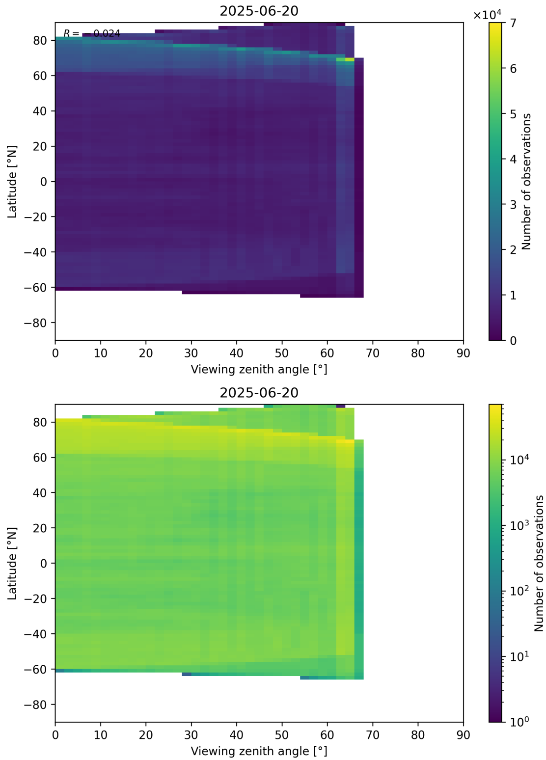
Figure 113: Scatter density plot of “Viewing zenith angle” against “Latitude” for 2025-06-19 to 2025-06-21.
