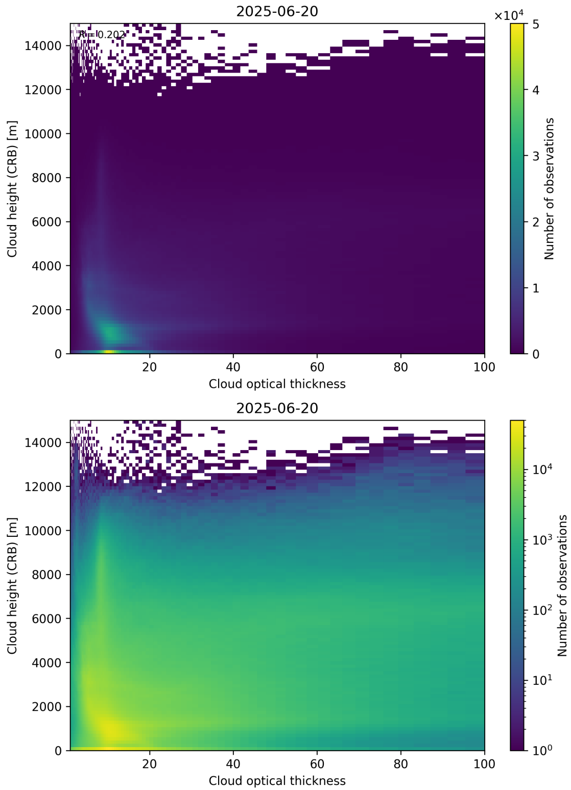
Figure 85: Scatter density plot of “Cloud optical thickness” against “Cloud height (CRB)” for 2025-06-19 to 2025-06-21.
