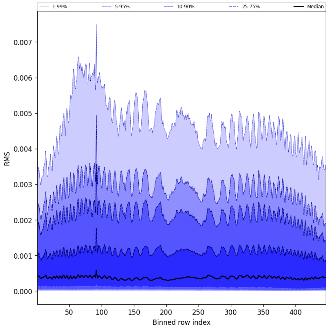
Figure 63: Along track statistics of “RMS” for 2025-06-19 to 2025-06-21
