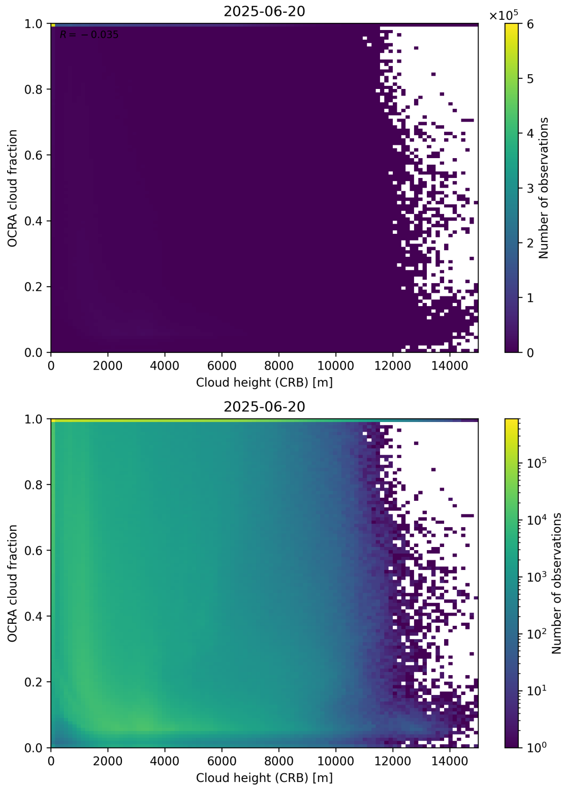
Figure 81: Scatter density plot of “Cloud height (CRB)” against “OCRA cloud fraction” for 2025-06-19 to 2025-06-21.
