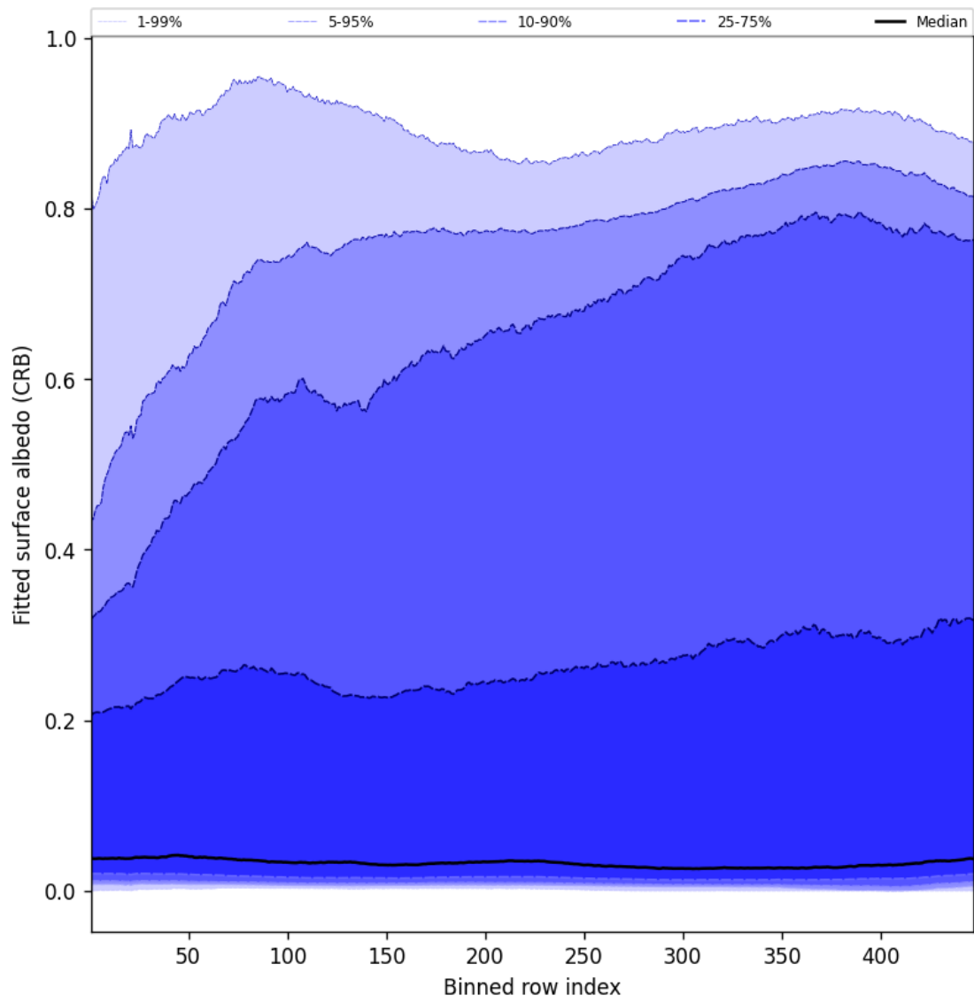
Figure 62: Along track statistics of “Fitted surface albedo (CRB)” for 2025-06-19 to 2025-06-21
