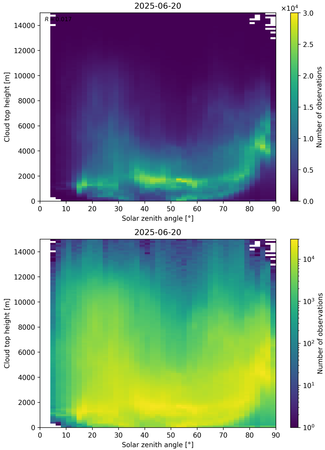
Figure 104: Scatter density plot of “Solar zenith angle” against “Cloud top height” for 2025-06-19 to 2025-06-21.
