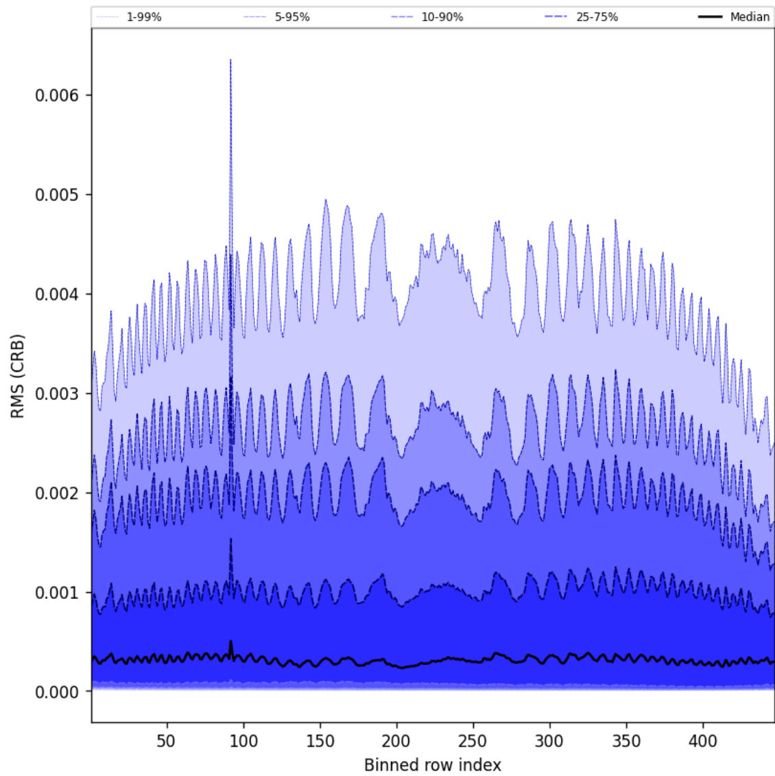
Figure 64: Along track statistics of “RMS (CRB)” for 2025-06-19 to 2025-06-21
