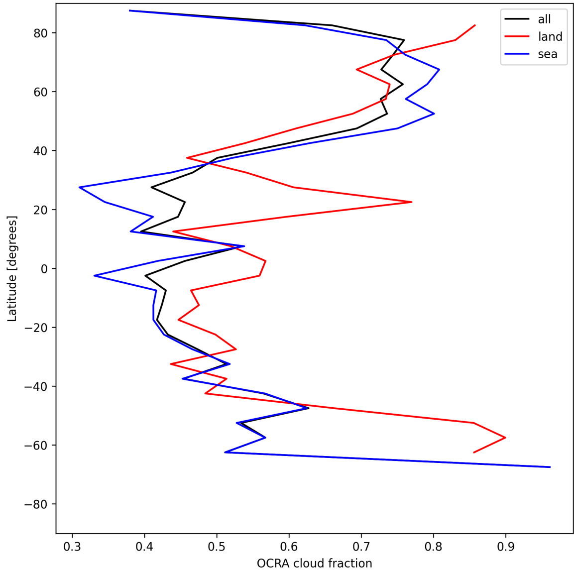
Figure 34: Zonal average of “OCRA cloud fraction” for 2025-06-19 to 2025-06-21.
