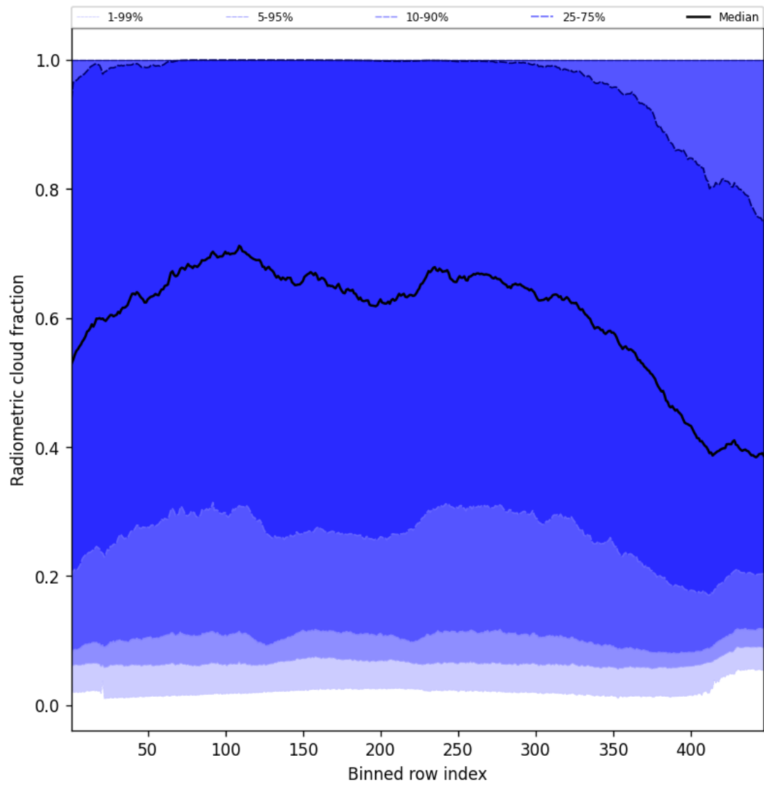
Figure 55: Along track statistics of “Radiometric cloud fraction” for 2025-06-19 to 2025-06-21
