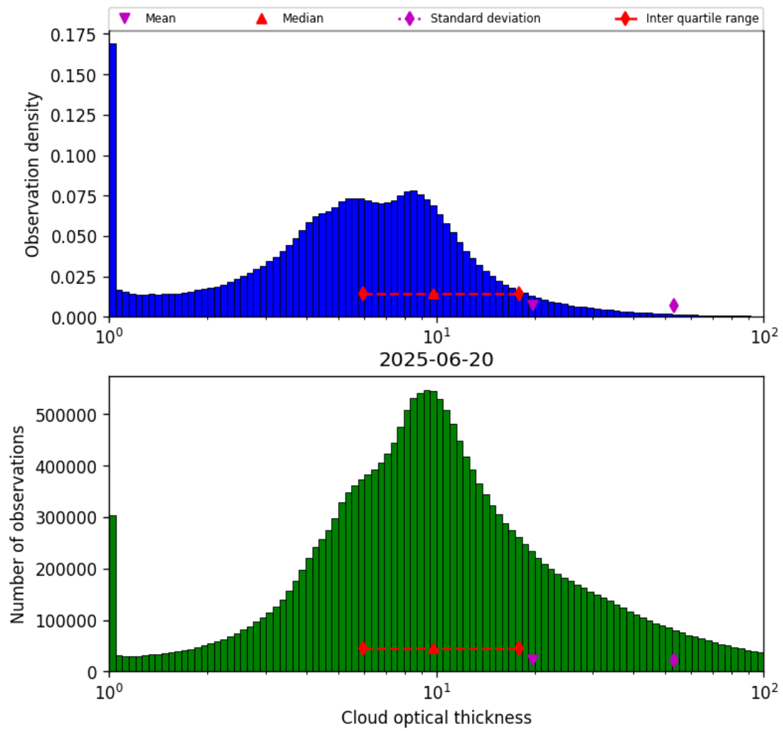
Figure 41: Histogram of “Cloud optical thickness” for 2025-06-19 to 2025-06-21
