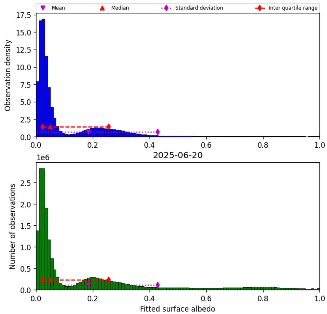
Figure 45: Histogram of “Fitted surface albedo” for 2025-06-19 to 2025-06-21
