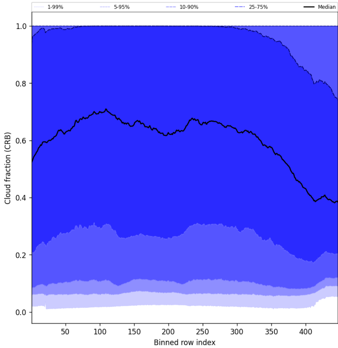
Figure 58: Along track statistics of “Cloud fraction (CRB)” for 2025-06-19 to 2025-06-21
