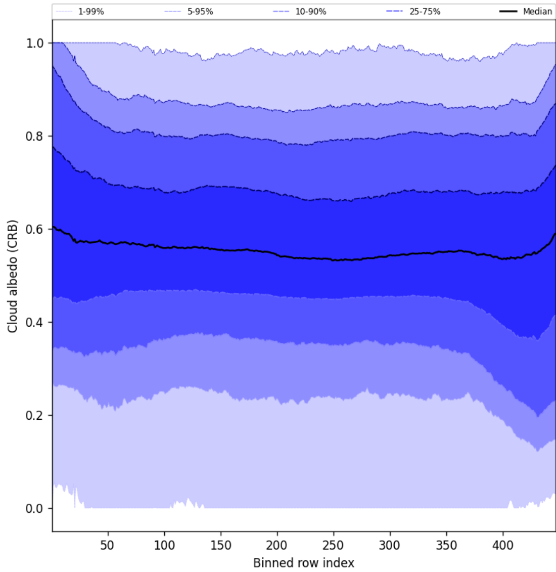
Figure 60: Along track statistics of “Cloud albedo (CRB)” for 2025-06-19 to 2025-06-21
