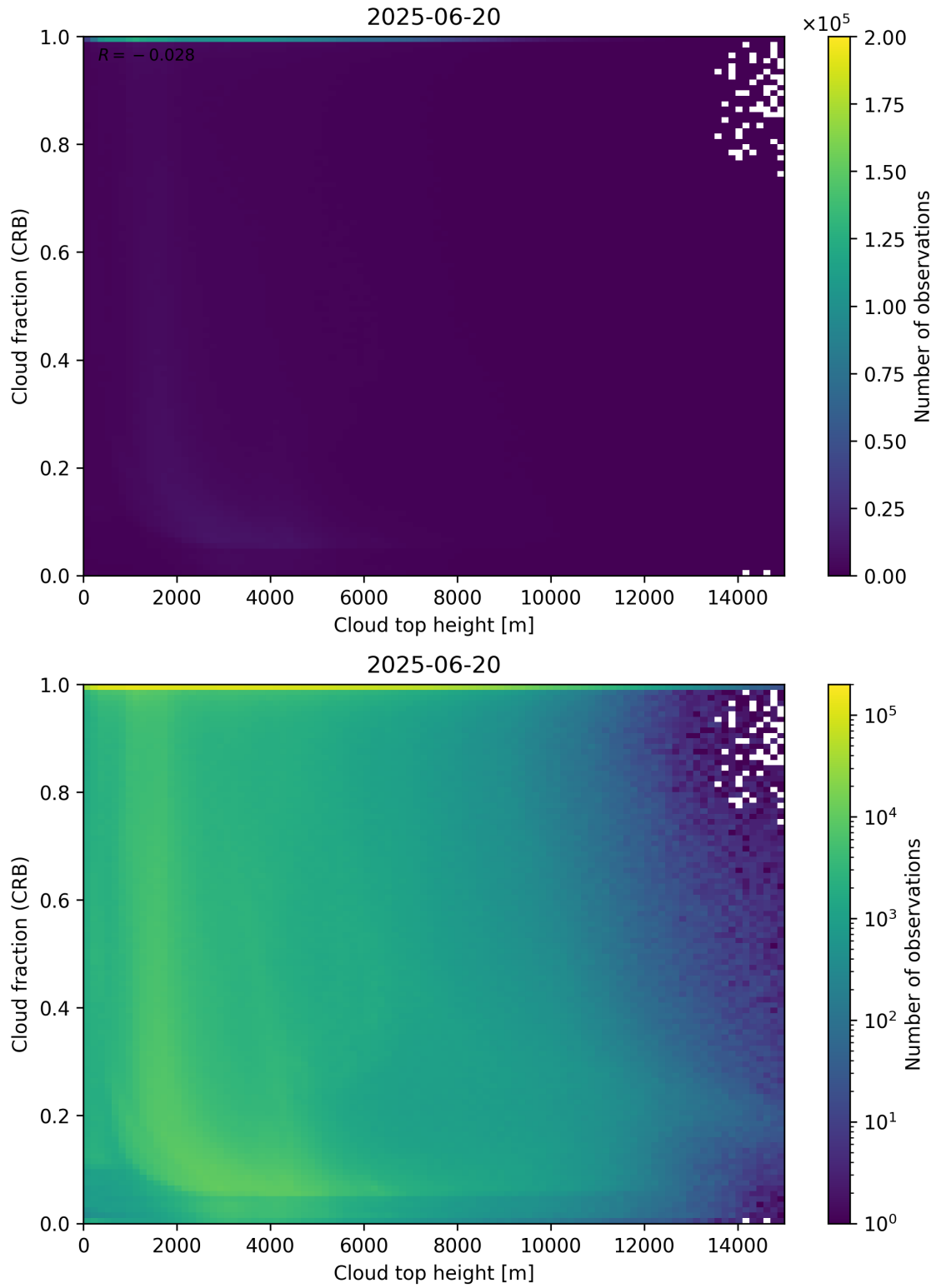
Figure 88: Scatter density plot of “Cloud top height” against “Cloud fraction (CRB)” for 2025-06-19 to 2025-06-21.
