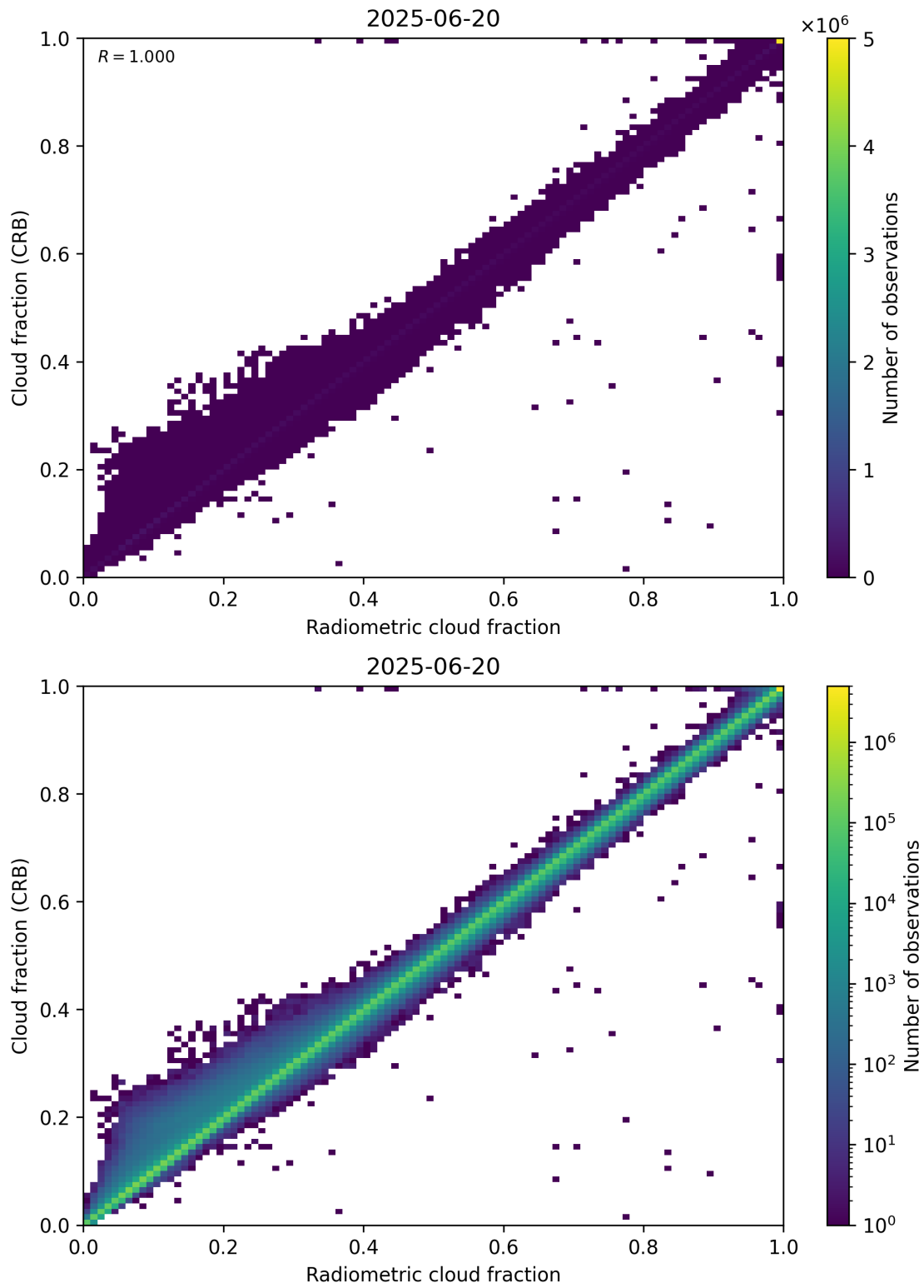
Figure 73: Scatter density plot of “Radiometric cloud fraction” against “Cloud fraction (CRB)” for 2025-06-19 to 2025-06-21.
