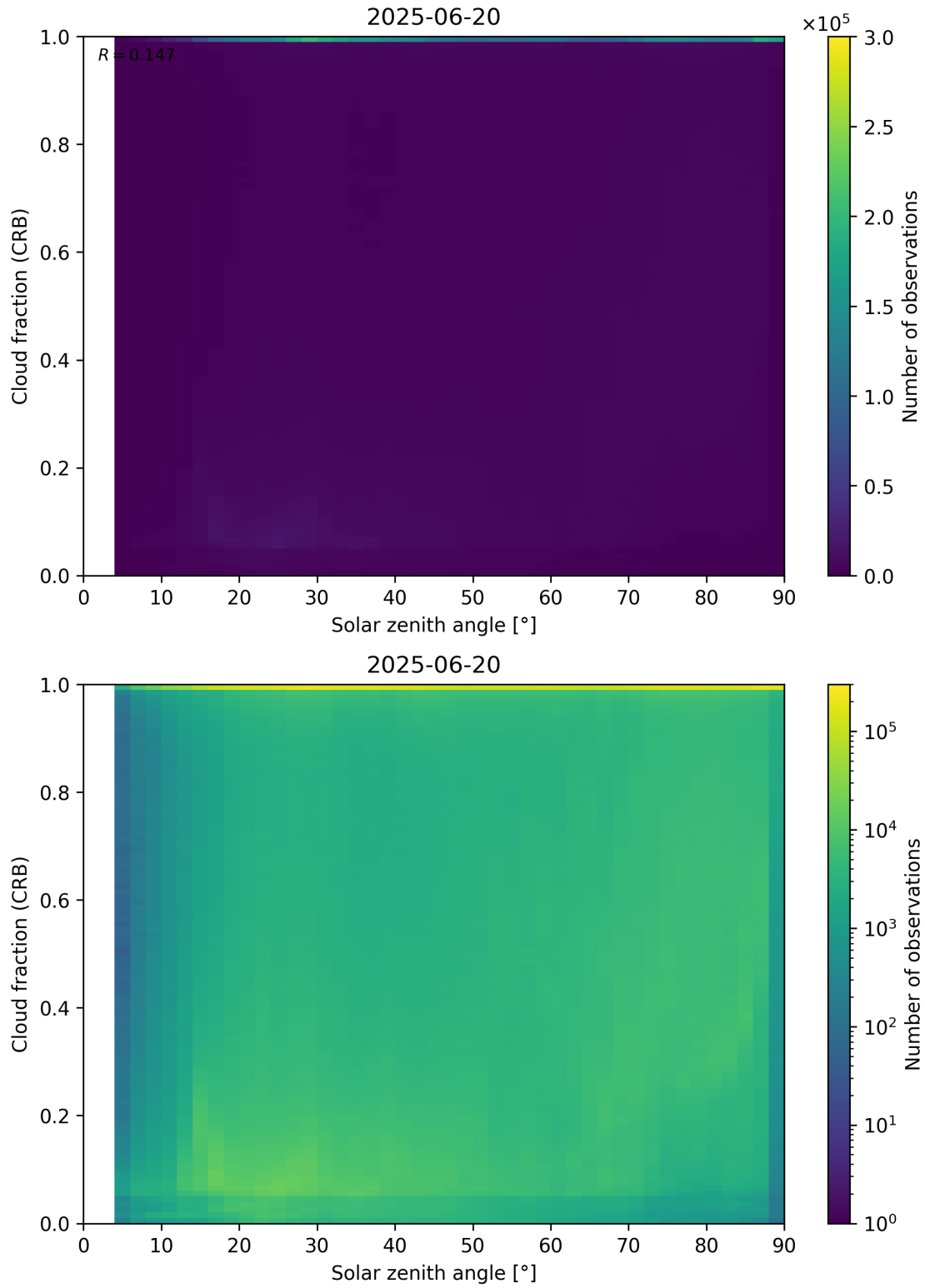
Figure 101: Scatter density plot of “Solar zenith angle” against “Cloud fraction (CRB)” for 2025-06-19 to 2025-06-21.
