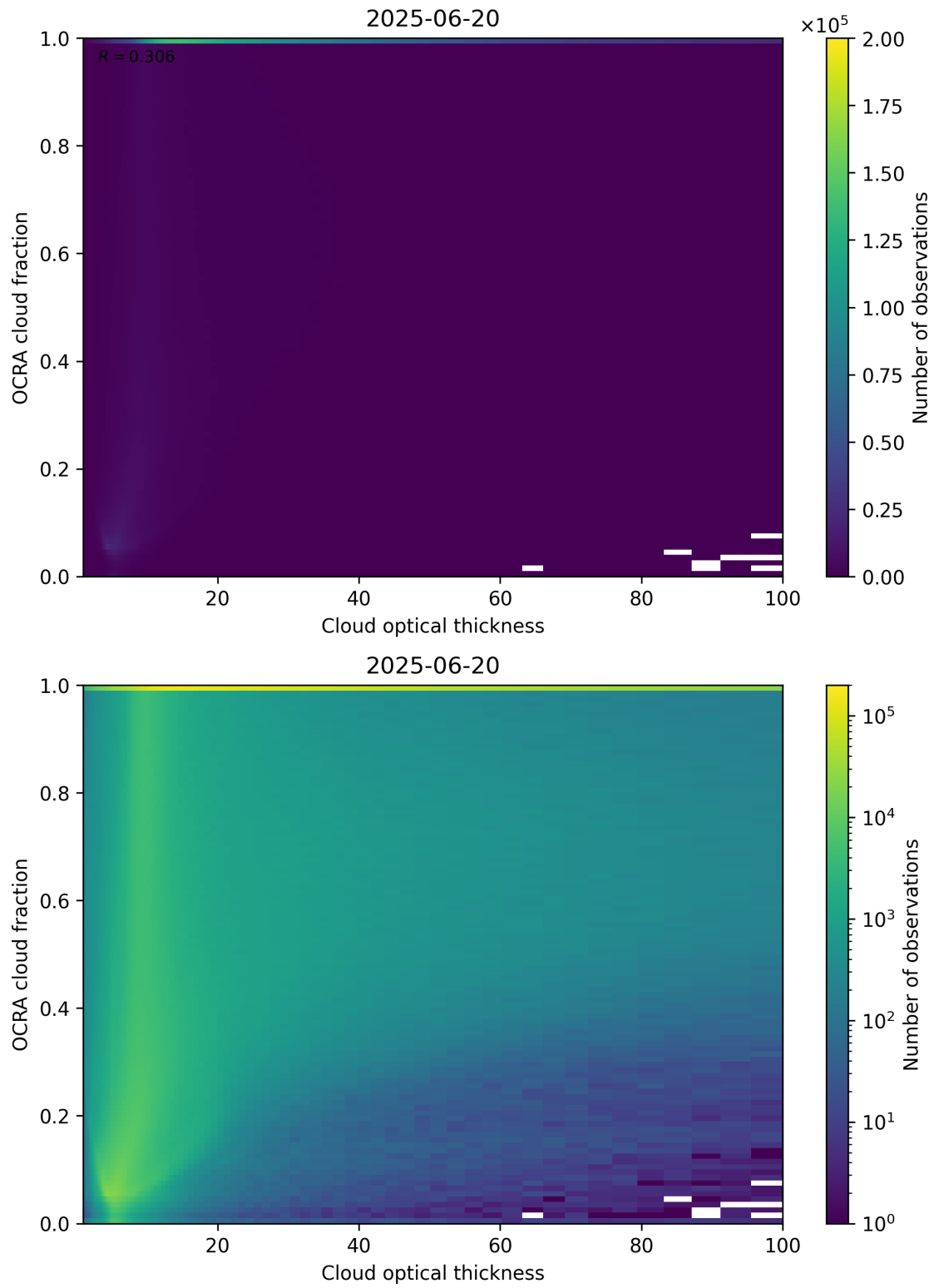
Figure 83: Scatter density plot of “Cloud optical thickness” against “OCRA cloud fraction” for 2025-06-19 to 2025-06-21.
