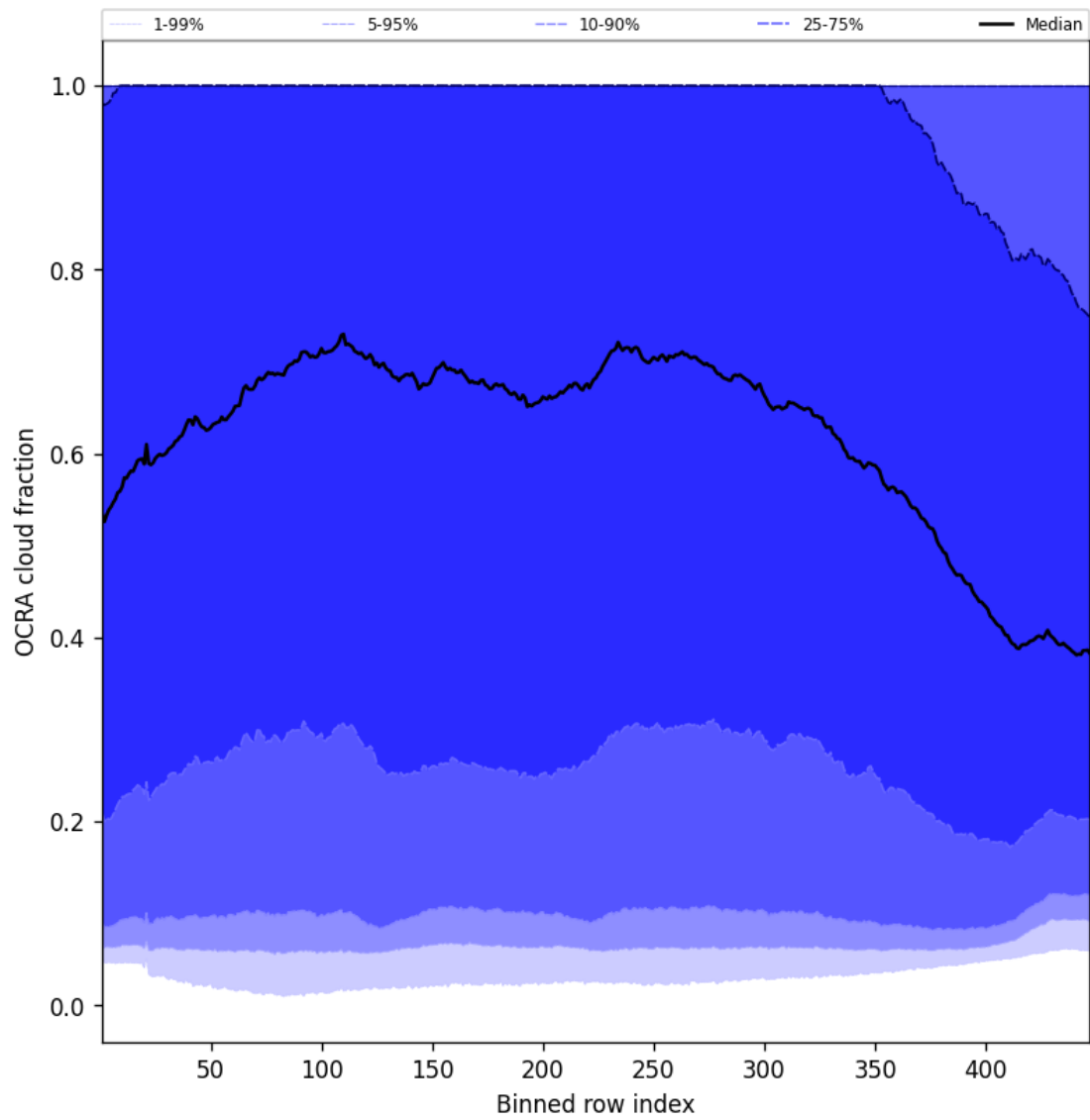
Figure 66: Along track statistics of “OCRA cloud fraction” for 2025-06-19 to 2025-06-21
