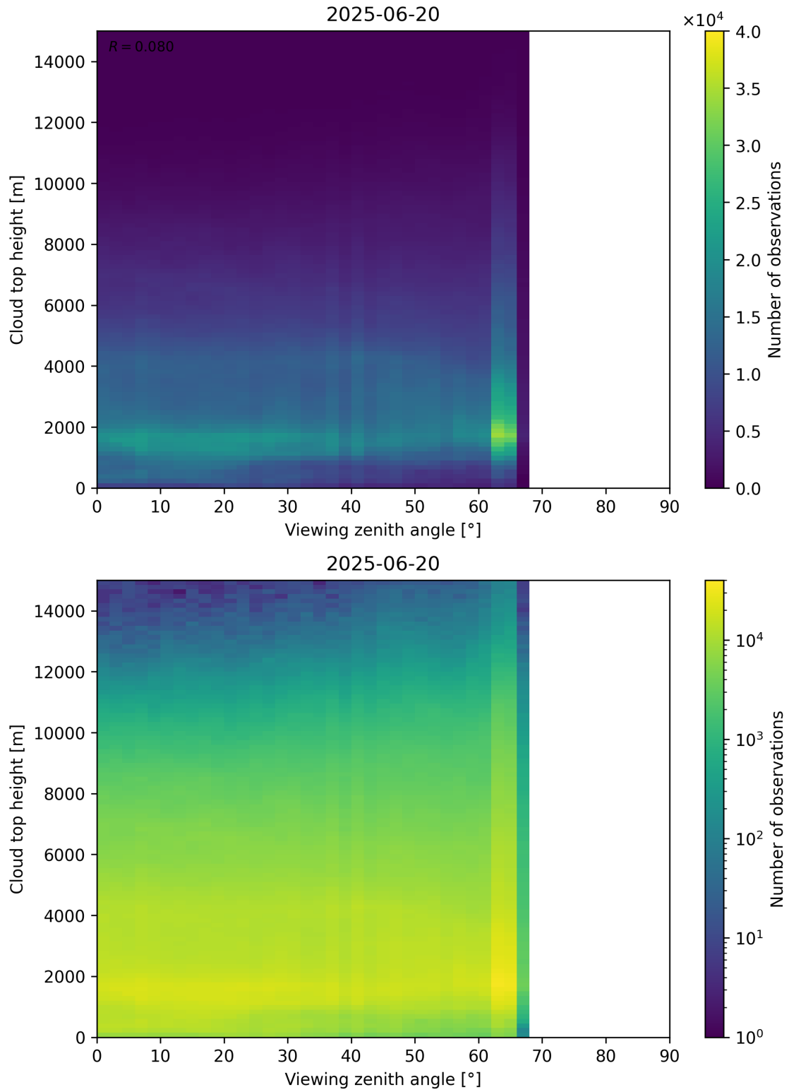
Figure 112: Scatter density plot of “Viewing zenith angle” against “Cloud top height” for 2025-06-19 to 2025-06-21.
