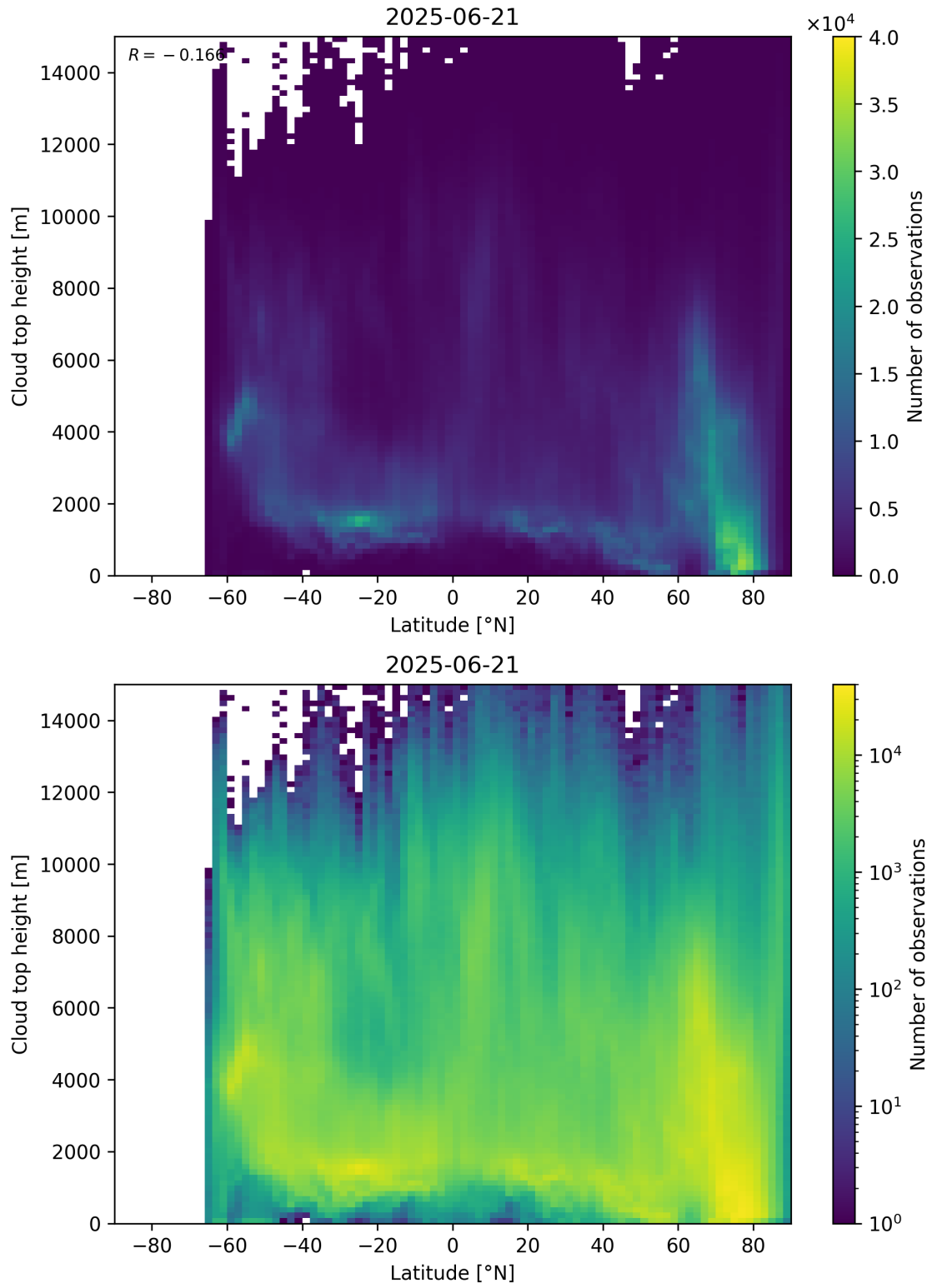
Figure 97: Scatter density plot of “Latitude” against “Cloud top height” for 2025-06-20 to 2025-06-22.
