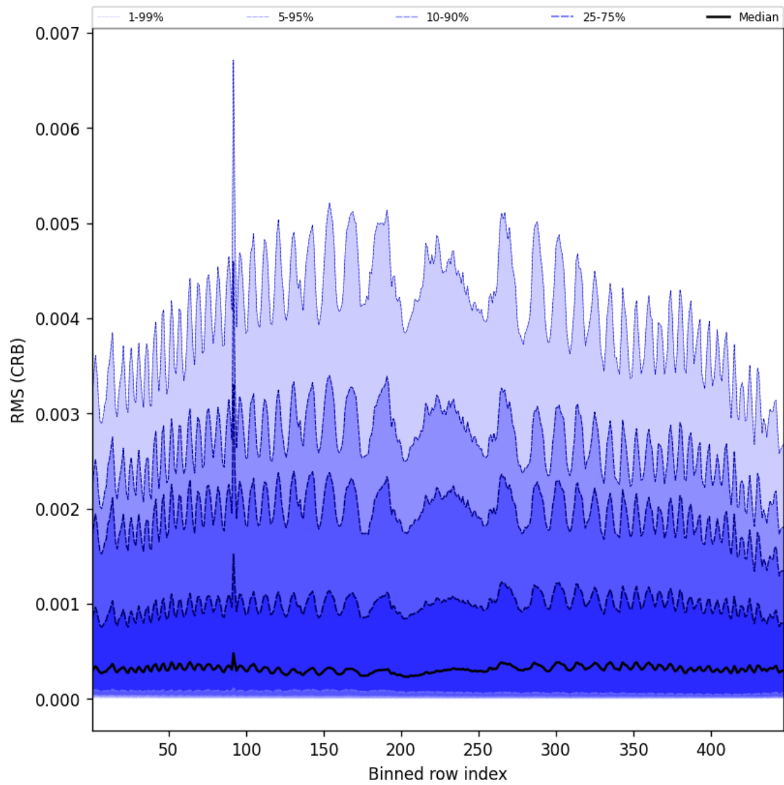
Figure 64: Along track statistics of “RMS (CRB)” for 2025-06-20 to 2025-06-22
