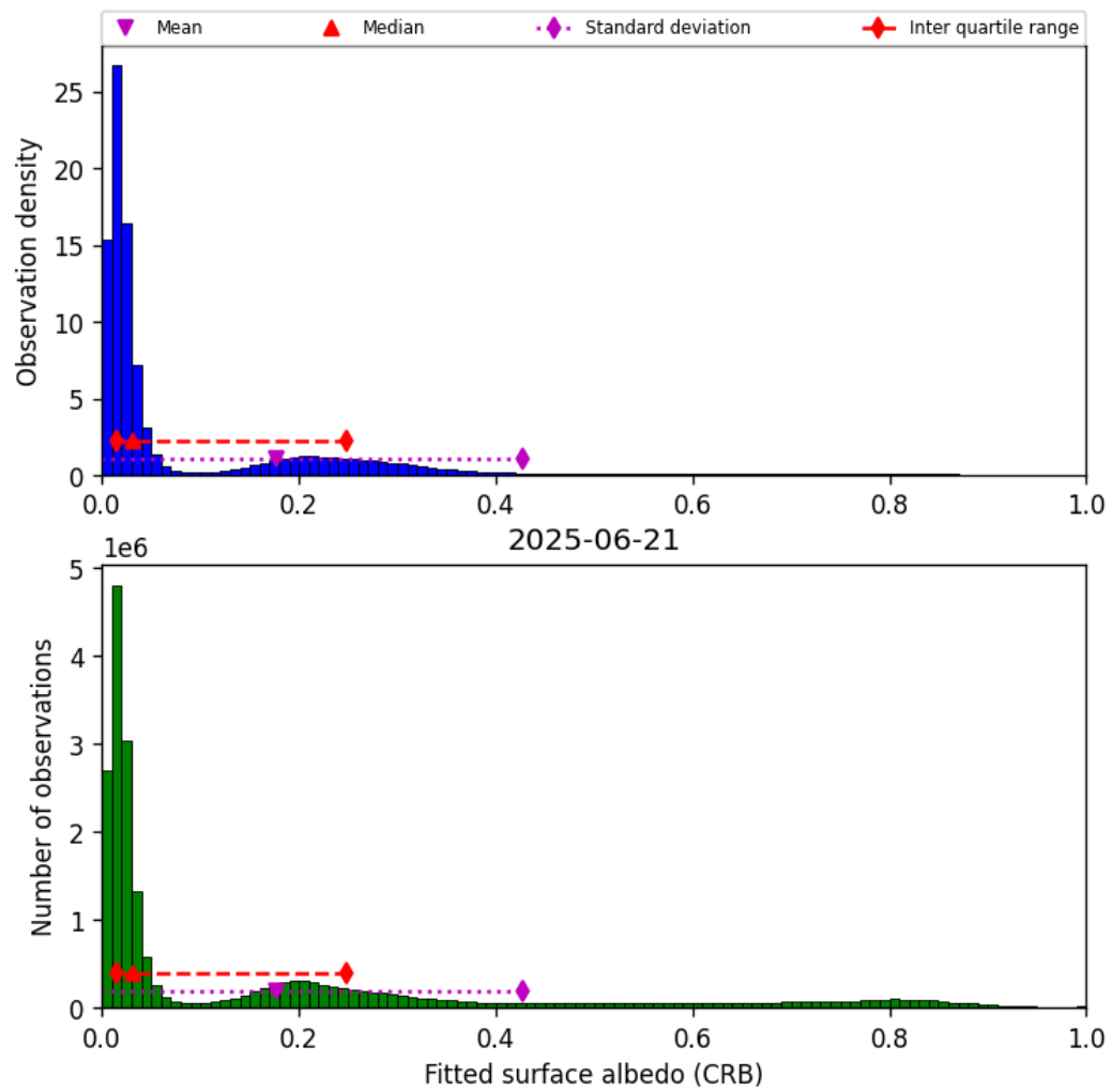
Figure 46: Histogram of “Fitted surface albedo (CRB)” for 2025-06-20 to 2025-06-22
