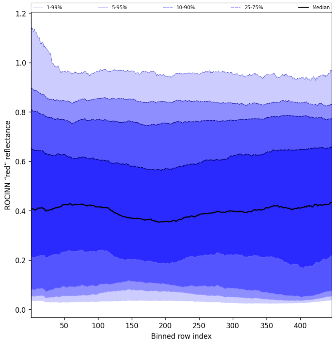
Figure 69: Along track statistics of “ROCINN “red” reflectance” for 2025-06-20 to 2025-06-22
