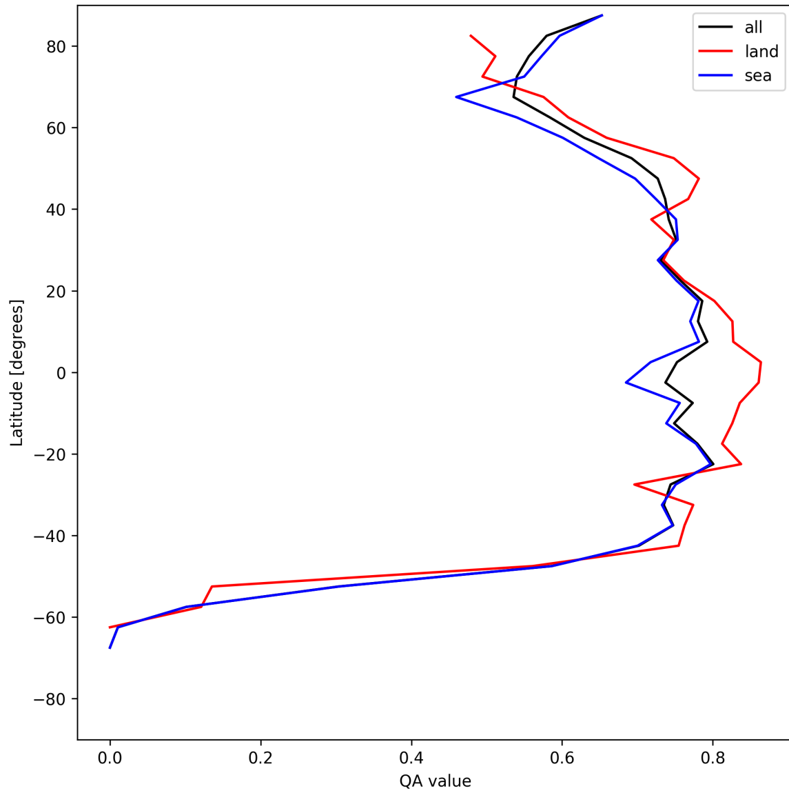
Figure 22: Zonal average of “QA value” for 2025-06-20 to 2025-06-22.
