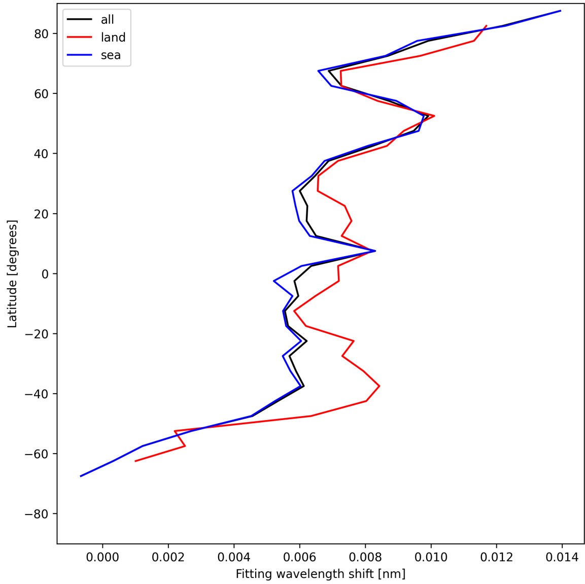
Figure 33: Zonal average of “Fitting wavelength shift” for 2025-06-20 to 2025-06-22.
