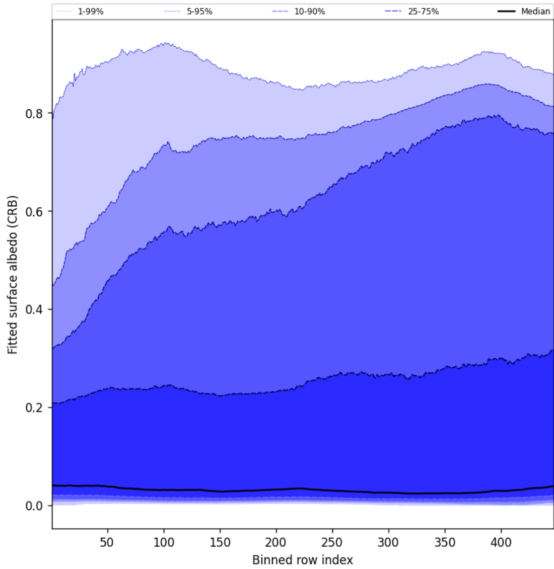
Figure 62: Along track statistics of “Fitted surface albedo (CRB)” for 2025-06-20 to 2025-06-22
