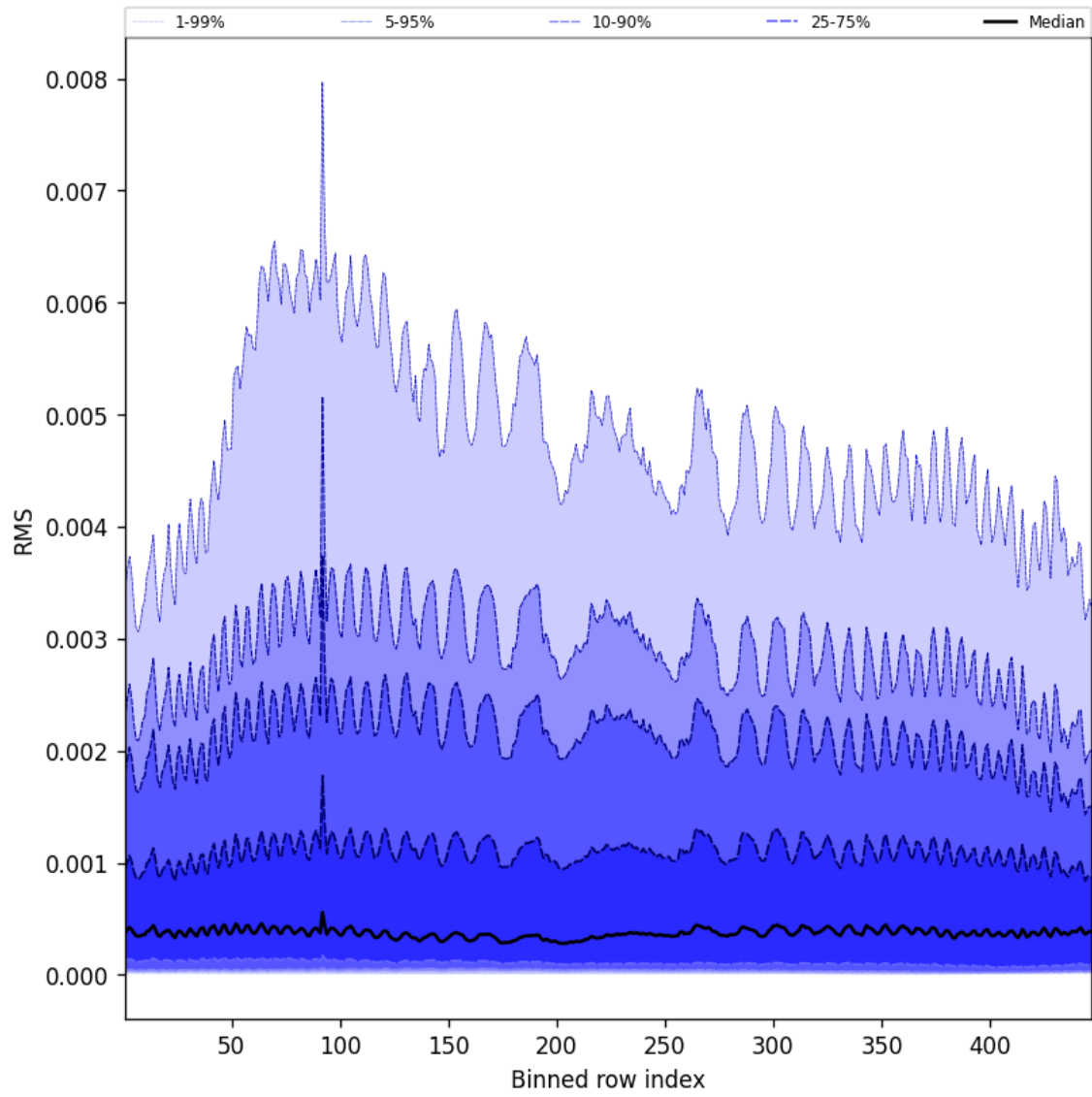
Figure 63: Along track statistics of “RMS” for 2025-06-20 to 2025-06-22
