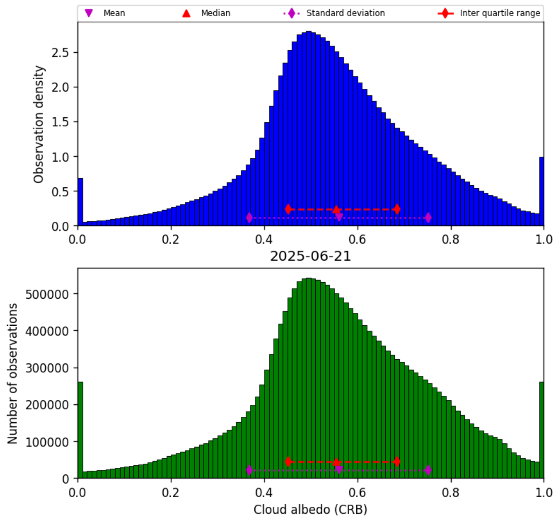
Figure 44: Histogram of “Cloud albedo (CRB)” for 2025-06-20 to 2025-06-22
