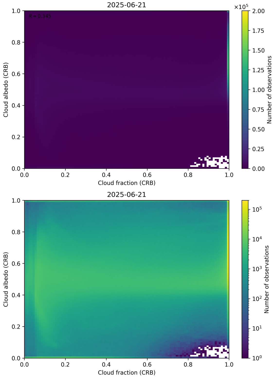
Figure 77: Scatter density plot of “Cloud fraction (CRB)” against “Cloud albedo (CRB)” for 2025-06-20 to 2025-06-22.
