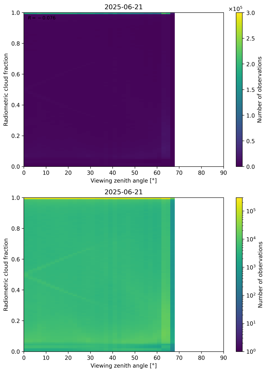
Figure 107: Scatter density plot of “Viewing zenith angle” against “Radiometric cloud fraction” for 2025-06-20 to 2025-06-22.
