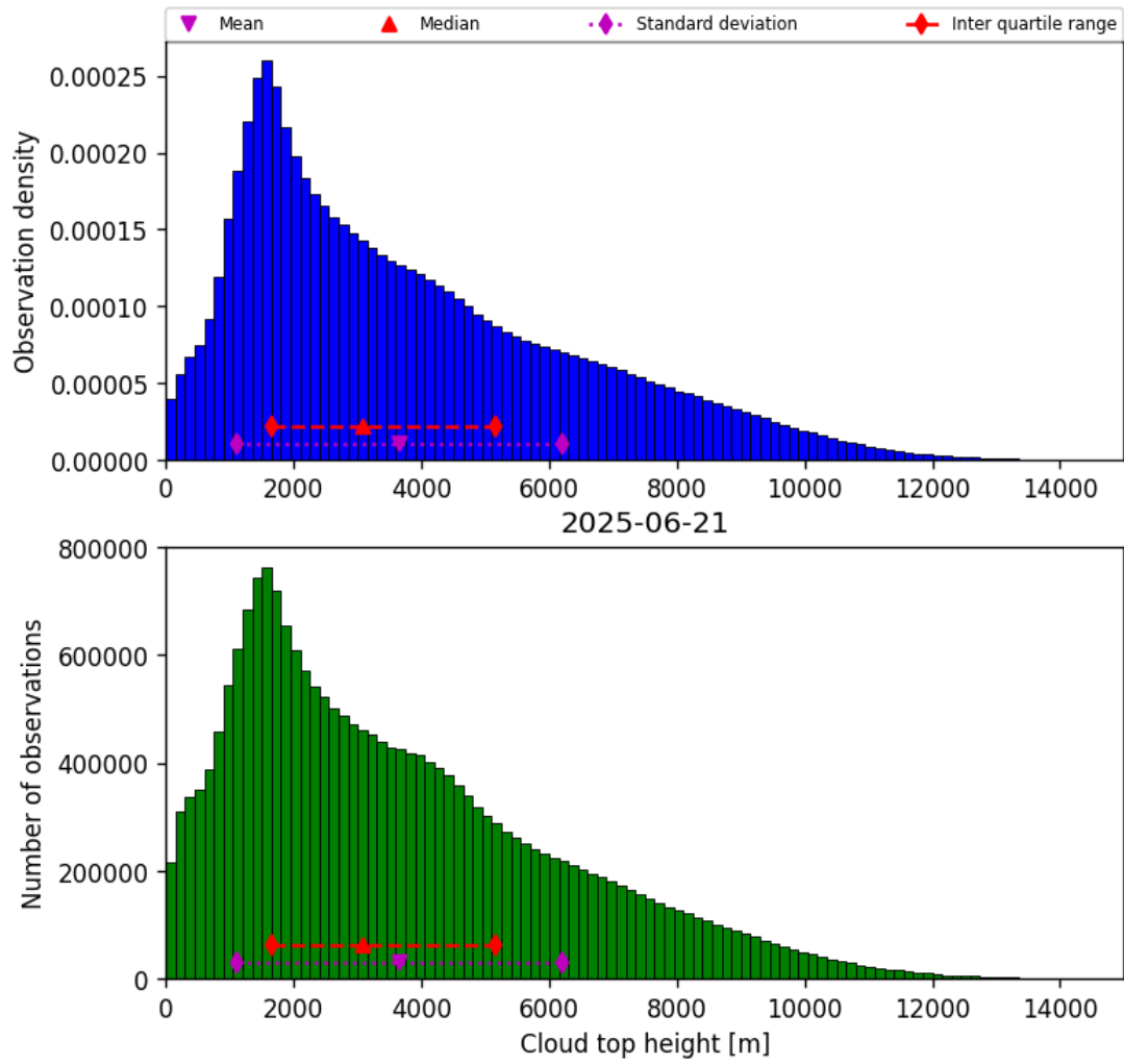
Figure 40: Histogram of “Cloud top height” for 2025-06-20 to 2025-06-22
