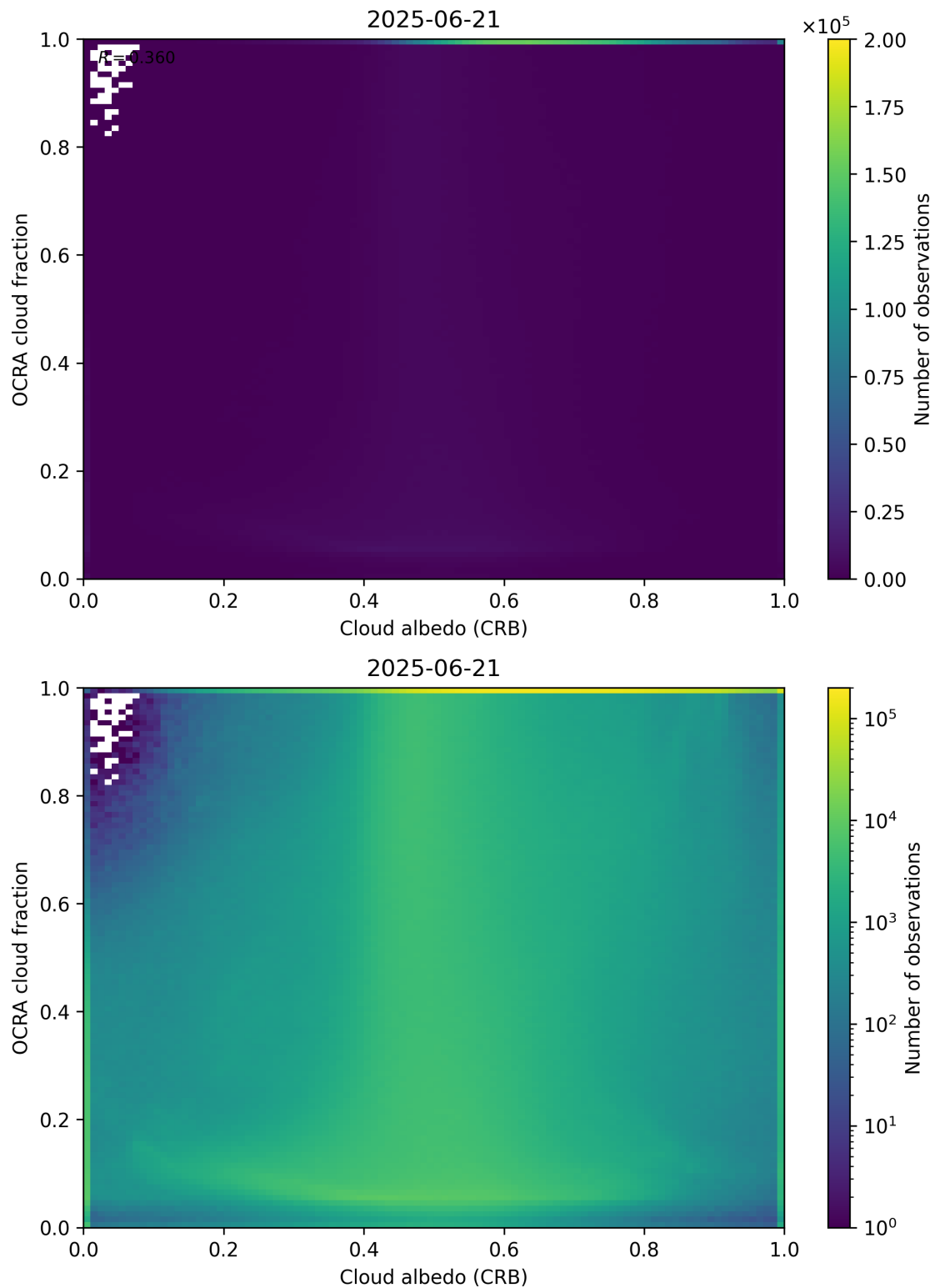
Figure 70: Scatter density plot of “Cloud albedo (CRB)” against “OCRA cloud fraction” for 2025-06-20 to 2025-06-22.
