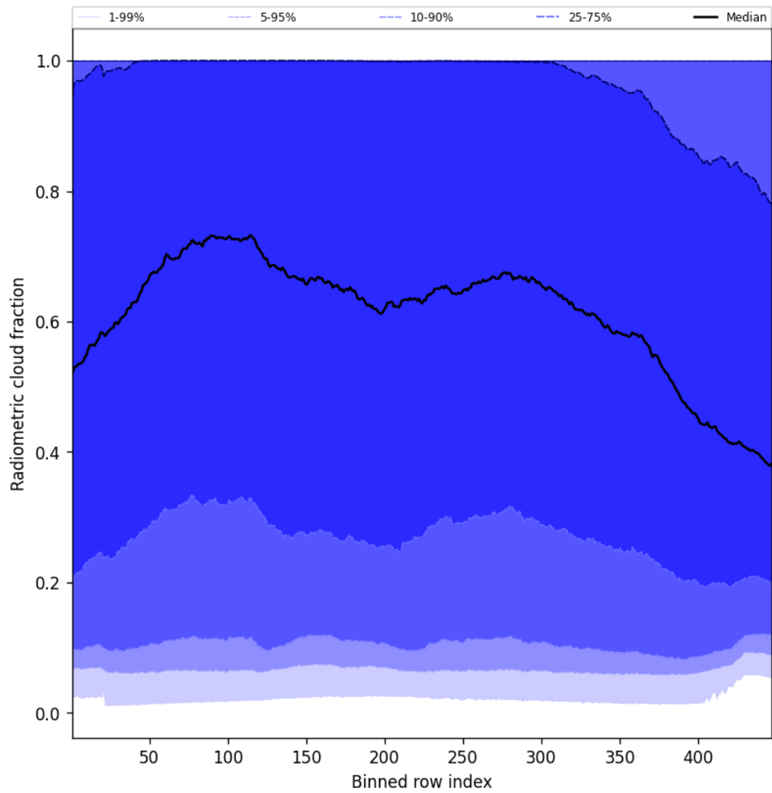
Figure 55: Along track statistics of “Radiometric cloud fraction” for 2025-06-20 to 2025-06-22
