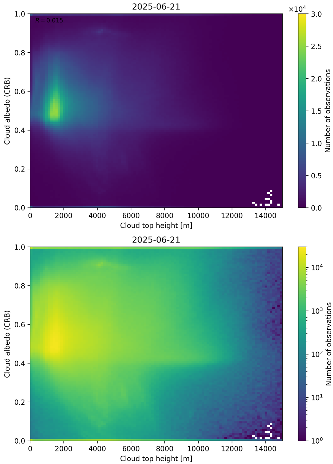
Figure 86: Scatter density plot of “Cloud top height” against “Cloud albedo (CRB)” for 2025-06-20 to 2025-06-22.
