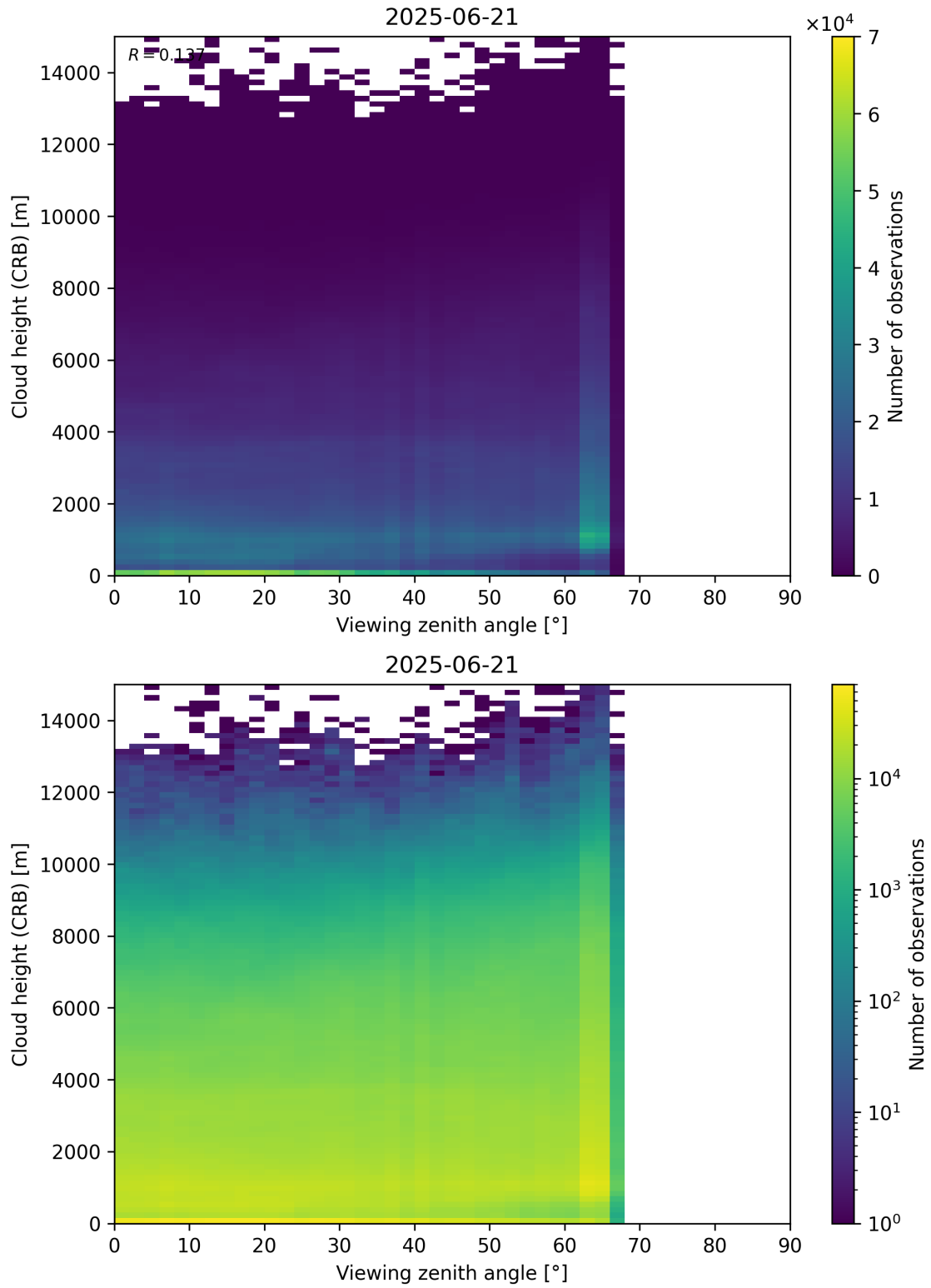
Figure 110: Scatter density plot of “Viewing zenith angle” against “Cloud height (CRB)” for 2025-06-20 to 2025-06-22.
