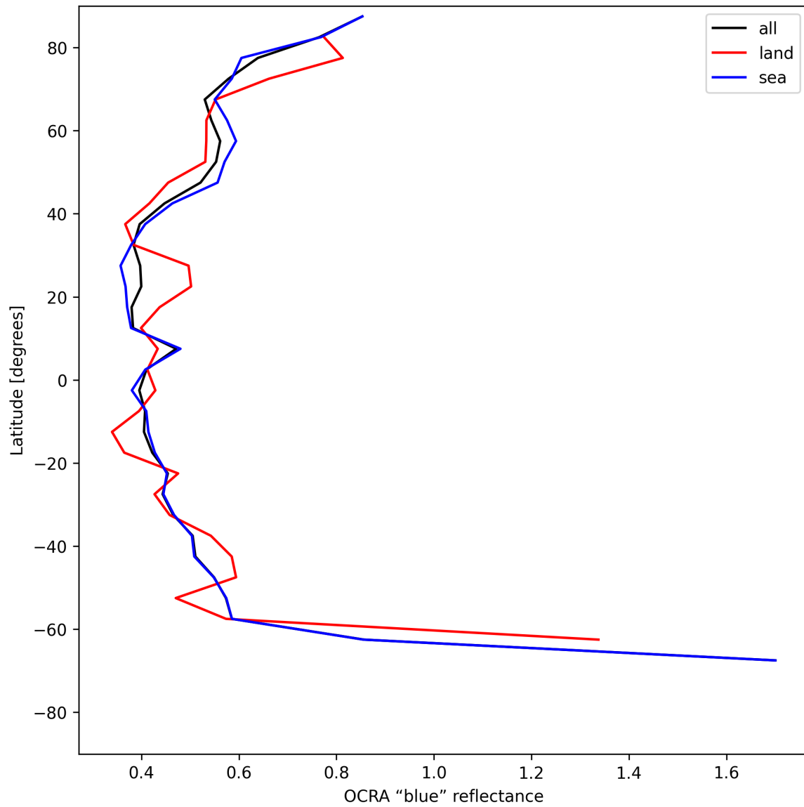
Figure 35: Zonal average of “OCRA “blue” reflectance” for 2025-06-20 to 2025-06-22.
