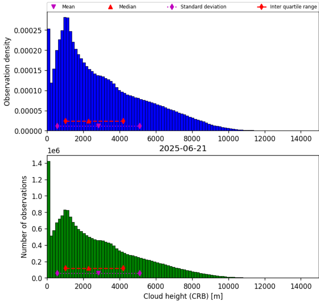
Figure 43: Histogram of “Cloud height (CRB)” for 2025-06-20 to 2025-06-22
