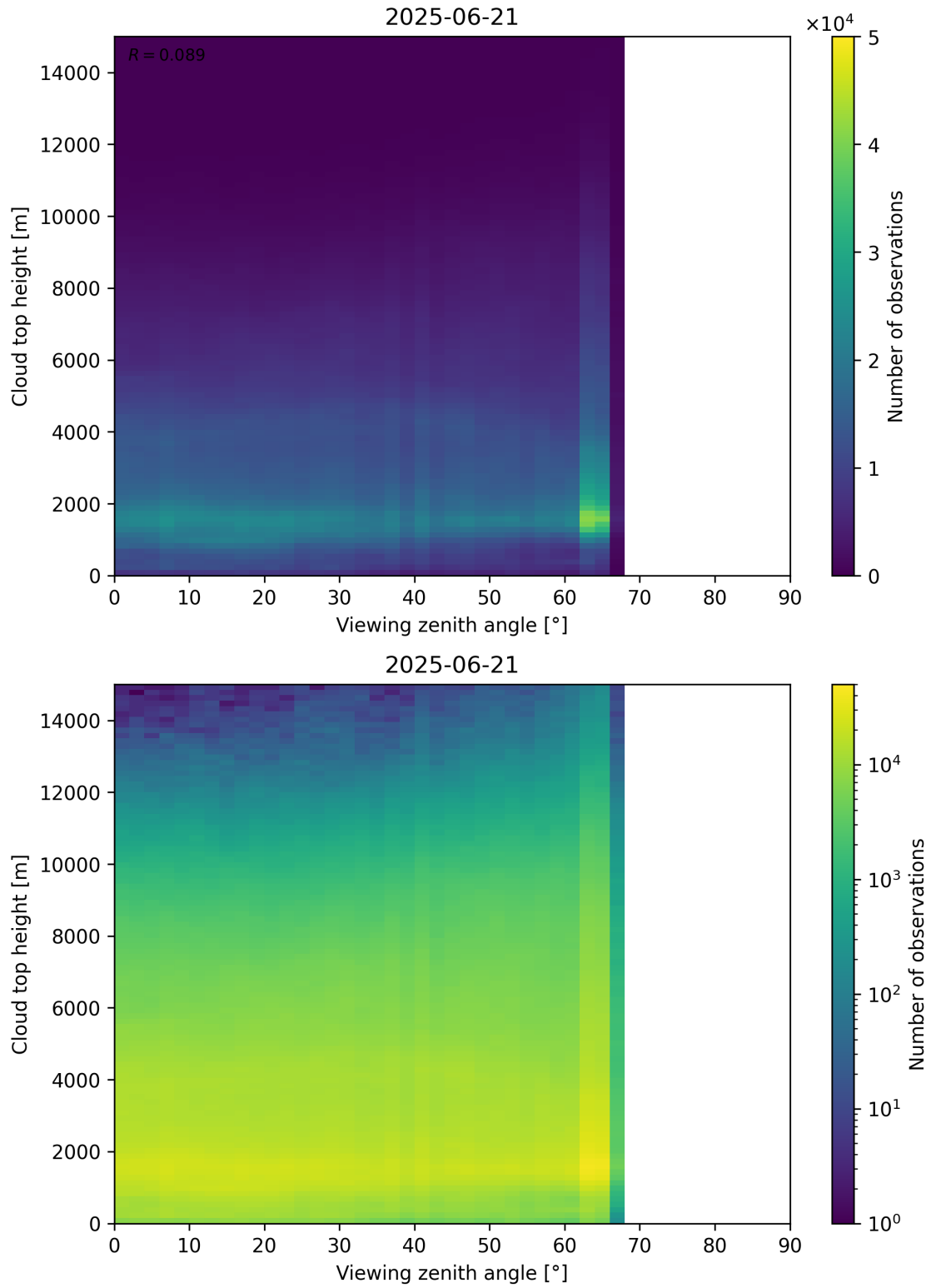
Figure 112: Scatter density plot of “Viewing zenith angle” against “Cloud top height” for 2025-06-20 to 2025-06-22.
