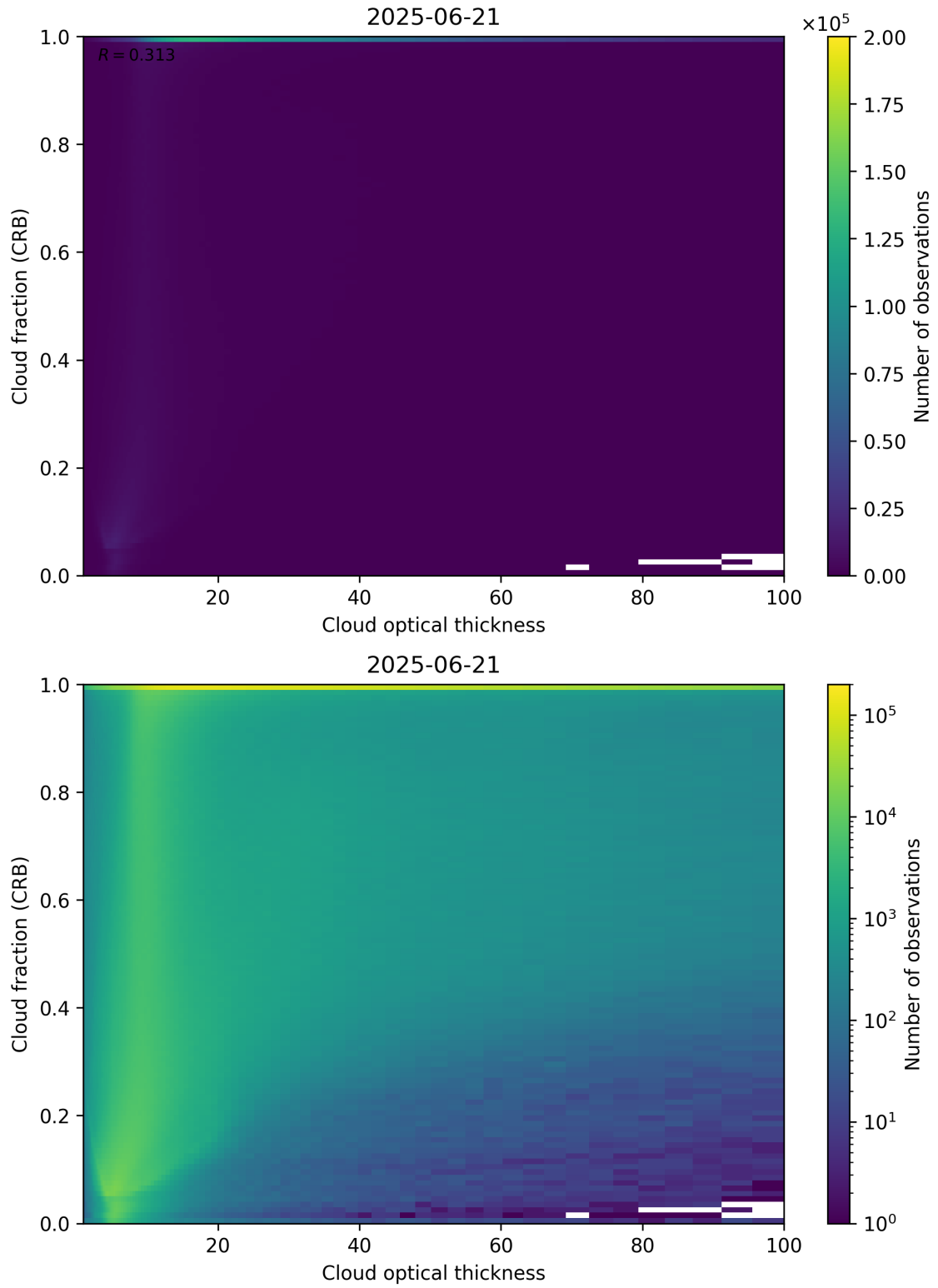
Figure 84: Scatter density plot of “Cloud optical thickness” against “Cloud fraction (CRB)” for 2025-06-20 to 2025-06-22.
