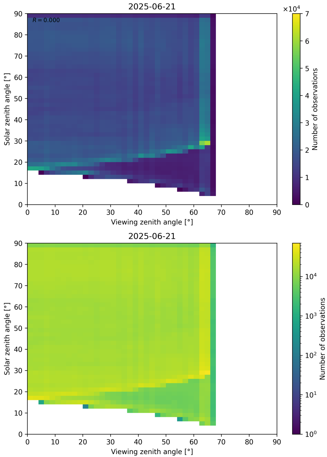
Figure 114: Scatter density plot of “Viewing zenith angle” against “Solar zenith angle” for 2025-06-20 to 2025-06-22.
