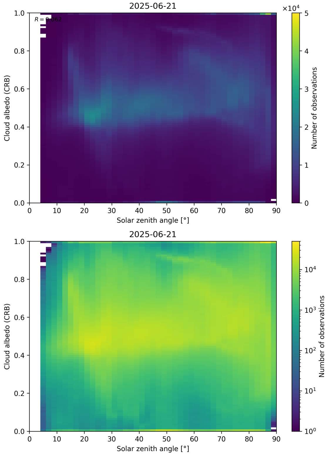
Figure 98: Scatter density plot of “Solar zenith angle” against “Cloud albedo (CRB)” for 2025-06-20 to 2025-06-22.
