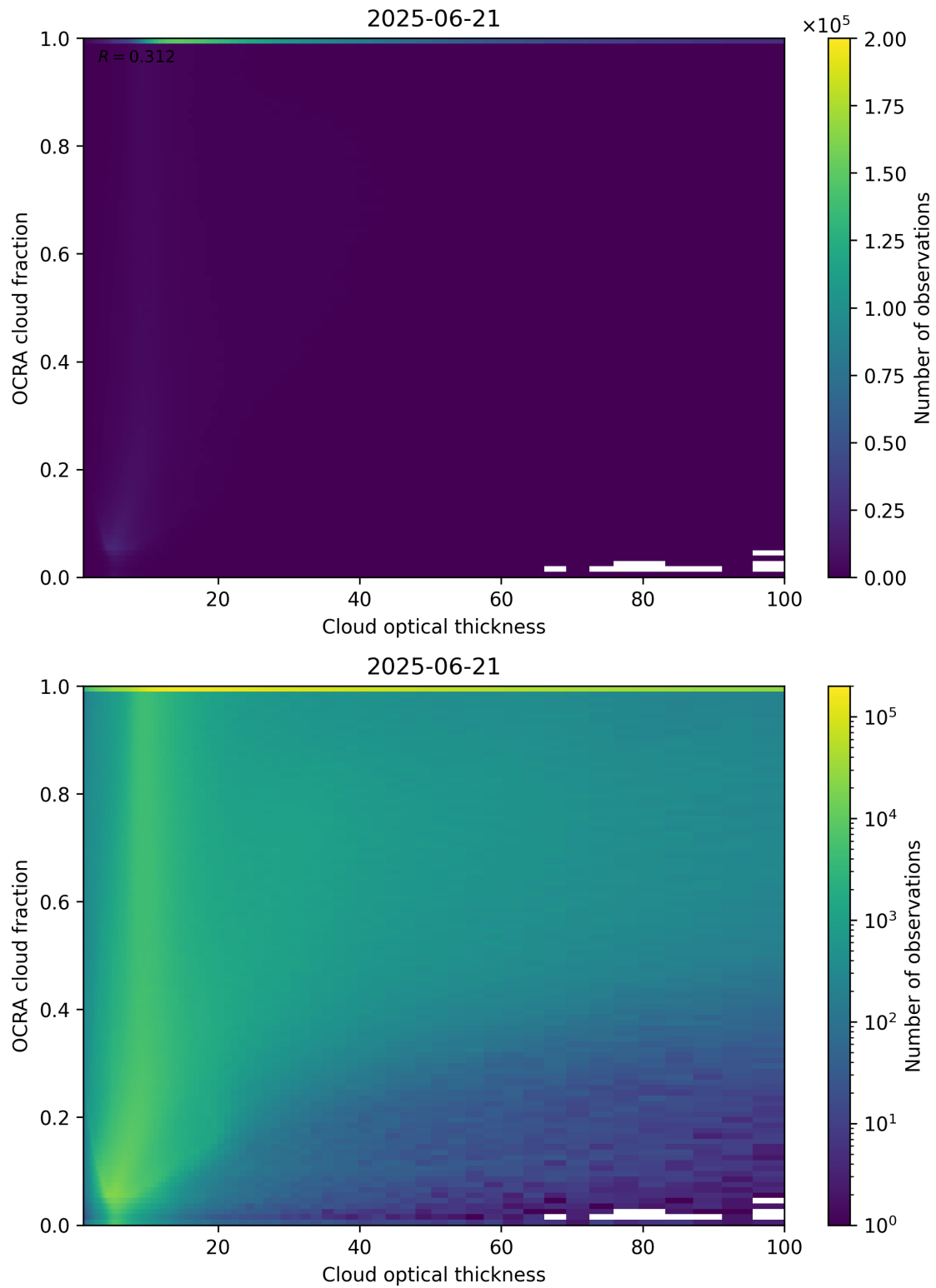
Figure 83: Scatter density plot of “Cloud optical thickness” against “OCRA cloud fraction” for 2025-06-20 to 2025-06-22.
