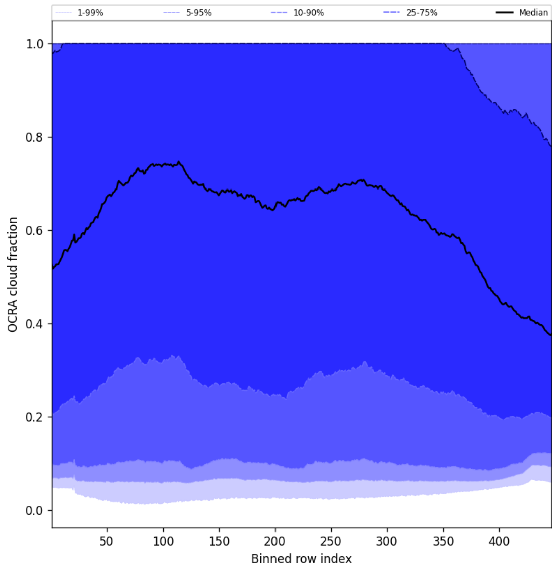
Figure 66: Along track statistics of “OCRA cloud fraction” for 2025-06-20 to 2025-06-22
