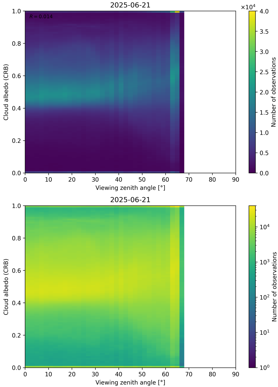
Figure 106: Scatter density plot of “Viewing zenith angle” against “Cloud albedo (CRB)” for 2025-06-20 to 2025-06-22.
