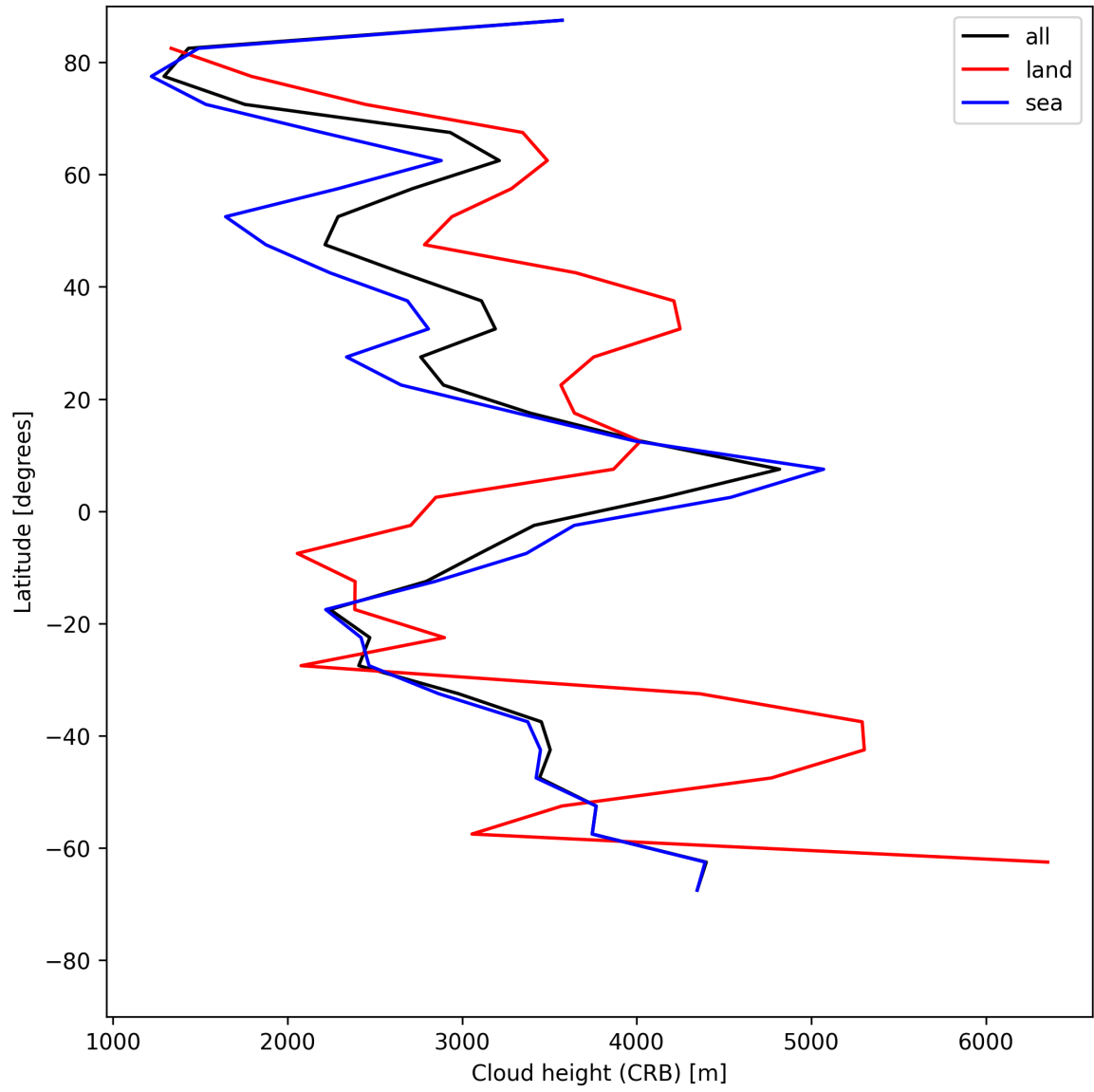
Figure 27: Zonal average of “Cloud height (CRB)” for 2025-06-20 to 2025-06-22.
