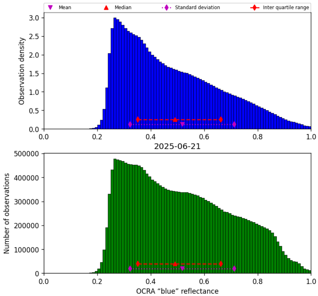
Figure 51: Histogram of “OCRA “blue” reflectance” for 2025-06-20 to 2025-06-22
