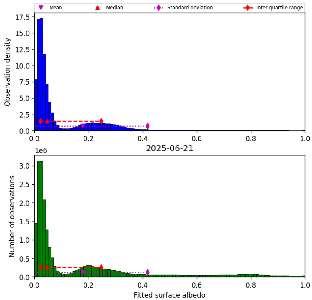
Figure 45: Histogram of “Fitted surface albedo” for 2025-06-20 to 2025-06-22
