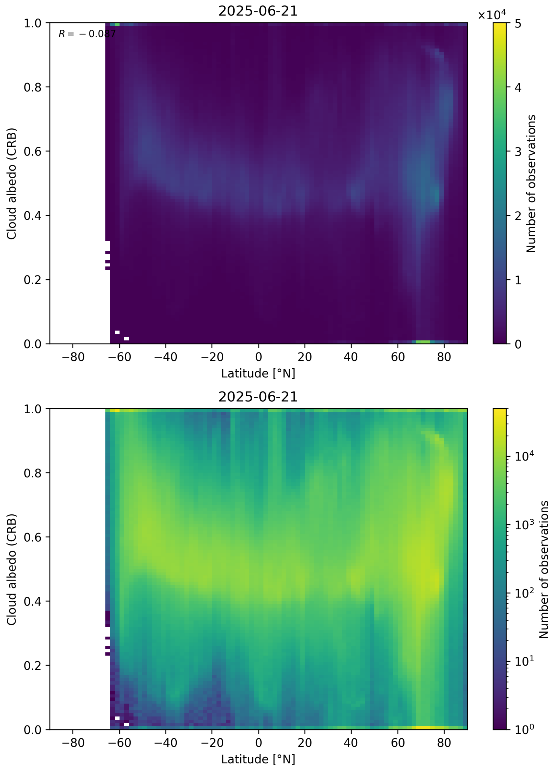
Figure 91: Scatter density plot of “Latitude” against “Cloud albedo (CRB)” for 2025-06-20 to 2025-06-22.
