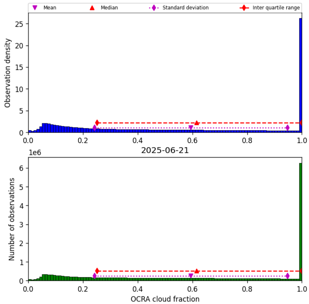
Figure 50: Histogram of “OCRA cloud fraction” for 2025-06-20 to 2025-06-22
