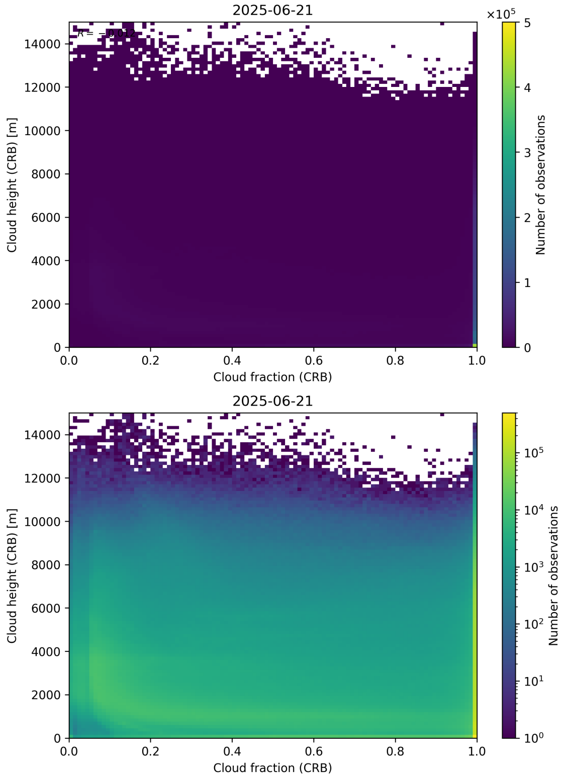
Figure 79: Scatter density plot of “Cloud fraction (CRB)” against “Cloud height (CRB)” for 2025-06-20 to 2025-06-22.
