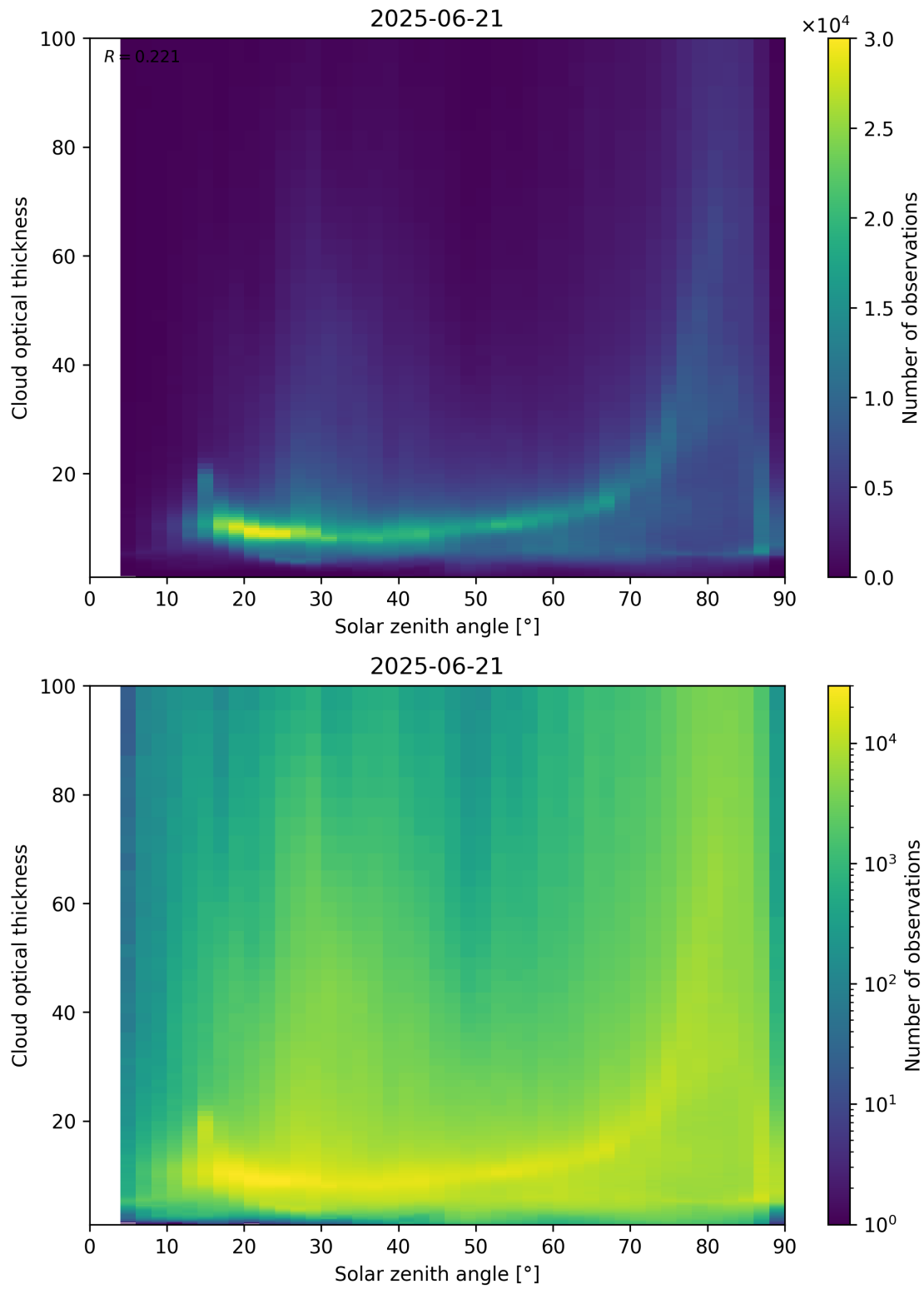
Figure 103: Scatter density plot of “Solar zenith angle” against “Cloud optical thickness” for 2025-06-20 to 2025-06-22.
