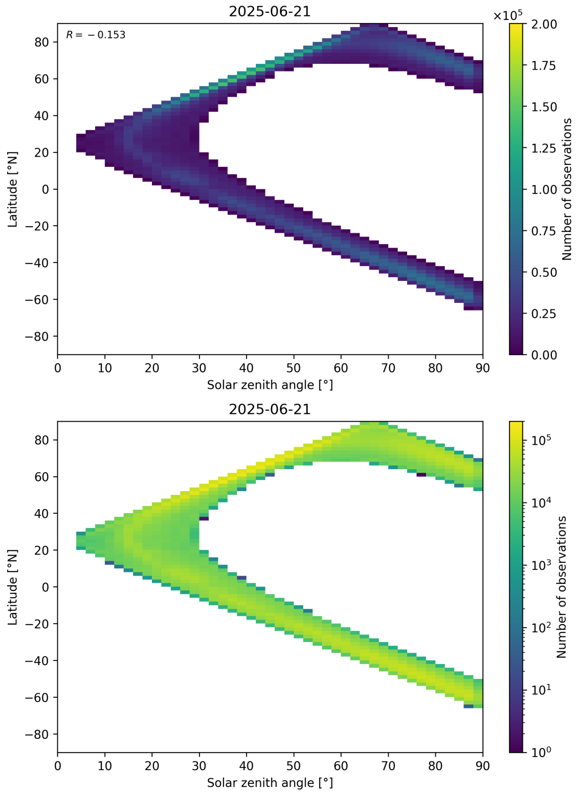
Figure 105: Scatter density plot of “Solar zenith angle” against “Latitude” for 2025-06-20 to 2025-06-22.
