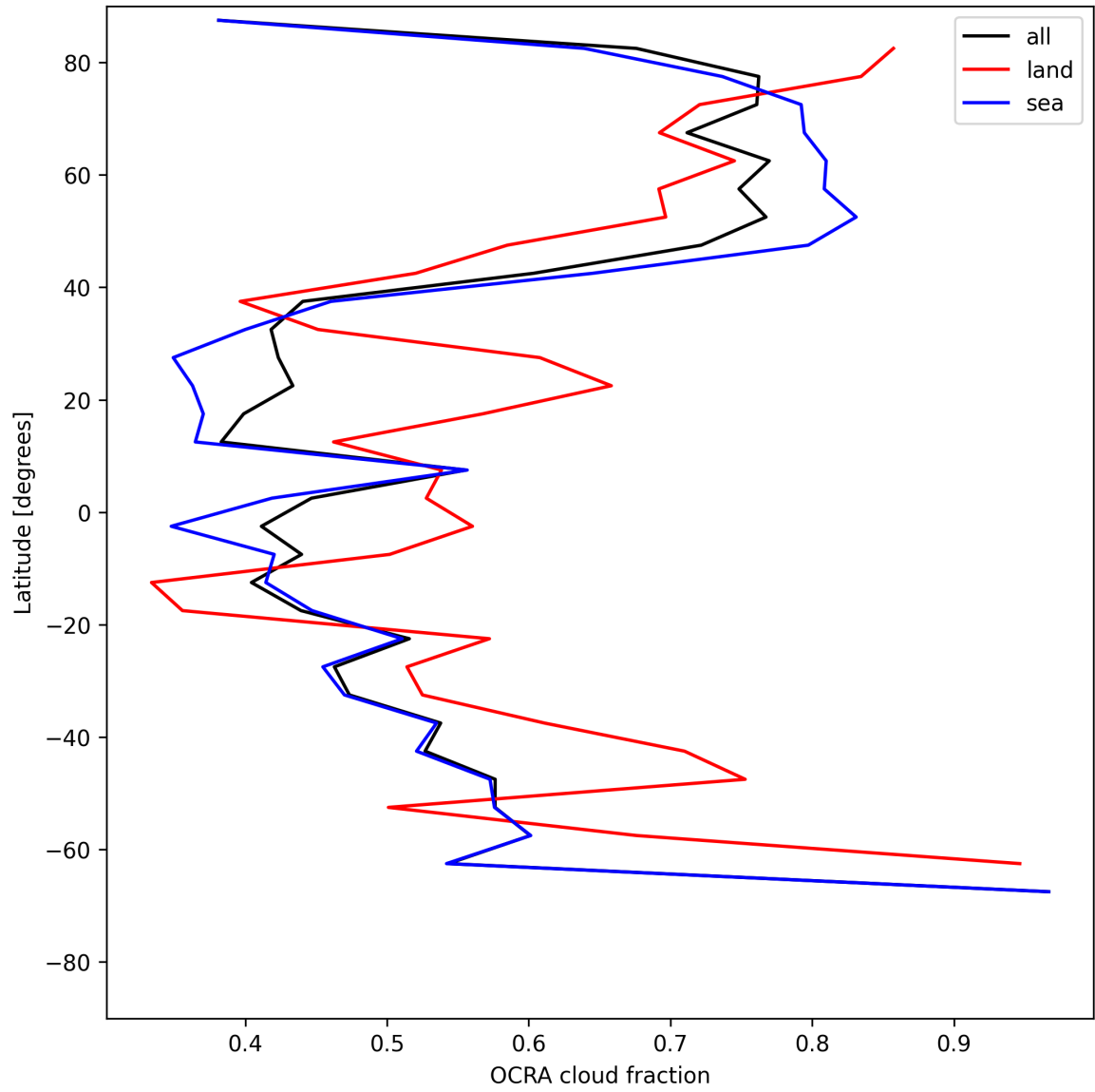
Figure 34: Zonal average of “OCRA cloud fraction” for 2025-06-20 to 2025-06-22.
