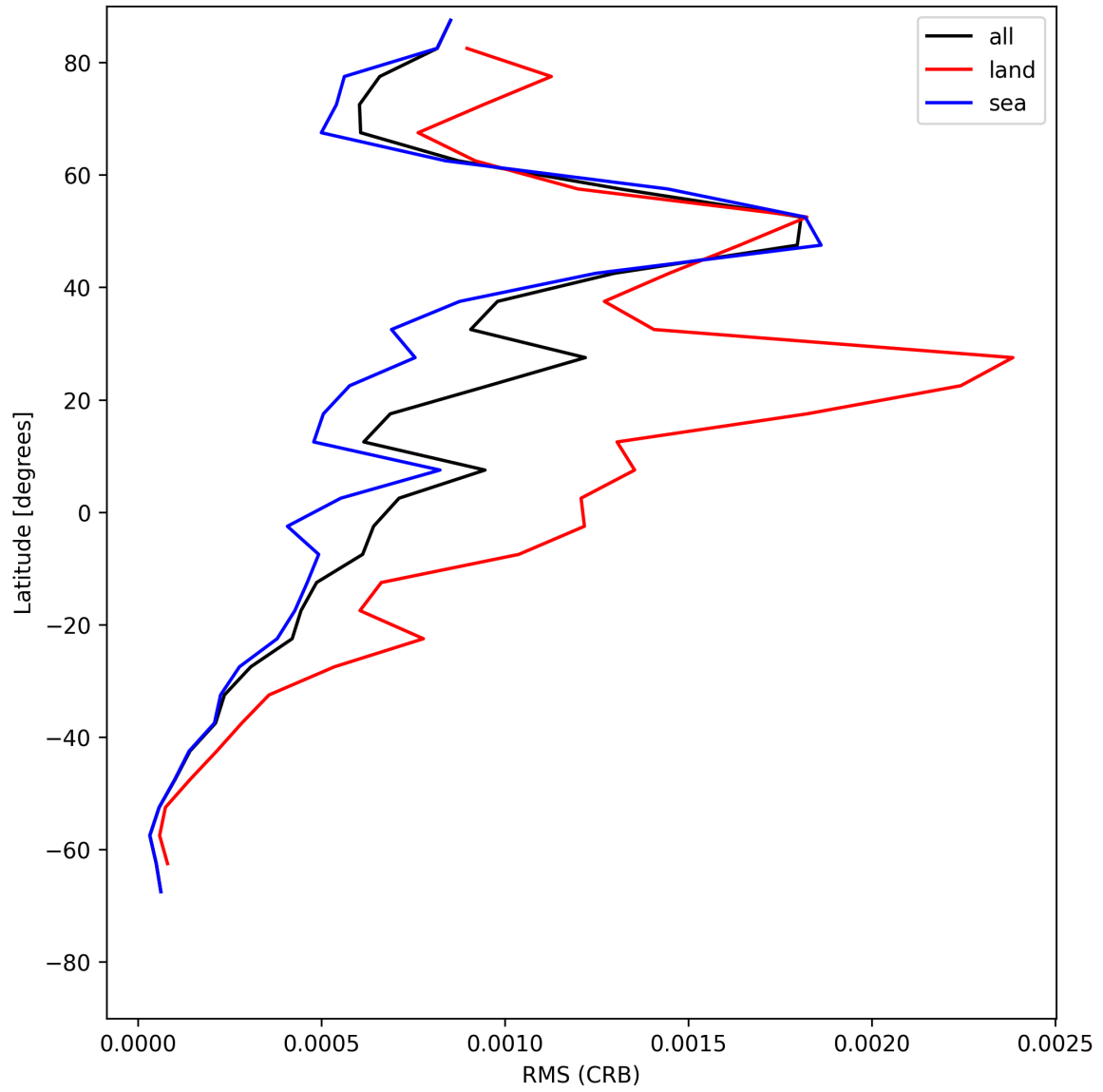
Figure 32: Zonal average of “RMS (CRB)” for 2025-06-20 to 2025-06-22.
