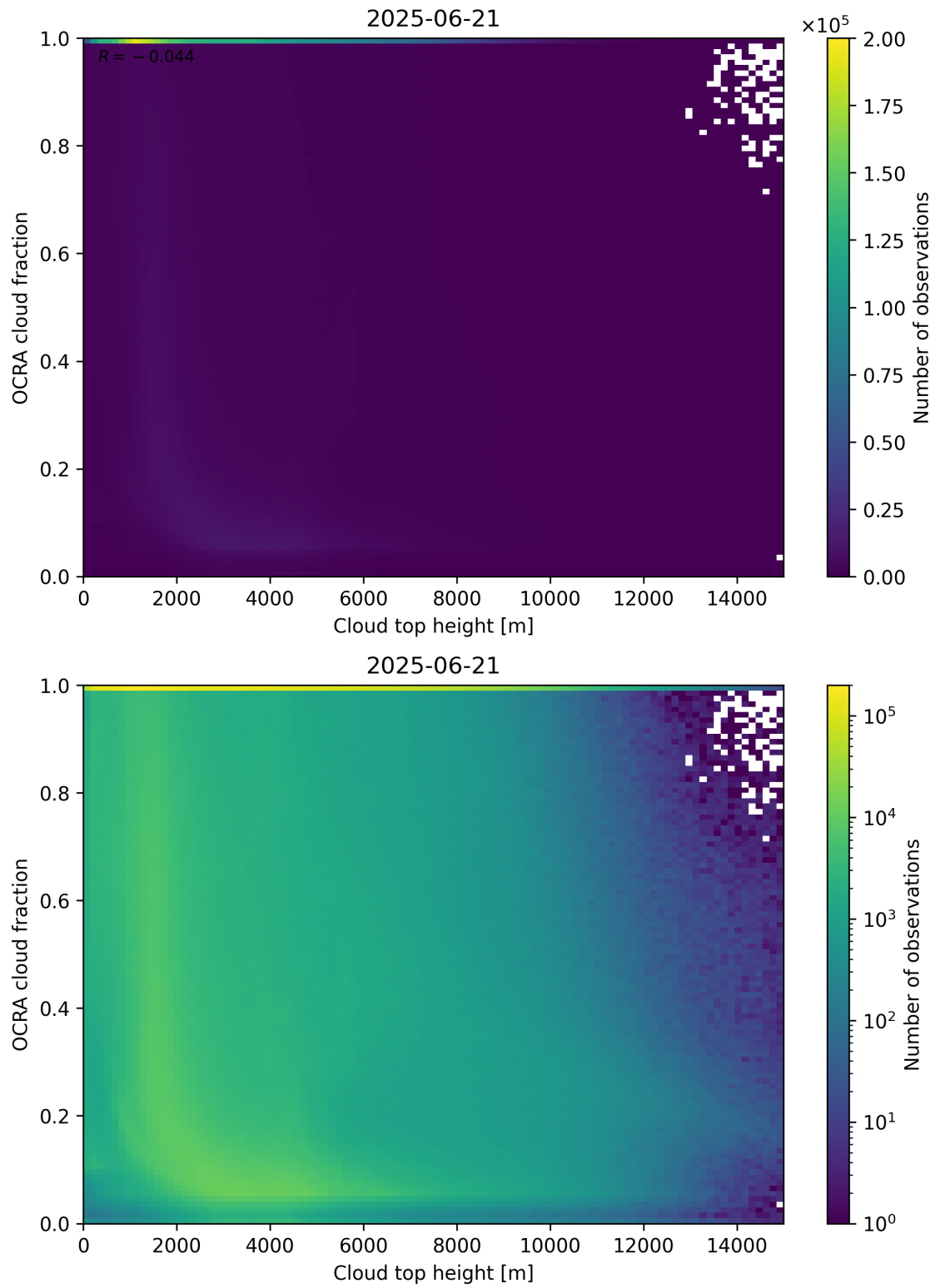
Figure 87: Scatter density plot of “Cloud top height” against “OCRA cloud fraction” for 2025-06-20 to 2025-06-22.
