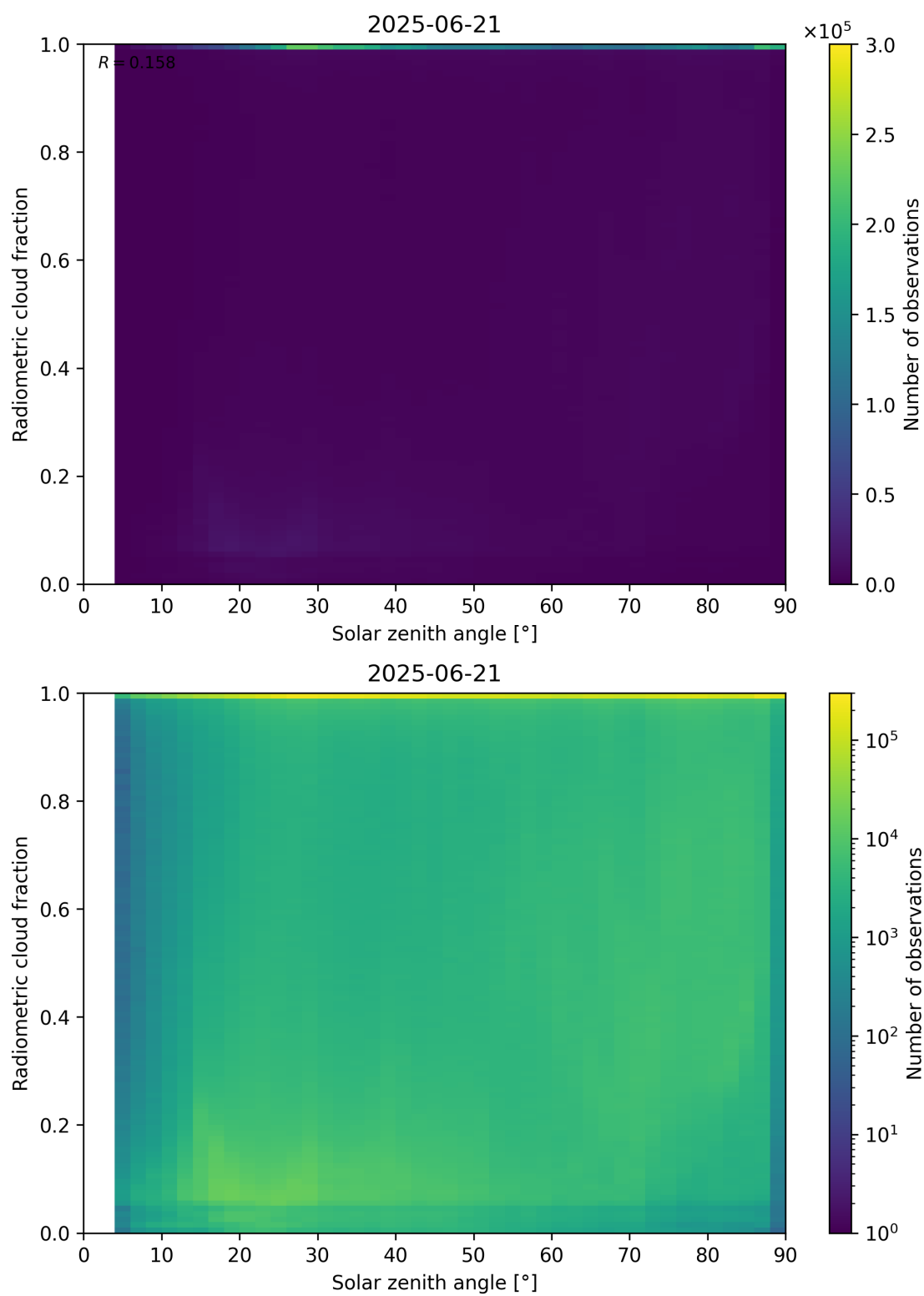
Figure 99: Scatter density plot of “Solar zenith angle” against “Radiometric cloud fraction” for 2025-06-20 to 2025-06-22.
