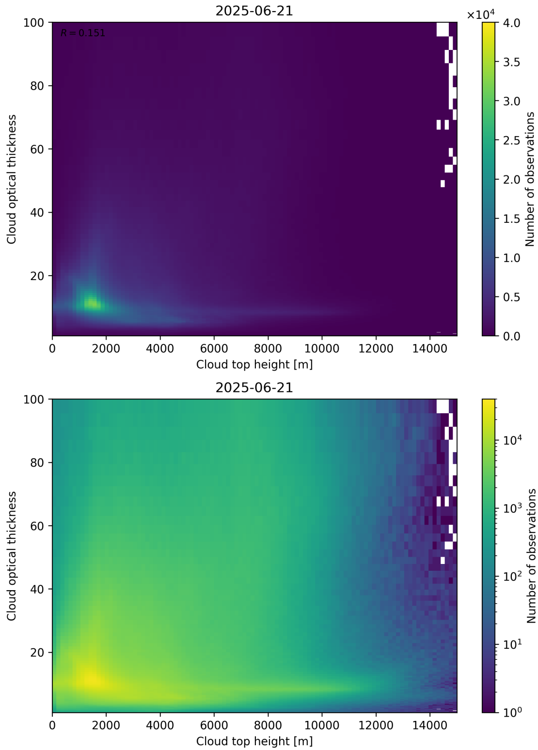
Figure 90: Scatter density plot of “Cloud top height” against “Cloud optical thickness” for 2025-06-20 to 2025-06-22.
