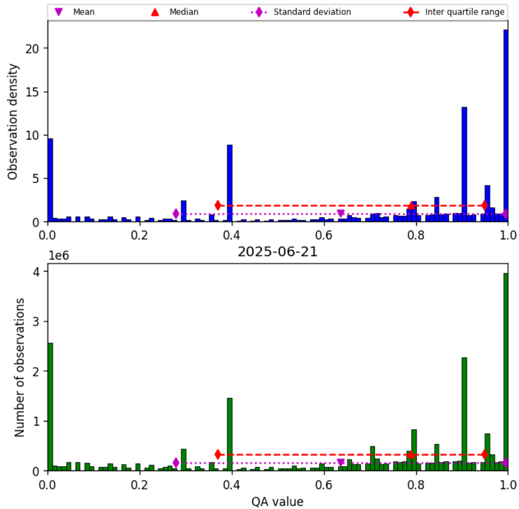
Figure 38: Histogram of “QA value” for 2025-06-20 to 2025-06-22
