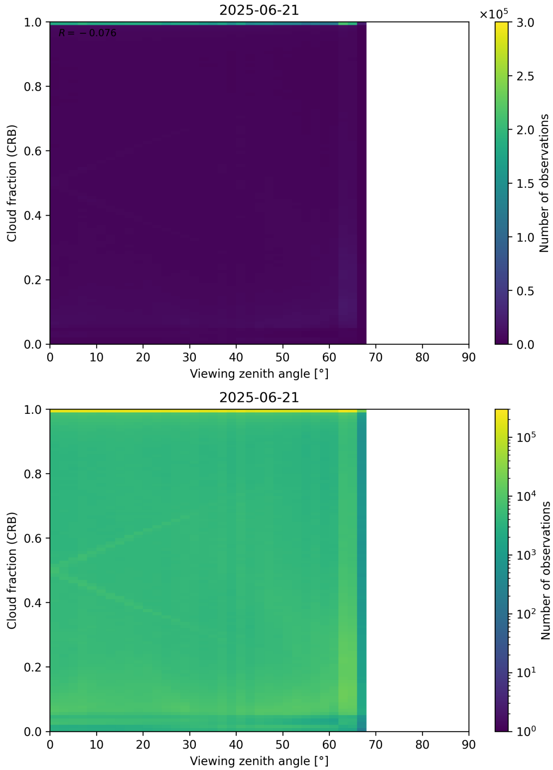
Figure 109: Scatter density plot of “Viewing zenith angle” against “Cloud fraction (CRB)” for 2025-06-20 to 2025-06-22.
