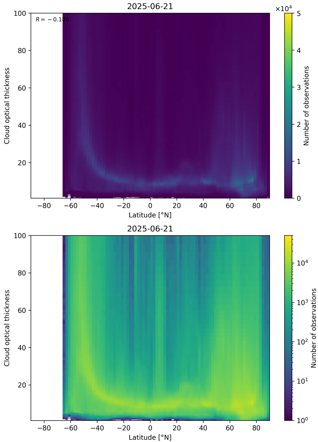
Figure 96: Scatter density plot of “Latitude” against “Cloud optical thickness” for 2025-06-20 to 2025-06-22.
