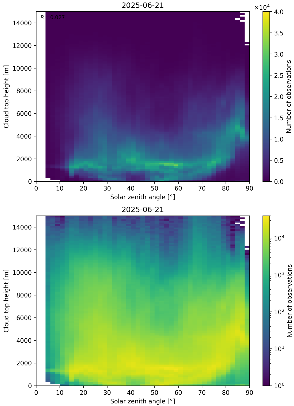
Figure 104: Scatter density plot of “Solar zenith angle” against “Cloud top height” for 2025-06-20 to 2025-06-22.
