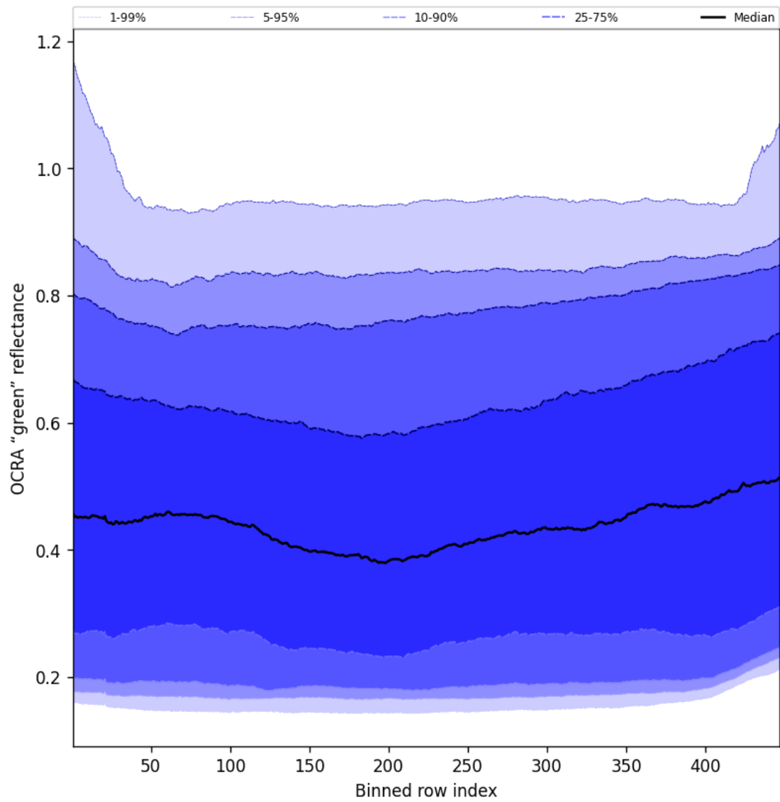
Figure 68: Along track statistics of “OCRA “green” reflectance” for 2025-06-20 to 2025-06-22
