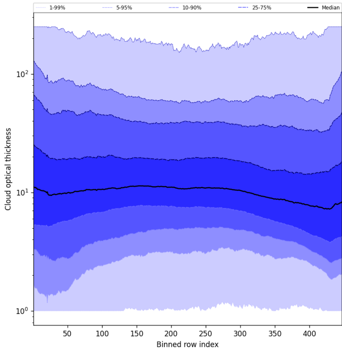
Figure 57: Along track statistics of “Cloud optical thickness” for 2025-06-20 to 2025-06-22
