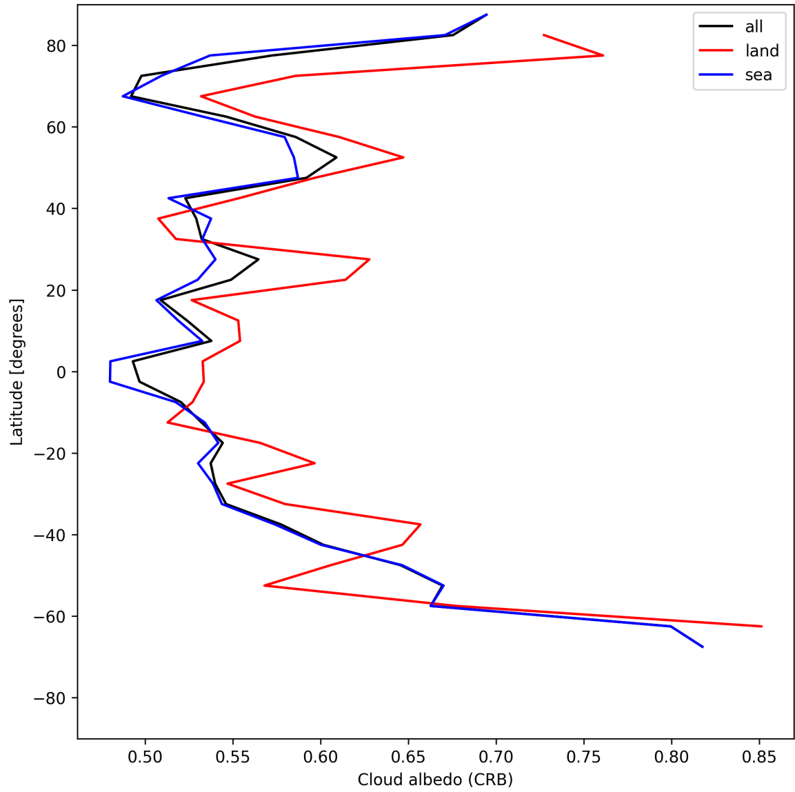
Figure 28: Zonal average of “Cloud albedo (CRB)” for 2025-06-20 to 2025-06-22.
