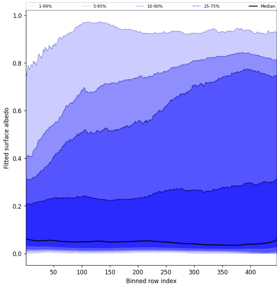
Figure 61: Along track statistics of “Fitted surface albedo” for 2025-06-20 to 2025-06-22
