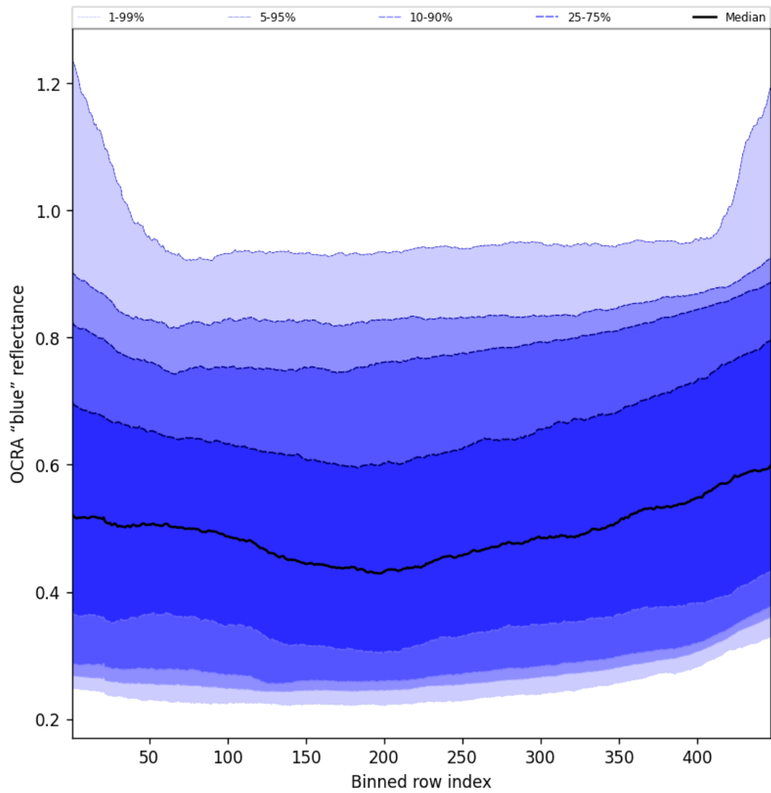
Figure 67: Along track statistics of “OCRA “blue” reflectance” for 2025-06-20 to 2025-06-22
