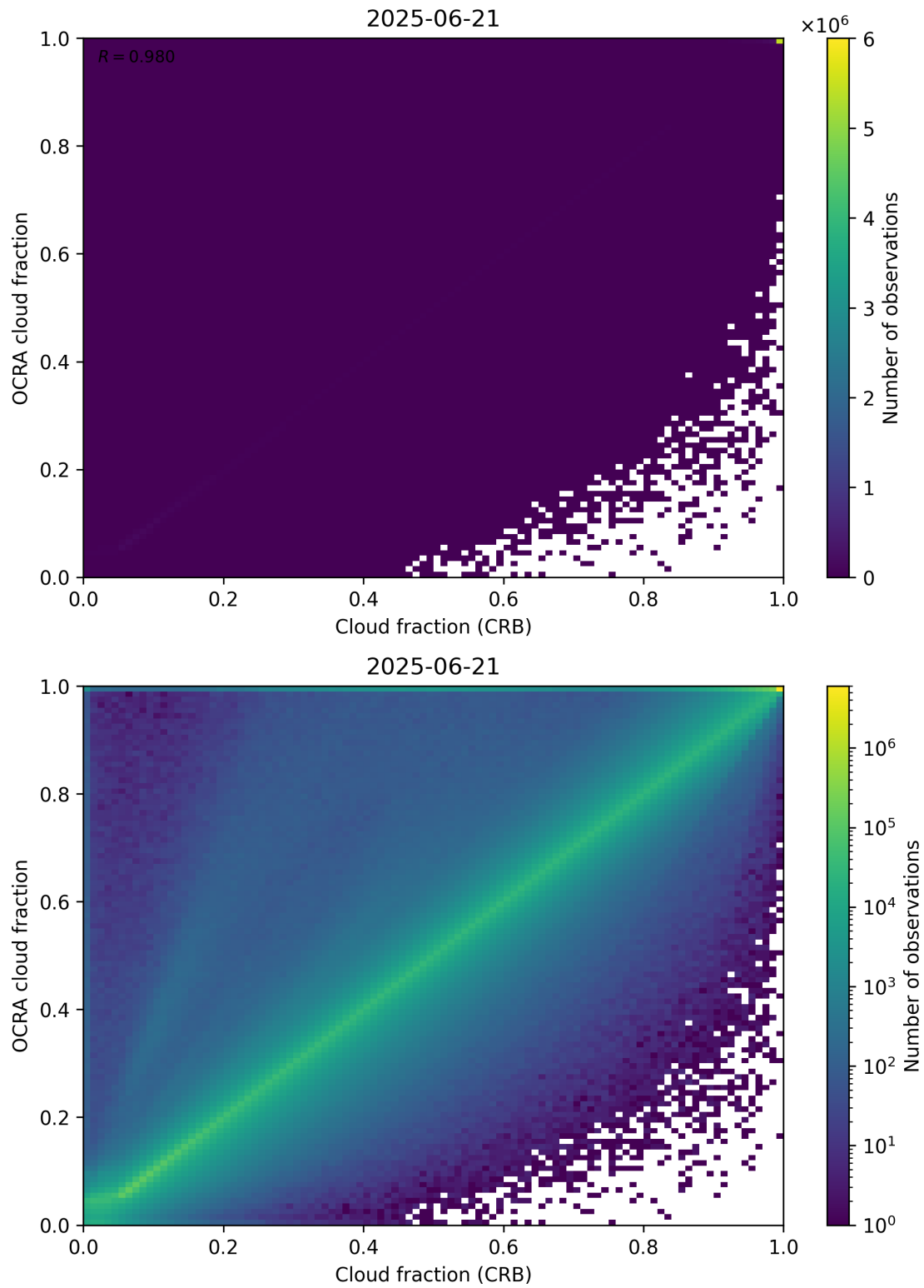
Figure 78: Scatter density plot of “Cloud fraction (CRB)” against “OCRA cloud fraction” for 2025-06-20 to 2025-06-22.
