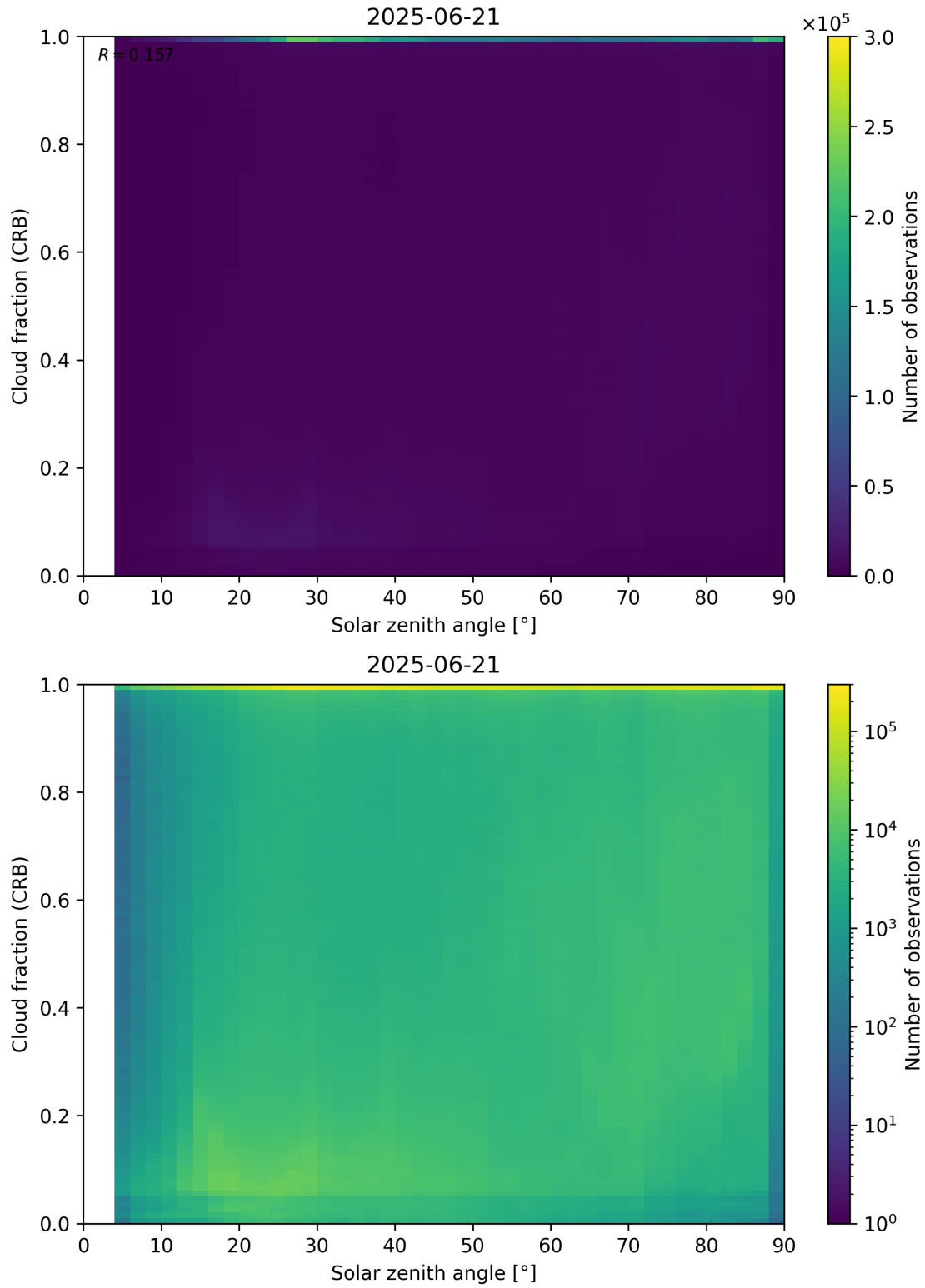
Figure 101: Scatter density plot of “Solar zenith angle” against “Cloud fraction (CRB)” for 2025-06-20 to 2025-06-22.
