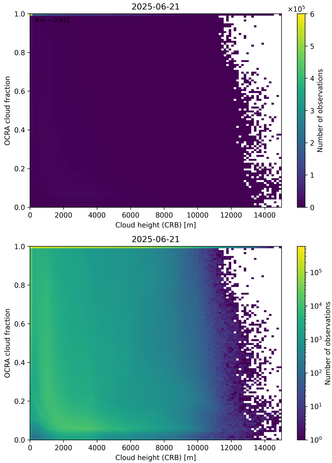
Figure 81: Scatter density plot of “Cloud height (CRB)” against “OCRA cloud fraction” for 2025-06-20 to 2025-06-22.
