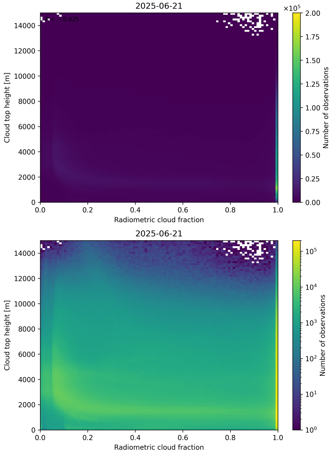
Figure 76: Scatter density plot of “Radiometric cloud fraction” against “Cloud top height” for 2025-06-20 to 2025-06-22.
