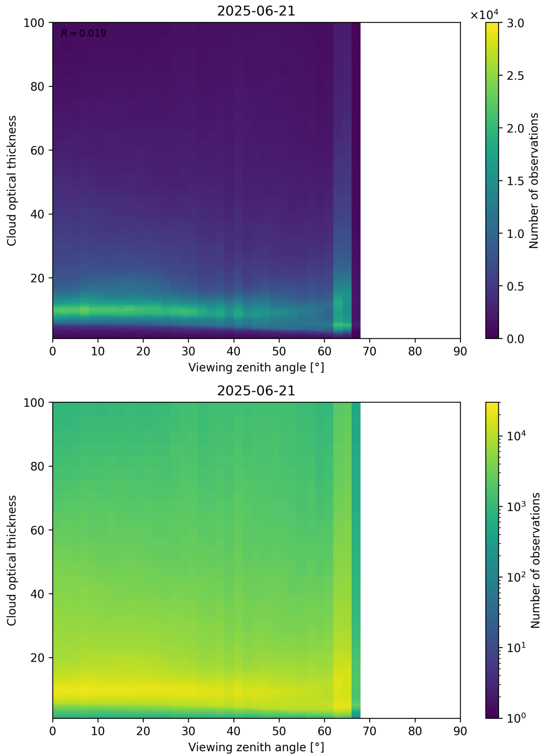
Figure 111: Scatter density plot of “Viewing zenith angle” against “Cloud optical thickness” for 2025-06-20 to 2025-06-22.
