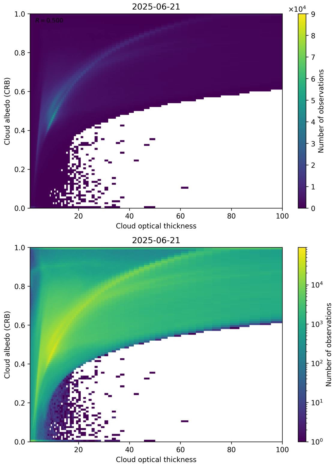
Figure 82: Scatter density plot of “Cloud optical thickness” against “Cloud albedo (CRB)” for 2025-06-20 to 2025-06-22.
