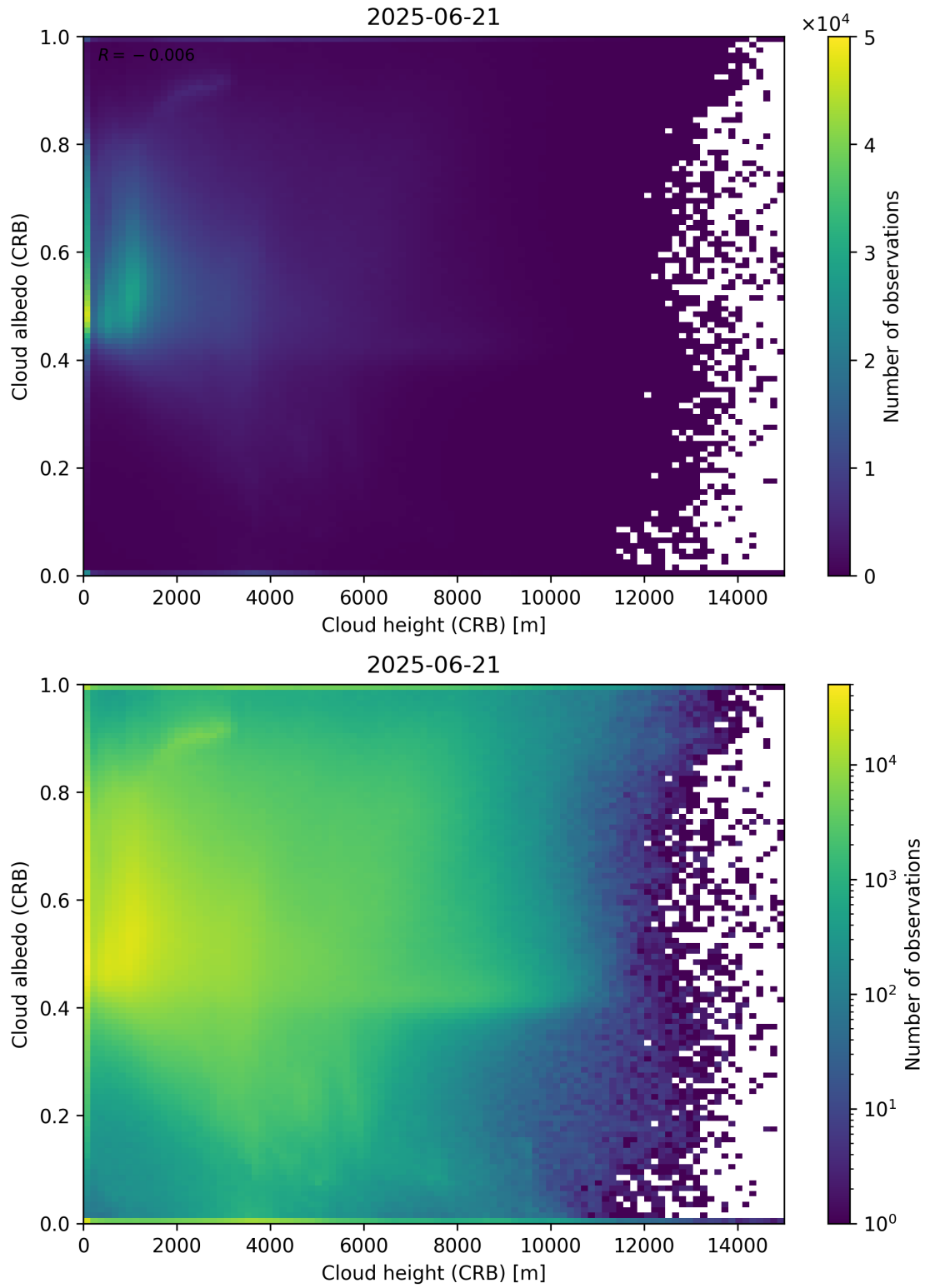
Figure 80: Scatter density plot of “Cloud height (CRB)” against “Cloud albedo (CRB)” for 2025-06-20 to 2025-06-22.
