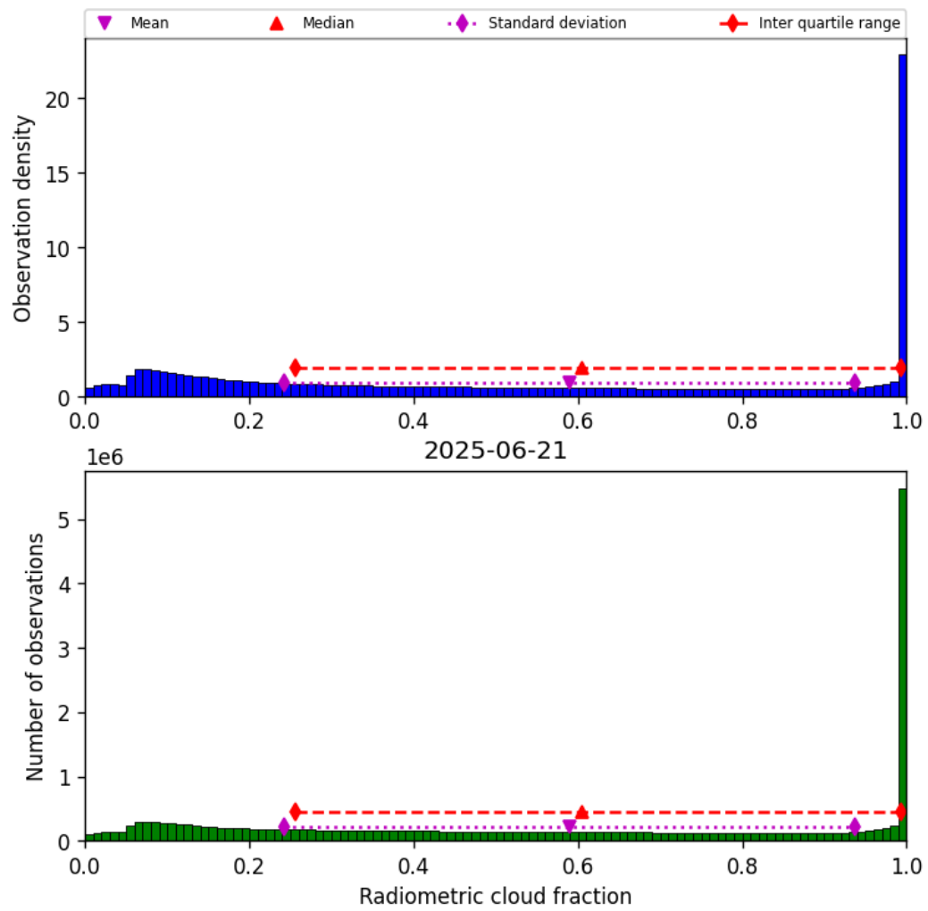
Figure 39: Histogram of “Radiometric cloud fraction” for 2025-06-20 to 2025-06-22
