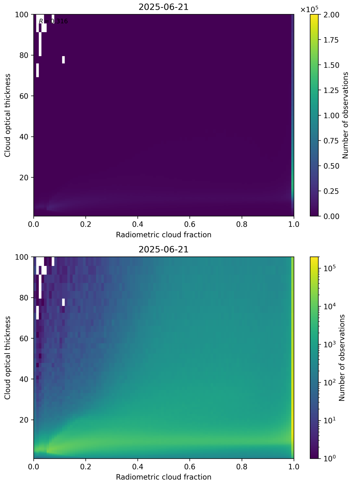
Figure 75: Scatter density plot of “Radiometric cloud fraction” against “Cloud optical thickness” for 2025-06-20 to 2025-06-22.
