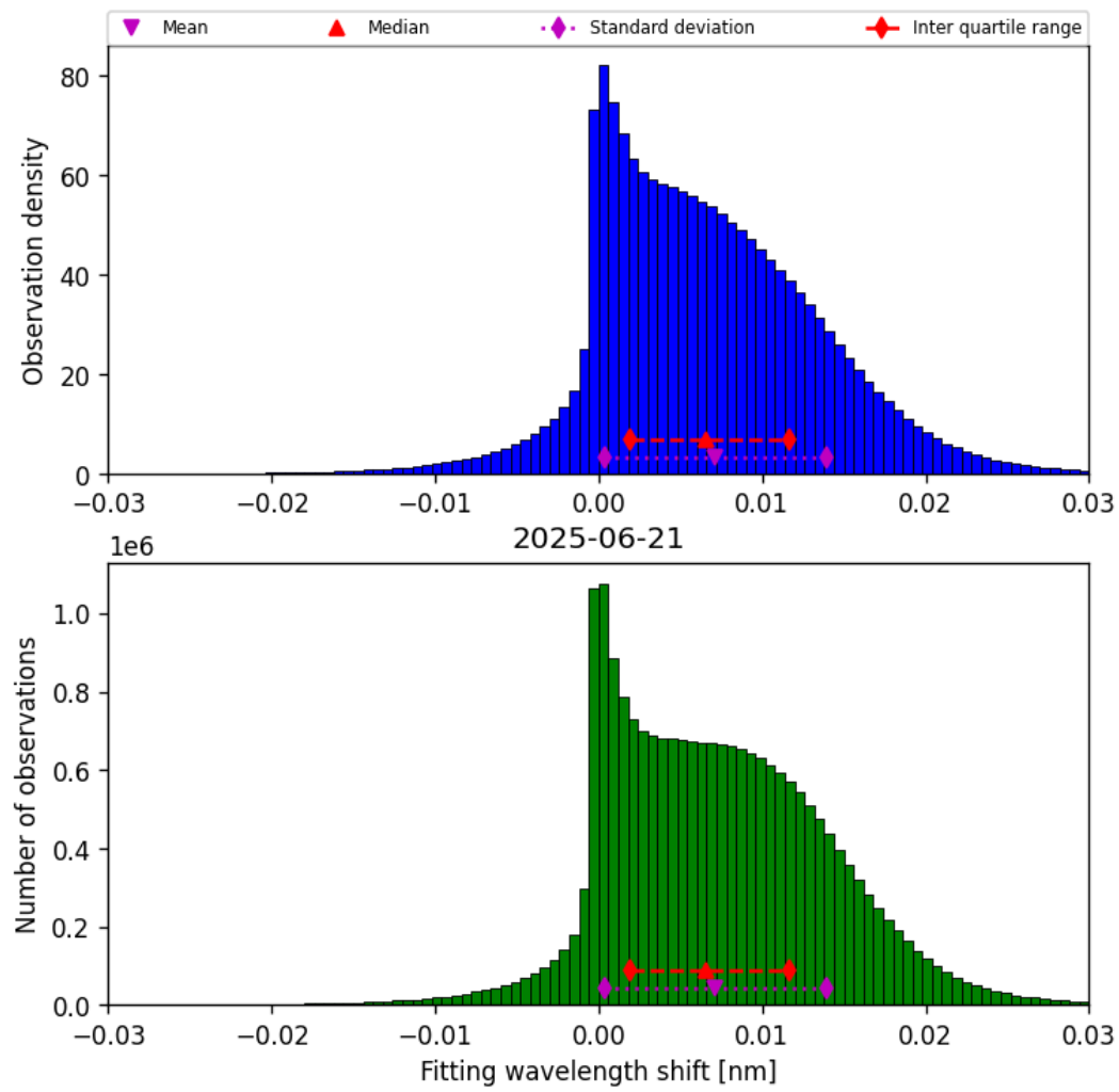
Figure 49: Histogram of “Fitting wavelength shift” for 2025-06-20 to 2025-06-22
