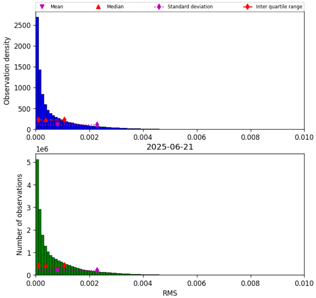
Figure 47: Histogram of “RMS” for 2025-06-20 to 2025-06-22
