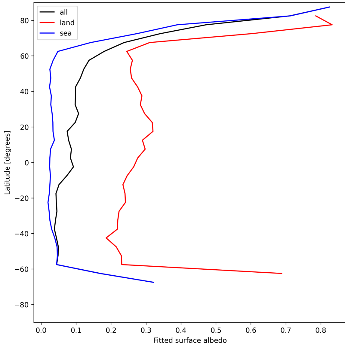
Figure 29: Zonal average of “Fitted surface albedo” for 2025-06-20 to 2025-06-22.
