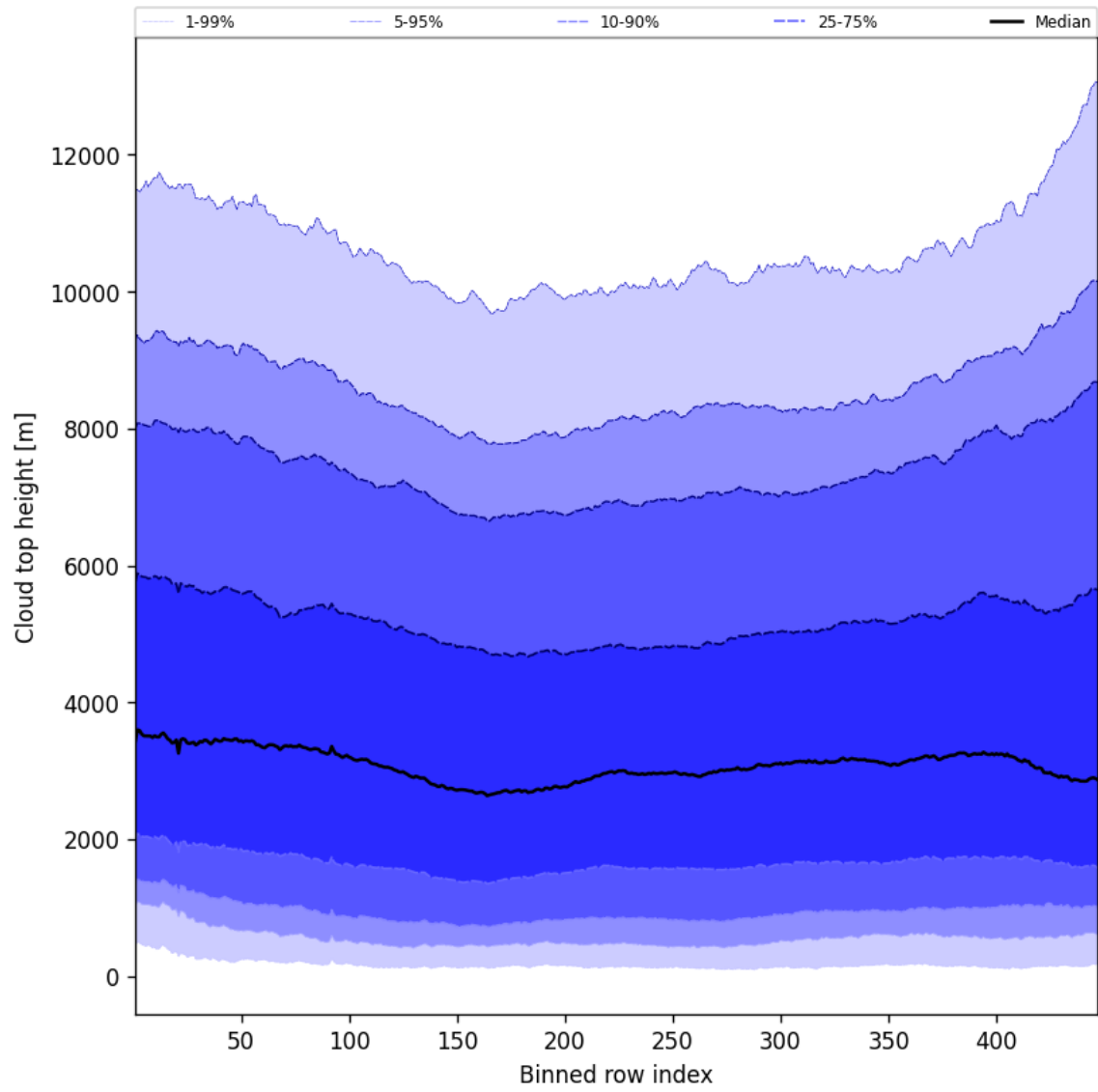
Figure 56: Along track statistics of “Cloud top height” for 2025-06-20 to 2025-06-22
