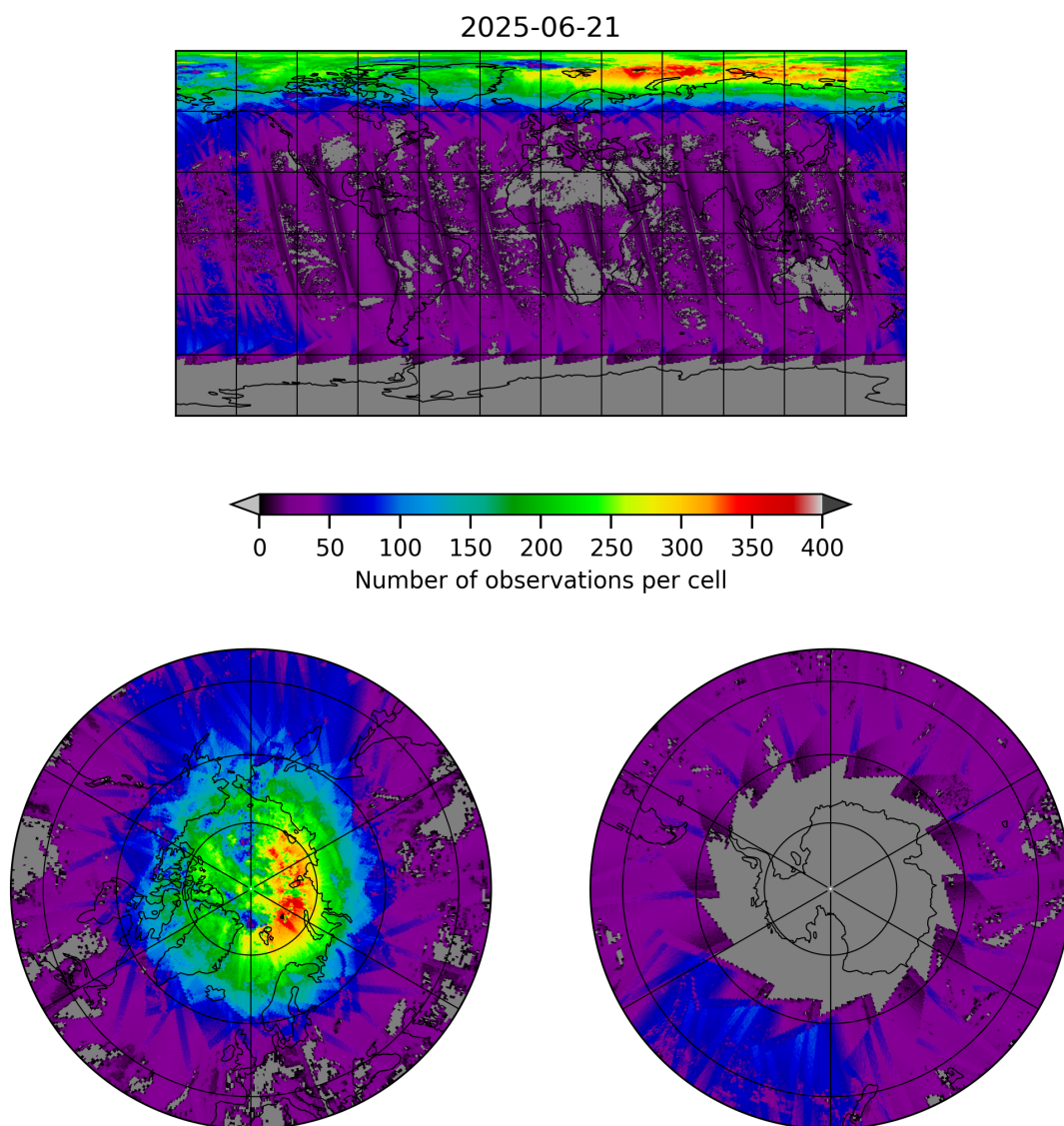
Figure 21: Map of the number of observations for 2025-06-20 to 2025-06-22
