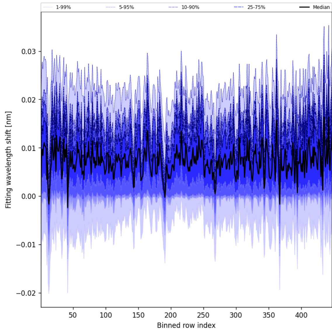
Figure 65: Along track statistics of “Fitting wavelength shift” for 2025-06-20 to 2025-06-22
