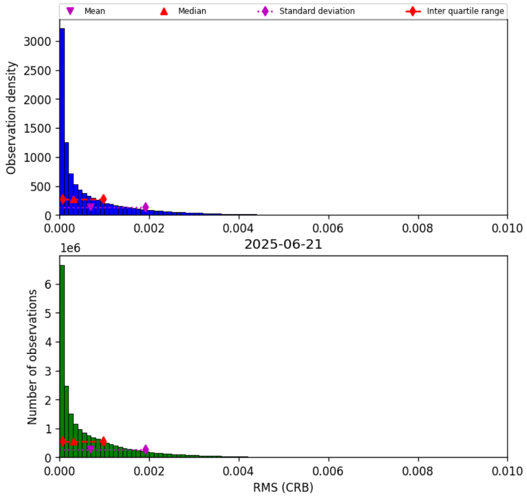
Figure 48: Histogram of “RMS (CRB)” for 2025-06-20 to 2025-06-22
