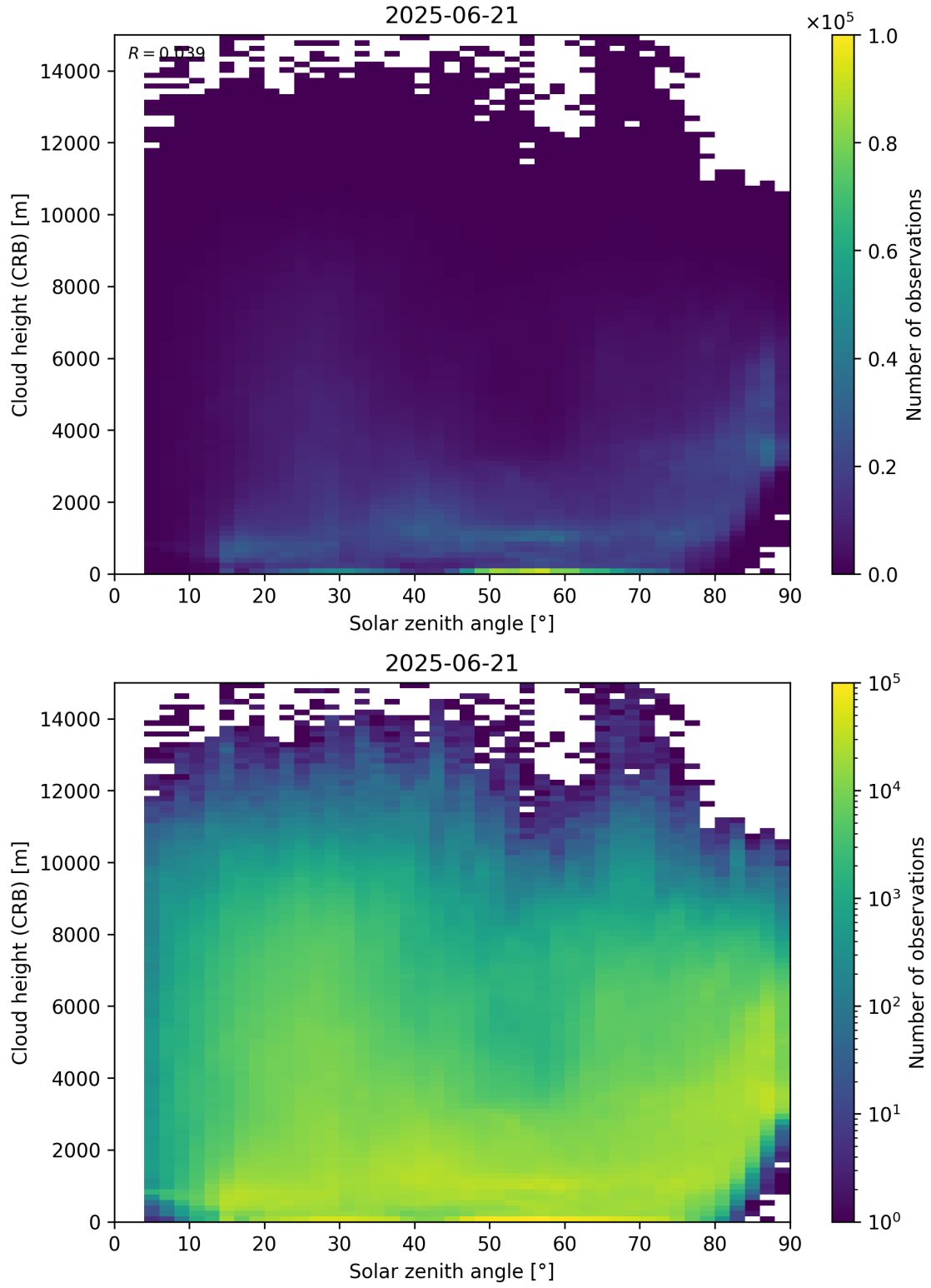
Figure 102: Scatter density plot of “Solar zenith angle” against “Cloud height (CRB)” for 2025-06-20 to 2025-06-22.
