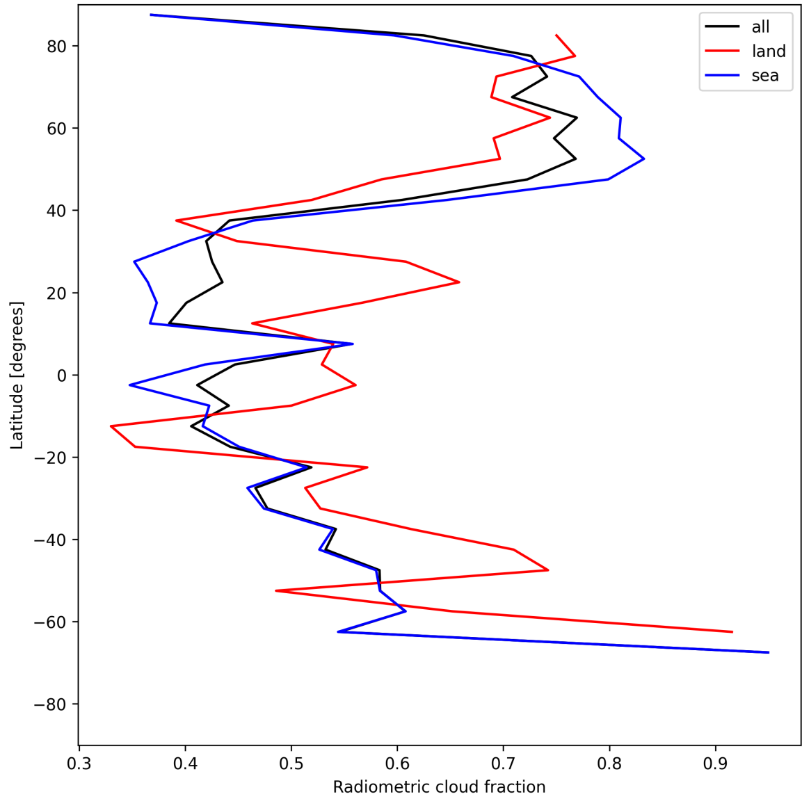
Figure 23: Zonal average of “Radiometric cloud fraction” for 2025-06-20 to 2025-06-22.
