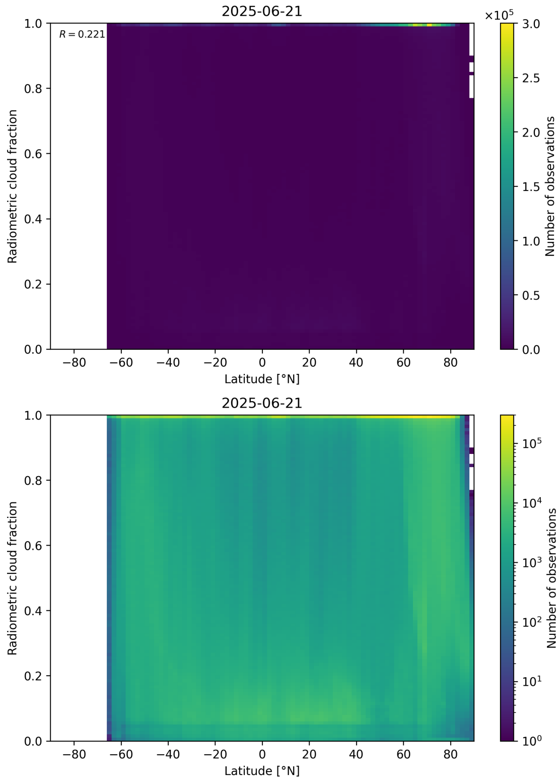
Figure 92: Scatter density plot of “Latitude” against “Radiometric cloud fraction” for 2025-06-20 to 2025-06-22.
