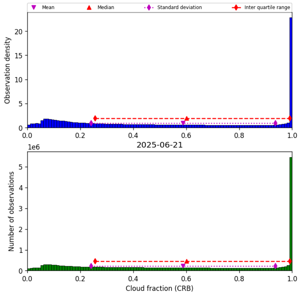
Figure 42: Histogram of “Cloud fraction (CRB)” for 2025-06-20 to 2025-06-22
