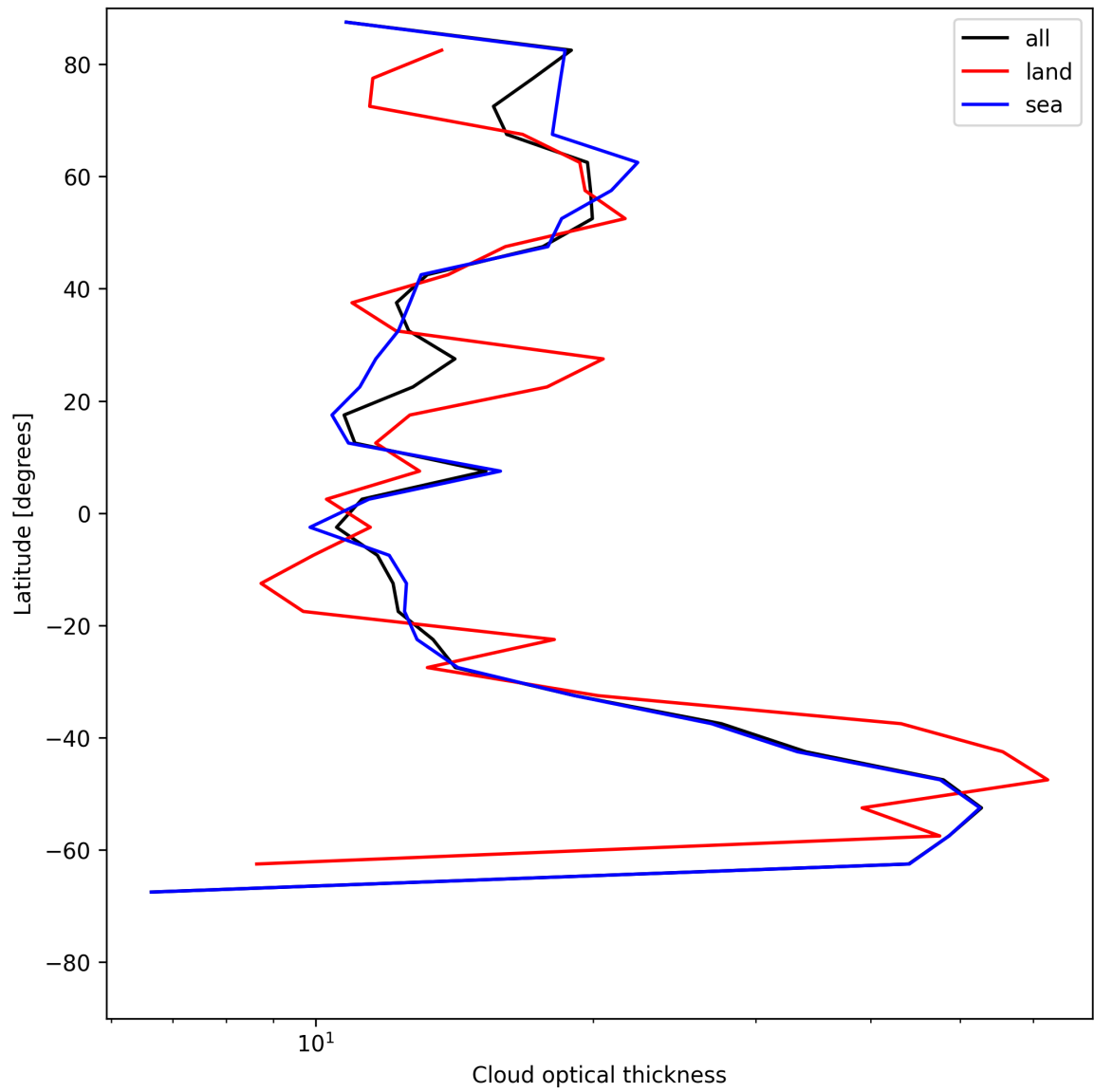
Figure 25: Zonal average of “Cloud optical thickness” for 2025-06-20 to 2025-06-22.
