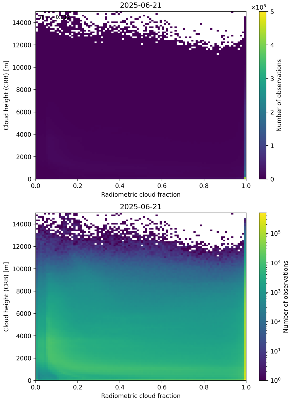
Figure 74: Scatter density plot of “Radiometric cloud fraction” against “Cloud height (CRB)” for 2025-06-20 to 2025-06-22.
