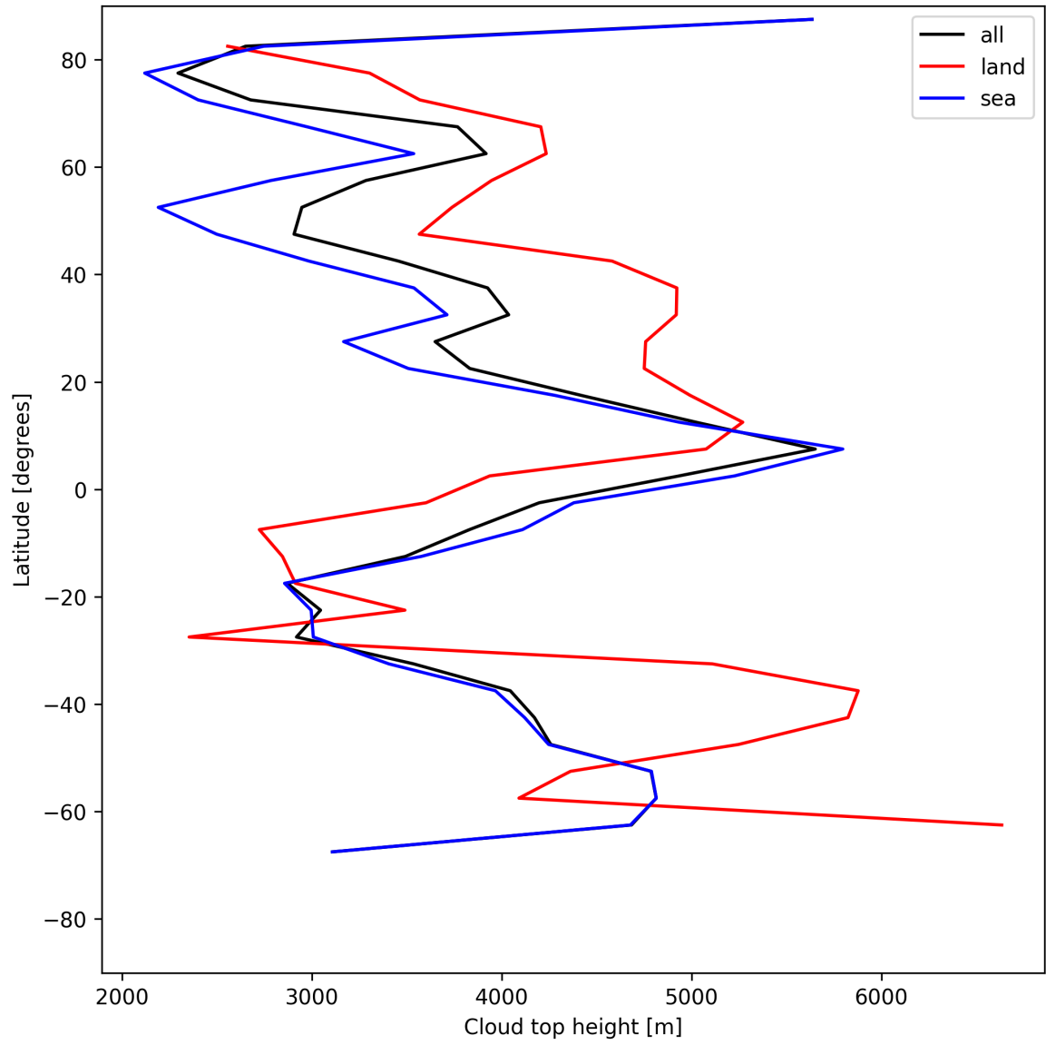
Figure 24: Zonal average of “Cloud top height” for 2025-06-20 to 2025-06-22.
