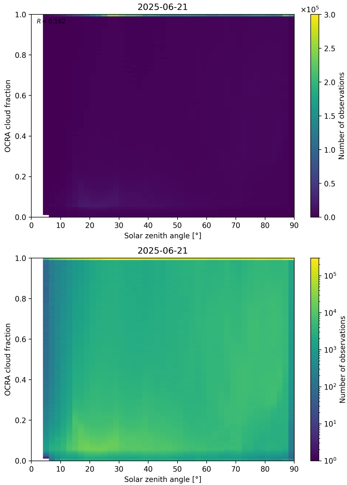
Figure 100: Scatter density plot of “Solar zenith angle” against “OCRA cloud fraction” for 2025-06-20 to 2025-06-22.
