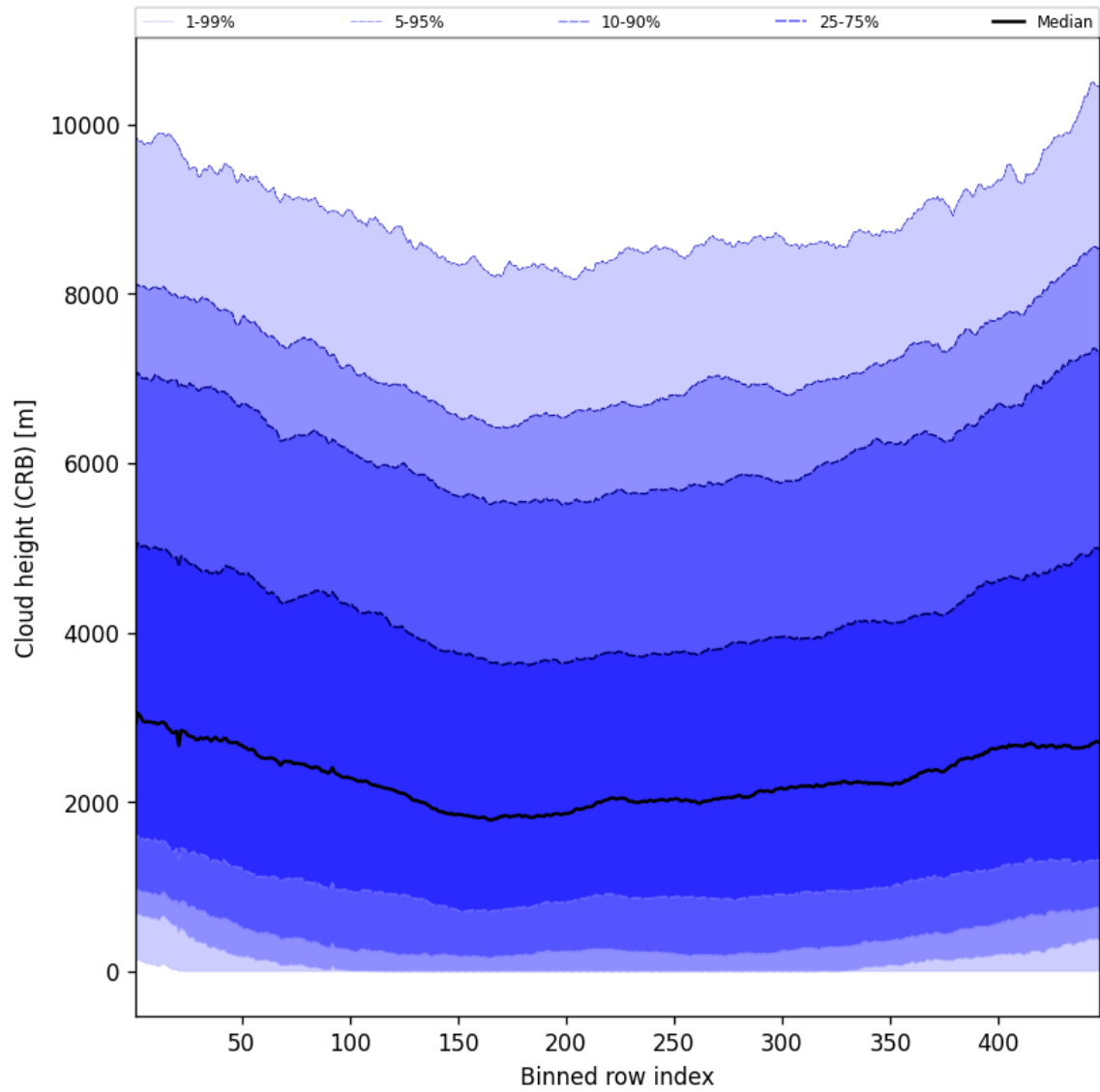
Figure 59: Along track statistics of “Cloud height (CRB)” for 2025-06-20 to 2025-06-22
