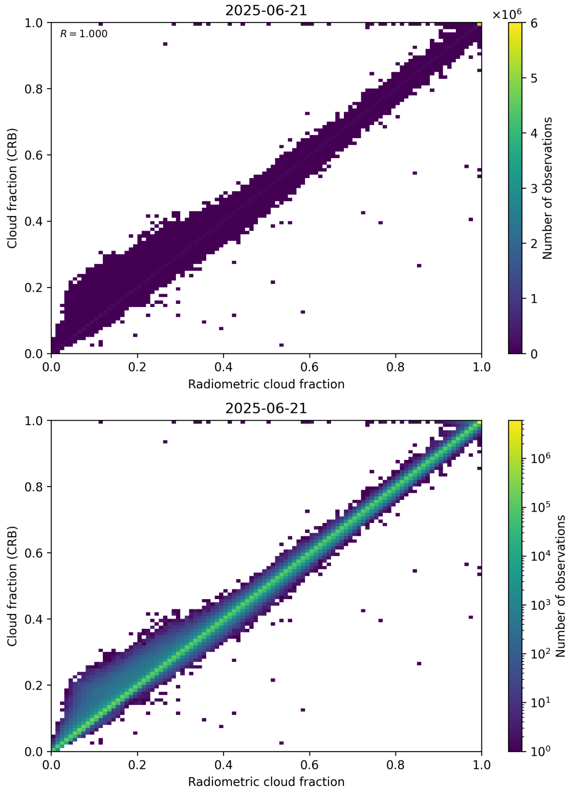
Figure 73: Scatter density plot of “Radiometric cloud fraction” against “Cloud fraction (CRB)” for 2025-06-20 to 2025-06-22.
