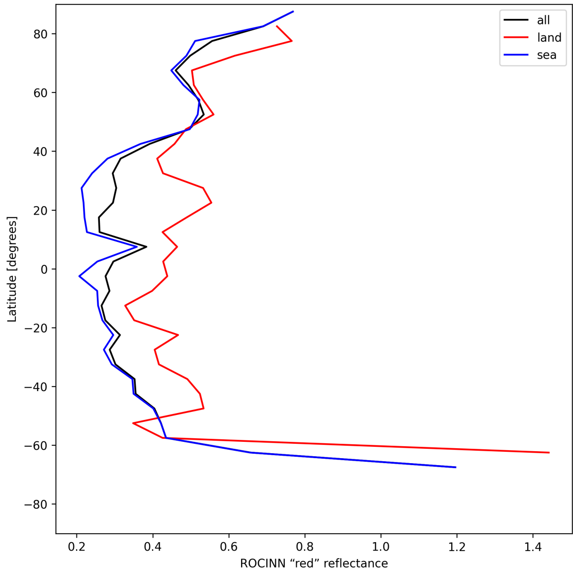
Figure 37: Zonal average of "ROCINN "red" reflectance" for 2025-06-20 to 2025-06-22.
