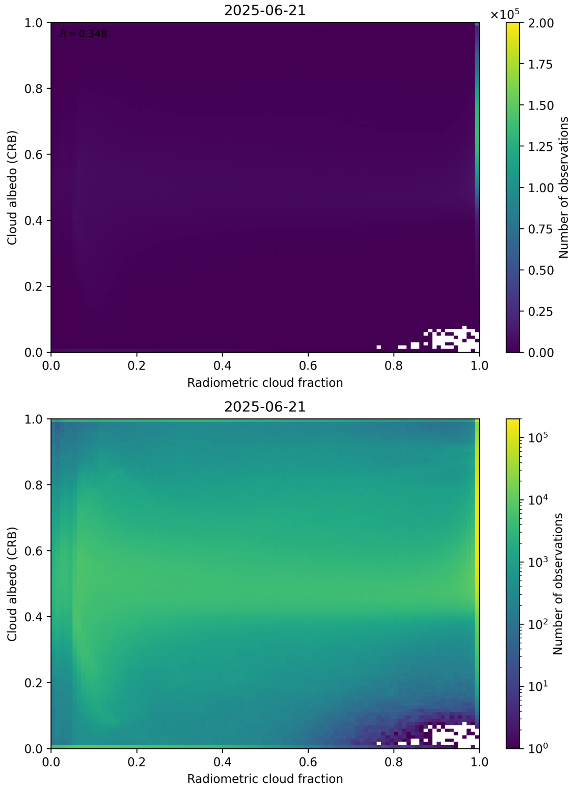
Figure 71: Scatter density plot of “Radiometric cloud fraction” against “Cloud albedo (CRB)” for 2025-06-20 to 2025-06-22.
