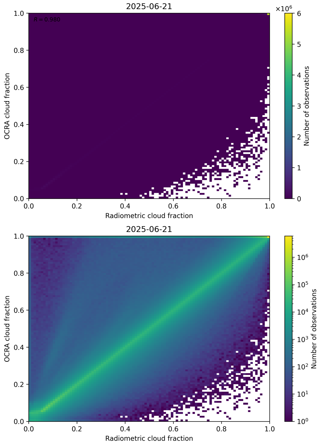
Figure 72: Scatter density plot of “Radiometric cloud fraction” against “OCRA cloud fraction” for 2025-06-20 to 2025-06-22.
