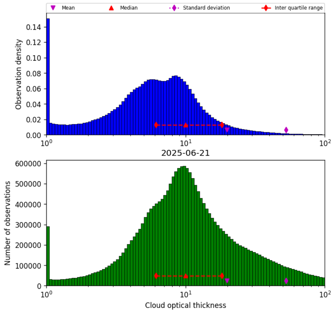
Figure 41: Histogram of “Cloud optical thickness” for 2025-06-20 to 2025-06-22
