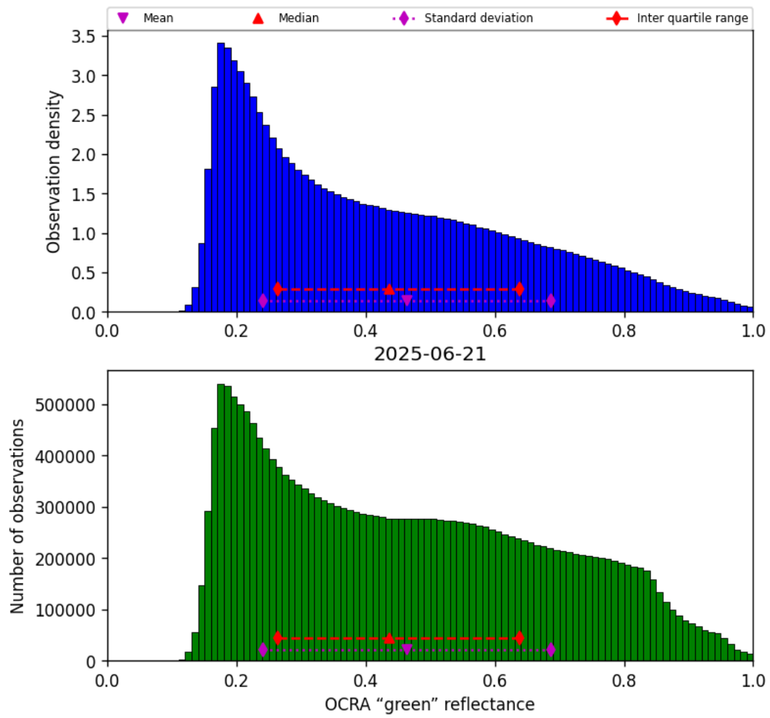
Figure 52: Histogram of “OCRA “green” reflectance” for 2025-06-20 to 2025-06-22
