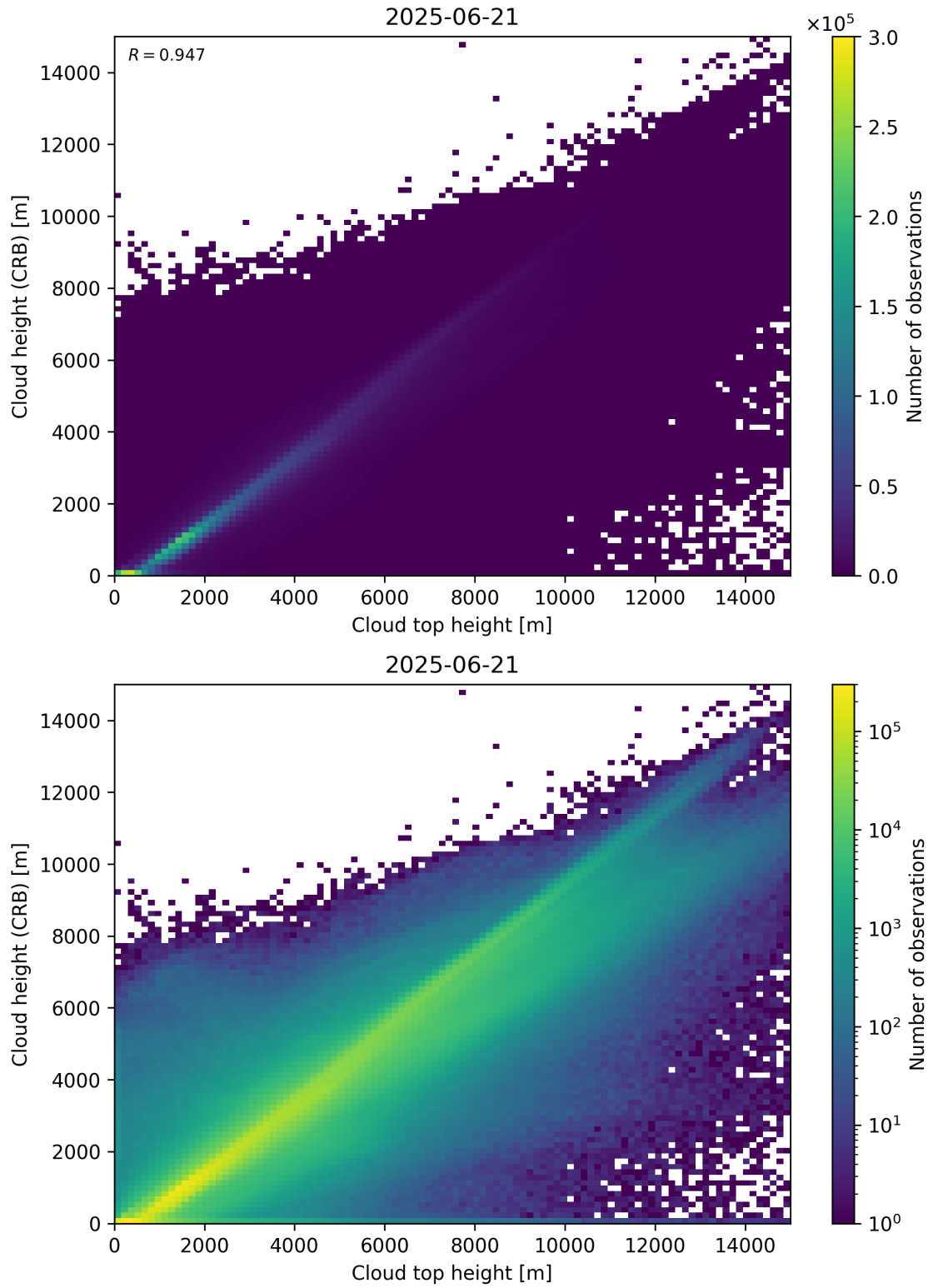
Figure 89: Scatter density plot of “Cloud top height” against “Cloud height (CRB)” for 2025-06-20 to 2025-06-22.
