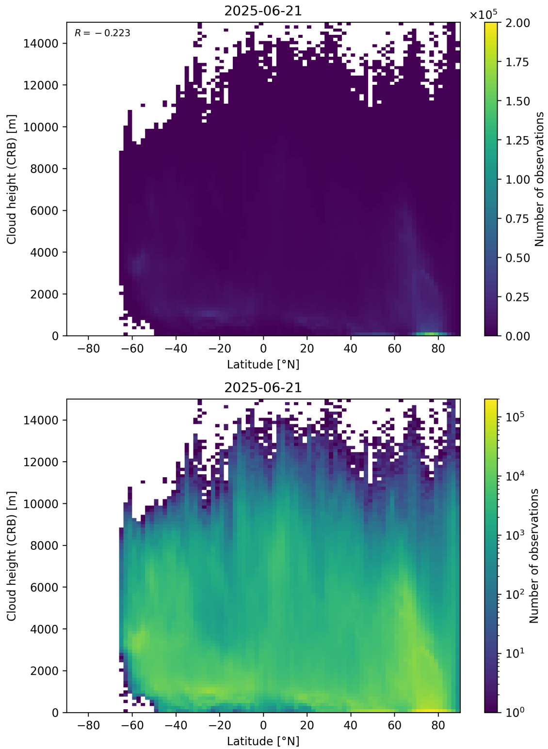
Figure 95: Scatter density plot of “Latitude” against “Cloud height (CRB)” for 2025-06-20 to 2025-06-22.
