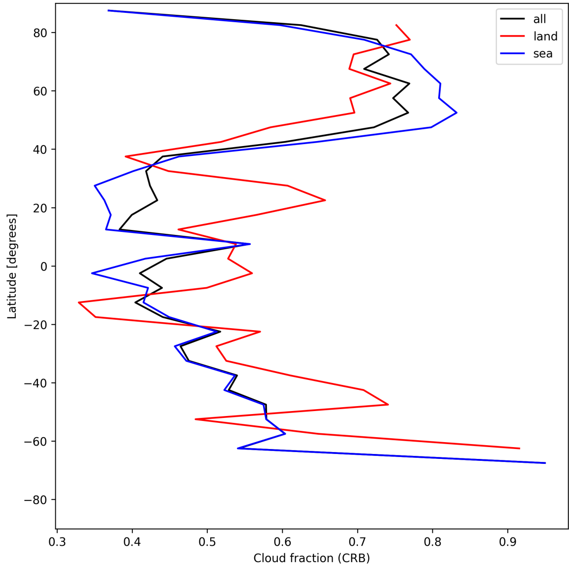
Figure 26: Zonal average of “Cloud fraction (CRB)” for 2025-06-20 to 2025-06-22.
