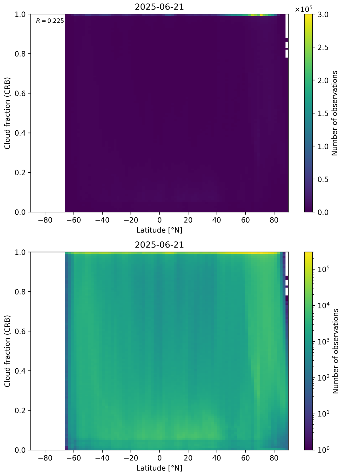
Figure 94: Scatter density plot of “Latitude” against “Cloud fraction (CRB)” for 2025-06-20 to 2025-06-22.
