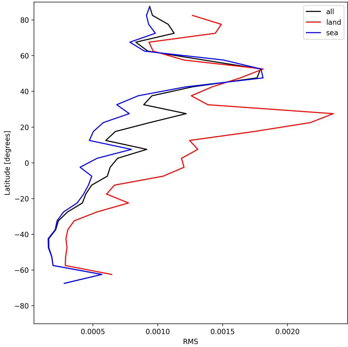
Figure 31: Zonal average of “RMS” for 2025-06-20 to 2025-06-22.
