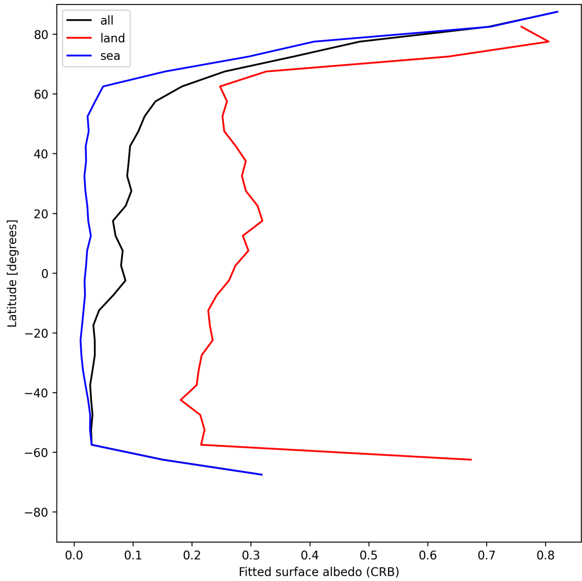
Figure 30: Zonal average of “Fitted surface albedo (CRB)” for 2025-06-20 to 2025-06-22.
