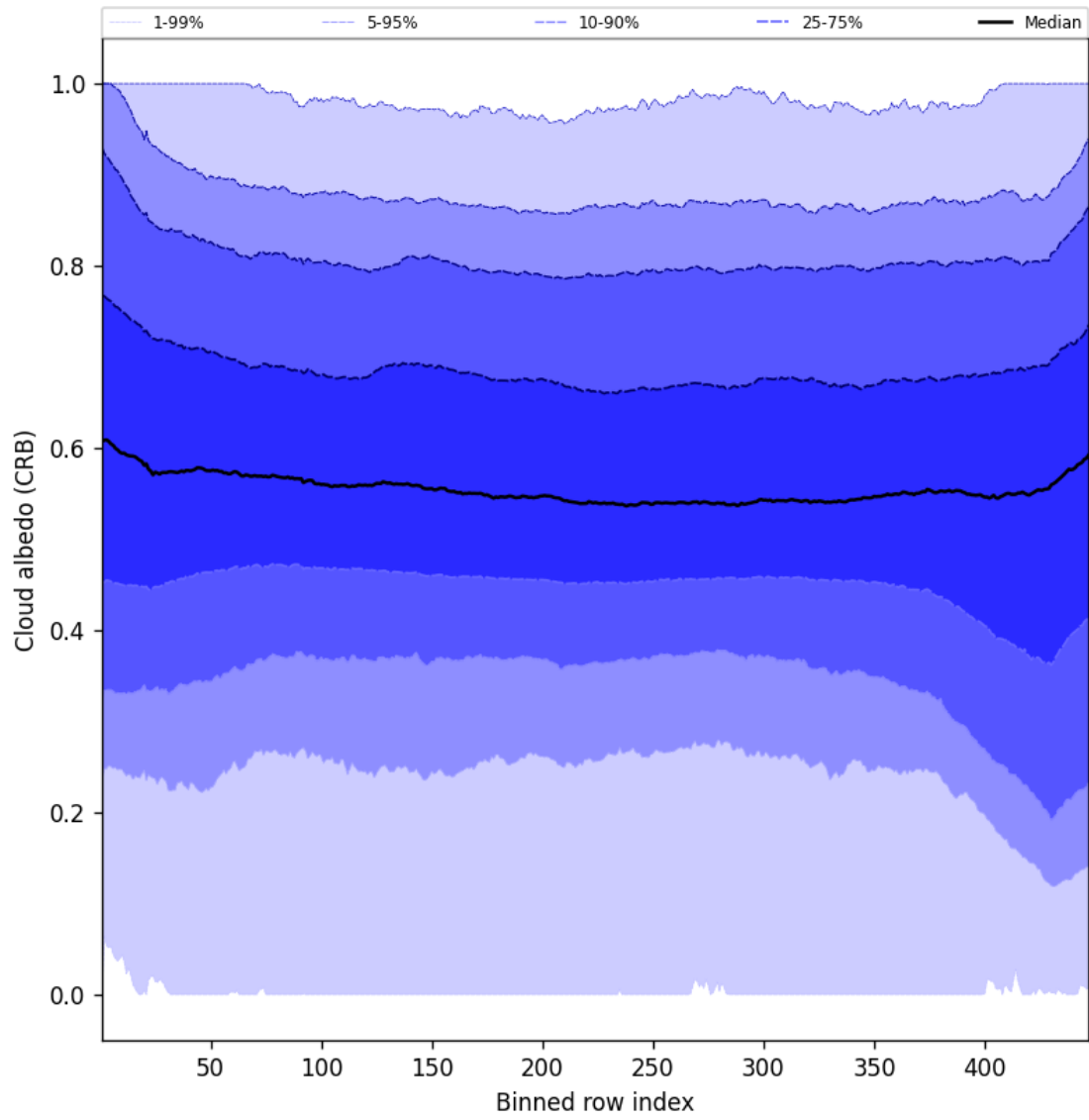
Figure 60: Along track statistics of “Cloud albedo (CRB)” for 2025-06-20 to 2025-06-22
