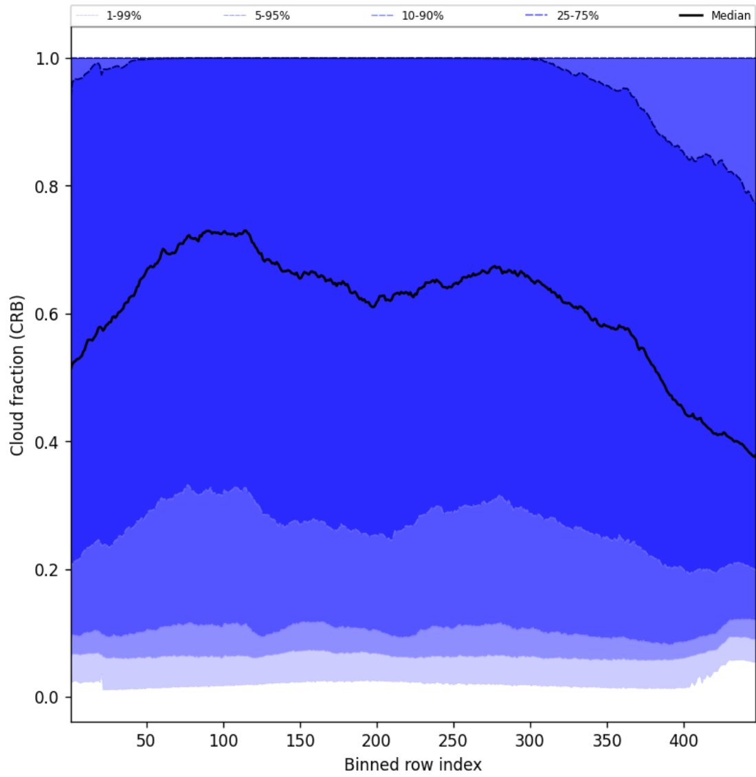
Figure 58: Along track statistics of “Cloud fraction (CRB)” for 2025-06-20 to 2025-06-22
