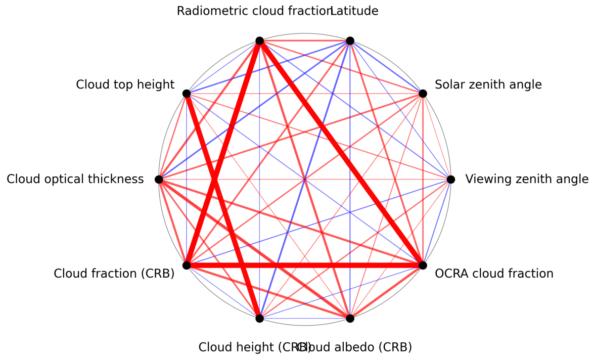
Figure 1: Map of correlation graph for 2025-06-20 to 2025-06-22.
