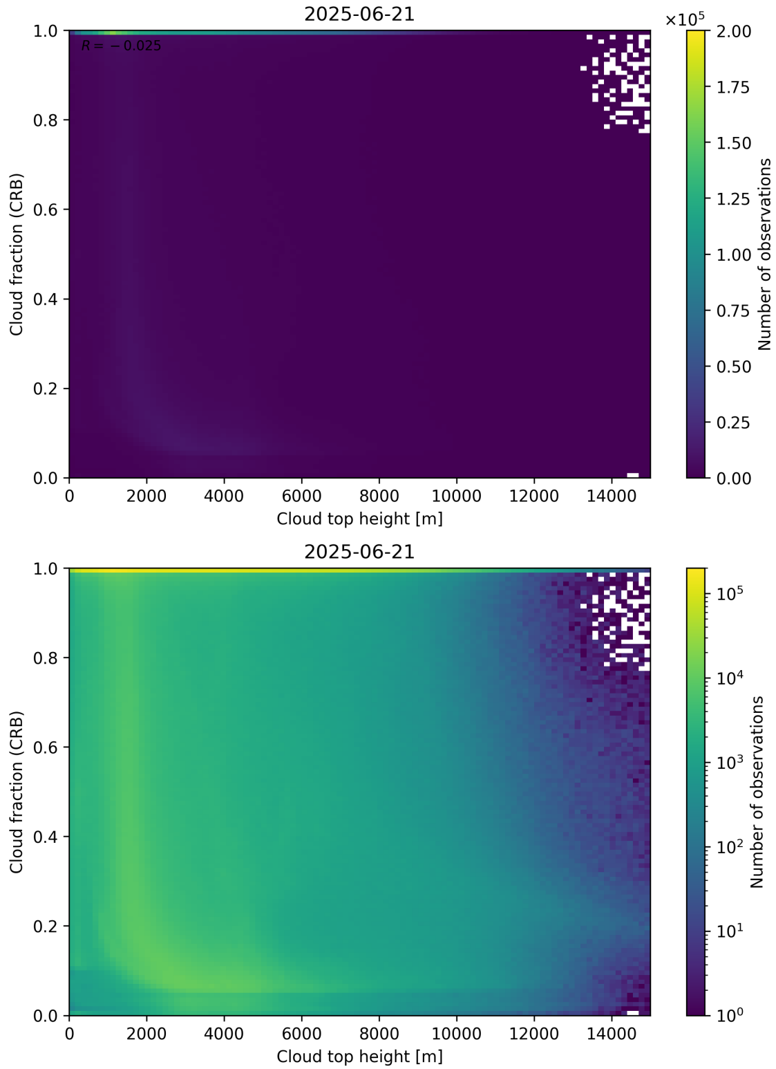
Figure 88: Scatter density plot of “Cloud top height” against “Cloud fraction (CRB)” for 2025-06-20 to 2025-06-22.
