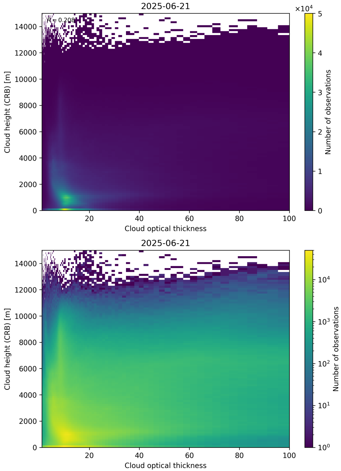
Figure 85: Scatter density plot of “Cloud optical thickness” against “Cloud height (CRB)” for 2025-06-20 to 2025-06-22.
