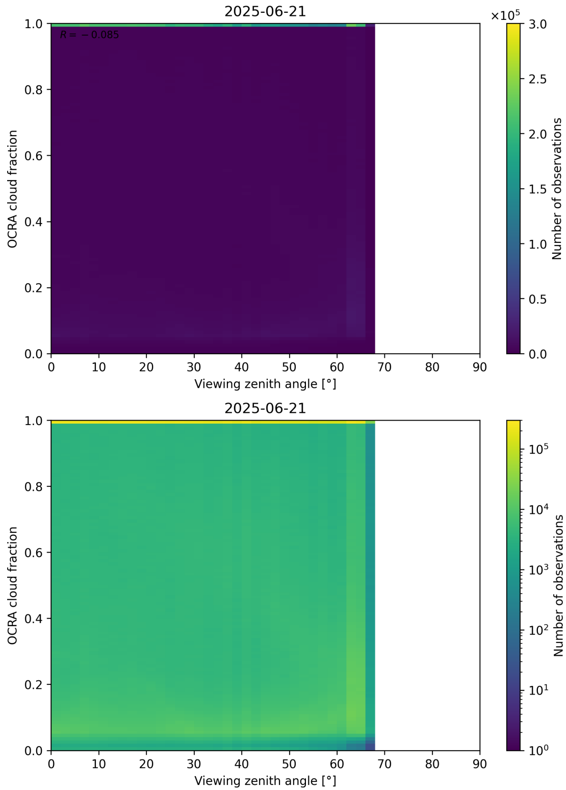
Figure 108: Scatter density plot of “Viewing zenith angle” against “OCRA cloud fraction” for 2025-06-20 to 2025-06-22.
