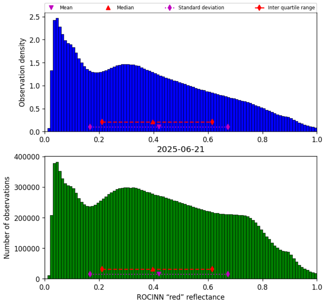
Figure 53: Histogram of “ROCINN “red” reflectance” for 2025-06-20 to 2025-06-22
