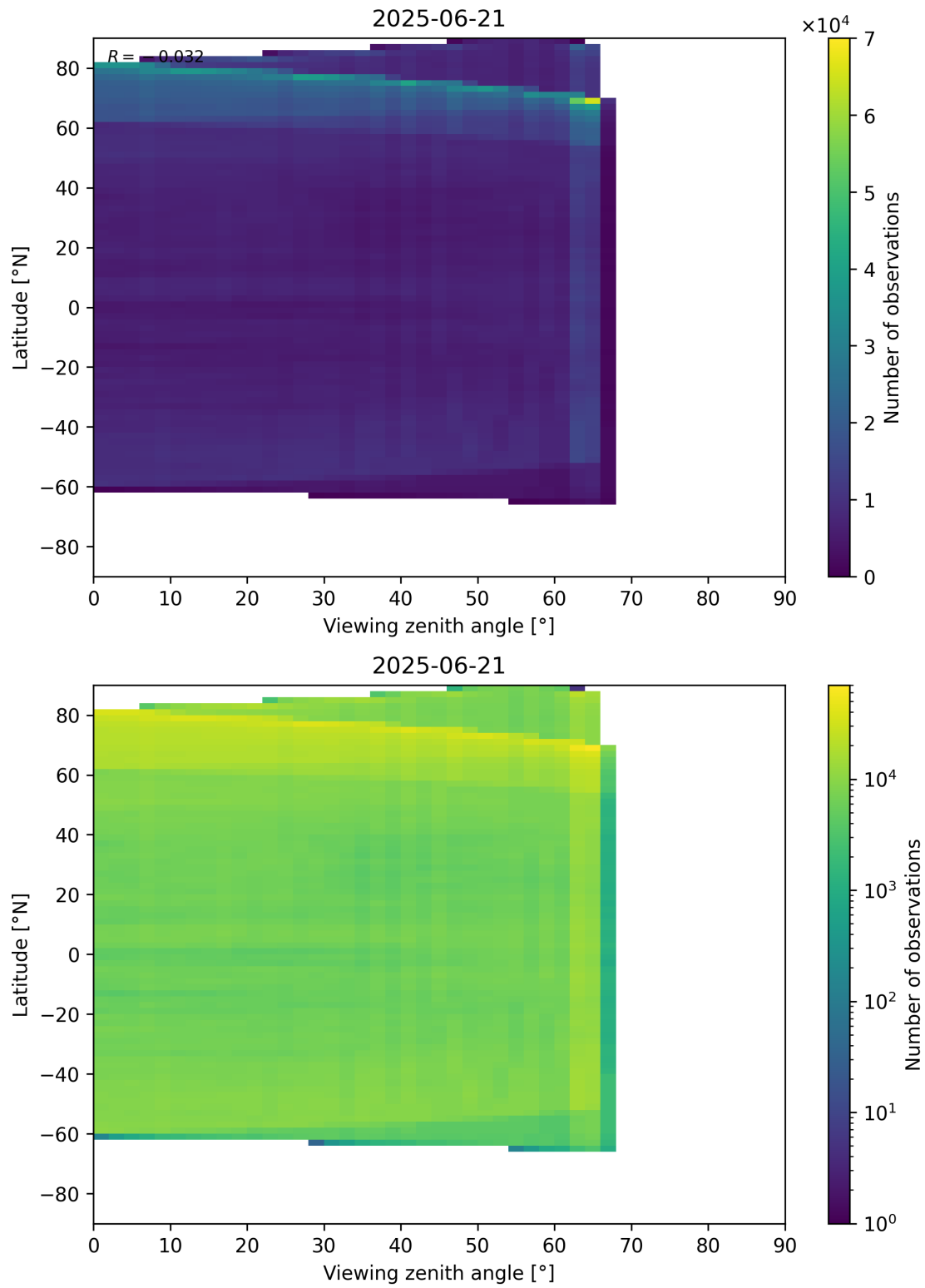
Figure 113: Scatter density plot of “Viewing zenith angle” against “Latitude” for 2025-06-20 to 2025-06-22.
