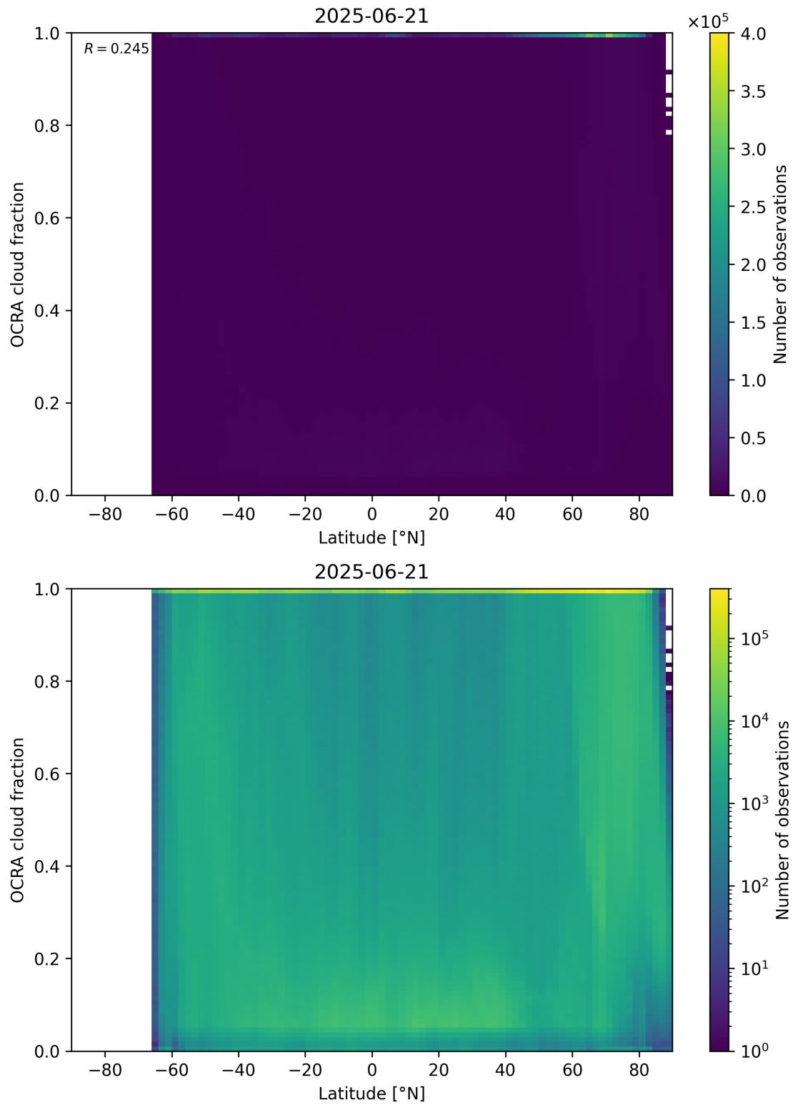
Figure 93: Scatter density plot of “Latitude” against “OCRA cloud fraction” for 2025-06-20 to 2025-06-22.
