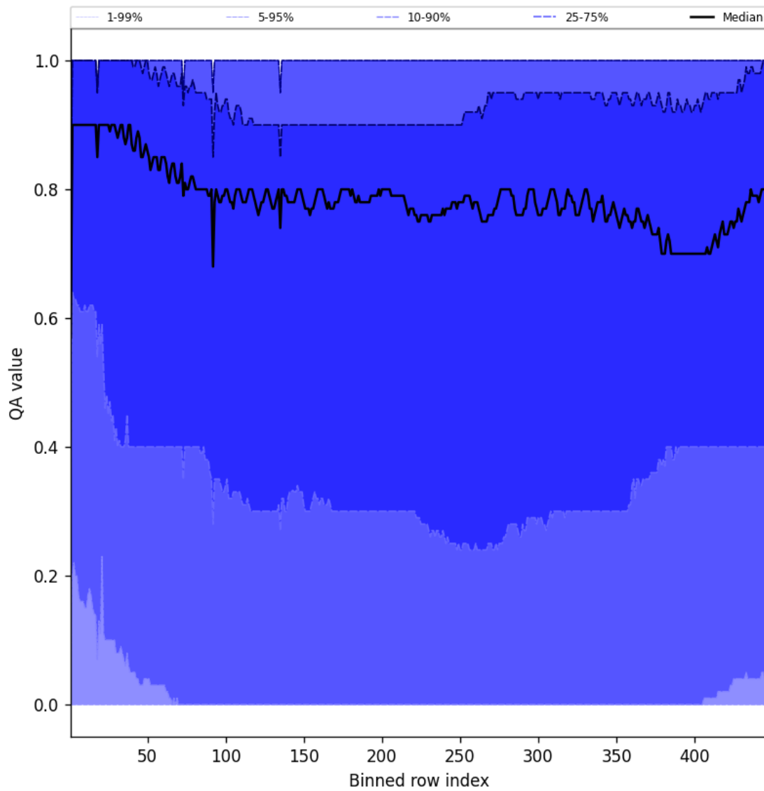
Figure 54: Along track statistics of “QA value” for 2025-06-20 to 2025-06-22
