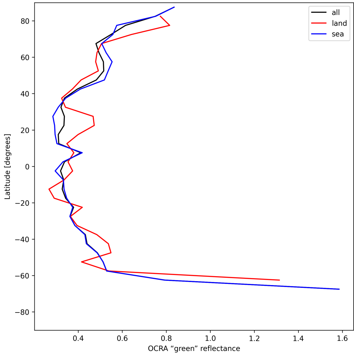
Figure 36: Zonal average of “OCRA “green” reflectance” for 2025-06-20 to 2025-06-22.
