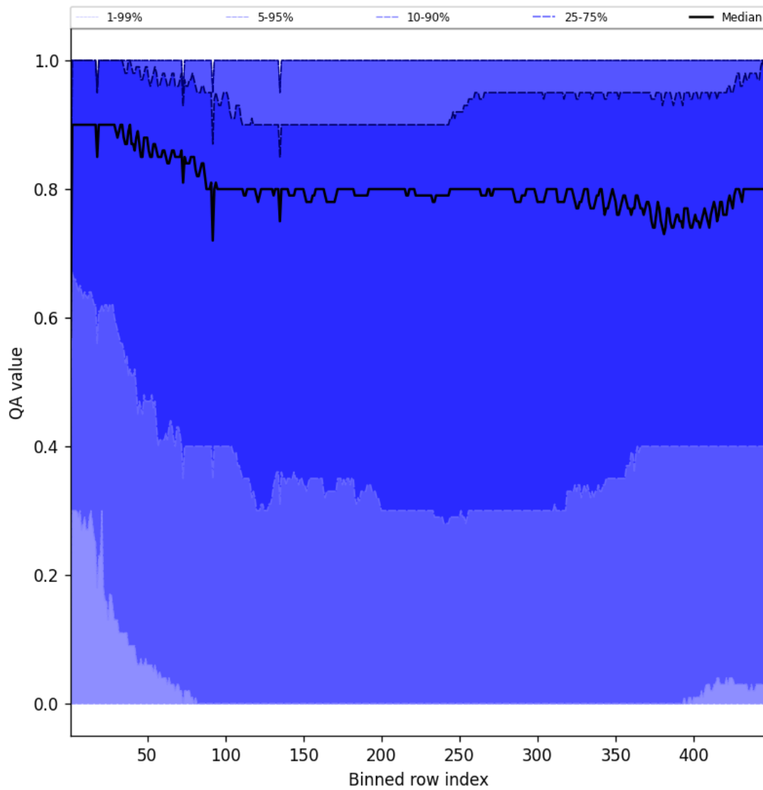
Figure 54: Along track statistics of “QA value” for 2025-06-22 to 2025-06-24
