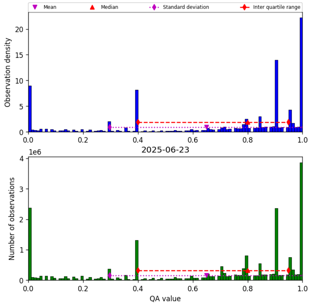
Figure 38: Histogram of “QA value” for 2025-06-22 to 2025-06-24
