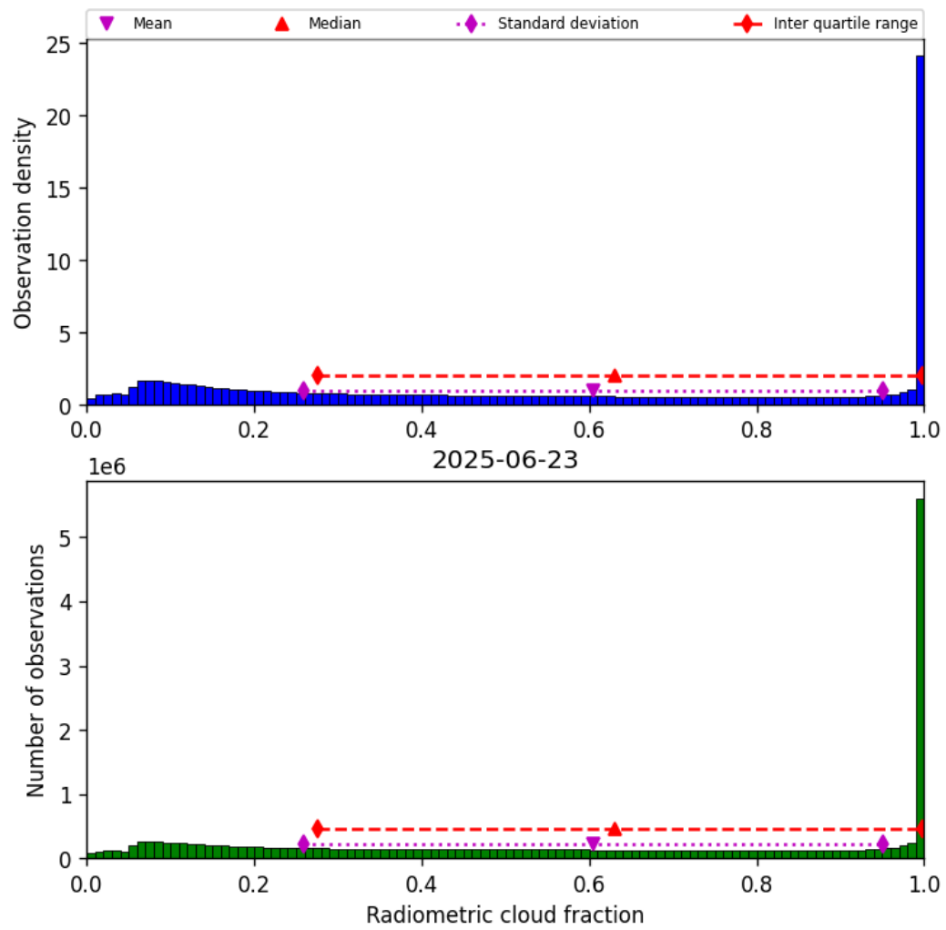
Figure 39: Histogram of “Radiometric cloud fraction” for 2025-06-22 to 2025-06-24
