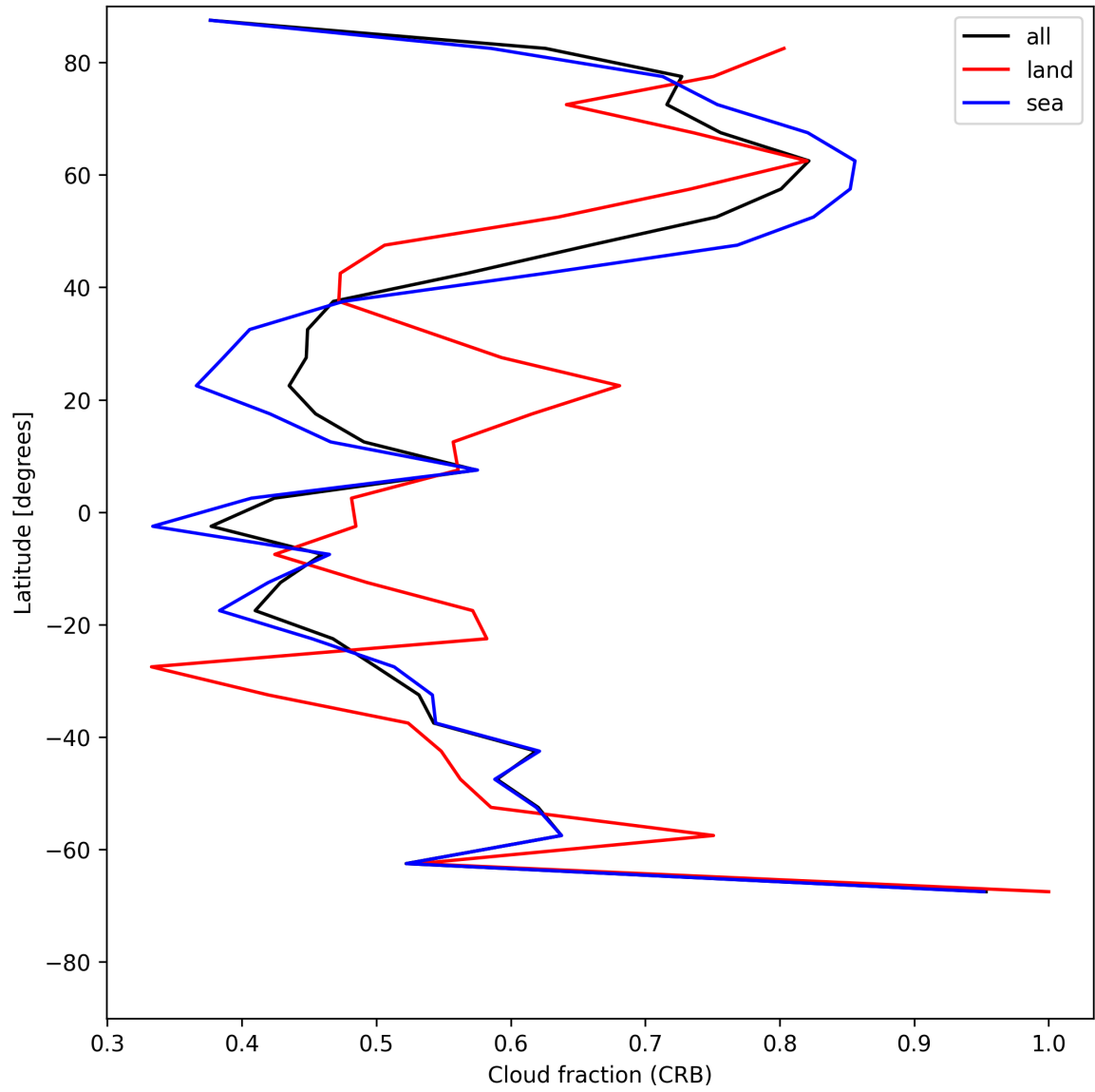
Figure 26: Zonal average of “Cloud fraction (CRB)” for 2025-06-22 to 2025-06-24.
