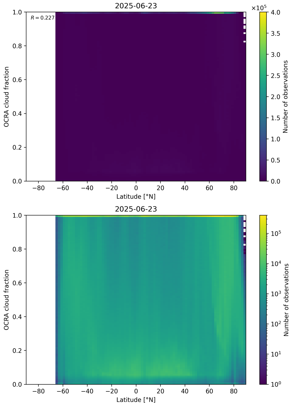
Figure 93: Scatter density plot of “Latitude” against “OCRA cloud fraction” for 2025-06-22 to 2025-06-24.
