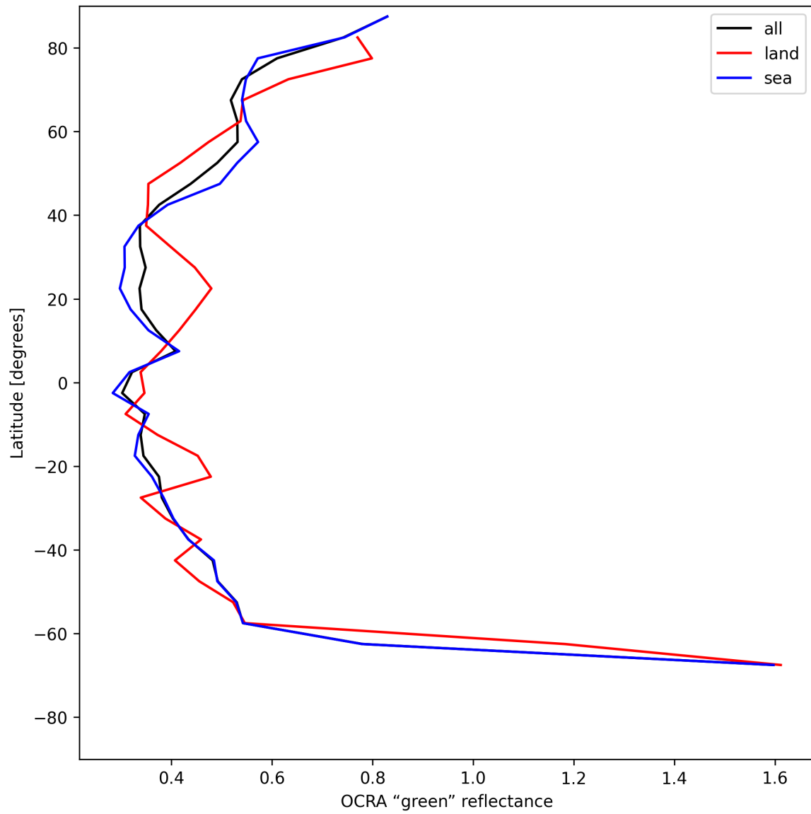
Figure 36: Zonal average of “OCRA “green” reflectance” for 2025-06-22 to 2025-06-24.
