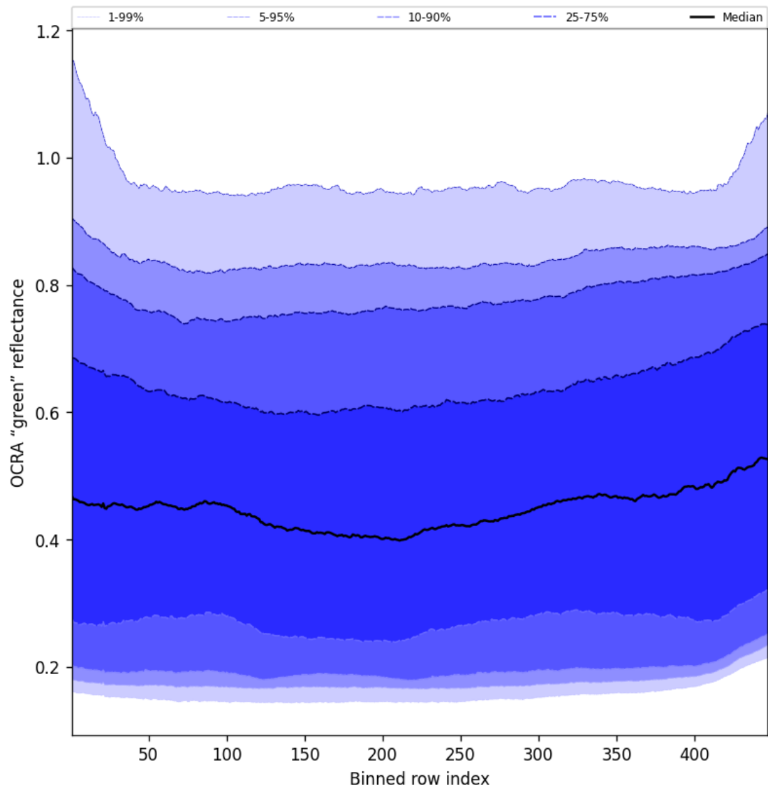
Figure 68: Along track statistics of “OCRA “green” reflectance” for 2025-06-22 to 2025-06-24
