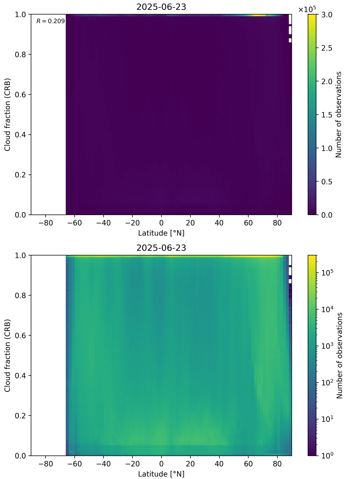
Figure 94: Scatter density plot of “Latitude” against “Cloud fraction (CRB)” for 2025-06-22 to 2025-06-24.
