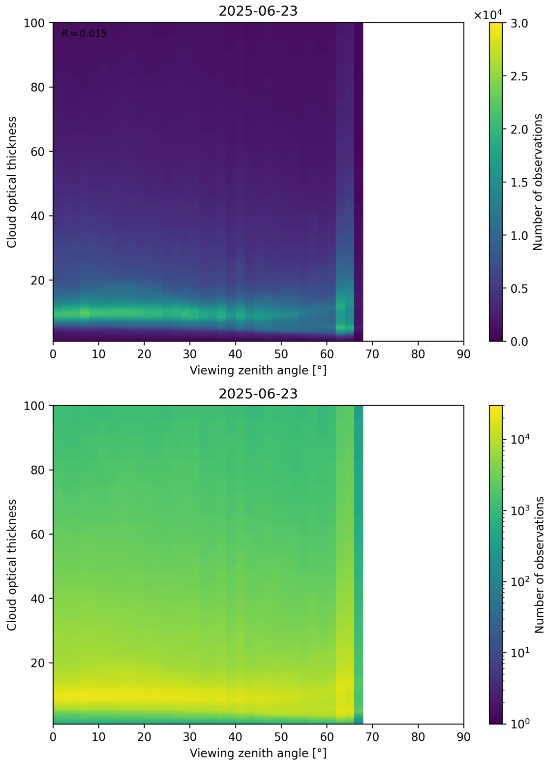
Figure 111: Scatter density plot of “Viewing zenith angle” against “Cloud optical thickness” for 2025-06-22 to 2025-06-24.
