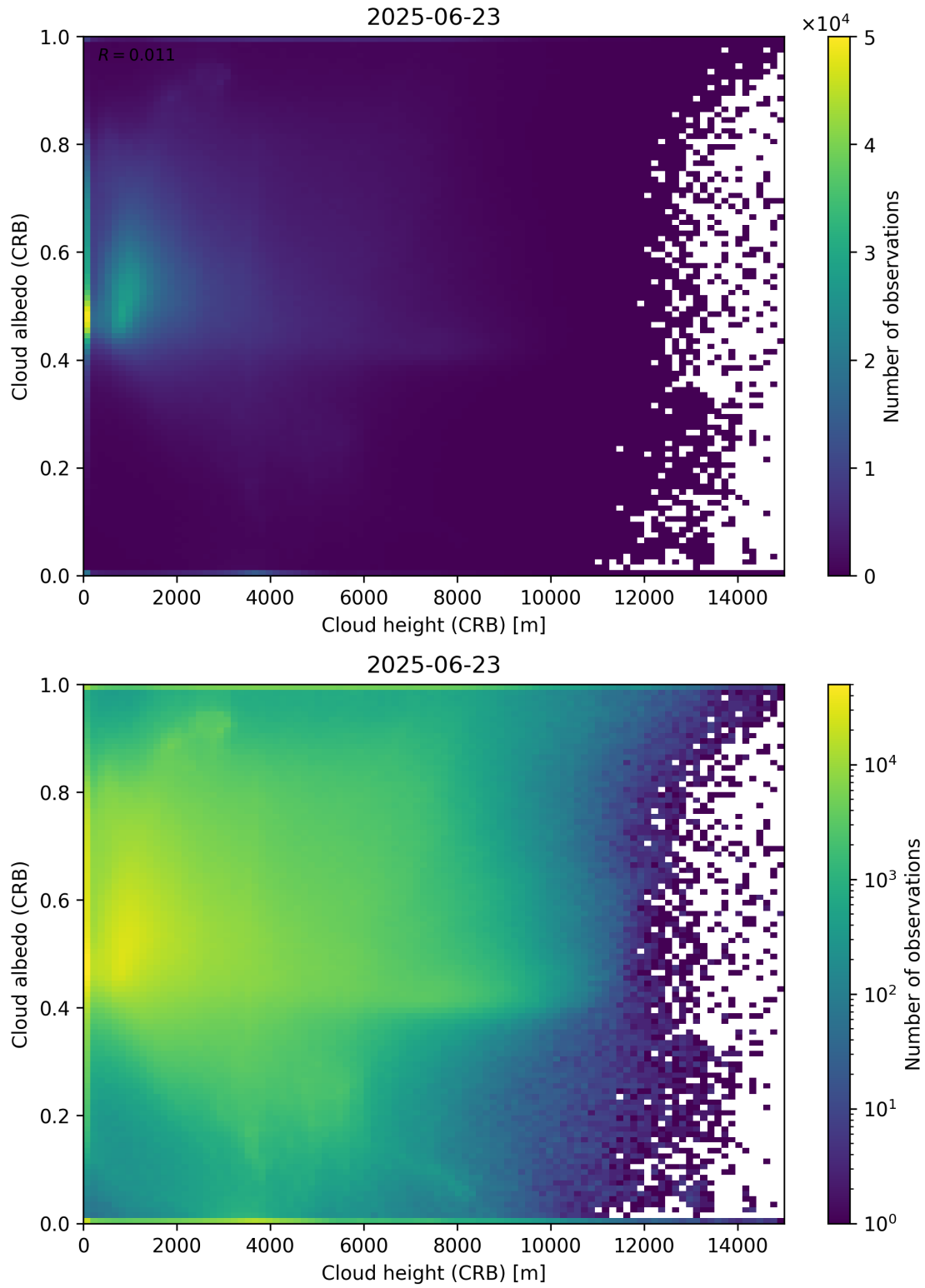
Figure 80: Scatter density plot of “Cloud height (CRB)” against “Cloud albedo (CRB)” for 2025-06-22 to 2025-06-24.
