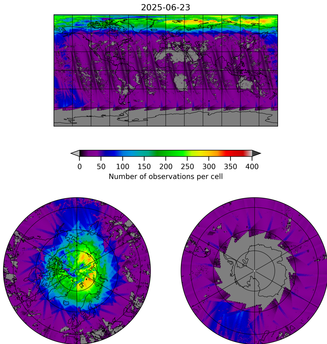
Figure 21: Map of the number of observations for 2025-06-22 to 2025-06-24
