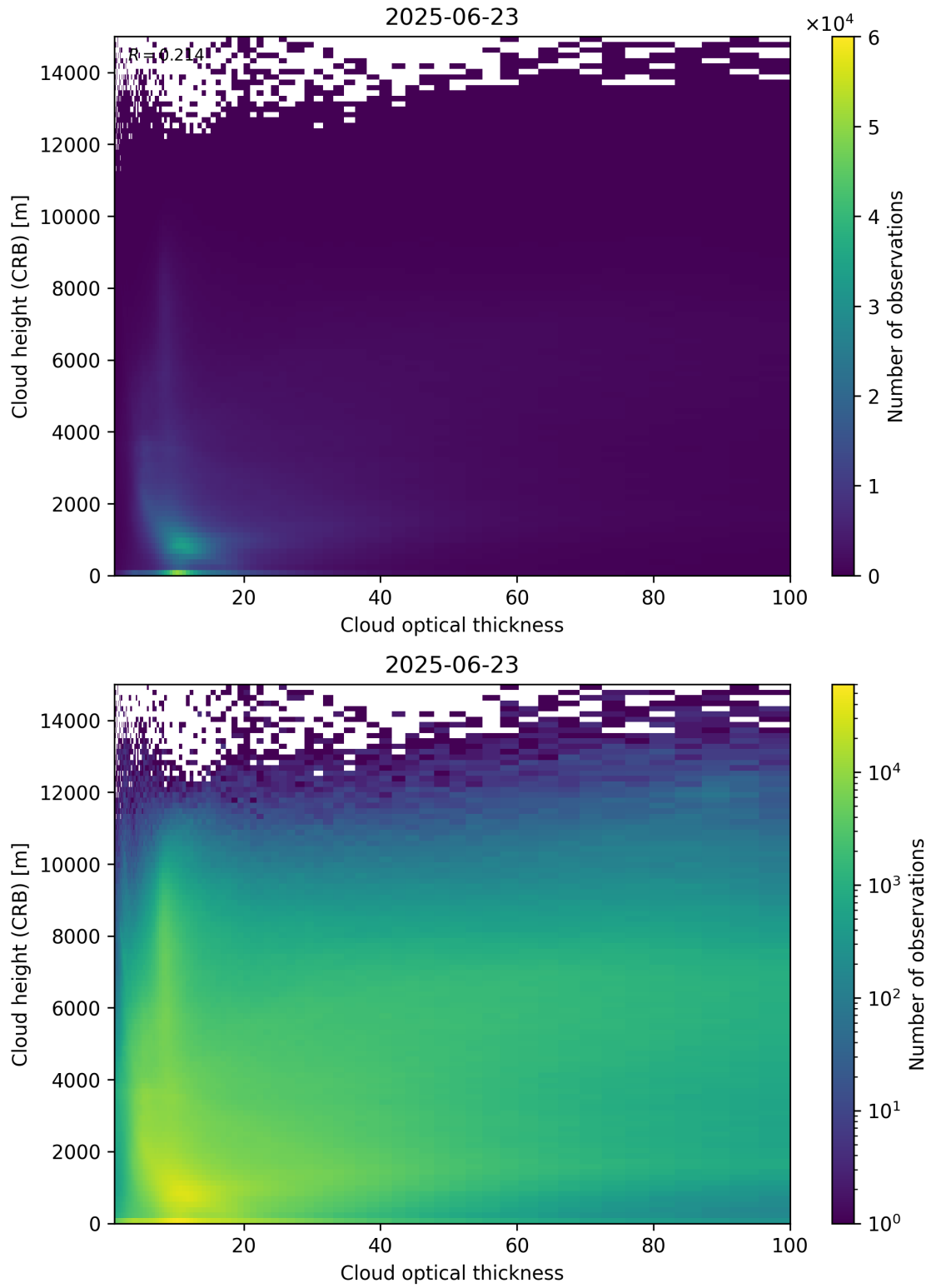
Figure 85: Scatter density plot of “Cloud optical thickness” against “Cloud height (CRB)” for 2025-06-22 to 2025-06-24.
