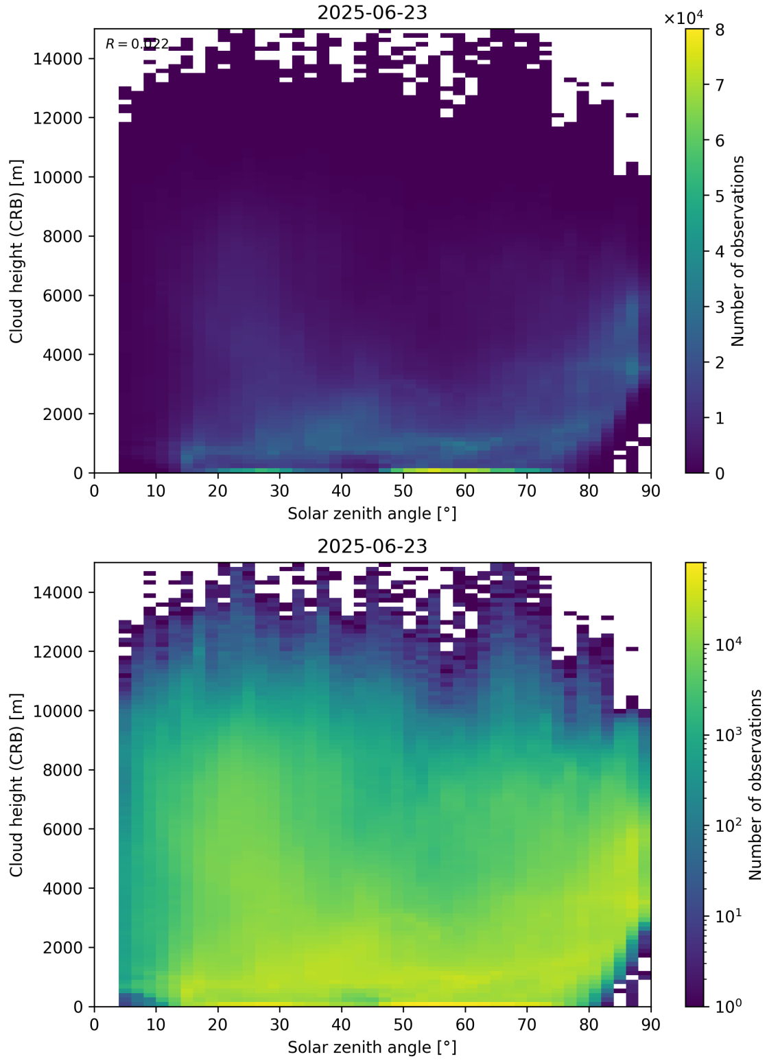
Figure 102: Scatter density plot of “Solar zenith angle” against “Cloud height (CRB)” for 2025-06-22 to 2025-06-24.
