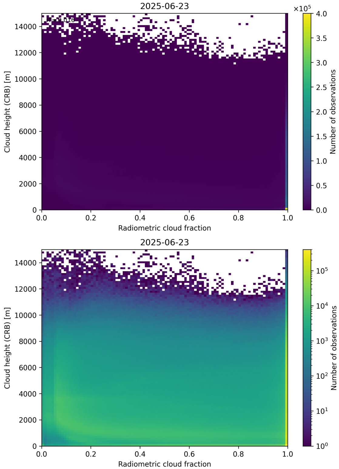
Figure 74: Scatter density plot of “Radiometric cloud fraction” against “Cloud height (CRB)” for 2025-06-22 to 2025-06-24.
