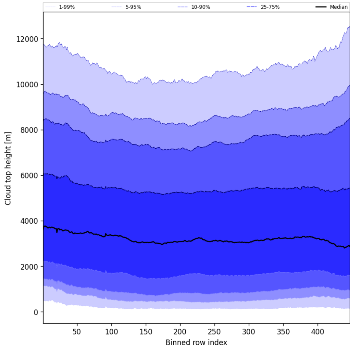
Figure 56: Along track statistics of “Cloud top height” for 2025-06-22 to 2025-06-24
