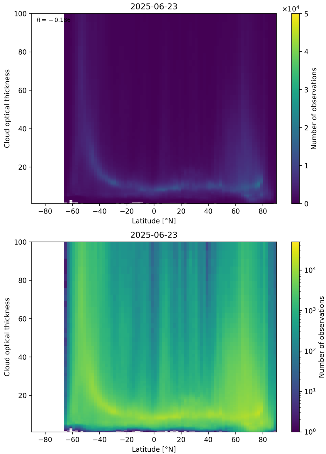
Figure 96: Scatter density plot of “Latitude” against “Cloud optical thickness” for 2025-06-22 to 2025-06-24.
