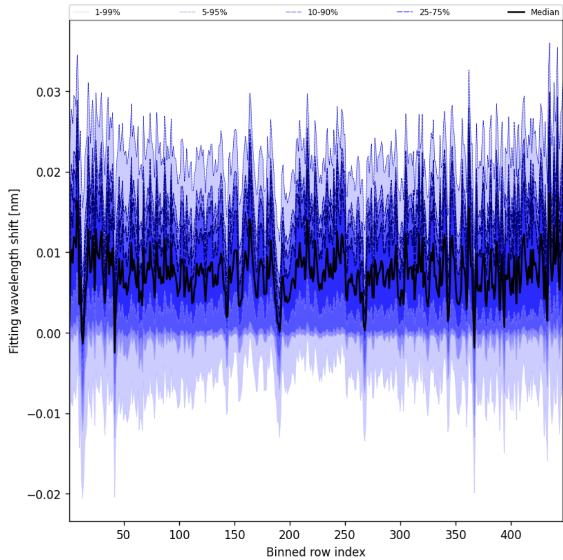
Figure 65: Along track statistics of “Fitting wavelength shift” for 2025-06-22 to 2025-06-24
