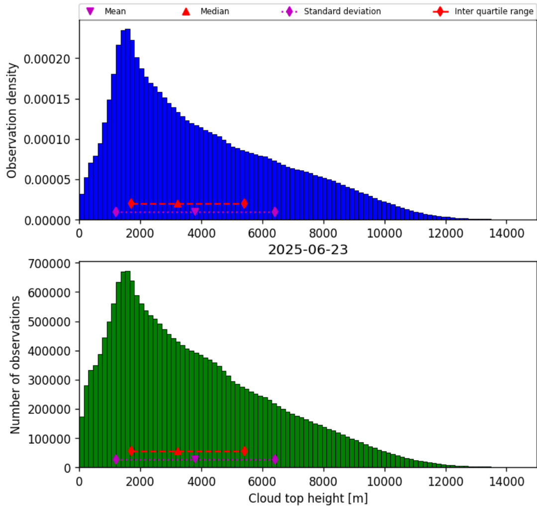
Figure 40: Histogram of “Cloud top height” for 2025-06-22 to 2025-06-24
