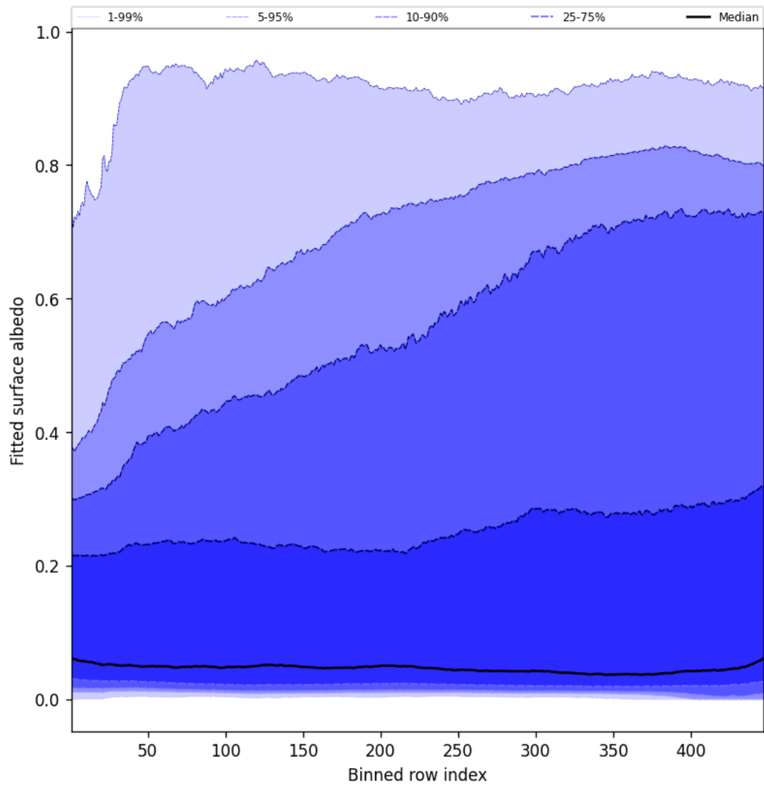
Figure 61: Along track statistics of “Fitted surface albedo” for 2025-06-22 to 2025-06-24
