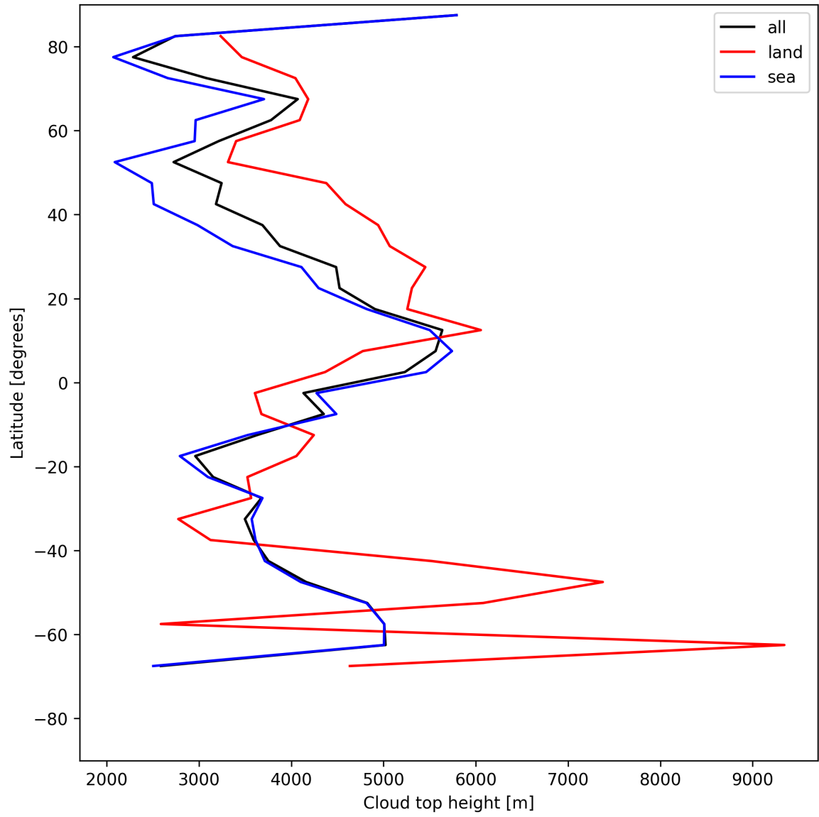
Figure 24: Zonal average of “Cloud top height” for 2025-06-22 to 2025-06-24.
