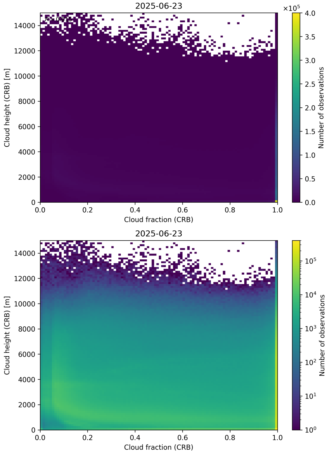
Figure 79: Scatter density plot of “Cloud fraction (CRB)” against “Cloud height (CRB)” for 2025-06-22 to 2025-06-24.
