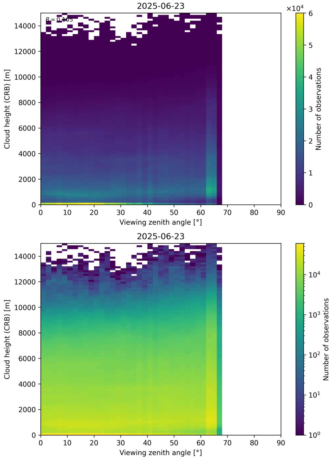
Figure 110: Scatter density plot of “Viewing zenith angle” against “Cloud height (CRB)” for 2025-06-22 to 2025-06-24.
