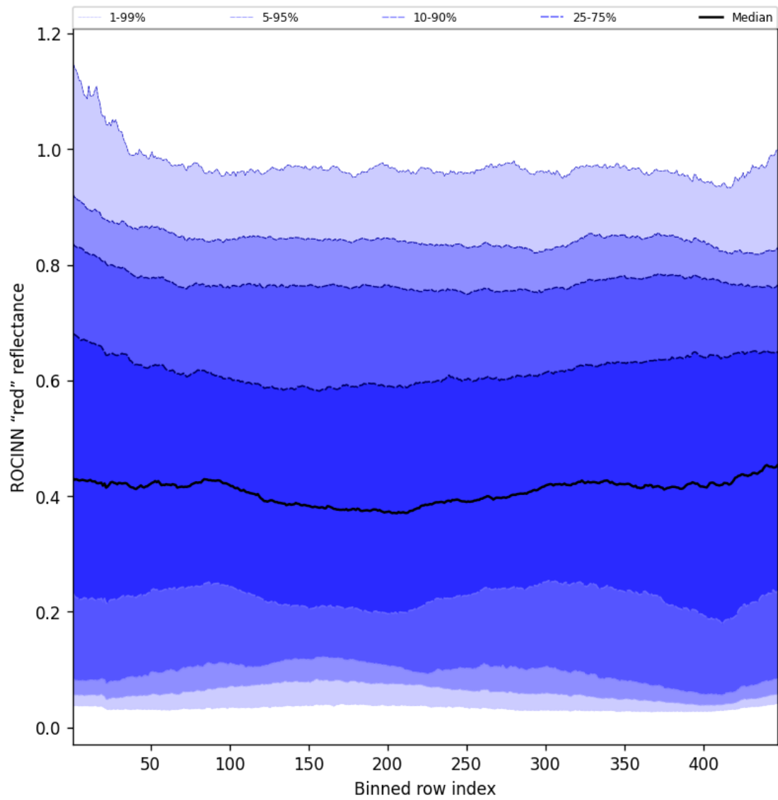
Figure 69: Along track statistics of “ROCINN “red” reflectance” for 2025-06-22 to 2025-06-24
