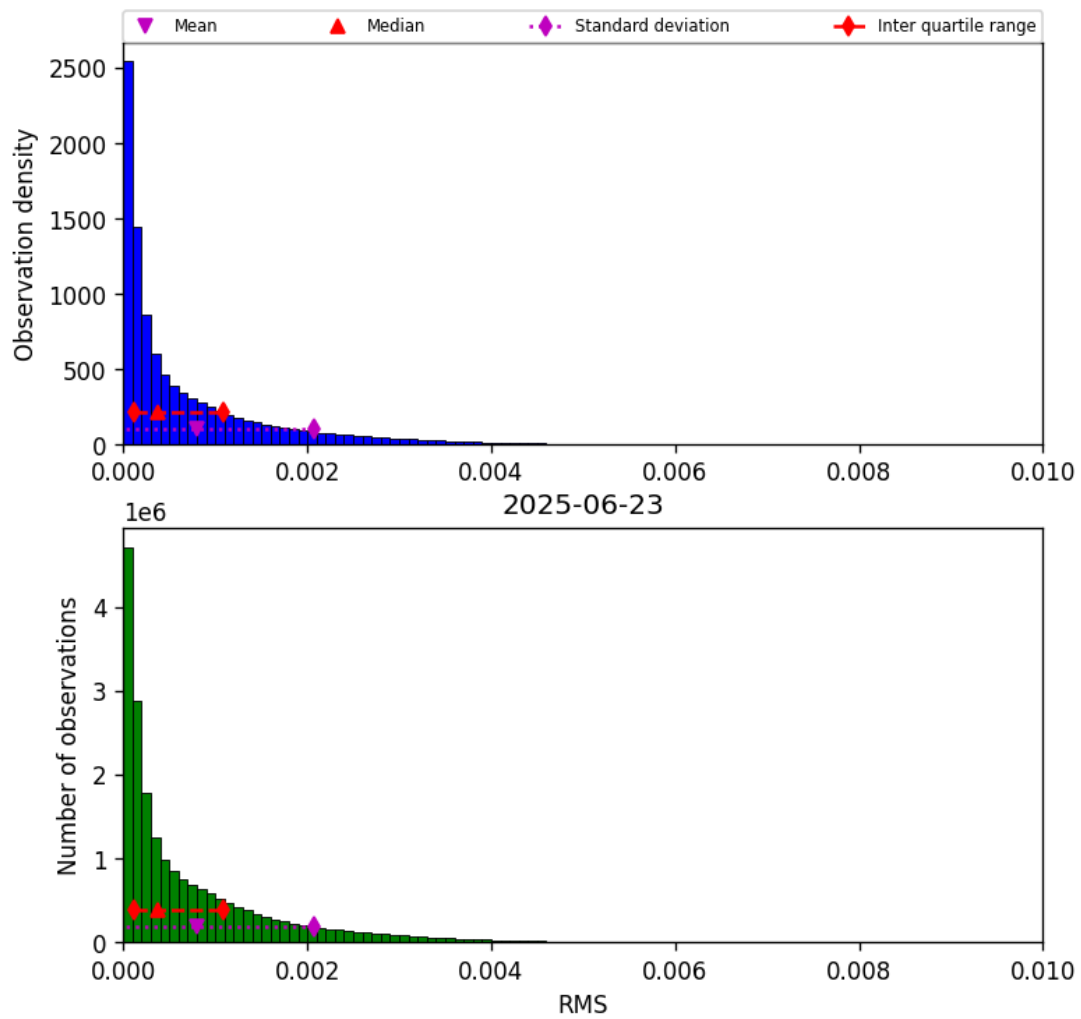
Figure 47: Histogram of “RMS” for 2025-06-22 to 2025-06-24
