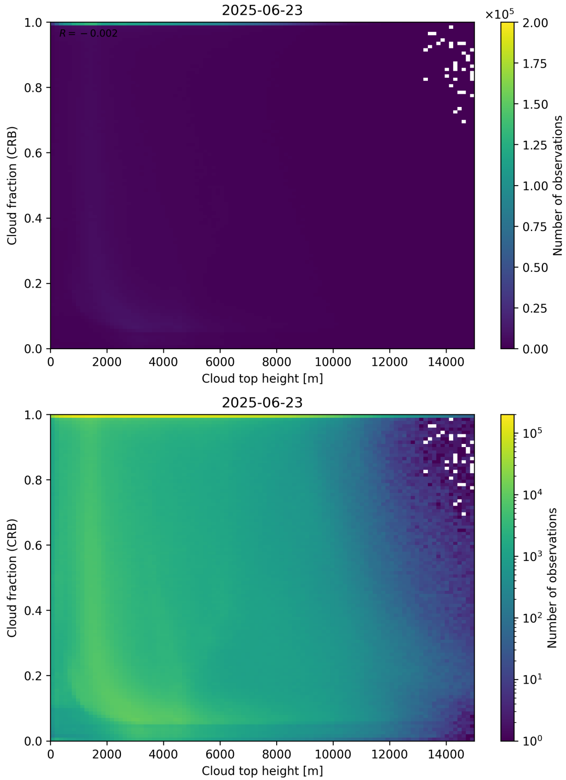
Figure 88: Scatter density plot of “Cloud top height” against “Cloud fraction (CRB)” for 2025-06-22 to 2025-06-24.
