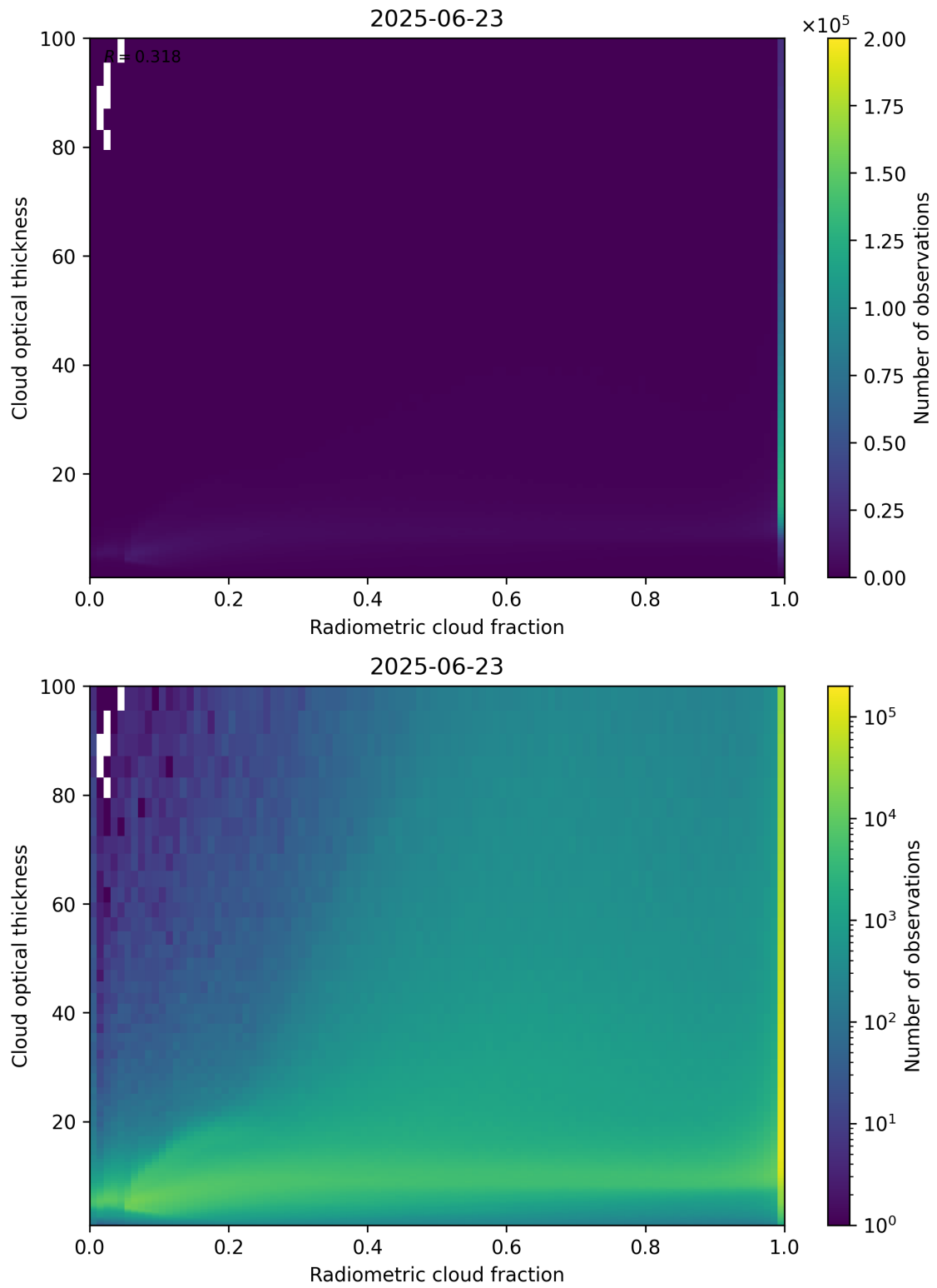
Figure 75: Scatter density plot of “Radiometric cloud fraction” against “Cloud optical thickness” for 2025-06-22 to 2025-06-24.
