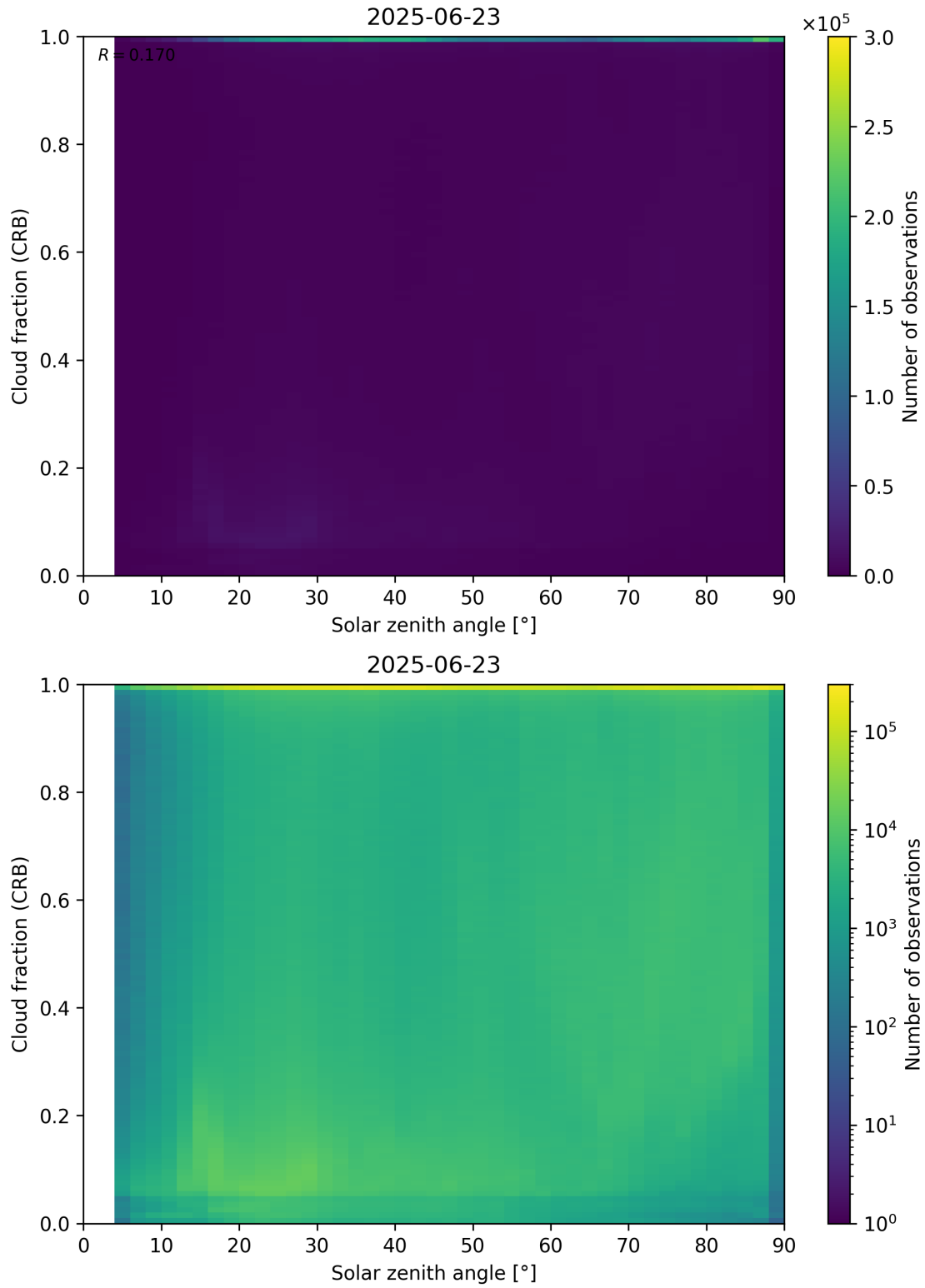
Figure 101: Scatter density plot of “Solar zenith angle” against “Cloud fraction (CRB)” for 2025-06-22 to 2025-06-24.
