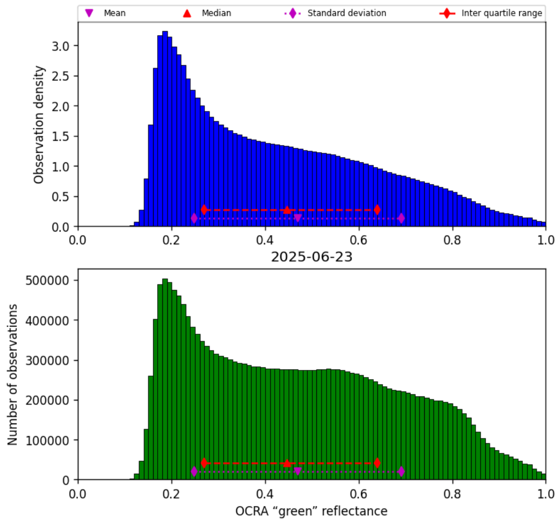
Figure 52: Histogram of “OCRA “green” reflectance” for 2025-06-22 to 2025-06-24
