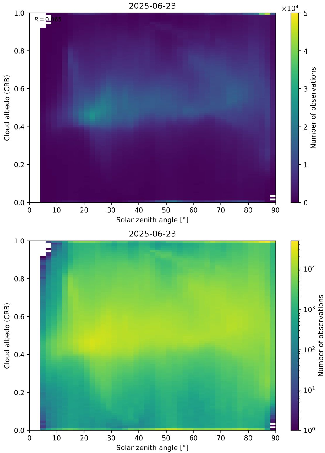
Figure 98: Scatter density plot of “Solar zenith angle” against “Cloud albedo (CRB)” for 2025-06-22 to 2025-06-24.
