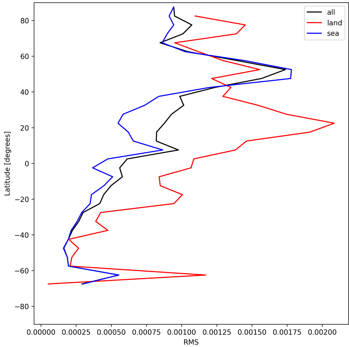
Figure 31: Zonal average of “RMS” for 2025-06-22 to 2025-06-24.
