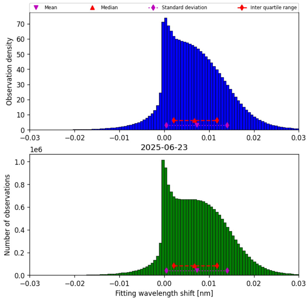
Figure 49: Histogram of “Fitting wavelength shift” for 2025-06-22 to 2025-06-24
