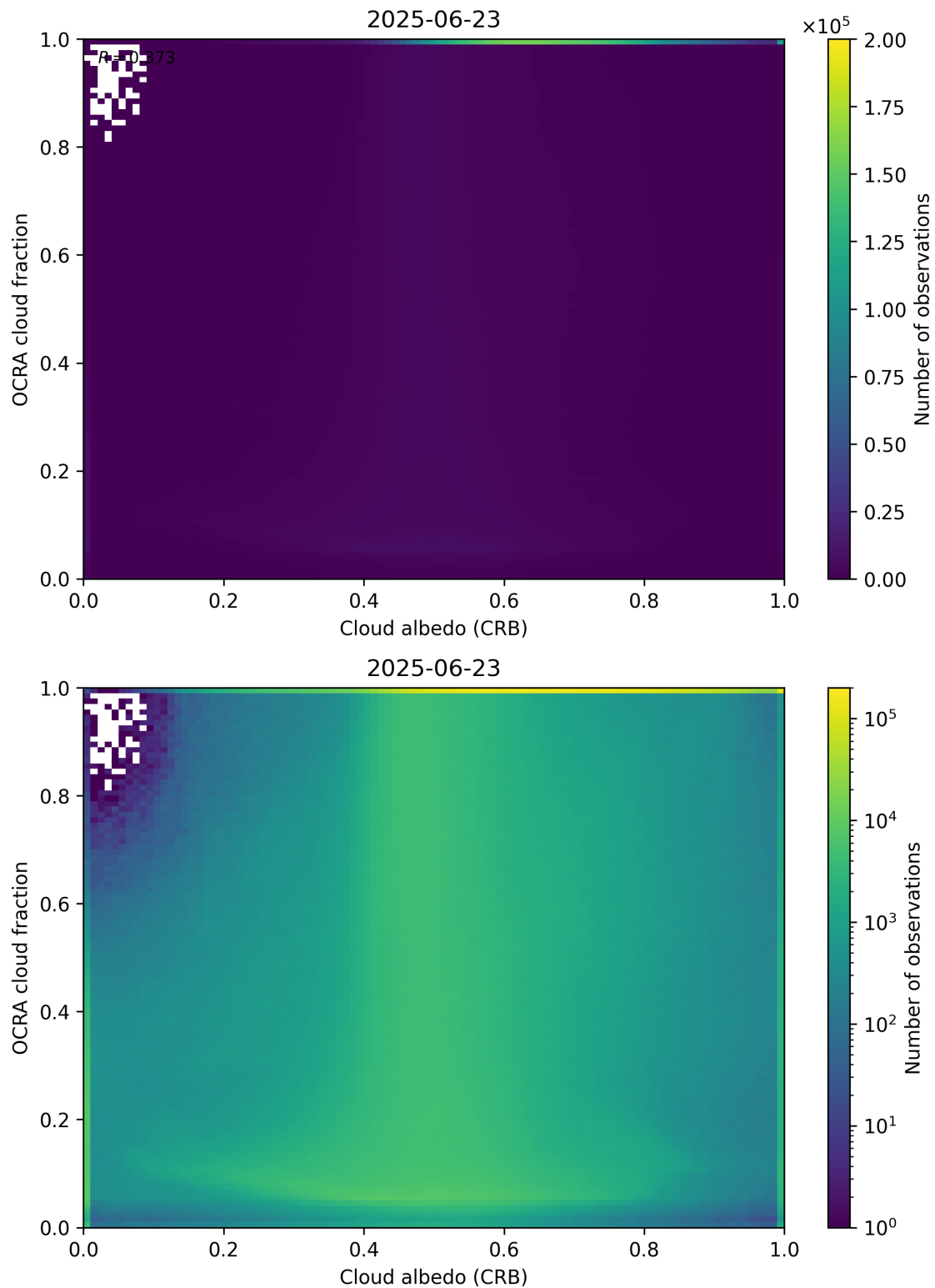
Figure 70: Scatter density plot of “Cloud albedo (CRB)” against “OCRA cloud fraction” for 2025-06-22 to 2025-06-24.
