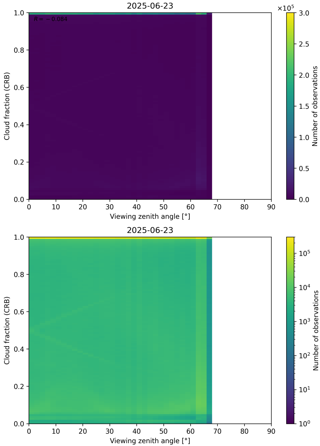
Figure 109: Scatter density plot of “Viewing zenith angle” against “Cloud fraction (CRB)” for 2025-06-22 to 2025-06-24.
