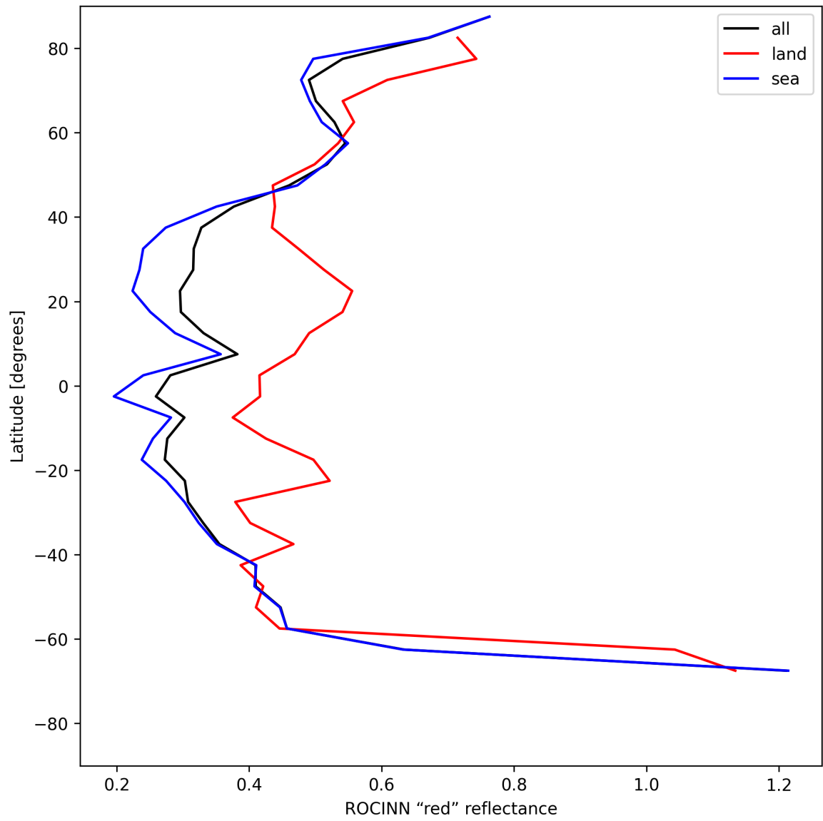
Figure 37: Zonal average of “ROCINN “red” reflectance” for 2025-06-22 to 2025-06-24.
