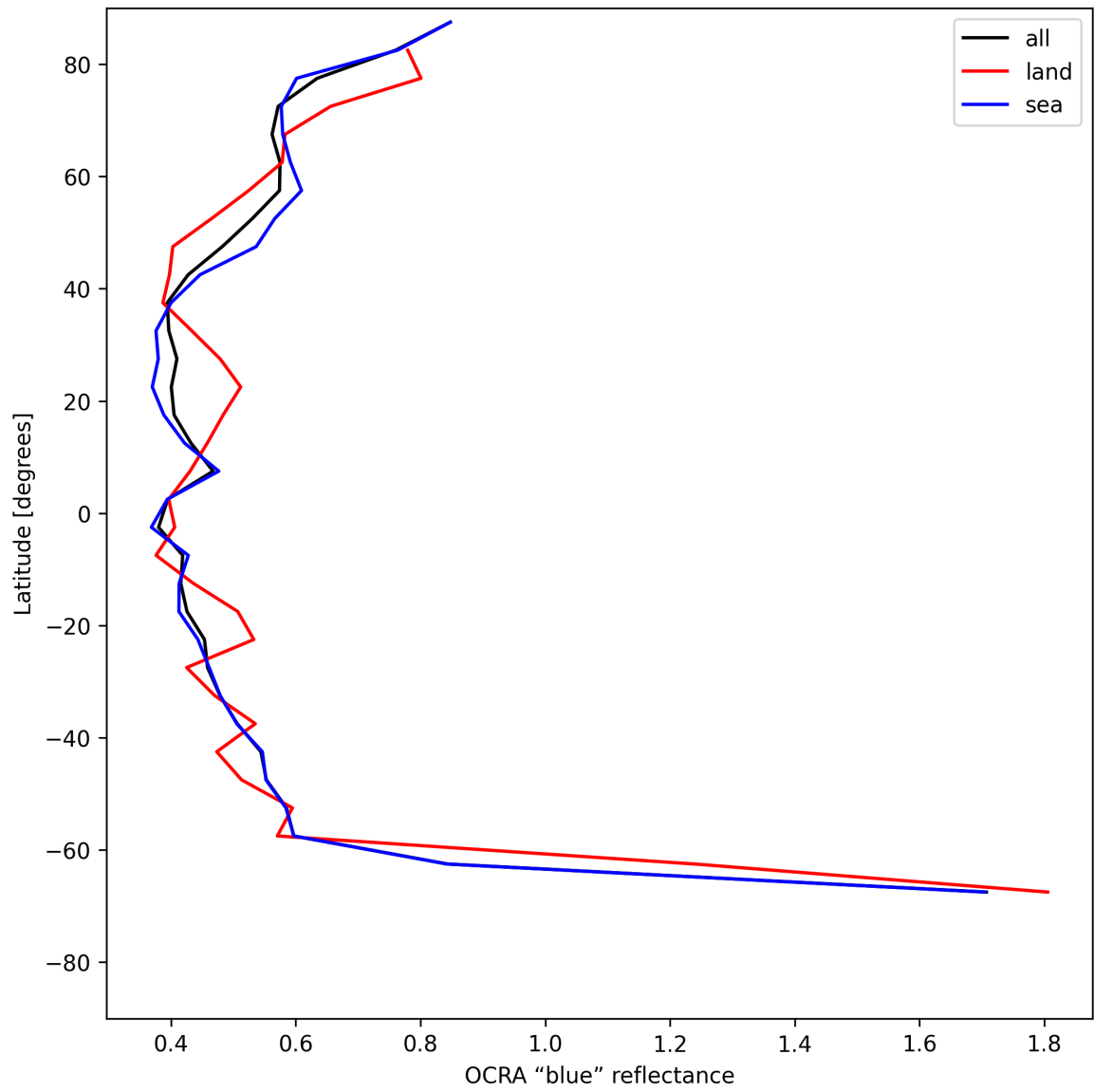
Figure 35: Zonal average of “OCRA “blue” reflectance” for 2025-06-22 to 2025-06-24.
