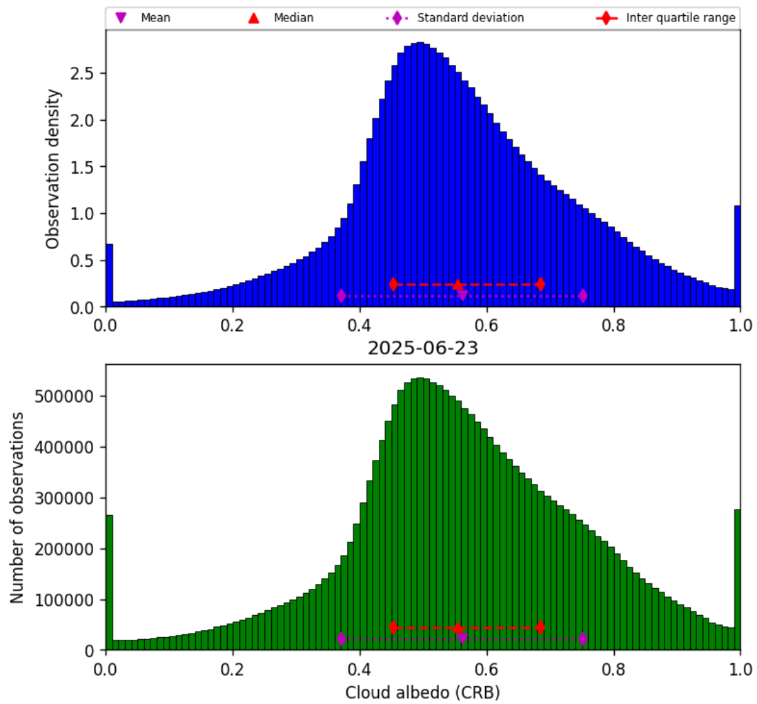
Figure 44: Histogram of “Cloud albedo (CRB)” for 2025-06-22 to 2025-06-24
