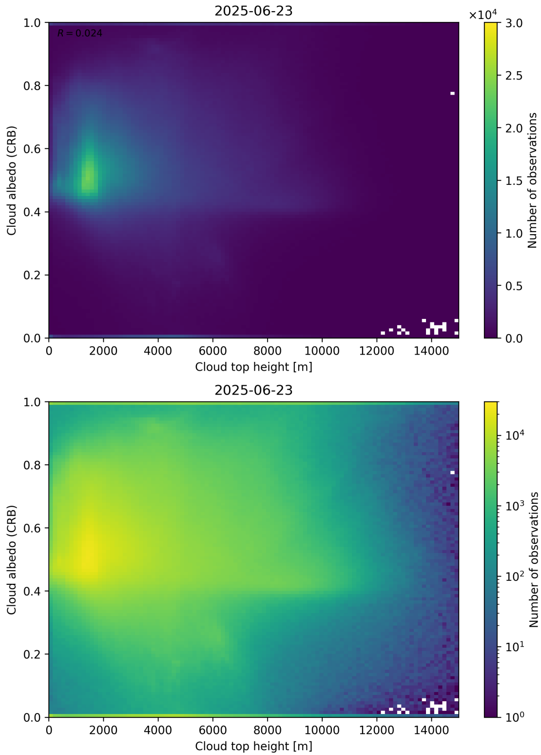
Figure 86: Scatter density plot of “Cloud top height” against “Cloud albedo (CRB)” for 2025-06-22 to 2025-06-24.
