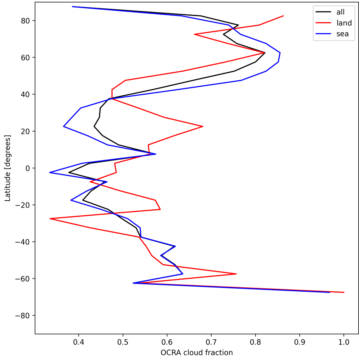
Figure 34: Zonal average of “OCRA cloud fraction” for 2025-06-22 to 2025-06-24.
