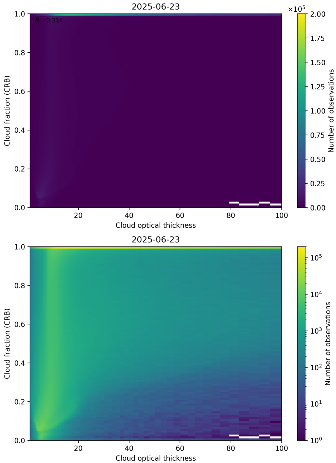
Figure 84: Scatter density plot of “Cloud optical thickness” against “Cloud fraction (CRB)” for 2025-06-22 to 2025-06-24.
