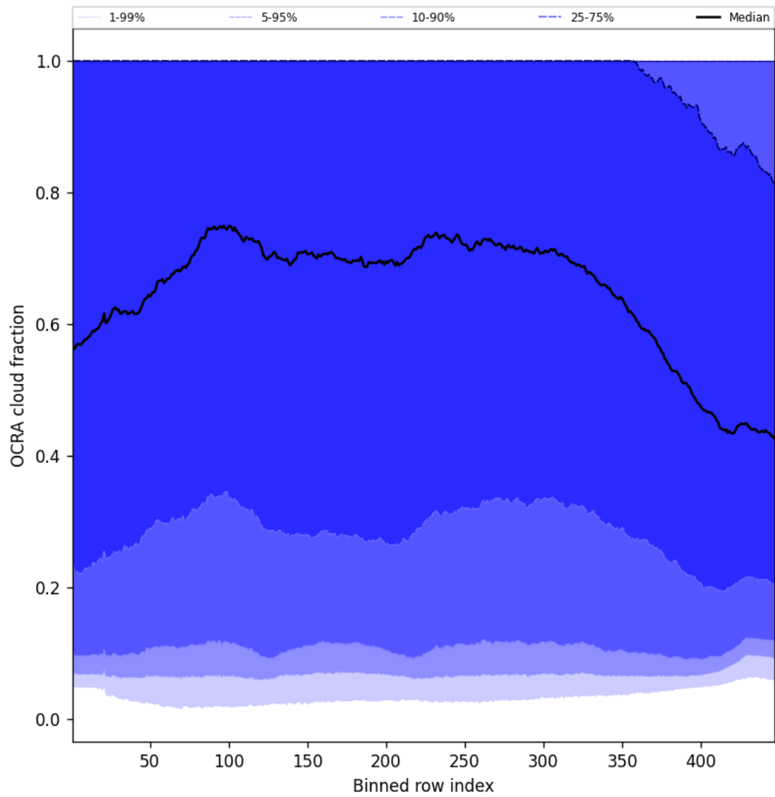
Figure 66: Along track statistics of “OCRA cloud fraction” for 2025-06-22 to 2025-06-24
