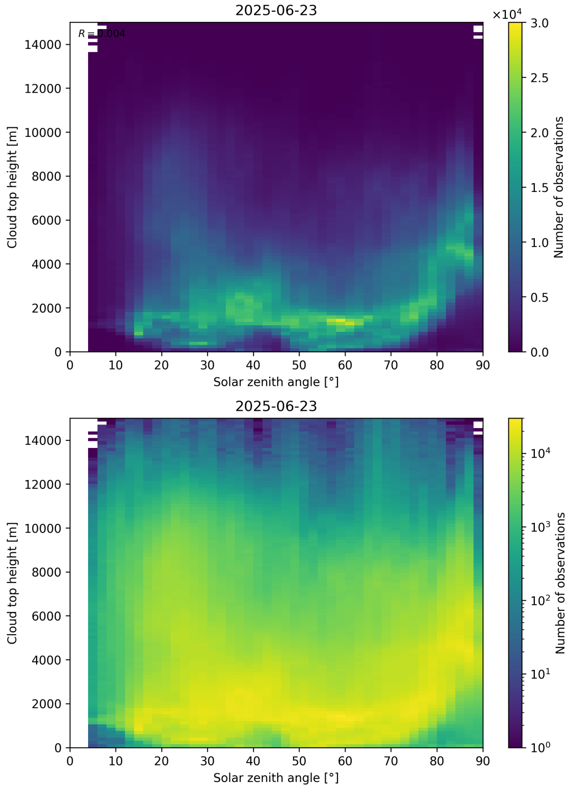
Figure 104: Scatter density plot of “Solar zenith angle” against “Cloud top height” for 2025-06-22 to 2025-06-24.
