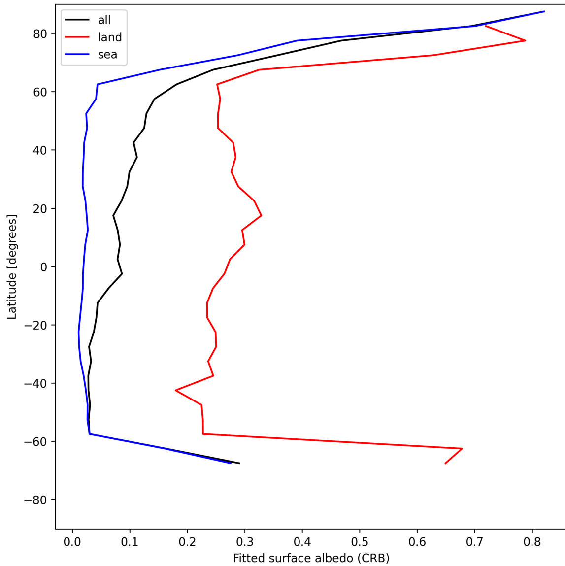
Figure 30: Zonal average of “Fitted surface albedo (CRB)” for 2025-06-22 to 2025-06-24.
