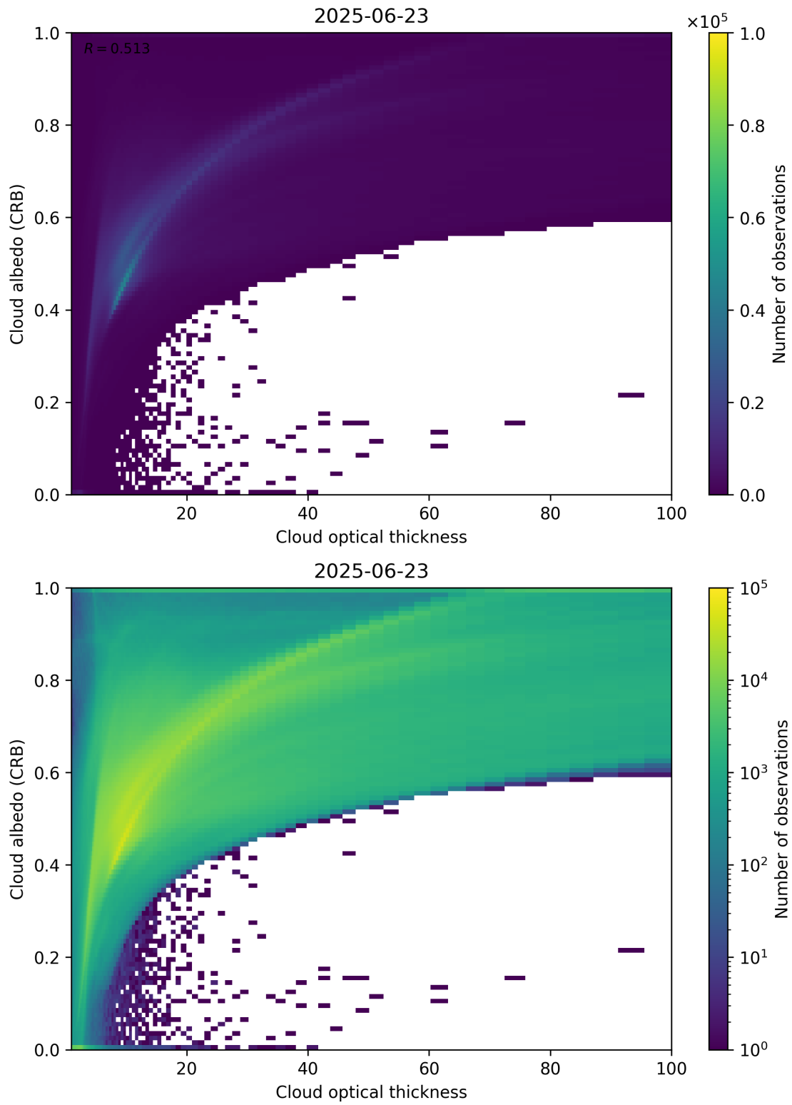
Figure 82: Scatter density plot of “Cloud optical thickness” against “Cloud albedo (CRB)” for 2025-06-22 to 2025-06-24.
