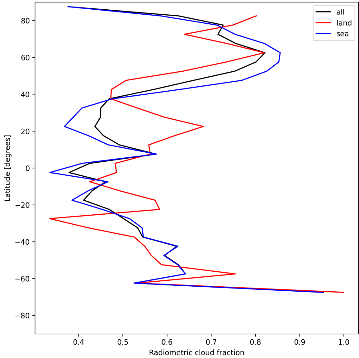
Figure 23: Zonal average of “Radiometric cloud fraction” for 2025-06-22 to 2025-06-24.
