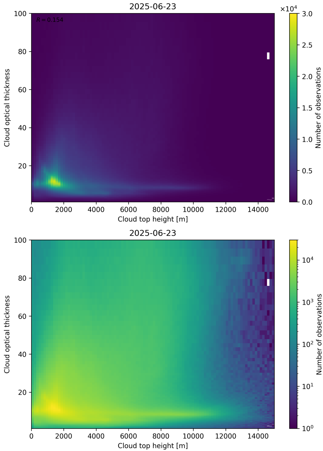
Figure 90: Scatter density plot of “Cloud top height” against “Cloud optical thickness” for 2025-06-22 to 2025-06-24.
