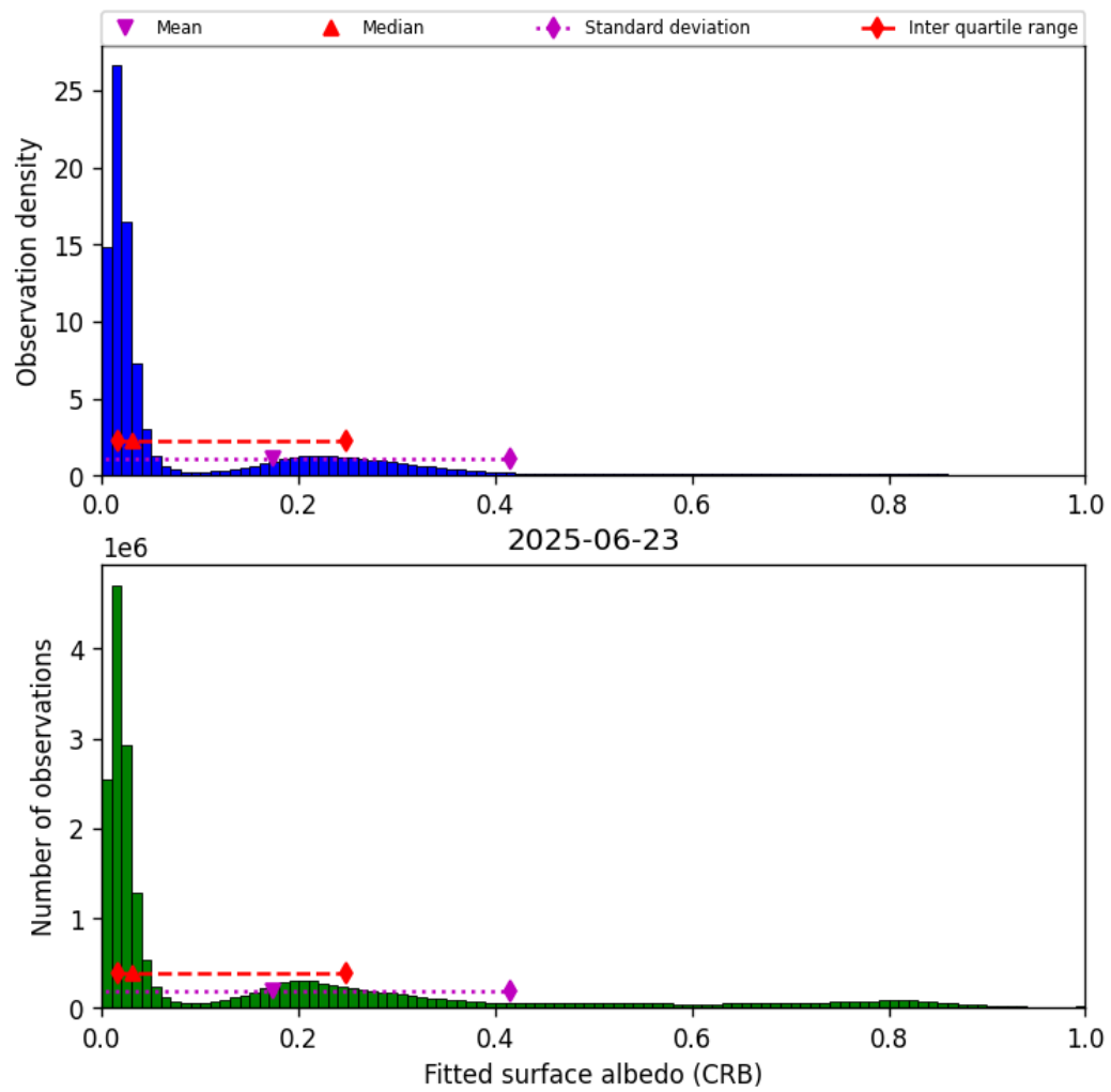
Figure 46: Histogram of “Fitted surface albedo (CRB)” for 2025-06-22 to 2025-06-24
