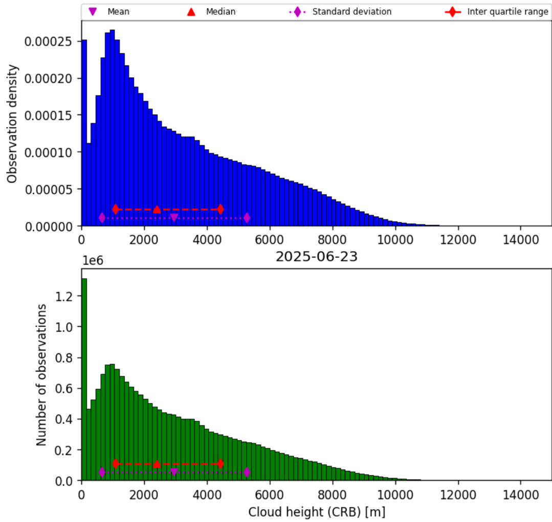
Figure 43: Histogram of “Cloud height (CRB)” for 2025-06-22 to 2025-06-24
