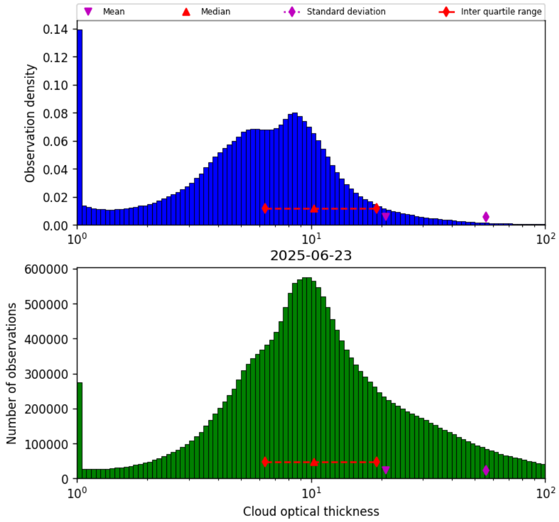
Figure 41: Histogram of “Cloud optical thickness” for 2025-06-22 to 2025-06-24
