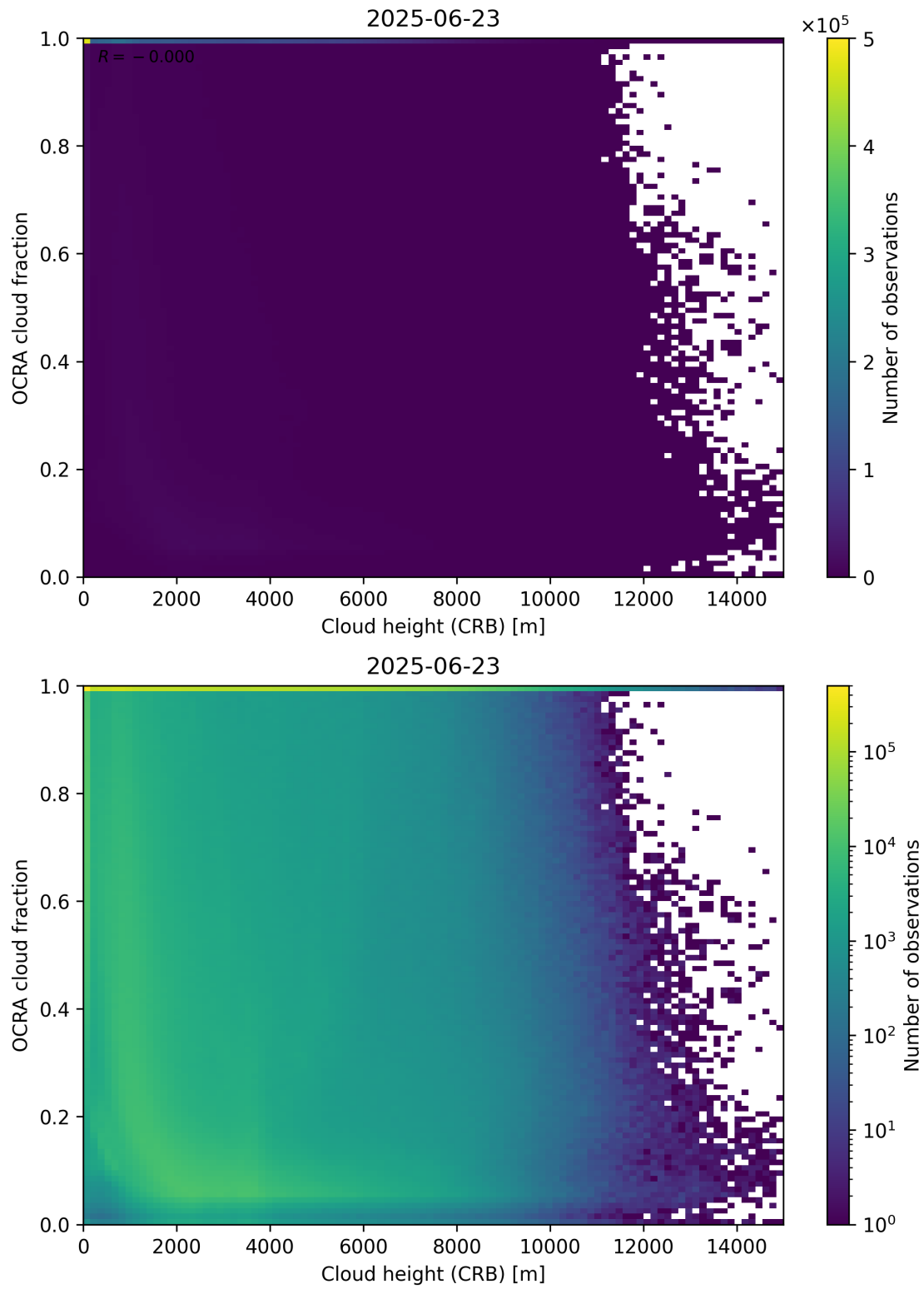
Figure 81: Scatter density plot of “Cloud height (CRB)” against “OCRA cloud fraction” for 2025-06-22 to 2025-06-24.
