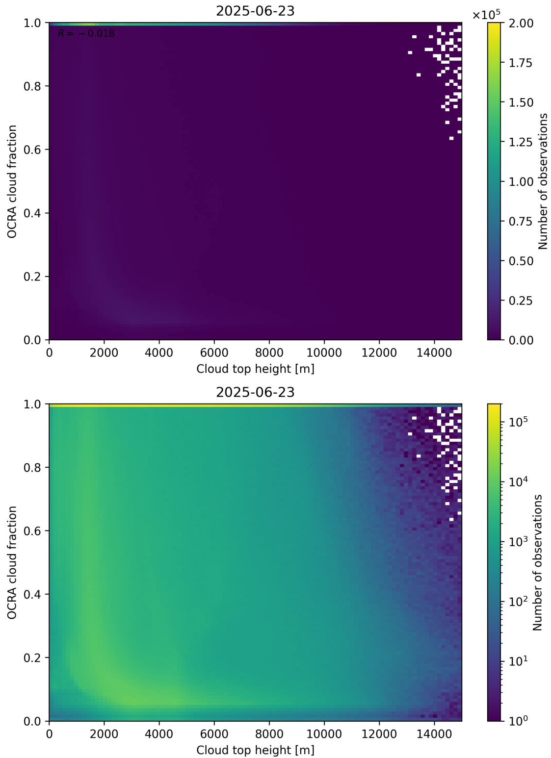
Figure 87: Scatter density plot of “Cloud top height” against “OCRA cloud fraction” for 2025-06-22 to 2025-06-24.
