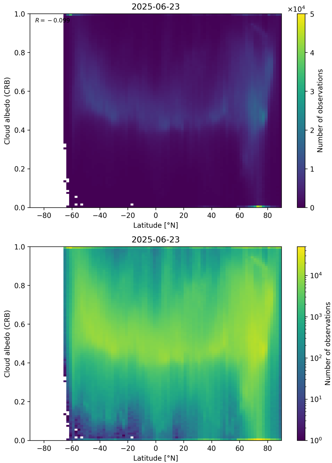
Figure 91: Scatter density plot of “Latitude” against “Cloud albedo (CRB)” for 2025-06-22 to 2025-06-24.
