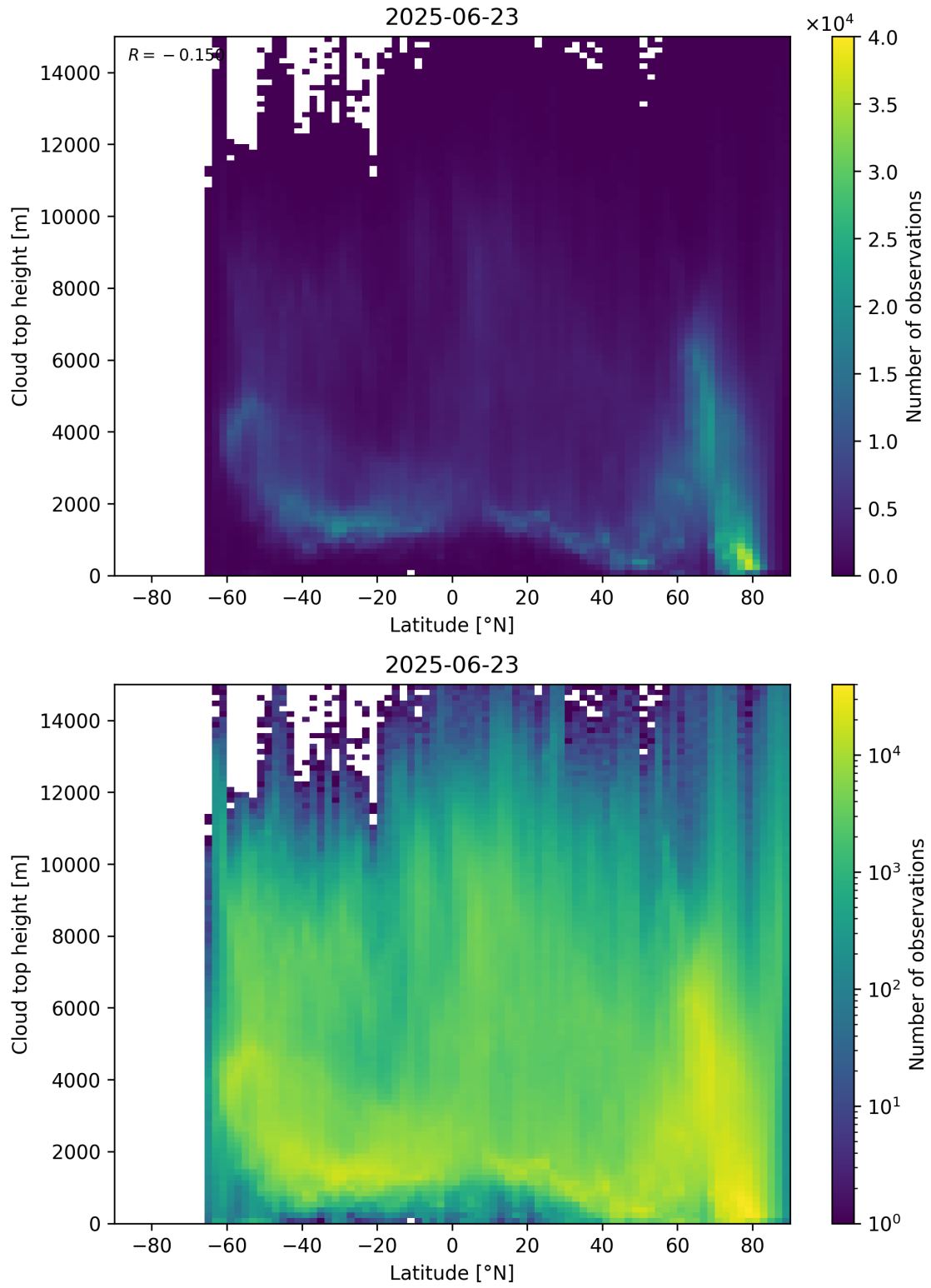
Figure 97: Scatter density plot of “Latitude” against “Cloud top height” for 2025-06-22 to 2025-06-24.
