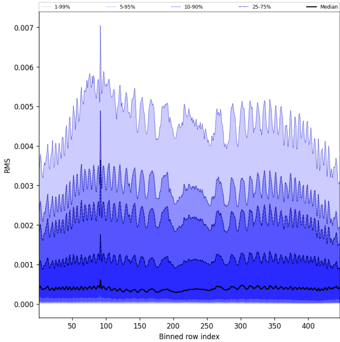
Figure 63: Along track statistics of “RMS” for 2025-06-22 to 2025-06-24
