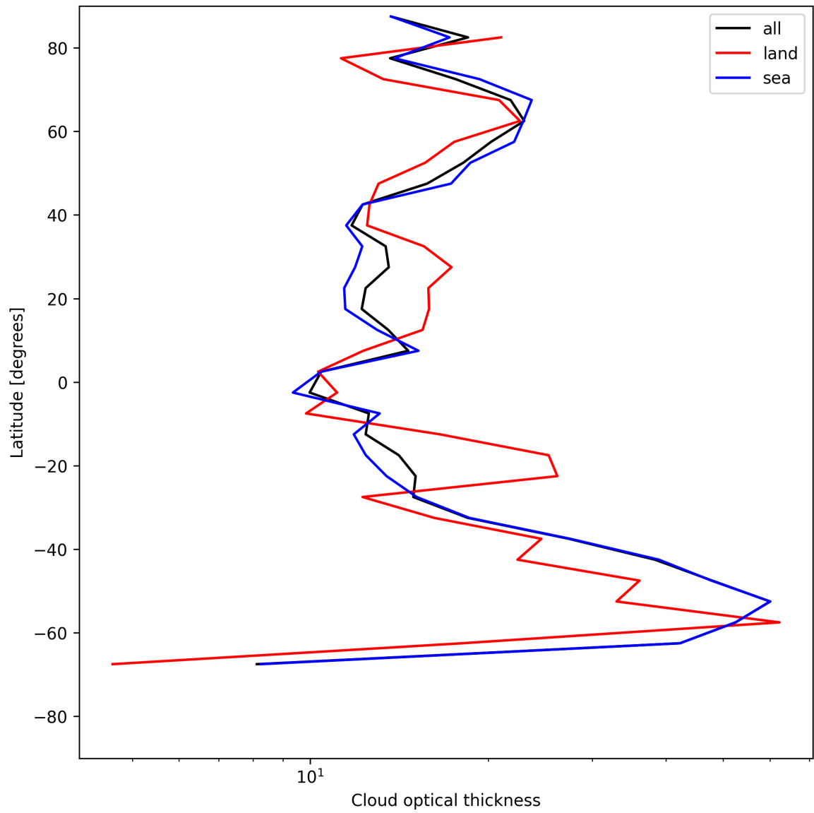
Figure 25: Zonal average of “Cloud optical thickness” for 2025-06-22 to 2025-06-24.
