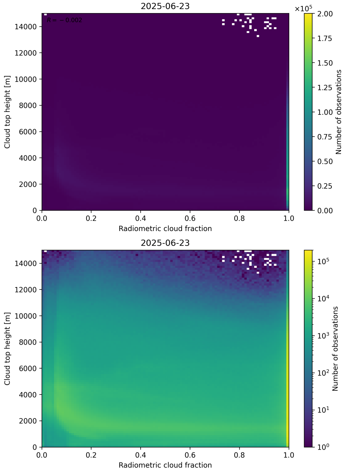
Figure 76: Scatter density plot of “Radiometric cloud fraction” against “Cloud top height” for 2025-06-22 to 2025-06-24.
