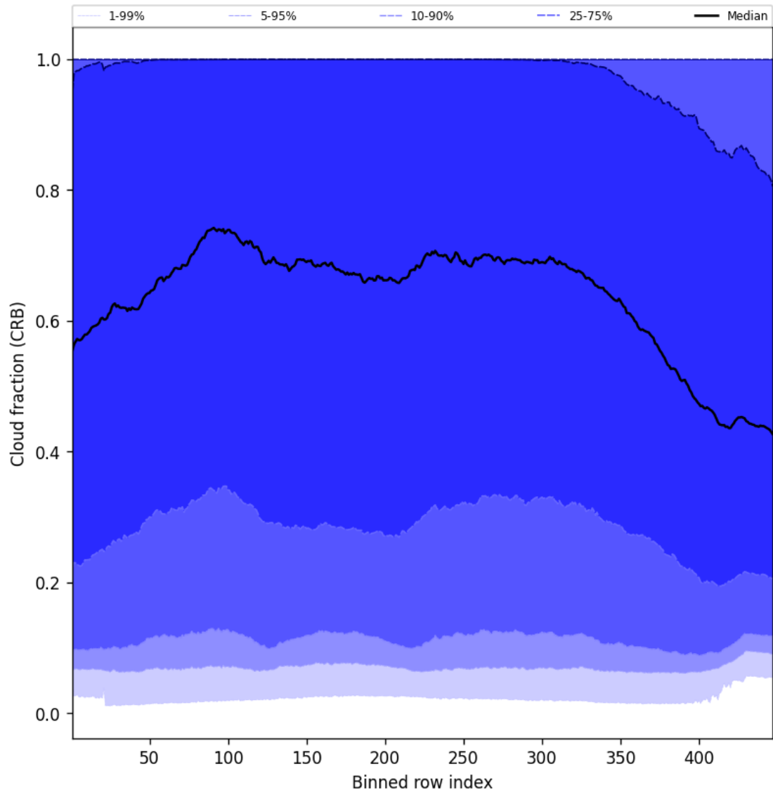
Figure 58: Along track statistics of “Cloud fraction (CRB)” for 2025-06-22 to 2025-06-24
