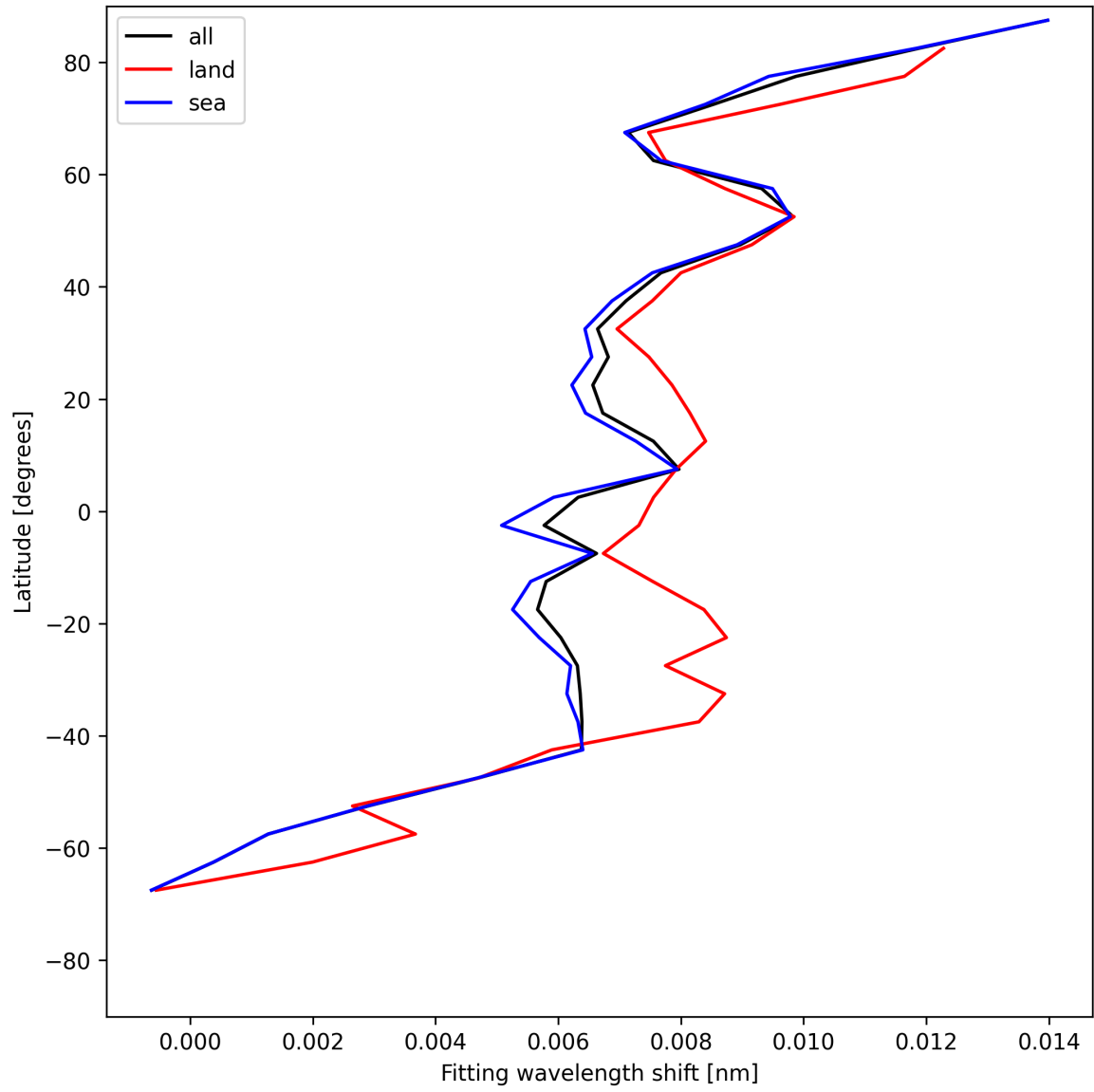
Figure 33: Zonal average of “Fitting wavelength shift” for 2025-06-22 to 2025-06-24.
