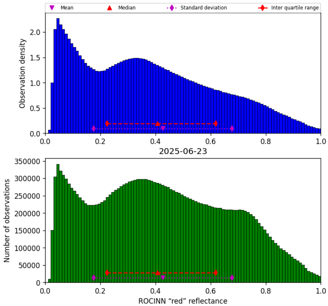
Figure 53: Histogram of “ROCINN “red” reflectance” for 2025-06-22 to 2025-06-24
