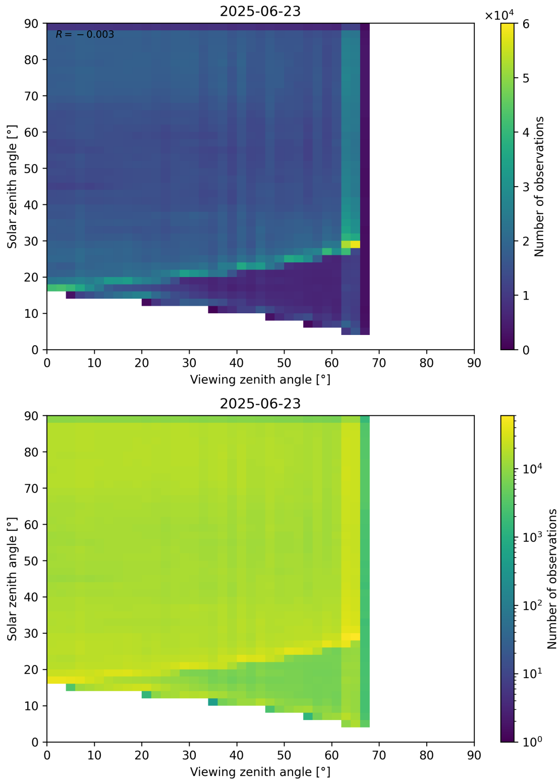
Figure 114: Scatter density plot of “Viewing zenith angle” against “Solar zenith angle” for 2025-06-22 to 2025-06-24.
