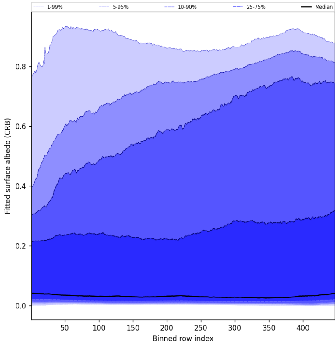
Figure 62: Along track statistics of “Fitted surface albedo (CRB)” for 2025-06-22 to 2025-06-24
