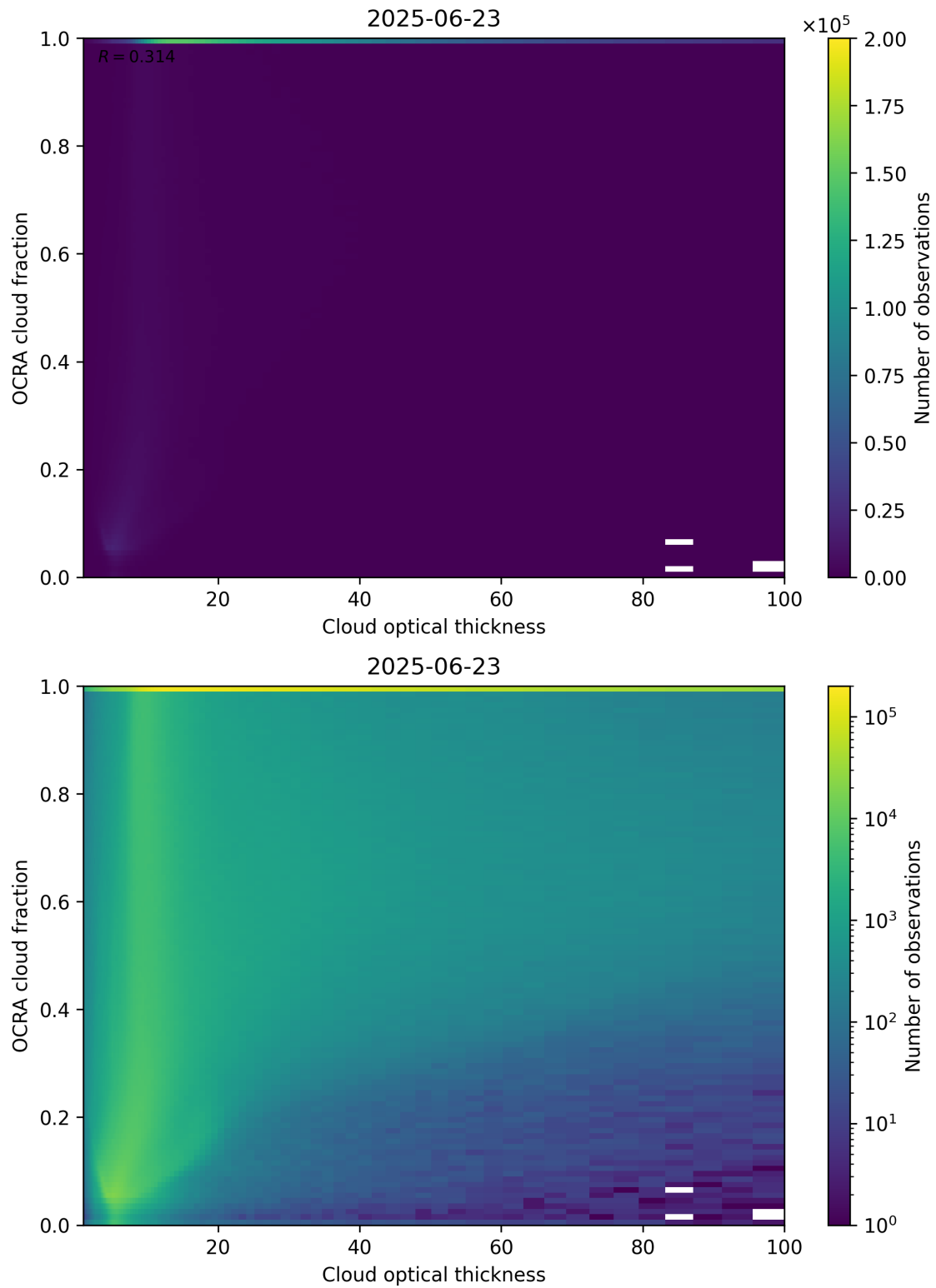
Figure 83: Scatter density plot of “Cloud optical thickness” against “OCRA cloud fraction” for 2025-06-22 to 2025-06-24.
