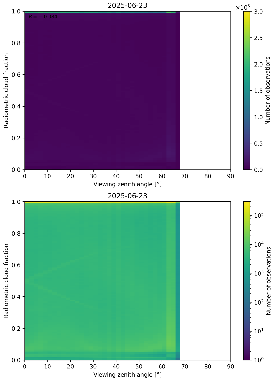
Figure 107: Scatter density plot of “Viewing zenith angle” against “Radiometric cloud fraction” for 2025-06-22 to 2025-06-24.
