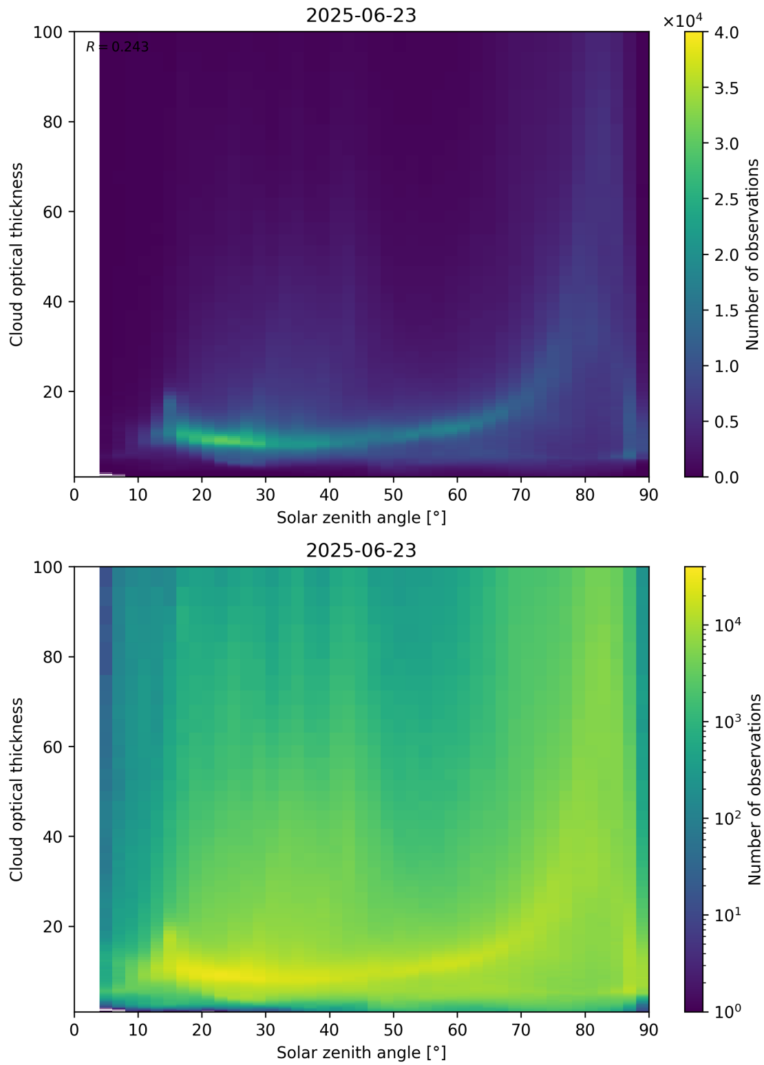
Figure 103: Scatter density plot of “Solar zenith angle” against “Cloud optical thickness” for 2025-06-22 to 2025-06-24.
