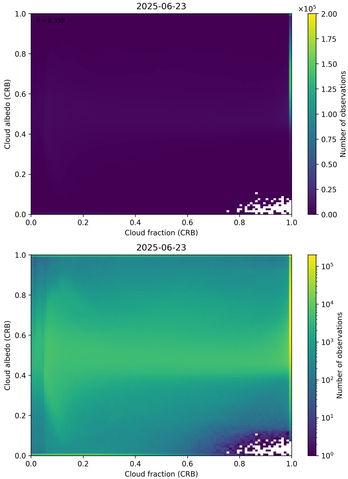
Figure 77: Scatter density plot of “Cloud fraction (CRB)” against “Cloud albedo (CRB)” for 2025-06-22 to 2025-06-24.
