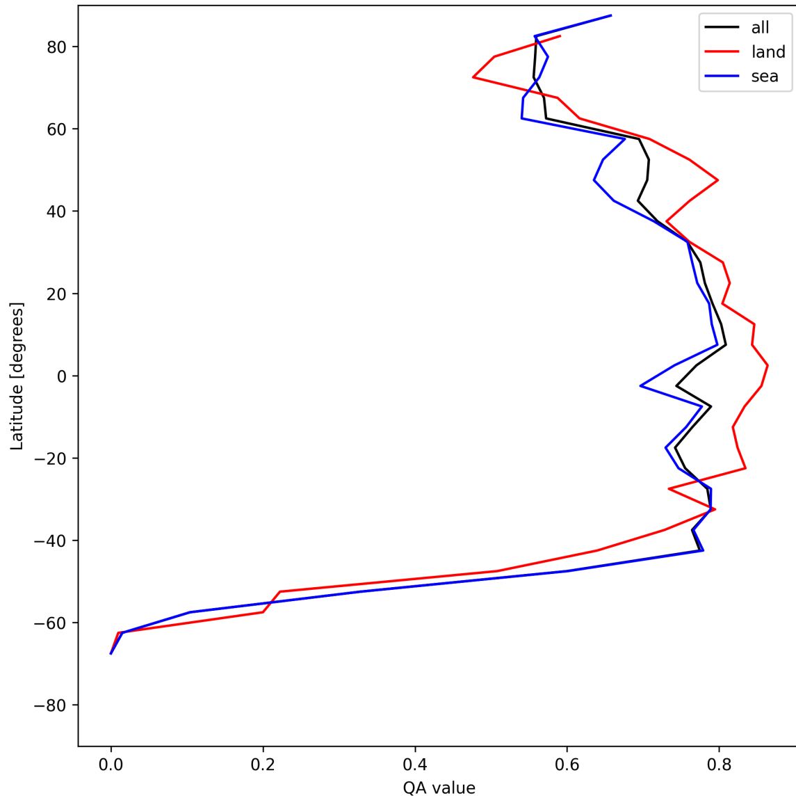
Figure 22: Zonal average of “QA value” for 2025-06-22 to 2025-06-24.
