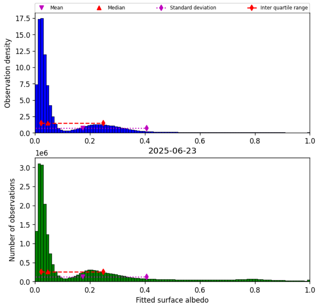
Figure 45: Histogram of “Fitted surface albedo” for 2025-06-22 to 2025-06-24
