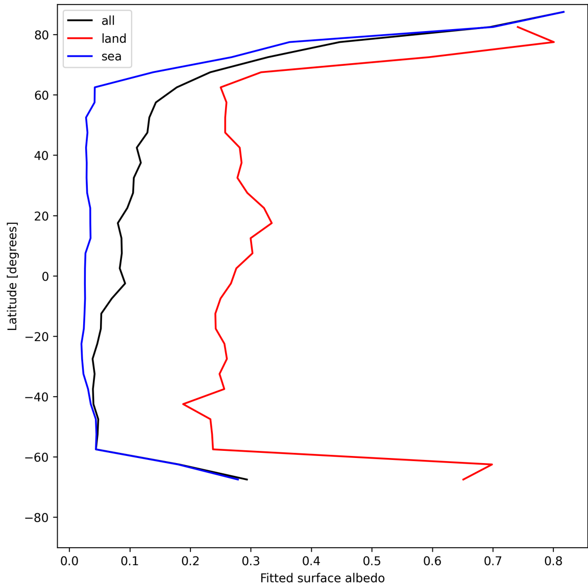
Figure 29: Zonal average of “Fitted surface albedo” for 2025-06-22 to 2025-06-24.
