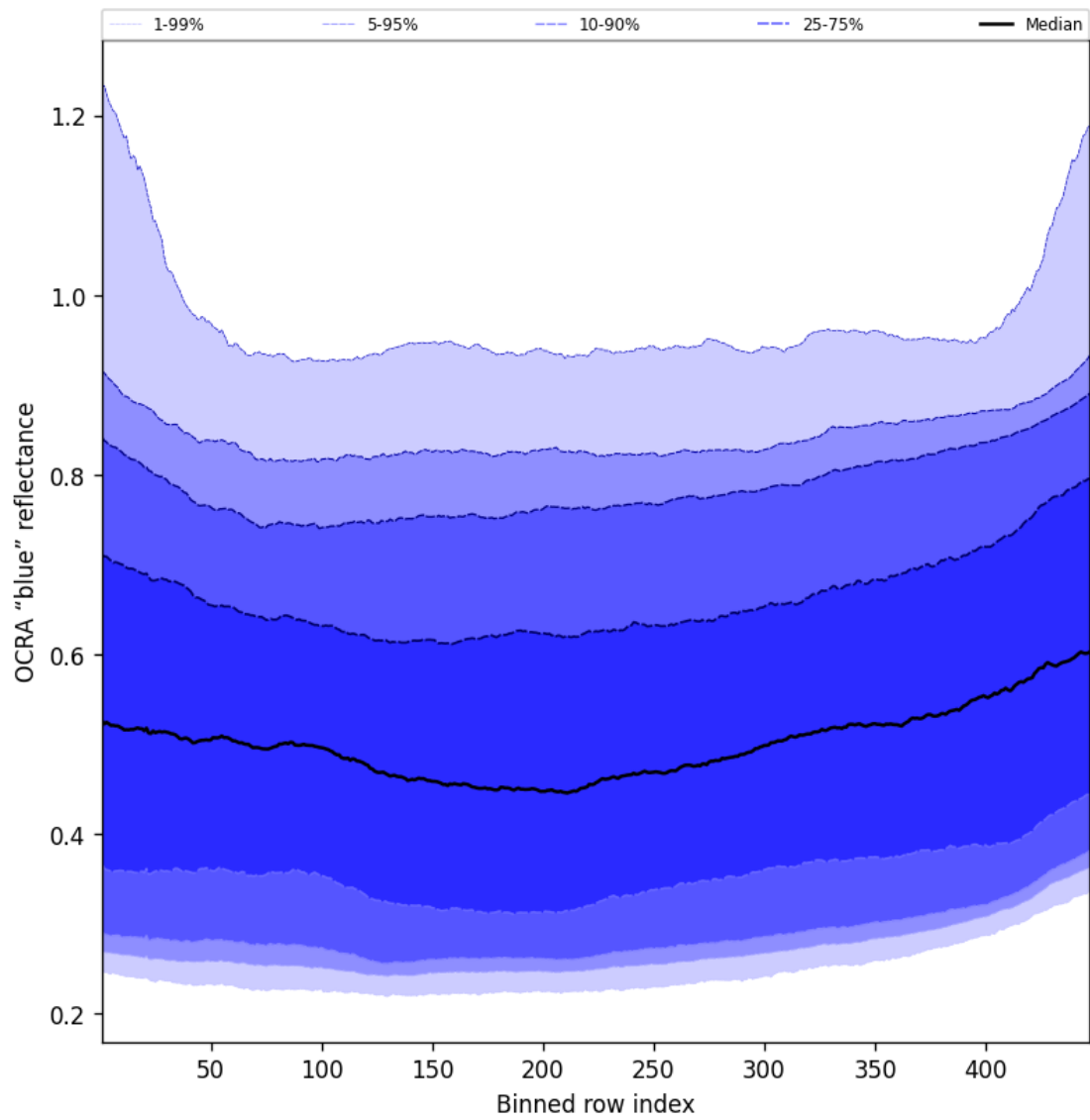
Figure 67: Along track statistics of “OCRA “blue” reflectance” for 2025-06-22 to 2025-06-24
