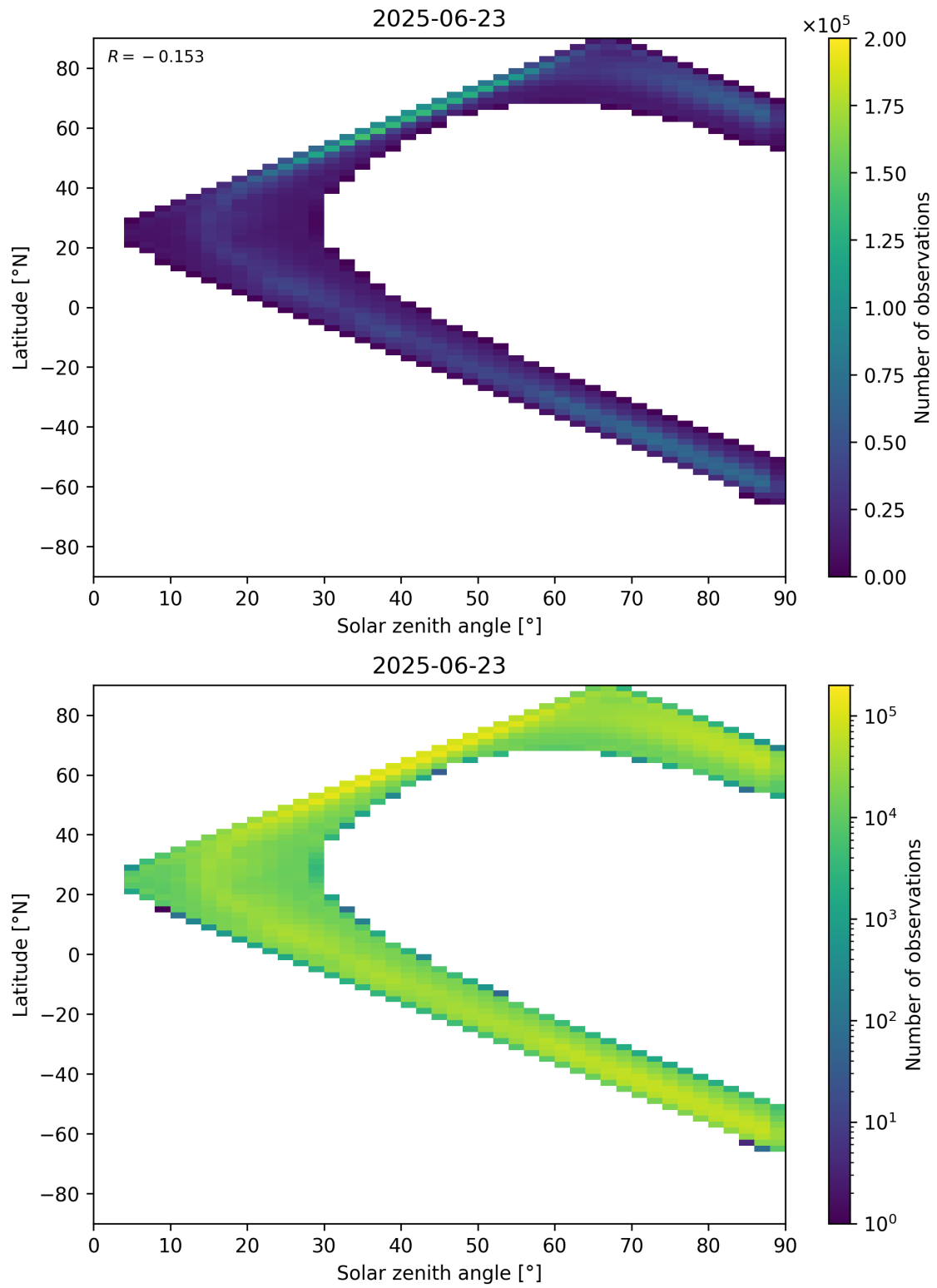
Figure 105: Scatter density plot of “Solar zenith angle” against “Latitude” for 2025-06-22 to 2025-06-24.
