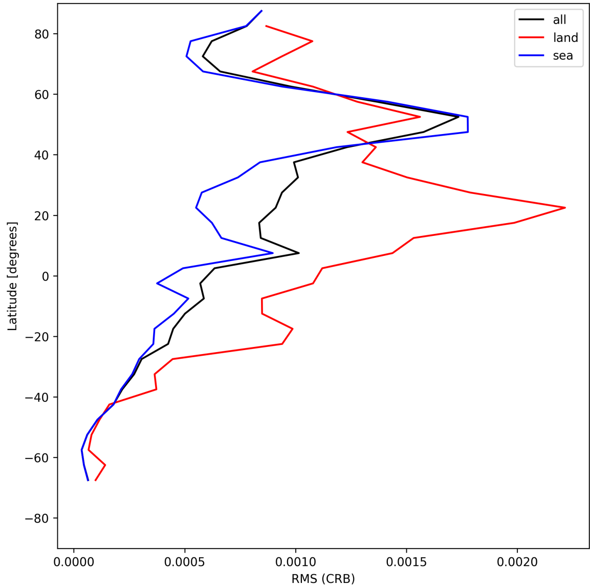
Figure 32: Zonal average of “RMS (CRB)” for 2025-06-22 to 2025-06-24.
