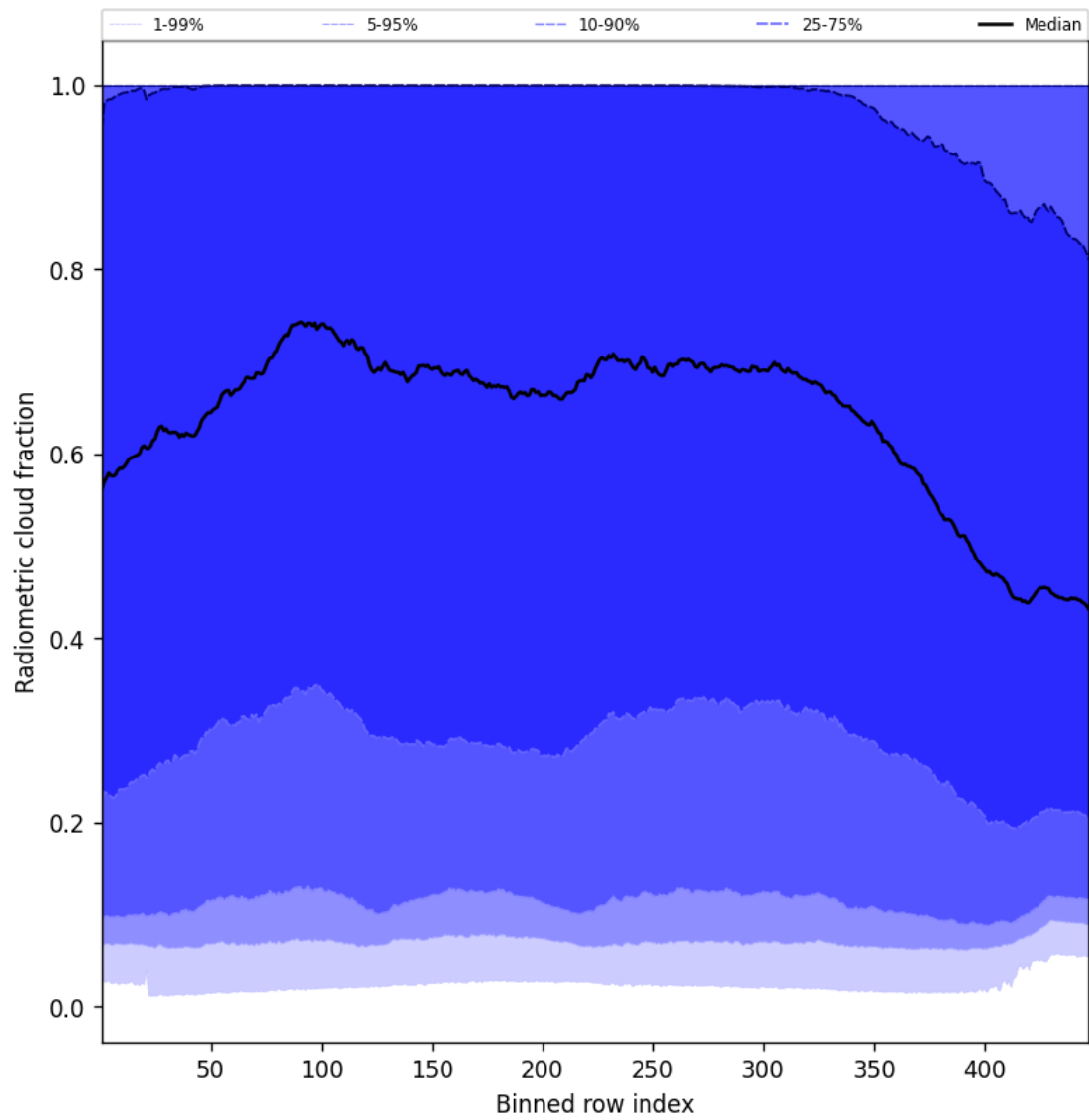
Figure 55: Along track statistics of “Radiometric cloud fraction” for 2025-06-22 to 2025-06-24
