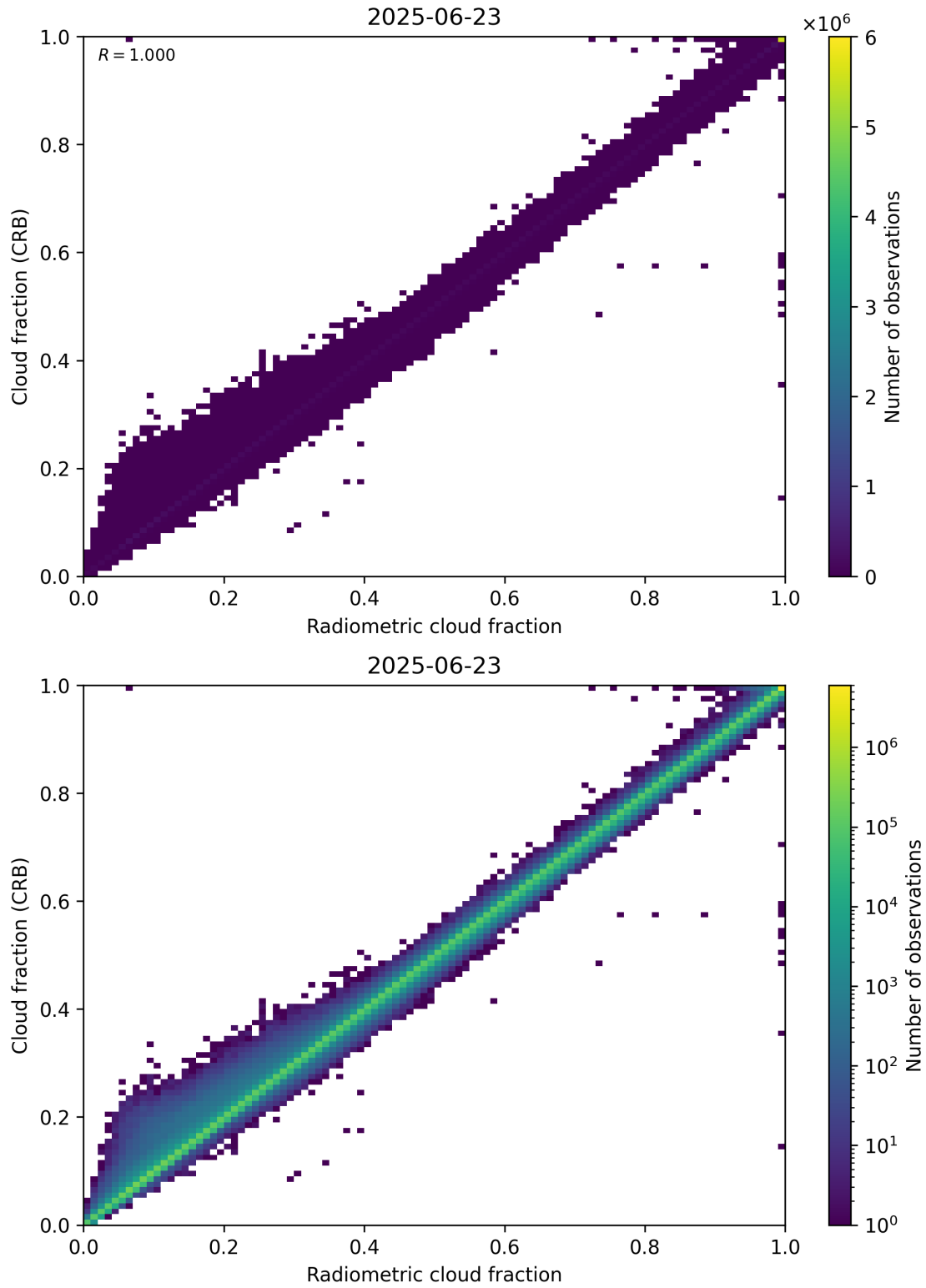
Figure 73: Scatter density plot of “Radiometric cloud fraction” against “Cloud fraction (CRB)” for 2025-06-22 to 2025-06-24.
