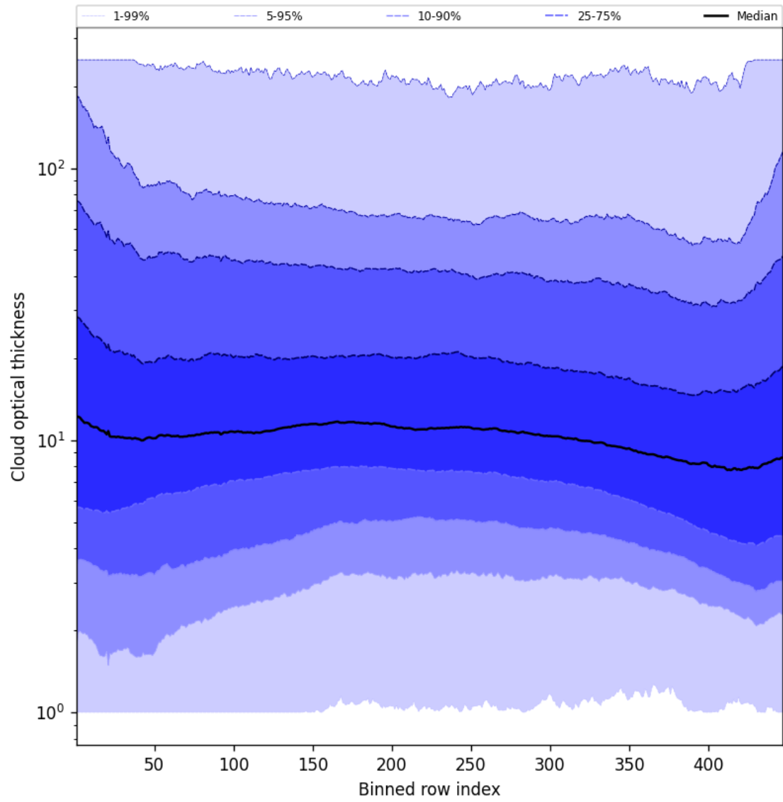
Figure 57: Along track statistics of “Cloud optical thickness” for 2025-06-22 to 2025-06-24
