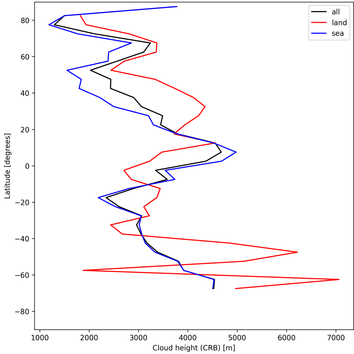
Figure 27: Zonal average of “Cloud height (CRB)” for 2025-06-22 to 2025-06-24.
