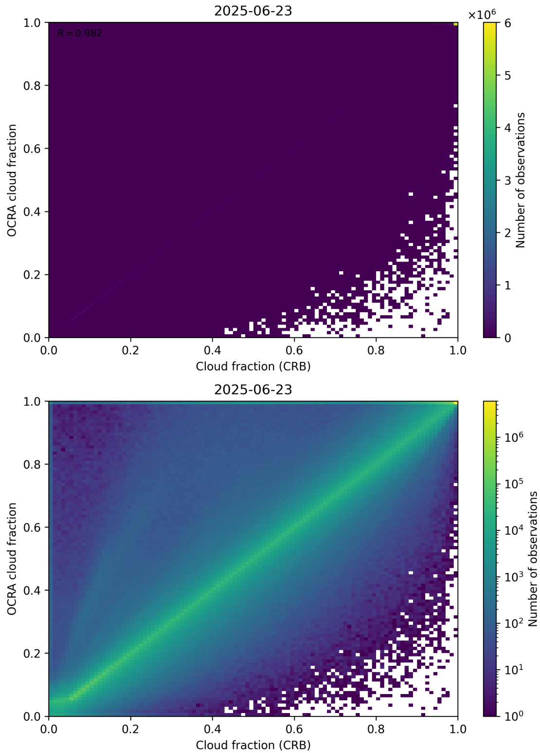
Figure 78: Scatter density plot of “Cloud fraction (CRB)” against “OCRA cloud fraction” for 2025-06-22 to 2025-06-24.
