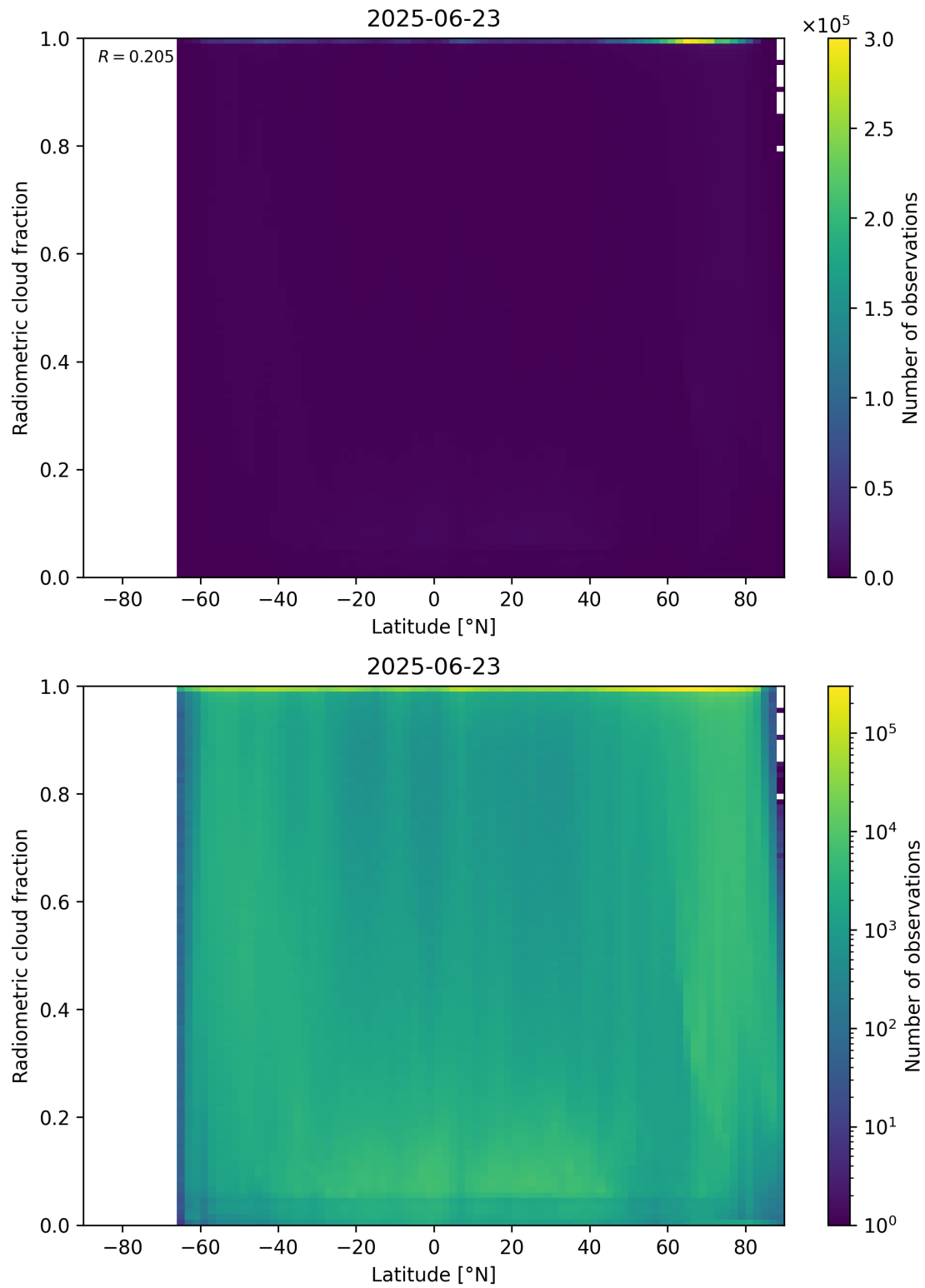
Figure 92: Scatter density plot of “Latitude” against “Radiometric cloud fraction” for 2025-06-22 to 2025-06-24.
