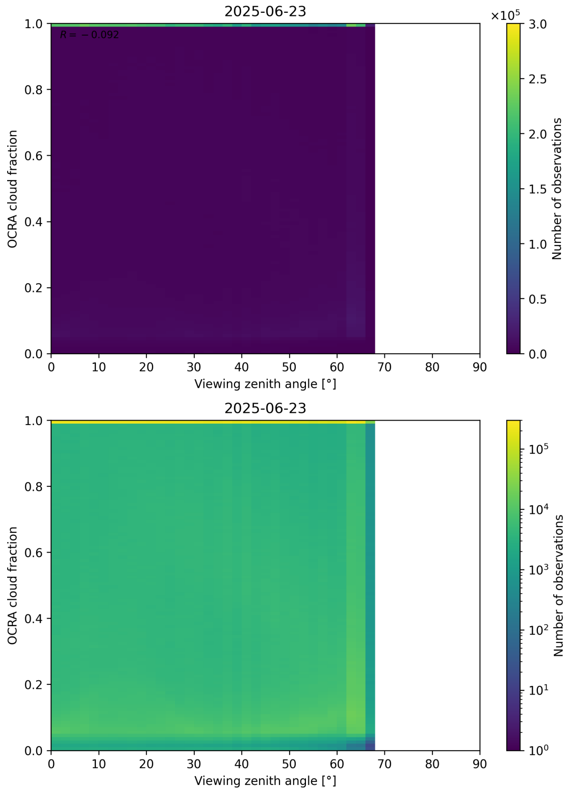
Figure 108: Scatter density plot of “Viewing zenith angle” against “OCRA cloud fraction” for 2025-06-22 to 2025-06-24.
