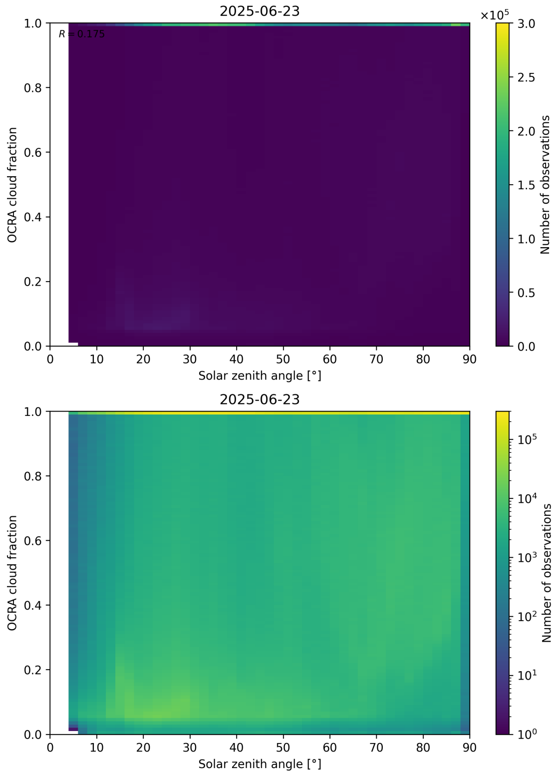
Figure 100: Scatter density plot of “Solar zenith angle” against “OCRA cloud fraction” for 2025-06-22 to 2025-06-24.
