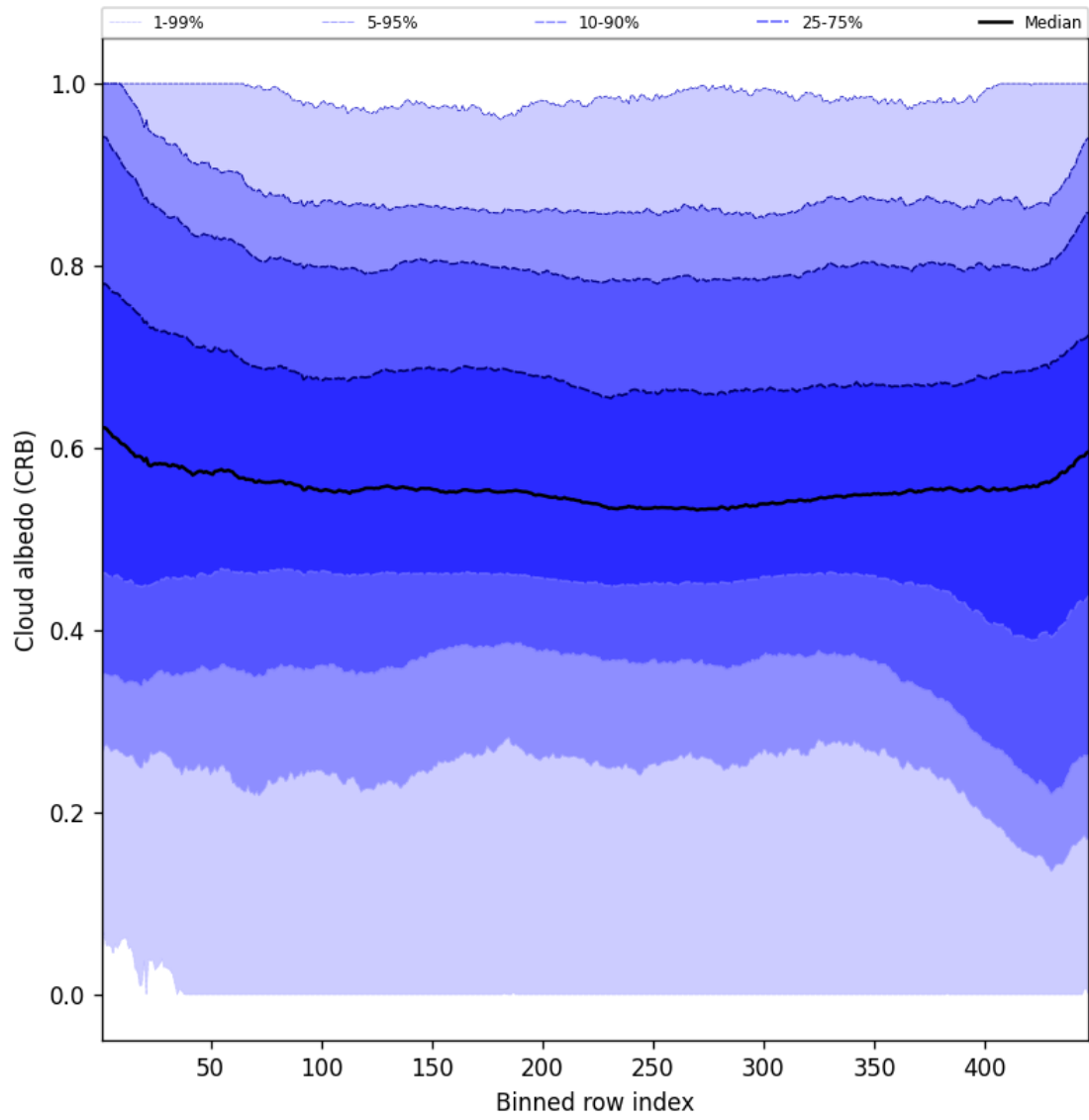
Figure 60: Along track statistics of “Cloud albedo (CRB)” for 2025-06-22 to 2025-06-24
