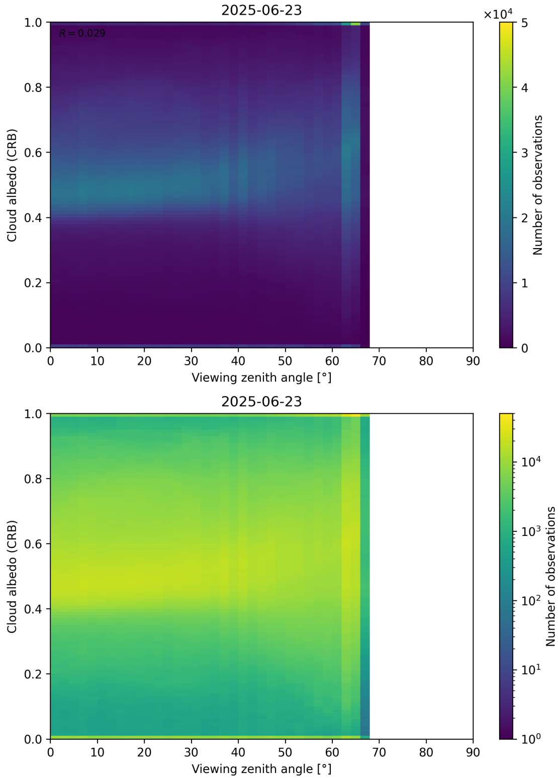
Figure 106: Scatter density plot of “Viewing zenith angle” against “Cloud albedo (CRB)” for 2025-06-22 to 2025-06-24.
