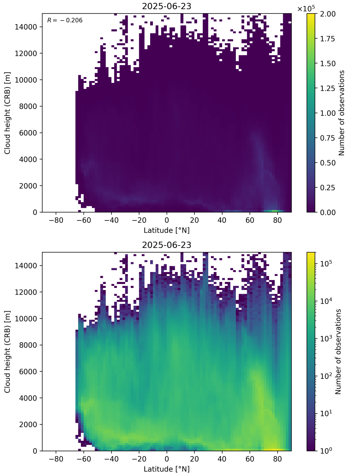
Figure 95: Scatter density plot of “Latitude” against “Cloud height (CRB)” for 2025-06-22 to 2025-06-24.
