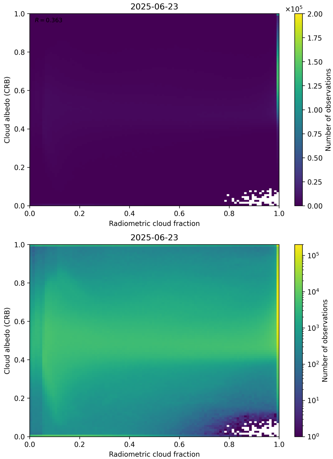
Figure 71: Scatter density plot of “Radiometric cloud fraction” against “Cloud albedo (CRB)” for 2025-06-22 to 2025-06-24.
