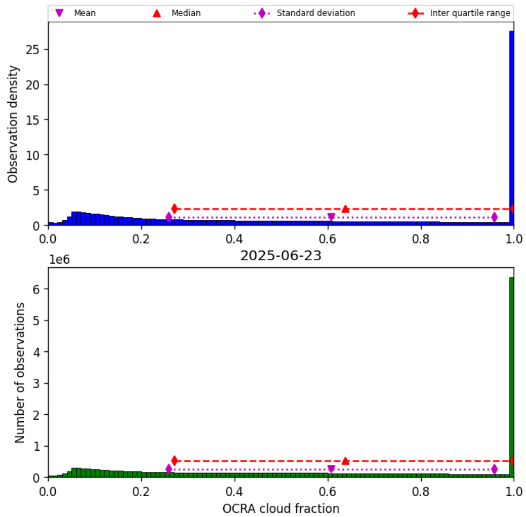
Figure 50: Histogram of “OCRA cloud fraction” for 2025-06-22 to 2025-06-24
