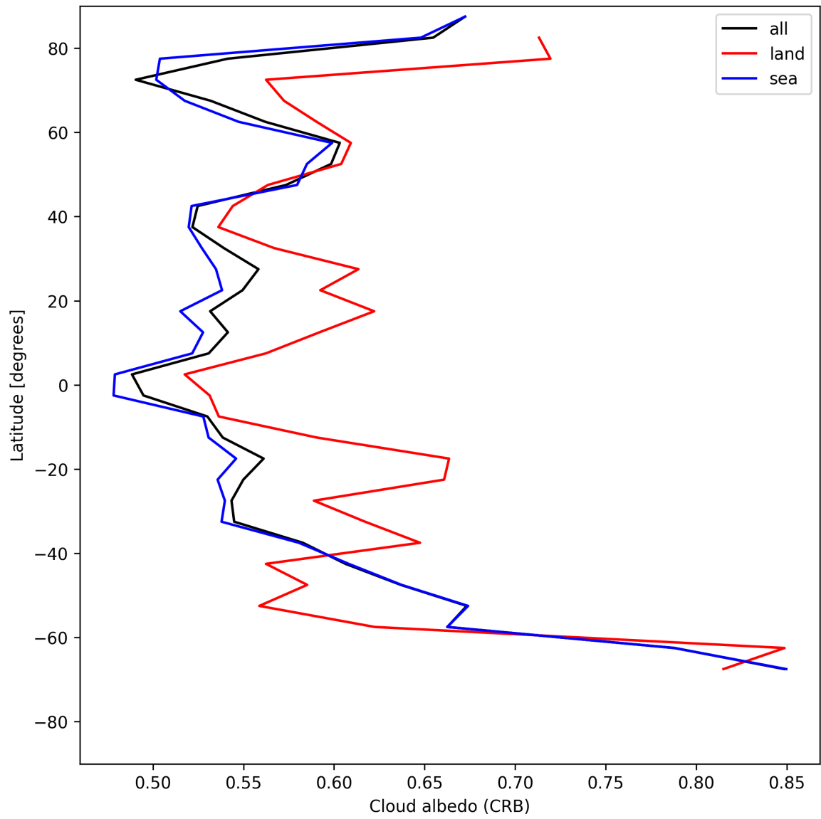
Figure 28: Zonal average of “Cloud albedo (CRB)” for 2025-06-22 to 2025-06-24.
