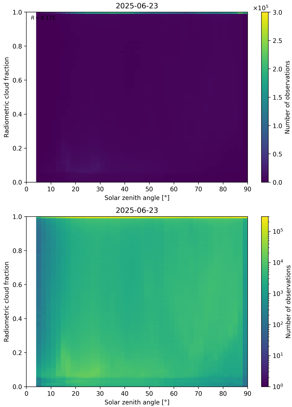
Figure 99: Scatter density plot of “Solar zenith angle” against “Radiometric cloud fraction” for 2025-06-22 to 2025-06-24.
