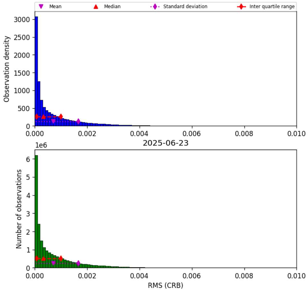
Figure 48: Histogram of “RMS (CRB)” for 2025-06-22 to 2025-06-24
