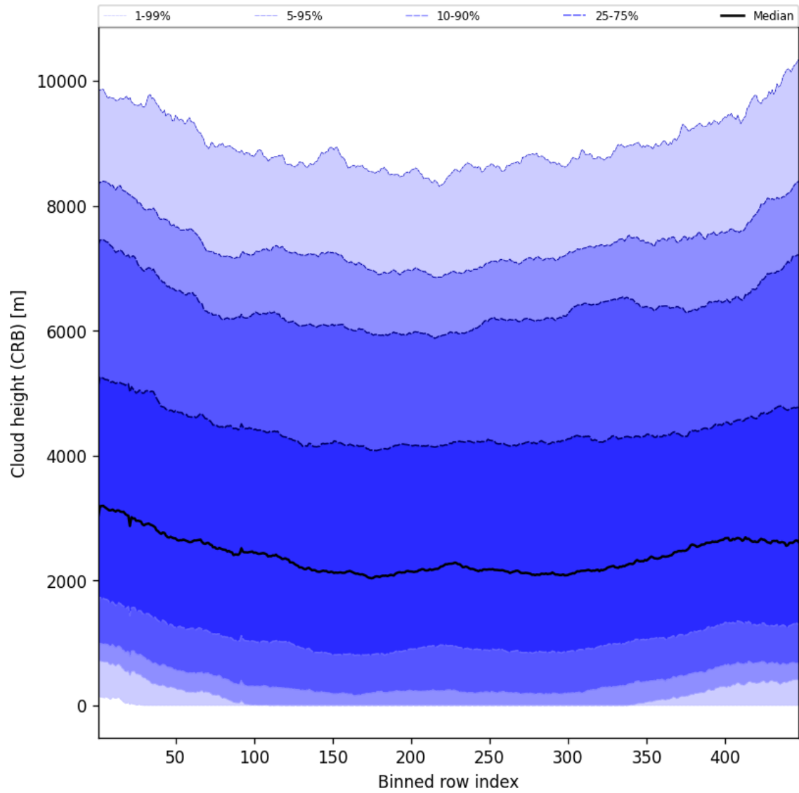
Figure 59: Along track statistics of “Cloud height (CRB)” for 2025-06-22 to 2025-06-24
