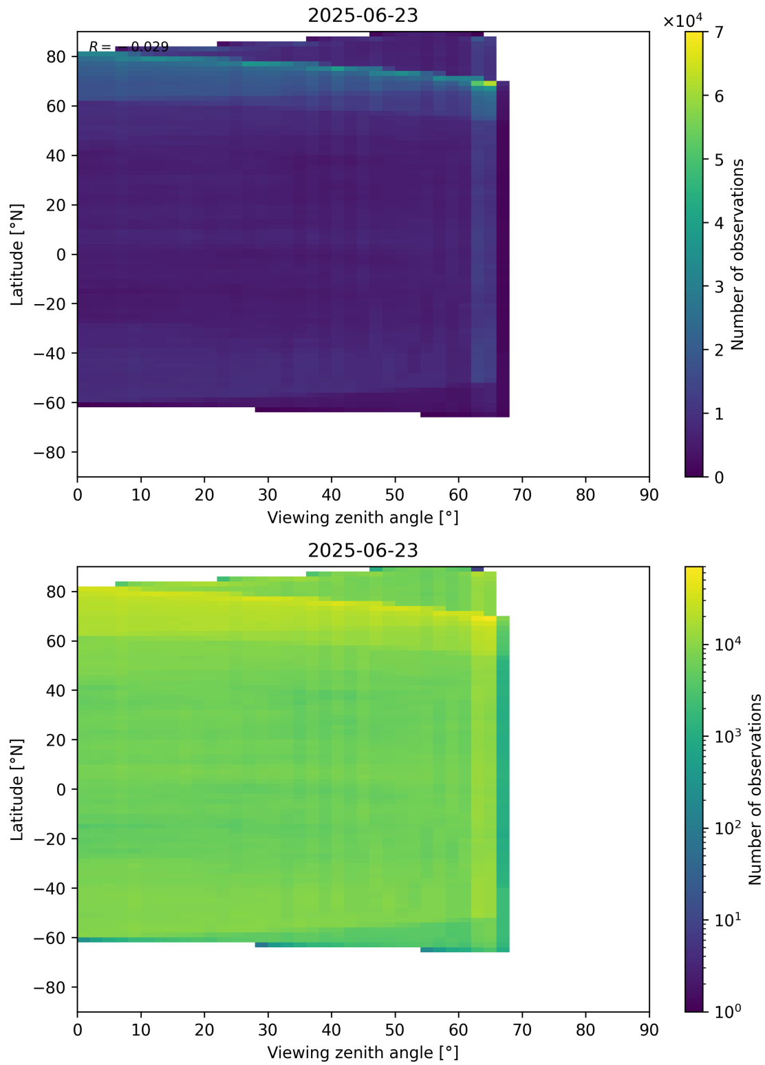
Figure 113: Scatter density plot of “Viewing zenith angle” against “Latitude” for 2025-06-22 to 2025-06-24.
