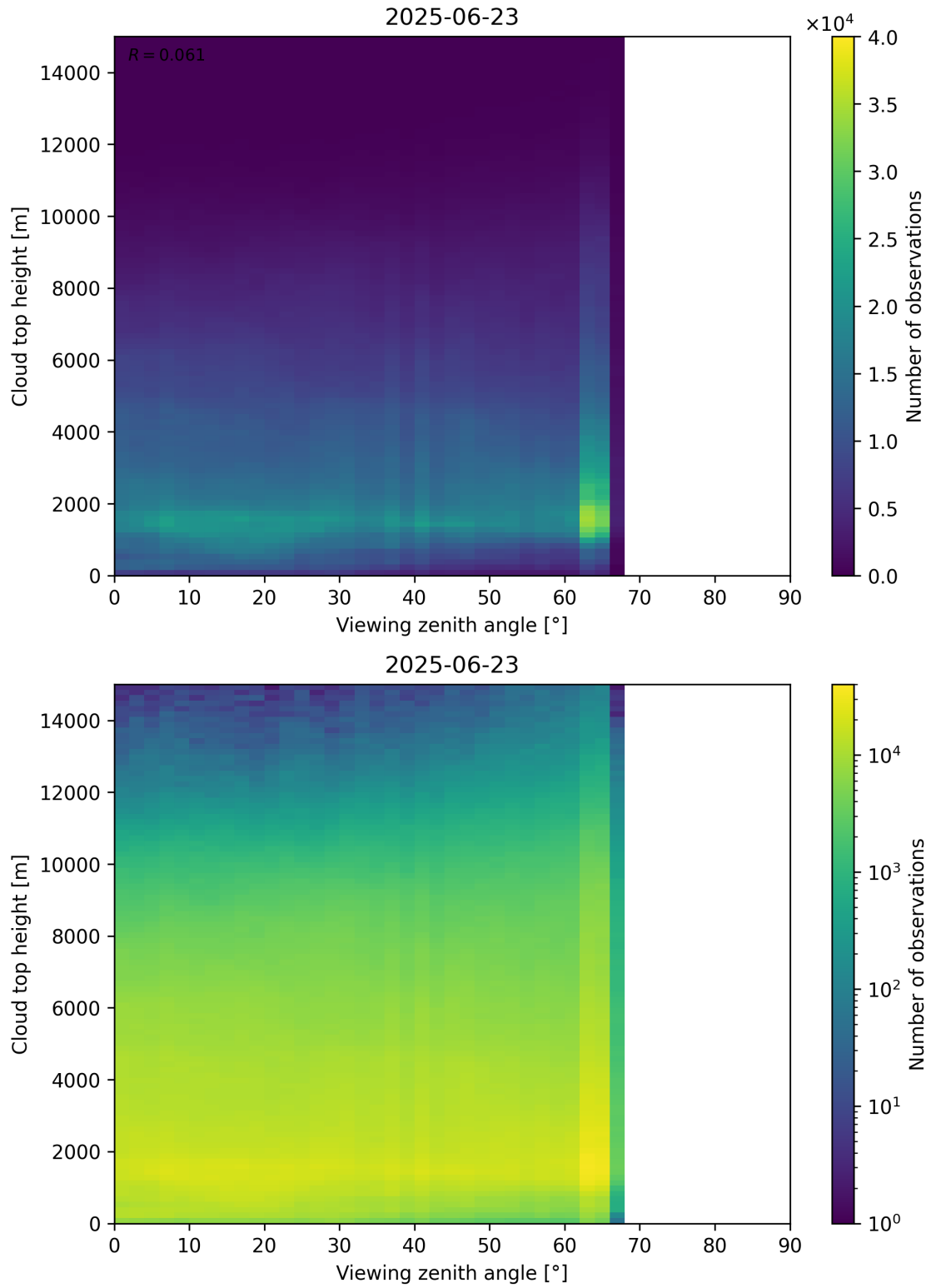
Figure 112: Scatter density plot of “Viewing zenith angle” against “Cloud top height” for 2025-06-22 to 2025-06-24.
