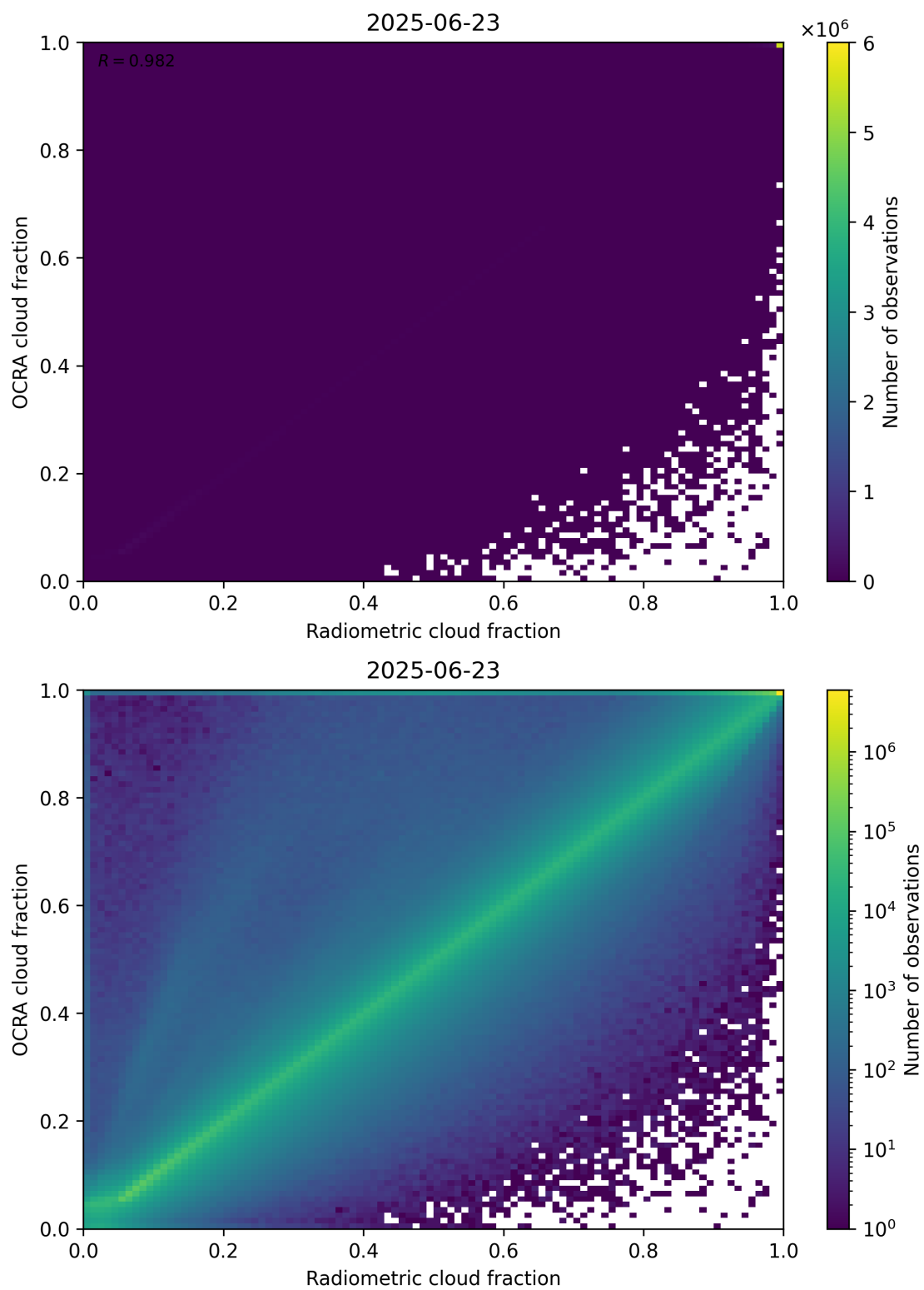
Figure 72: Scatter density plot of “Radiometric cloud fraction” against “OCRA cloud fraction” for 2025-06-22 to 2025-06-24.
