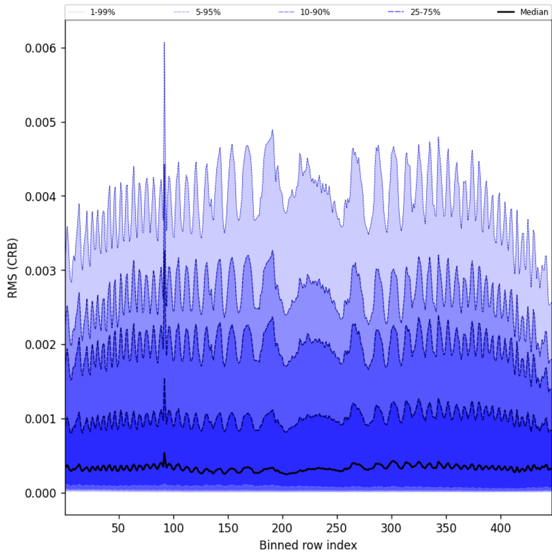
Figure 64: Along track statistics of "RMS (CRB)" for 2025-06-22 to 2025-06-24
