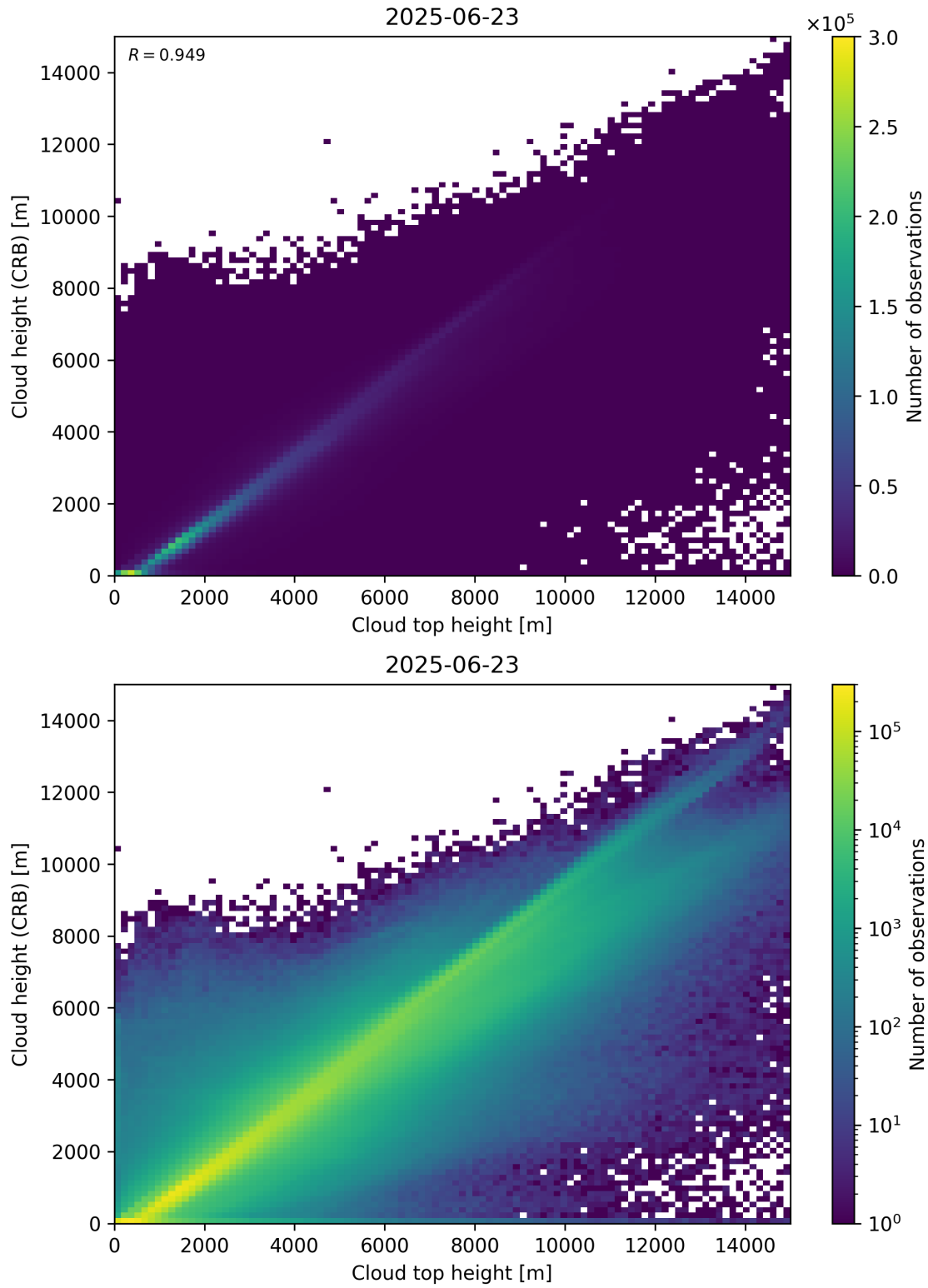
Figure 89: Scatter density plot of “Cloud top height” against “Cloud height (CRB)” for 2025-06-22 to 2025-06-24.
