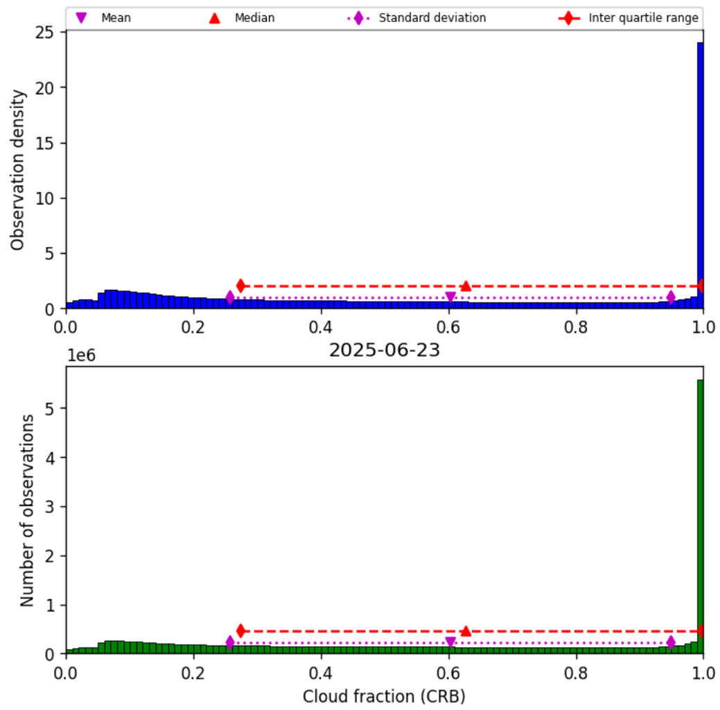
Figure 42: Histogram of “Cloud fraction (CRB)” for 2025-06-22 to 2025-06-24
