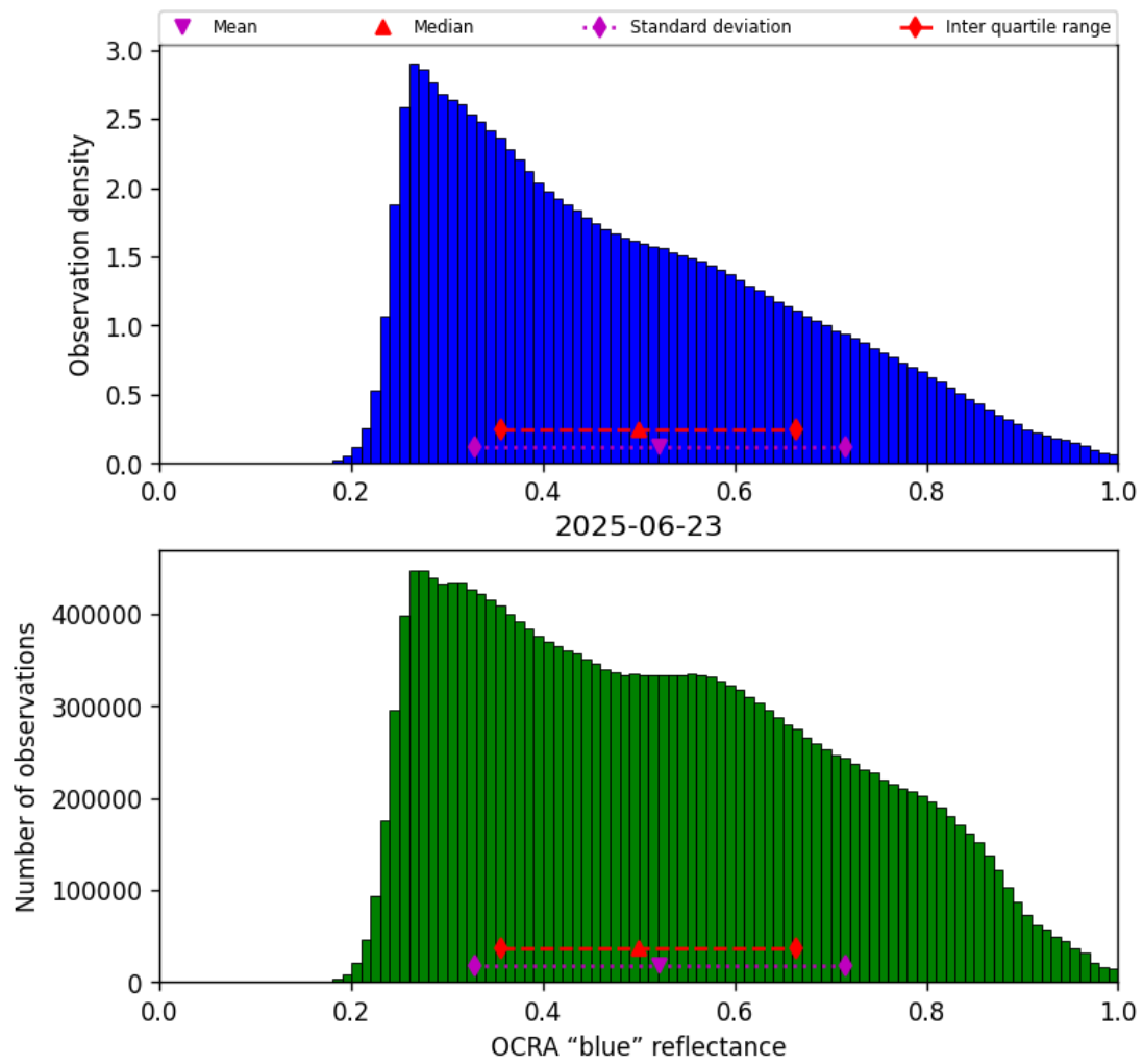
Figure 51: Histogram of “OCRA “blue” reflectance” for 2025-06-22 to 2025-06-24
