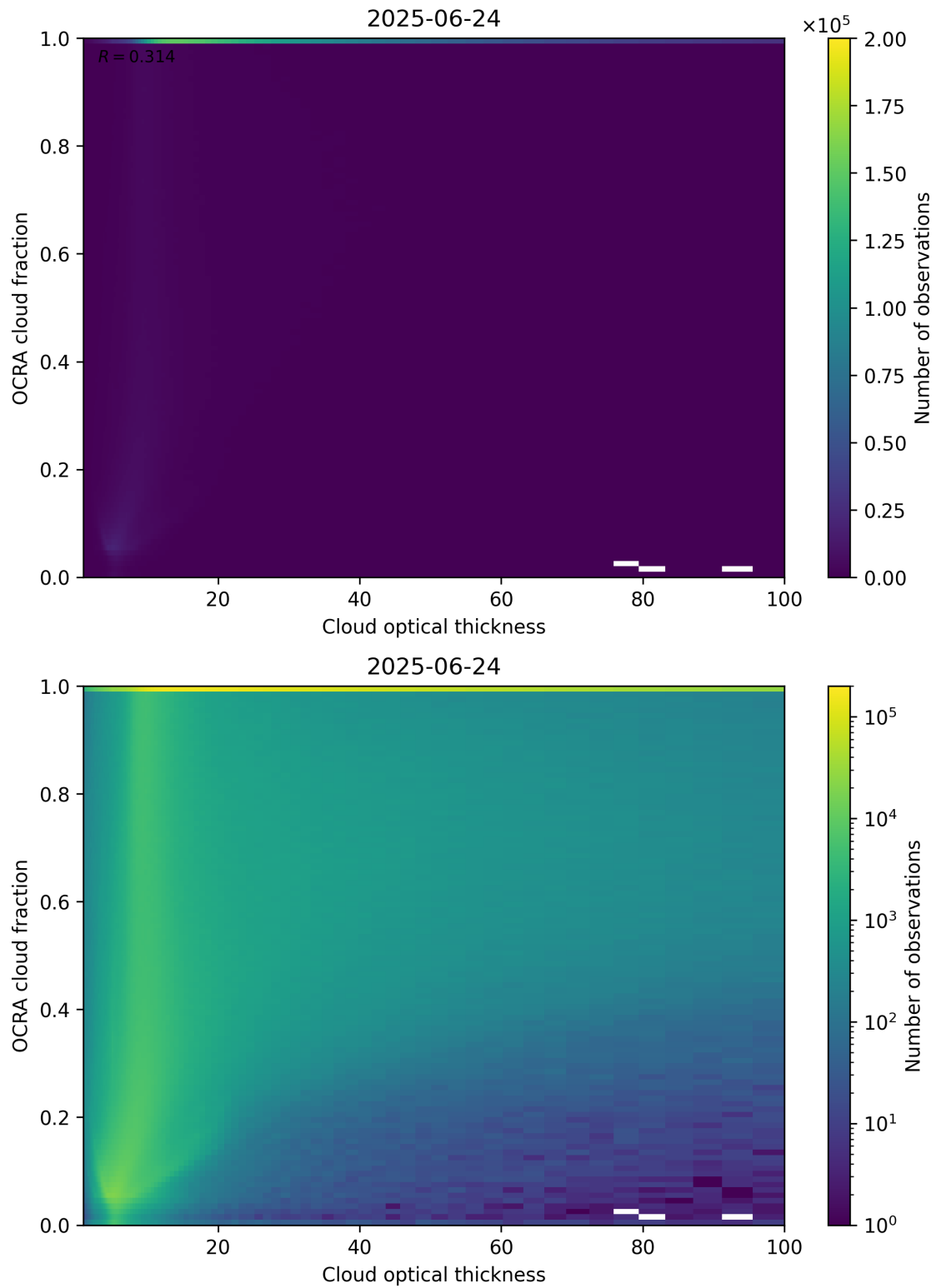
Figure 83: Scatter density plot of “Cloud optical thickness” against “OCRA cloud fraction” for 2025-06-23 to 2025-06-25.
