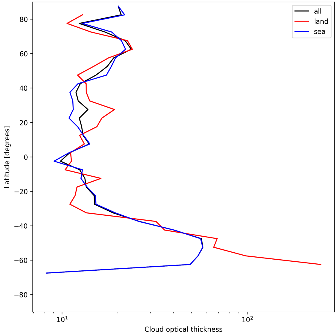
Figure 25: Zonal average of “Cloud optical thickness” for 2025-06-23 to 2025-06-25.
