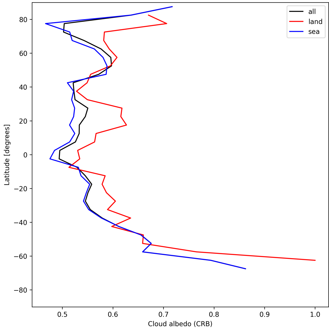
Figure 28: Zonal average of “Cloud albedo (CRB)” for 2025-06-23 to 2025-06-25.
