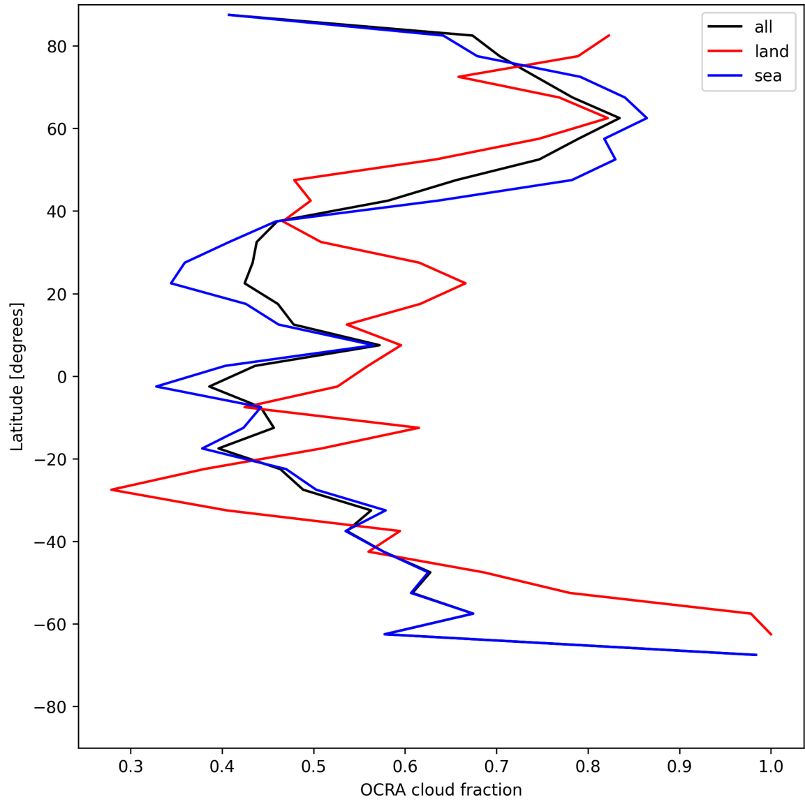
Figure 34: Zonal average of “OCRA cloud fraction” for 2025-06-23 to 2025-06-25.
