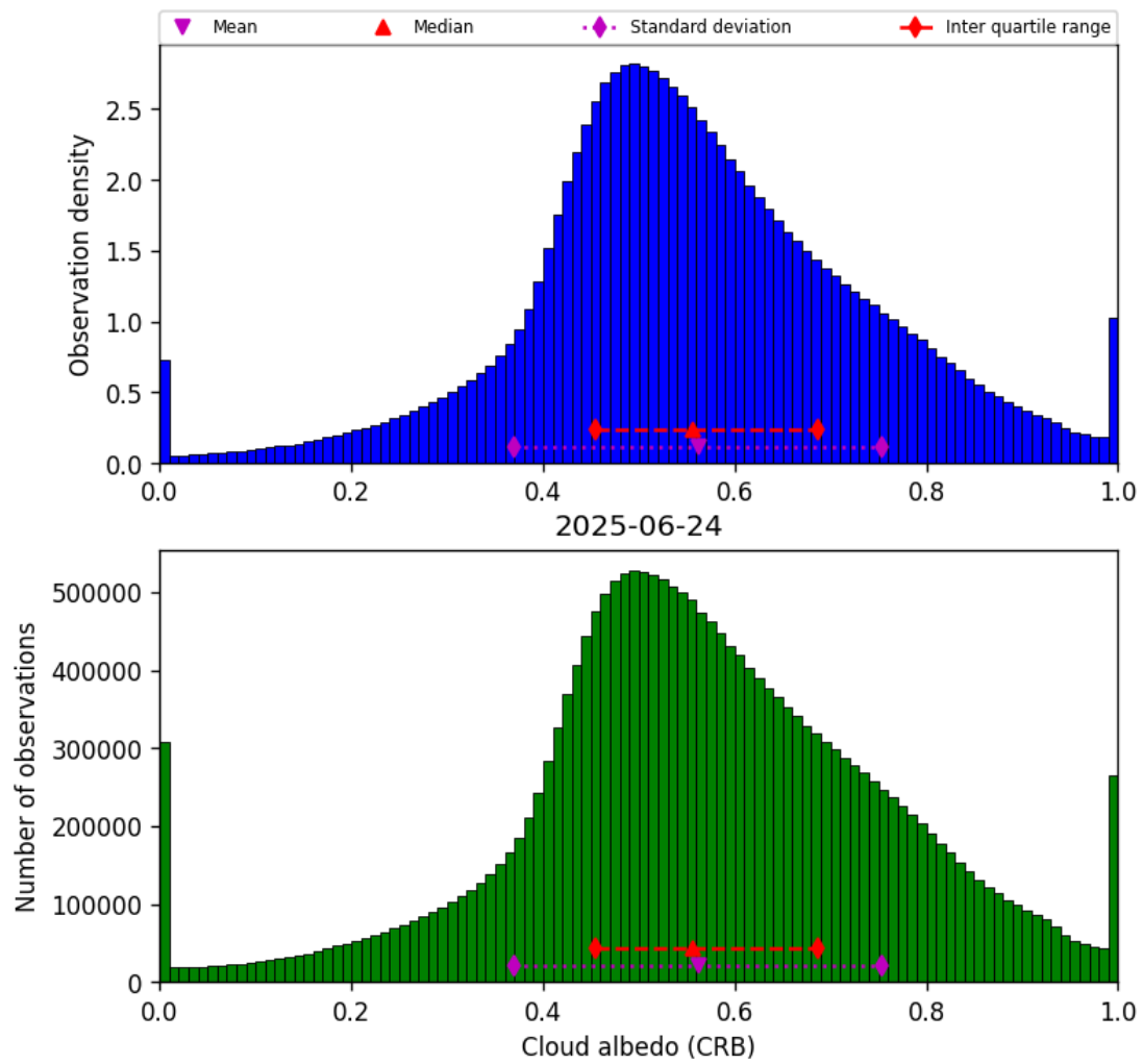
Figure 44: Histogram of “Cloud albedo (CRB)” for 2025-06-23 to 2025-06-25
