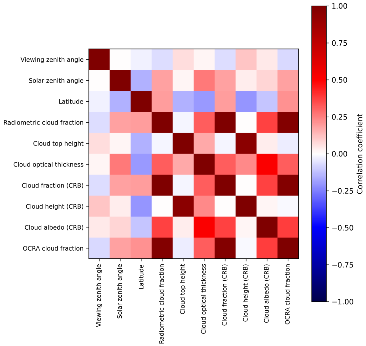
Figure 2: Map of correlation matrix for 2025-06-23 to 2025-06-25.
