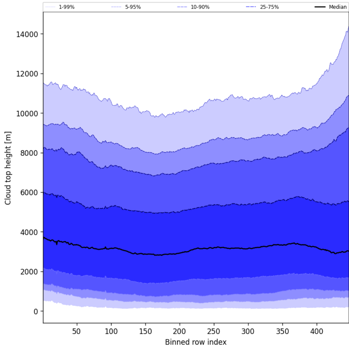
Figure 56: Along track statistics of “Cloud top height” for 2025-06-23 to 2025-06-25
