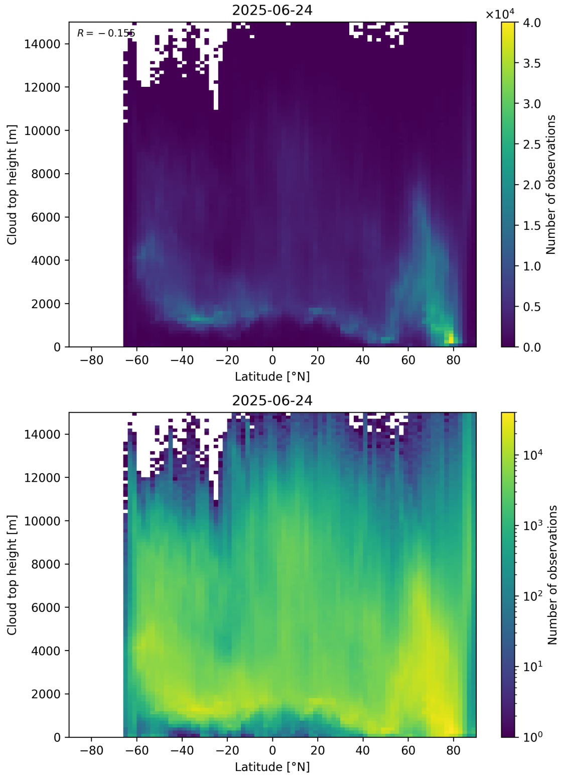
Figure 97: Scatter density plot of “Latitude” against “Cloud top height” for 2025-06-23 to 2025-06-25.
