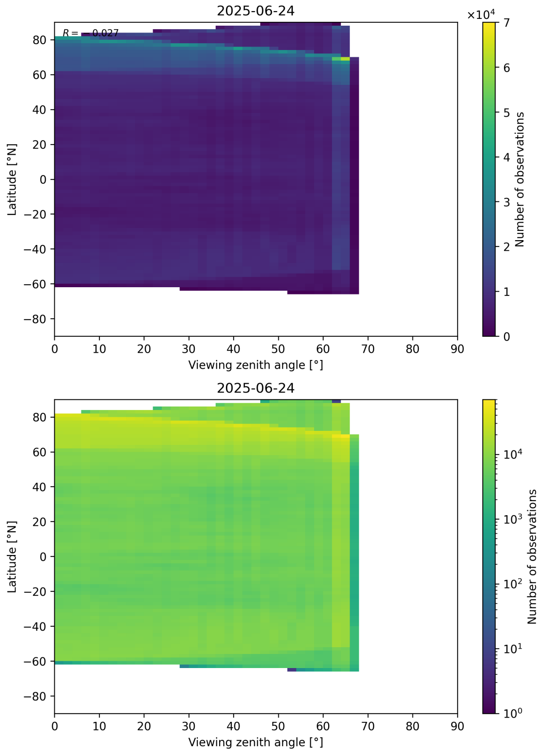
Figure 113: Scatter density plot of “Viewing zenith angle” against “Latitude” for 2025-06-23 to 2025-06-25.
