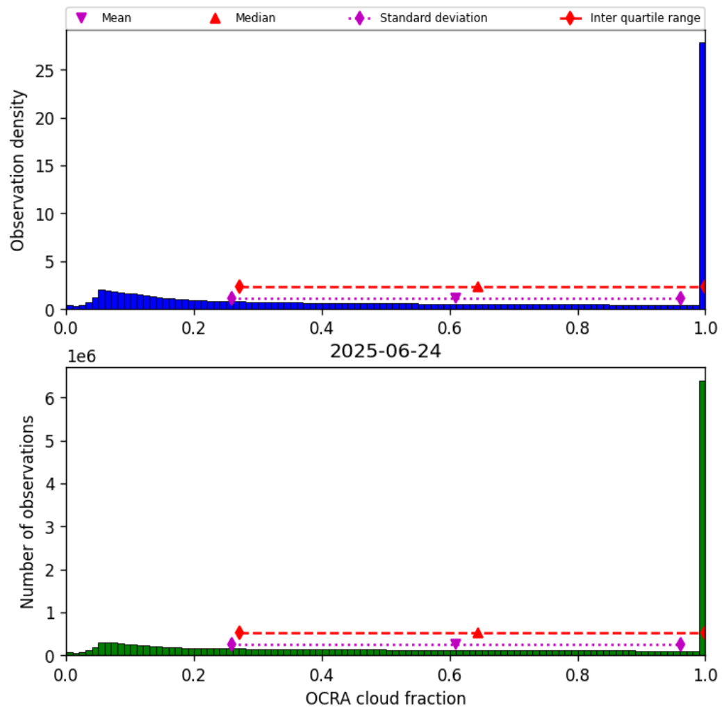
Figure 50: Histogram of “OCRA cloud fraction” for 2025-06-23 to 2025-06-25
