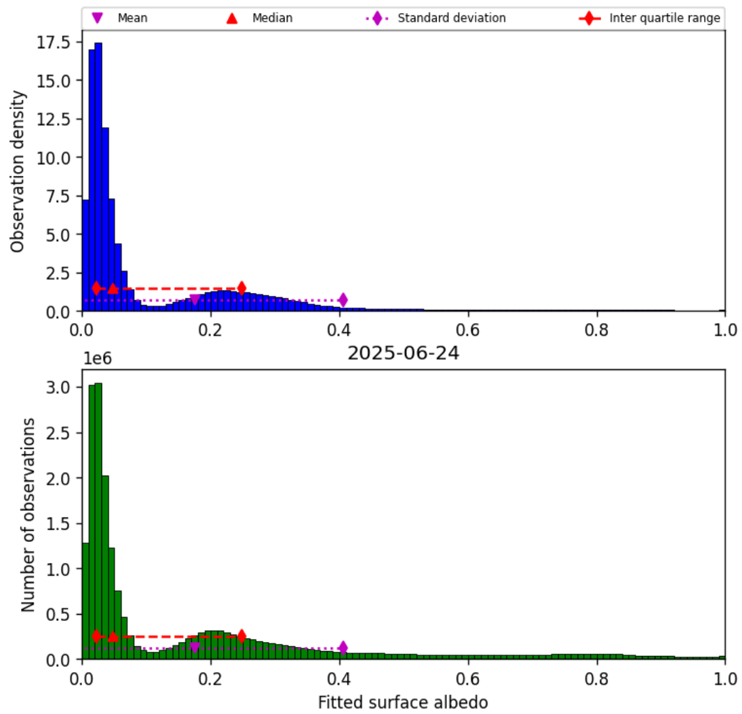
Figure 45: Histogram of “Fitted surface albedo” for 2025-06-23 to 2025-06-25
