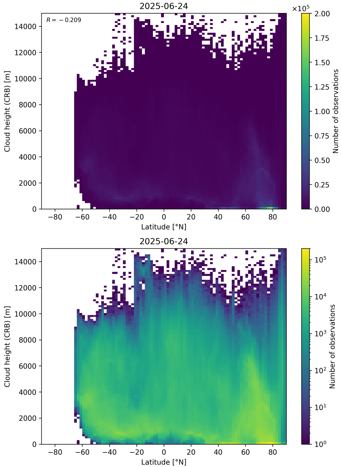
Figure 95: Scatter density plot of “Latitude” against “Cloud height (CRB)” for 2025-06-23 to 2025-06-25.
