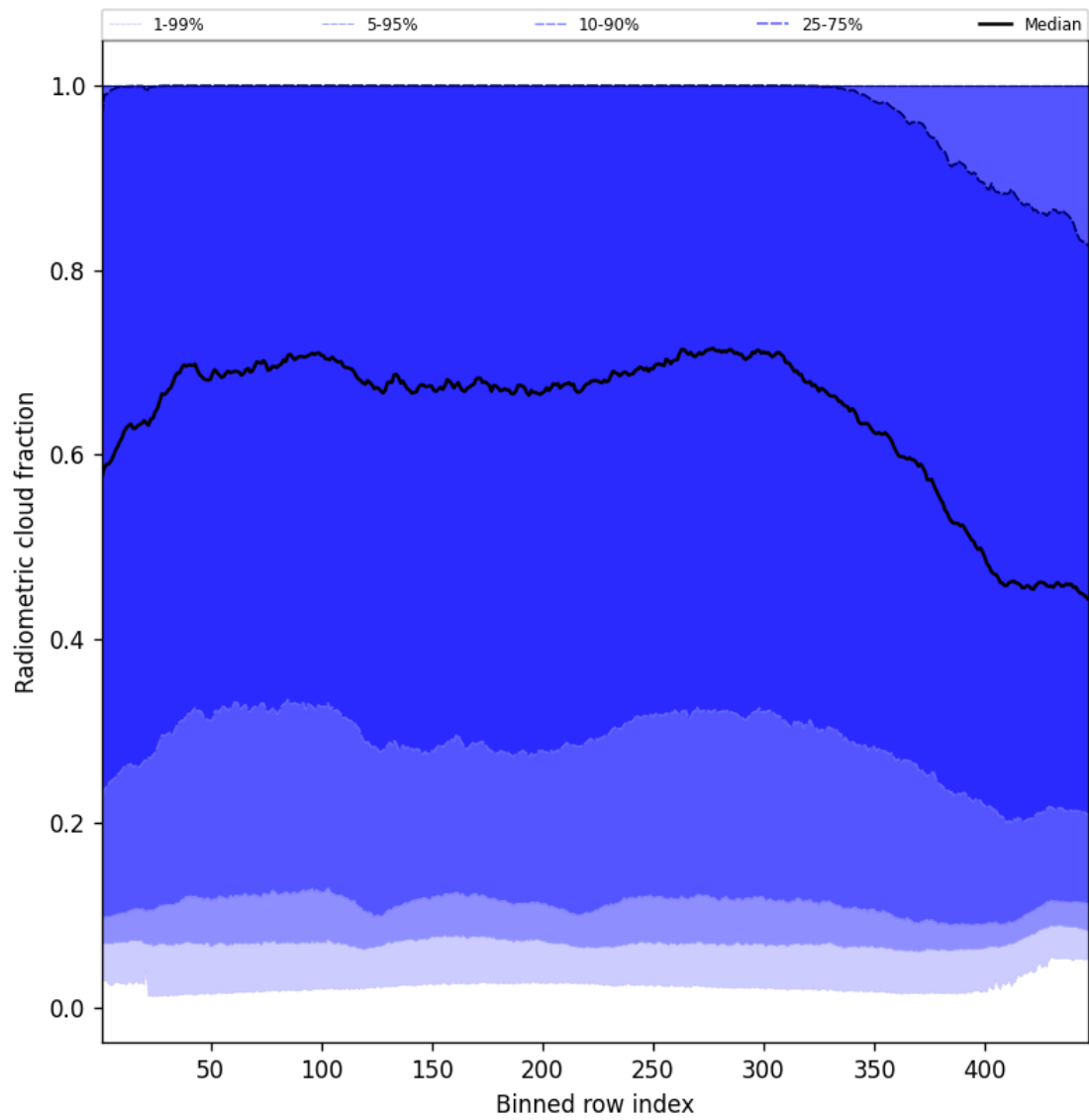
Figure 55: Along track statistics of “Radiometric cloud fraction” for 2025-06-23 to 2025-06-25
