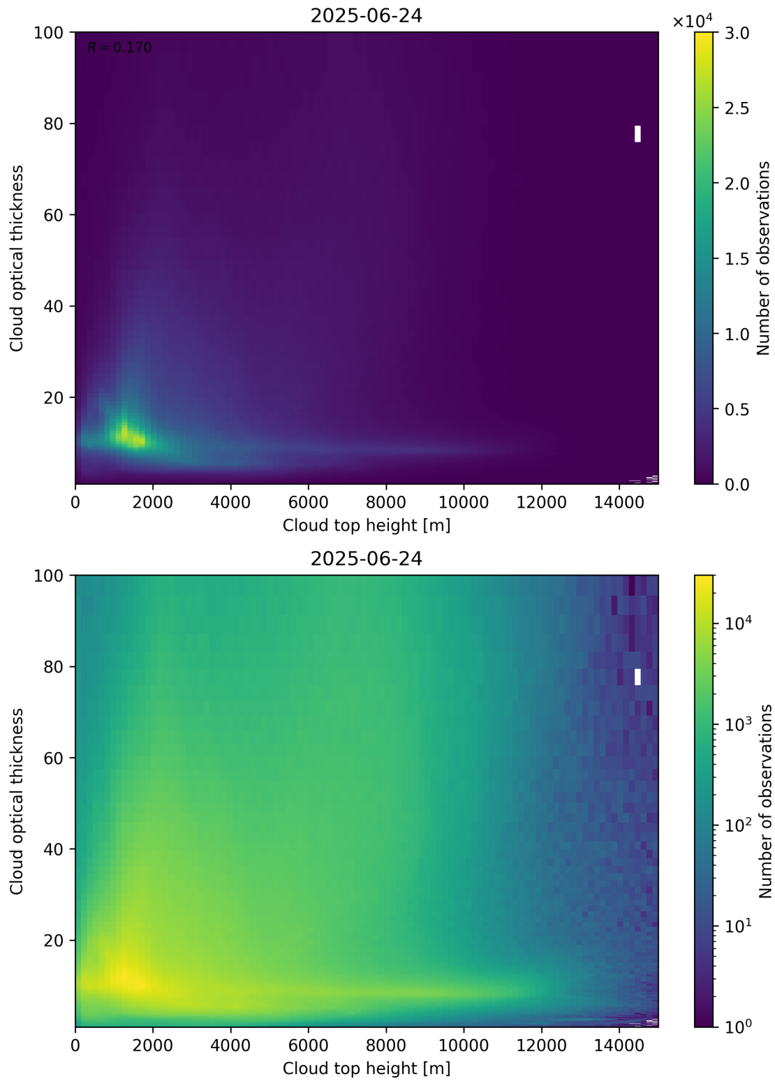
Figure 90: Scatter density plot of “Cloud top height” against “Cloud optical thickness” for 2025-06-23 to 2025-06-25.
