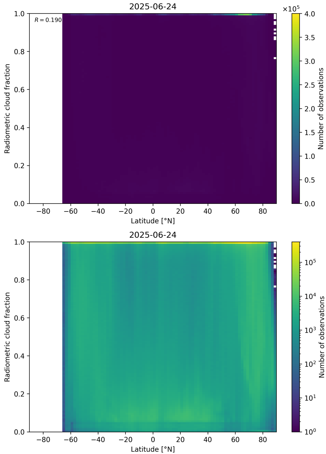
Figure 92: Scatter density plot of “Latitude” against “Radiometric cloud fraction” for 2025-06-23 to 2025-06-25.
