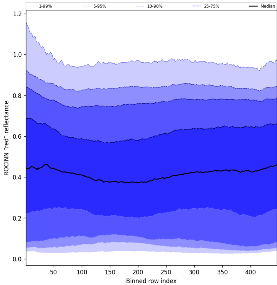
Figure 69: Along track statistics of “ROCINN “red” reflectance” for 2025-06-23 to 2025-06-25
