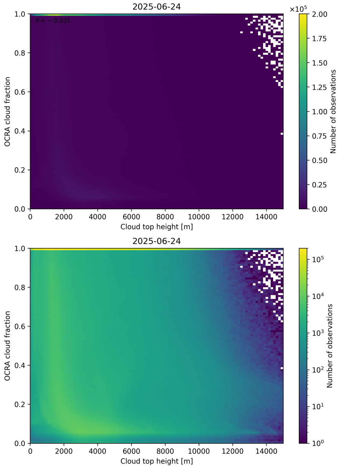
Figure 87: Scatter density plot of “Cloud top height” against “OCRA cloud fraction” for 2025-06-23 to 2025-06-25.
