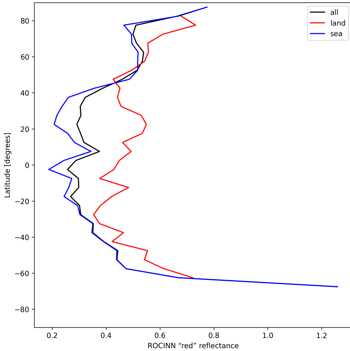
Figure 37: Zonal average of “ROCINN “red” reflectance” for 2025-06-23 to 2025-06-25.
