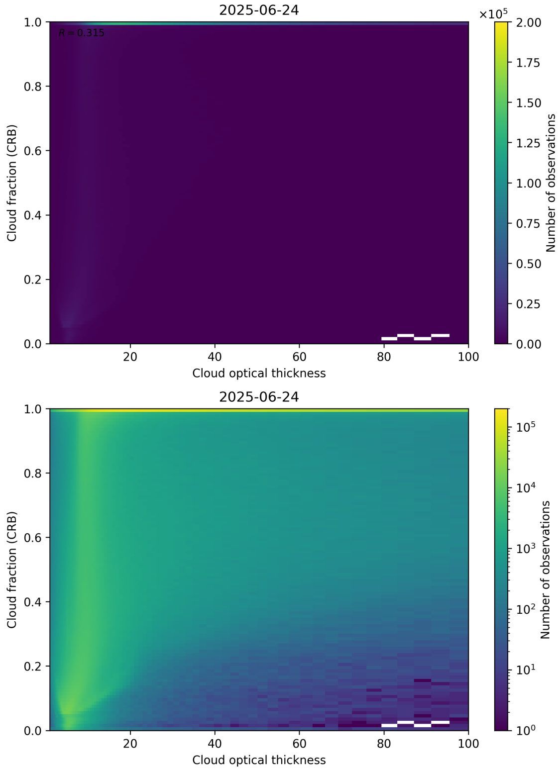
Figure 84: Scatter density plot of “Cloud optical thickness” against “Cloud fraction (CRB)” for 2025-06-23 to 2025-06-25.
