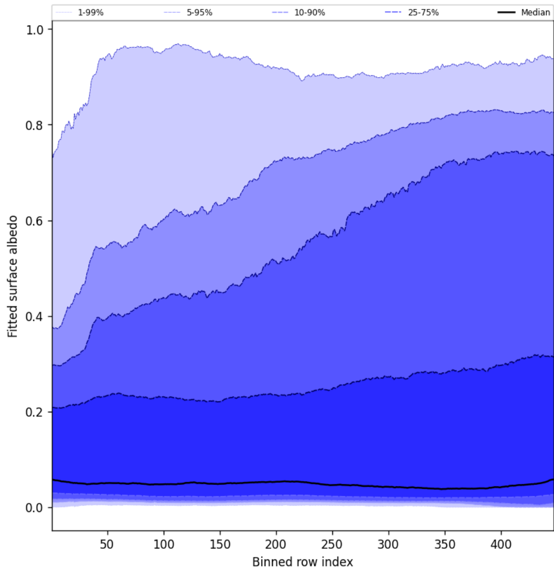
Figure 61: Along track statistics of “Fitted surface albedo” for 2025-06-23 to 2025-06-25
