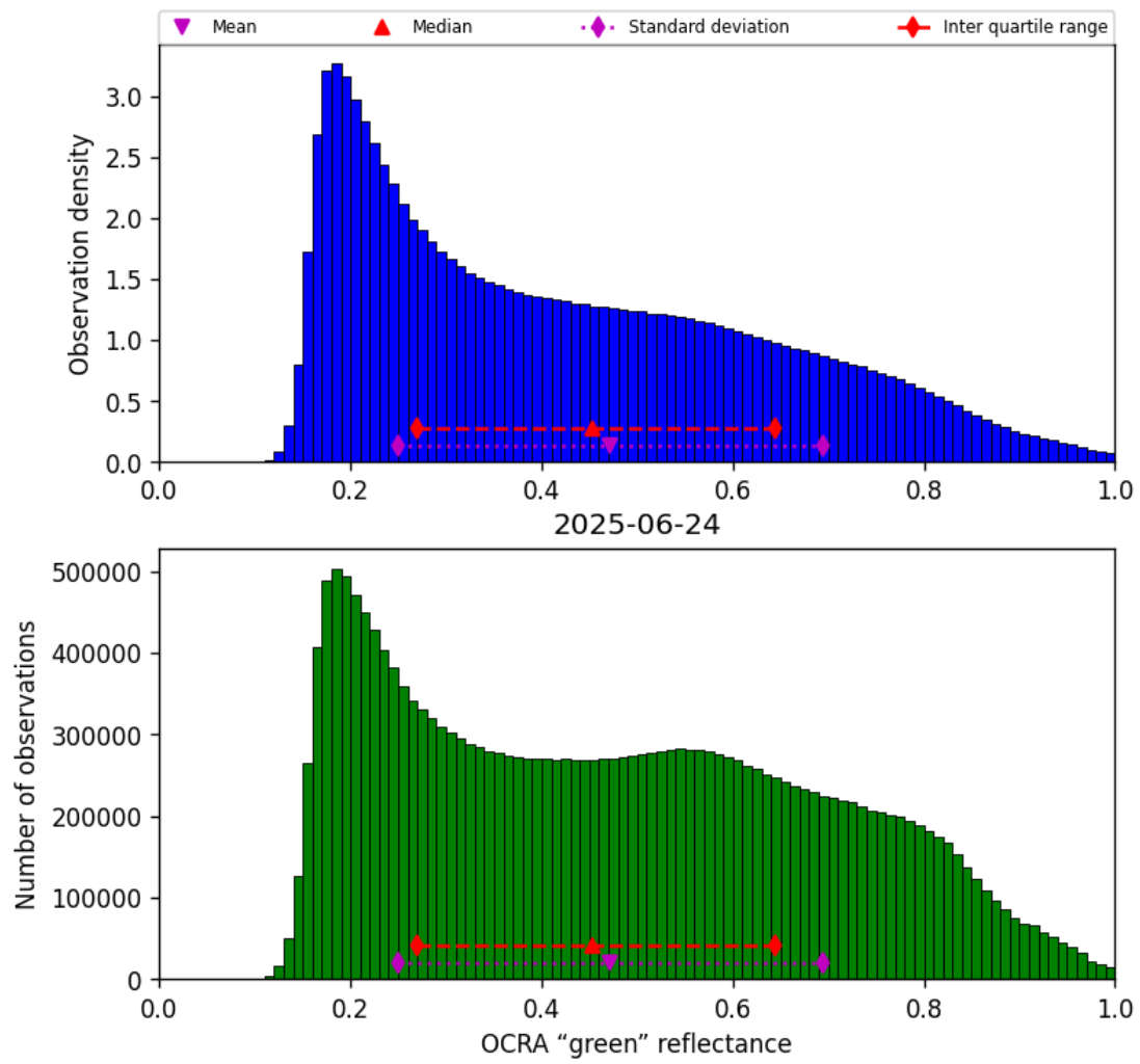
Figure 52: Histogram of “OCRA “green” reflectance” for 2025-06-23 to 2025-06-25
