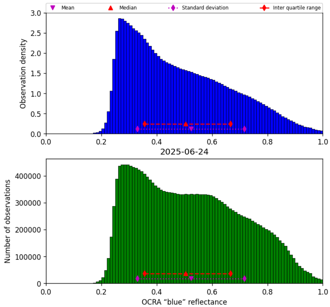
Figure 51: Histogram of “OCRA “blue” reflectance” for 2025-06-23 to 2025-06-25
