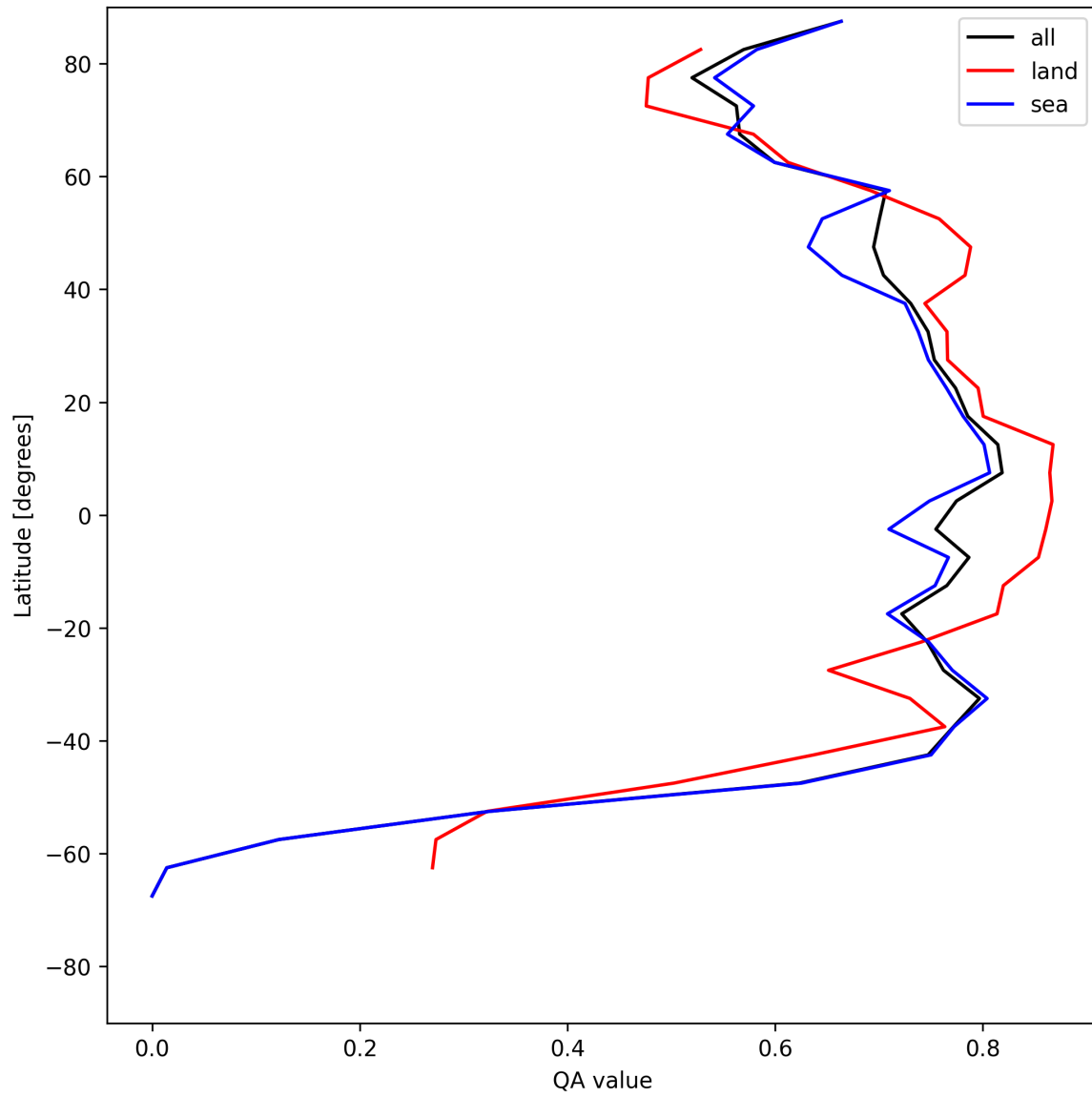
Figure 22: Zonal average of “QA value” for 2025-06-23 to 2025-06-25.
