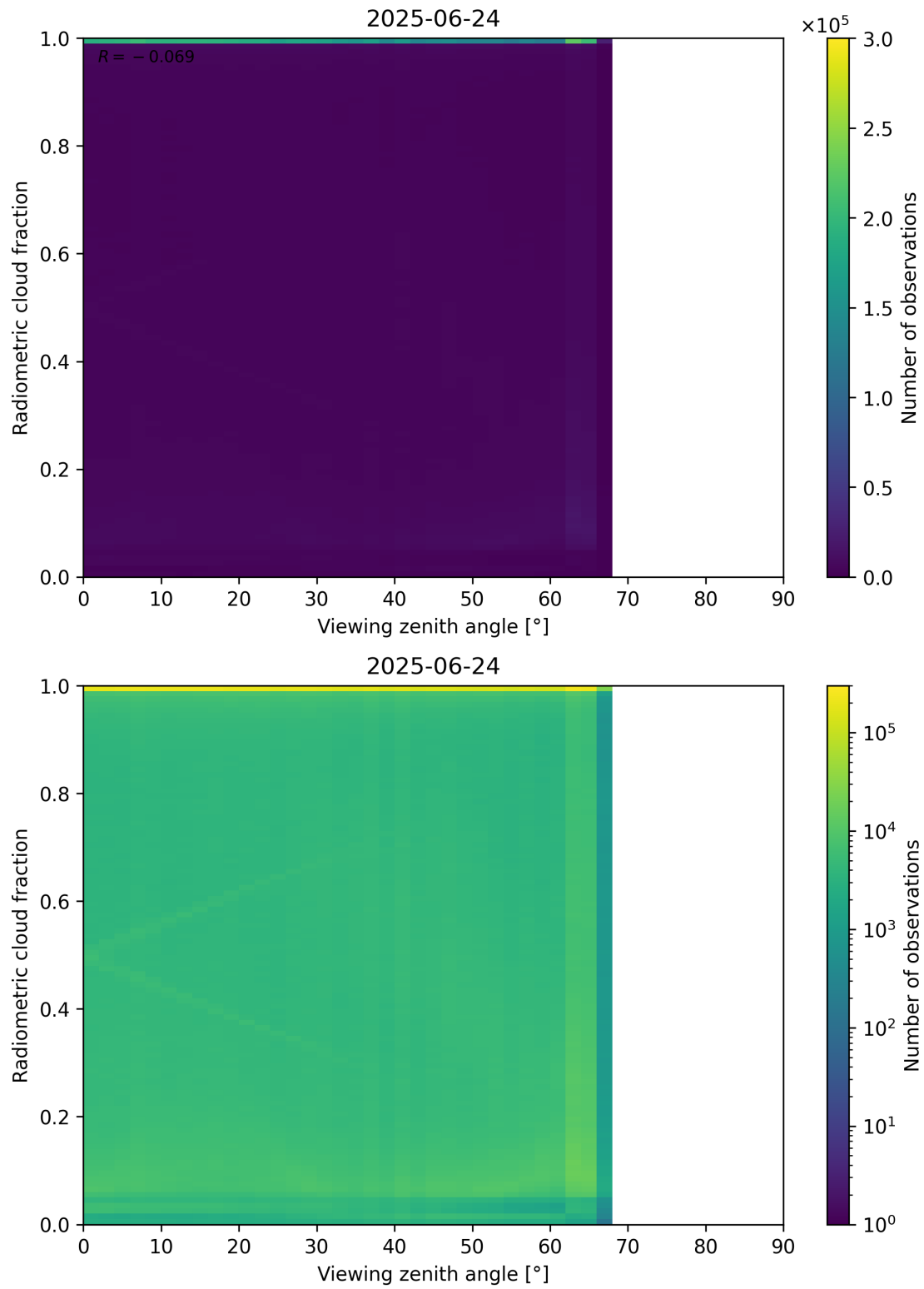
Figure 107: Scatter density plot of “Viewing zenith angle” against “Radiometric cloud fraction” for 2025-06-23 to 2025-06-25.
