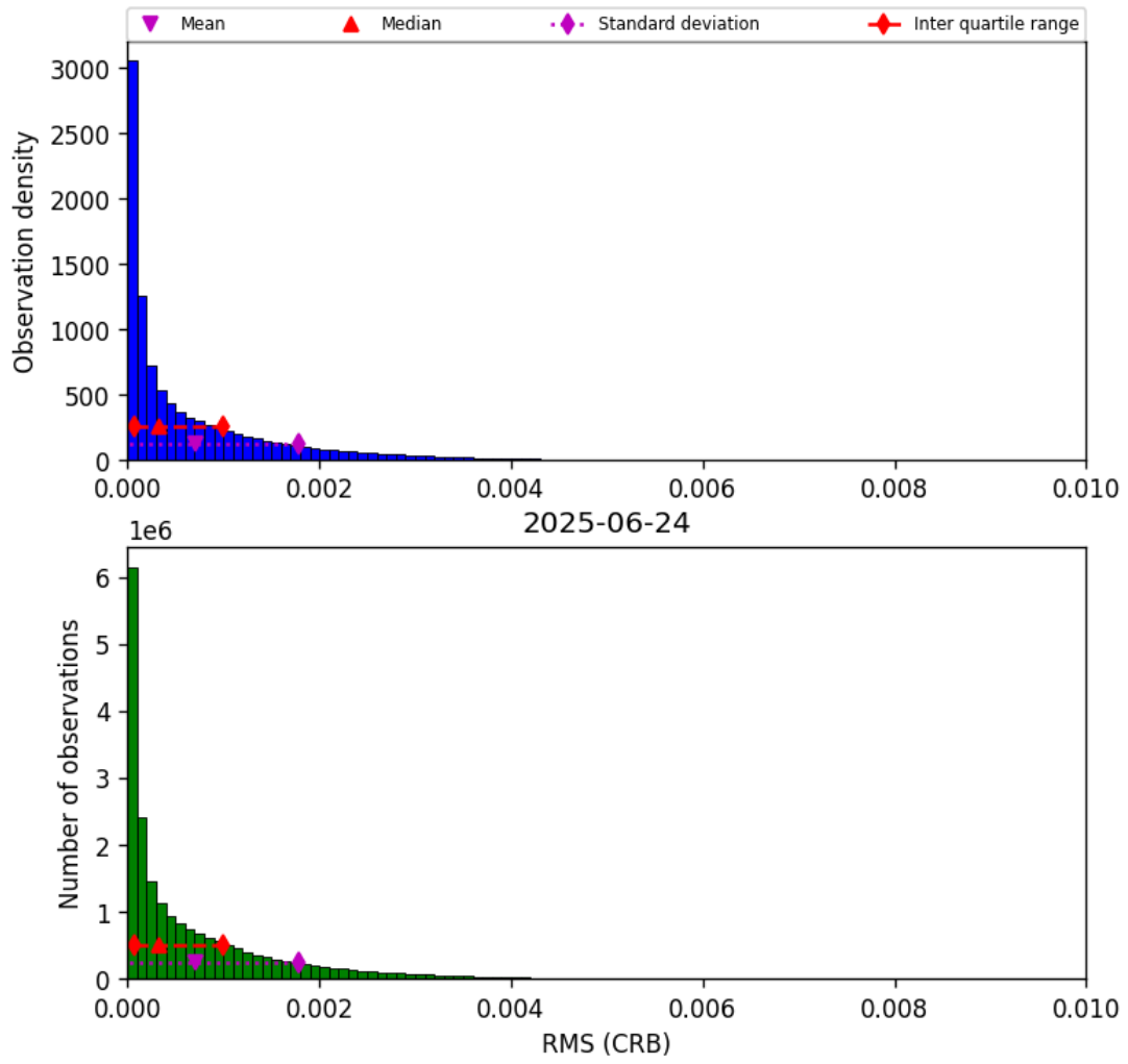
Figure 48: Histogram of “RMS (CRB)” for 2025-06-23 to 2025-06-25
