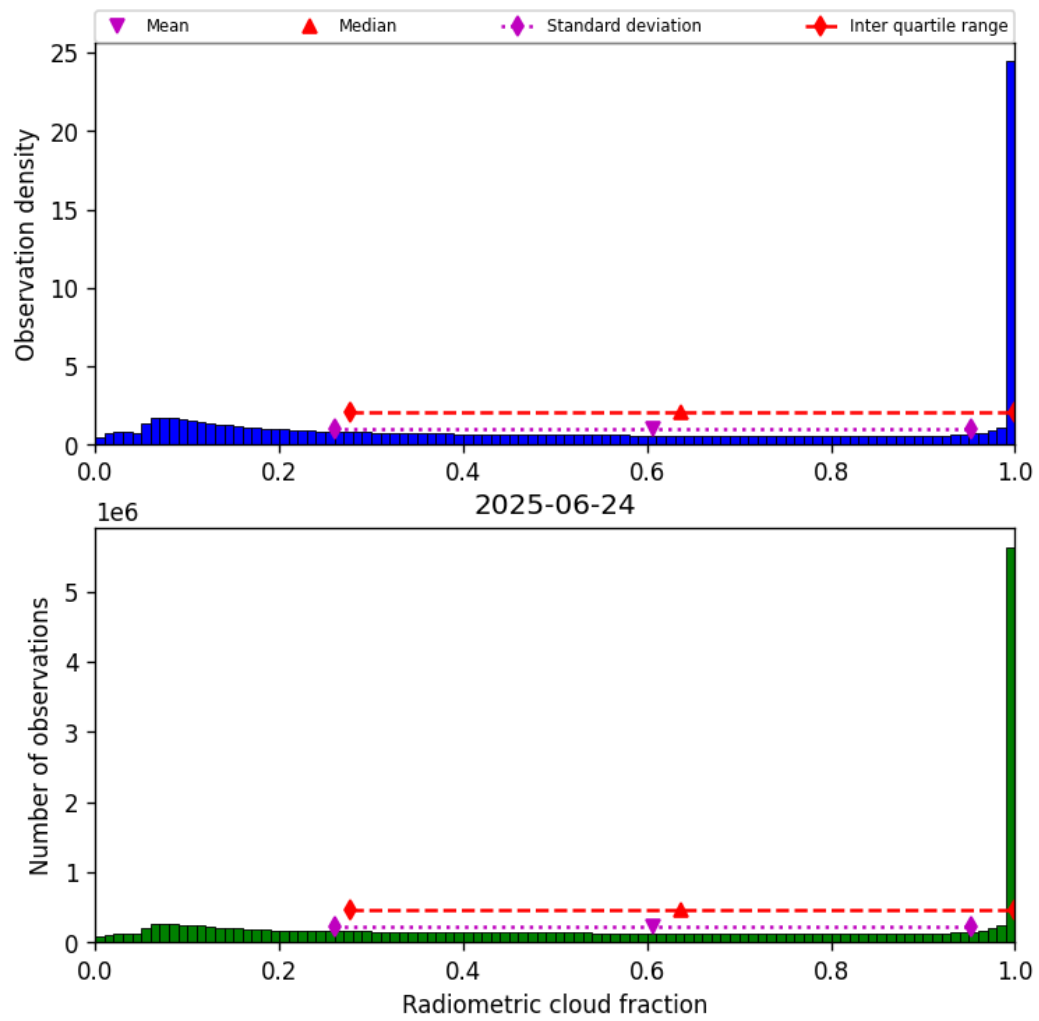
Figure 39: Histogram of “Radiometric cloud fraction” for 2025-06-23 to 2025-06-25
