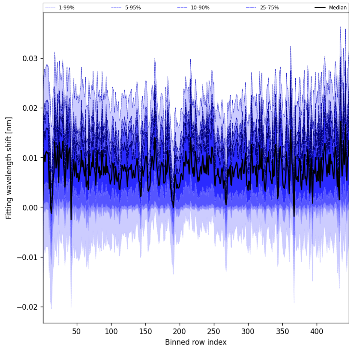
Figure 65: Along track statistics of “Fitting wavelength shift” for 2025-06-23 to 2025-06-25
