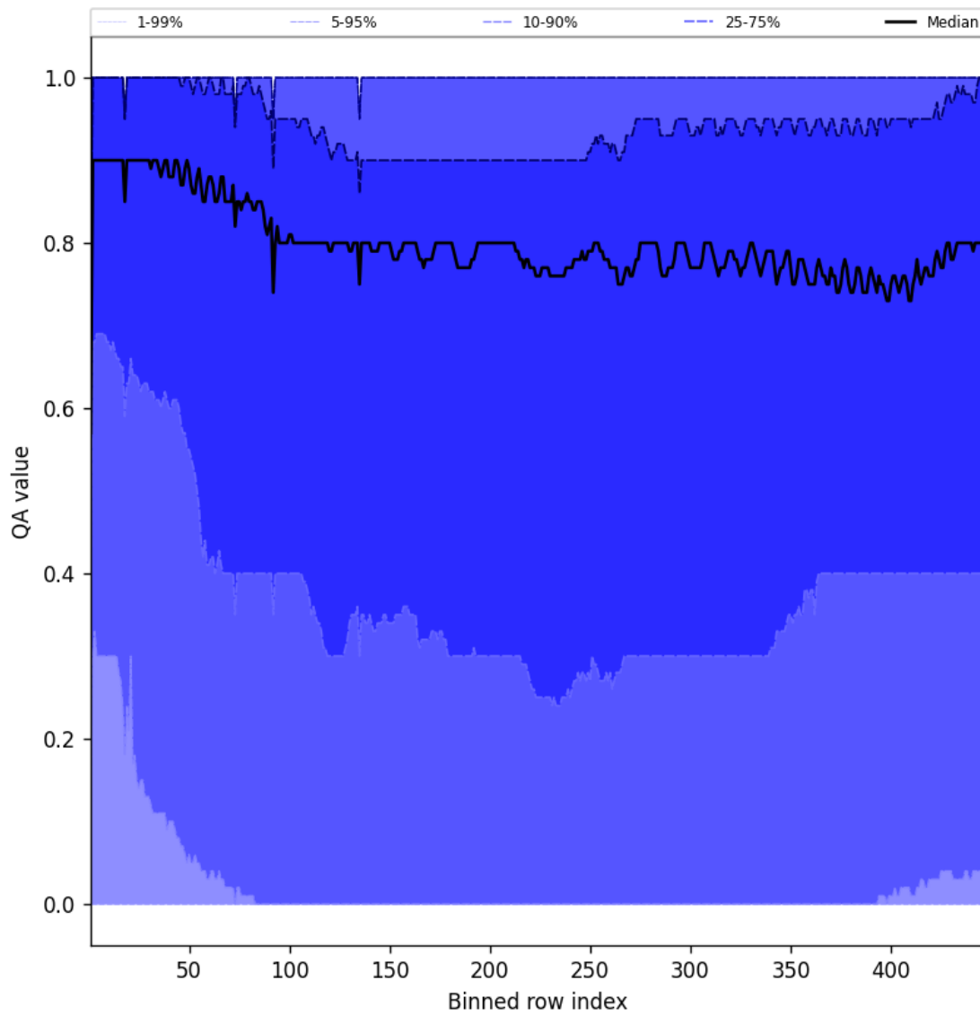
Figure 54: Along track statistics of “QA value” for 2025-06-23 to 2025-06-25
