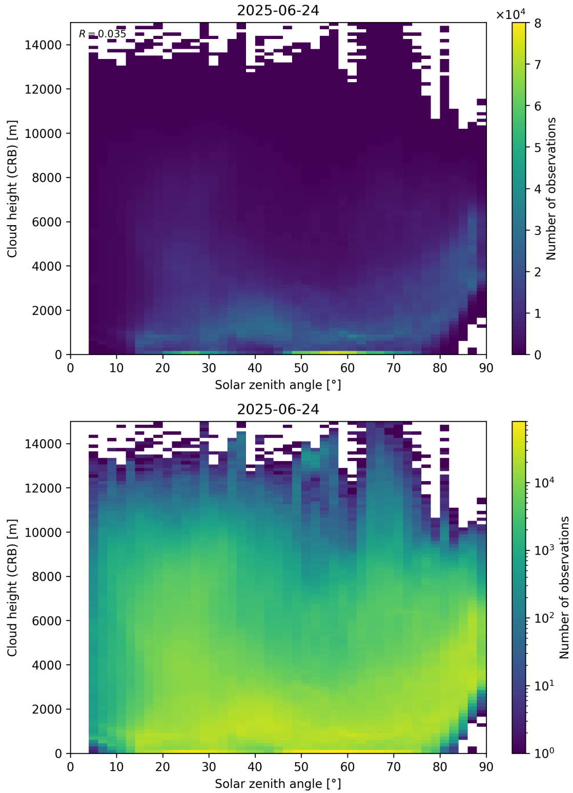
Figure 102: Scatter density plot of “Solar zenith angle” against “Cloud height (CRB)” for 2025-06-23 to 2025-06-25.
