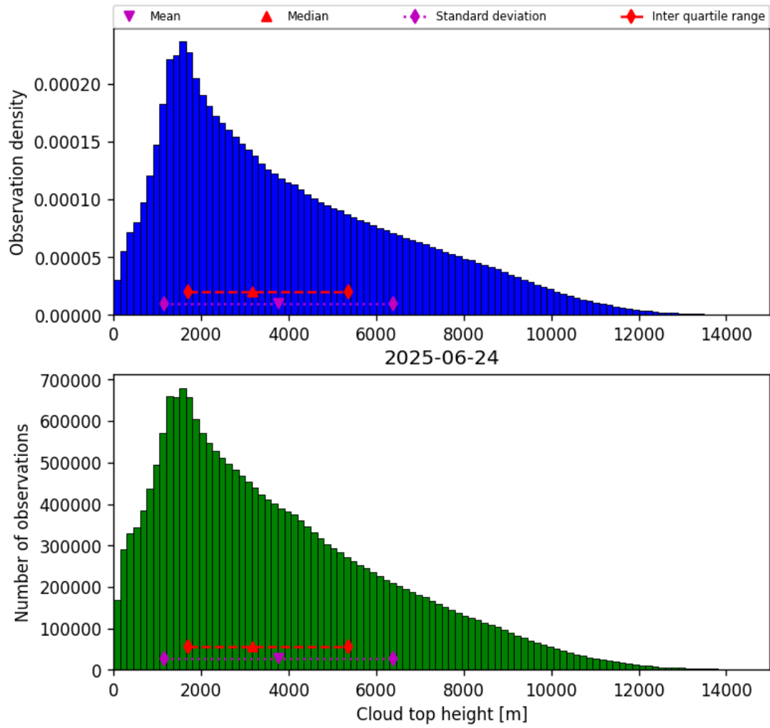
Figure 40: Histogram of “Cloud top height” for 2025-06-23 to 2025-06-25
