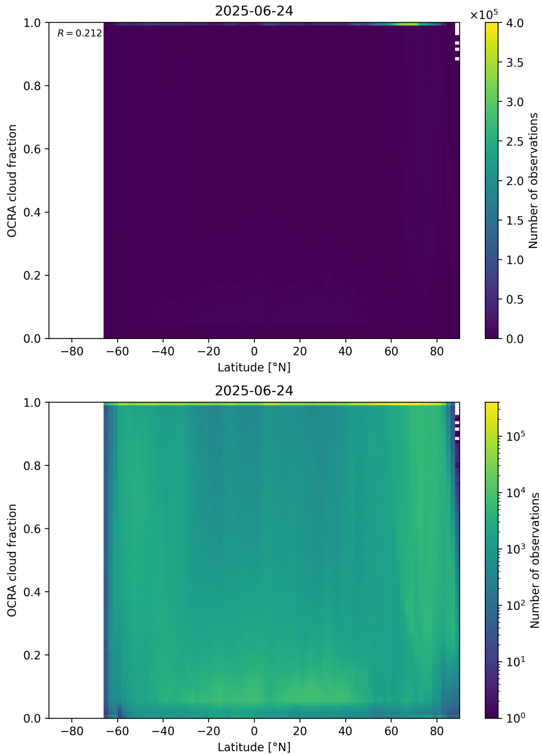
Figure 93: Scatter density plot of “Latitude” against “OCRA cloud fraction” for 2025-06-23 to 2025-06-25.
