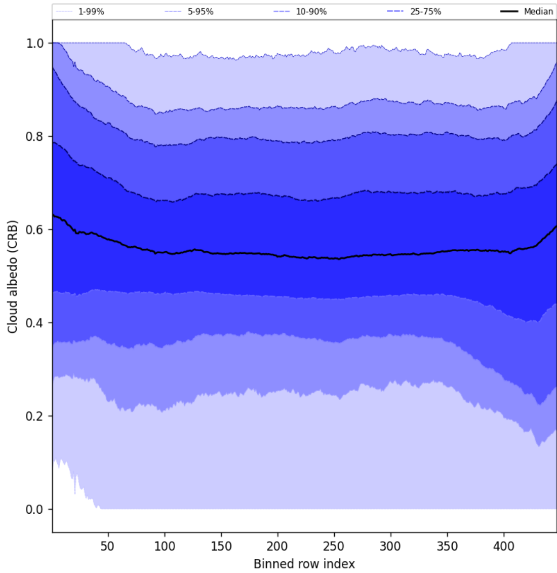
Figure 60: Along track statistics of “Cloud albedo (CRB)” for 2025-06-23 to 2025-06-25
