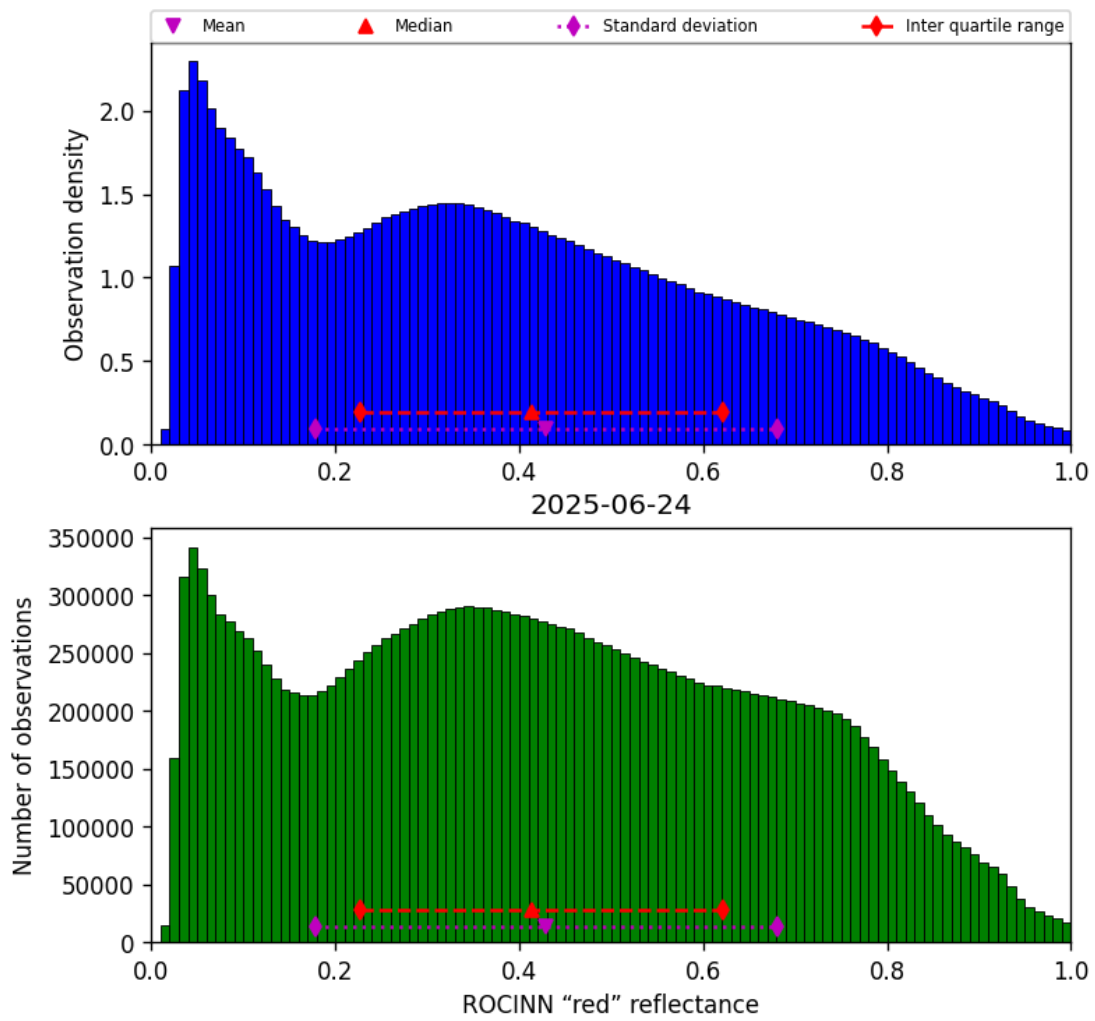
Figure 53: Histogram of “ROCINN “red” reflectance” for 2025-06-23 to 2025-06-25
