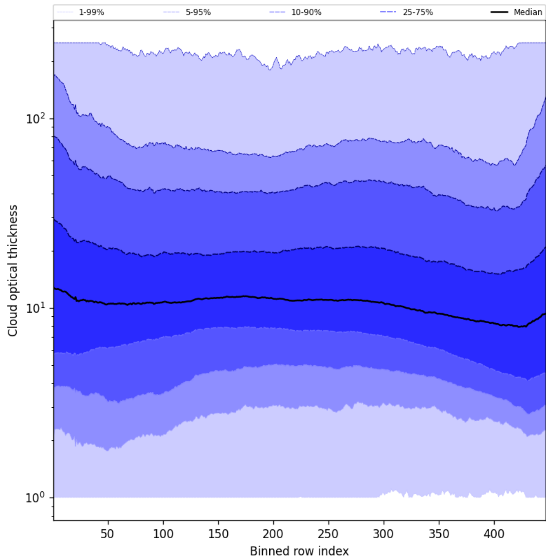
Figure 57: Along track statistics of “Cloud optical thickness” for 2025-06-23 to 2025-06-25
