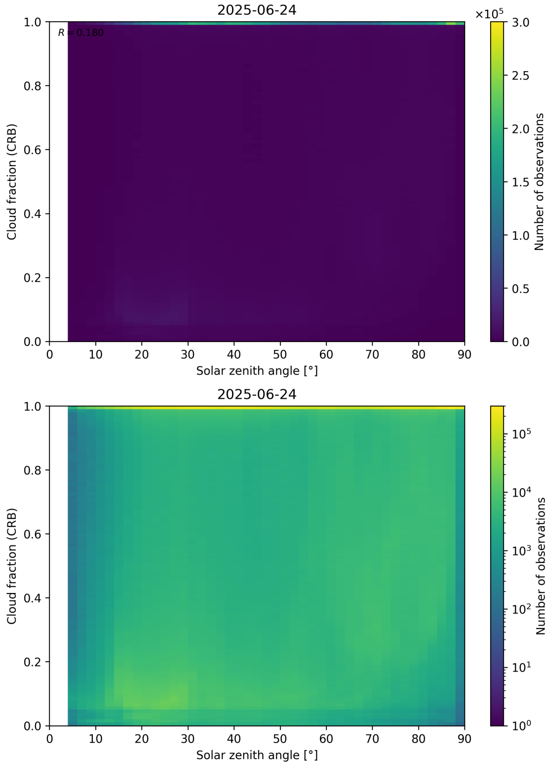
Figure 101: Scatter density plot of “Solar zenith angle” against “Cloud fraction (CRB)” for 2025-06-23 to 2025-06-25.
