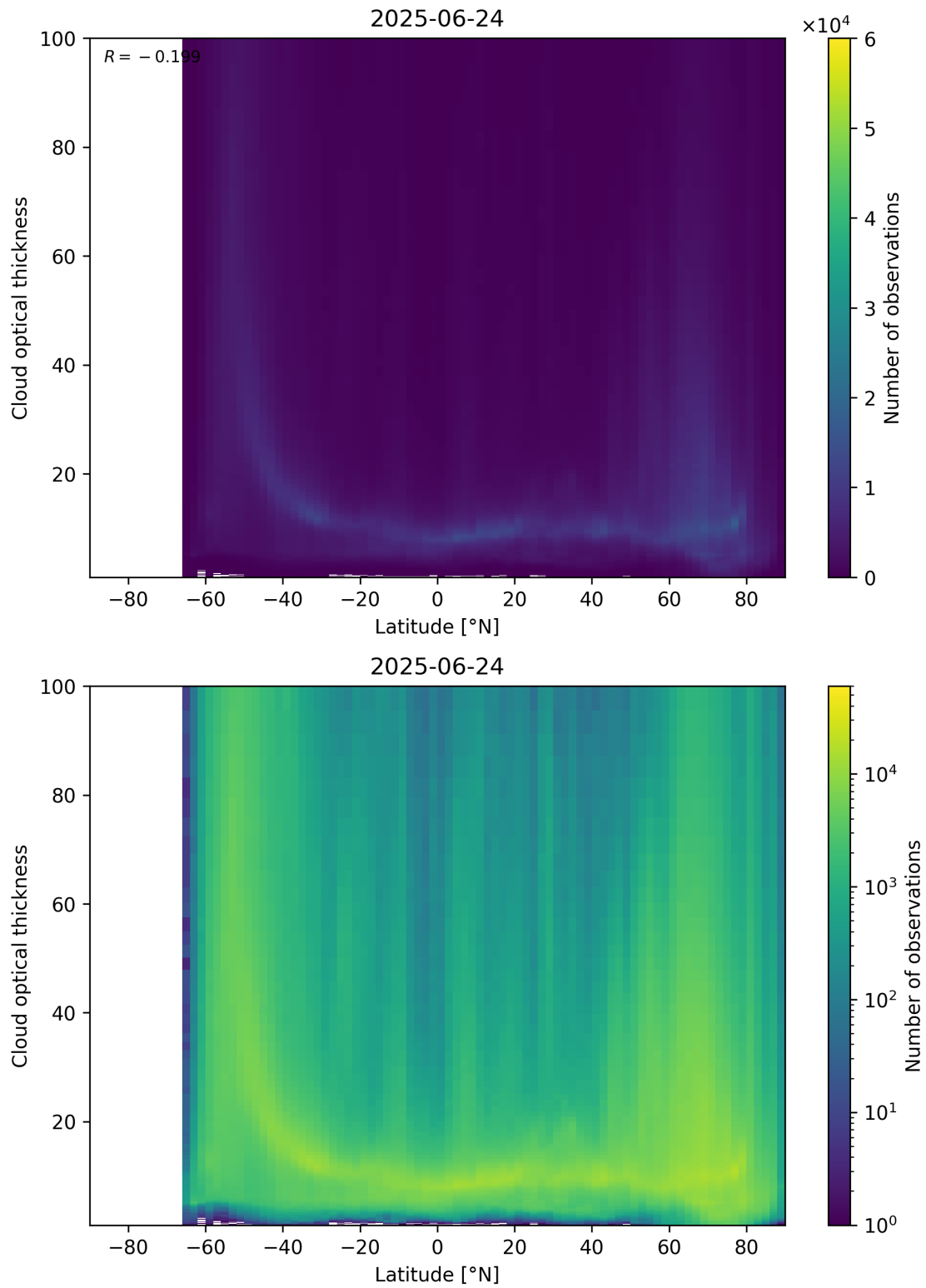
Figure 96: Scatter density plot of “Latitude” against “Cloud optical thickness” for 2025-06-23 to 2025-06-25.
