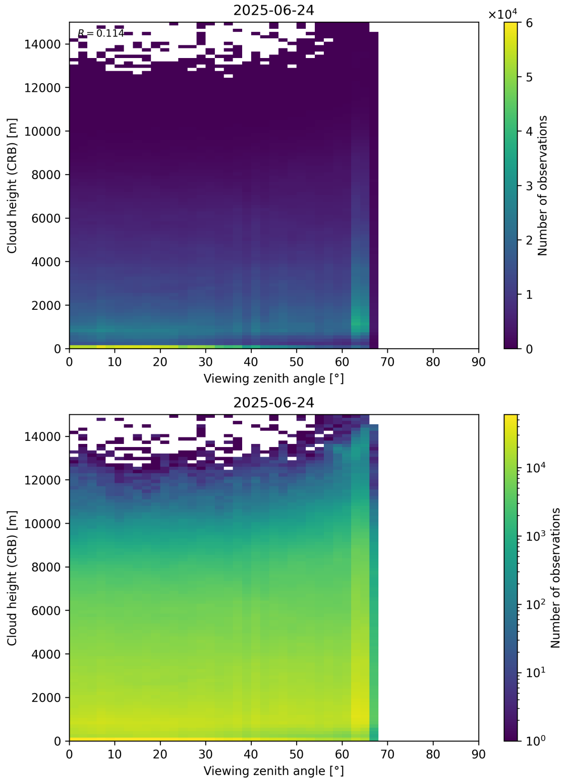
Figure 110: Scatter density plot of “Viewing zenith angle” against “Cloud height (CRB)” for 2025-06-23 to 2025-06-25.
