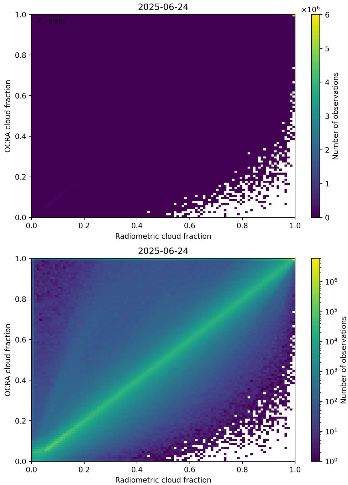
Figure 72: Scatter density plot of “Radiometric cloud fraction” against “OCRA cloud fraction” for 2025-06-23 to 2025-06-25.
