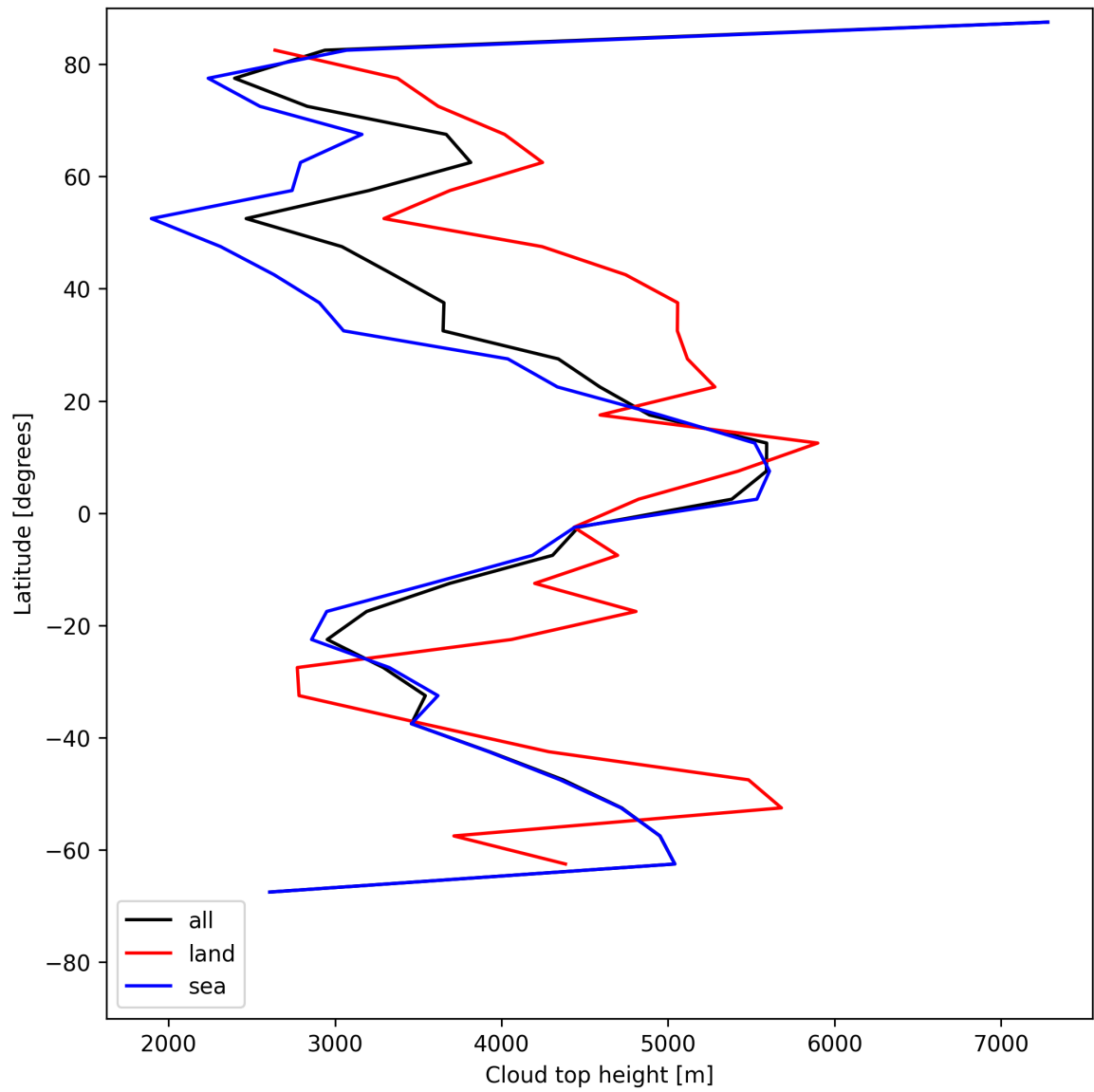
Figure 24: Zonal average of “Cloud top height” for 2025-06-23 to 2025-06-25.
