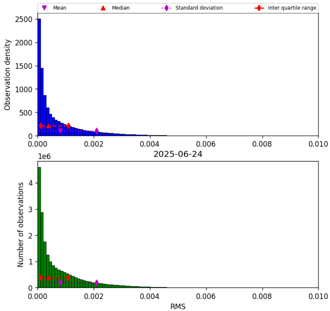
Figure 47: Histogram of “RMS” for 2025-06-23 to 2025-06-25
