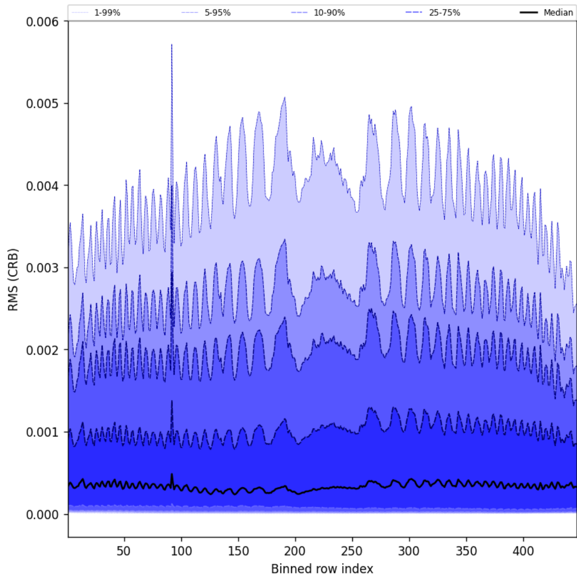
Figure 64: Along track statistics of “RMS (CRB)” for 2025-06-23 to 2025-06-25
