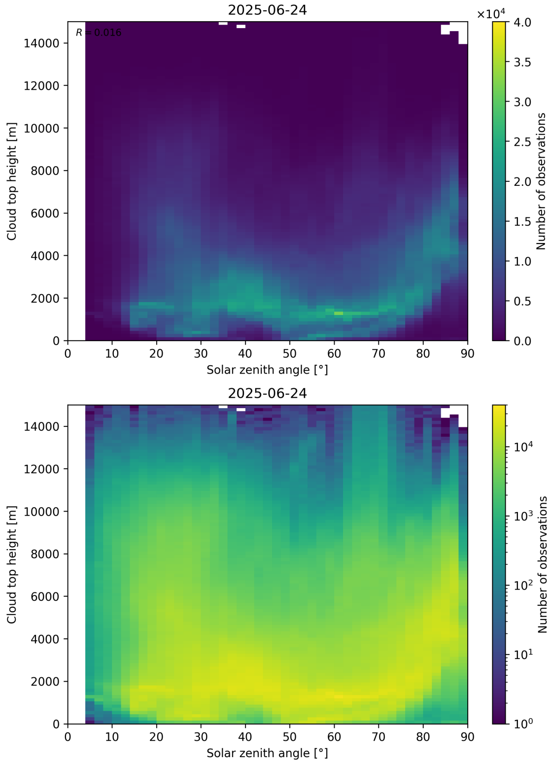
Figure 104: Scatter density plot of “Solar zenith angle” against “Cloud top height” for 2025-06-23 to 2025-06-25.
