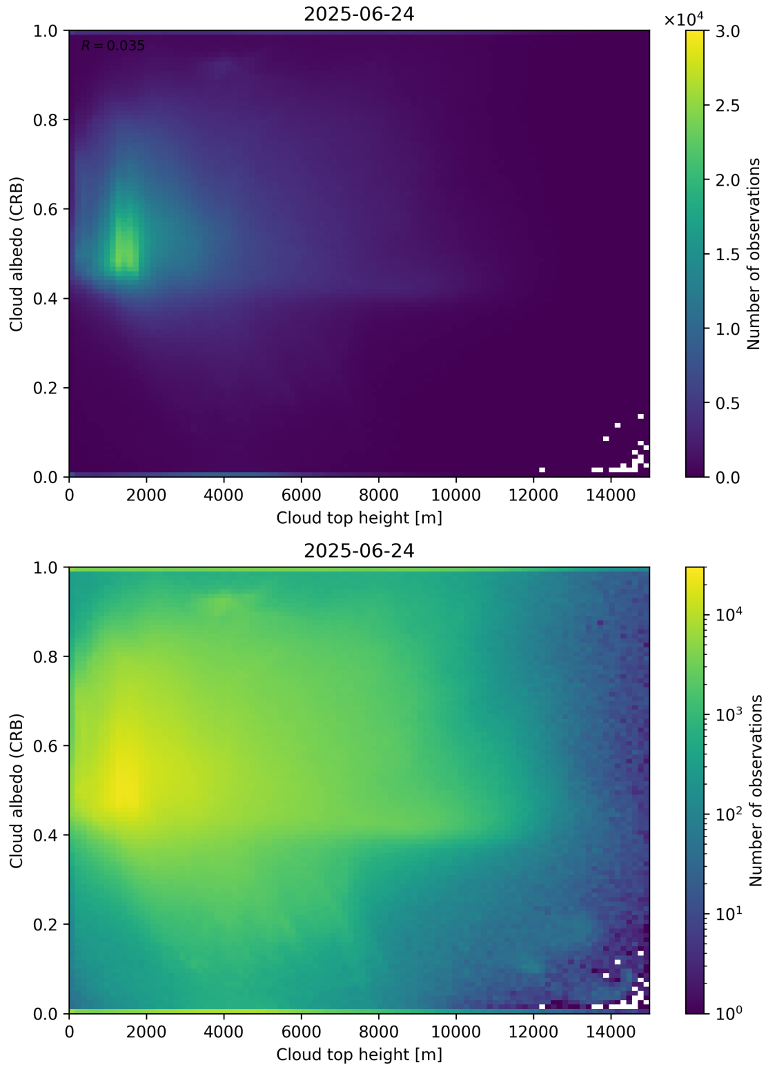
Figure 86: Scatter density plot of “Cloud top height” against “Cloud albedo (CRB)” for 2025-06-23 to 2025-06-25.
