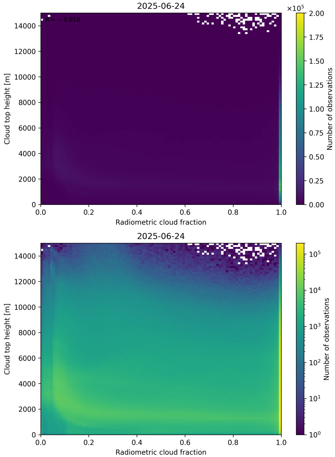
Figure 76: Scatter density plot of “Radiometric cloud fraction” against “Cloud top height” for 2025-06-23 to 2025-06-25.
