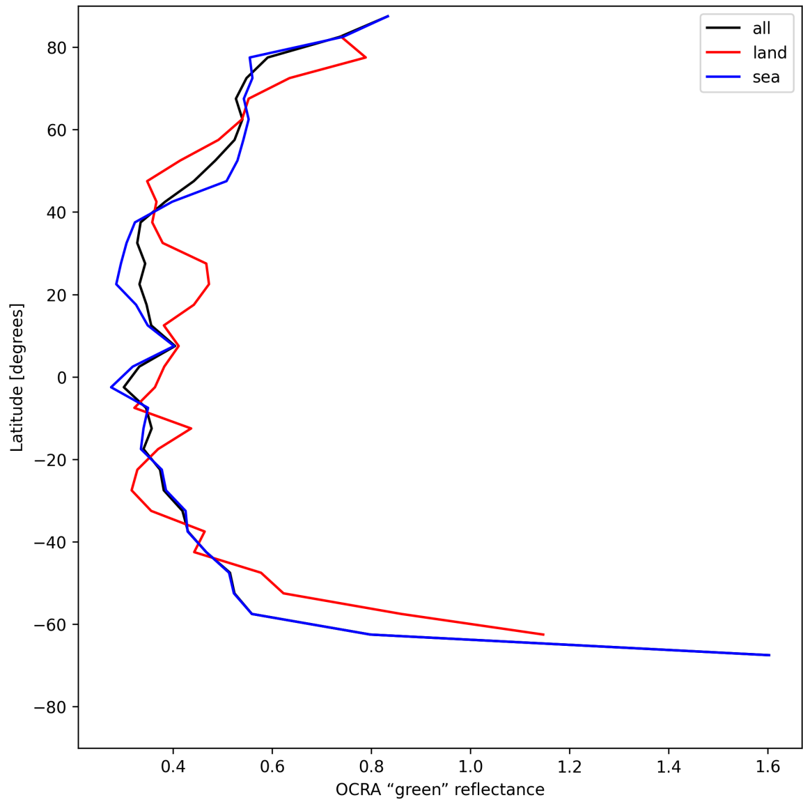
Figure 36: Zonal average of “OCRA “green” reflectance” for 2025-06-23 to 2025-06-25.
