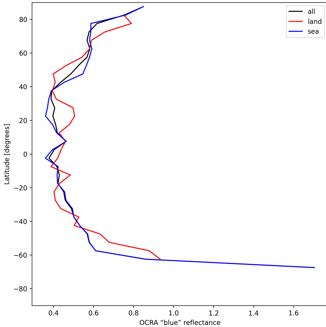
Figure 35: Zonal average of “OCRA “blue” reflectance” for 2025-06-23 to 2025-06-25.
