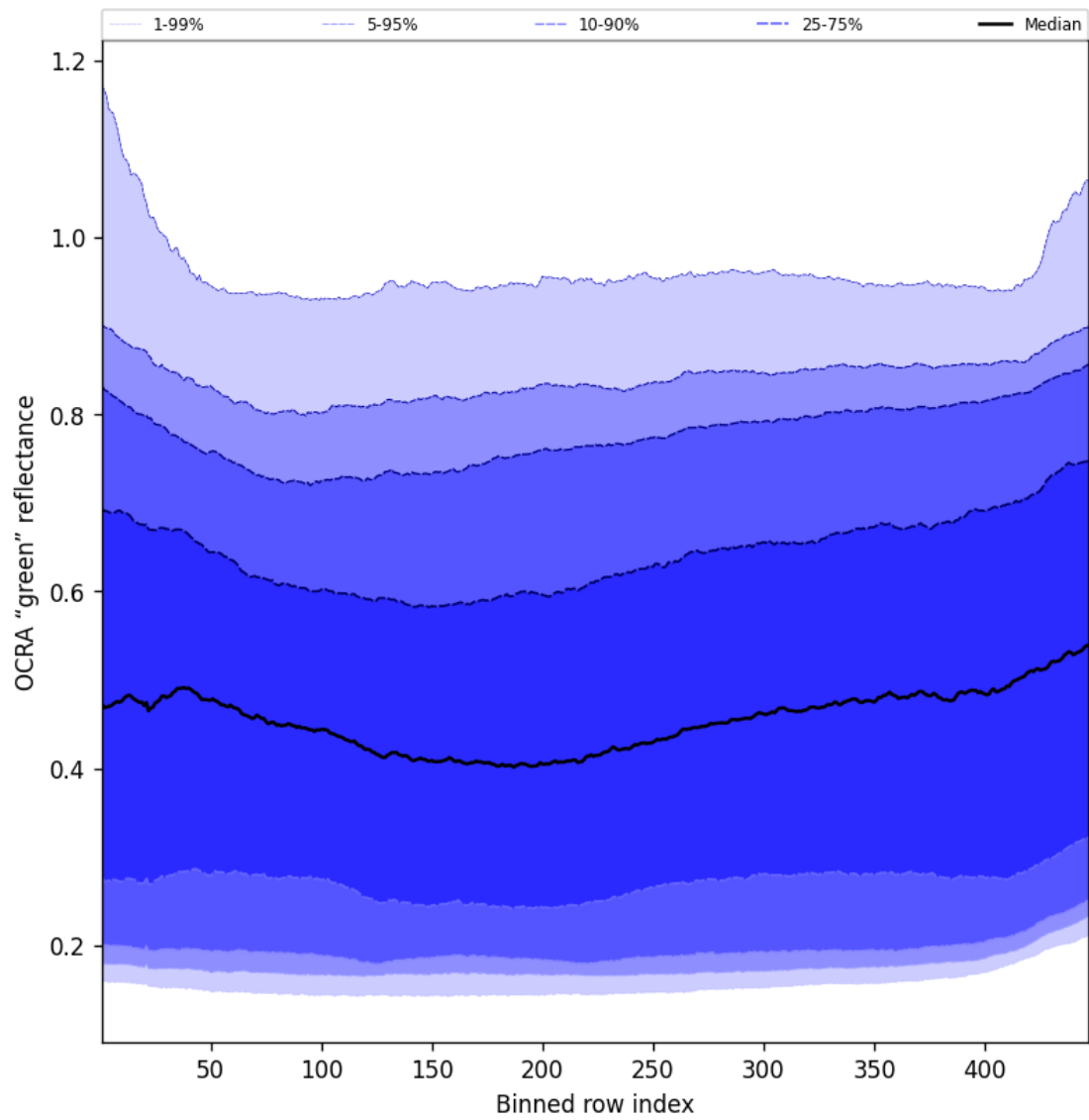
Figure 68: Along track statistics of “OCRA “green” reflectance” for 2025-06-23 to 2025-06-25
