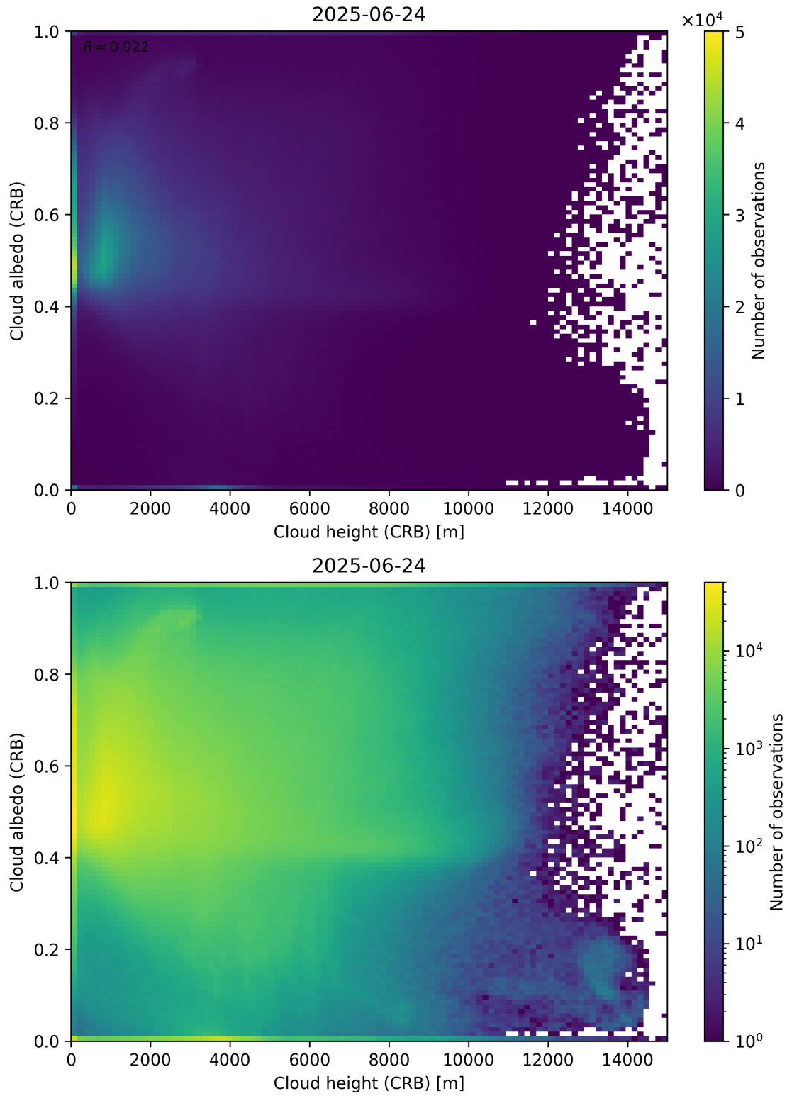
Figure 80: Scatter density plot of “Cloud height (CRB)” against “Cloud albedo (CRB)” for 2025-06-23 to 2025-06-25.
