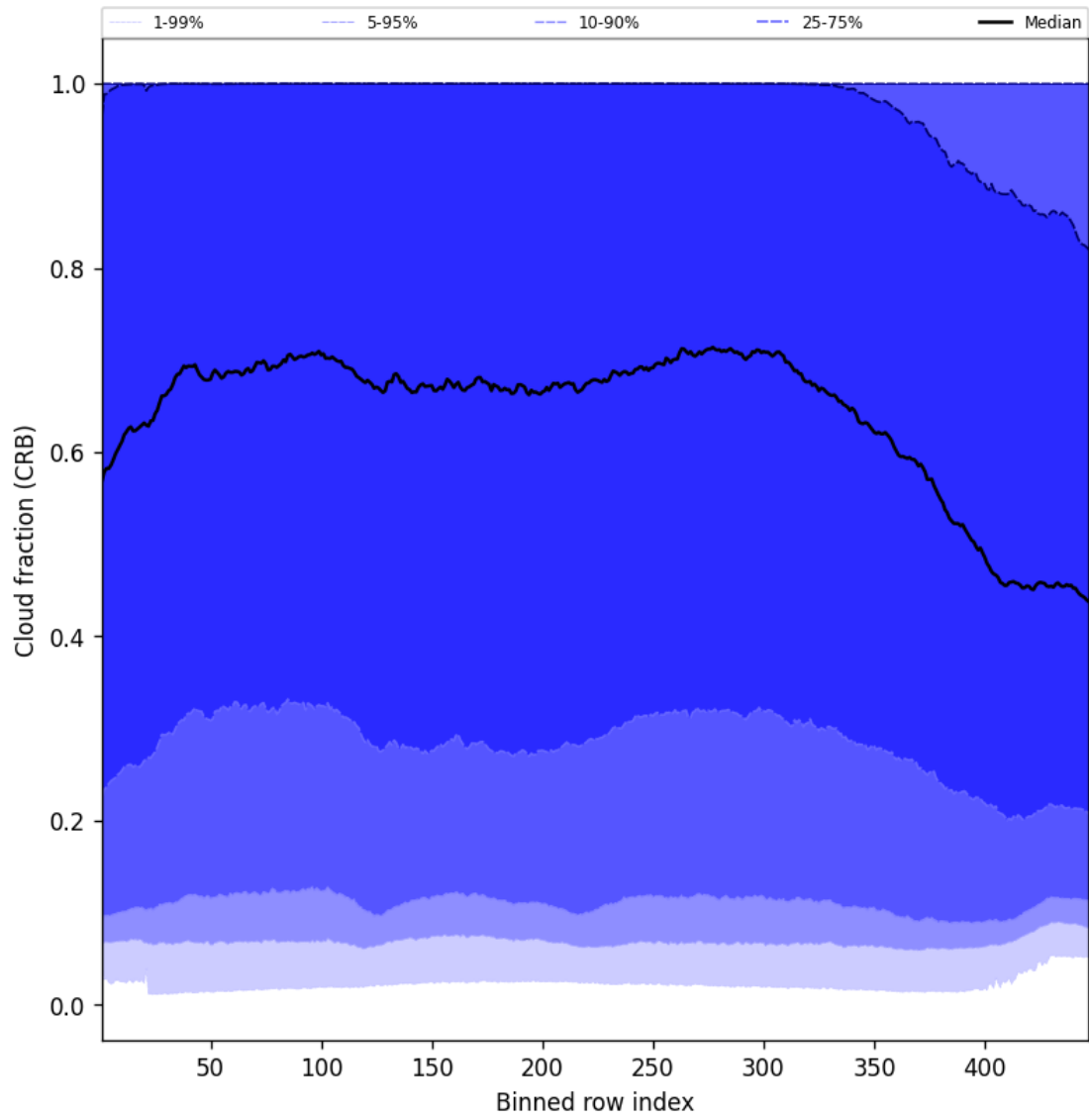
Figure 58: Along track statistics of “Cloud fraction (CRB)” for 2025-06-23 to 2025-06-25
