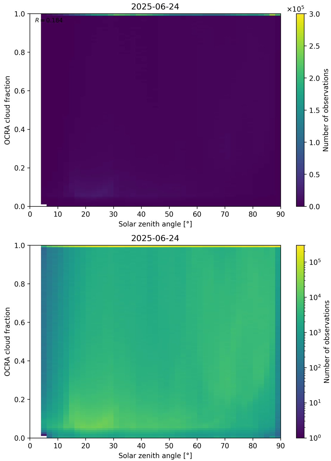
Figure 100: Scatter density plot of “Solar zenith angle” against “OCRA cloud fraction” for 2025-06-23 to 2025-06-25.
