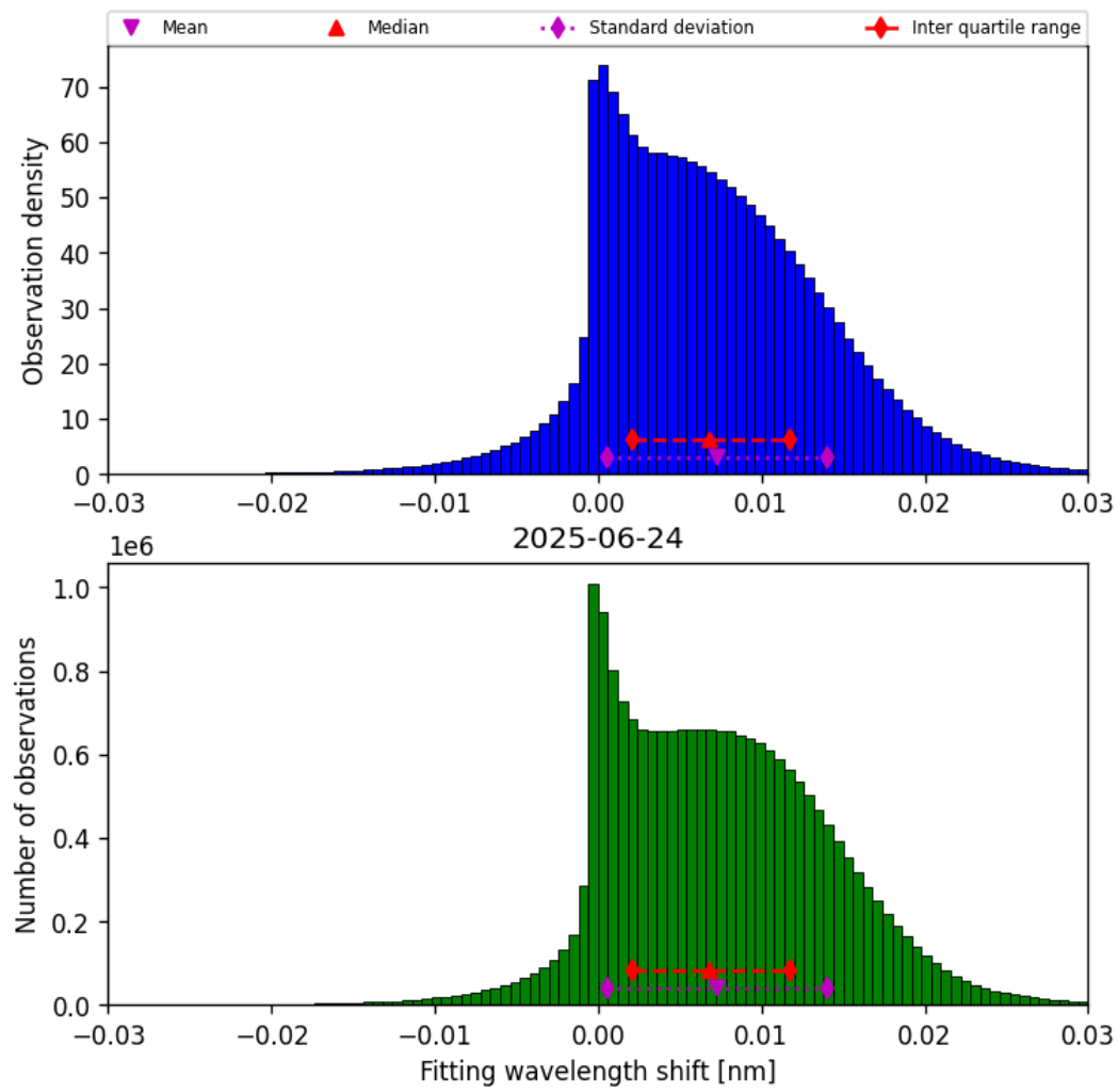
Figure 49: Histogram of “Fitting wavelength shift” for 2025-06-23 to 2025-06-25
