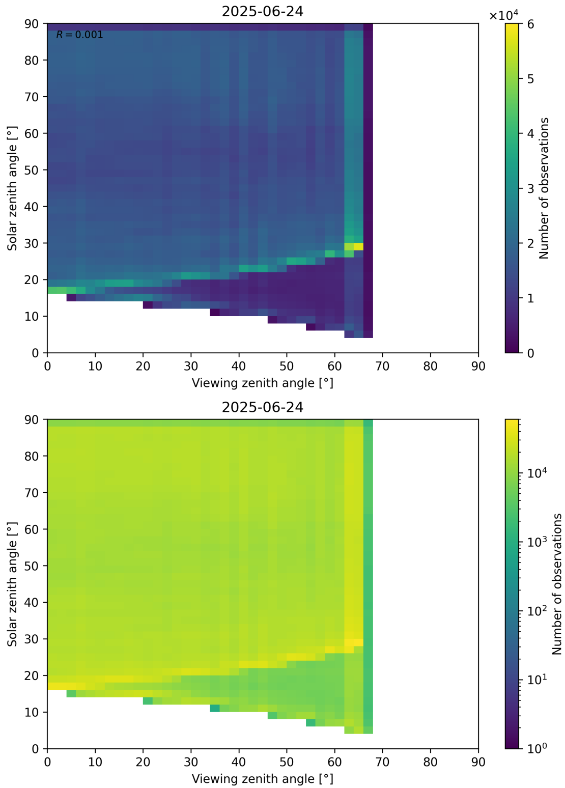
Figure 114: Scatter density plot of “Viewing zenith angle” against “Solar zenith angle” for 2025-06-23 to 2025-06-25.
