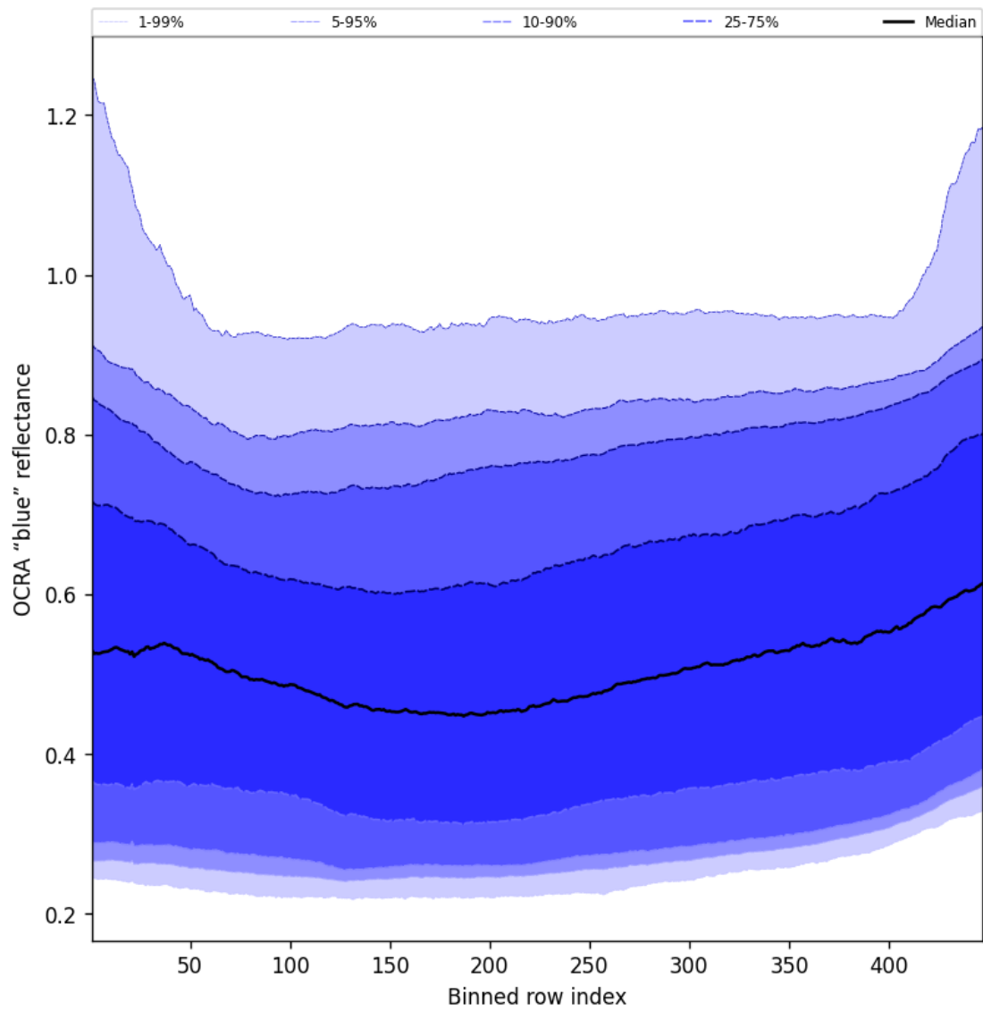
Figure 67: Along track statistics of “OCRA “blue” reflectance” for 2025-06-23 to 2025-06-25
