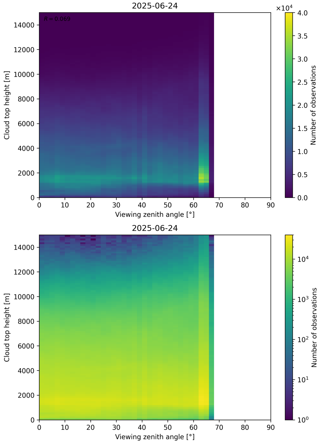
Figure 112: Scatter density plot of “Viewing zenith angle” against “Cloud top height” for 2025-06-23 to 2025-06-25.
