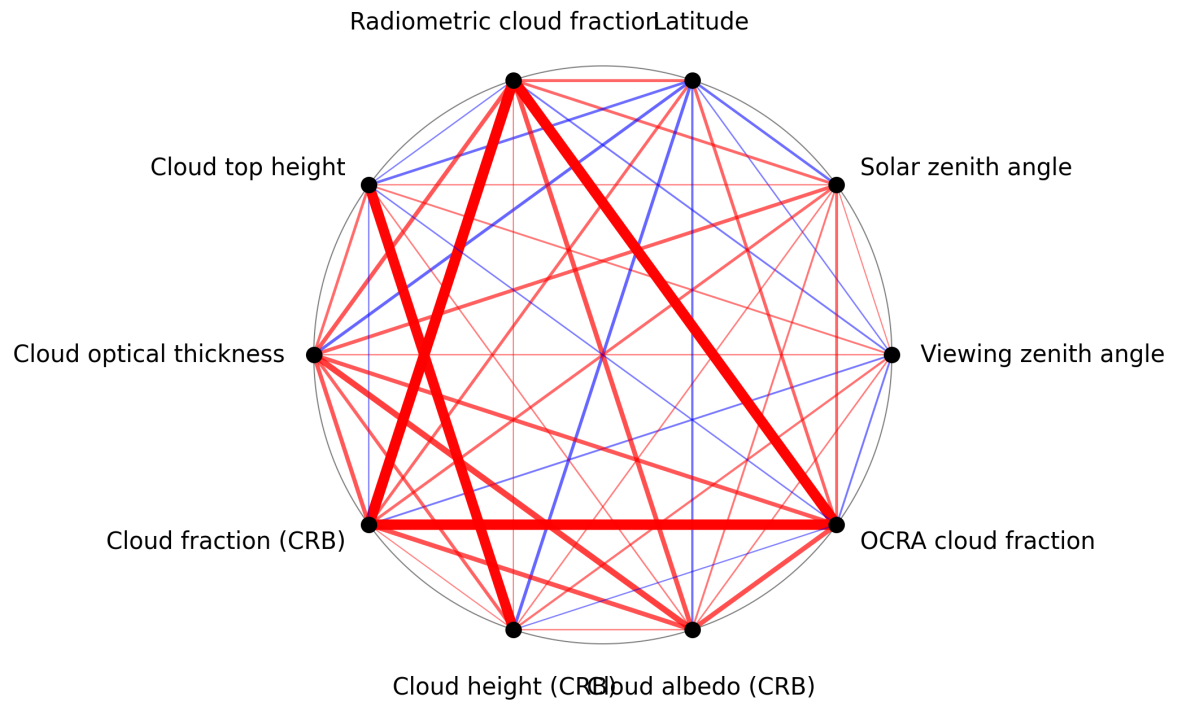
Figure 1: Map of correlation graph for 2025-06-23 to 2025-06-25.
