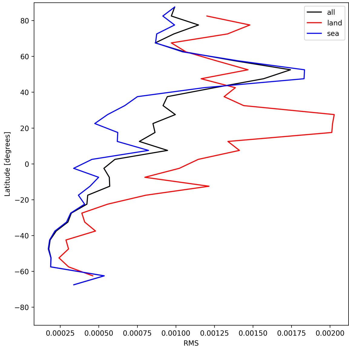
Figure 31: Zonal average of “RMS” for 2025-06-23 to 2025-06-25.
