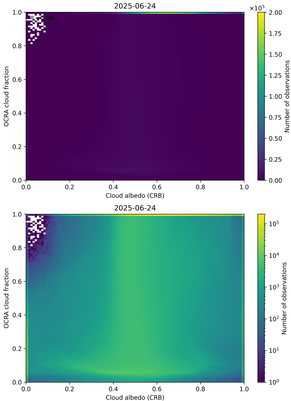
Figure 70: Scatter density plot of “Cloud albedo (CRB)” against “OCRA cloud fraction” for 2025-06-23 to 2025-06-25.
