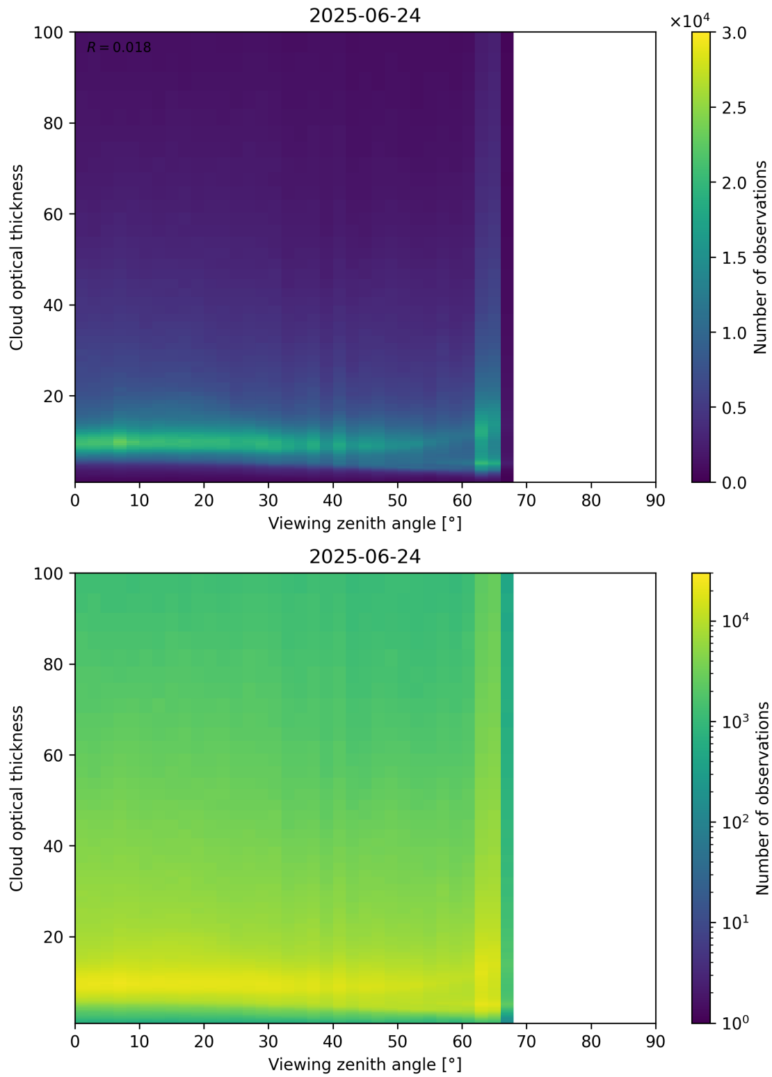
Figure 111: Scatter density plot of “Viewing zenith angle” against “Cloud optical thickness” for 2025-06-23 to 2025-06-25.
