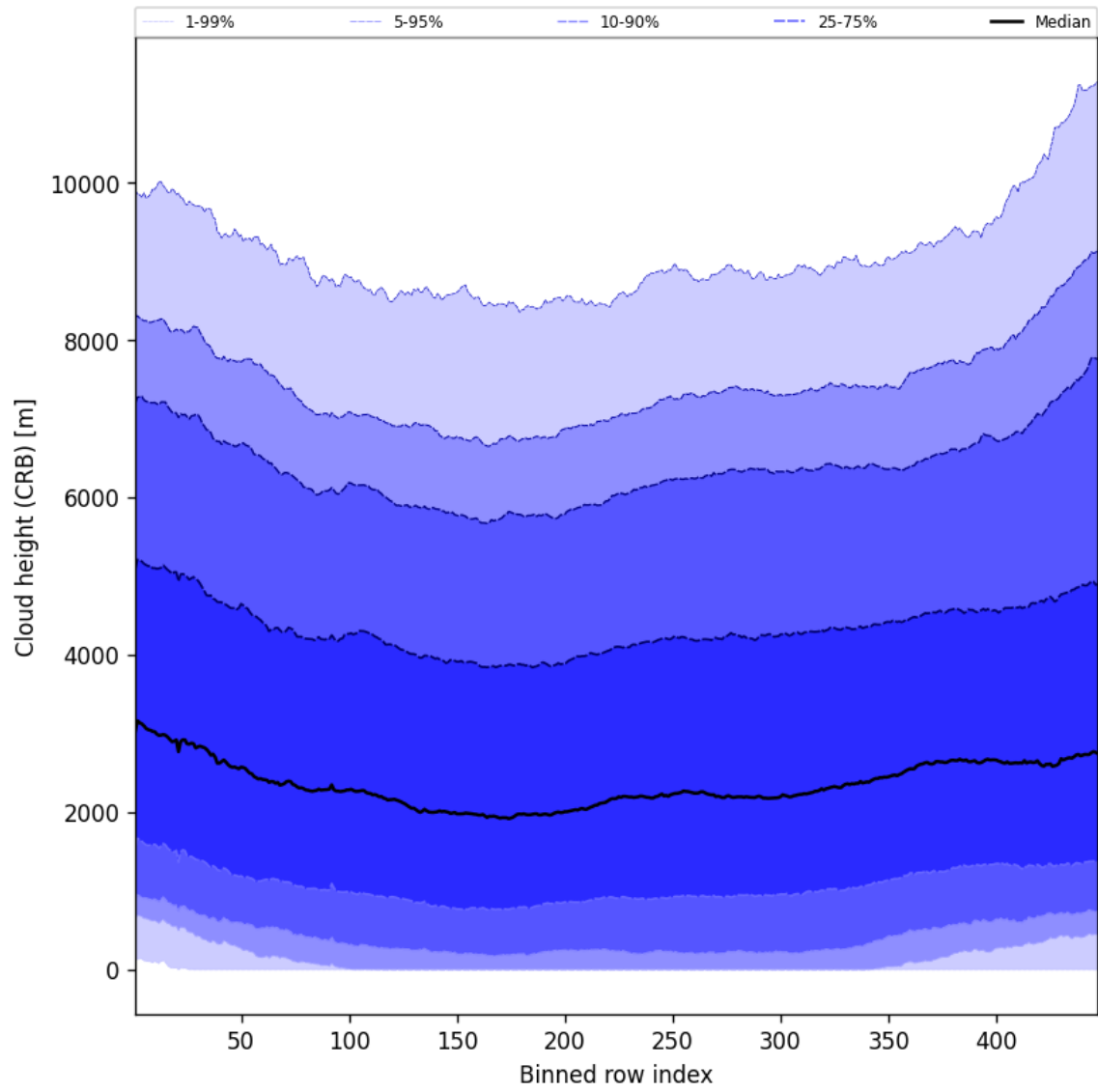
Figure 59: Along track statistics of “Cloud height (CRB)” for 2025-06-23 to 2025-06-25
