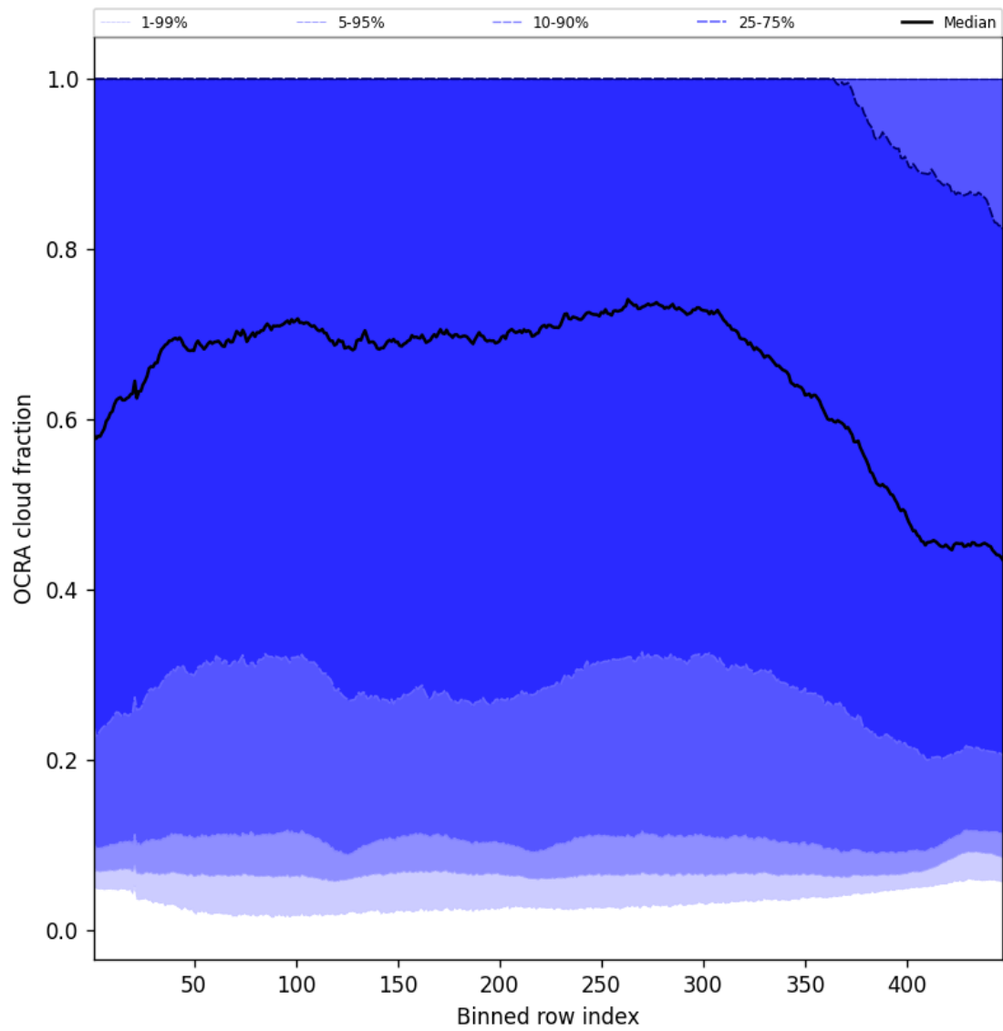
Figure 66: Along track statistics of “OCRA cloud fraction” for 2025-06-23 to 2025-06-25
