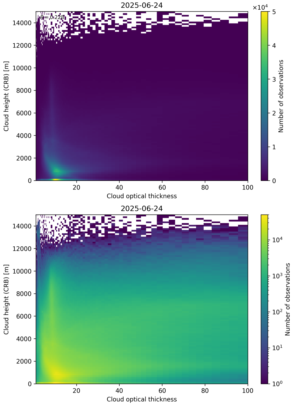
Figure 85: Scatter density plot of “Cloud optical thickness” against “Cloud height (CRB)” for 2025-06-23 to 2025-06-25.
