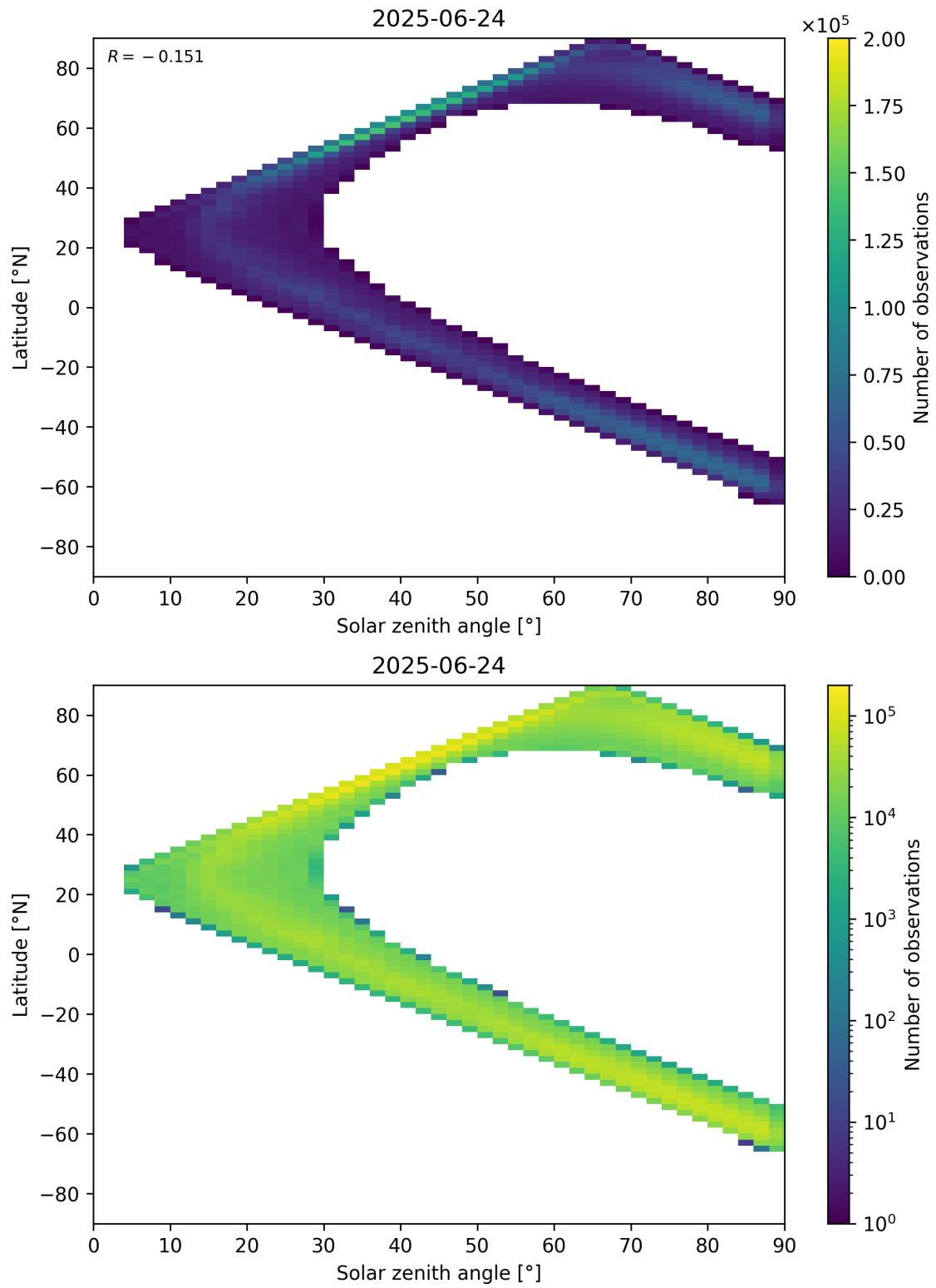
Figure 105: Scatter density plot of “Solar zenith angle” against “Latitude” for 2025-06-23 to 2025-06-25.
