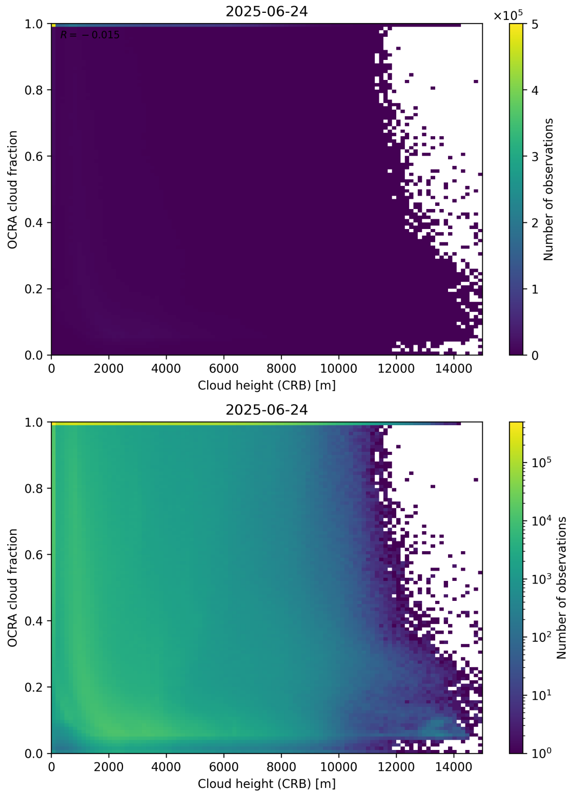
Figure 81: Scatter density plot of “Cloud height (CRB)” against “OCRA cloud fraction” for 2025-06-23 to 2025-06-25.
