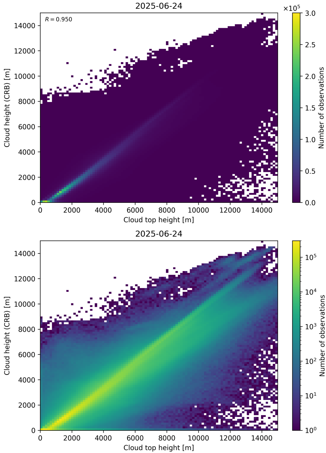
Figure 89: Scatter density plot of “Cloud top height” against “Cloud height (CRB)” for 2025-06-23 to 2025-06-25.
