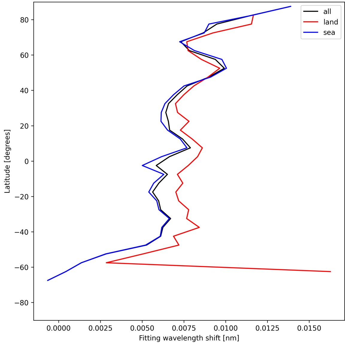
Figure 33: Zonal average of “Fitting wavelength shift” for 2025-06-23 to 2025-06-25.
