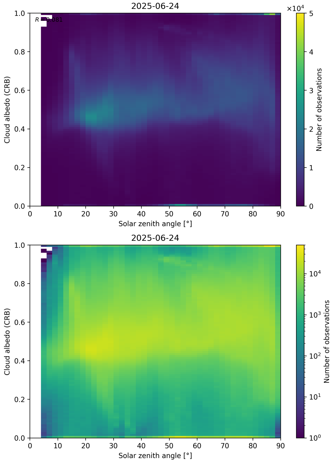
Figure 98: Scatter density plot of “Solar zenith angle” against “Cloud albedo (CRB)” for 2025-06-23 to 2025-06-25.
