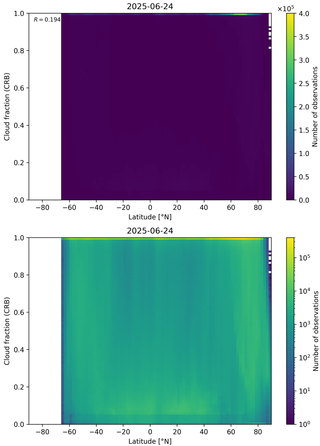
Figure 94: Scatter density plot of “Latitude” against “Cloud fraction (CRB)” for 2025-06-23 to 2025-06-25.
