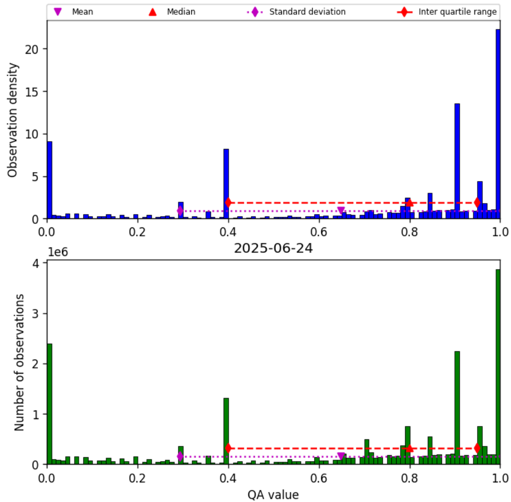
Figure 38: Histogram of “QA value” for 2025-06-23 to 2025-06-25
