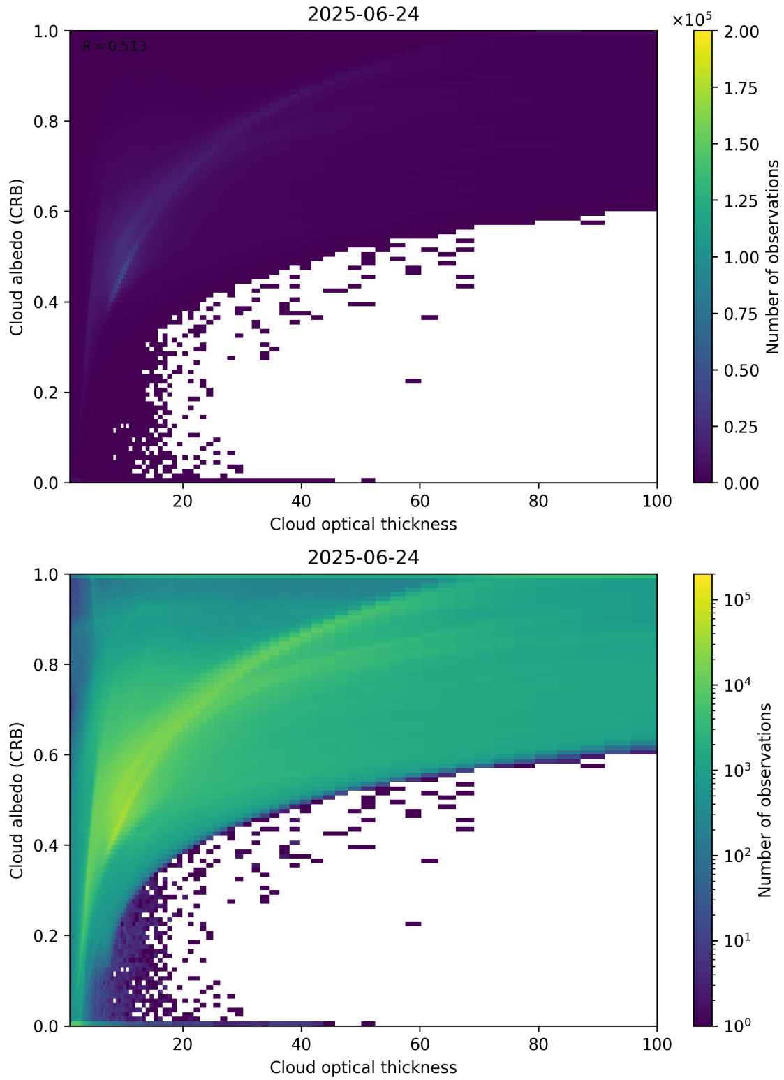
Figure 82: Scatter density plot of “Cloud optical thickness” against “Cloud albedo (CRB)” for 2025-06-23 to 2025-06-25.
