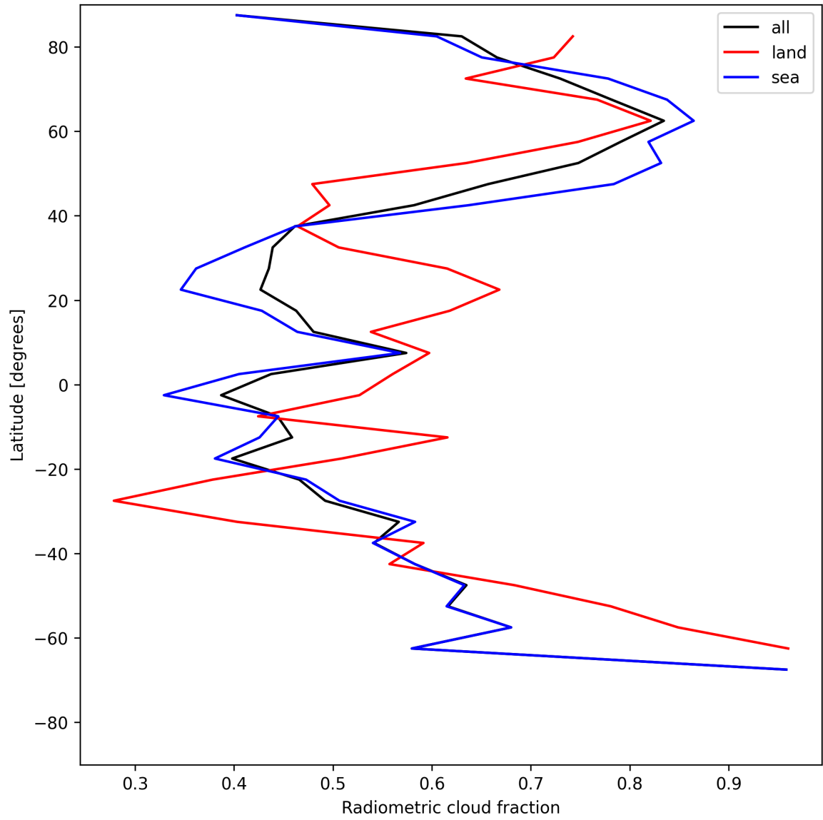
Figure 23: Zonal average of “Radiometric cloud fraction” for 2025-06-23 to 2025-06-25.
