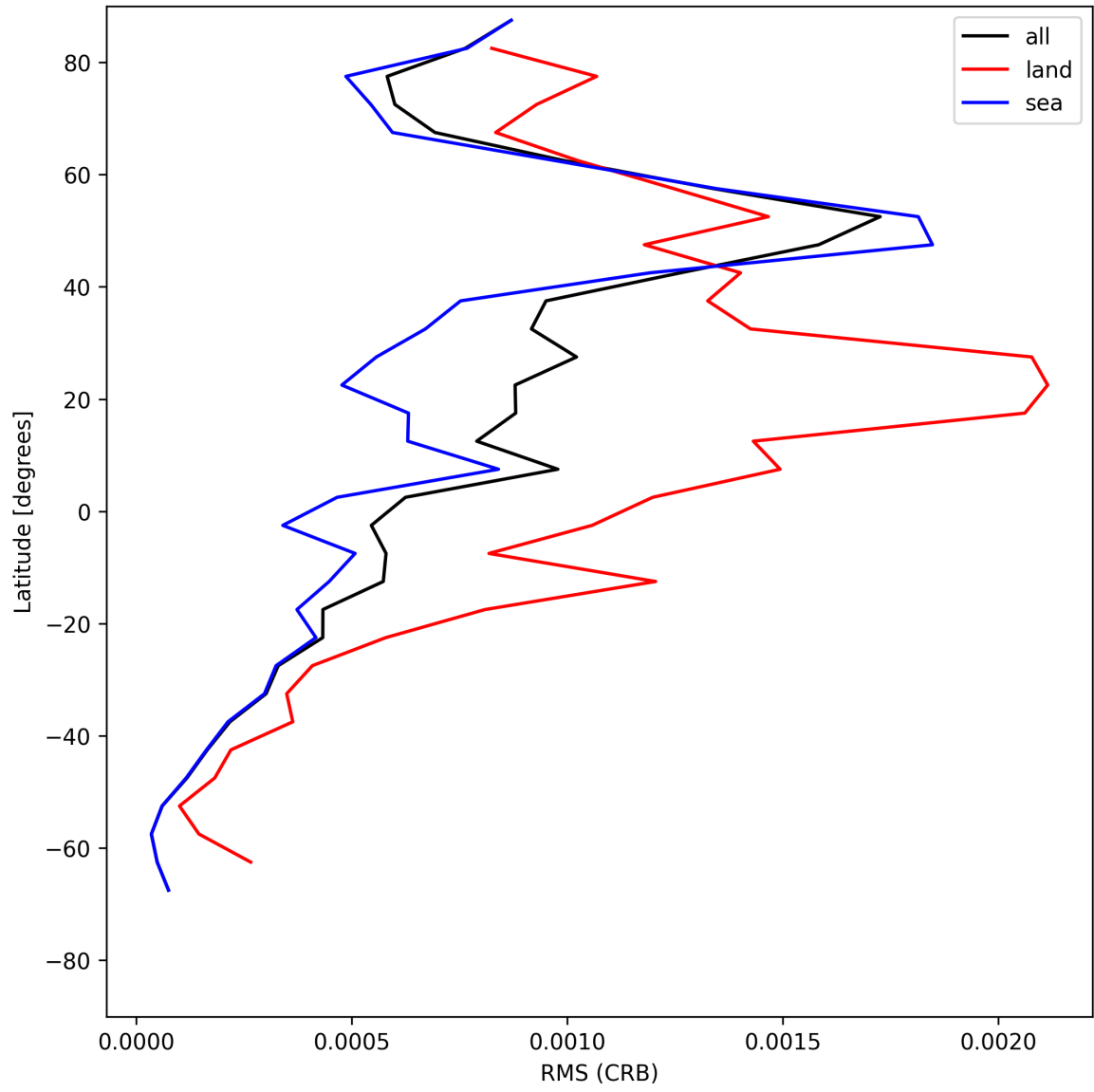
Figure 32: Zonal average of “RMS (CRB)” for 2025-06-23 to 2025-06-25.
