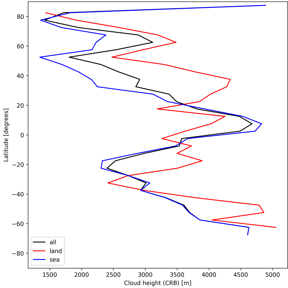
Figure 27: Zonal average of “Cloud height (CRB)” for 2025-06-23 to 2025-06-25.
