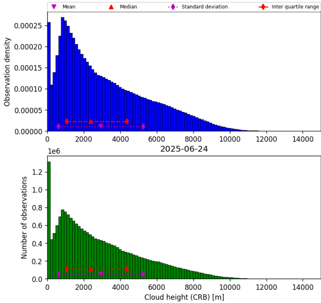
Figure 43: Histogram of “Cloud height (CRB)” for 2025-06-23 to 2025-06-25
