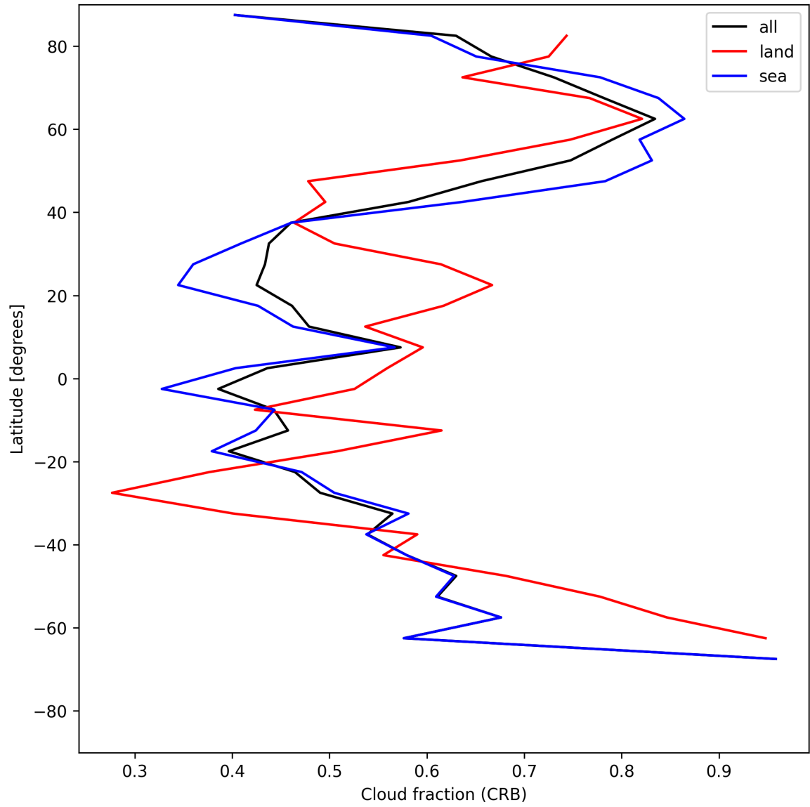
Figure 26: Zonal average of “Cloud fraction (CRB)” for 2025-06-23 to 2025-06-25.
