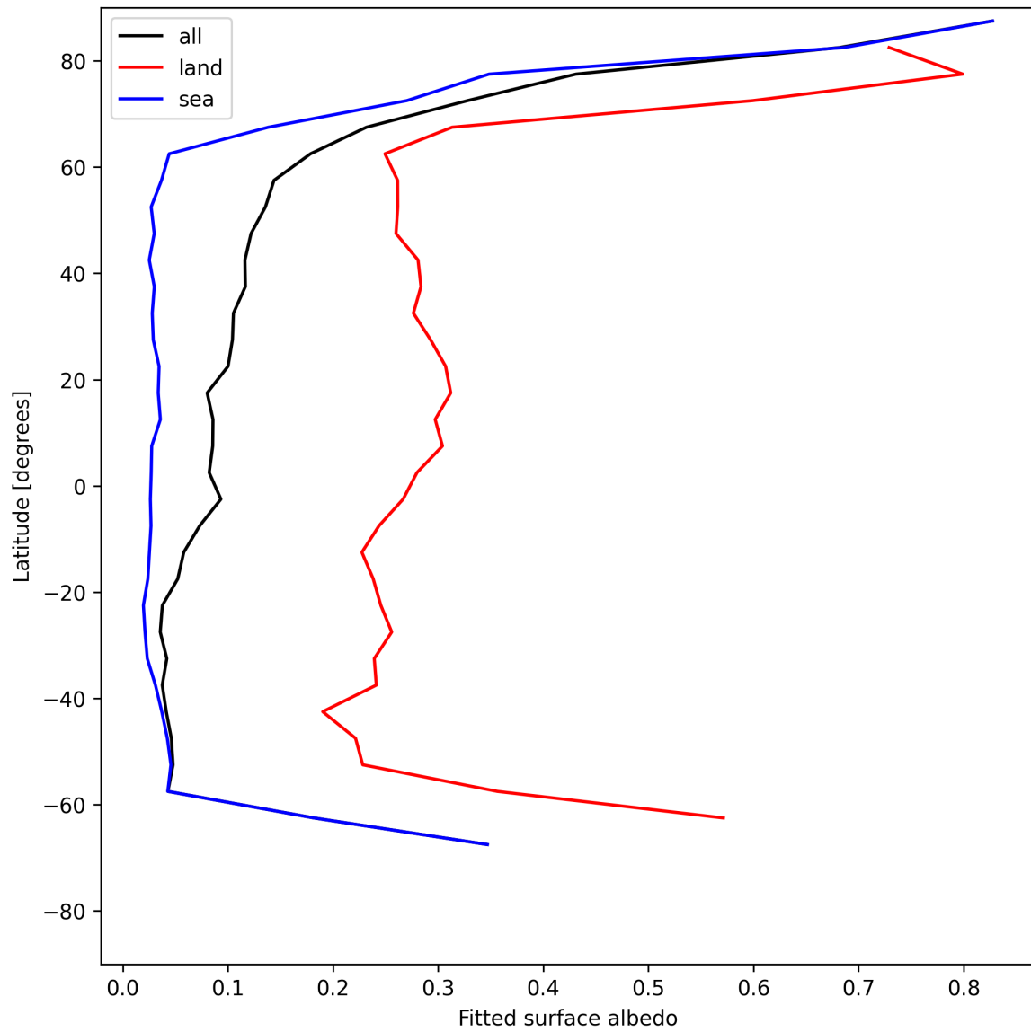
Figure 29: Zonal average of “Fitted surface albedo” for 2025-06-23 to 2025-06-25.
