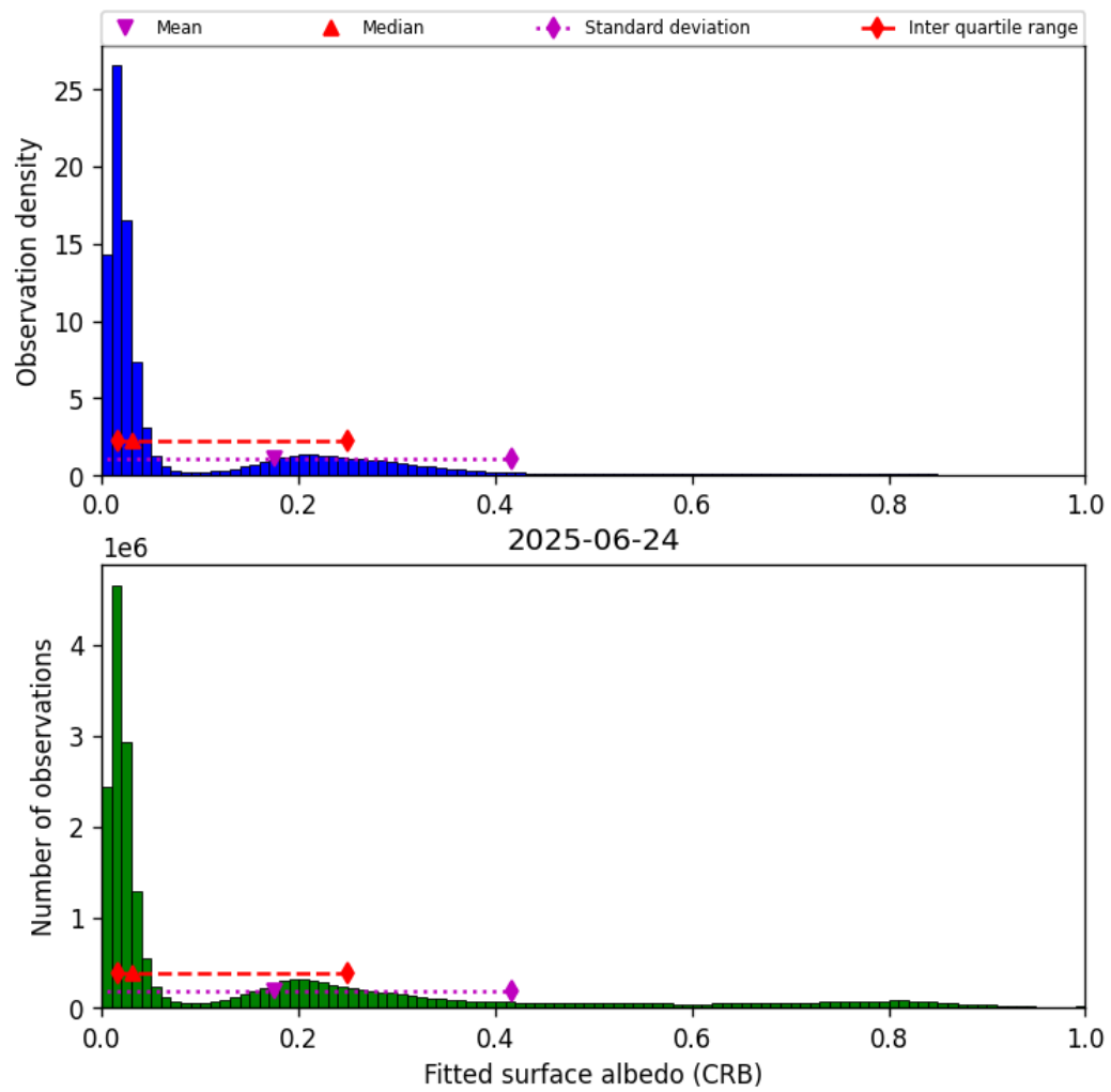
Figure 46: Histogram of “Fitted surface albedo (CRB)” for 2025-06-23 to 2025-06-25
