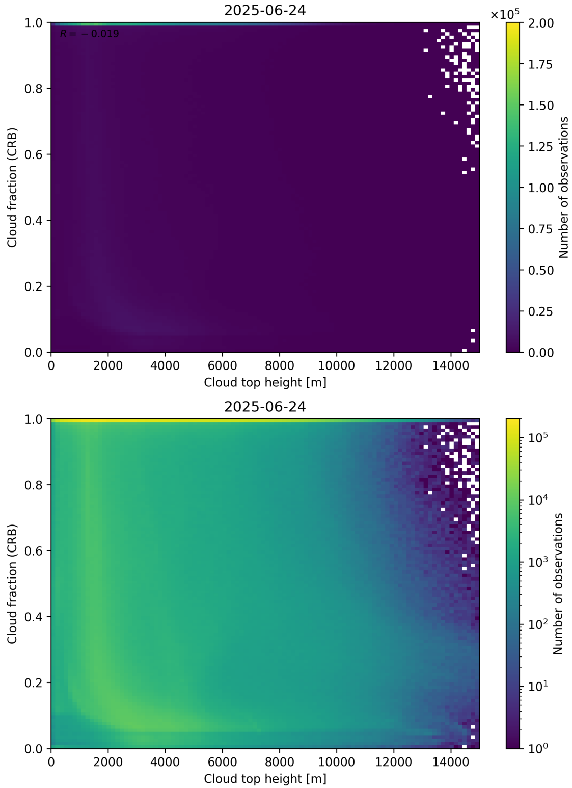
Figure 88: Scatter density plot of “Cloud top height” against “Cloud fraction (CRB)” for 2025-06-23 to 2025-06-25.
