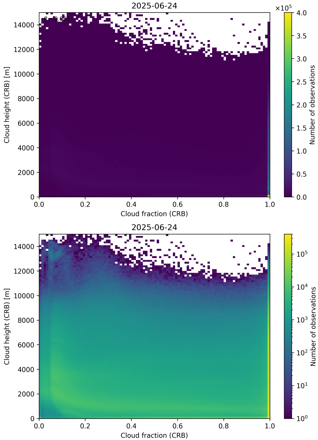
Figure 79: Scatter density plot of “Cloud fraction (CRB)” against “Cloud height (CRB)” for 2025-06-23 to 2025-06-25.
