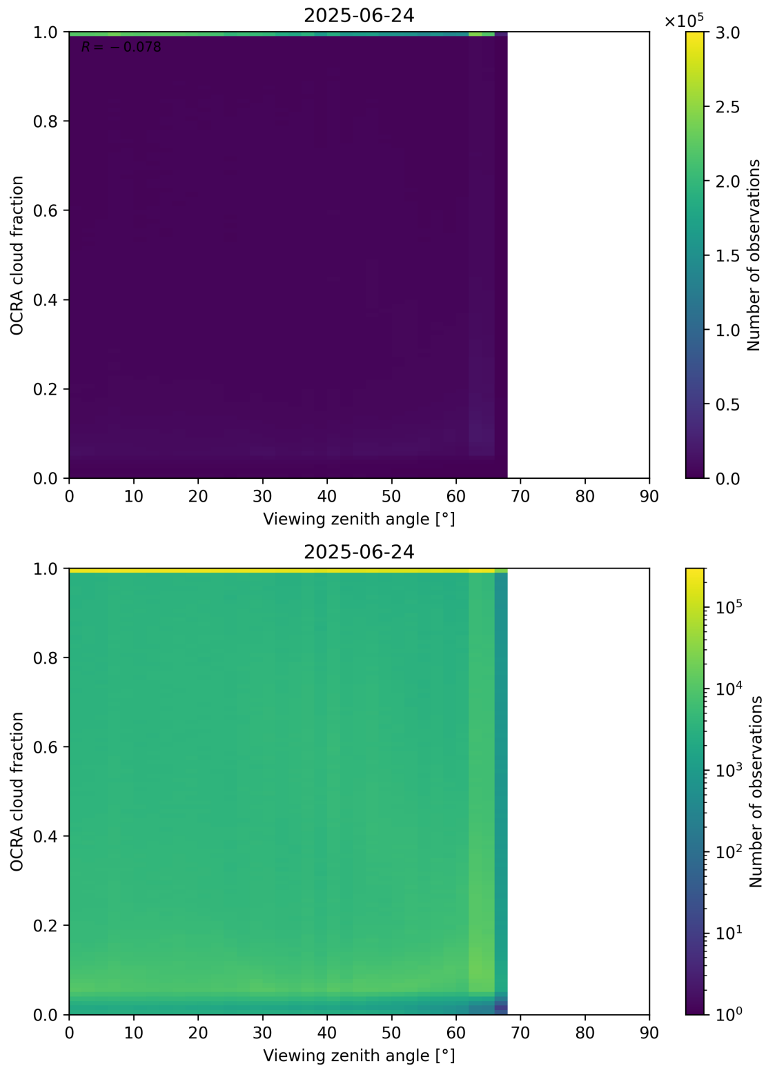
Figure 108: Scatter density plot of “Viewing zenith angle” against “OCRA cloud fraction” for 2025-06-23 to 2025-06-25.
