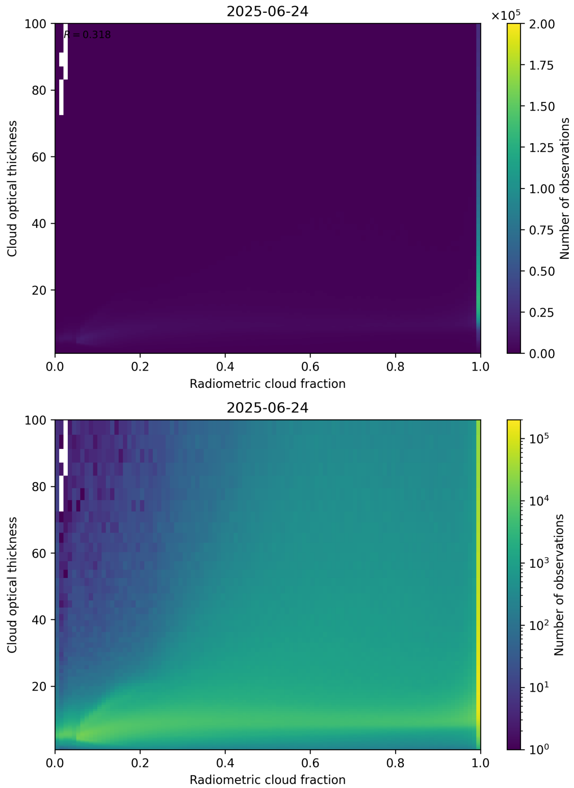
Figure 75: Scatter density plot of “Radiometric cloud fraction” against “Cloud optical thickness” for 2025-06-23 to 2025-06-25.
