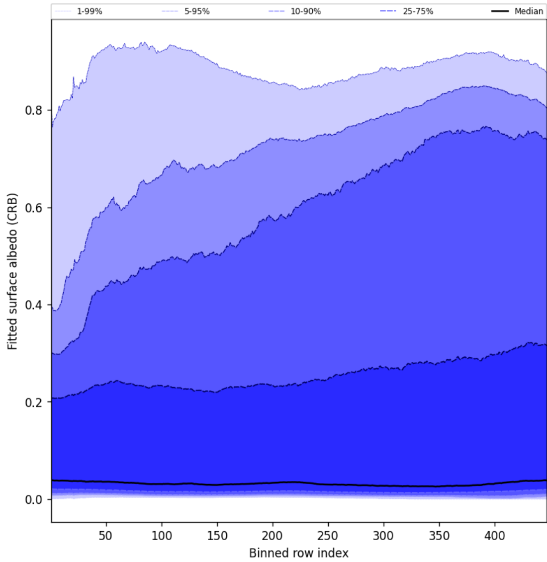
Figure 62: Along track statistics of “Fitted surface albedo (CRB)” for 2025-06-23 to 2025-06-25
