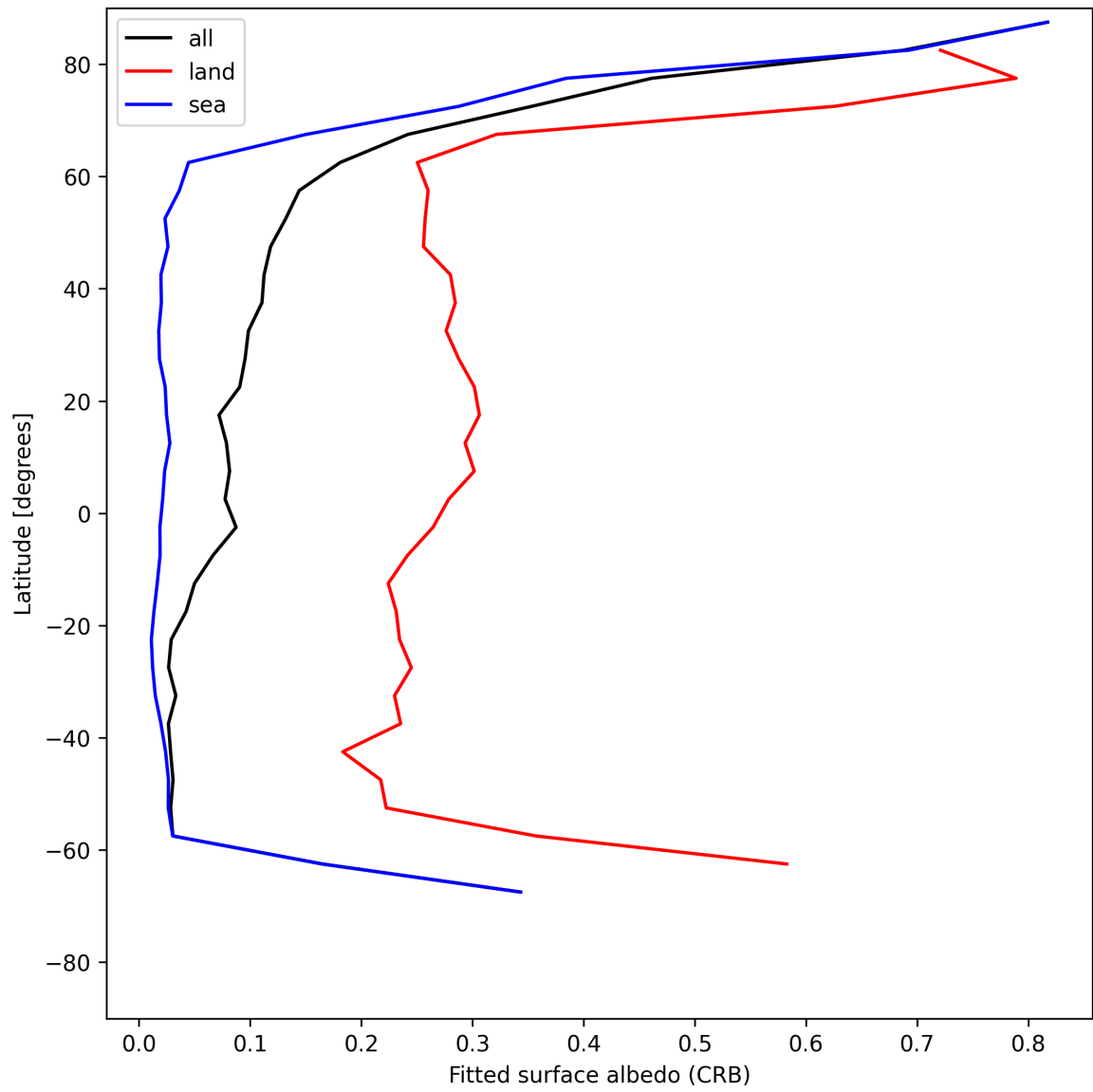
Figure 30: Zonal average of “Fitted surface albedo (CRB)” for 2025-06-23 to 2025-06-25.
