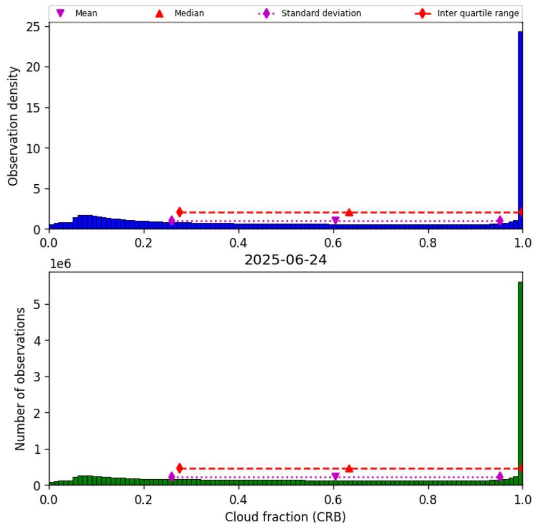
Figure 42: Histogram of “Cloud fraction (CRB)” for 2025-06-23 to 2025-06-25
