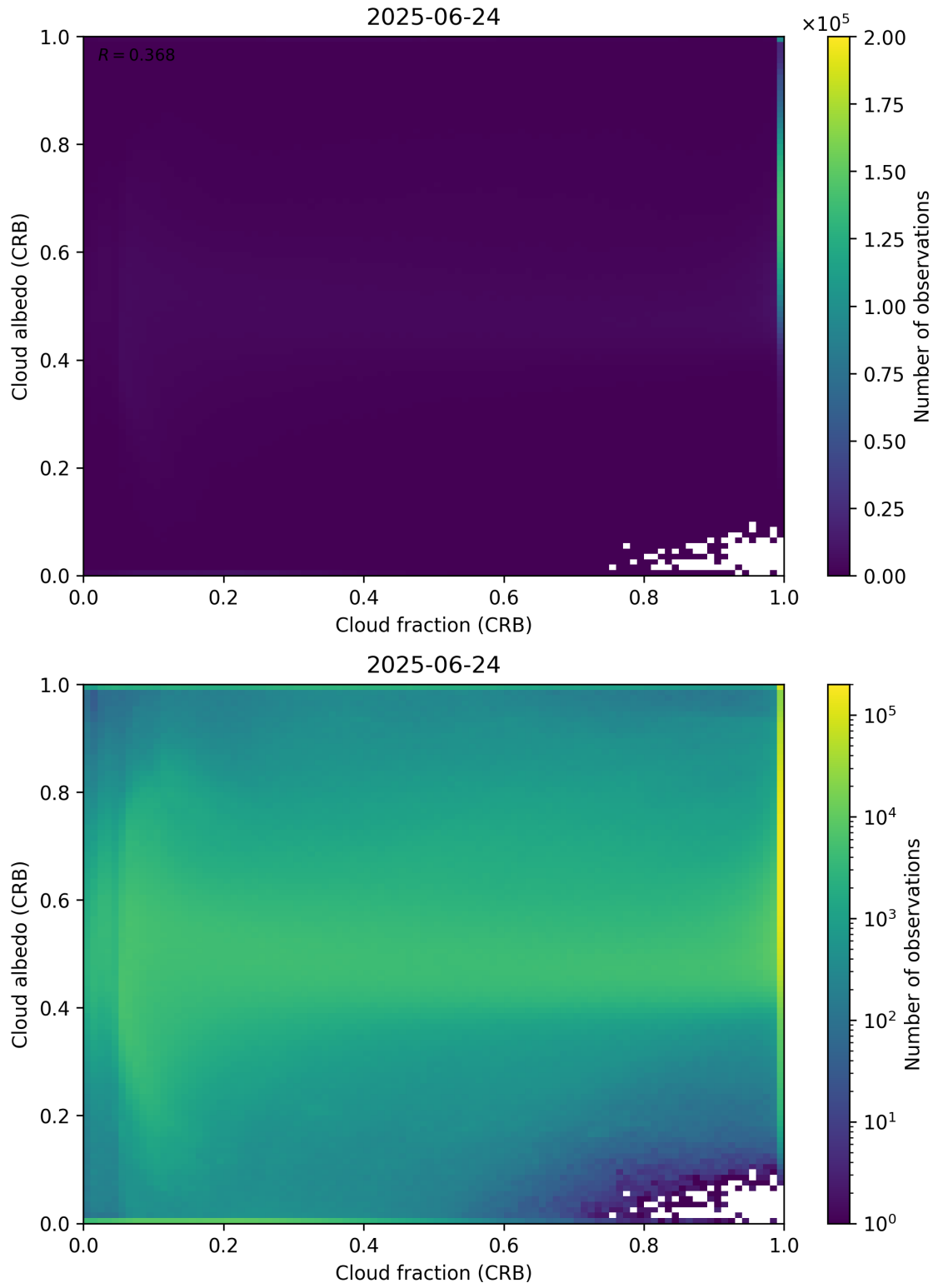
Figure 77: Scatter density plot of “Cloud fraction (CRB)” against “Cloud albedo (CRB)” for 2025-06-23 to 2025-06-25.
