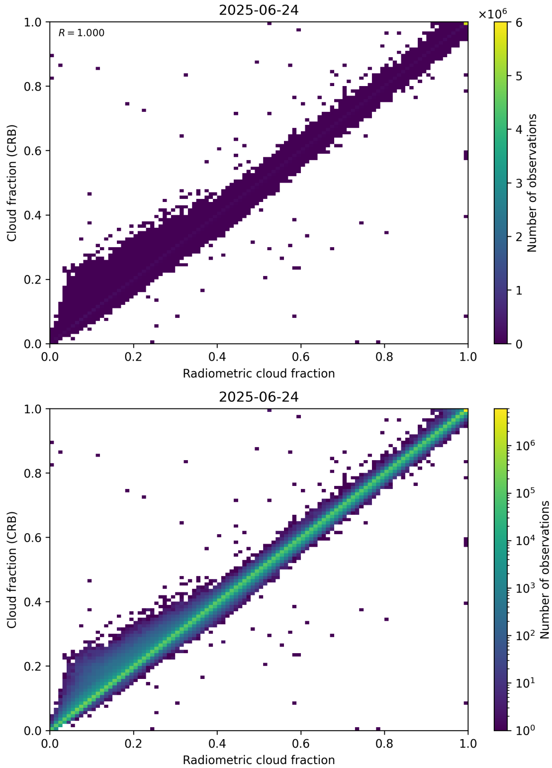
Figure 73: Scatter density plot of “Radiometric cloud fraction” against “Cloud fraction (CRB)” for 2025-06-23 to 2025-06-25.
