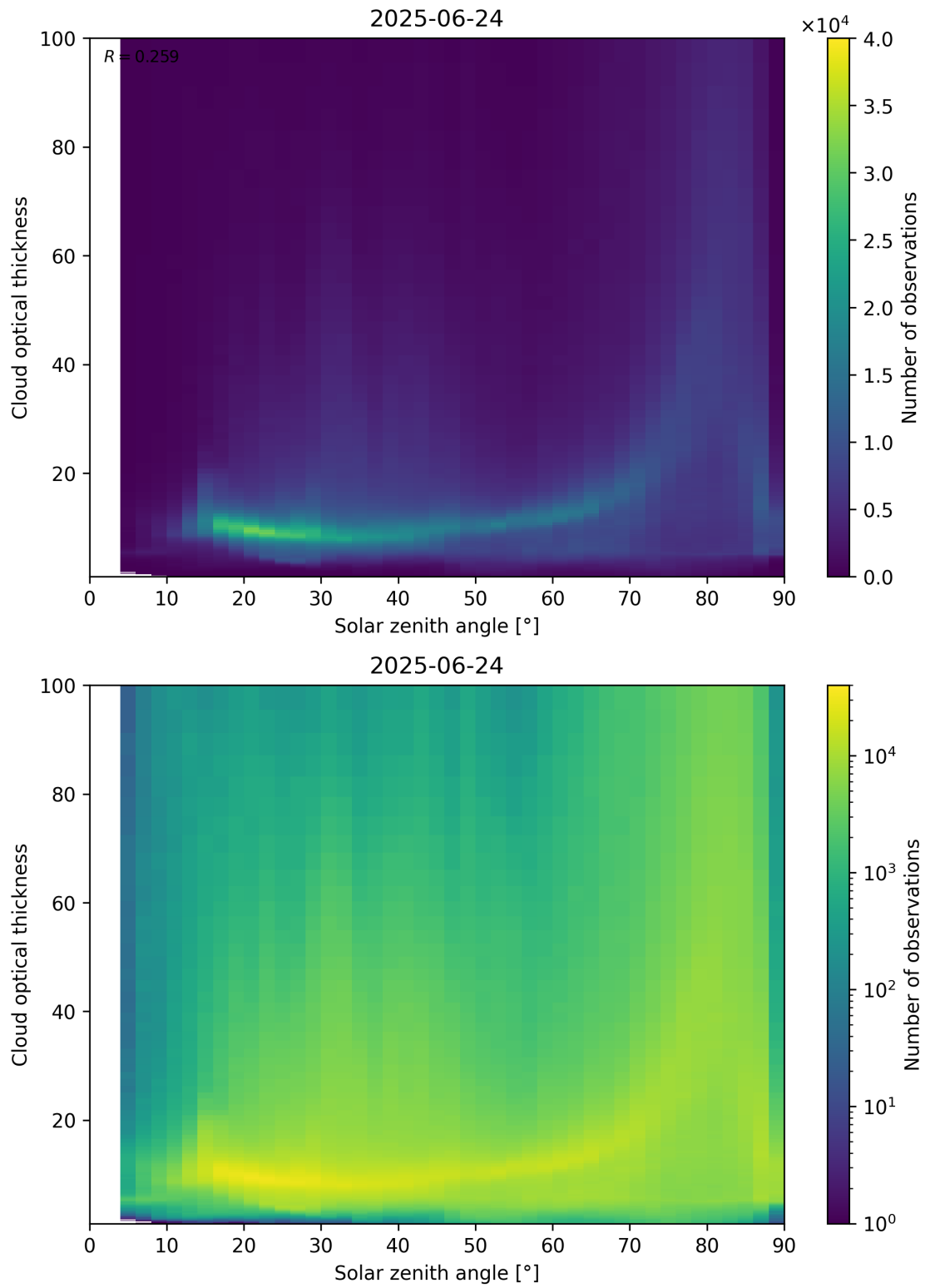
Figure 103: Scatter density plot of “Solar zenith angle” against “Cloud optical thickness” for 2025-06-23 to 2025-06-25.
