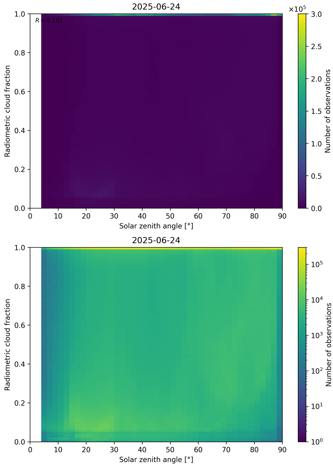
Figure 99: Scatter density plot of “Solar zenith angle” against “Radiometric cloud fraction” for 2025-06-23 to 2025-06-25.
