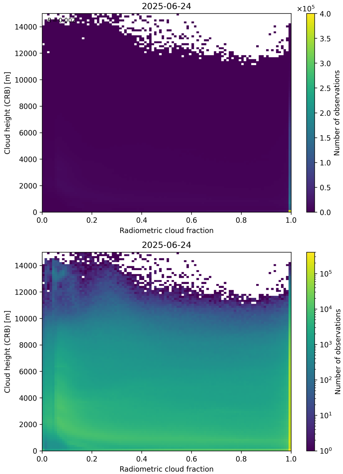
Figure 74: Scatter density plot of “Radiometric cloud fraction” against “Cloud height (CRB)” for 2025-06-23 to 2025-06-25.
