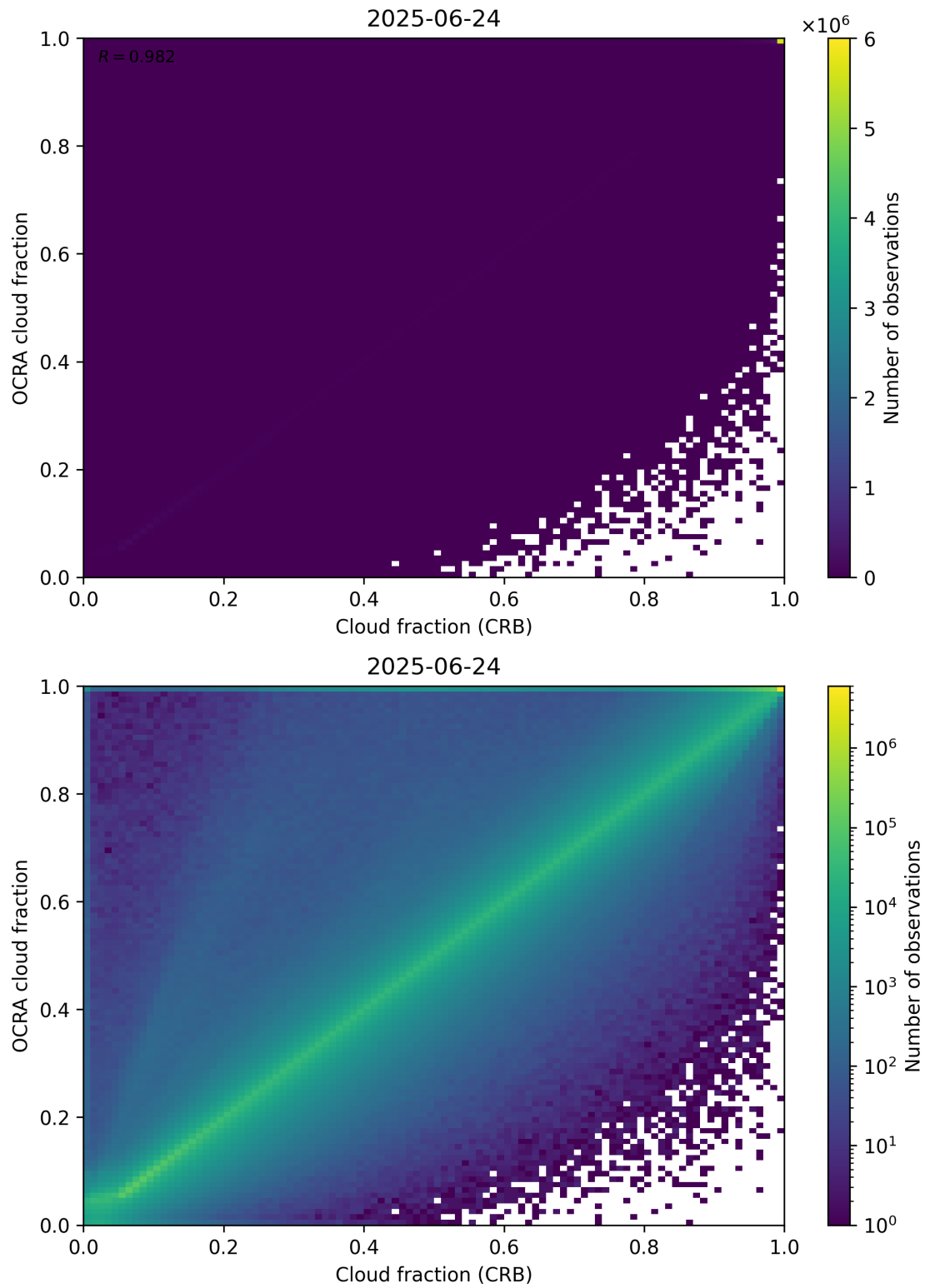
Figure 78: Scatter density plot of “Cloud fraction (CRB)” against “OCRA cloud fraction” for 2025-06-23 to 2025-06-25.
