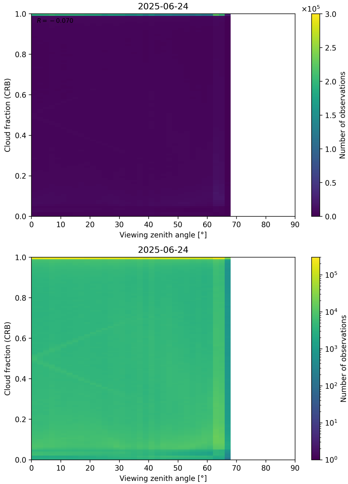
Figure 109: Scatter density plot of “Viewing zenith angle” against “Cloud fraction (CRB)” for 2025-06-23 to 2025-06-25.
