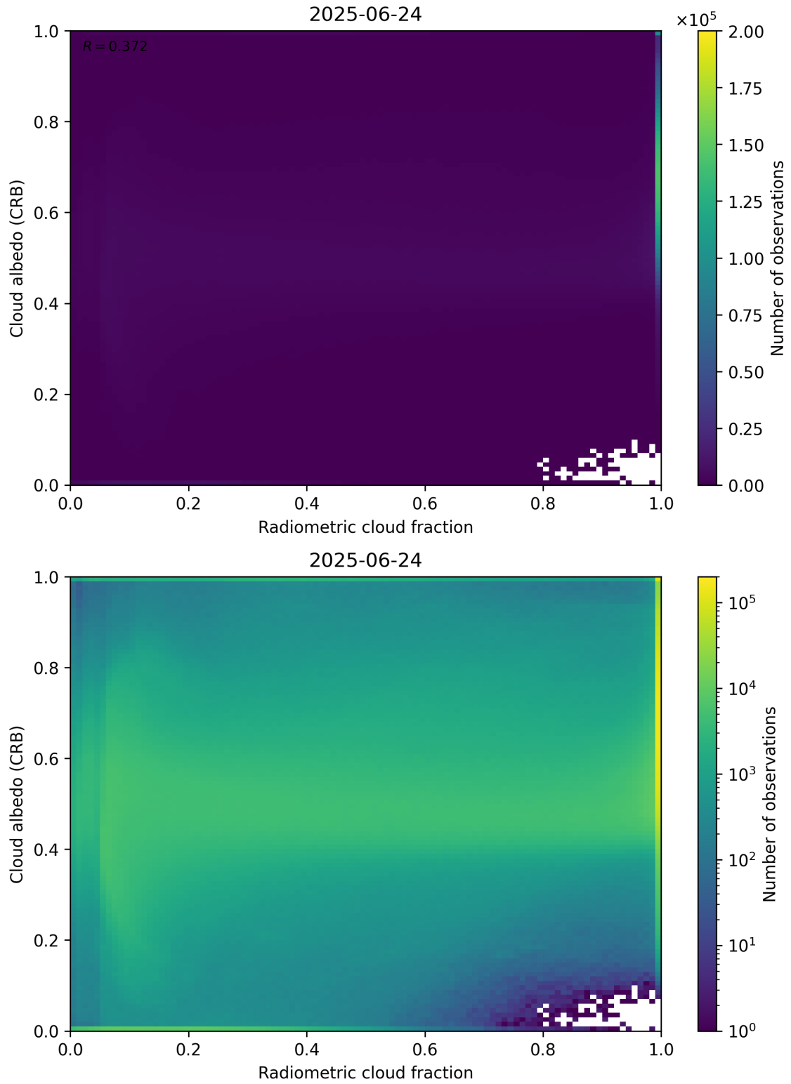
Figure 71: Scatter density plot of “Radiometric cloud fraction” against “Cloud albedo (CRB)” for 2025-06-23 to 2025-06-25.
