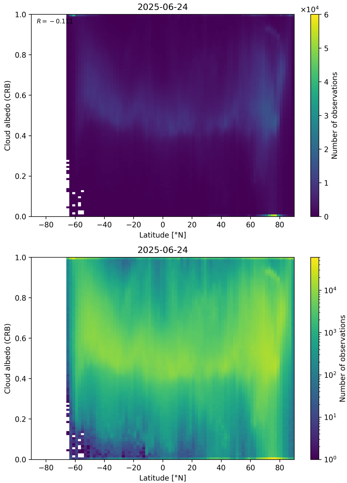
Figure 91: Scatter density plot of “Latitude” against “Cloud albedo (CRB)” for 2025-06-23 to 2025-06-25.
