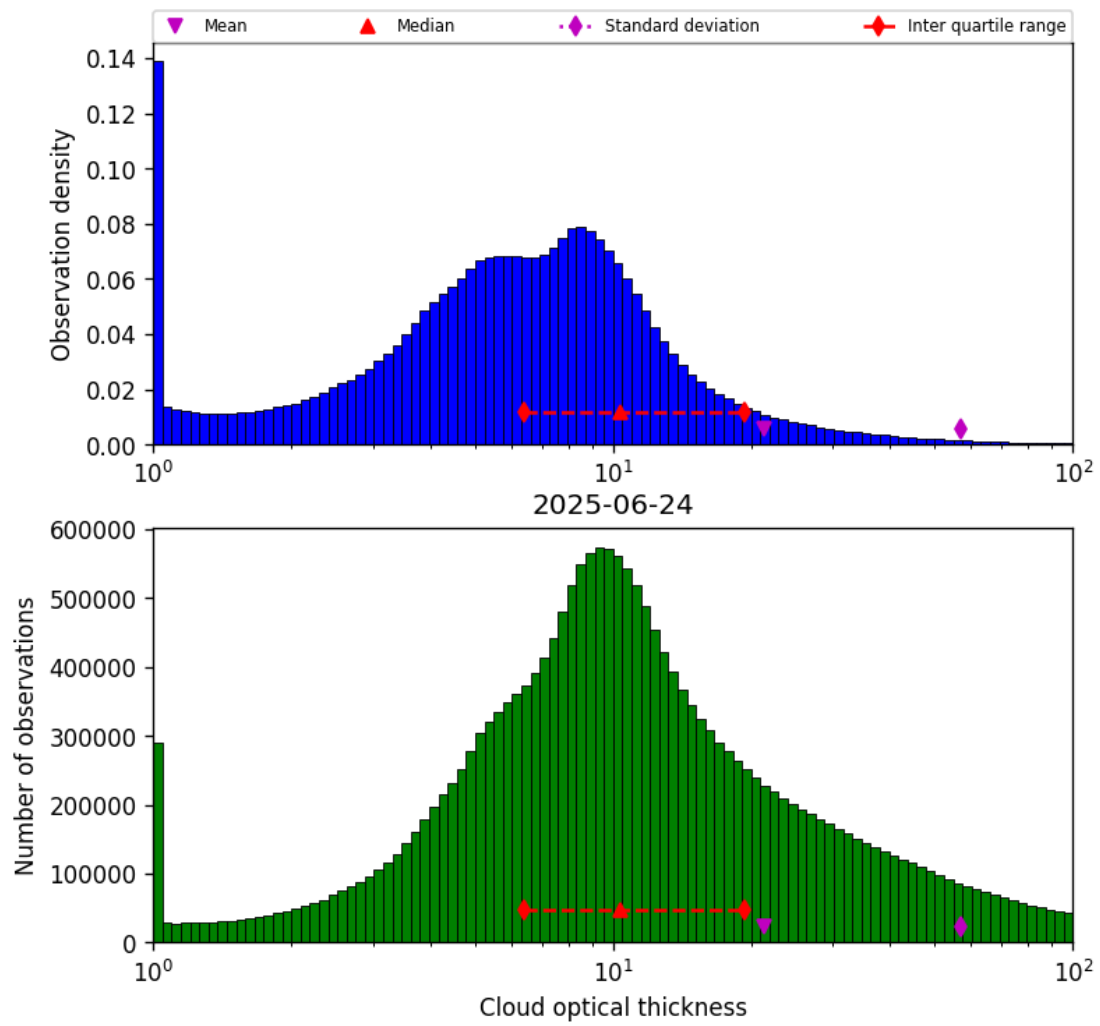
Figure 41: Histogram of “Cloud optical thickness” for 2025-06-23 to 2025-06-25
