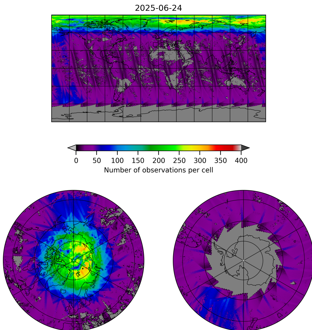
Figure 21: Map of the number of observations for 2025-06-23 to 2025-06-25
