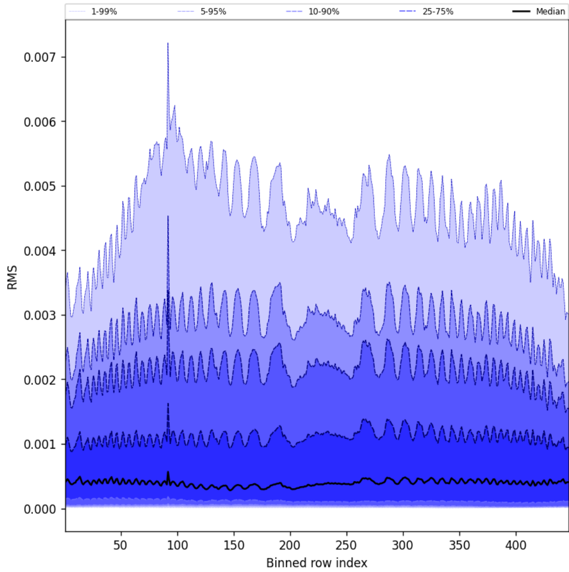
Figure 63: Along track statistics of “RMS” for 2025-06-23 to 2025-06-25
