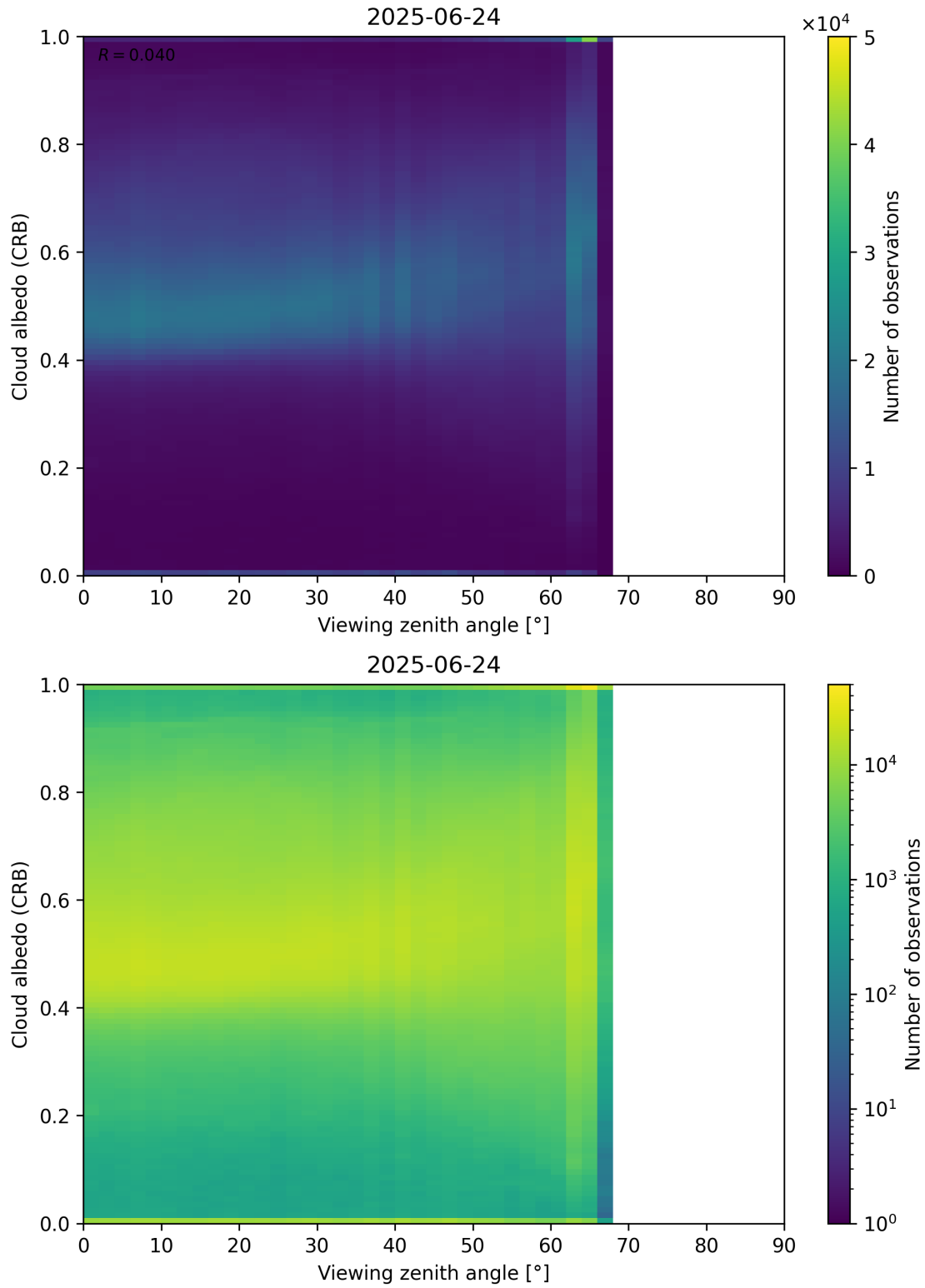
Figure 106: Scatter density plot of “Viewing zenith angle” against “Cloud albedo (CRB)” for 2025-06-23 to 2025-06-25.
