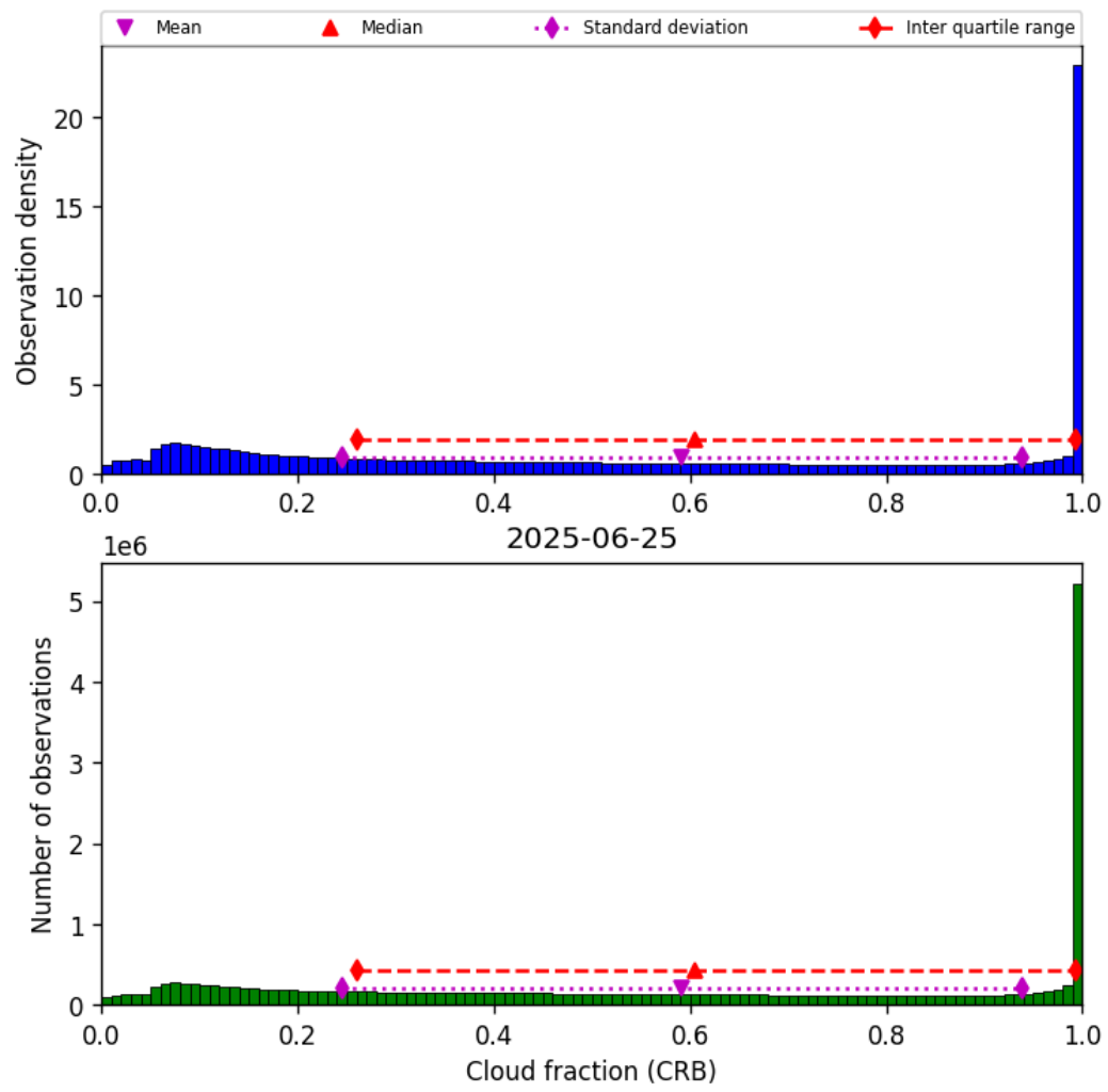
Figure 42: Histogram of “Cloud fraction (CRB)” for 2025-06-24 to 2025-06-26
