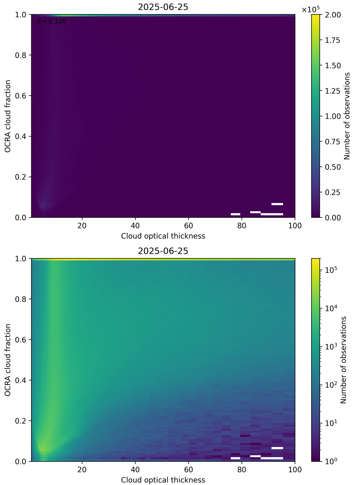
Figure 83: Scatter density plot of “Cloud optical thickness” against “OCRA cloud fraction” for 2025-06-24 to 2025-06-26.
