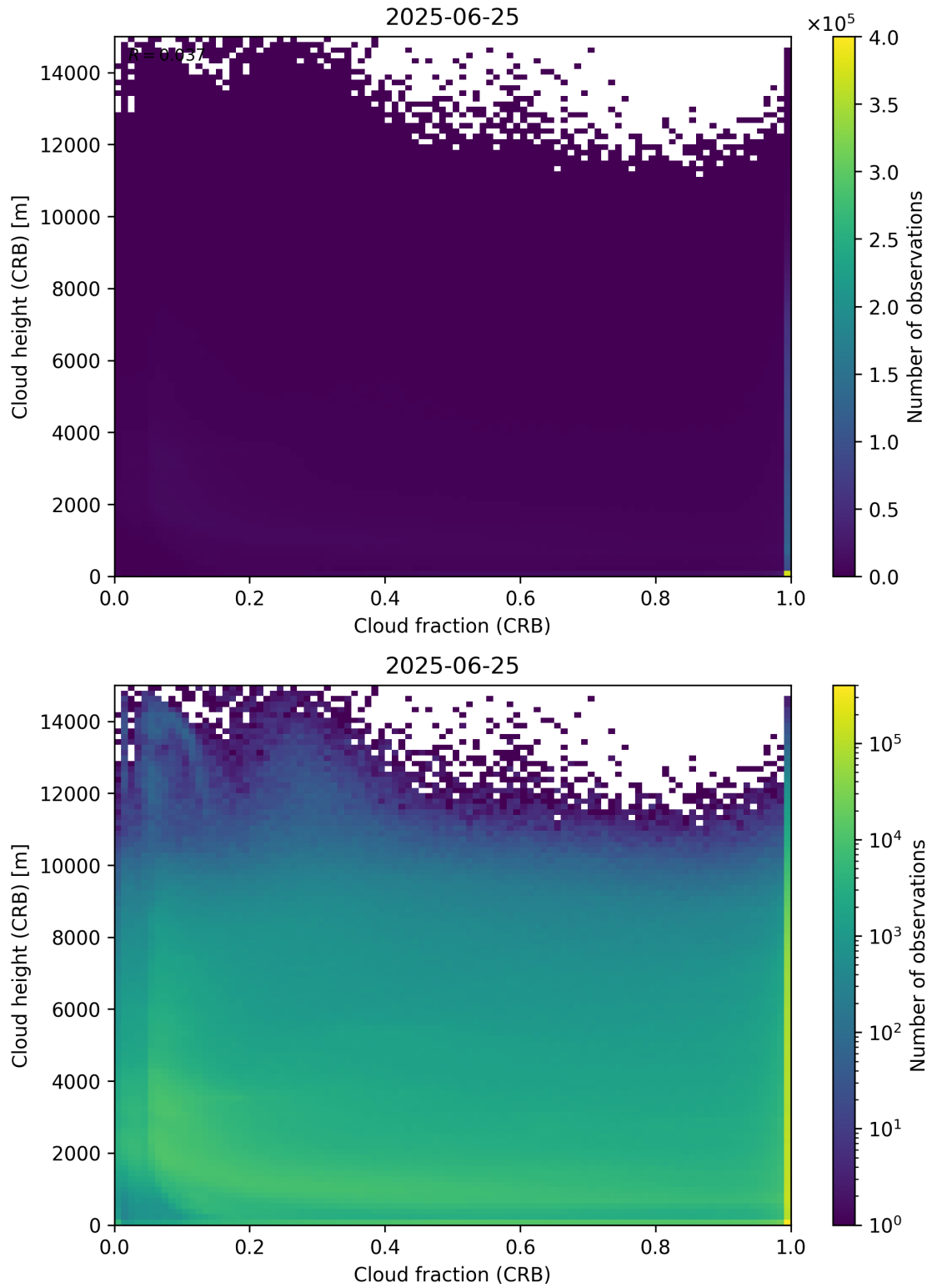
Figure 79: Scatter density plot of “Cloud fraction (CRB)” against “Cloud height (CRB)” for 2025-06-24 to 2025-06-26.
