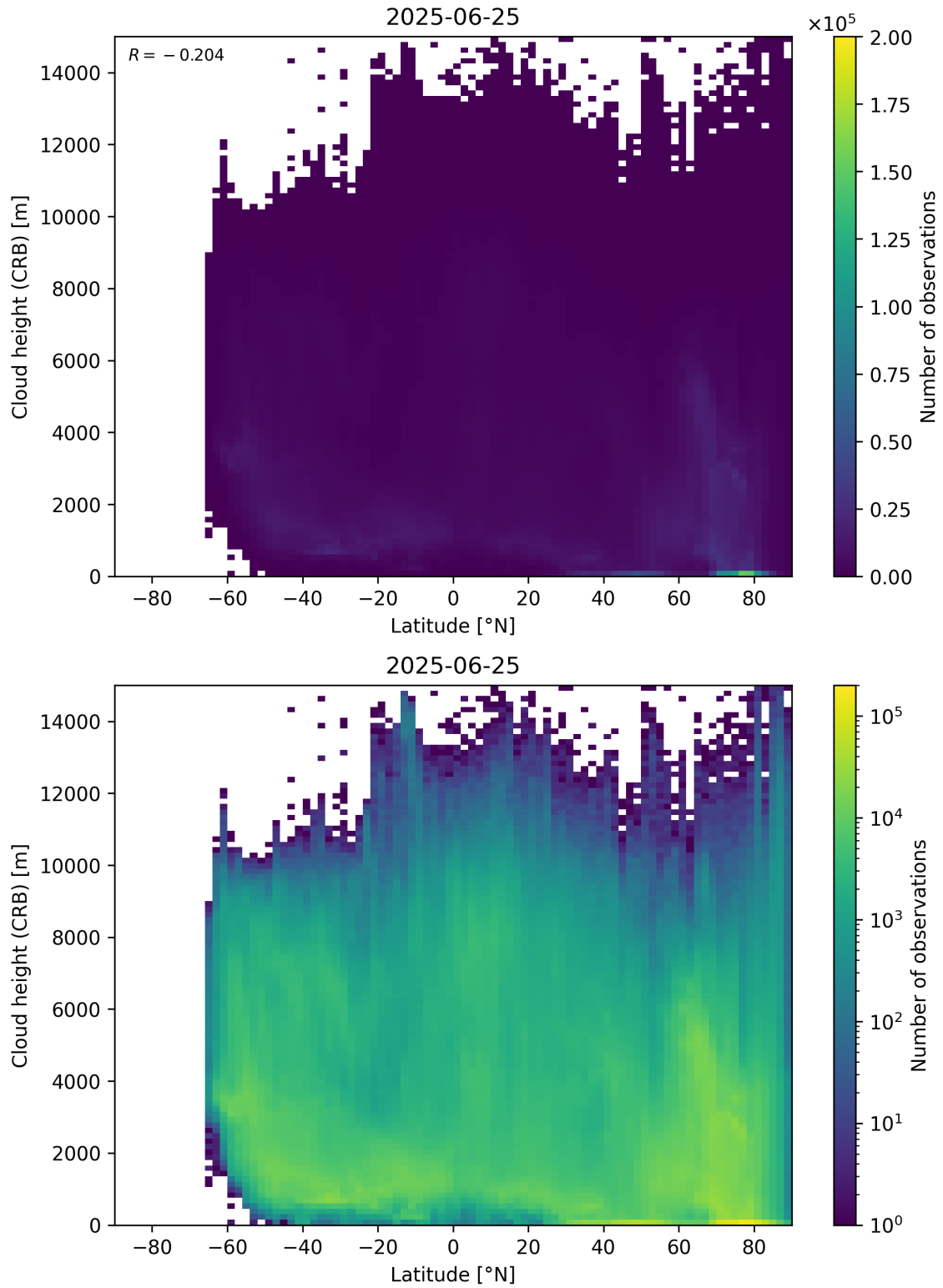
Figure 95: Scatter density plot of “Latitude” against “Cloud height (CRB)” for 2025-06-24 to 2025-06-26.
