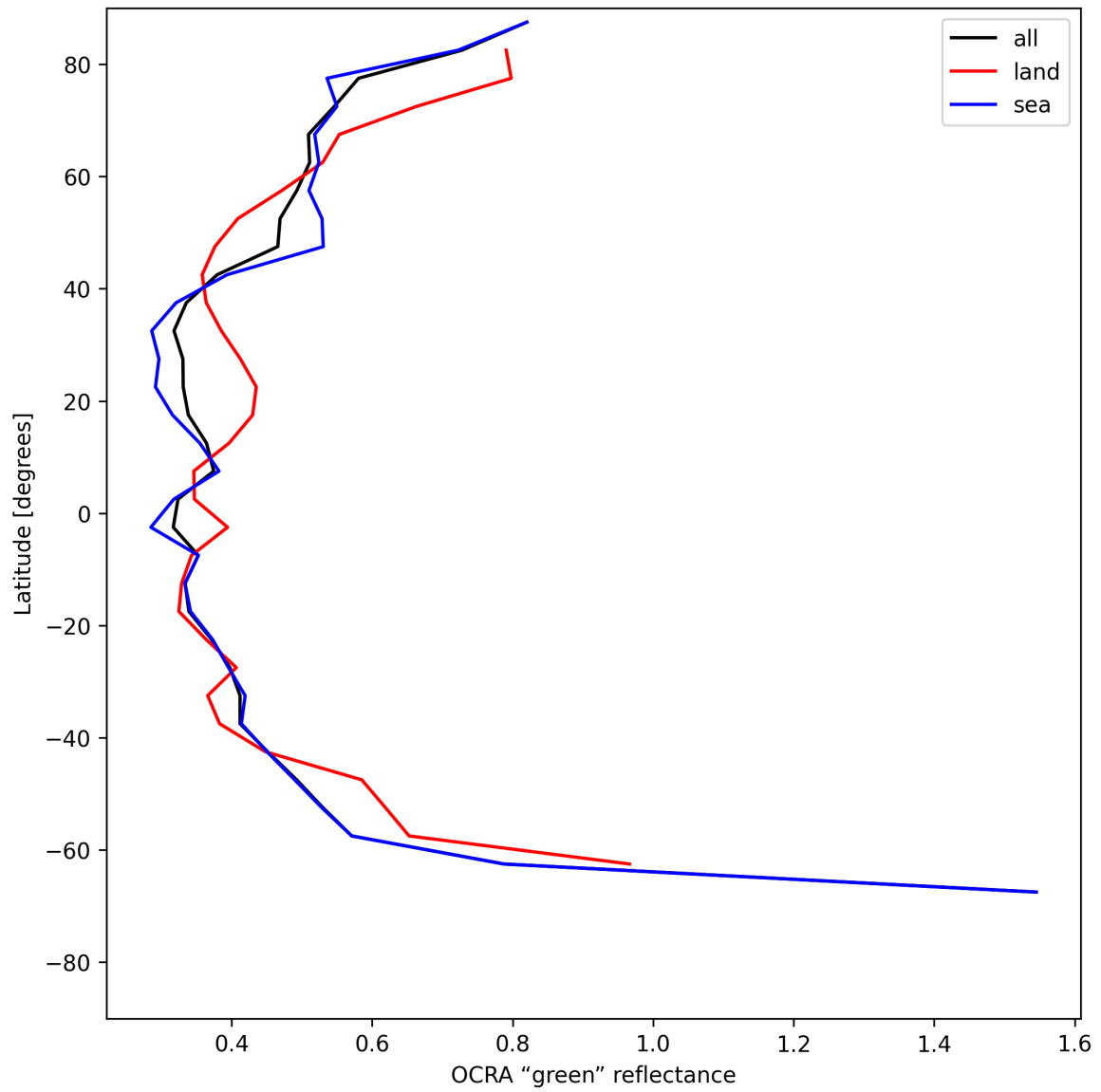
Figure 36: Zonal average of "OCRA "green" reflectance" for 2025-06-24 to 2025-06-26.
