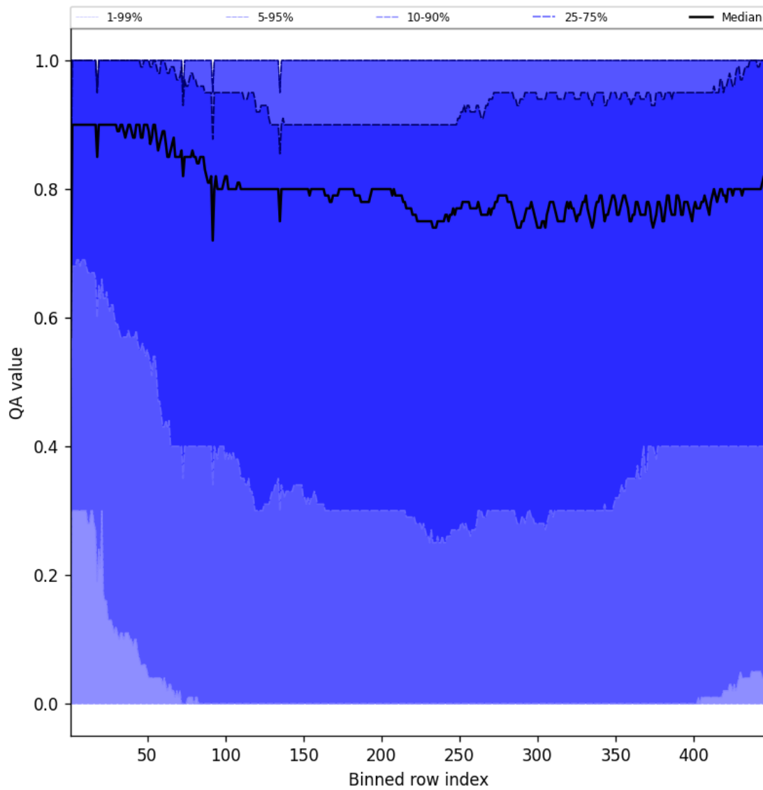
Figure 54: Along track statistics of “QA value” for 2025-06-24 to 2025-06-26
