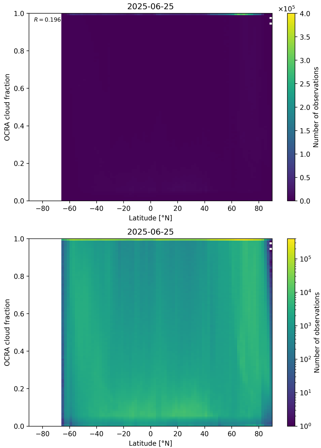
Figure 93: Scatter density plot of “Latitude” against “OCRA cloud fraction” for 2025-06-24 to 2025-06-26.
