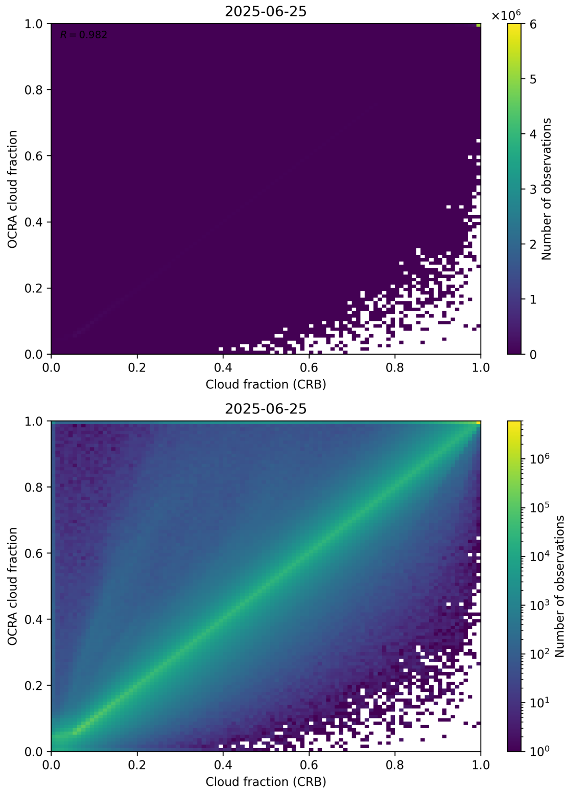
Figure 78: Scatter density plot of “Cloud fraction (CRB)” against “OCRA cloud fraction” for 2025-06-24 to 2025-06-26.
