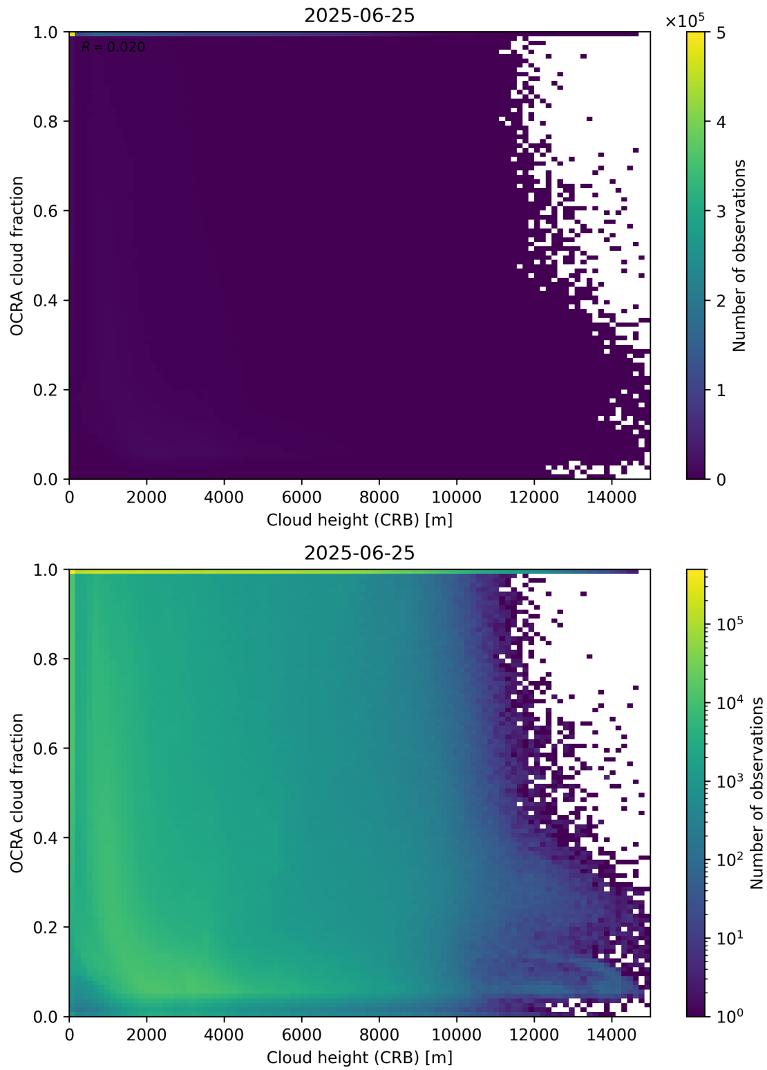
Figure 81: Scatter density plot of “Cloud height (CRB)” against “OCRA cloud fraction” for 2025-06-24 to 2025-06-26.
