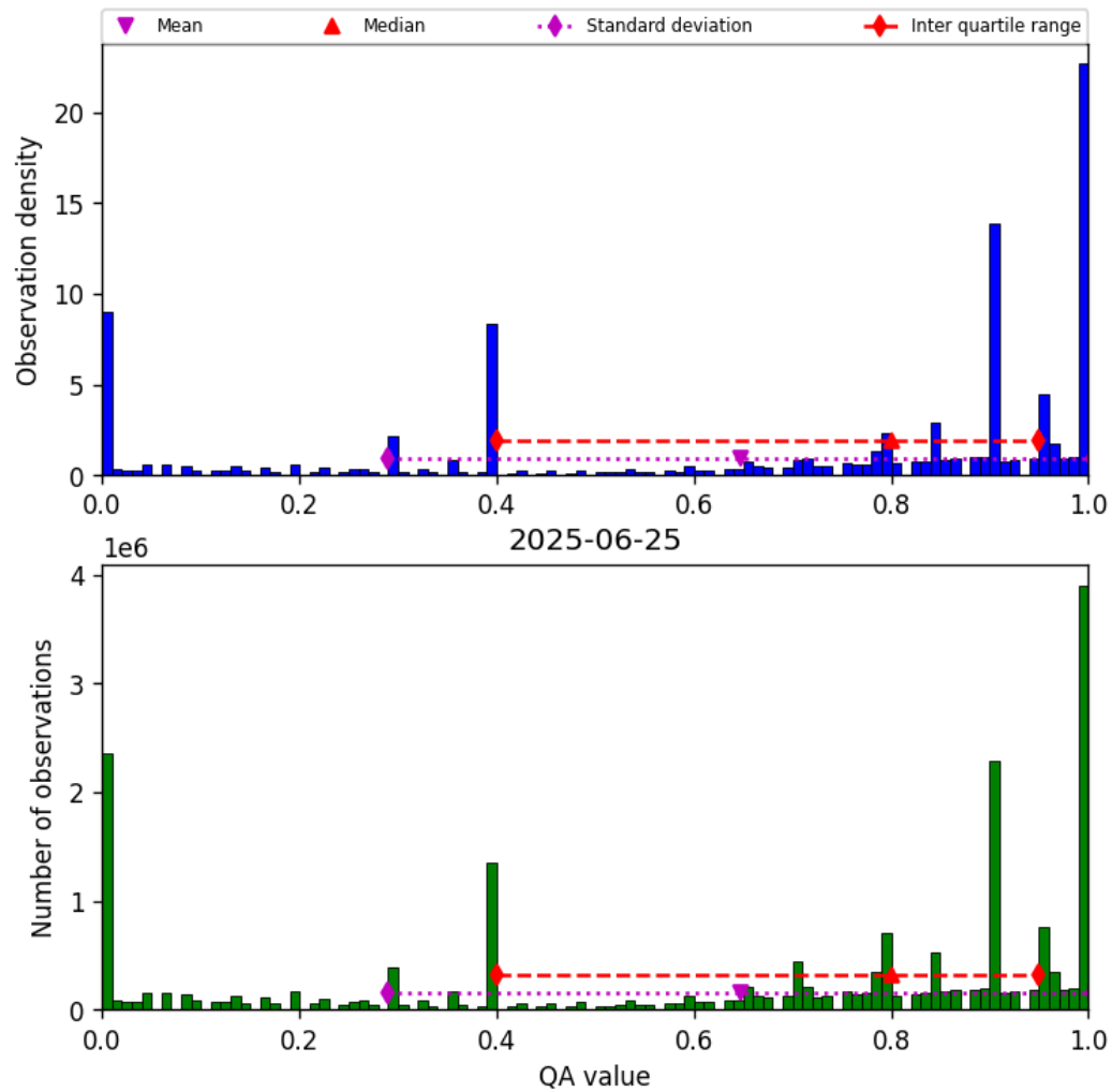
Figure 38: Histogram of “QA value” for 2025-06-24 to 2025-06-26
