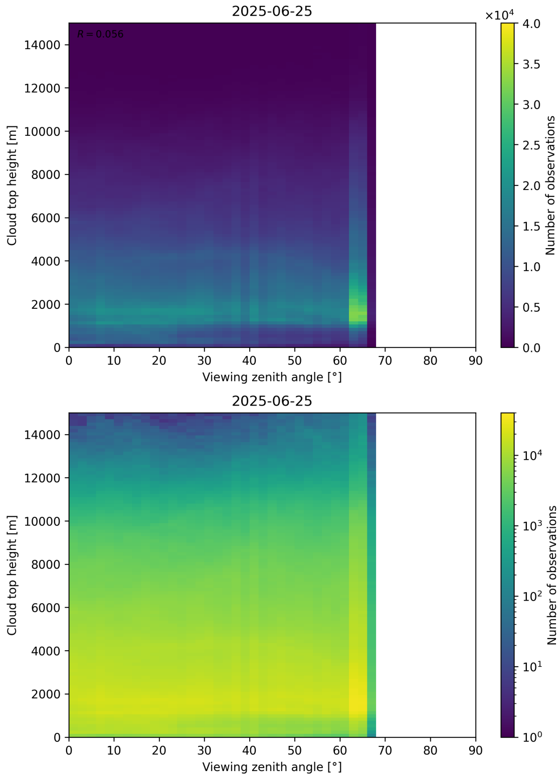
Figure 112: Scatter density plot of “Viewing zenith angle” against “Cloud top height” for 2025-06-24 to 2025-06-26.
