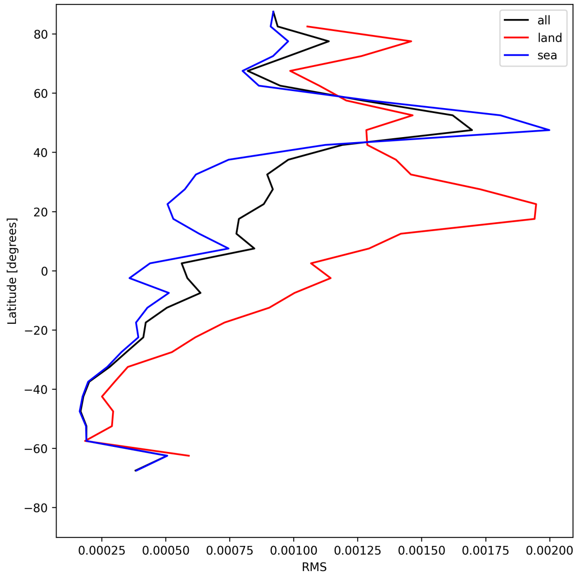
Figure 31: Zonal average of “RMS” for 2025-06-24 to 2025-06-26.
