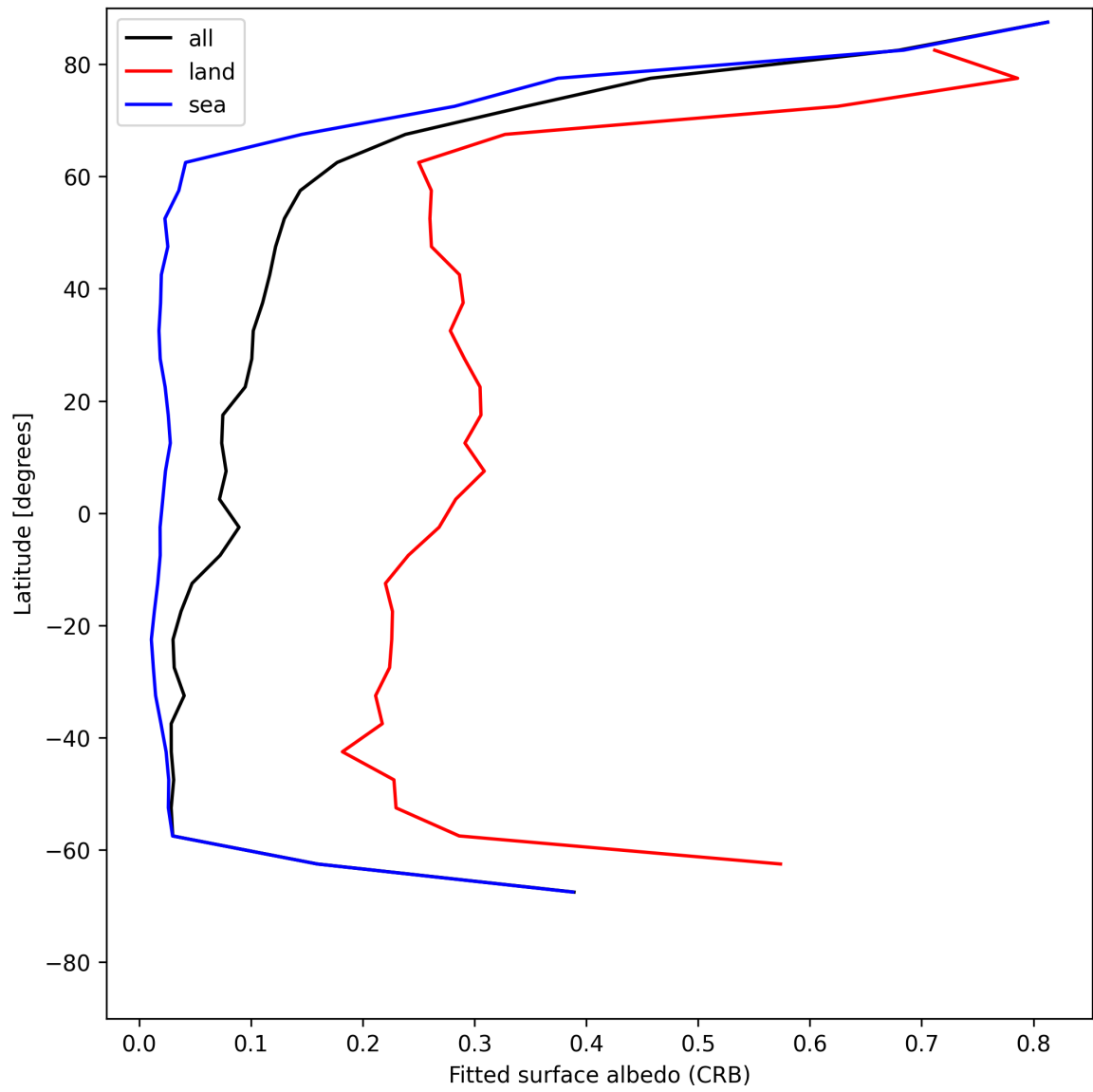
Figure 30: Zonal average of “Fitted surface albedo (CRB)” for 2025-06-24 to 2025-06-26.
