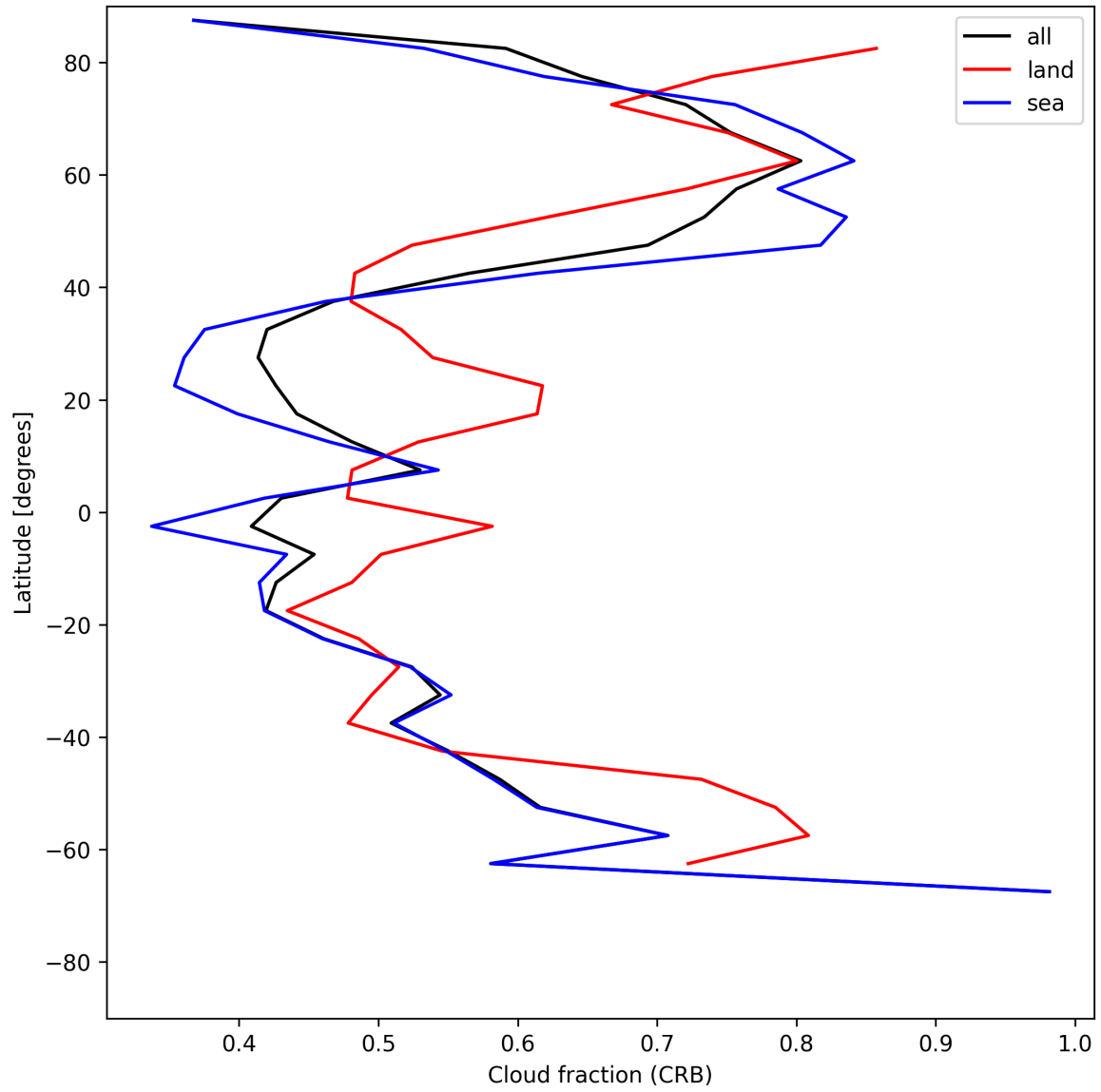
Figure 26: Zonal average of “Cloud fraction (CRB)” for 2025-06-24 to 2025-06-26.
