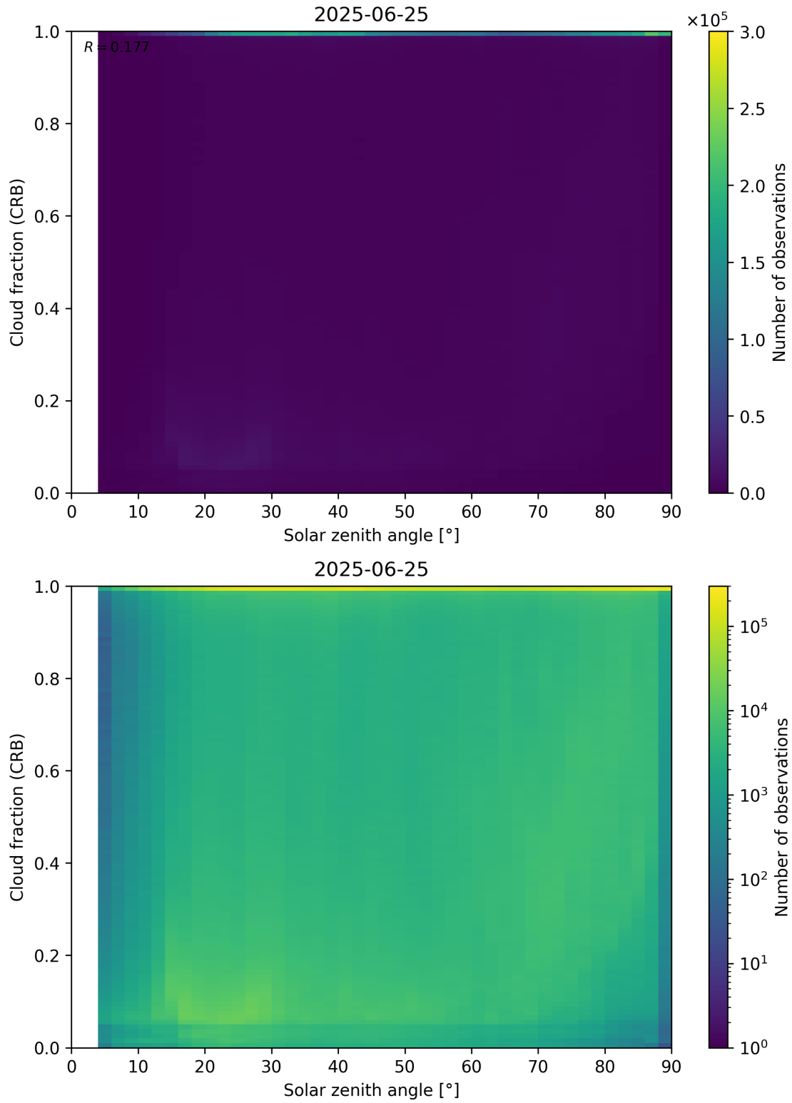
Figure 101: Scatter density plot of “Solar zenith angle” against “Cloud fraction (CRB)” for 2025-06-24 to 2025-06-26.
