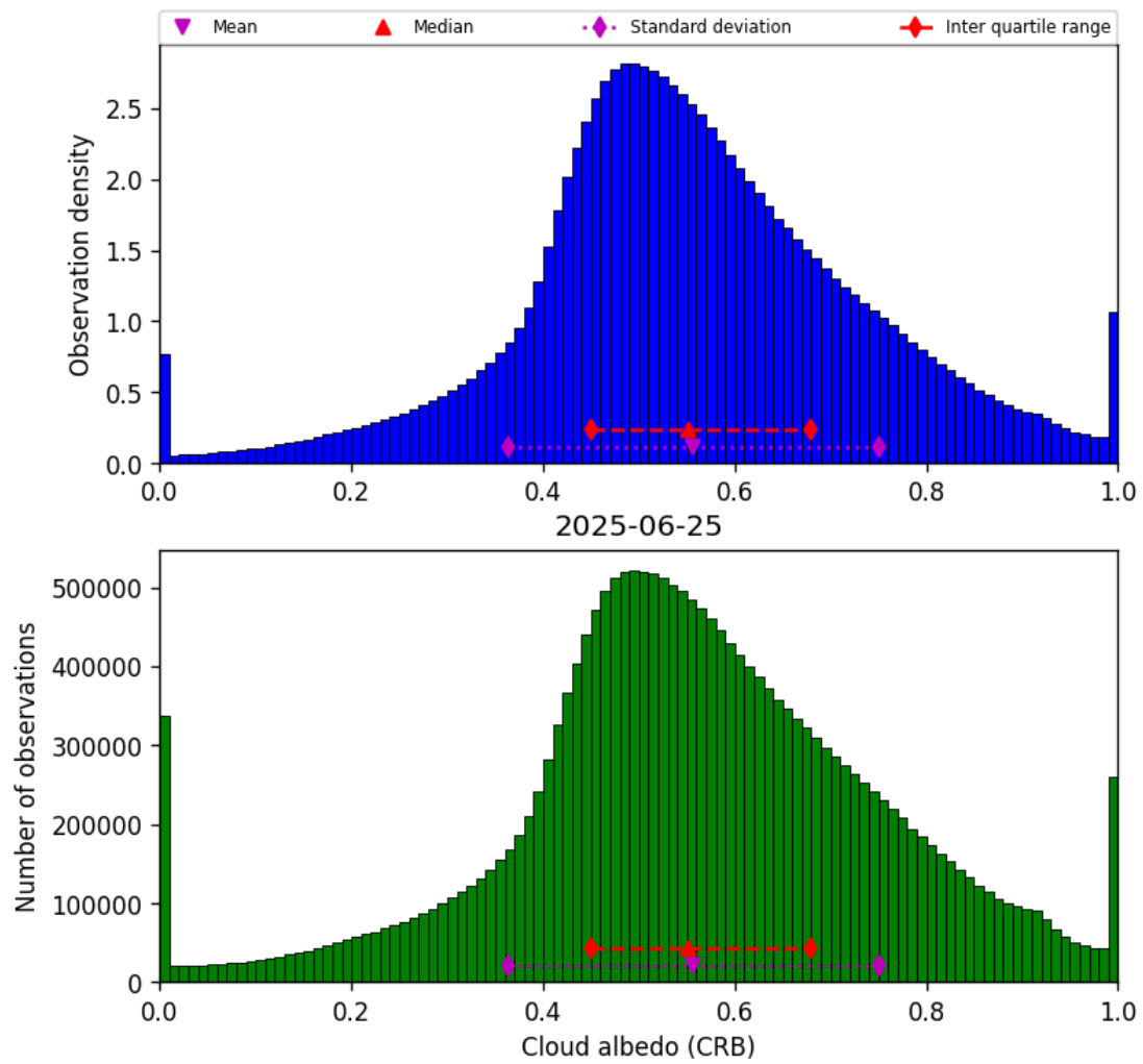
Figure 44: Histogram of “Cloud albedo (CRB)” for 2025-06-24 to 2025-06-26
