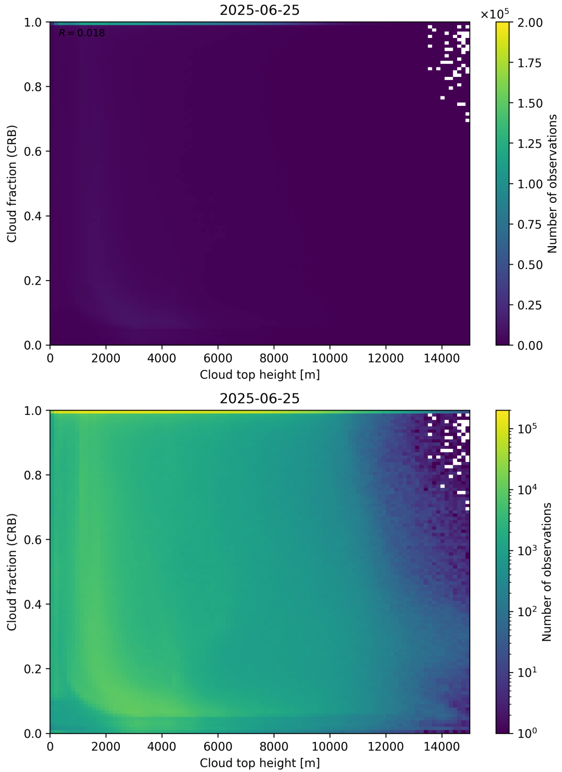
Figure 88: Scatter density plot of “Cloud top height” against “Cloud fraction (CRB)” for 2025-06-24 to 2025-06-26.
