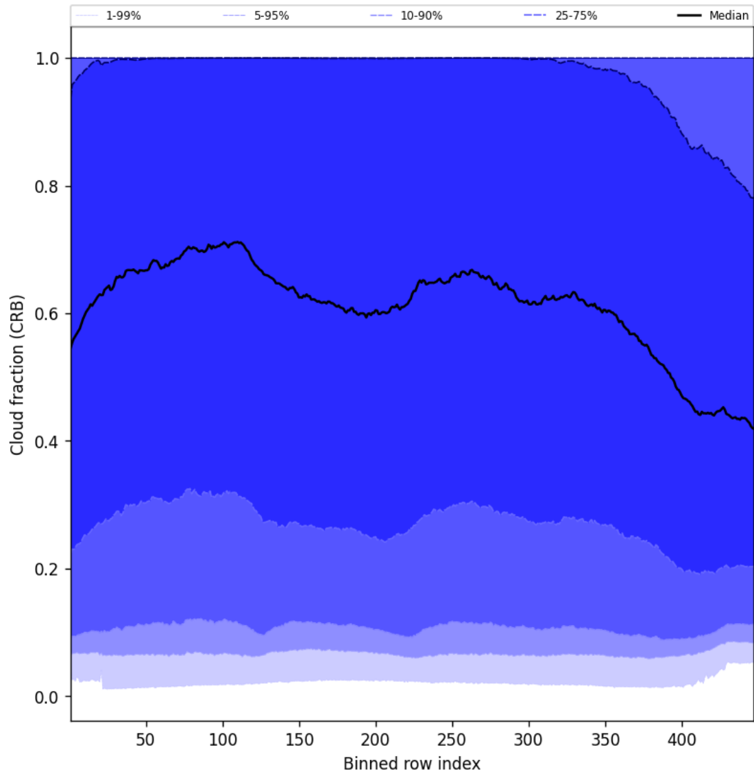
Figure 58: Along track statistics of “Cloud fraction (CRB)” for 2025-06-24 to 2025-06-26
