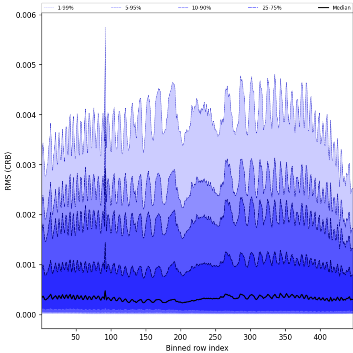
Figure 64: Along track statistics of “RMS (CRB)” for 2025-06-24 to 2025-06-26
