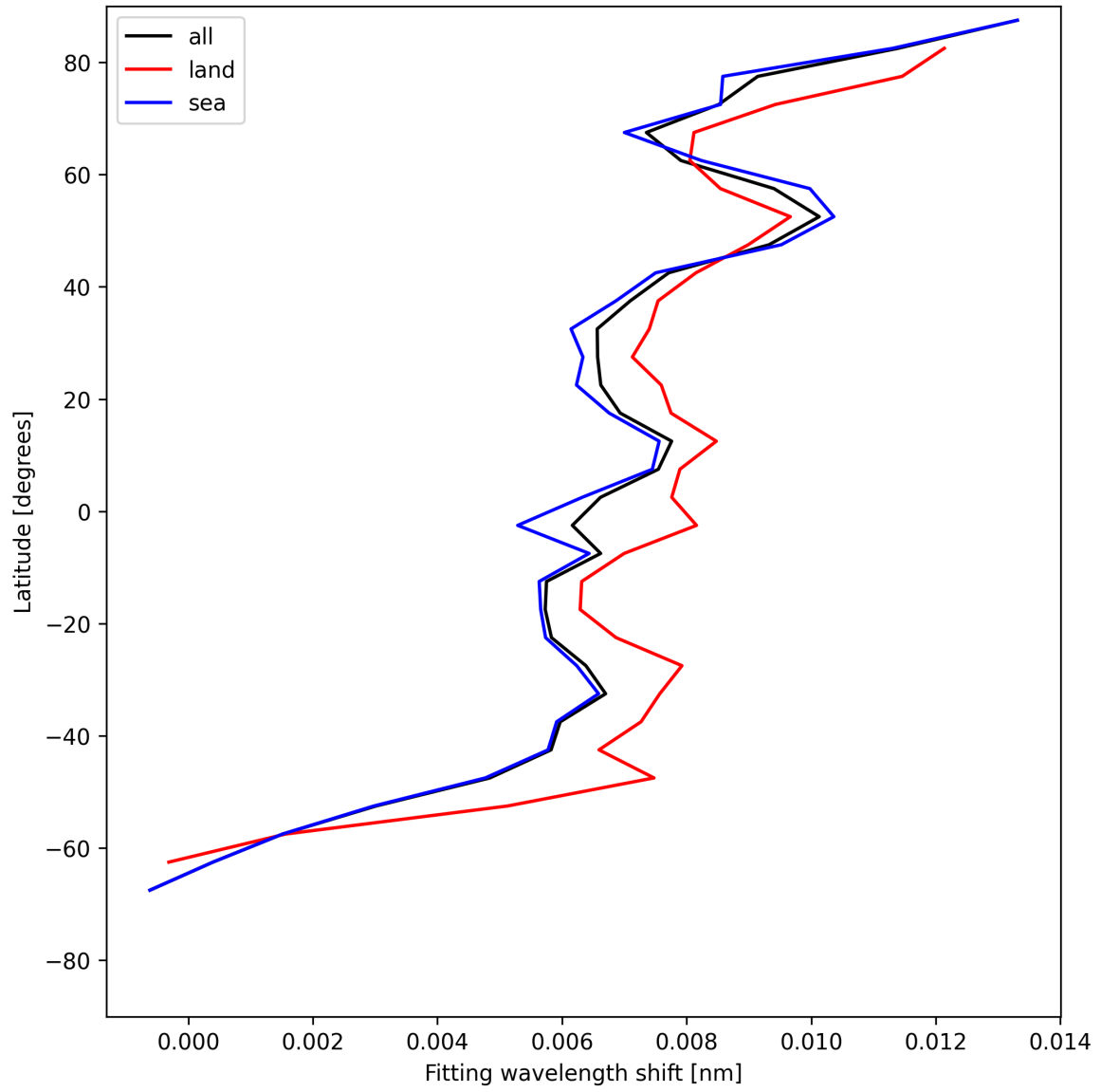
Figure 33: Zonal average of “Fitting wavelength shift” for 2025-06-24 to 2025-06-26.
