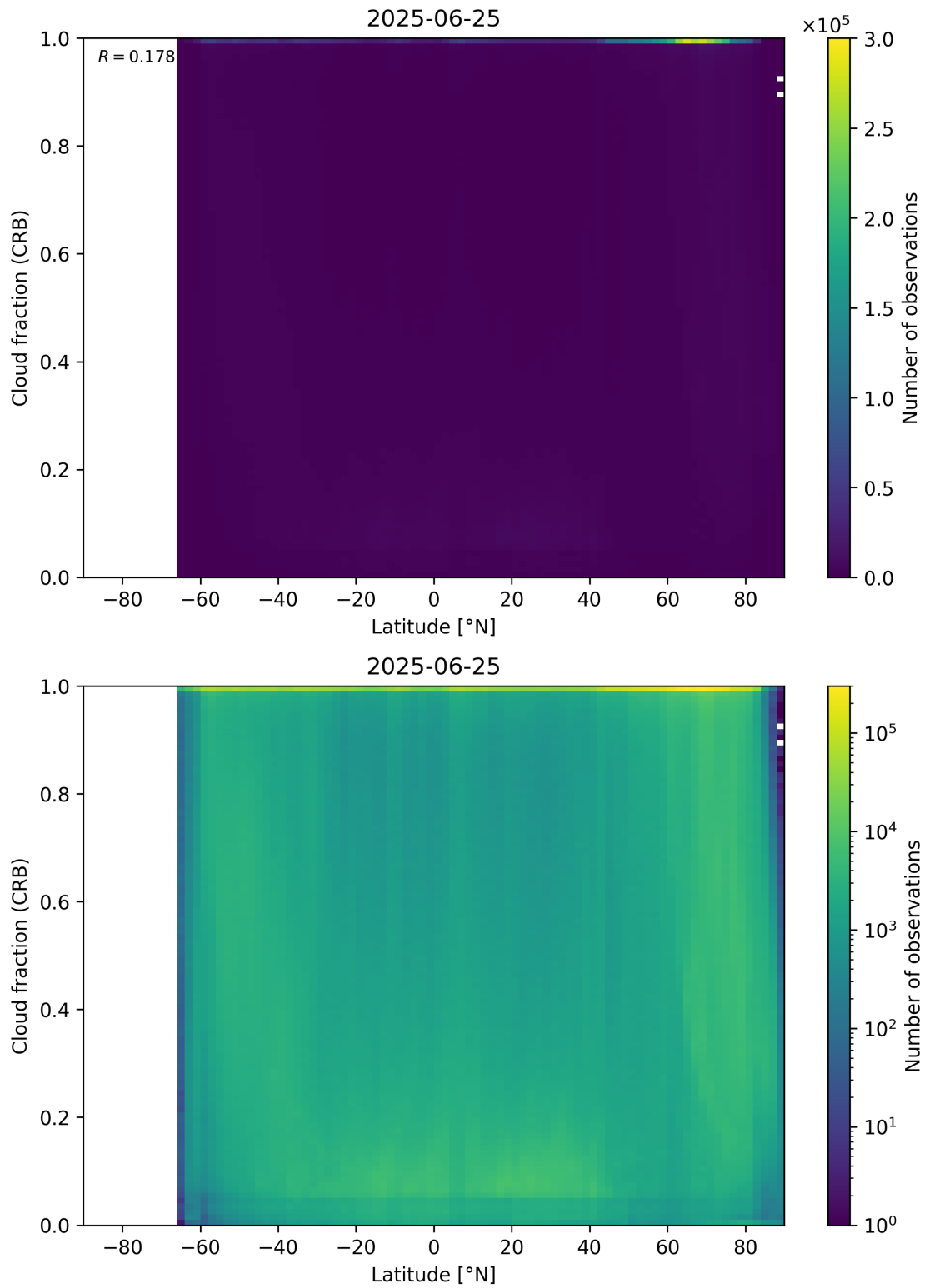
Figure 94: Scatter density plot of “Latitude” against “Cloud fraction (CRB)” for 2025-06-24 to 2025-06-26.
