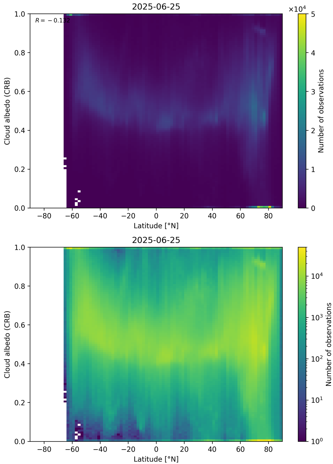
Figure 91: Scatter density plot of “Latitude” against “Cloud albedo (CRB)” for 2025-06-24 to 2025-06-26.
