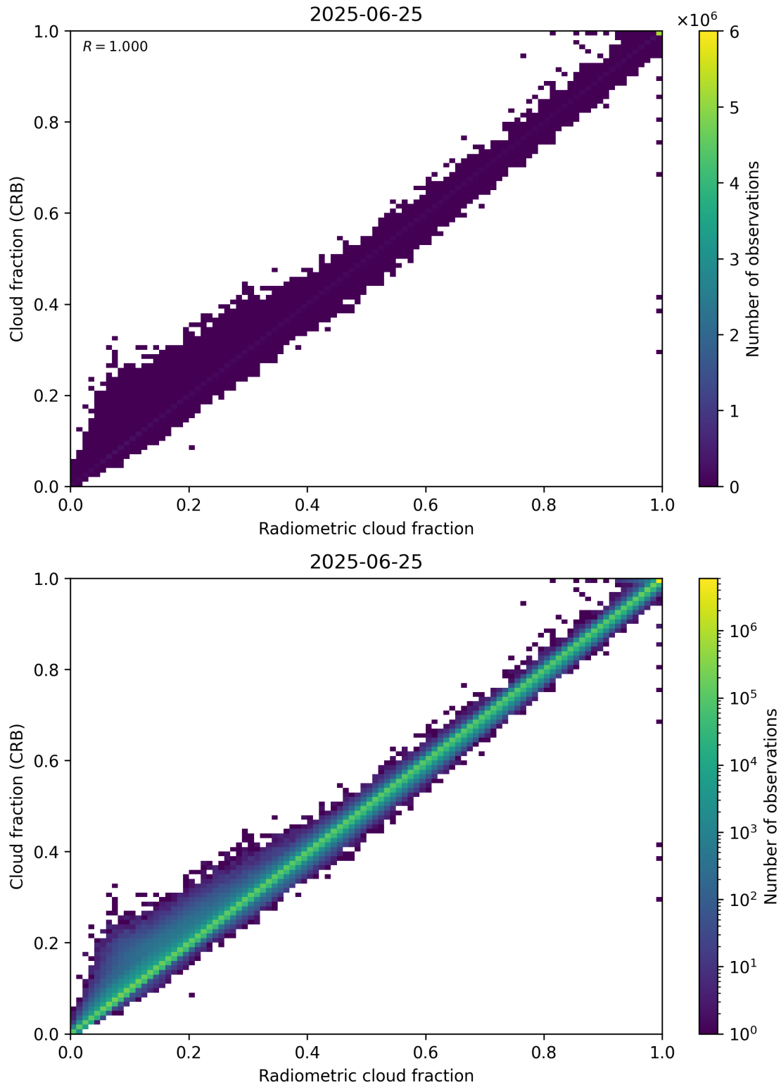
Figure 73: Scatter density plot of “Radiometric cloud fraction” against “Cloud fraction (CRB)” for 2025-06-24 to 2025-06-26.
