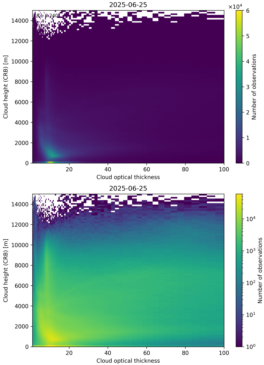
Figure 85: Scatter density plot of “Cloud optical thickness” against “Cloud height (CRB)” for 2025-06-24 to 2025-06-26.
