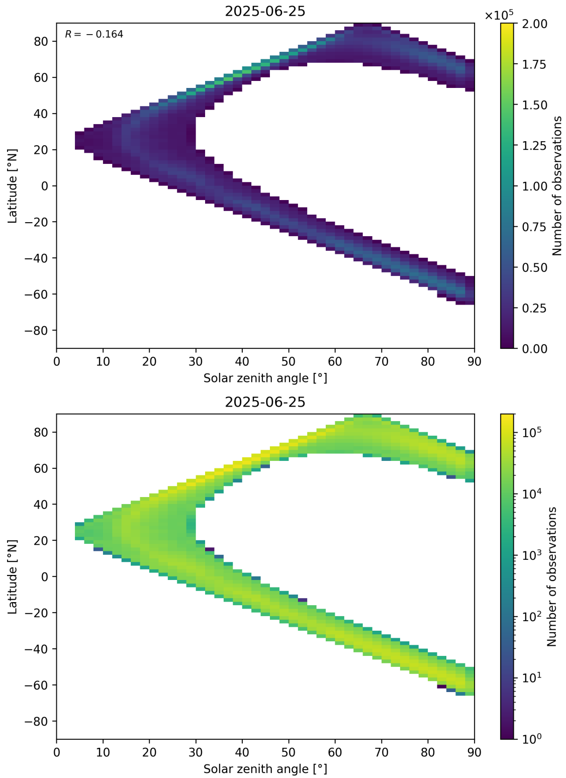
Figure 105: Scatter density plot of “Solar zenith angle” against “Latitude” for 2025-06-24 to 2025-06-26.
