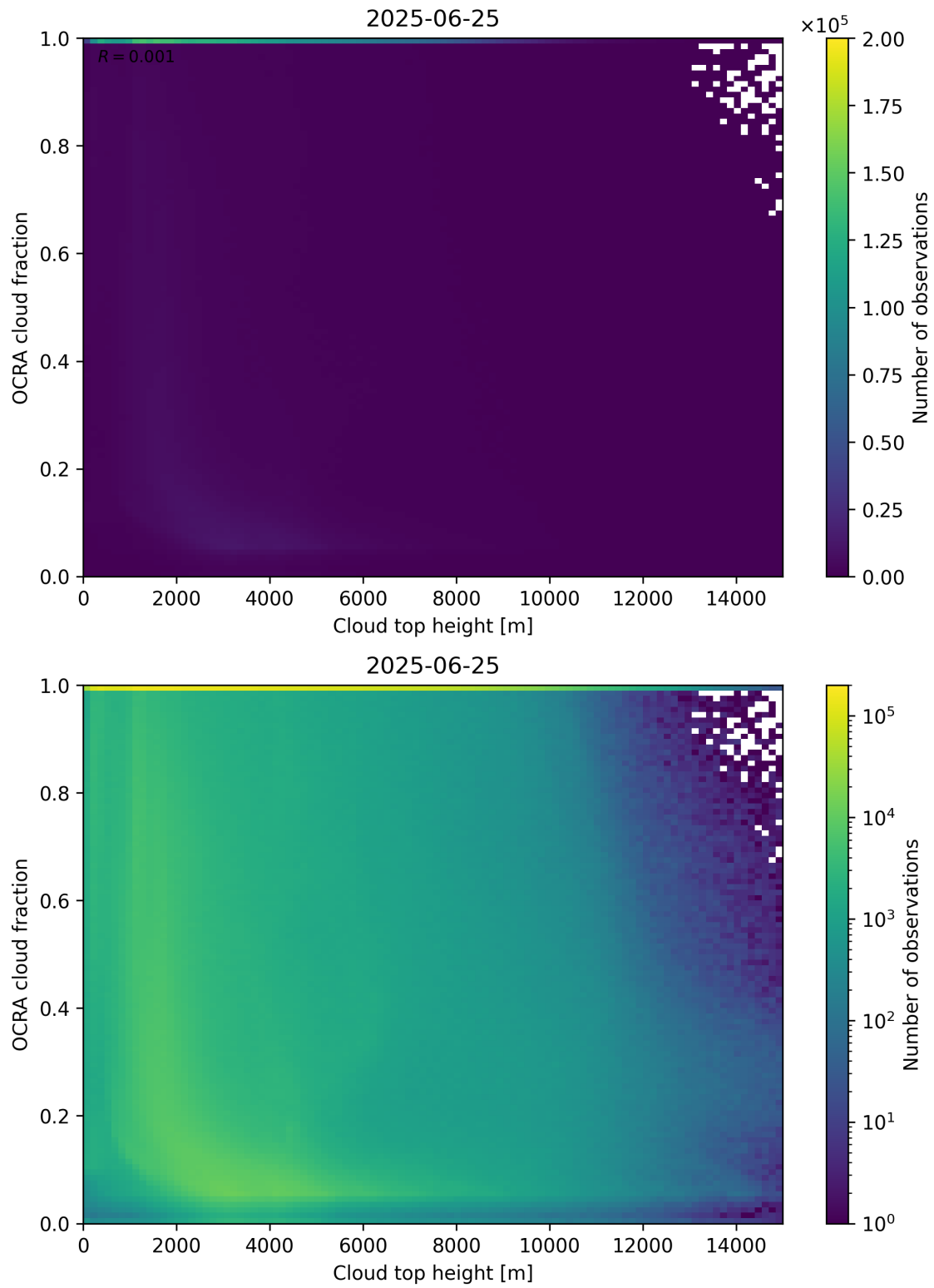
Figure 87: Scatter density plot of “Cloud top height” against “OCRA cloud fraction” for 2025-06-24 to 2025-06-26.
