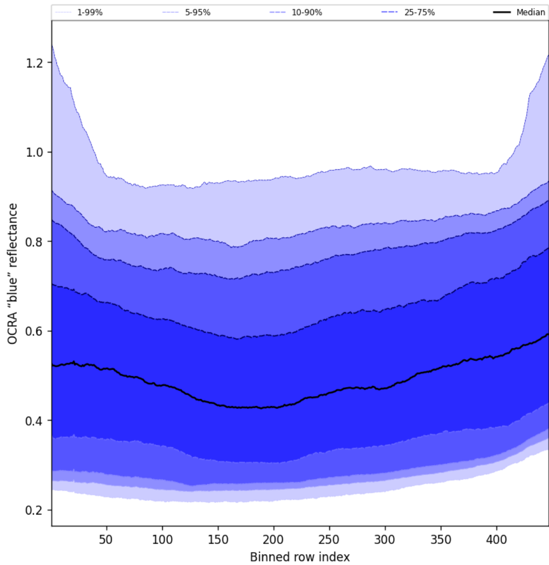
Figure 67: Along track statistics of “OCRA “blue” reflectance” for 2025-06-24 to 2025-06-26
