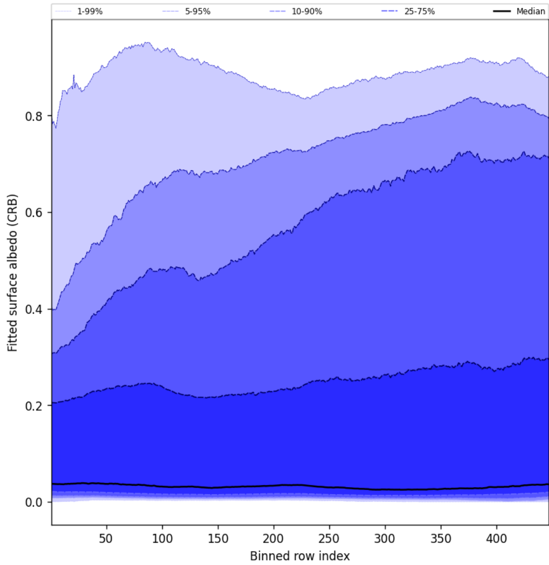
Figure 62: Along track statistics of “Fitted surface albedo (CRB)” for 2025-06-24 to 2025-06-26
