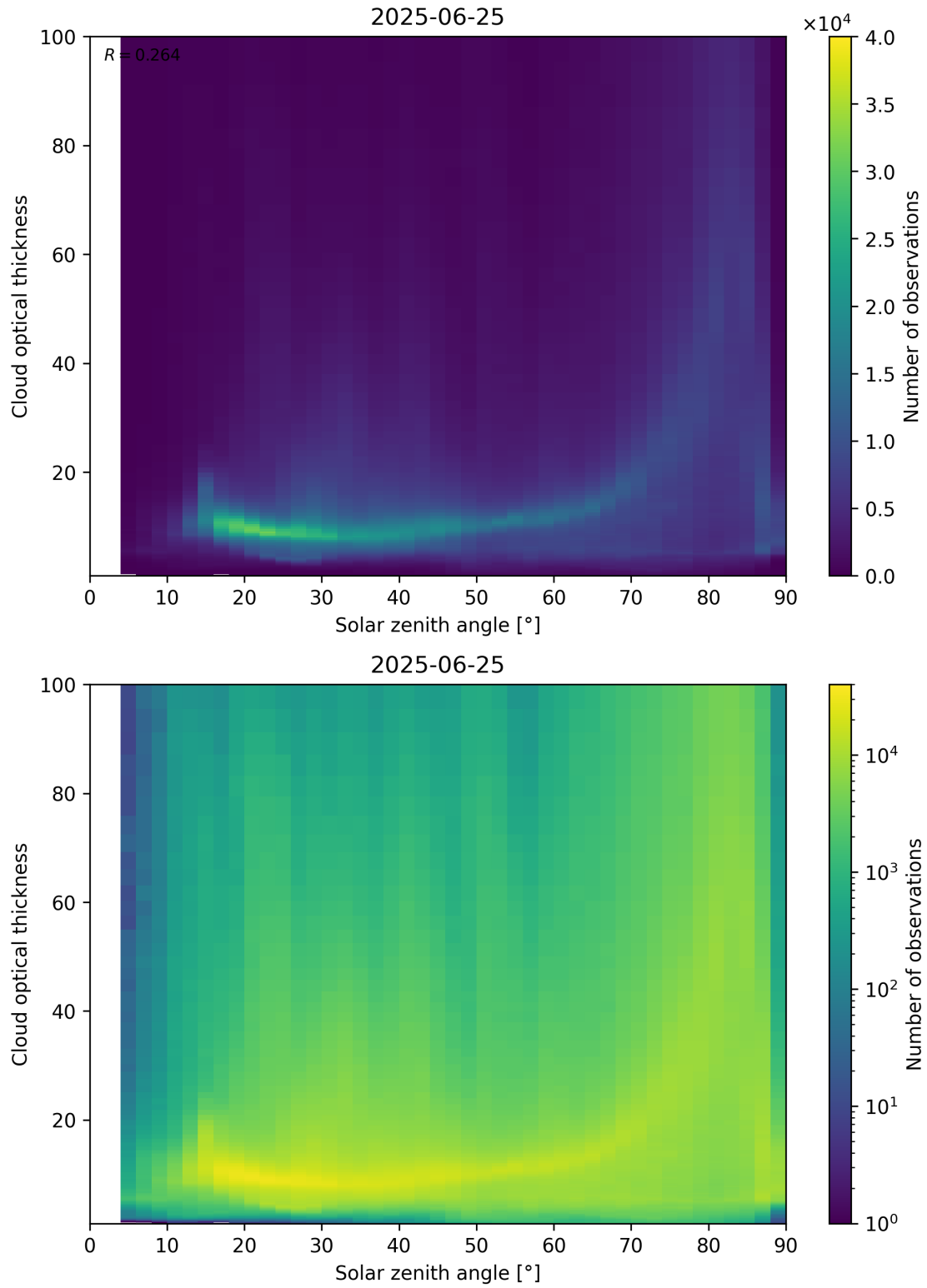
Figure 103: Scatter density plot of “Solar zenith angle” against “Cloud optical thickness” for 2025-06-24 to 2025-06-26.
