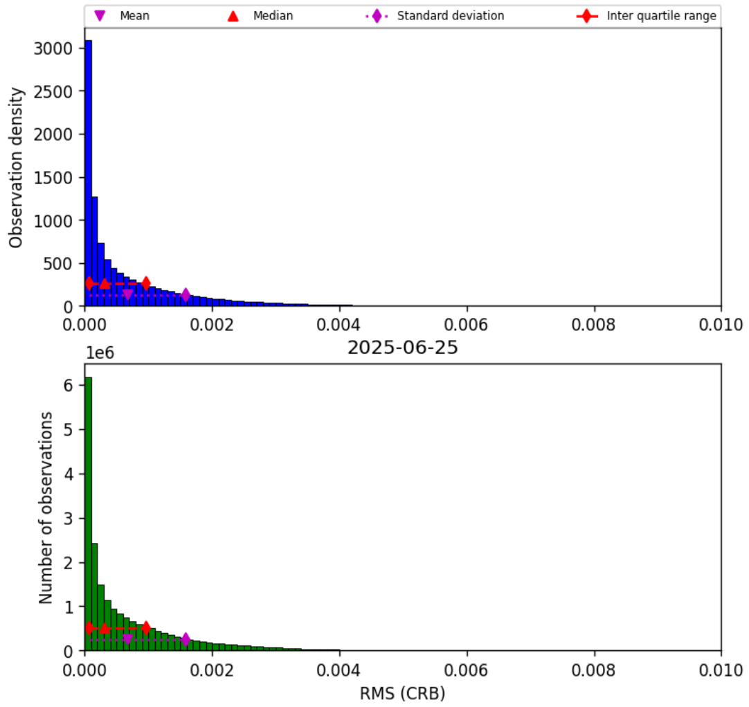
Figure 48: Histogram of “RMS (CRB)” for 2025-06-24 to 2025-06-26
