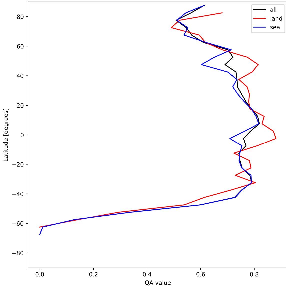
Figure 22: Zonal average of “QA value” for 2025-06-24 to 2025-06-26.
