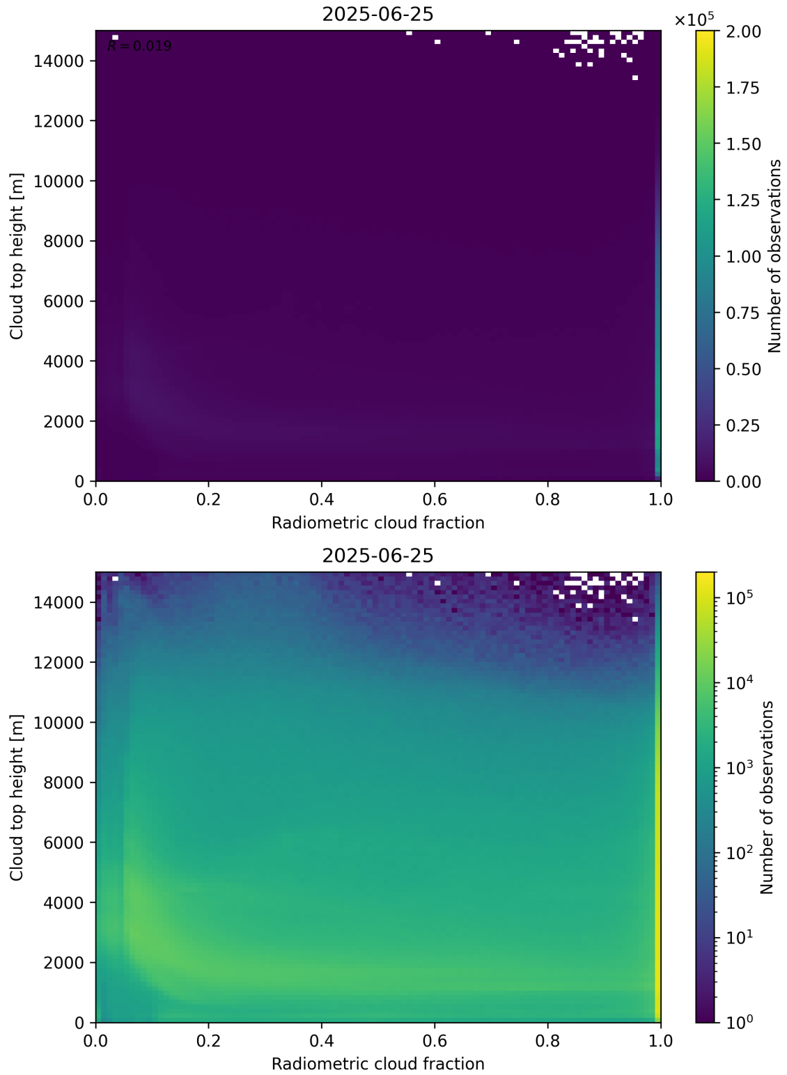
Figure 76: Scatter density plot of “Radiometric cloud fraction” against “Cloud top height” for 2025-06-24 to 2025-06-26.
