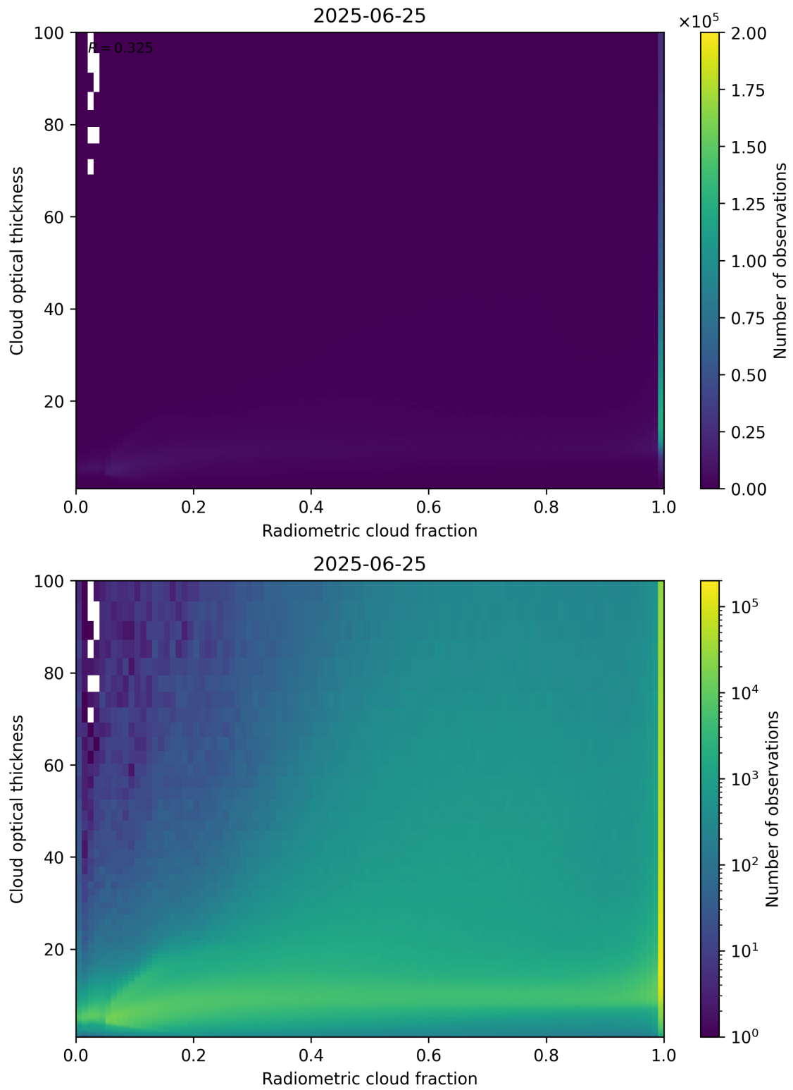
Figure 75: Scatter density plot of “Radiometric cloud fraction” against “Cloud optical thickness” for 2025-06-24 to 2025-06-26.
