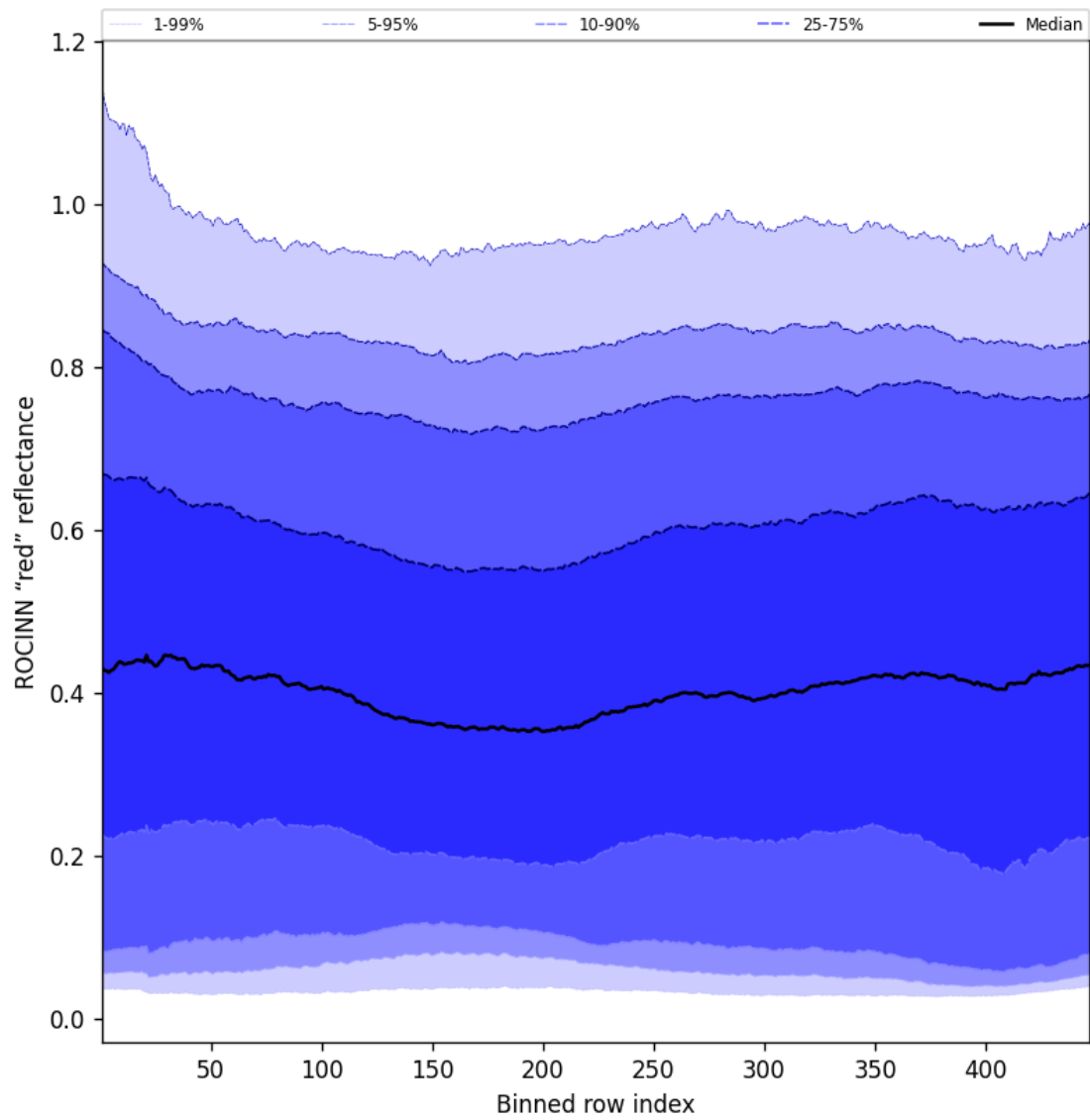
Figure 69: Along track statistics of "ROCINN "red" reflectance" for 2025-06-24 to 2025-06-26
