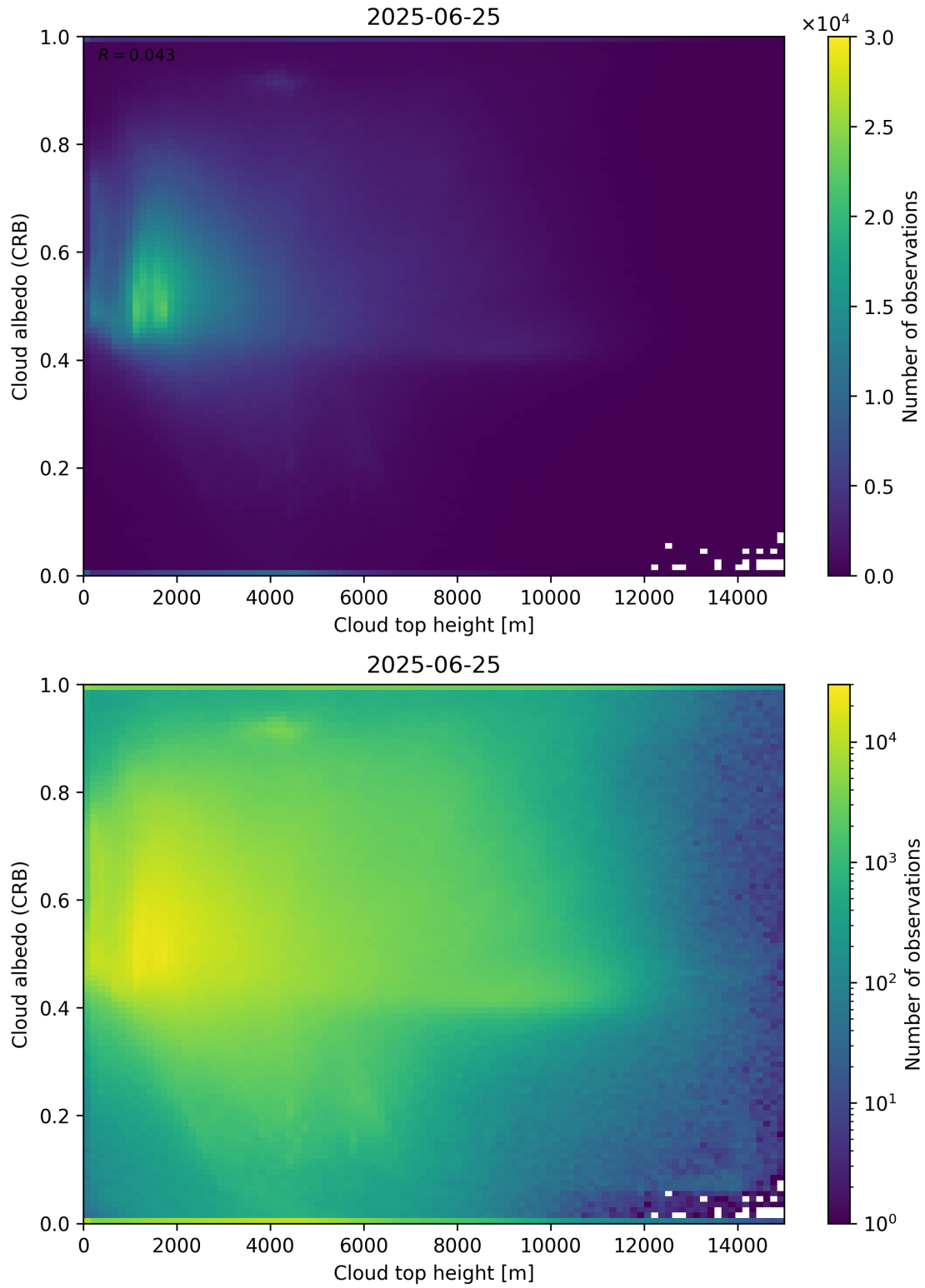
Figure 86: Scatter density plot of “Cloud top height” against “Cloud albedo (CRB)” for 2025-06-24 to 2025-06-26.
