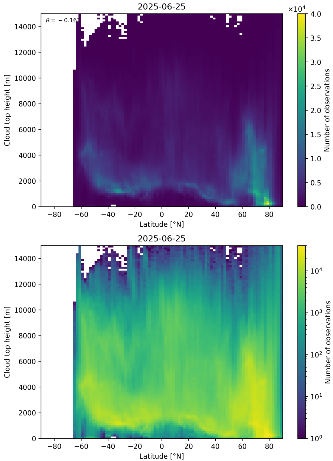
Figure 97: Scatter density plot of “Latitude” against “Cloud top height” for 2025-06-24 to 2025-06-26.
