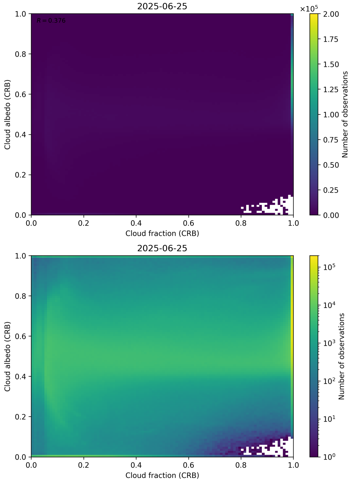
Figure 77: Scatter density plot of “Cloud fraction (CRB)” against “Cloud albedo (CRB)” for 2025-06-24 to 2025-06-26.
