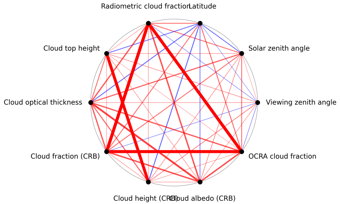
Figure 1: Map of correlation graph for 2025-06-24 to 2025-06-26.
