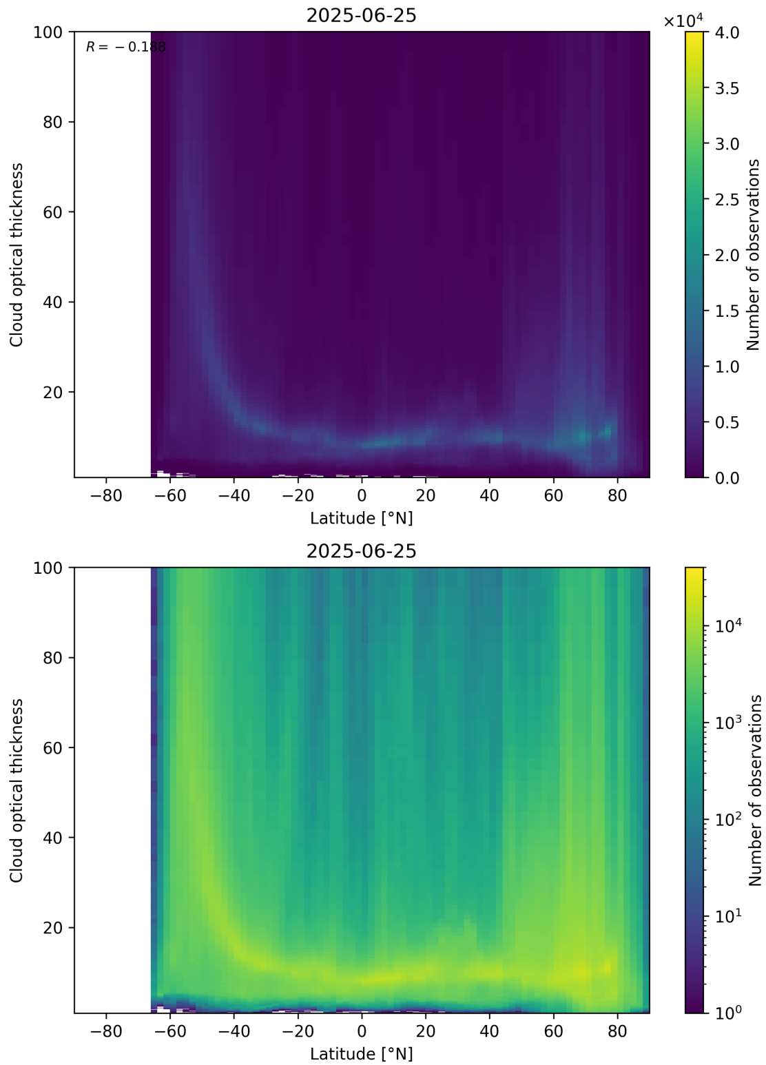
Figure 96: Scatter density plot of “Latitude” against “Cloud optical thickness” for 2025-06-24 to 2025-06-26.
