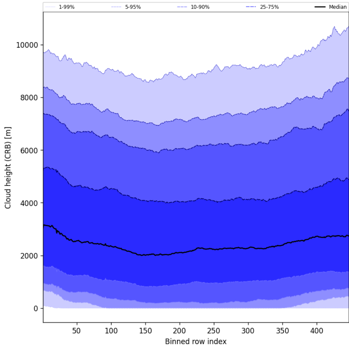
Figure 59: Along track statistics of “Cloud height (CRB)” for 2025-06-24 to 2025-06-26
