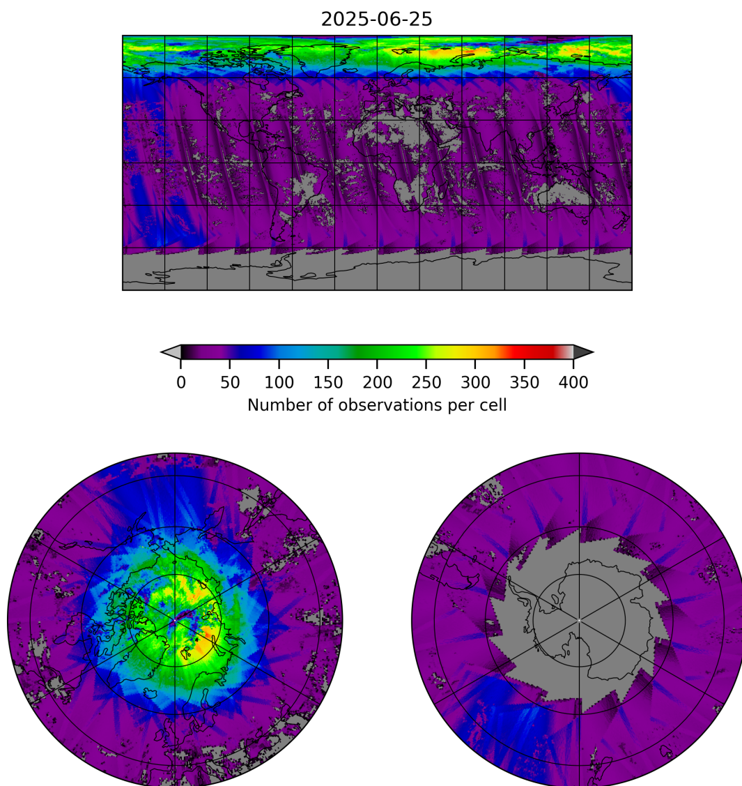
Figure 21: Map of the number of observations for 2025-06-24 to 2025-06-26
