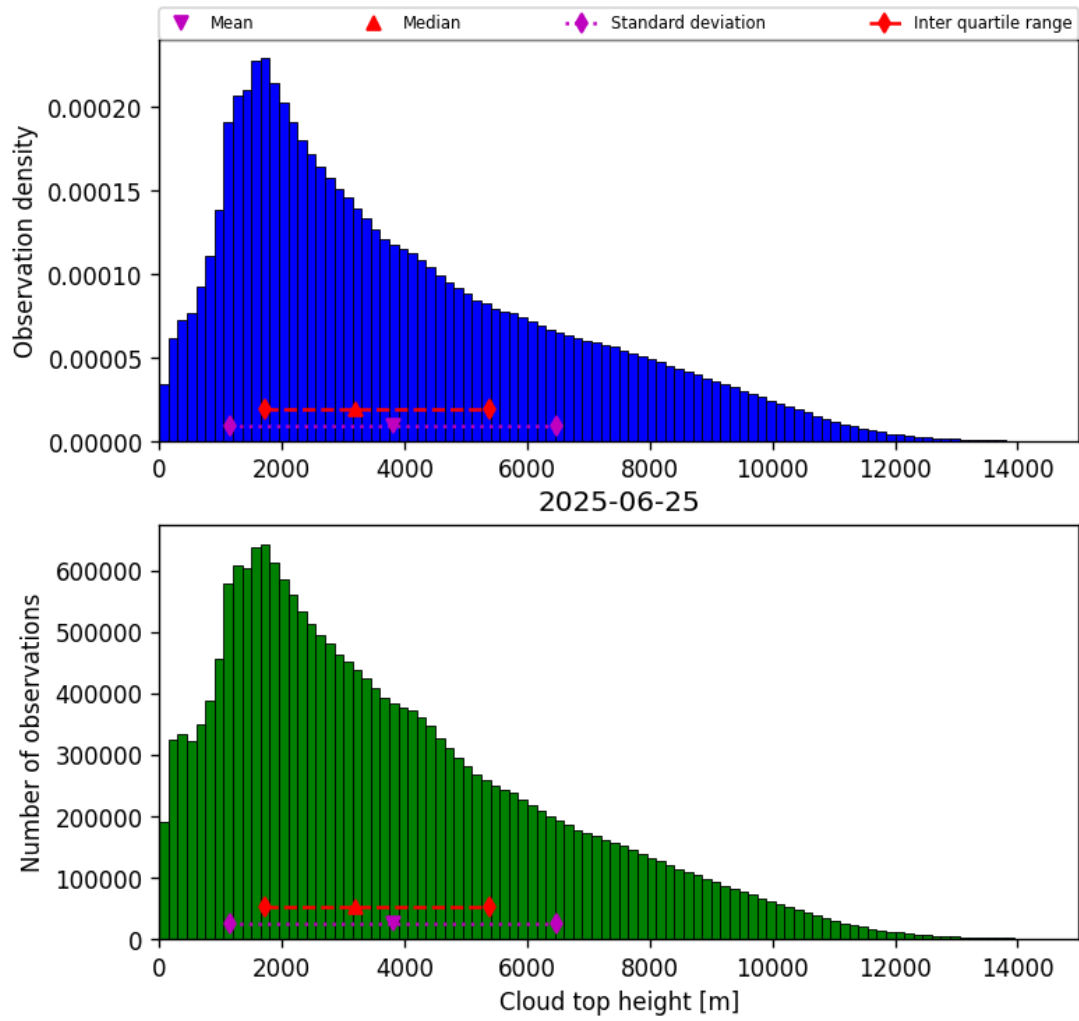
Figure 40: Histogram of “Cloud top height” for 2025-06-24 to 2025-06-26
