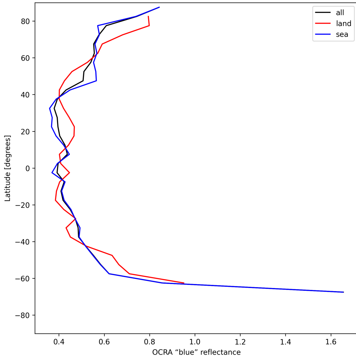
Figure 35: Zonal average of “OCRA “blue” reflectance” for 2025-06-24 to 2025-06-26.
