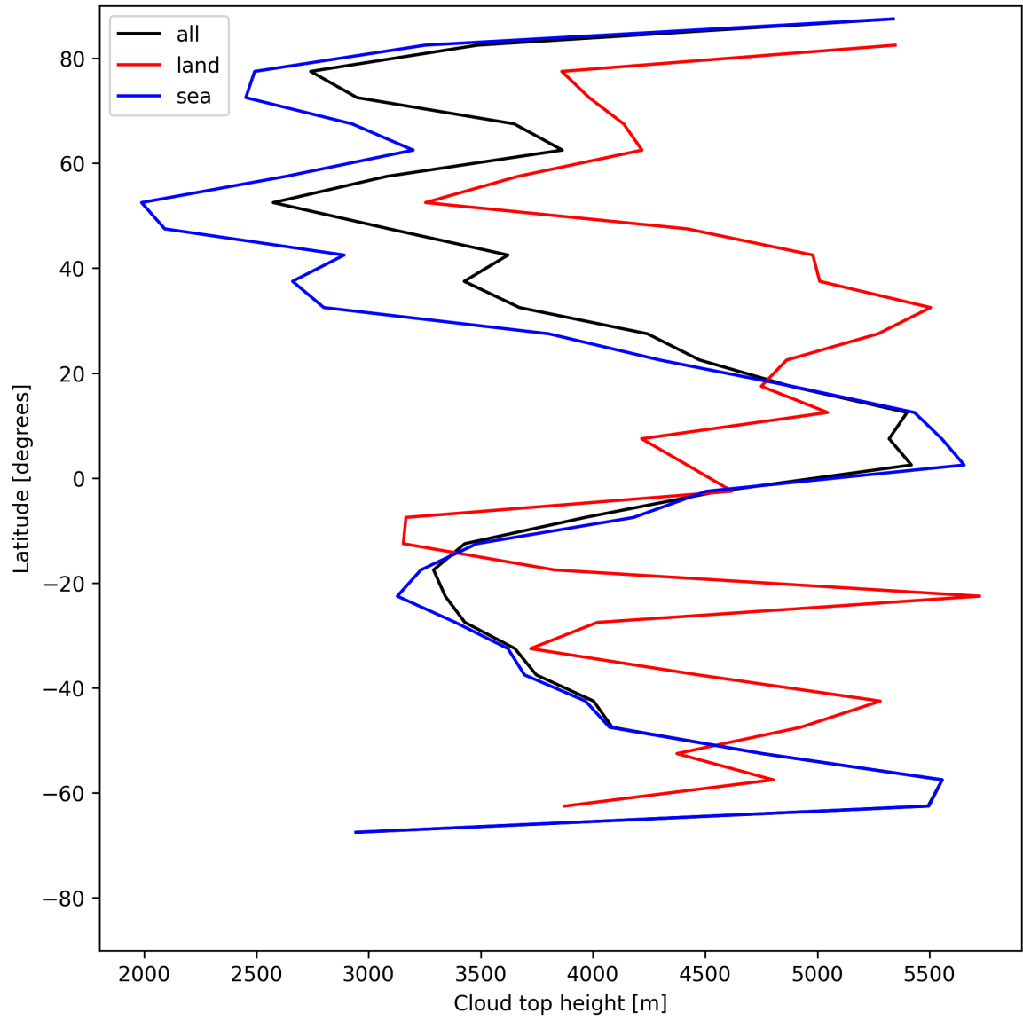
Figure 24: Zonal average of “Cloud top height” for 2025-06-24 to 2025-06-26.
