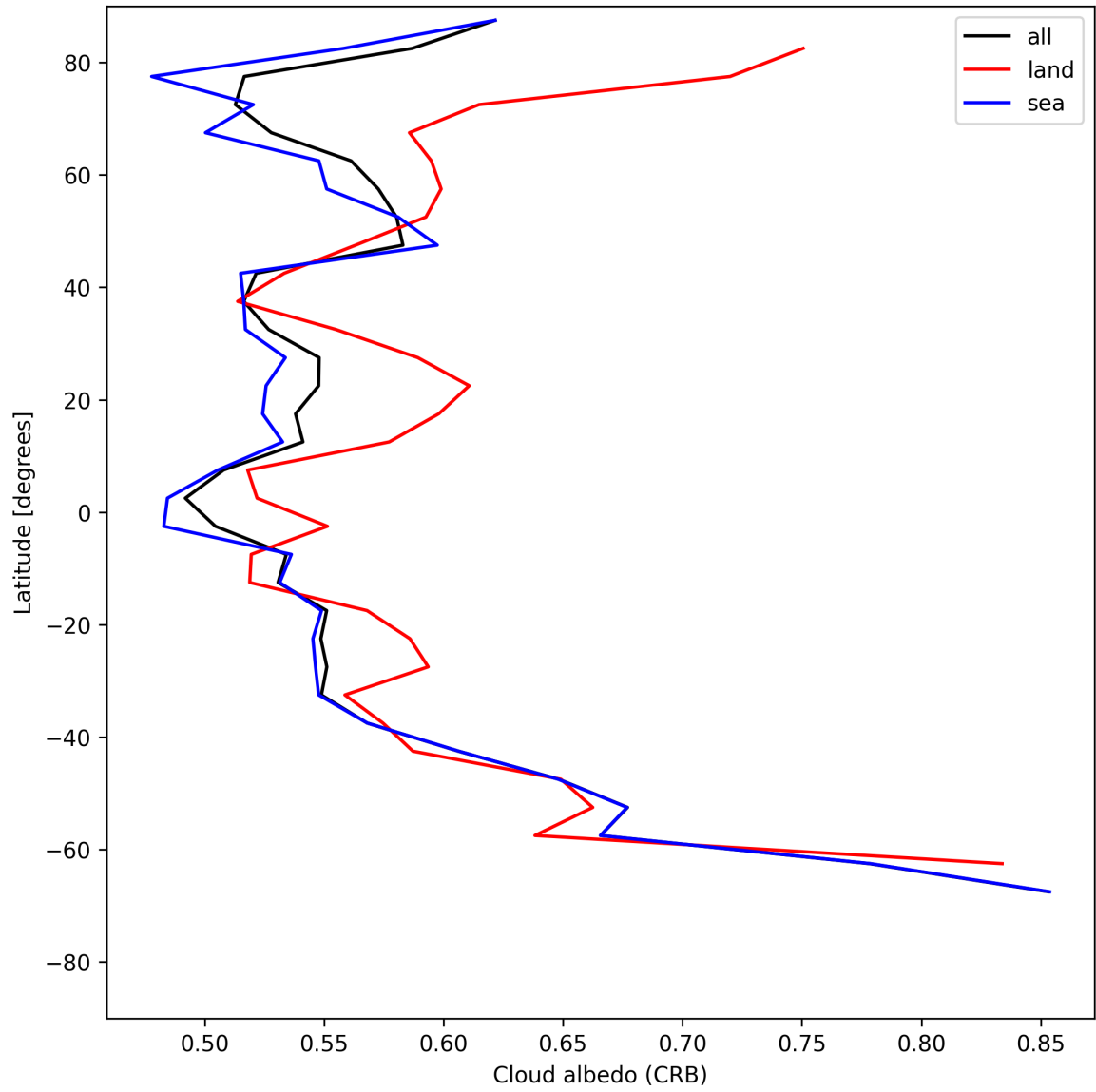
Figure 28: Zonal average of “Cloud albedo (CRB)” for 2025-06-24 to 2025-06-26.
