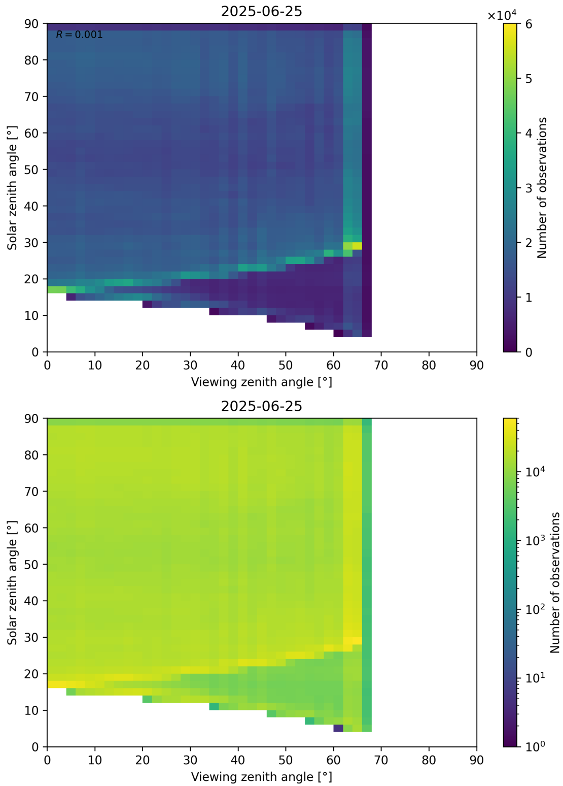
Figure 114: Scatter density plot of “Viewing zenith angle” against “Solar zenith angle” for 2025-06-24 to 2025-06-26.
