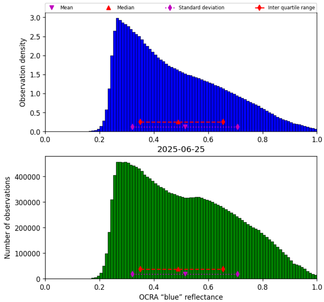
Figure 51: Histogram of “OCRA “blue” reflectance” for 2025-06-24 to 2025-06-26
