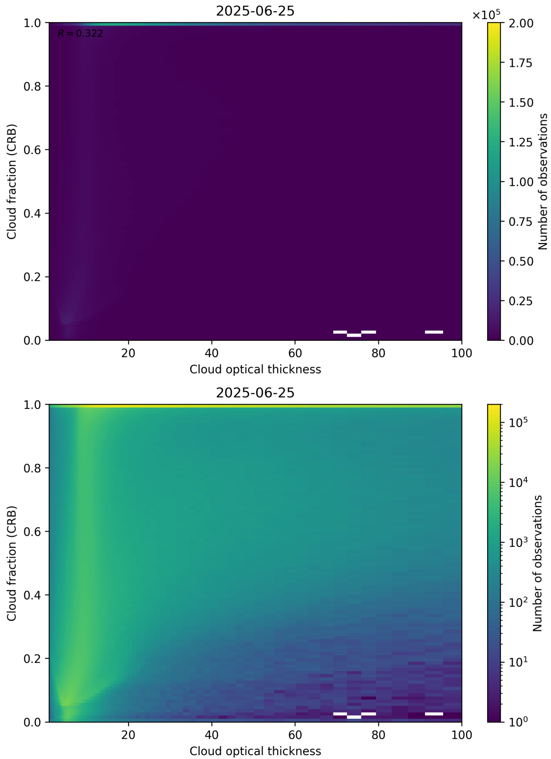
Figure 84: Scatter density plot of “Cloud optical thickness” against “Cloud fraction (CRB)” for 2025-06-24 to 2025-06-26.
