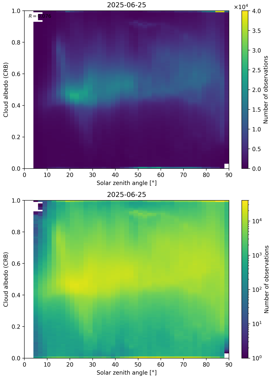
Figure 98: Scatter density plot of “Solar zenith angle” against “Cloud albedo (CRB)” for 2025-06-24 to 2025-06-26.
