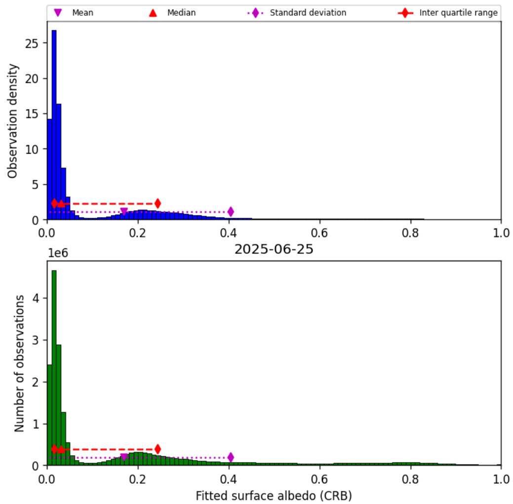
Figure 46: Histogram of “Fitted surface albedo (CRB)” for 2025-06-24 to 2025-06-26
