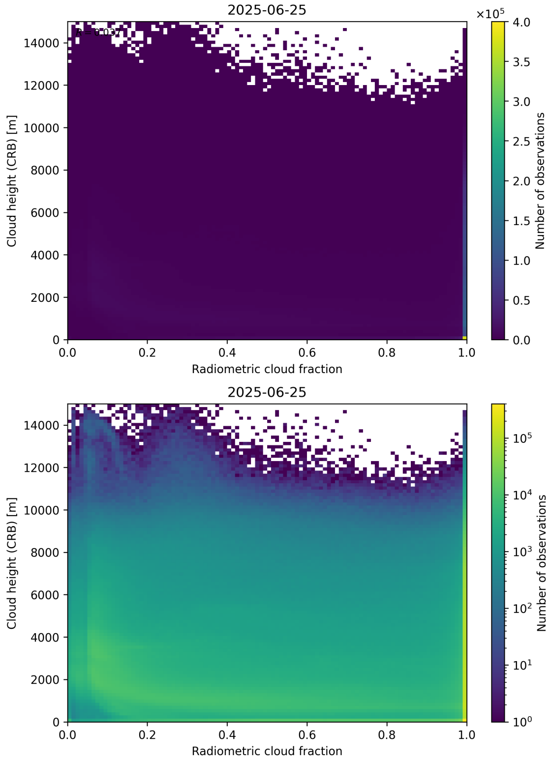
Figure 74: Scatter density plot of “Radiometric cloud fraction” against “Cloud height (CRB)” for 2025-06-24 to 2025-06-26.
