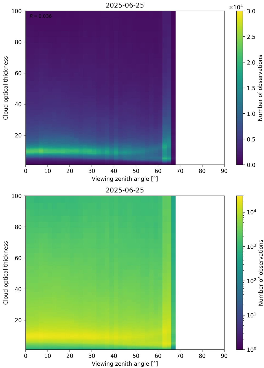
Figure 111: Scatter density plot of “Viewing zenith angle” against “Cloud optical thickness” for 2025-06-24 to 2025-06-26.
