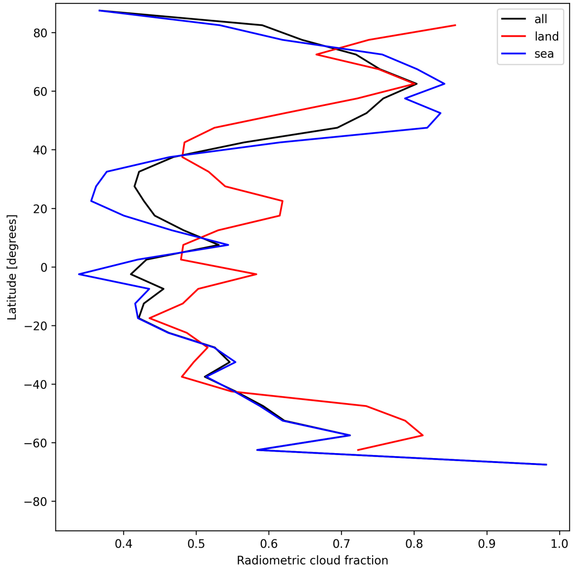
Figure 23: Zonal average of “Radiometric cloud fraction” for 2025-06-24 to 2025-06-26.
