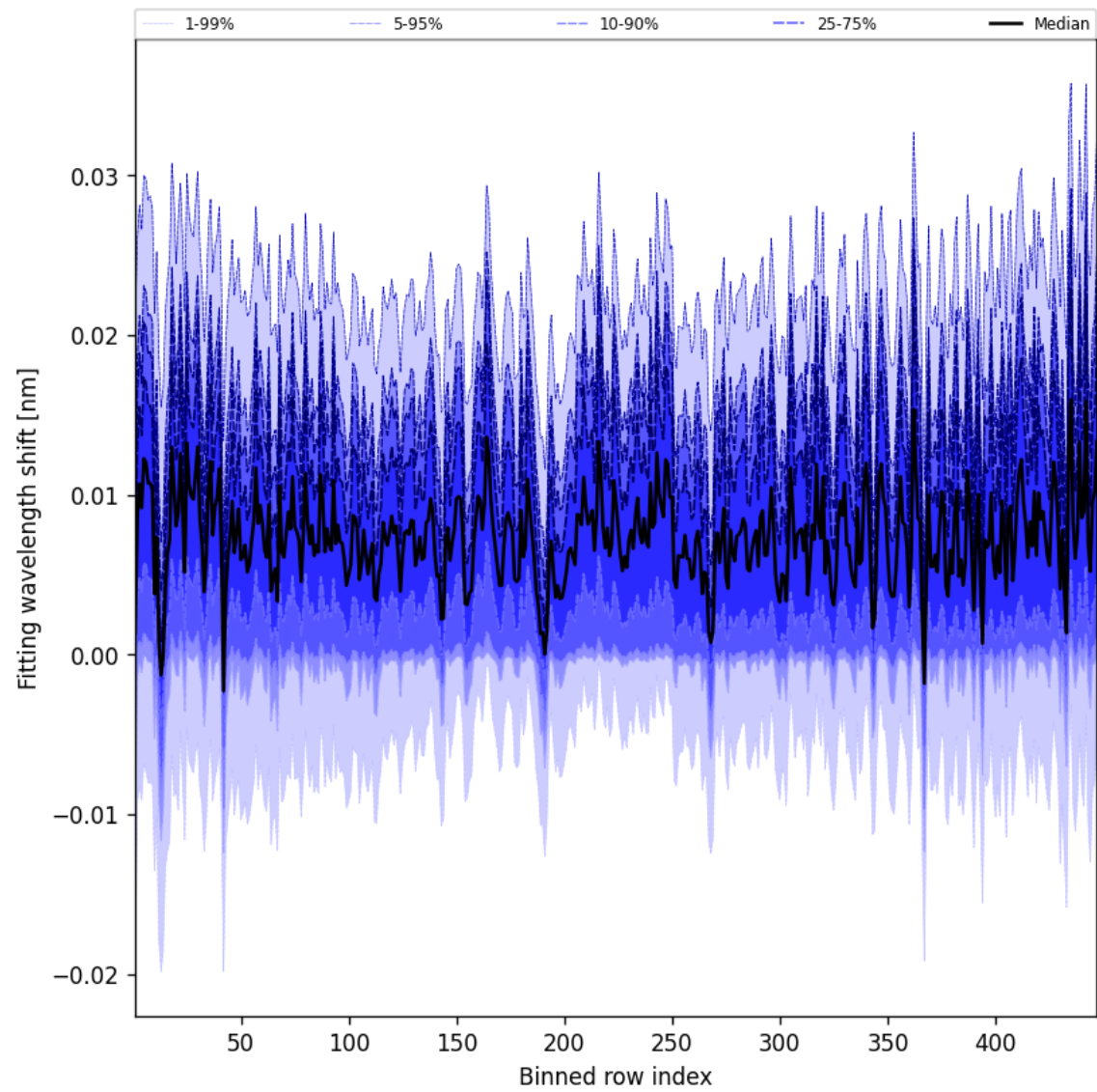
Figure 65: Along track statistics of “Fitting wavelength shift” for 2025-06-24 to 2025-06-26
