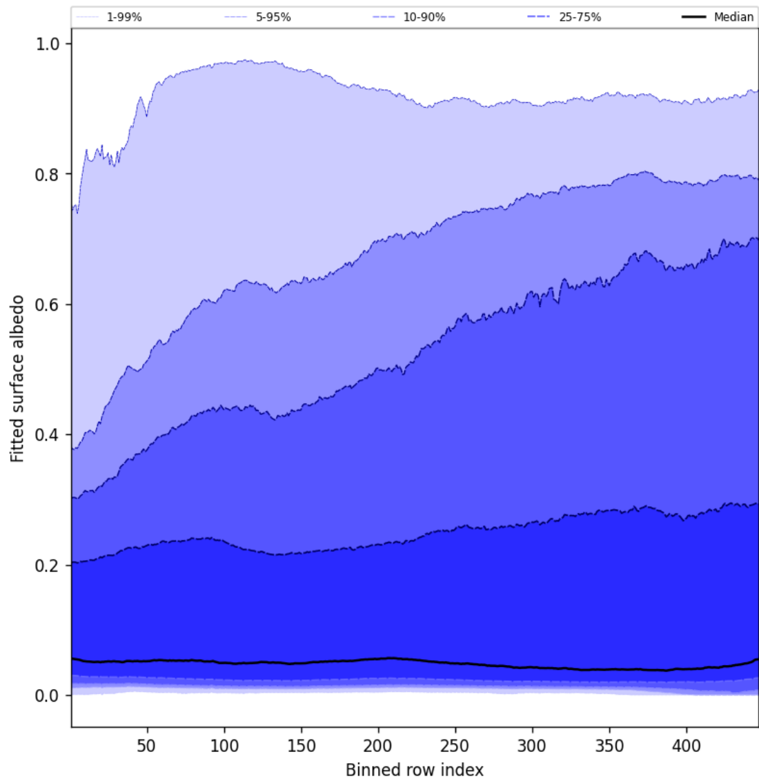
Figure 61: Along track statistics of “Fitted surface albedo” for 2025-06-24 to 2025-06-26
