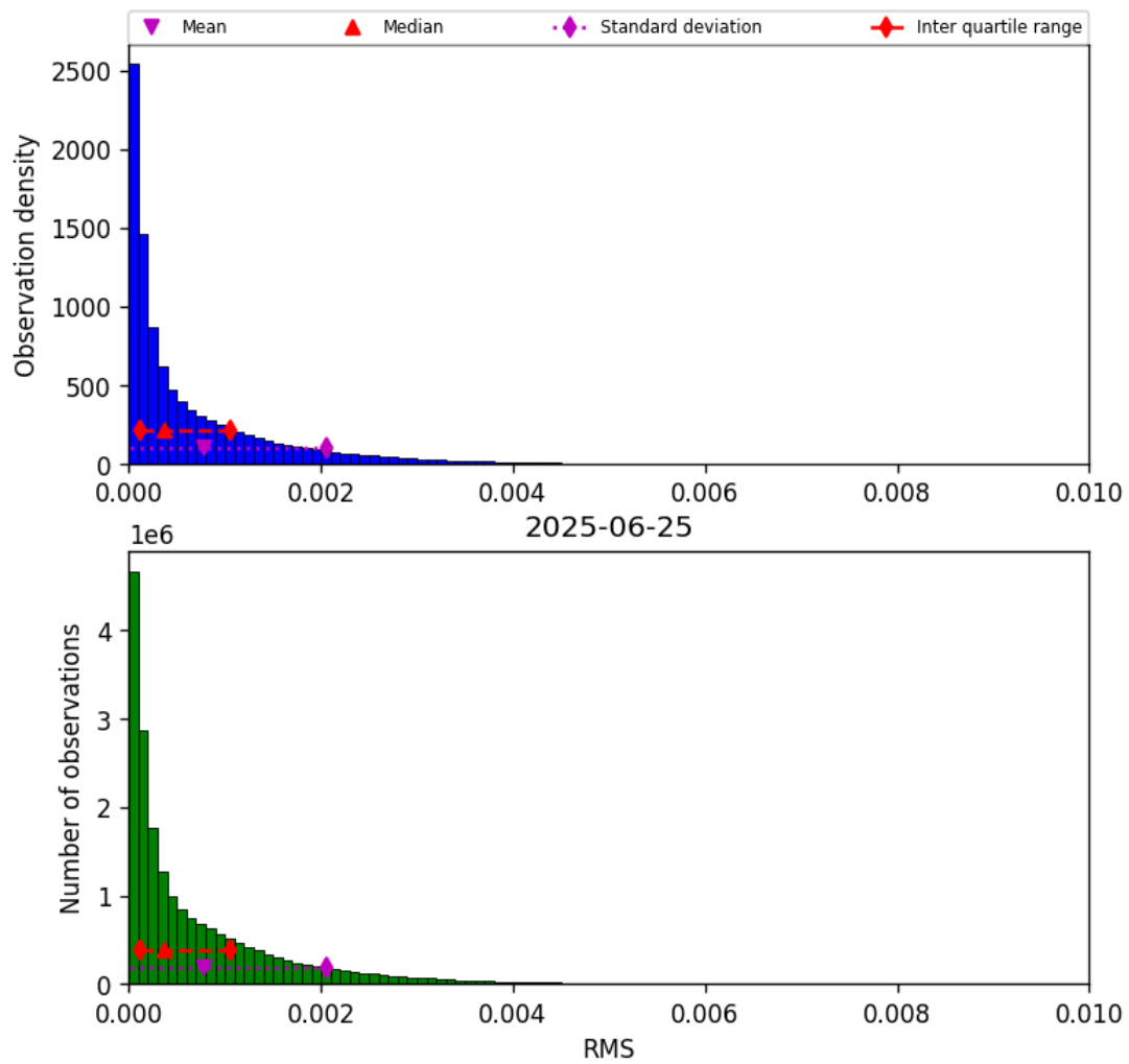
Figure 47: Histogram of “RMS” for 2025-06-24 to 2025-06-26
