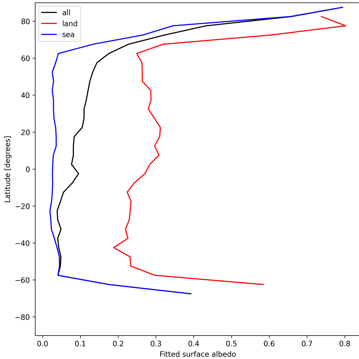
Figure 29: Zonal average of “Fitted surface albedo” for 2025-06-24 to 2025-06-26.
