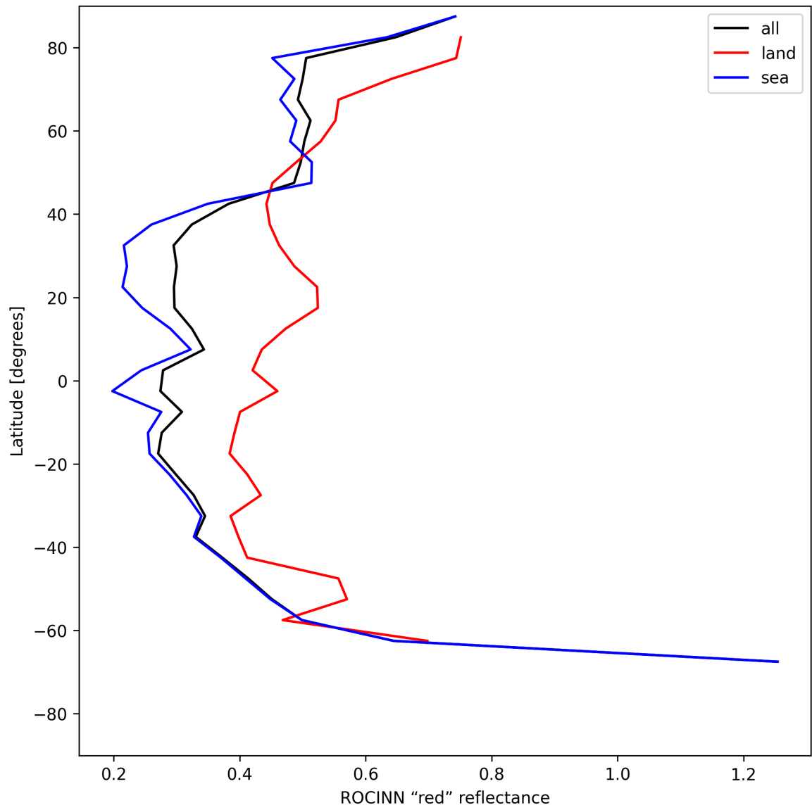
Figure 37: Zonal average of “ROCINN “red” reflectance” for 2025-06-24 to 2025-06-26.
