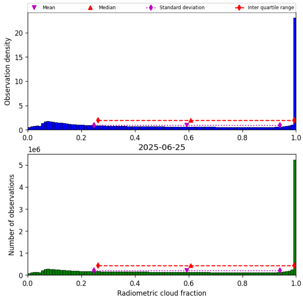
Figure 39: Histogram of “Radiometric cloud fraction” for 2025-06-24 to 2025-06-26
