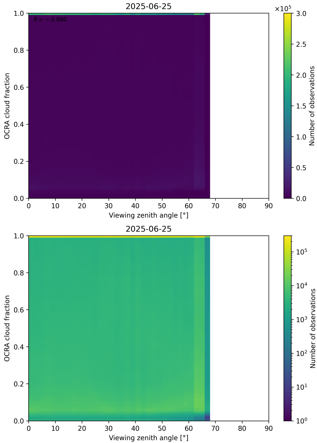
Figure 108: Scatter density plot of “Viewing zenith angle” against “OCRA cloud fraction” for 2025-06-24 to 2025-06-26.
