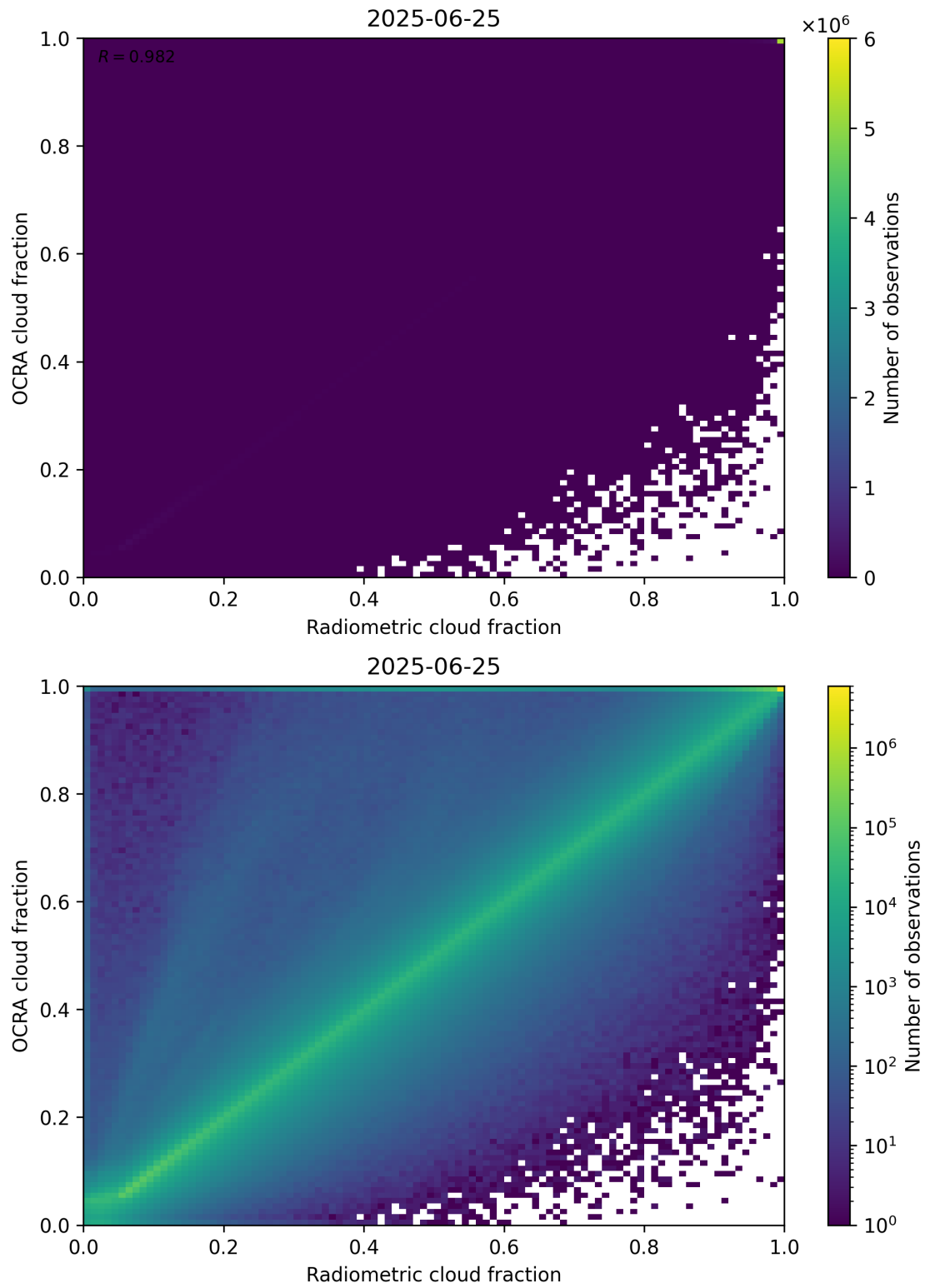
Figure 72: Scatter density plot of “Radiometric cloud fraction” against “OCRA cloud fraction” for 2025-06-24 to 2025-06-26.
