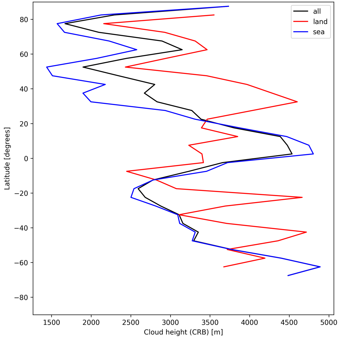
Figure 27: Zonal average of “Cloud height (CRB)” for 2025-06-24 to 2025-06-26.
