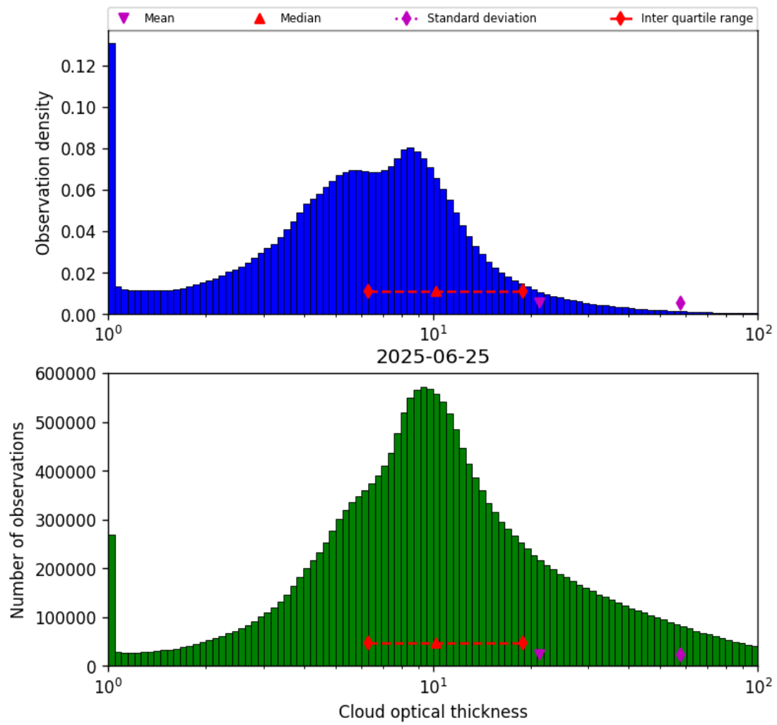
Figure 41: Histogram of “Cloud optical thickness” for 2025-06-24 to 2025-06-26
