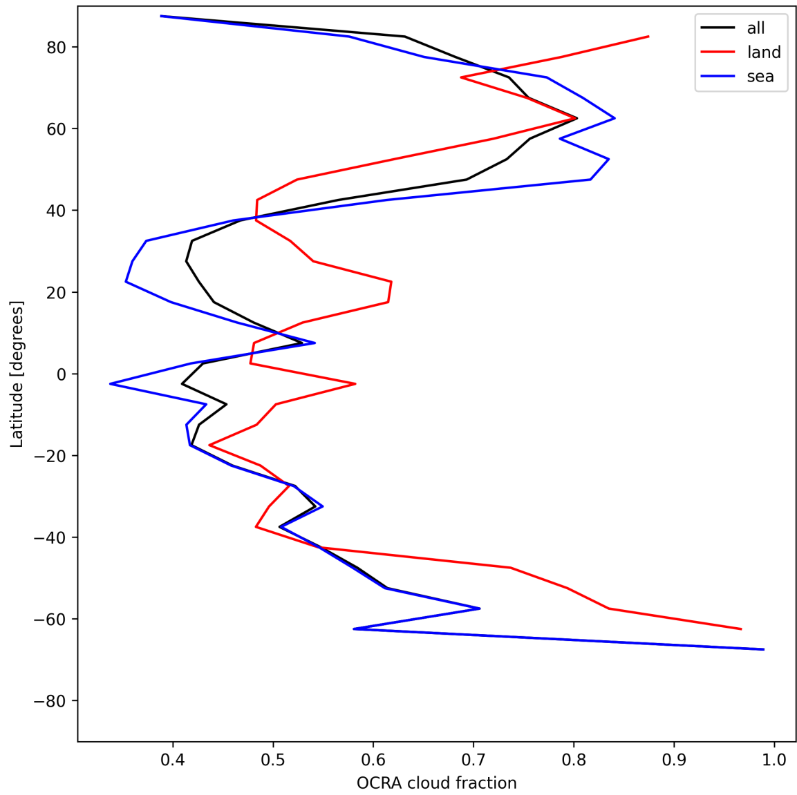
Figure 34: Zonal average of “OCRA cloud fraction” for 2025-06-24 to 2025-06-26.
