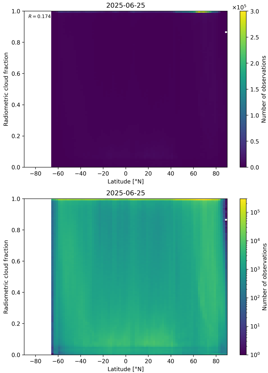
Figure 92: Scatter density plot of “Latitude” against “Radiometric cloud fraction” for 2025-06-24 to 2025-06-26.
