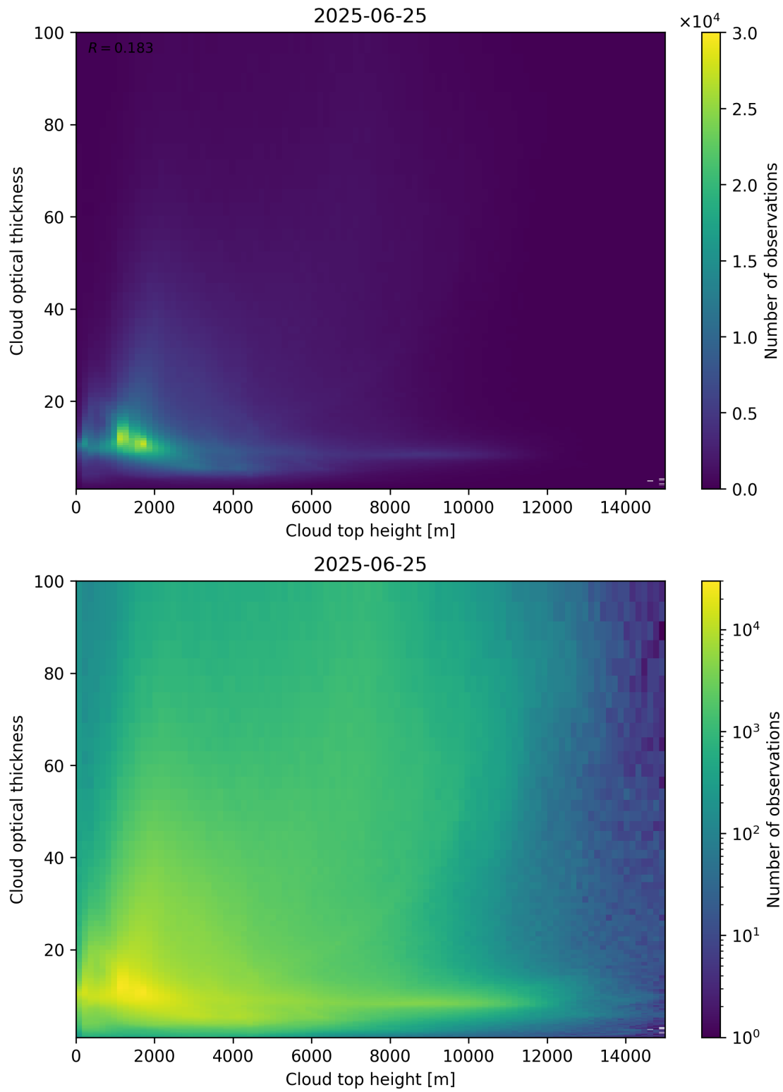
Figure 90: Scatter density plot of “Cloud top height” against “Cloud optical thickness” for 2025-06-24 to 2025-06-26.
