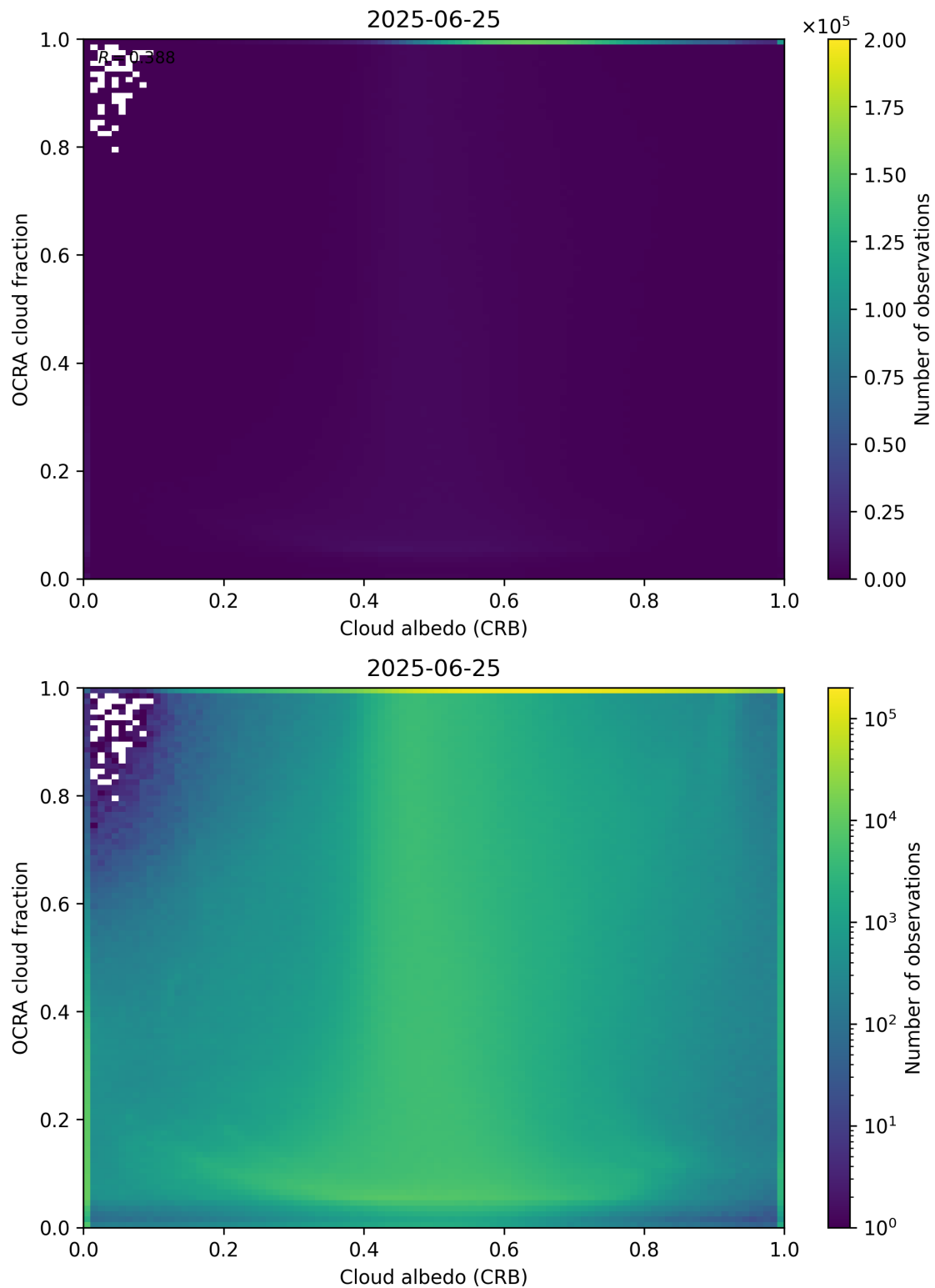
Figure 70: Scatter density plot of “Cloud albedo (CRB)” against “OCRA cloud fraction” for 2025-06-24 to 2025-06-26.
