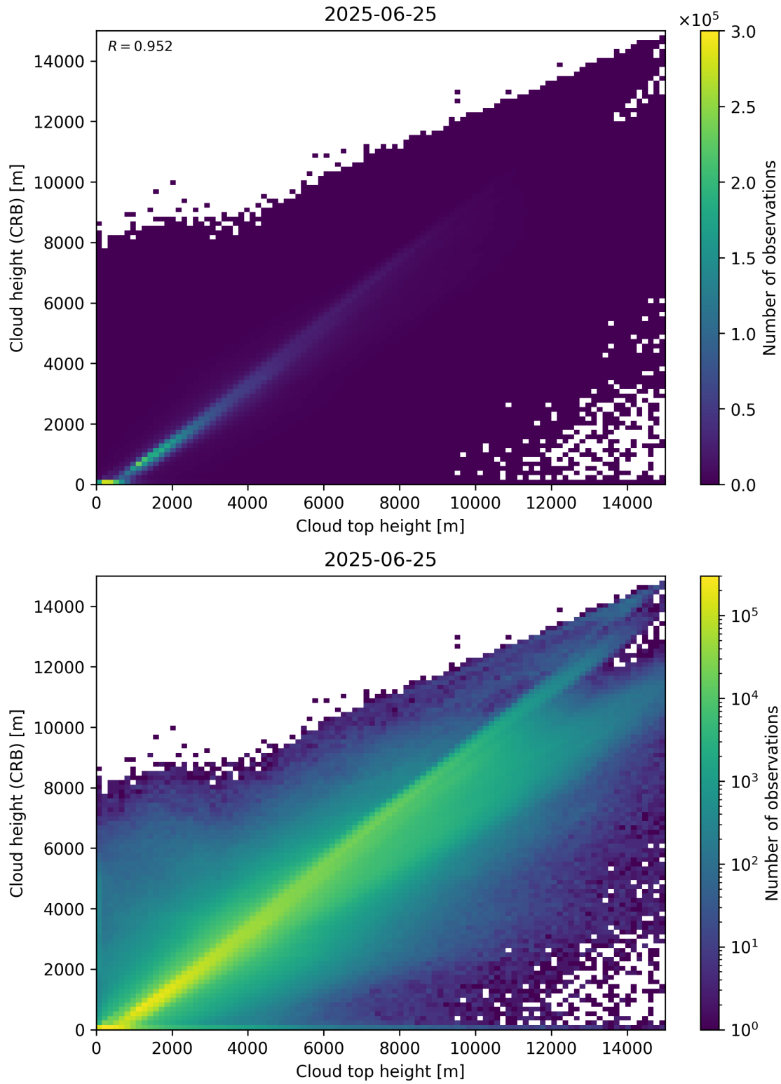
Figure 89: Scatter density plot of “Cloud top height” against “Cloud height (CRB)” for 2025-06-24 to 2025-06-26.
