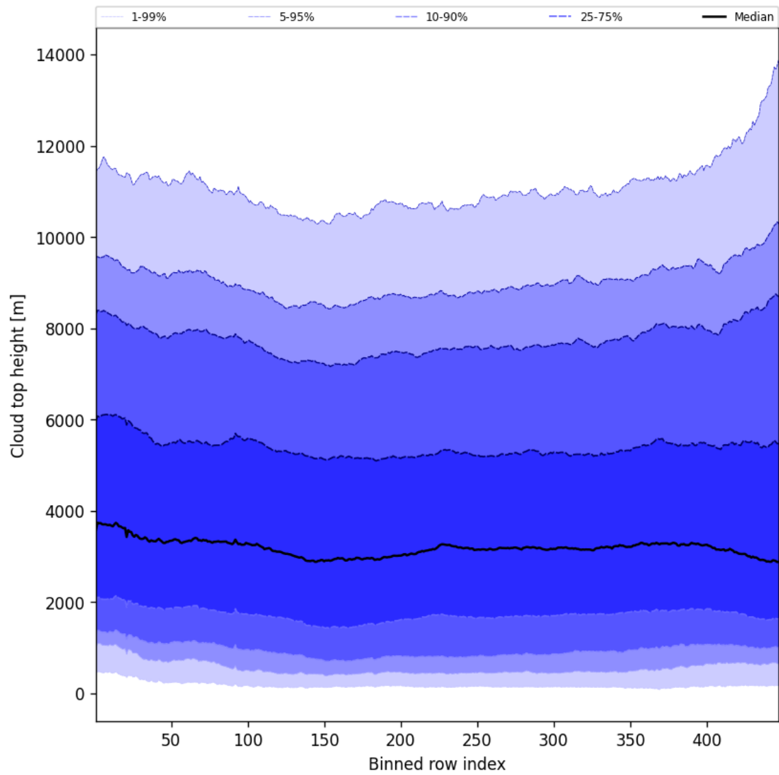
Figure 56: Along track statistics of “Cloud top height” for 2025-06-24 to 2025-06-26
