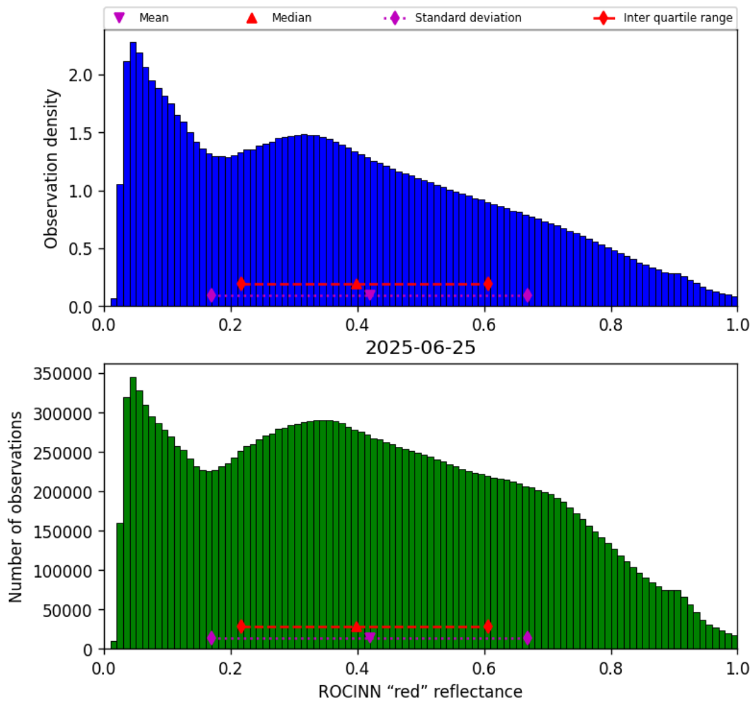
Figure 53: Histogram of “ROCINN “red” reflectance” for 2025-06-24 to 2025-06-26
