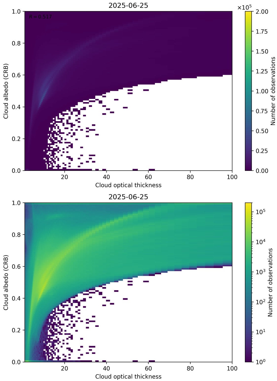
Figure 82: Scatter density plot of “Cloud optical thickness” against “Cloud albedo (CRB)” for 2025-06-24 to 2025-06-26.
