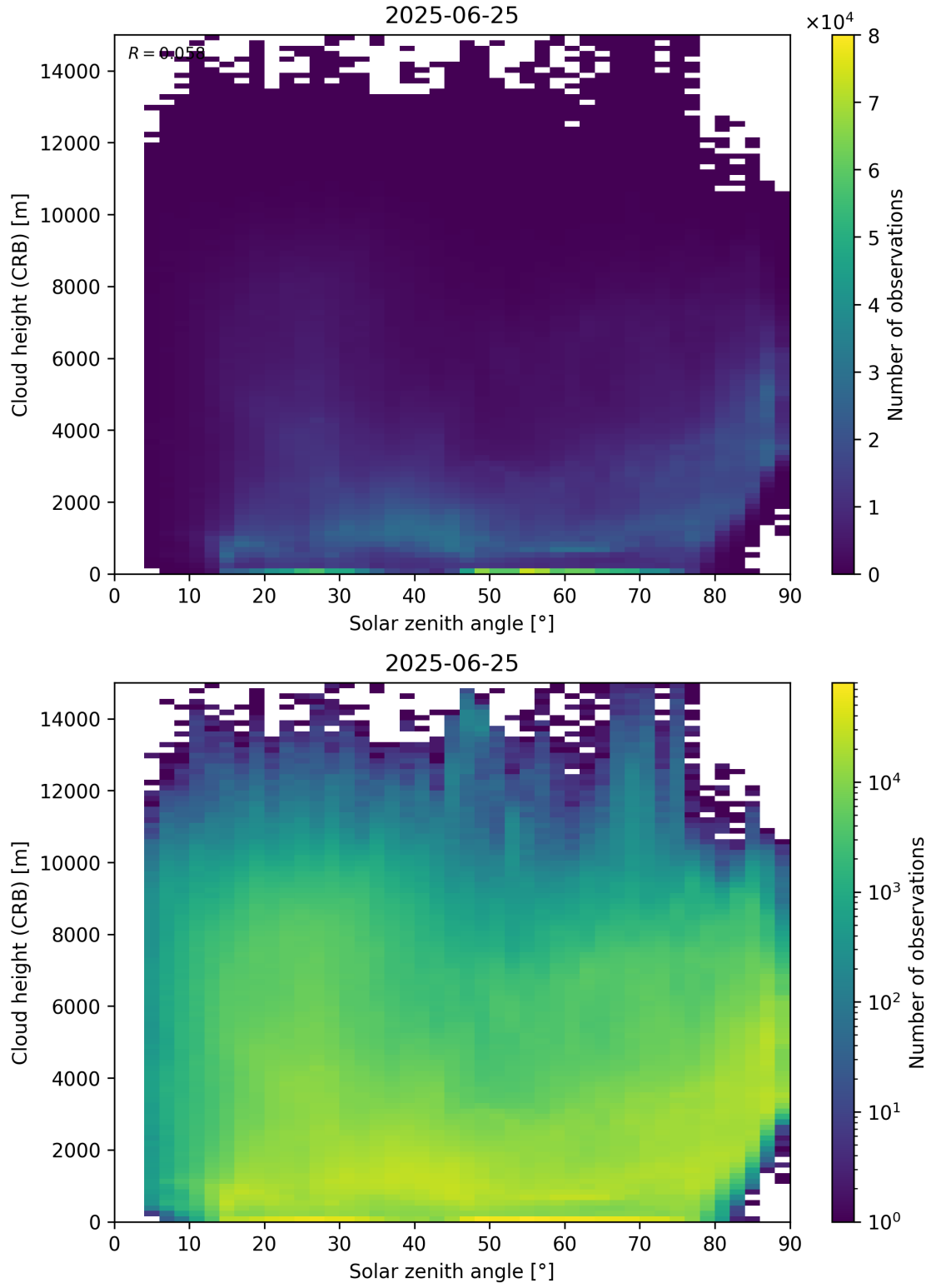
Figure 102: Scatter density plot of “Solar zenith angle” against “Cloud height (CRB)” for 2025-06-24 to 2025-06-26.
