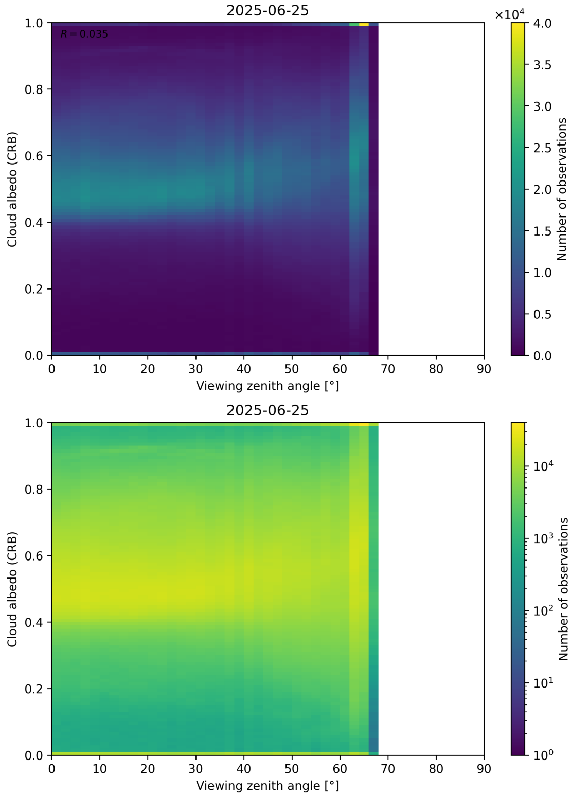
Figure 106: Scatter density plot of “Viewing zenith angle” against “Cloud albedo (CRB)” for 2025-06-24 to 2025-06-26.
