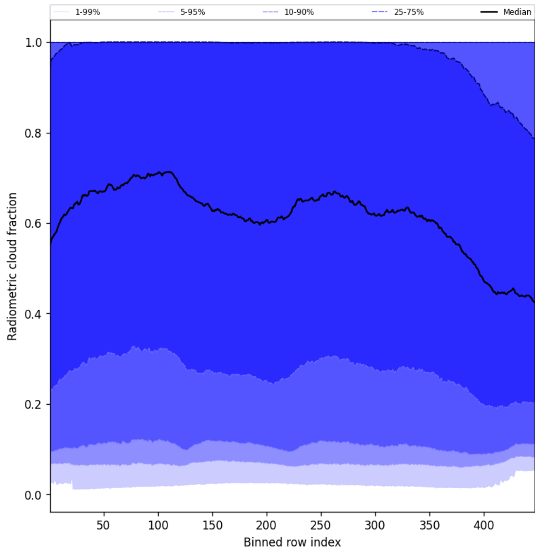
Figure 55: Along track statistics of “Radiometric cloud fraction” for 2025-06-24 to 2025-06-26
