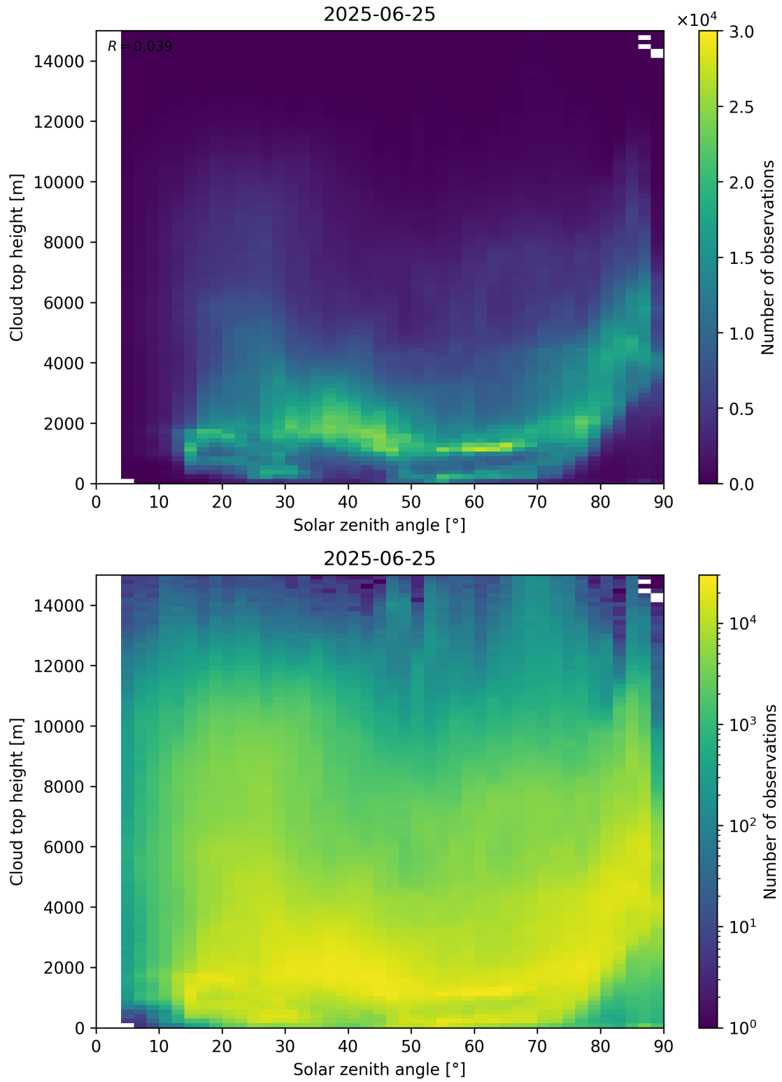
Figure 104: Scatter density plot of “Solar zenith angle” against “Cloud top height” for 2025-06-24 to 2025-06-26.
