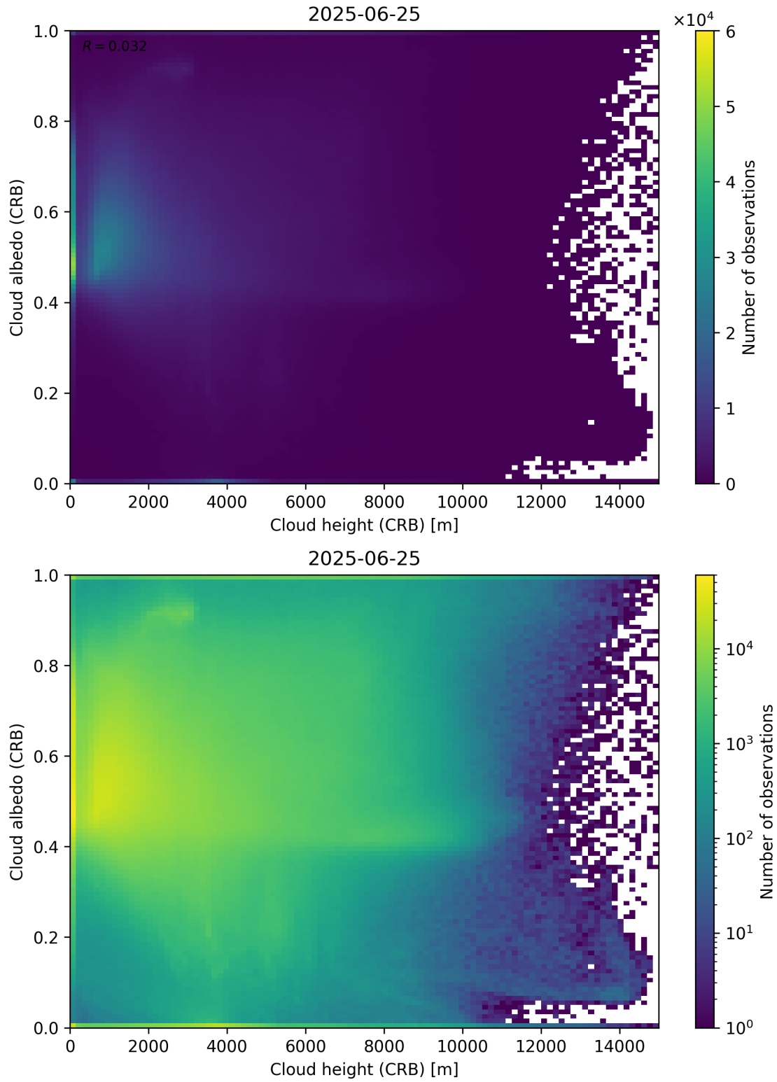
Figure 80: Scatter density plot of “Cloud height (CRB)” against “Cloud albedo (CRB)” for 2025-06-24 to 2025-06-26.
