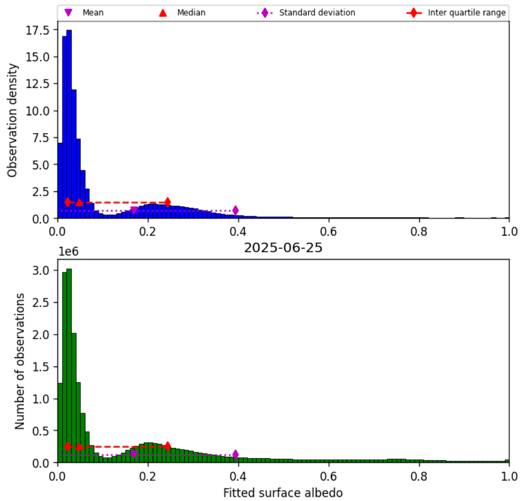
Figure 45: Histogram of “Fitted surface albedo” for 2025-06-24 to 2025-06-26
