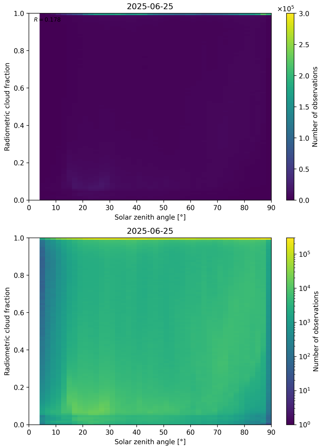
Figure 99: Scatter density plot of “Solar zenith angle” against “Radiometric cloud fraction” for 2025-06-24 to 2025-06-26.
