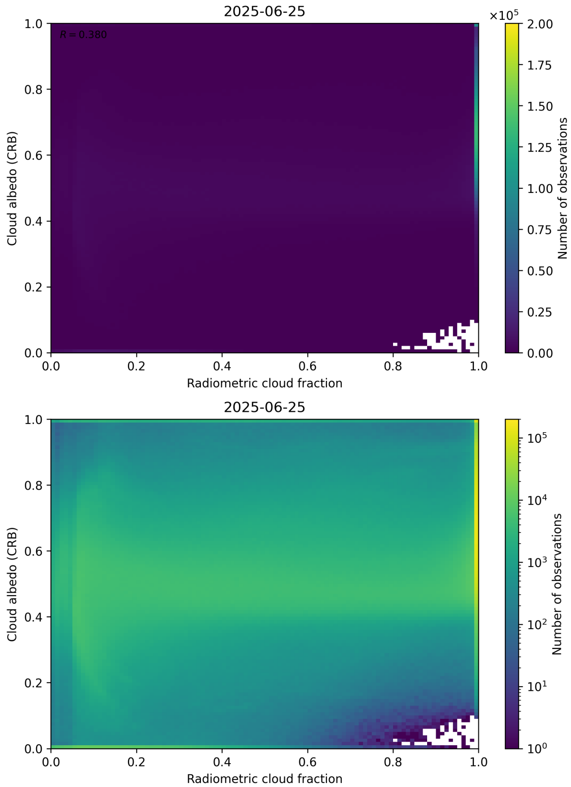
Figure 71: Scatter density plot of “Radiometric cloud fraction” against “Cloud albedo (CRB)” for 2025-06-24 to 2025-06-26.
