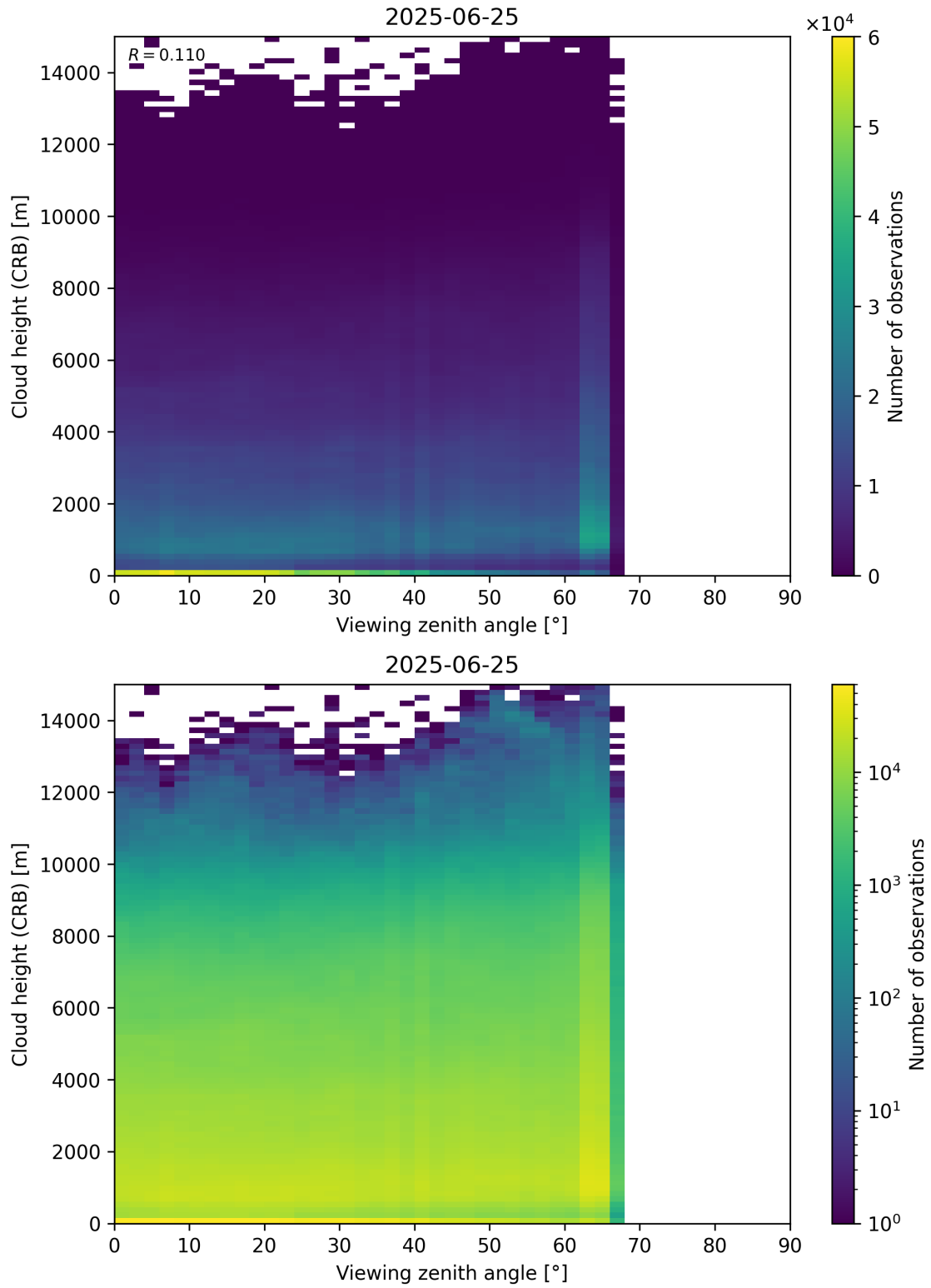
Figure 110: Scatter density plot of “Viewing zenith angle” against “Cloud height (CRB)” for 2025-06-24 to 2025-06-26.
