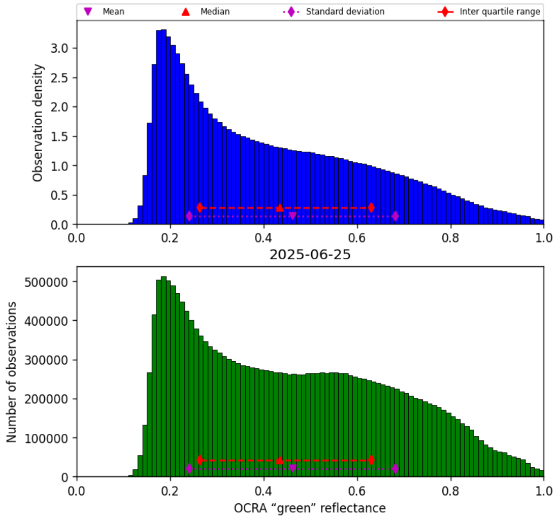
Figure 52: Histogram of “OCRA “green” reflectance” for 2025-06-24 to 2025-06-26
