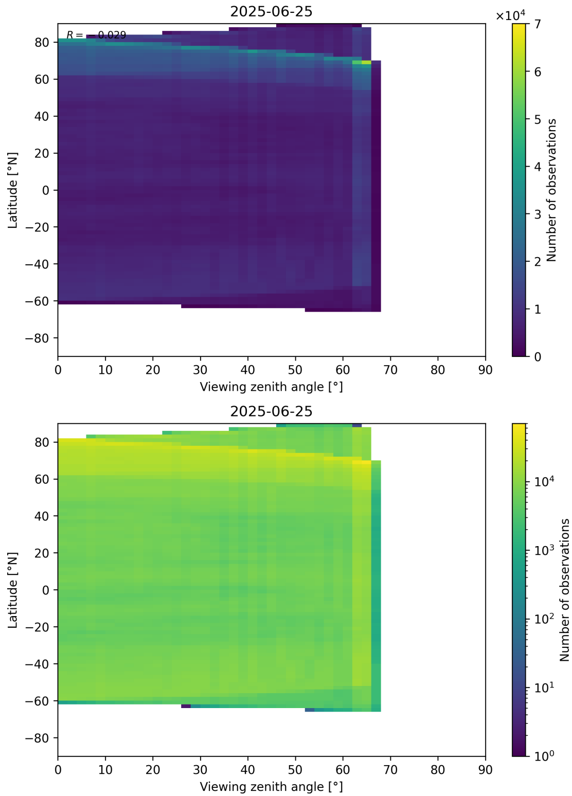
Figure 113: Scatter density plot of “Viewing zenith angle” against “Latitude” for 2025-06-24 to 2025-06-26.
