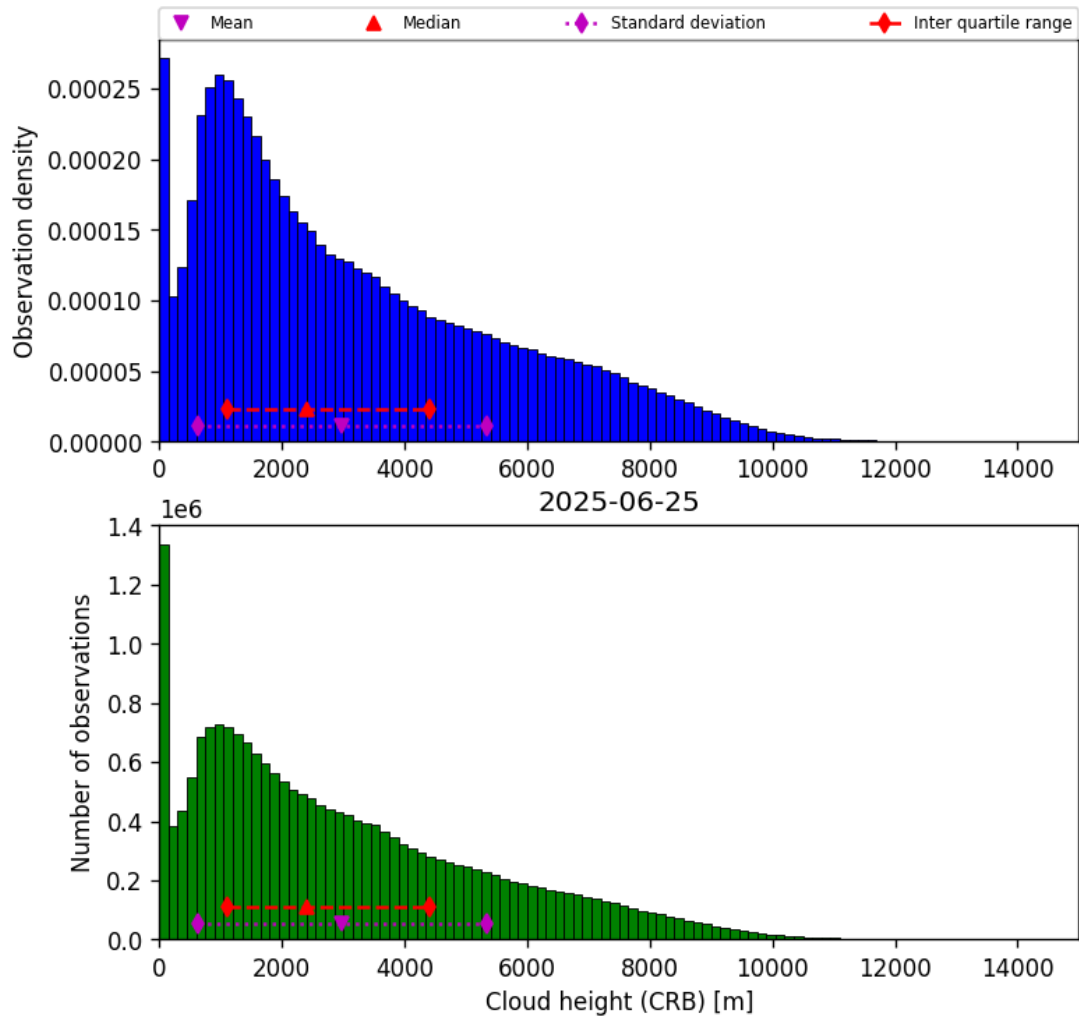
Figure 43: Histogram of “Cloud height (CRB)” for 2025-06-24 to 2025-06-26
