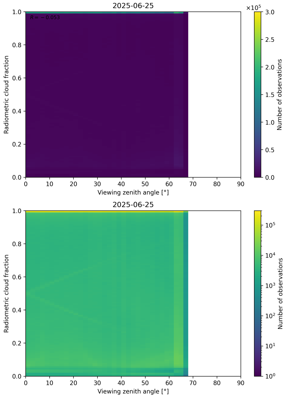
Figure 107: Scatter density plot of “Viewing zenith angle” against “Radiometric cloud fraction” for 2025-06-24 to 2025-06-26.
