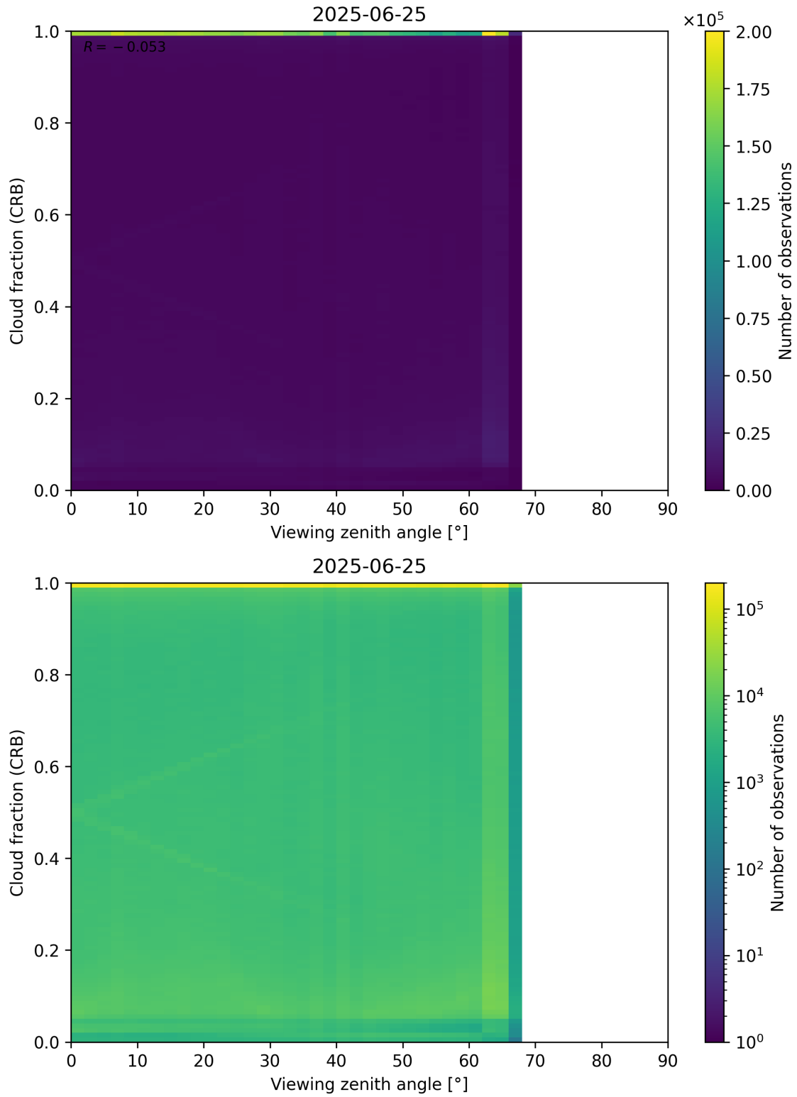
Figure 109: Scatter density plot of “Viewing zenith angle” against “Cloud fraction (CRB)” for 2025-06-24 to 2025-06-26.
