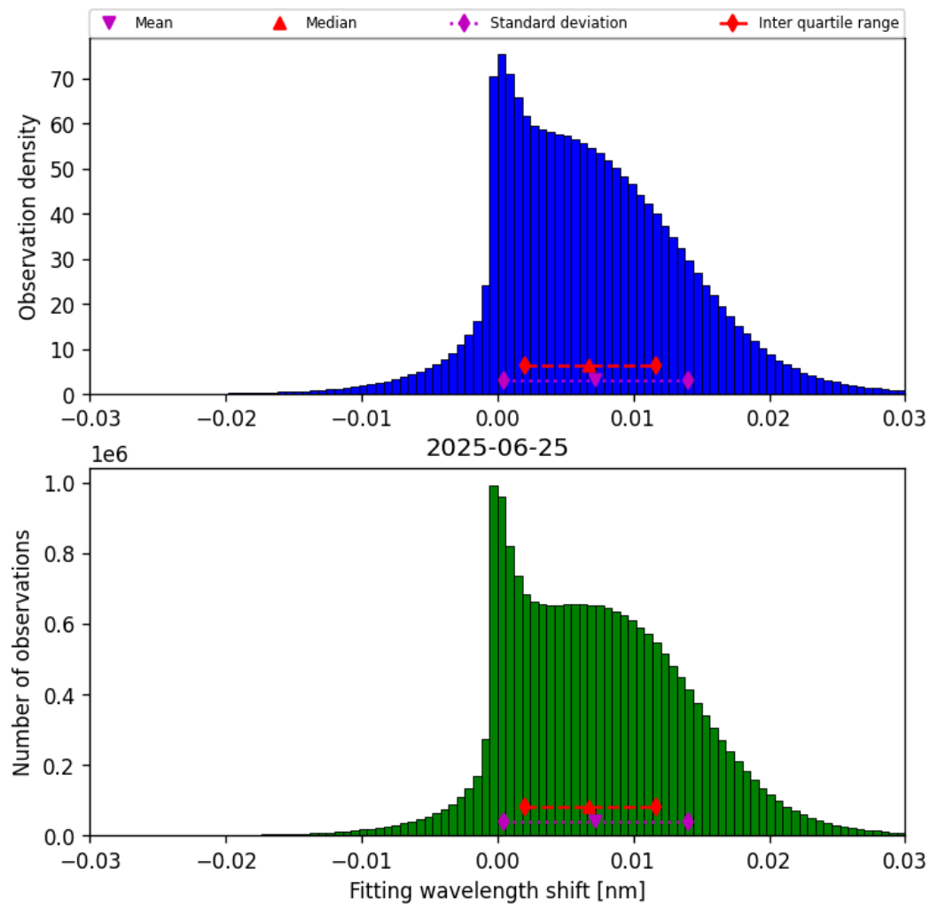
Figure 49: Histogram of “Fitting wavelength shift” for 2025-06-24 to 2025-06-26
