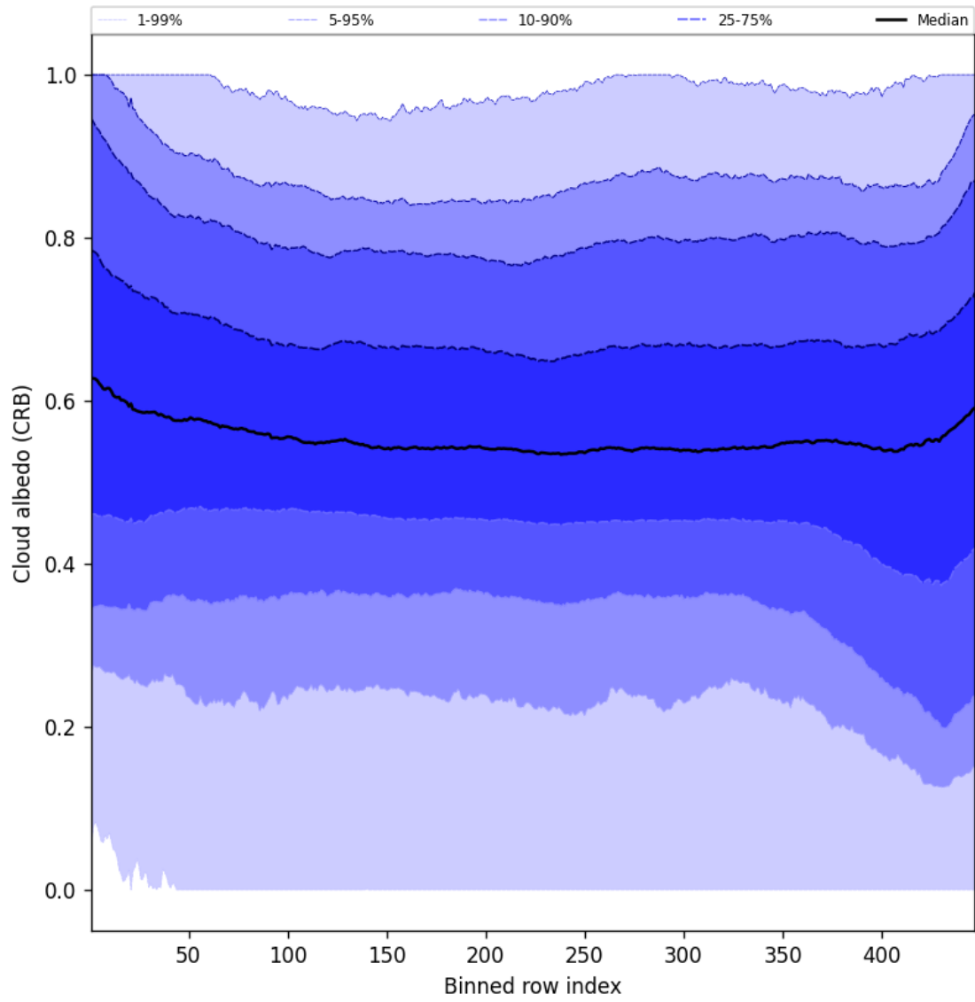
Figure 60: Along track statistics of “Cloud albedo (CRB)” for 2025-06-24 to 2025-06-26
