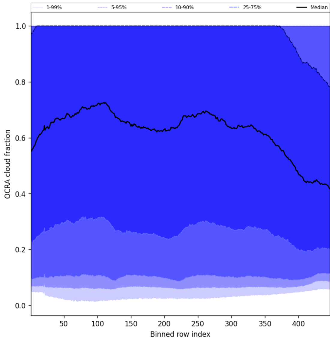
Figure 66: Along track statistics of “OCRA cloud fraction” for 2025-06-24 to 2025-06-26
