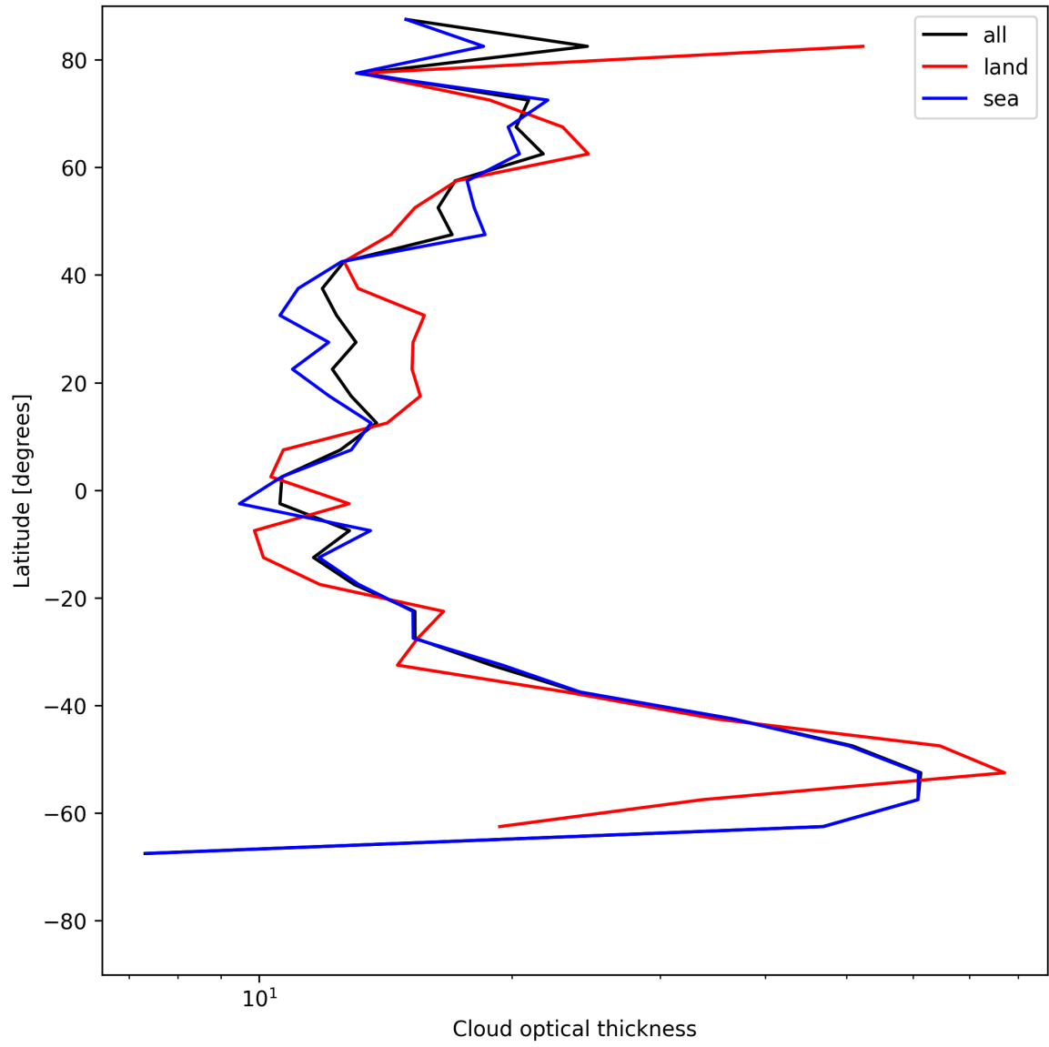
Figure 25: Zonal average of “Cloud optical thickness” for 2025-06-24 to 2025-06-26.
