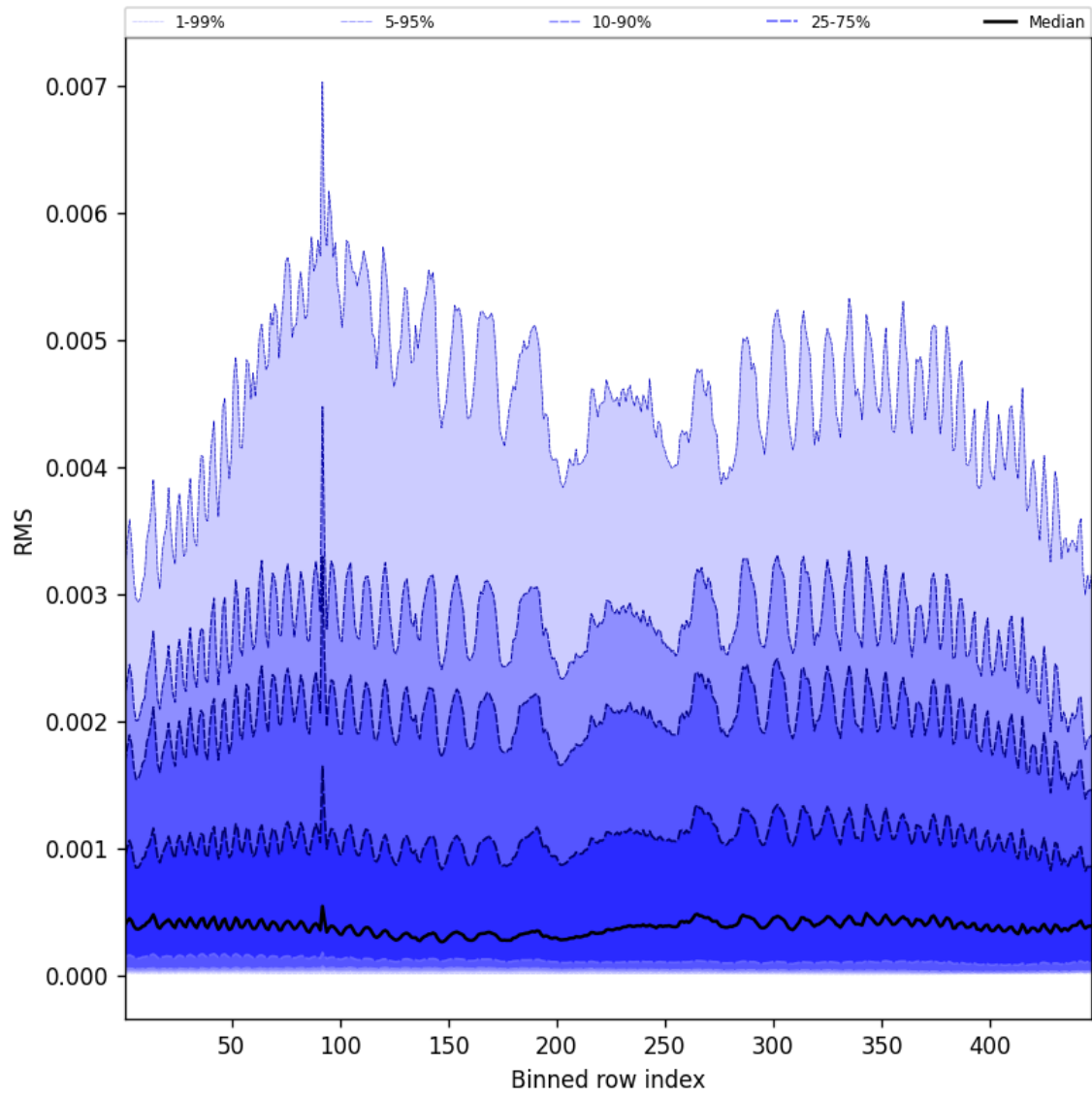
Figure 63: Along track statistics of “RMS” for 2025-06-24 to 2025-06-26
