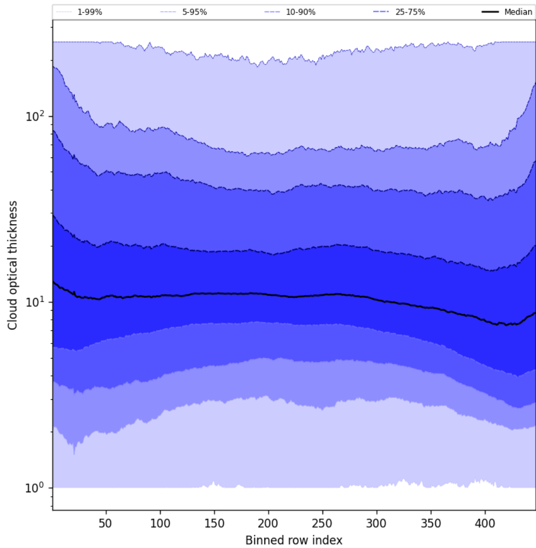
Figure 57: Along track statistics of “Cloud optical thickness” for 2025-06-24 to 2025-06-26
