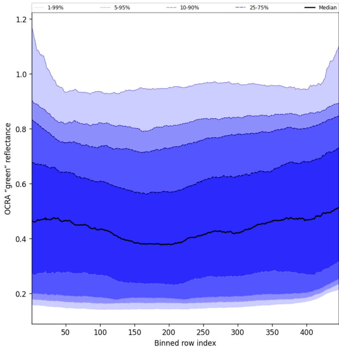
Figure 68: Along track statistics of “OCRA “green” reflectance” for 2025-06-24 to 2025-06-26
