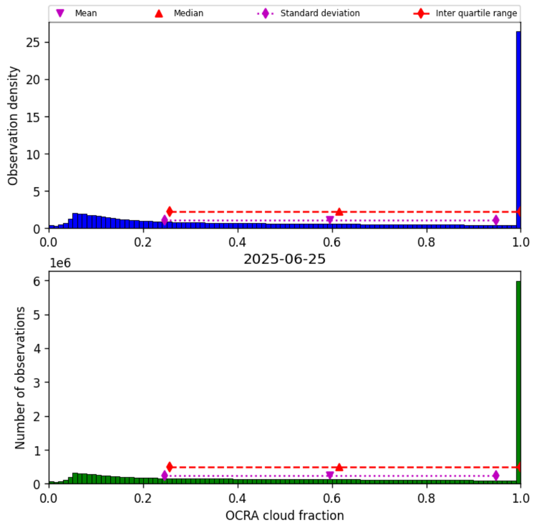
Figure 50: Histogram of “OCRA cloud fraction” for 2025-06-24 to 2025-06-26
