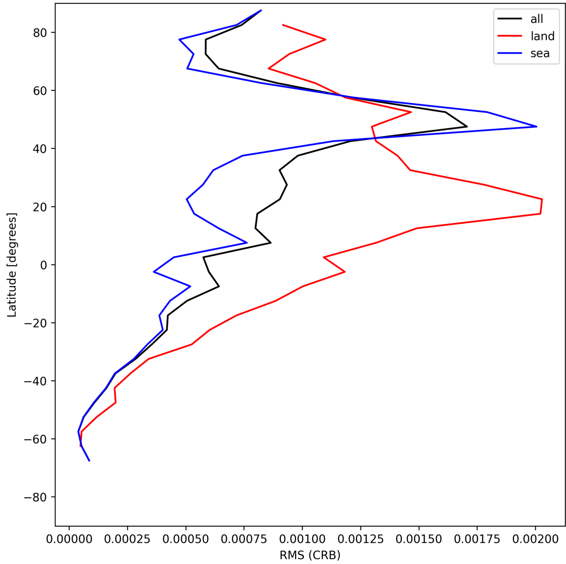
Figure 32: Zonal average of “RMS (CRB)” for 2025-06-24 to 2025-06-26.
