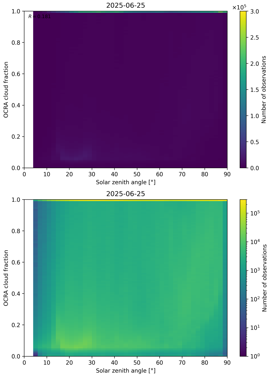
Figure 100: Scatter density plot of “Solar zenith angle” against “OCRA cloud fraction” for 2025-06-24 to 2025-06-26.
