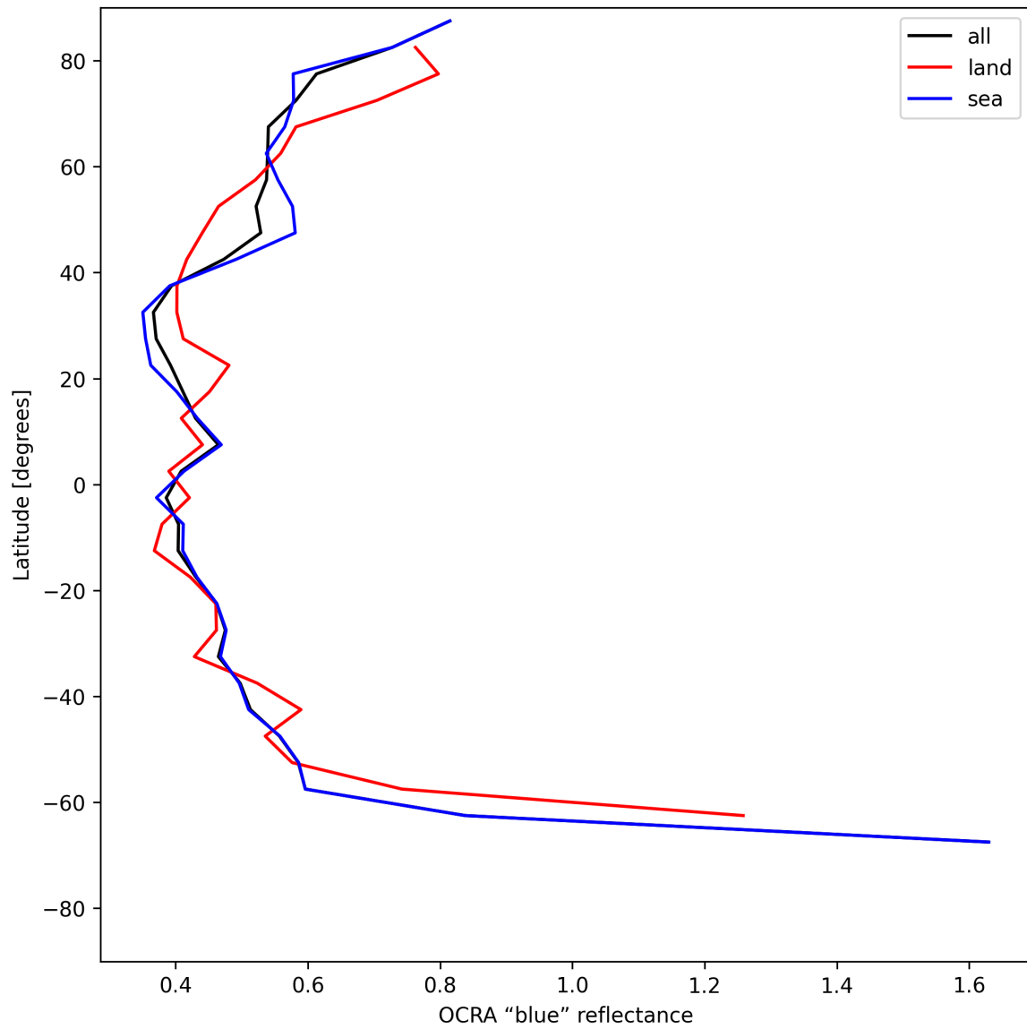
Figure 35: Zonal average of “OCRA “blue” reflectance” for 2025-06-25 to 2025-06-27.
