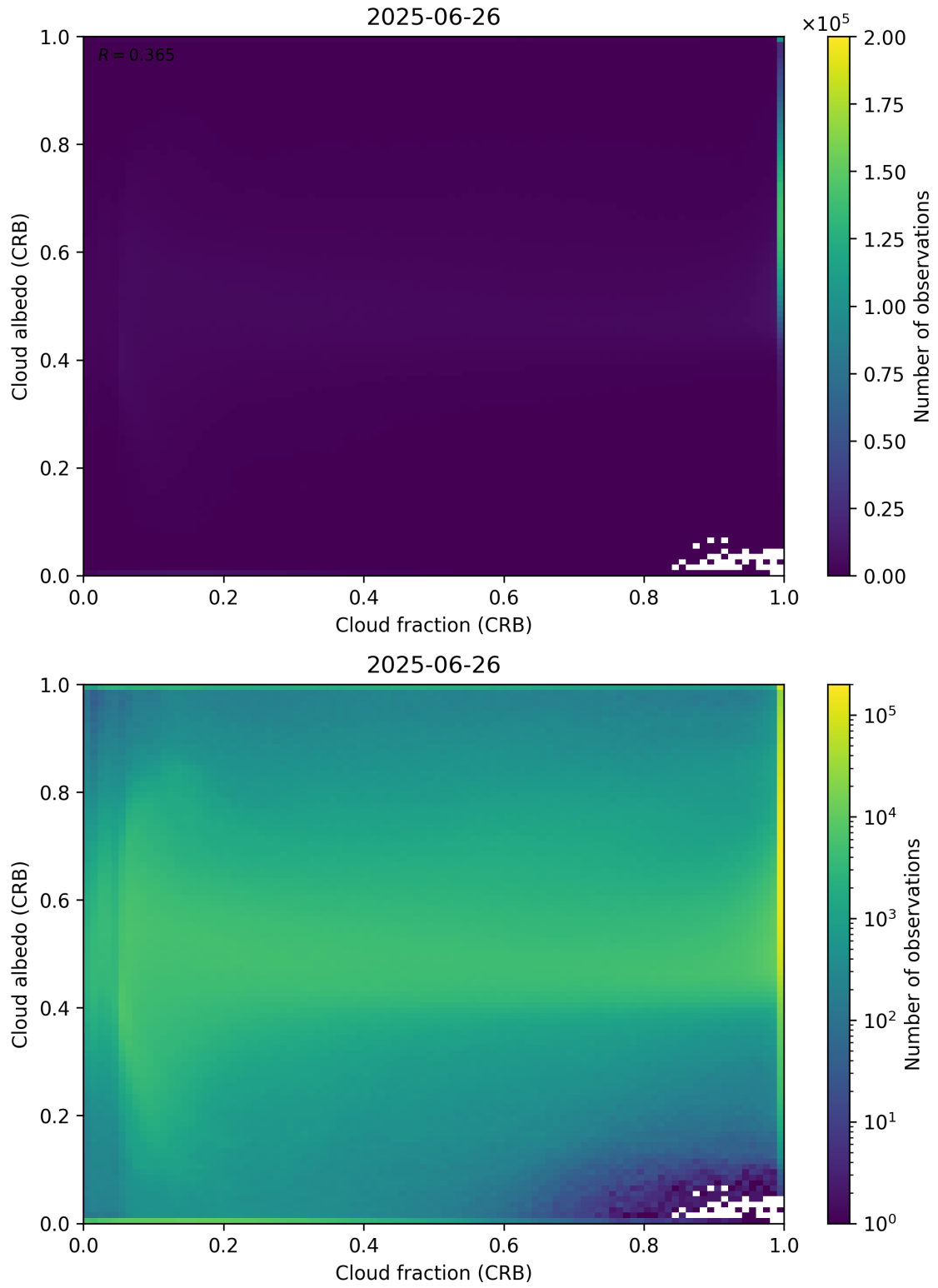
Figure 77: Scatter density plot of “Cloud fraction (CRB)” against “Cloud albedo (CRB)” for 2025-06-25 to 2025-06-27.
