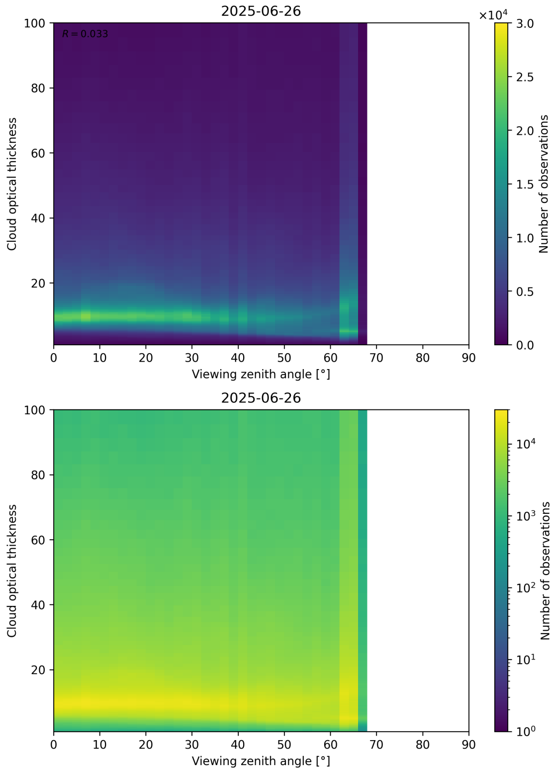
Figure 111: Scatter density plot of “Viewing zenith angle” against “Cloud optical thickness” for 2025-06-25 to 2025-06-27.
