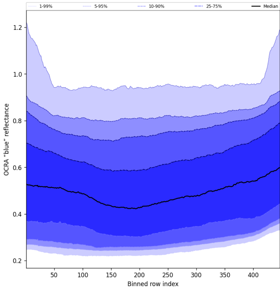
Figure 67: Along track statistics of “OCRA “blue” reflectance” for 2025-06-25 to 2025-06-27
