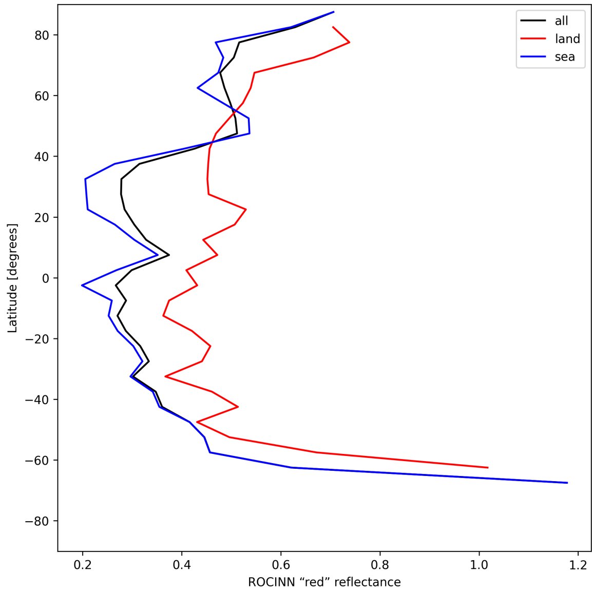
Figure 37: Zonal average of “ROCINN “red” reflectance” for 2025-06-25 to 2025-06-27.
