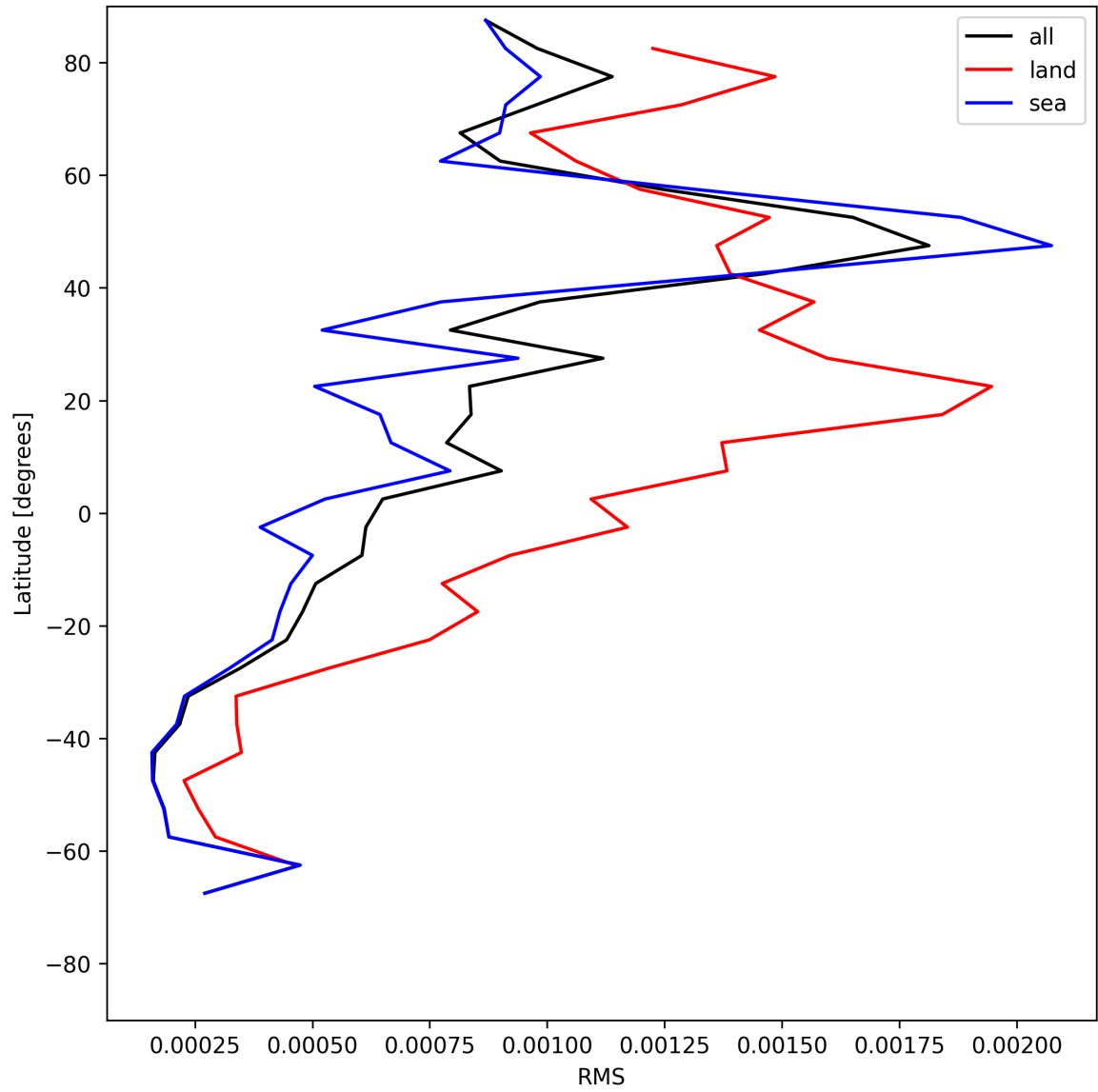
Figure 31: Zonal average of “RMS” for 2025-06-25 to 2025-06-27.
