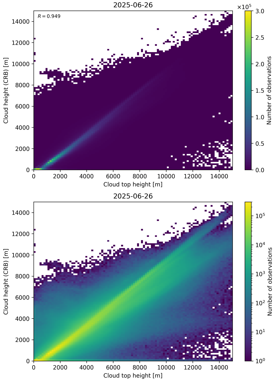
Figure 89: Scatter density plot of “Cloud top height” against “Cloud height (CRB)” for 2025-06-25 to 2025-06-27.
