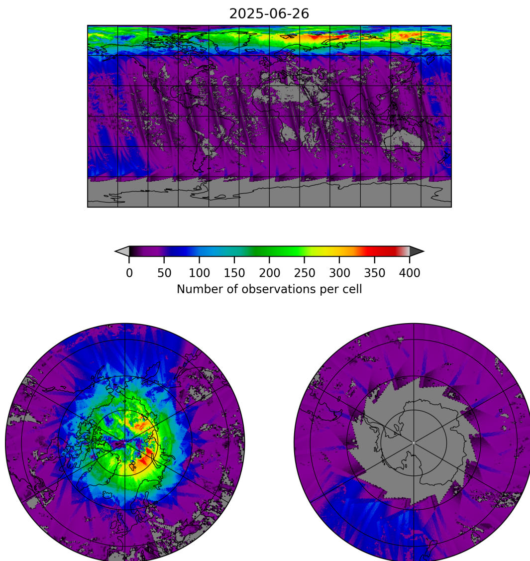
Figure 21: Map of the number of observations for 2025-06-25 to 2025-06-27
