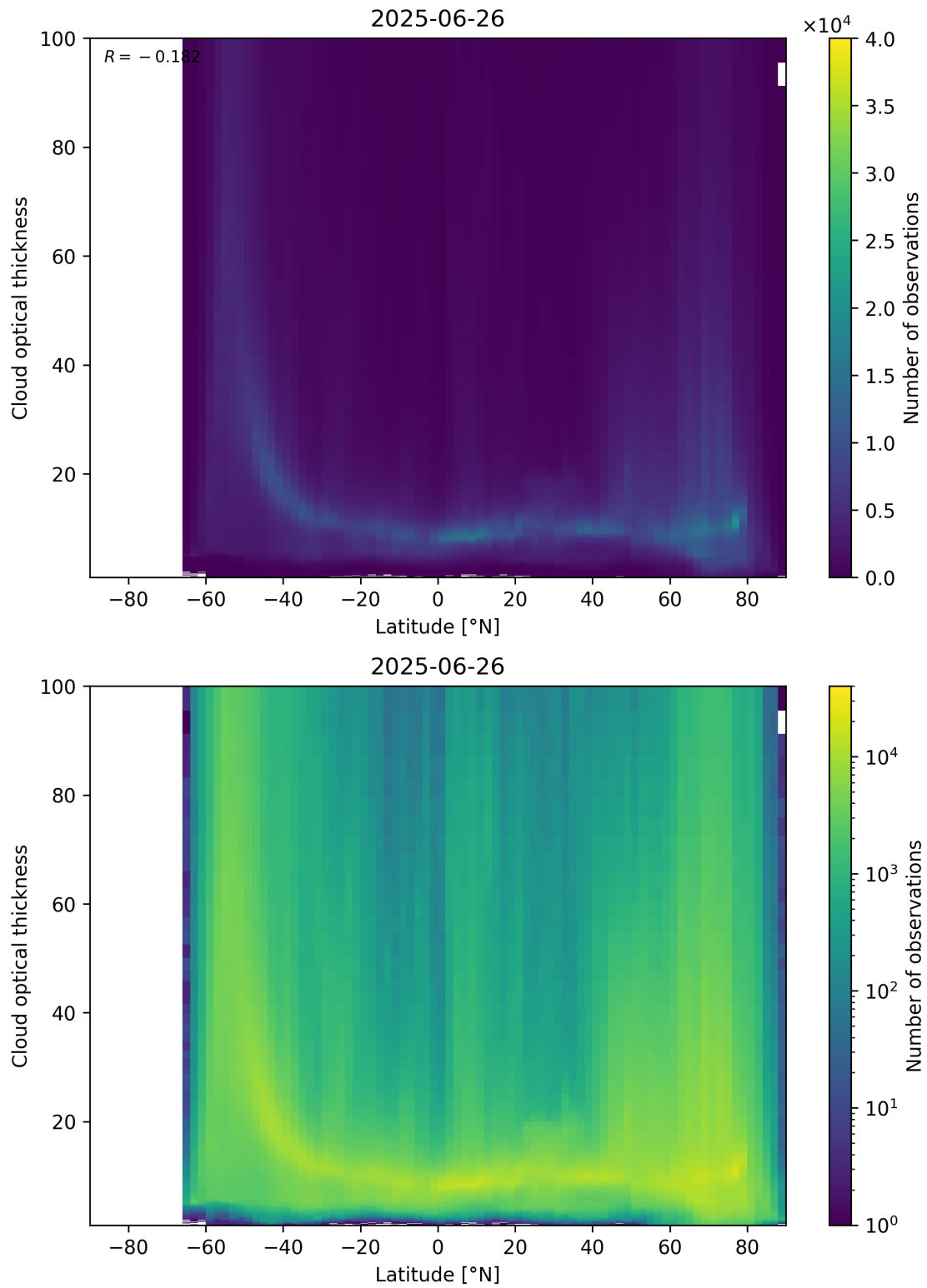
Figure 96: Scatter density plot of “Latitude” against “Cloud optical thickness” for 2025-06-25 to 2025-06-27.
