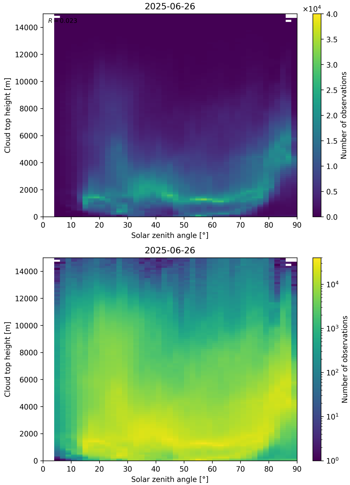
Figure 104: Scatter density plot of “Solar zenith angle” against “Cloud top height” for 2025-06-25 to 2025-06-27.
