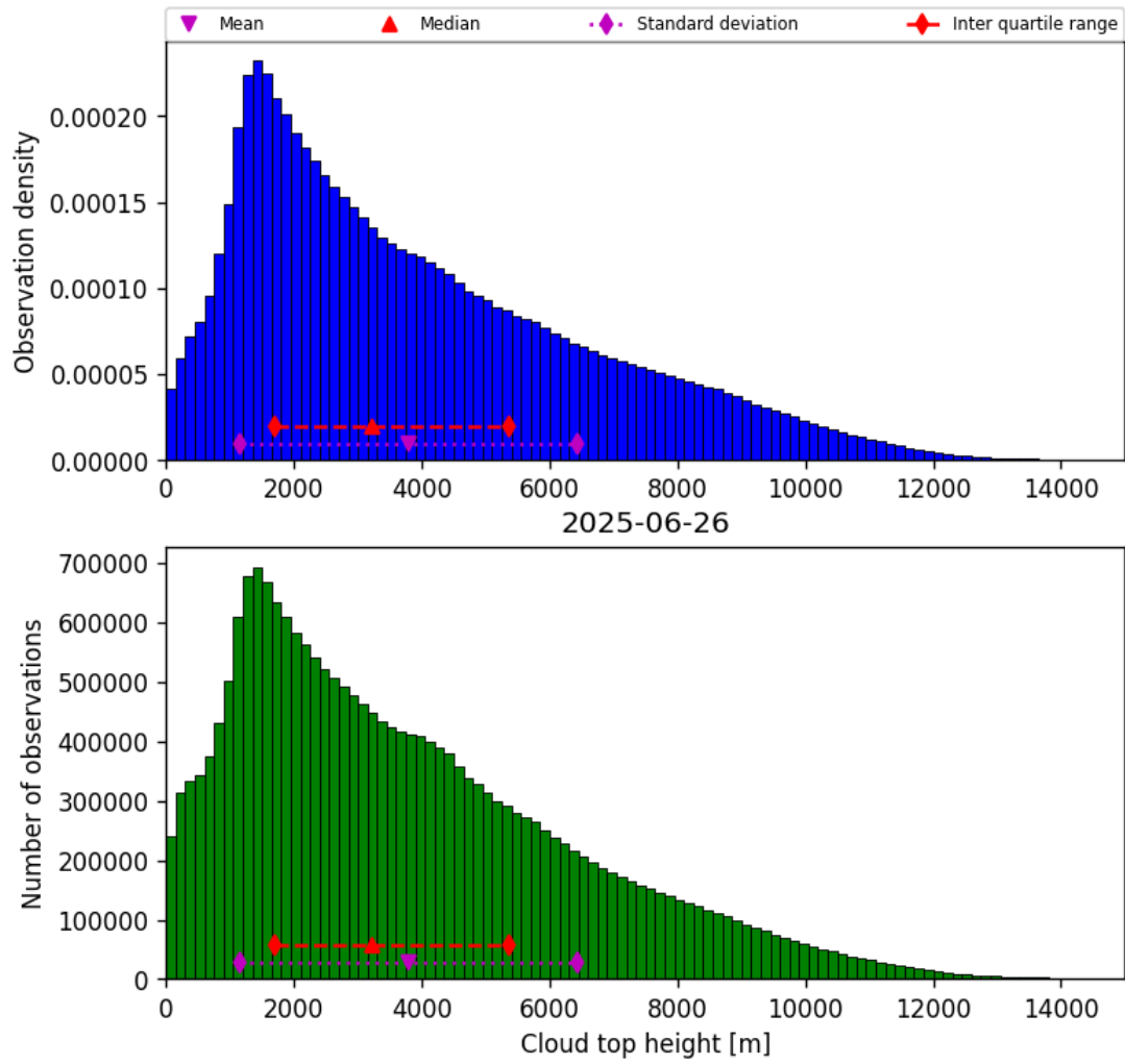
Figure 40: Histogram of “Cloud top height” for 2025-06-25 to 2025-06-27
