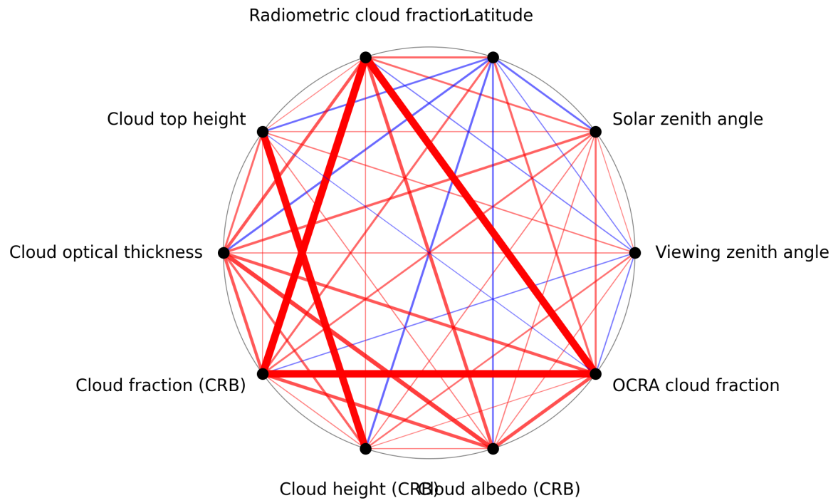
Figure 1: Map of correlation graph for 2025-06-25 to 2025-06-27.
