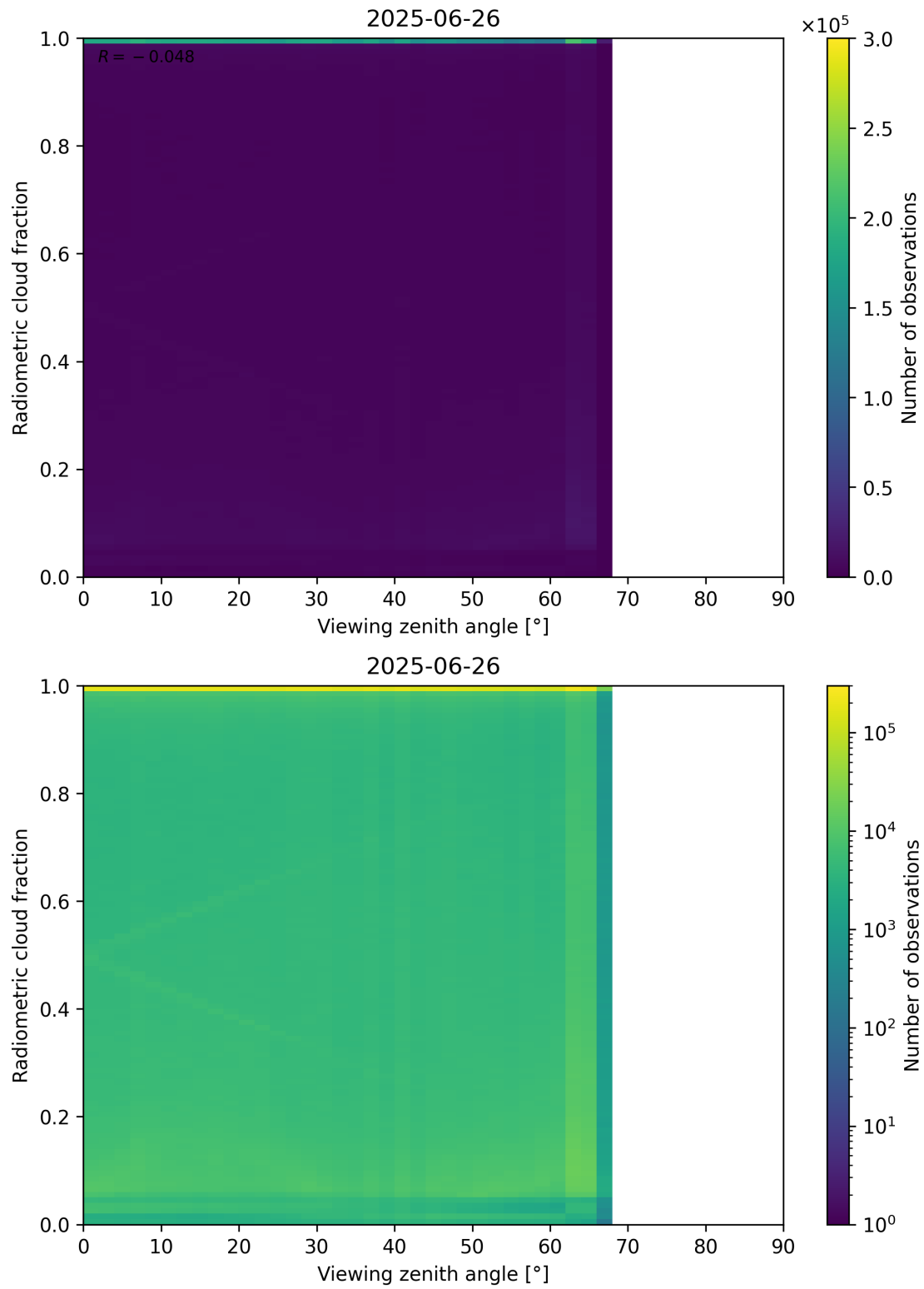
Figure 107: Scatter density plot of “Viewing zenith angle” against “Radiometric cloud fraction” for 2025-06-25 to 2025-06-27.
