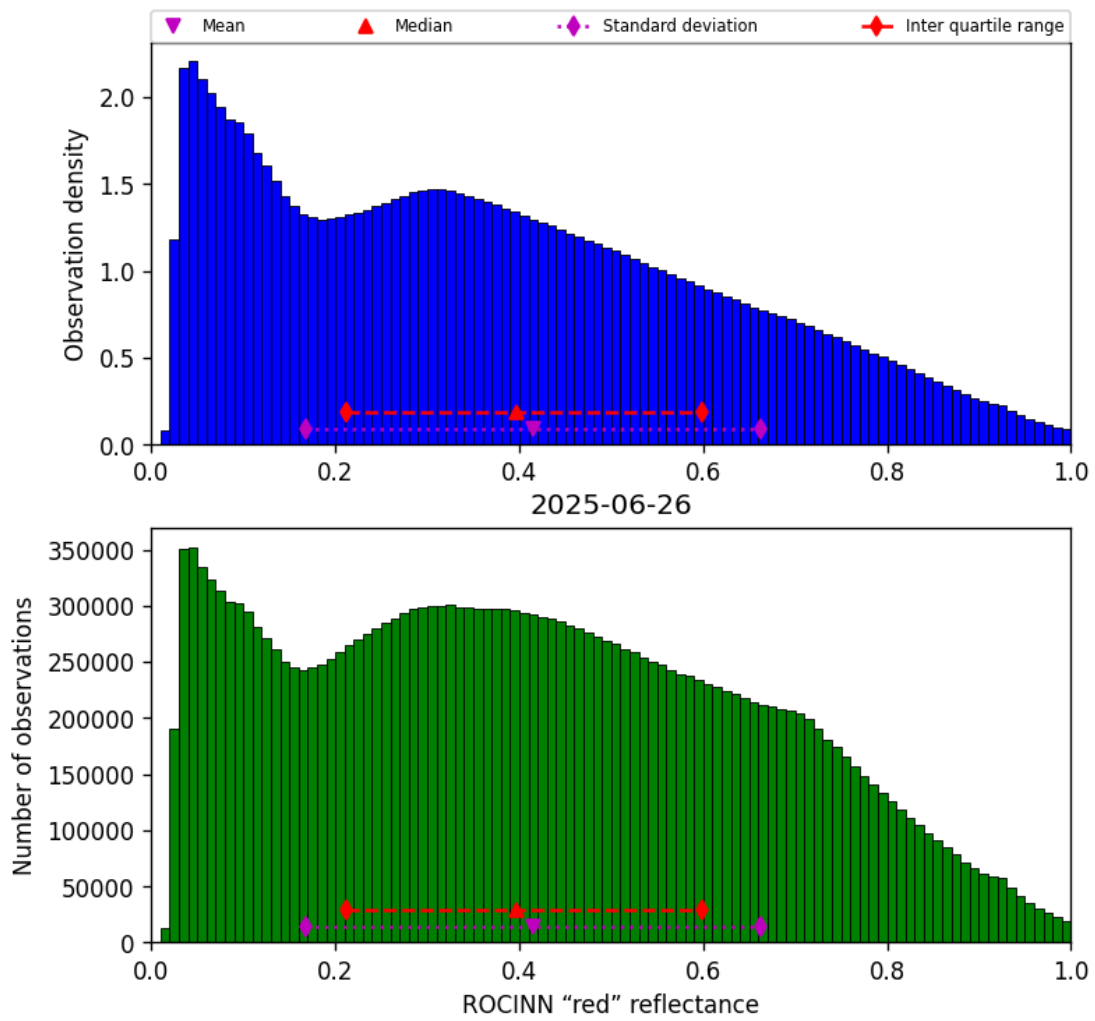
Figure 53: Histogram of “ROCINN “red” reflectance” for 2025-06-25 to 2025-06-27
