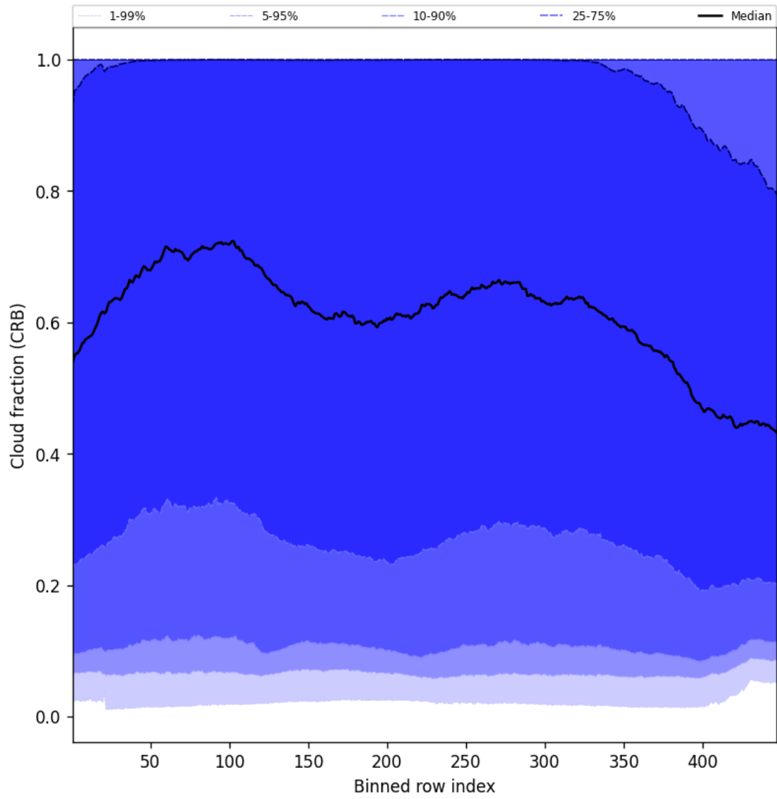
Figure 58: Along track statistics of “Cloud fraction (CRB)” for 2025-06-25 to 2025-06-27
