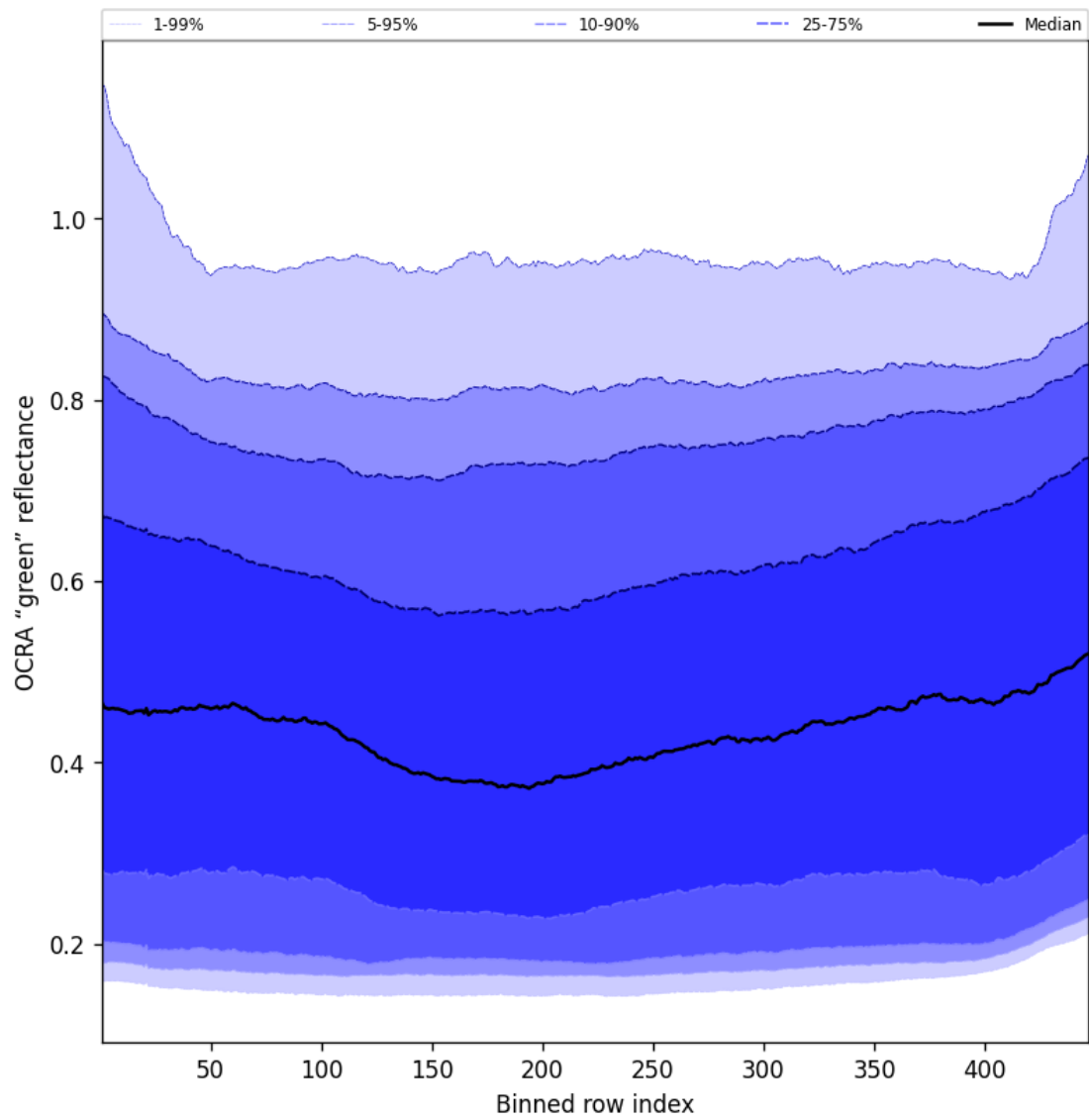
Figure 68: Along track statistics of “OCRA “green” reflectance” for 2025-06-25 to 2025-06-27
