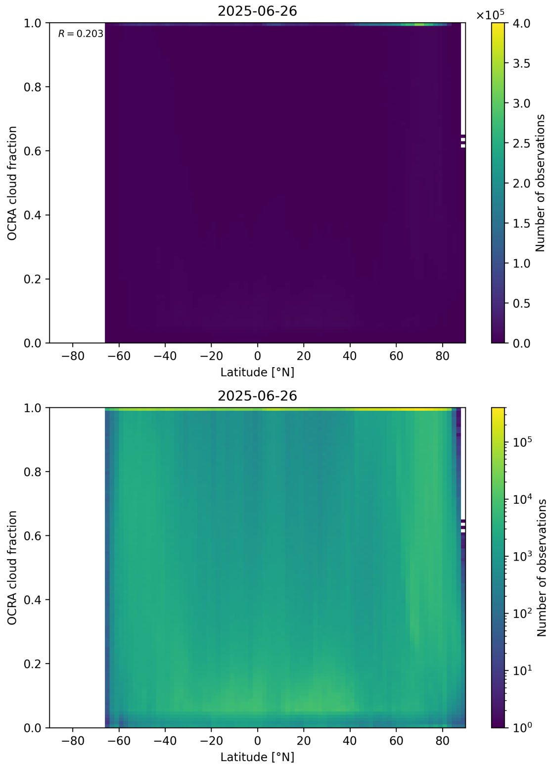
Figure 93: Scatter density plot of “Latitude” against “OCRA cloud fraction” for 2025-06-25 to 2025-06-27.
