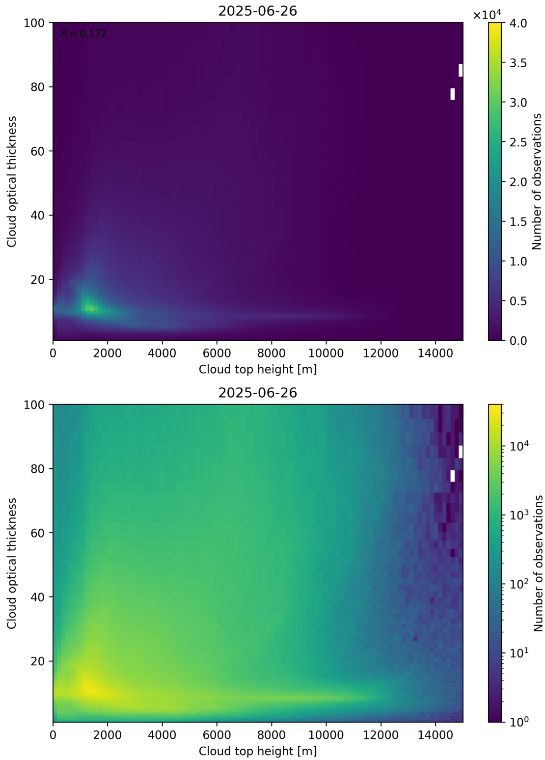
Figure 90: Scatter density plot of “Cloud top height” against “Cloud optical thickness” for 2025-06-25 to 2025-06-27.
