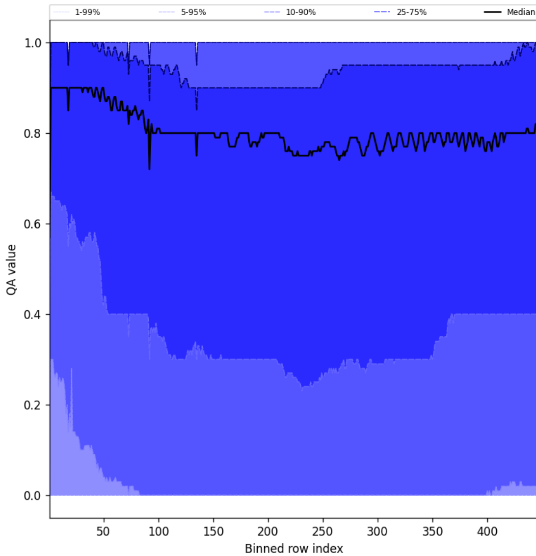
Figure 54: Along track statistics of “QA value” for 2025-06-25 to 2025-06-27
