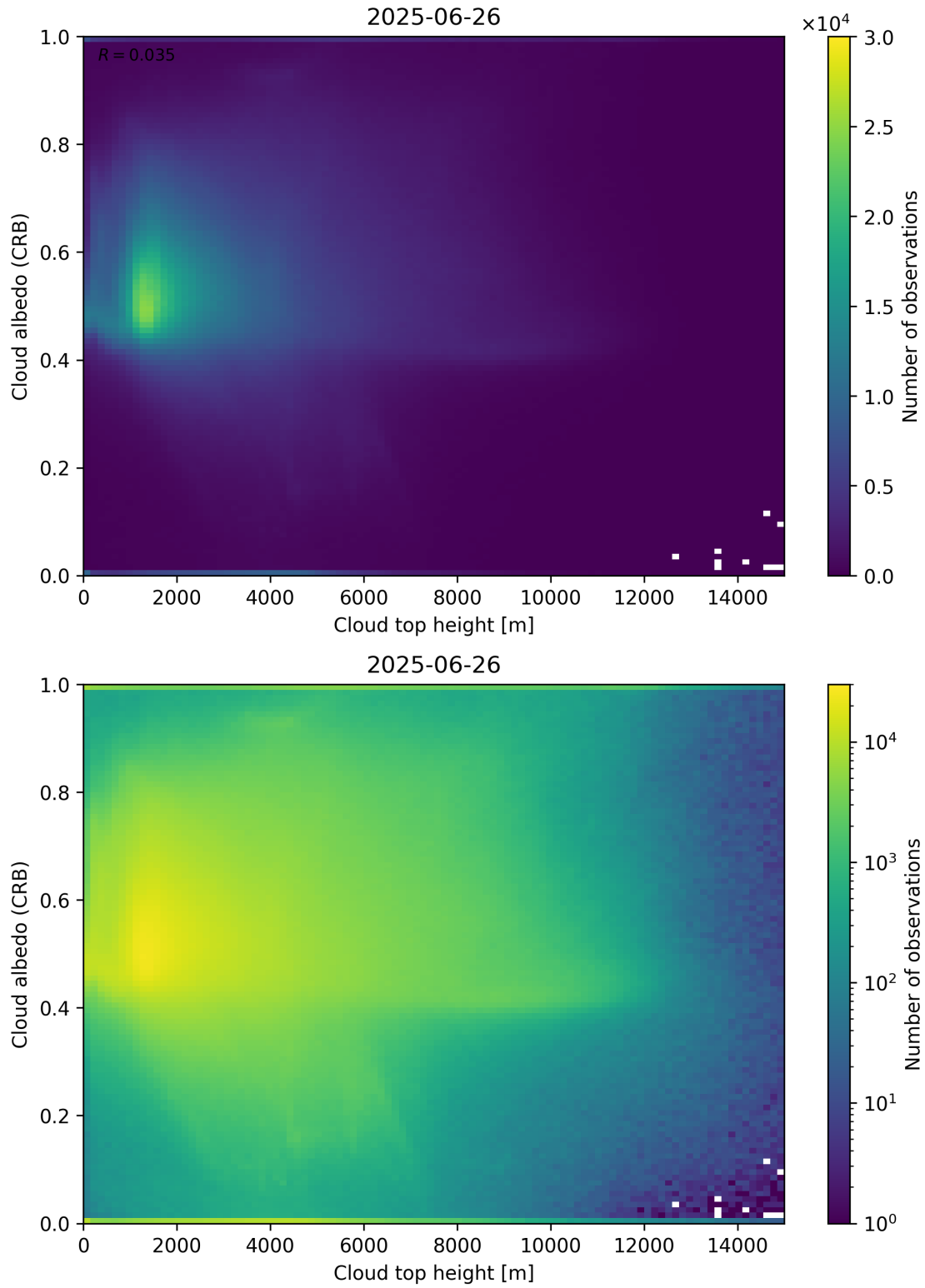
Figure 86: Scatter density plot of “Cloud top height” against “Cloud albedo (CRB)” for 2025-06-25 to 2025-06-27.
