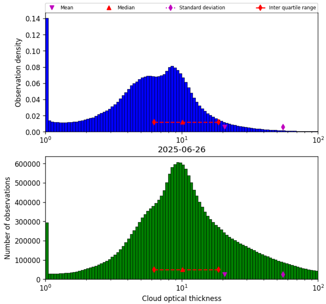
Figure 41: Histogram of “Cloud optical thickness” for 2025-06-25 to 2025-06-27
