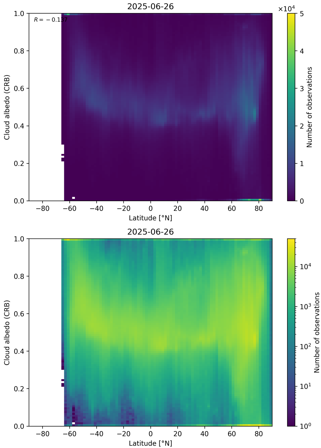
Figure 91: Scatter density plot of “Latitude” against “Cloud albedo (CRB)” for 2025-06-25 to 2025-06-27.
