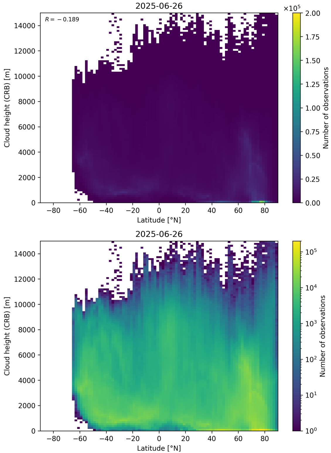
Figure 95: Scatter density plot of “Latitude” against “Cloud height (CRB)” for 2025-06-25 to 2025-06-27.
