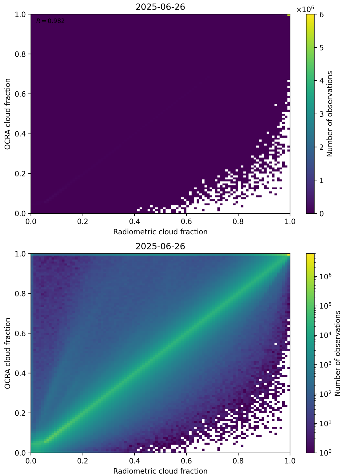
Figure 72: Scatter density plot of “Radiometric cloud fraction” against “OCRA cloud fraction” for 2025-06-25 to 2025-06-27.
