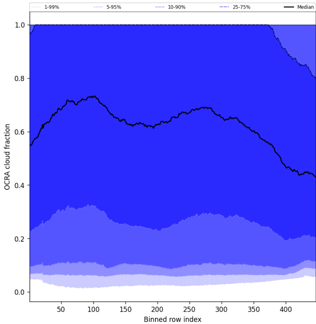
Figure 66: Along track statistics of “OCRA cloud fraction” for 2025-06-25 to 2025-06-27
