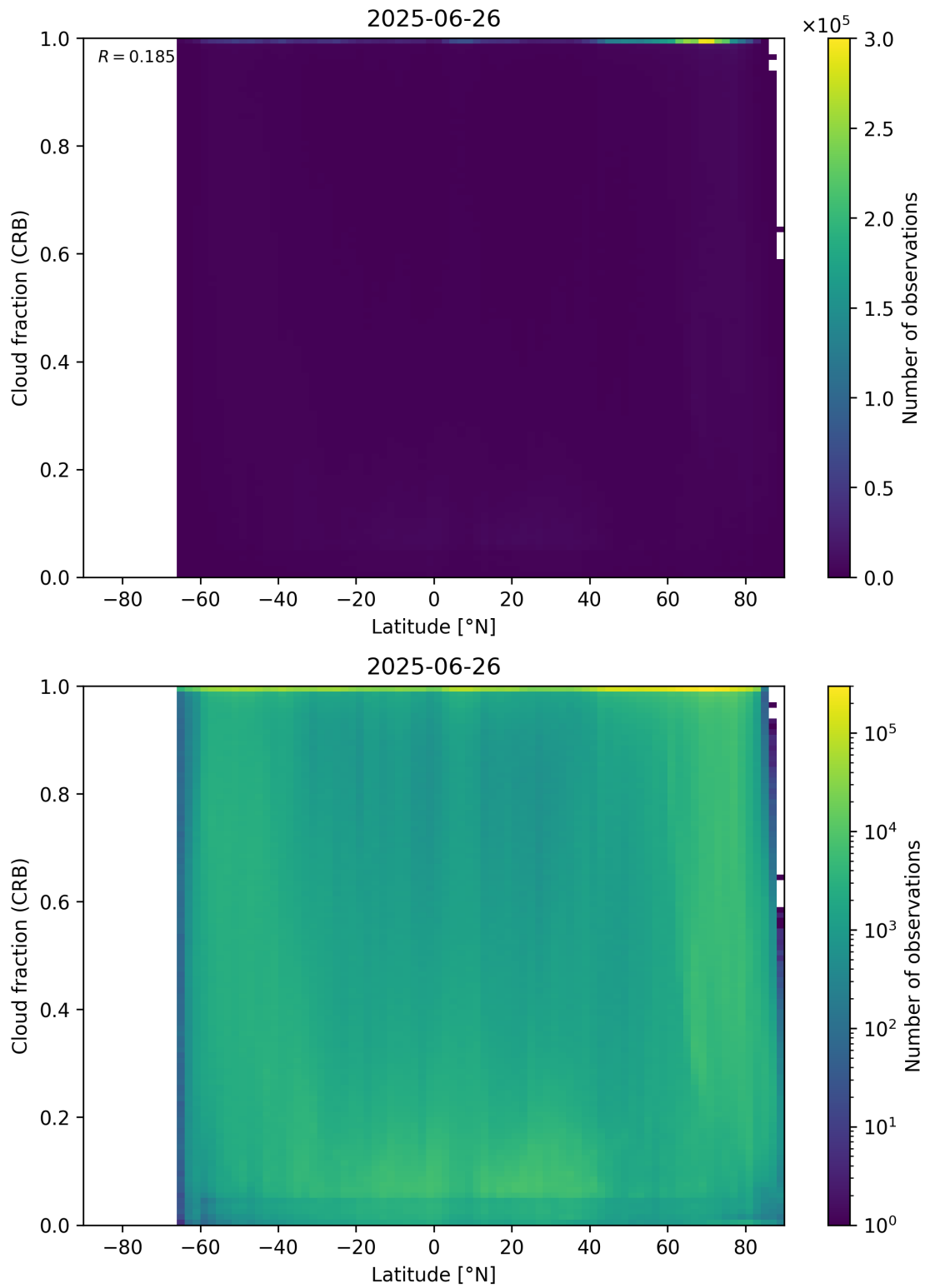
Figure 94: Scatter density plot of “Latitude” against “Cloud fraction (CRB)” for 2025-06-25 to 2025-06-27.
