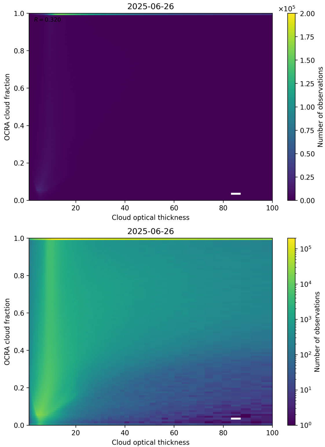
Figure 83: Scatter density plot of “Cloud optical thickness” against “OCRA cloud fraction” for 2025-06-25 to 2025-06-27.
