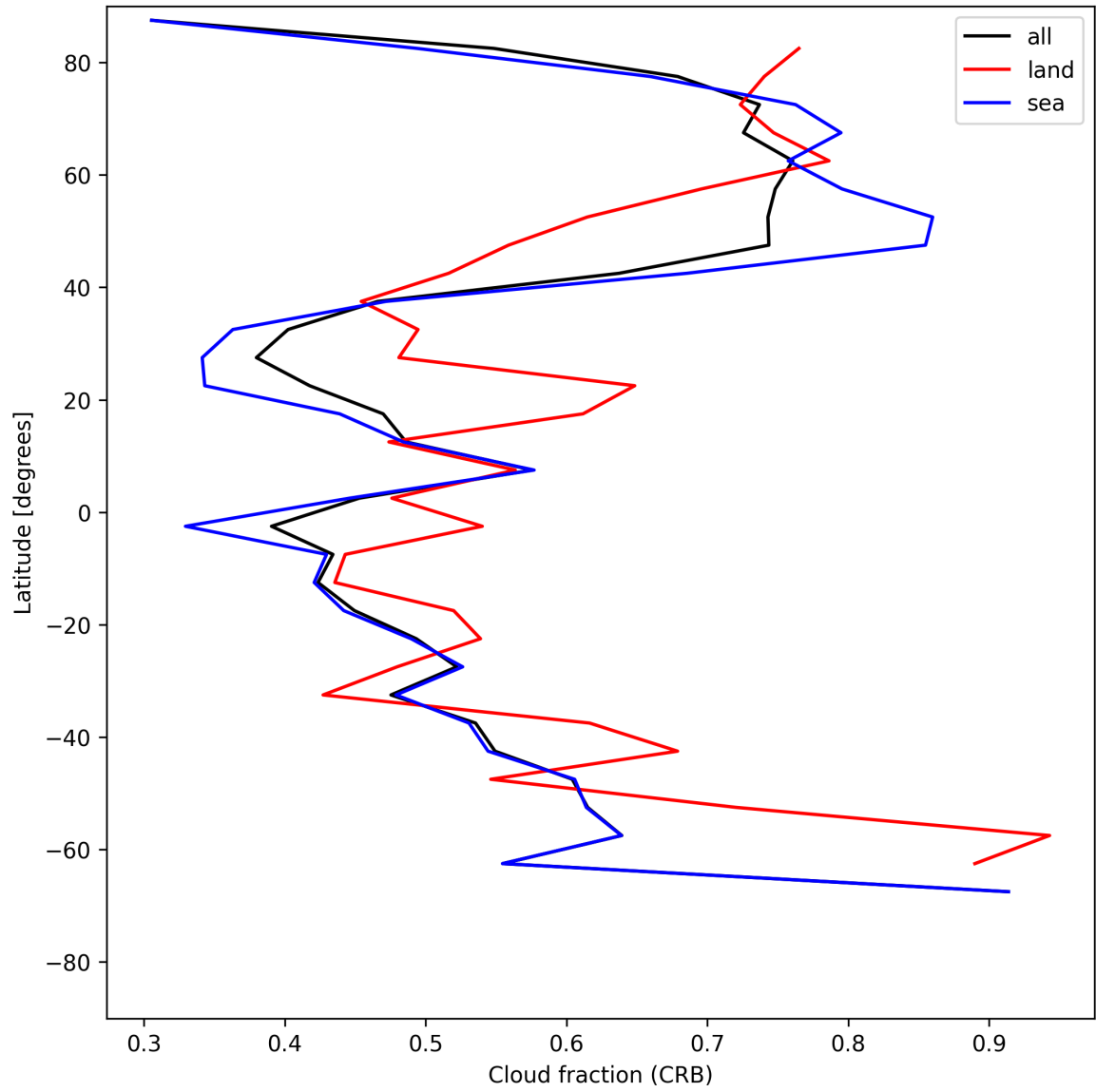
Figure 26: Zonal average of “Cloud fraction (CRB)” for 2025-06-25 to 2025-06-27.
