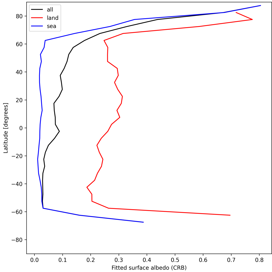
Figure 30: Zonal average of “Fitted surface albedo (CRB)” for 2025-06-25 to 2025-06-27.
