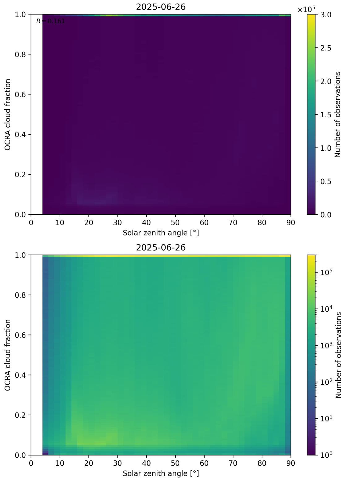
Figure 100: Scatter density plot of “Solar zenith angle” against “OCRA cloud fraction” for 2025-06-25 to 2025-06-27.
