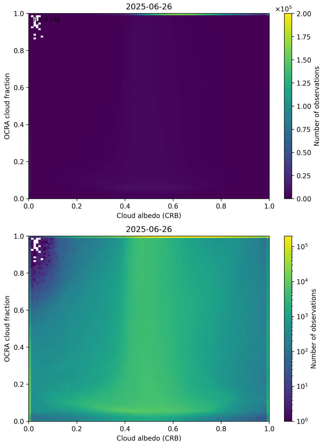
Figure 70: Scatter density plot of “Cloud albedo (CRB)” against “OCRA cloud fraction” for 2025-06-25 to 2025-06-27.
