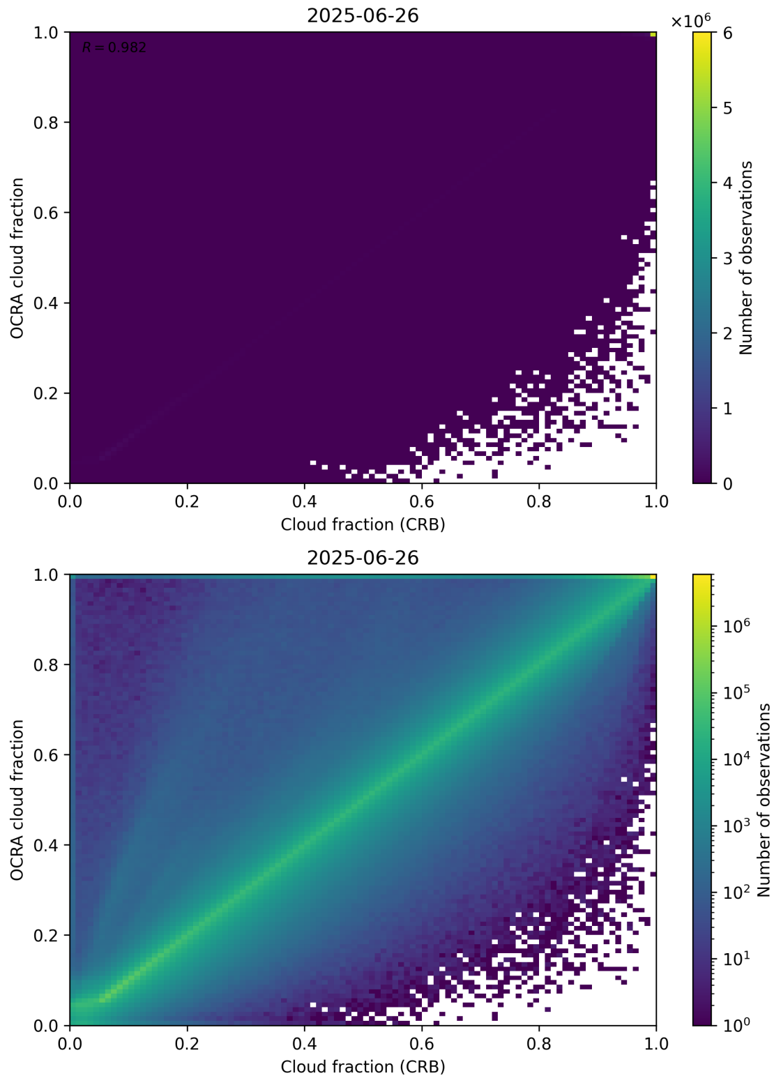
Figure 78: Scatter density plot of “Cloud fraction (CRB)” against “OCRA cloud fraction” for 2025-06-25 to 2025-06-27.
