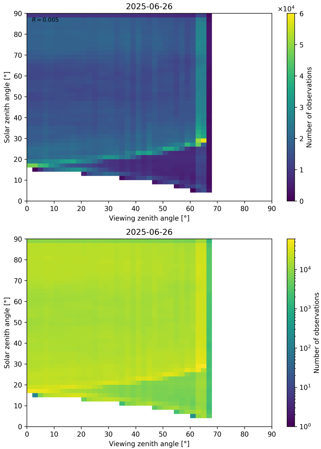
Figure 114: Scatter density plot of “Viewing zenith angle” against “Solar zenith angle” for 2025-06-25 to 2025-06-27.
