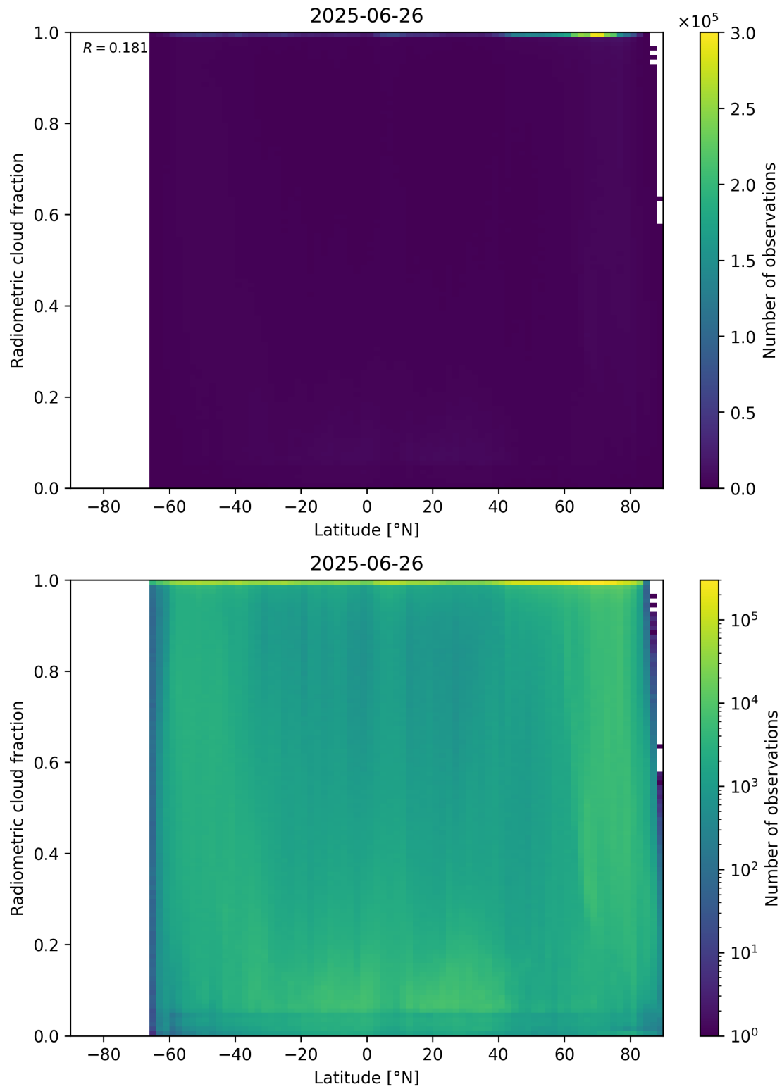
Figure 92: Scatter density plot of “Latitude” against “Radiometric cloud fraction” for 2025-06-25 to 2025-06-27.
