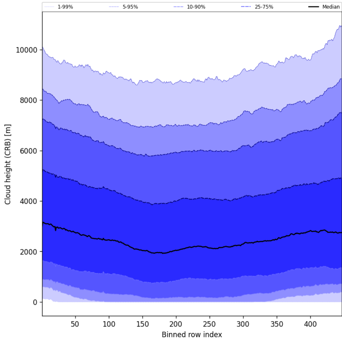
Figure 59: Along track statistics of “Cloud height (CRB)” for 2025-06-25 to 2025-06-27
