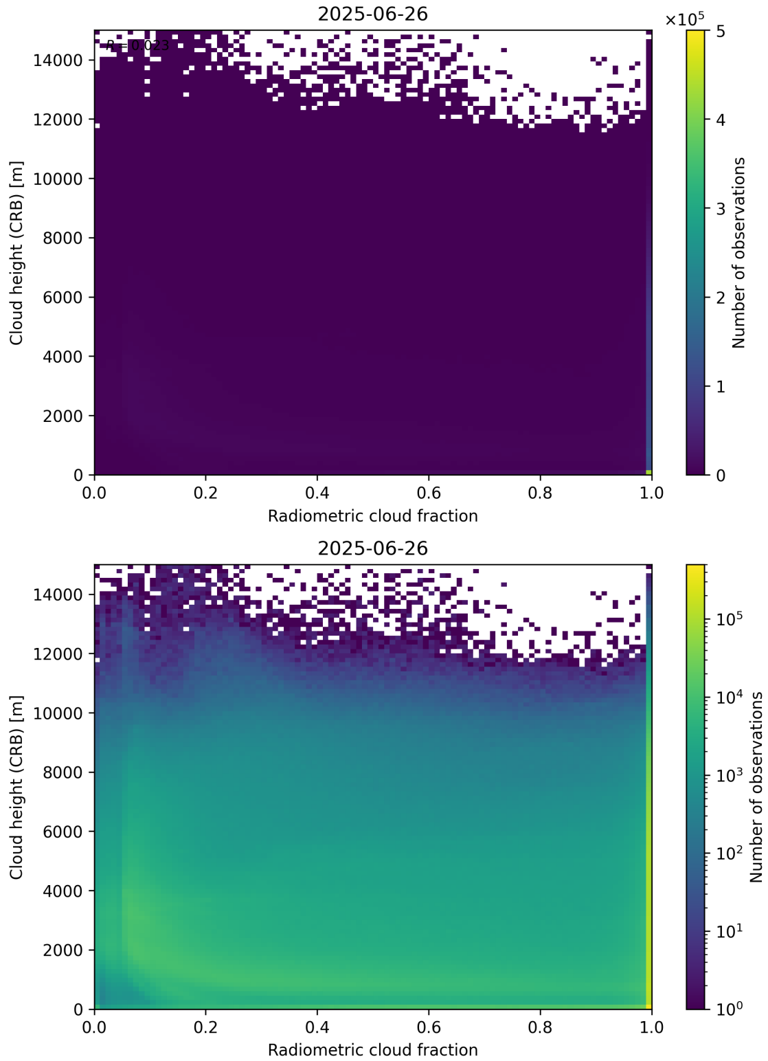
Figure 74: Scatter density plot of “Radiometric cloud fraction” against “Cloud height (CRB)” for 2025-06-25 to 2025-06-27.
