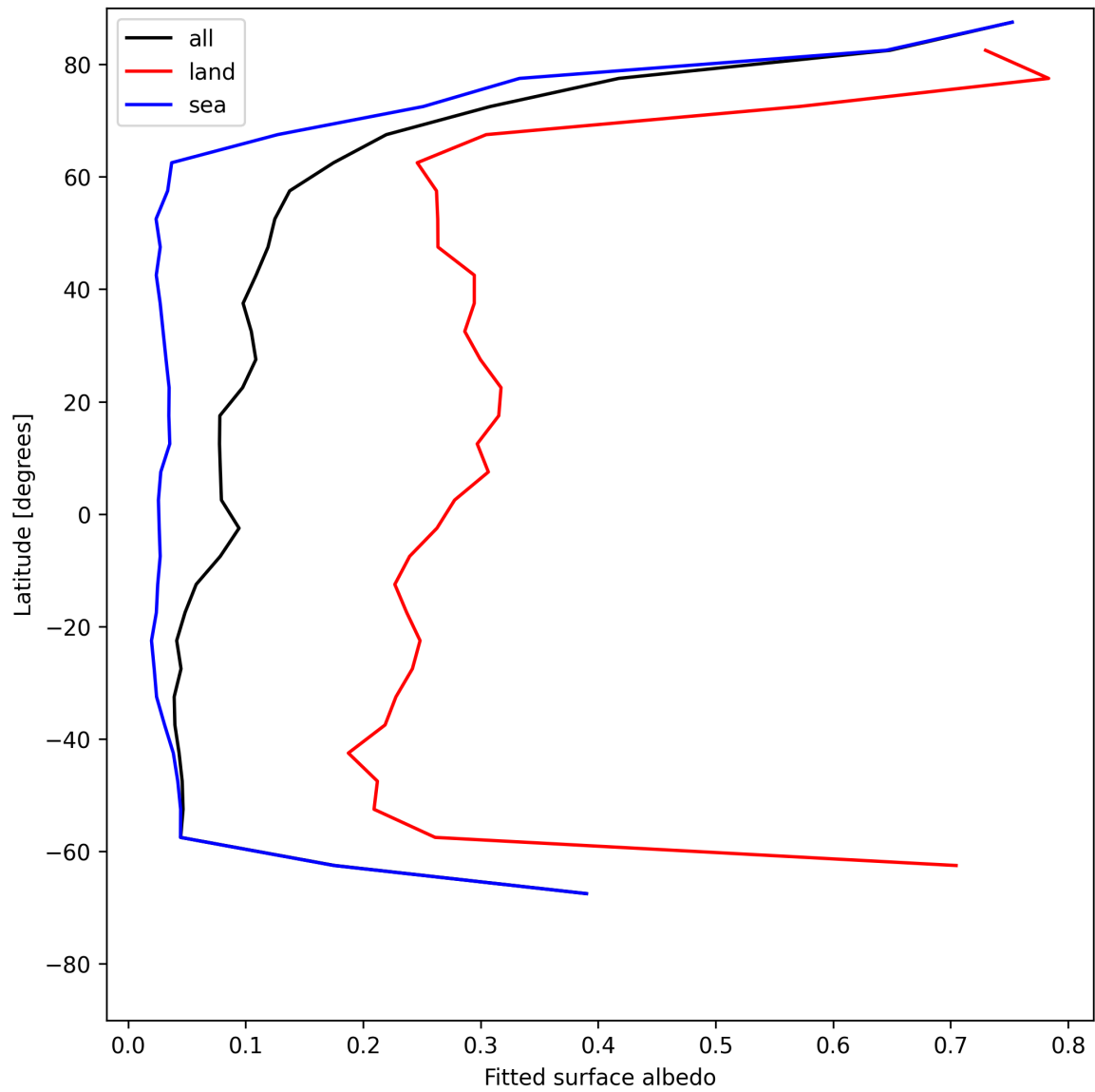
Figure 29: Zonal average of “Fitted surface albedo” for 2025-06-25 to 2025-06-27.
