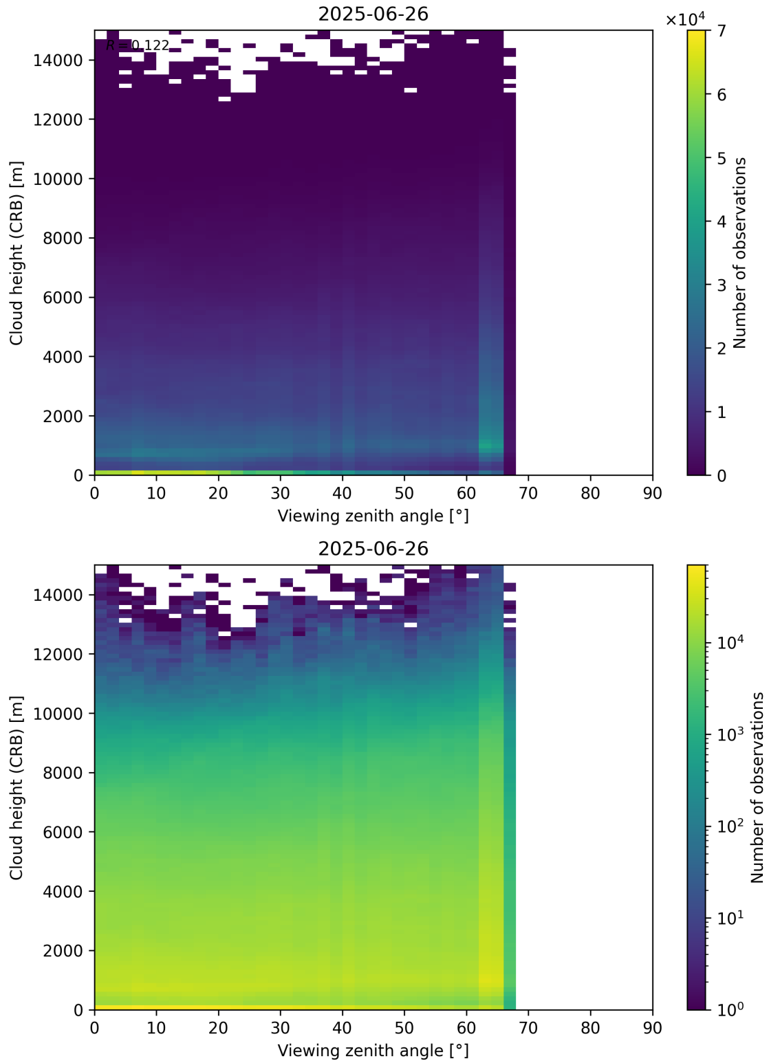
Figure 110: Scatter density plot of “Viewing zenith angle” against “Cloud height (CRB)” for 2025-06-25 to 2025-06-27.
