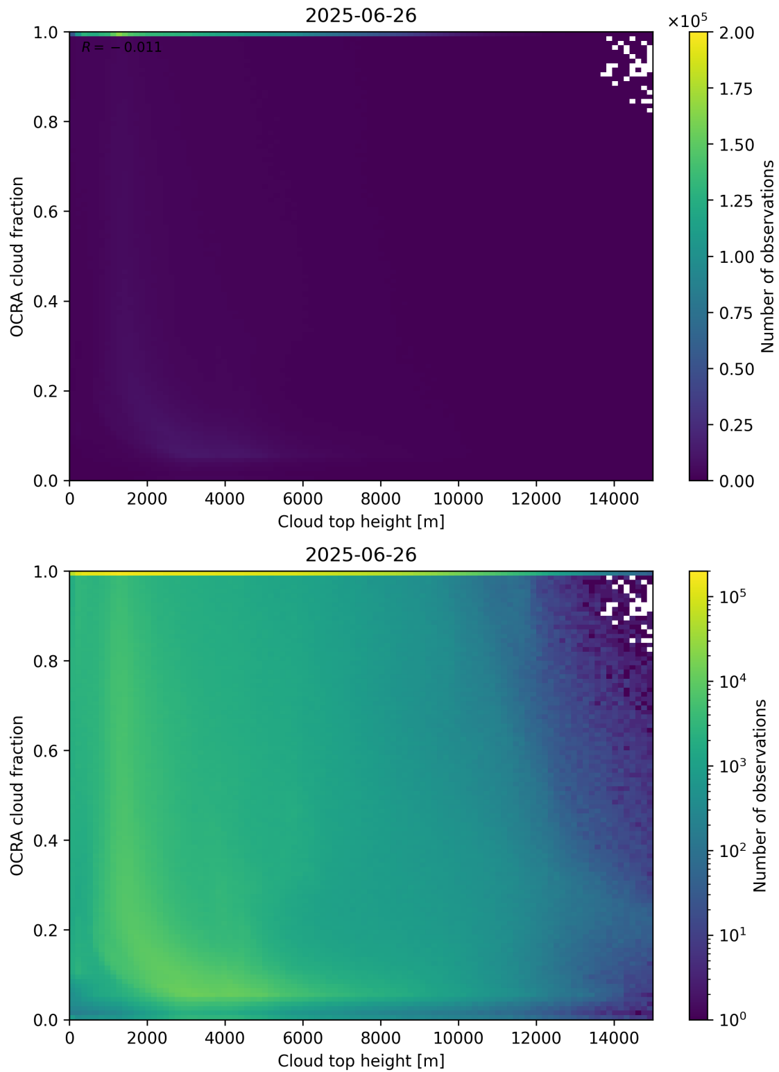
Figure 87: Scatter density plot of “Cloud top height” against “OCRA cloud fraction” for 2025-06-25 to 2025-06-27.
