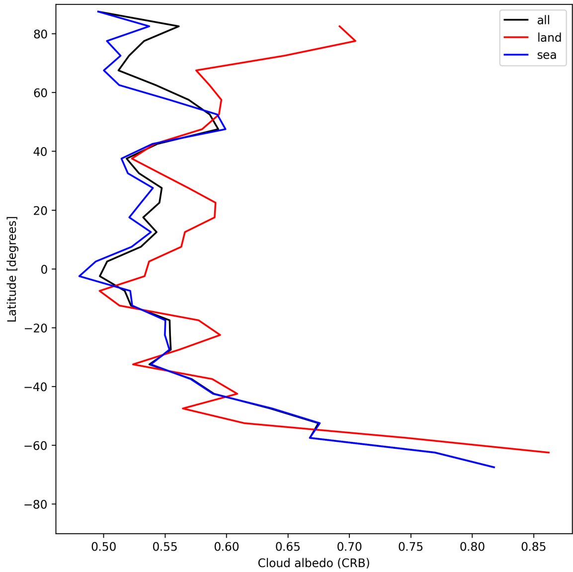
Figure 28: Zonal average of “Cloud albedo (CRB)” for 2025-06-25 to 2025-06-27.
