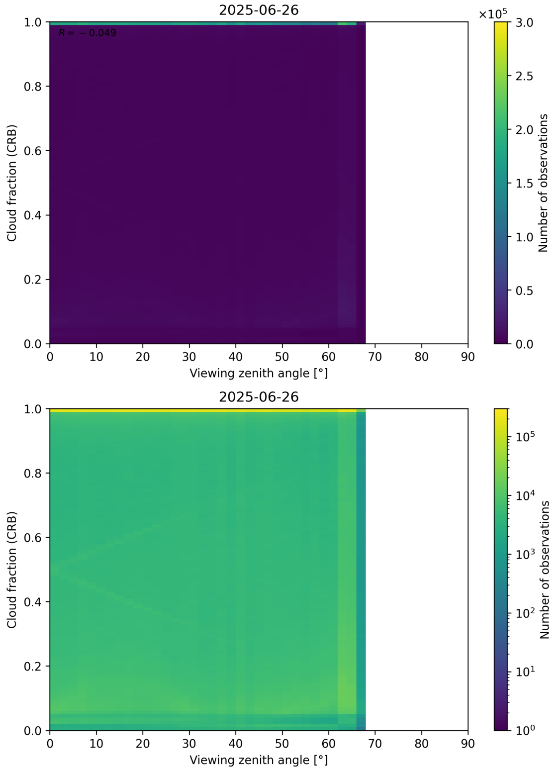
Figure 109: Scatter density plot of “Viewing zenith angle” against “Cloud fraction (CRB)” for 2025-06-25 to 2025-06-27.
