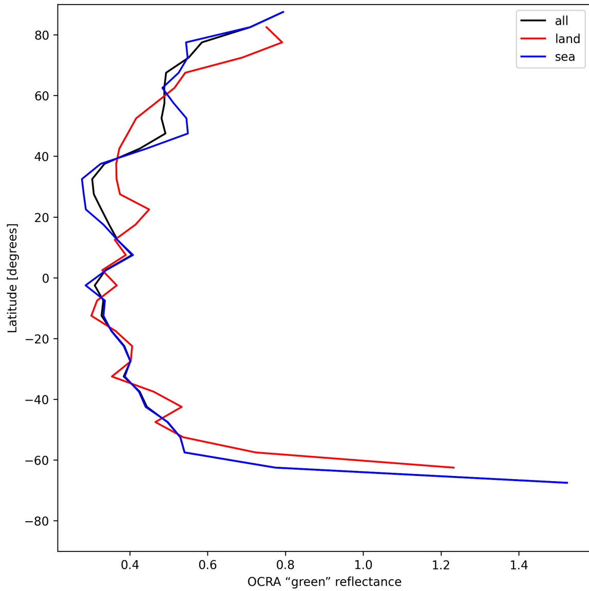
Figure 36: Zonal average of “OCRA “green” reflectance” for 2025-06-25 to 2025-06-27.
