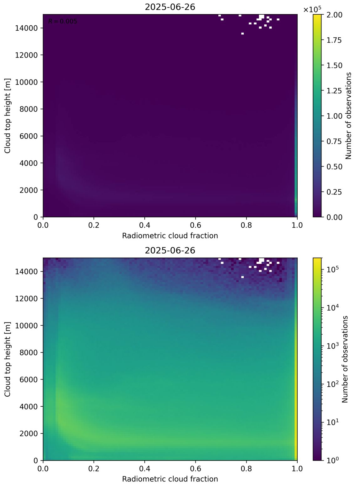
Figure 76: Scatter density plot of “Radiometric cloud fraction” against “Cloud top height” for 2025-06-25 to 2025-06-27.
