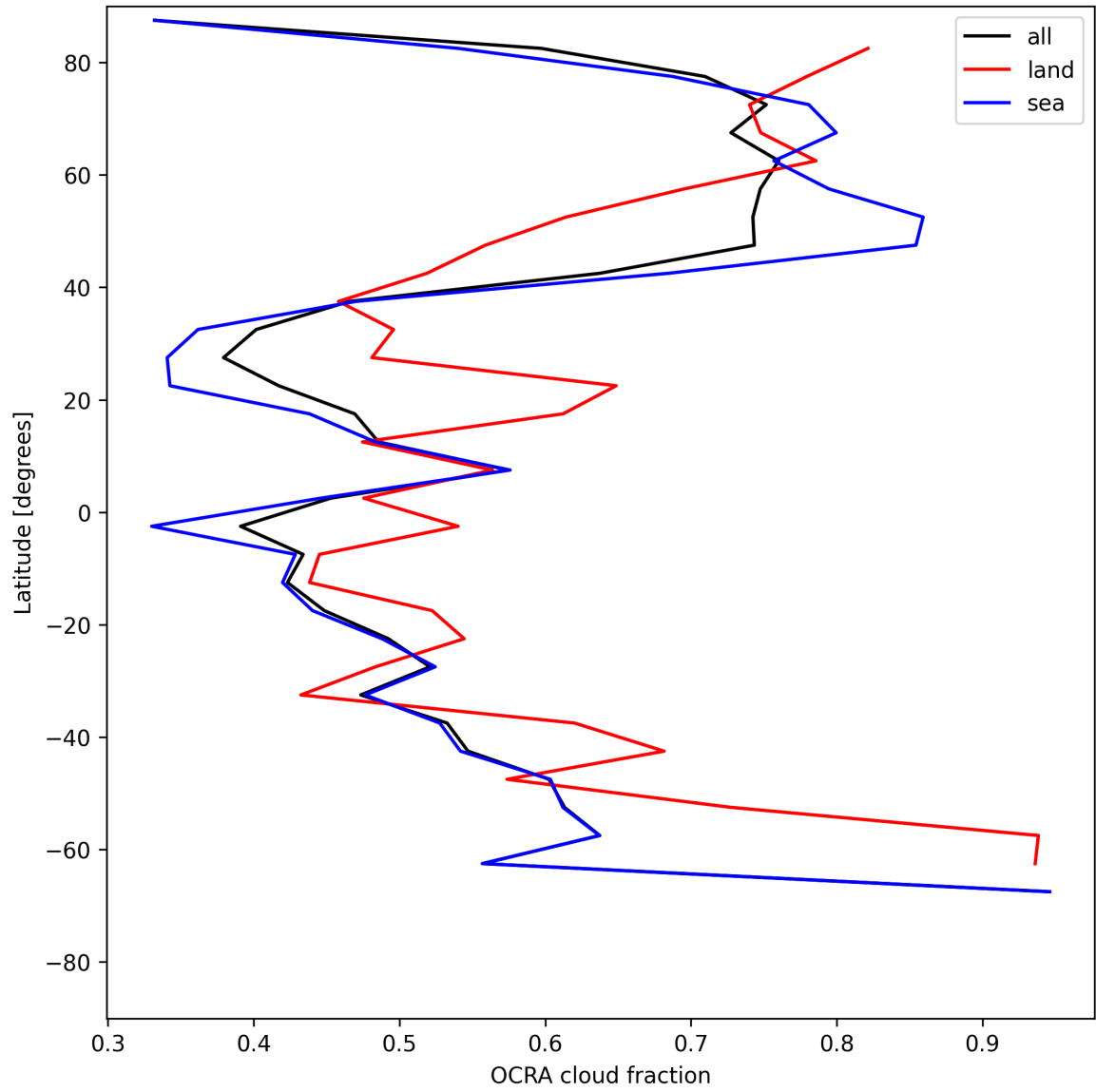
Figure 34: Zonal average of “OCRA cloud fraction” for 2025-06-25 to 2025-06-27.
