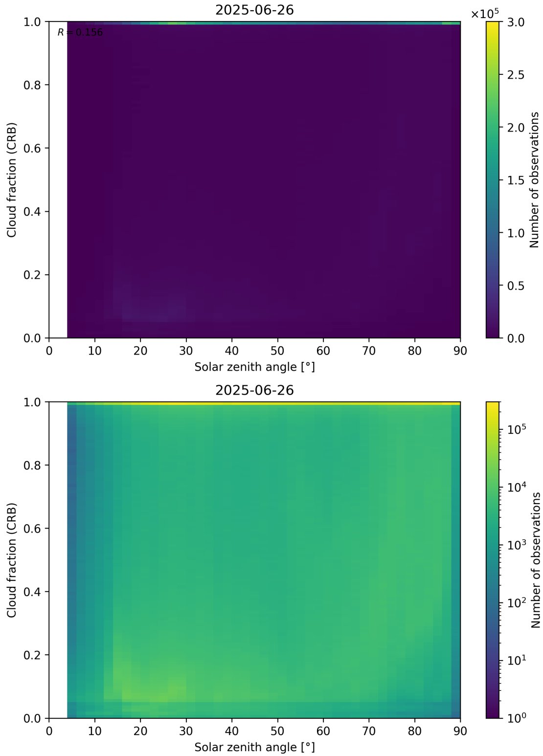
Figure 101: Scatter density plot of “Solar zenith angle” against “Cloud fraction (CRB)” for 2025-06-25 to 2025-06-27.
