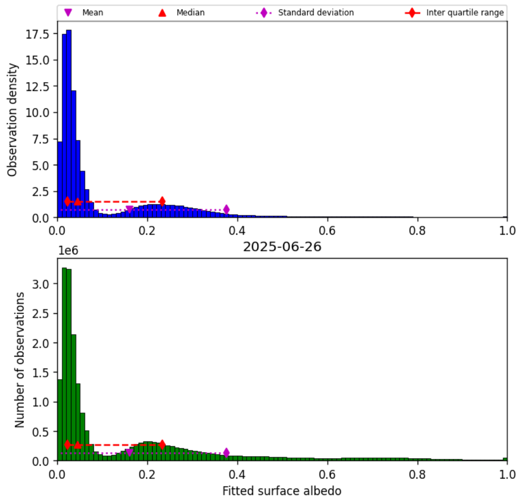
Figure 45: Histogram of “Fitted surface albedo” for 2025-06-25 to 2025-06-27
