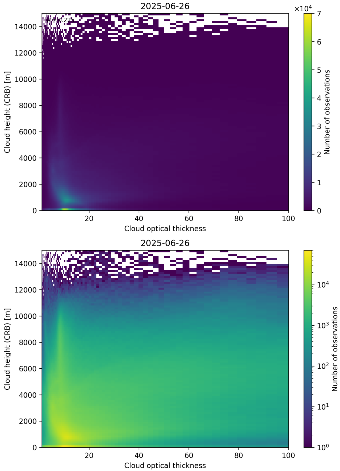
Figure 85: Scatter density plot of “Cloud optical thickness” against “Cloud height (CRB)” for 2025-06-25 to 2025-06-27.
