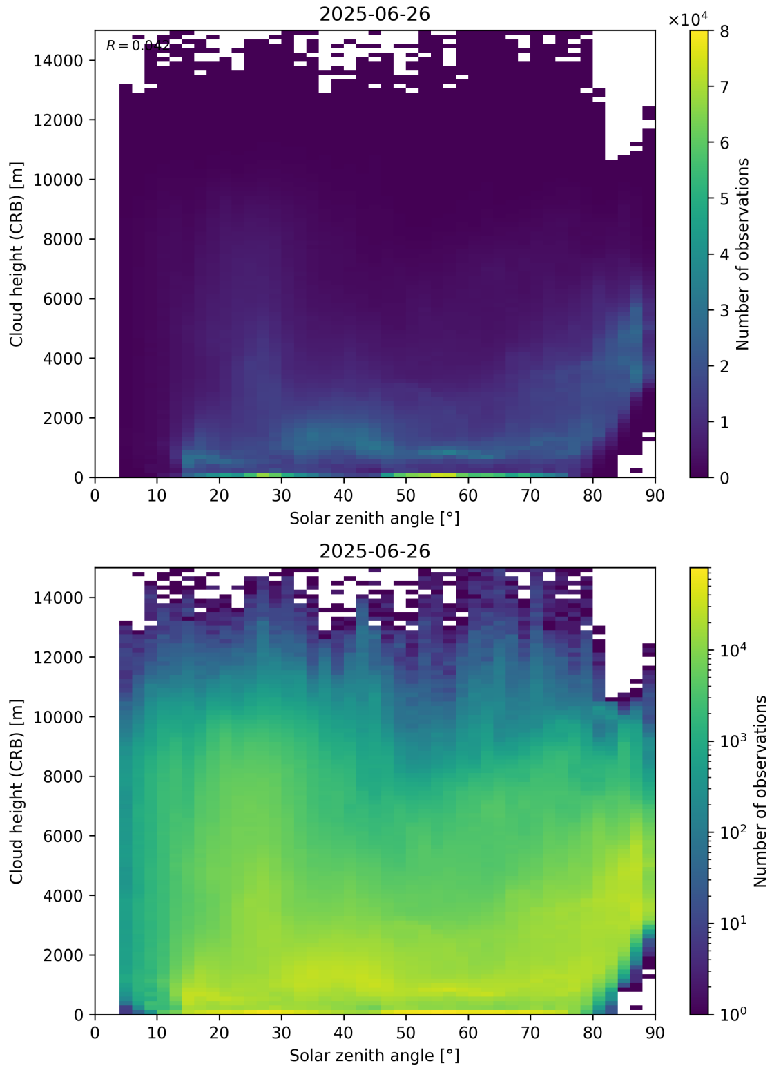
Figure 102: Scatter density plot of “Solar zenith angle” against “Cloud height (CRB)” for 2025-06-25 to 2025-06-27.
