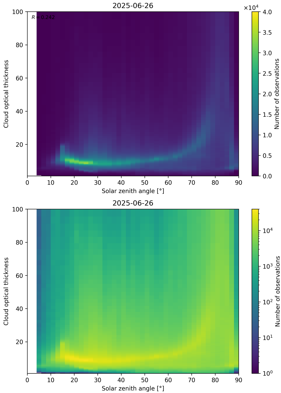
Figure 103: Scatter density plot of “Solar zenith angle” against “Cloud optical thickness” for 2025-06-25 to 2025-06-27.
