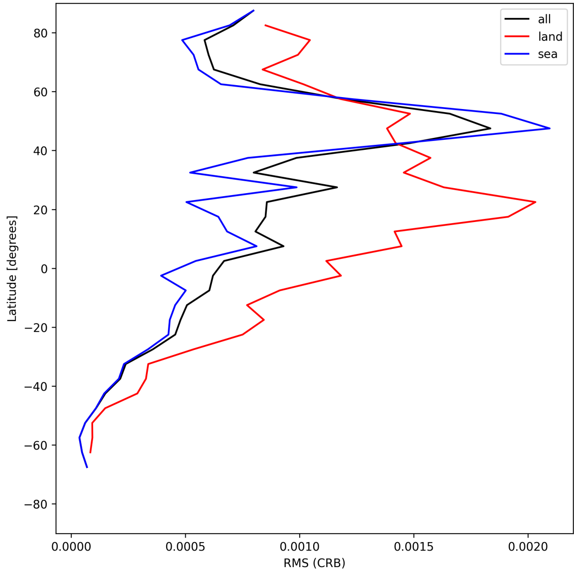
Figure 32: Zonal average of “RMS (CRB)” for 2025-06-25 to 2025-06-27.
