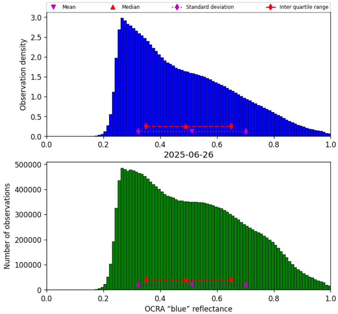
Figure 51: Histogram of “OCRA “blue” reflectance” for 2025-06-25 to 2025-06-27
