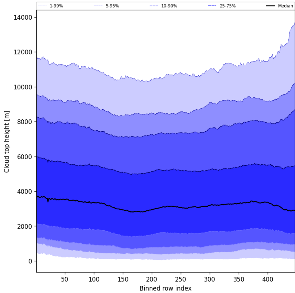
Figure 56: Along track statistics of “Cloud top height” for 2025-06-25 to 2025-06-27
