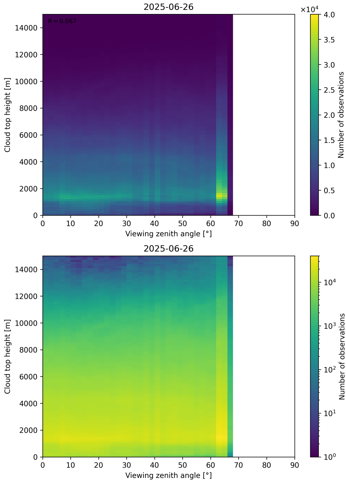
Figure 112: Scatter density plot of “Viewing zenith angle” against “Cloud top height” for 2025-06-25 to 2025-06-27.
