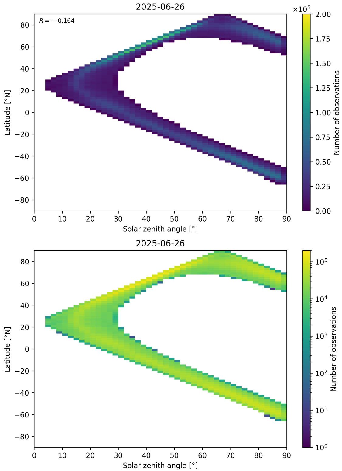
Figure 105: Scatter density plot of “Solar zenith angle” against “Latitude” for 2025-06-25 to 2025-06-27.
