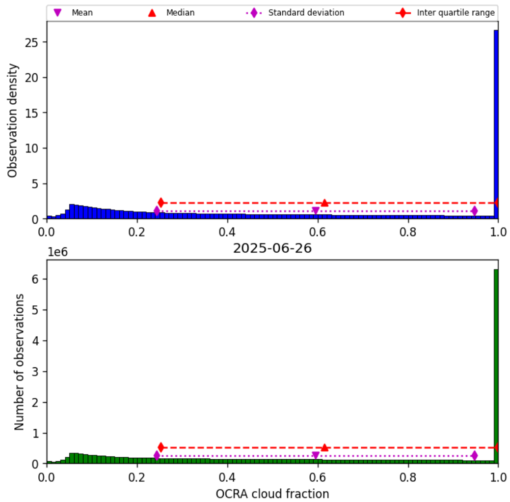
Figure 50: Histogram of “OCRA cloud fraction” for 2025-06-25 to 2025-06-27
