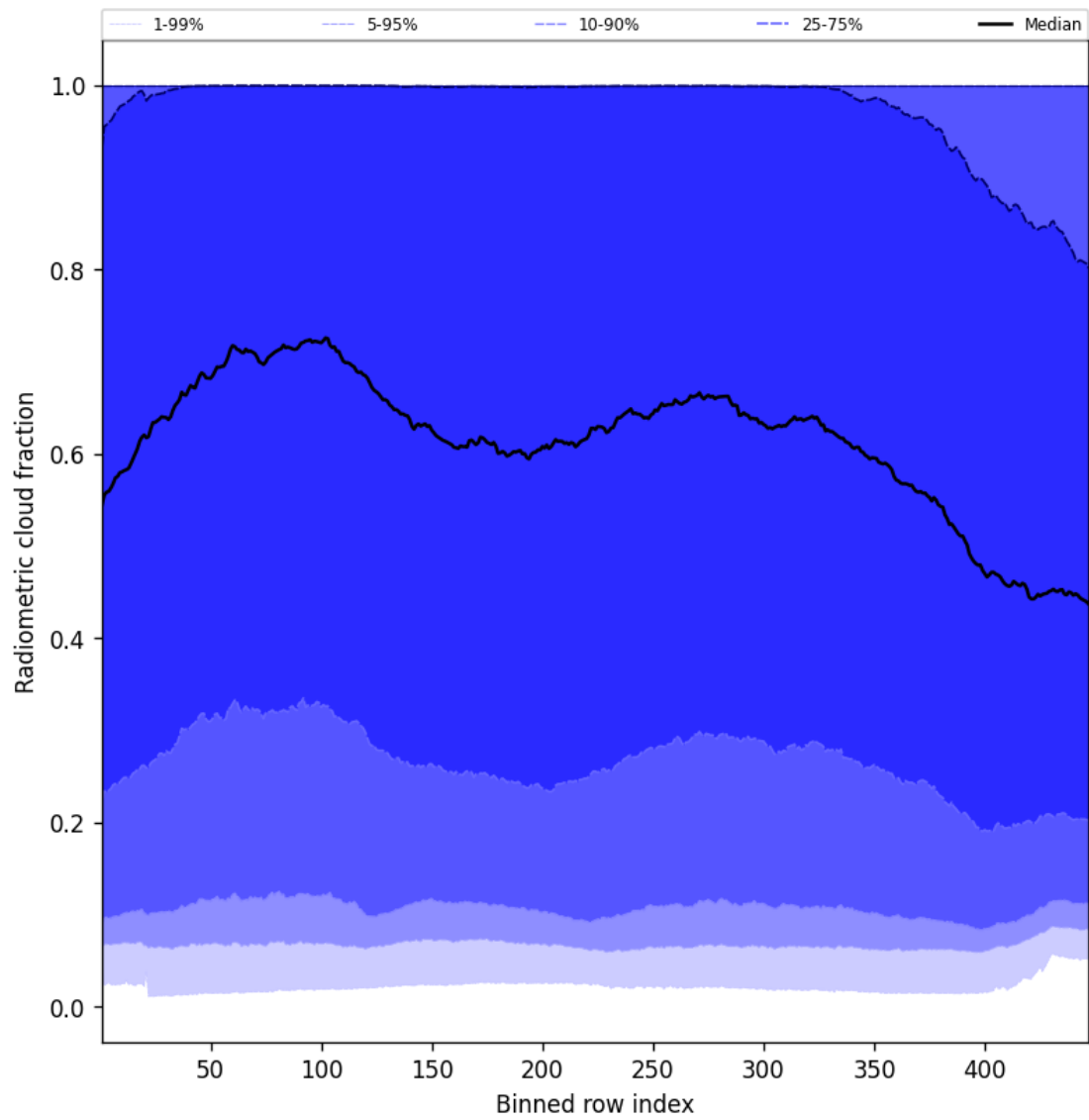
Figure 55: Along track statistics of “Radiometric cloud fraction” for 2025-06-25 to 2025-06-27
