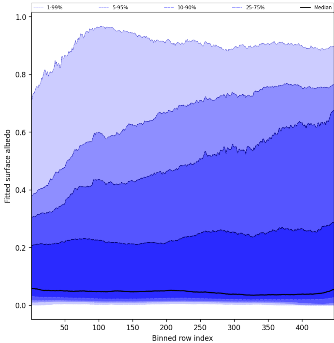
Figure 61: Along track statistics of “Fitted surface albedo” for 2025-06-25 to 2025-06-27
