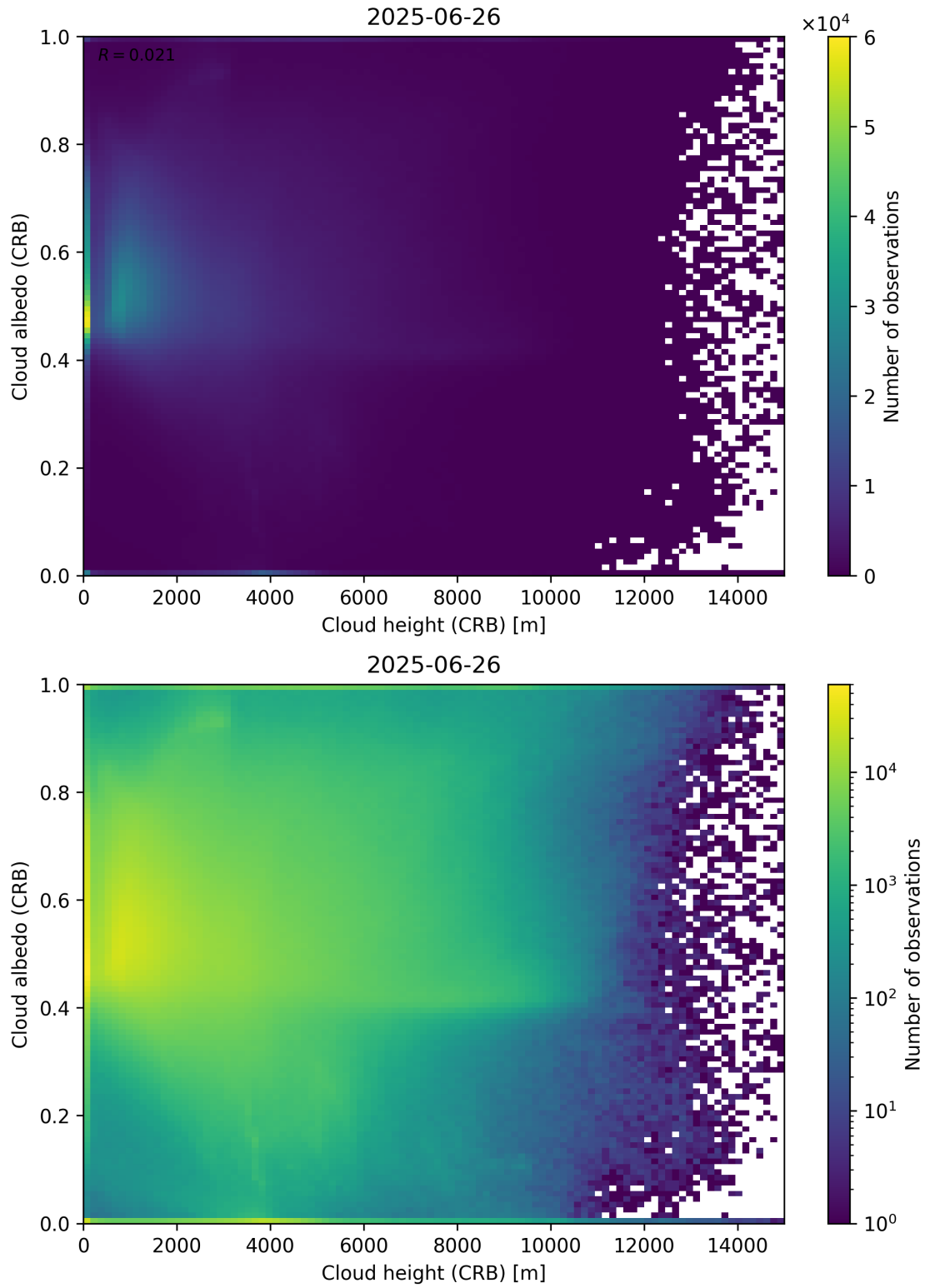
Figure 80: Scatter density plot of “Cloud height (CRB)” against “Cloud albedo (CRB)” for 2025-06-25 to 2025-06-27.
