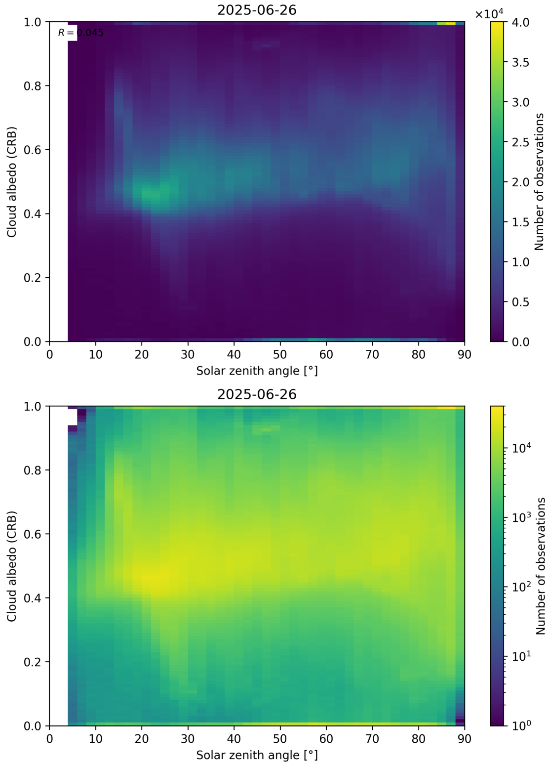
Figure 98: Scatter density plot of “Solar zenith angle” against “Cloud albedo (CRB)” for 2025-06-25 to 2025-06-27.
