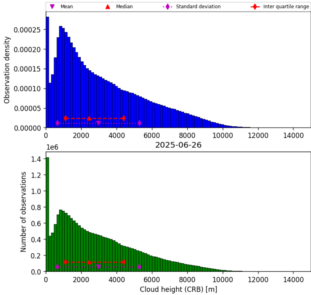
Figure 43: Histogram of “Cloud height (CRB)” for 2025-06-25 to 2025-06-27
