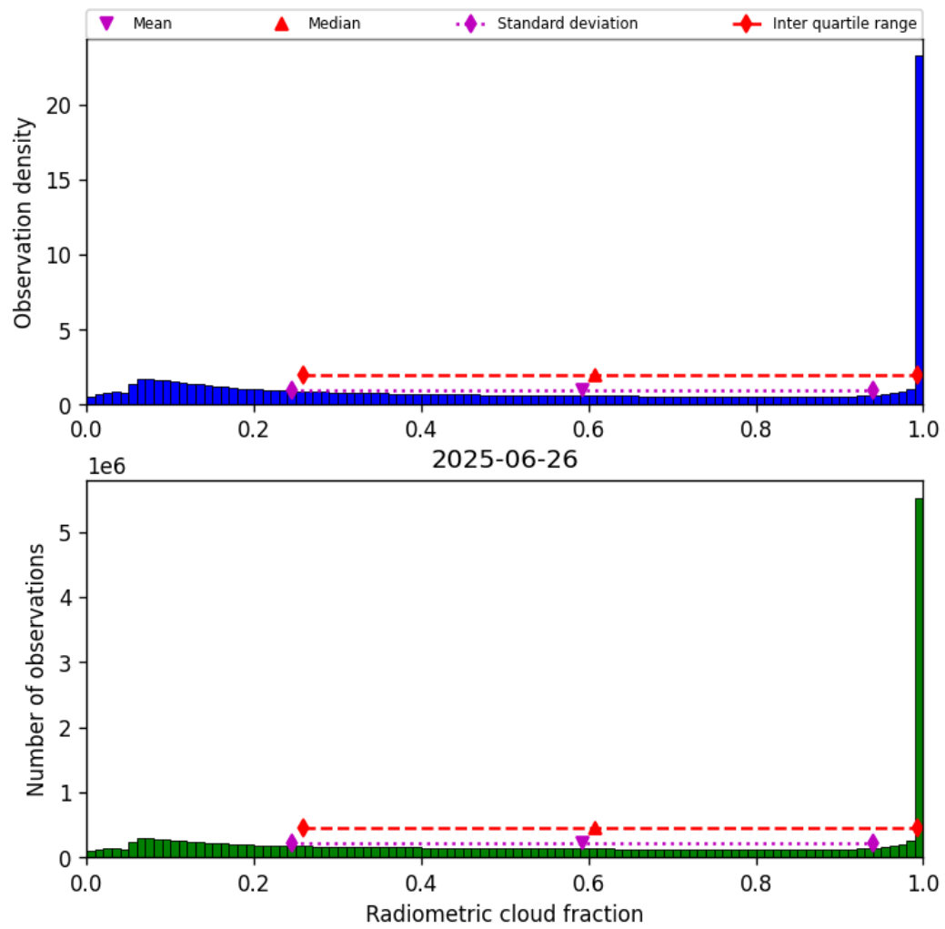
Figure 39: Histogram of “Radiometric cloud fraction” for 2025-06-25 to 2025-06-27
