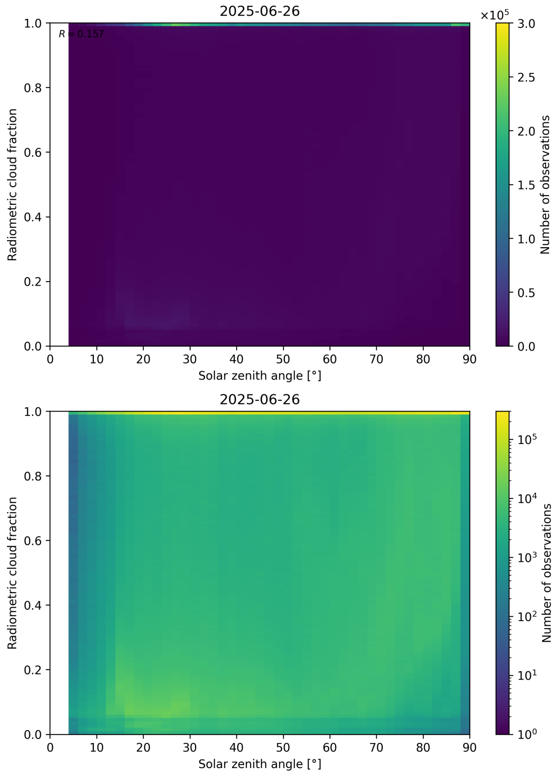
Figure 99: Scatter density plot of “Solar zenith angle” against “Radiometric cloud fraction” for 2025-06-25 to 2025-06-27.
