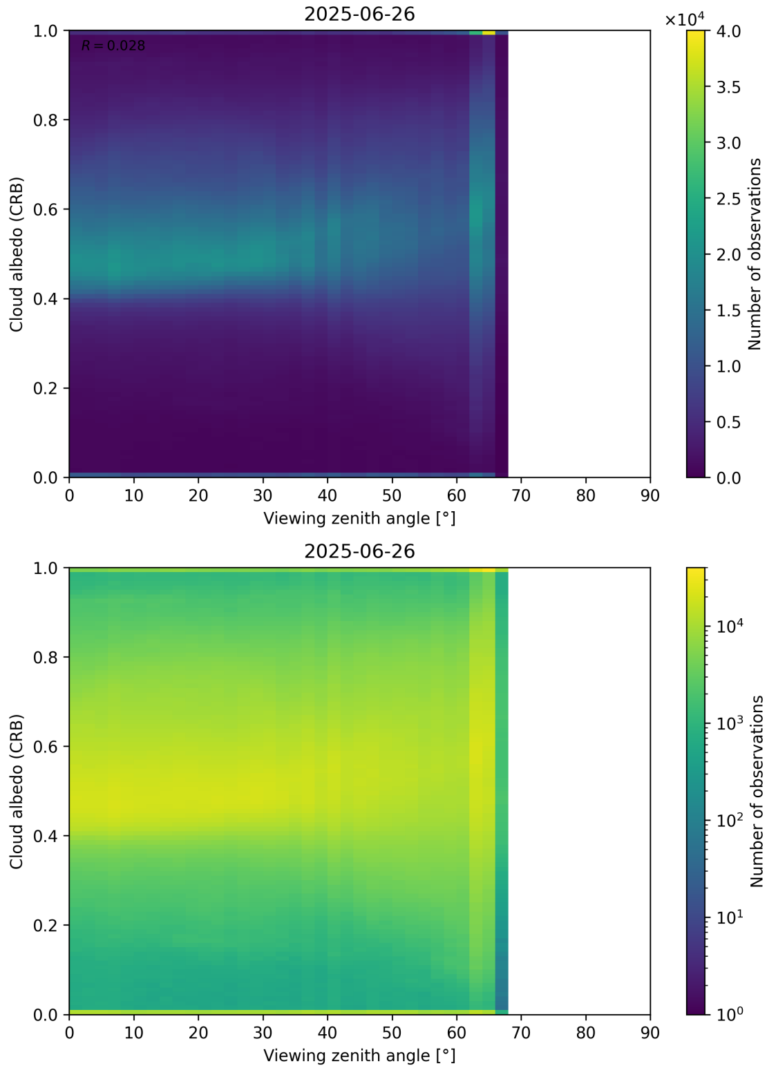
Figure 106: Scatter density plot of “Viewing zenith angle” against “Cloud albedo (CRB)” for 2025-06-25 to 2025-06-27.
