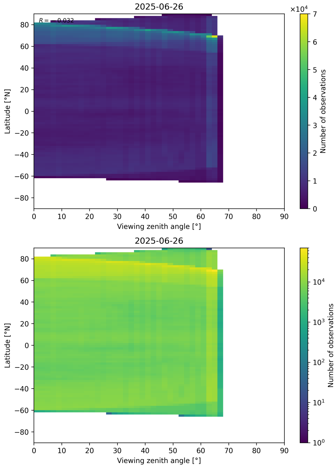
Figure 113: Scatter density plot of “Viewing zenith angle” against “Latitude” for 2025-06-25 to 2025-06-27.
