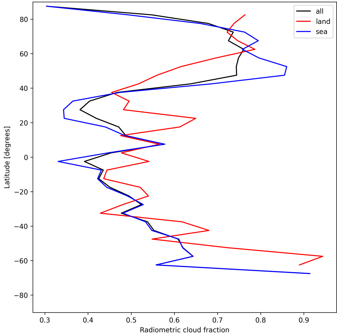
Figure 23: Zonal average of “Radiometric cloud fraction” for 2025-06-25 to 2025-06-27.
