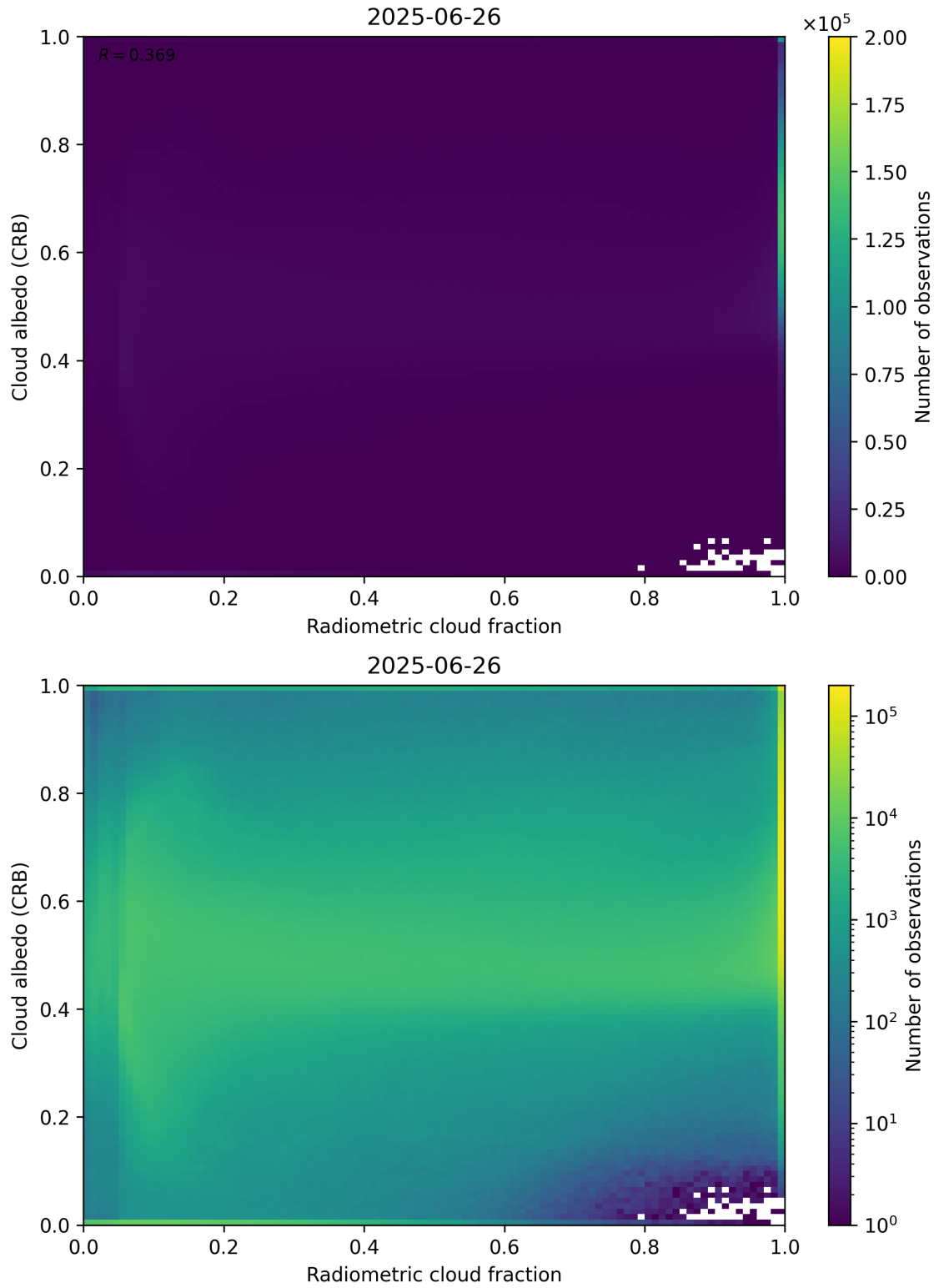
Figure 71: Scatter density plot of “Radiometric cloud fraction” against “Cloud albedo (CRB)” for 2025-06-25 to 2025-06-27.
