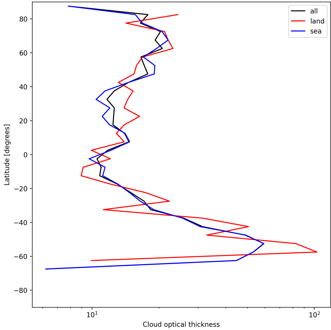
Figure 25: Zonal average of “Cloud optical thickness” for 2025-06-25 to 2025-06-27.
