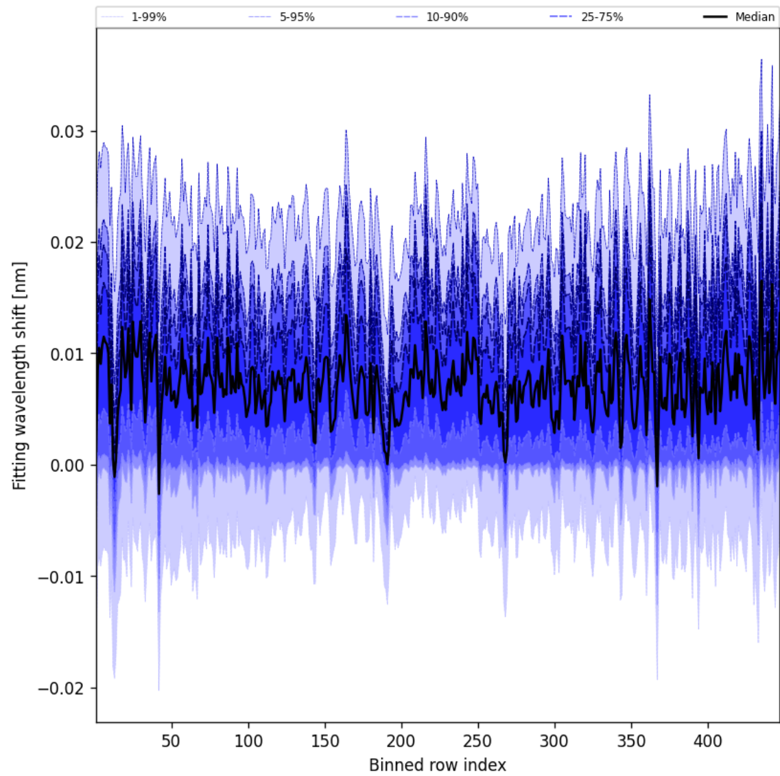
Figure 65: Along track statistics of “Fitting wavelength shift” for 2025-06-25 to 2025-06-27
