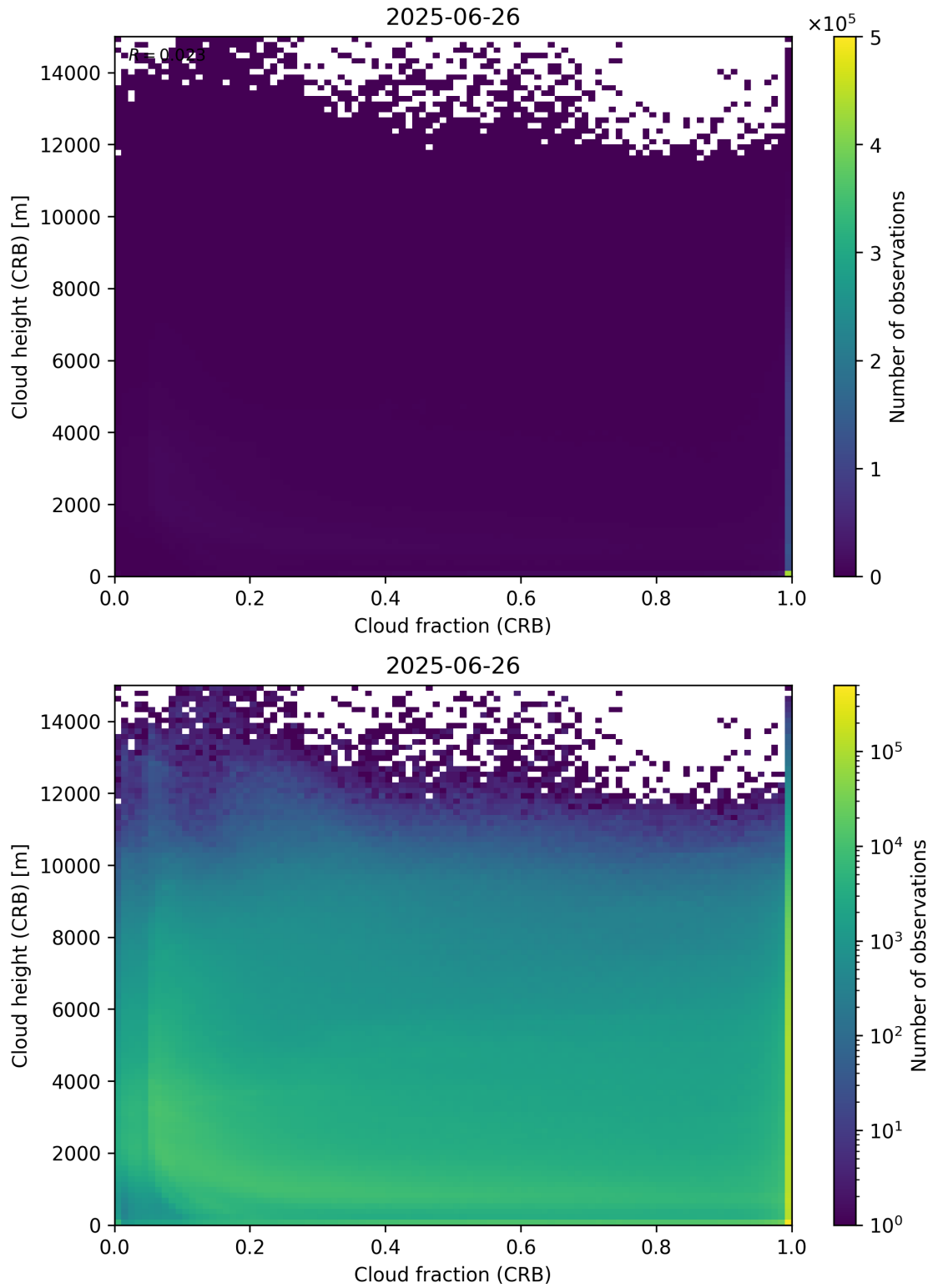
Figure 79: Scatter density plot of “Cloud fraction (CRB)” against “Cloud height (CRB)” for 2025-06-25 to 2025-06-27.
