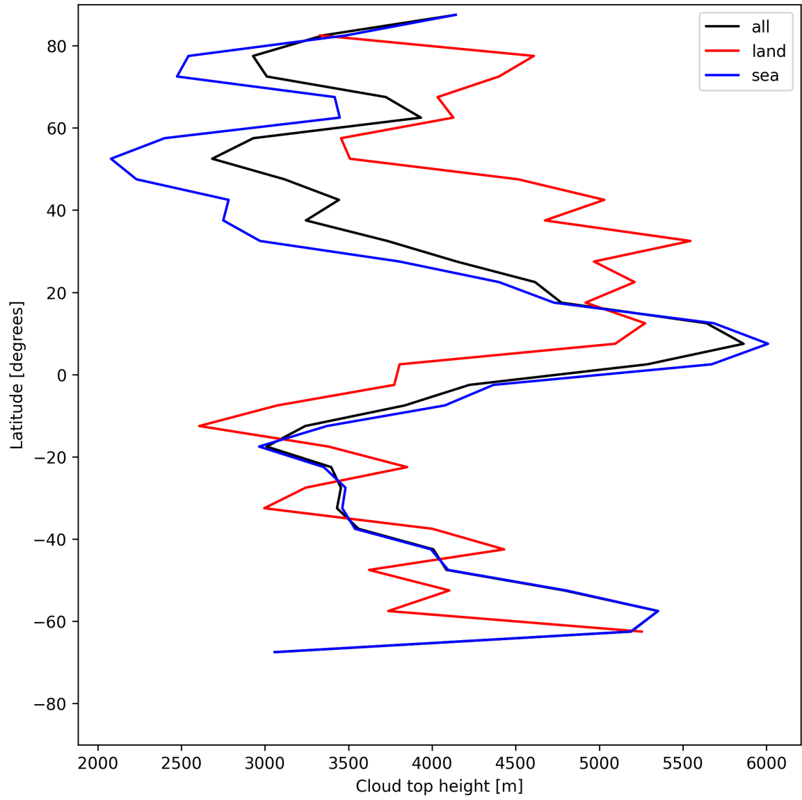
Figure 24: Zonal average of “Cloud top height” for 2025-06-25 to 2025-06-27.
