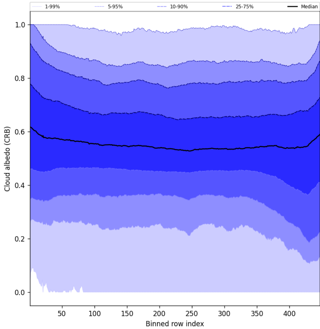
Figure 60: Along track statistics of “Cloud albedo (CRB)” for 2025-06-25 to 2025-06-27
