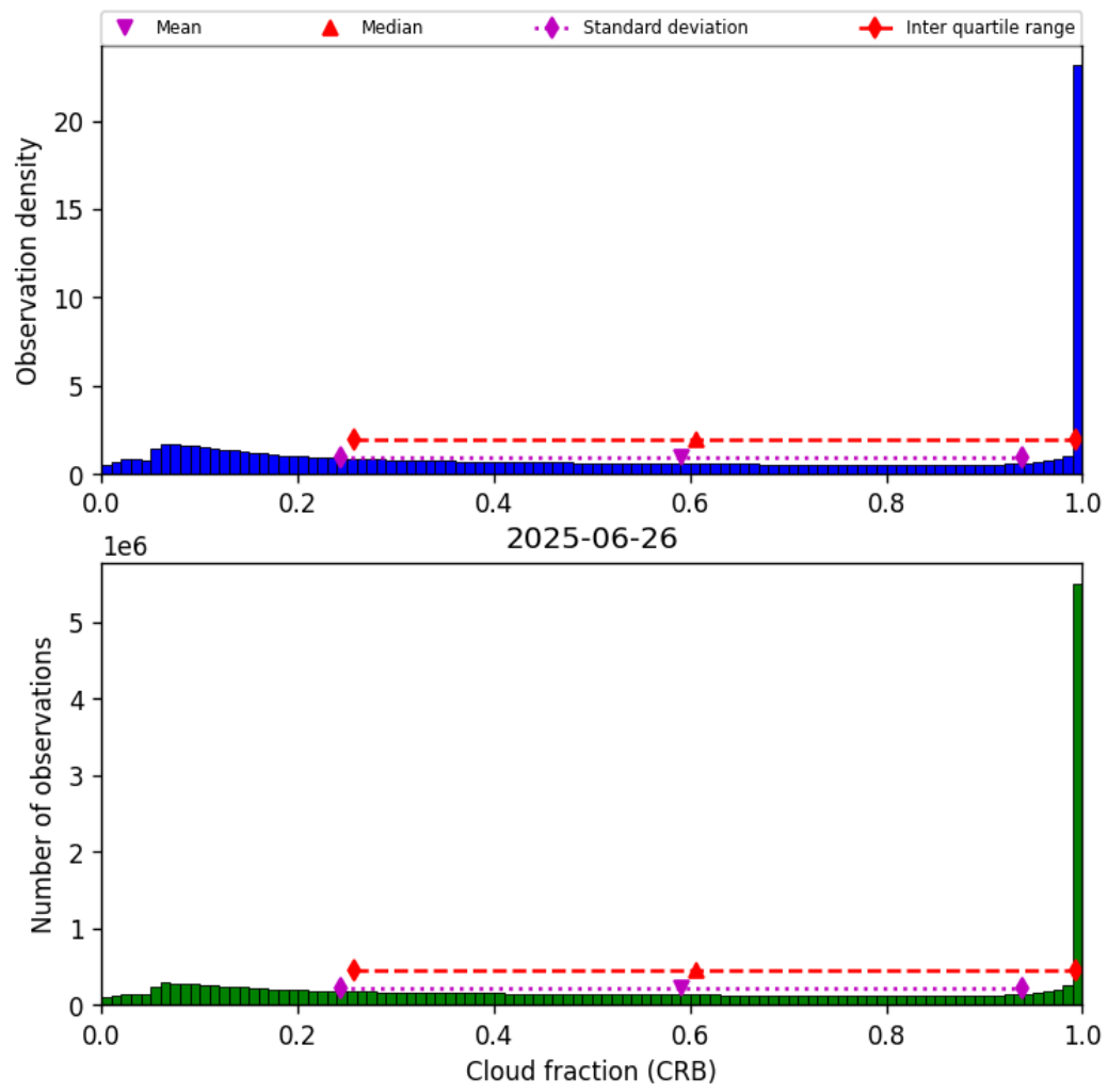
Figure 42: Histogram of “Cloud fraction (CRB)” for 2025-06-25 to 2025-06-27
