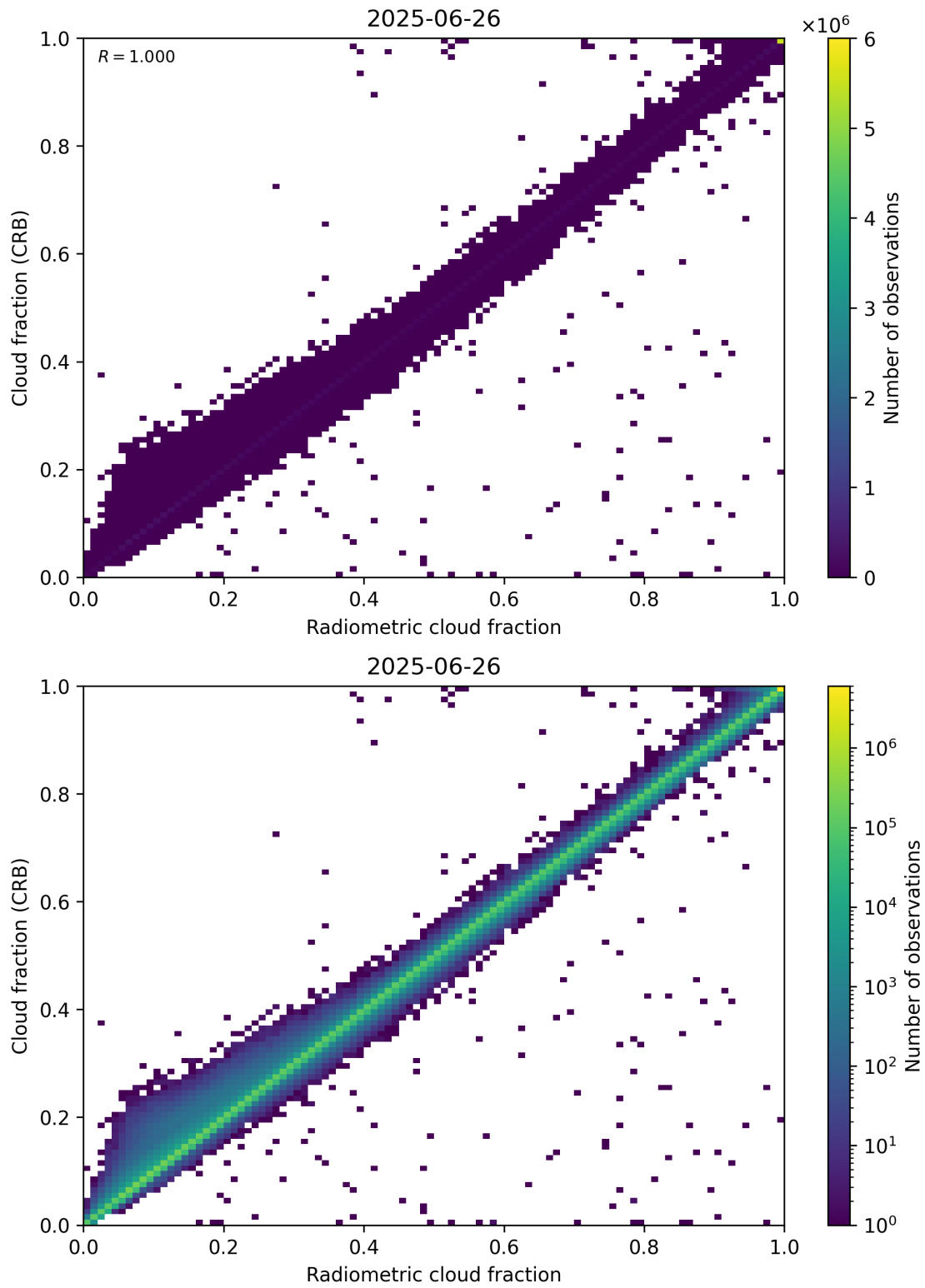
Figure 73: Scatter density plot of “Radiometric cloud fraction” against “Cloud fraction (CRB)” for 2025-06-25 to 2025-06-27.
