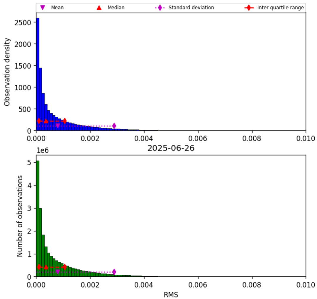
Figure 47: Histogram of “RMS” for 2025-06-25 to 2025-06-27
