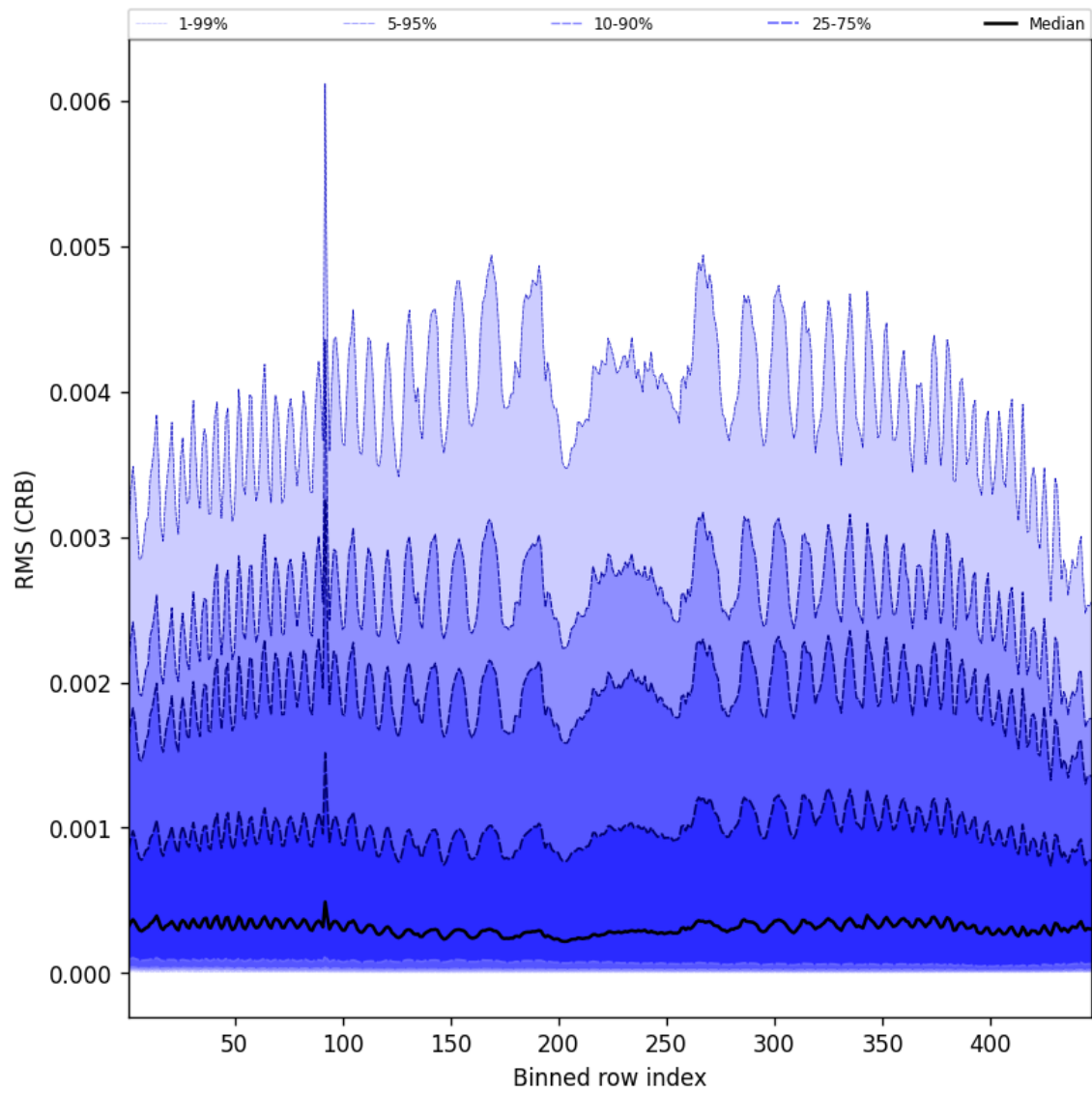
Figure 64: Along track statistics of “RMS (CRB)” for 2025-06-25 to 2025-06-27
