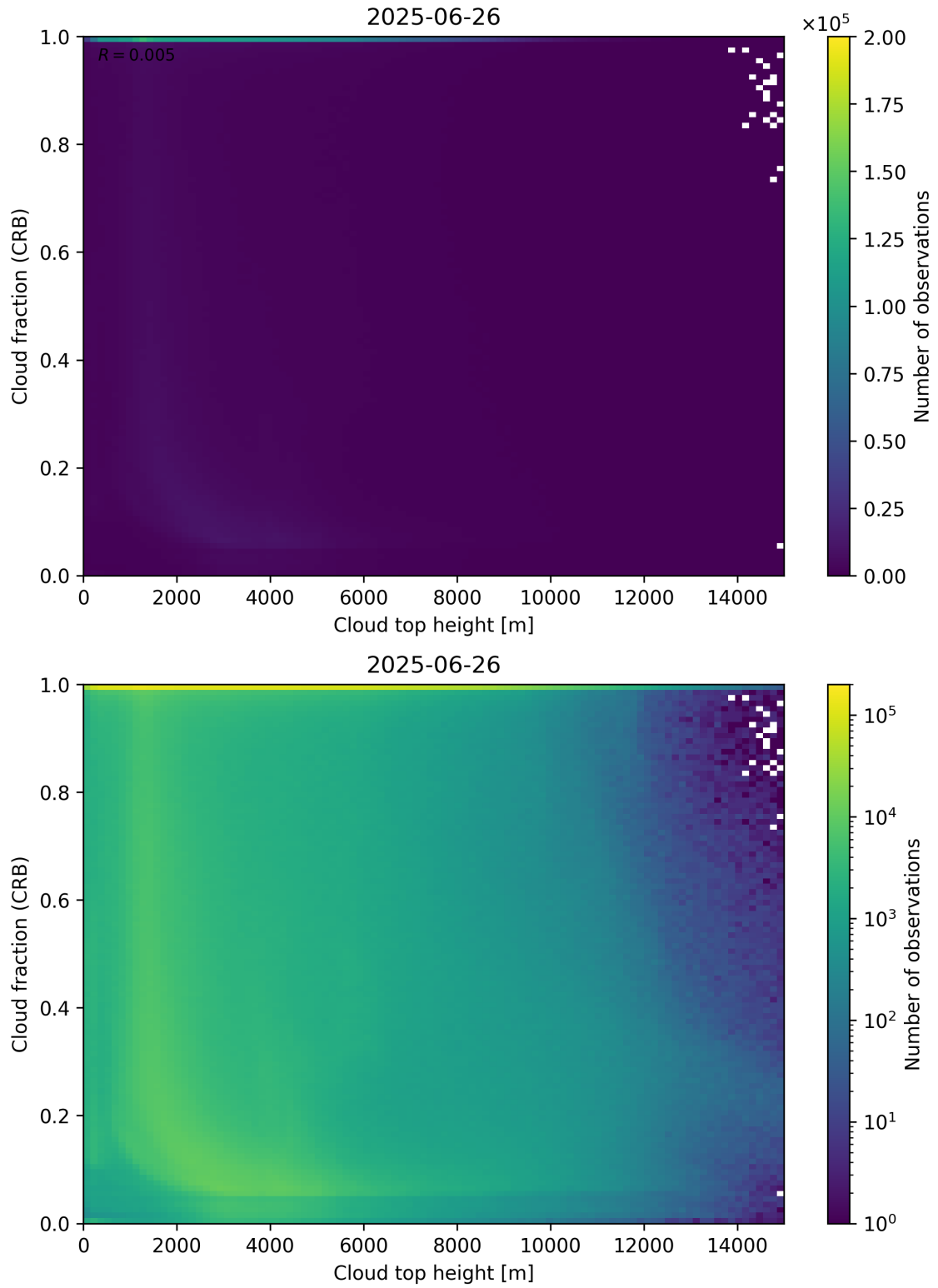
Figure 88: Scatter density plot of “Cloud top height” against “Cloud fraction (CRB)” for 2025-06-25 to 2025-06-27.
