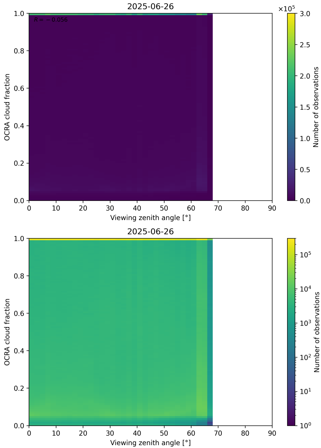
Figure 108: Scatter density plot of “Viewing zenith angle” against “OCRA cloud fraction” for 2025-06-25 to 2025-06-27.
