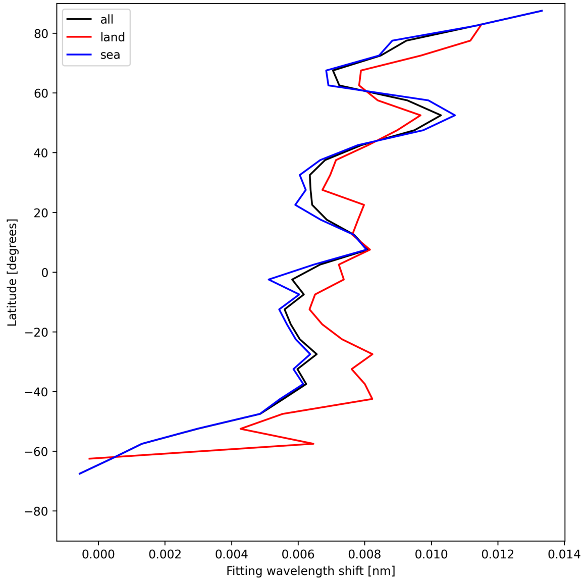
Figure 33: Zonal average of “Fitting wavelength shift” for 2025-06-25 to 2025-06-27.
