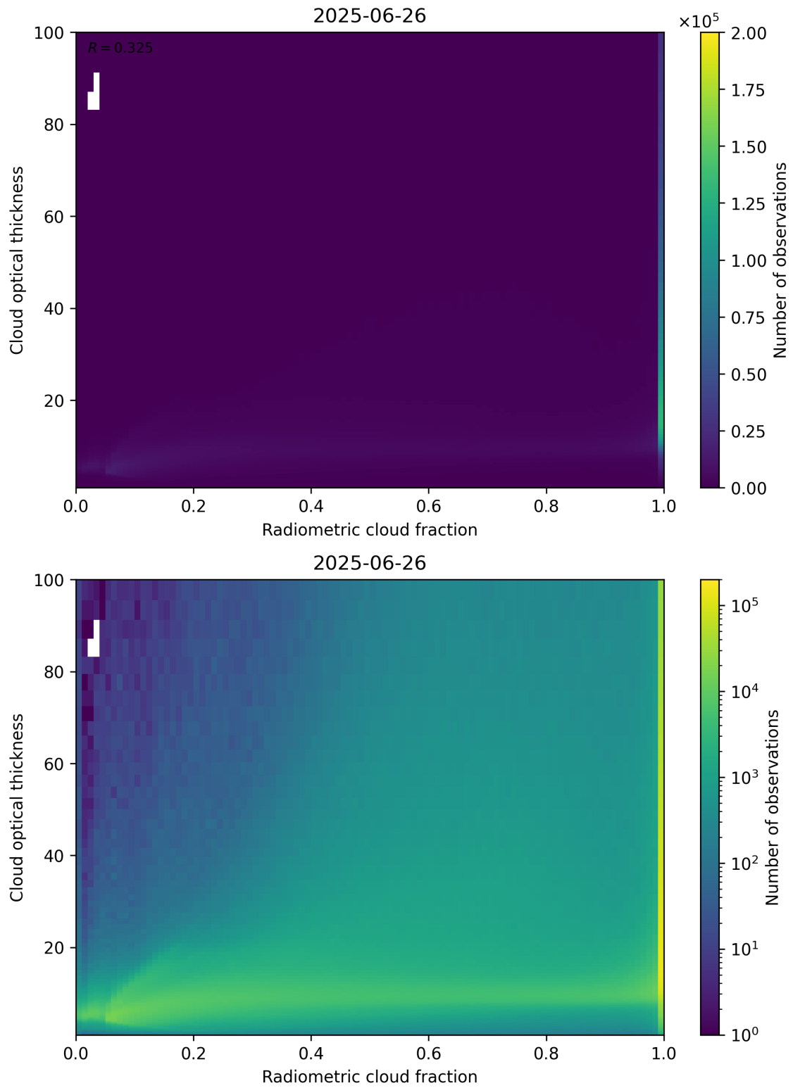
Figure 75: Scatter density plot of “Radiometric cloud fraction” against “Cloud optical thickness” for 2025-06-25 to 2025-06-27.
