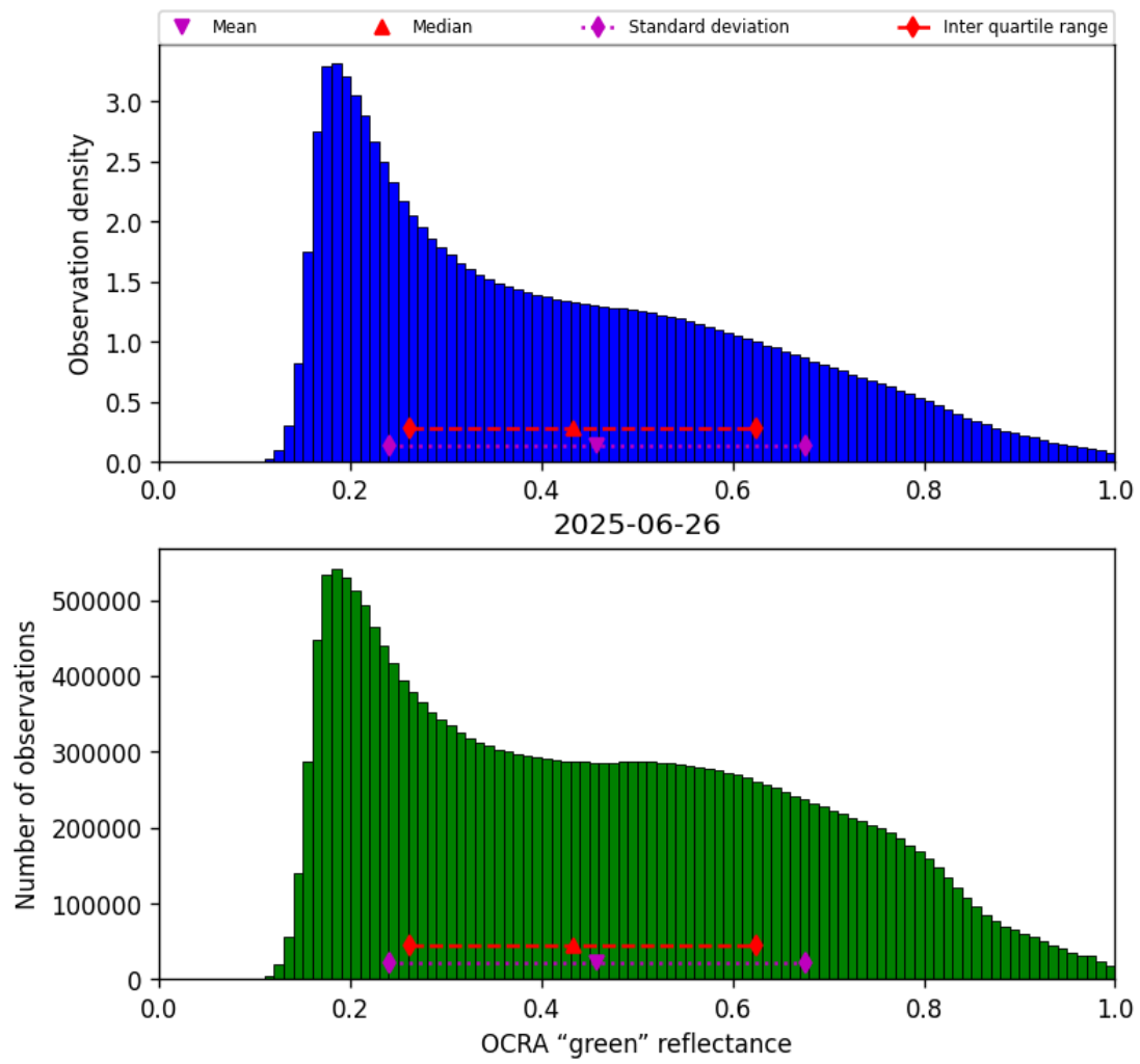
Figure 52: Histogram of “OCRA “green” reflectance” for 2025-06-25 to 2025-06-27
