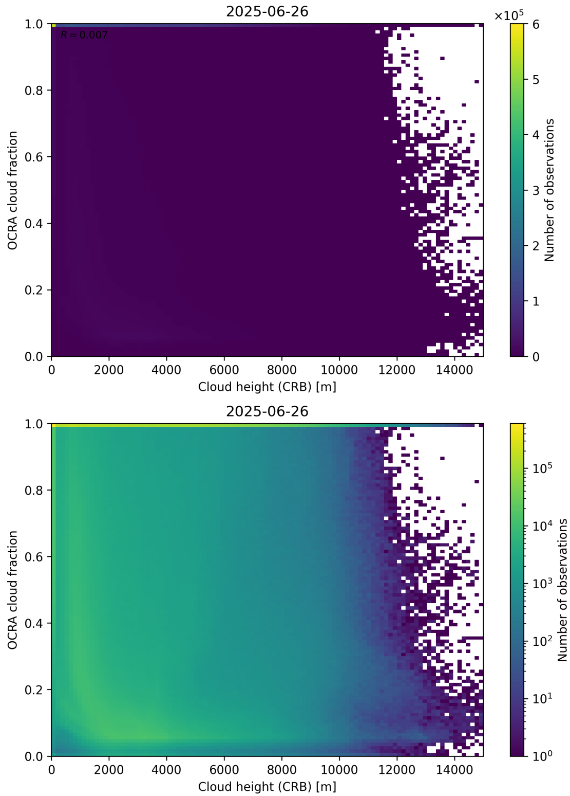
Figure 81: Scatter density plot of “Cloud height (CRB)” against “OCRA cloud fraction” for 2025-06-25 to 2025-06-27.
