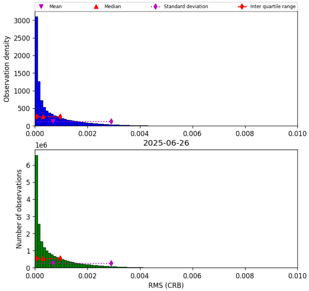
Figure 48: Histogram of “RMS (CRB)” for 2025-06-25 to 2025-06-27
