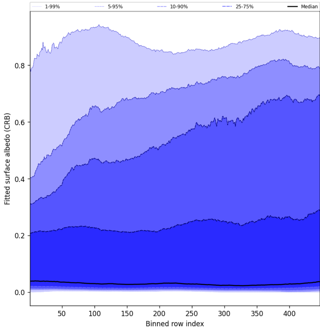
Figure 62: Along track statistics of “Fitted surface albedo (CRB)” for 2025-06-25 to 2025-06-27
