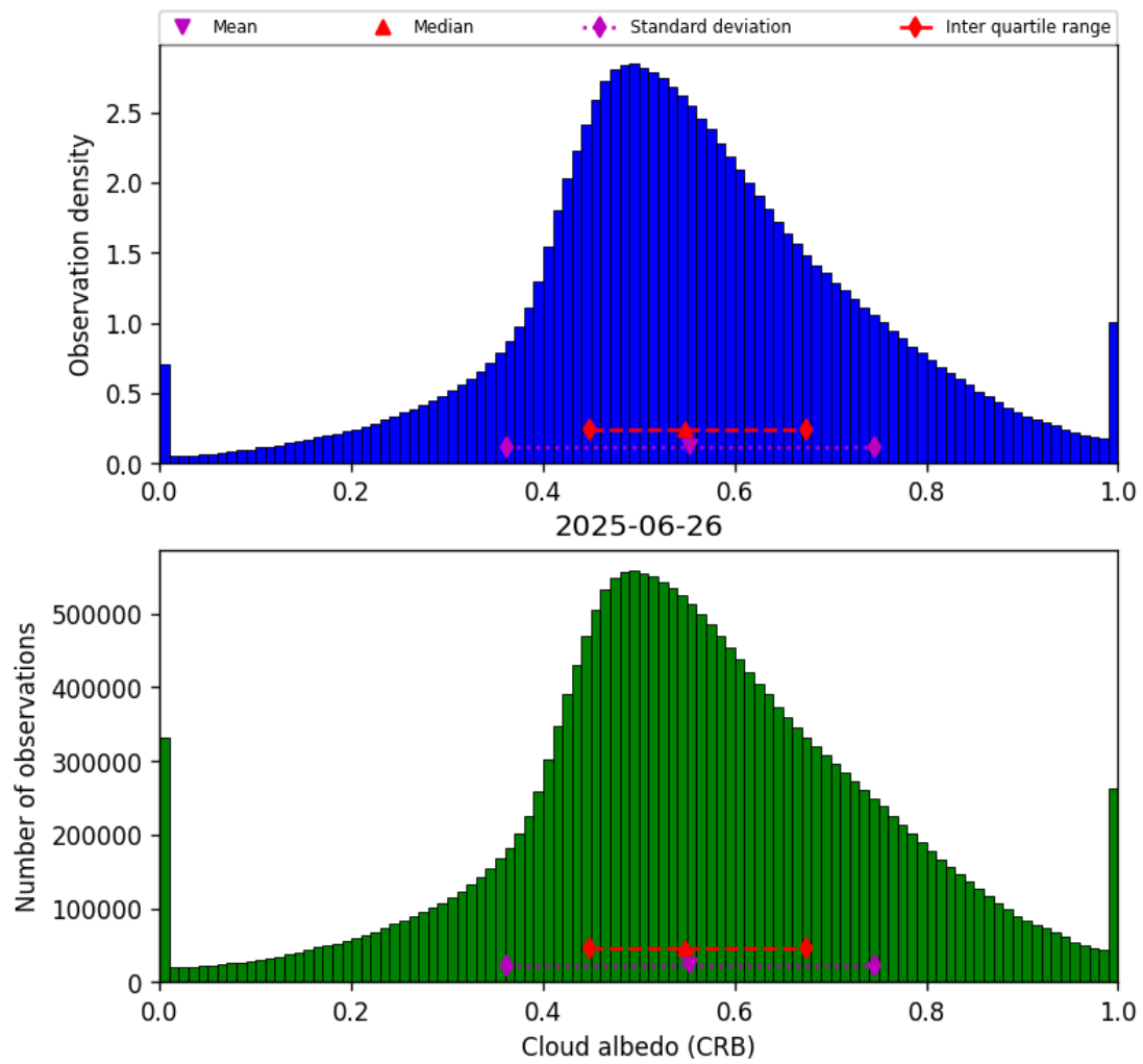
Figure 44: Histogram of “Cloud albedo (CRB)” for 2025-06-25 to 2025-06-27
