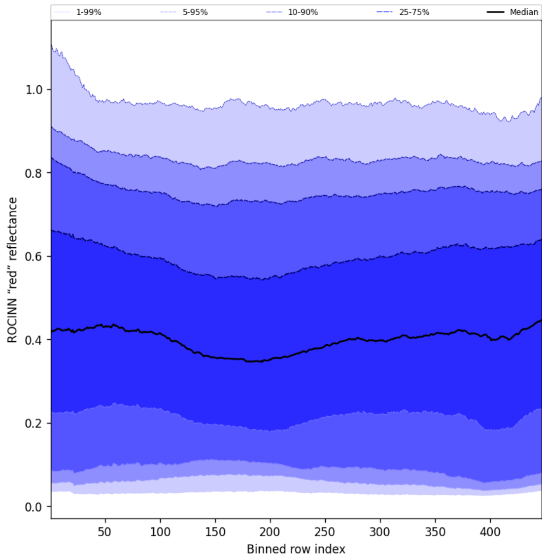
Figure 69: Along track statistics of “ROCINN “red” reflectance” for 2025-06-25 to 2025-06-27
