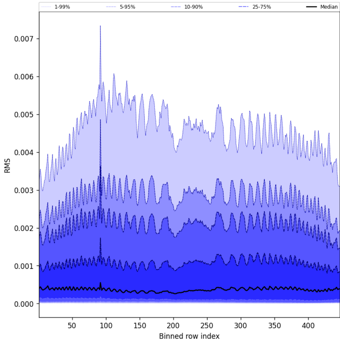
Figure 63: Along track statistics of “RMS” for 2025-06-25 to 2025-06-27
