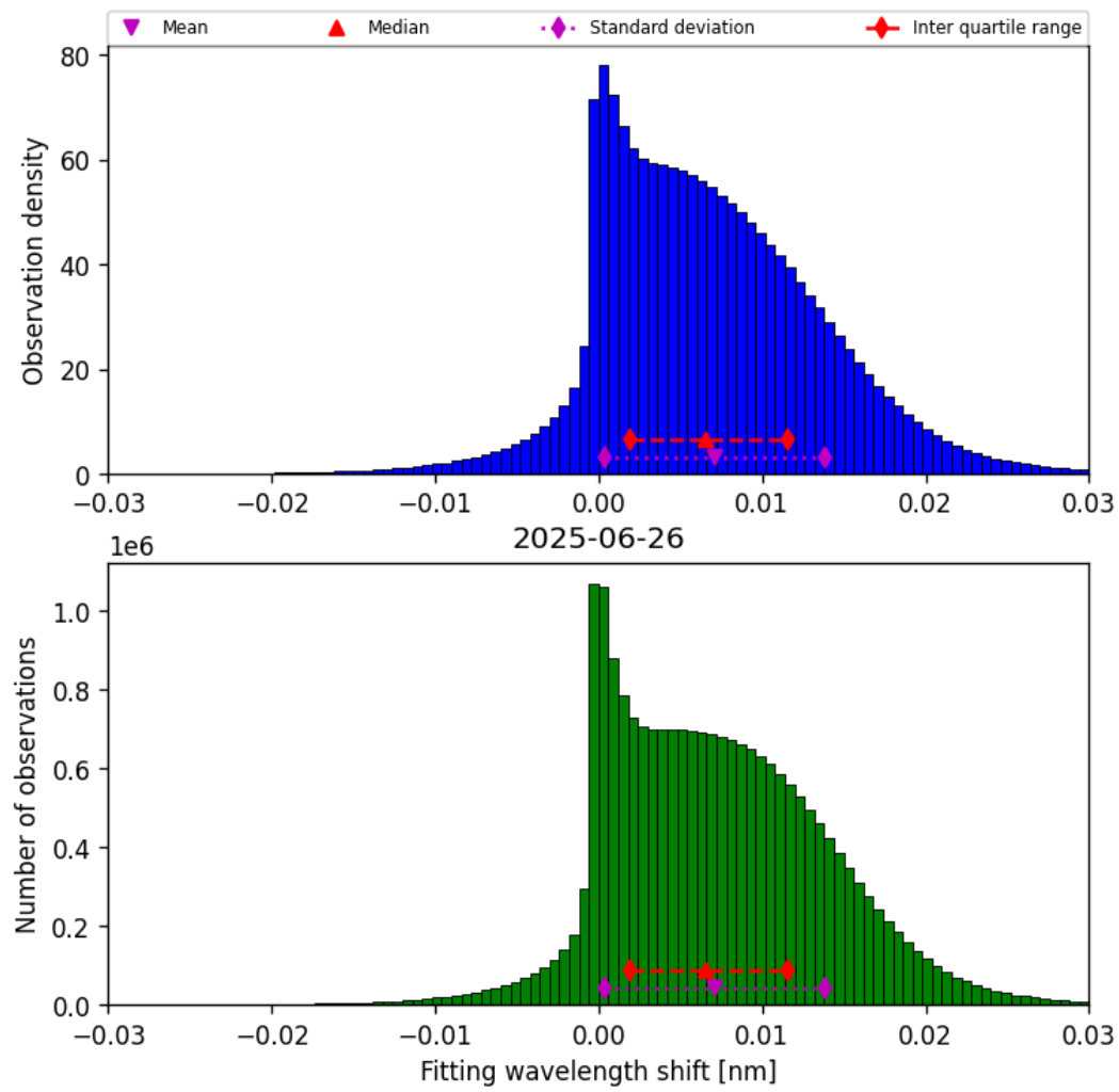
Figure 49: Histogram of “Fitting wavelength shift” for 2025-06-25 to 2025-06-27
