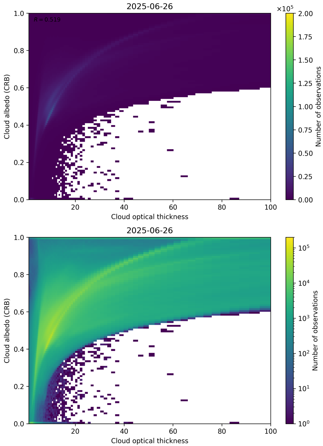
Figure 82: Scatter density plot of “Cloud optical thickness” against “Cloud albedo (CRB)” for 2025-06-25 to 2025-06-27.
