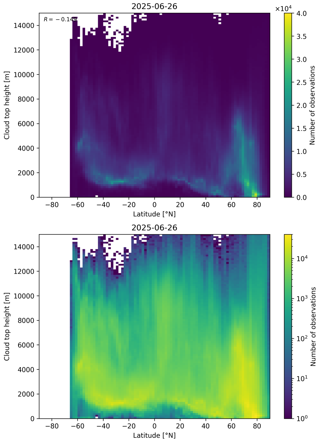
Figure 97: Scatter density plot of “Latitude” against “Cloud top height” for 2025-06-25 to 2025-06-27.
