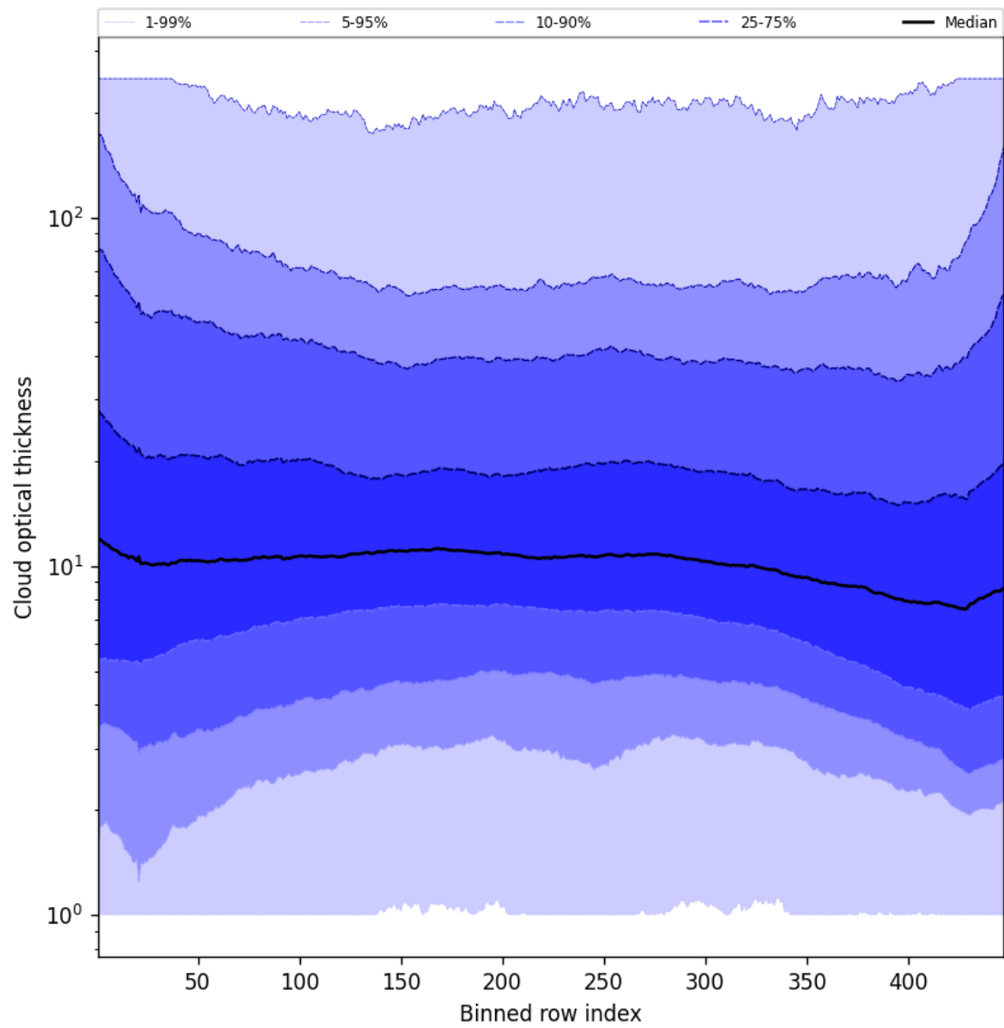
Figure 57: Along track statistics of “Cloud optical thickness” for 2025-06-25 to 2025-06-27
