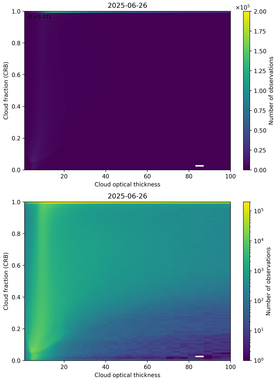
Figure 84: Scatter density plot of “Cloud optical thickness” against “Cloud fraction (CRB)” for 2025-06-25 to 2025-06-27.
