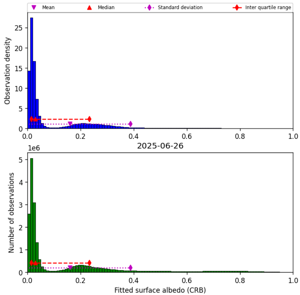
Figure 46: Histogram of “Fitted surface albedo (CRB)” for 2025-06-25 to 2025-06-27
