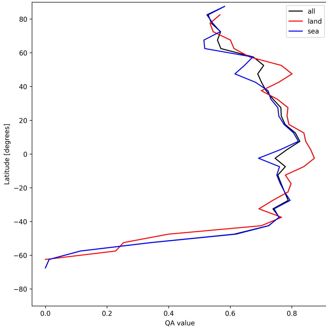
Figure 22: Zonal average of “QA value” for 2025-06-25 to 2025-06-27.
