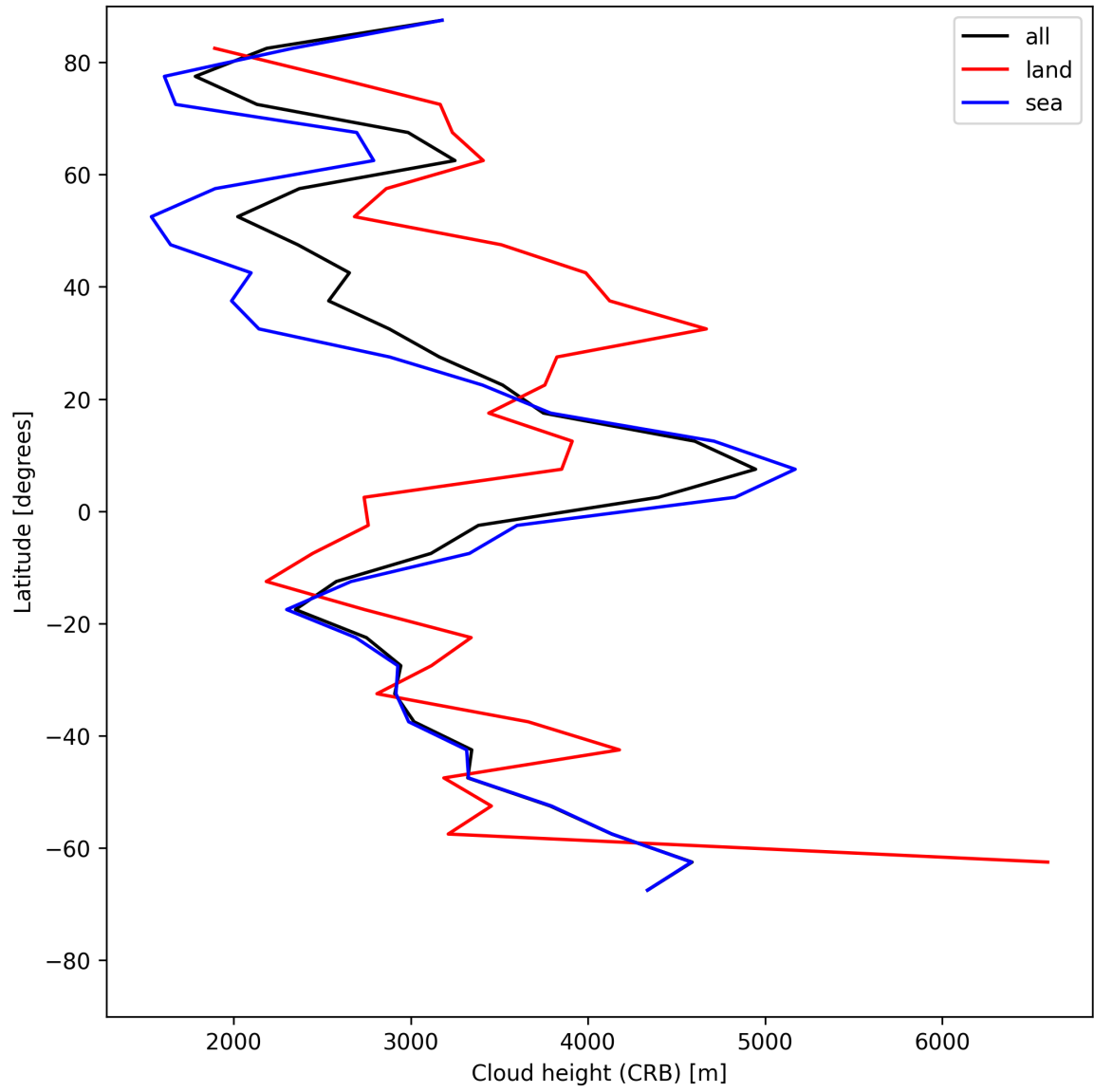
Figure 27: Zonal average of “Cloud height (CRB)” for 2025-06-25 to 2025-06-27.
