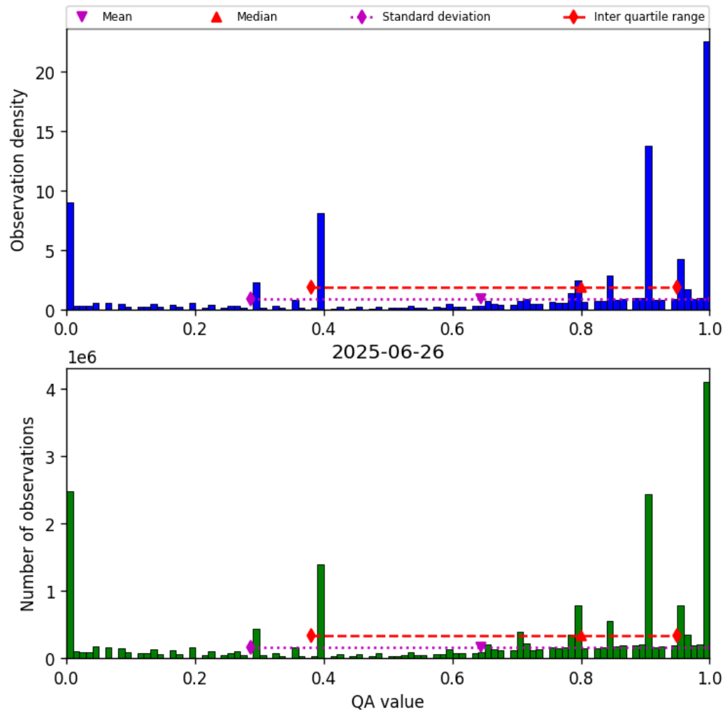
Figure 38: Histogram of “QA value” for 2025-06-25 to 2025-06-27
