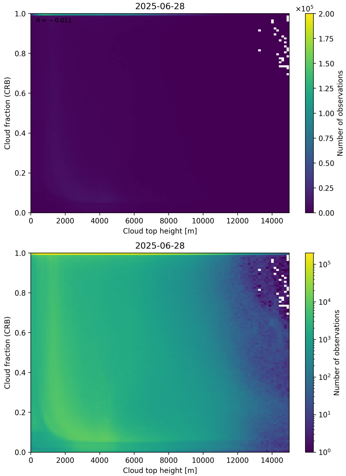
Figure 88: Scatter density plot of “Cloud top height” against “Cloud fraction (CRB)” for 2025-06-27 to 2025-06-29.
