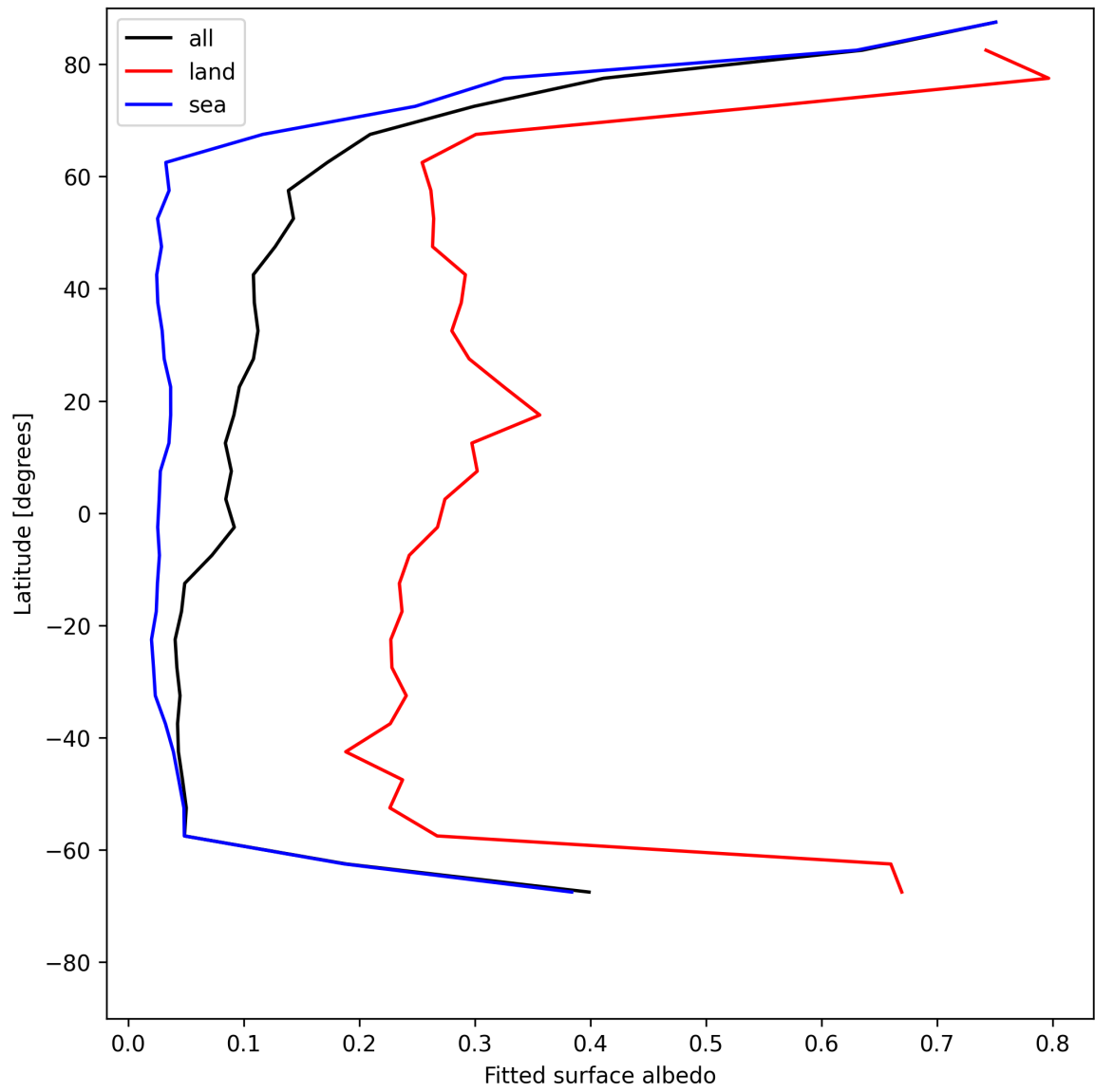
Figure 29: Zonal average of “Fitted surface albedo” for 2025-06-27 to 2025-06-29.
