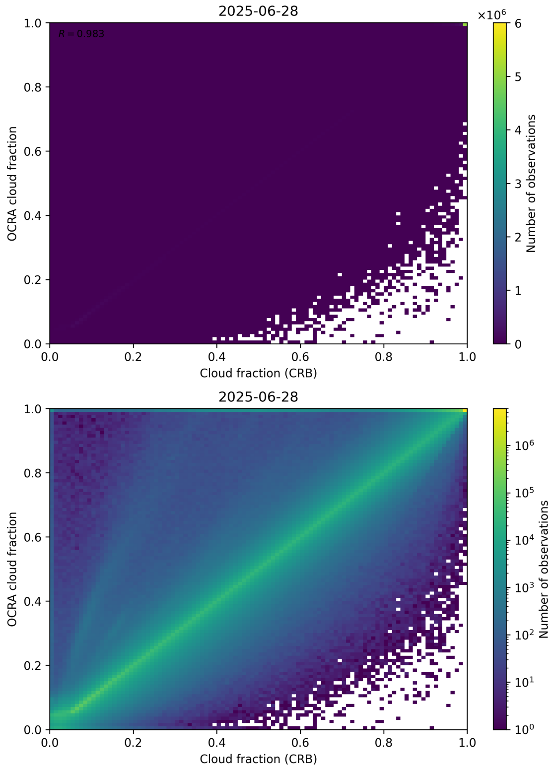
Figure 78: Scatter density plot of “Cloud fraction (CRB)” against “OCRA cloud fraction” for 2025-06-27 to 2025-06-29.
