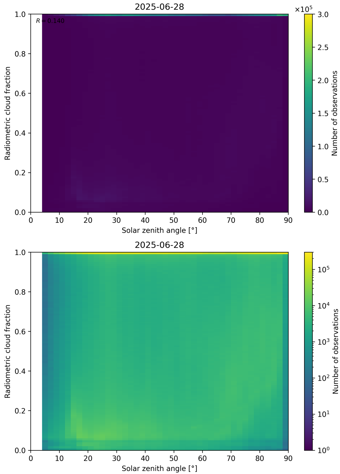
Figure 99: Scatter density plot of “Solar zenith angle” against “Radiometric cloud fraction” for 2025-06-27 to 2025-06-29.
