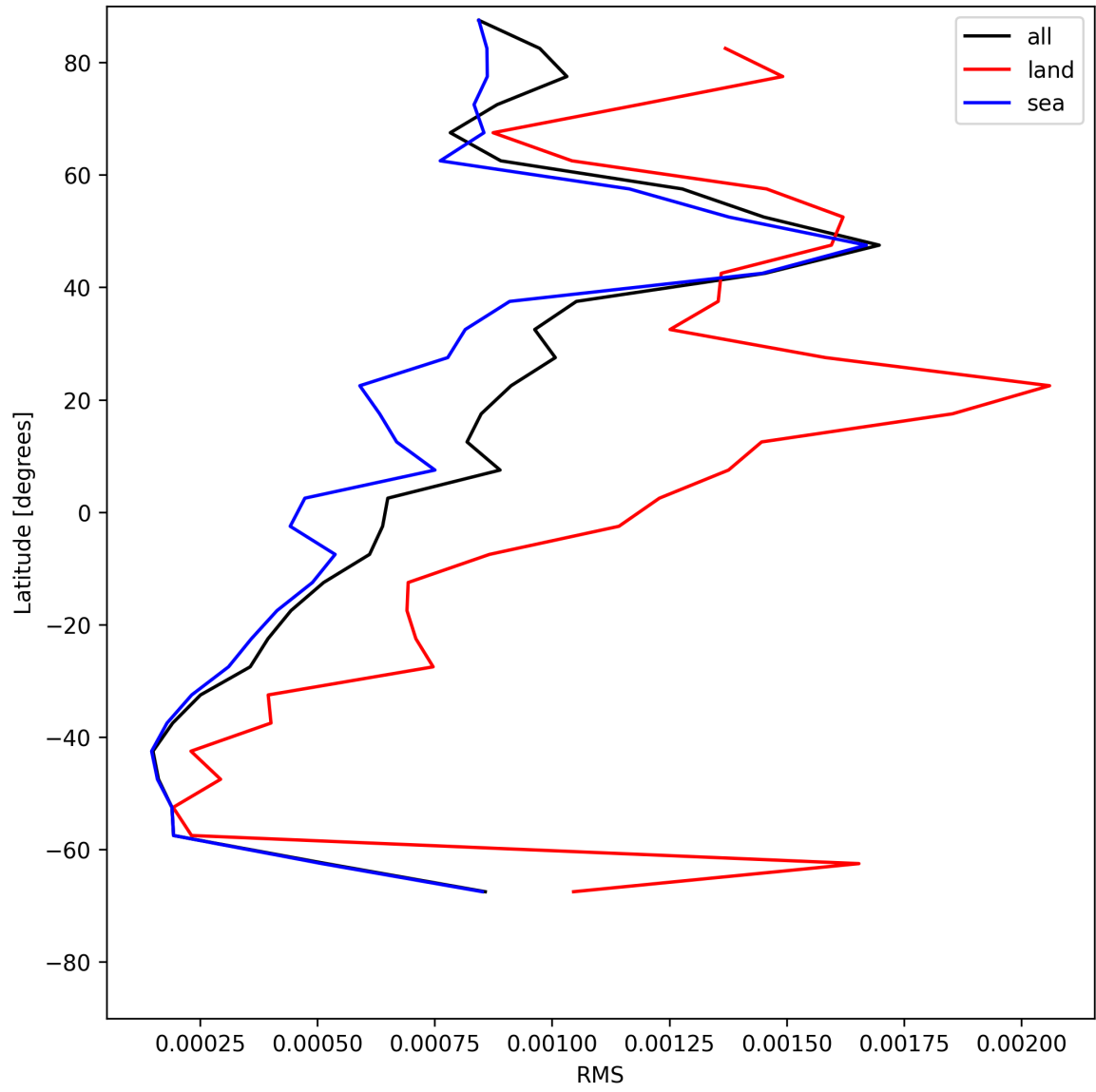
Figure 31: Zonal average of “RMS” for 2025-06-27 to 2025-06-29.
