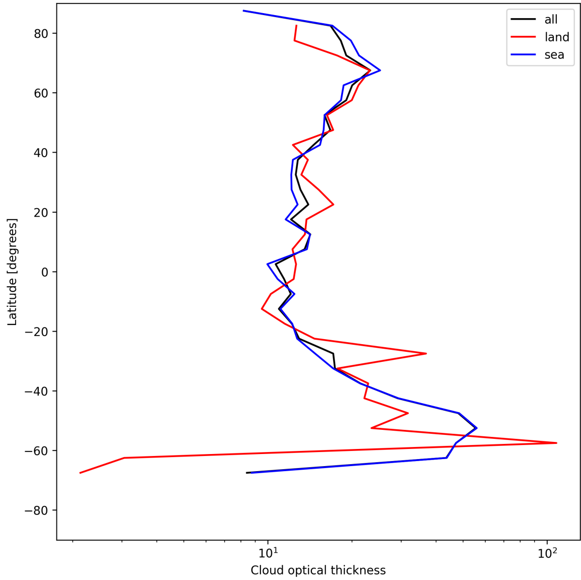
Figure 25: Zonal average of “Cloud optical thickness” for 2025-06-27 to 2025-06-29.
