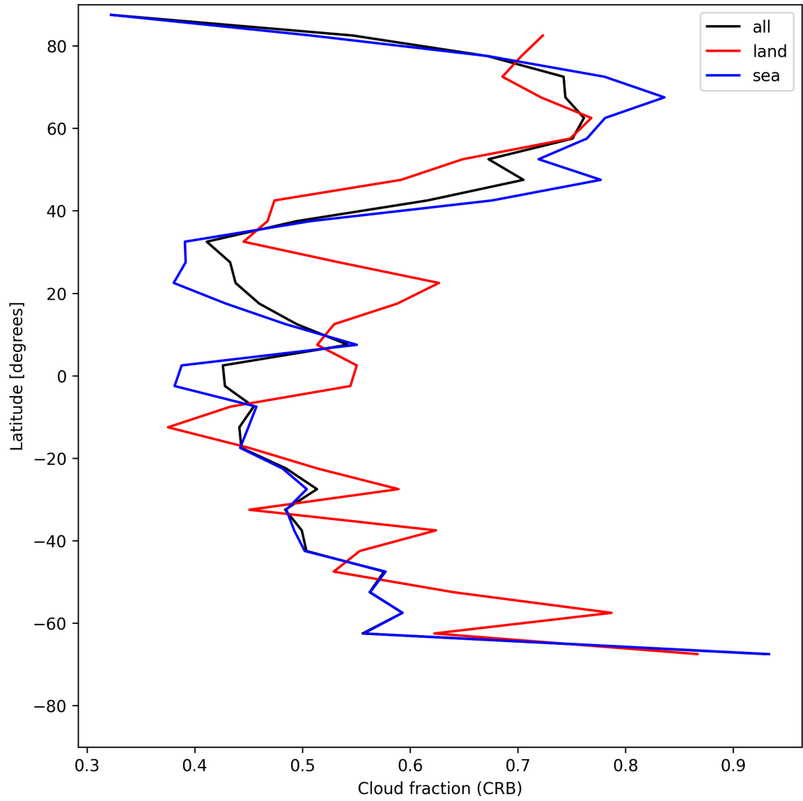
Figure 26: Zonal average of “Cloud fraction (CRB)” for 2025-06-27 to 2025-06-29.
