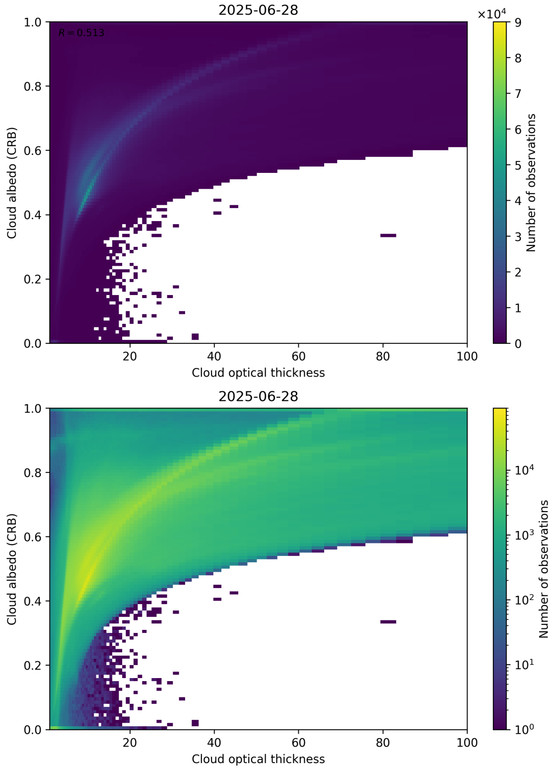
Figure 82: Scatter density plot of “Cloud optical thickness” against “Cloud albedo (CRB)” for 2025-06-27 to 2025-06-29.
