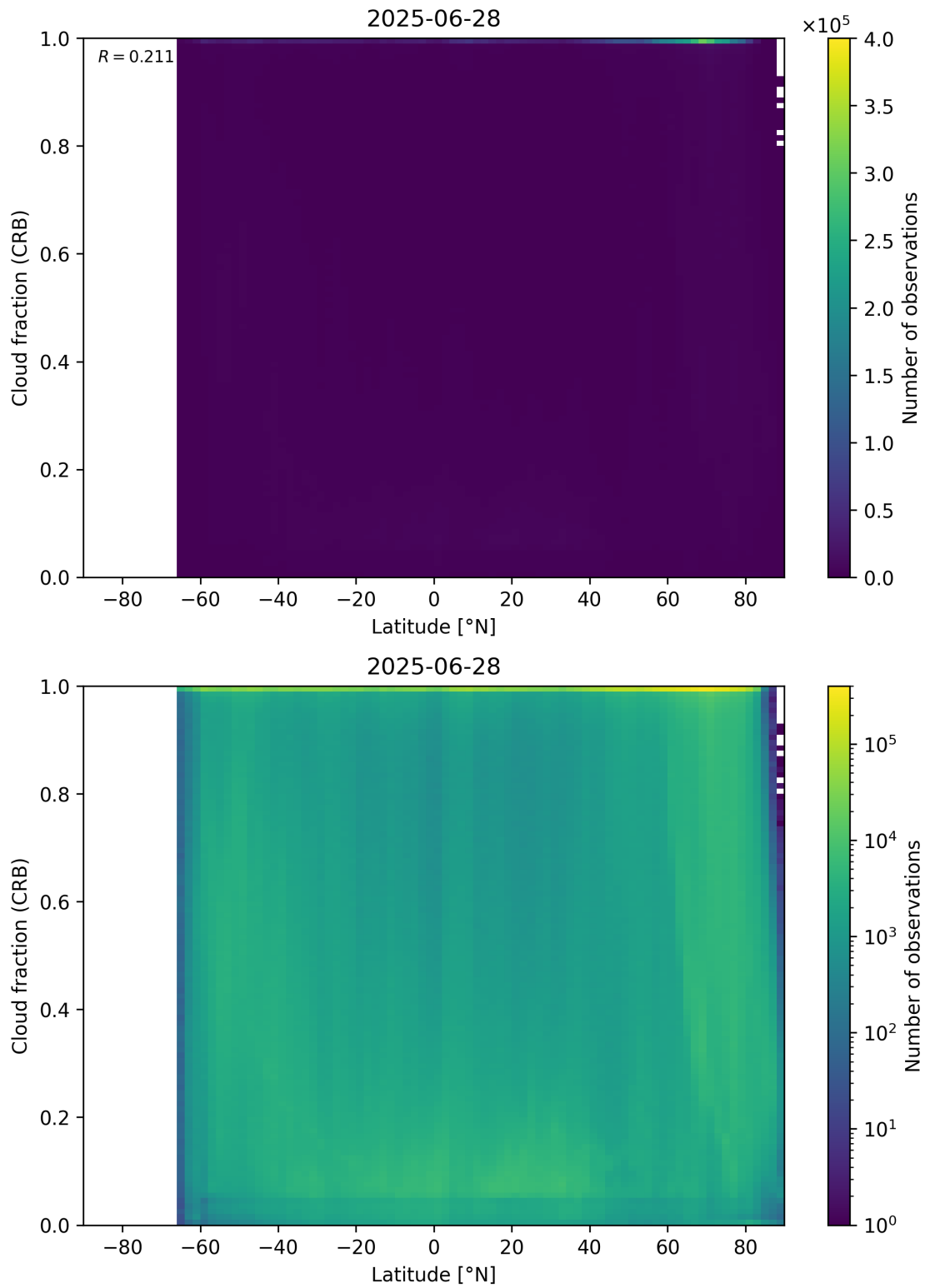
Figure 94: Scatter density plot of “Latitude” against “Cloud fraction (CRB)” for 2025-06-27 to 2025-06-29.
