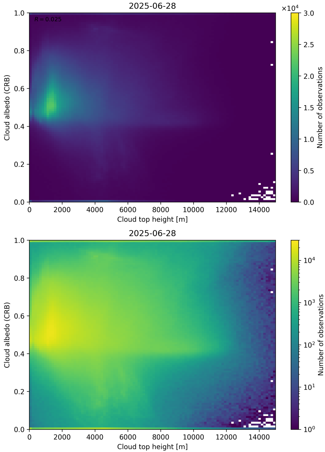
Figure 86: Scatter density plot of “Cloud top height” against “Cloud albedo (CRB)” for 2025-06-27 to 2025-06-29.
