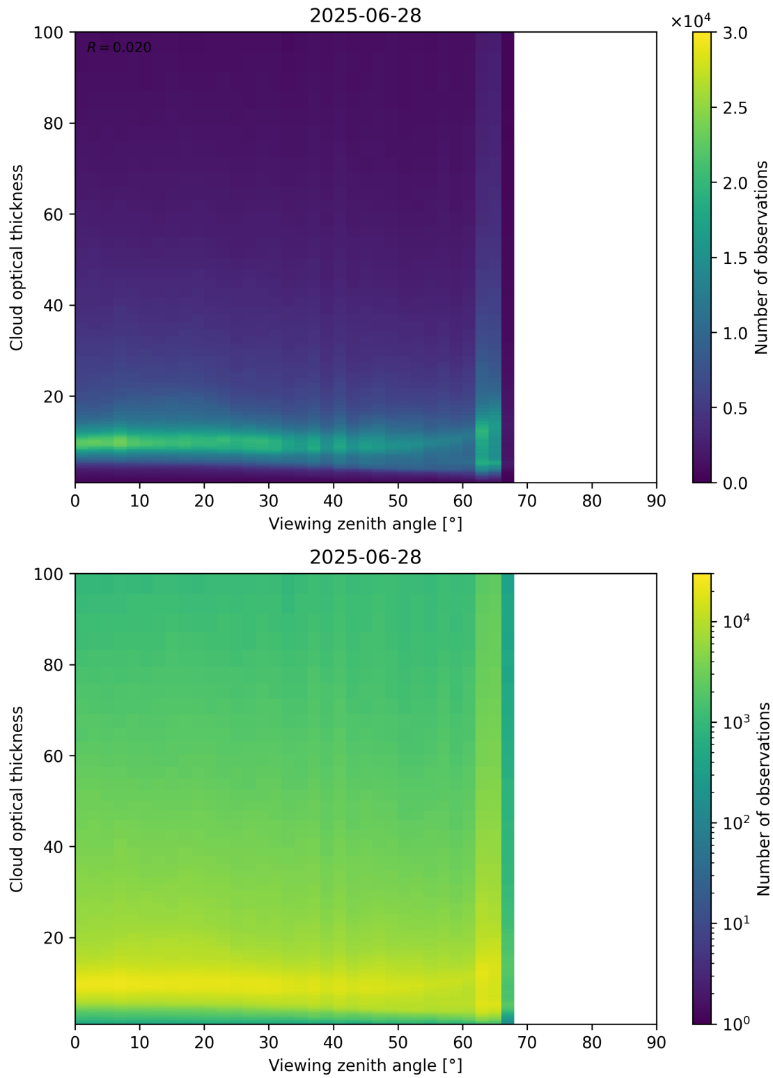
Figure 111: Scatter density plot of “Viewing zenith angle” against “Cloud optical thickness” for 2025-06-27 to 2025-06-29.
