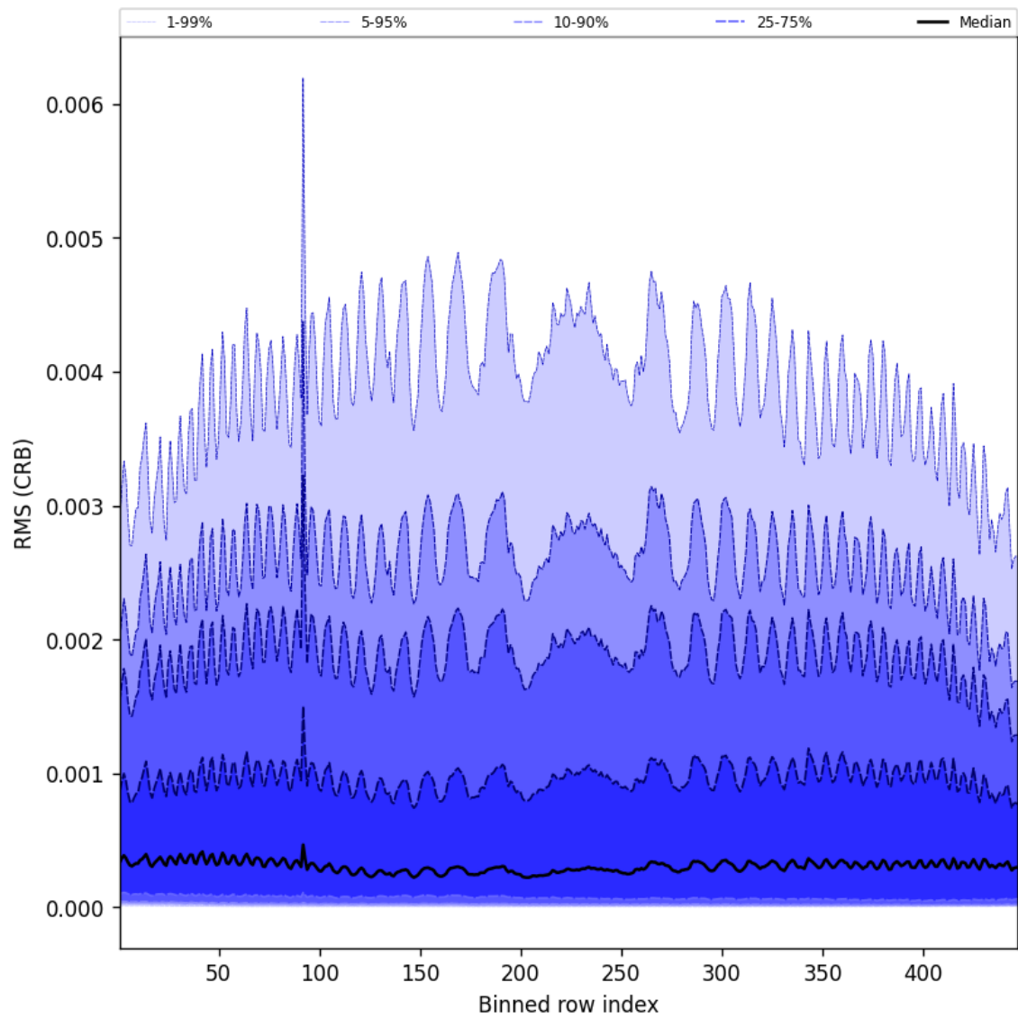
Figure 64: Along track statistics of “RMS (CRB)” for 2025-06-27 to 2025-06-29
