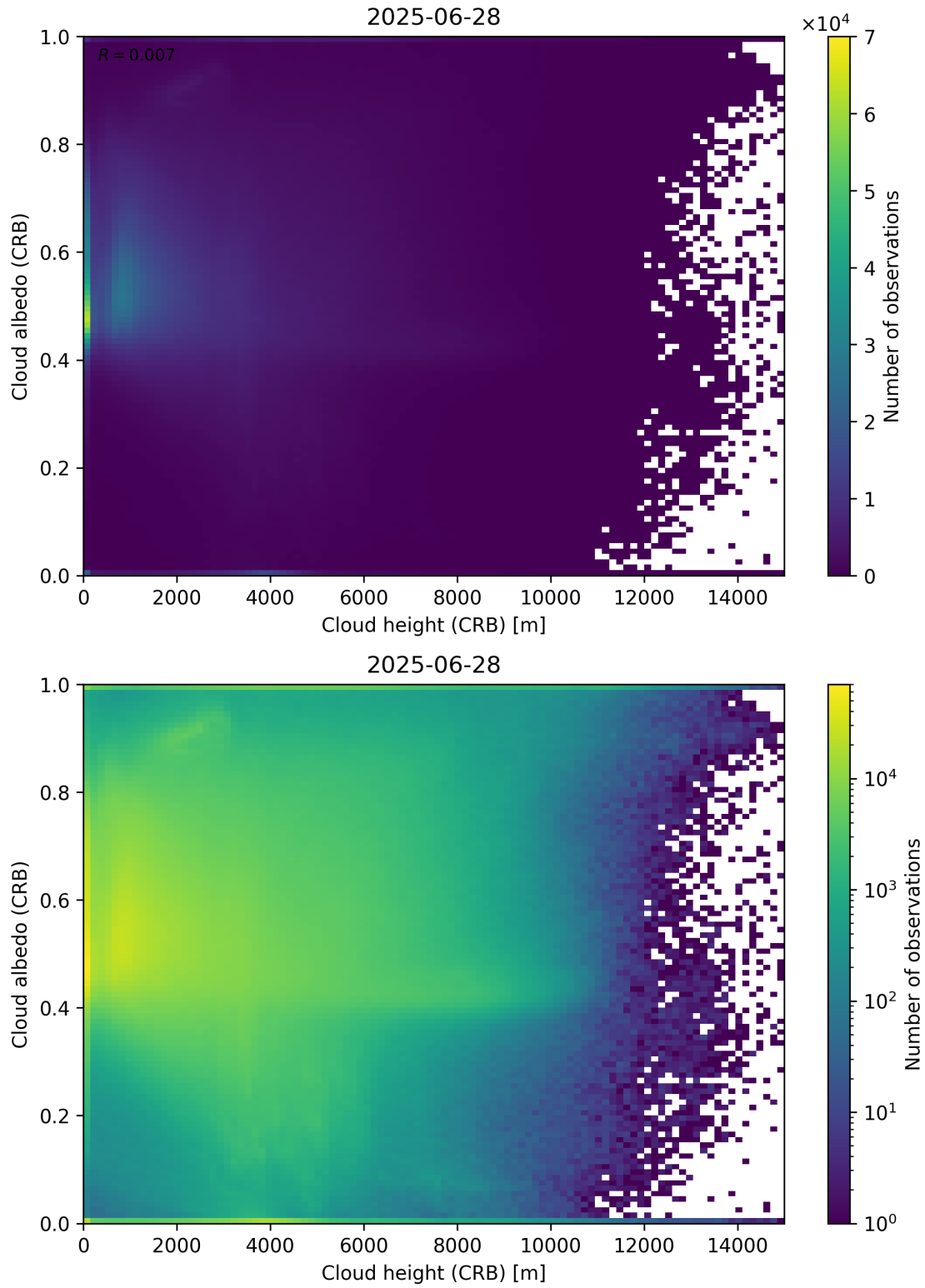
Figure 80: Scatter density plot of “Cloud height (CRB)” against “Cloud albedo (CRB)” for 2025-06-27 to 2025-06-29.
