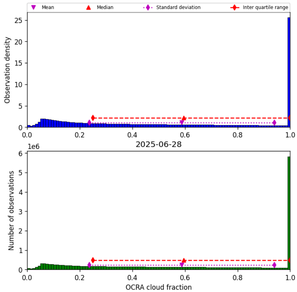
Figure 50: Histogram of “OCRA cloud fraction” for 2025-06-27 to 2025-06-29
