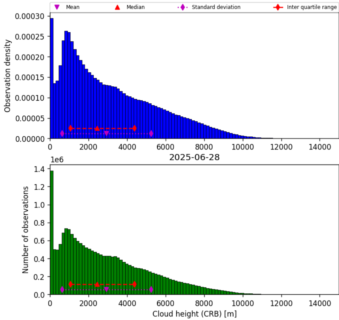
Figure 43: Histogram of “Cloud height (CRB)” for 2025-06-27 to 2025-06-29
