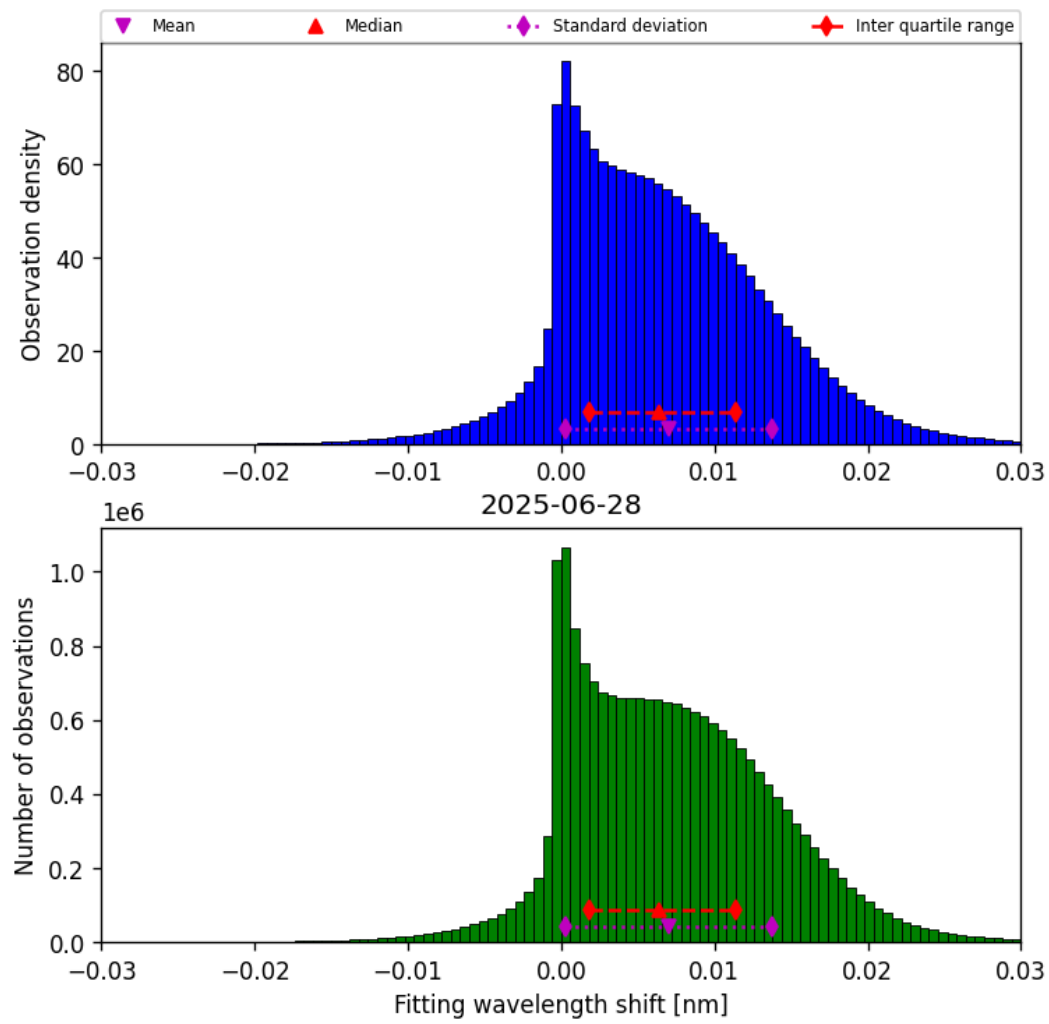
Figure 49: Histogram of “Fitting wavelength shift” for 2025-06-27 to 2025-06-29
