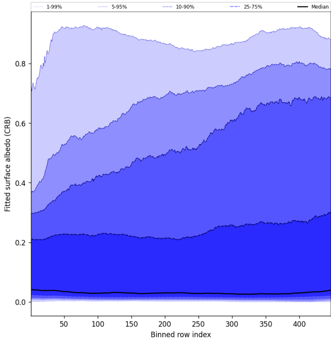
Figure 62: Along track statistics of “Fitted surface albedo (CRB)” for 2025-06-27 to 2025-06-29
