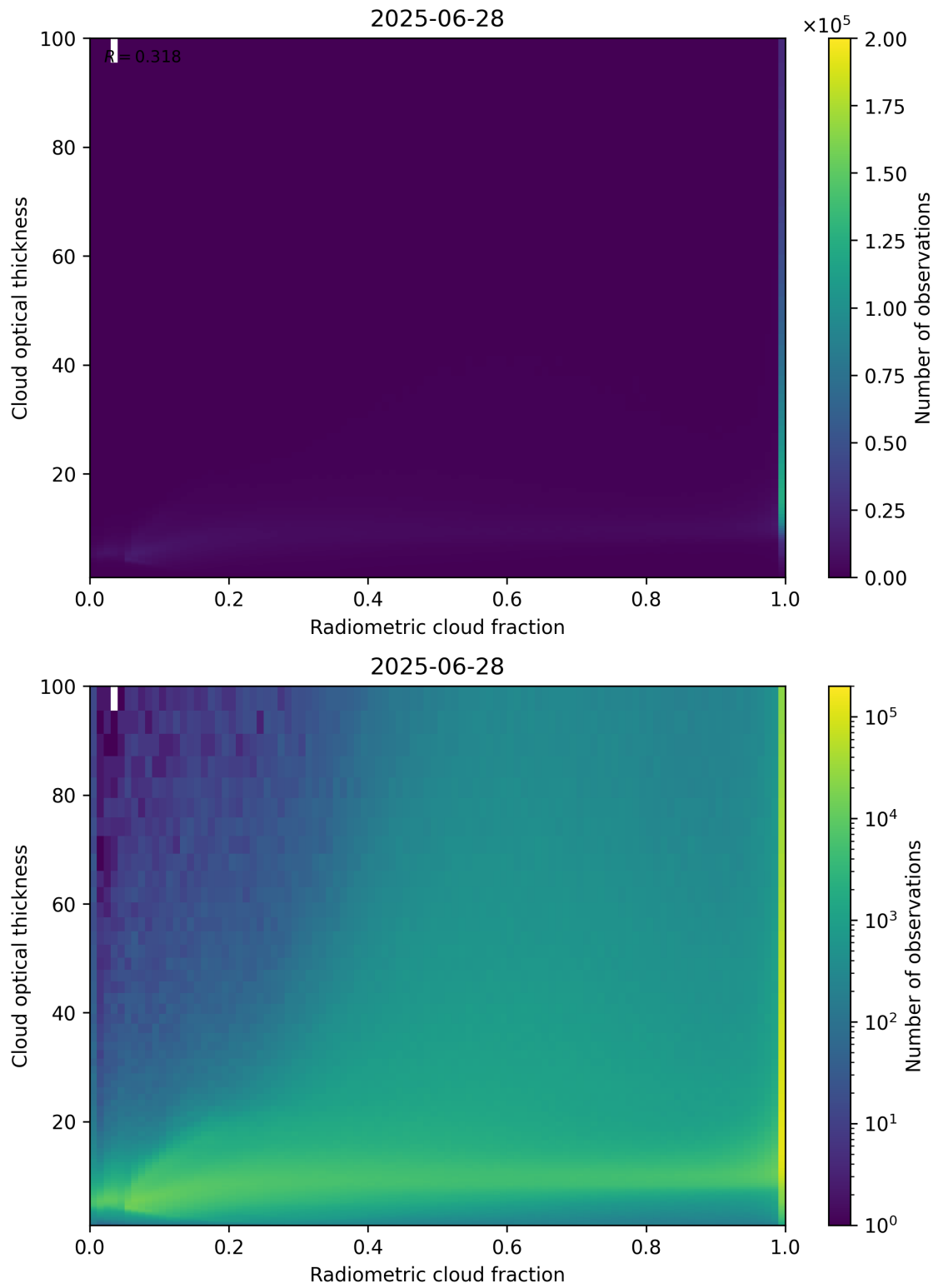
Figure 75: Scatter density plot of “Radiometric cloud fraction” against “Cloud optical thickness” for 2025-06-27 to 2025-06-29.
