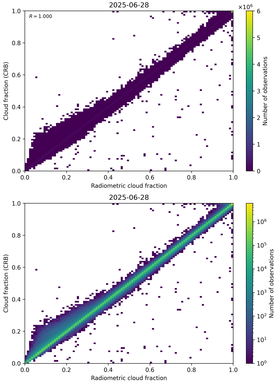
Figure 73: Scatter density plot of “Radiometric cloud fraction” against “Cloud fraction (CRB)” for 2025-06-27 to 2025-06-29.
