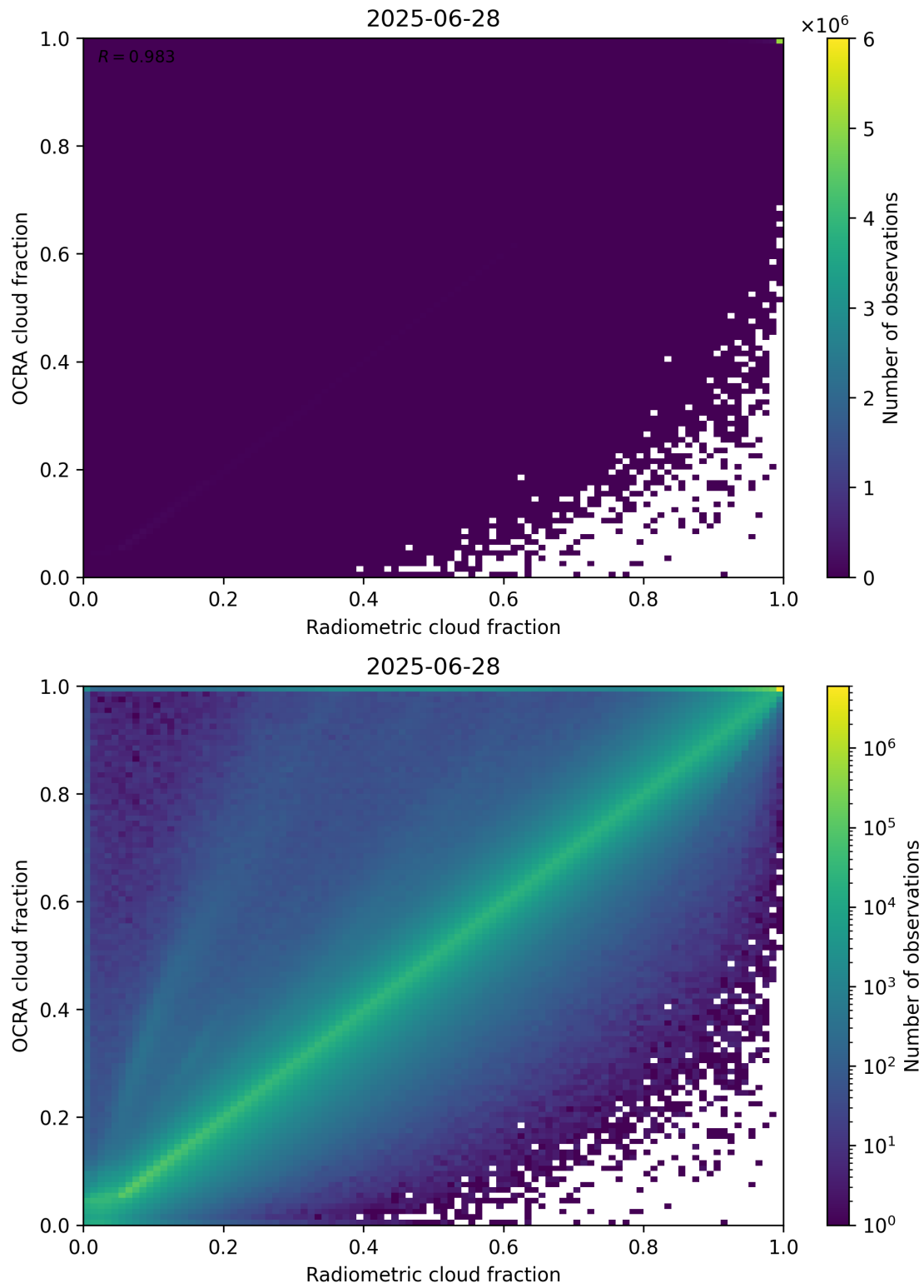
Figure 72: Scatter density plot of “Radiometric cloud fraction” against “OCRA cloud fraction” for 2025-06-27 to 2025-06-29.
