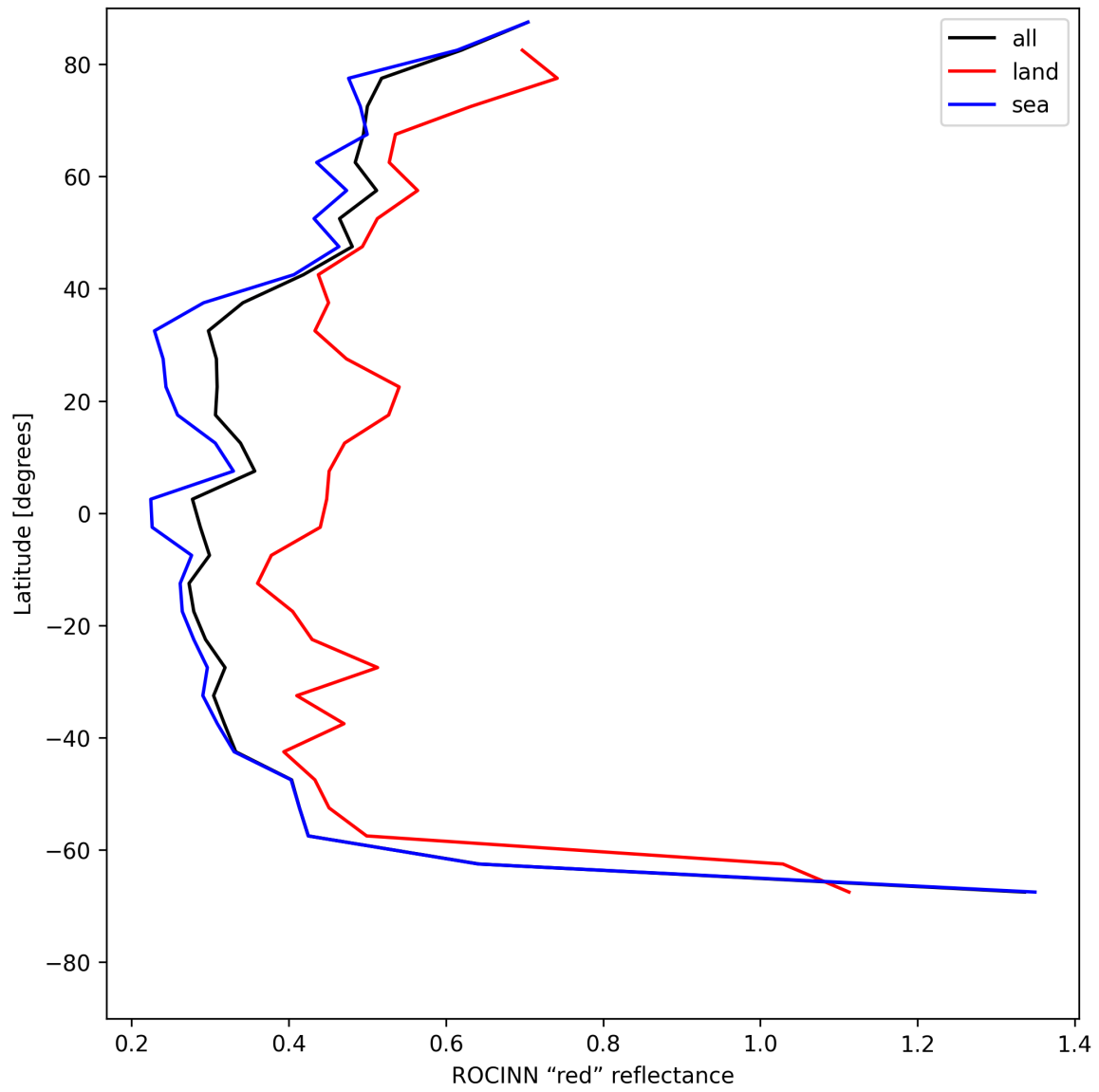
Figure 37: Zonal average of “ROCINN “red” reflectance” for 2025-06-27 to 2025-06-29.
