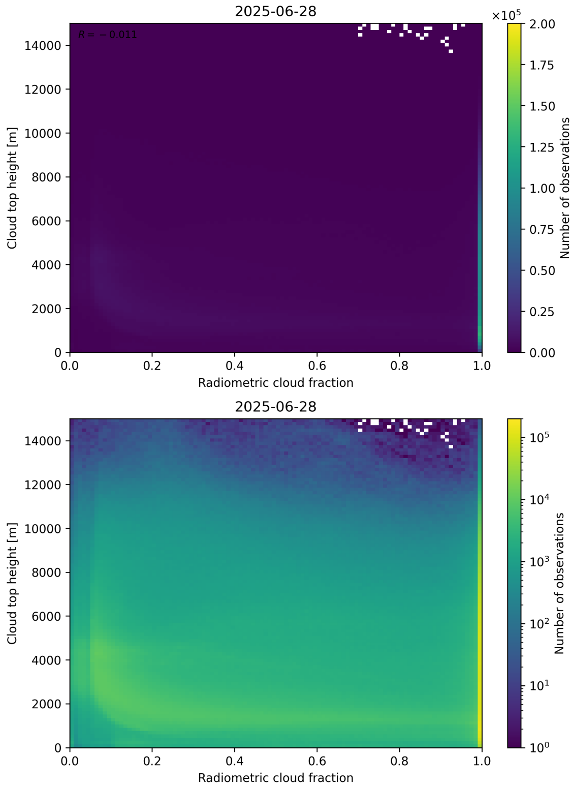
Figure 76: Scatter density plot of “Radiometric cloud fraction” against “Cloud top height” for 2025-06-27 to 2025-06-29.
