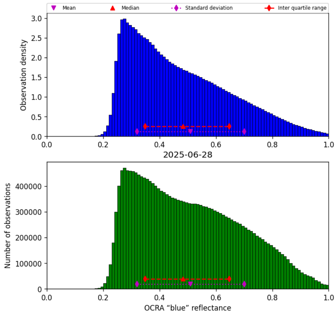
Figure 51: Histogram of “OCRA “blue” reflectance” for 2025-06-27 to 2025-06-29
