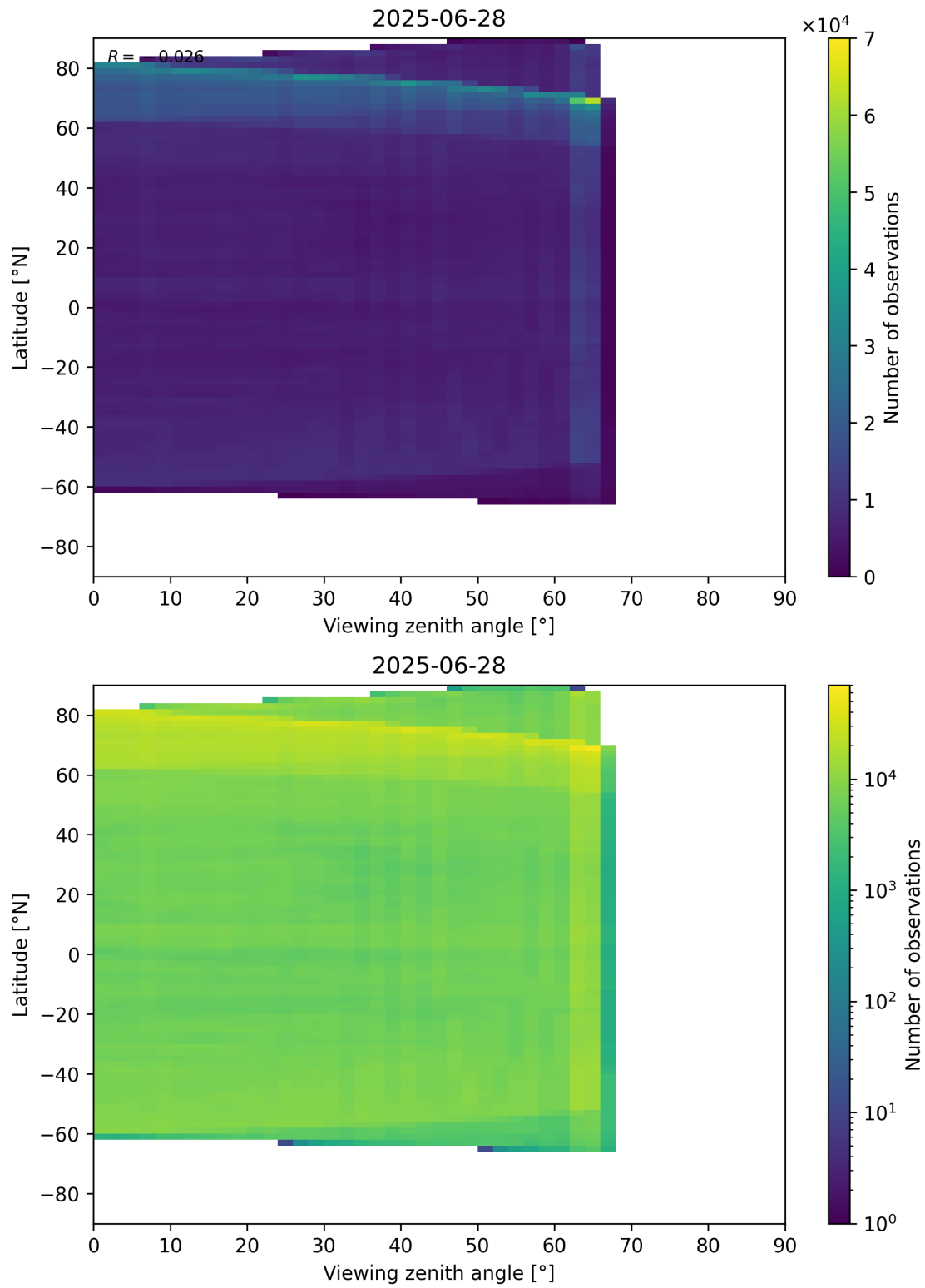
Figure 113: Scatter density plot of “Viewing zenith angle” against “Latitude” for 2025-06-27 to 2025-06-29.
