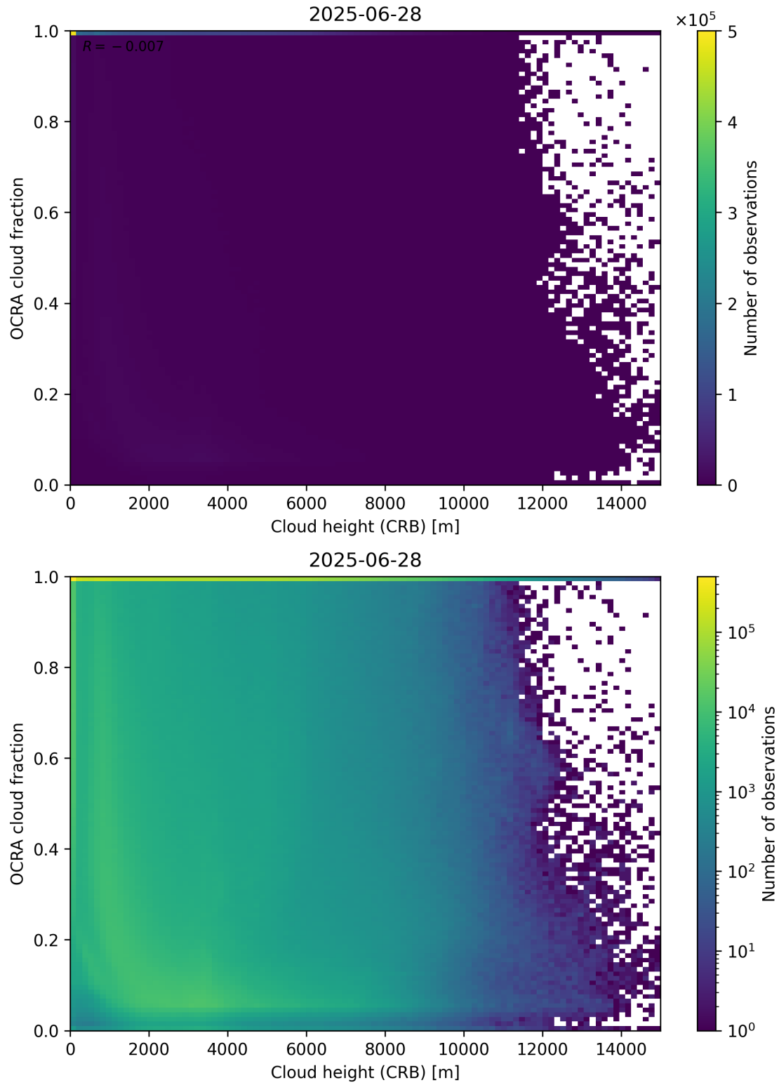
Figure 81: Scatter density plot of “Cloud height (CRB)” against “OCRA cloud fraction” for 2025-06-27 to 2025-06-29.
