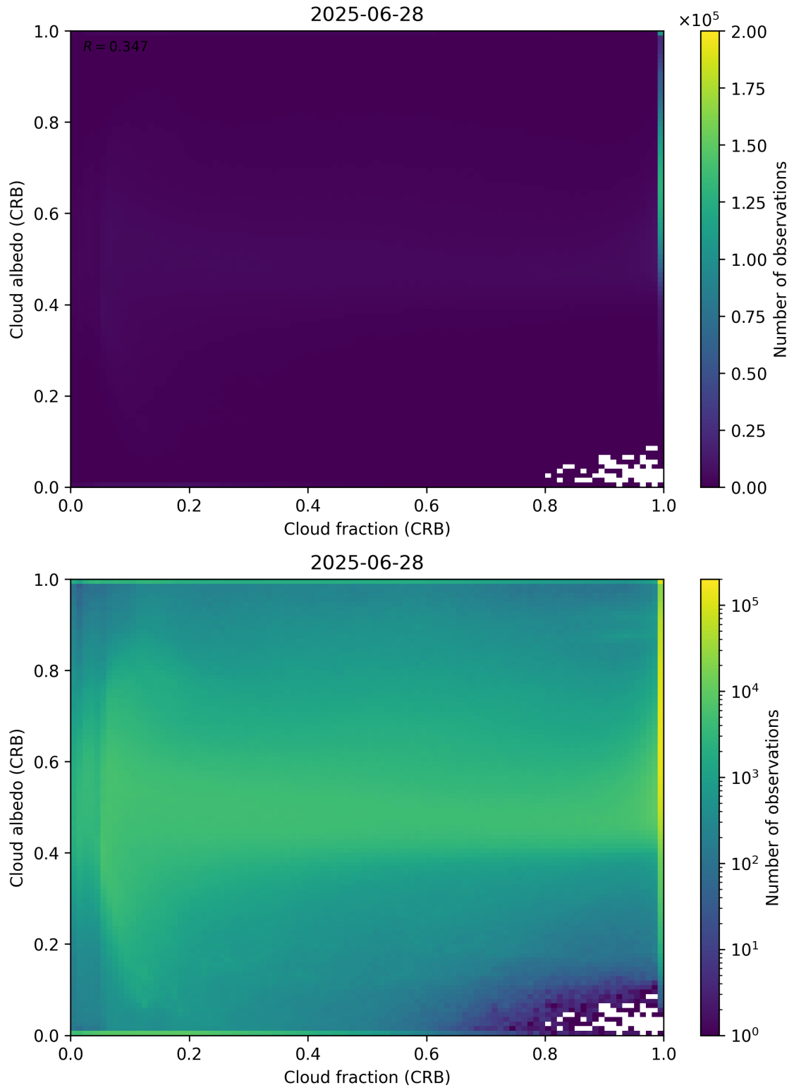
Figure 77: Scatter density plot of “Cloud fraction (CRB)” against “Cloud albedo (CRB)” for 2025-06-27 to 2025-06-29.
