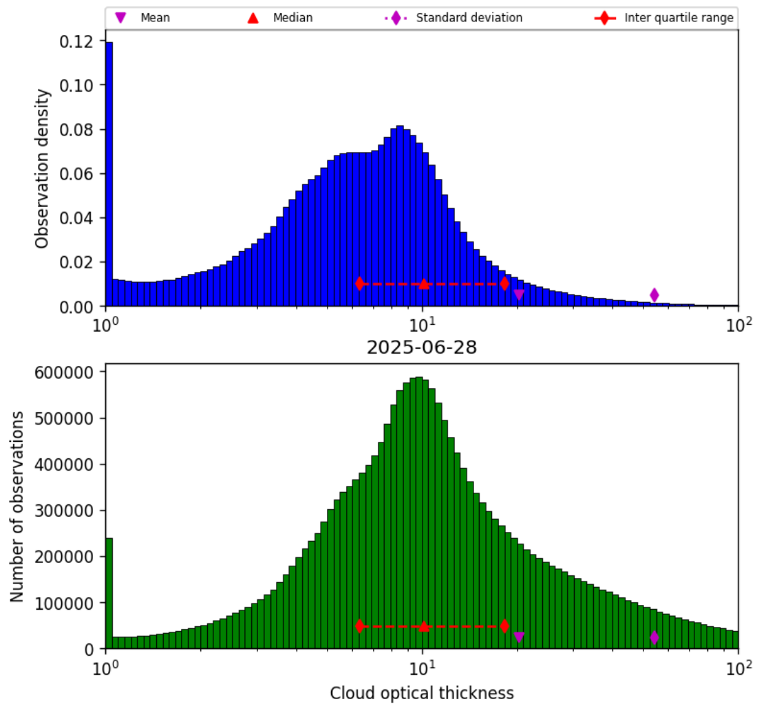
Figure 41: Histogram of “Cloud optical thickness” for 2025-06-27 to 2025-06-29
