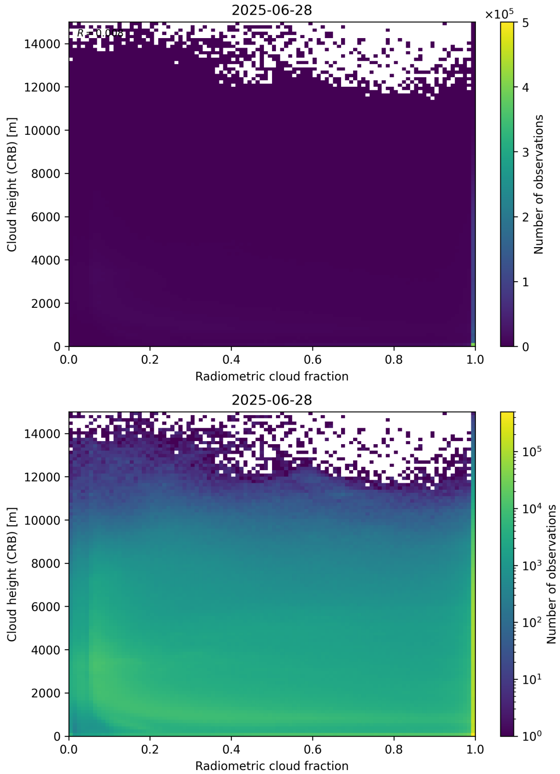
Figure 74: Scatter density plot of “Radiometric cloud fraction” against “Cloud height (CRB)” for 2025-06-27 to 2025-06-29.
