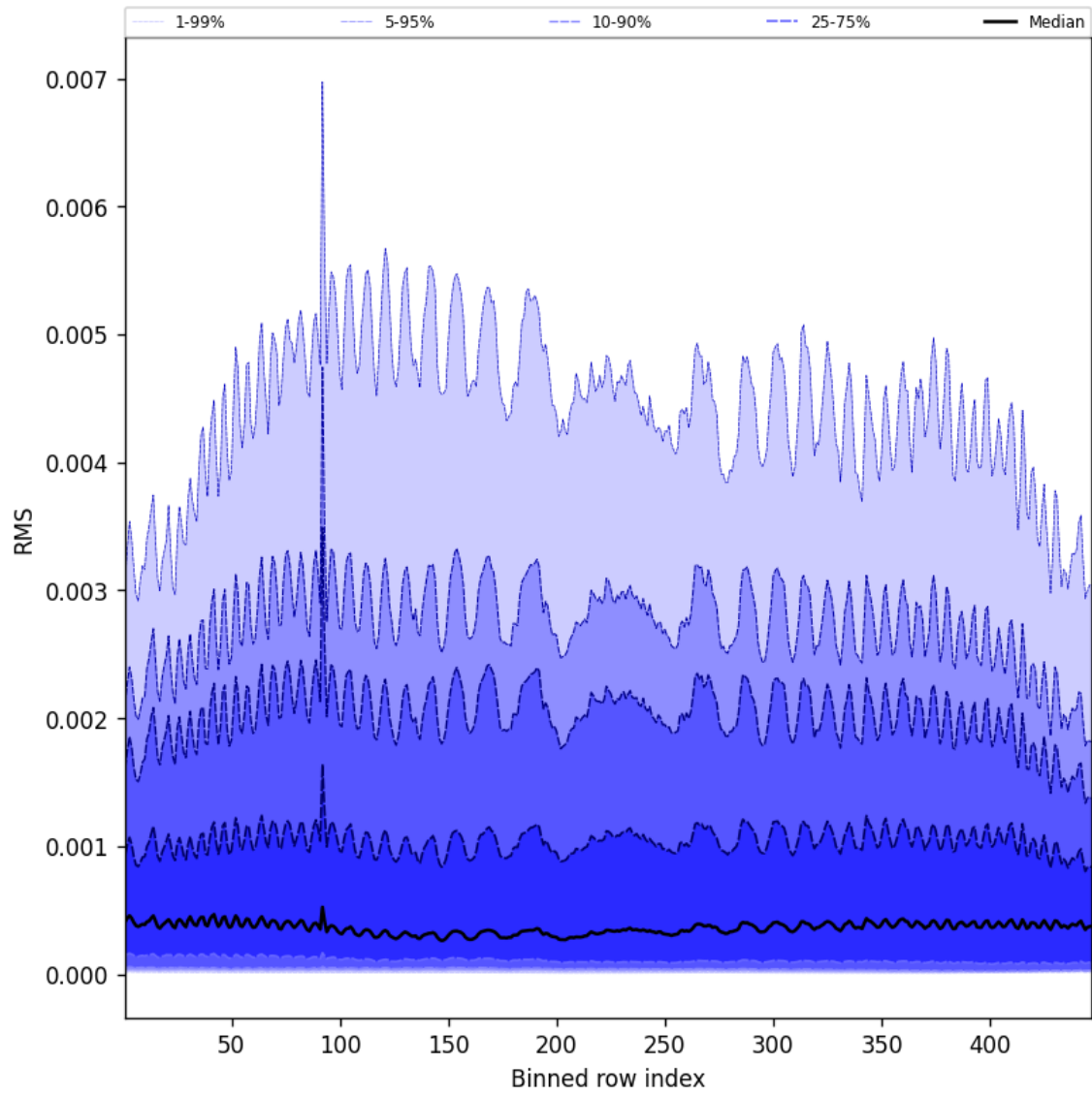
Figure 63: Along track statistics of “RMS” for 2025-06-27 to 2025-06-29
