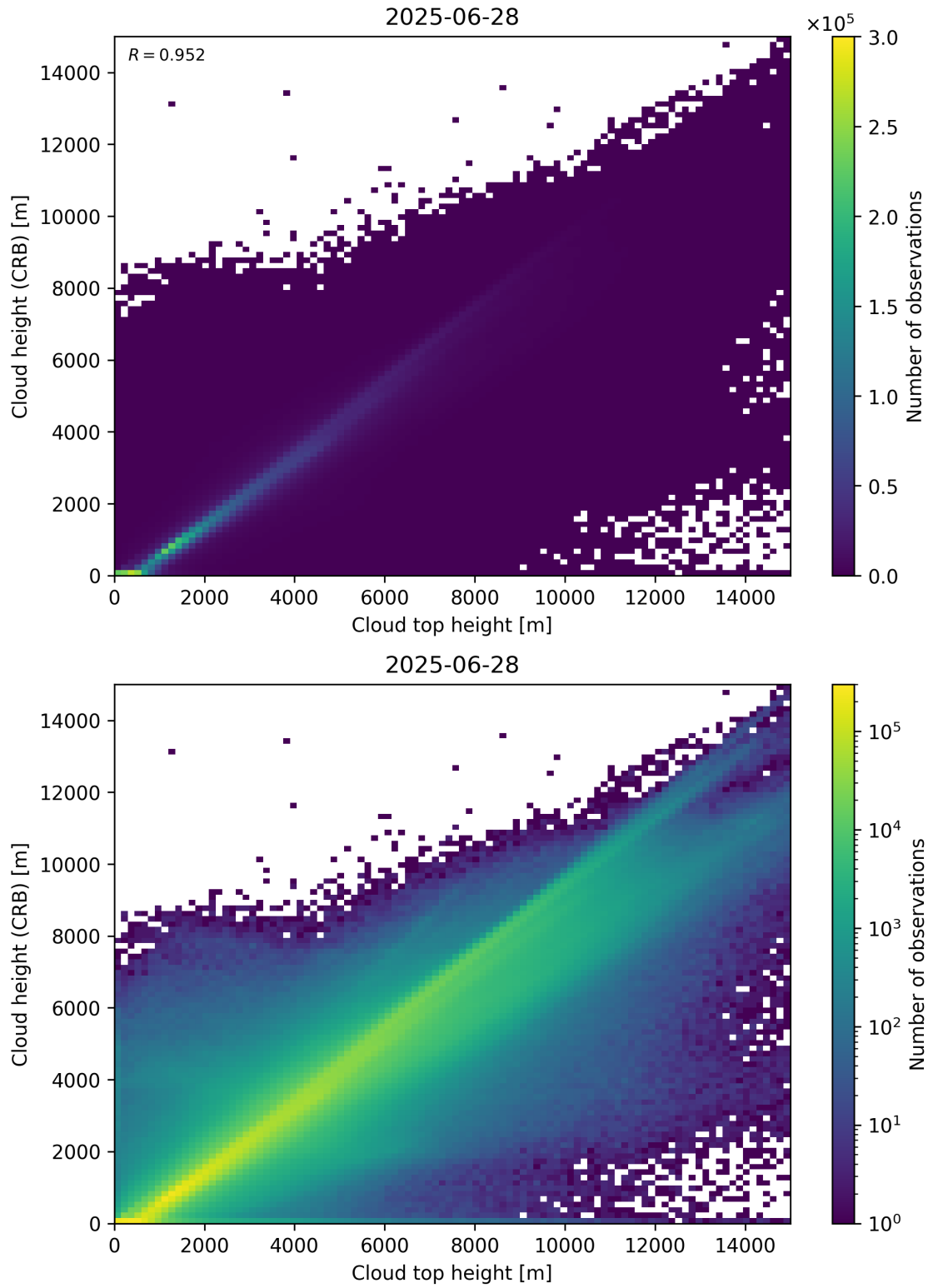
Figure 89: Scatter density plot of “Cloud top height” against “Cloud height (CRB)” for 2025-06-27 to 2025-06-29.
