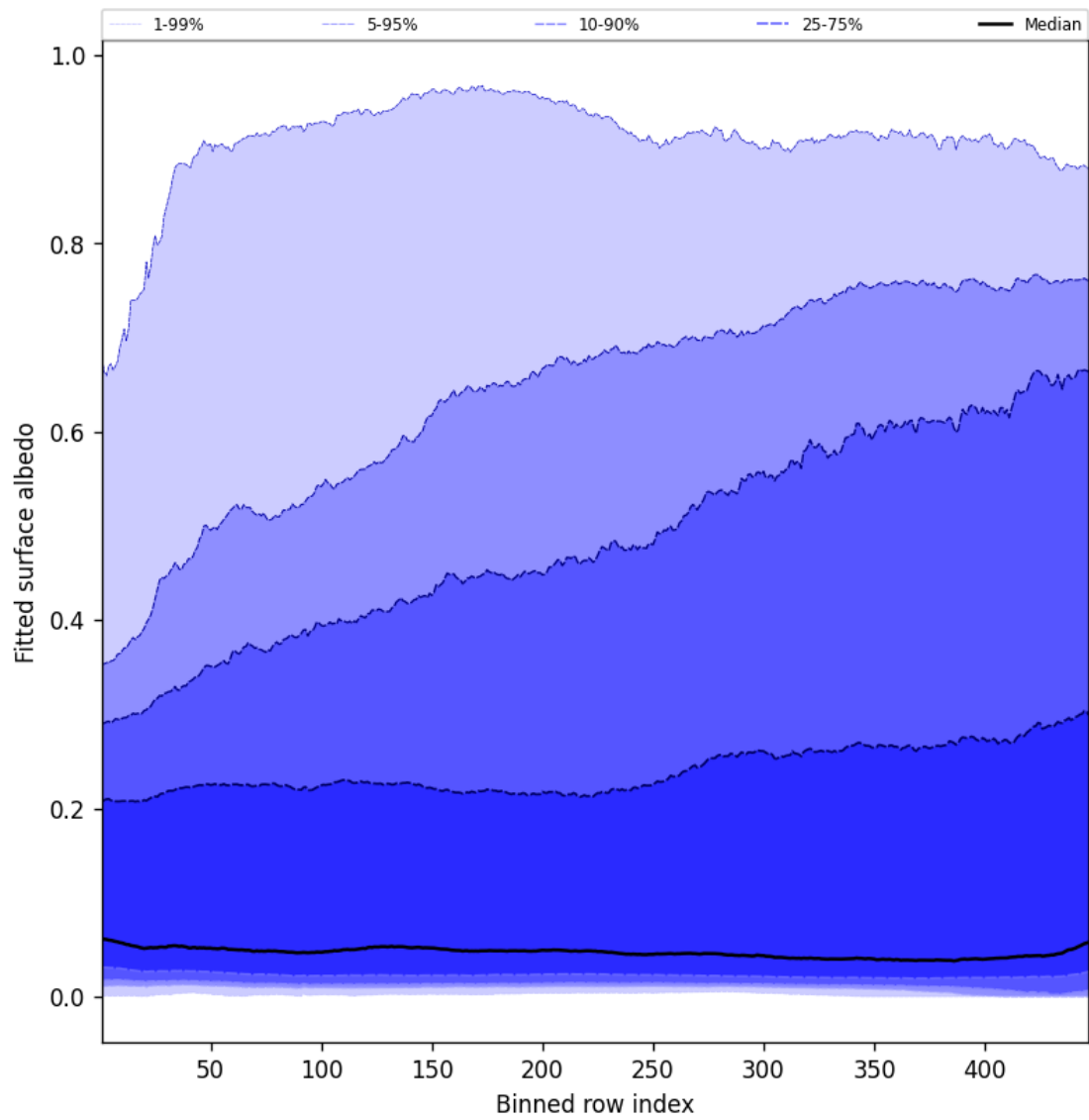
Figure 61: Along track statistics of “Fitted surface albedo” for 2025-06-27 to 2025-06-29
