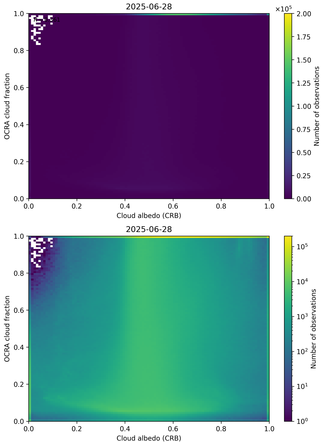
Figure 70: Scatter density plot of “Cloud albedo (CRB)” against “OCRA cloud fraction” for 2025-06-27 to 2025-06-29.
