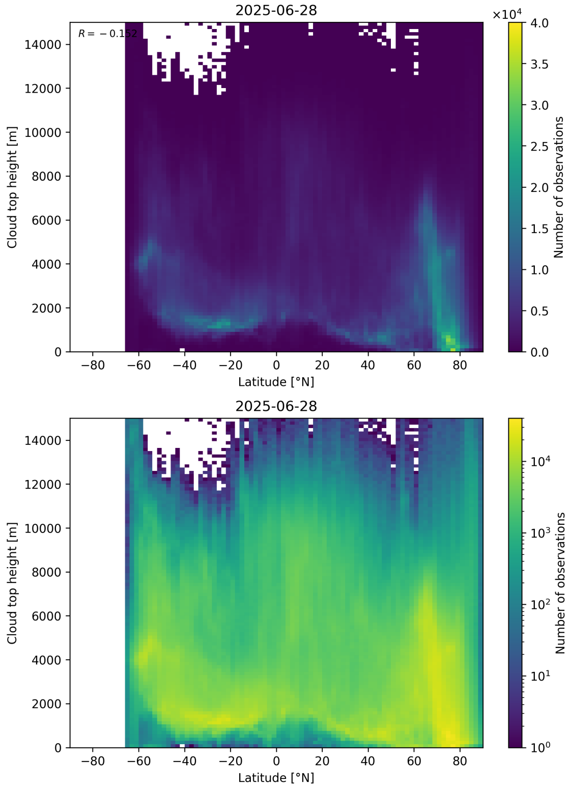
Figure 97: Scatter density plot of “Latitude” against “Cloud top height” for 2025-06-27 to 2025-06-29.
