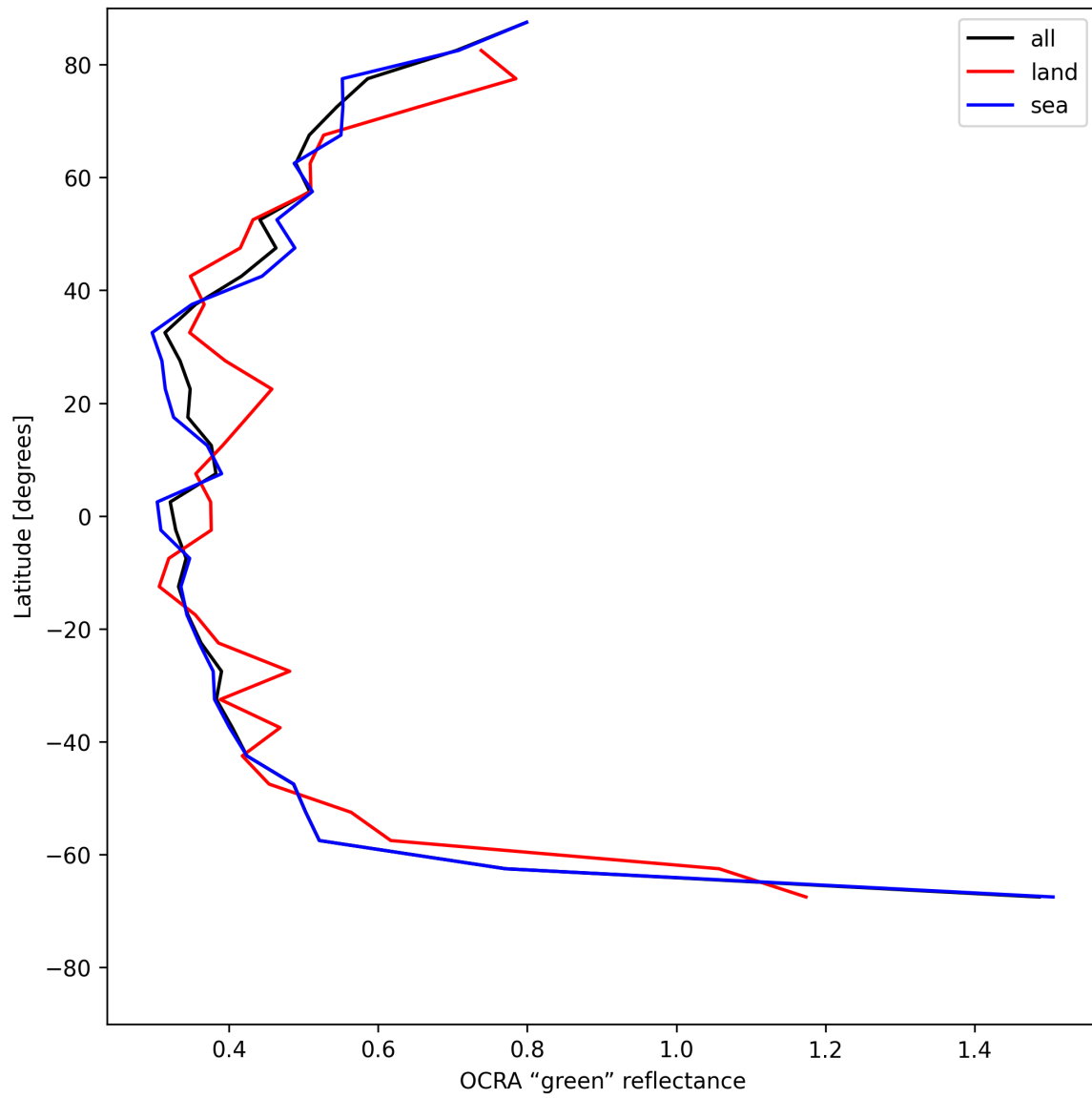
Figure 36: Zonal average of “OCRA “green” reflectance” for 2025-06-27 to 2025-06-29.
