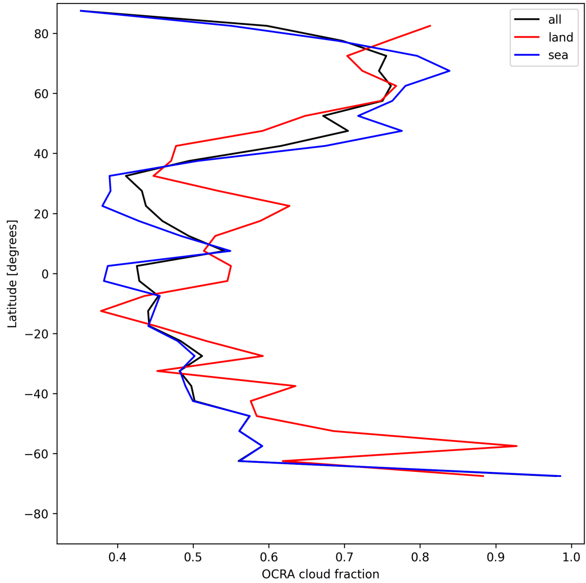
Figure 34: Zonal average of “OCRA cloud fraction” for 2025-06-27 to 2025-06-29.
