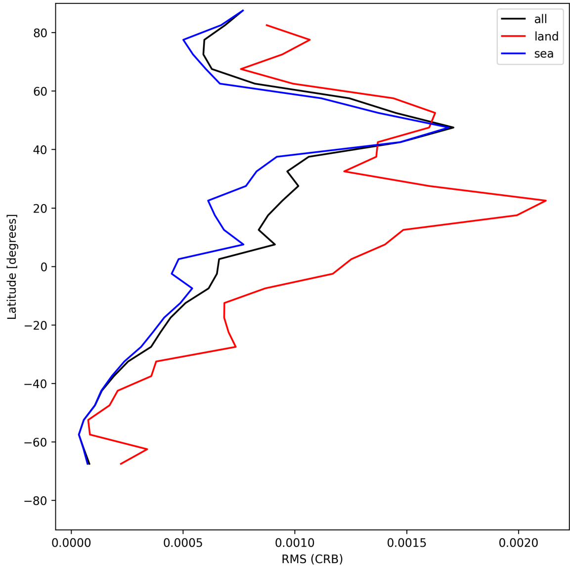
Figure 32: Zonal average of “RMS (CRB)” for 2025-06-27 to 2025-06-29.
