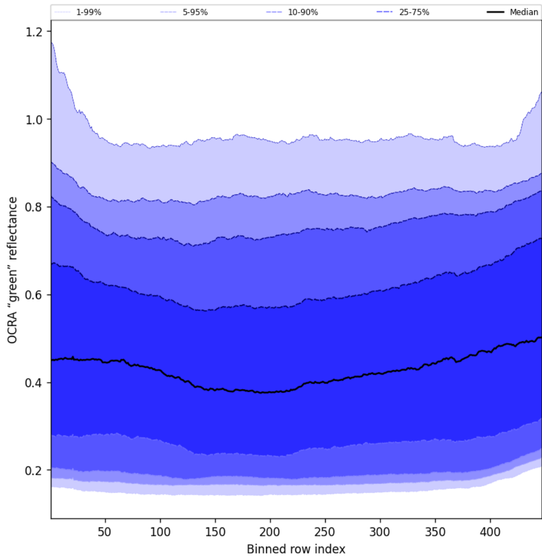
Figure 68: Along track statistics of “OCRA “green” reflectance” for 2025-06-27 to 2025-06-29
