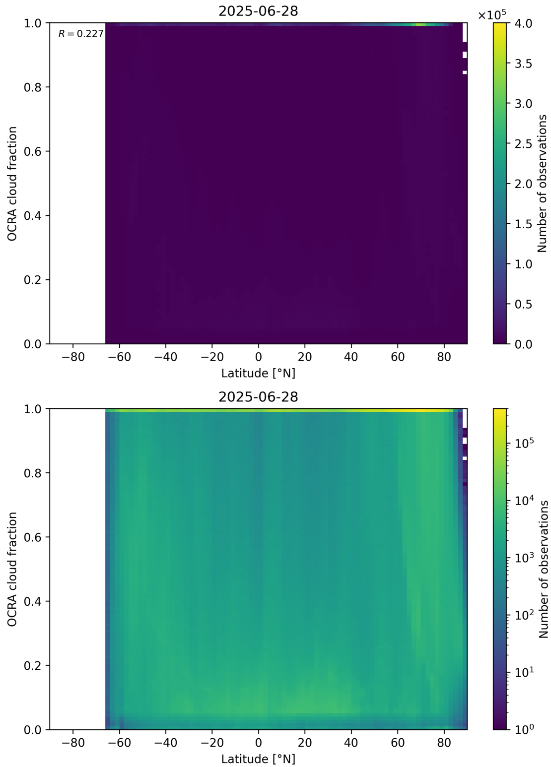
Figure 93: Scatter density plot of “Latitude” against “OCRA cloud fraction” for 2025-06-27 to 2025-06-29.
