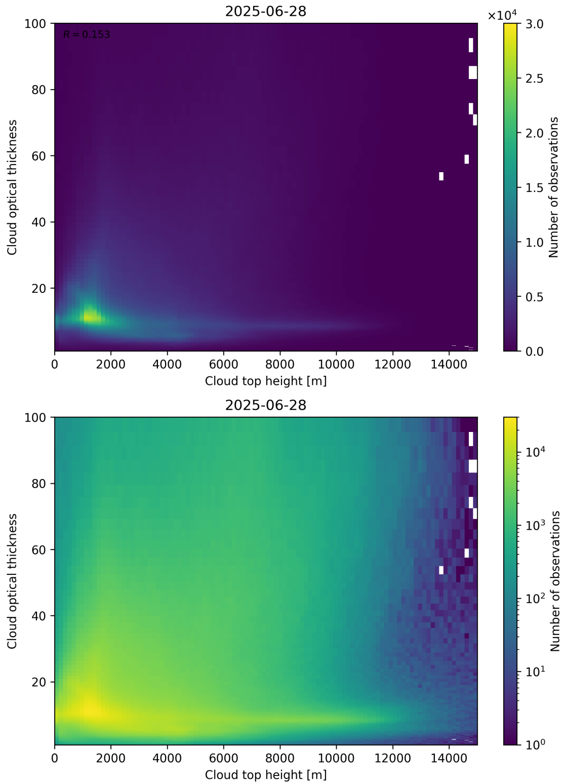
Figure 90: Scatter density plot of “Cloud top height” against “Cloud optical thickness” for 2025-06-27 to 2025-06-29.
