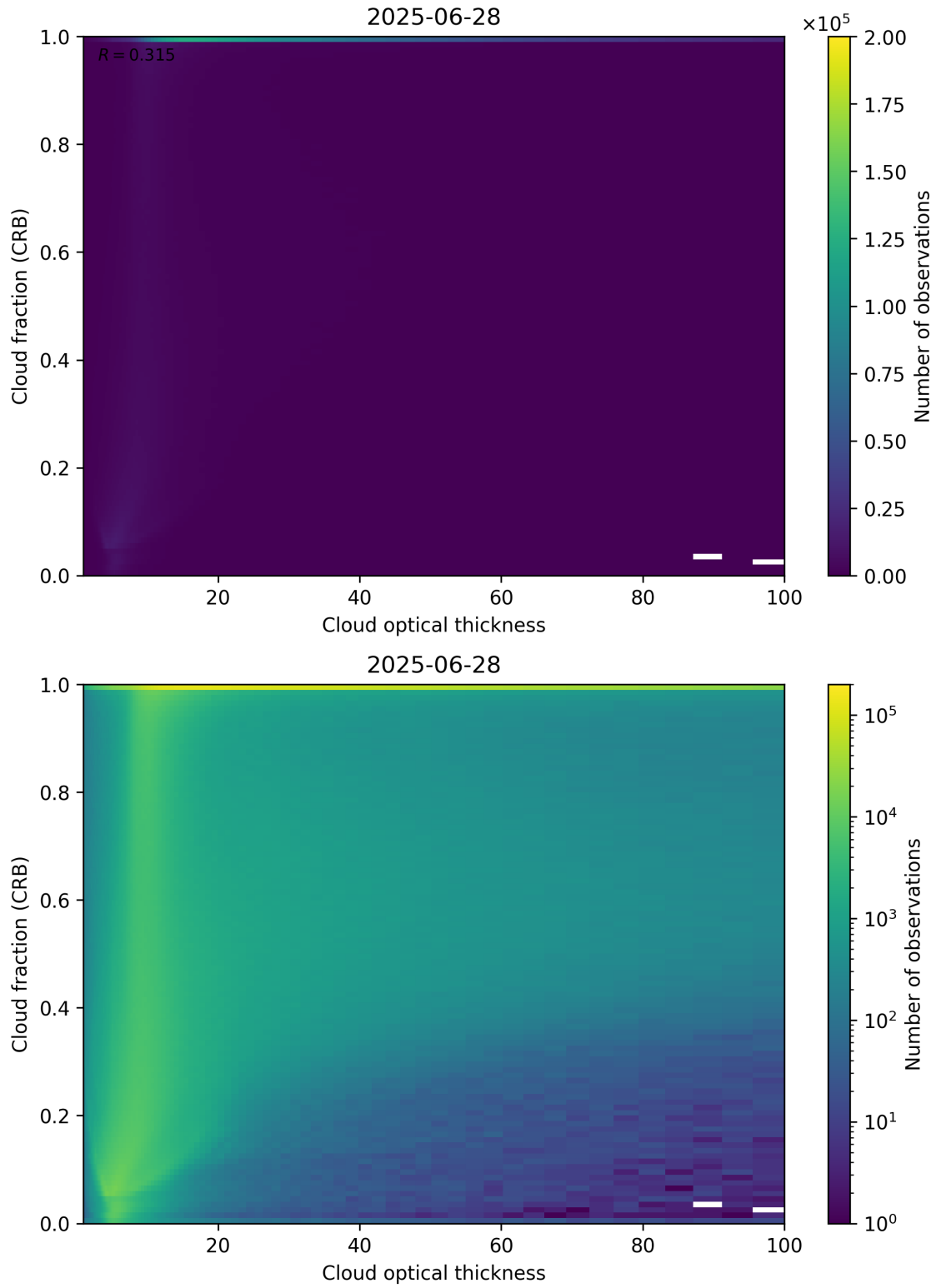
Figure 84: Scatter density plot of “Cloud optical thickness” against “Cloud fraction (CRB)” for 2025-06-27 to 2025-06-29.
