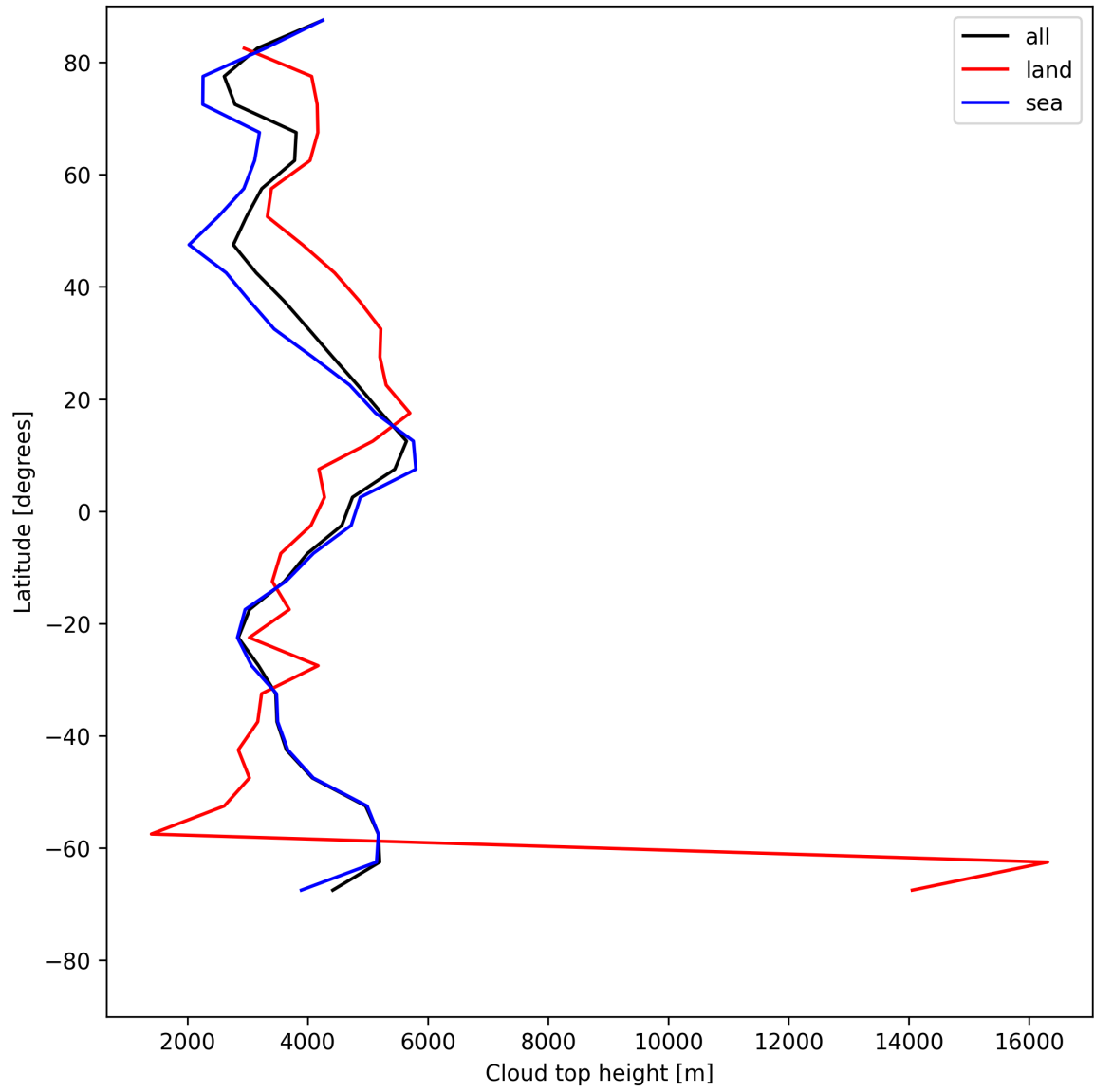
Figure 24: Zonal average of “Cloud top height” for 2025-06-27 to 2025-06-29.
