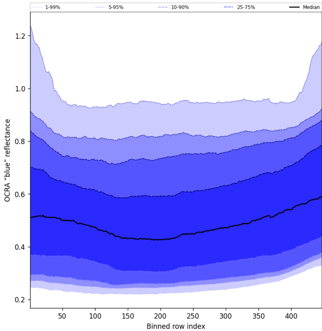
Figure 67: Along track statistics of “OCRA “blue” reflectance” for 2025-06-27 to 2025-06-29
