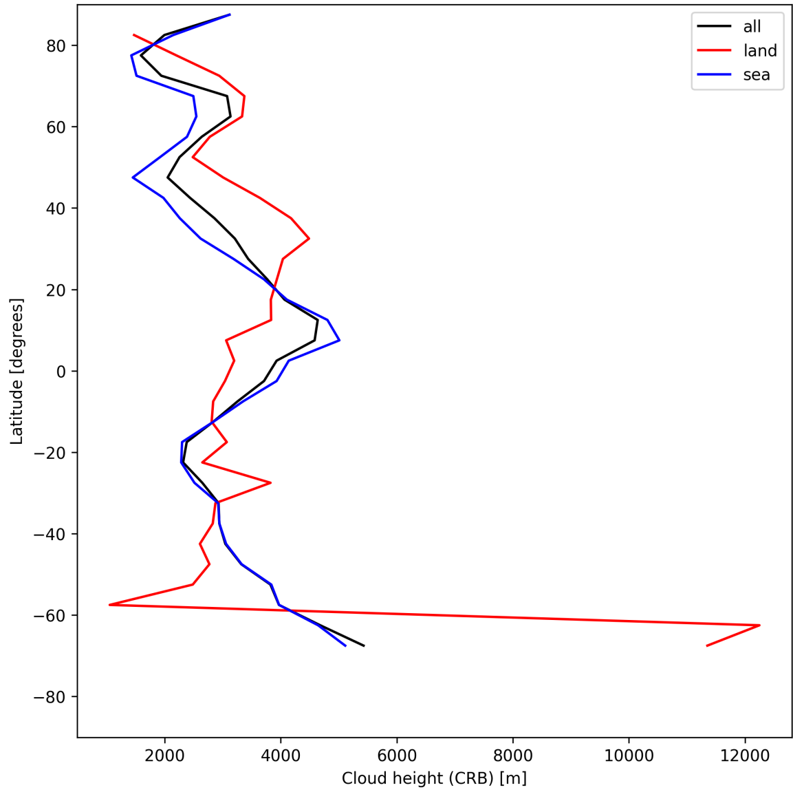
Figure 27: Zonal average of “Cloud height (CRB)” for 2025-06-27 to 2025-06-29.
