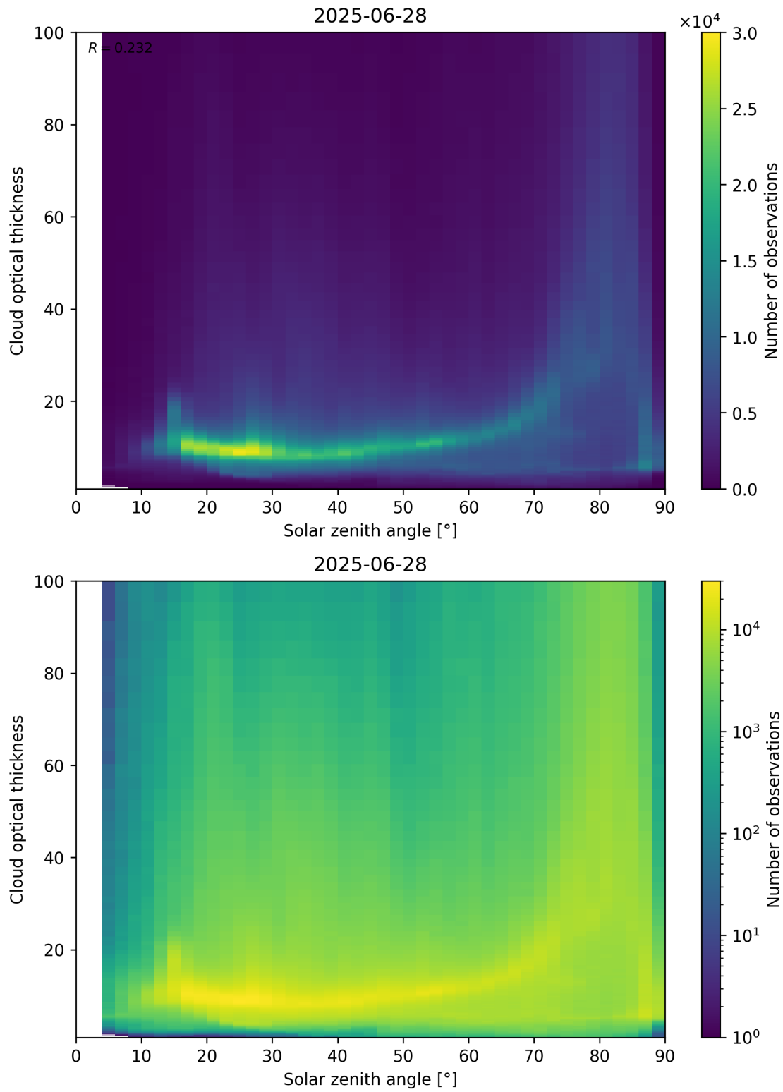
Figure 103: Scatter density plot of “Solar zenith angle” against “Cloud optical thickness” for 2025-06-27 to 2025-06-29.
