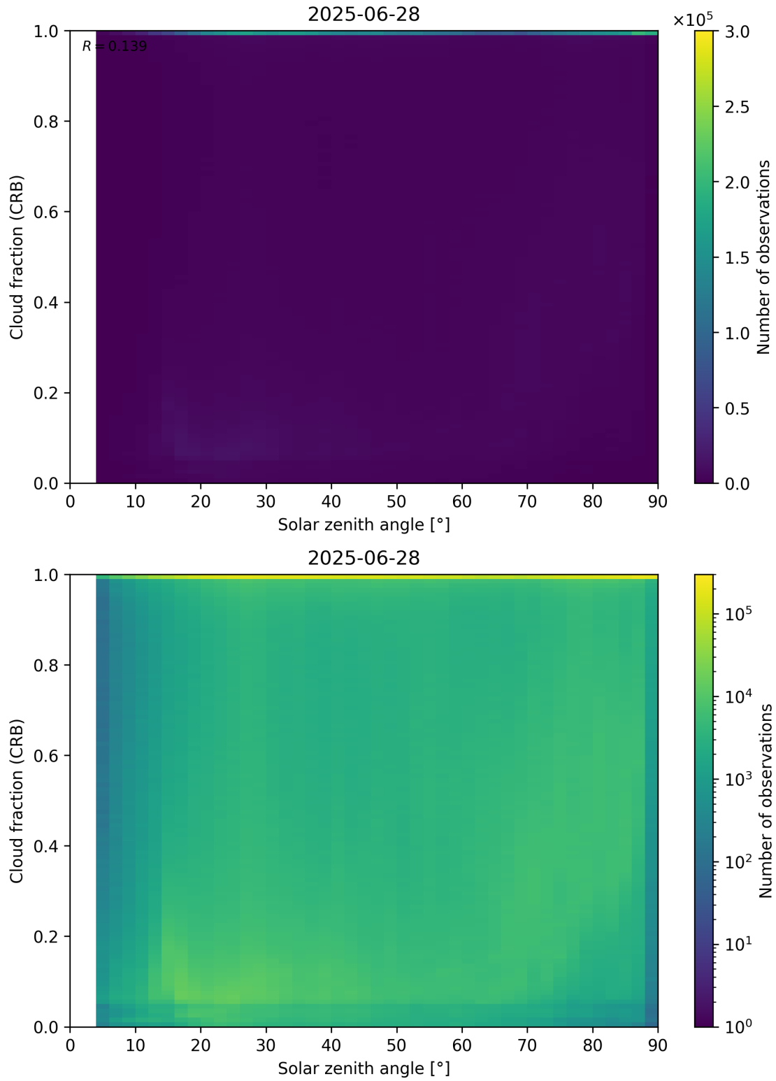
Figure 101: Scatter density plot of “Solar zenith angle” against “Cloud fraction (CRB)” for 2025-06-27 to 2025-06-29.
