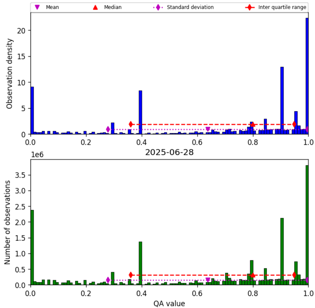
Figure 38: Histogram of “QA value” for 2025-06-27 to 2025-06-29
