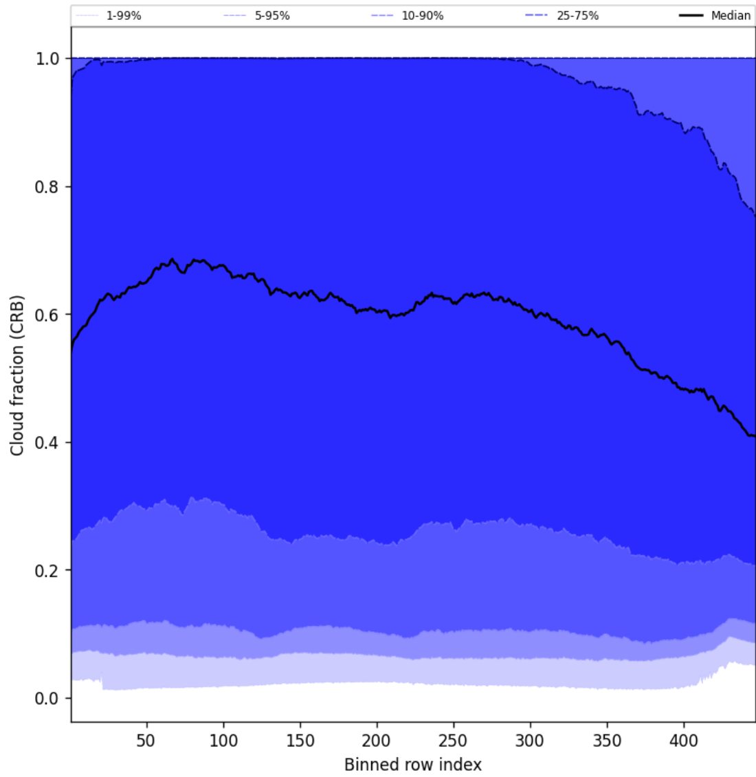
Figure 58: Along track statistics of “Cloud fraction (CRB)” for 2025-06-27 to 2025-06-29
