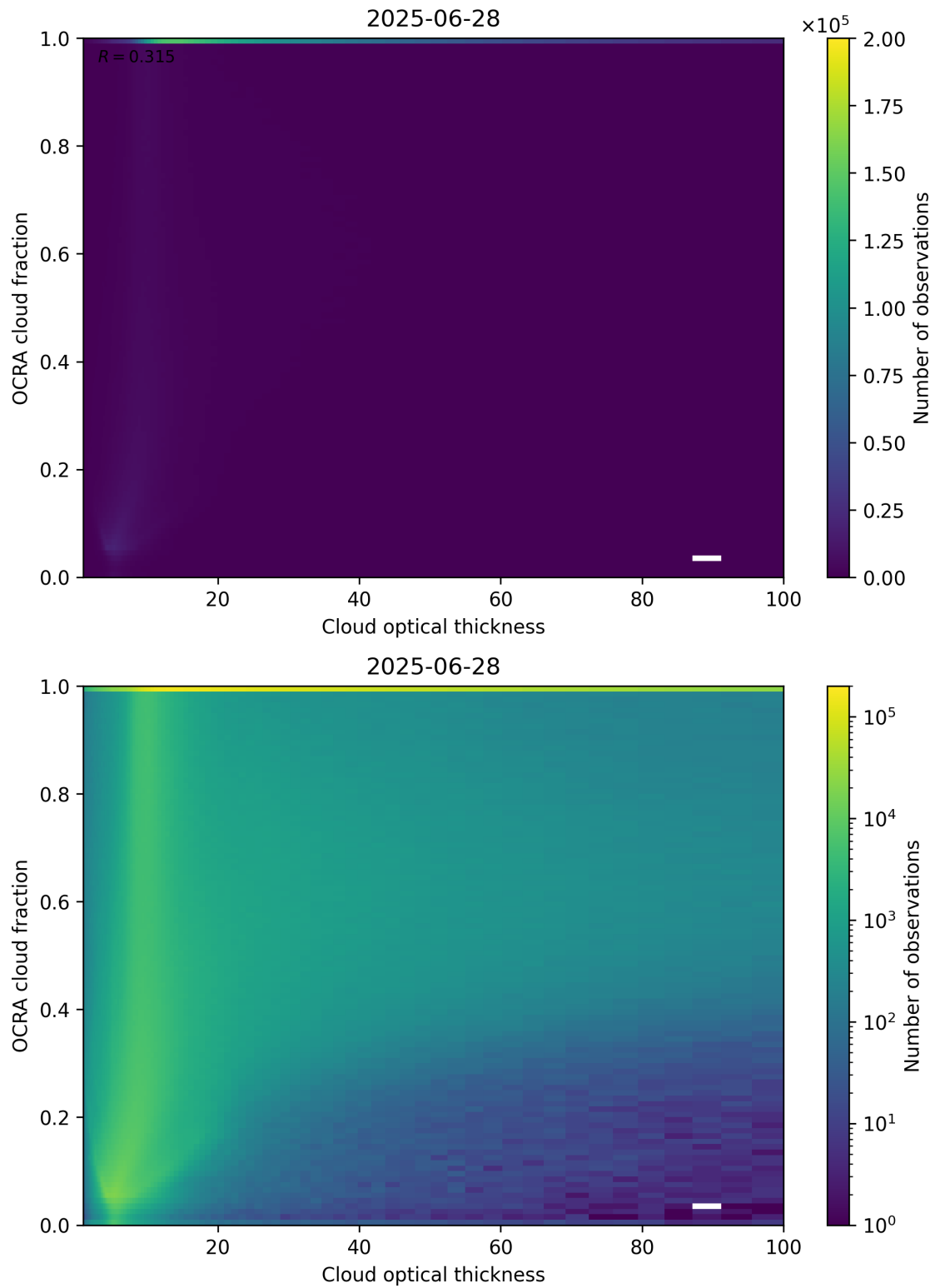
Figure 83: Scatter density plot of “Cloud optical thickness” against “OCRA cloud fraction” for 2025-06-27 to 2025-06-29.
