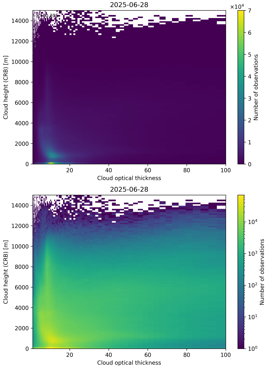
Figure 85: Scatter density plot of “Cloud optical thickness” against “Cloud height (CRB)” for 2025-06-27 to 2025-06-29.
