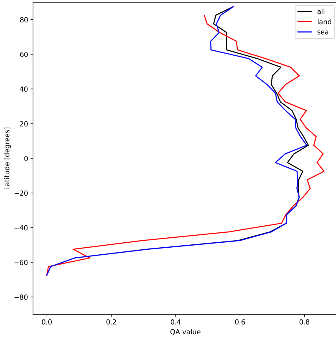
Figure 22: Zonal average of “QA value” for 2025-06-27 to 2025-06-29.
