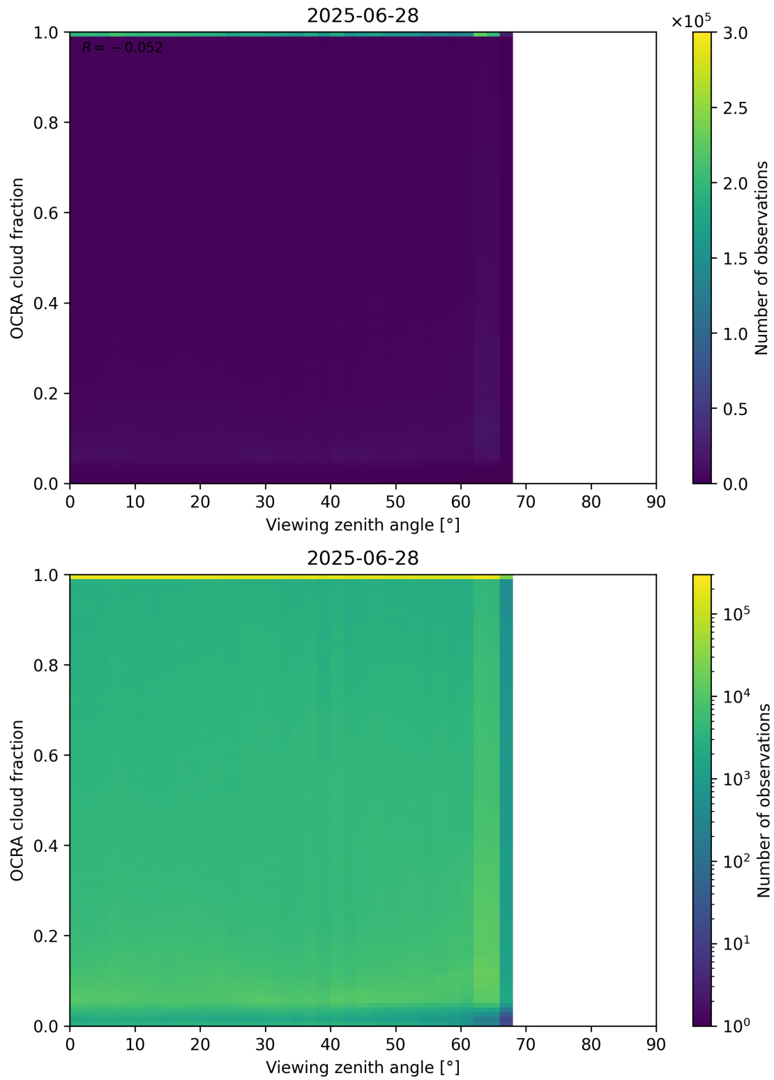
Figure 108: Scatter density plot of “Viewing zenith angle” against “OCRA cloud fraction” for 2025-06-27 to 2025-06-29.
