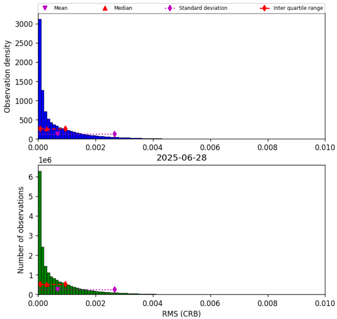
Figure 48: Histogram of “RMS (CRB)” for 2025-06-27 to 2025-06-29
