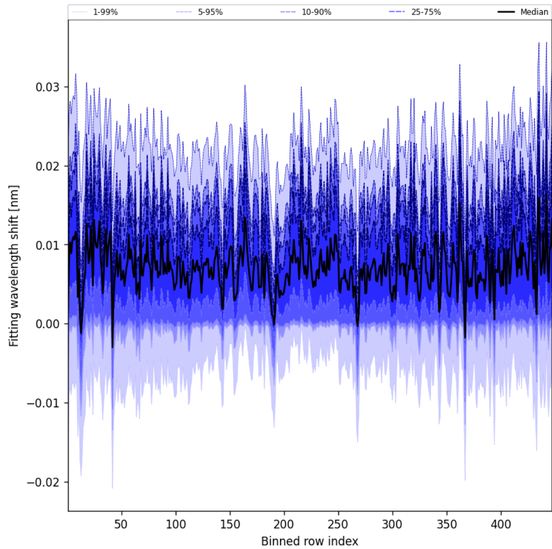
Figure 65: Along track statistics of “Fitting wavelength shift” for 2025-06-27 to 2025-06-29
