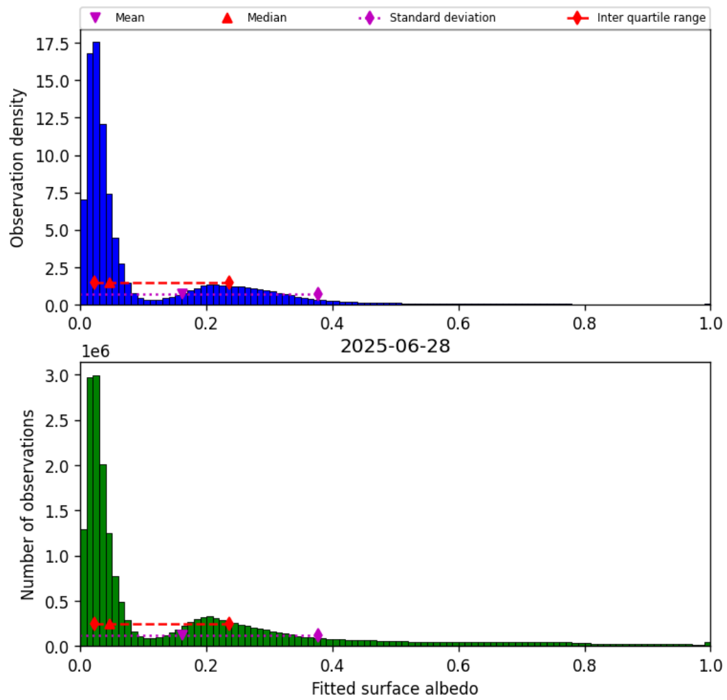
Figure 45: Histogram of “Fitted surface albedo” for 2025-06-27 to 2025-06-29
