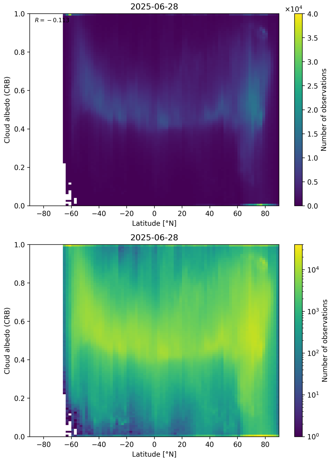
Figure 91: Scatter density plot of “Latitude” against “Cloud albedo (CRB)” for 2025-06-27 to 2025-06-29.
