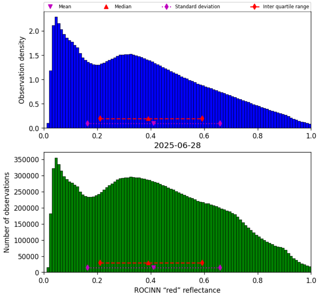
Figure 53: Histogram of “ROCINN “red” reflectance” for 2025-06-27 to 2025-06-29
