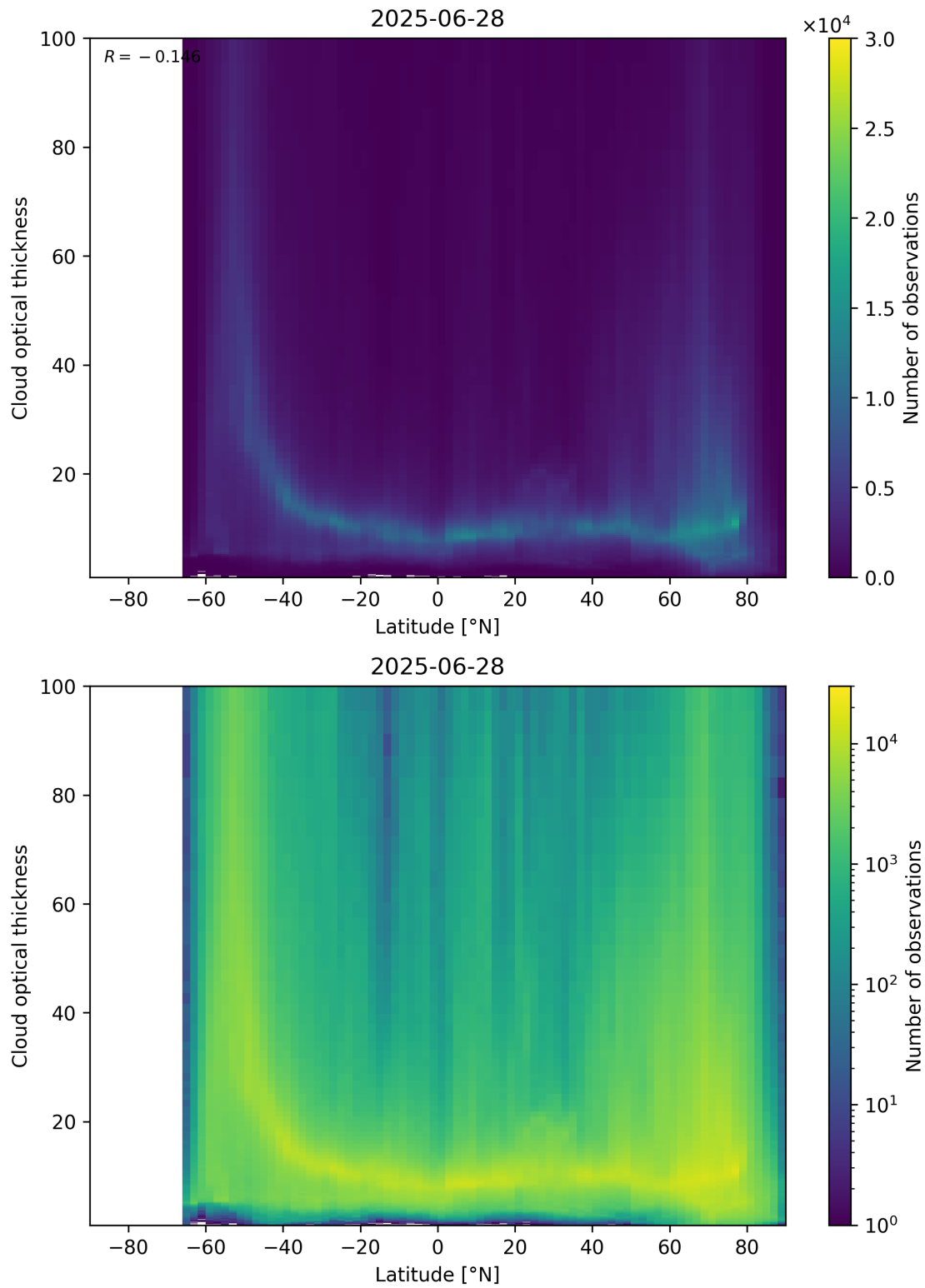
Figure 96: Scatter density plot of “Latitude” against “Cloud optical thickness” for 2025-06-27 to 2025-06-29.
