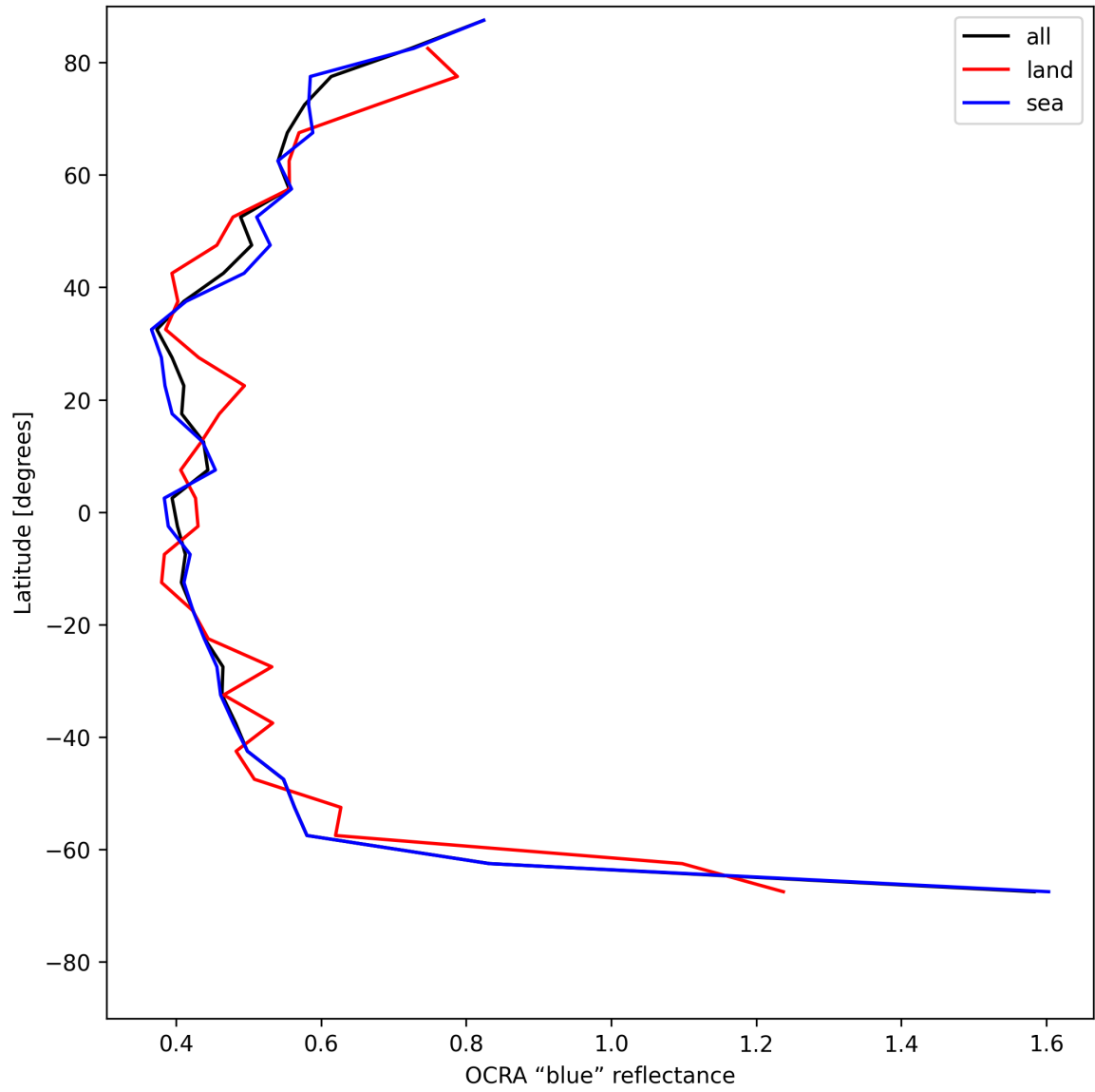
Figure 35: Zonal average of “OCRA “blue” reflectance” for 2025-06-27 to 2025-06-29.
