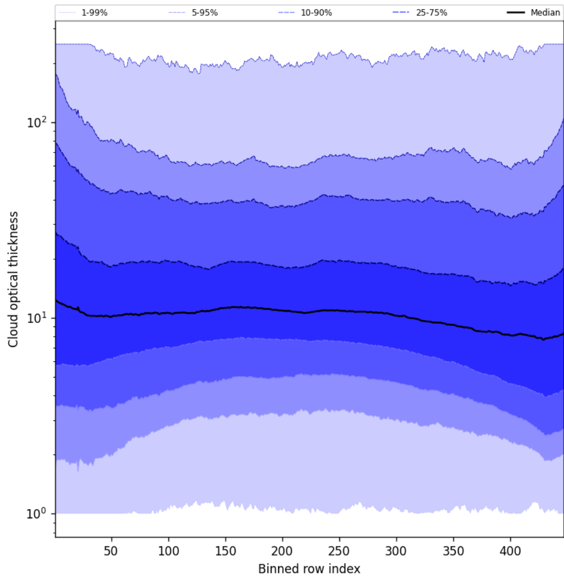
Figure 57: Along track statistics of “Cloud optical thickness” for 2025-06-27 to 2025-06-29
