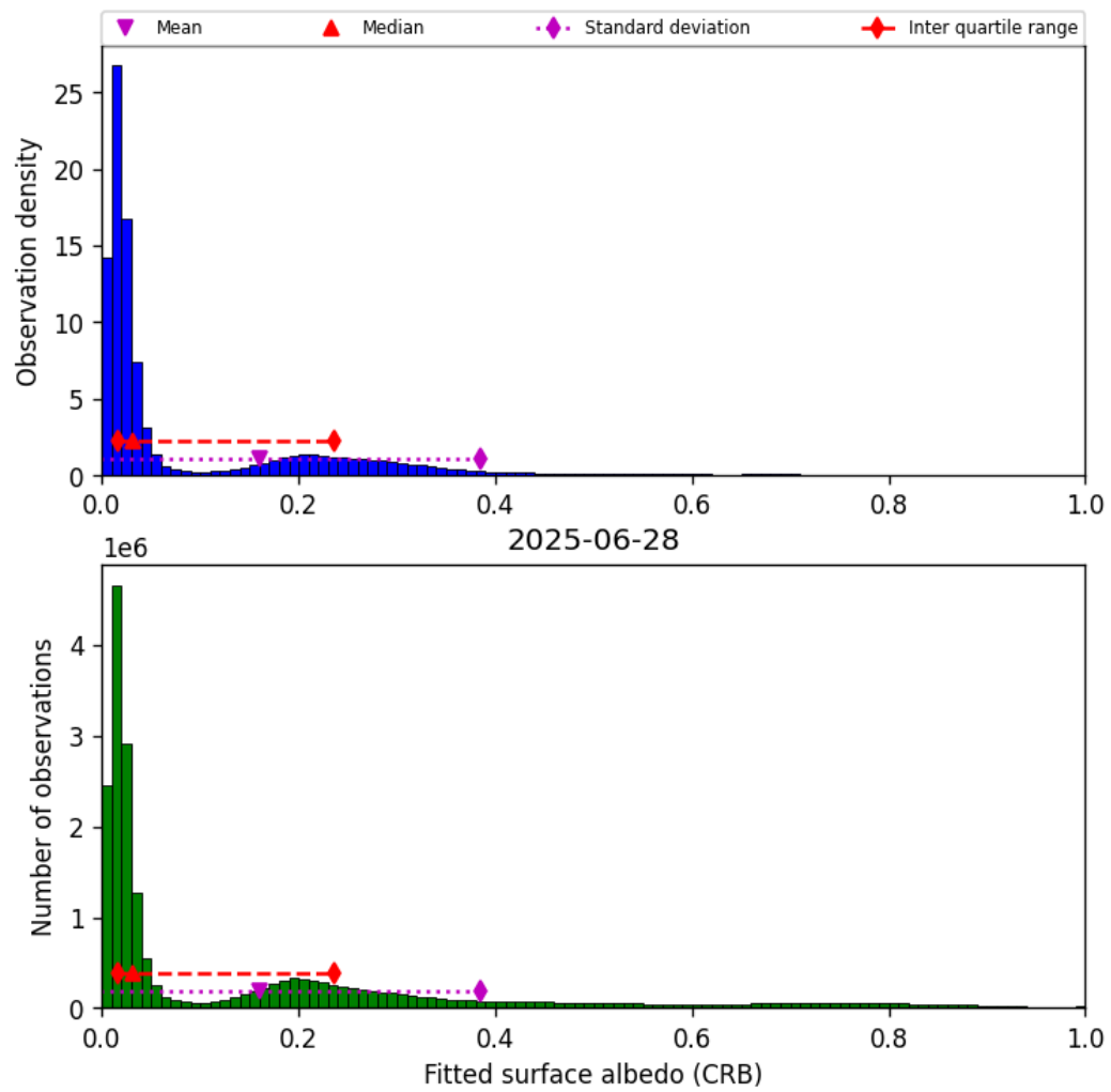
Figure 46: Histogram of “Fitted surface albedo (CRB)” for 2025-06-27 to 2025-06-29
