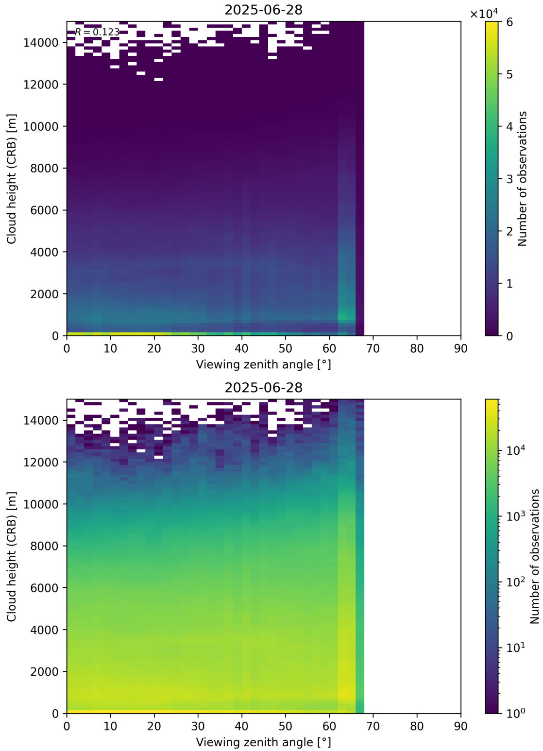
Figure 110: Scatter density plot of “Viewing zenith angle” against “Cloud height (CRB)” for 2025-06-27 to 2025-06-29.
