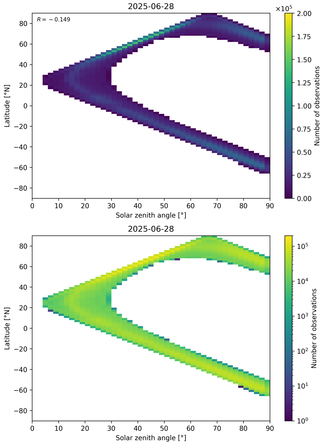
Figure 105: Scatter density plot of “Solar zenith angle” against “Latitude” for 2025-06-27 to 2025-06-29.
