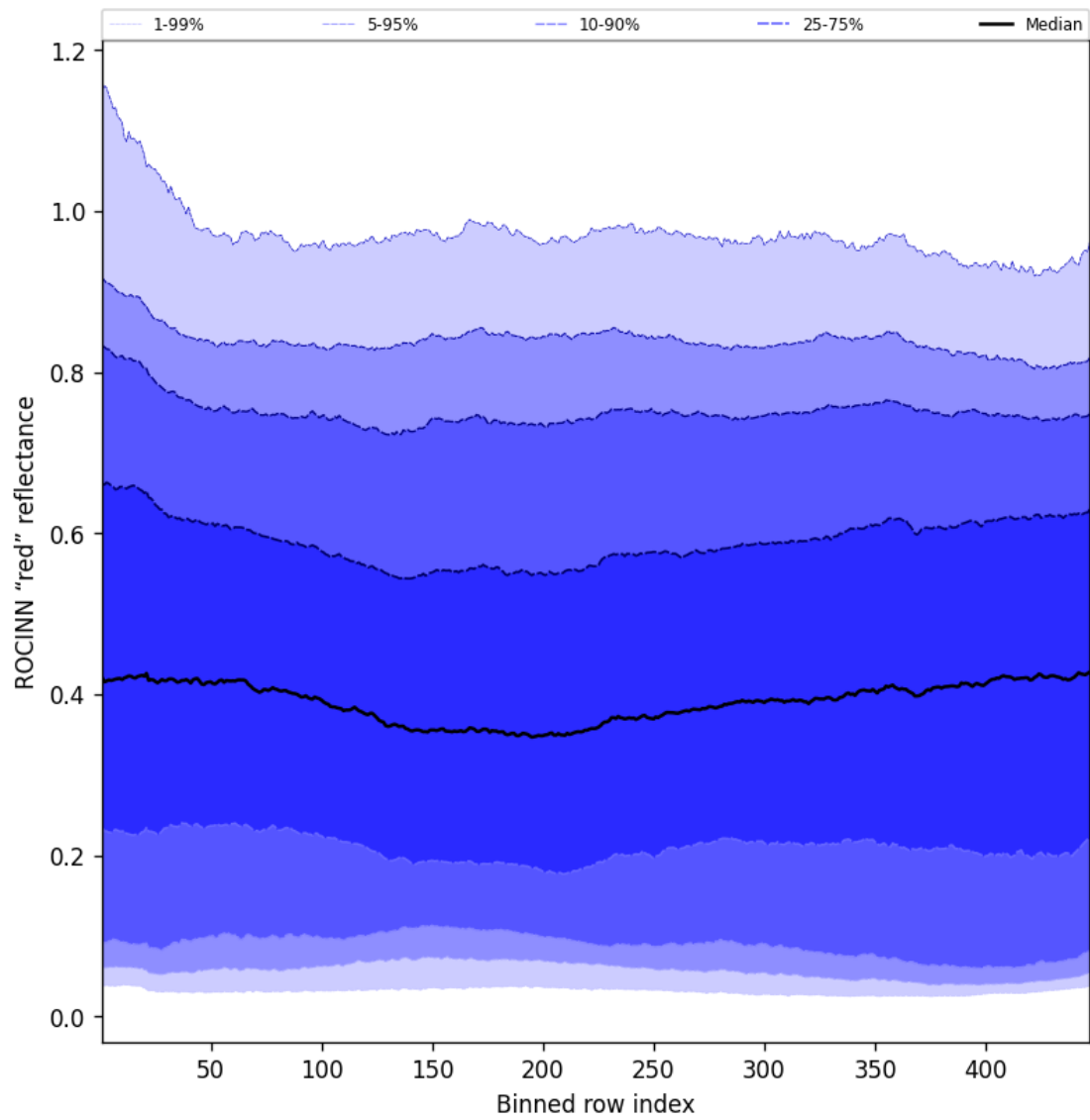
Figure 69: Along track statistics of “ROCINN “red” reflectance” for 2025-06-27 to 2025-06-29
