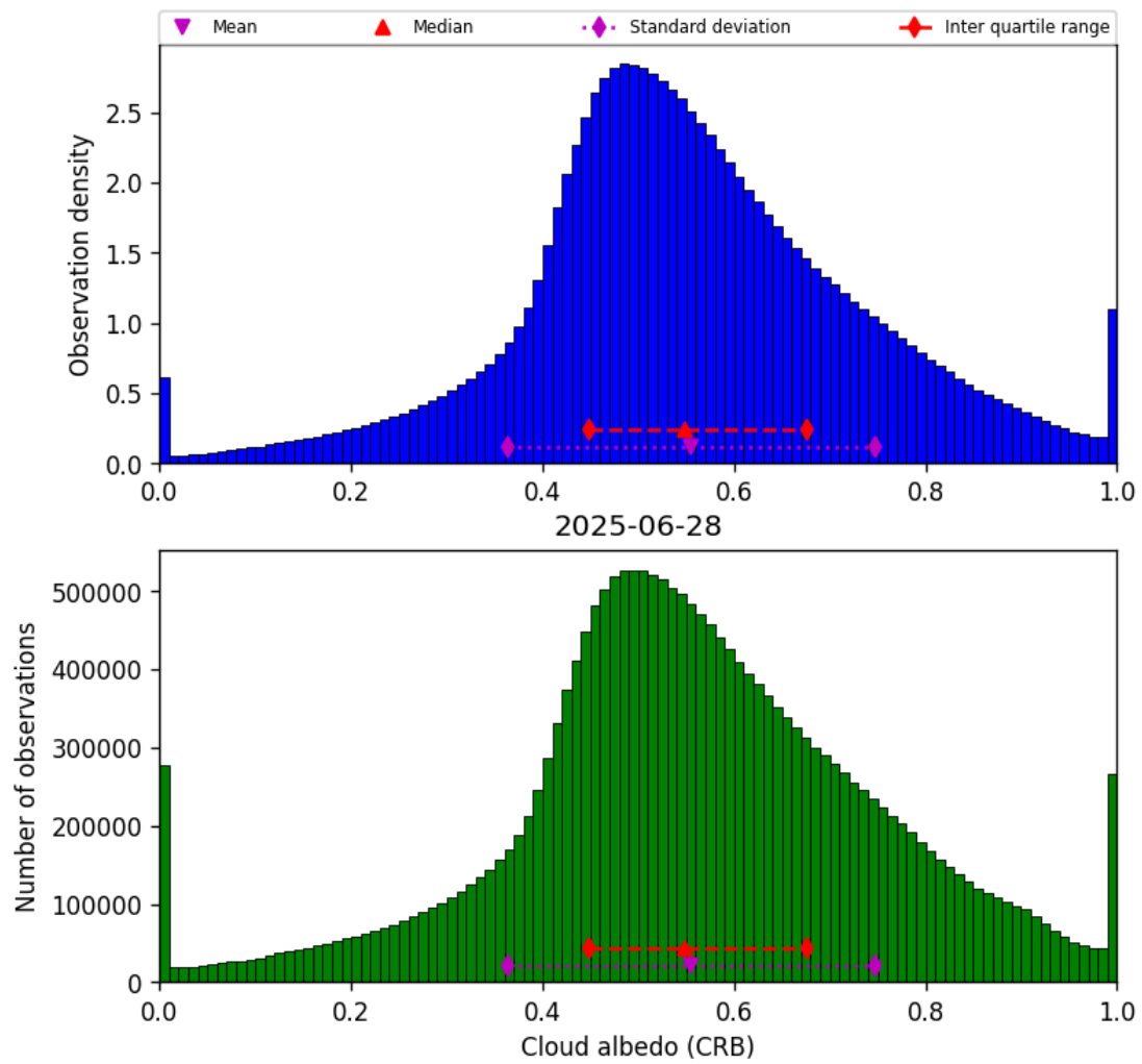
Figure 44: Histogram of “Cloud albedo (CRB)” for 2025-06-27 to 2025-06-29
