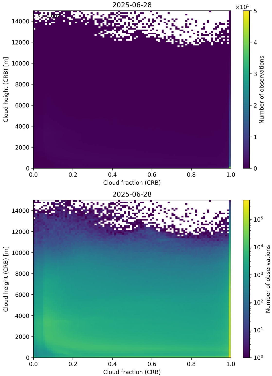
Figure 79: Scatter density plot of “Cloud fraction (CRB)” against “Cloud height (CRB)” for 2025-06-27 to 2025-06-29.
