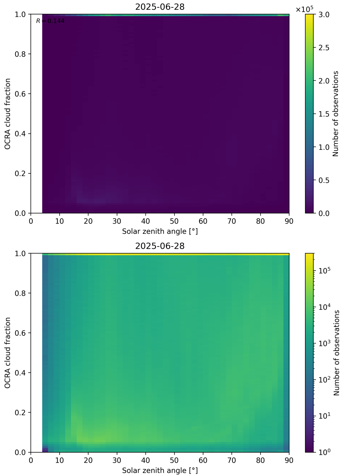
Figure 100: Scatter density plot of “Solar zenith angle” against “OCRA cloud fraction” for 2025-06-27 to 2025-06-29.
