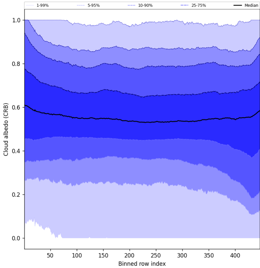
Figure 60: Along track statistics of “Cloud albedo (CRB)” for 2025-06-27 to 2025-06-29
