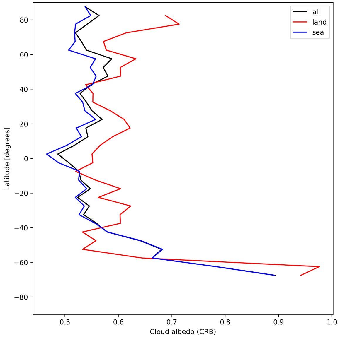
Figure 28: Zonal average of “Cloud albedo (CRB)” for 2025-06-27 to 2025-06-29.
