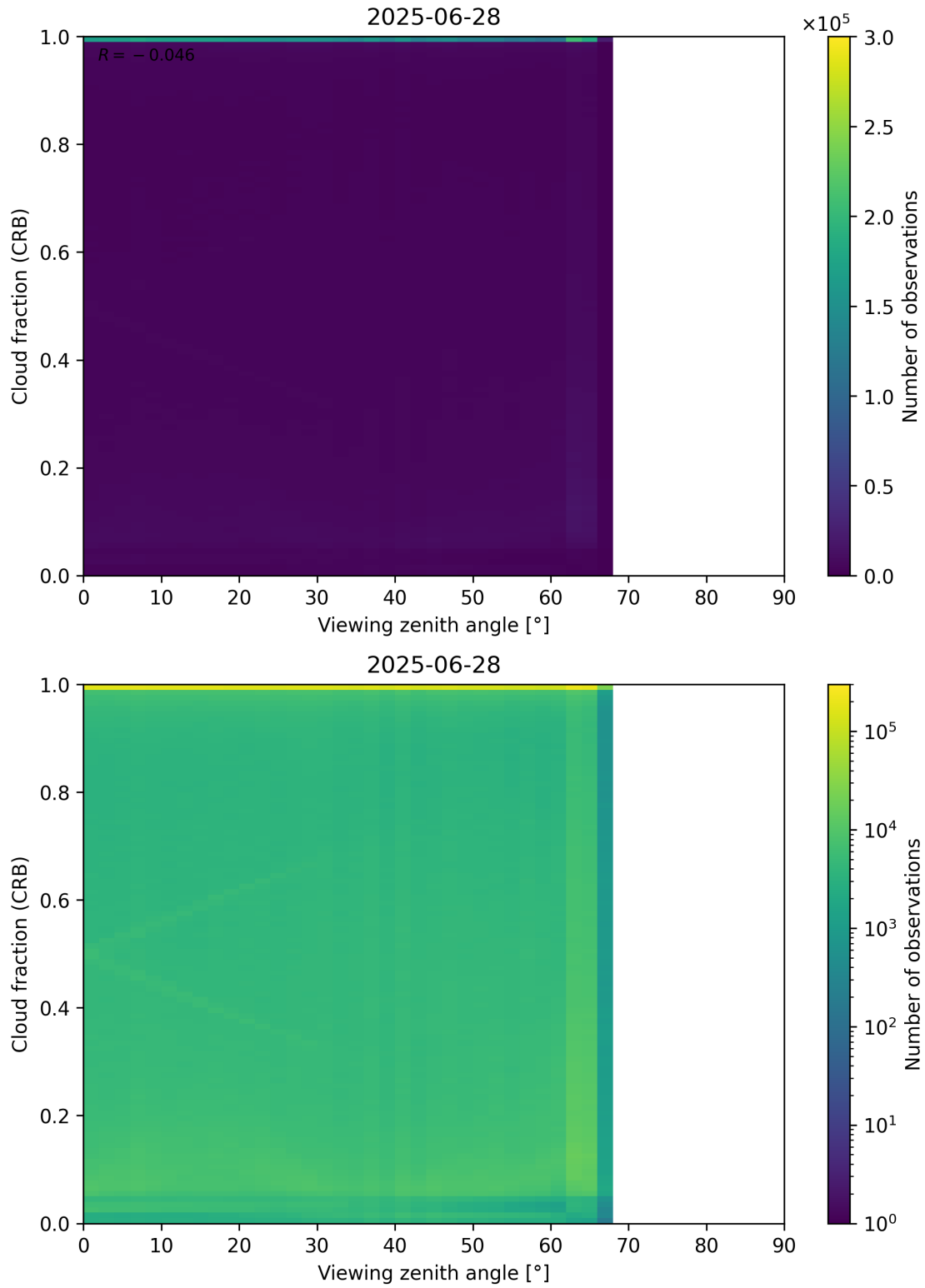
Figure 109: Scatter density plot of “Viewing zenith angle” against “Cloud fraction (CRB)” for 2025-06-27 to 2025-06-29.
