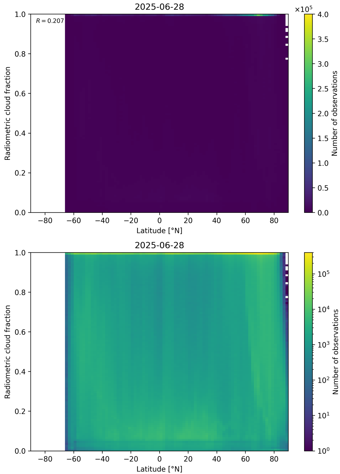
Figure 92: Scatter density plot of “Latitude” against “Radiometric cloud fraction” for 2025-06-27 to 2025-06-29.
