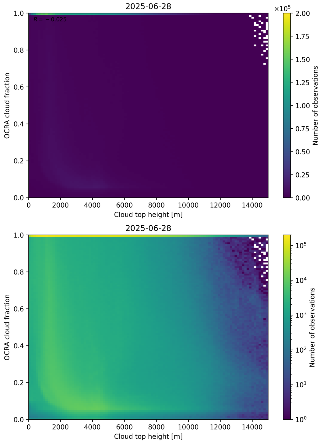
Figure 87: Scatter density plot of “Cloud top height” against “OCRA cloud fraction” for 2025-06-27 to 2025-06-29.
