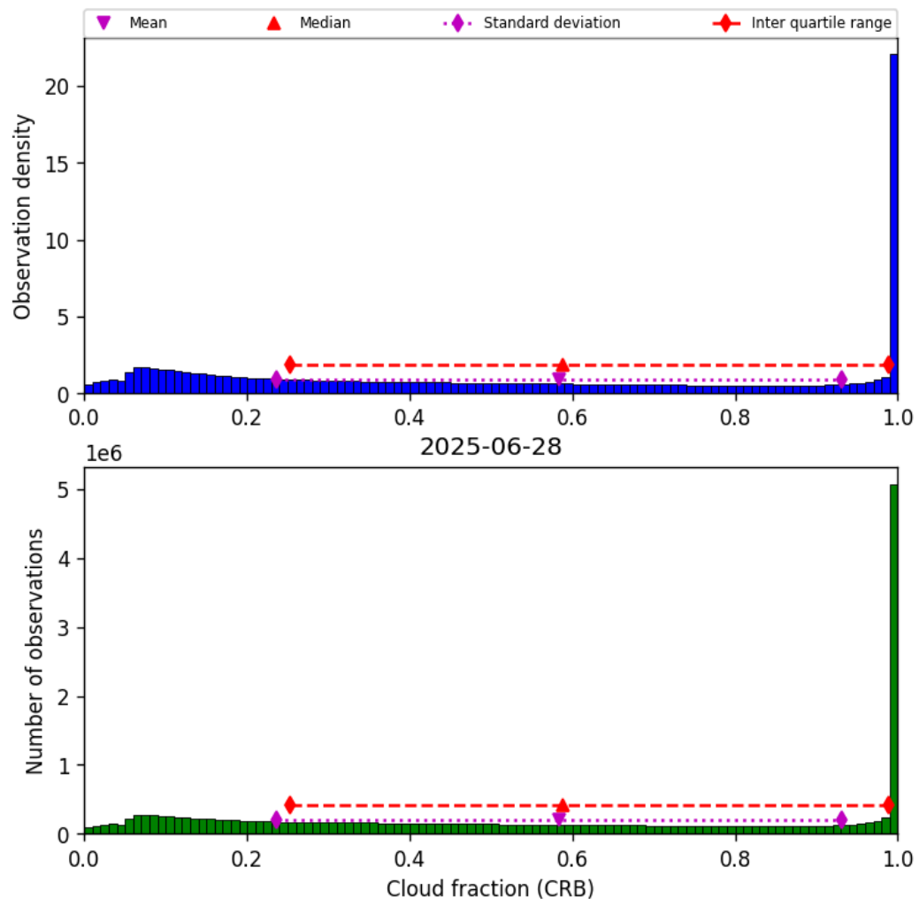
Figure 42: Histogram of “Cloud fraction (CRB)” for 2025-06-27 to 2025-06-29
