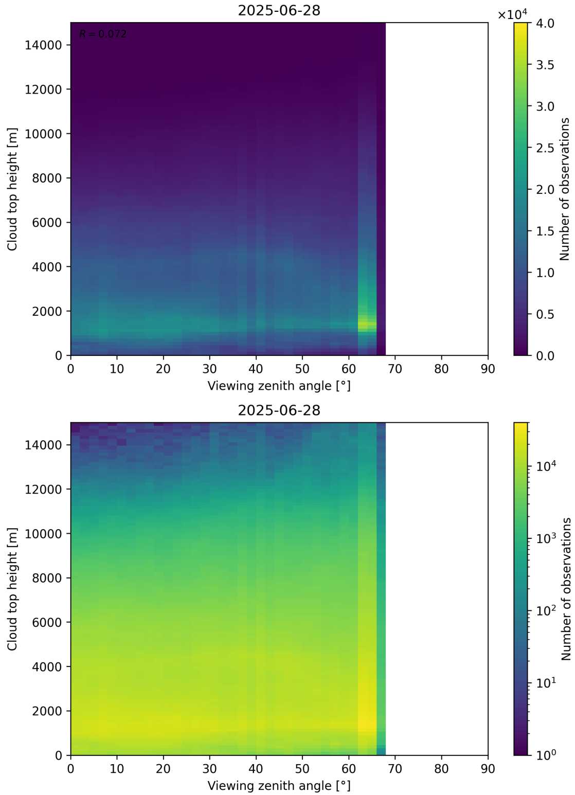
Figure 112: Scatter density plot of “Viewing zenith angle” against “Cloud top height” for 2025-06-27 to 2025-06-29.
