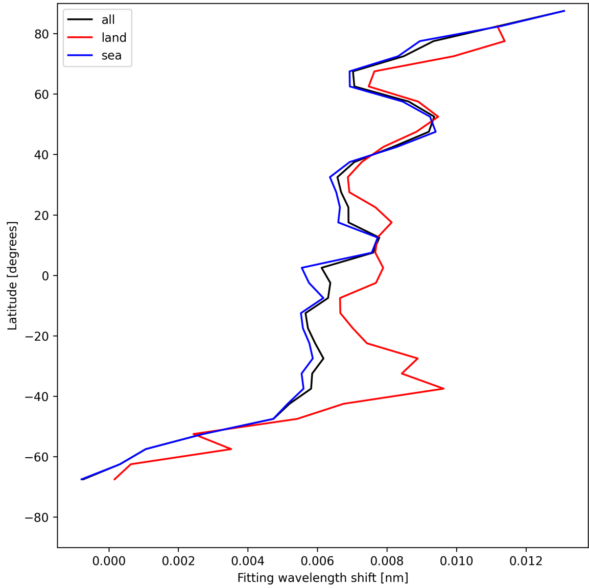
Figure 33: Zonal average of “Fitting wavelength shift” for 2025-06-27 to 2025-06-29.
