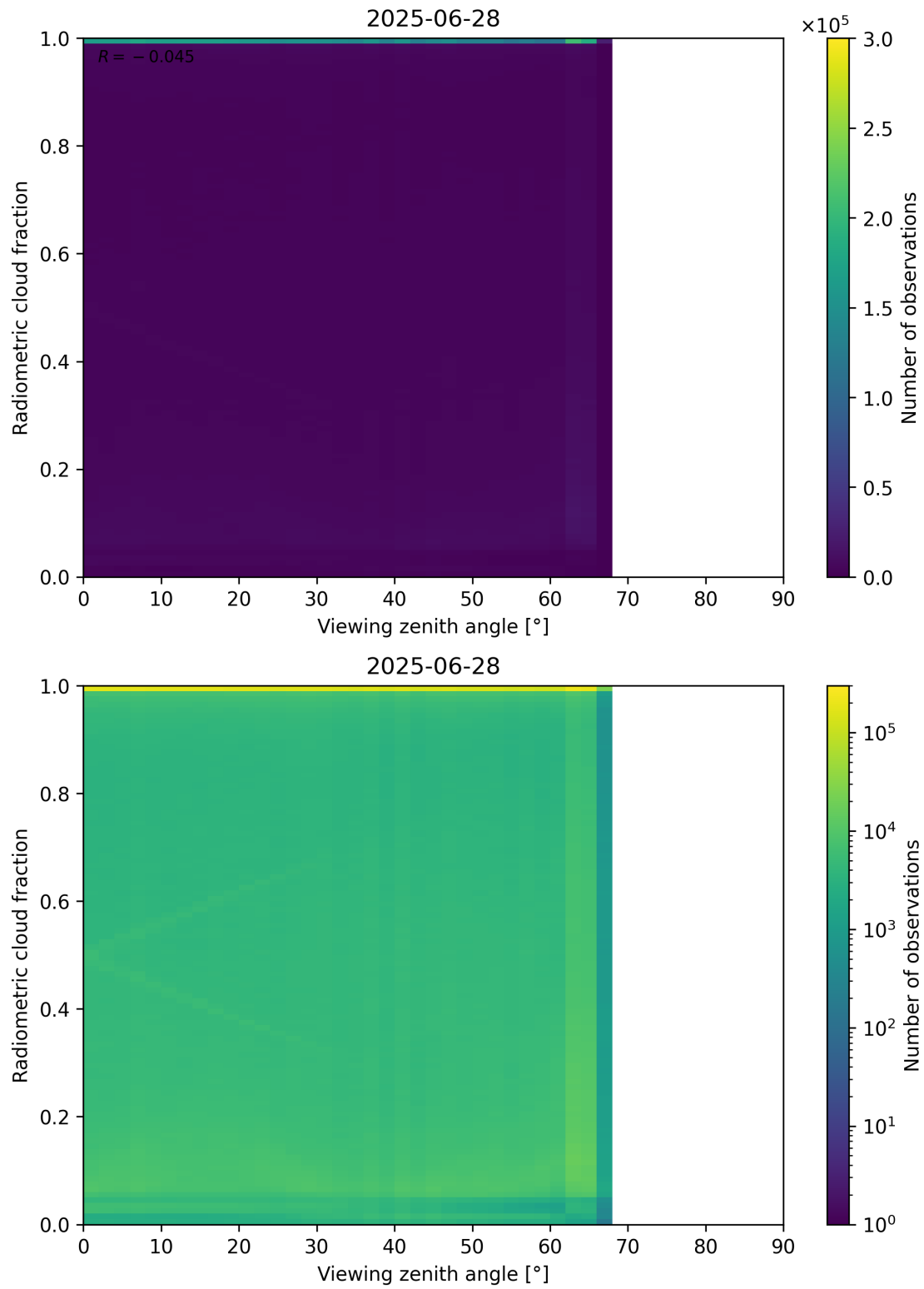
Figure 107: Scatter density plot of “Viewing zenith angle” against “Radiometric cloud fraction” for 2025-06-27 to 2025-06-29.
