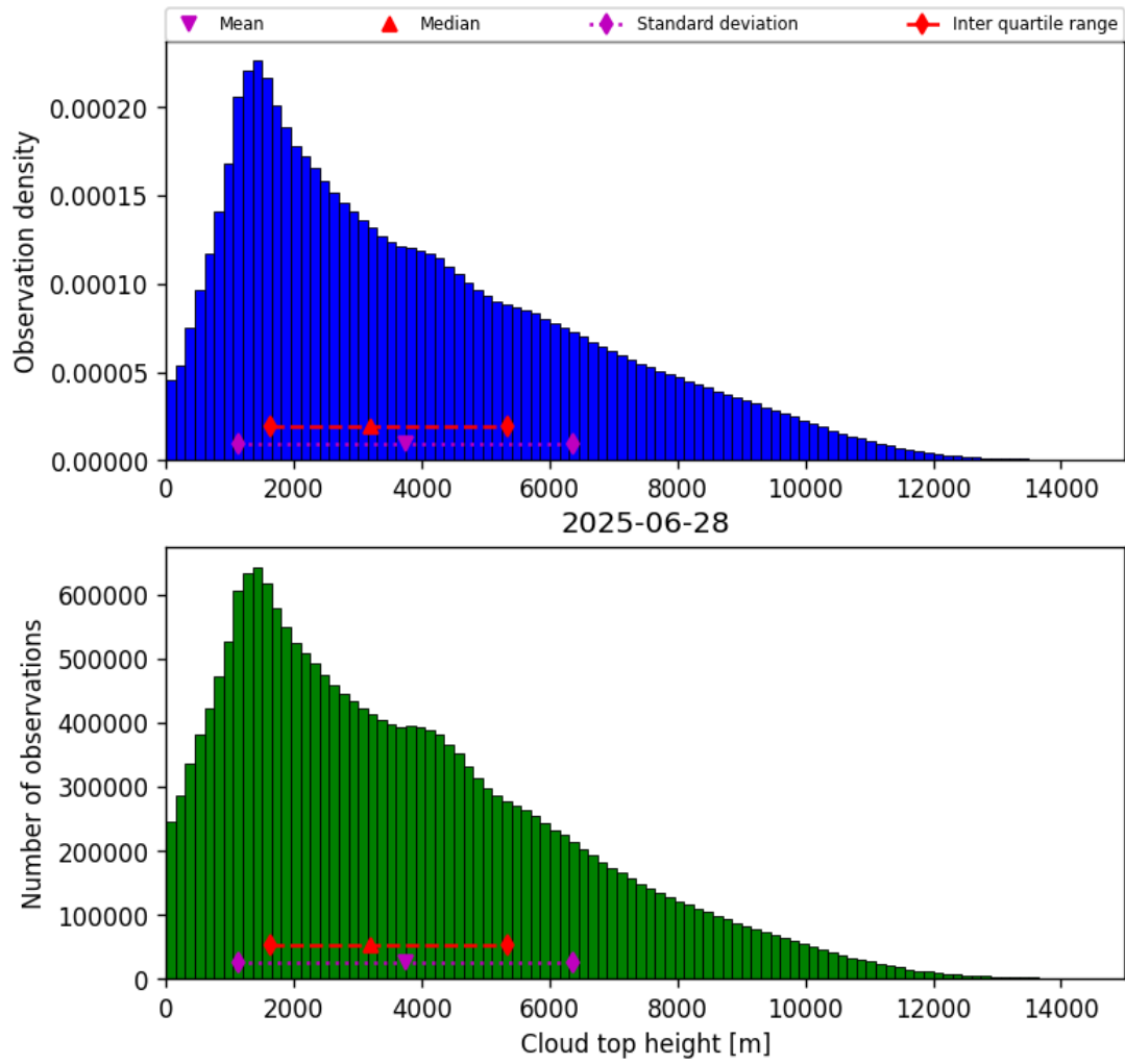
Figure 40: Histogram of “Cloud top height” for 2025-06-27 to 2025-06-29
