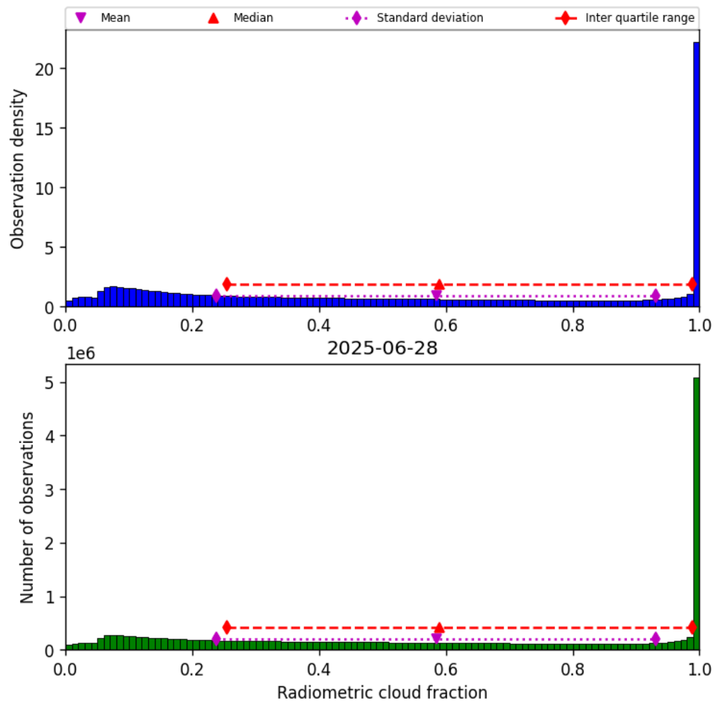
Figure 39: Histogram of “Radiometric cloud fraction” for 2025-06-27 to 2025-06-29
