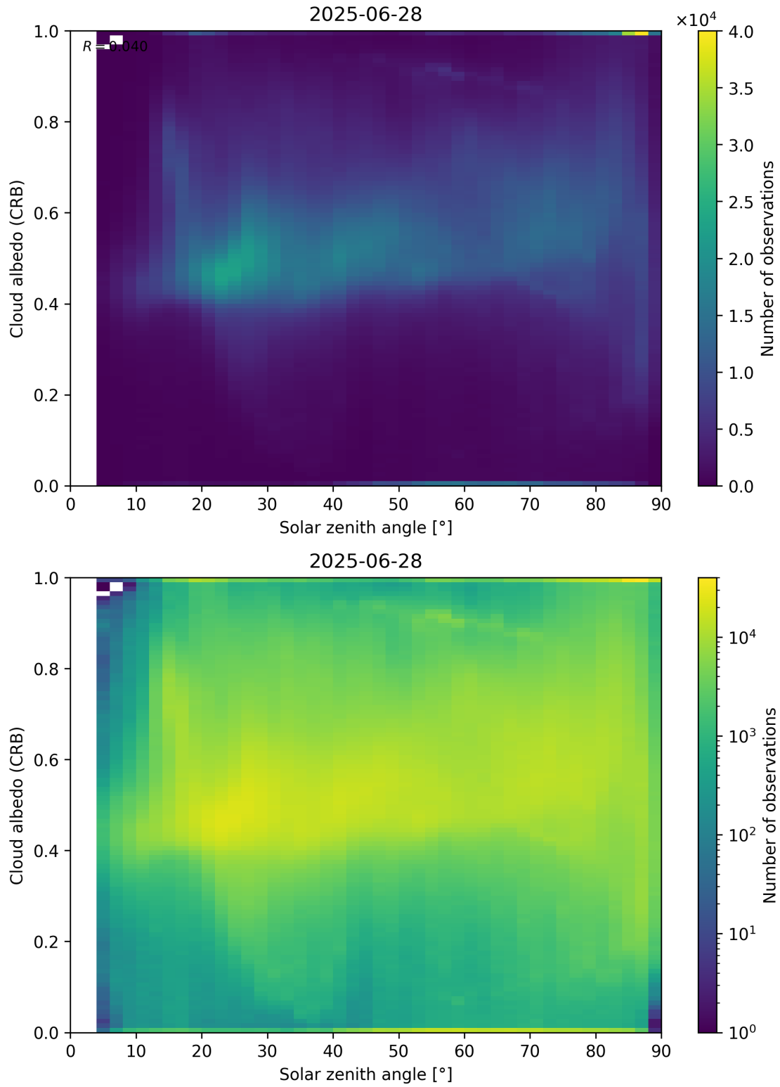
Figure 98: Scatter density plot of “Solar zenith angle” against “Cloud albedo (CRB)” for 2025-06-27 to 2025-06-29.
