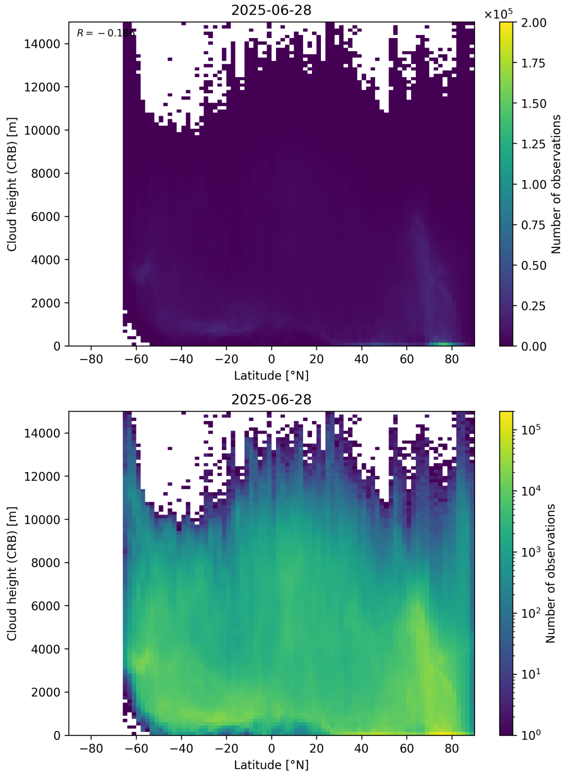
Figure 95: Scatter density plot of “Latitude” against “Cloud height (CRB)” for 2025-06-27 to 2025-06-29.
