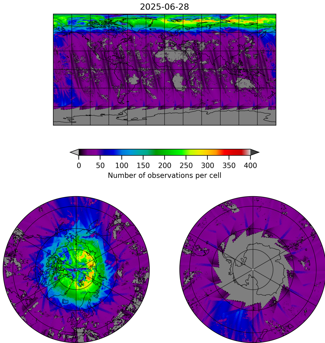
Figure 21: Map of the number of observations for 2025-06-27 to 2025-06-29
