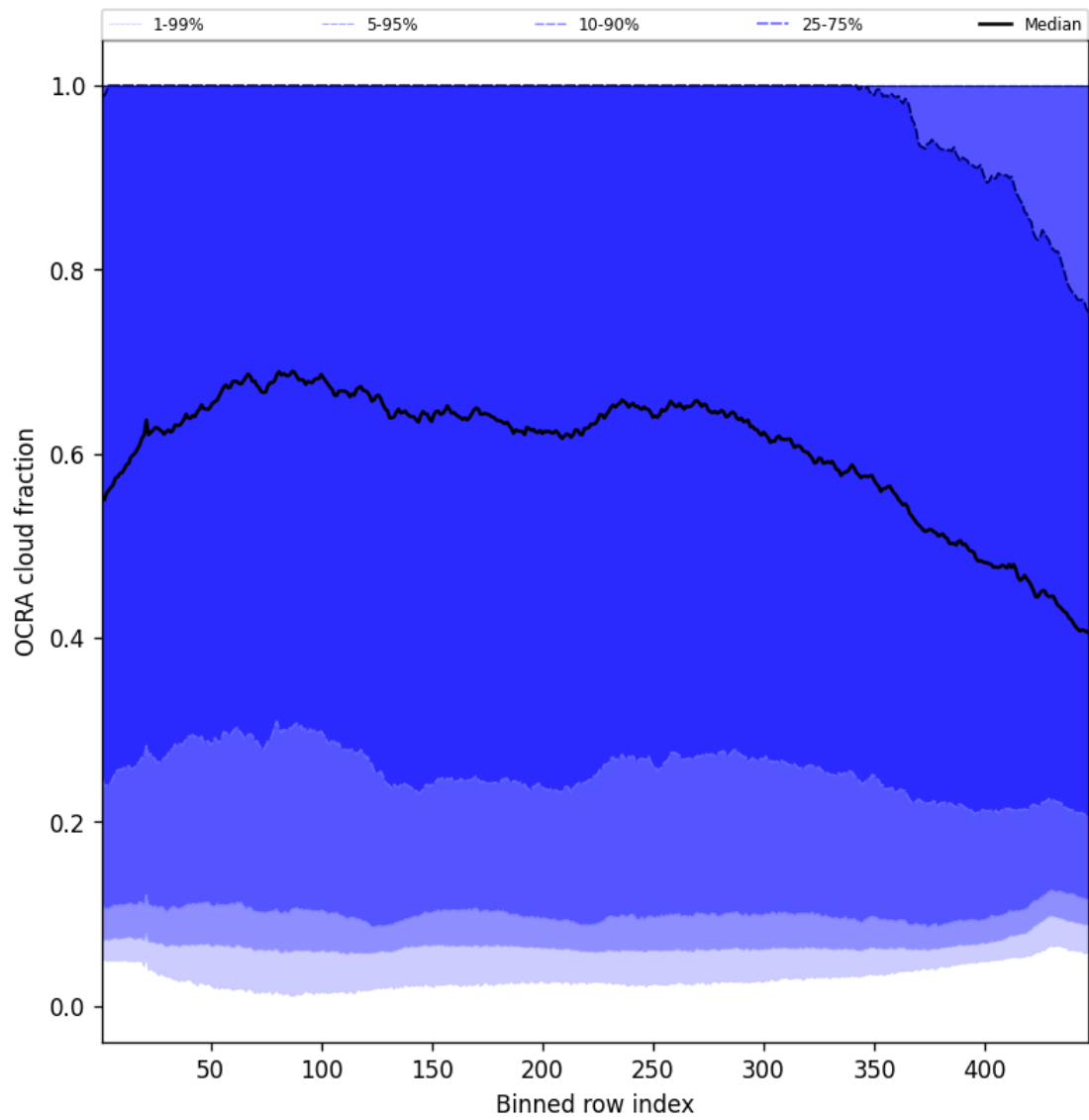
Figure 66: Along track statistics of “OCRA cloud fraction” for 2025-06-27 to 2025-06-29
