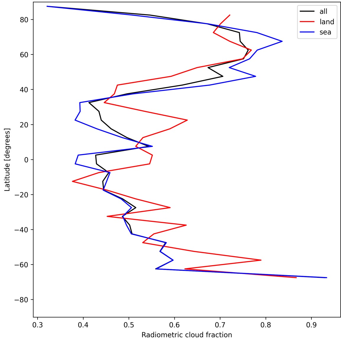
Figure 23: Zonal average of “Radiometric cloud fraction” for 2025-06-27 to 2025-06-29.
