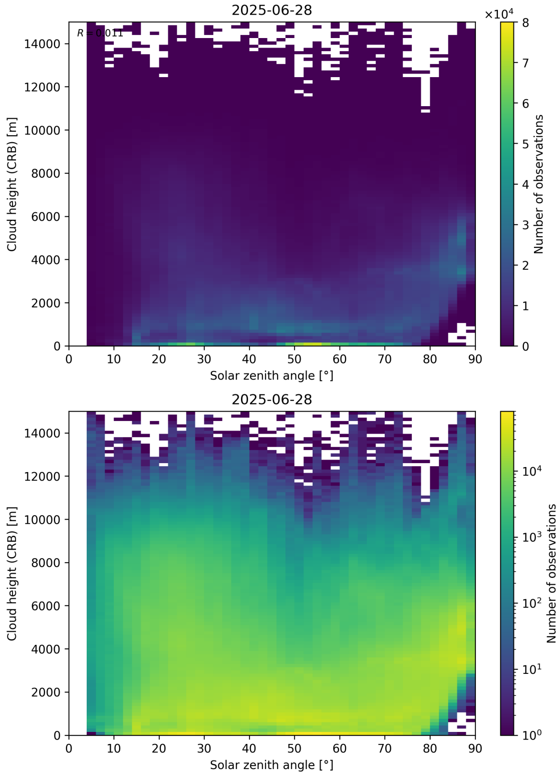
Figure 102: Scatter density plot of “Solar zenith angle” against “Cloud height (CRB)” for 2025-06-27 to 2025-06-29.
