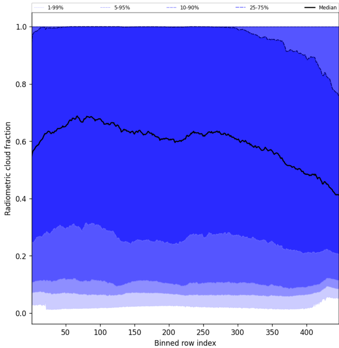
Figure 55: Along track statistics of “Radiometric cloud fraction” for 2025-06-27 to 2025-06-29
