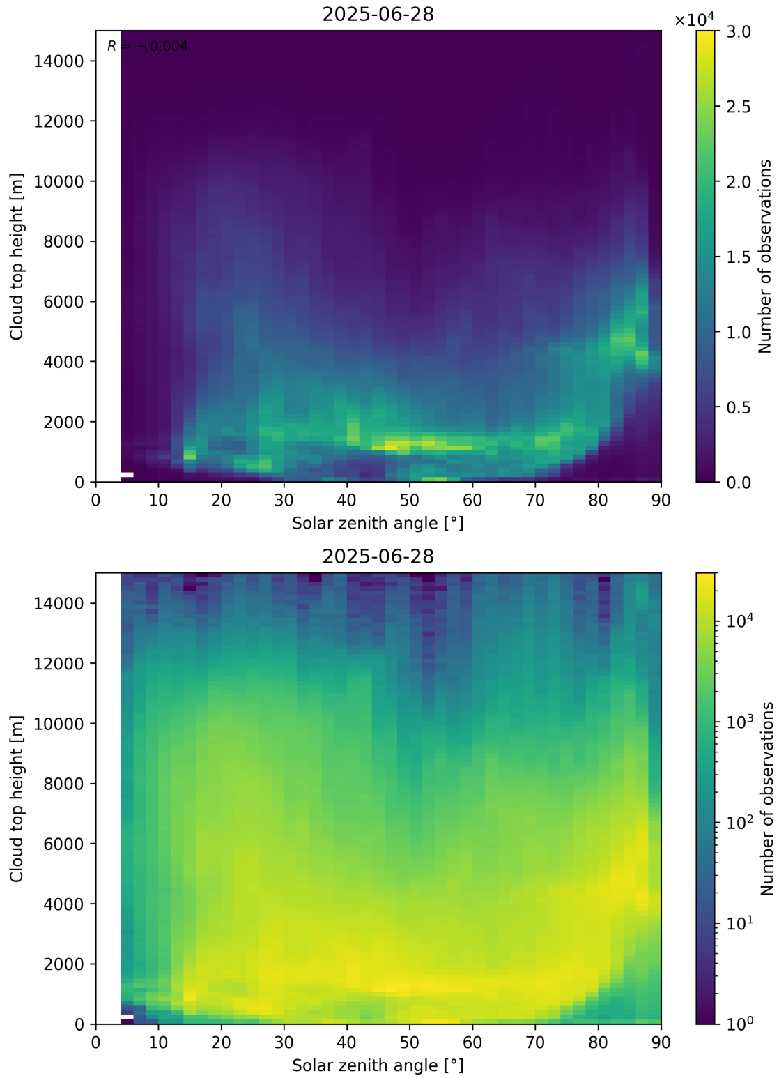
Figure 104: Scatter density plot of “Solar zenith angle” against “Cloud top height” for 2025-06-27 to 2025-06-29.
