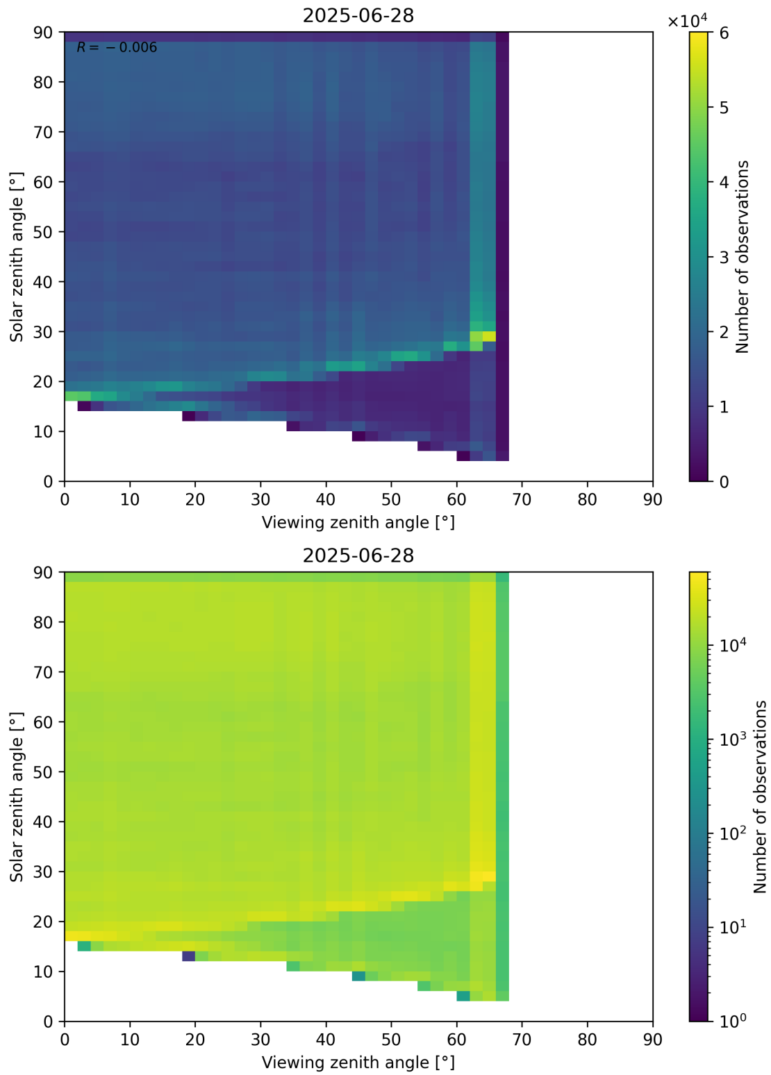
Figure 114: Scatter density plot of “Viewing zenith angle” against “Solar zenith angle” for 2025-06-27 to 2025-06-29.
