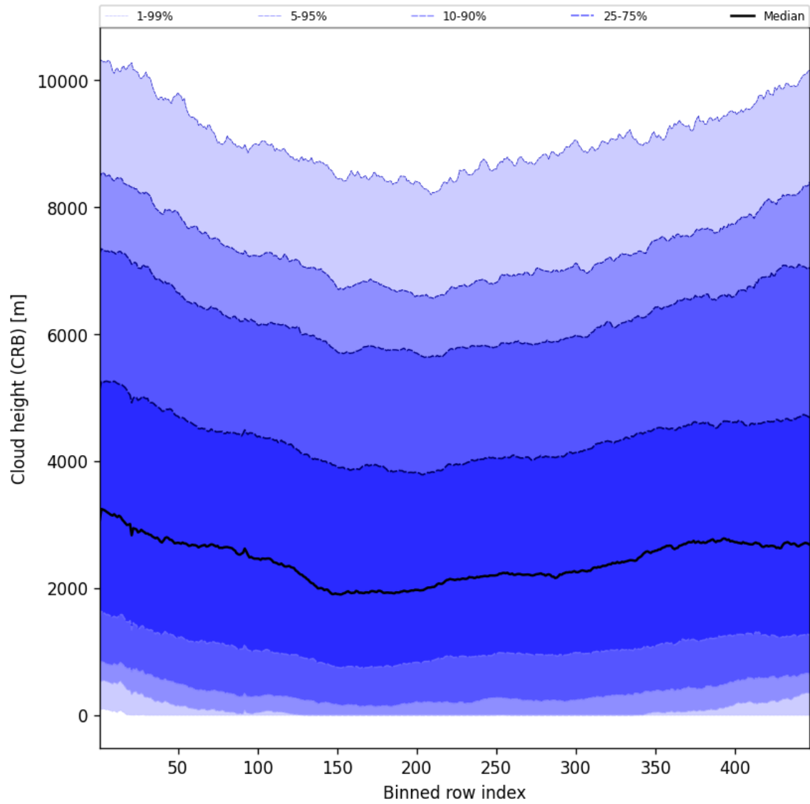
Figure 59: Along track statistics of “Cloud height (CRB)” for 2025-06-27 to 2025-06-29
