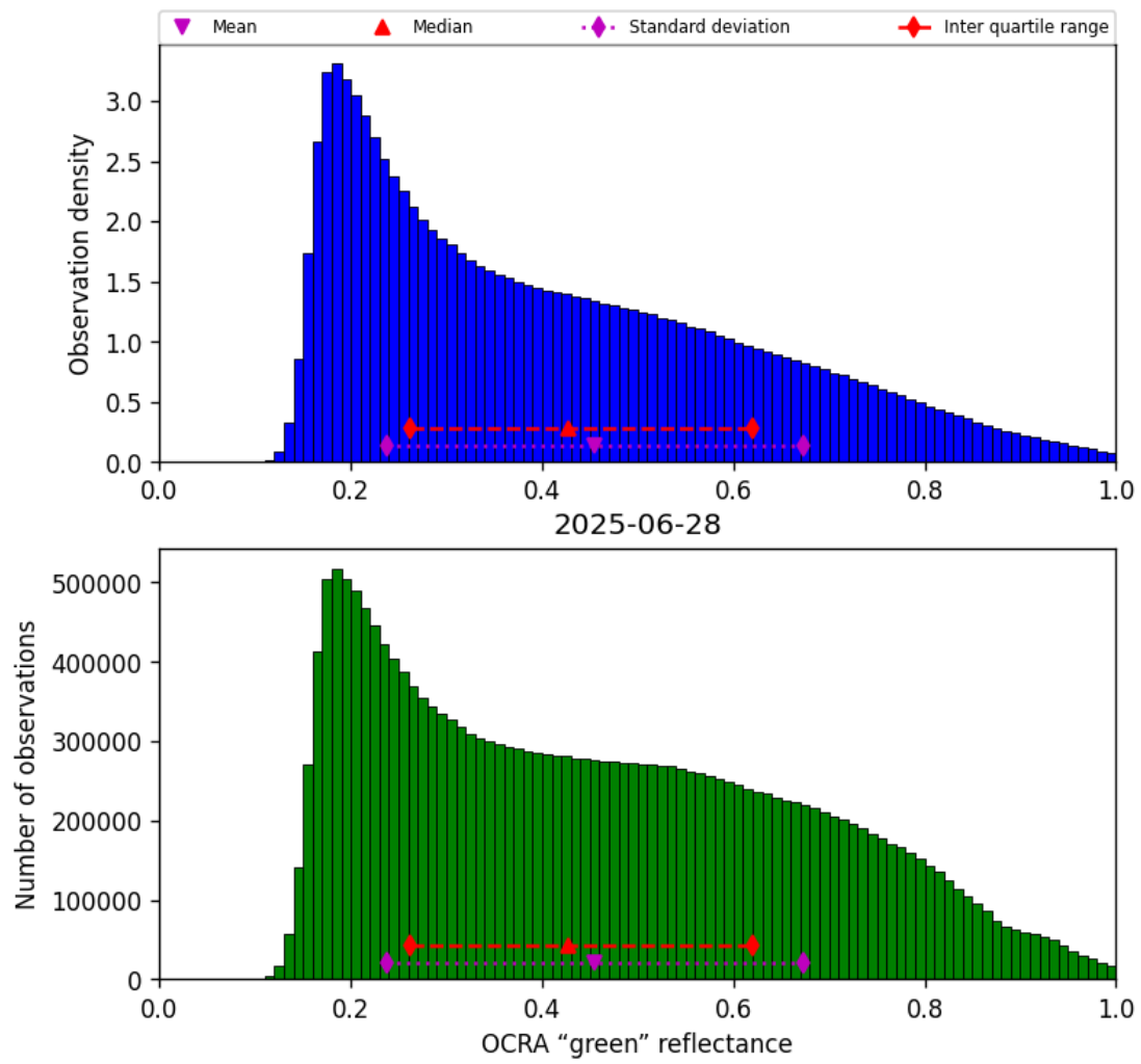
Figure 52: Histogram of “OCRA “green” reflectance” for 2025-06-27 to 2025-06-29
