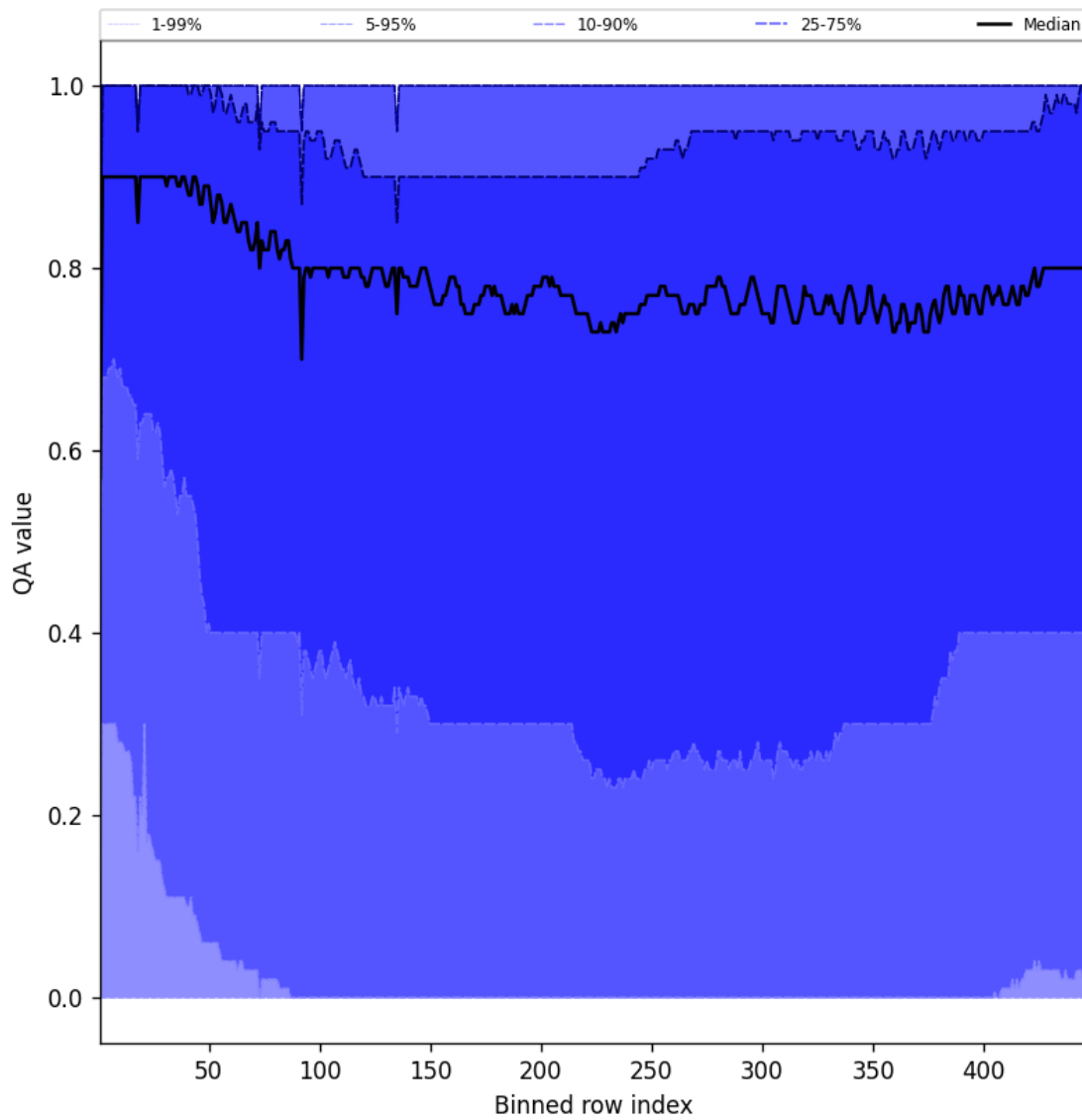
Figure 54: Along track statistics of “QA value” for 2025-06-27 to 2025-06-29
