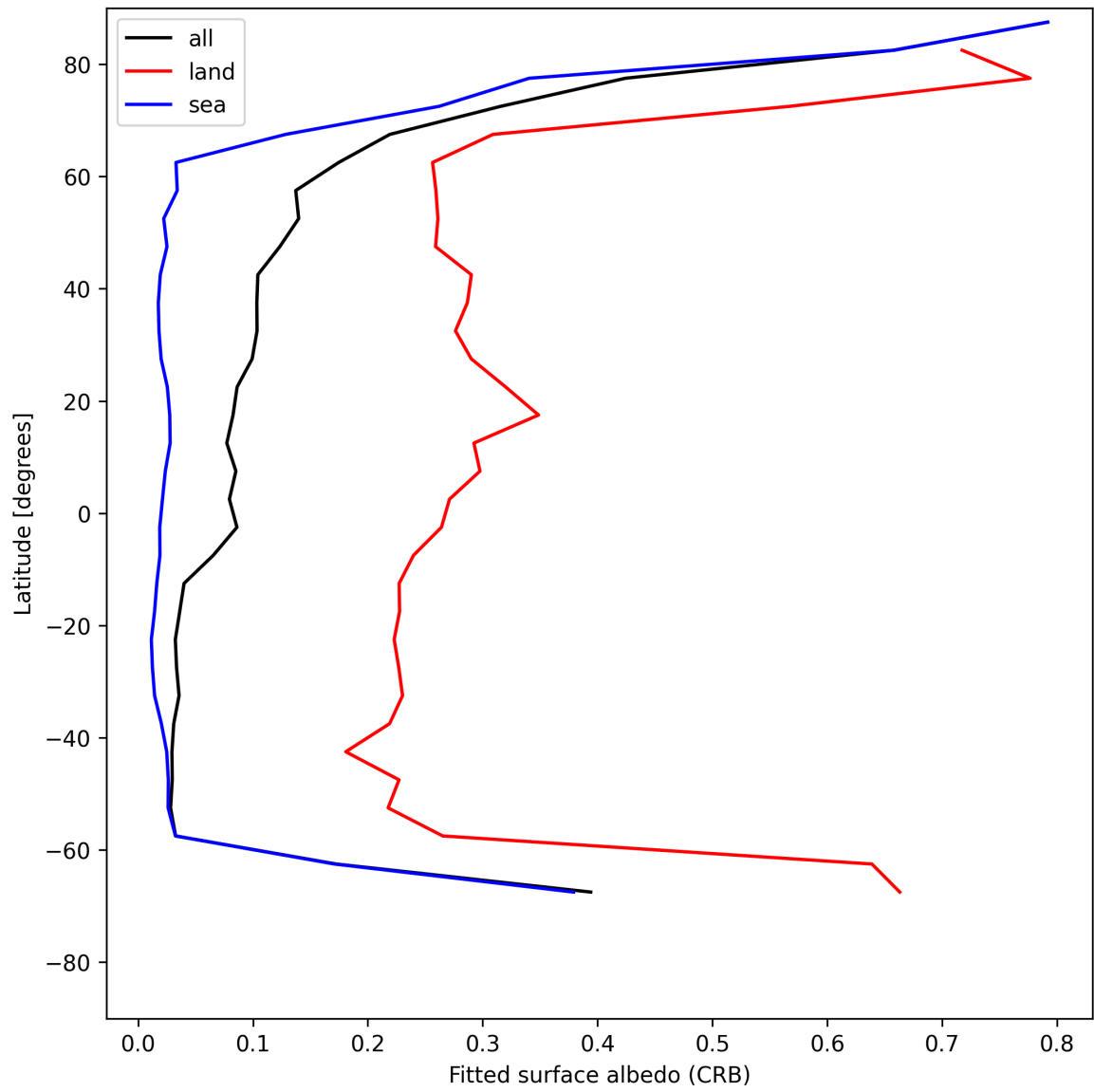
Figure 30: Zonal average of “Fitted surface albedo (CRB)” for 2025-06-27 to 2025-06-29.
