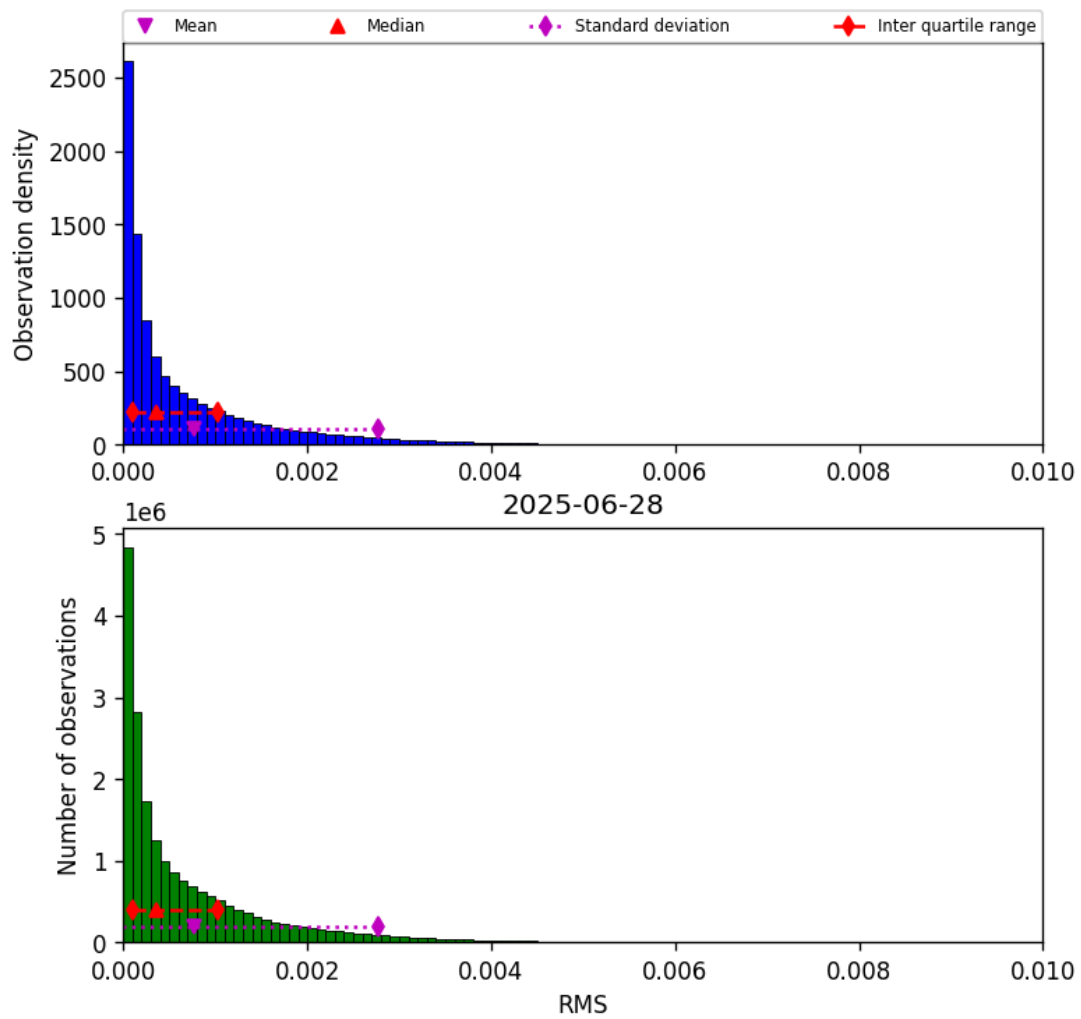
Figure 47: Histogram of “RMS” for 2025-06-27 to 2025-06-29
