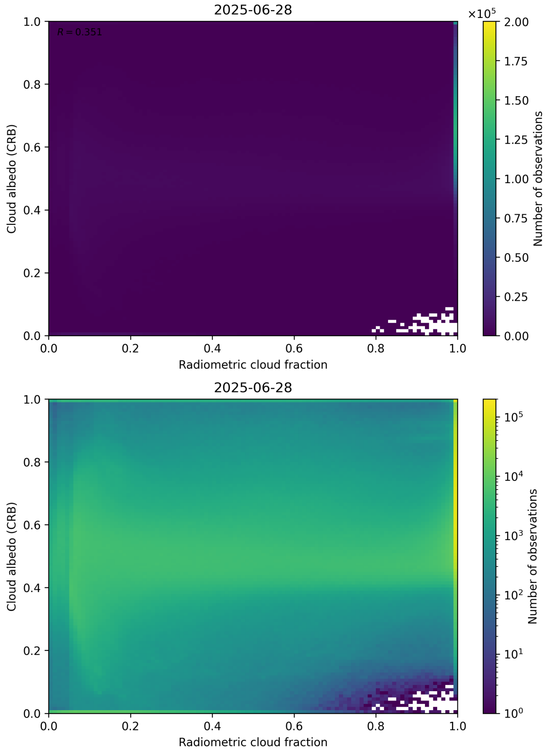
Figure 71: Scatter density plot of “Radiometric cloud fraction” against “Cloud albedo (CRB)” for 2025-06-27 to 2025-06-29.
