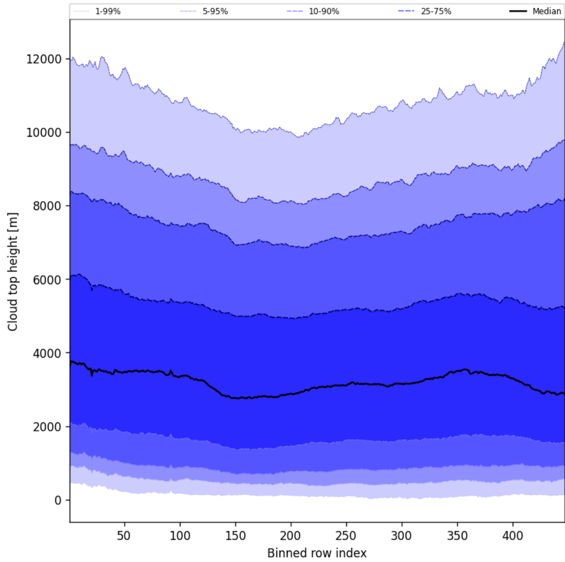
Figure 56: Along track statistics of “Cloud top height” for 2025-06-27 to 2025-06-29
