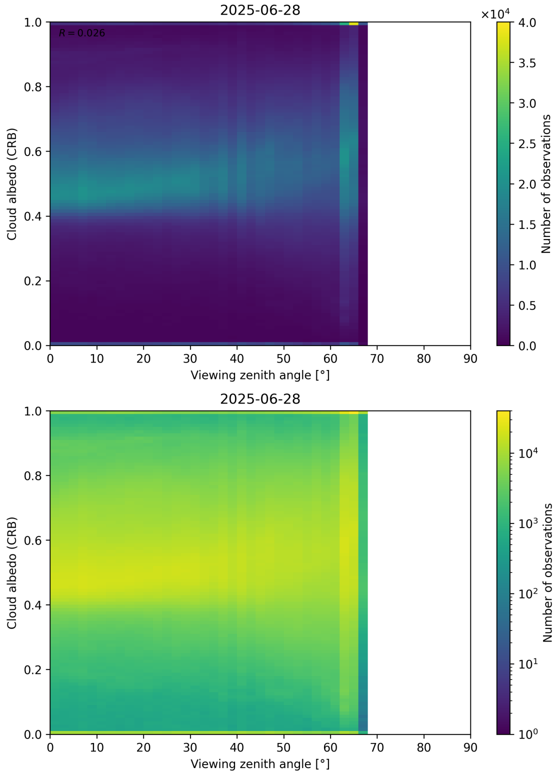
Figure 106: Scatter density plot of “Viewing zenith angle” against “Cloud albedo (CRB)” for 2025-06-27 to 2025-06-29.
