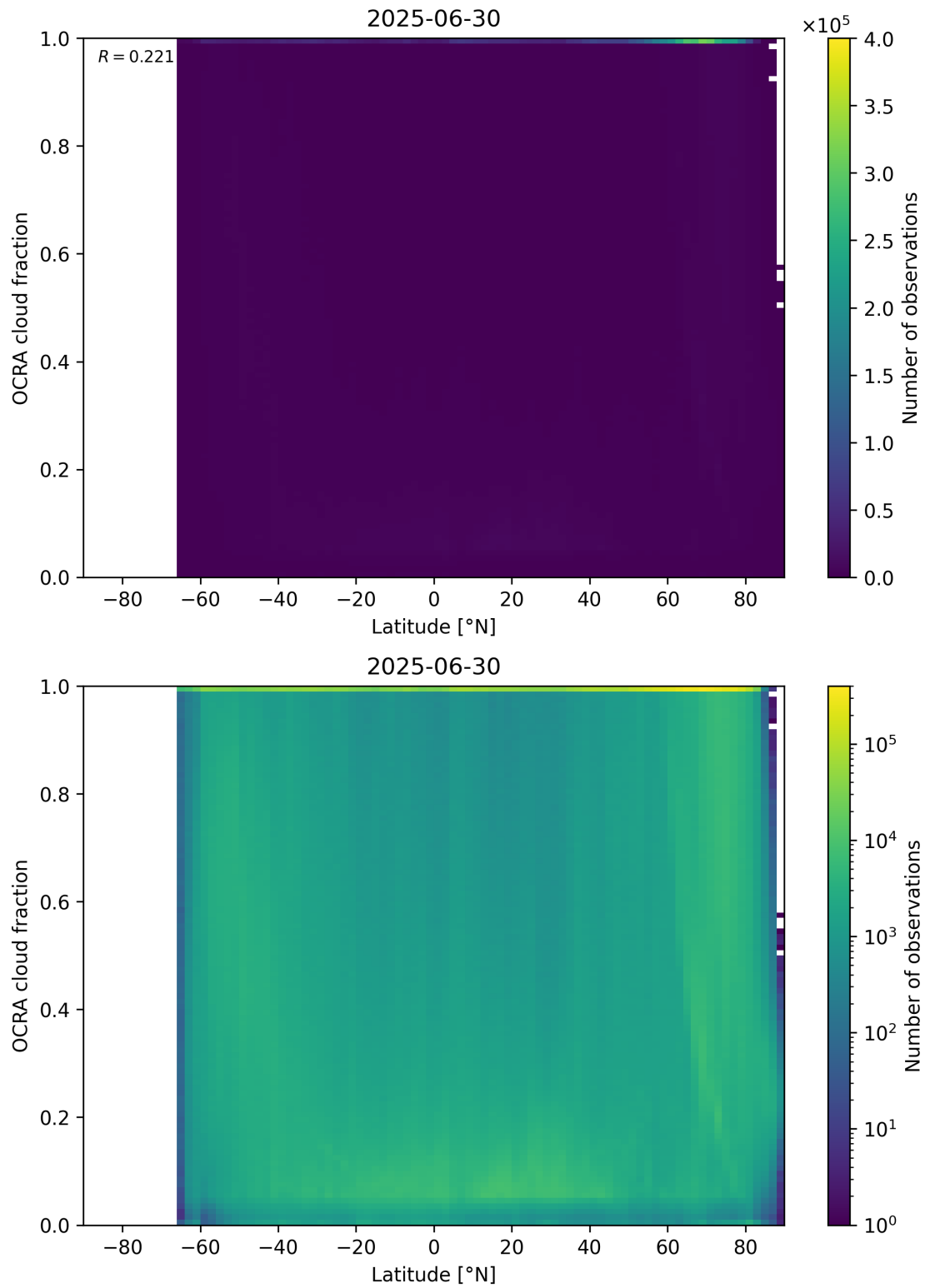
Figure 93: Scatter density plot of “Latitude” against “OCRA cloud fraction” for 2025-06-29 to 2025-07-01.
