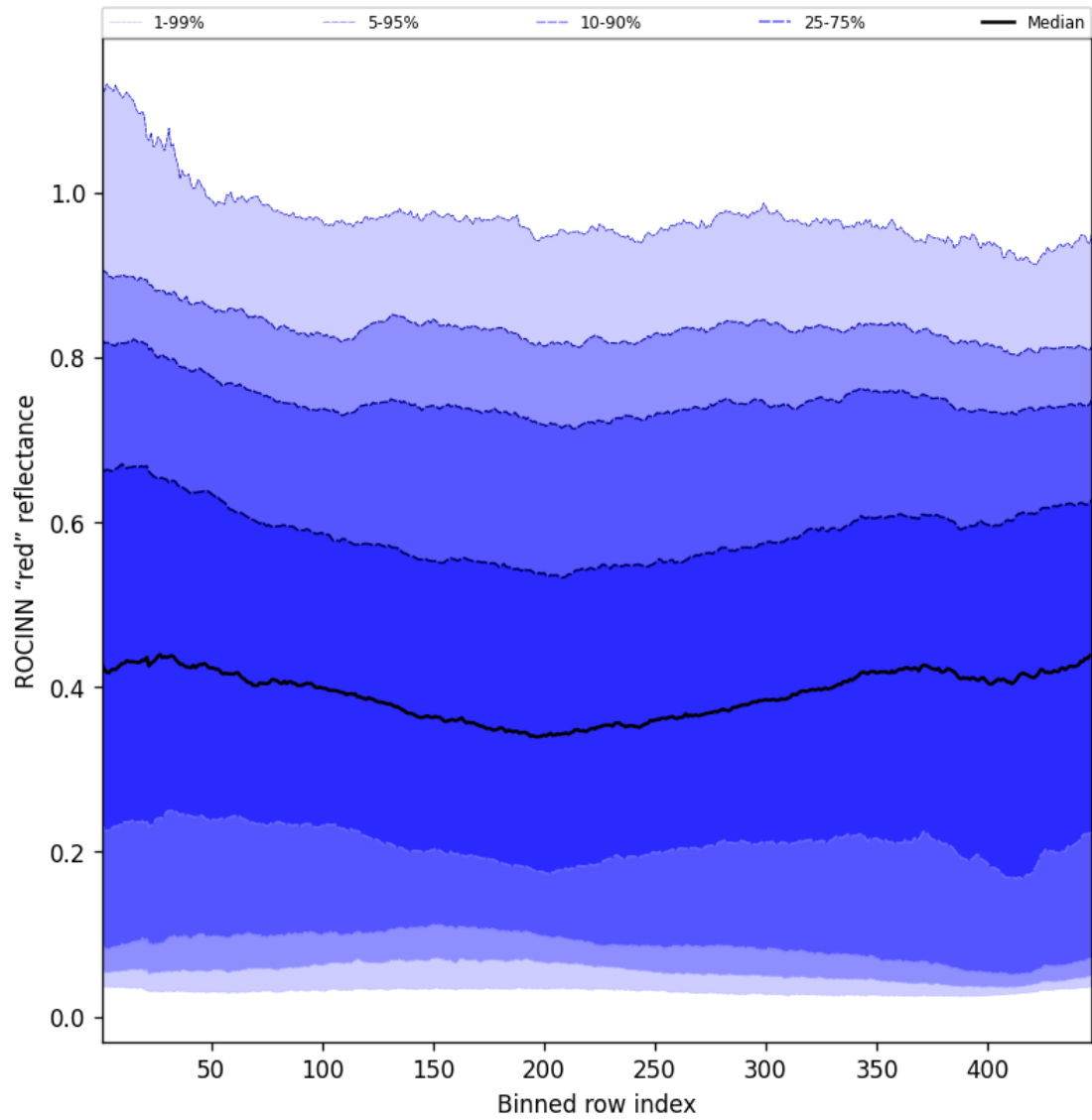
Figure 69: Along track statistics of "ROCINN "red" reflectance" for 2025-06-29 to 2025-07-01
