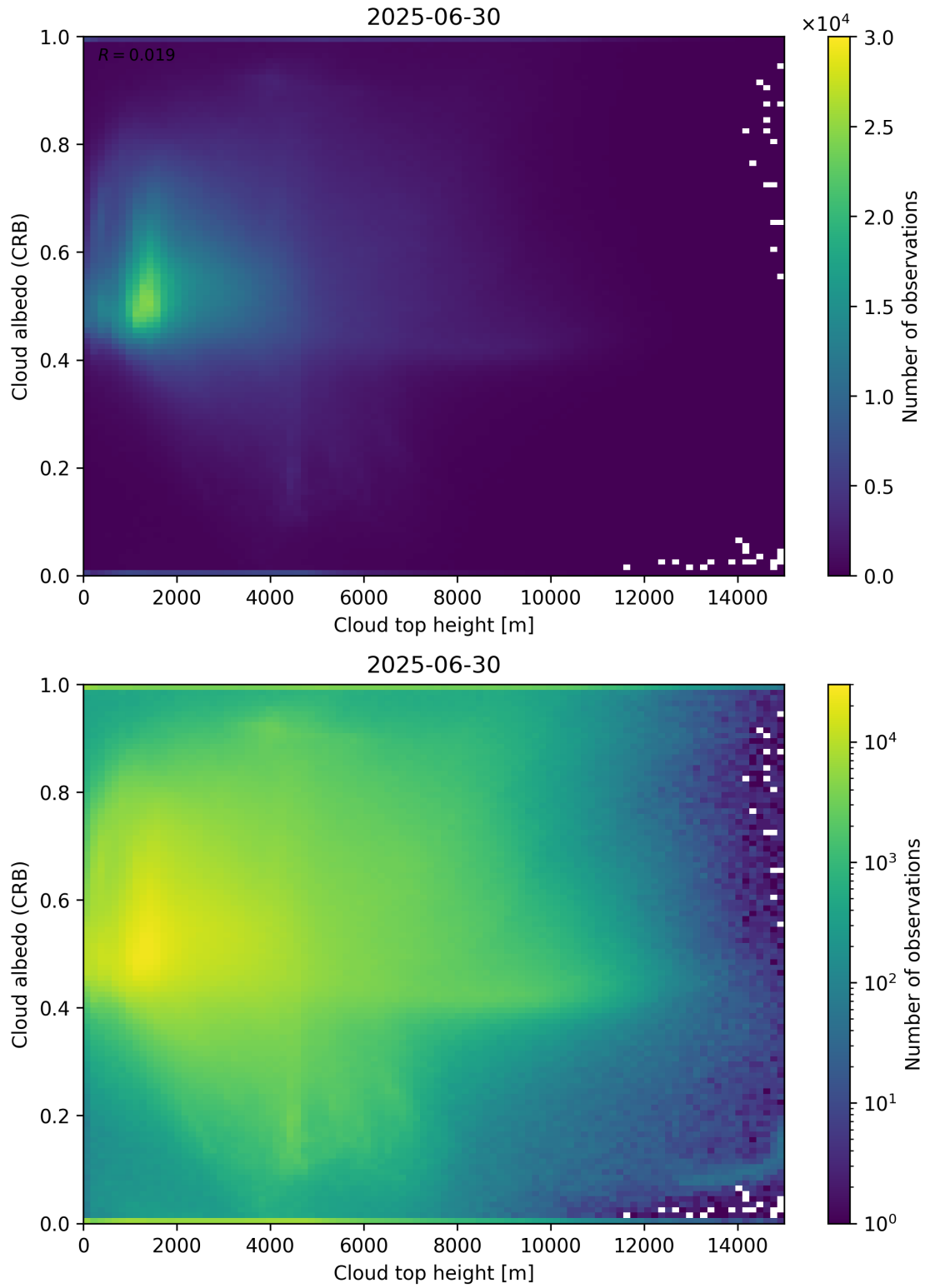
Figure 86: Scatter density plot of “Cloud top height” against “Cloud albedo (CRB)” for 2025-06-29 to 2025-07-01.
