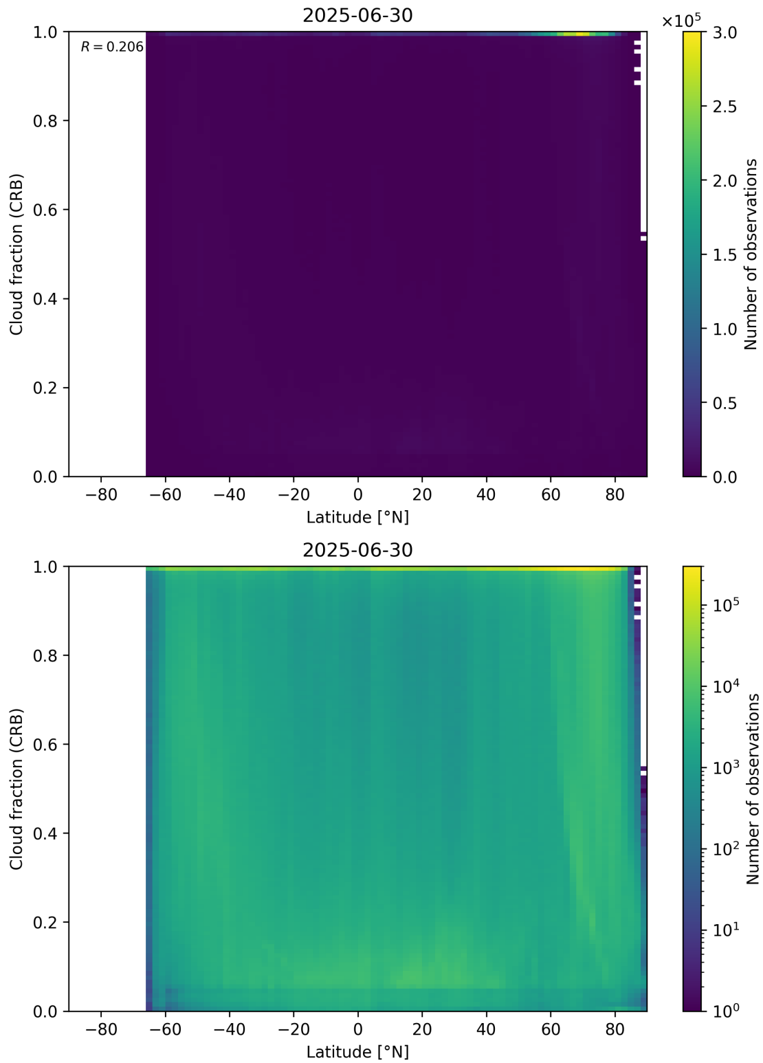
Figure 94: Scatter density plot of “Latitude” against “Cloud fraction (CRB)” for 2025-06-29 to 2025-07-01.
