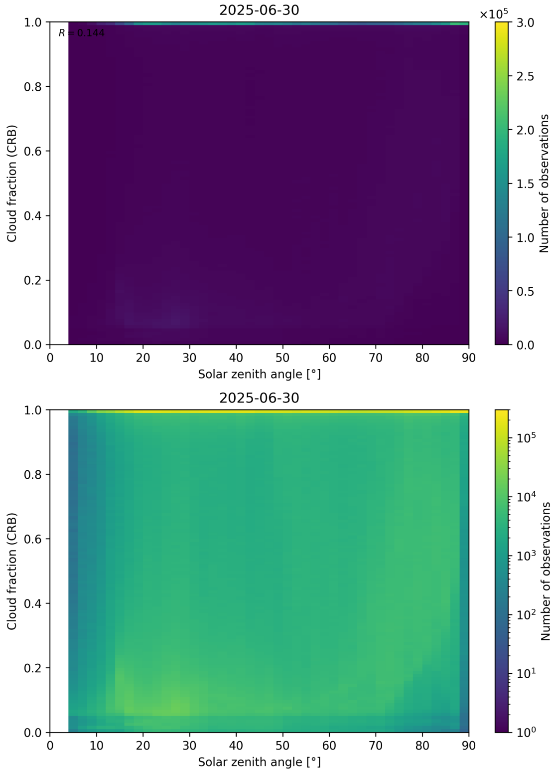
Figure 101: Scatter density plot of “Solar zenith angle” against “Cloud fraction (CRB)” for 2025-06-29 to 2025-07-01.
