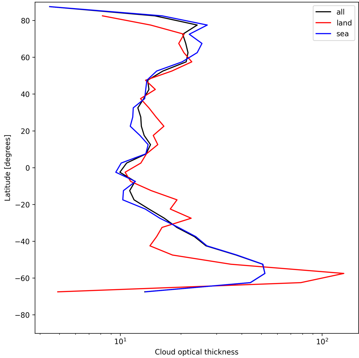
Figure 25: Zonal average of “Cloud optical thickness” for 2025-06-29 to 2025-07-01.
