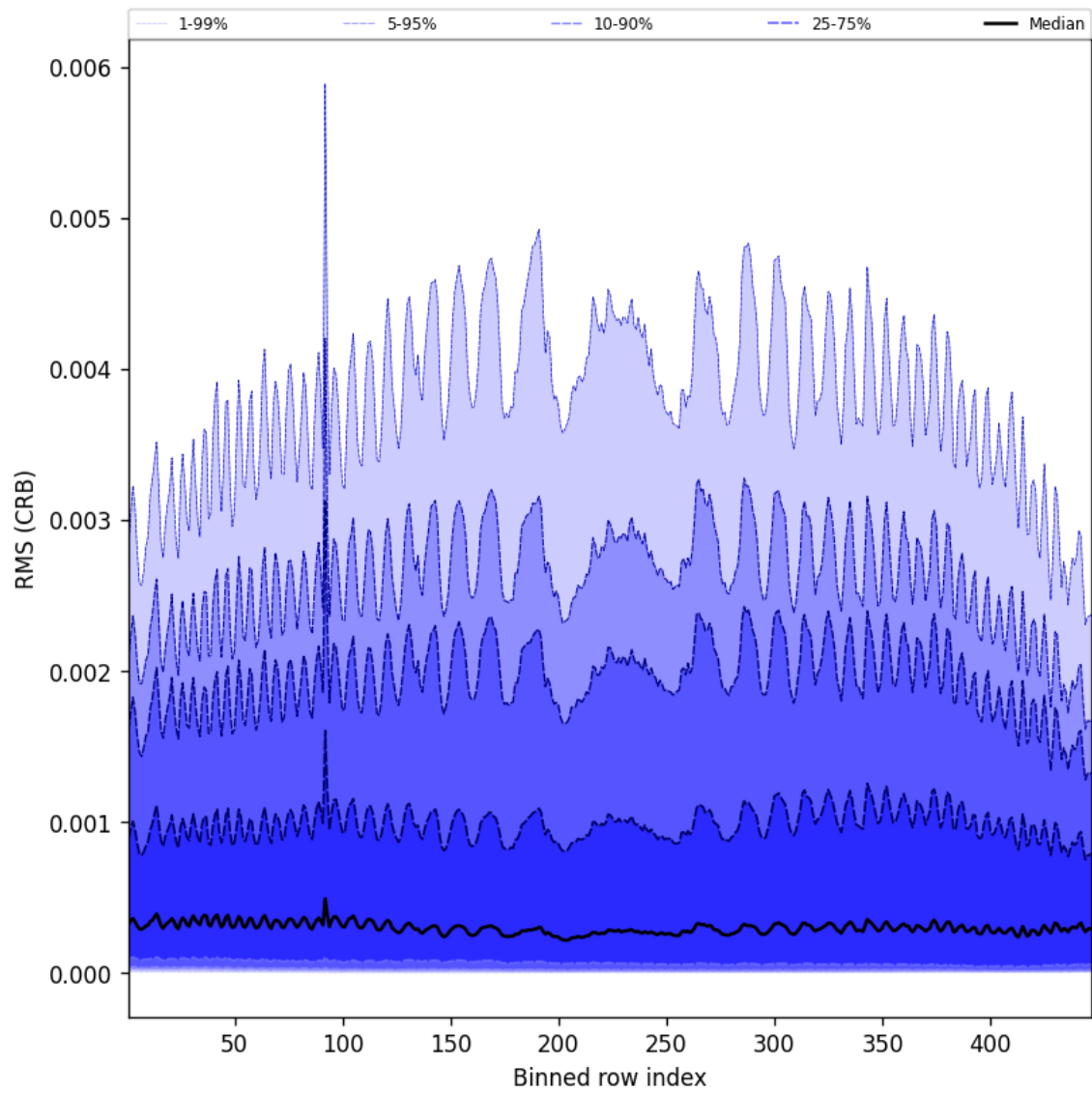
Figure 64: Along track statistics of “RMS (CRB)” for 2025-06-29 to 2025-07-01
