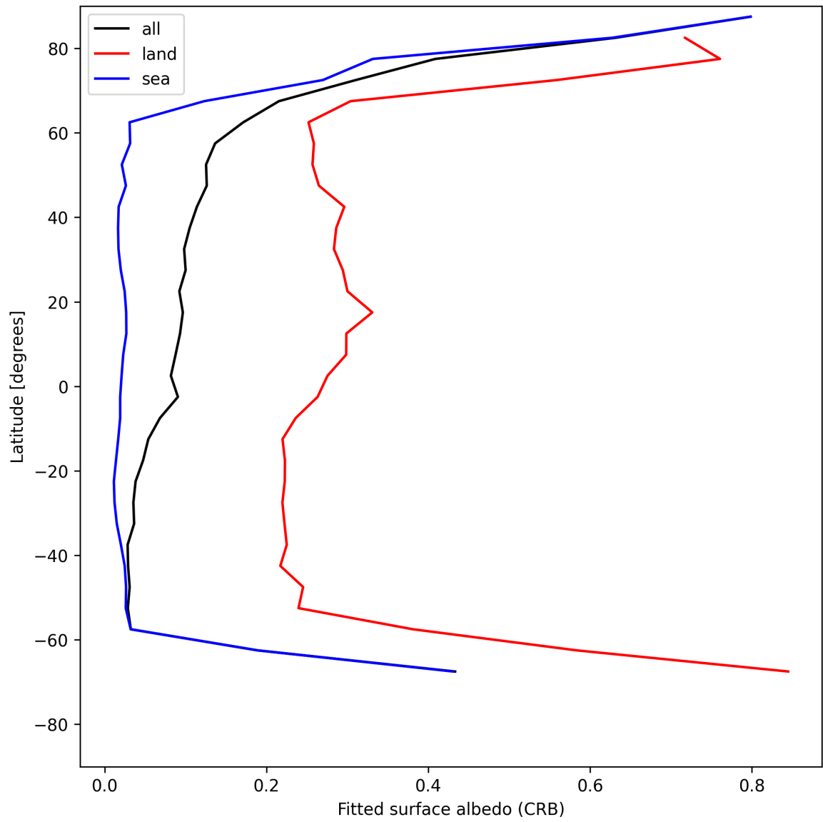
Figure 30: Zonal average of “Fitted surface albedo (CRB)” for 2025-06-29 to 2025-07-01.
