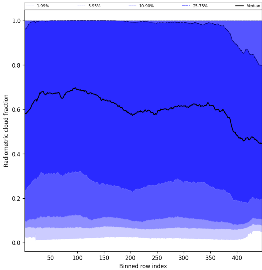
Figure 55: Along track statistics of “Radiometric cloud fraction” for 2025-06-29 to 2025-07-01
