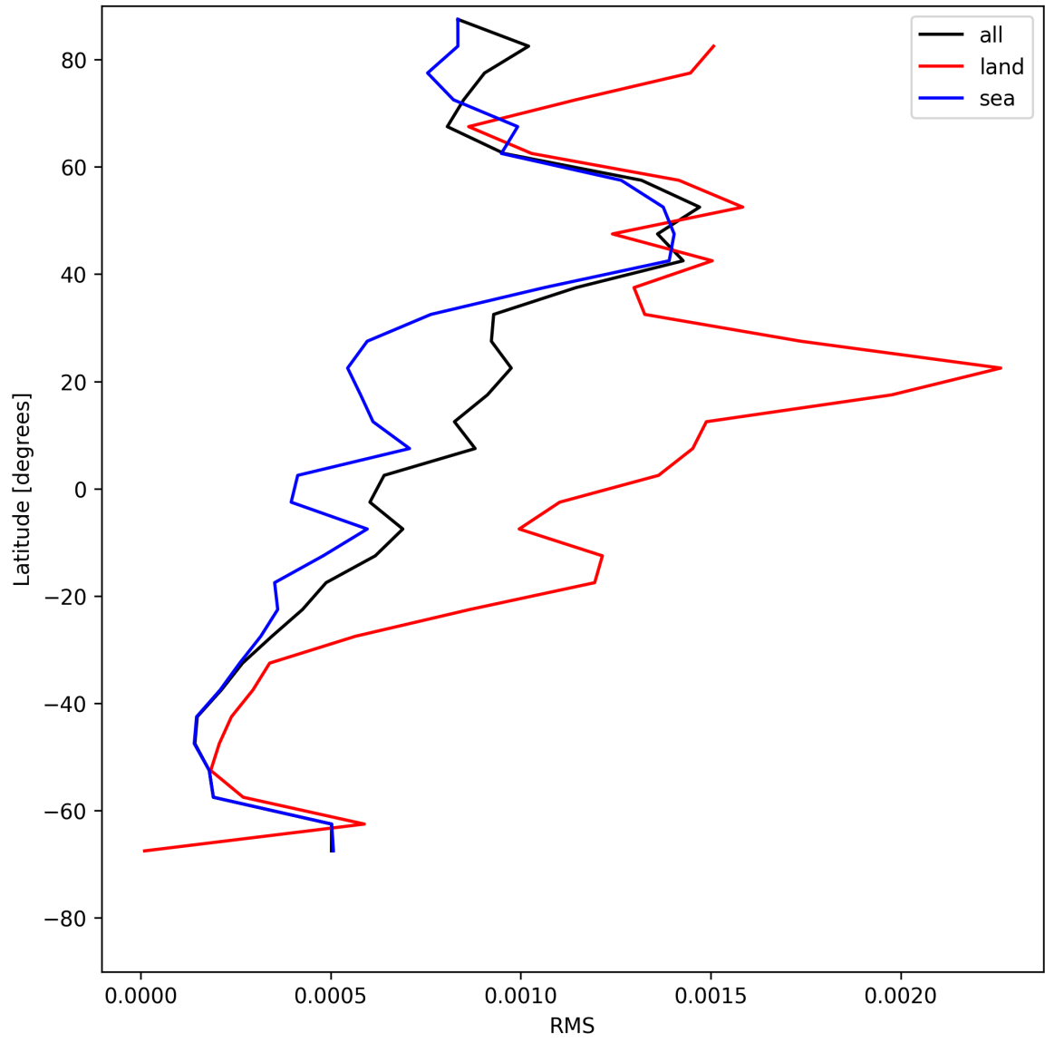
Figure 31: Zonal average of “RMS” for 2025-06-29 to 2025-07-01.
