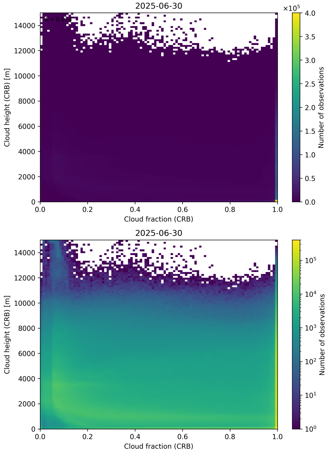
Figure 79: Scatter density plot of “Cloud fraction (CRB)” against “Cloud height (CRB)” for 2025-06-29 to 2025-07-01.
