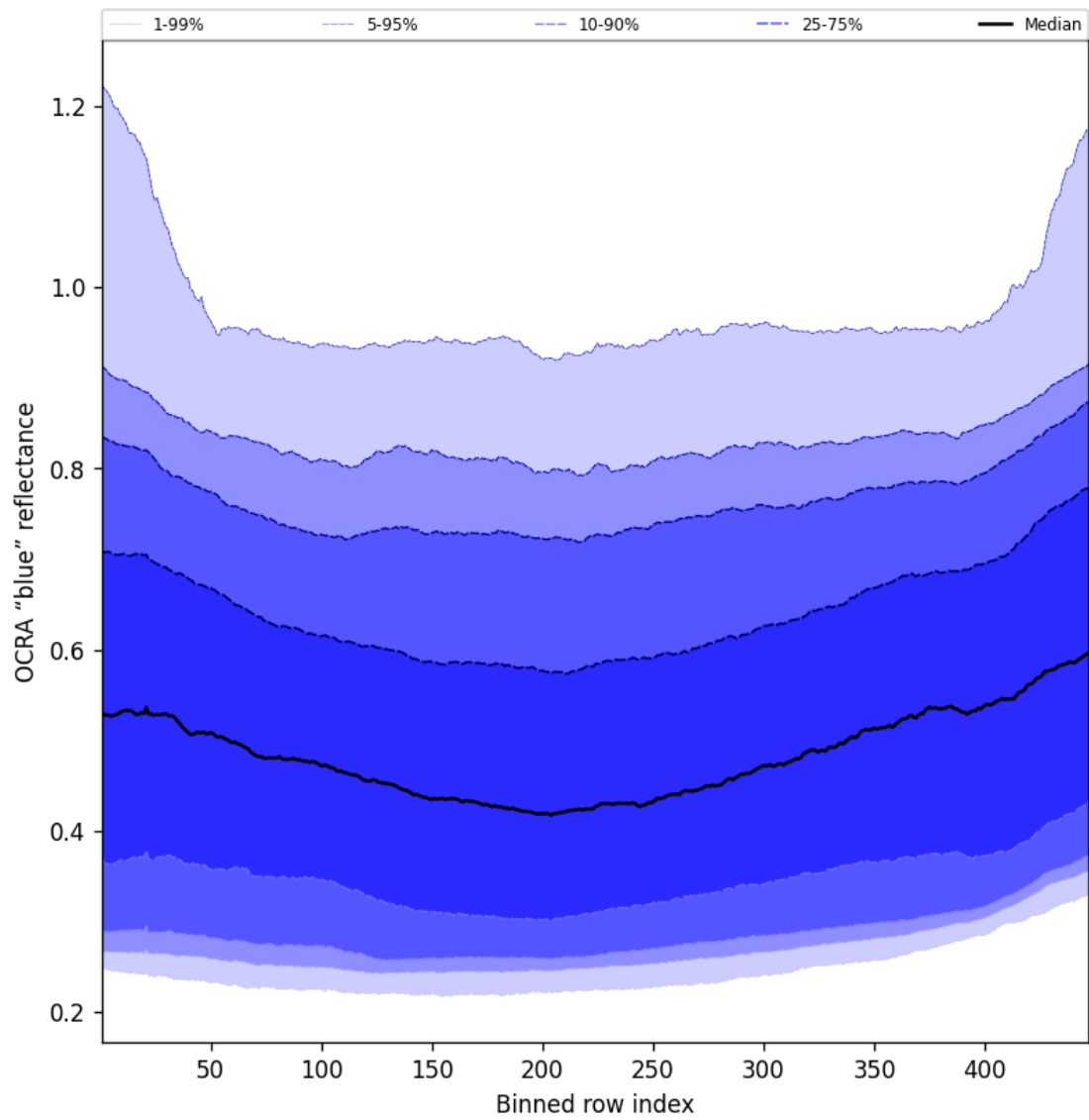
Figure 67: Along track statistics of “OCRA “blue” reflectance” for 2025-06-29 to 2025-07-01
