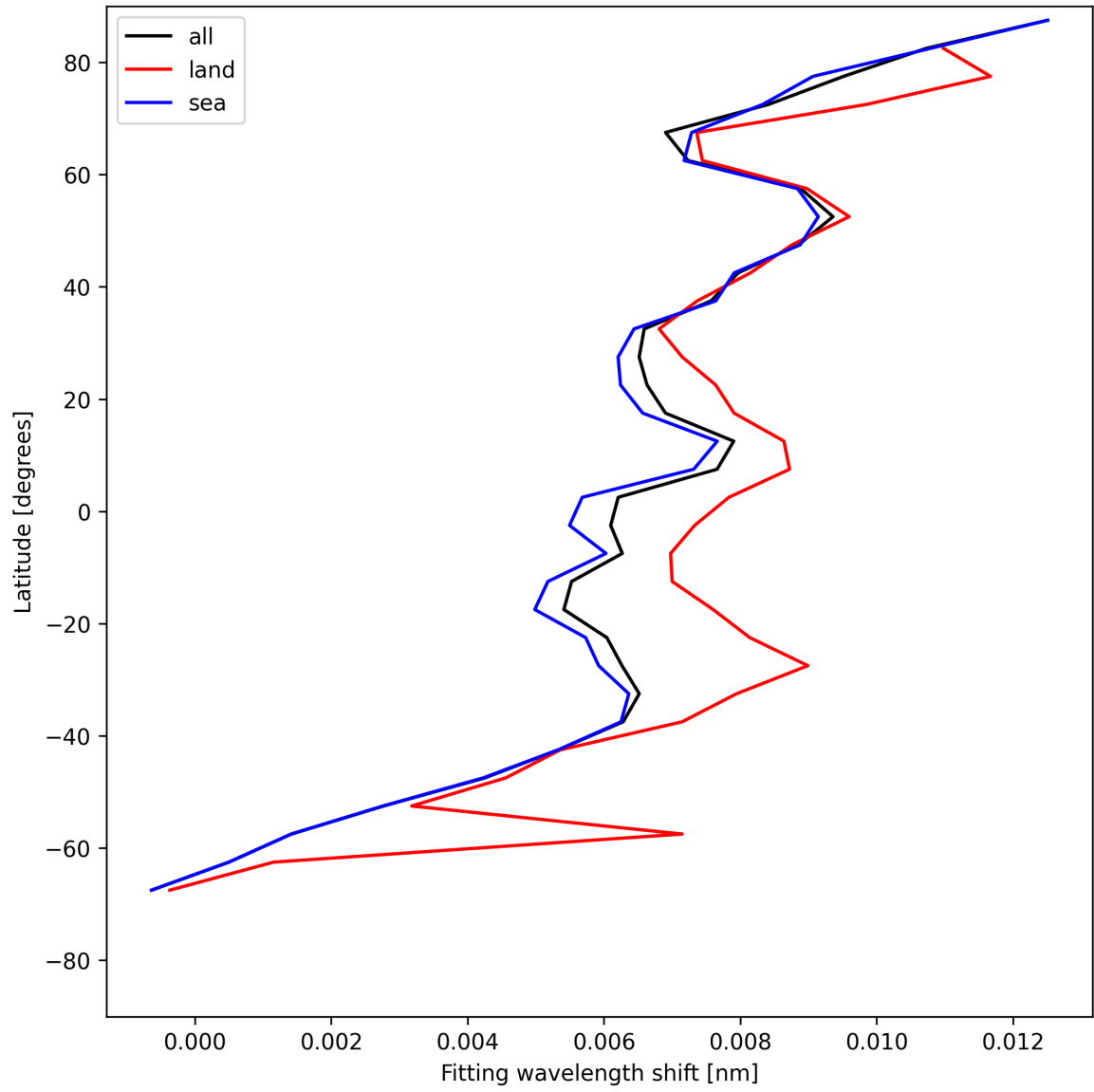
Figure 33: Zonal average of “Fitting wavelength shift” for 2025-06-29 to 2025-07-01.
