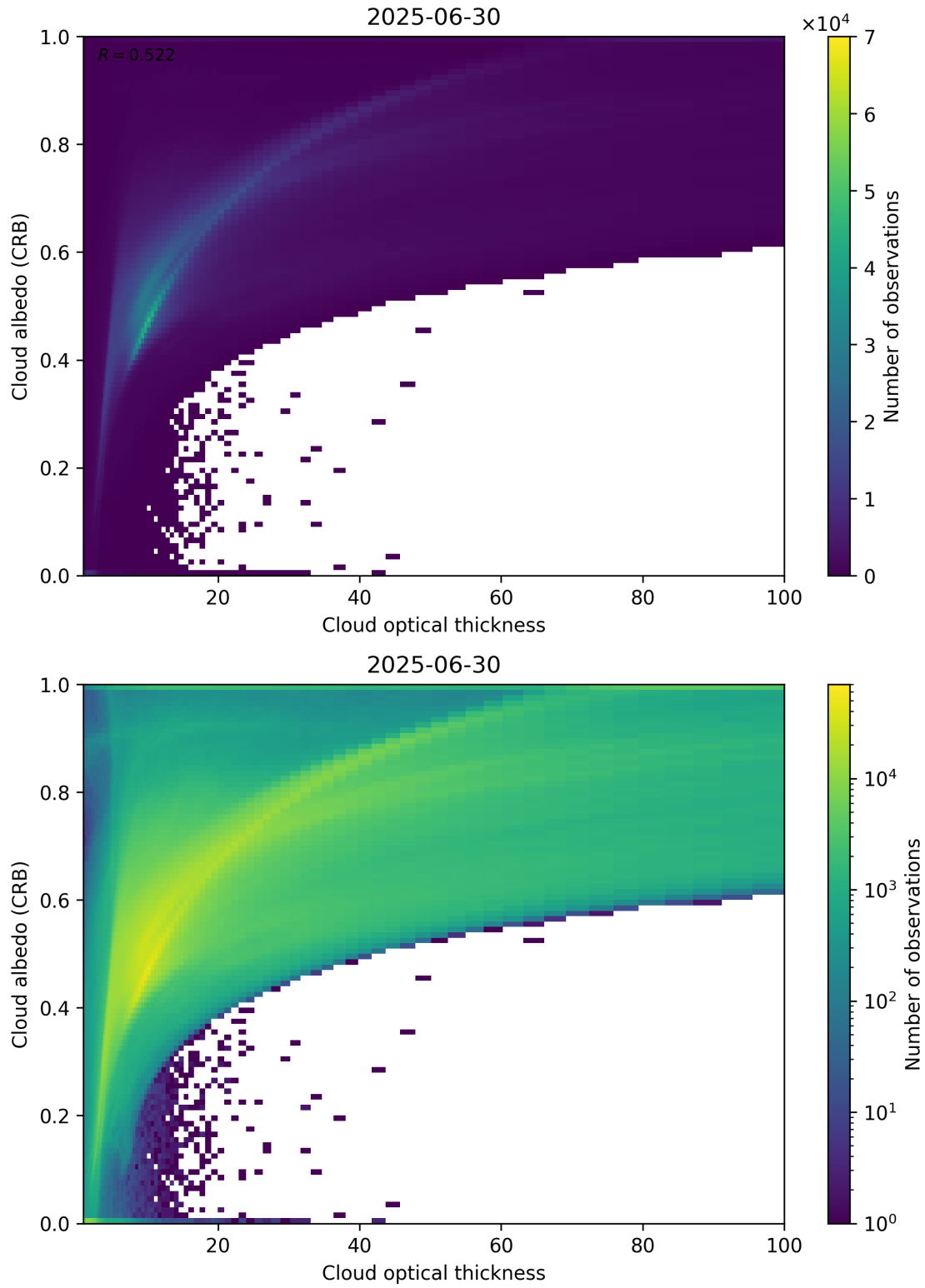
Figure 82: Scatter density plot of “Cloud optical thickness” against “Cloud albedo (CRB)” for 2025-06-29 to 2025-07-01.
