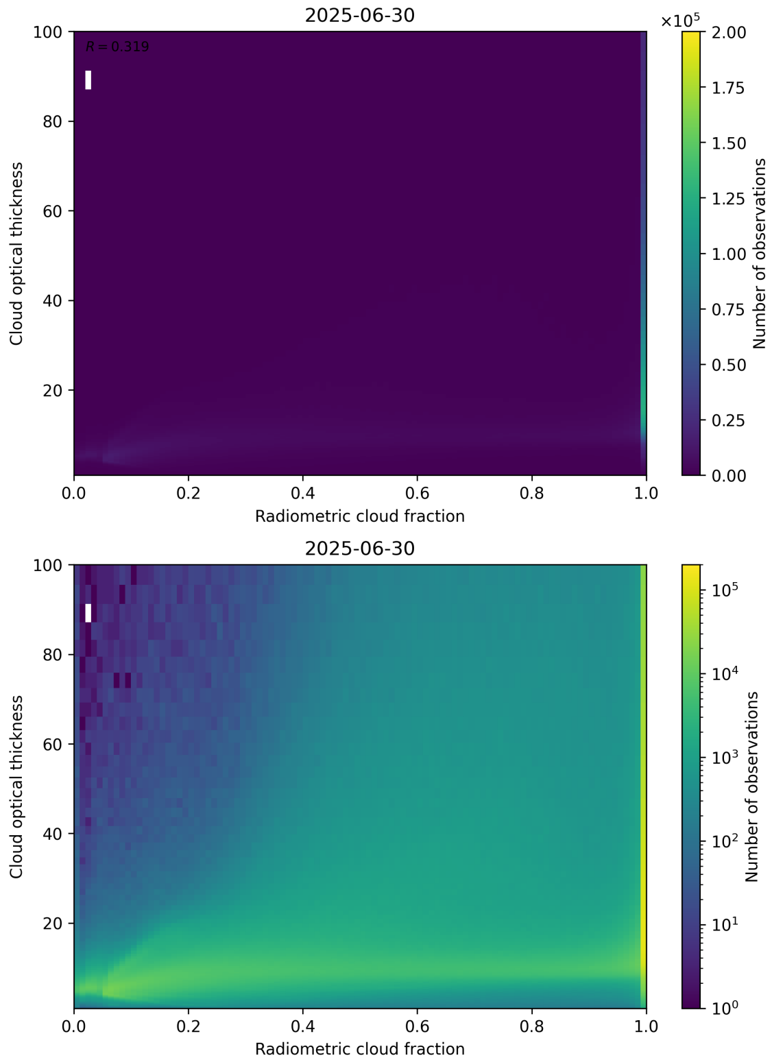
Figure 75: Scatter density plot of “Radiometric cloud fraction” against “Cloud optical thickness” for 2025-06-29 to 2025-07-01.
