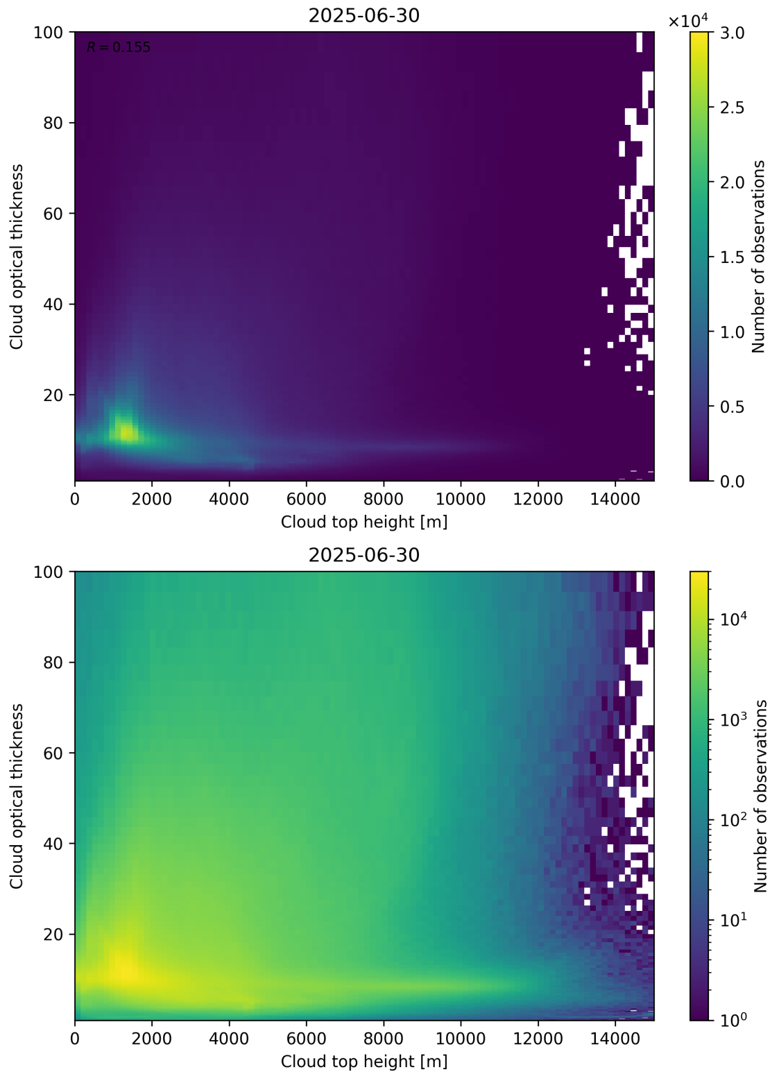
Figure 90: Scatter density plot of “Cloud top height” against “Cloud optical thickness” for 2025-06-29 to 2025-07-01.
