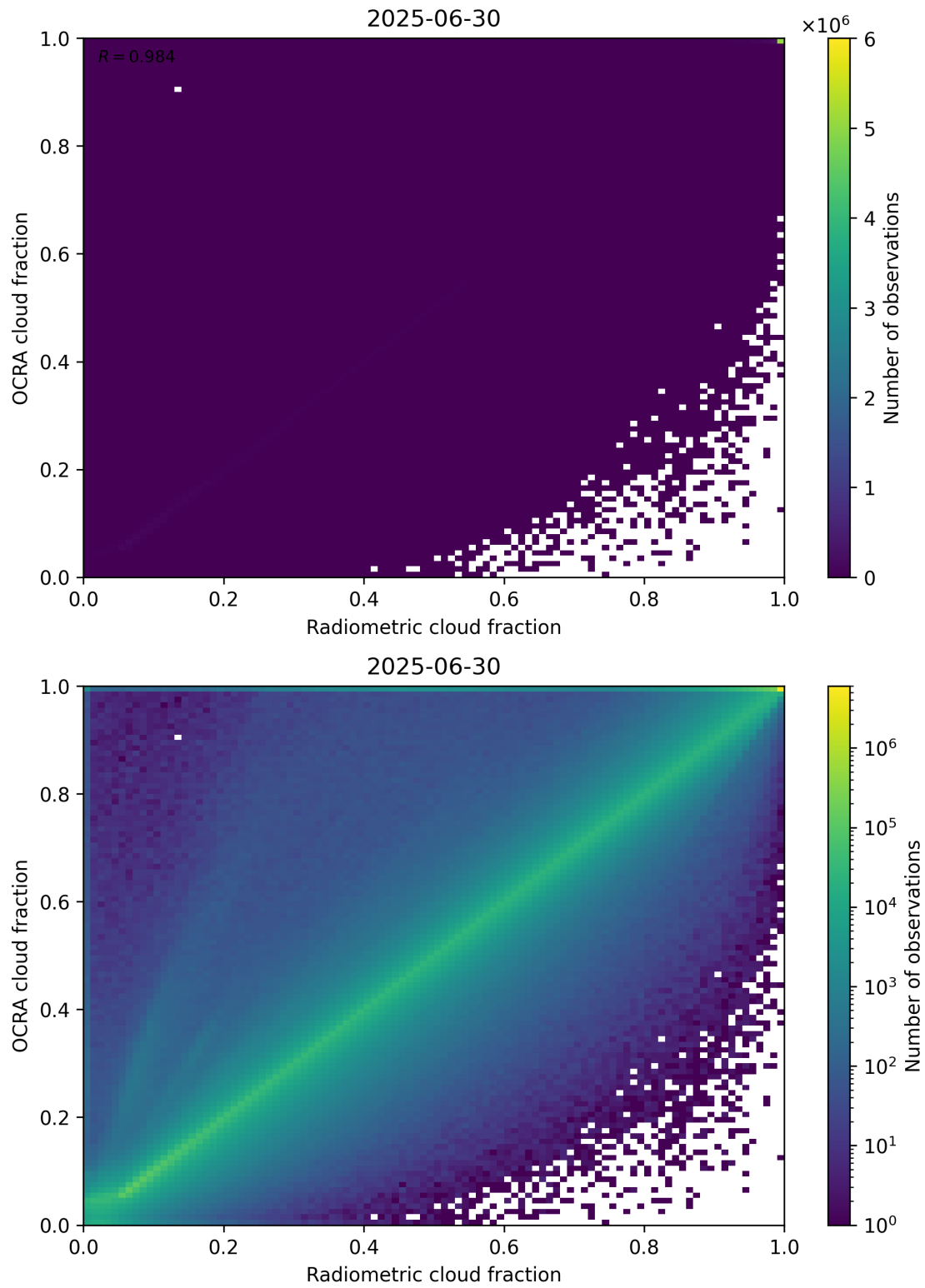
Figure 72: Scatter density plot of “Radiometric cloud fraction” against “OCRA cloud fraction” for 2025-06-29 to 2025-07-01.
