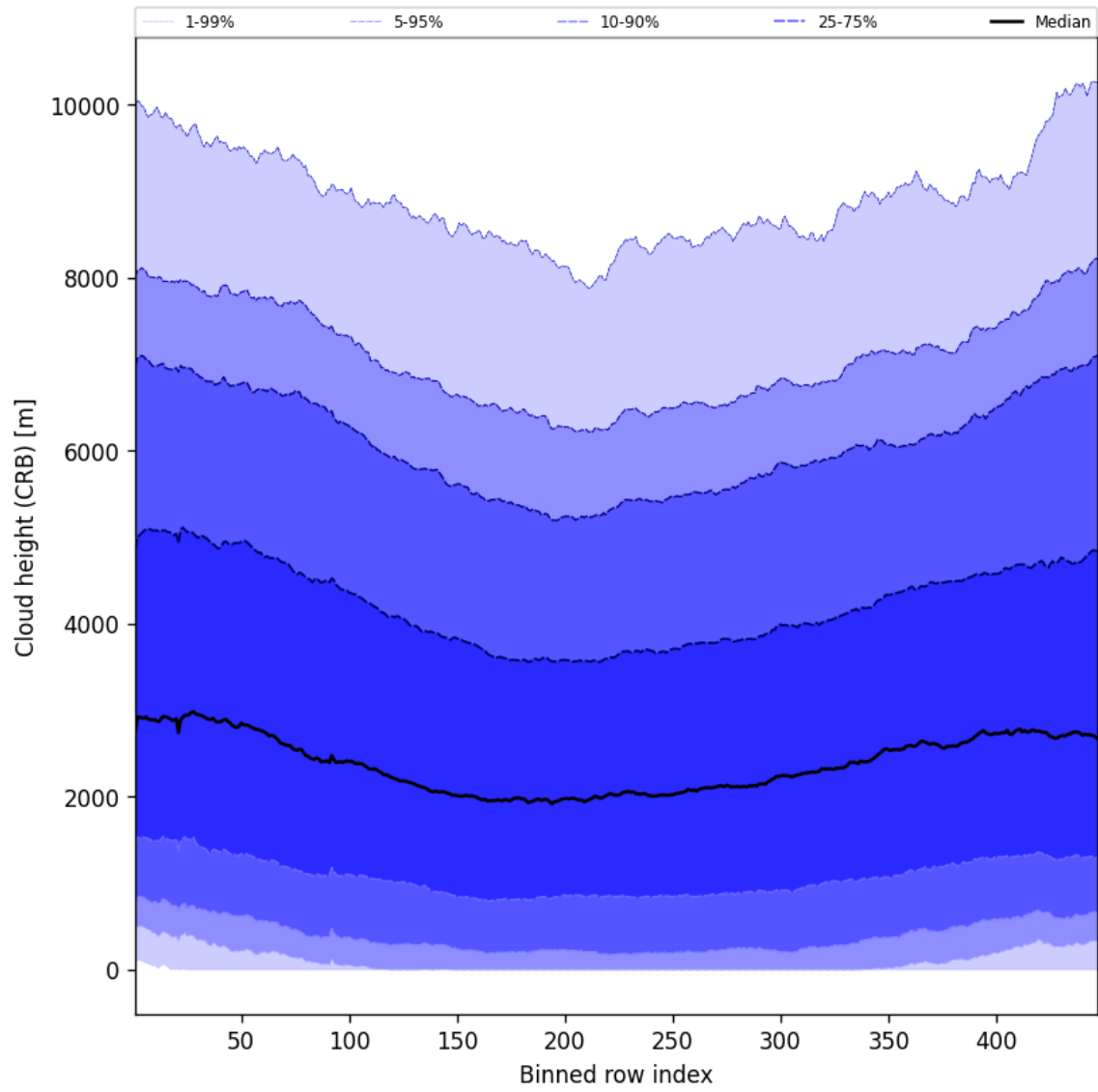
Figure 59: Along track statistics of “Cloud height (CRB)” for 2025-06-29 to 2025-07-01
