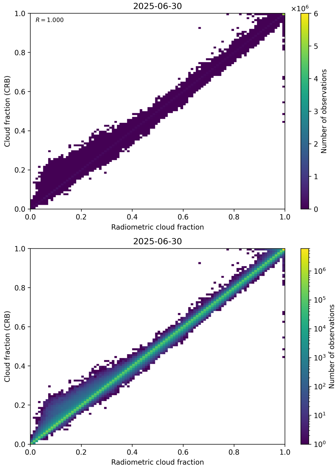
Figure 73: Scatter density plot of “Radiometric cloud fraction” against “Cloud fraction (CRB)” for 2025-06-29 to 2025-07-01.
