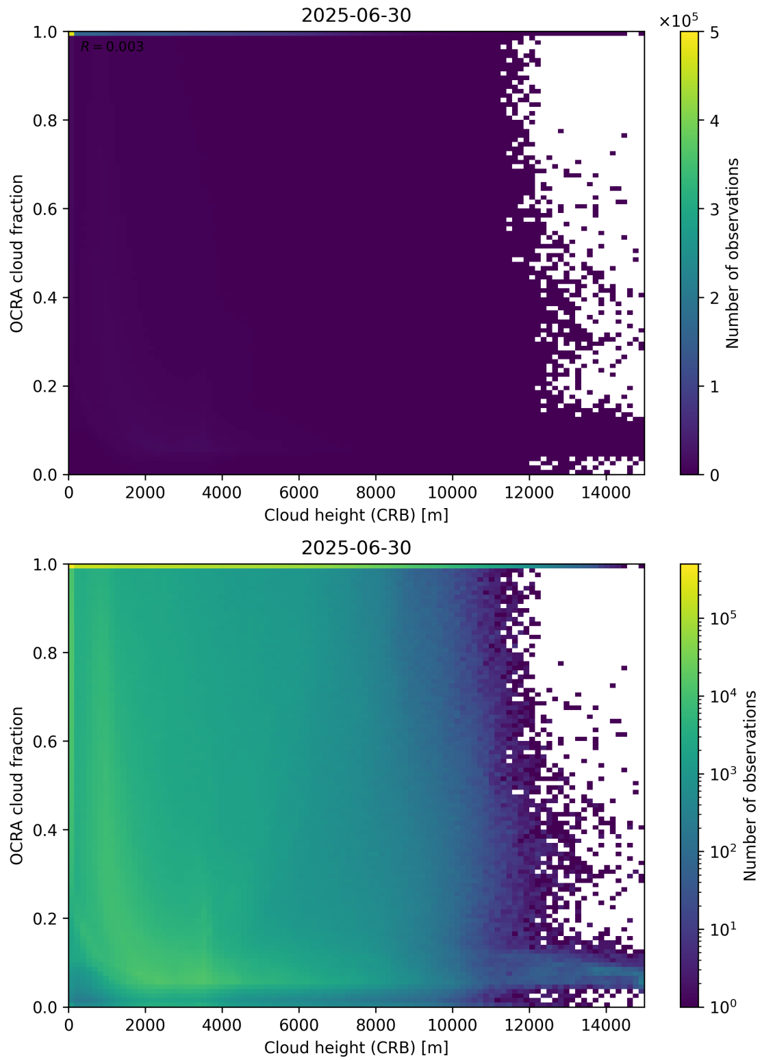
Figure 81: Scatter density plot of “Cloud height (CRB)” against “OCRA cloud fraction” for 2025-06-29 to 2025-07-01.
