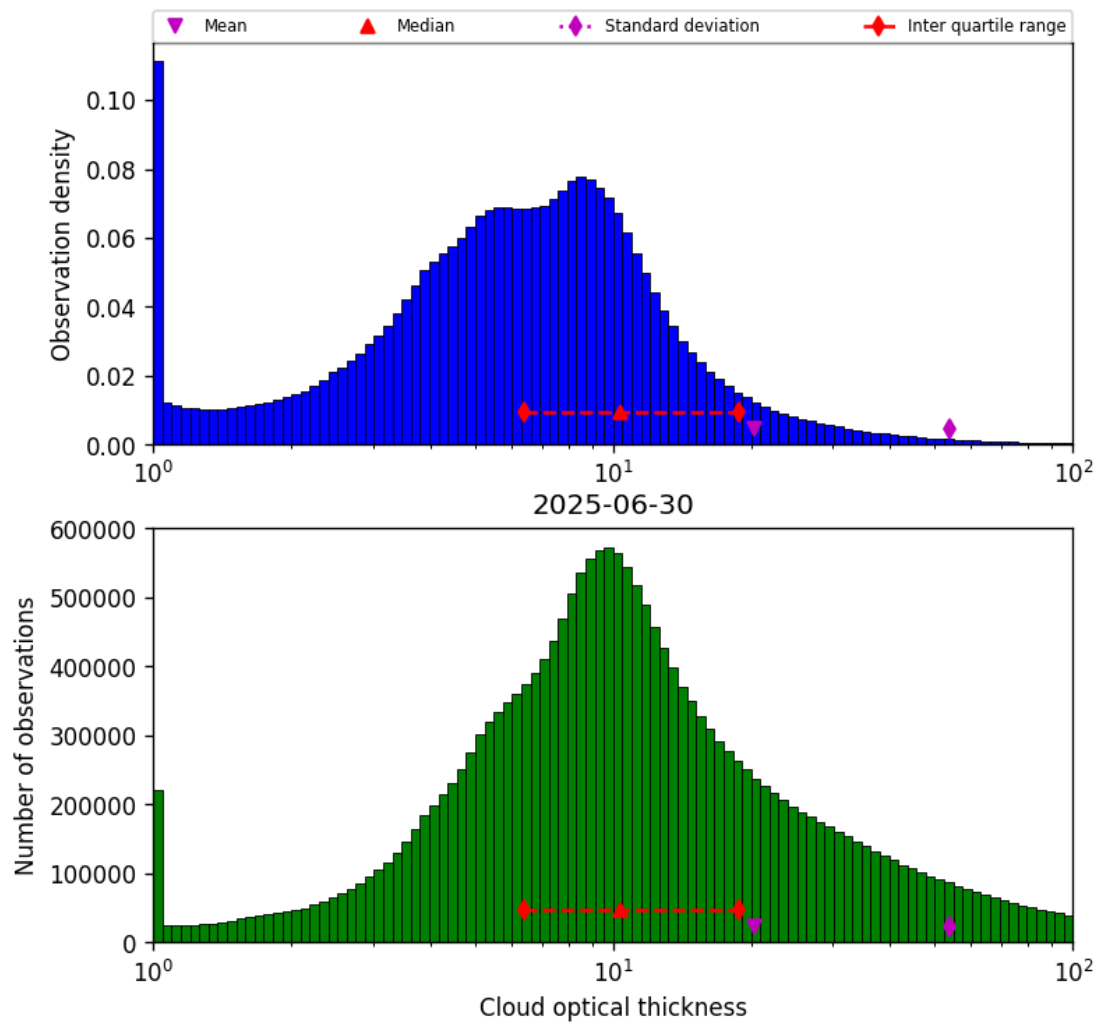
Figure 41: Histogram of “Cloud optical thickness” for 2025-06-29 to 2025-07-01
