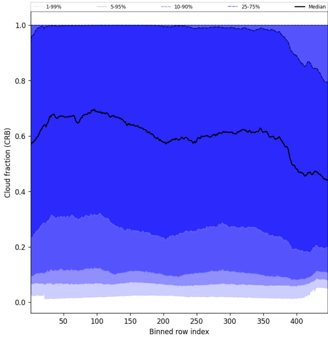
Figure 58: Along track statistics of “Cloud fraction (CRB)” for 2025-06-29 to 2025-07-01
