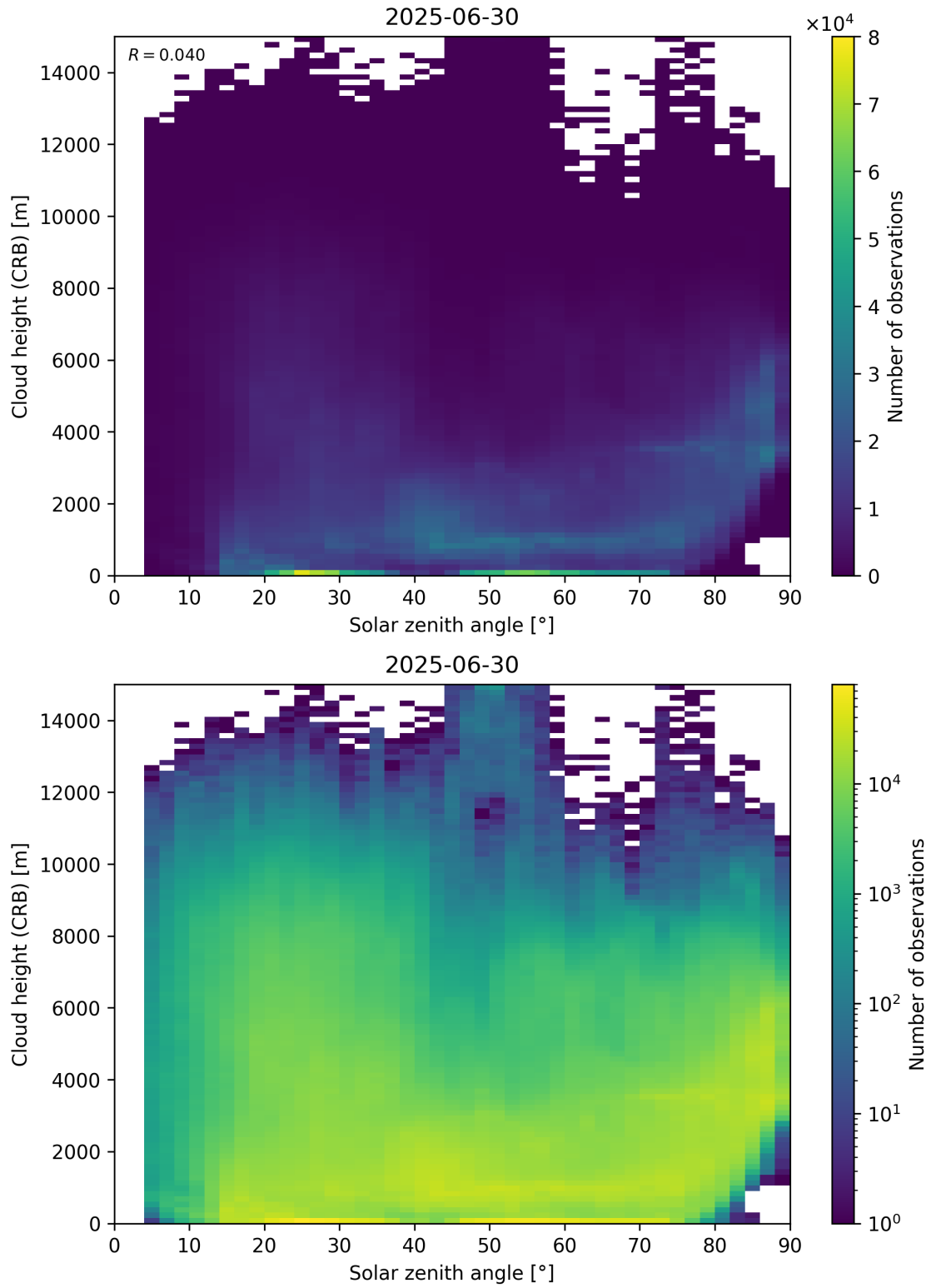
Figure 102: Scatter density plot of “Solar zenith angle” against “Cloud height (CRB)” for 2025-06-29 to 2025-07-01.
