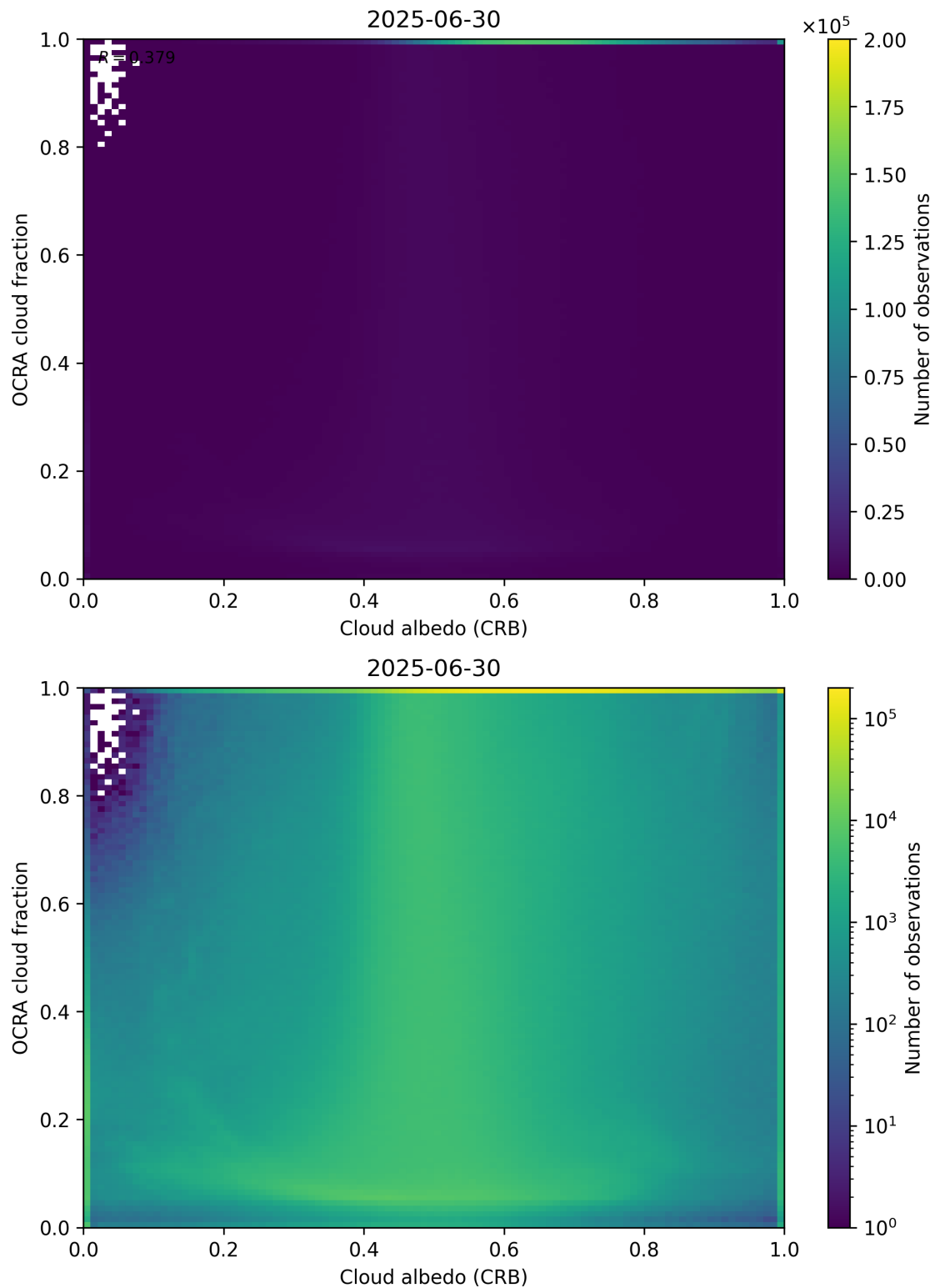
Figure 70: Scatter density plot of “Cloud albedo (CRB)” against “OCRA cloud fraction” for 2025-06-29 to 2025-07-01.
