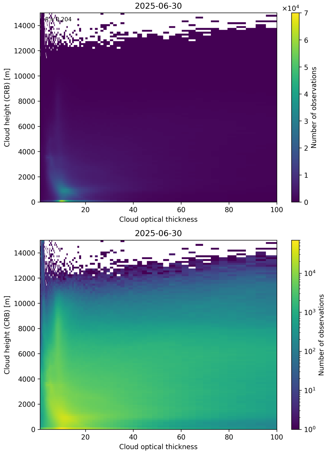
Figure 85: Scatter density plot of “Cloud optical thickness” against “Cloud height (CRB)” for 2025-06-29 to 2025-07-01.
