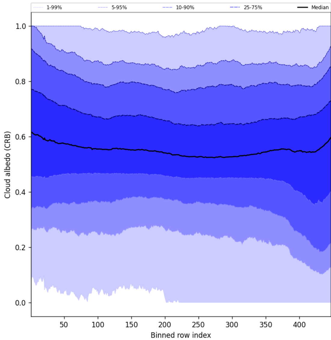
Figure 60: Along track statistics of “Cloud albedo (CRB)” for 2025-06-29 to 2025-07-01
