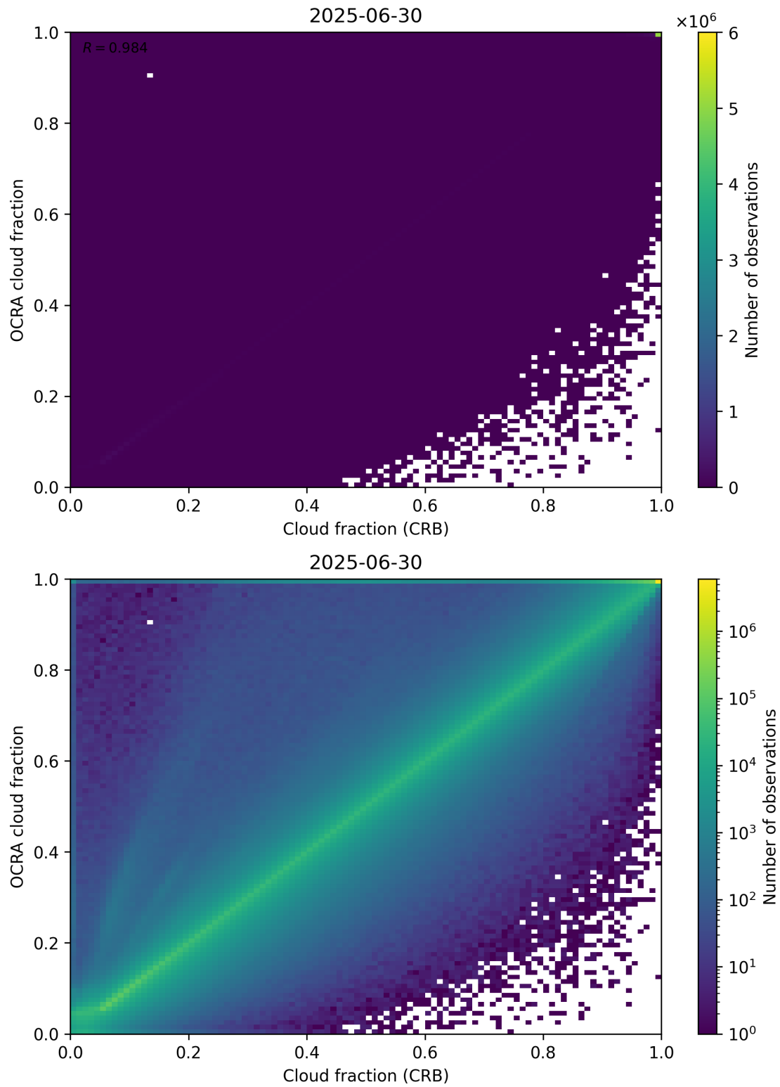
Figure 78: Scatter density plot of “Cloud fraction (CRB)” against “OCRA cloud fraction” for 2025-06-29 to 2025-07-01.
