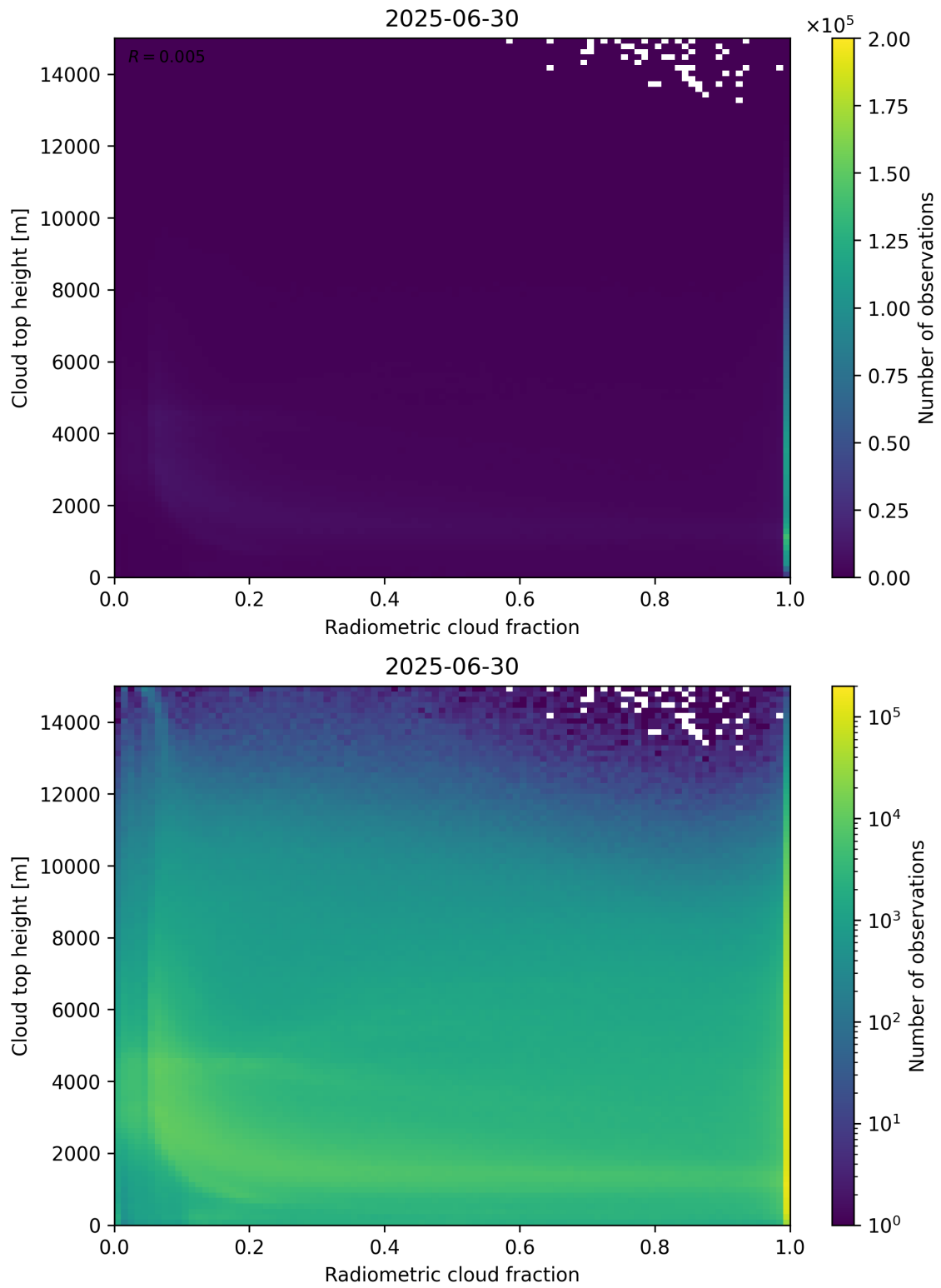
Figure 76: Scatter density plot of “Radiometric cloud fraction” against “Cloud top height” for 2025-06-29 to 2025-07-01.
