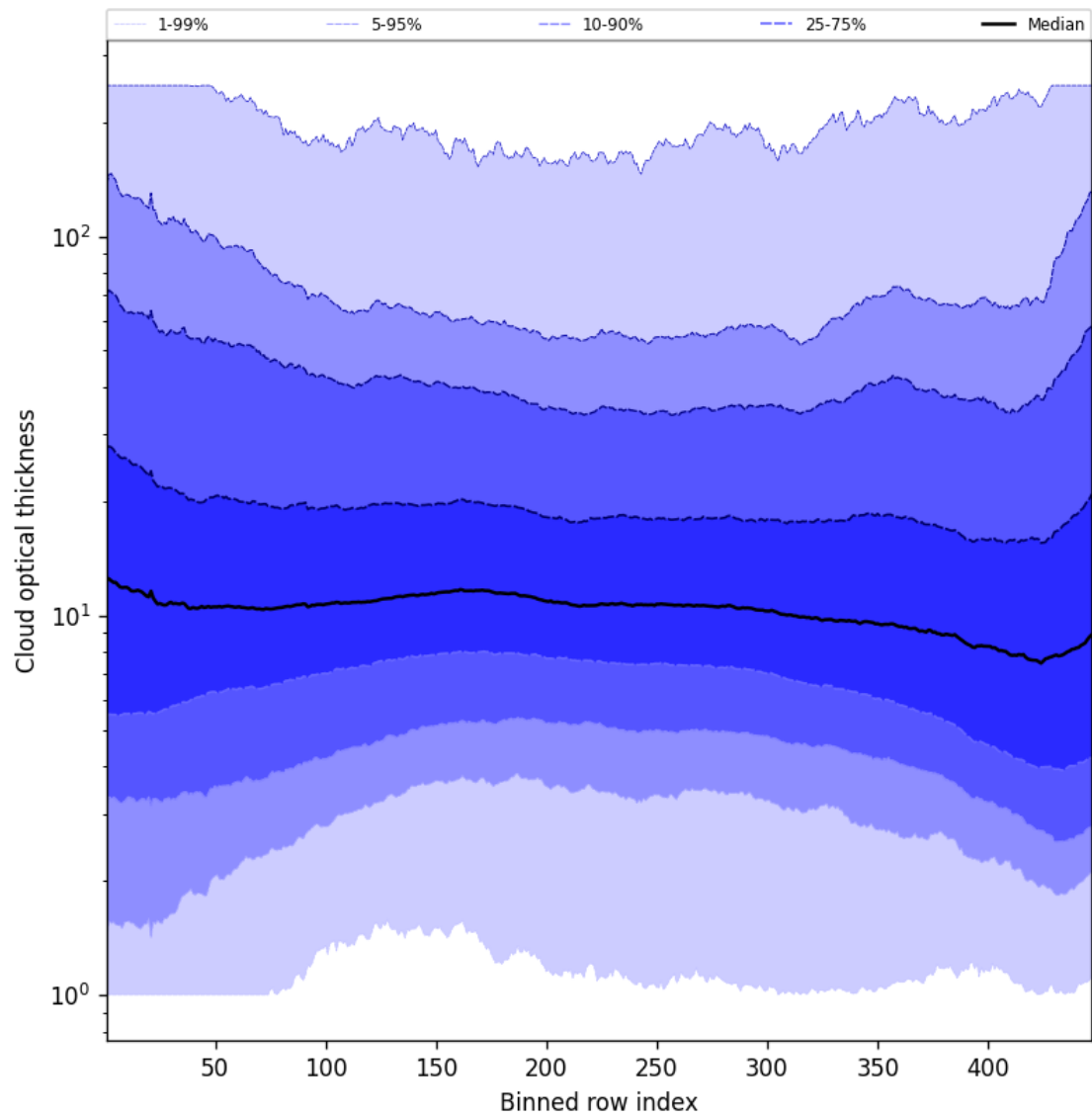
Figure 57: Along track statistics of “Cloud optical thickness” for 2025-06-29 to 2025-07-01
