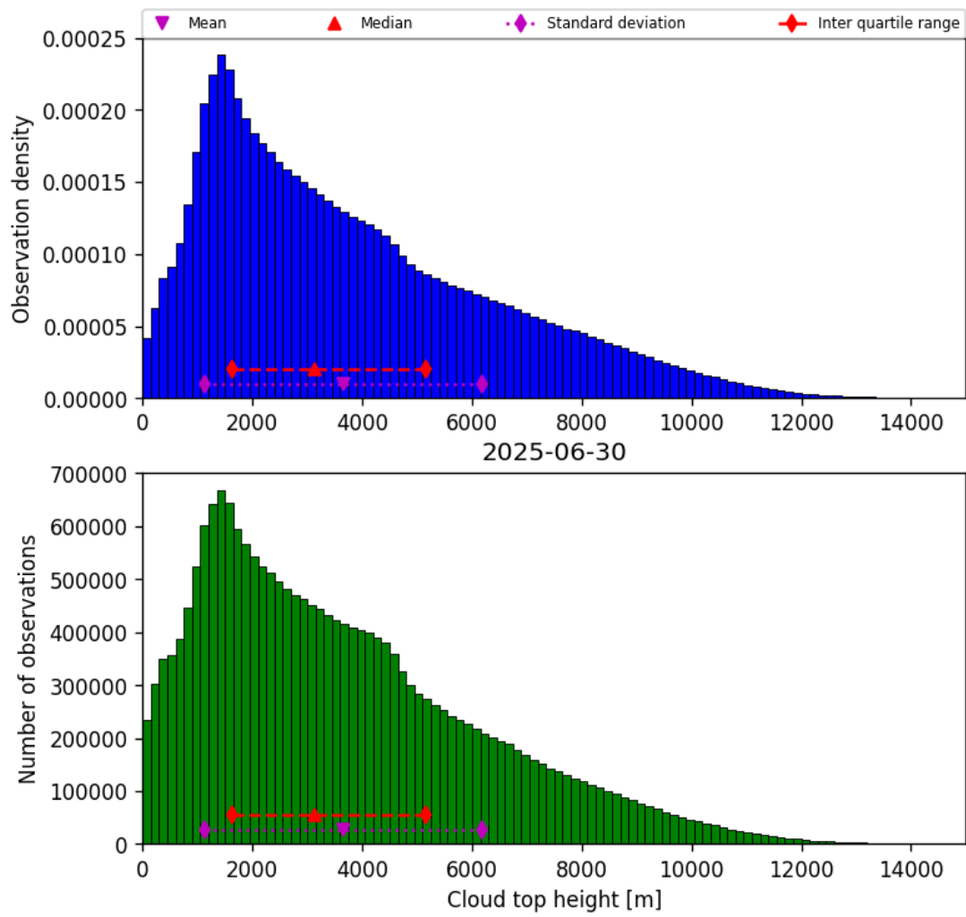
Figure 40: Histogram of “Cloud top height” for 2025-06-29 to 2025-07-01
