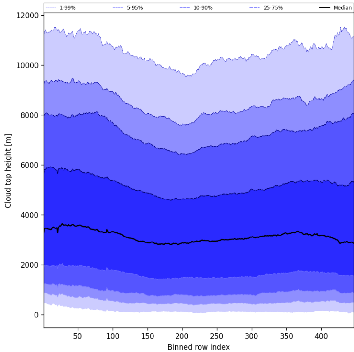
Figure 56: Along track statistics of “Cloud top height” for 2025-06-29 to 2025-07-01
