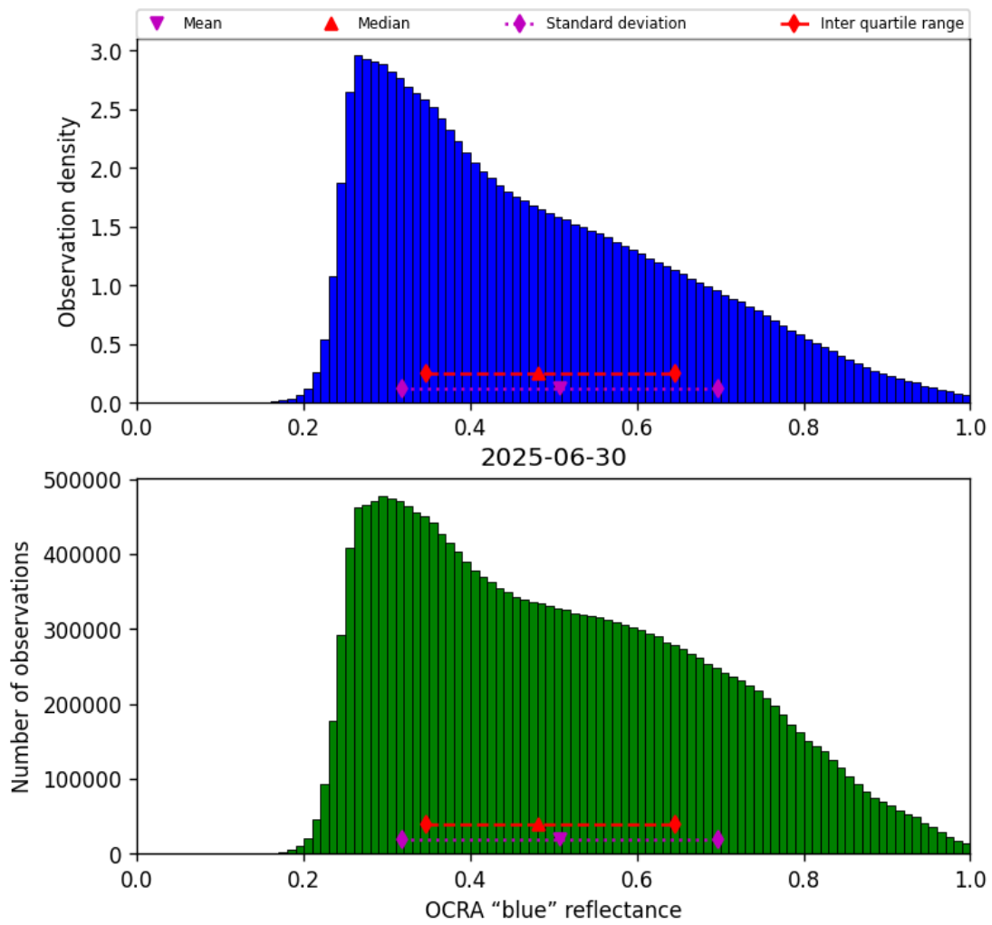
Figure 51: Histogram of “OCRA “blue” reflectance” for 2025-06-29 to 2025-07-01
