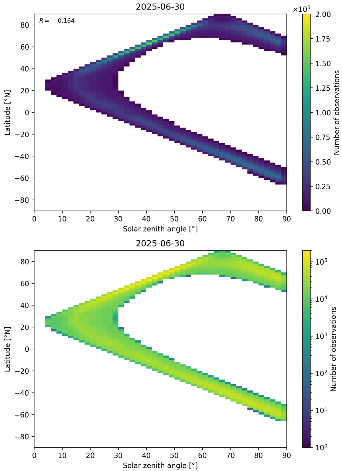
Figure 105: Scatter density plot of “Solar zenith angle” against “Latitude” for 2025-06-29 to 2025-07-01.
