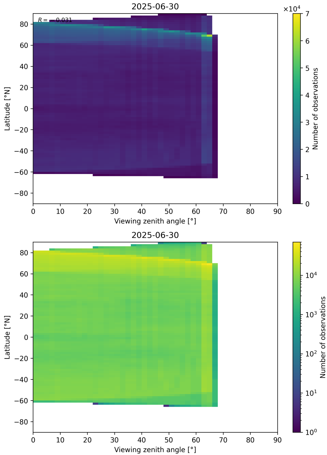
Figure 113: Scatter density plot of “Viewing zenith angle” against “Latitude” for 2025-06-29 to 2025-07-01.
