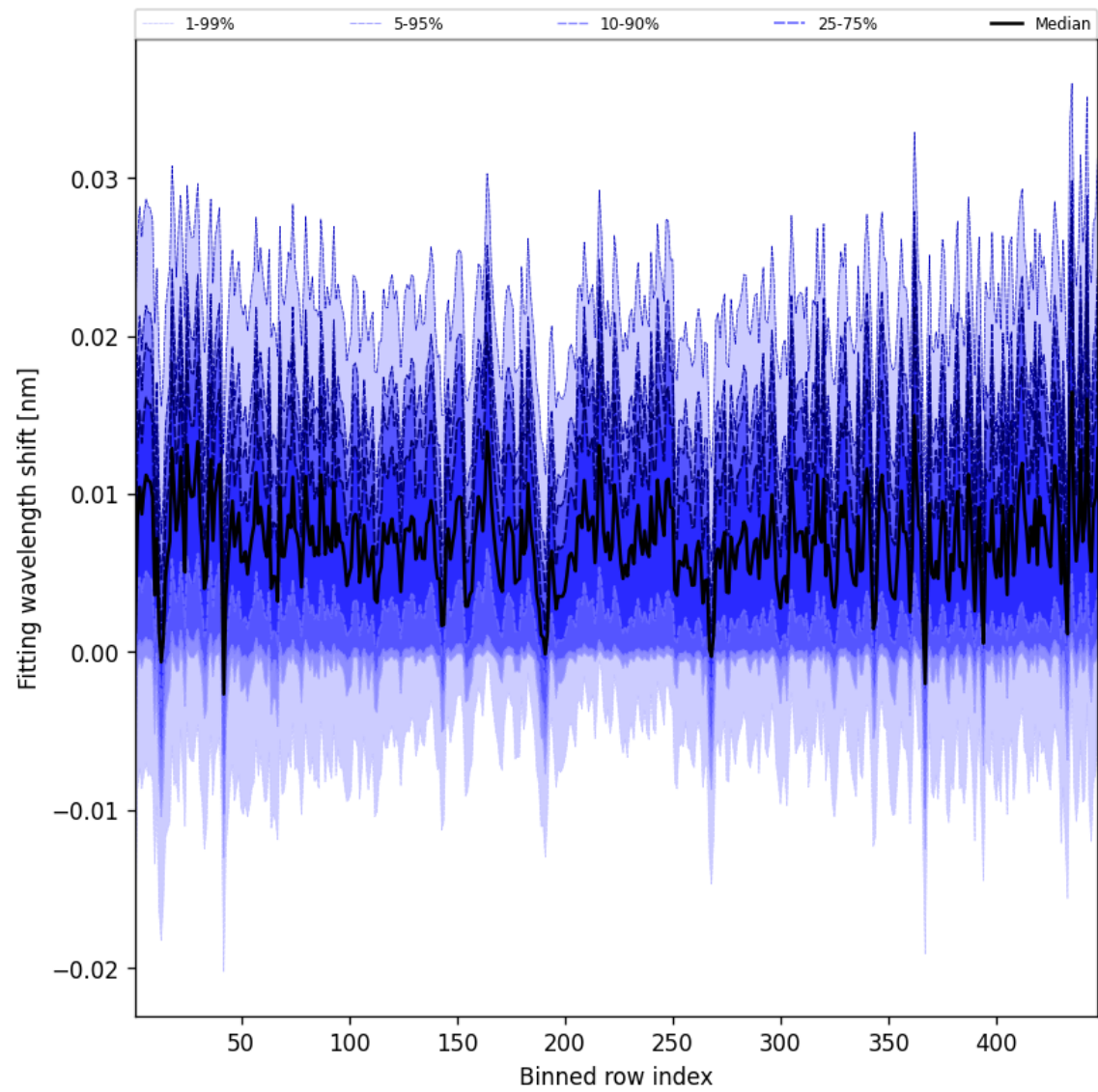
Figure 65: Along track statistics of “Fitting wavelength shift” for 2025-06-29 to 2025-07-01
