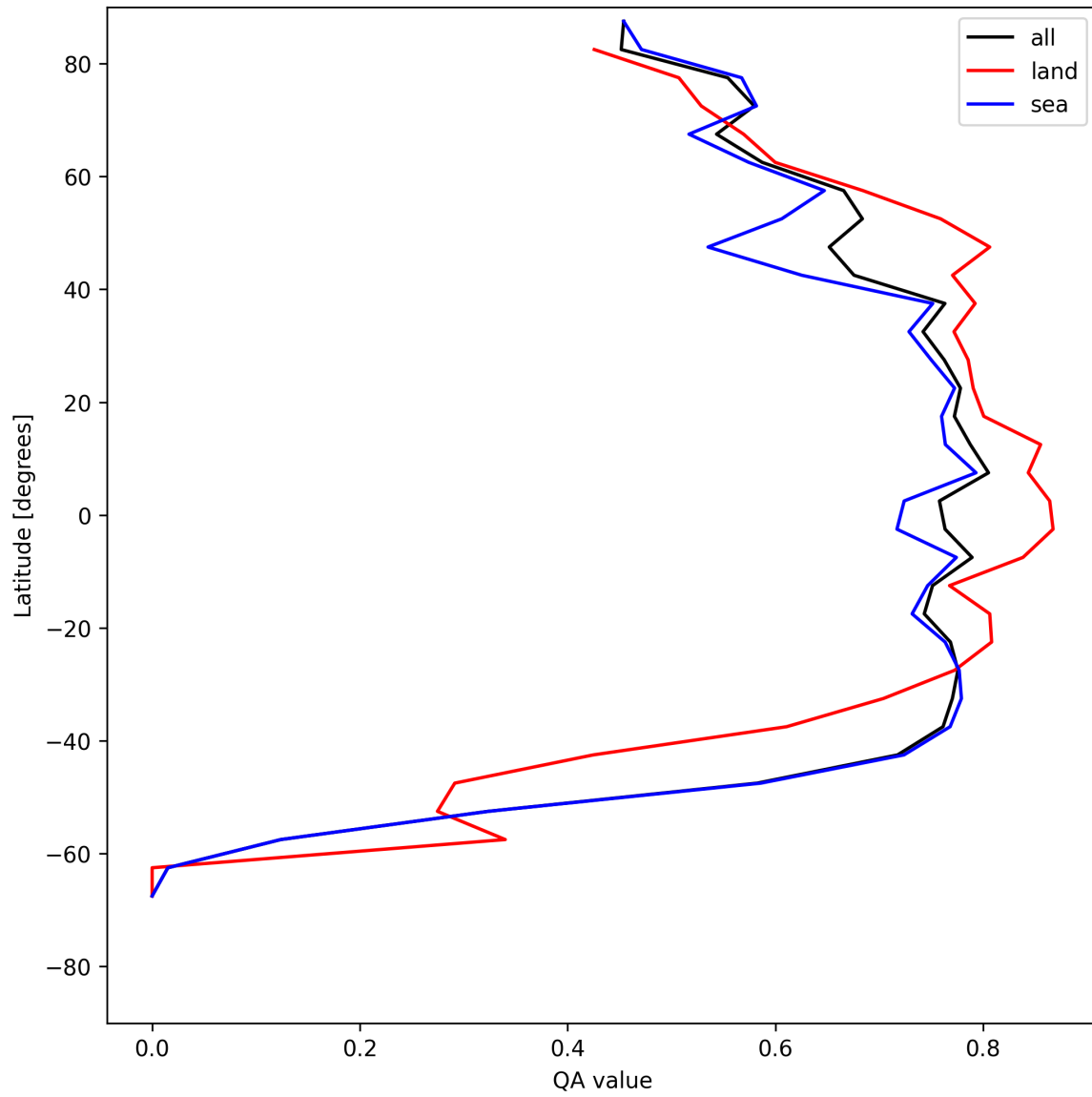
Figure 22: Zonal average of “QA value” for 2025-06-29 to 2025-07-01.
