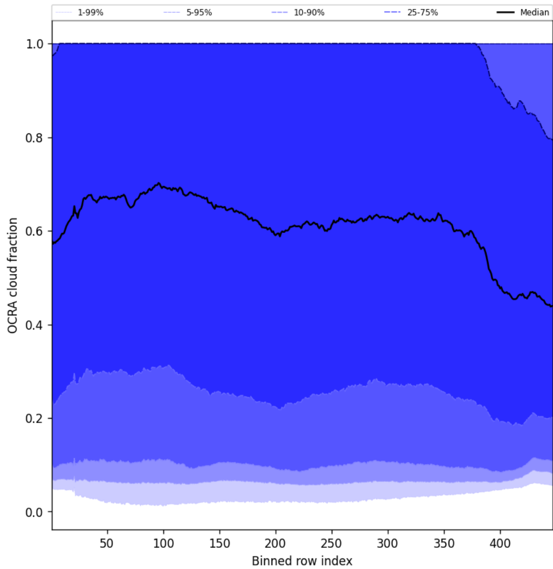
Figure 66: Along track statistics of “OCRA cloud fraction” for 2025-06-29 to 2025-07-01
