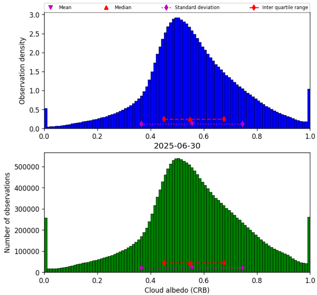
Figure 44: Histogram of “Cloud albedo (CRB)” for 2025-06-29 to 2025-07-01
