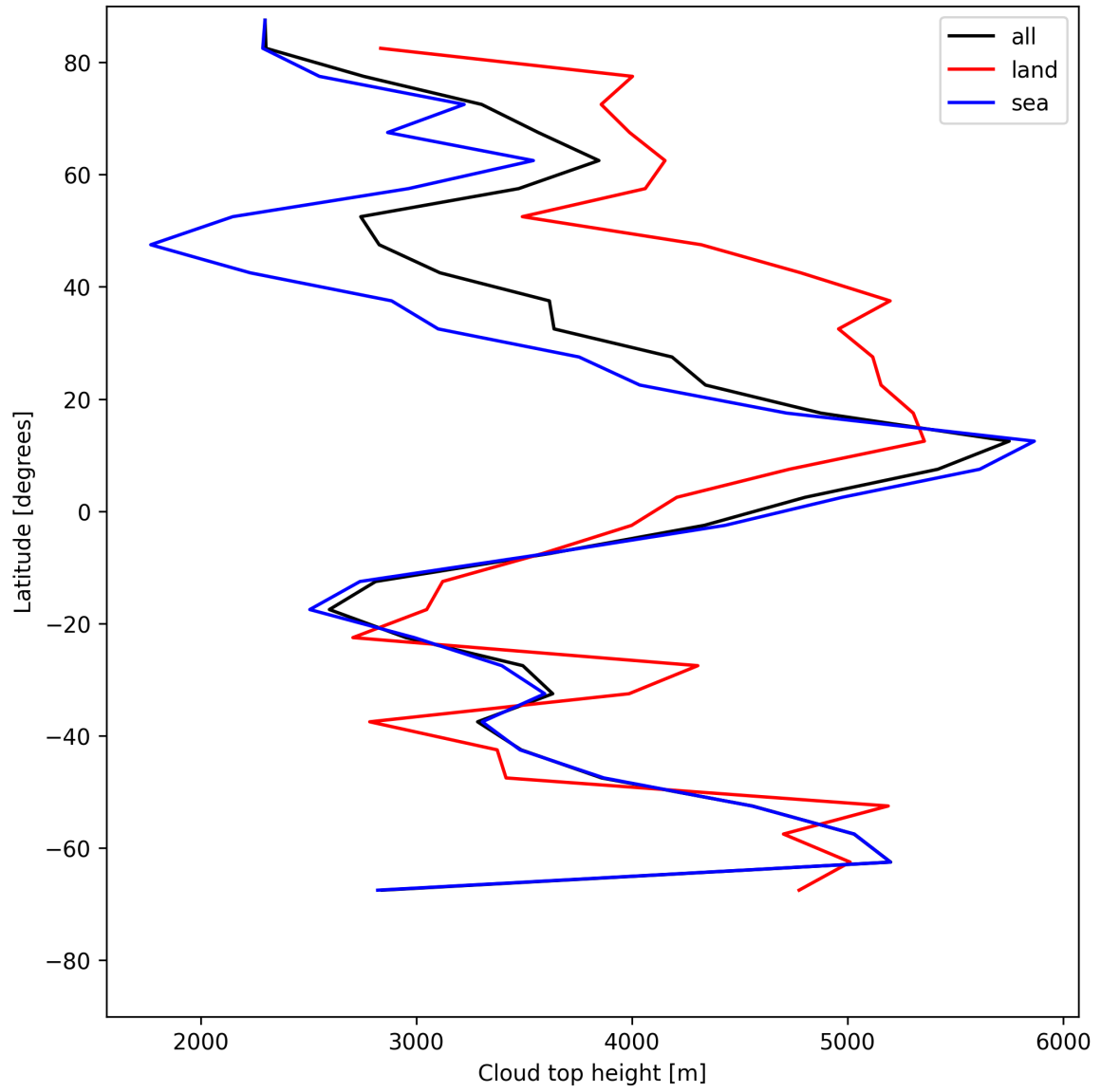
Figure 24: Zonal average of “Cloud top height” for 2025-06-29 to 2025-07-01.
