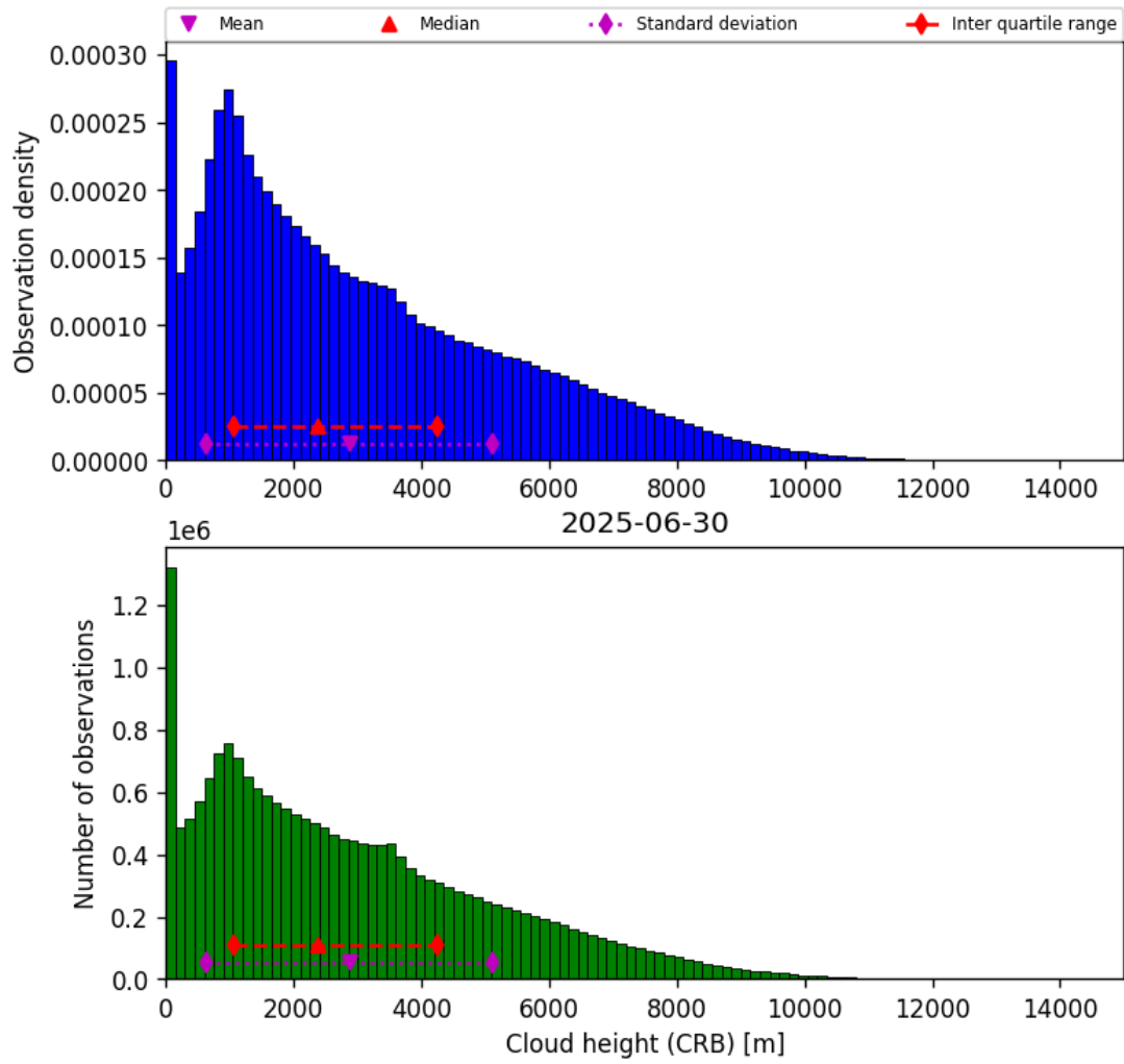
Figure 43: Histogram of “Cloud height (CRB)” for 2025-06-29 to 2025-07-01
