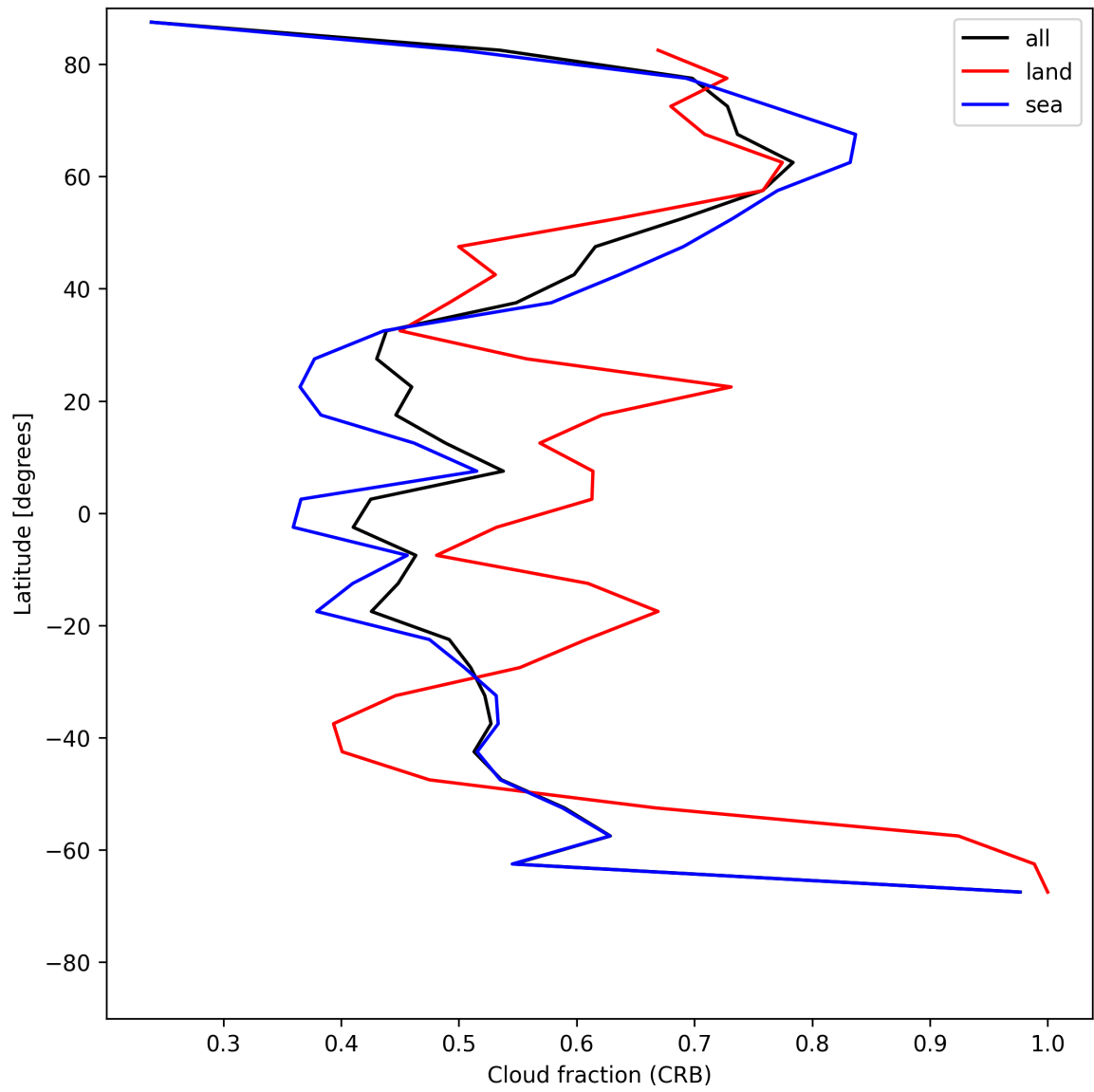
Figure 26: Zonal average of “Cloud fraction (CRB)” for 2025-06-29 to 2025-07-01.
