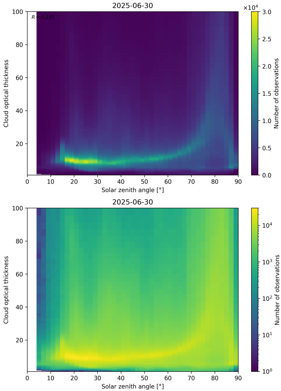
Figure 103: Scatter density plot of “Solar zenith angle” against “Cloud optical thickness” for 2025-06-29 to 2025-07-01.
