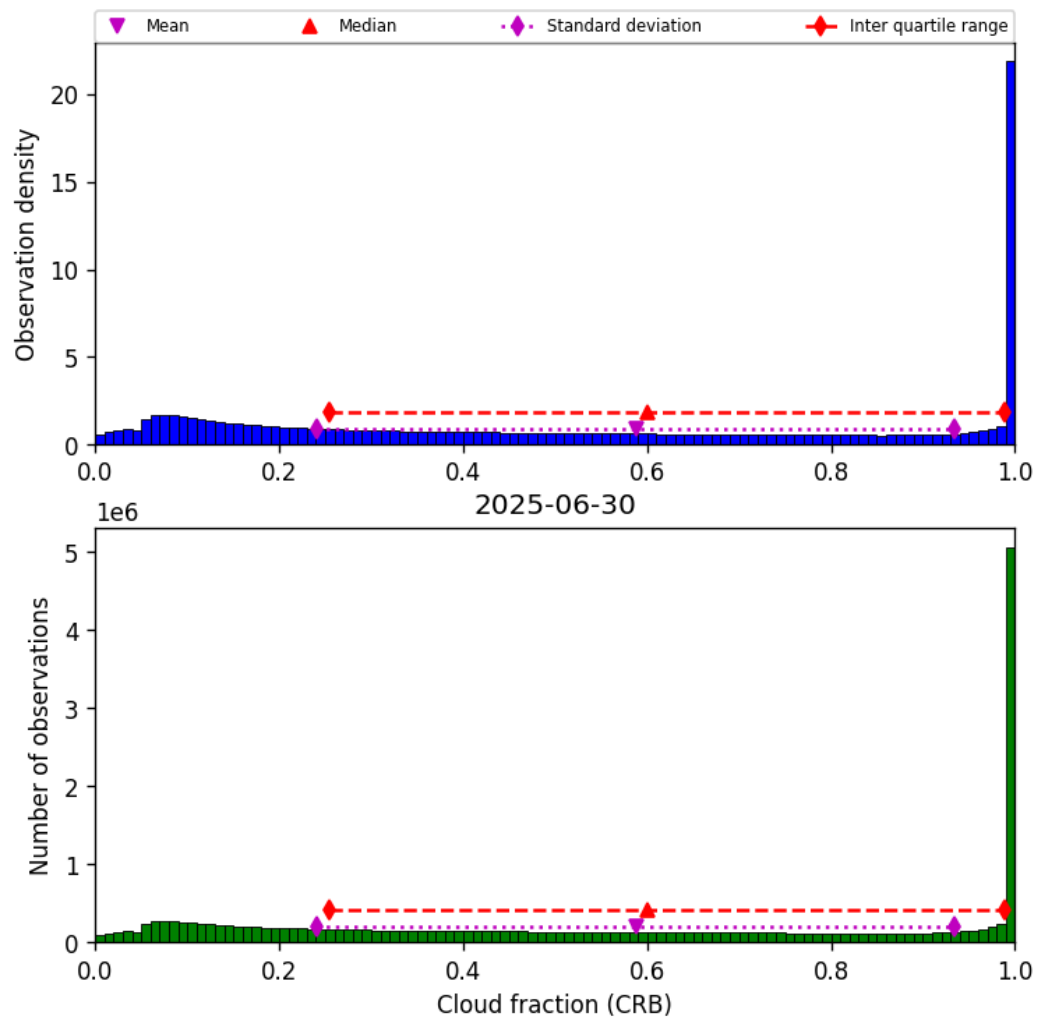
Figure 42: Histogram of “Cloud fraction (CRB)” for 2025-06-29 to 2025-07-01
