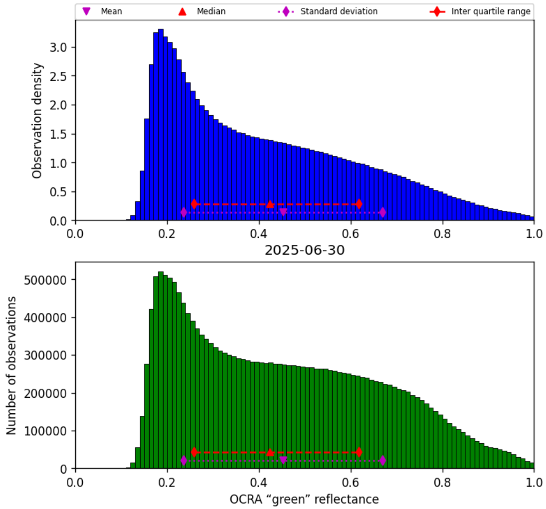
Figure 52: Histogram of “OCRA “green” reflectance” for 2025-06-29 to 2025-07-01
