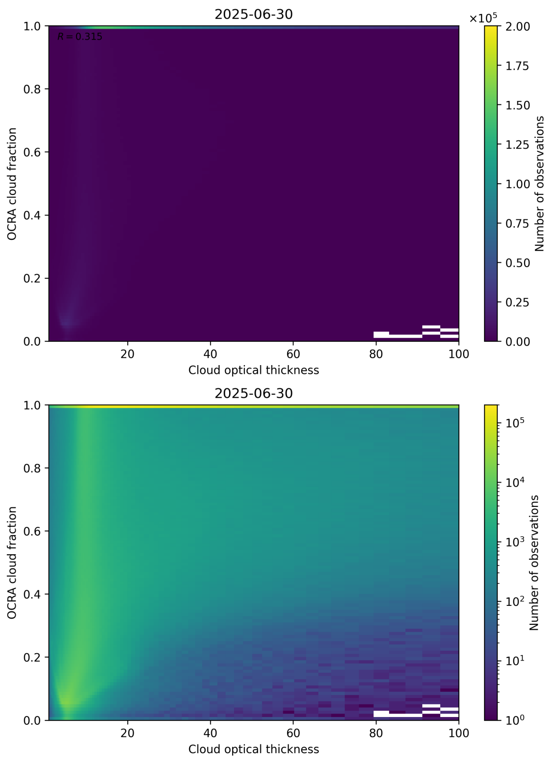
Figure 83: Scatter density plot of “Cloud optical thickness” against “OCRA cloud fraction” for 2025-06-29 to 2025-07-01.
