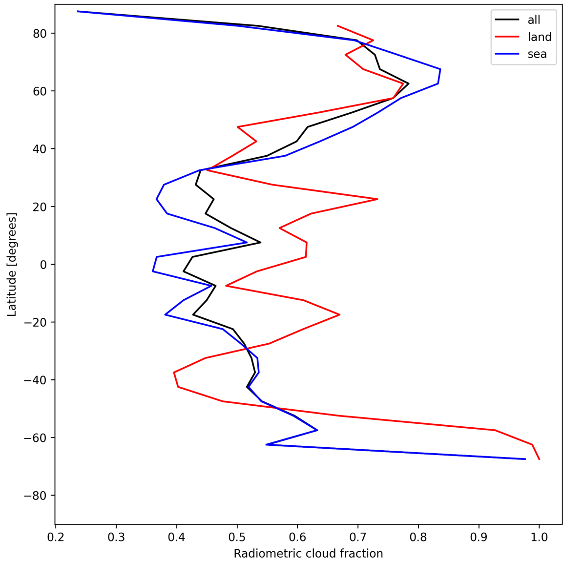
Figure 23: Zonal average of “Radiometric cloud fraction” for 2025-06-29 to 2025-07-01.
