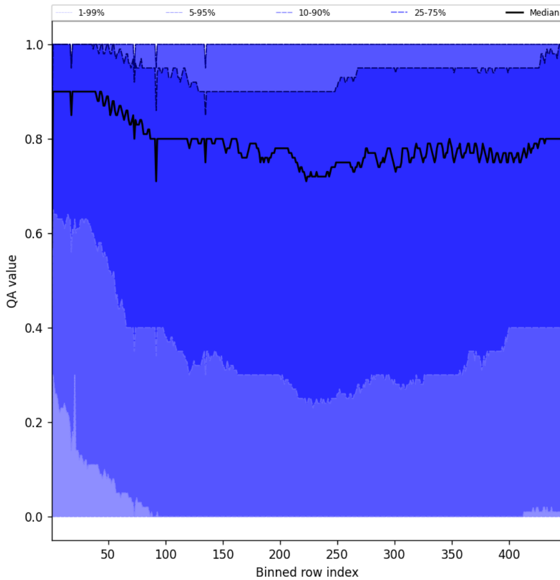
Figure 54: Along track statistics of “QA value” for 2025-06-29 to 2025-07-01
