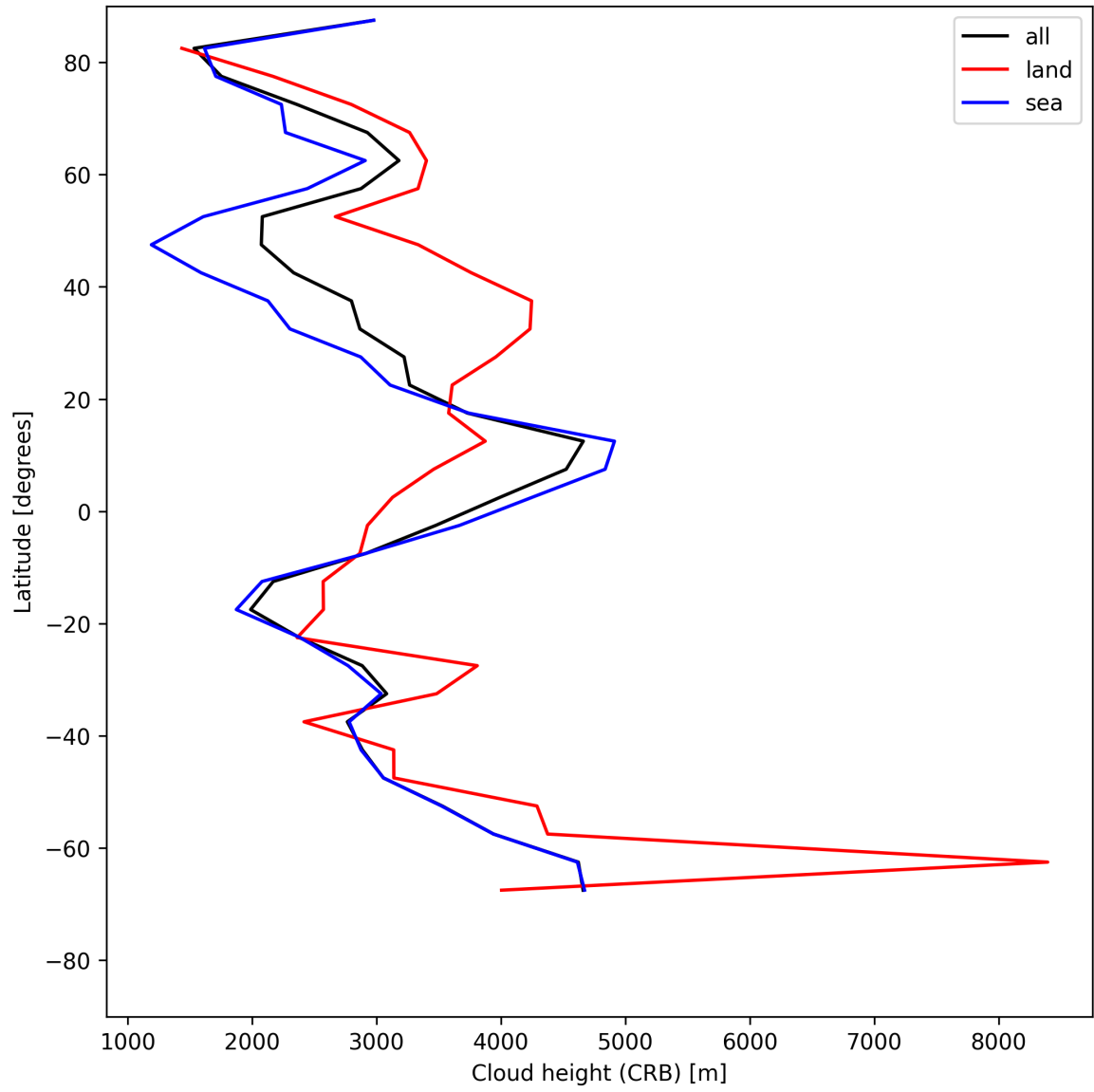
Figure 27: Zonal average of “Cloud height (CRB)” for 2025-06-29 to 2025-07-01.
