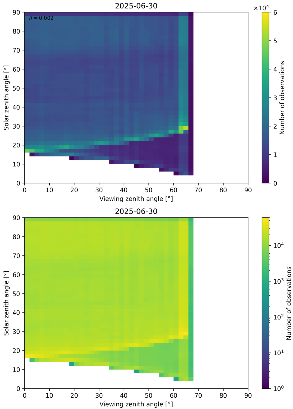
Figure 114: Scatter density plot of “Viewing zenith angle” against “Solar zenith angle” for 2025-06-29 to 2025-07-01.
