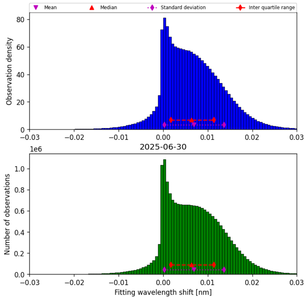
Figure 49: Histogram of “Fitting wavelength shift” for 2025-06-29 to 2025-07-01
