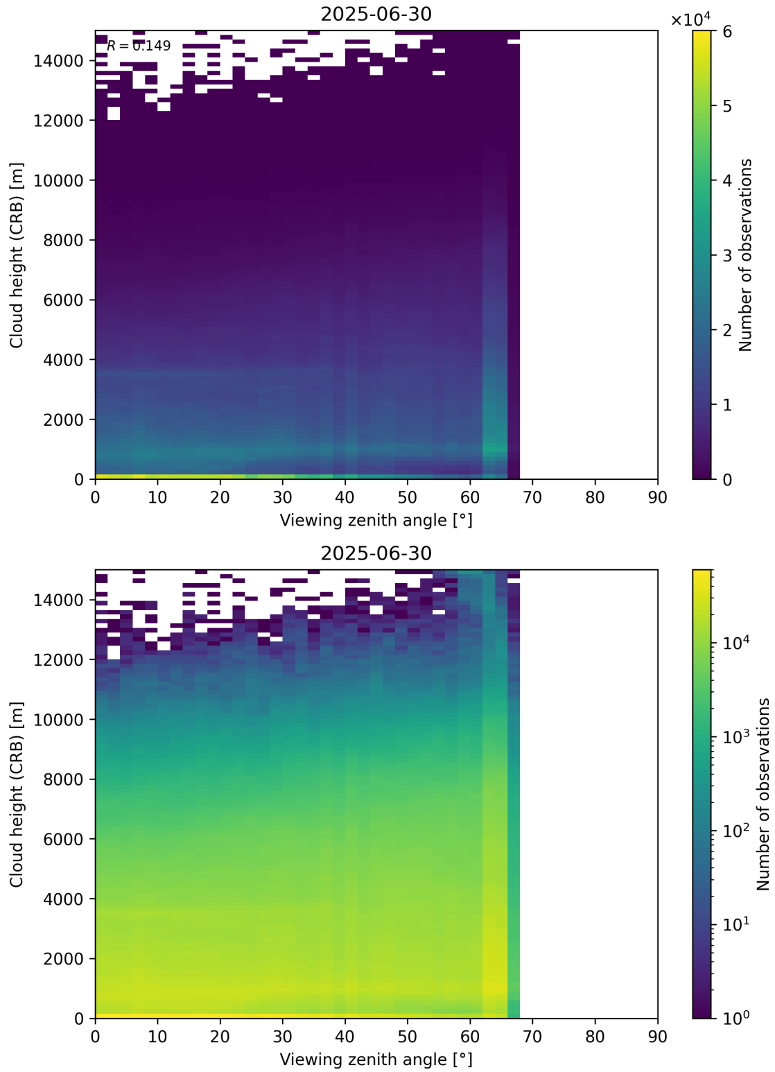
Figure 110: Scatter density plot of “Viewing zenith angle” against “Cloud height (CRB)” for 2025-06-29 to 2025-07-01.
