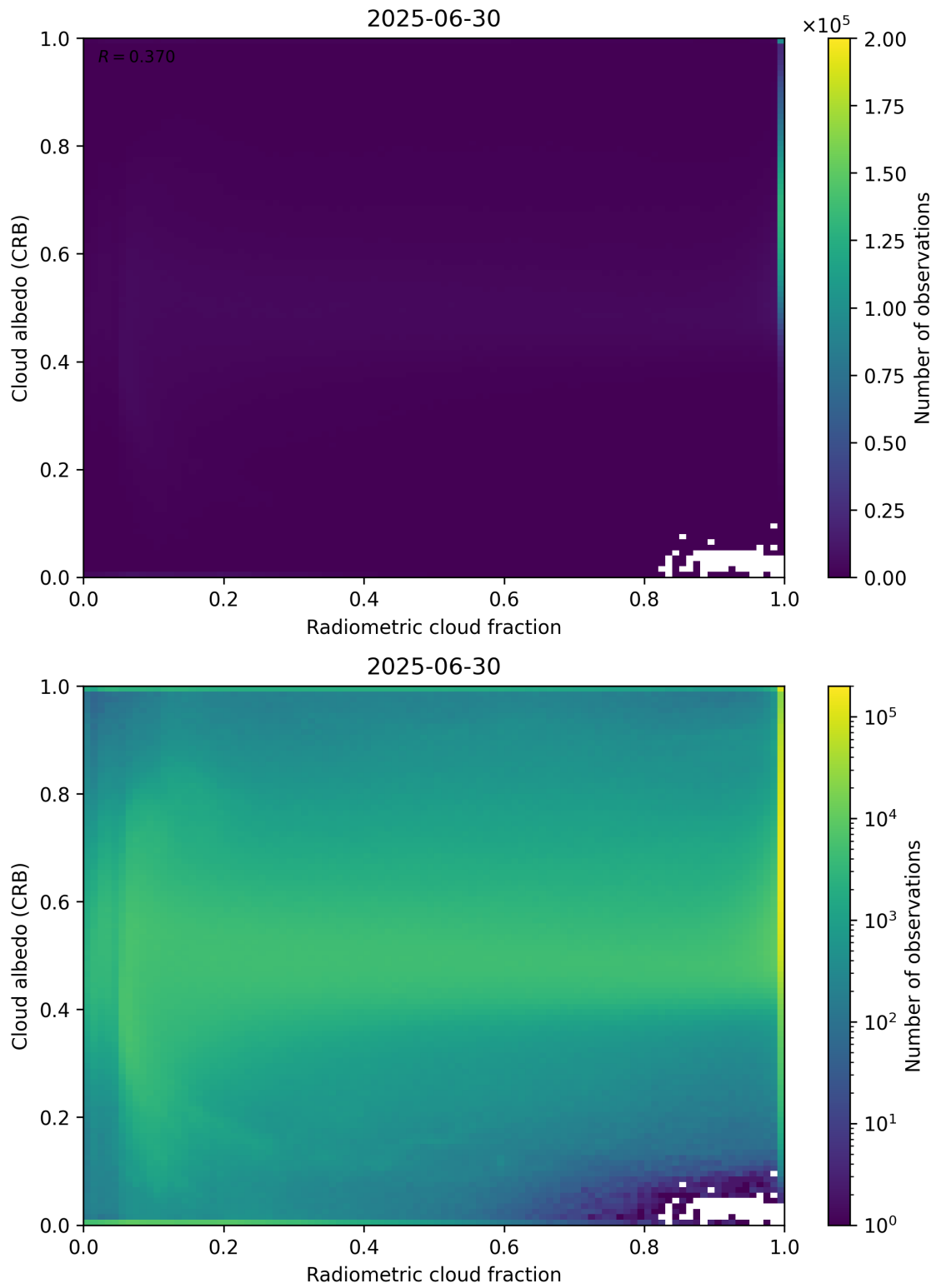
Figure 71: Scatter density plot of “Radiometric cloud fraction” against “Cloud albedo (CRB)” for 2025-06-29 to 2025-07-01.
