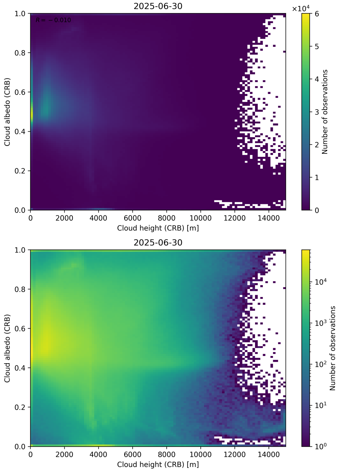
Figure 80: Scatter density plot of “Cloud height (CRB)” against “Cloud albedo (CRB)” for 2025-06-29 to 2025-07-01.
