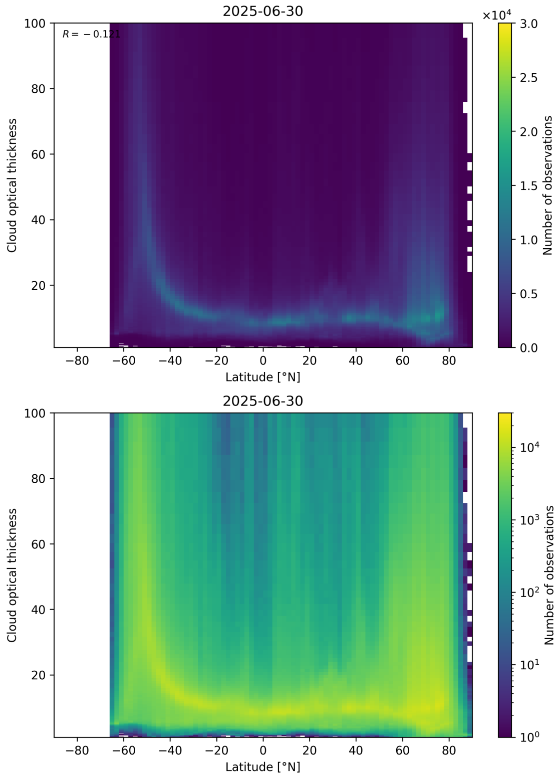
Figure 96: Scatter density plot of “Latitude” against “Cloud optical thickness” for 2025-06-29 to 2025-07-01.
