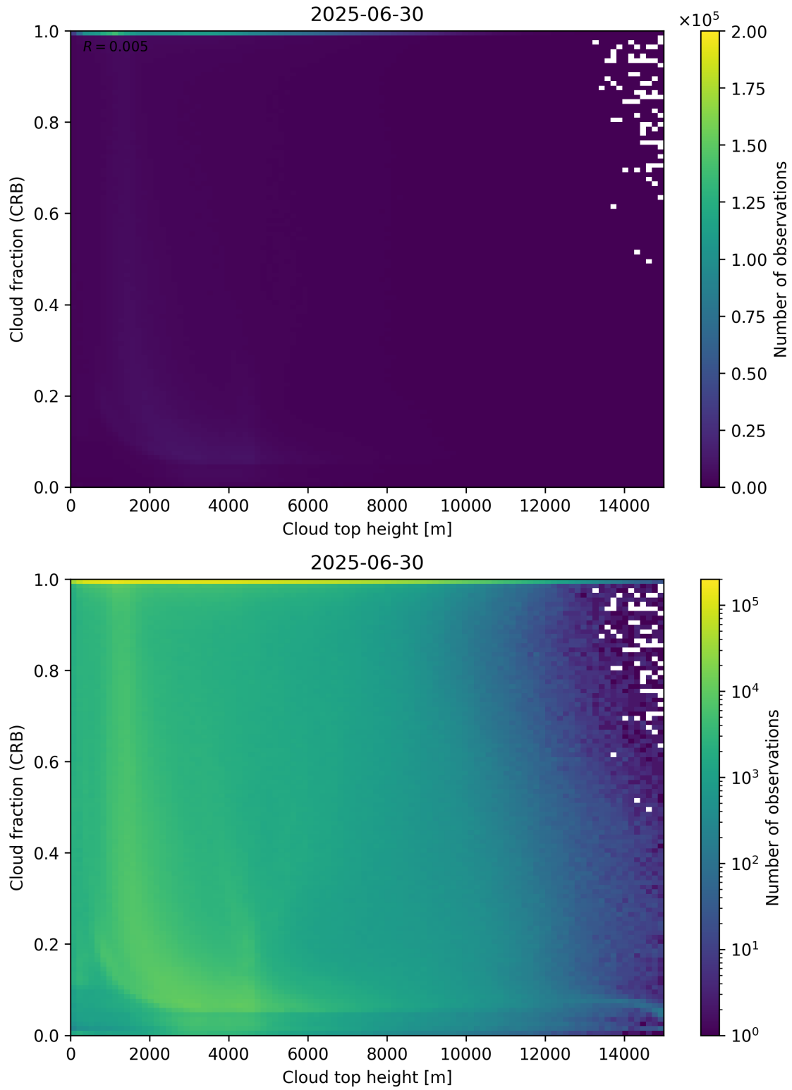
Figure 88: Scatter density plot of “Cloud top height” against “Cloud fraction (CRB)” for 2025-06-29 to 2025-07-01.
