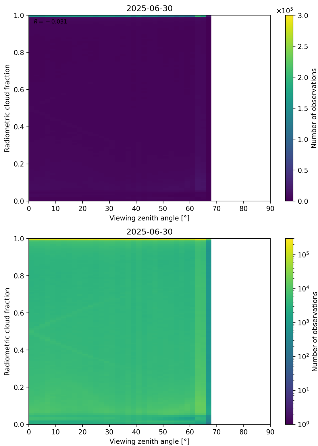
Figure 107: Scatter density plot of “Viewing zenith angle” against “Radiometric cloud fraction” for 2025-06-29 to 2025-07-01.
