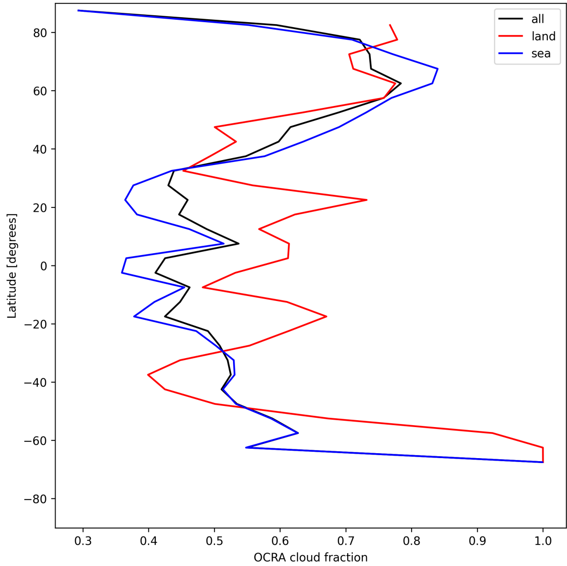
Figure 34: Zonal average of “OCRA cloud fraction” for 2025-06-29 to 2025-07-01.
