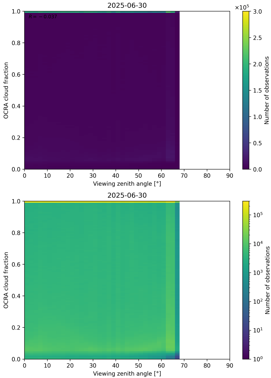
Figure 108: Scatter density plot of “Viewing zenith angle” against “OCRA cloud fraction” for 2025-06-29 to 2025-07-01.
