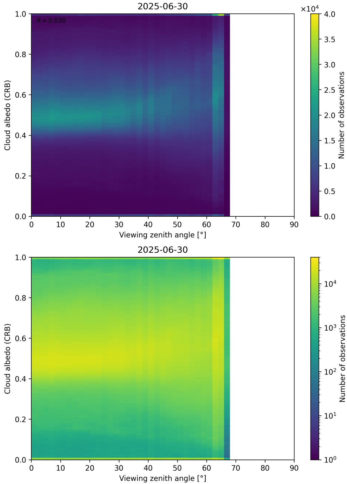
Figure 106: Scatter density plot of “Viewing zenith angle” against “Cloud albedo (CRB)” for 2025-06-29 to 2025-07-01.
