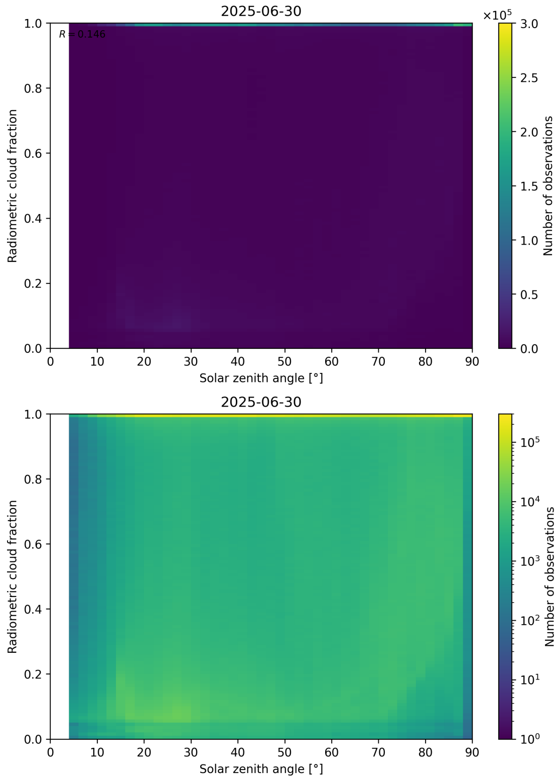
Figure 99: Scatter density plot of “Solar zenith angle” against “Radiometric cloud fraction” for 2025-06-29 to 2025-07-01.
