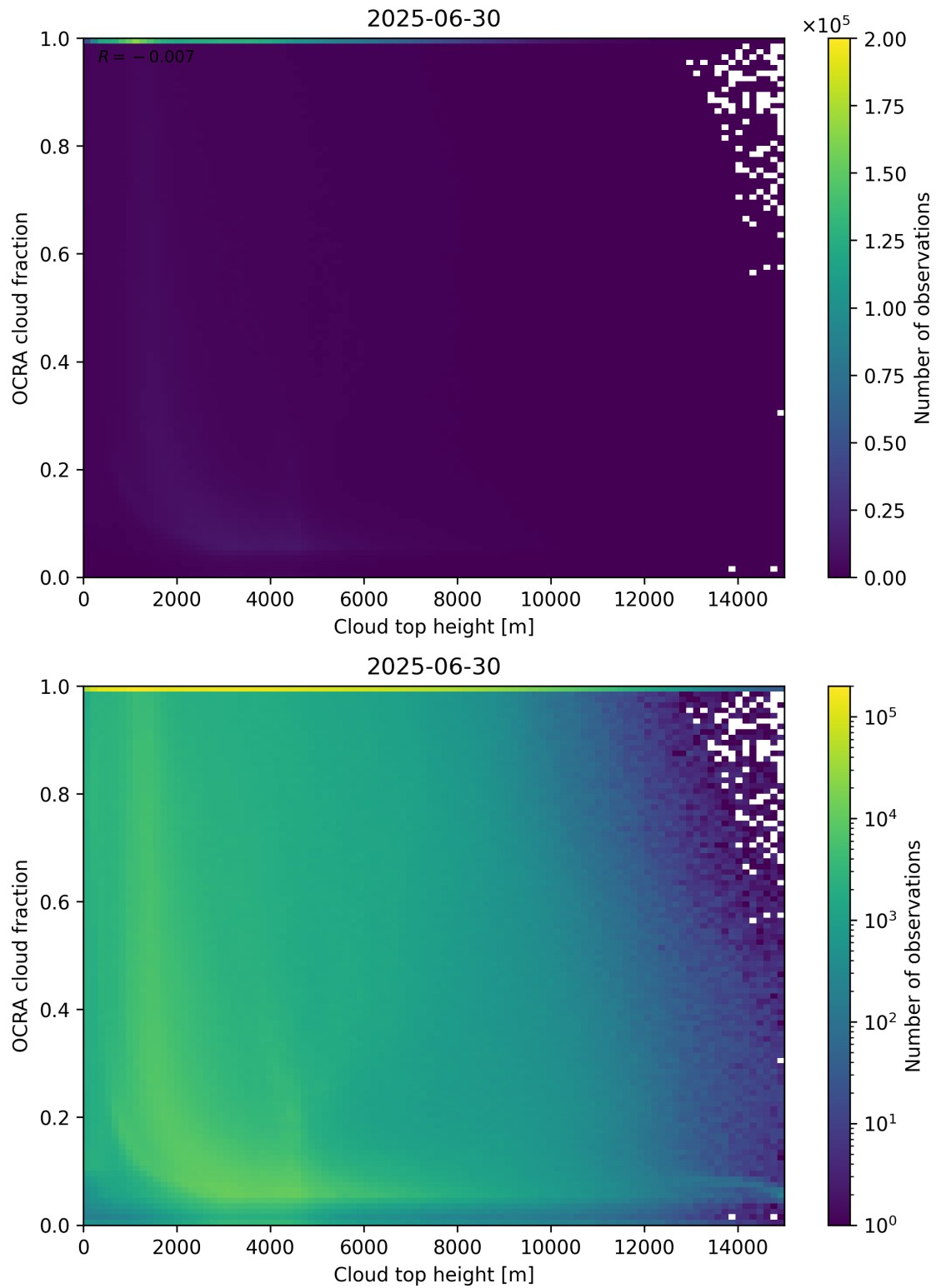
Figure 87: Scatter density plot of “Cloud top height” against “OCRA cloud fraction” for 2025-06-29 to 2025-07-01.
