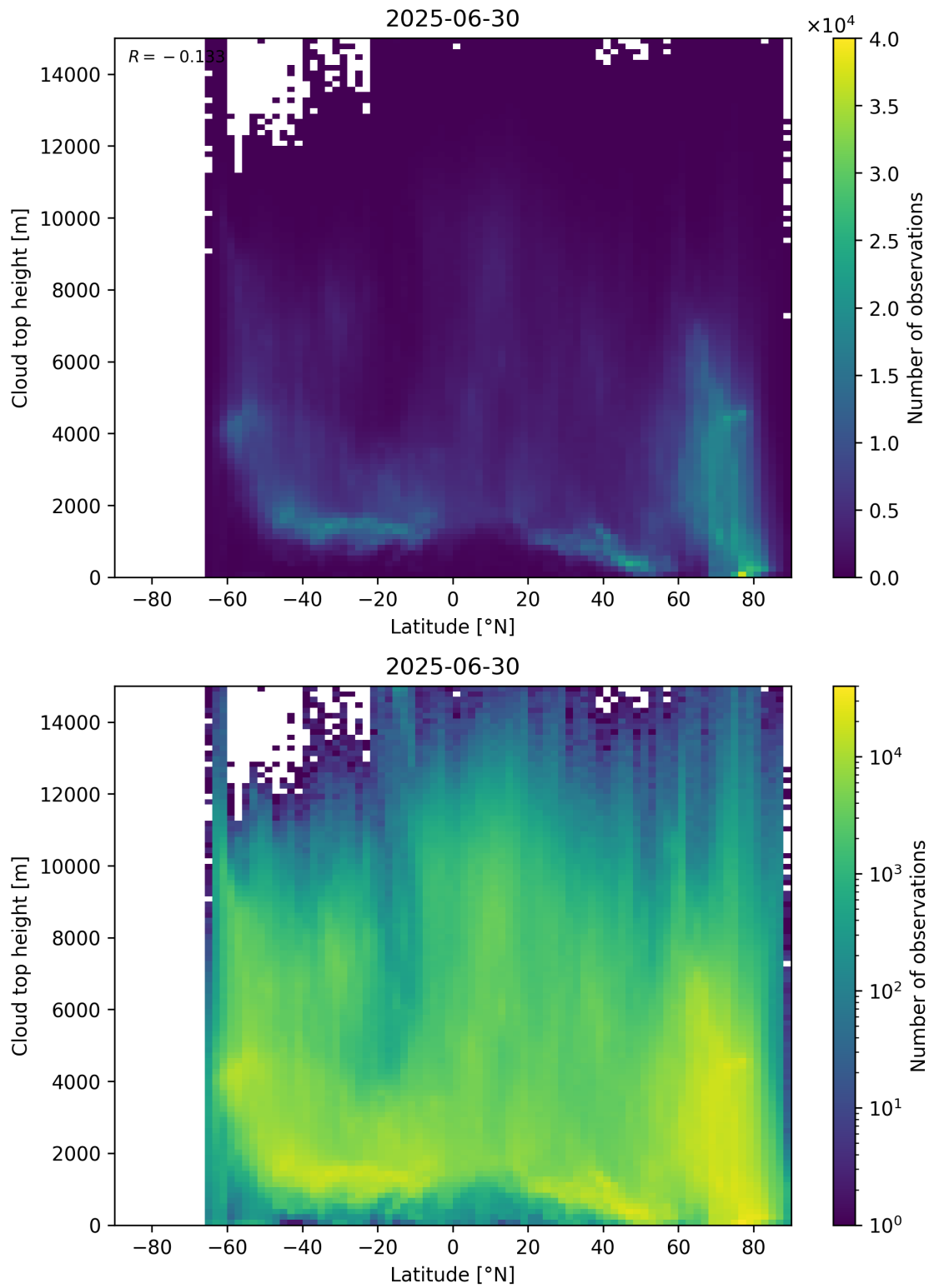
Figure 97: Scatter density plot of “Latitude” against “Cloud top height” for 2025-06-29 to 2025-07-01.
