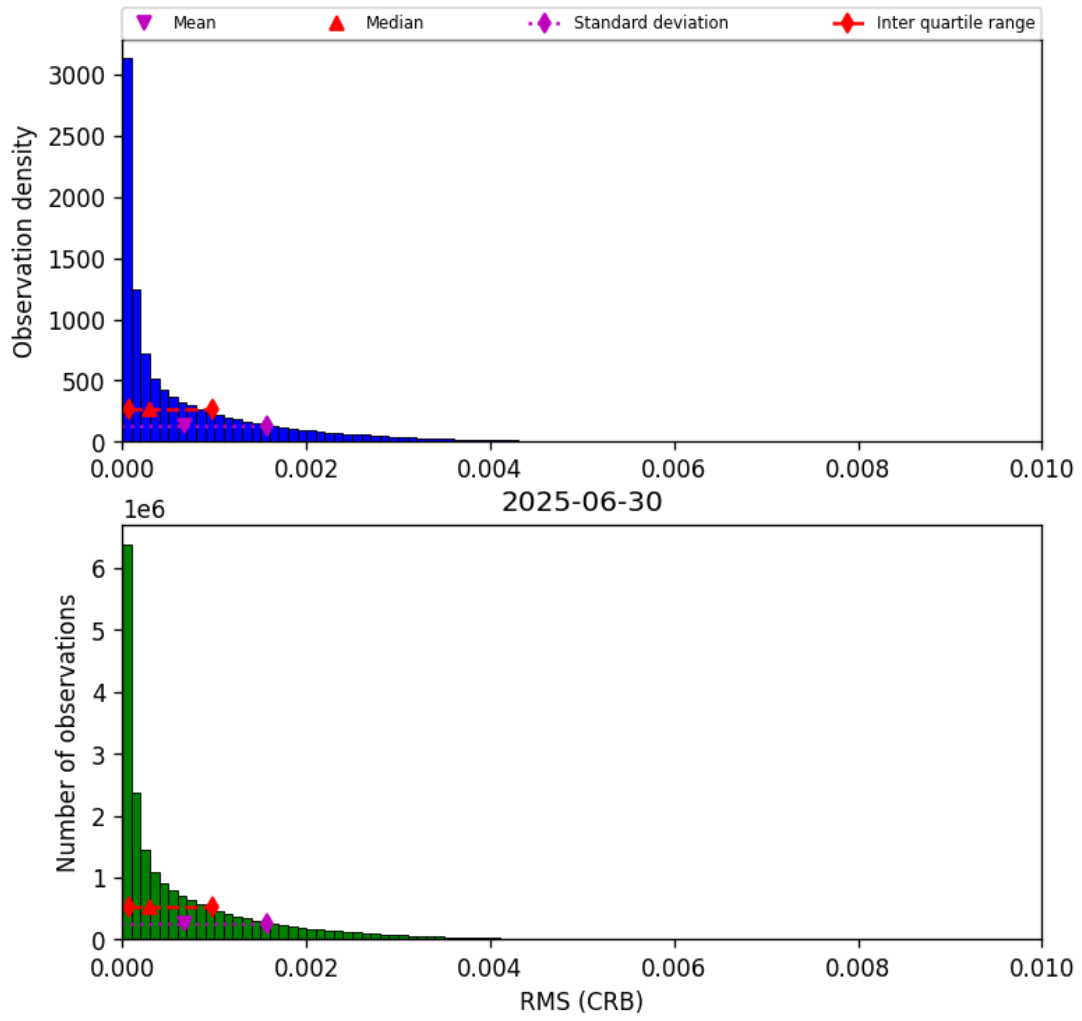
Figure 48: Histogram of “RMS (CRB)” for 2025-06-29 to 2025-07-01
