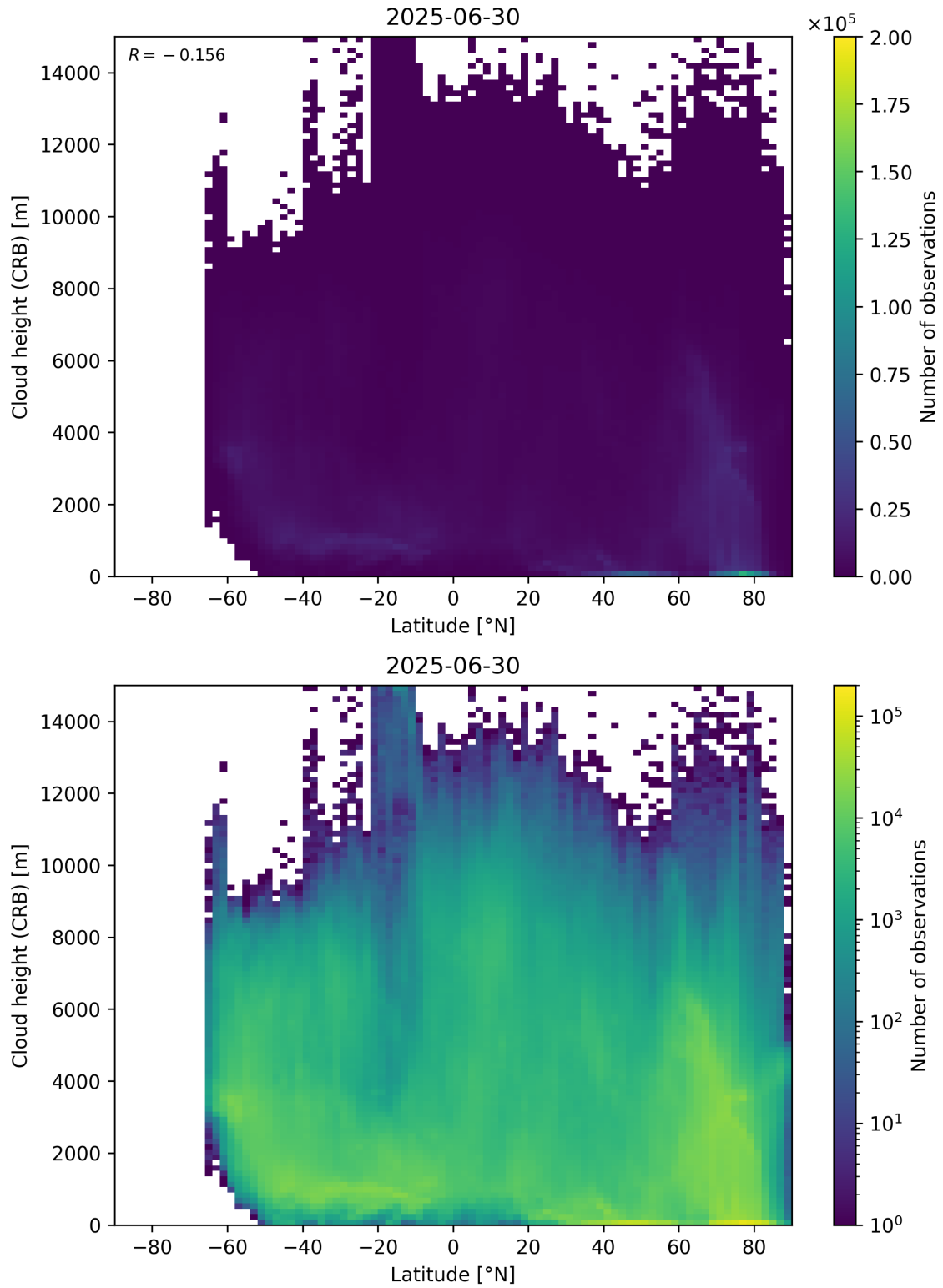
Figure 95: Scatter density plot of “Latitude” against “Cloud height (CRB)” for 2025-06-29 to 2025-07-01.
