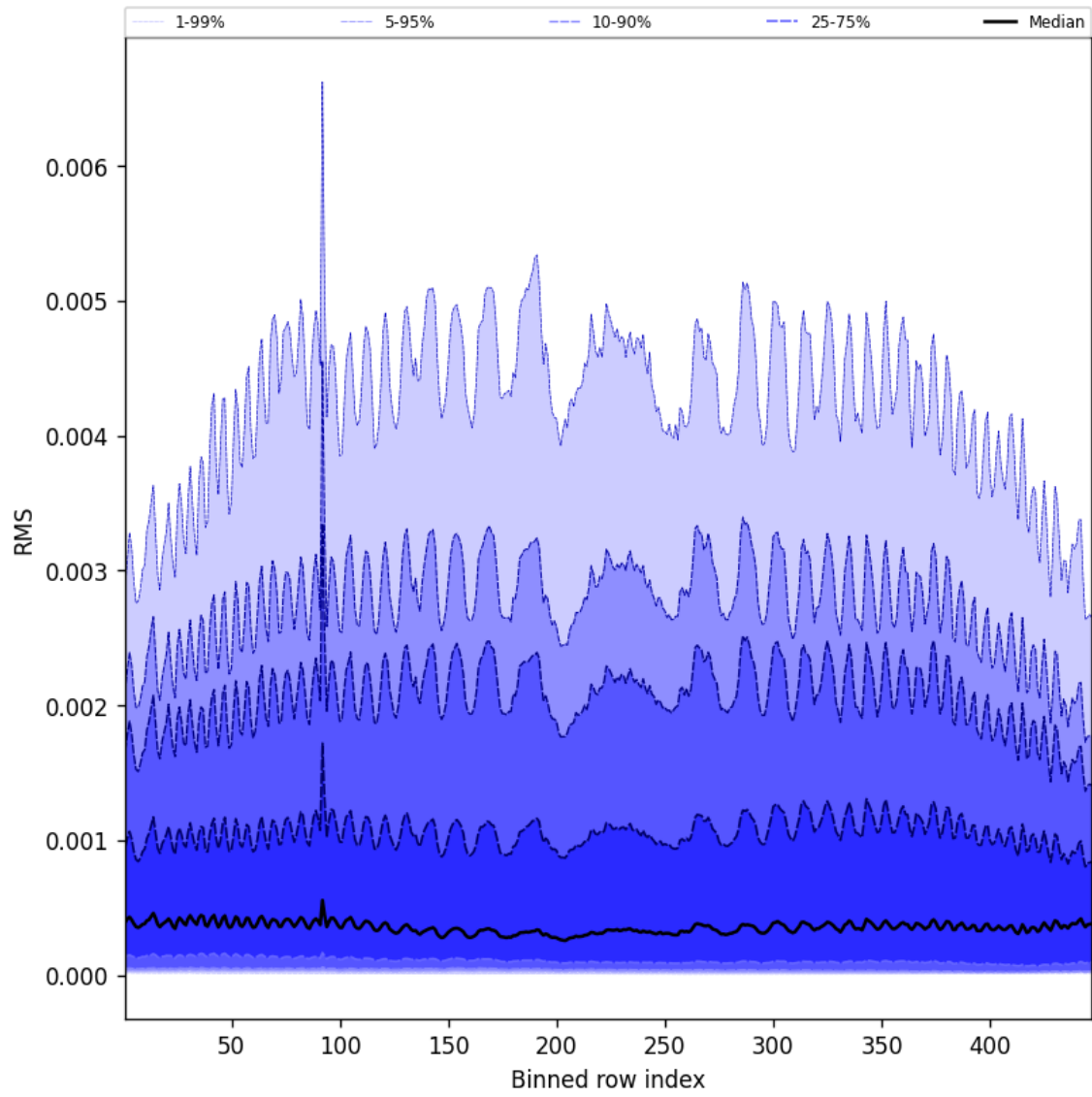
Figure 63: Along track statistics of “RMS” for 2025-06-29 to 2025-07-01
