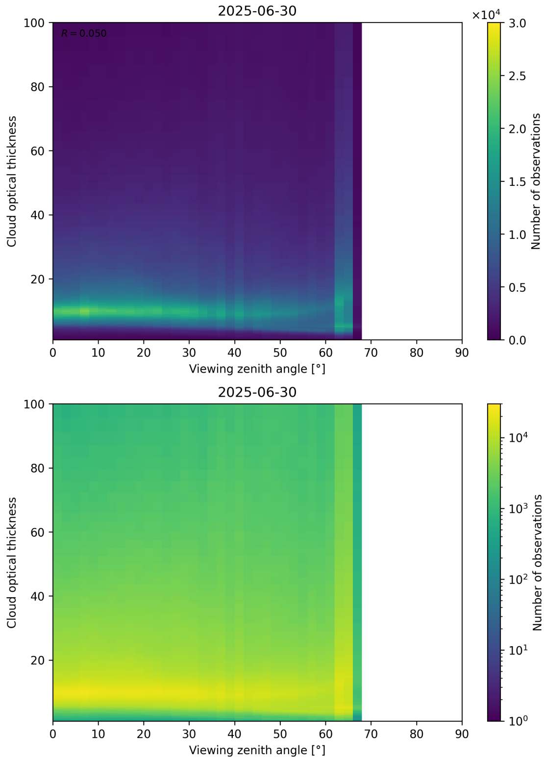
Figure 111: Scatter density plot of “Viewing zenith angle” against “Cloud optical thickness” for 2025-06-29 to 2025-07-01.
