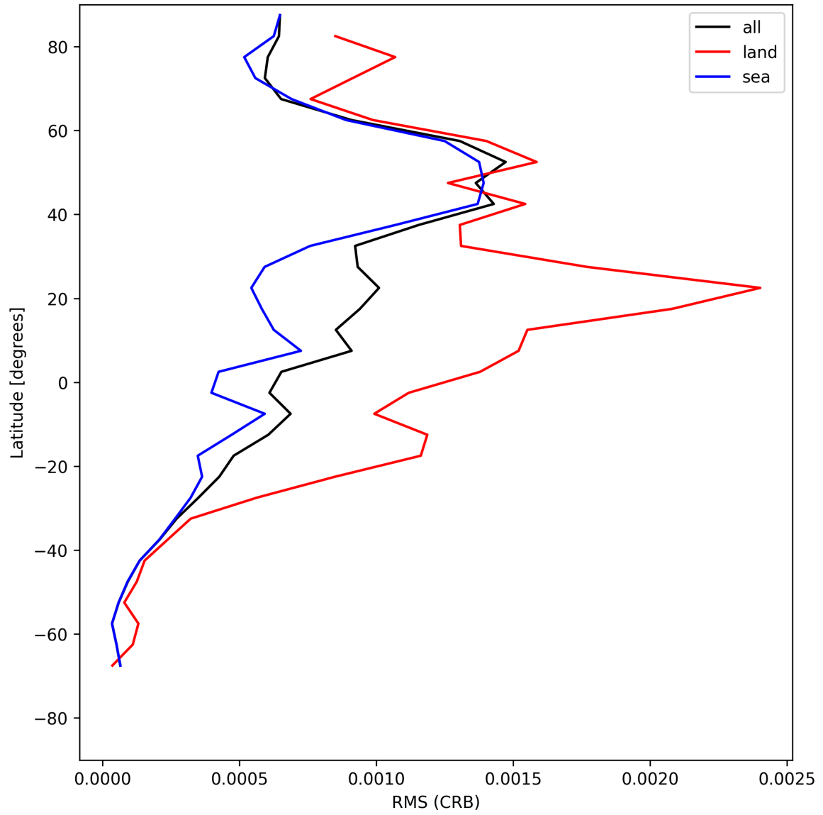
Figure 32: Zonal average of “RMS (CRB)” for 2025-06-29 to 2025-07-01.
