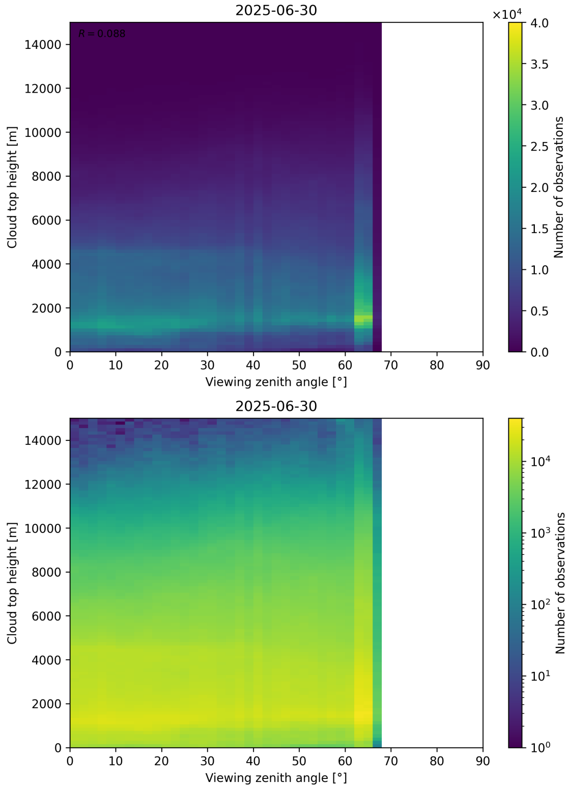
Figure 112: Scatter density plot of “Viewing zenith angle” against “Cloud top height” for 2025-06-29 to 2025-07-01.
