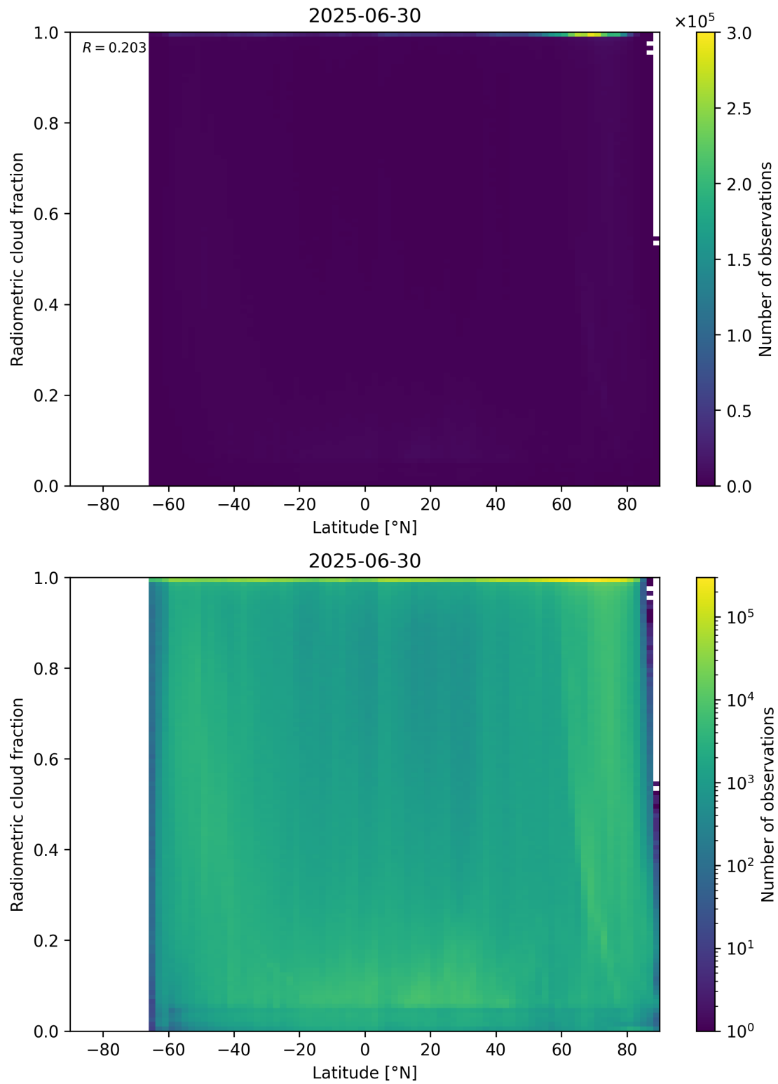
Figure 92: Scatter density plot of “Latitude” against “Radiometric cloud fraction” for 2025-06-29 to 2025-07-01.
