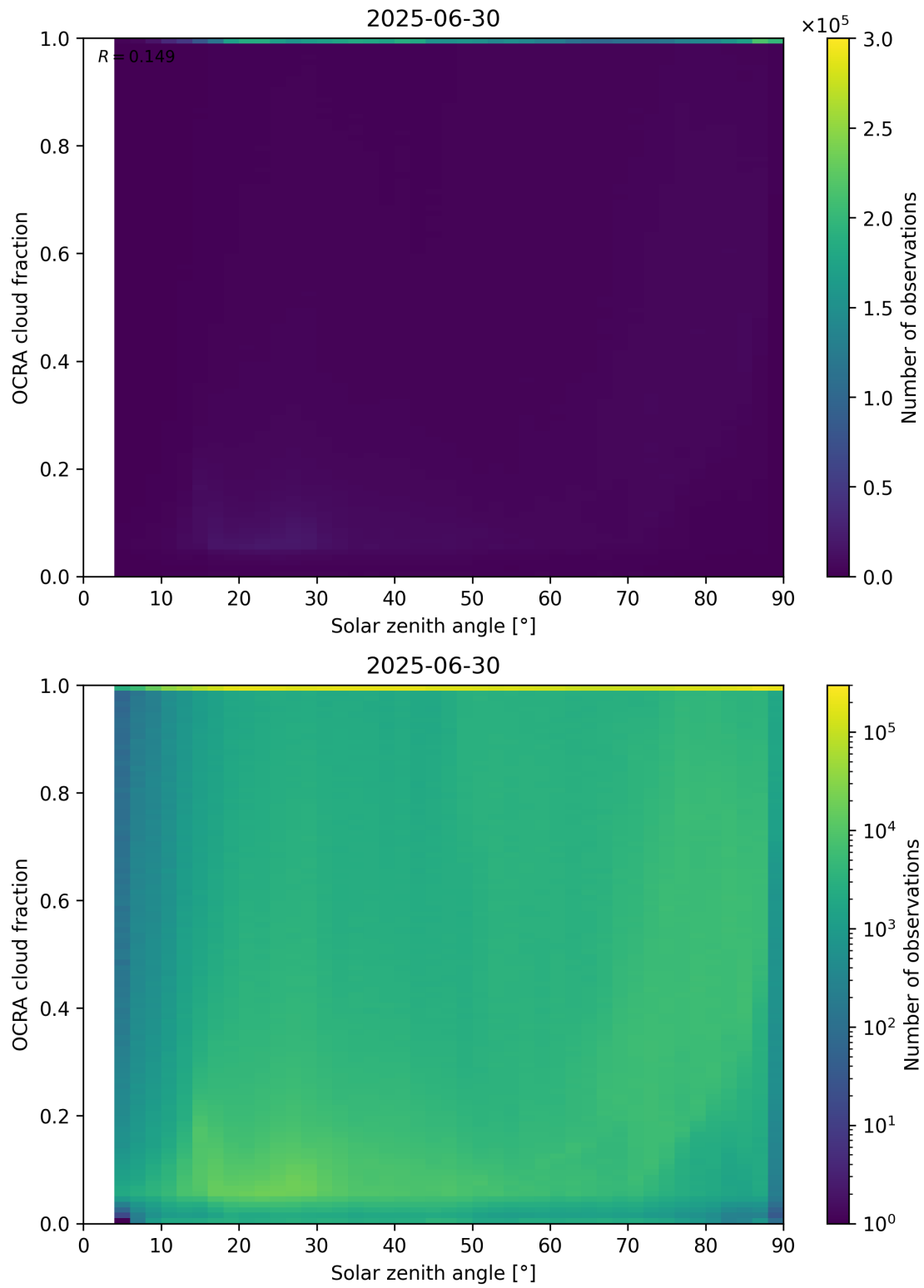
Figure 100: Scatter density plot of “Solar zenith angle” against “OCRA cloud fraction” for 2025-06-29 to 2025-07-01.
