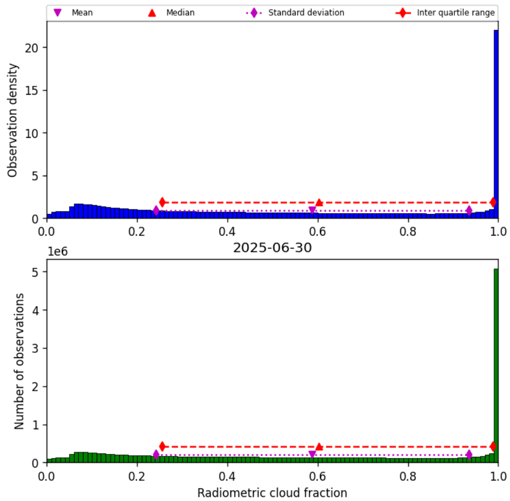
Figure 39: Histogram of “Radiometric cloud fraction” for 2025-06-29 to 2025-07-01
