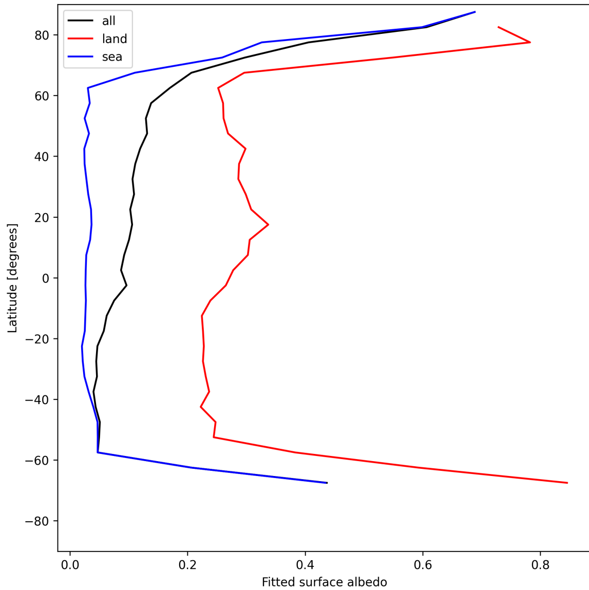
Figure 29: Zonal average of “Fitted surface albedo” for 2025-06-29 to 2025-07-01.
