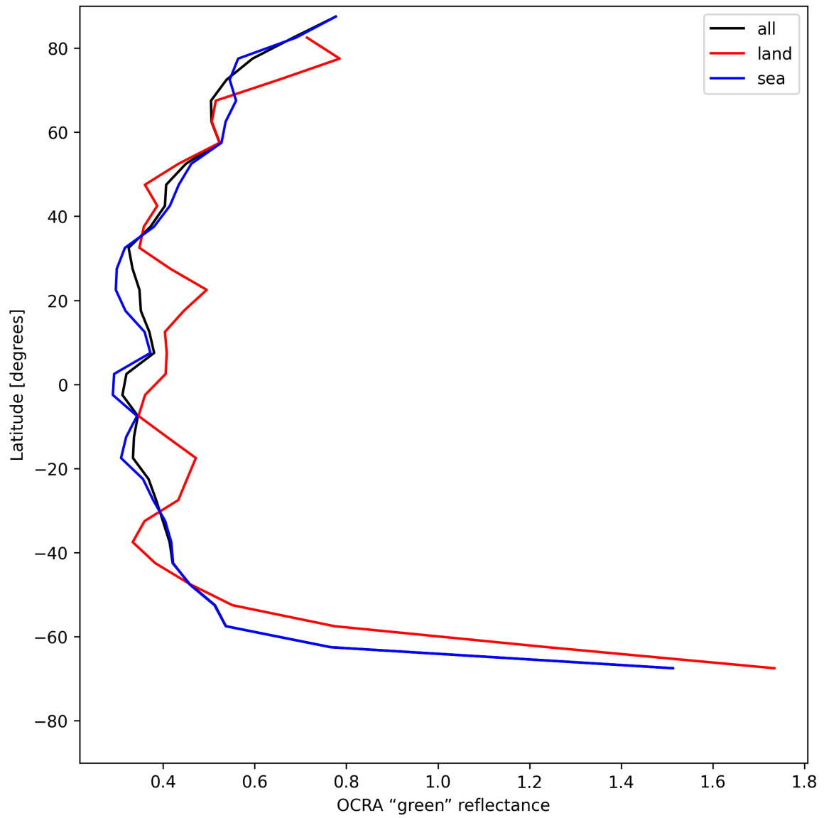
Figure 36: Zonal average of “OCRA “green” reflectance” for 2025-06-29 to 2025-07-01.
