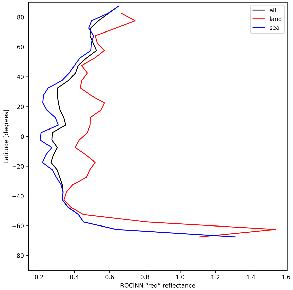
Figure 37: Zonal average of “ROCINN “red” reflectance” for 2025-06-29 to 2025-07-01.
