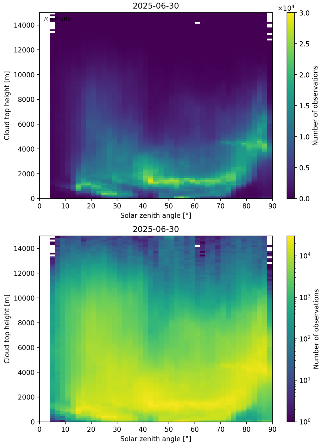
Figure 104: Scatter density plot of “Solar zenith angle” against “Cloud top height” for 2025-06-29 to 2025-07-01.
