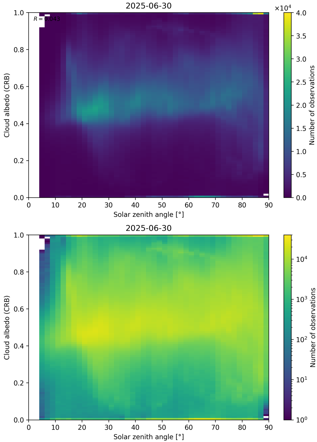
Figure 98: Scatter density plot of “Solar zenith angle” against “Cloud albedo (CRB)” for 2025-06-29 to 2025-07-01.
