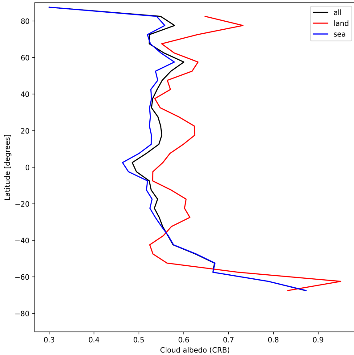
Figure 28: Zonal average of “Cloud albedo (CRB)” for 2025-06-29 to 2025-07-01.
