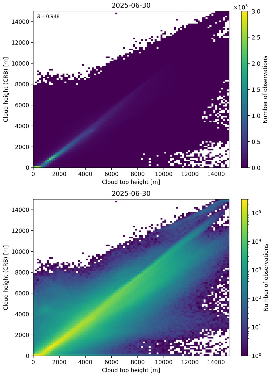
Figure 89: Scatter density plot of “Cloud top height” against “Cloud height (CRB)” for 2025-06-29 to 2025-07-01.
