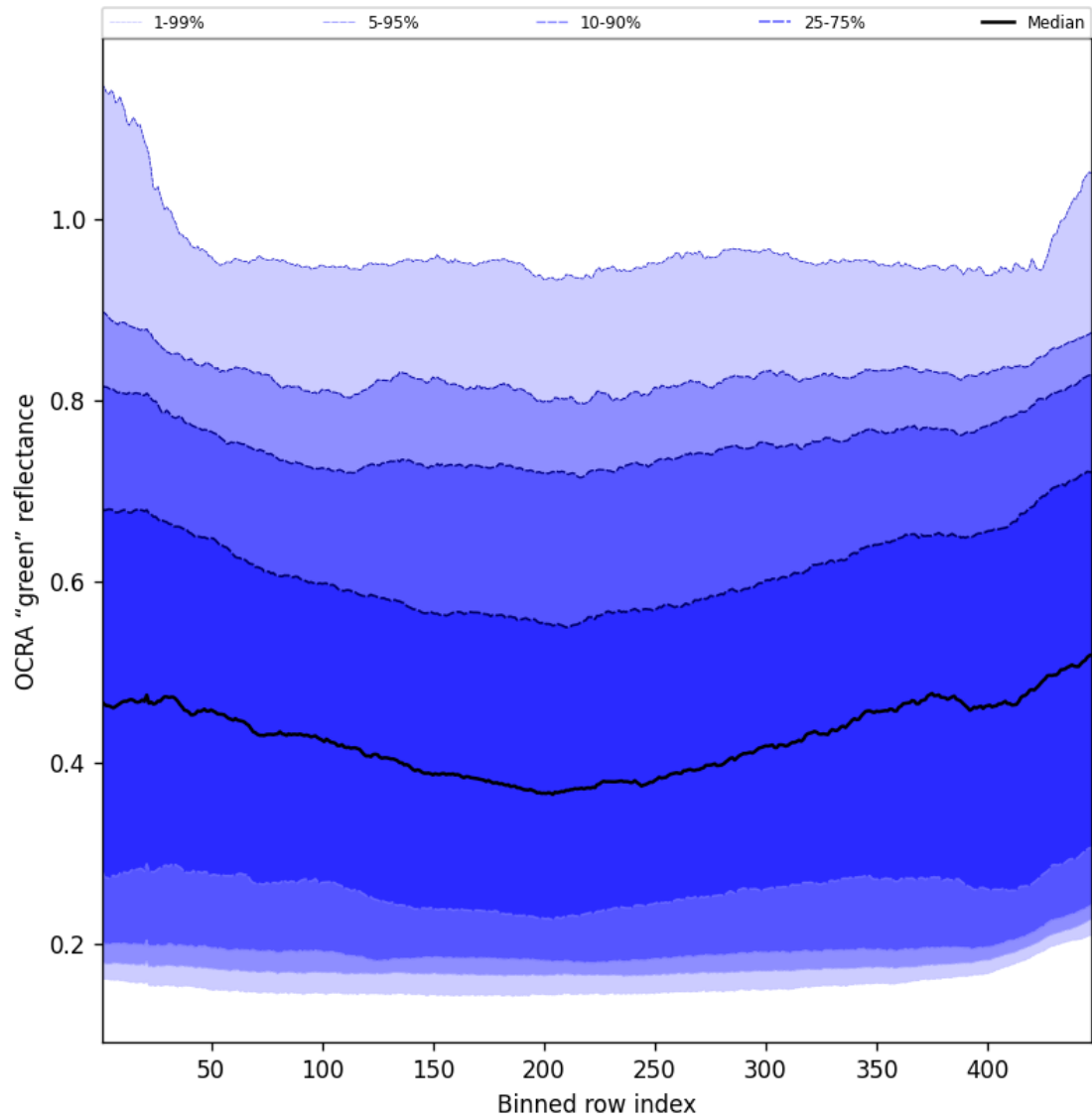
Figure 68: Along track statistics of “OCRA “green” reflectance” for 2025-06-29 to 2025-07-01
