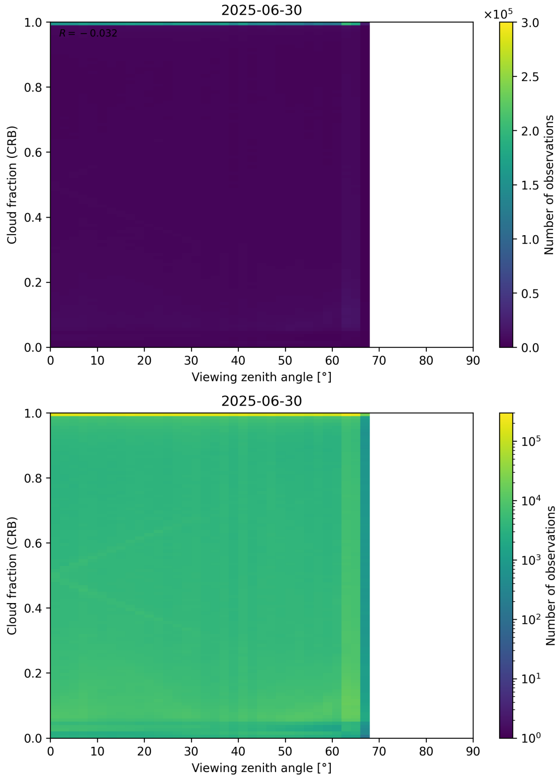
Figure 109: Scatter density plot of “Viewing zenith angle” against “Cloud fraction (CRB)” for 2025-06-29 to 2025-07-01.
