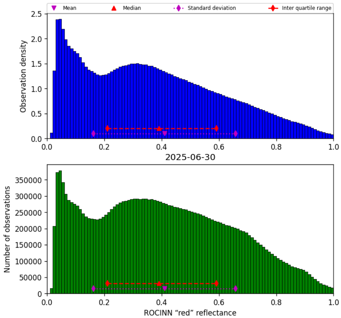
Figure 53: Histogram of “ROCINN “red” reflectance” for 2025-06-29 to 2025-07-01
