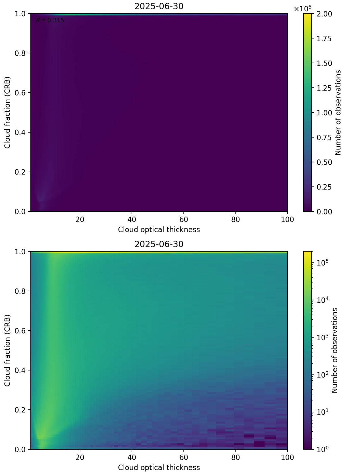
Figure 84: Scatter density plot of “Cloud optical thickness” against “Cloud fraction (CRB)” for 2025-06-29 to 2025-07-01.
