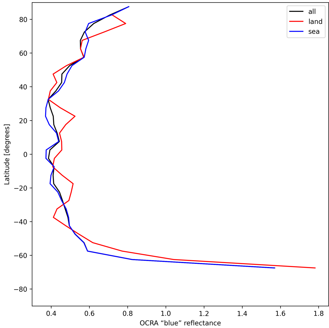
Figure 35: Zonal average of “OCRA “blue” reflectance” for 2025-06-29 to 2025-07-01.
