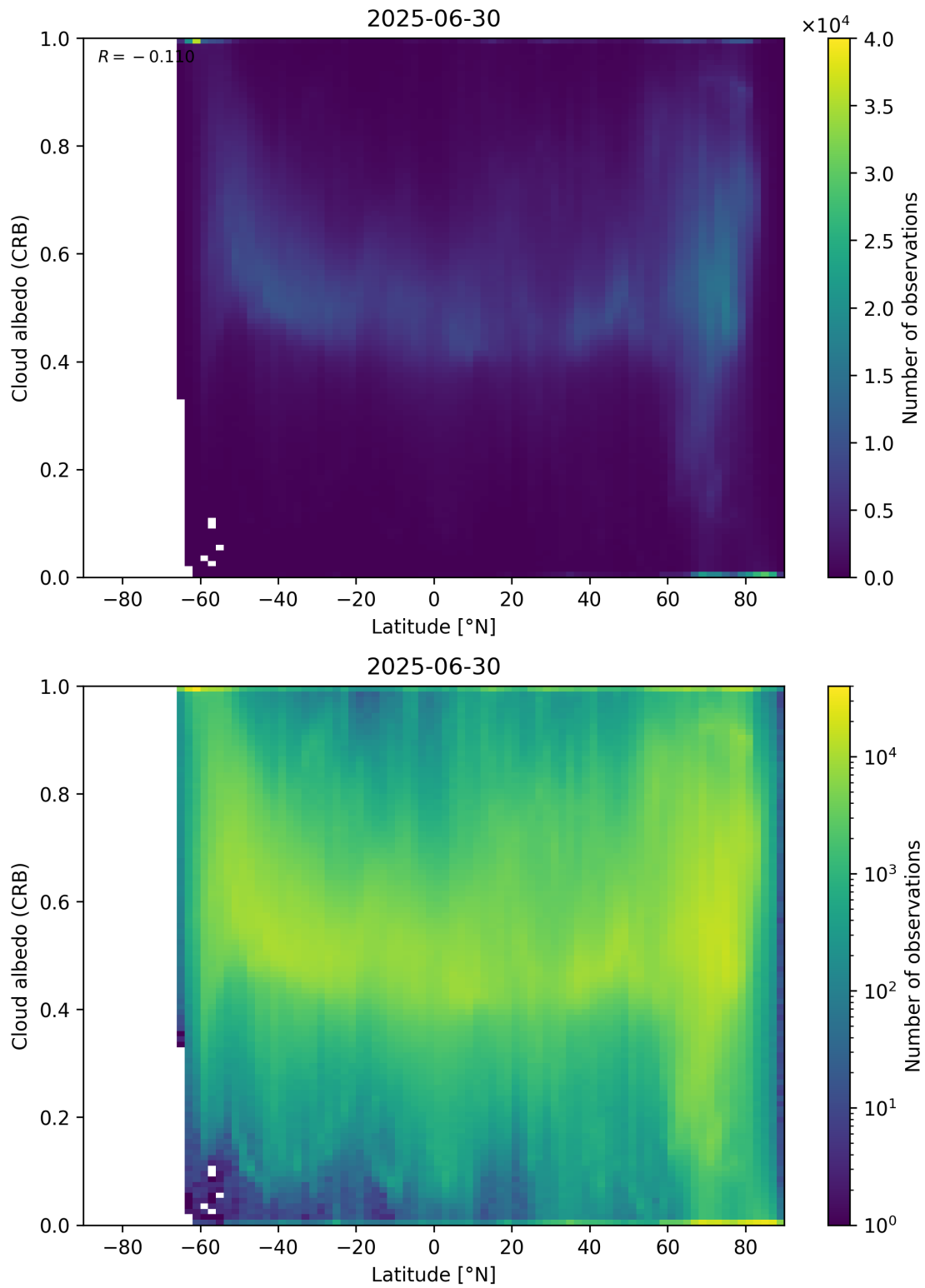
Figure 91: Scatter density plot of “Latitude” against “Cloud albedo (CRB)” for 2025-06-29 to 2025-07-01.
