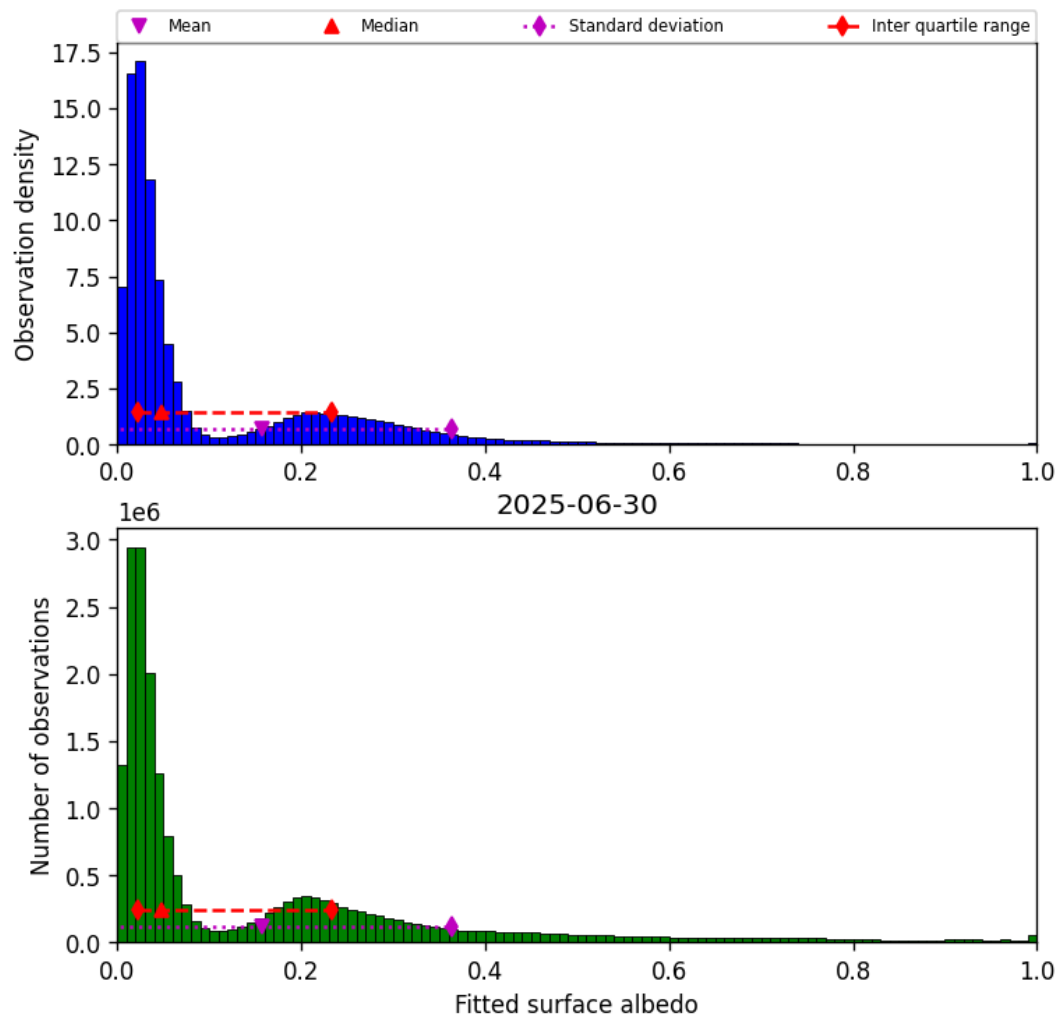
Figure 45: Histogram of “Fitted surface albedo” for 2025-06-29 to 2025-07-01
