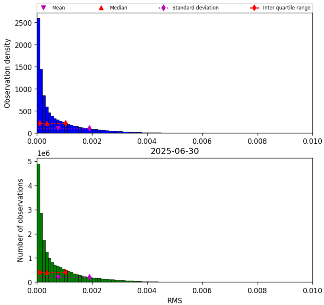
Figure 47: Histogram of “RMS” for 2025-06-29 to 2025-07-01
