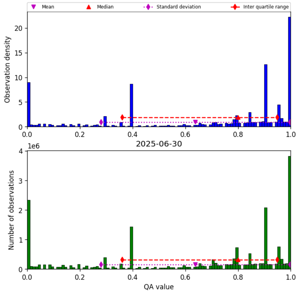
Figure 38: Histogram of “QA value” for 2025-06-29 to 2025-07-01
