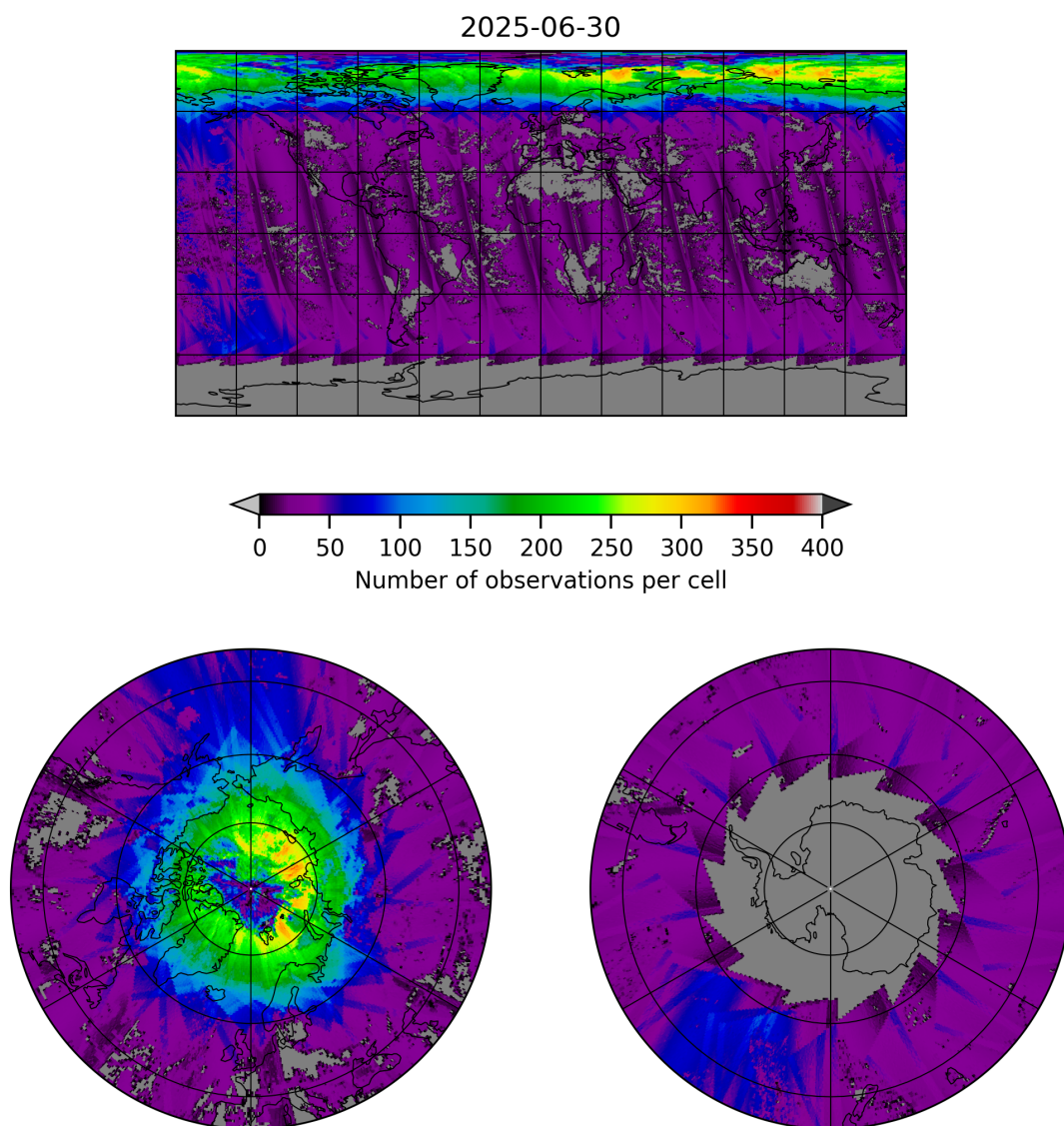
Figure 21: Map of the number of observations for 2025-06-29 to 2025-07-01
