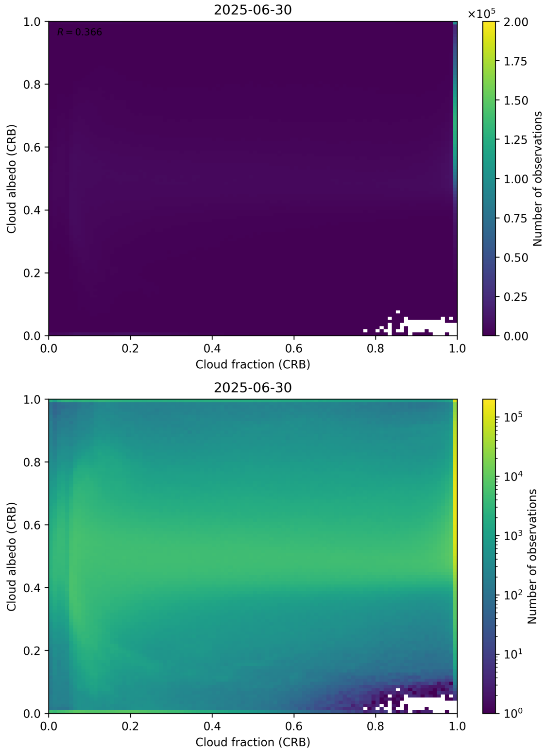
Figure 77: Scatter density plot of “Cloud fraction (CRB)” against “Cloud albedo (CRB)” for 2025-06-29 to 2025-07-01.
