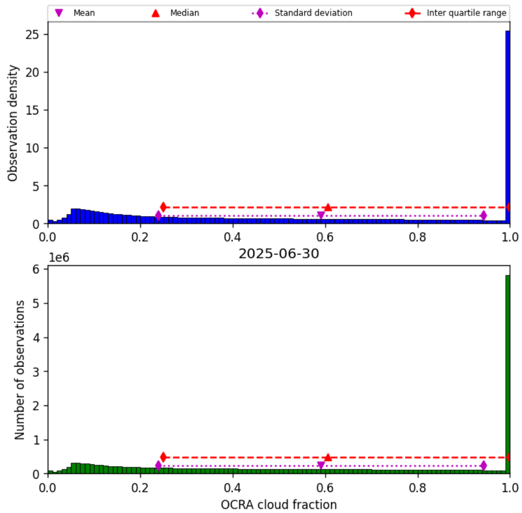
Figure 50: Histogram of “OCRA cloud fraction” for 2025-06-29 to 2025-07-01
