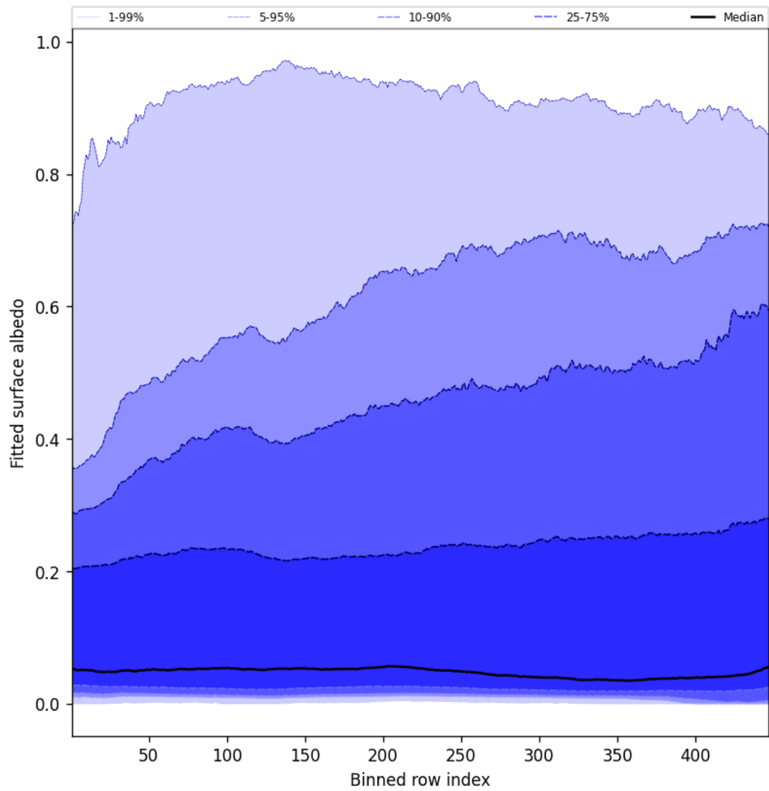
Figure 61: Along track statistics of “Fitted surface albedo” for 2025-06-29 to 2025-07-01
