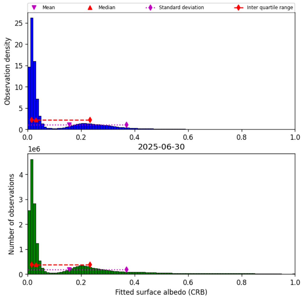
Figure 46: Histogram of “Fitted surface albedo (CRB)” for 2025-06-29 to 2025-07-01
