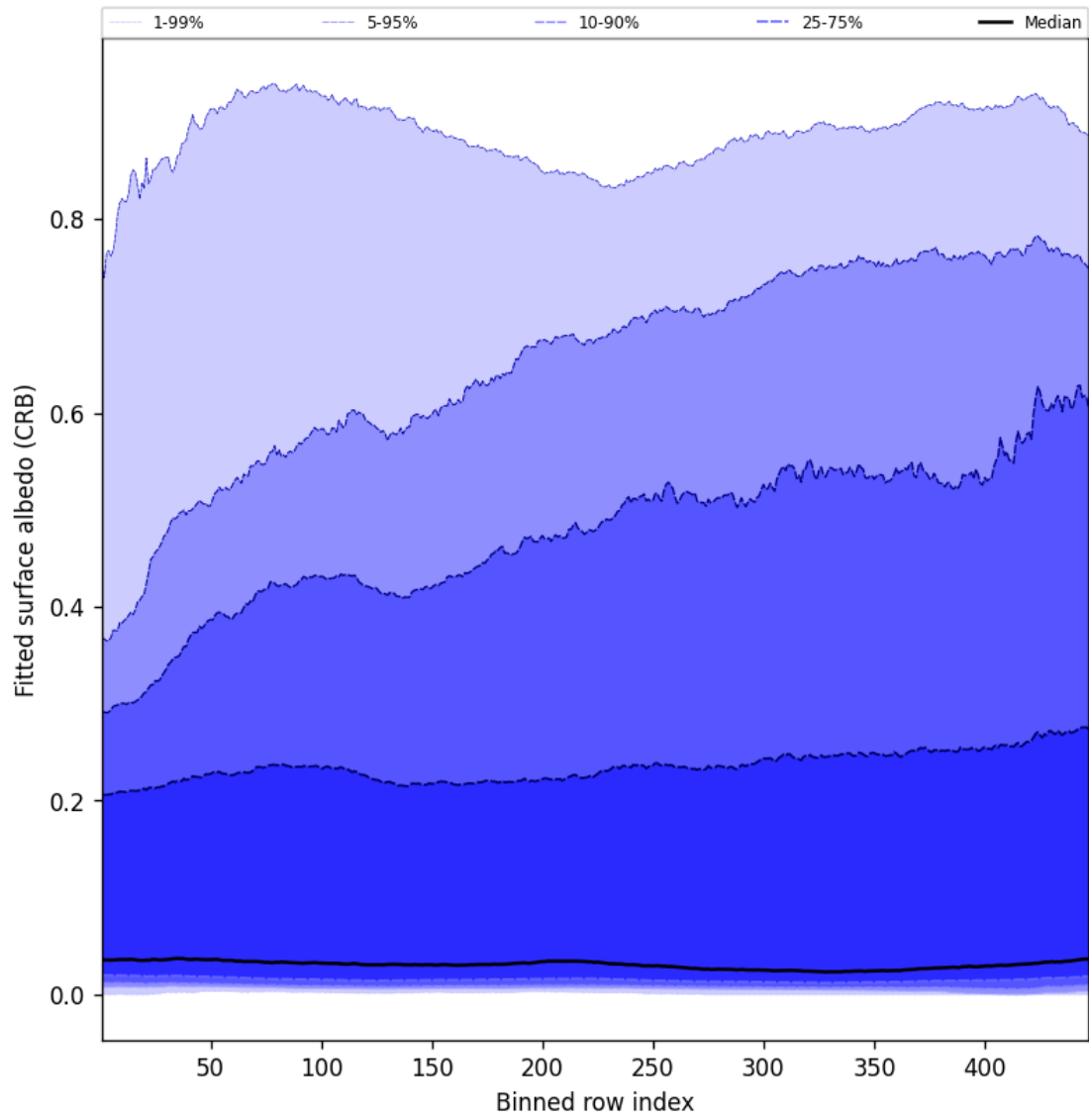
Figure 62: Along track statistics of “Fitted surface albedo (CRB)” for 2025-06-29 to 2025-07-01
