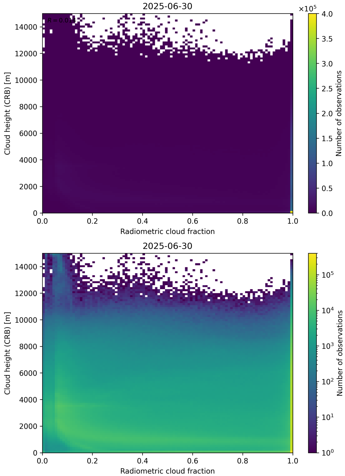
Figure 74: Scatter density plot of “Radiometric cloud fraction” against “Cloud height (CRB)” for 2025-06-29 to 2025-07-01.
