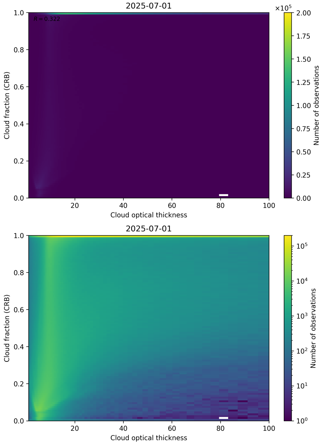
Figure 84: Scatter density plot of “Cloud optical thickness” against “Cloud fraction (CRB)” for 2025-06-30 to 2025-07-02.
