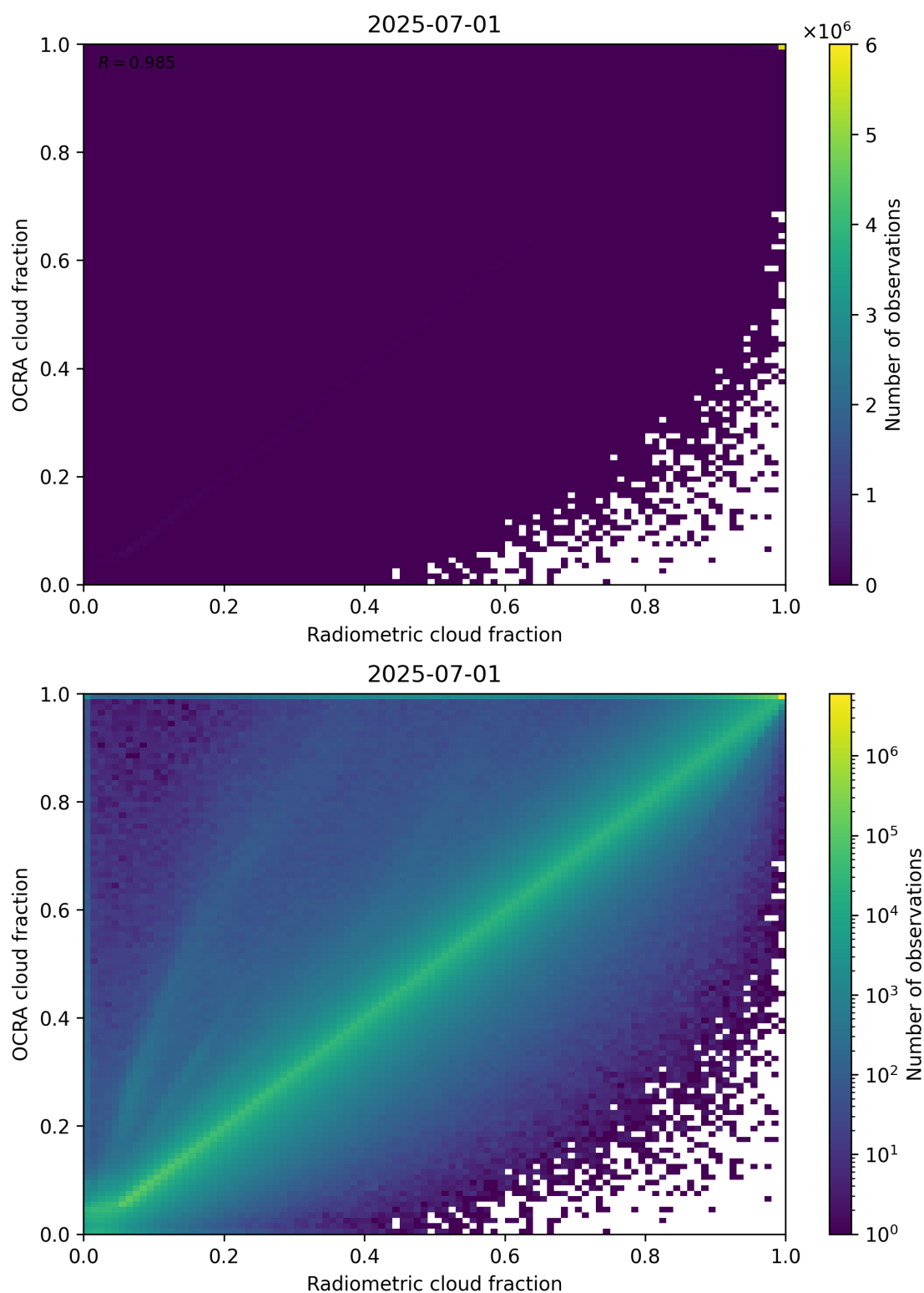
Figure 72: Scatter density plot of “Radiometric cloud fraction” against “OCRA cloud fraction” for 2025-06-30 to 2025-07-02.
