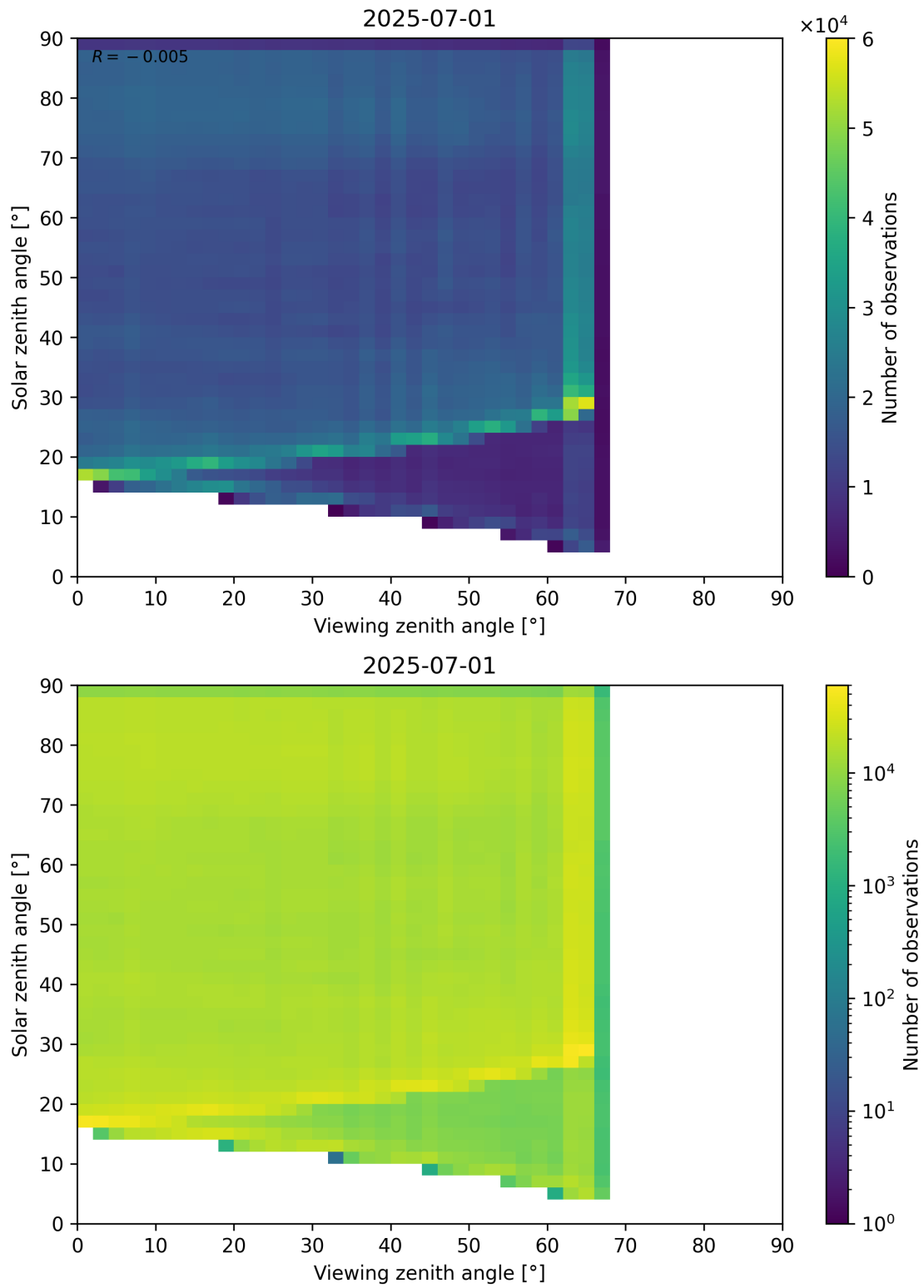
Figure 114: Scatter density plot of “Viewing zenith angle” against “Solar zenith angle” for 2025-06-30 to 2025-07-02.
