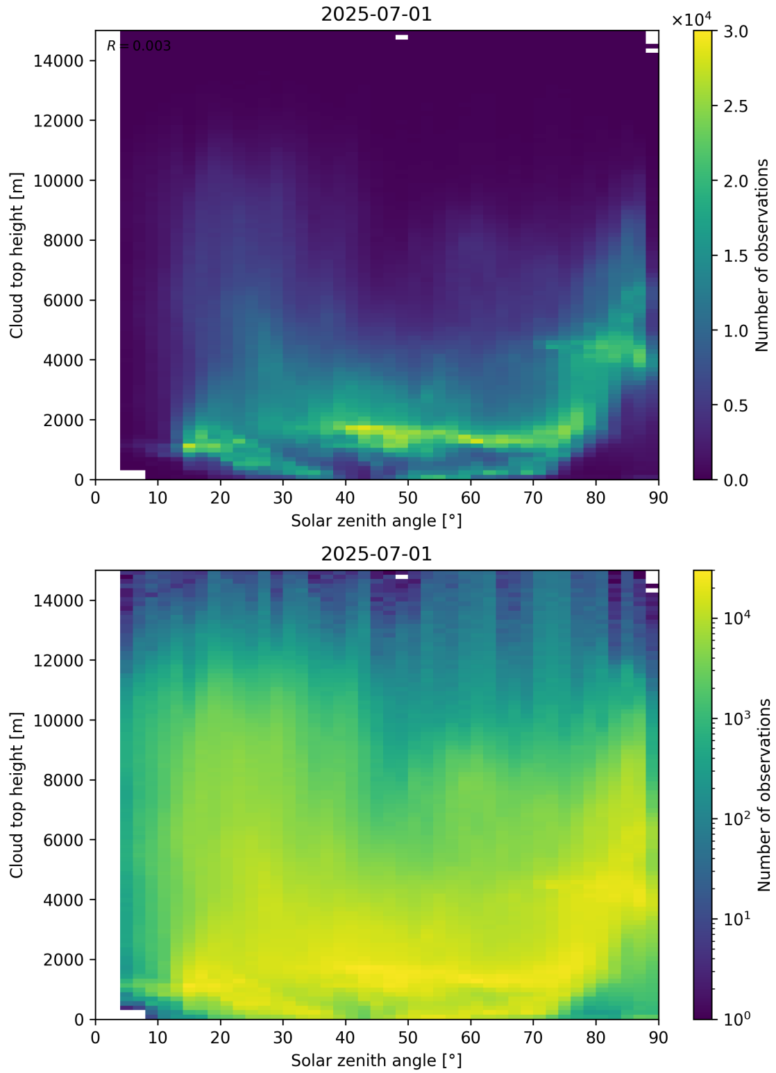
Figure 104: Scatter density plot of “Solar zenith angle” against “Cloud top height” for 2025-06-30 to 2025-07-02.
