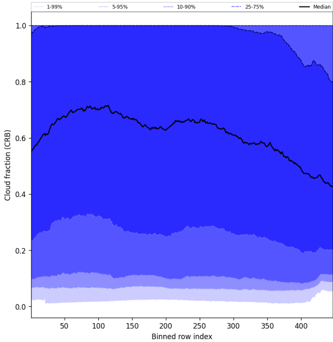
Figure 58: Along track statistics of “Cloud fraction (CRB)” for 2025-06-30 to 2025-07-02
