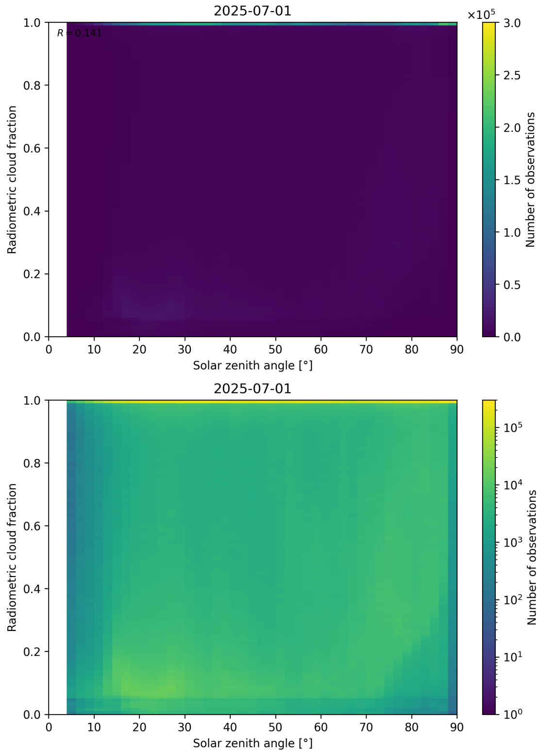
Figure 99: Scatter density plot of “Solar zenith angle” against “Radiometric cloud fraction” for 2025-06-30 to 2025-07-02.
