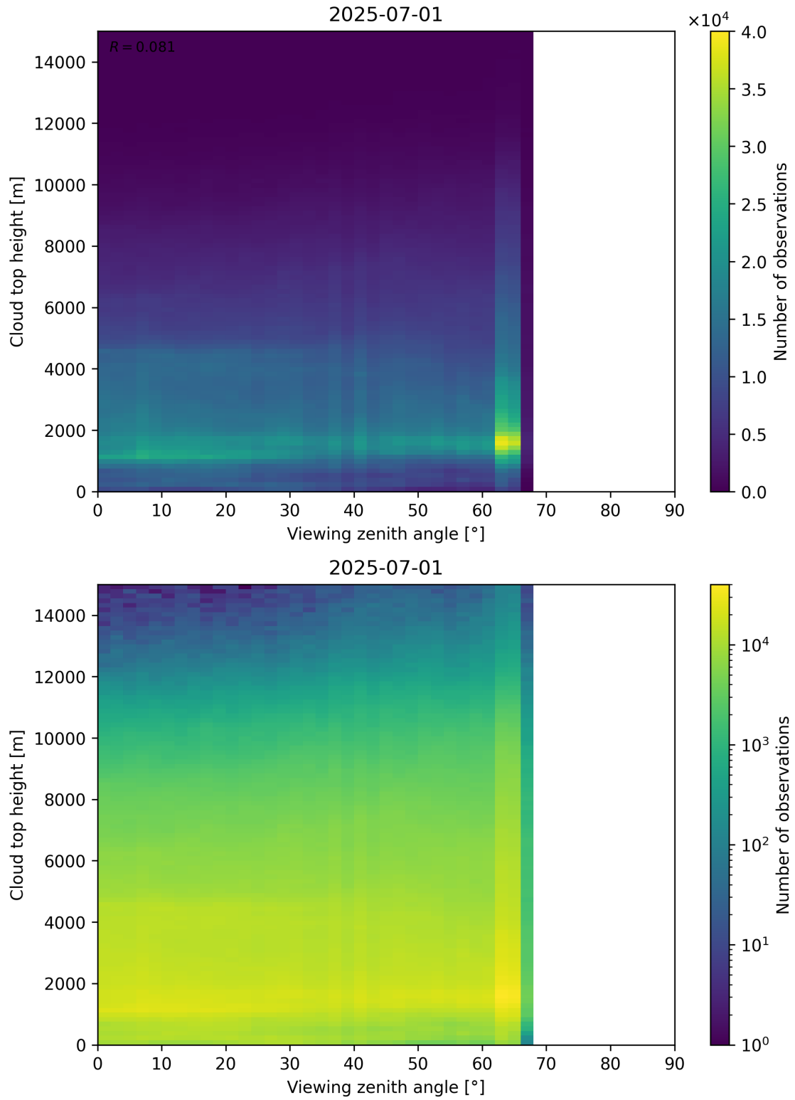
Figure 112: Scatter density plot of “Viewing zenith angle” against “Cloud top height” for 2025-06-30 to 2025-07-02.
