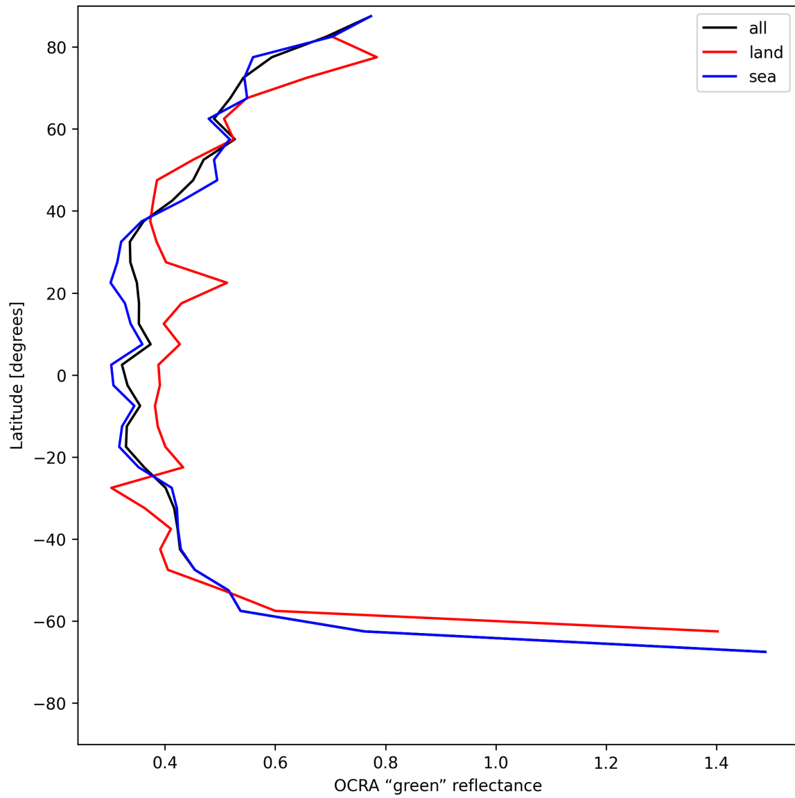
Figure 36: Zonal average of “OCRA “green” reflectance” for 2025-06-30 to 2025-07-02.
