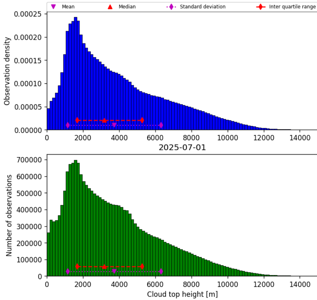
Figure 40: Histogram of “Cloud top height” for 2025-06-30 to 2025-07-02
