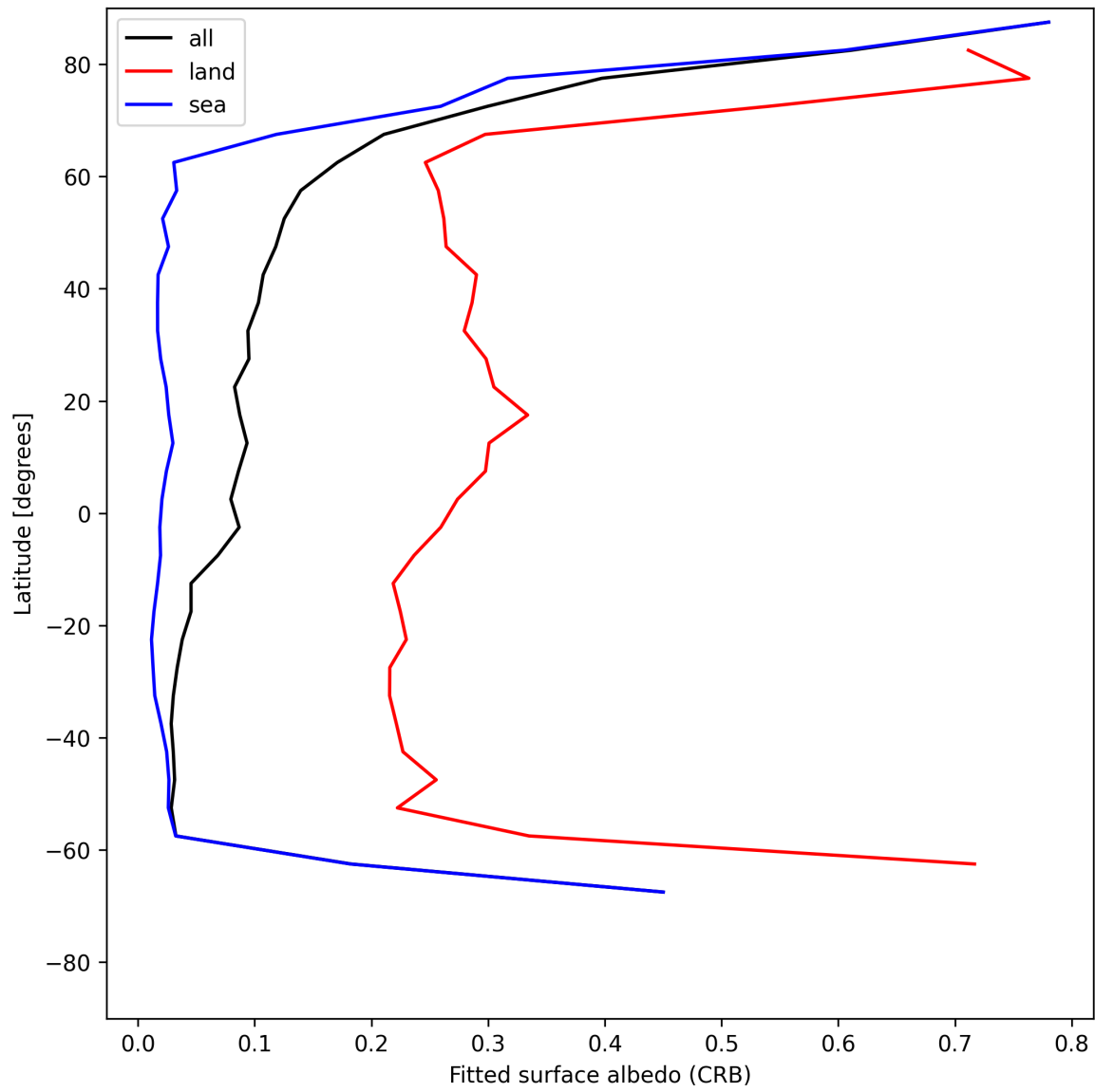
Figure 30: Zonal average of “Fitted surface albedo (CRB)” for 2025-06-30 to 2025-07-02.
