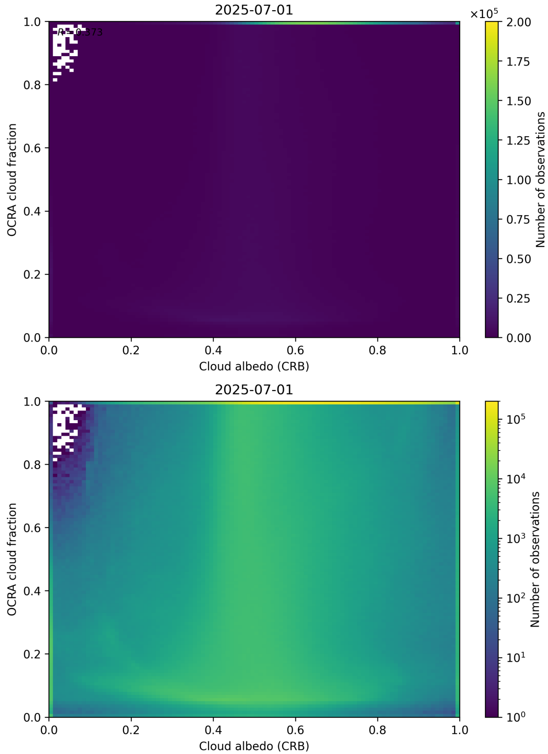
Figure 70: Scatter density plot of “Cloud albedo (CRB)” against “OCRA cloud fraction” for 2025-06-30 to 2025-07-02.
