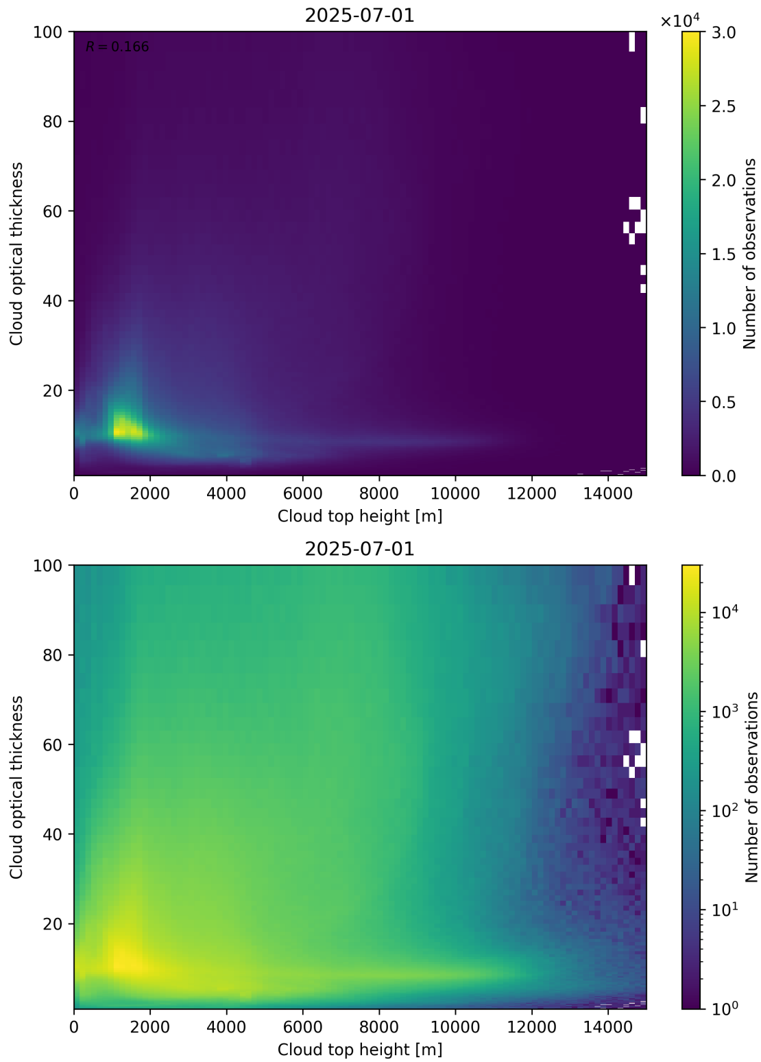
Figure 90: Scatter density plot of “Cloud top height” against “Cloud optical thickness” for 2025-06-30 to 2025-07-02.
