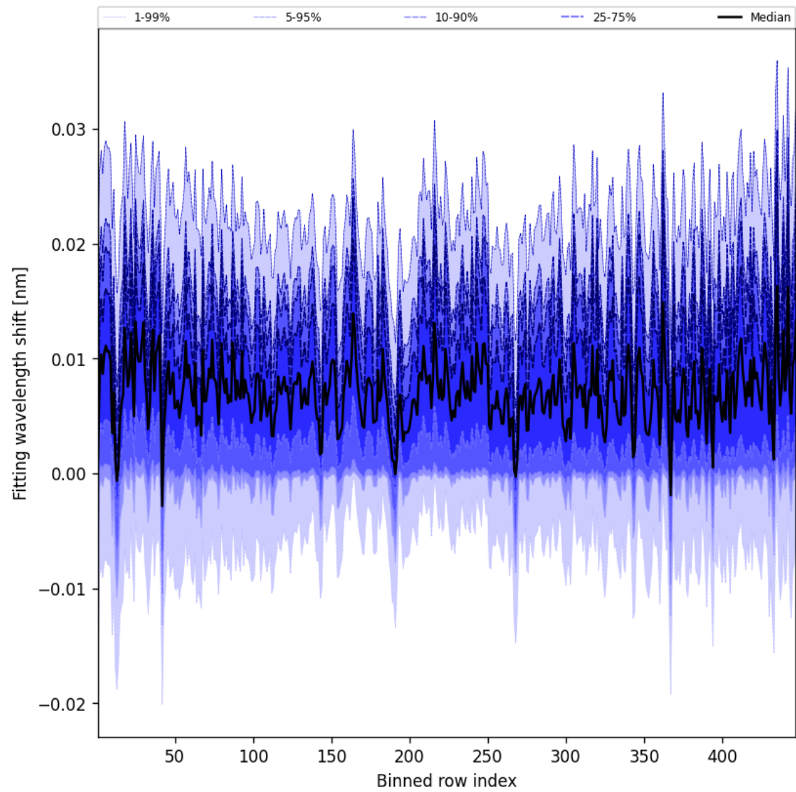
Figure 65: Along track statistics of “Fitting wavelength shift” for 2025-06-30 to 2025-07-02
