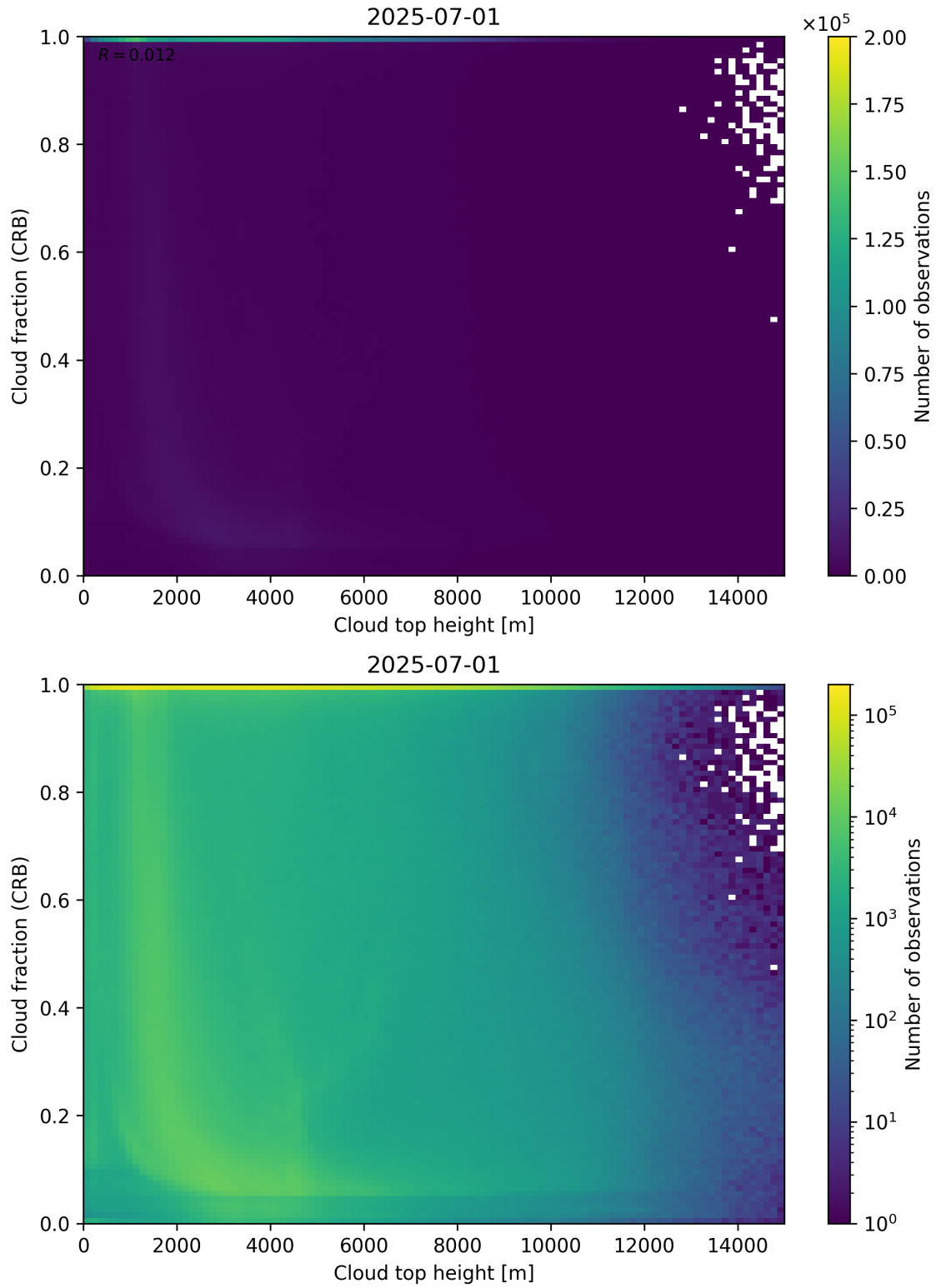
Figure 88: Scatter density plot of “Cloud top height” against “Cloud fraction (CRB)” for 2025-06-30 to 2025-07-02.
