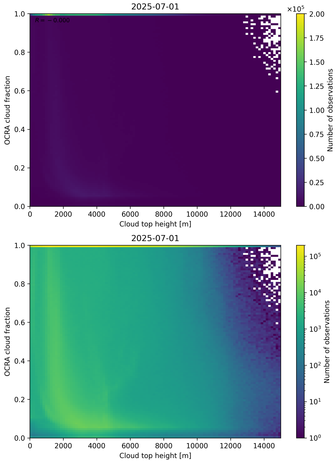
Figure 87: Scatter density plot of “Cloud top height” against “OCRA cloud fraction” for 2025-06-30 to 2025-07-02.
