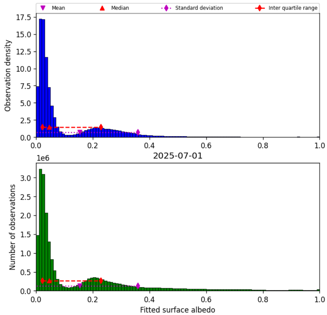
Figure 45: Histogram of “Fitted surface albedo” for 2025-06-30 to 2025-07-02
