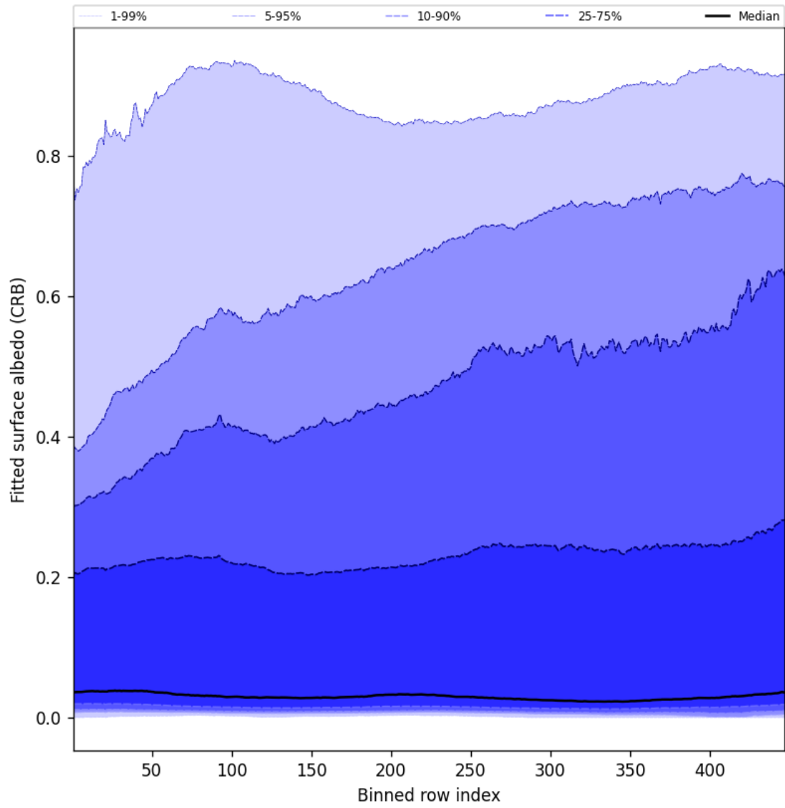
Figure 62: Along track statistics of “Fitted surface albedo (CRB)” for 2025-06-30 to 2025-07-02
