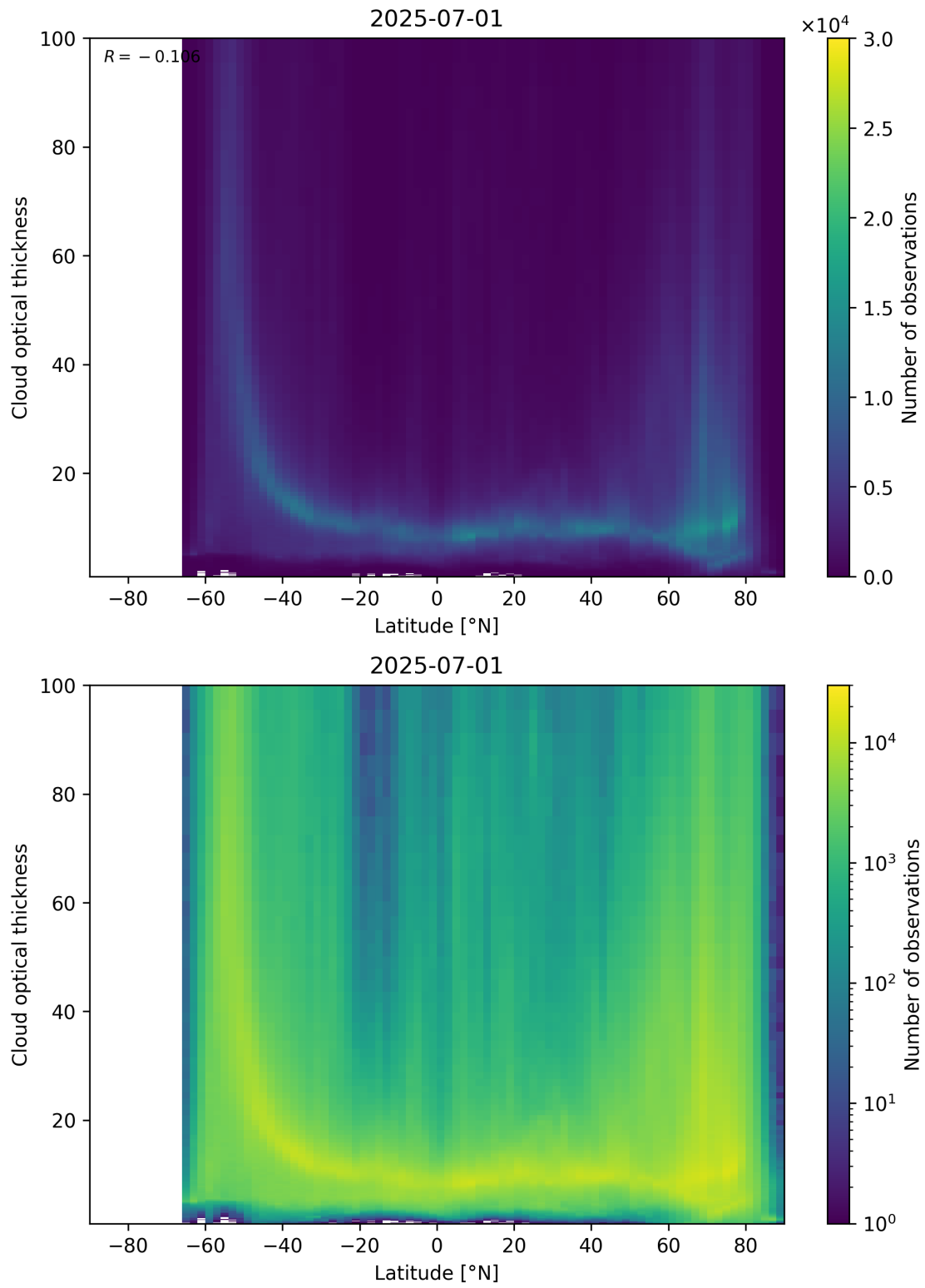
Figure 96: Scatter density plot of “Latitude” against “Cloud optical thickness” for 2025-06-30 to 2025-07-02.
