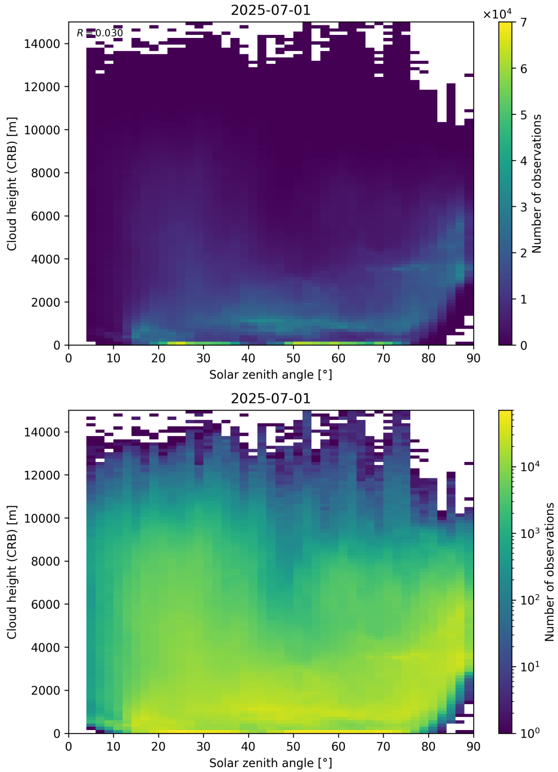
Figure 102: Scatter density plot of “Solar zenith angle” against “Cloud height (CRB)” for 2025-06-30 to 2025-07-02.
