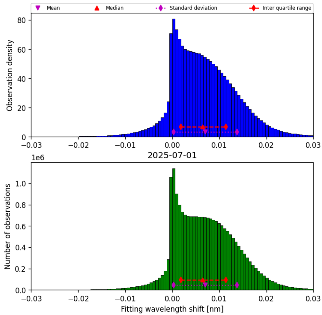
Figure 49: Histogram of “Fitting wavelength shift” for 2025-06-30 to 2025-07-02
