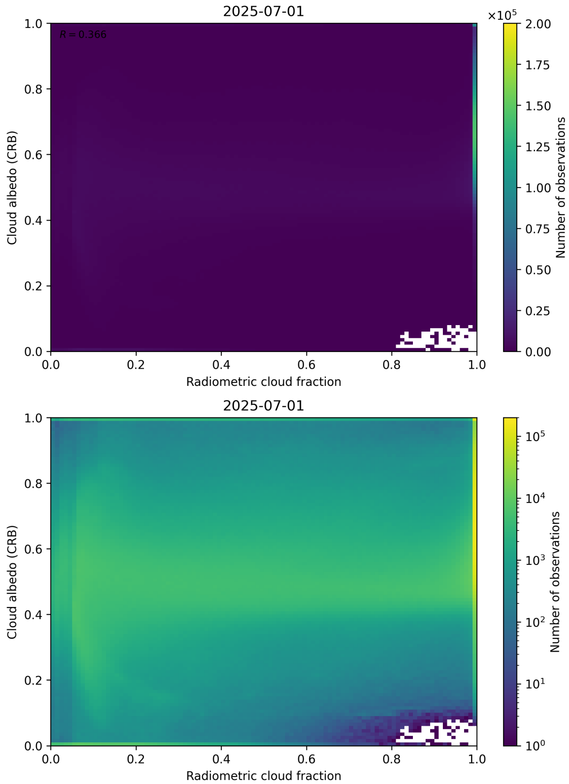
Figure 71: Scatter density plot of “Radiometric cloud fraction” against “Cloud albedo (CRB)” for 2025-06-30 to 2025-07-02.
