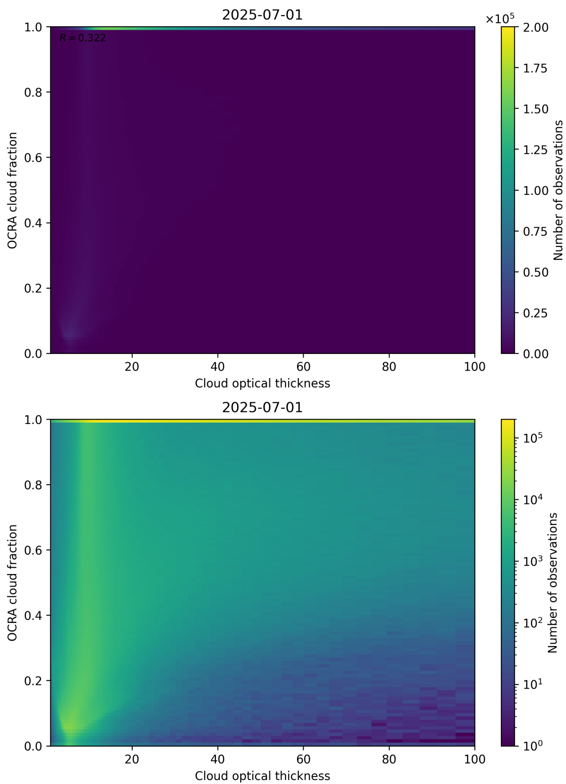
Figure 83: Scatter density plot of “Cloud optical thickness” against “OCRA cloud fraction” for 2025-06-30 to 2025-07-02.
