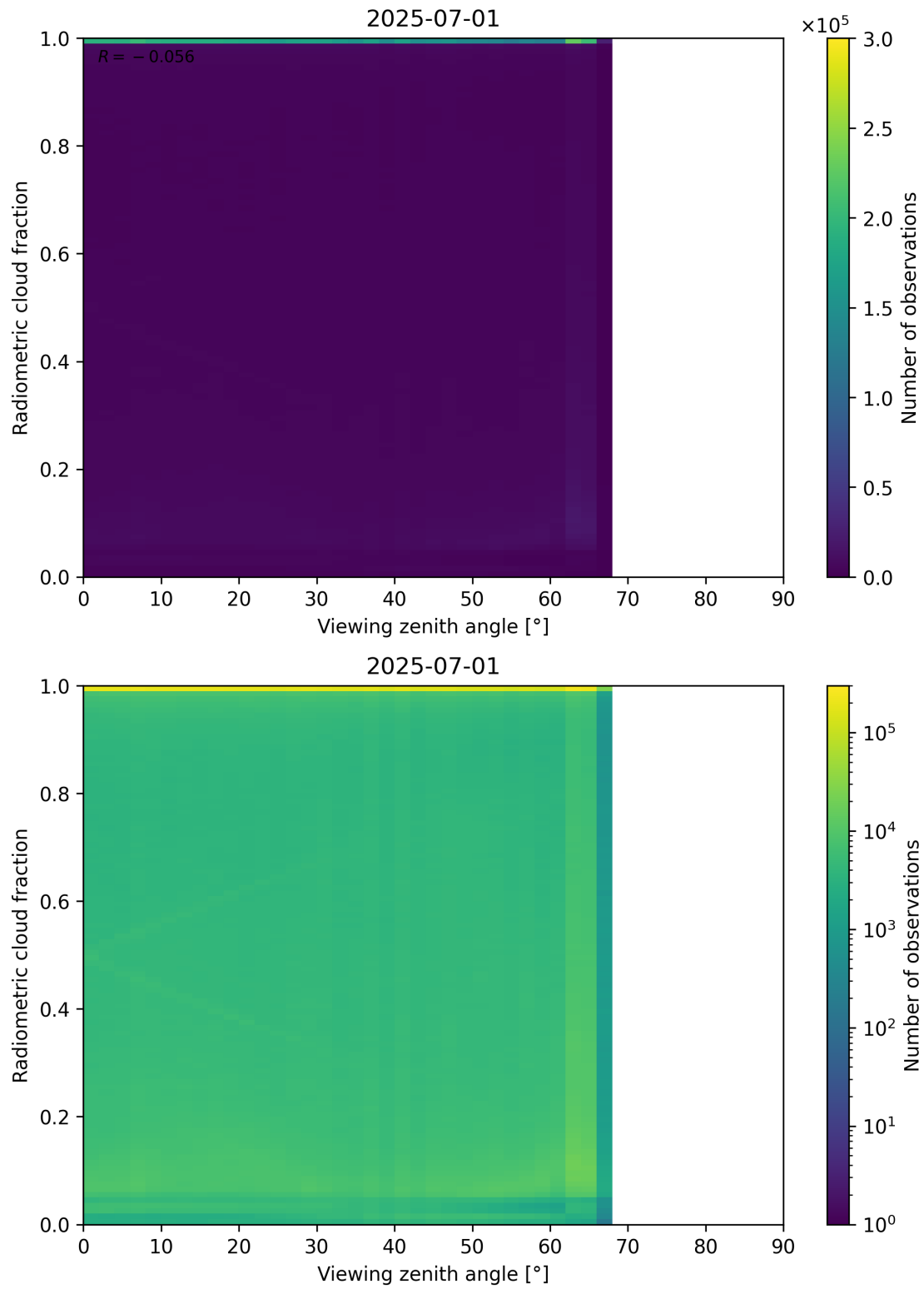
Figure 107: Scatter density plot of “Viewing zenith angle” against “Radiometric cloud fraction” for 2025-06-30 to 2025-07-02.
