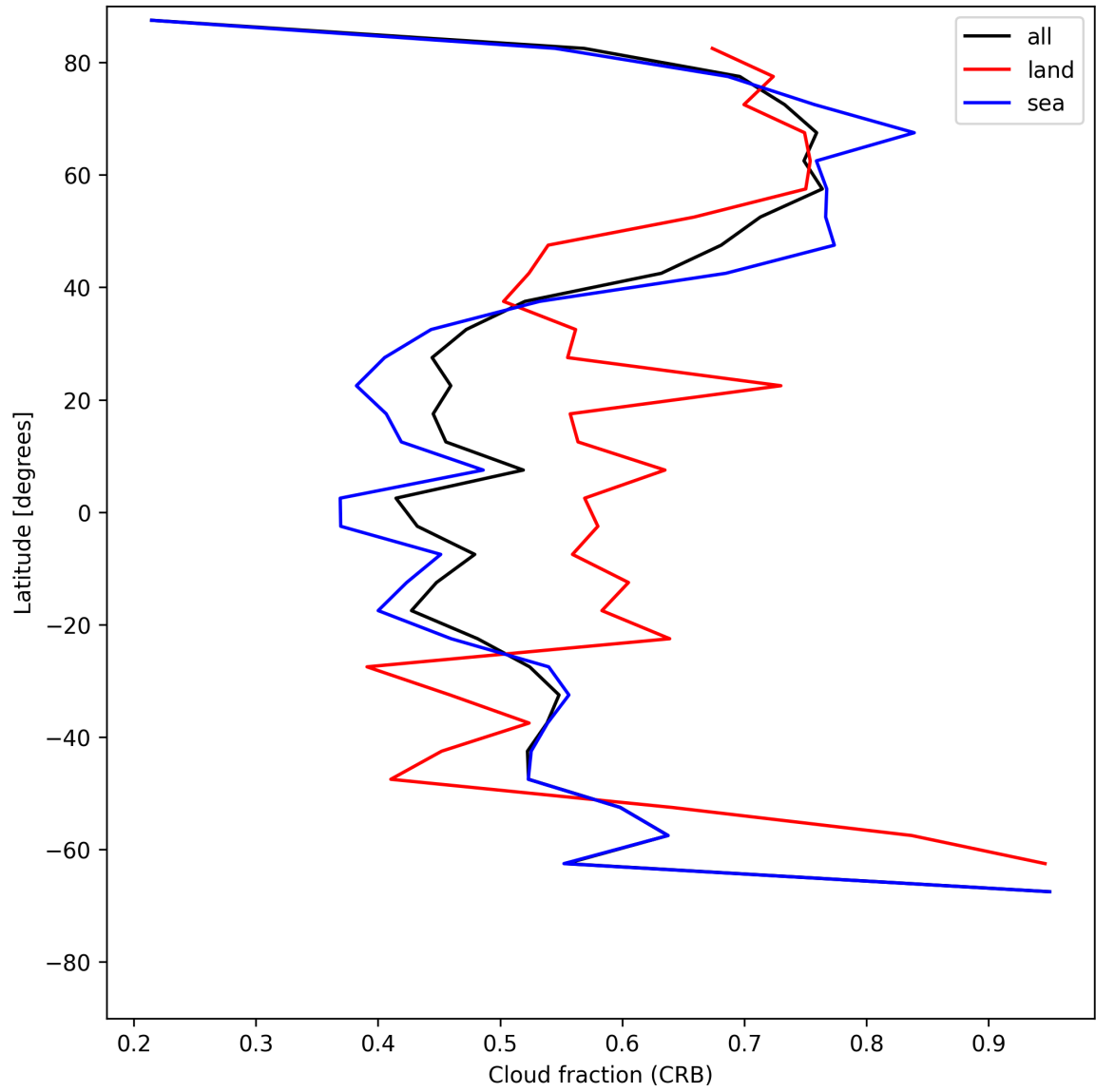
Figure 26: Zonal average of “Cloud fraction (CRB)” for 2025-06-30 to 2025-07-02.
