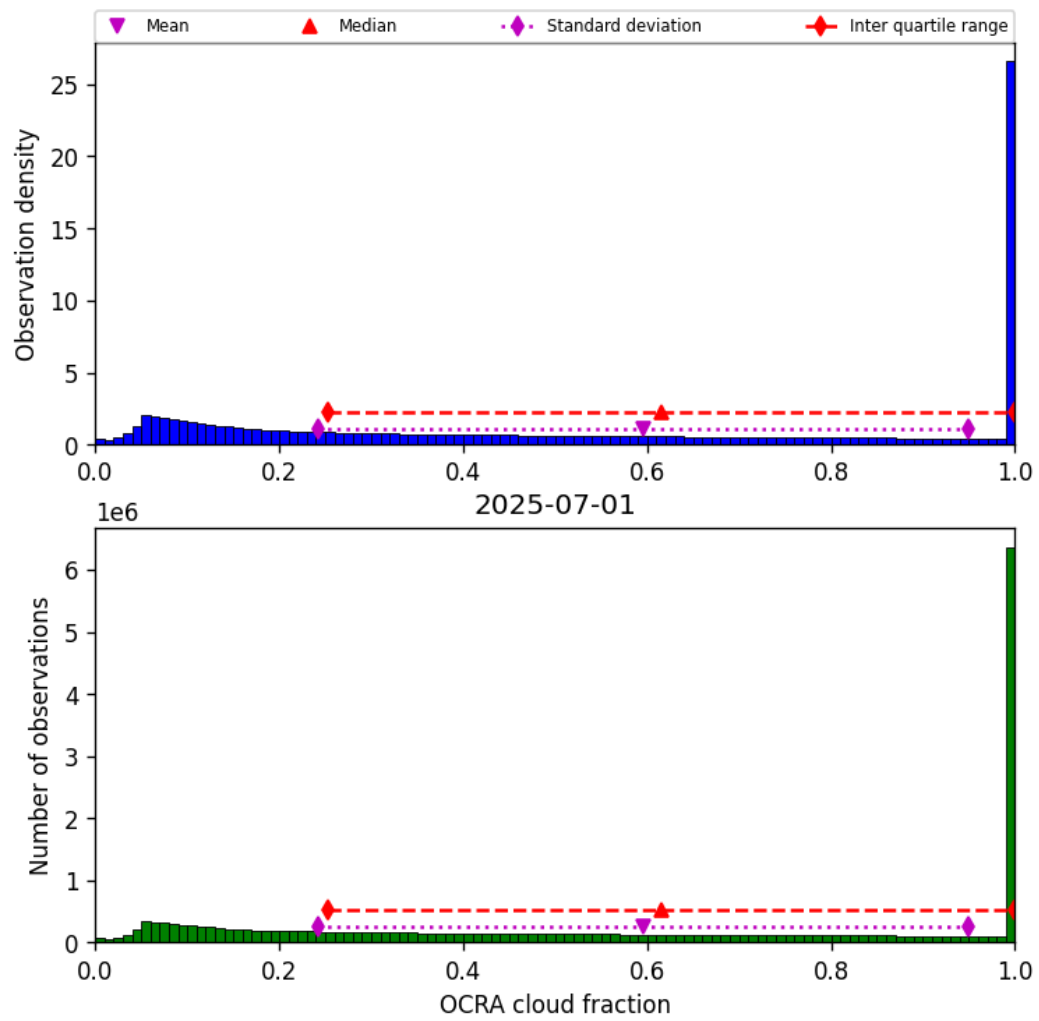
Figure 50: Histogram of “OCRA cloud fraction” for 2025-06-30 to 2025-07-02
