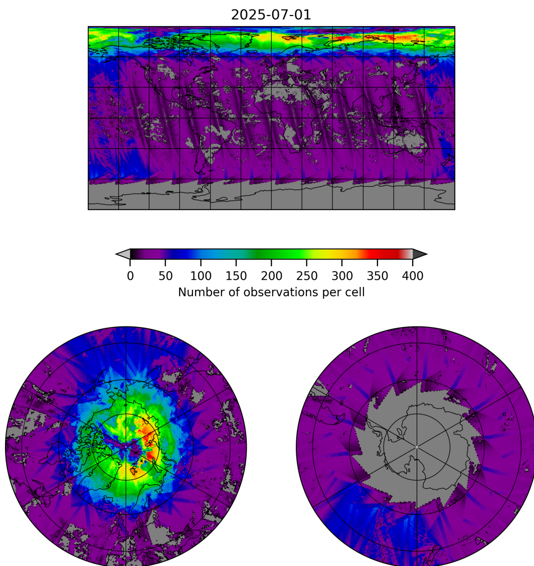
Figure 21: Map of the number of observations for 2025-06-30 to 2025-07-02
