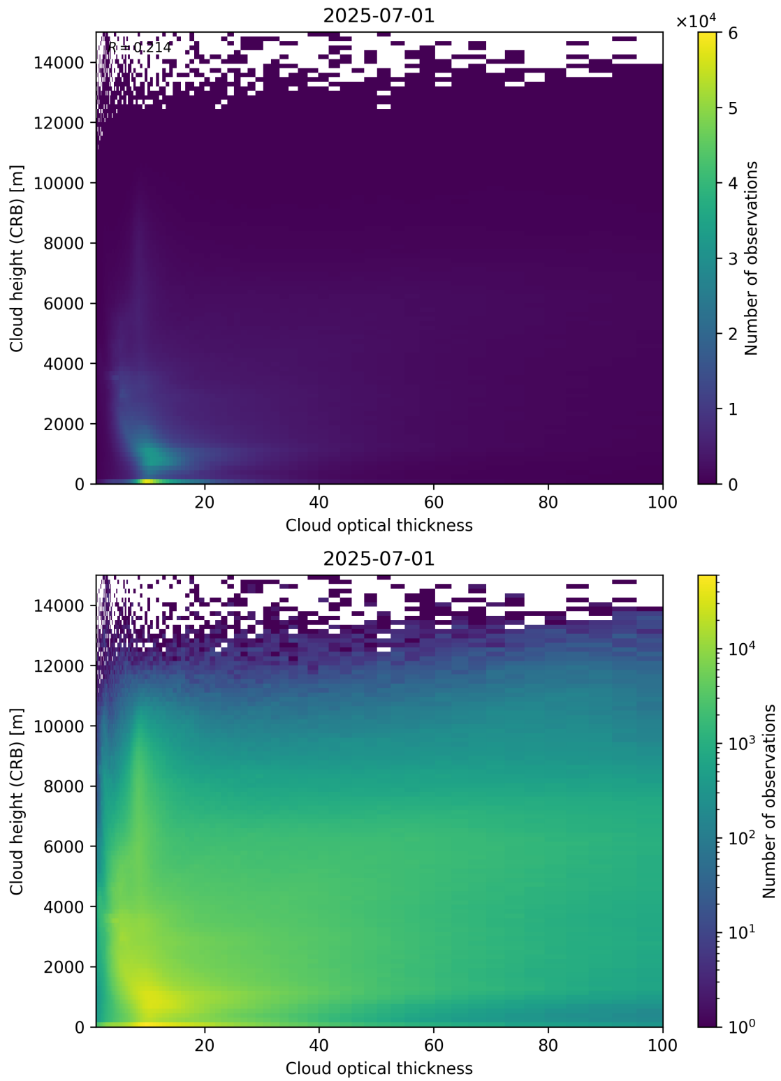
Figure 85: Scatter density plot of “Cloud optical thickness” against “Cloud height (CRB)” for 2025-06-30 to 2025-07-02.
