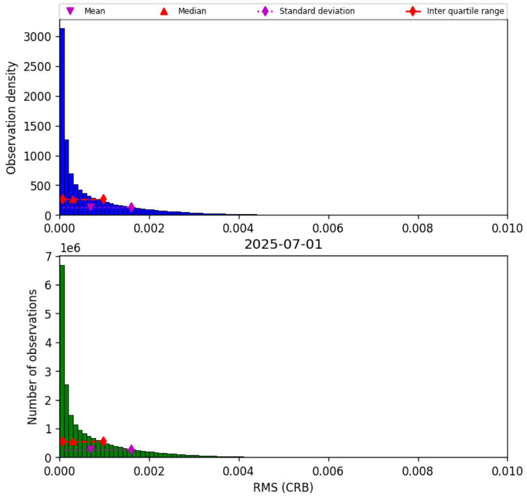
Figure 48: Histogram of “RMS (CRB)” for 2025-06-30 to 2025-07-02
