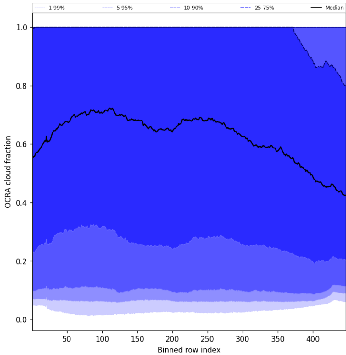
Figure 66: Along track statistics of “OCRA cloud fraction” for 2025-06-30 to 2025-07-02
