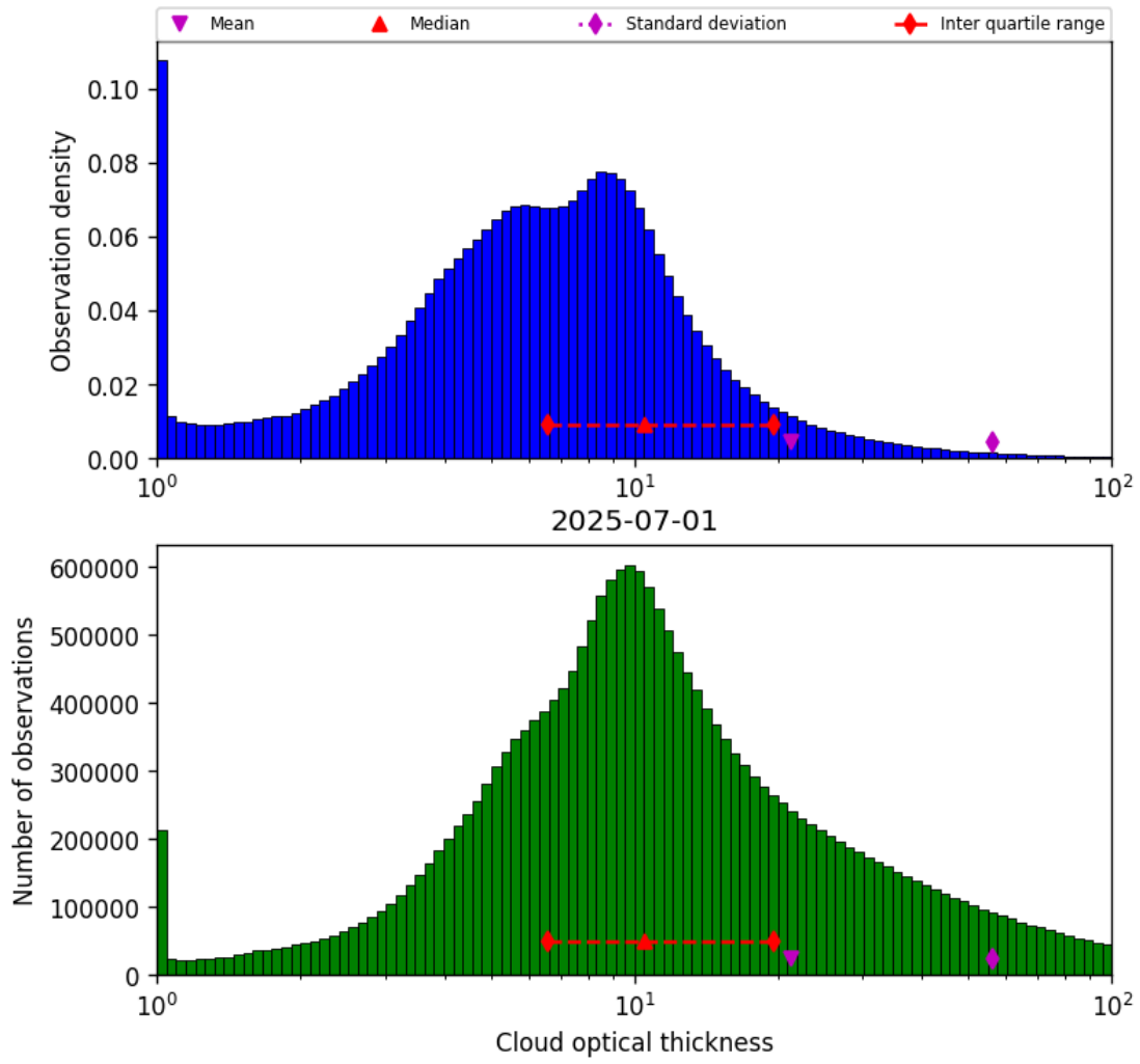
Figure 41: Histogram of “Cloud optical thickness” for 2025-06-30 to 2025-07-02
