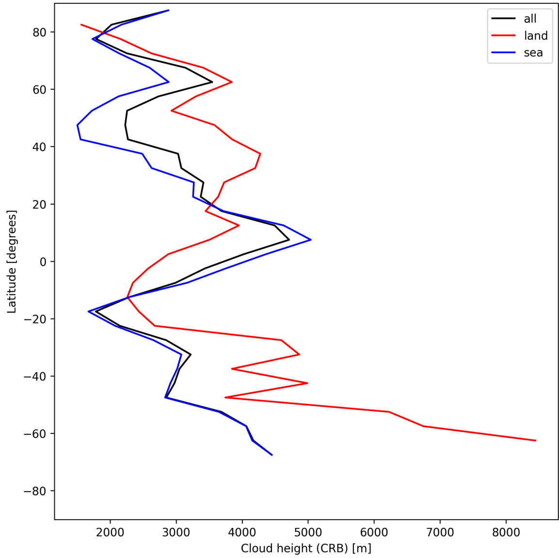
Figure 27: Zonal average of “Cloud height (CRB)” for 2025-06-30 to 2025-07-02.
