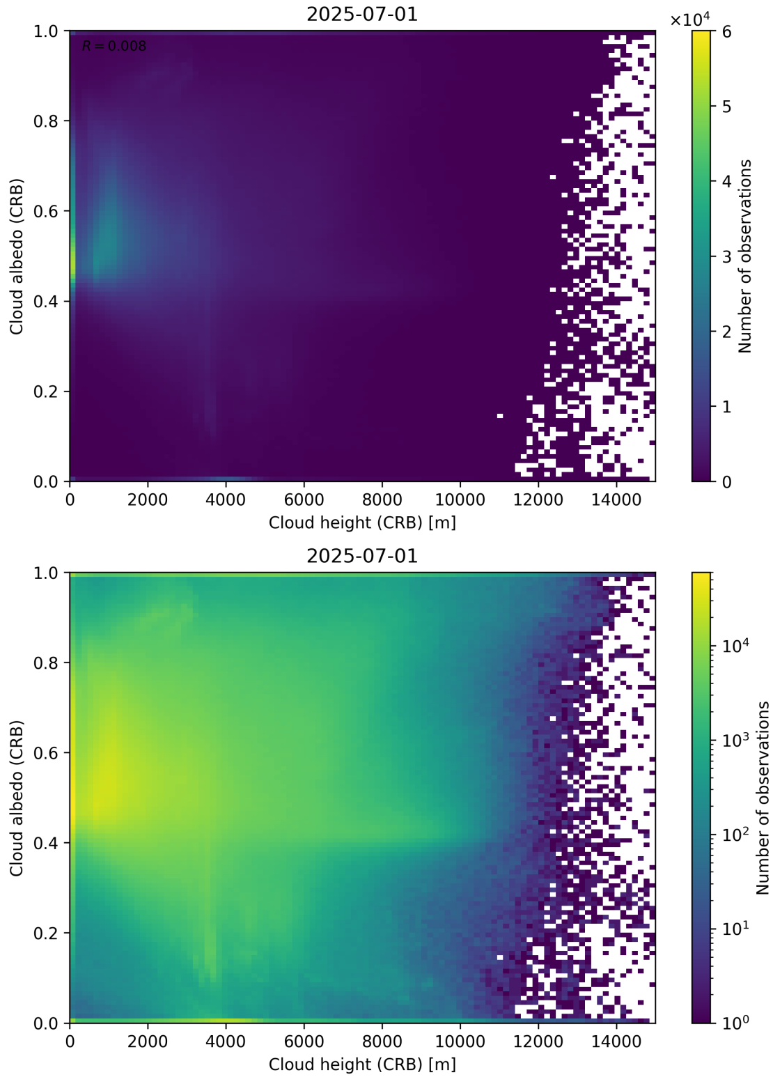
Figure 80: Scatter density plot of “Cloud height (CRB)” against “Cloud albedo (CRB)” for 2025-06-30 to 2025-07-02.
