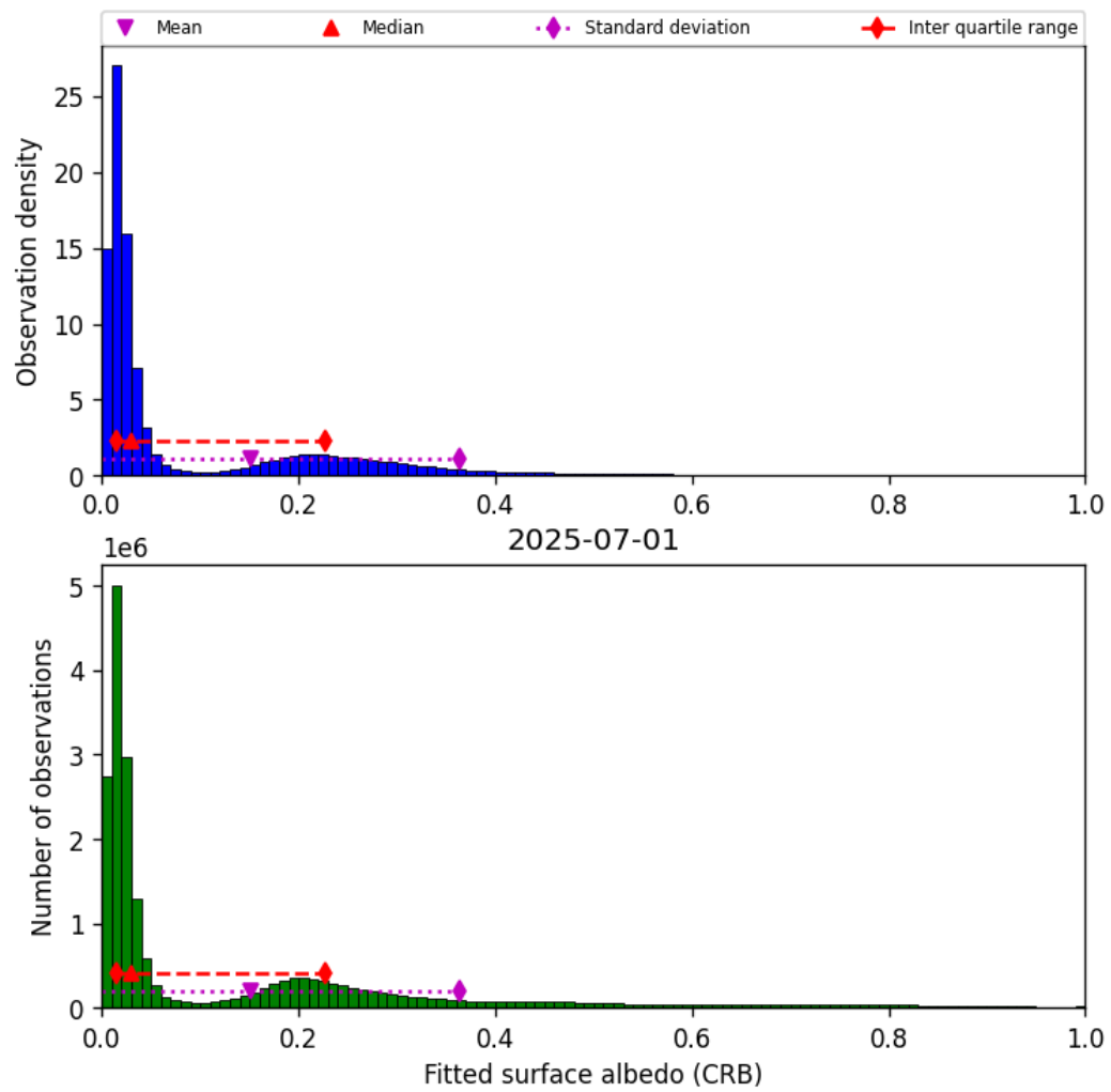
Figure 46: Histogram of “Fitted surface albedo (CRB)” for 2025-06-30 to 2025-07-02
