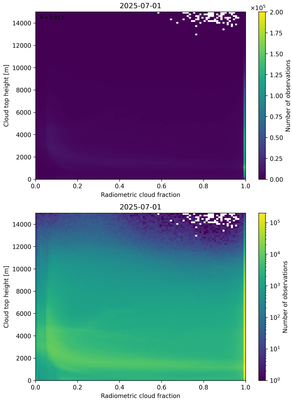
Figure 76: Scatter density plot of “Radiometric cloud fraction” against “Cloud top height” for 2025-06-30 to 2025-07-02.
