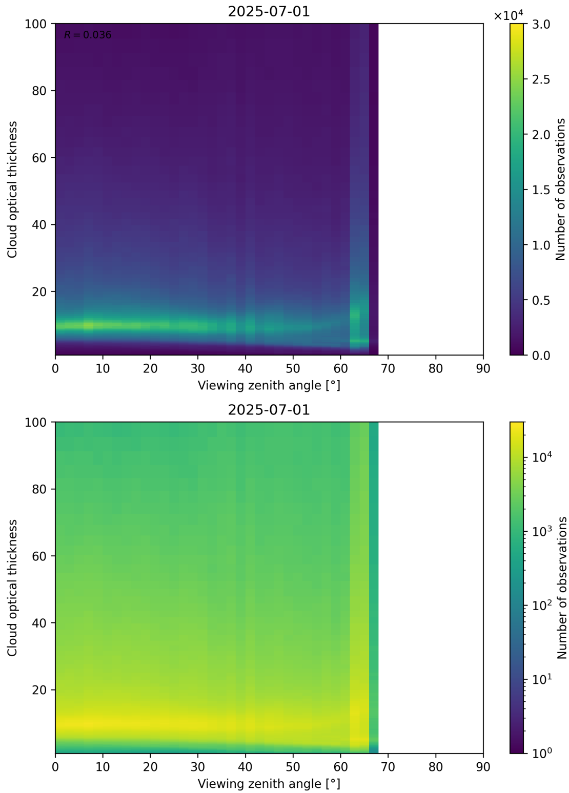
Figure 111: Scatter density plot of “Viewing zenith angle” against “Cloud optical thickness” for 2025-06-30 to 2025-07-02.
