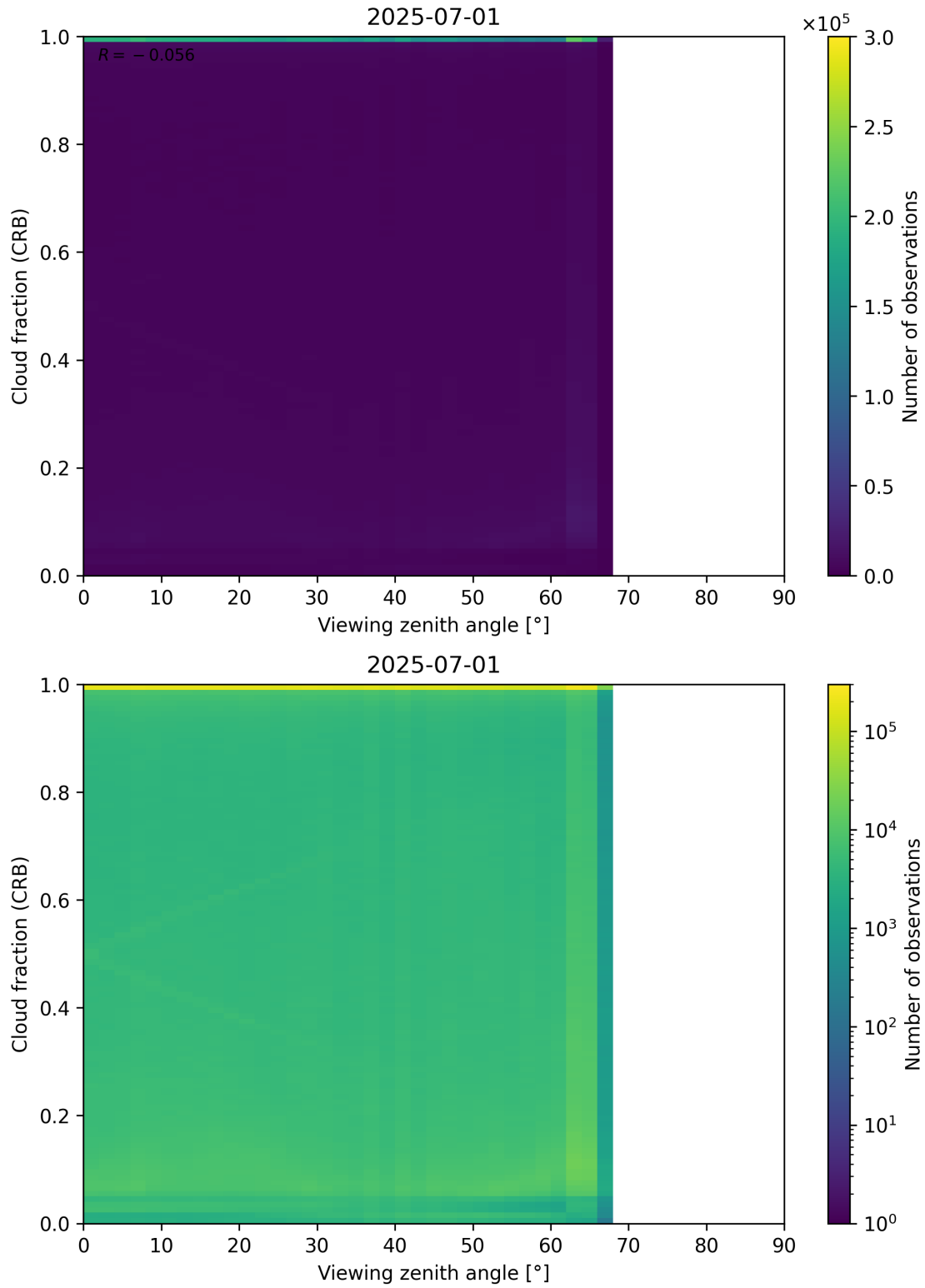
Figure 109: Scatter density plot of “Viewing zenith angle” against “Cloud fraction (CRB)” for 2025-06-30 to 2025-07-02.
