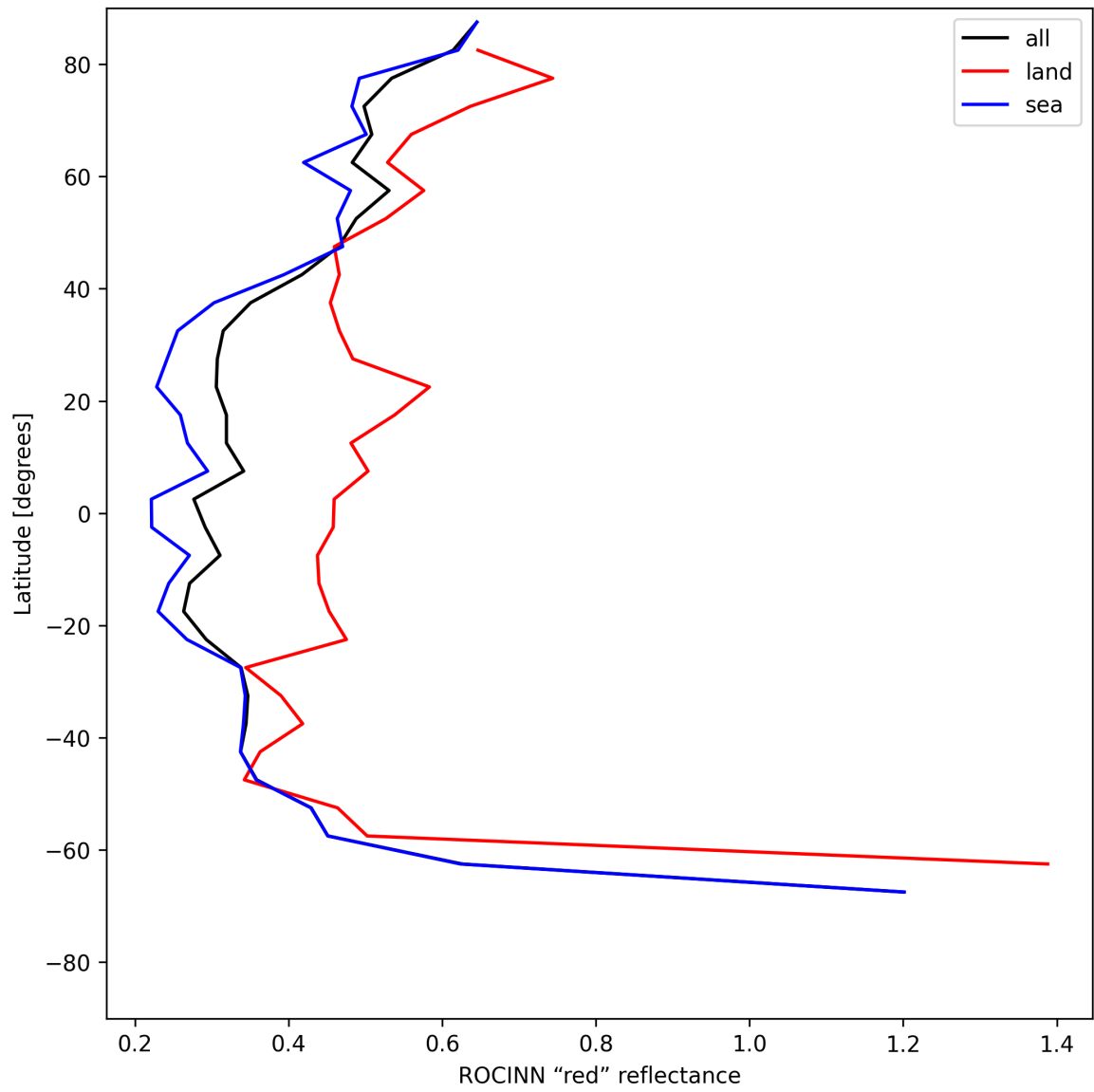
Figure 37: Zonal average of “ROCINN “red” reflectance” for 2025-06-30 to 2025-07-02.
