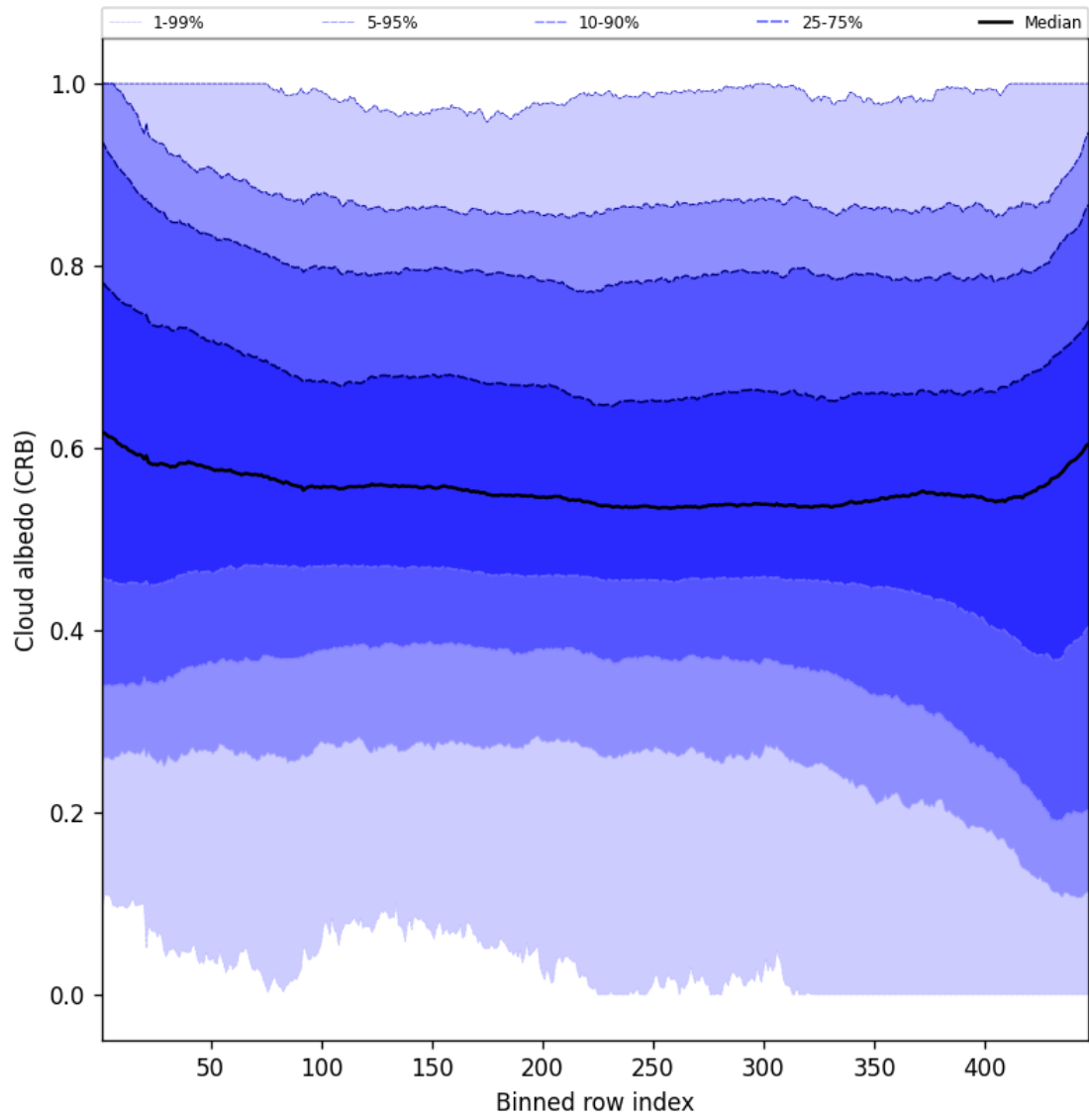
Figure 60: Along track statistics of “Cloud albedo (CRB)” for 2025-06-30 to 2025-07-02
