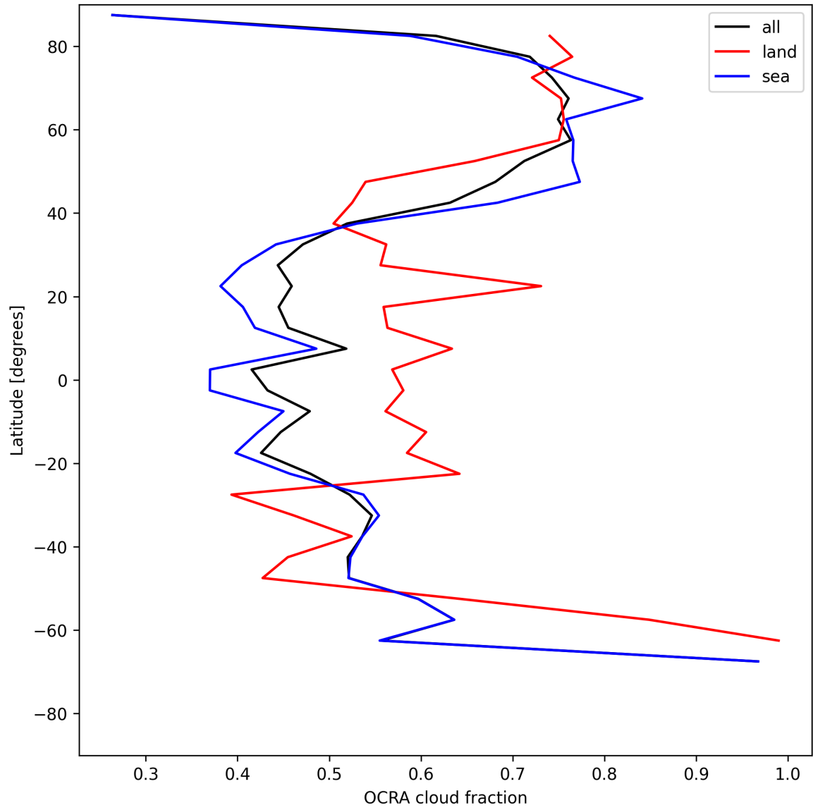
Figure 34: Zonal average of “OCRA cloud fraction” for 2025-06-30 to 2025-07-02.
