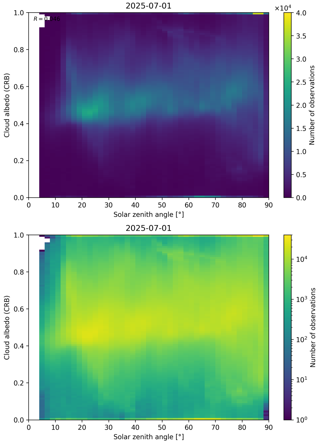
Figure 98: Scatter density plot of “Solar zenith angle” against “Cloud albedo (CRB)” for 2025-06-30 to 2025-07-02.
