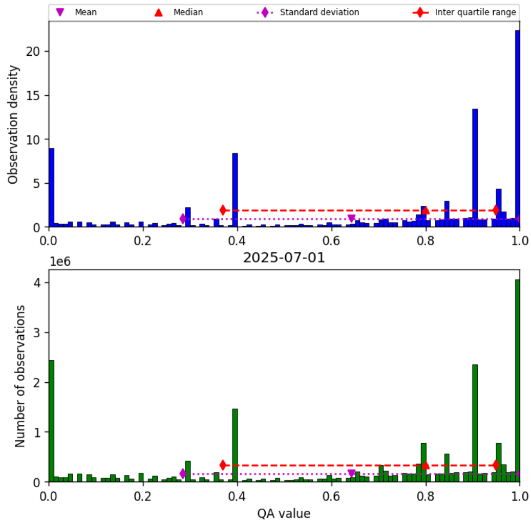
Figure 38: Histogram of “QA value” for 2025-06-30 to 2025-07-02
