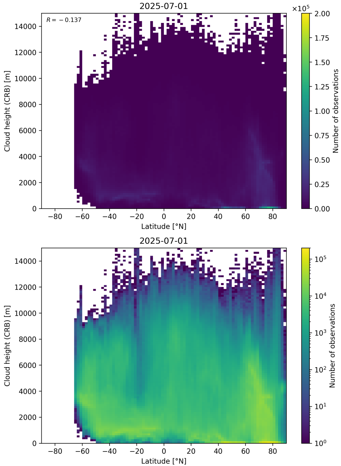
Figure 95: Scatter density plot of “Latitude” against “Cloud height (CRB)” for 2025-06-30 to 2025-07-02.
