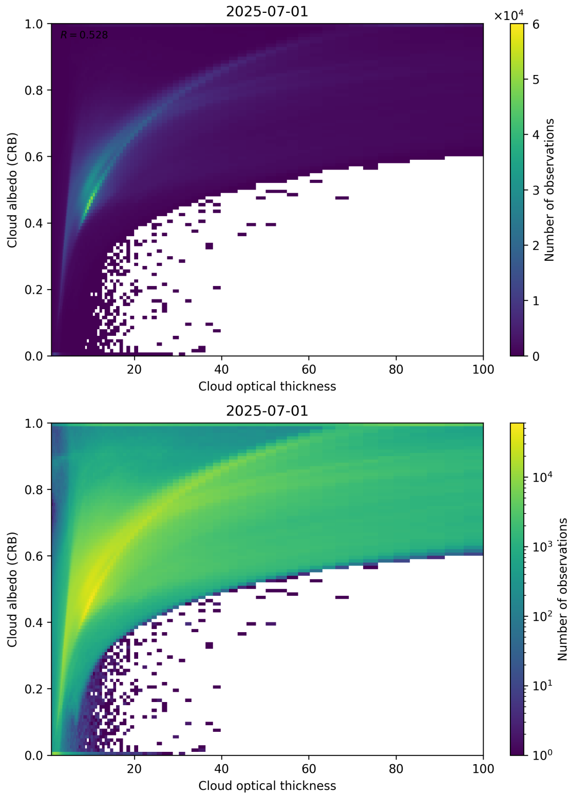
Figure 82: Scatter density plot of “Cloud optical thickness” against “Cloud albedo (CRB)” for 2025-06-30 to 2025-07-02.
