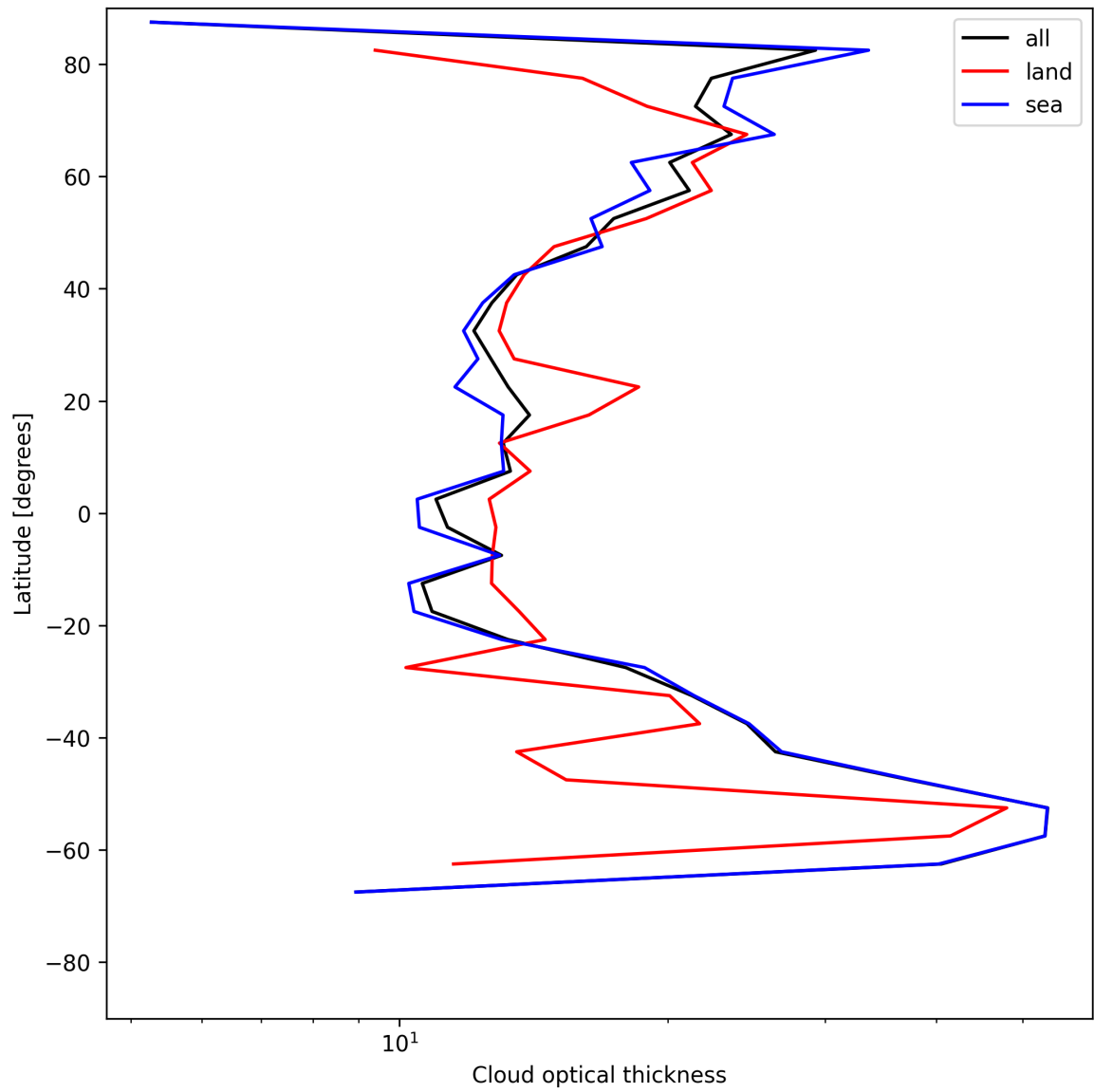
Figure 25: Zonal average of “Cloud optical thickness” for 2025-06-30 to 2025-07-02.
