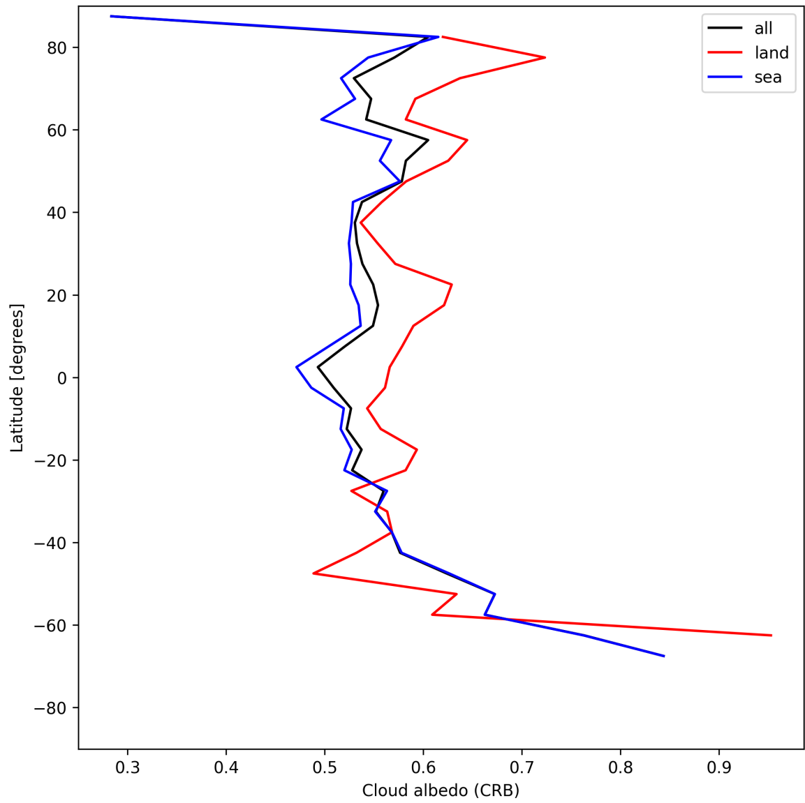
Figure 28: Zonal average of “Cloud albedo (CRB)” for 2025-06-30 to 2025-07-02.
