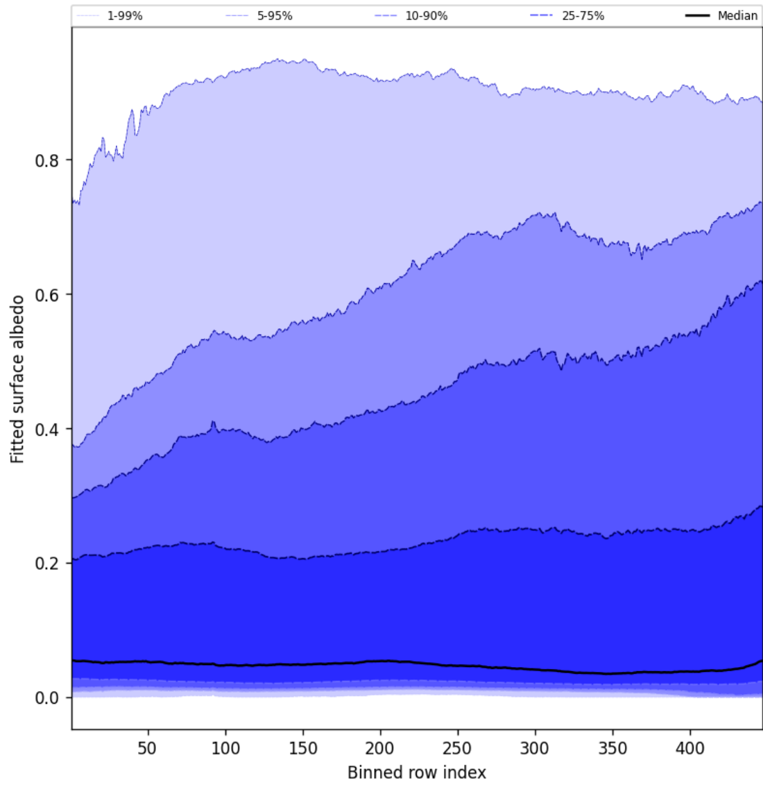
Figure 61: Along track statistics of “Fitted surface albedo” for 2025-06-30 to 2025-07-02
