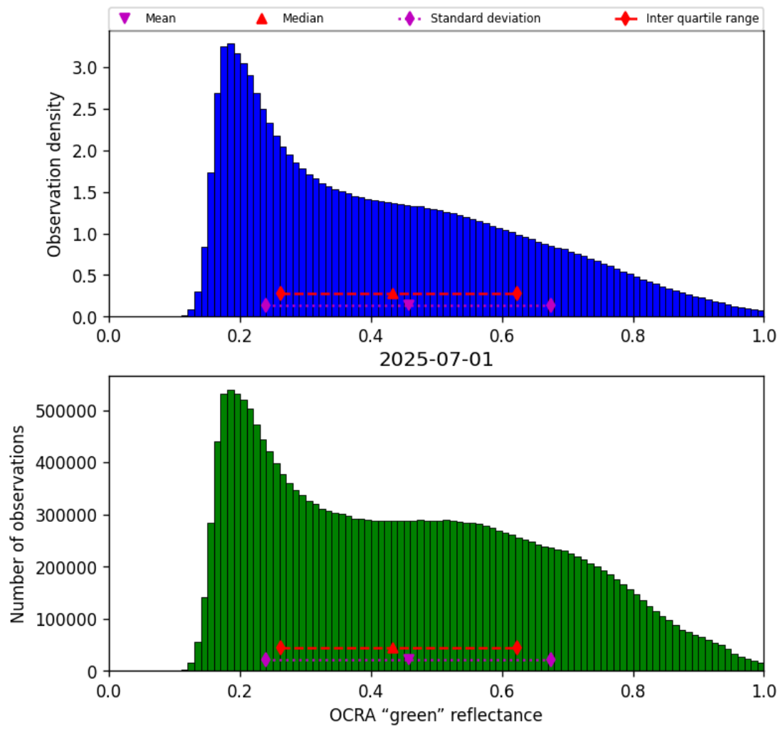
Figure 52: Histogram of “OCRA “green” reflectance” for 2025-06-30 to 2025-07-02
