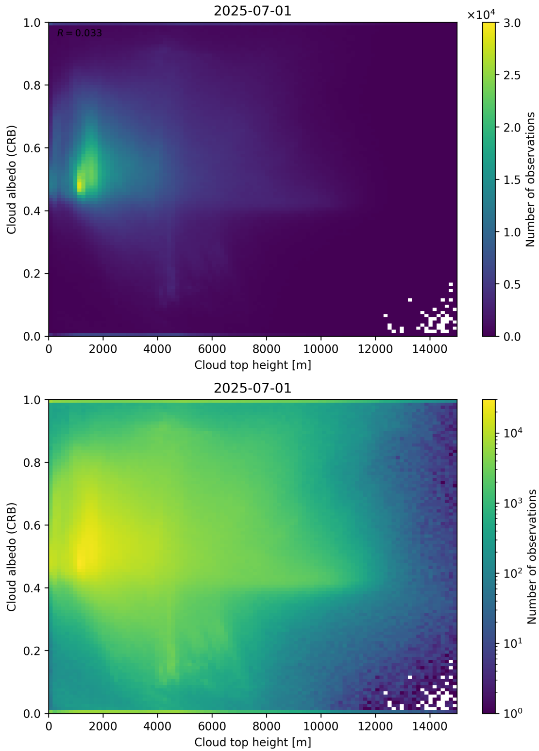
Figure 86: Scatter density plot of “Cloud top height” against “Cloud albedo (CRB)” for 2025-06-30 to 2025-07-02.
