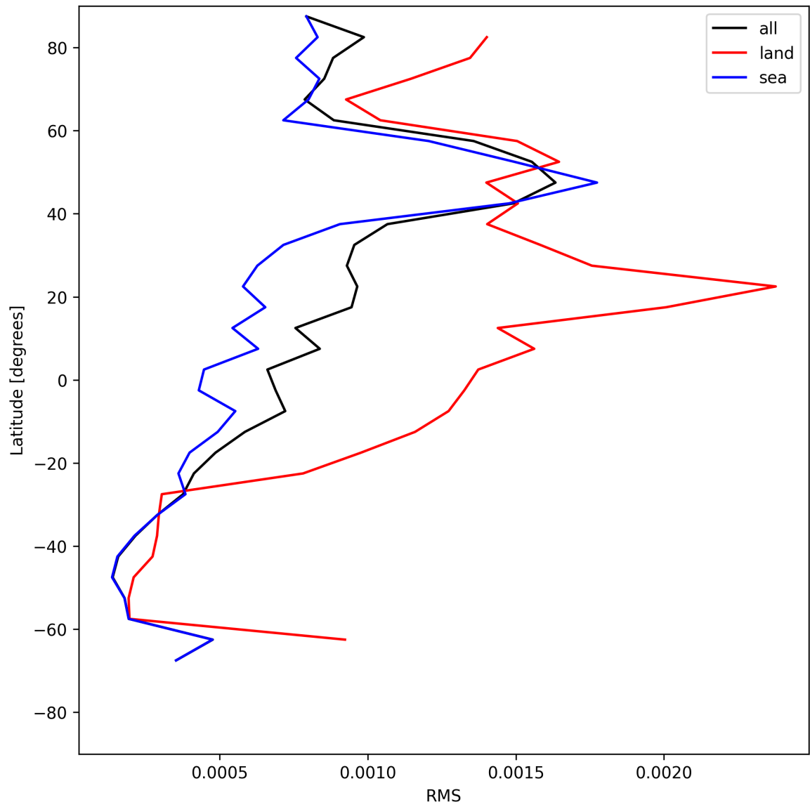
Figure 31: Zonal average of “RMS” for 2025-06-30 to 2025-07-02.
