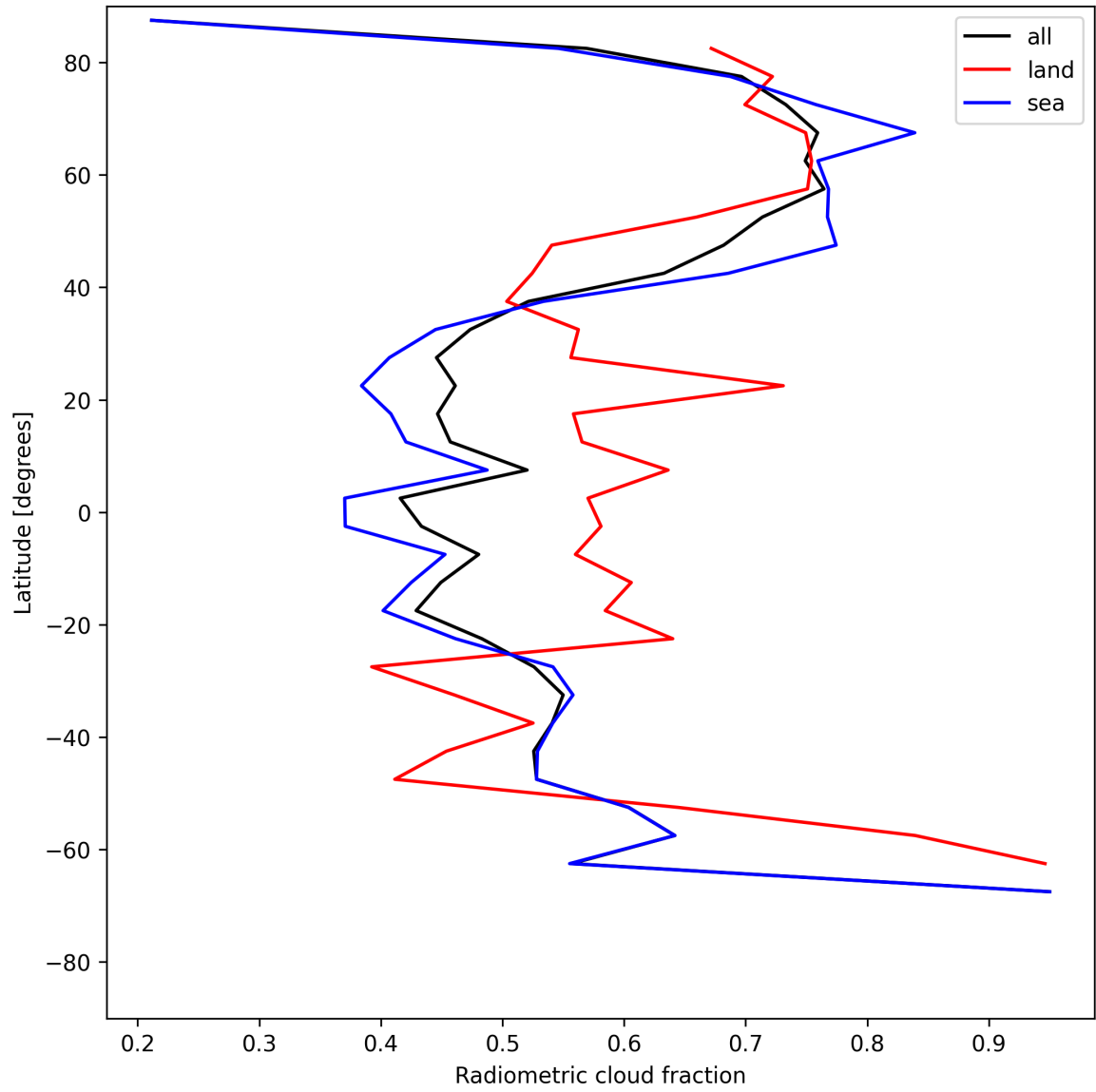
Figure 23: Zonal average of “Radiometric cloud fraction” for 2025-06-30 to 2025-07-02.
