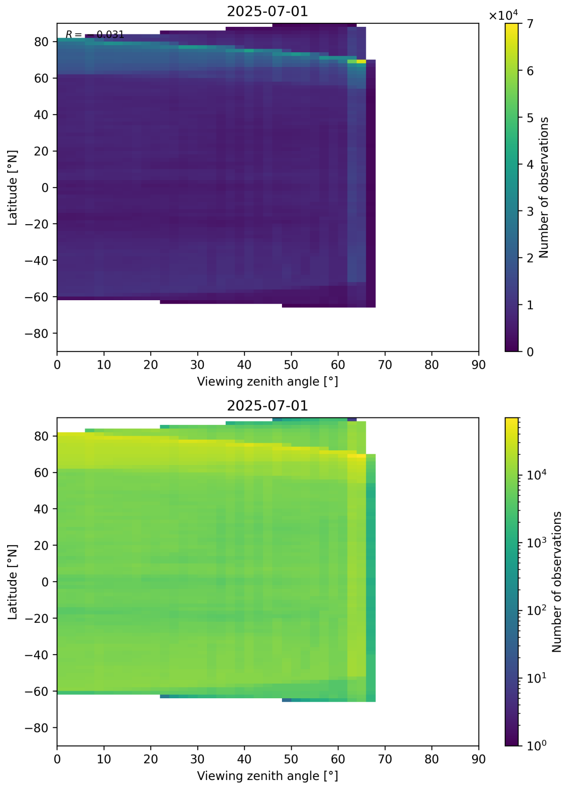
Figure 113: Scatter density plot of “Viewing zenith angle” against “Latitude” for 2025-06-30 to 2025-07-02.
