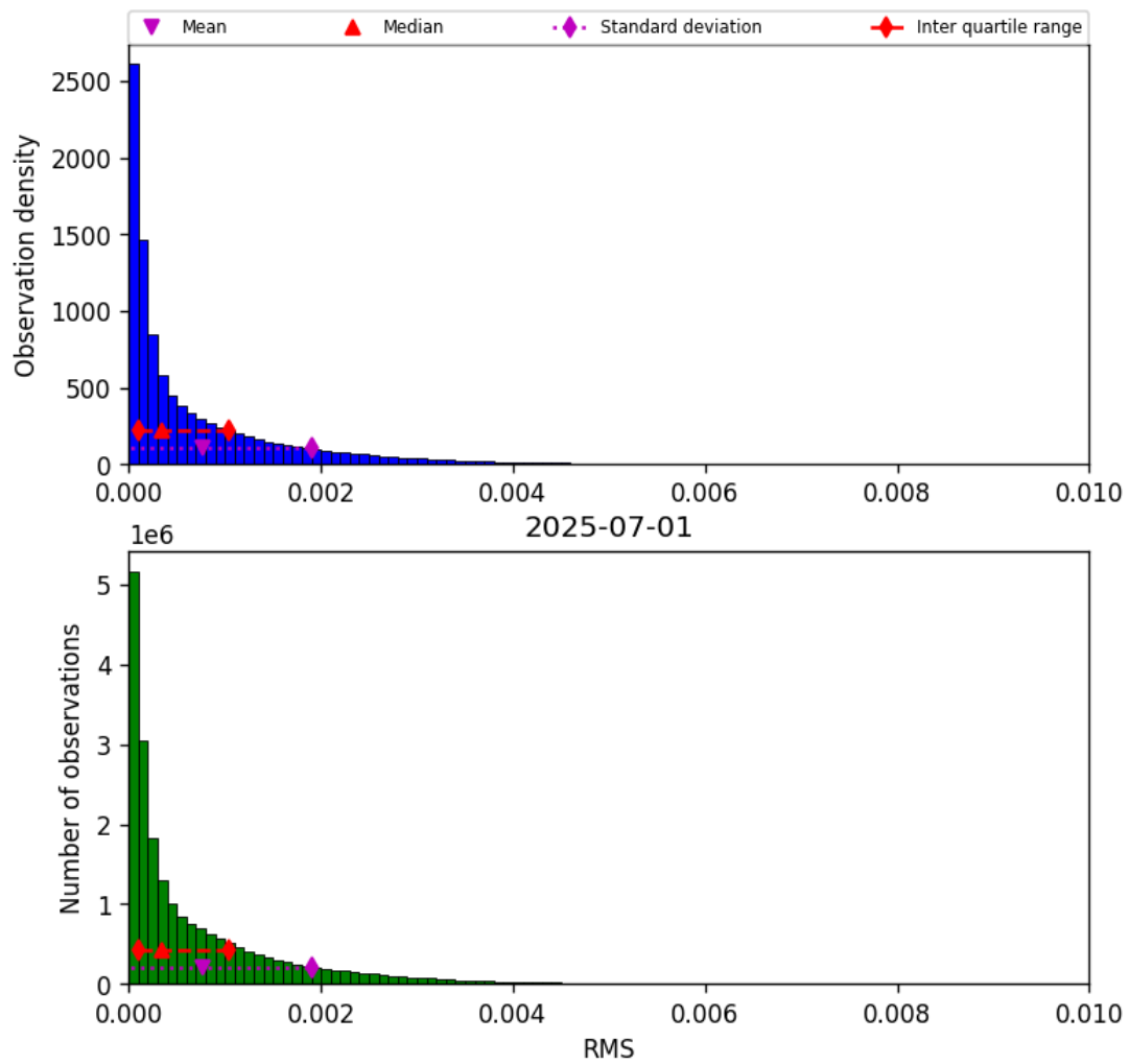
Figure 47: Histogram of “RMS” for 2025-06-30 to 2025-07-02
