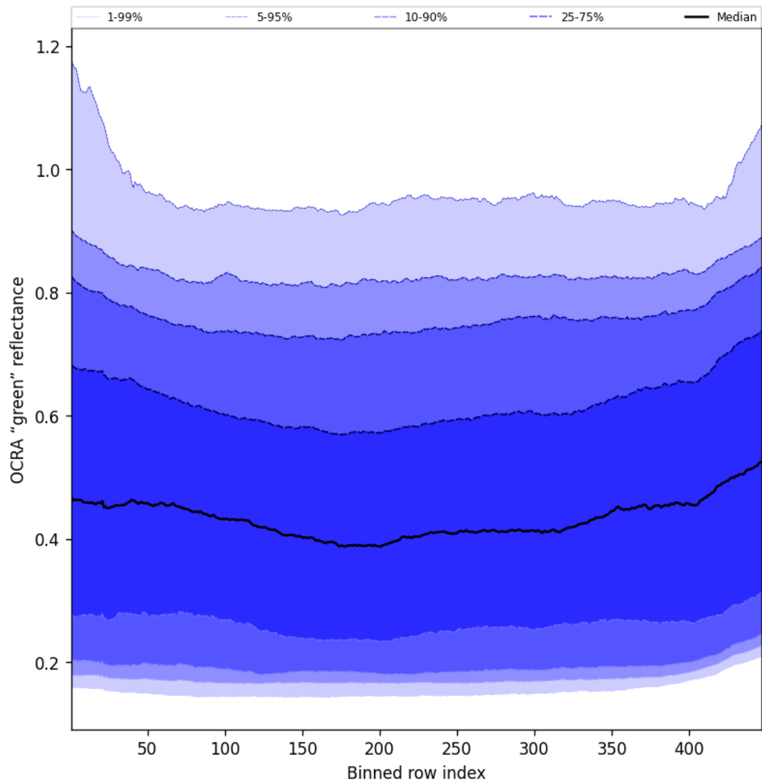
Figure 68: Along track statistics of "OCRA "green" reflectance" for 2025-06-30 to 2025-07-02
