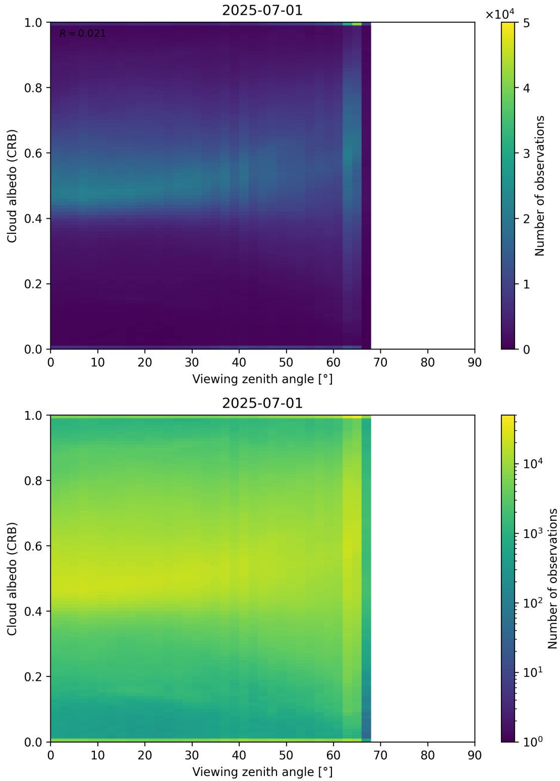
Figure 106: Scatter density plot of “Viewing zenith angle” against “Cloud albedo (CRB)” for 2025-06-30 to 2025-07-02.
