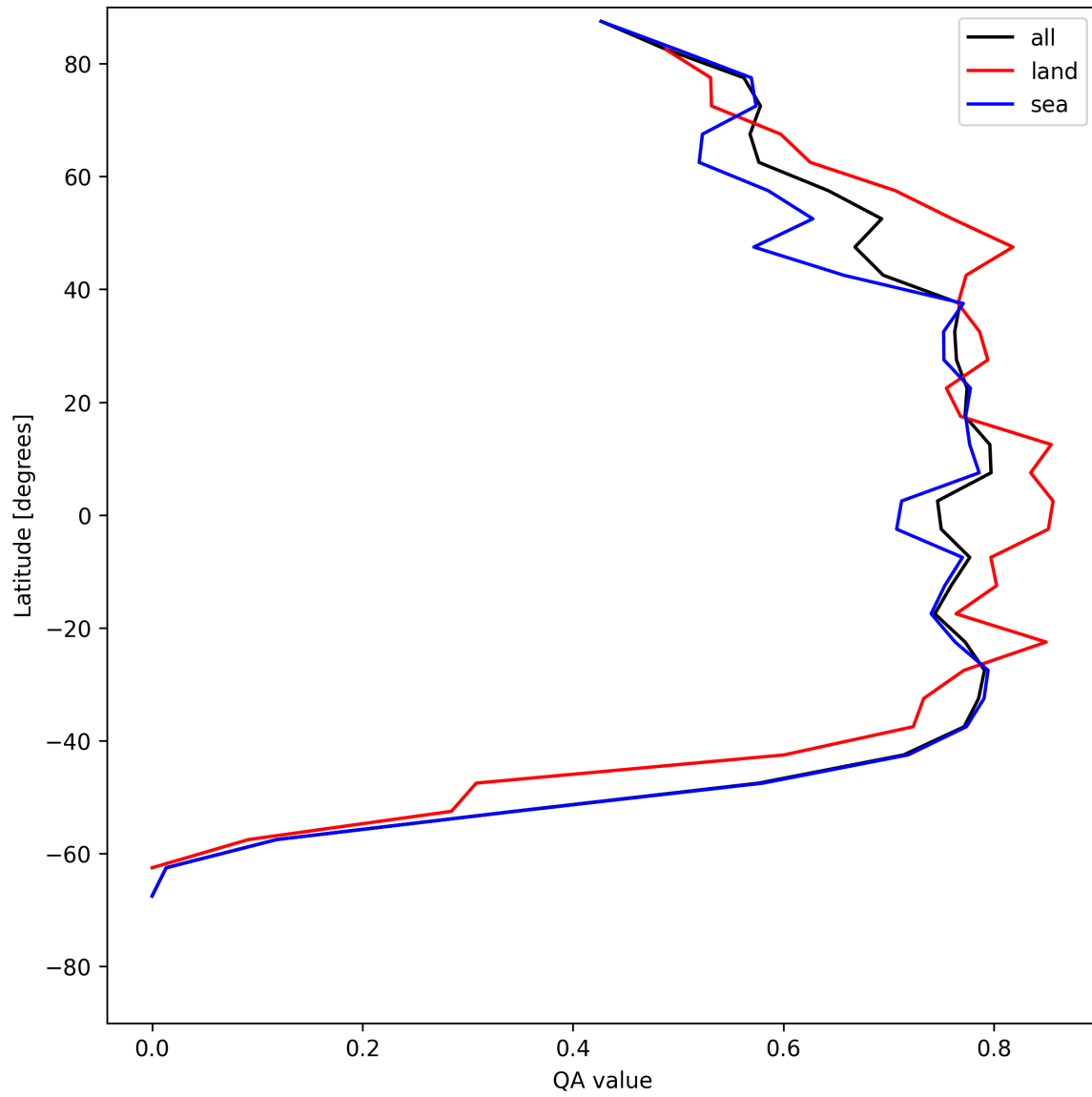
Figure 22: Zonal average of “QA value” for 2025-06-30 to 2025-07-02.
