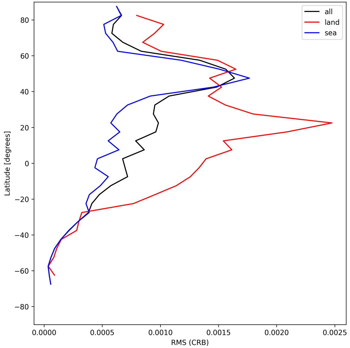
Figure 32: Zonal average of “RMS (CRB)” for 2025-06-30 to 2025-07-02.
