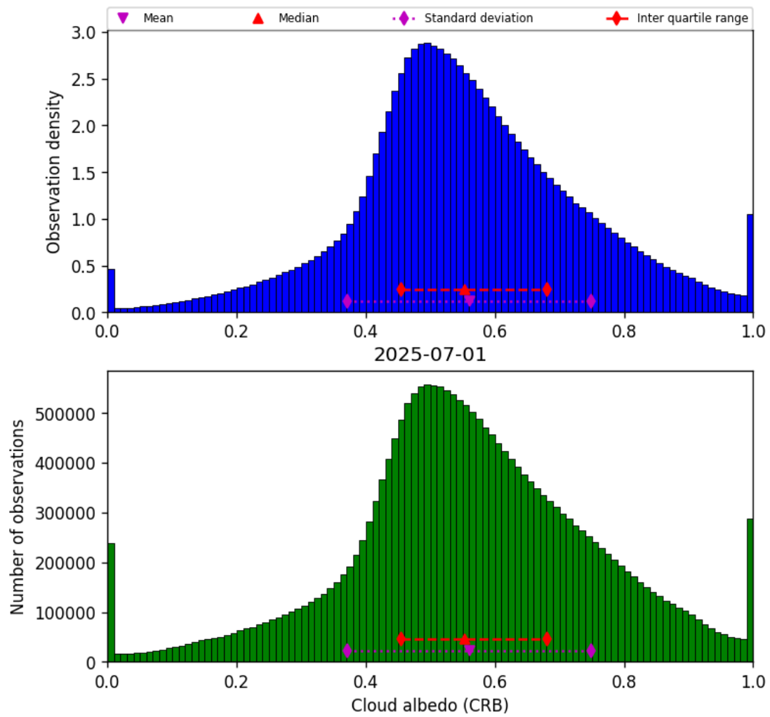
Figure 44: Histogram of “Cloud albedo (CRB)” for 2025-06-30 to 2025-07-02
