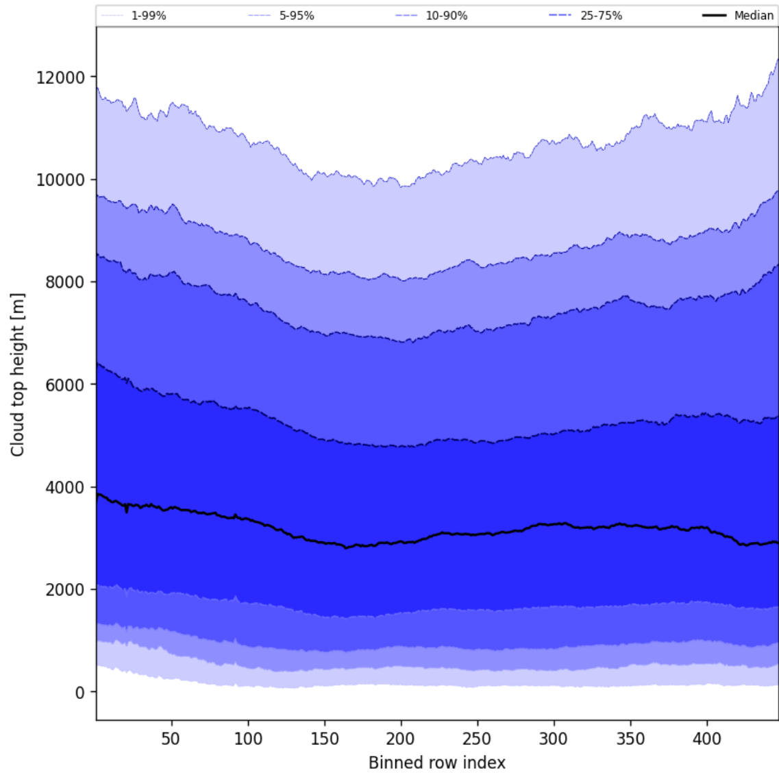
Figure 56: Along track statistics of “Cloud top height” for 2025-06-30 to 2025-07-02
