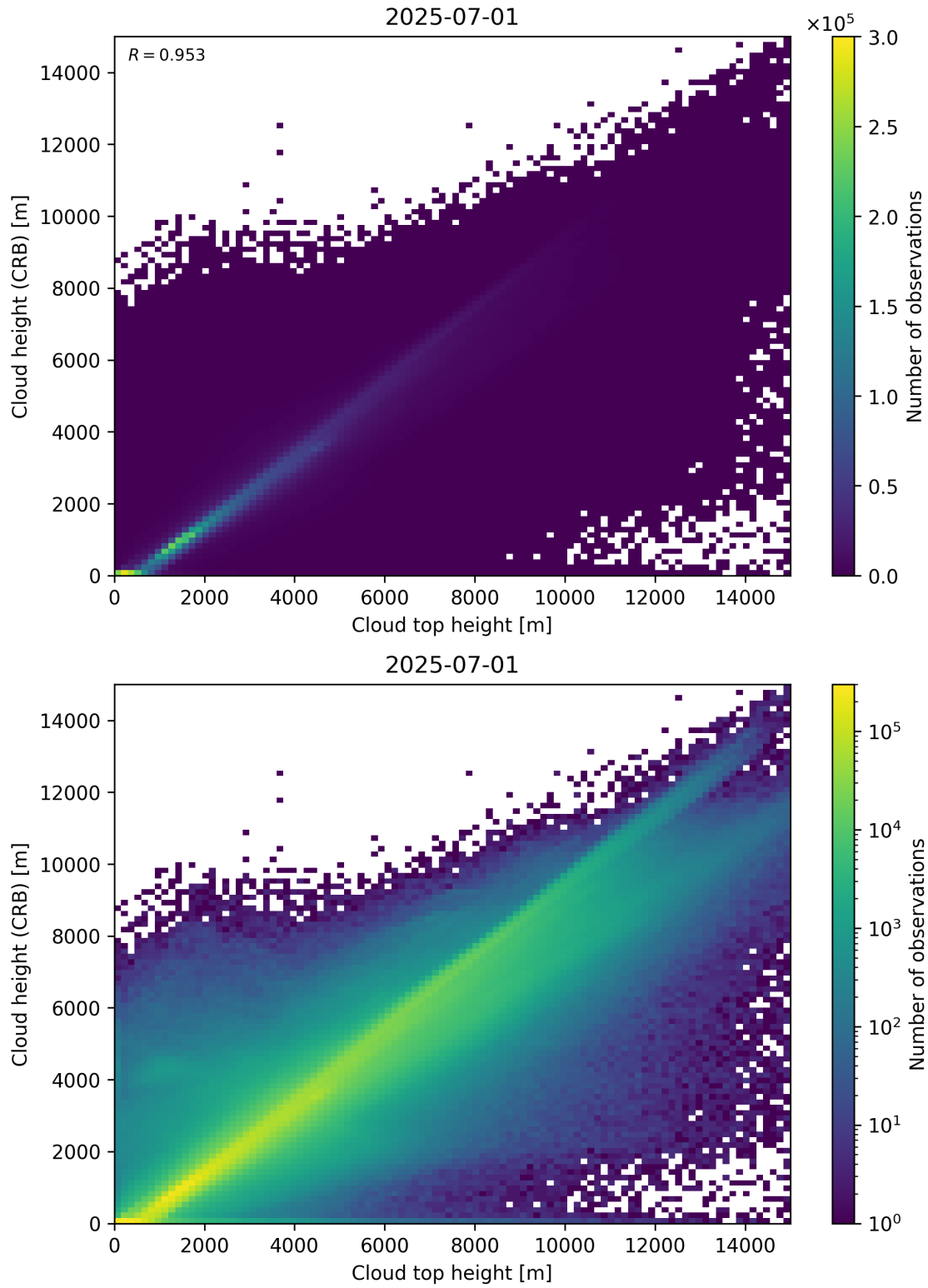
Figure 89: Scatter density plot of “Cloud top height” against “Cloud height (CRB)” for 2025-06-30 to 2025-07-02.
