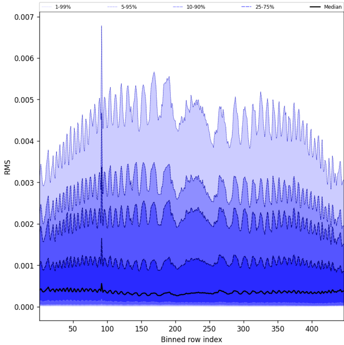
Figure 63: Along track statistics of “RMS” for 2025-06-30 to 2025-07-02
