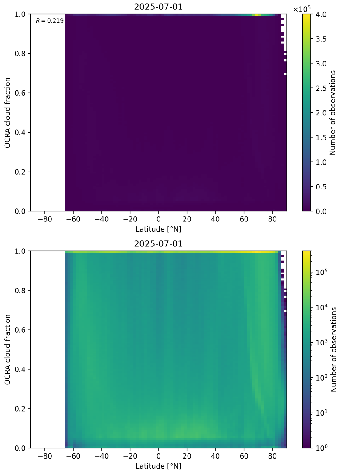
Figure 93: Scatter density plot of “Latitude” against “OCRA cloud fraction” for 2025-06-30 to 2025-07-02.
