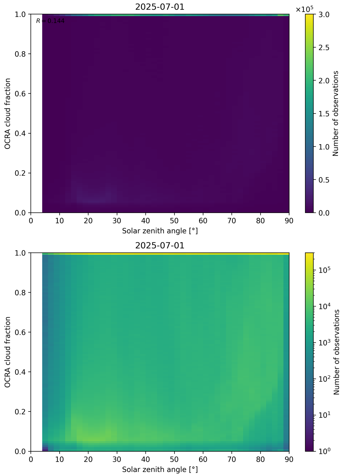
Figure 100: Scatter density plot of “Solar zenith angle” against “OCRA cloud fraction” for 2025-06-30 to 2025-07-02.
