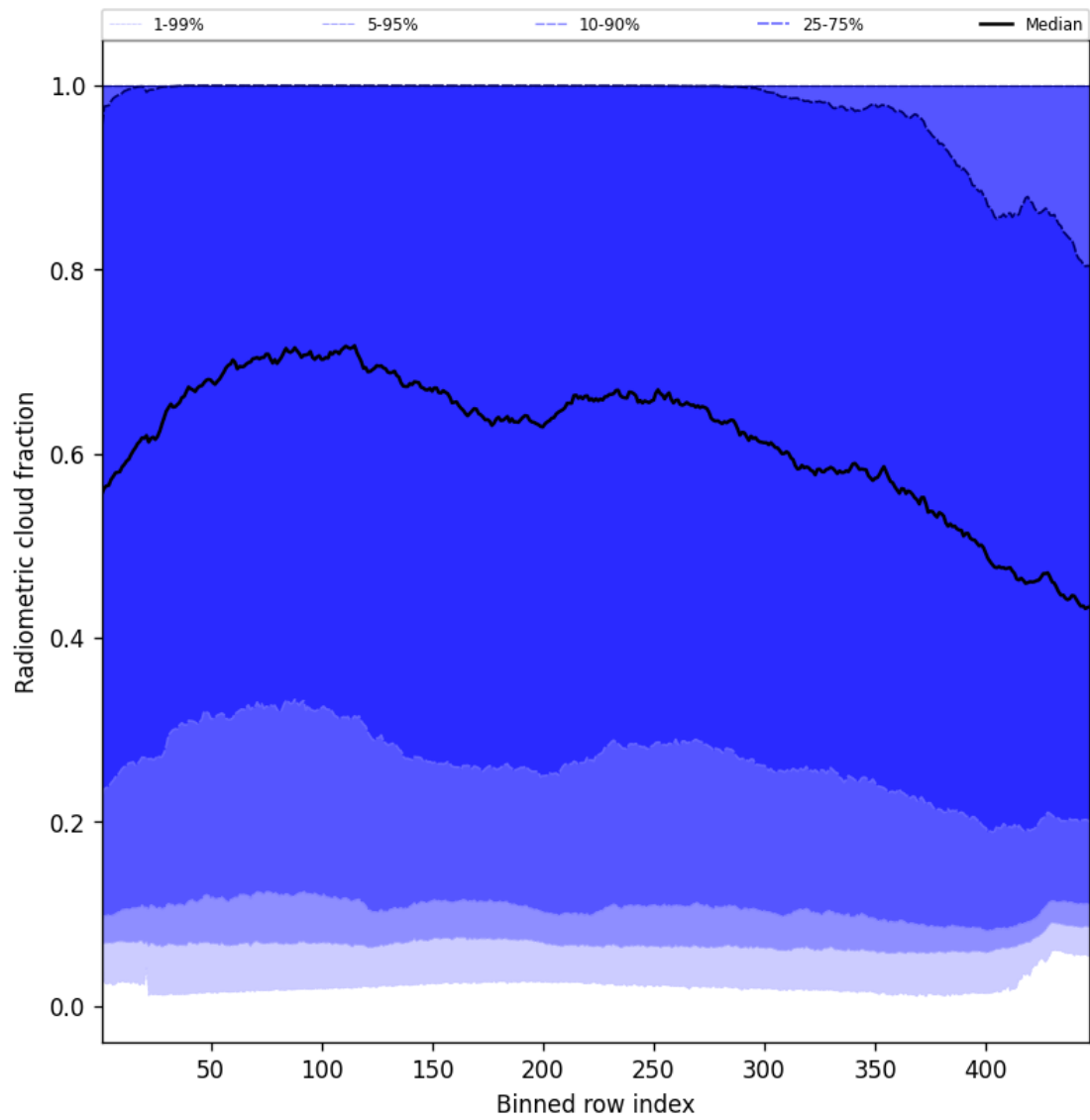
Figure 55: Along track statistics of “Radiometric cloud fraction” for 2025-06-30 to 2025-07-02
