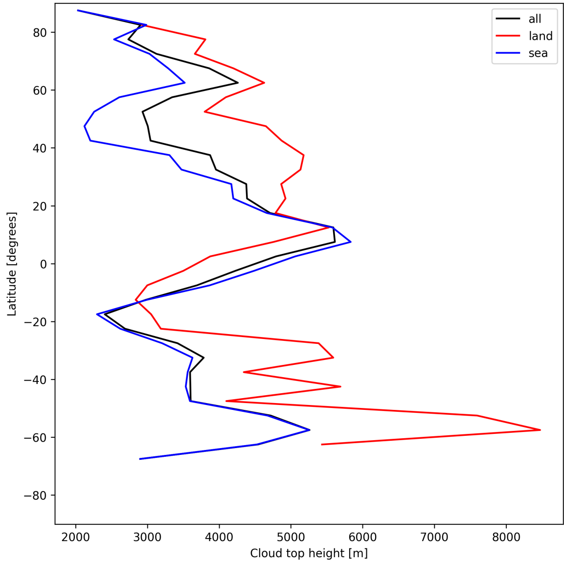
Figure 24: Zonal average of “Cloud top height” for 2025-06-30 to 2025-07-02.
