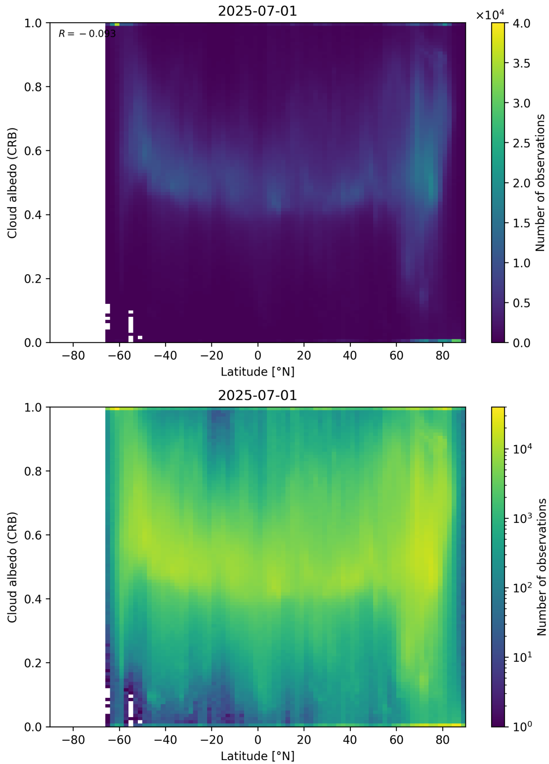
Figure 91: Scatter density plot of “Latitude” against “Cloud albedo (CRB)” for 2025-06-30 to 2025-07-02.
