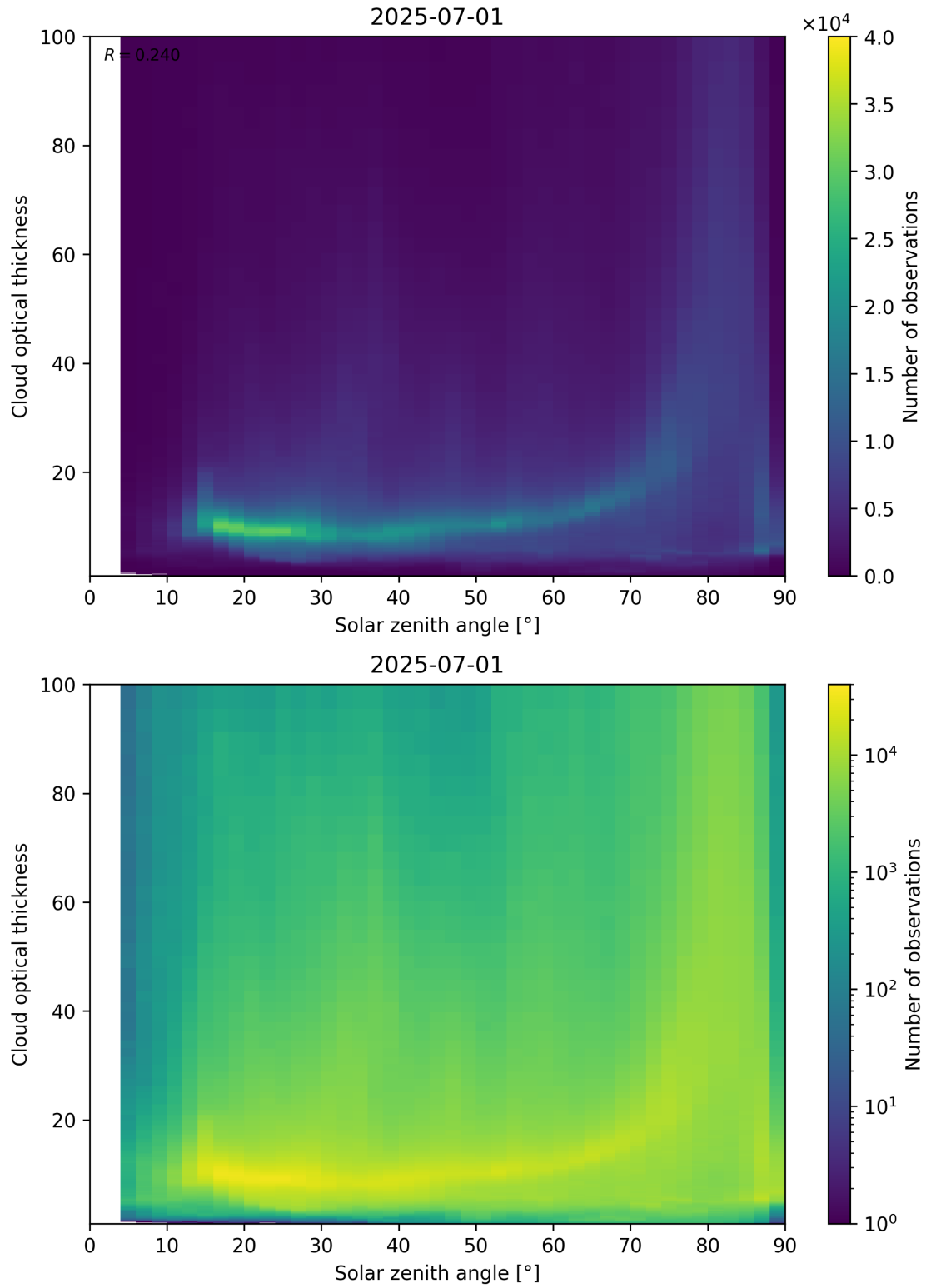
Figure 103: Scatter density plot of “Solar zenith angle” against “Cloud optical thickness” for 2025-06-30 to 2025-07-02.
