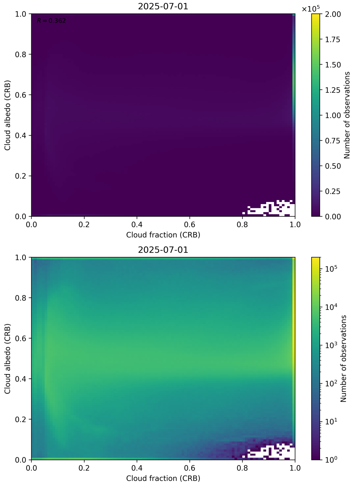
Figure 77: Scatter density plot of “Cloud fraction (CRB)” against “Cloud albedo (CRB)” for 2025-06-30 to 2025-07-02.
