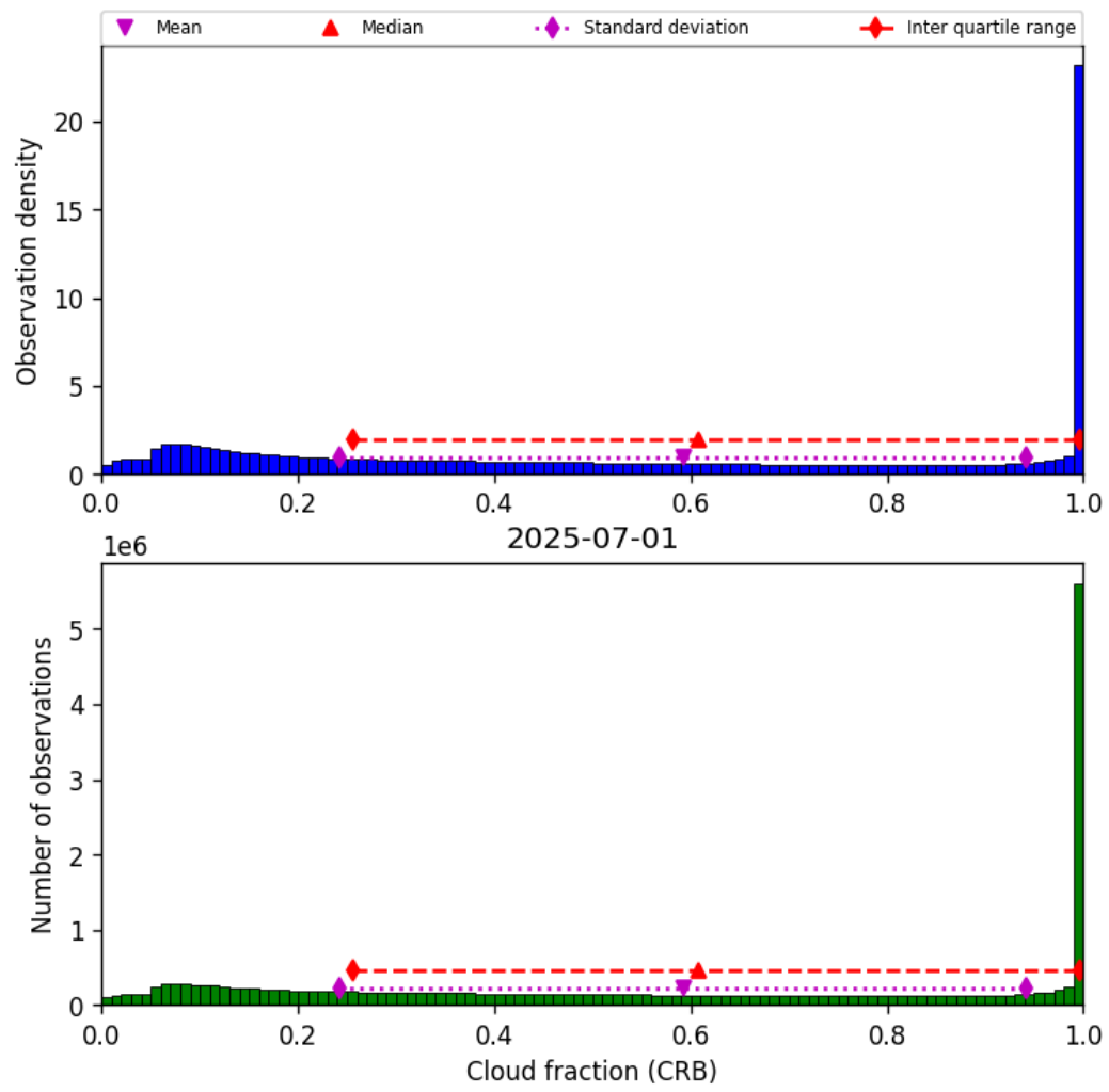
Figure 42: Histogram of “Cloud fraction (CRB)” for 2025-06-30 to 2025-07-02
