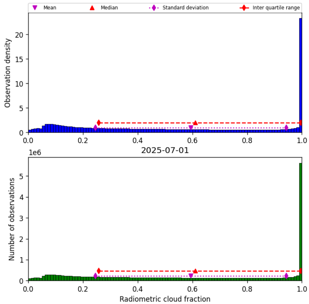
Figure 39: Histogram of “Radiometric cloud fraction” for 2025-06-30 to 2025-07-02
