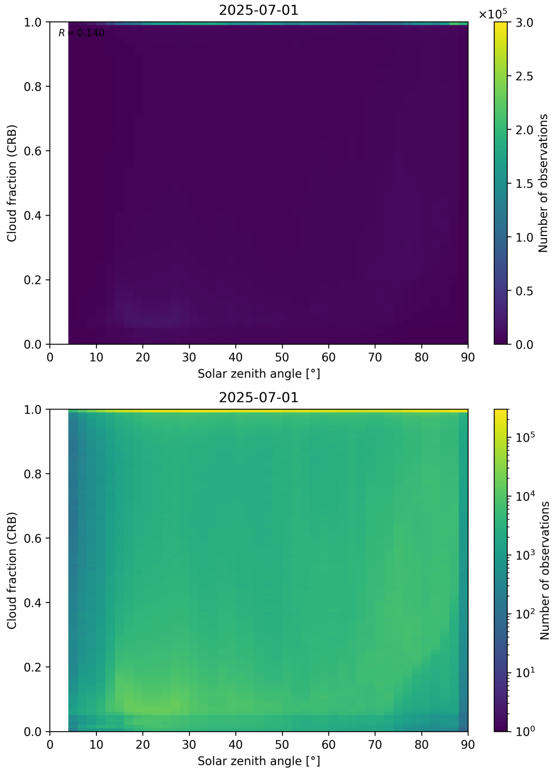
Figure 101: Scatter density plot of “Solar zenith angle” against “Cloud fraction (CRB)” for 2025-06-30 to 2025-07-02.
