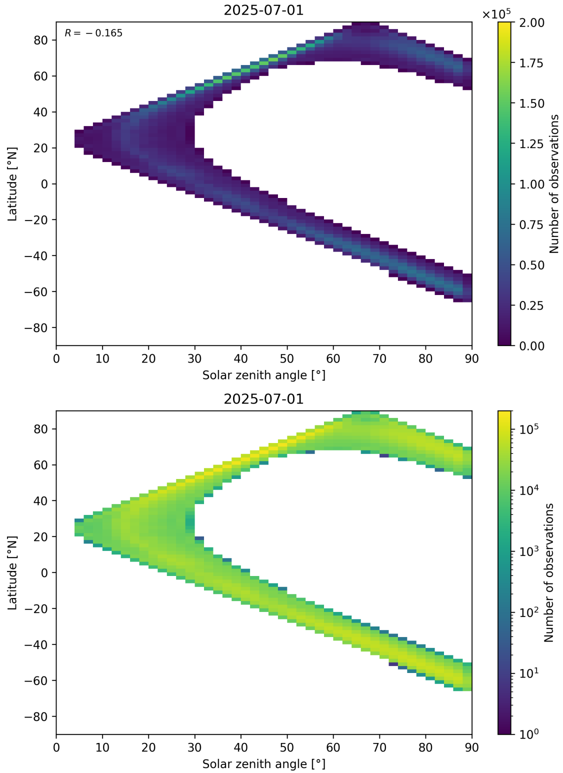
Figure 105: Scatter density plot of “Solar zenith angle” against “Latitude” for 2025-06-30 to 2025-07-02.
