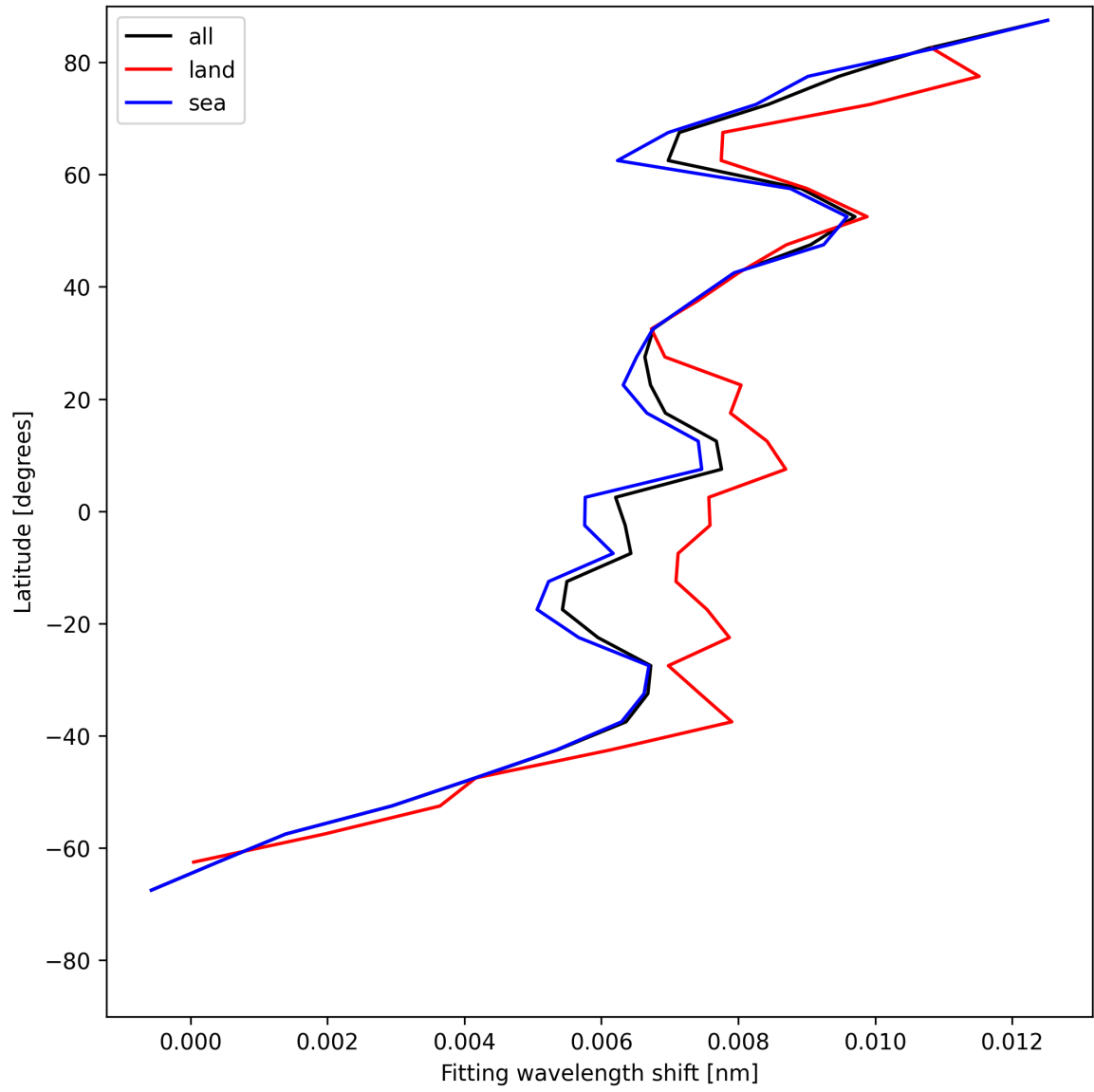
Figure 33: Zonal average of “Fitting wavelength shift” for 2025-06-30 to 2025-07-02.
