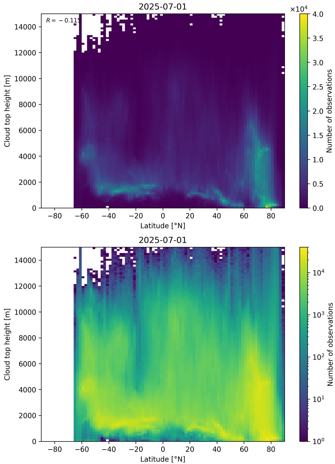
Figure 97: Scatter density plot of “Latitude” against “Cloud top height” for 2025-06-30 to 2025-07-02.
