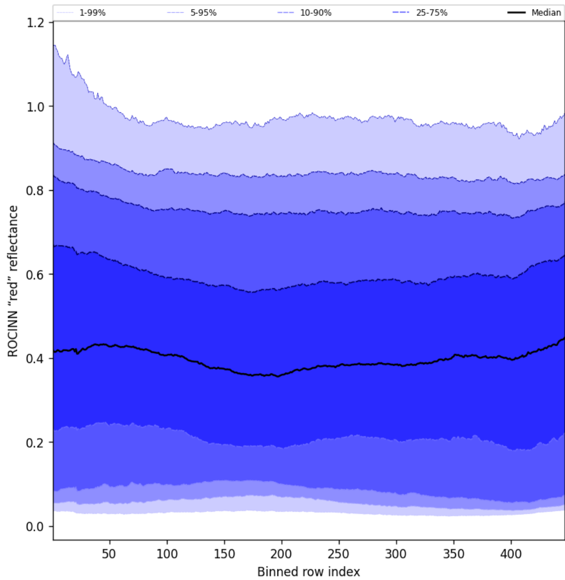
Figure 69: Along track statistics of "ROCINN "red" reflectance" for 2025-06-30 to 2025-07-02
