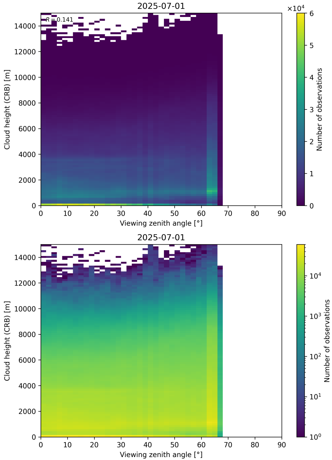
Figure 110: Scatter density plot of “Viewing zenith angle” against “Cloud height (CRB)” for 2025-06-30 to 2025-07-02.
