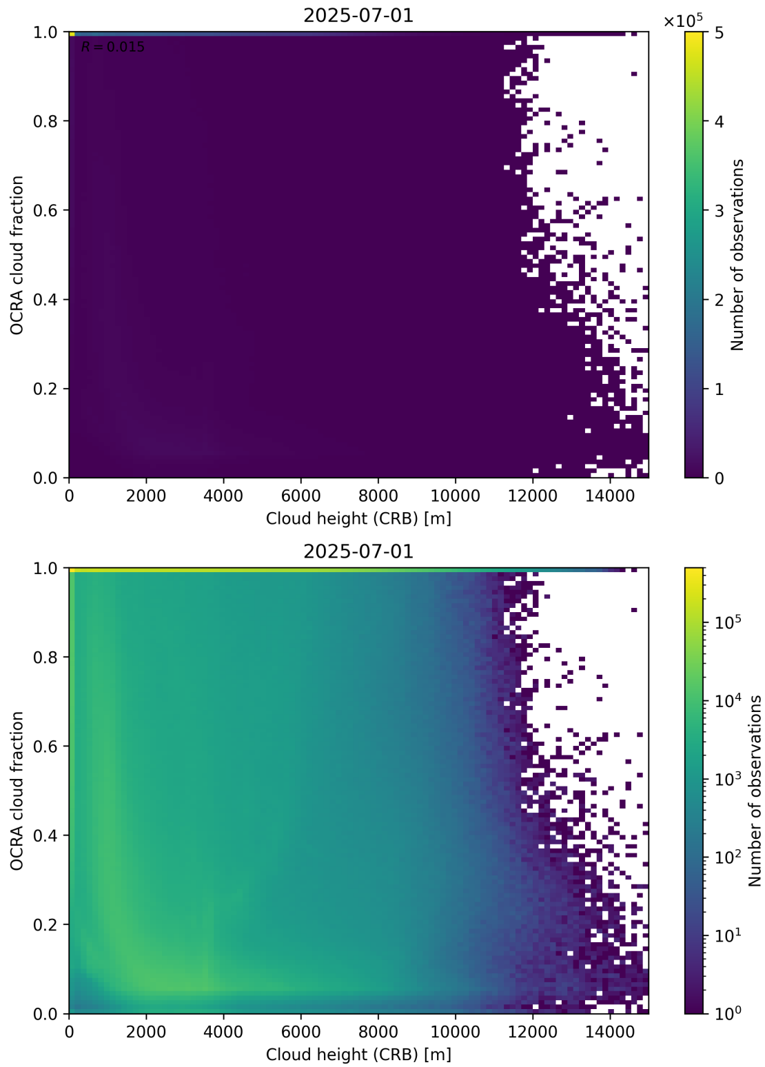
Figure 81: Scatter density plot of “Cloud height (CRB)” against “OCRA cloud fraction” for 2025-06-30 to 2025-07-02.
