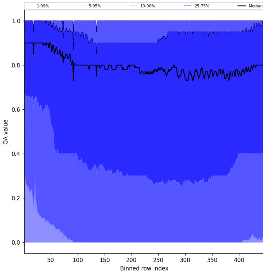
Figure 54: Along track statistics of “QA value” for 2025-06-30 to 2025-07-02
