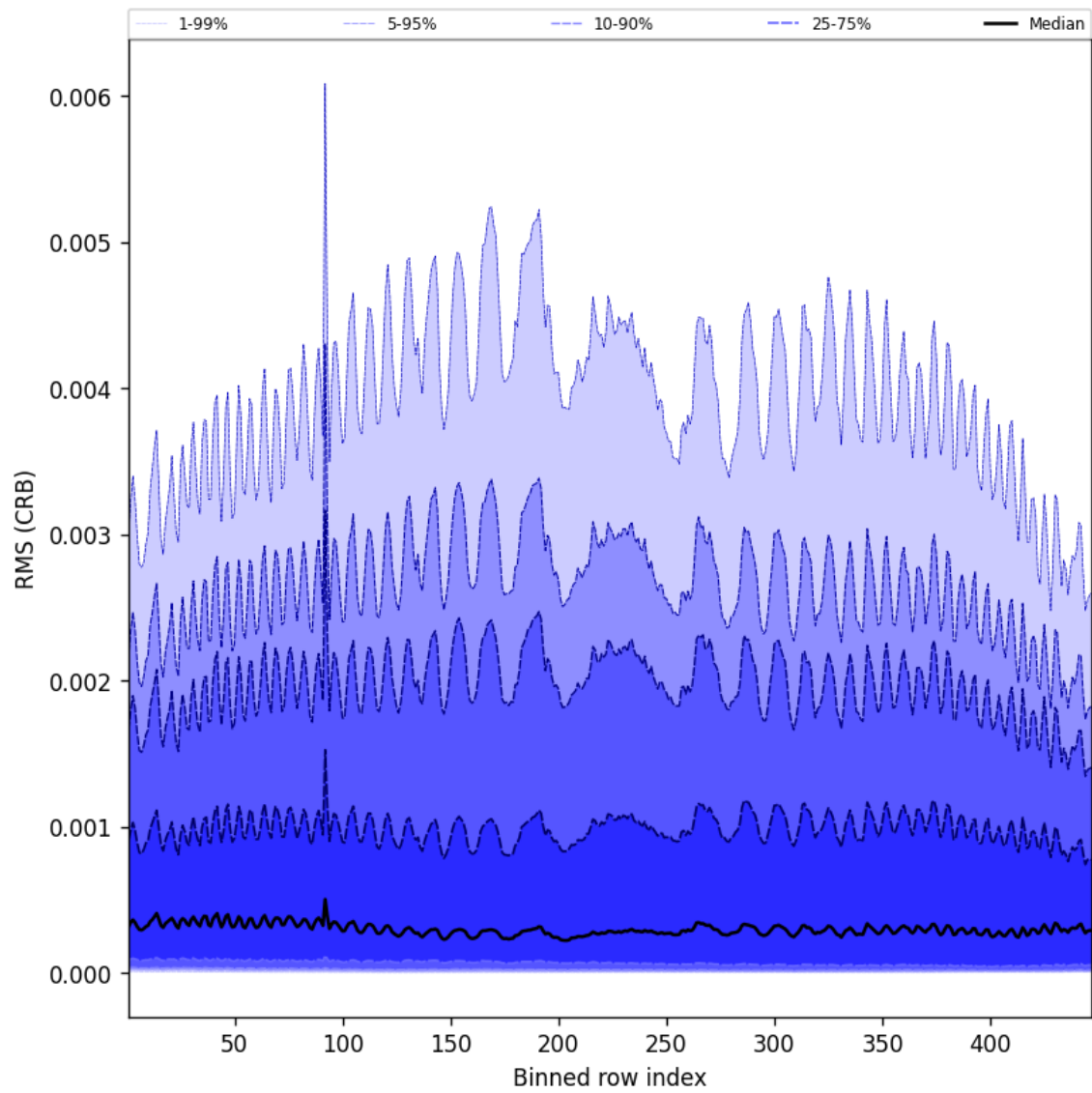
Figure 64: Along track statistics of “RMS (CRB)” for 2025-06-30 to 2025-07-02
