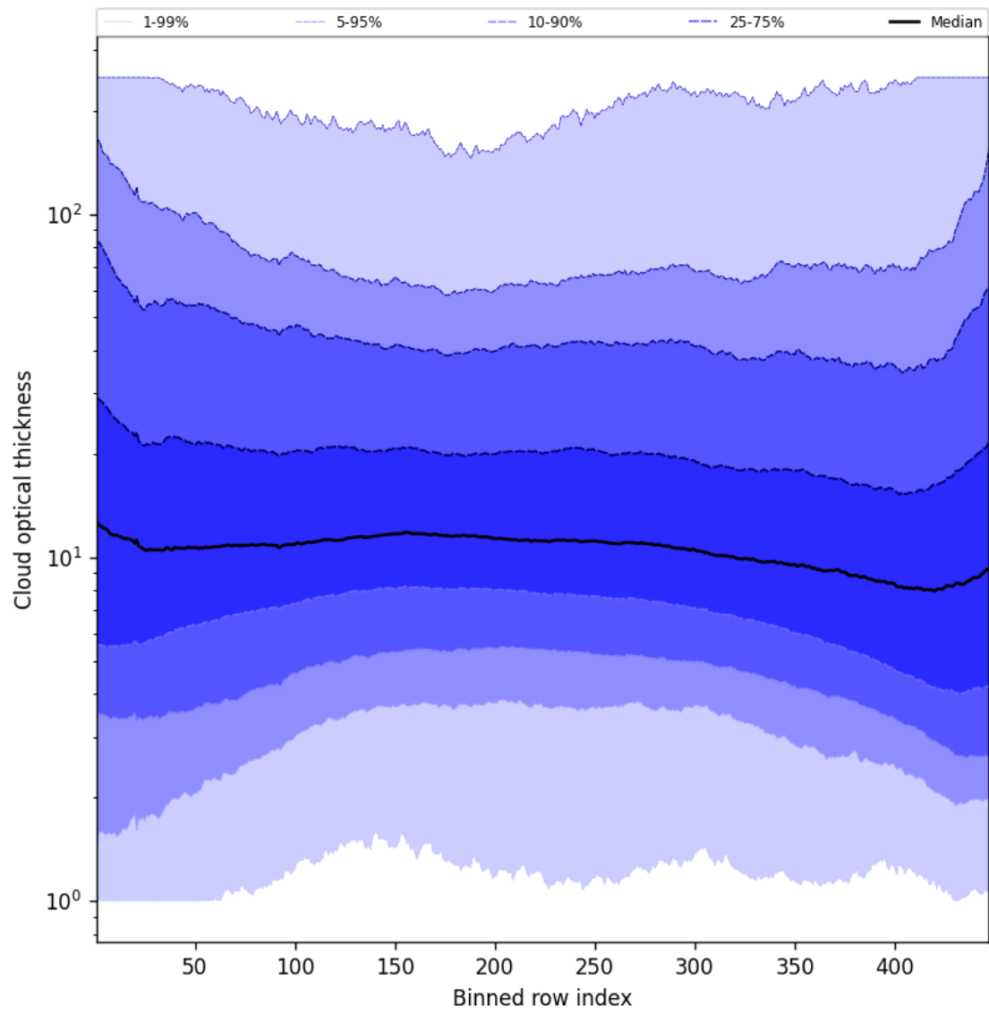
Figure 57: Along track statistics of “Cloud optical thickness” for 2025-06-30 to 2025-07-02
