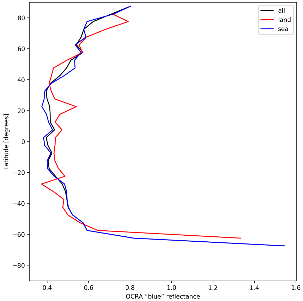
Figure 35: Zonal average of “OCRA “blue” reflectance” for 2025-06-30 to 2025-07-02.
