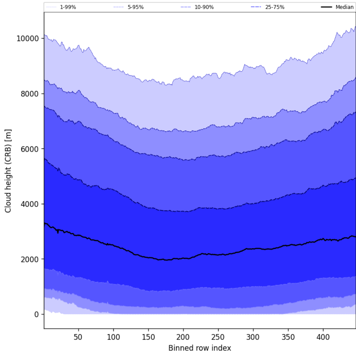
Figure 59: Along track statistics of “Cloud height (CRB)” for 2025-06-30 to 2025-07-02
