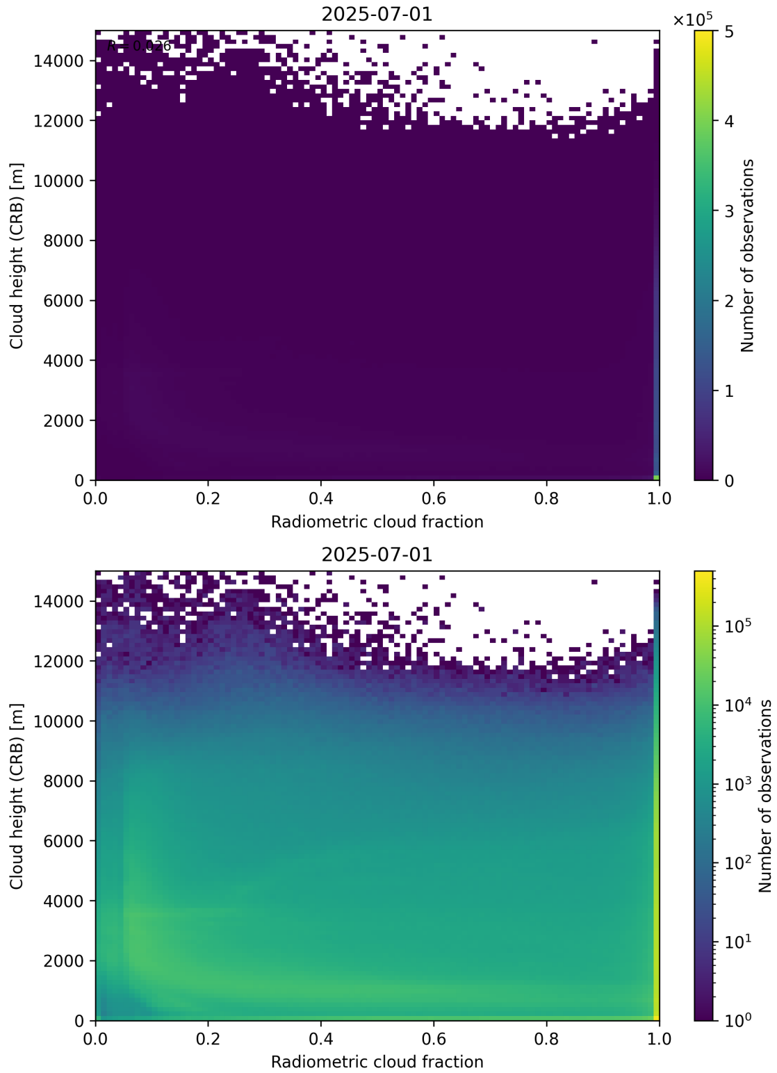
Figure 74: Scatter density plot of “Radiometric cloud fraction” against “Cloud height (CRB)” for 2025-06-30 to 2025-07-02.
