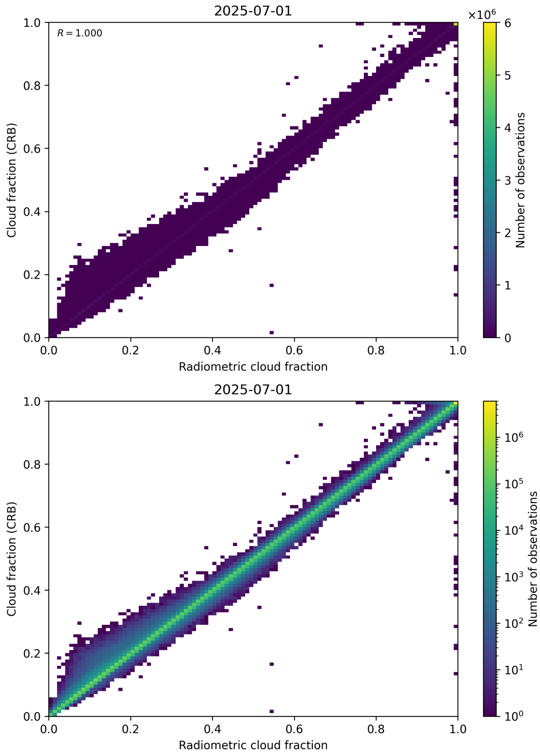
Figure 73: Scatter density plot of “Radiometric cloud fraction” against “Cloud fraction (CRB)” for 2025-06-30 to 2025-07-02.
