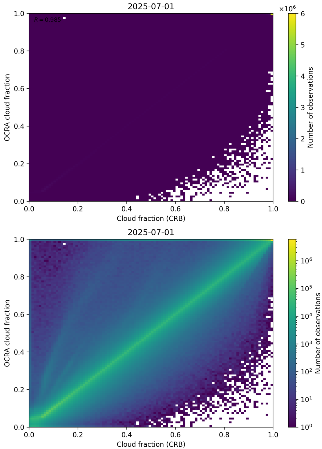
Figure 78: Scatter density plot of “Cloud fraction (CRB)” against “OCRA cloud fraction” for 2025-06-30 to 2025-07-02.
