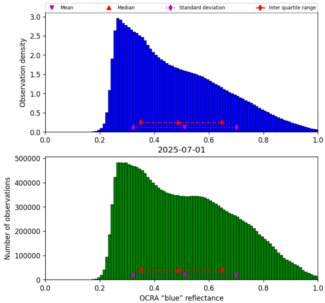
Figure 51: Histogram of “OCRA “blue” reflectance” for 2025-06-30 to 2025-07-02
