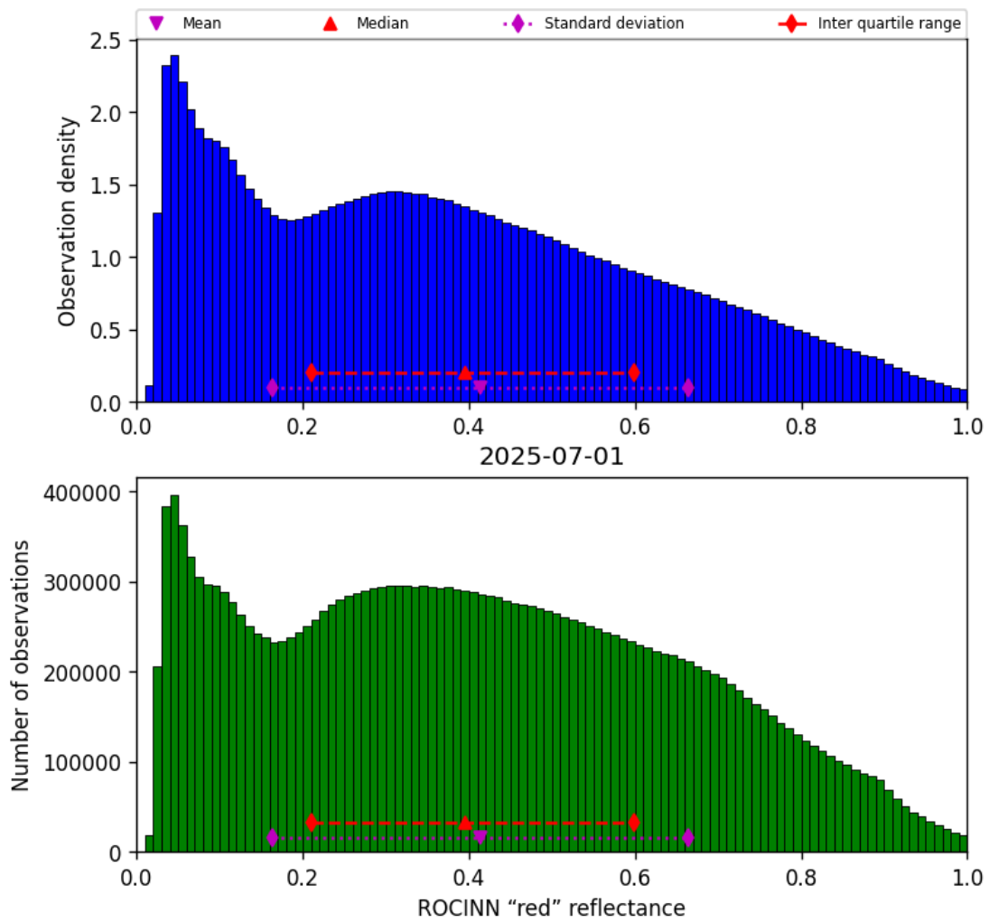
Figure 53: Histogram of “ROCINN “red” reflectance” for 2025-06-30 to 2025-07-02
