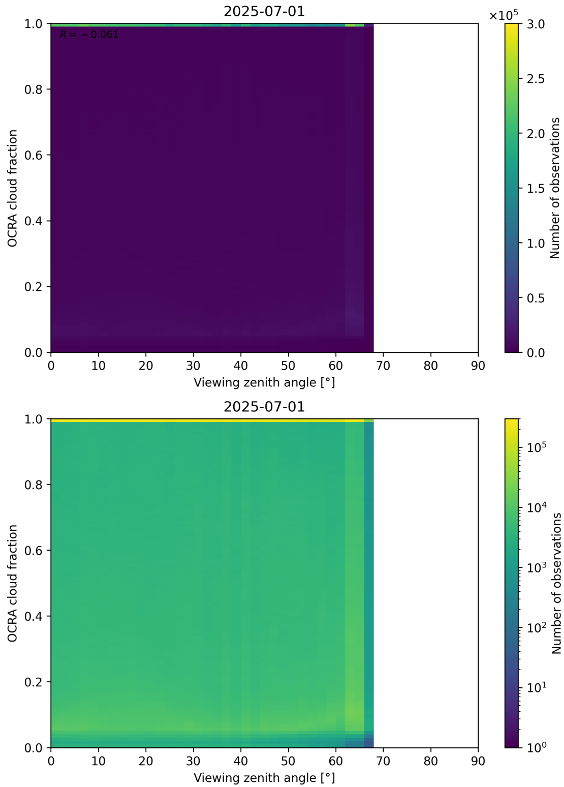
Figure 108: Scatter density plot of “Viewing zenith angle” against “OCRA cloud fraction” for 2025-06-30 to 2025-07-02.
