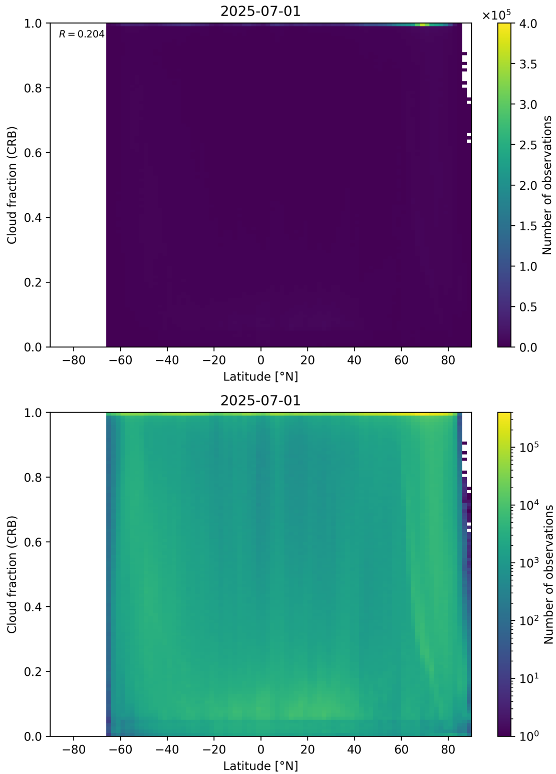
Figure 94: Scatter density plot of “Latitude” against “Cloud fraction (CRB)” for 2025-06-30 to 2025-07-02.
