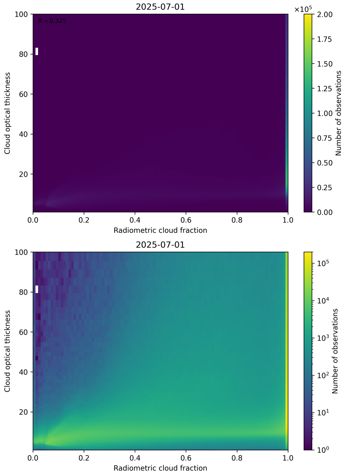
Figure 75: Scatter density plot of “Radiometric cloud fraction” against “Cloud optical thickness” for 2025-06-30 to 2025-07-02.
