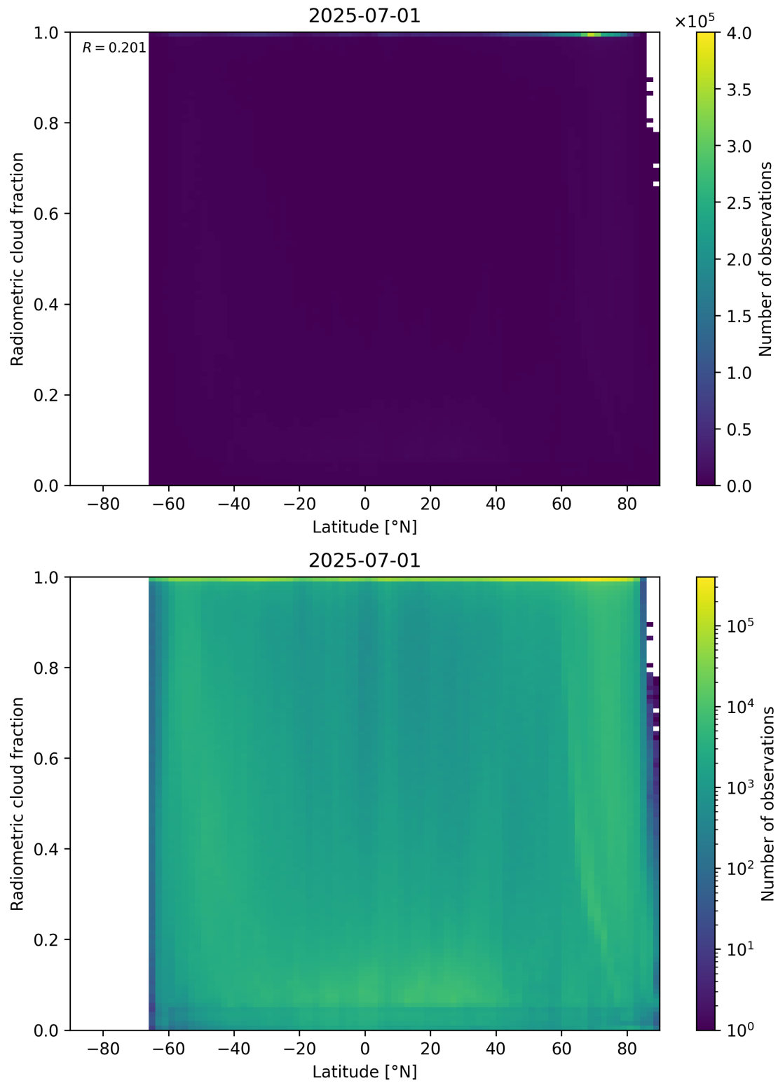
Figure 92: Scatter density plot of “Latitude” against “Radiometric cloud fraction” for 2025-06-30 to 2025-07-02.
