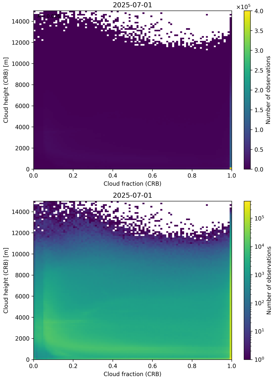
Figure 79: Scatter density plot of “Cloud fraction (CRB)” against “Cloud height (CRB)” for 2025-06-30 to 2025-07-02.
