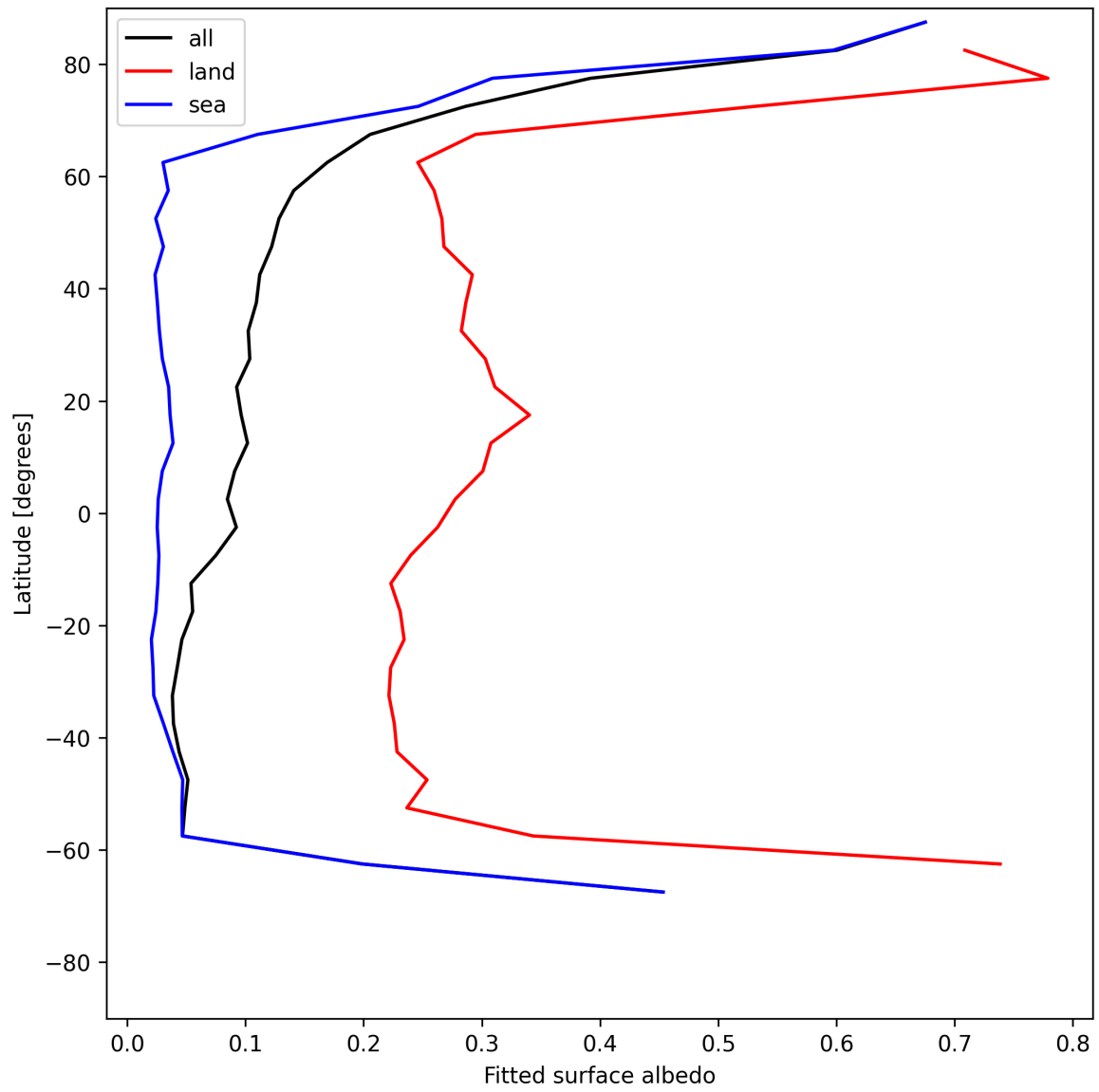
Figure 29: Zonal average of “Fitted surface albedo” for 2025-06-30 to 2025-07-02.
