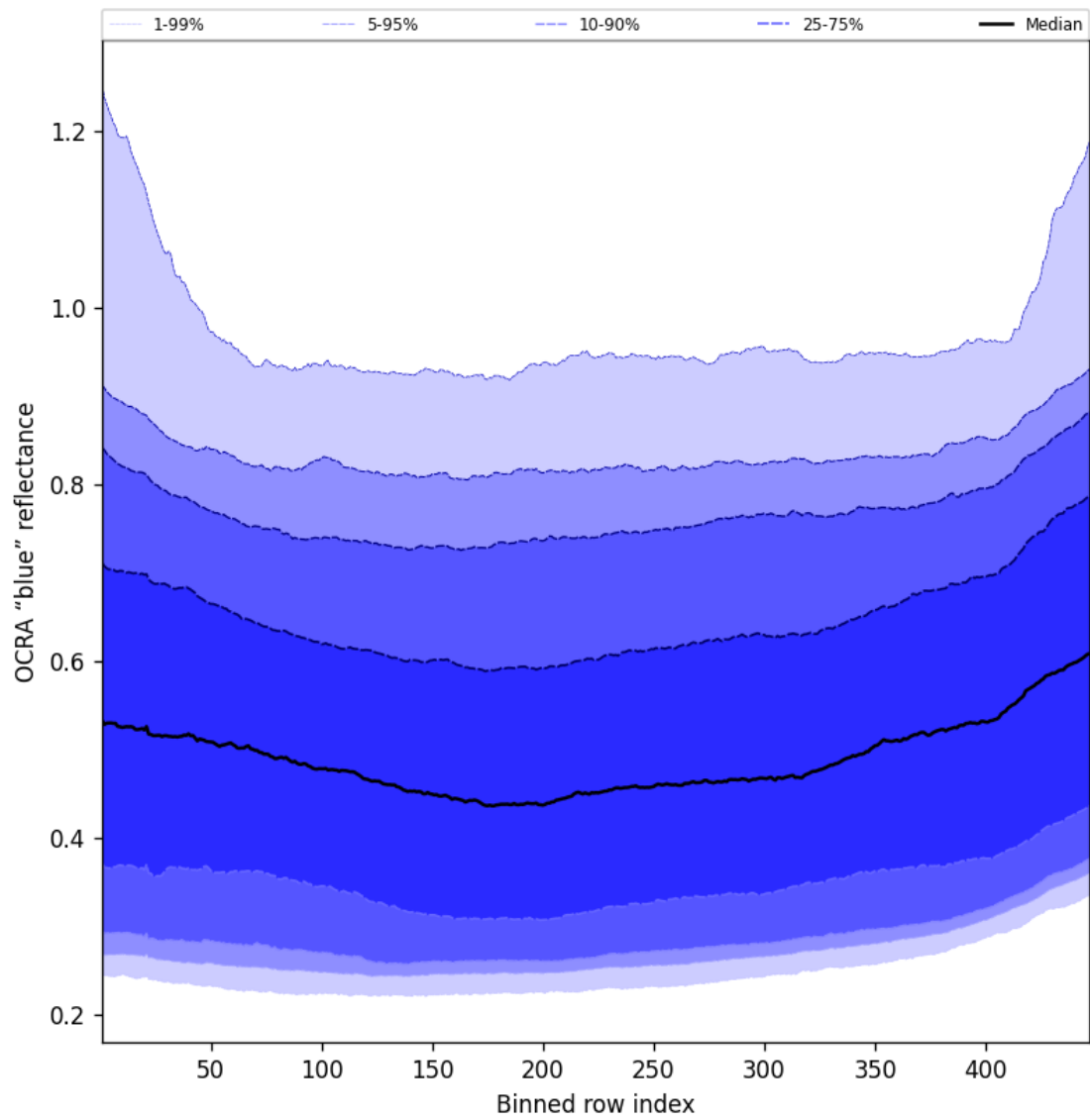
Figure 67: Along track statistics of “OCRA “blue” reflectance” for 2025-06-30 to 2025-07-02
