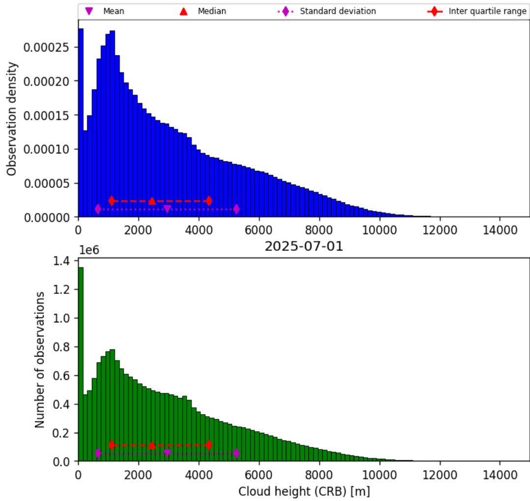
Figure 43: Histogram of “Cloud height (CRB)” for 2025-06-30 to 2025-07-02
