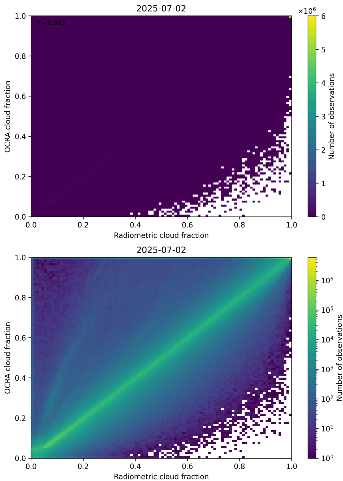
Figure 72: Scatter density plot of “Radiometric cloud fraction” against “OCRA cloud fraction” for 2025-07-02 to 2025-07-03.
