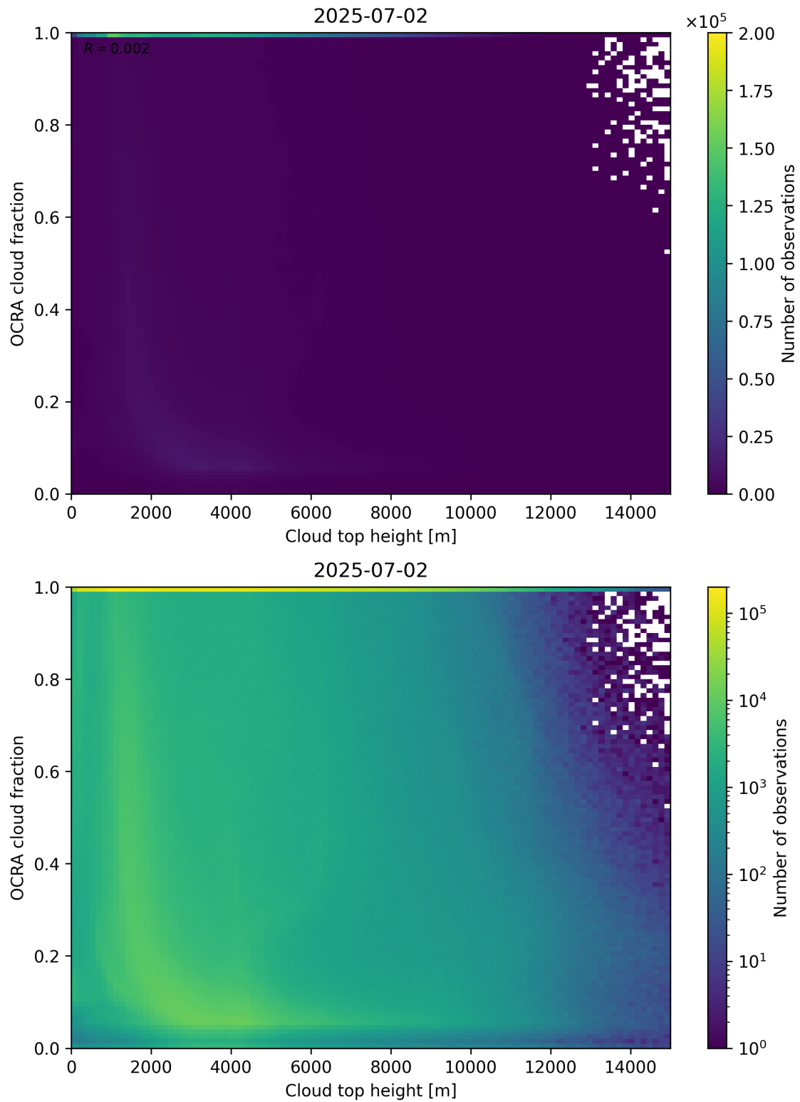
Figure 87: Scatter density plot of “Cloud top height” against “OCRA cloud fraction” for 2025-07-02 to 2025-07-03.
