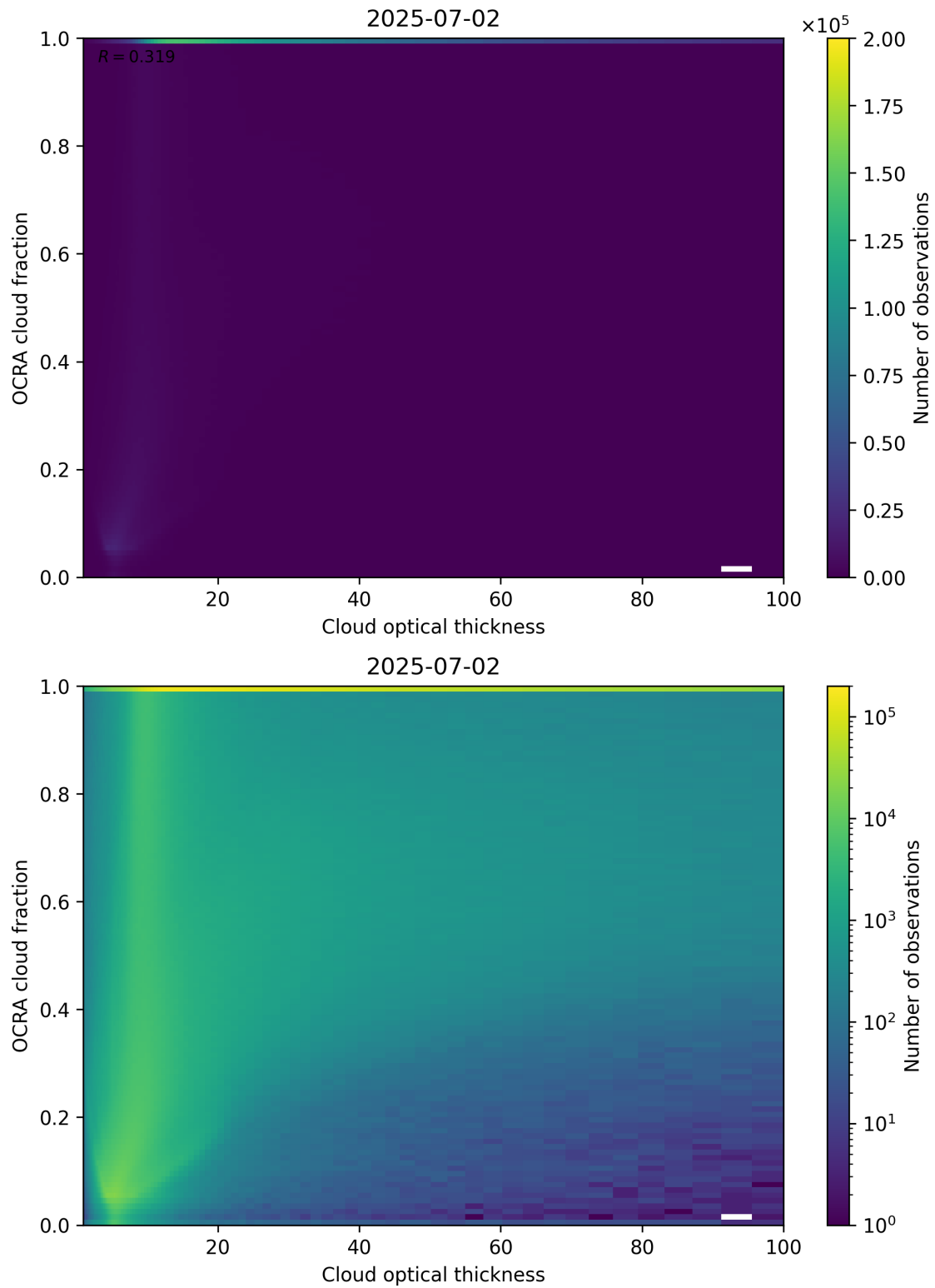
Figure 83: Scatter density plot of “Cloud optical thickness” against “OCRA cloud fraction” for 2025-07-02 to 2025-07-03.
