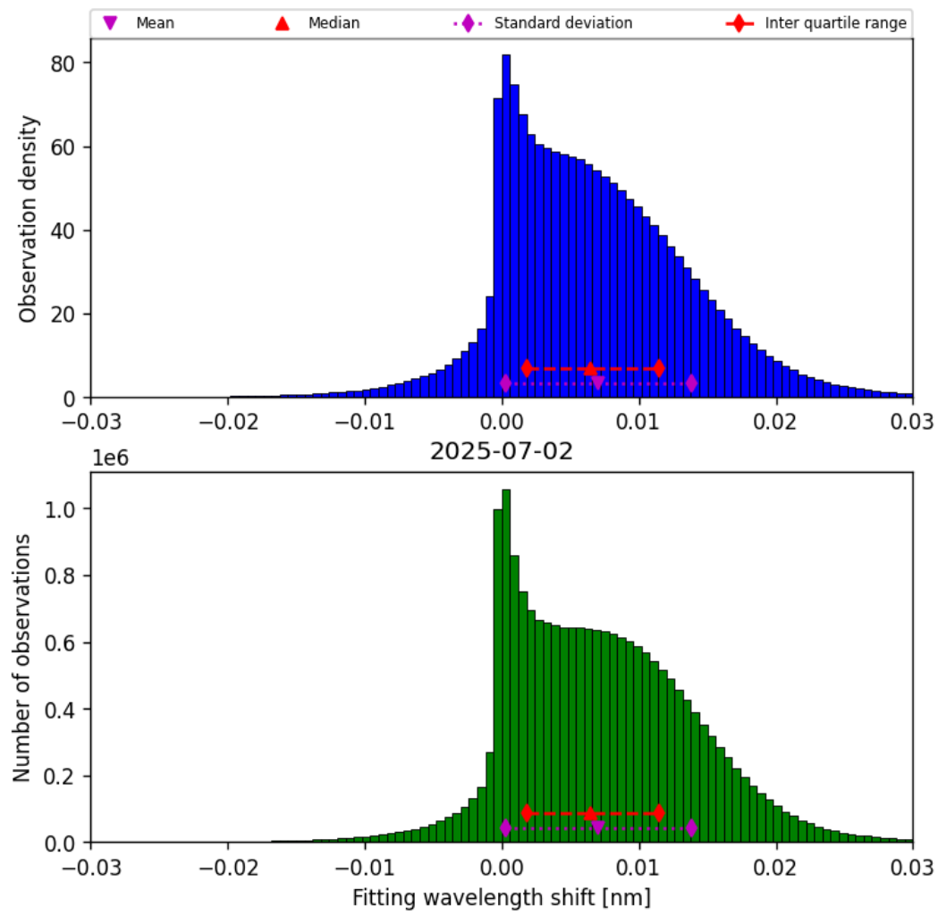
Figure 49: Histogram of “Fitting wavelength shift” for 2025-07-02 to 2025-07-03
