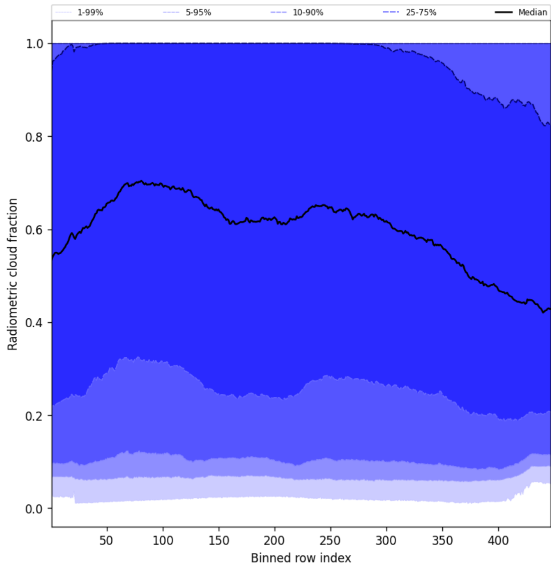
Figure 55: Along track statistics of “Radiometric cloud fraction” for 2025-07-02 to 2025-07-03
