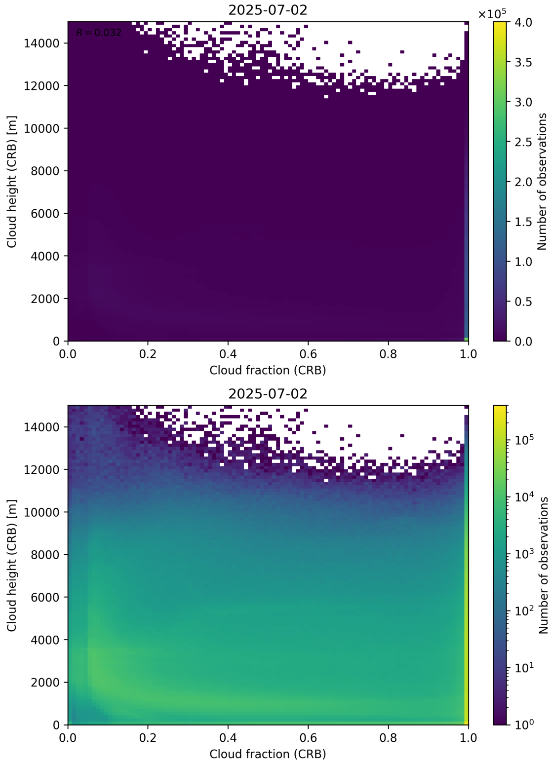
Figure 79: Scatter density plot of “Cloud fraction (CRB)” against “Cloud height (CRB)” for 2025-07-02 to 2025-07-03.
