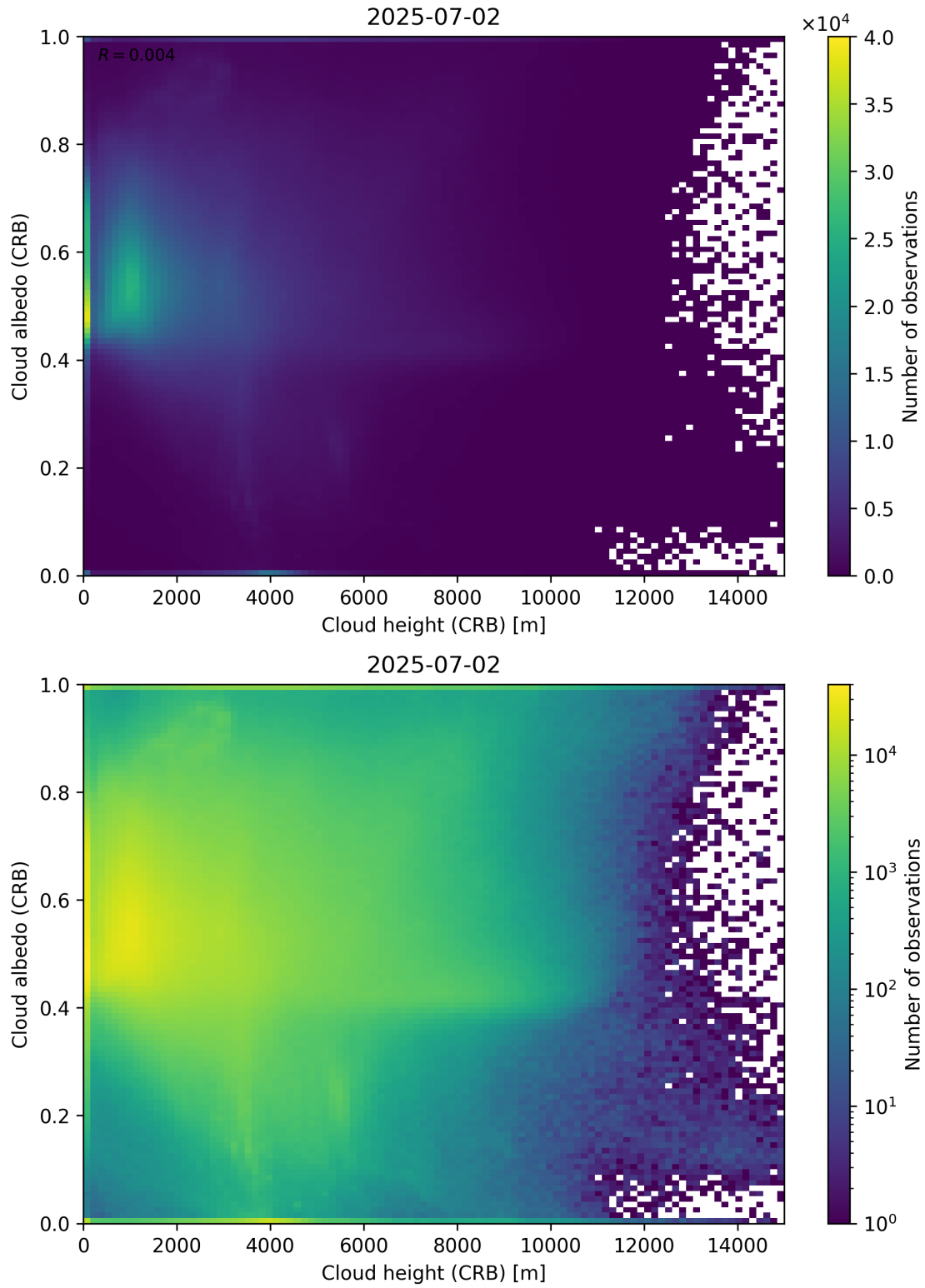
Figure 80: Scatter density plot of “Cloud height (CRB)” against “Cloud albedo (CRB)” for 2025-07-02 to 2025-07-03.
