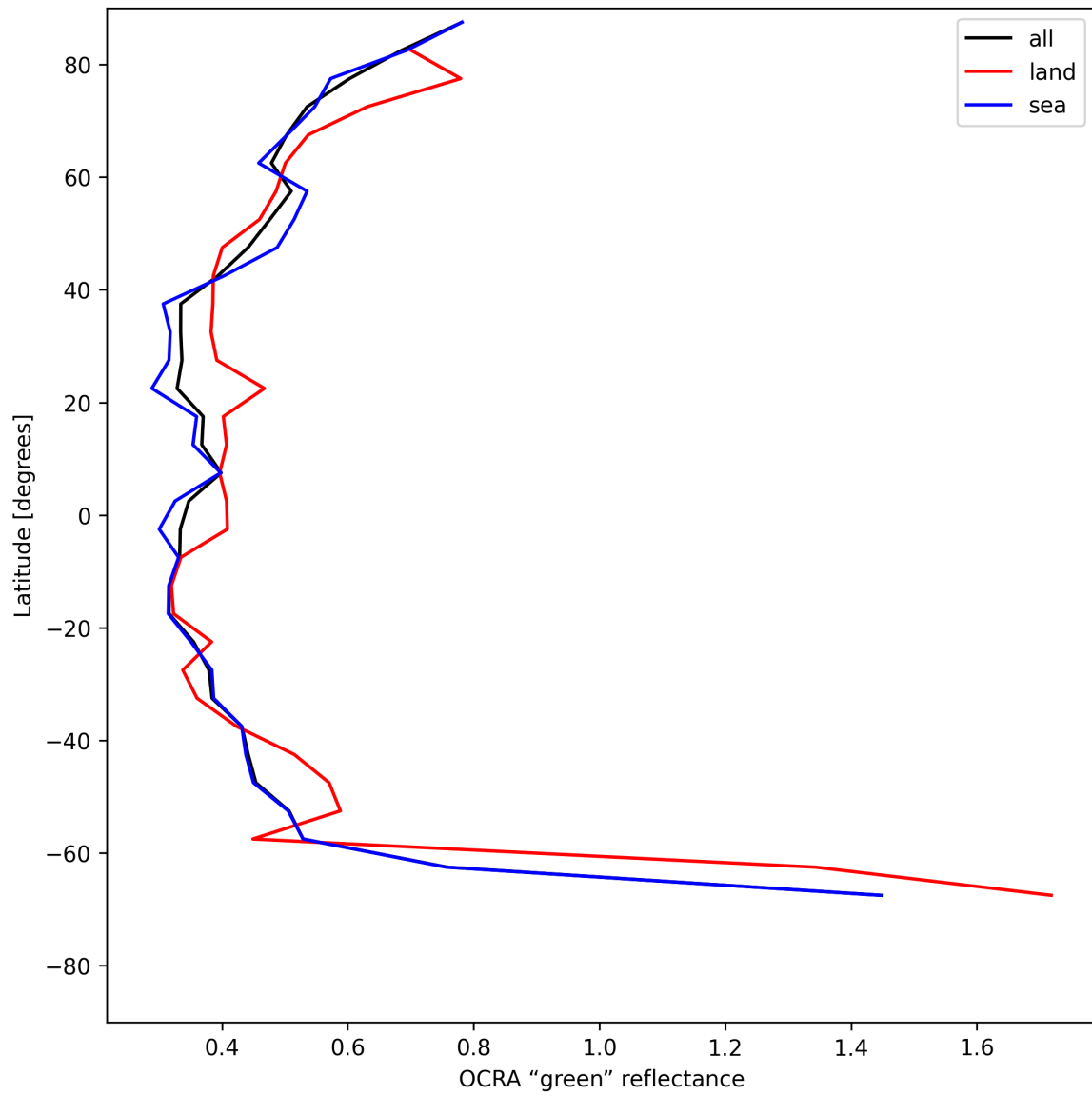
Figure 36: Zonal average of “OCRA “green” reflectance” for 2025-07-02 to 2025-07-03.
