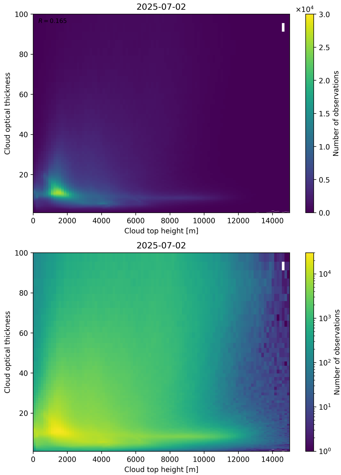
Figure 90: Scatter density plot of “Cloud top height” against “Cloud optical thickness” for 2025-07-02 to 2025-07-03.
