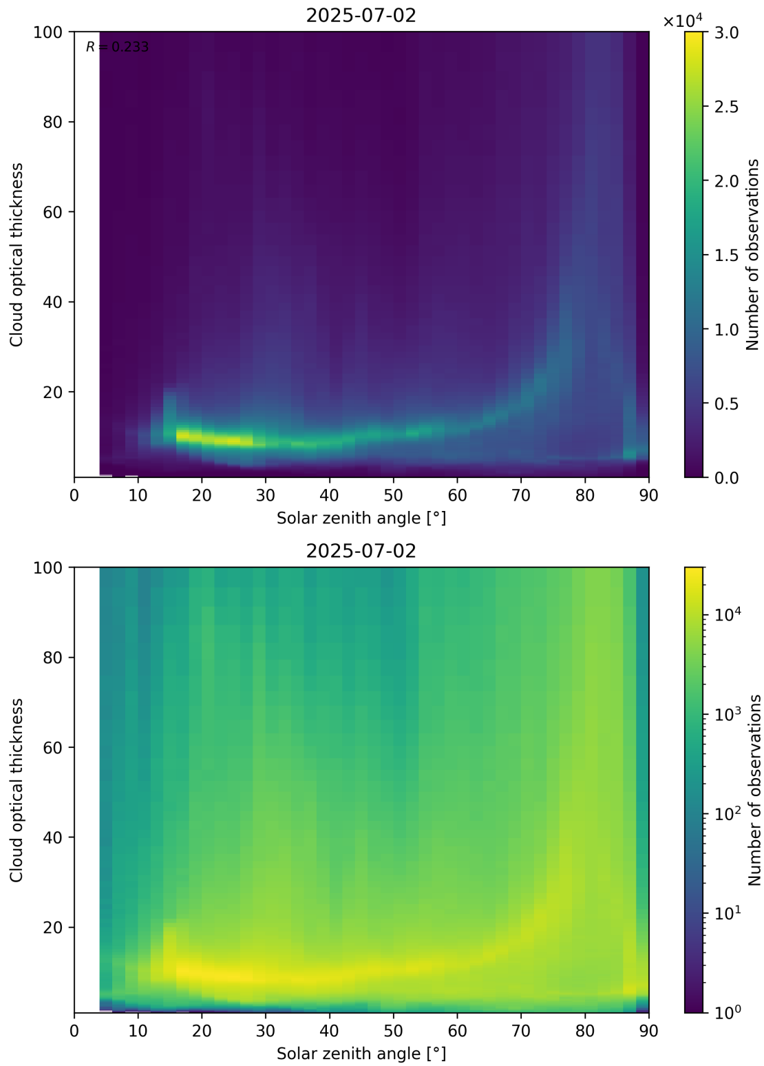
Figure 103: Scatter density plot of “Solar zenith angle” against “Cloud optical thickness” for 2025-07-02 to 2025-07-03.
