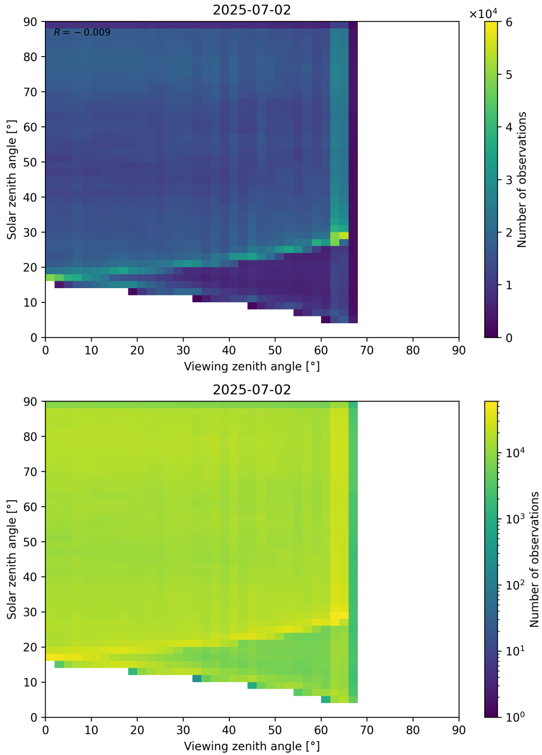
Figure 114: Scatter density plot of “Viewing zenith angle” against “Solar zenith angle” for 2025-07-02 to 2025-07-03.
