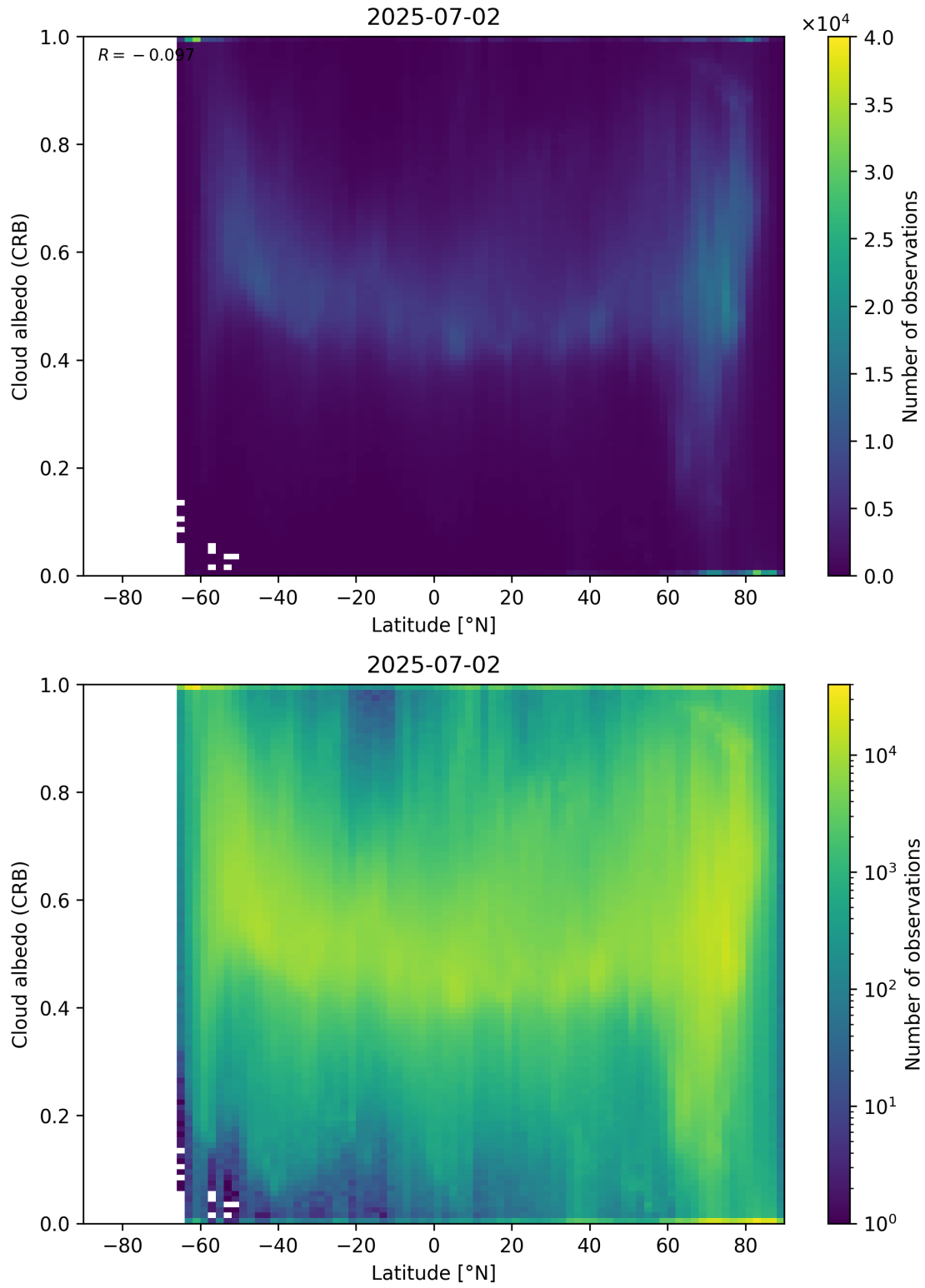
Figure 91: Scatter density plot of “Latitude” against “Cloud albedo (CRB)” for 2025-07-02 to 2025-07-03.
