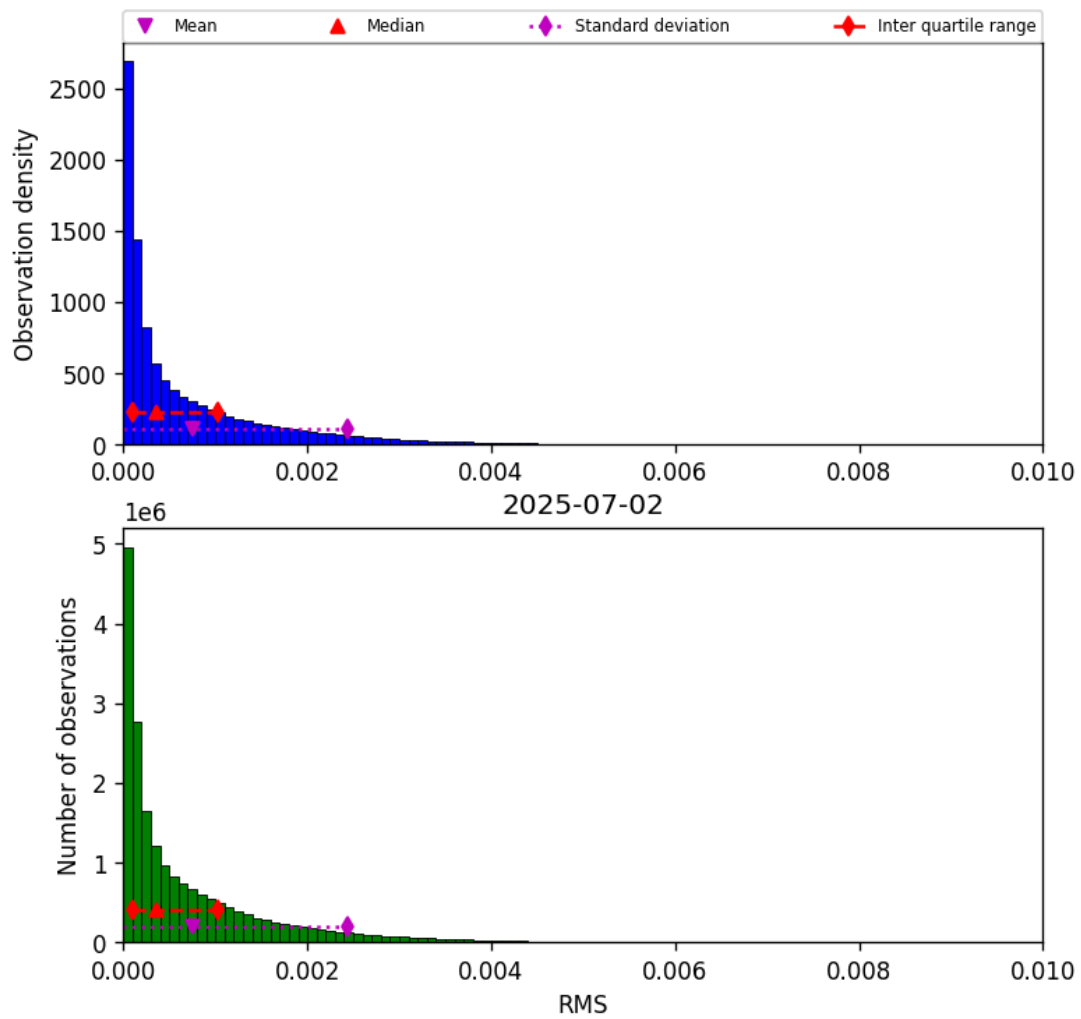
Figure 47: Histogram of “RMS” for 2025-07-02 to 2025-07-03
