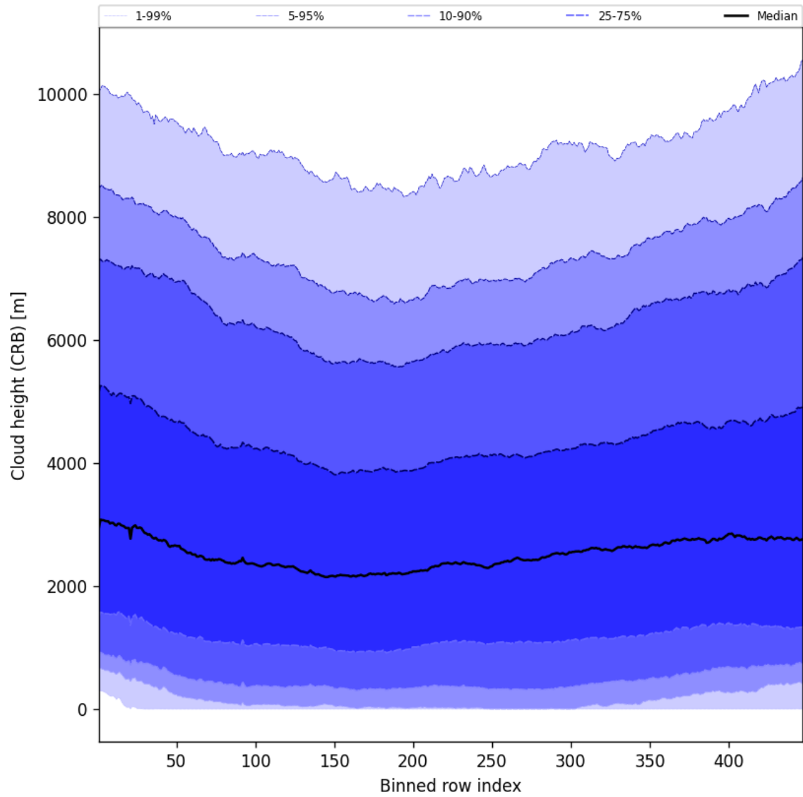
Figure 59: Along track statistics of “Cloud height (CRB)” for 2025-07-02 to 2025-07-03
