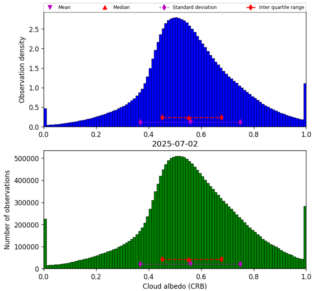
Figure 44: Histogram of “Cloud albedo (CRB)” for 2025-07-02 to 2025-07-03
