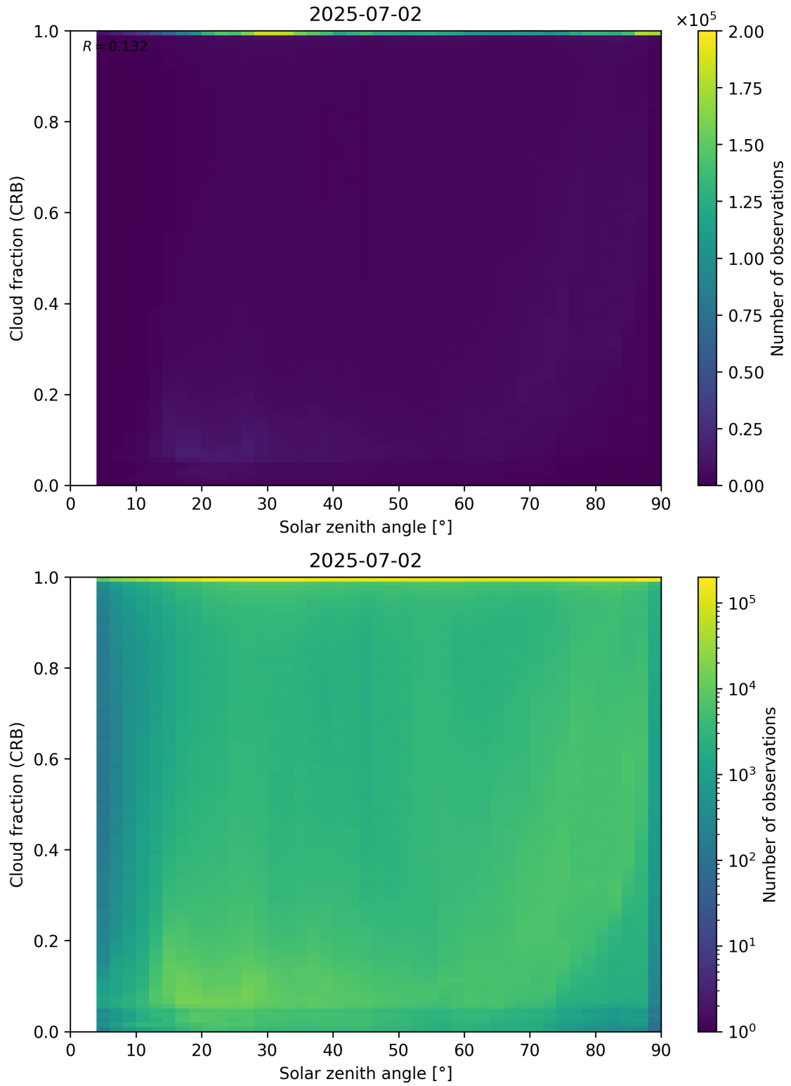
Figure 101: Scatter density plot of “Solar zenith angle” against “Cloud fraction (CRB)” for 2025-07-02 to 2025-07-03.
