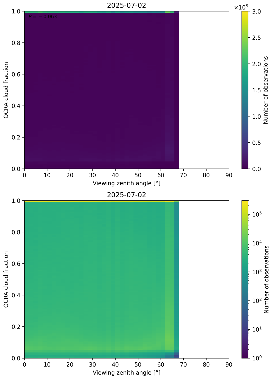
Figure 108: Scatter density plot of “Viewing zenith angle” against “OCRA cloud fraction” for 2025-07-02 to 2025-07-03.
