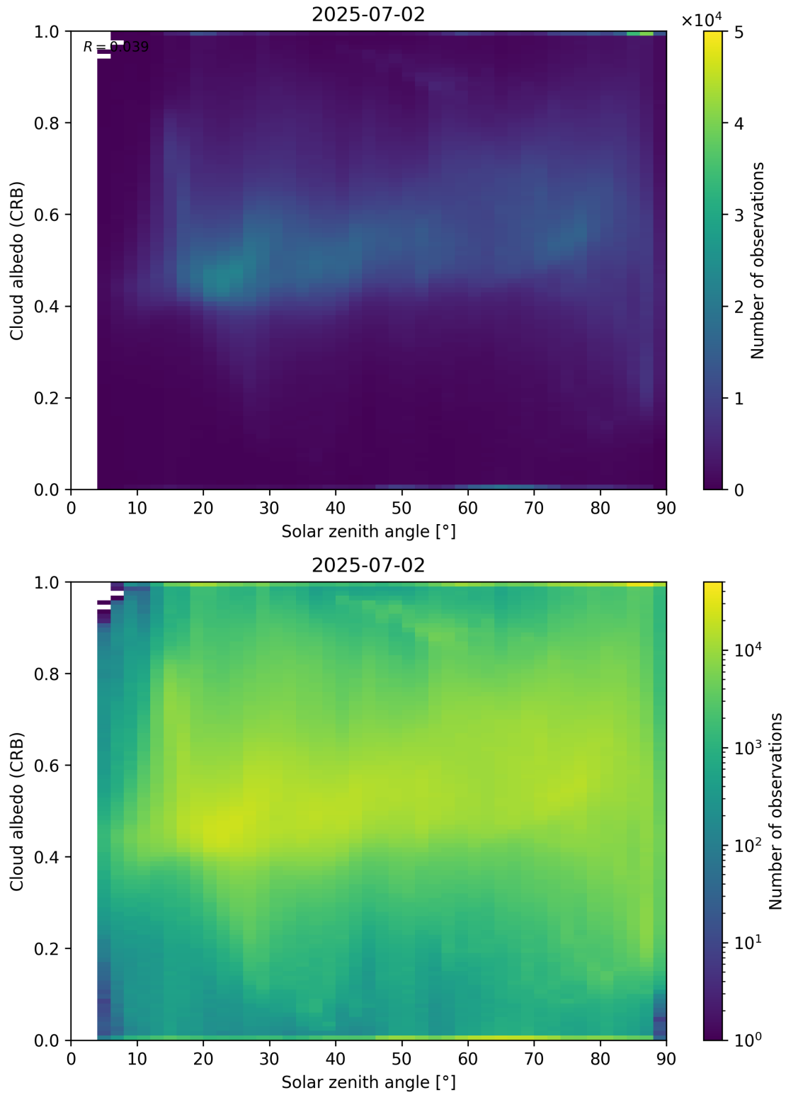
Figure 98: Scatter density plot of “Solar zenith angle” against “Cloud albedo (CRB)” for 2025-07-02 to 2025-07-03.
