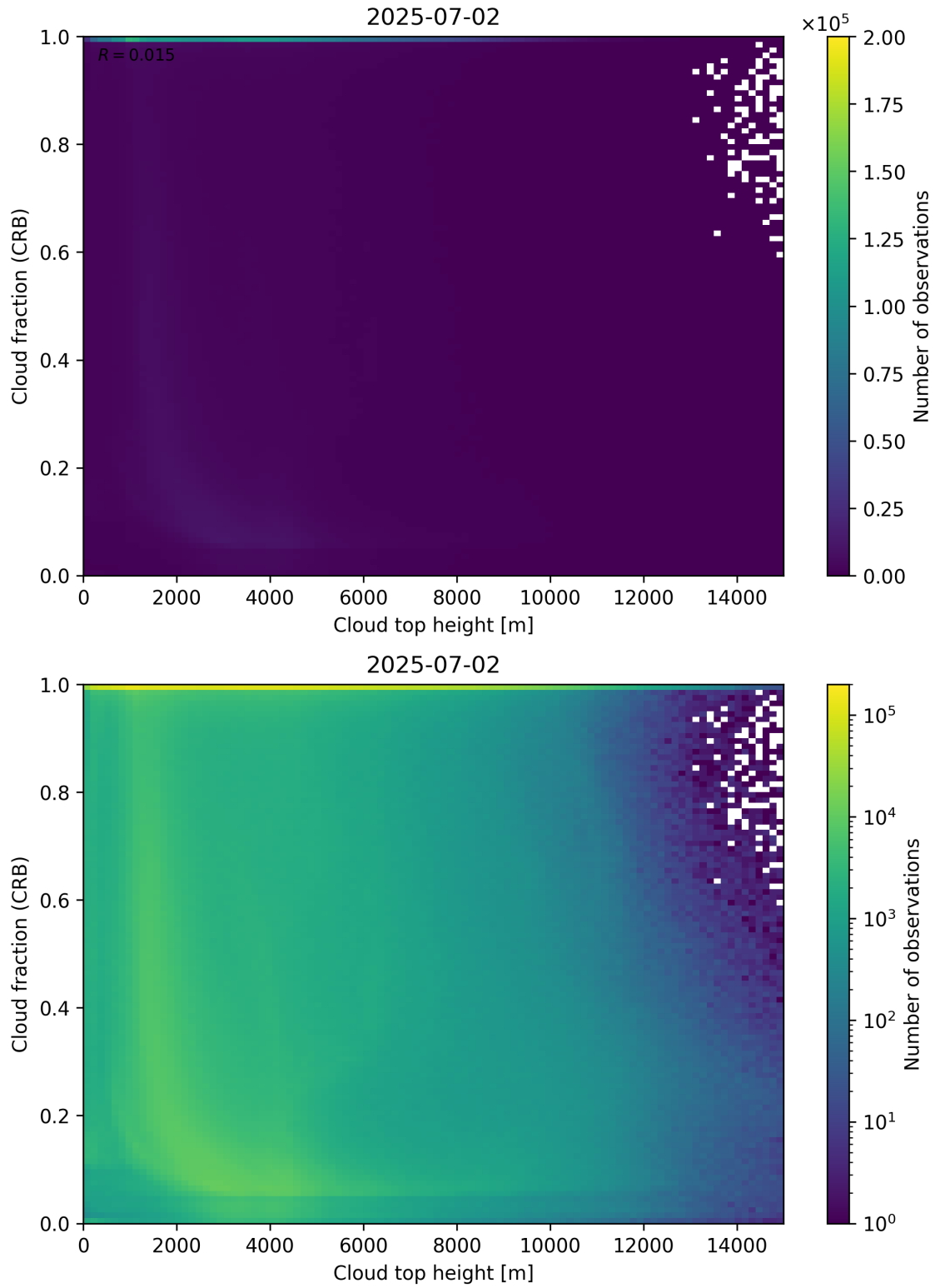
Figure 88: Scatter density plot of “Cloud top height” against “Cloud fraction (CRB)” for 2025-07-02 to 2025-07-03.
