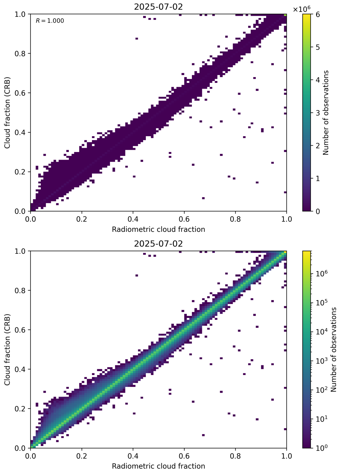
Figure 73: Scatter density plot of “Radiometric cloud fraction” against “Cloud fraction (CRB)” for 2025-07-02 to 2025-07-03.
