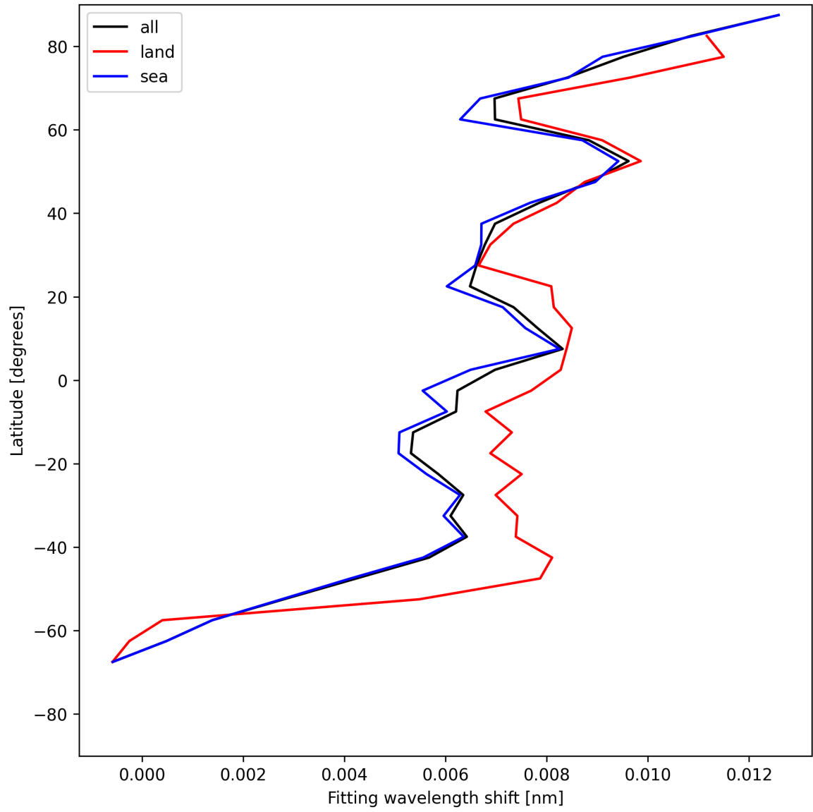
Figure 33: Zonal average of “Fitting wavelength shift” for 2025-07-02 to 2025-07-03.
