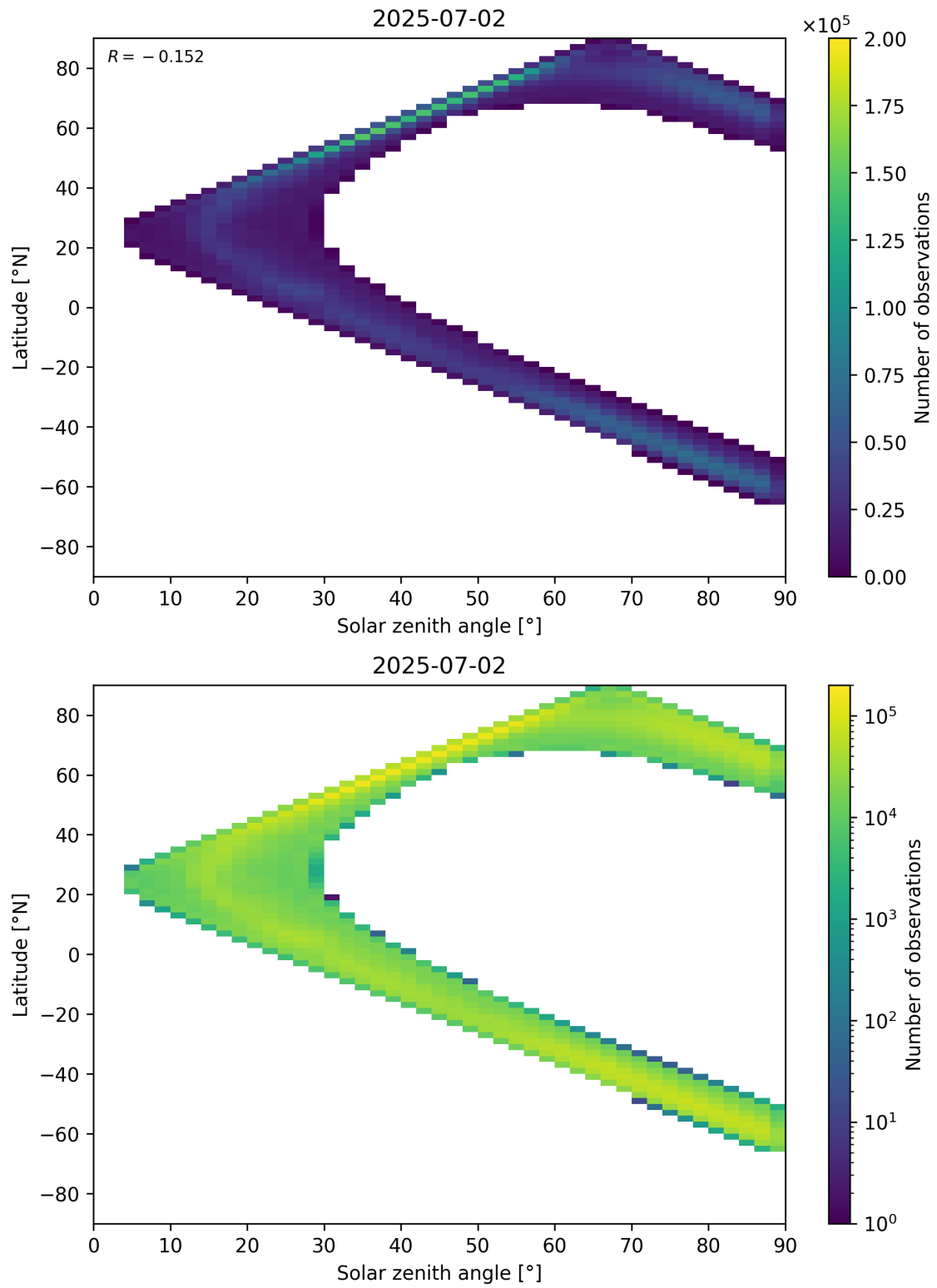
Figure 105: Scatter density plot of “Solar zenith angle” against “Latitude” for 2025-07-02 to 2025-07-03.
