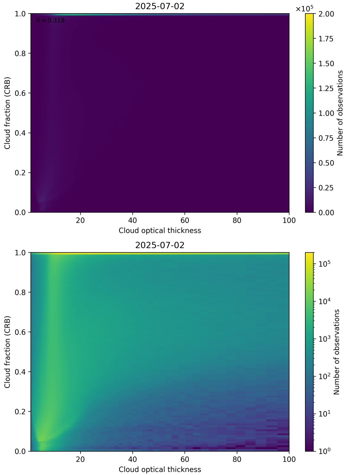
Figure 84: Scatter density plot of “Cloud optical thickness” against “Cloud fraction (CRB)” for 2025-07-02 to 2025-07-03.
