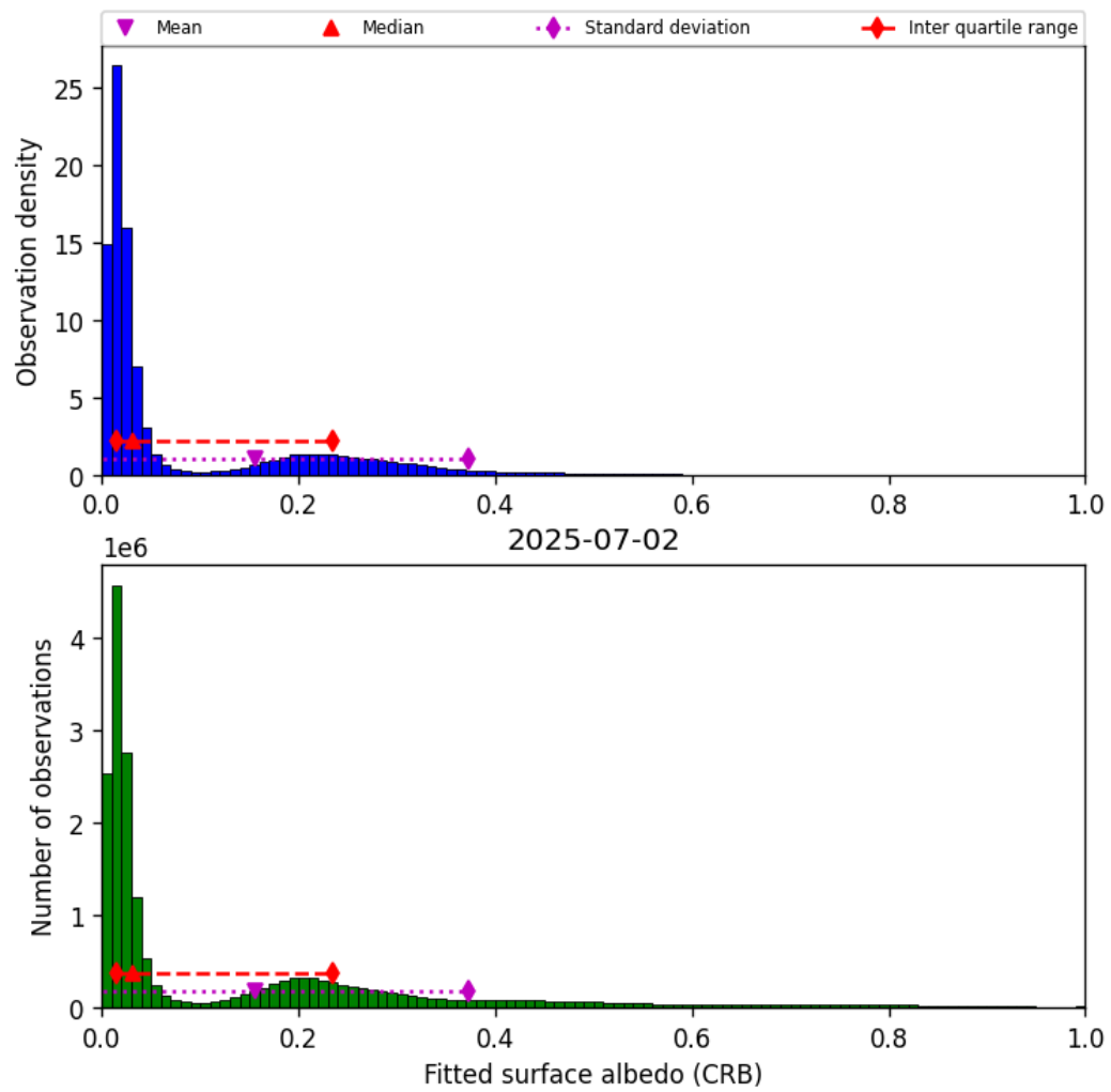
Figure 46: Histogram of “Fitted surface albedo (CRB)” for 2025-07-02 to 2025-07-03
