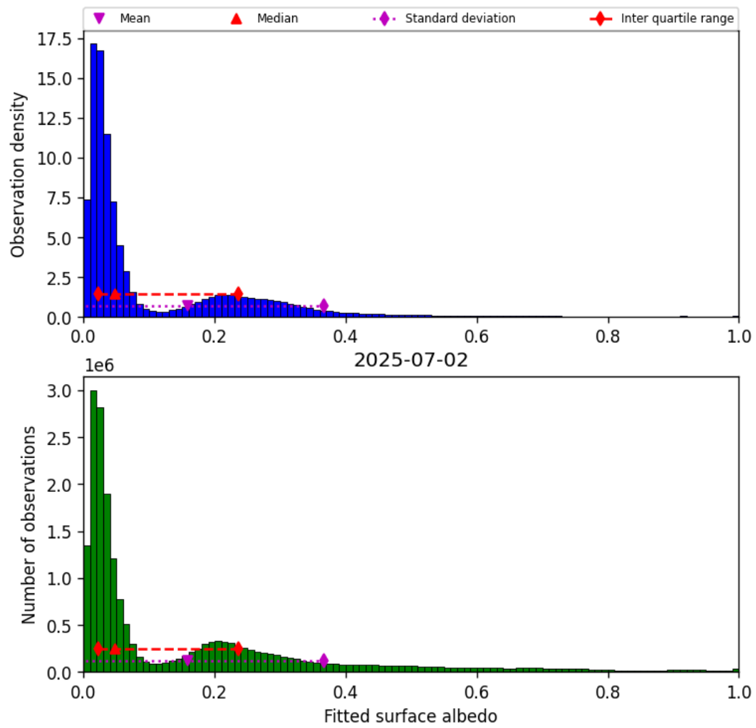
Figure 45: Histogram of “Fitted surface albedo” for 2025-07-02 to 2025-07-03
