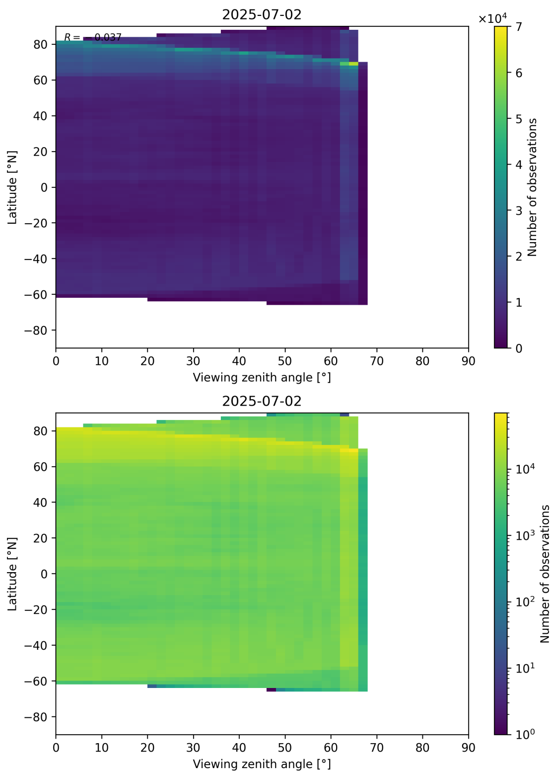
Figure 113: Scatter density plot of “Viewing zenith angle” against “Latitude” for 2025-07-02 to 2025-07-03.
