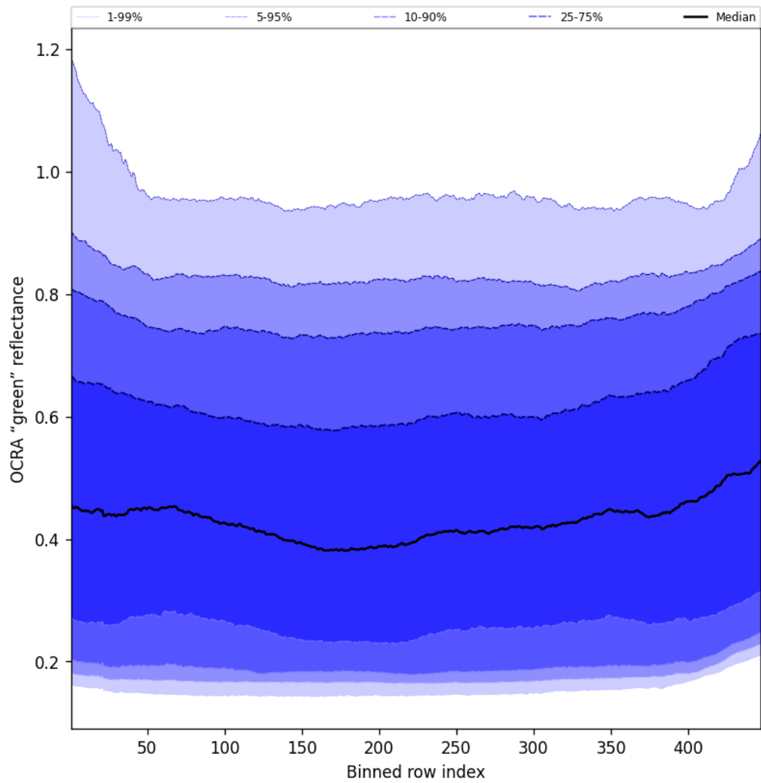
Figure 68: Along track statistics of “OCRA “green” reflectance” for 2025-07-02 to 2025-07-03
