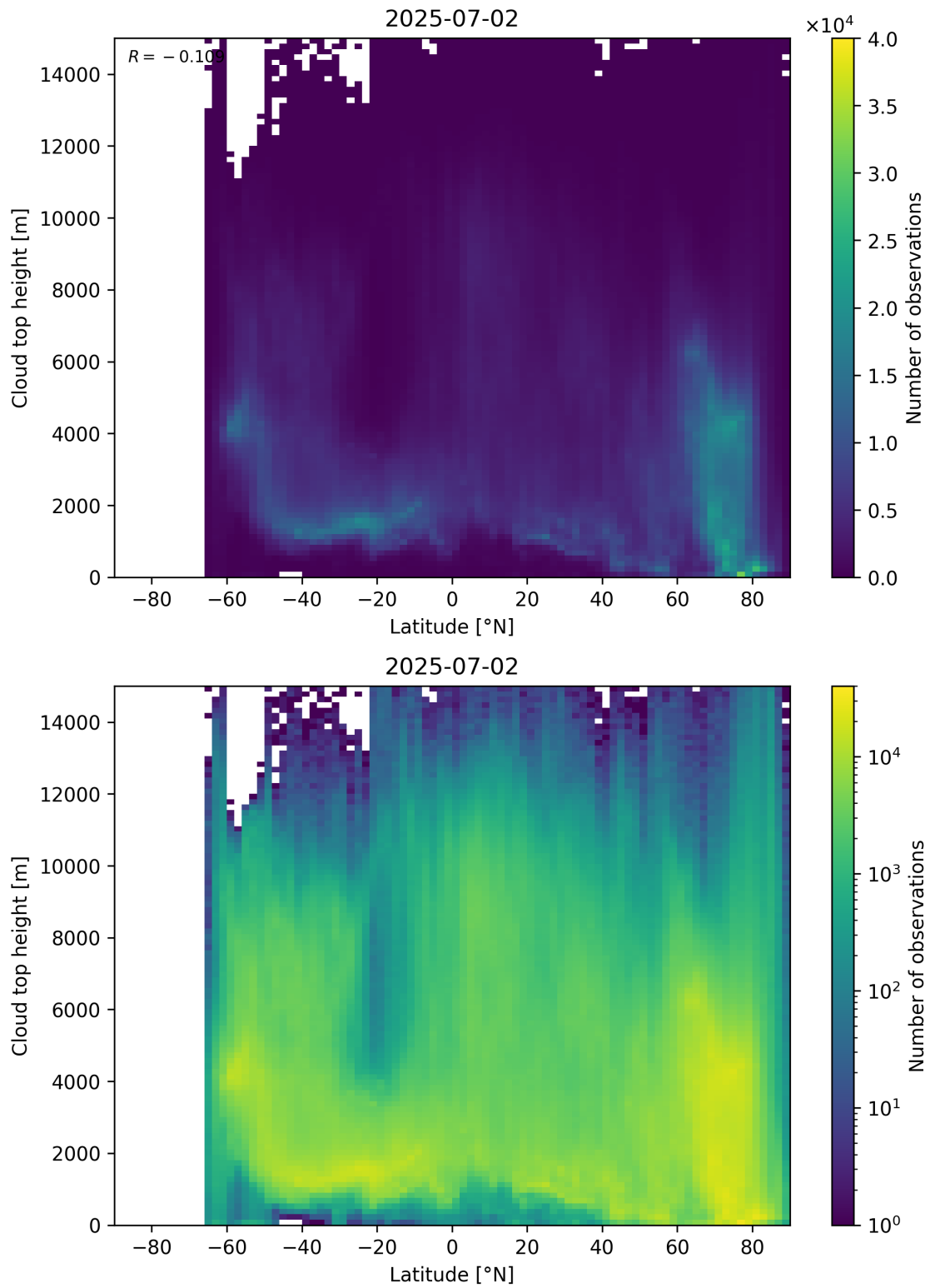
Figure 97: Scatter density plot of “Latitude” against “Cloud top height” for 2025-07-02 to 2025-07-03.
