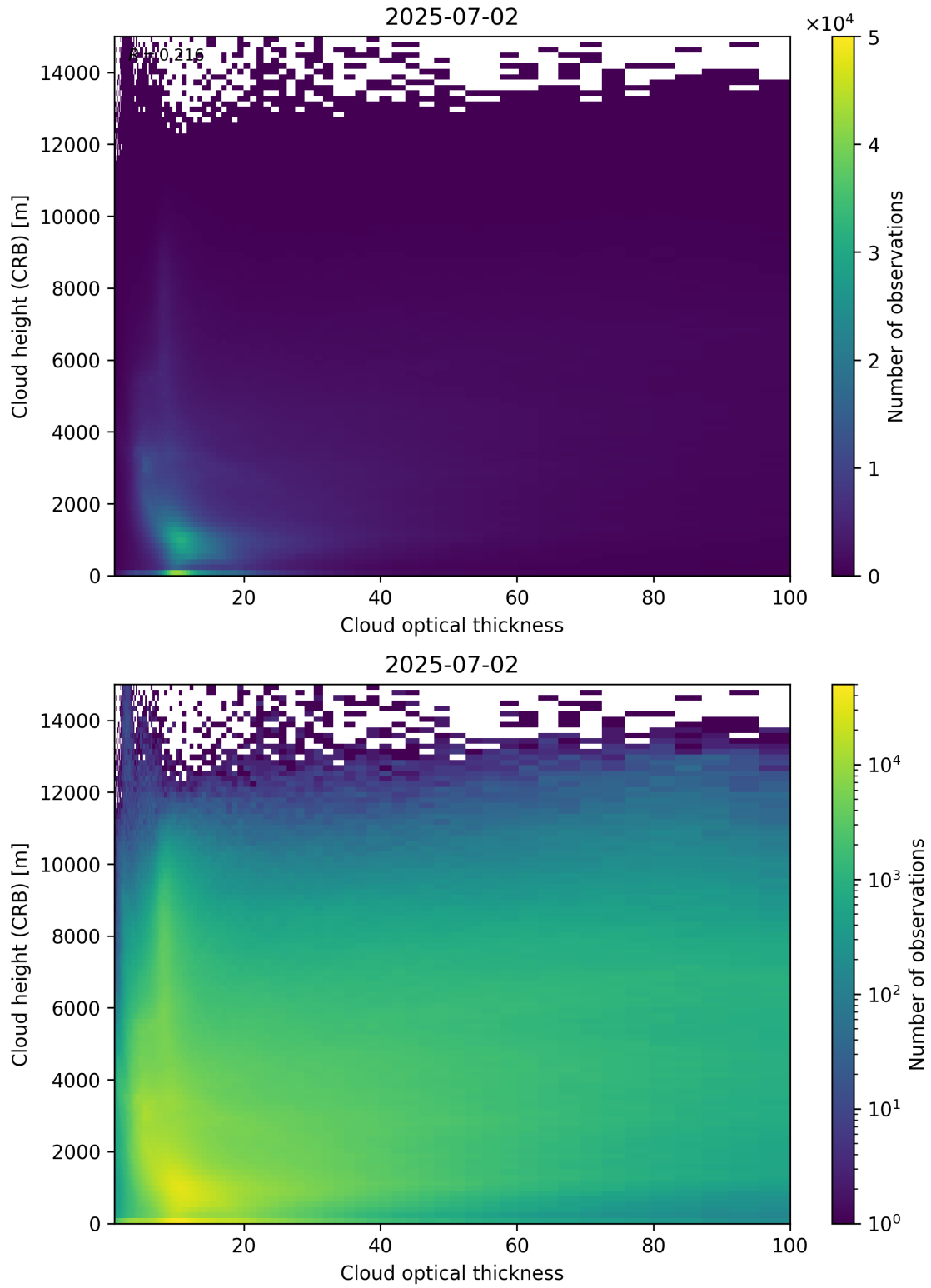
Figure 85: Scatter density plot of “Cloud optical thickness” against “Cloud height (CRB)” for 2025-07-02 to 2025-07-03.
