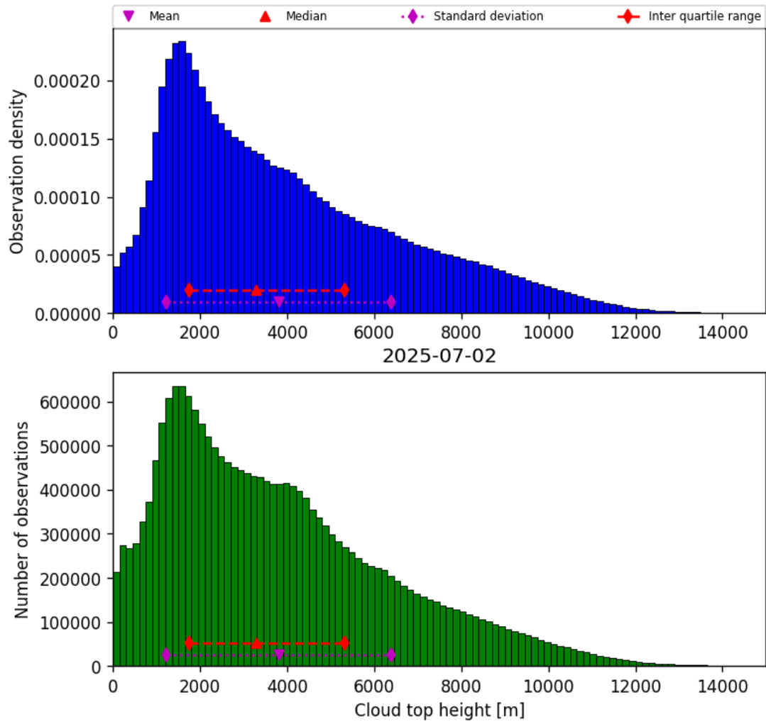
Figure 40: Histogram of “Cloud top height” for 2025-07-02 to 2025-07-03
