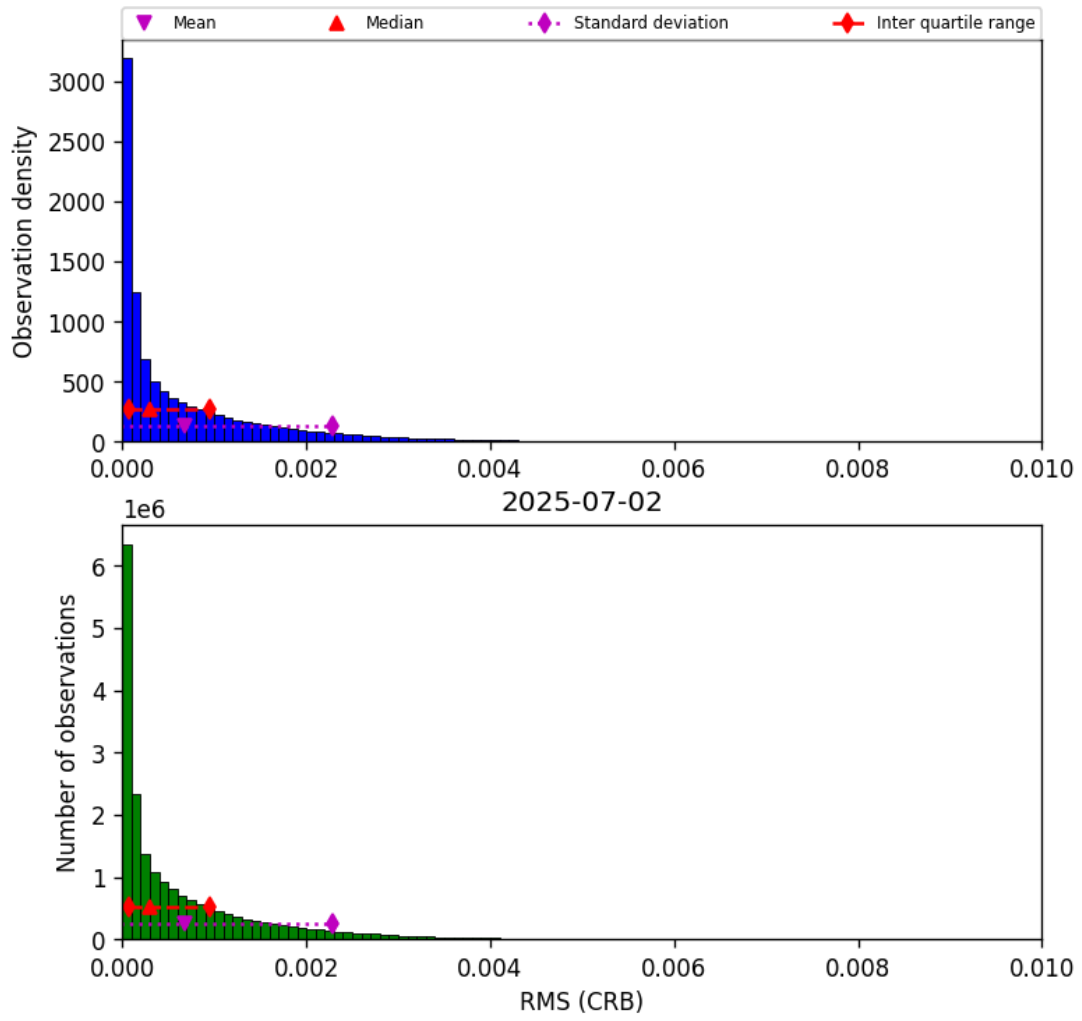
Figure 48: Histogram of “RMS (CRB)” for 2025-07-02 to 2025-07-03
