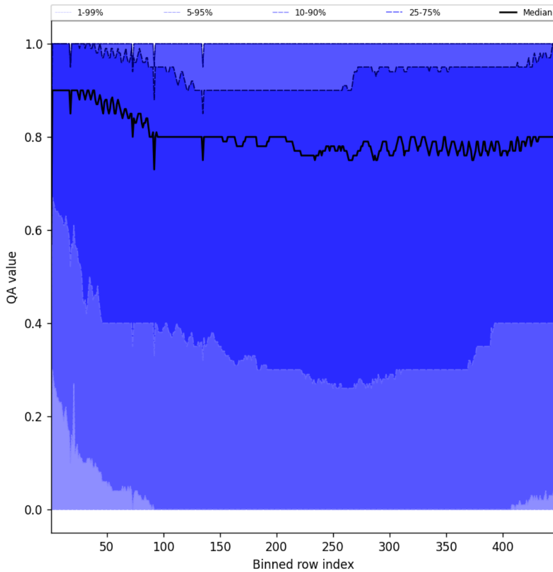
Figure 54: Along track statistics of “QA value” for 2025-07-02 to 2025-07-03
