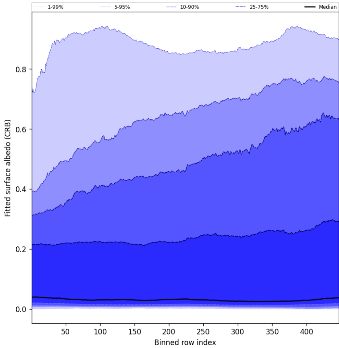
Figure 62: Along track statistics of “Fitted surface albedo (CRB)” for 2025-07-02 to 2025-07-03
