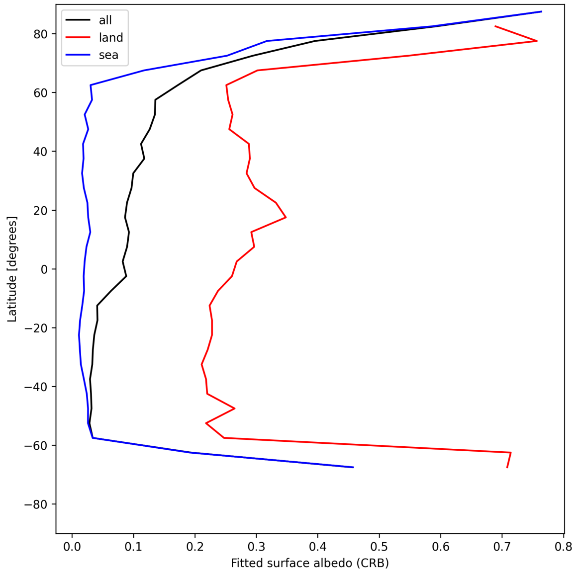
Figure 30: Zonal average of “Fitted surface albedo (CRB)” for 2025-07-02 to 2025-07-03.
