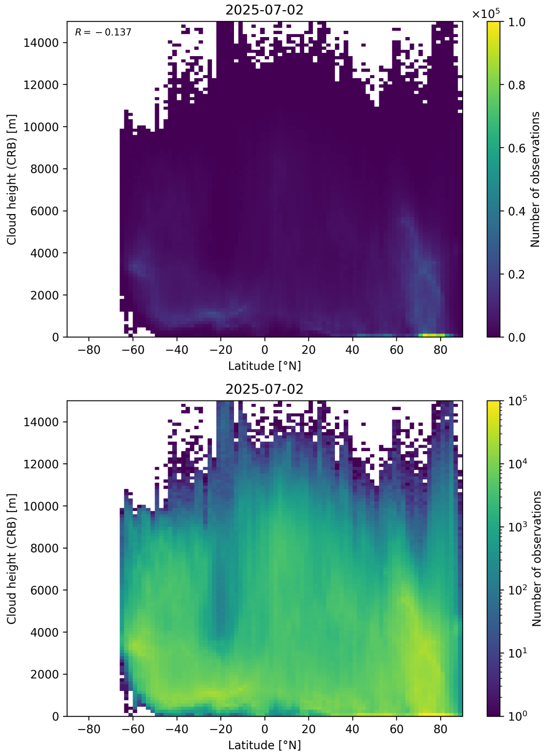
Figure 95: Scatter density plot of “Latitude” against “Cloud height (CRB)” for 2025-07-02 to 2025-07-03.
