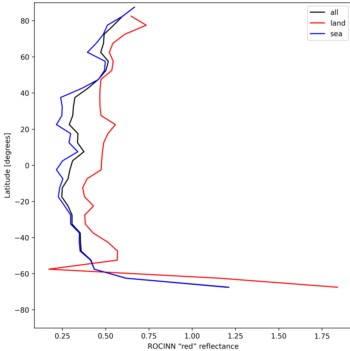
Figure 37: Zonal average of “ROCINN “red” reflectance” for 2025-07-02 to 2025-07-03.
