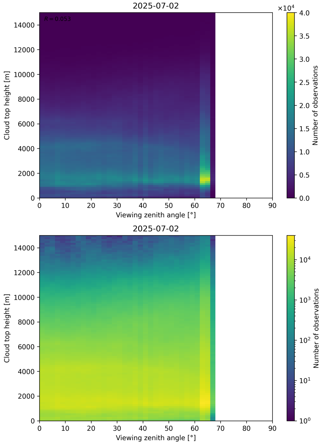
Figure 112: Scatter density plot of “Viewing zenith angle” against “Cloud top height” for 2025-07-02 to 2025-07-03.
