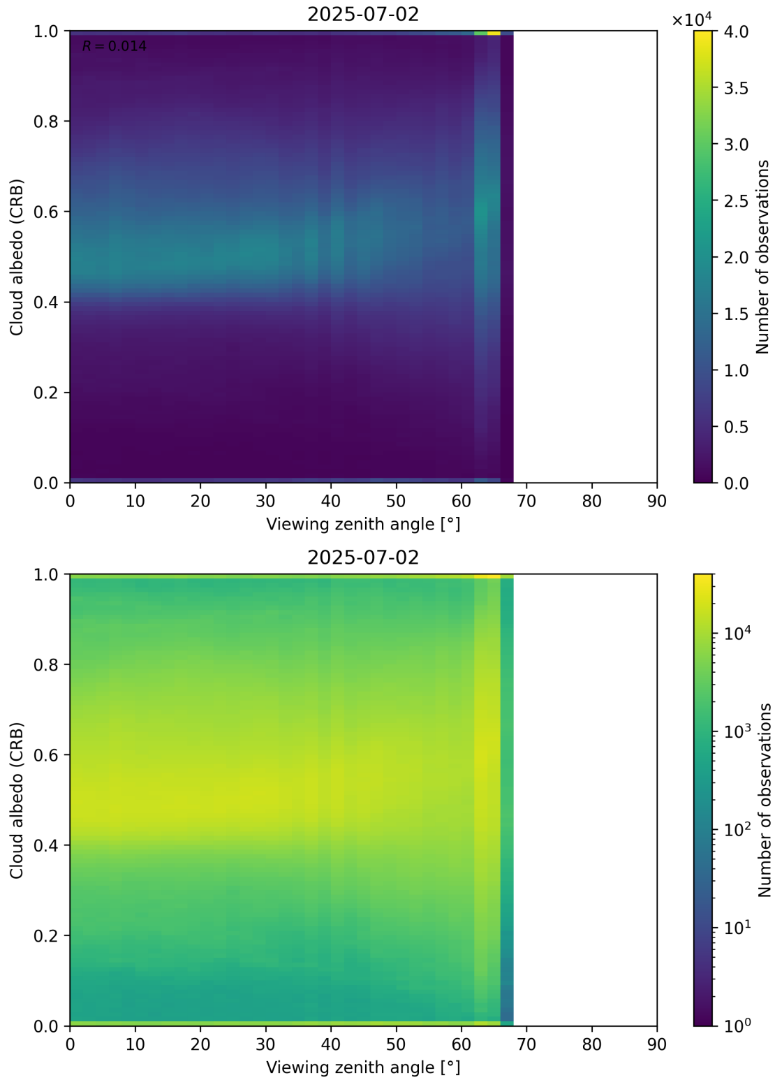
Figure 106: Scatter density plot of “Viewing zenith angle” against “Cloud albedo (CRB)” for 2025-07-02 to 2025-07-03.
