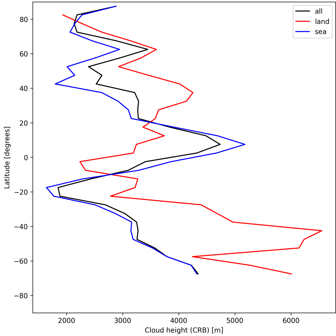
Figure 27: Zonal average of “Cloud height (CRB)” for 2025-07-02 to 2025-07-03.
