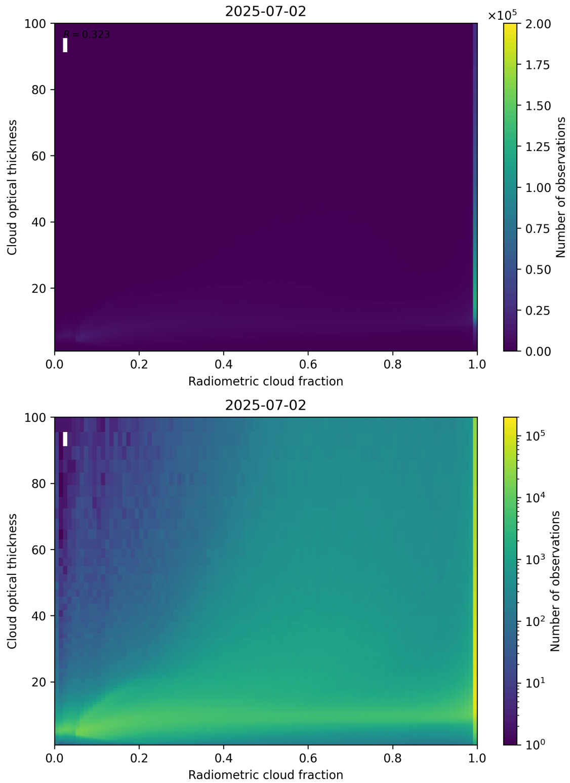
Figure 75: Scatter density plot of “Radiometric cloud fraction” against “Cloud optical thickness” for 2025-07-02 to 2025-07-03.
