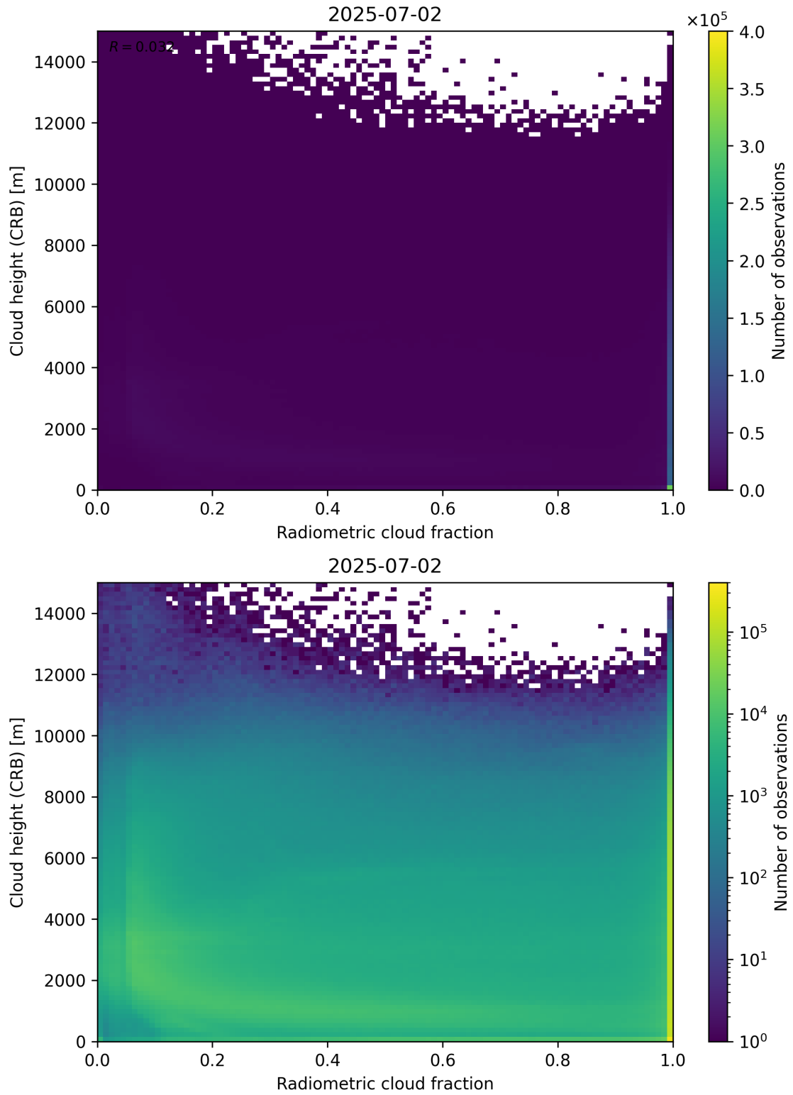
Figure 74: Scatter density plot of “Radiometric cloud fraction” against “Cloud height (CRB)” for 2025-07-02 to 2025-07-03.
