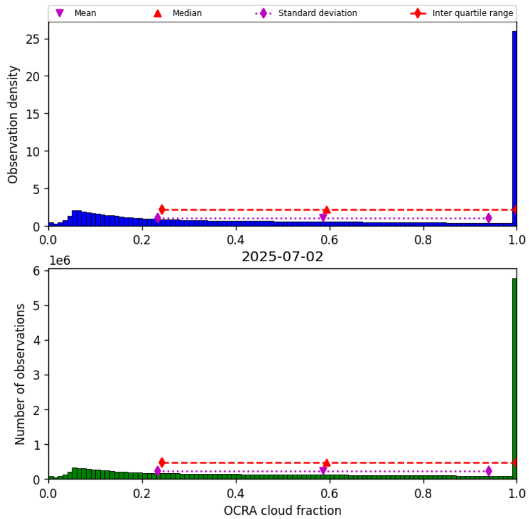
Figure 50: Histogram of “OCRA cloud fraction” for 2025-07-02 to 2025-07-03
