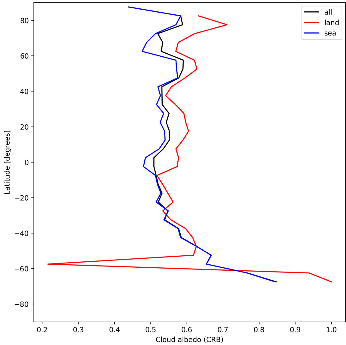
Figure 28: Zonal average of “Cloud albedo (CRB)” for 2025-07-02 to 2025-07-03.
