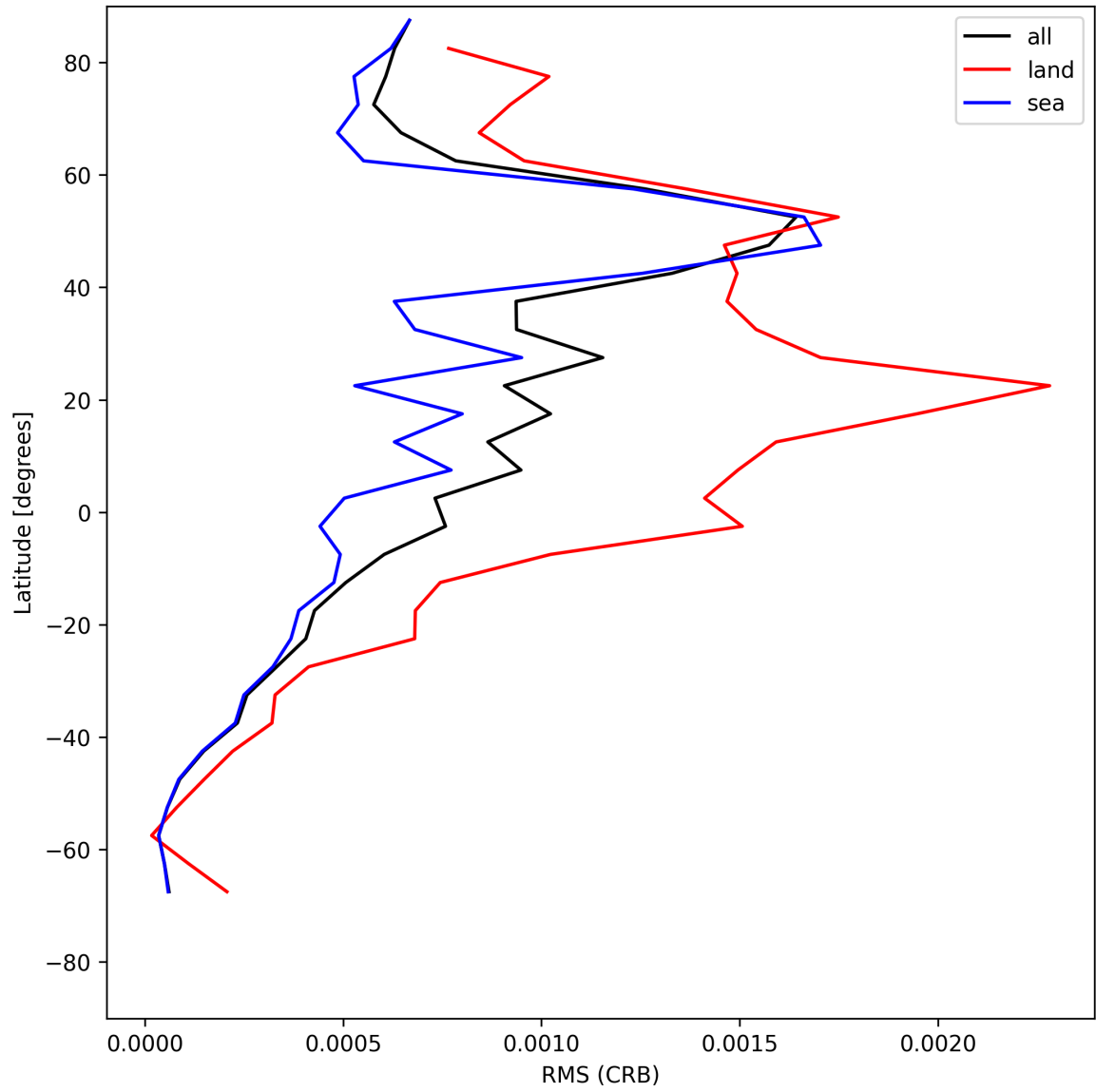
Figure 32: Zonal average of “RMS (CRB)” for 2025-07-02 to 2025-07-03.
