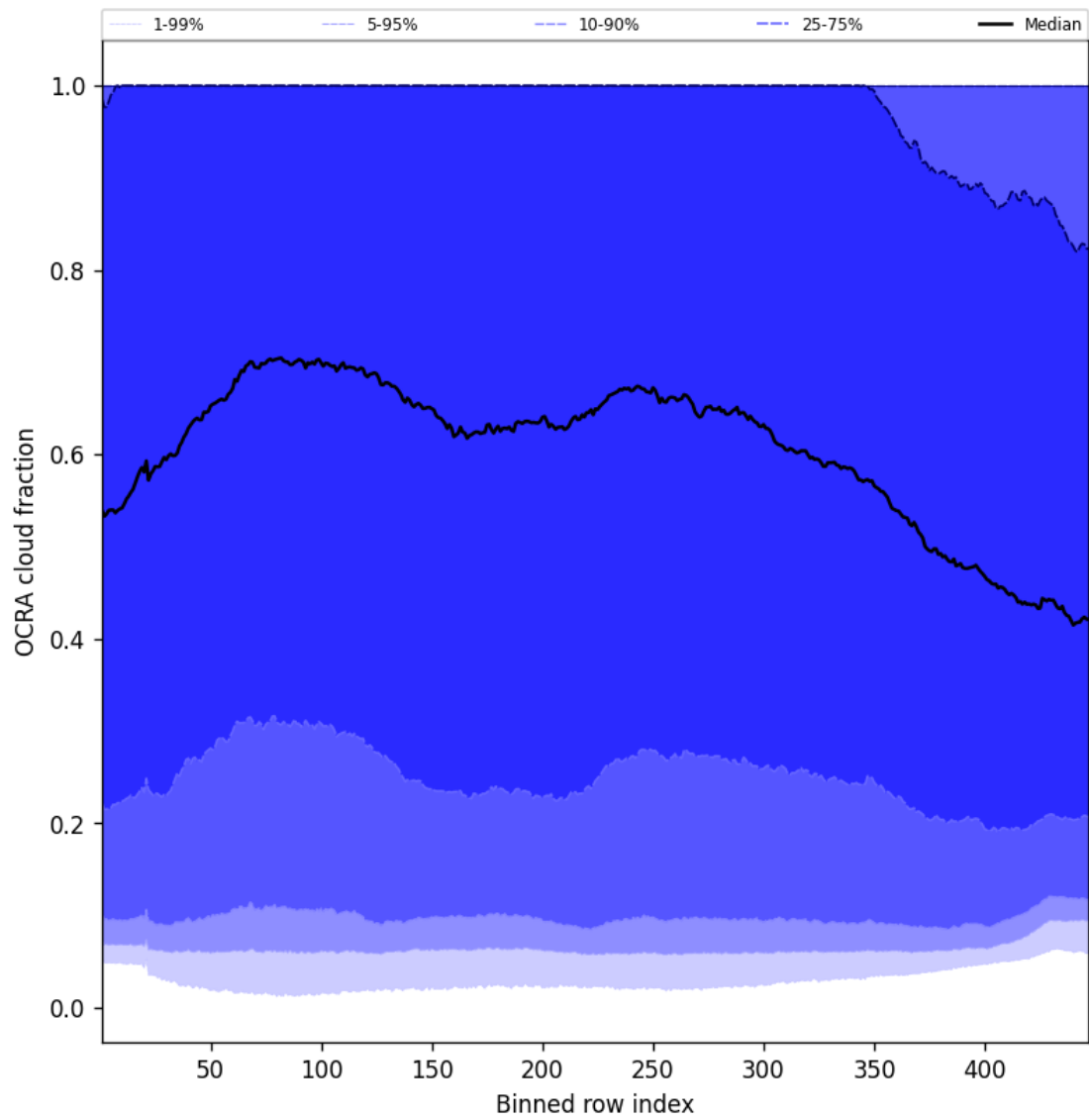
Figure 66: Along track statistics of “OCRA cloud fraction” for 2025-07-02 to 2025-07-03
