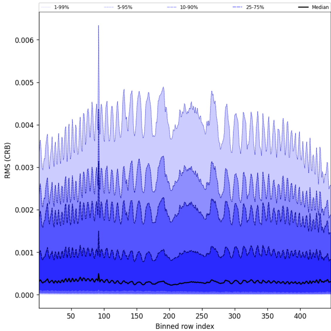
Figure 64: Along track statistics of “RMS (CRB)” for 2025-07-02 to 2025-07-03
