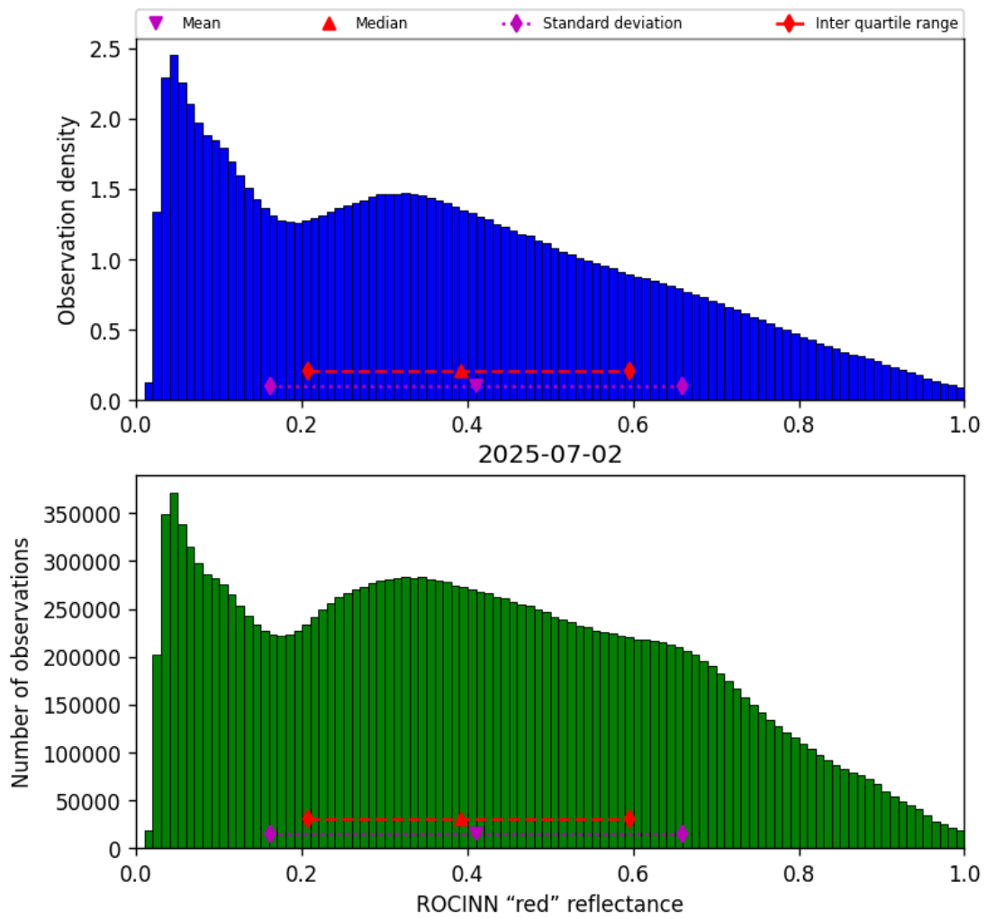
Figure 53: Histogram of “ROCINN “red” reflectance” for 2025-07-02 to 2025-07-03
