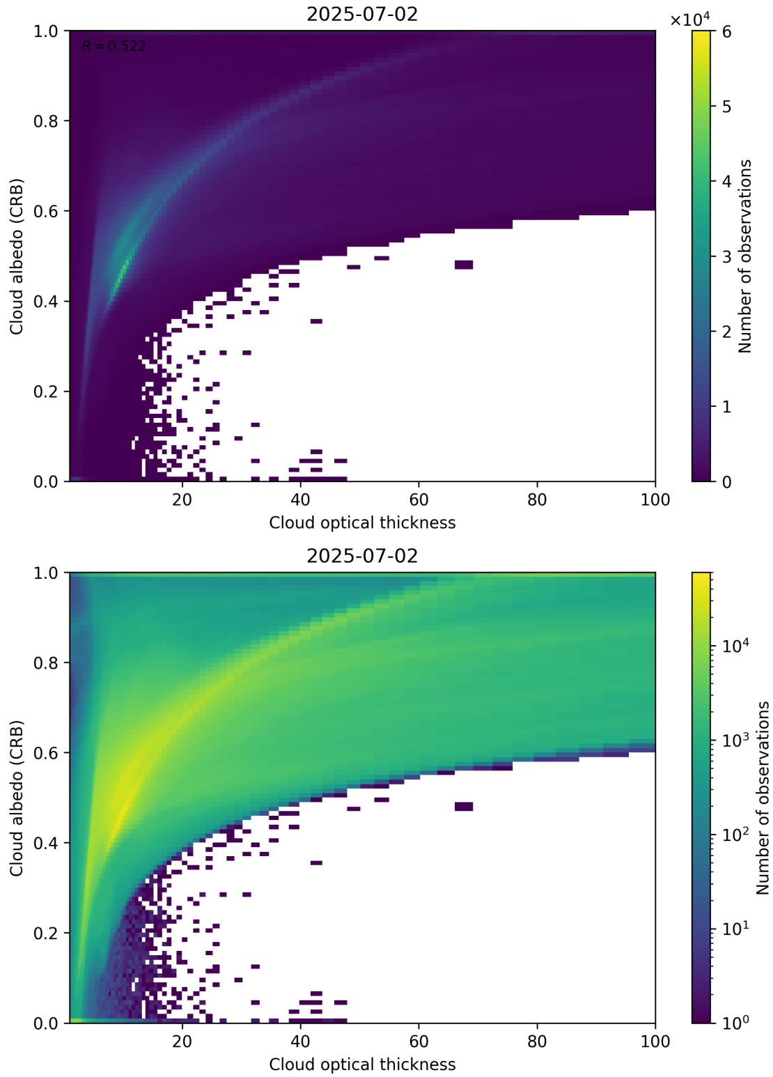
Figure 82: Scatter density plot of “Cloud optical thickness” against “Cloud albedo (CRB)” for 2025-07-02 to 2025-07-03.
