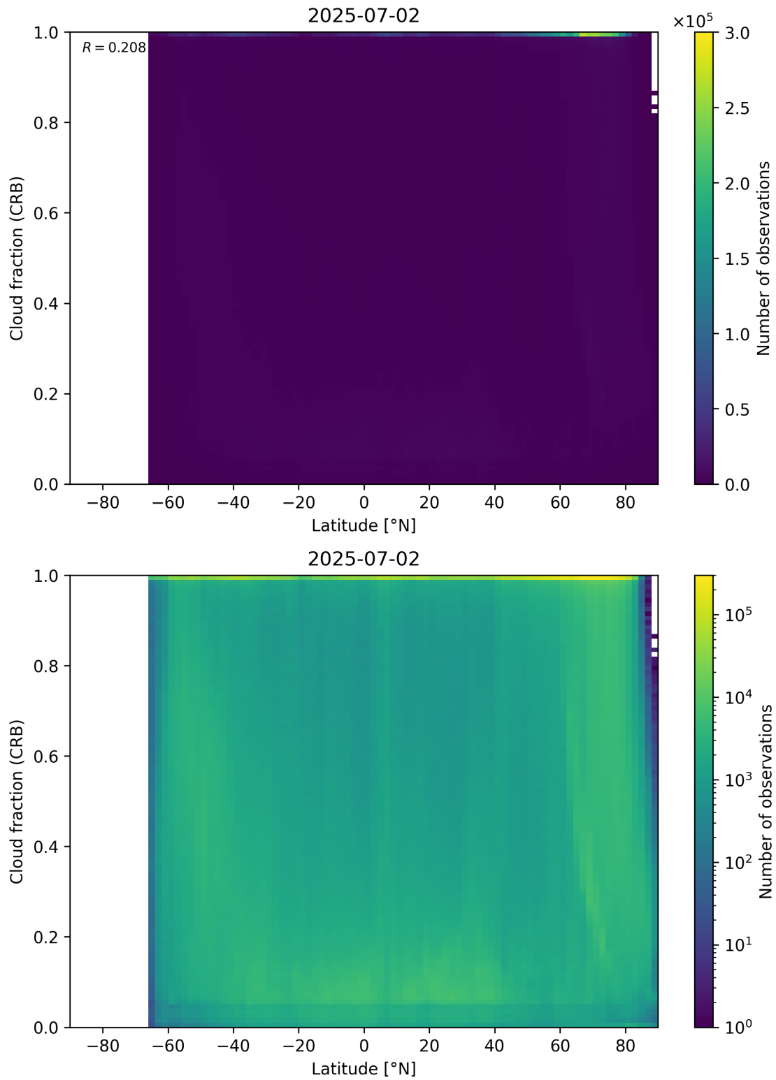
Figure 94: Scatter density plot of “Latitude” against “Cloud fraction (CRB)” for 2025-07-02 to 2025-07-03.
