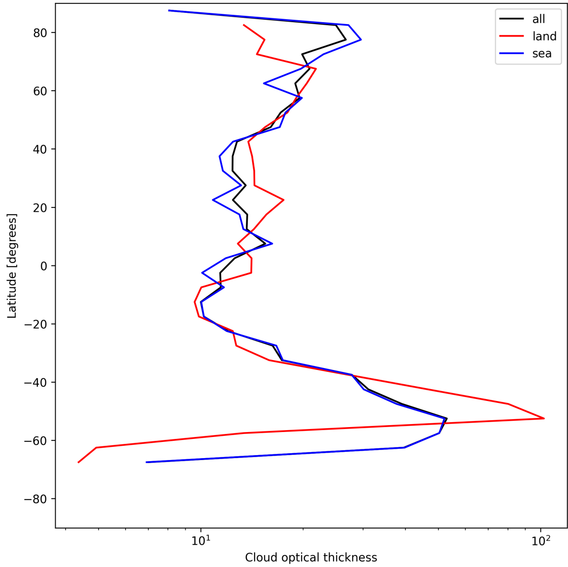
Figure 25: Zonal average of “Cloud optical thickness” for 2025-07-02 to 2025-07-03.
