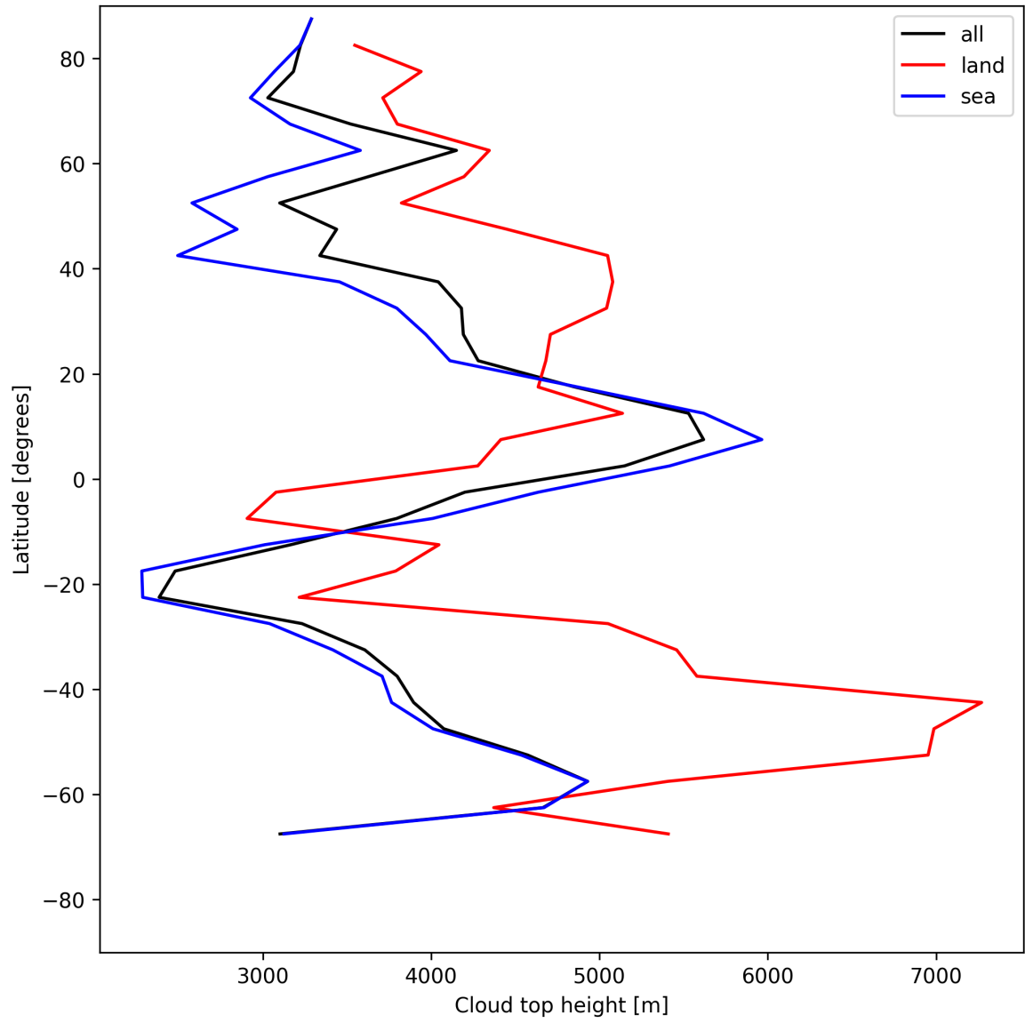
Figure 24: Zonal average of “Cloud top height” for 2025-07-02 to 2025-07-03.
