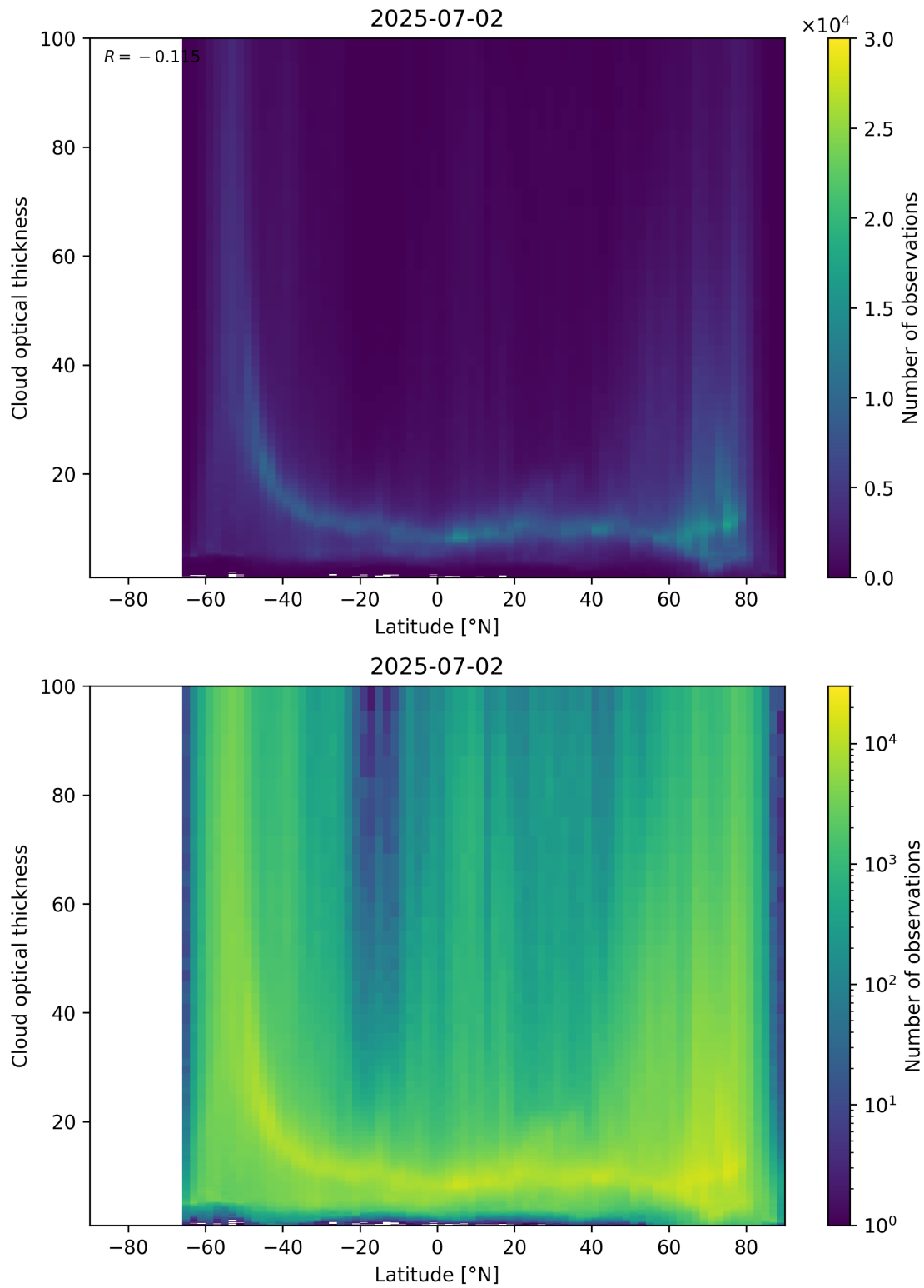
Figure 96: Scatter density plot of “Latitude” against “Cloud optical thickness” for 2025-07-02 to 2025-07-03.
