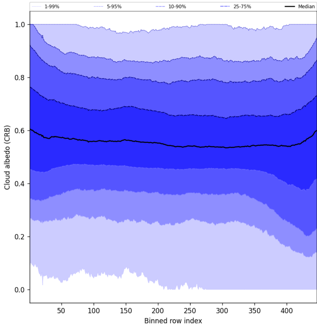
Figure 60: Along track statistics of “Cloud albedo (CRB)” for 2025-07-02 to 2025-07-03
