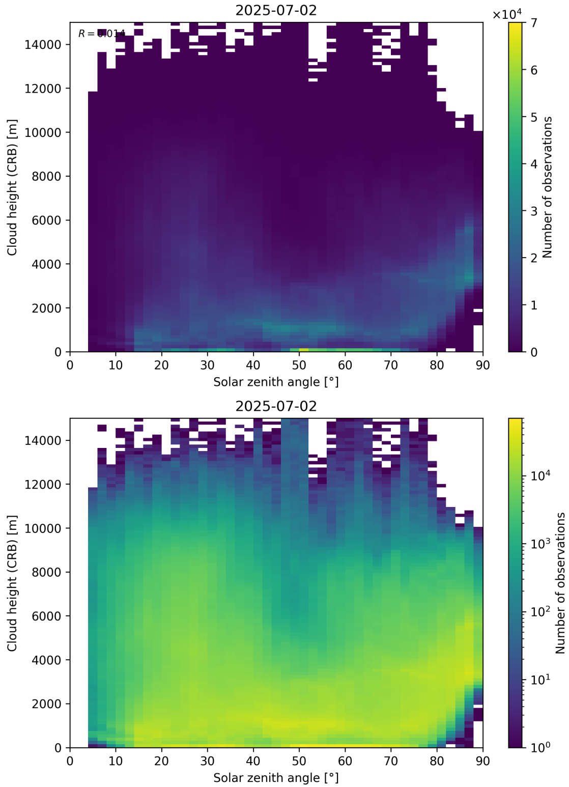
Figure 102: Scatter density plot of “Solar zenith angle” against “Cloud height (CRB)” for 2025-07-02 to 2025-07-03.
