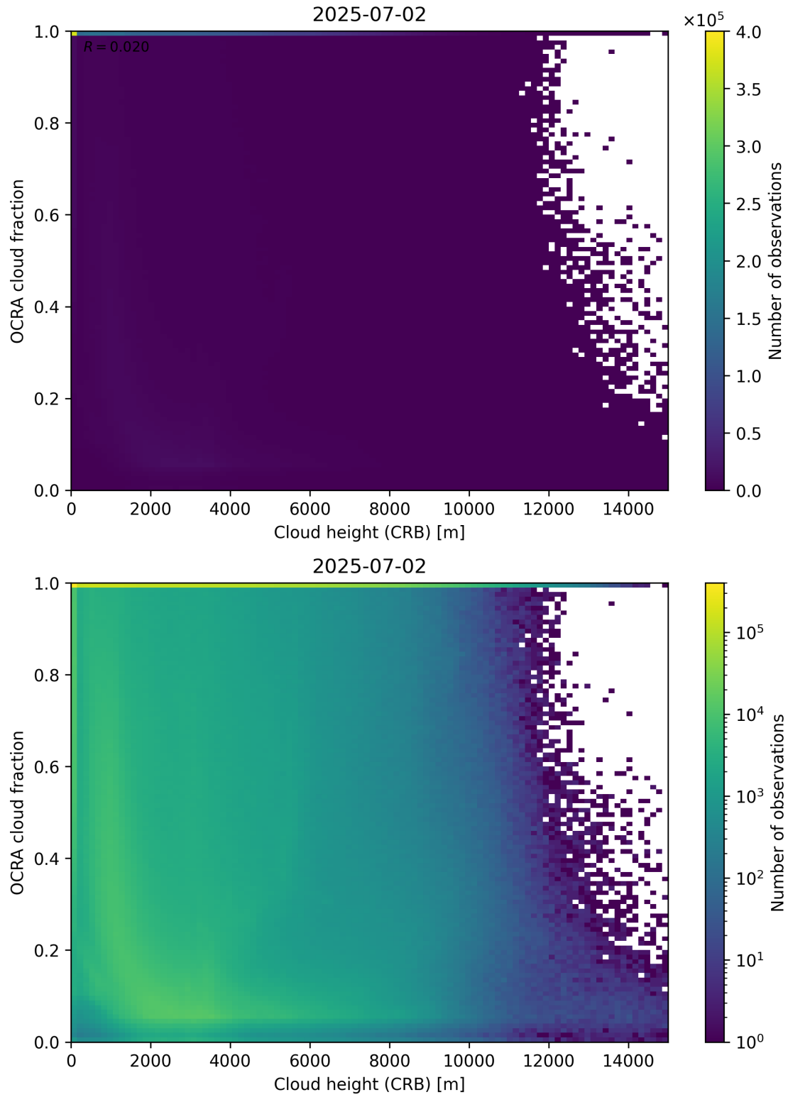
Figure 81: Scatter density plot of “Cloud height (CRB)” against “OCRA cloud fraction” for 2025-07-02 to 2025-07-03.
