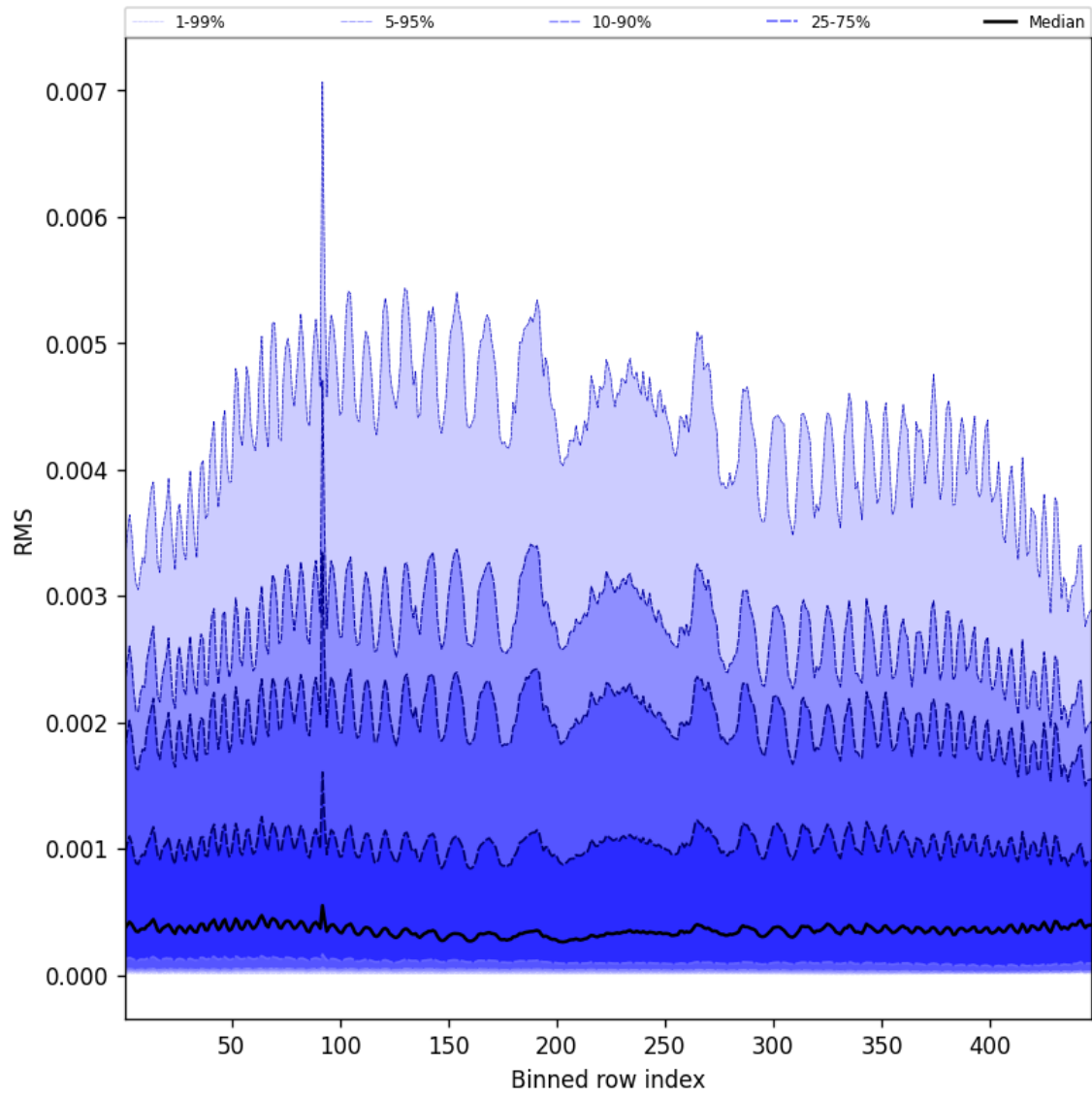
Figure 63: Along track statistics of “RMS” for 2025-07-02 to 2025-07-03
