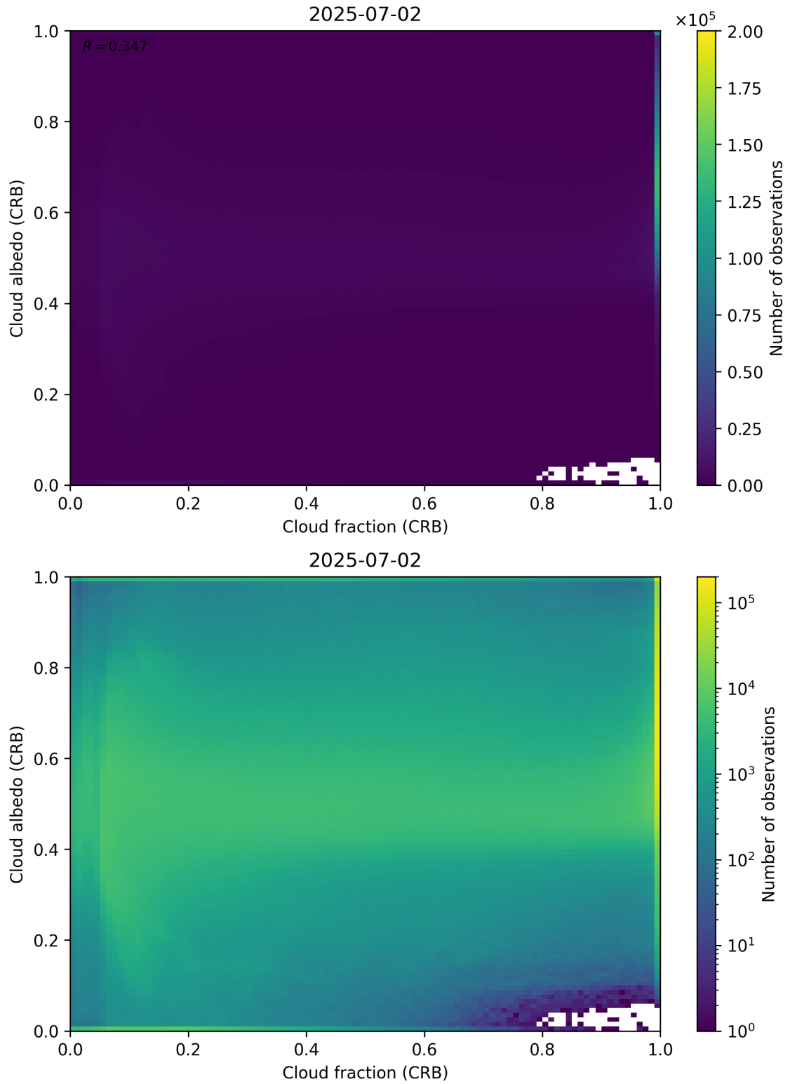
Figure 77: Scatter density plot of “Cloud fraction (CRB)” against “Cloud albedo (CRB)” for 2025-07-02 to 2025-07-03.
