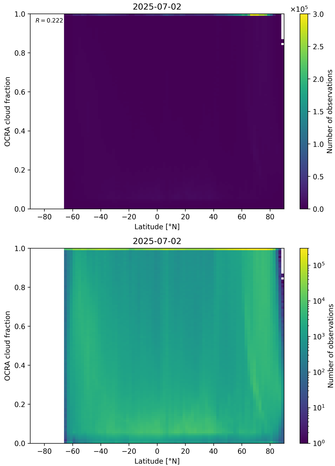
Figure 93: Scatter density plot of “Latitude” against “OCRA cloud fraction” for 2025-07-02 to 2025-07-03.
