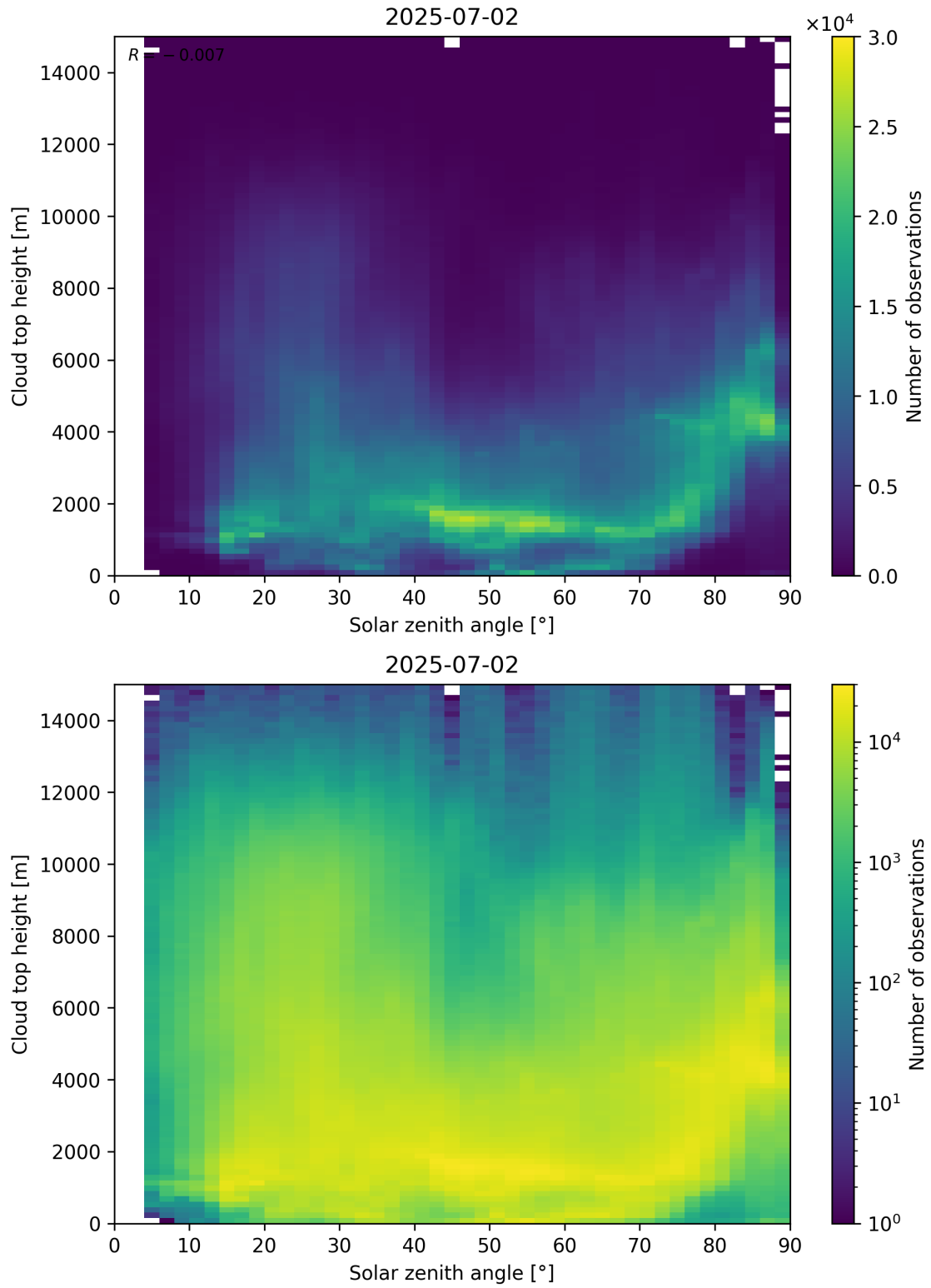
Figure 104: Scatter density plot of “Solar zenith angle” against “Cloud top height” for 2025-07-02 to 2025-07-03.
