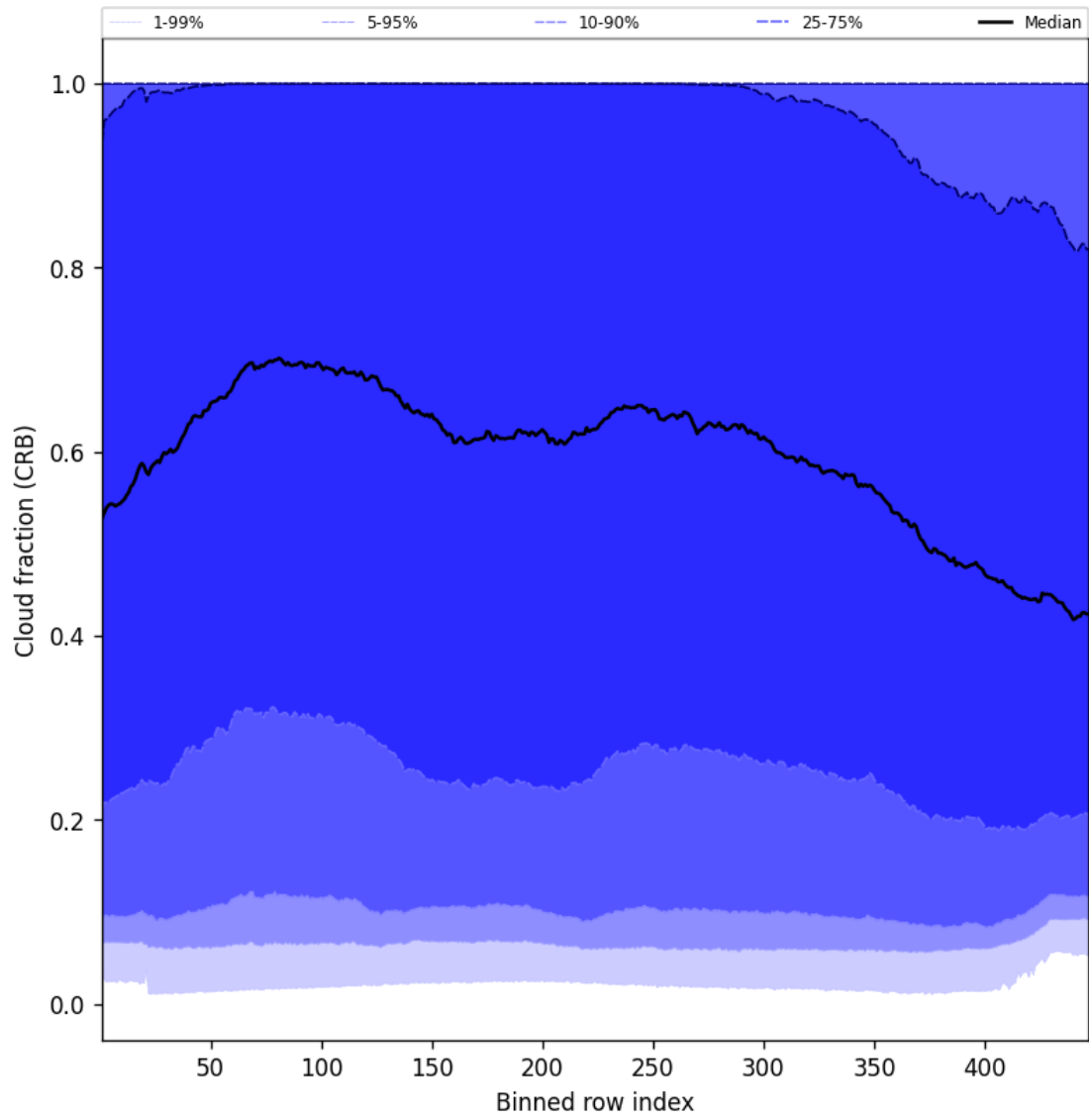
Figure 58: Along track statistics of “Cloud fraction (CRB)” for 2025-07-02 to 2025-07-03
