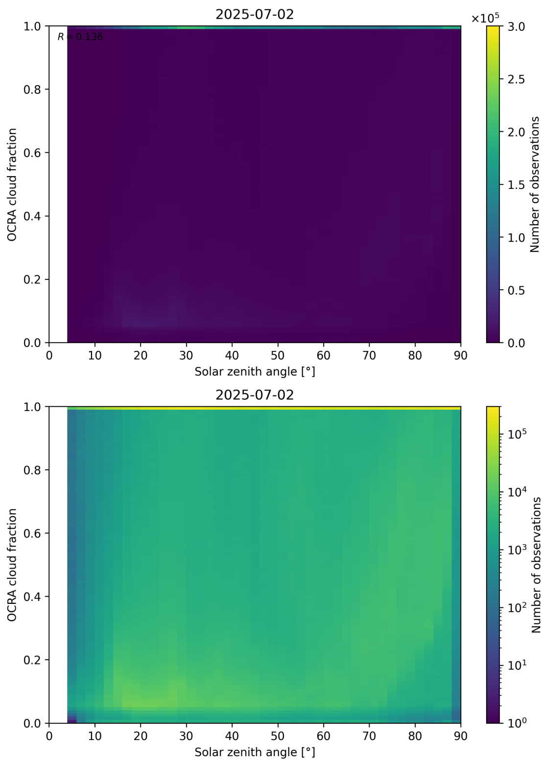
Figure 100: Scatter density plot of “Solar zenith angle” against “OCRA cloud fraction” for 2025-07-02 to 2025-07-03.
