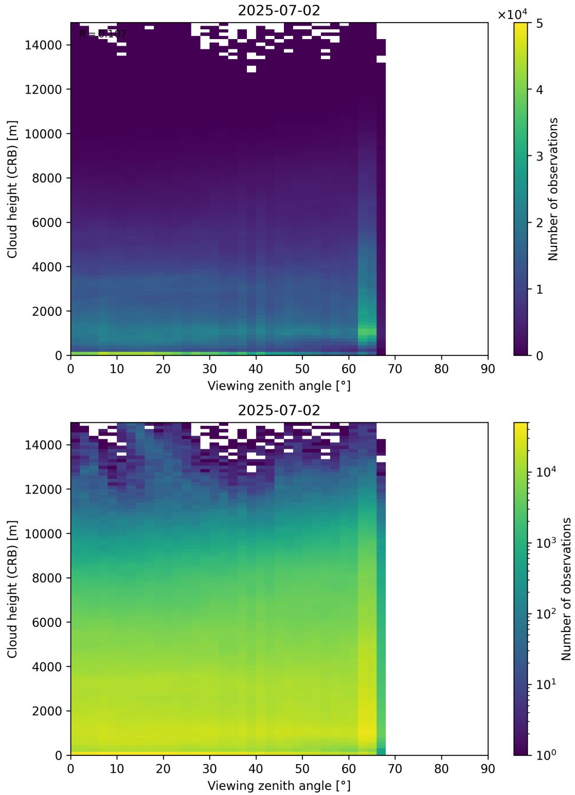
Figure 110: Scatter density plot of “Viewing zenith angle” against “Cloud height (CRB)” for 2025-07-02 to 2025-07-03.
