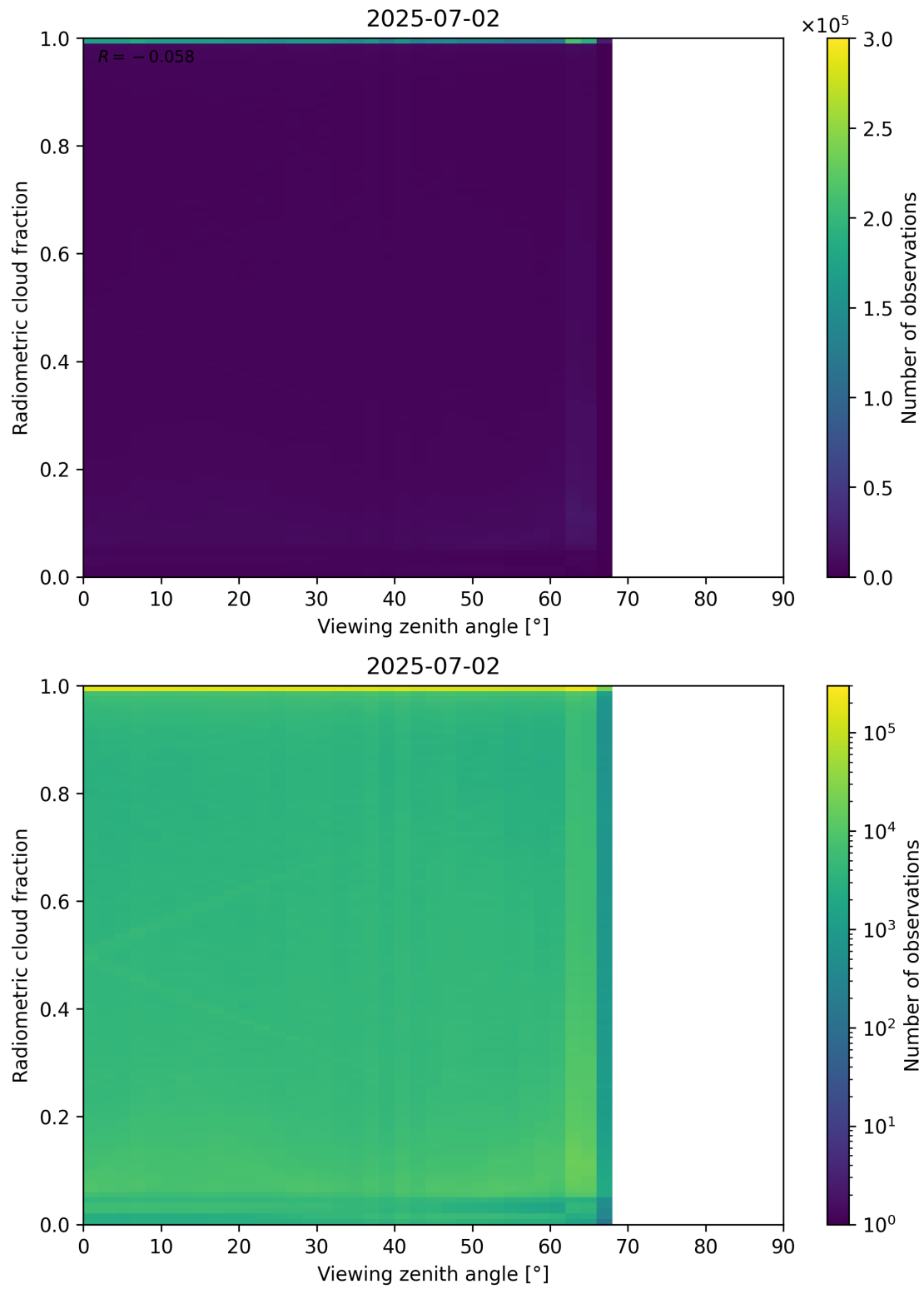
Figure 107: Scatter density plot of “Viewing zenith angle” against “Radiometric cloud fraction” for 2025-07-02 to 2025-07-03.
