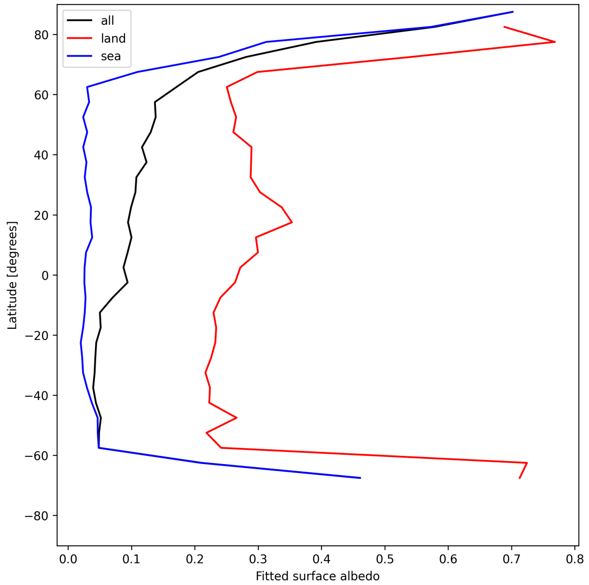
Figure 29: Zonal average of “Fitted surface albedo” for 2025-07-02 to 2025-07-03.
