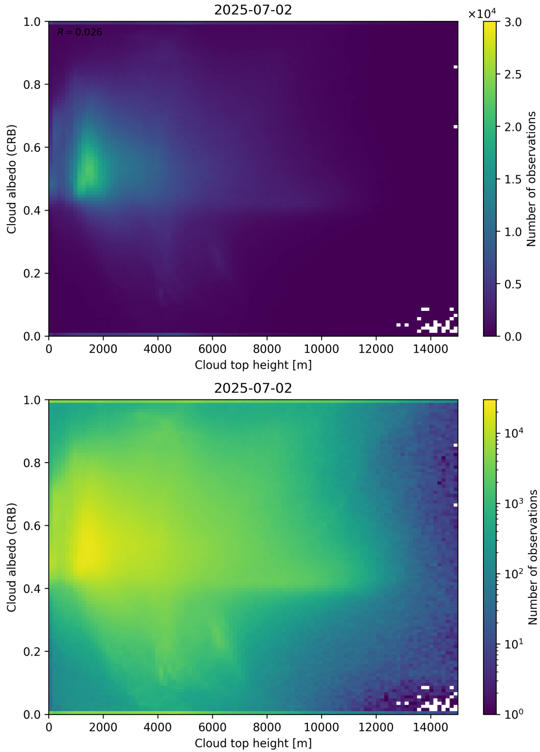
Figure 86: Scatter density plot of “Cloud top height” against “Cloud albedo (CRB)” for 2025-07-02 to 2025-07-03.
