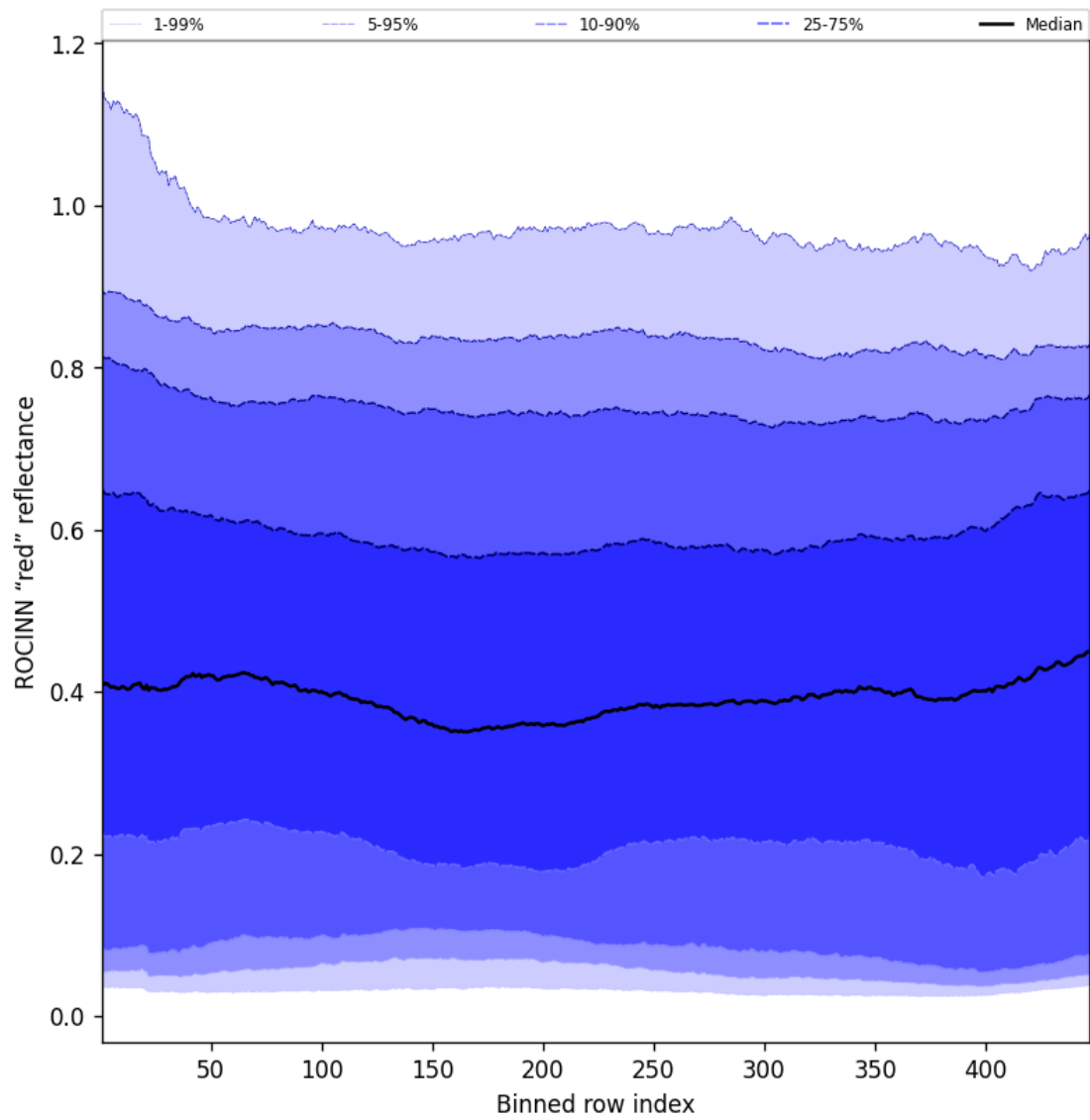
Figure 69: Along track statistics of “ROCINN “red” reflectance” for 2025-07-02 to 2025-07-03
