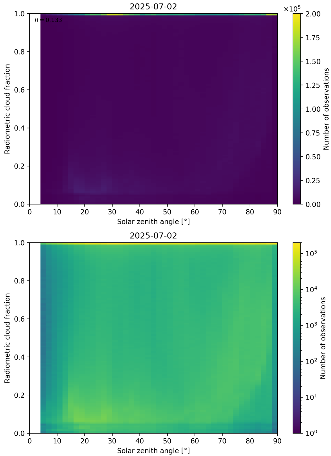
Figure 99: Scatter density plot of “Solar zenith angle” against “Radiometric cloud fraction” for 2025-07-02 to 2025-07-03.
