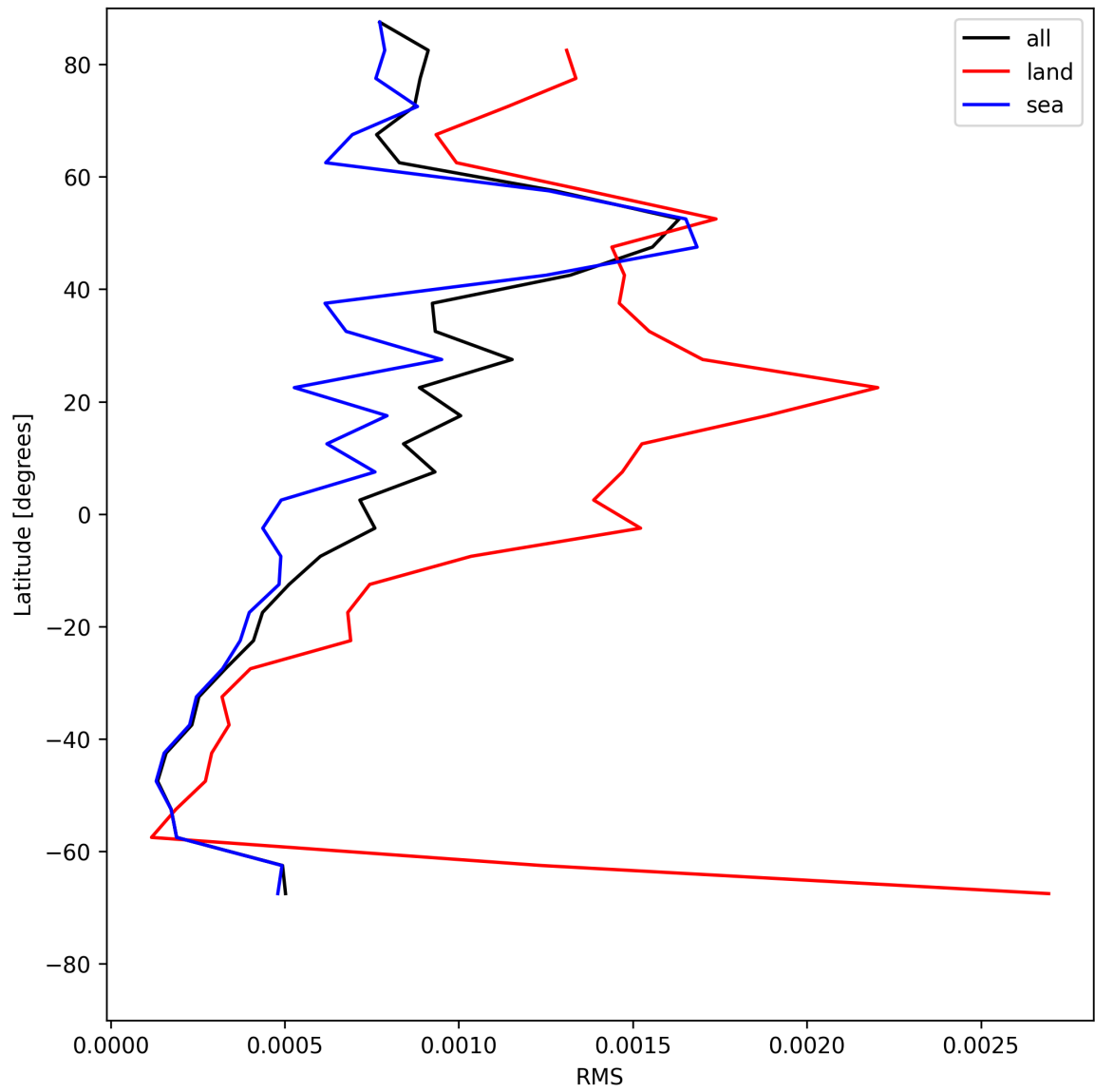
Figure 31: Zonal average of “RMS” for 2025-07-02 to 2025-07-03.
