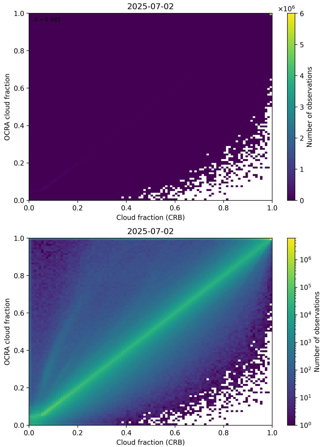
Figure 78: Scatter density plot of “Cloud fraction (CRB)” against “OCRA cloud fraction” for 2025-07-02 to 2025-07-03.
