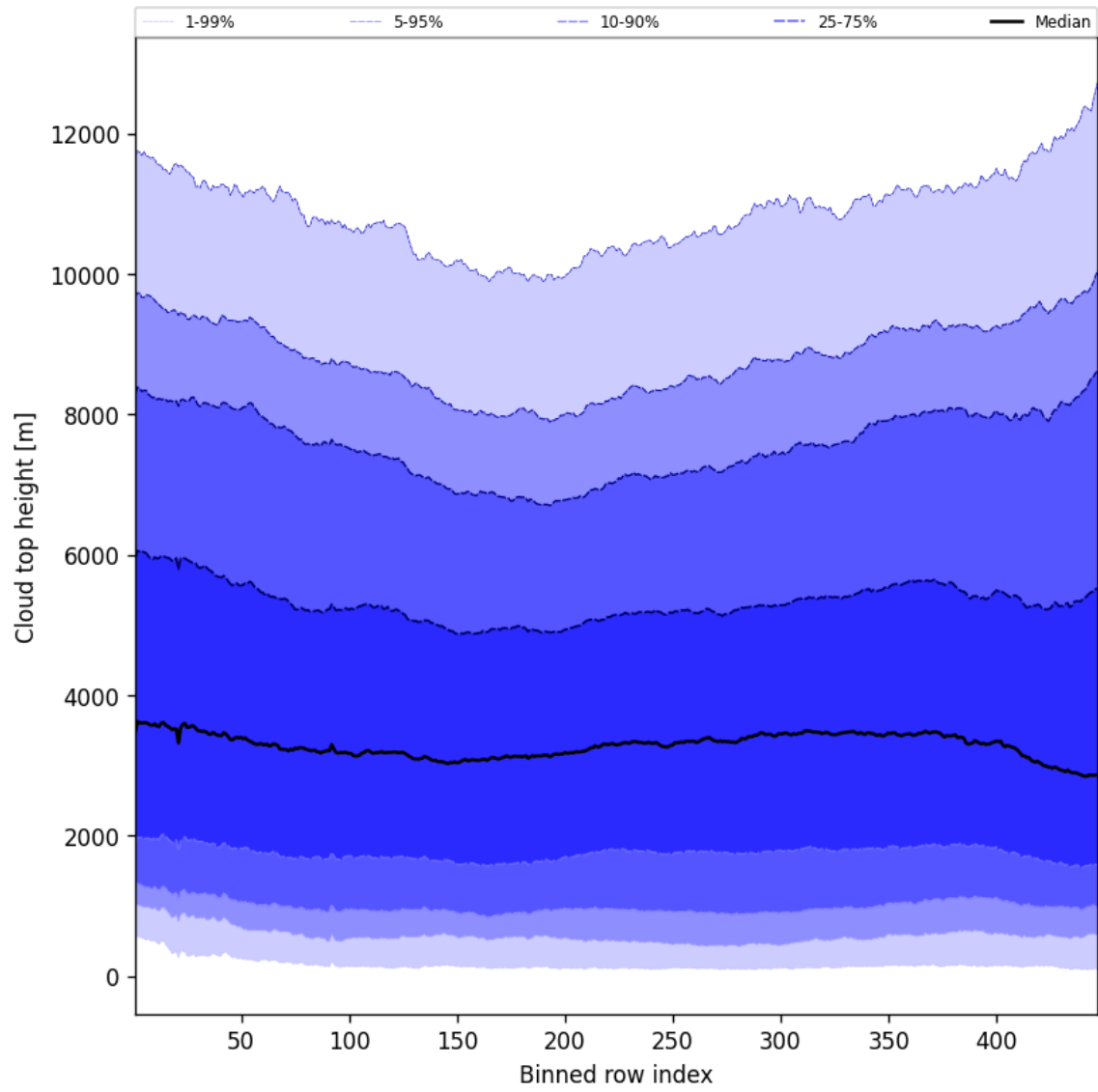
Figure 56: Along track statistics of “Cloud top height” for 2025-07-02 to 2025-07-03
