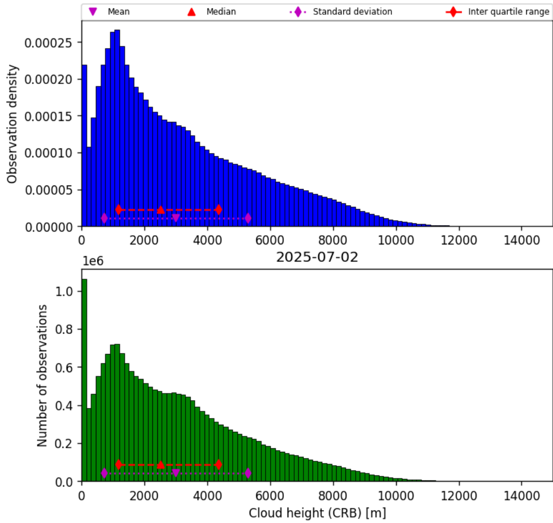
Figure 43: Histogram of “Cloud height (CRB)” for 2025-07-02 to 2025-07-03
