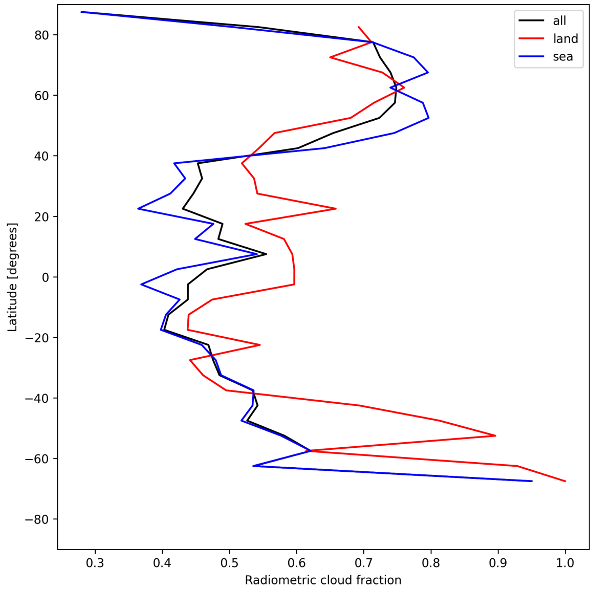
Figure 23: Zonal average of “Radiometric cloud fraction” for 2025-07-02 to 2025-07-03.
