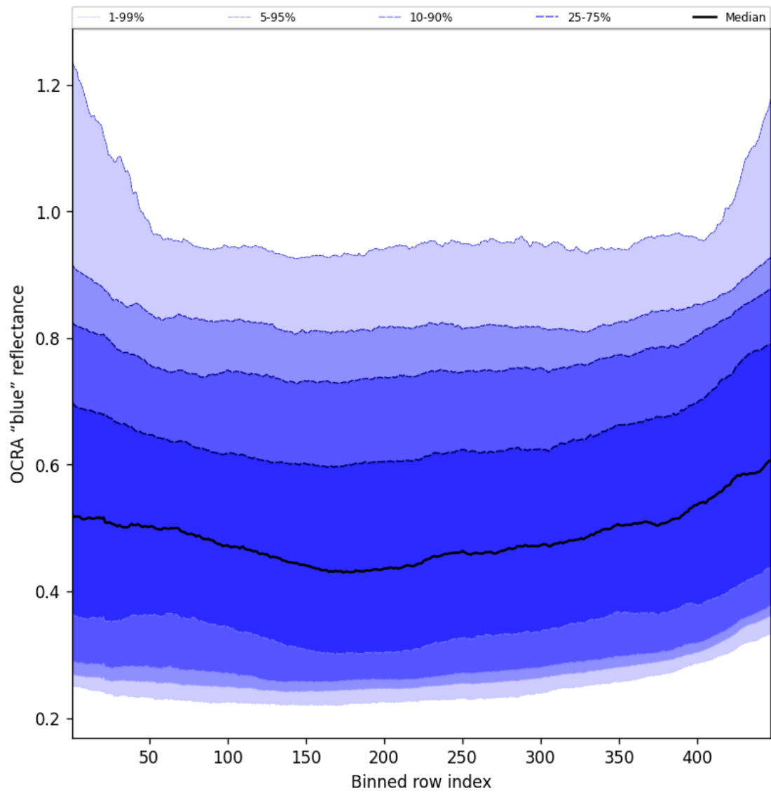
Figure 67: Along track statistics of "OCRA "blue" reflectance" for 2025-07-02 to 2025-07-03
