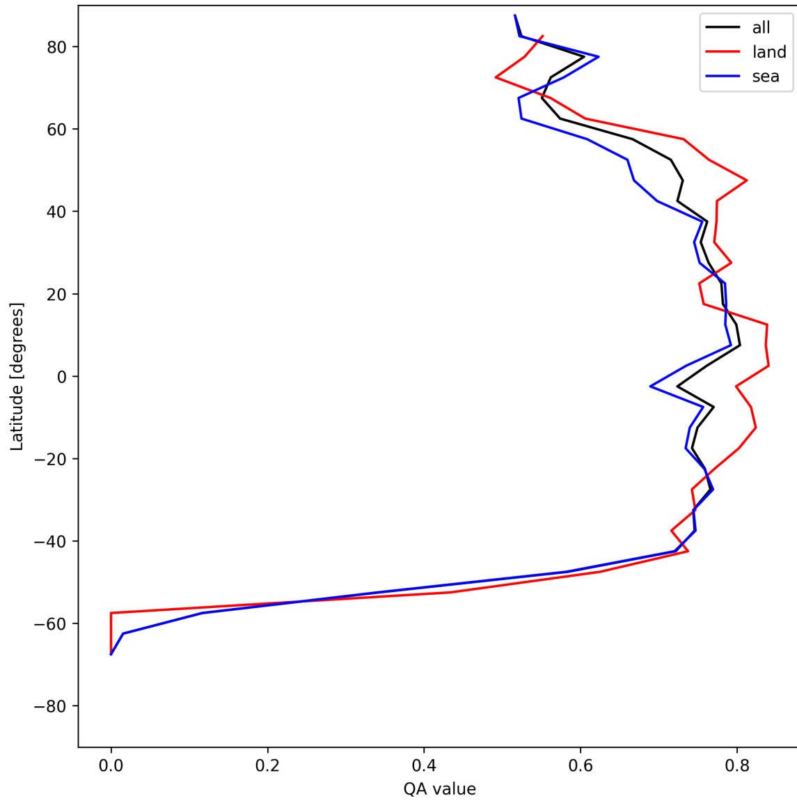
Figure 22: Zonal average of “QA value” for 2025-07-02 to 2025-07-03.
