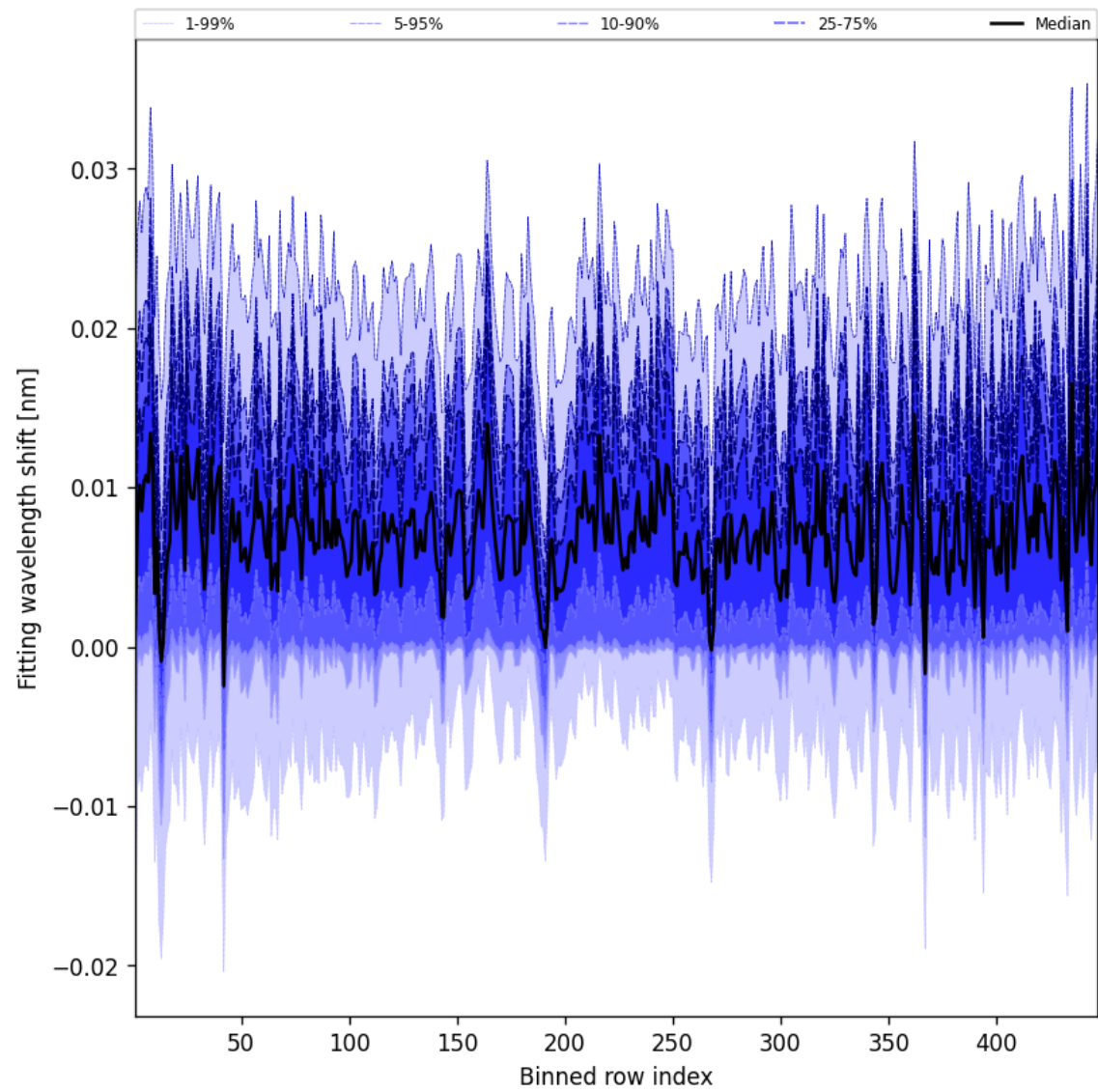
Figure 65: Along track statistics of “Fitting wavelength shift” for 2025-07-02 to 2025-07-03
