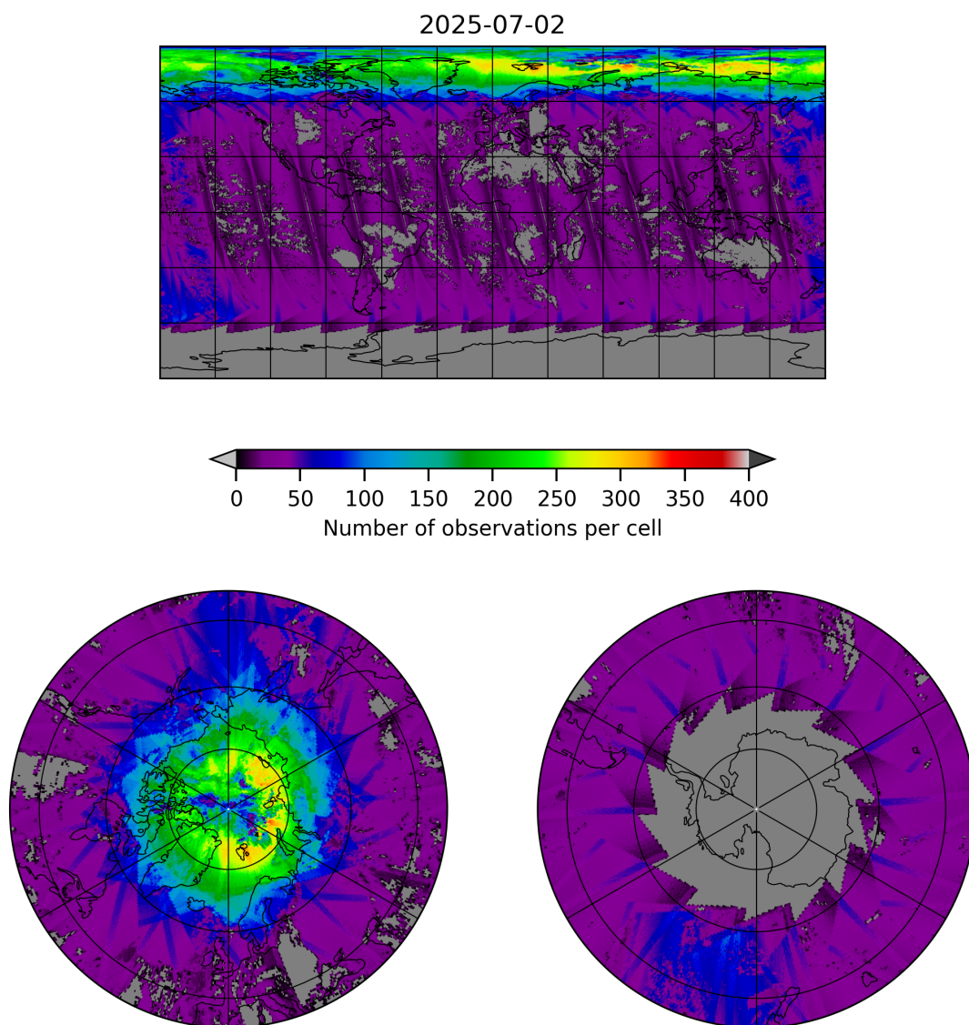
Figure 21: Map of the number of observations for 2025-07-02 to 2025-07-03
