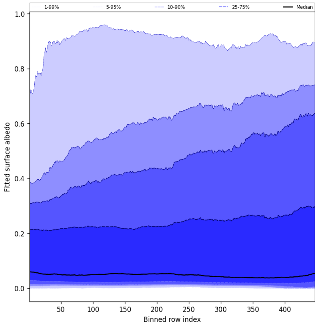
Figure 61: Along track statistics of “Fitted surface albedo” for 2025-07-02 to 2025-07-03
