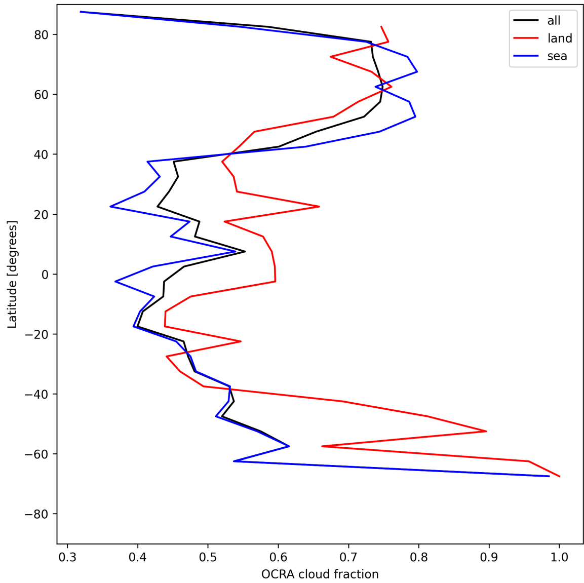
Figure 34: Zonal average of “OCRA cloud fraction” for 2025-07-02 to 2025-07-03.
