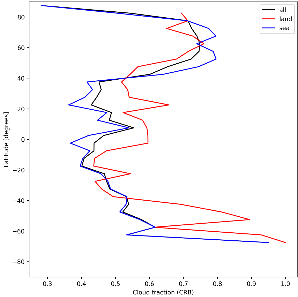
Figure 26: Zonal average of “Cloud fraction (CRB)” for 2025-07-02 to 2025-07-03.
