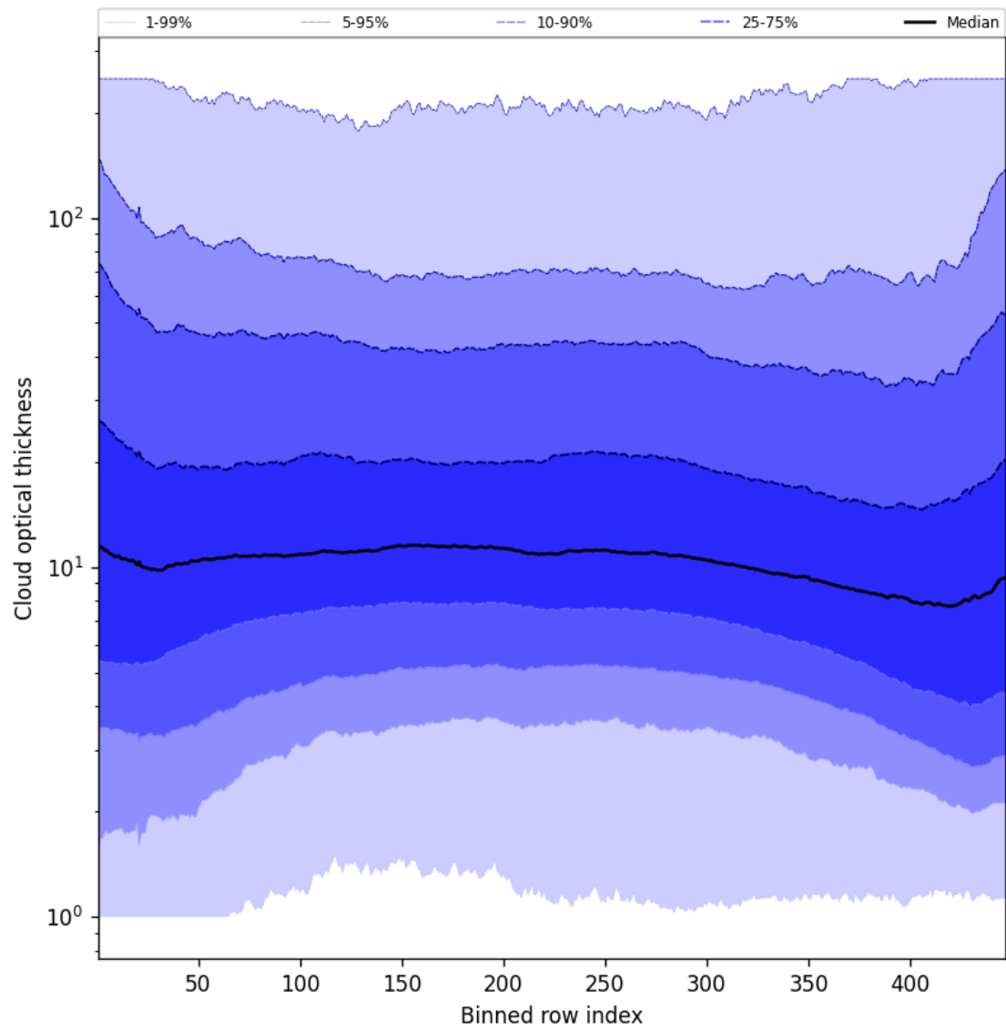
Figure 57: Along track statistics of “Cloud optical thickness” for 2025-07-02 to 2025-07-03
