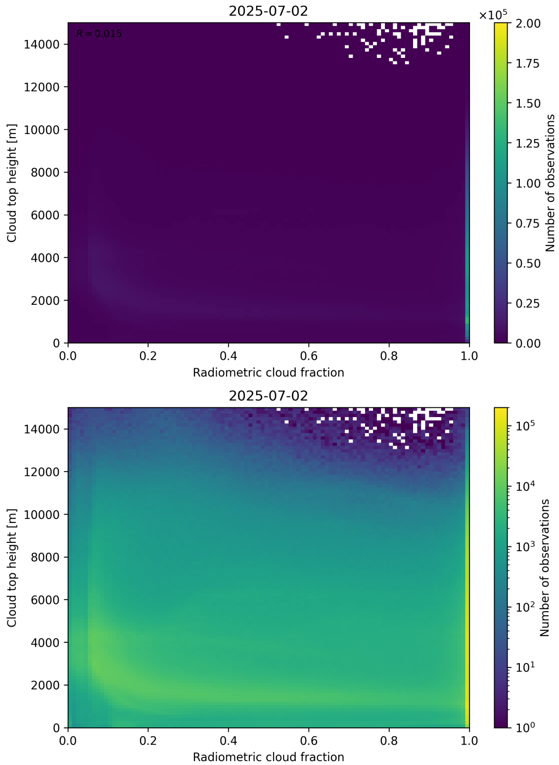
Figure 76: Scatter density plot of “Radiometric cloud fraction” against “Cloud top height” for 2025-07-02 to 2025-07-03.
