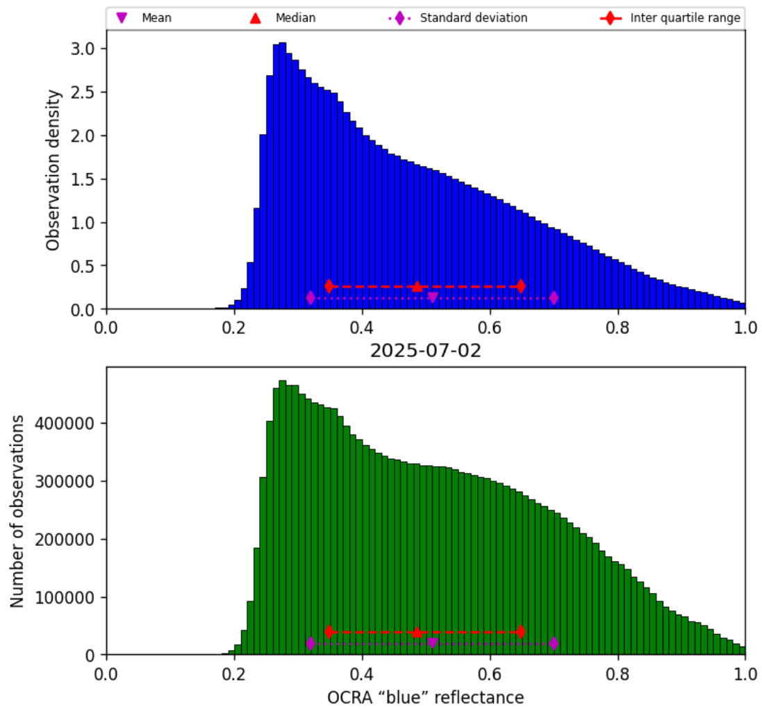
Figure 51: Histogram of “OCRA “blue” reflectance” for 2025-07-02 to 2025-07-03
