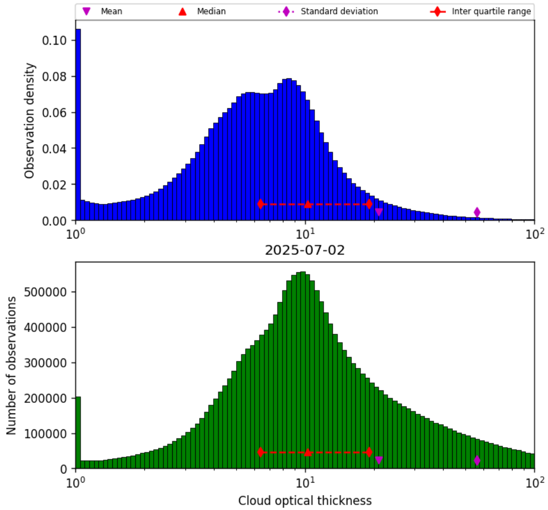
Figure 41: Histogram of “Cloud optical thickness” for 2025-07-02 to 2025-07-03
