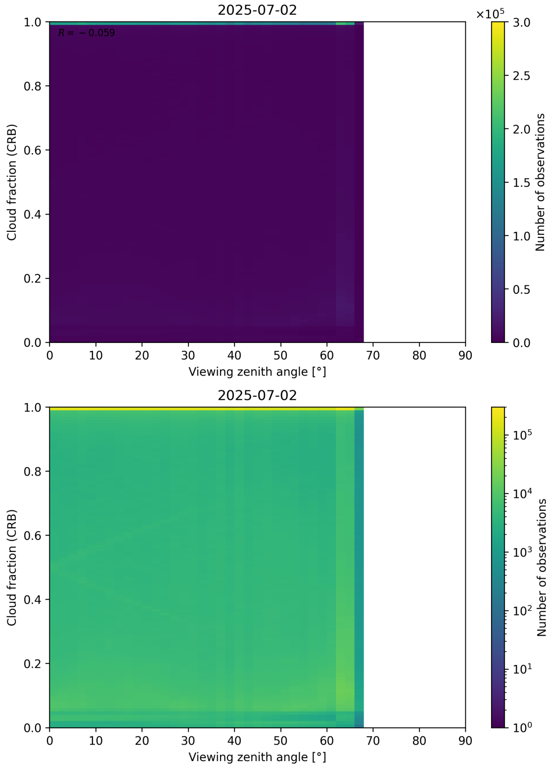
Figure 109: Scatter density plot of “Viewing zenith angle” against “Cloud fraction (CRB)” for 2025-07-02 to 2025-07-03.
