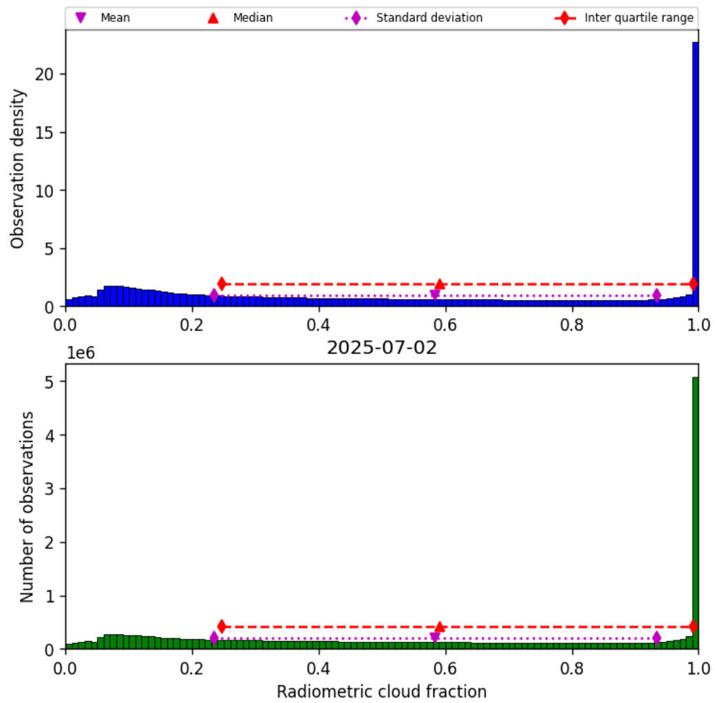
Figure 39: Histogram of “Radiometric cloud fraction” for 2025-07-02 to 2025-07-03
