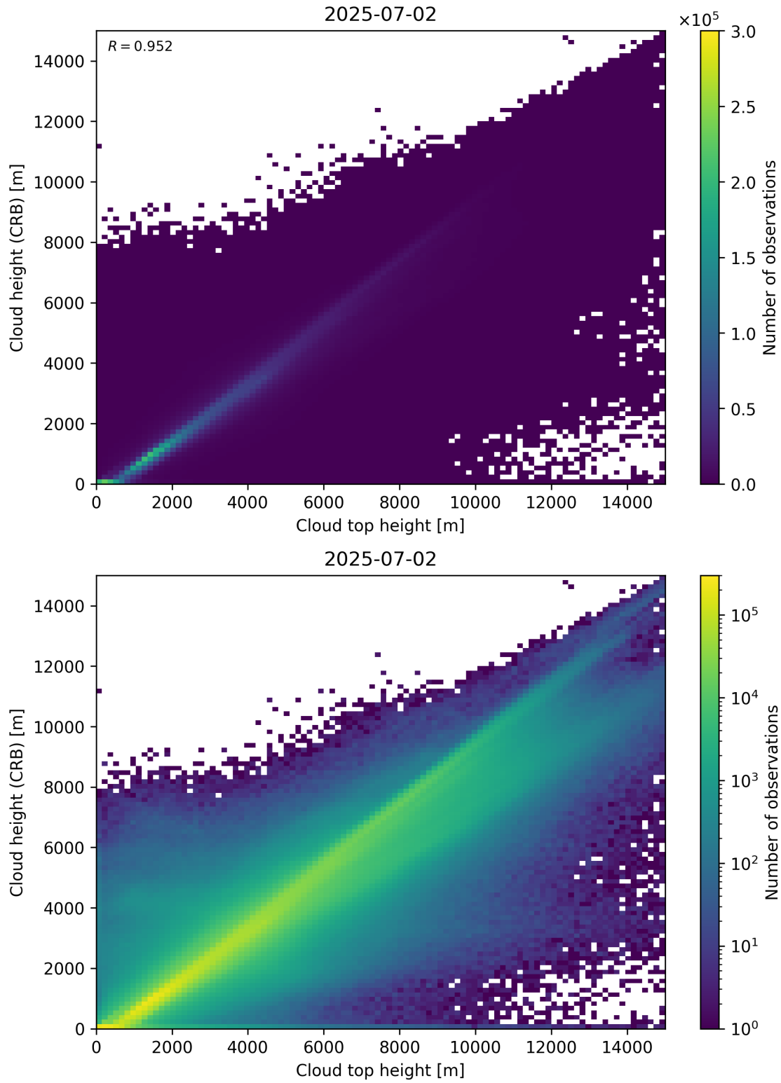
Figure 89: Scatter density plot of “Cloud top height” against “Cloud height (CRB)” for 2025-07-02 to 2025-07-03.
