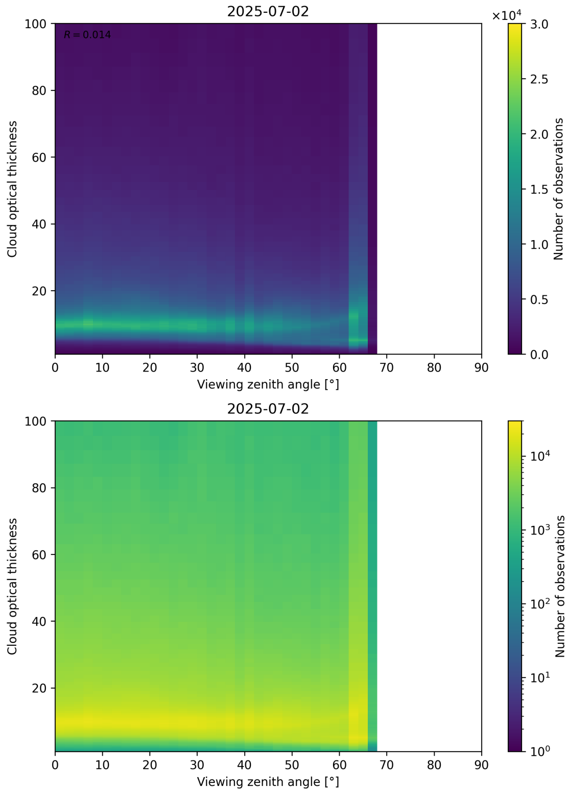
Figure 111: Scatter density plot of “Viewing zenith angle” against “Cloud optical thickness” for 2025-07-02 to 2025-07-03.
