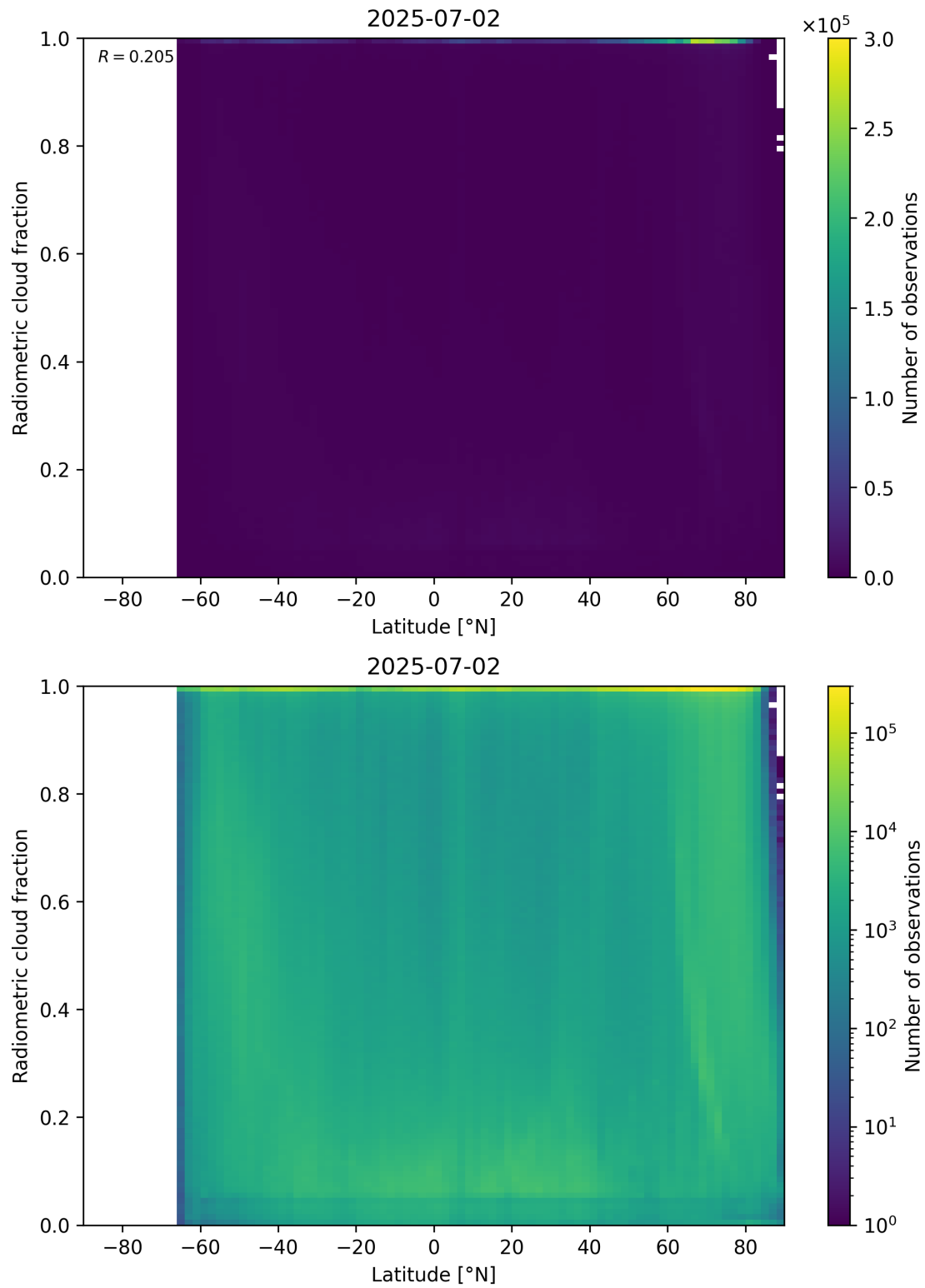
Figure 92: Scatter density plot of “Latitude” against “Radiometric cloud fraction” for 2025-07-02 to 2025-07-03.
