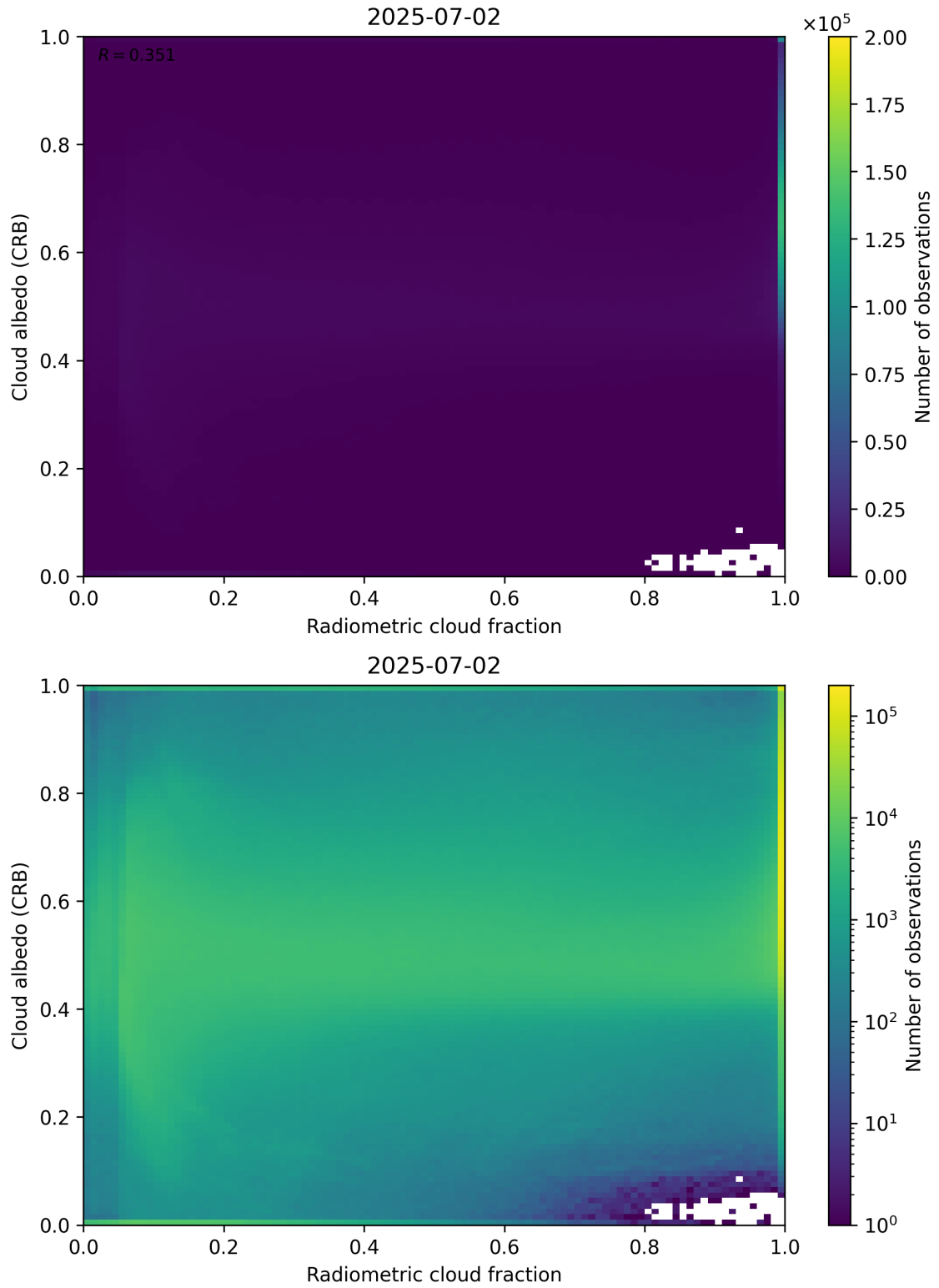
Figure 71: Scatter density plot of “Radiometric cloud fraction” against “Cloud albedo (CRB)” for 2025-07-02 to 2025-07-03.
