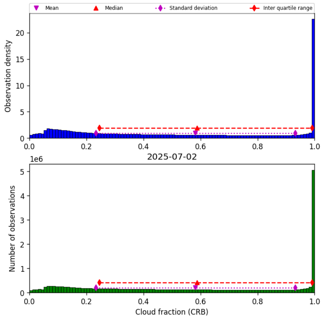
Figure 42: Histogram of “Cloud fraction (CRB)” for 2025-07-02 to 2025-07-03
