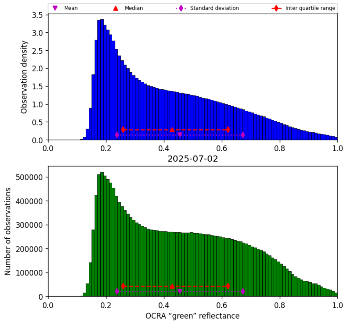
Figure 52: Histogram of “OCRA “green” reflectance” for 2025-07-02 to 2025-07-03
