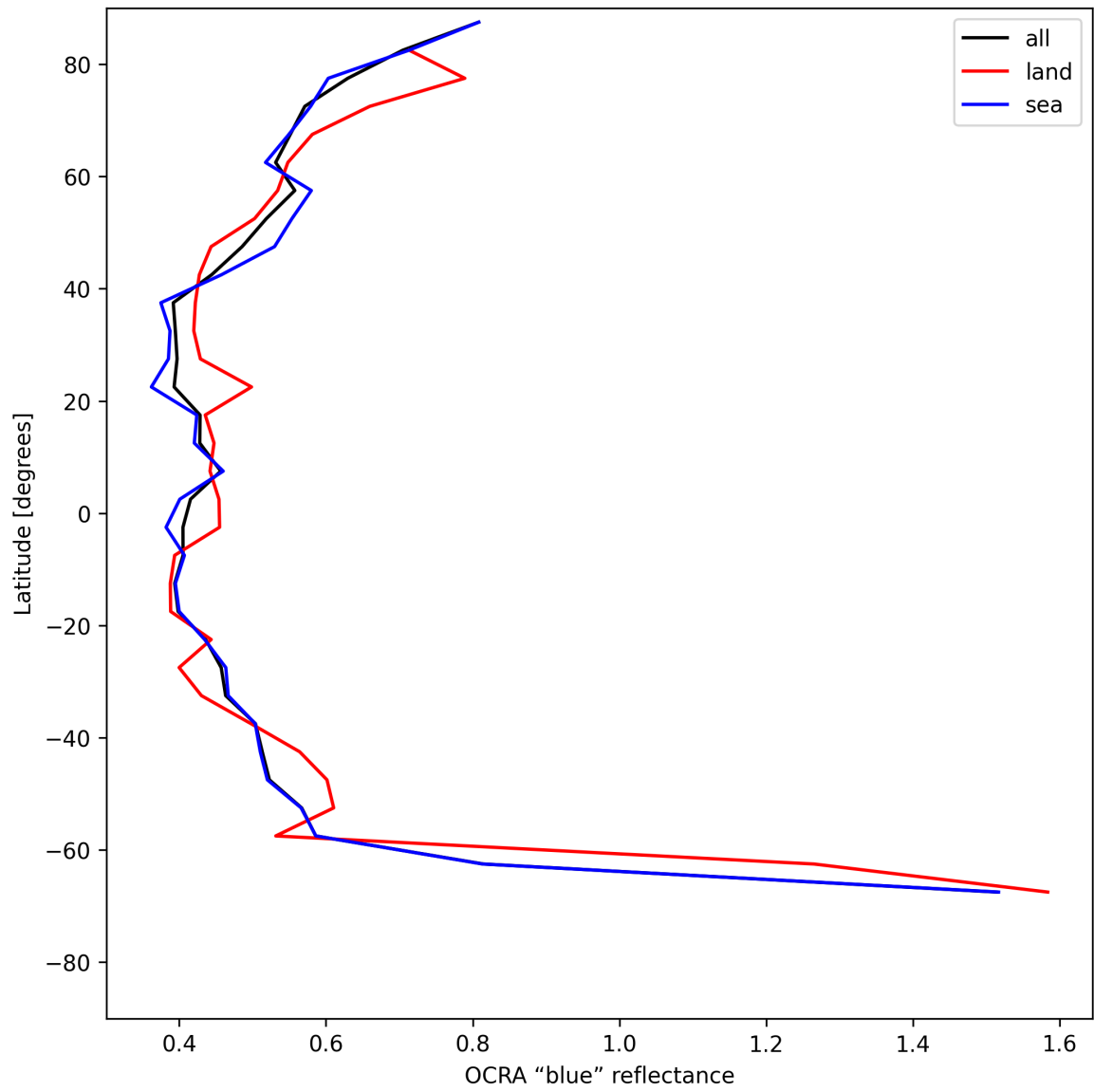
Figure 35: Zonal average of “OCRA “blue” reflectance” for 2025-07-02 to 2025-07-03.
