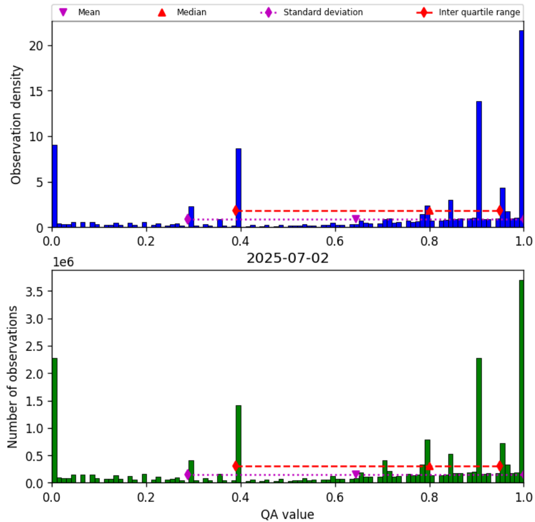
Figure 38: Histogram of “QA value” for 2025-07-02 to 2025-07-03
