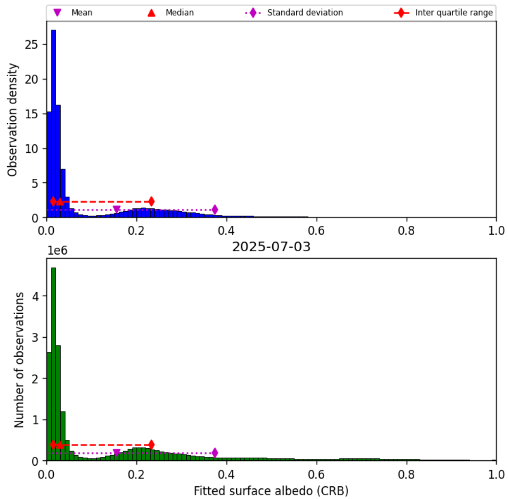
Figure 46: Histogram of “Fitted surface albedo (CRB)” for 2025-07-03 to 2025-07-04
