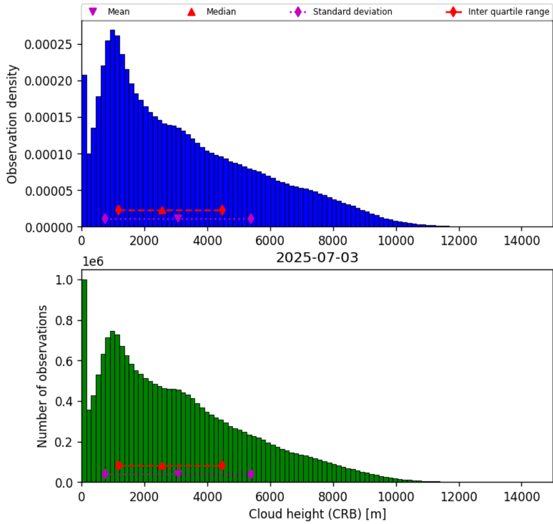
Figure 43: Histogram of “Cloud height (CRB)” for 2025-07-03 to 2025-07-04
