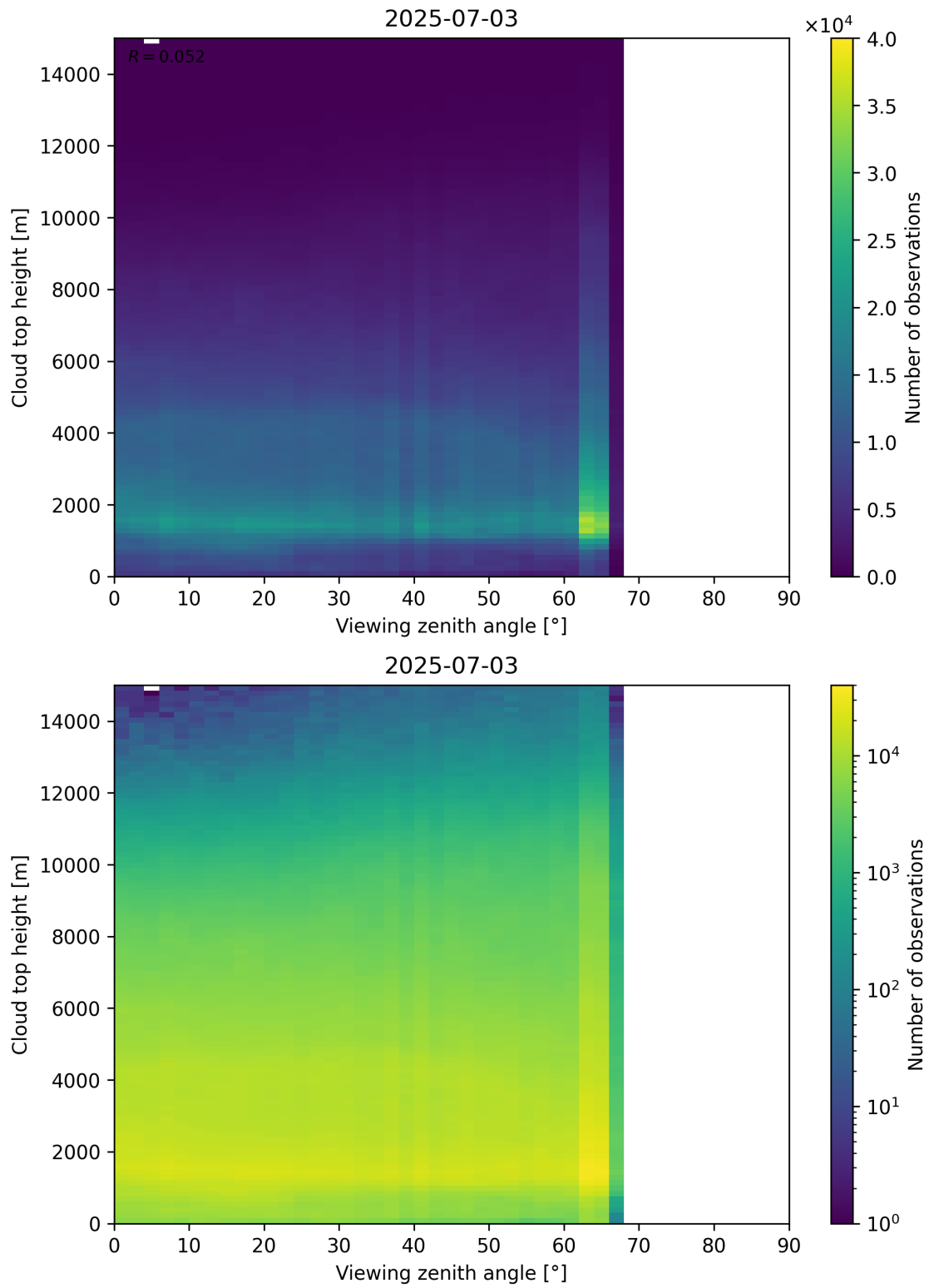
Figure 112: Scatter density plot of “Viewing zenith angle” against “Cloud top height” for 2025-07-03 to 2025-07-04.
