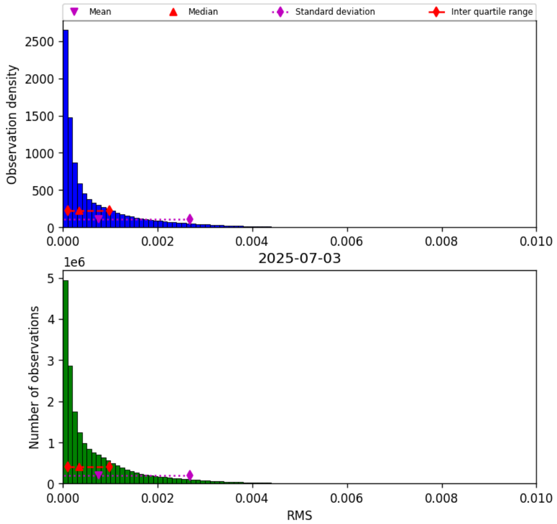
Figure 47: Histogram of “RMS” for 2025-07-03 to 2025-07-04
