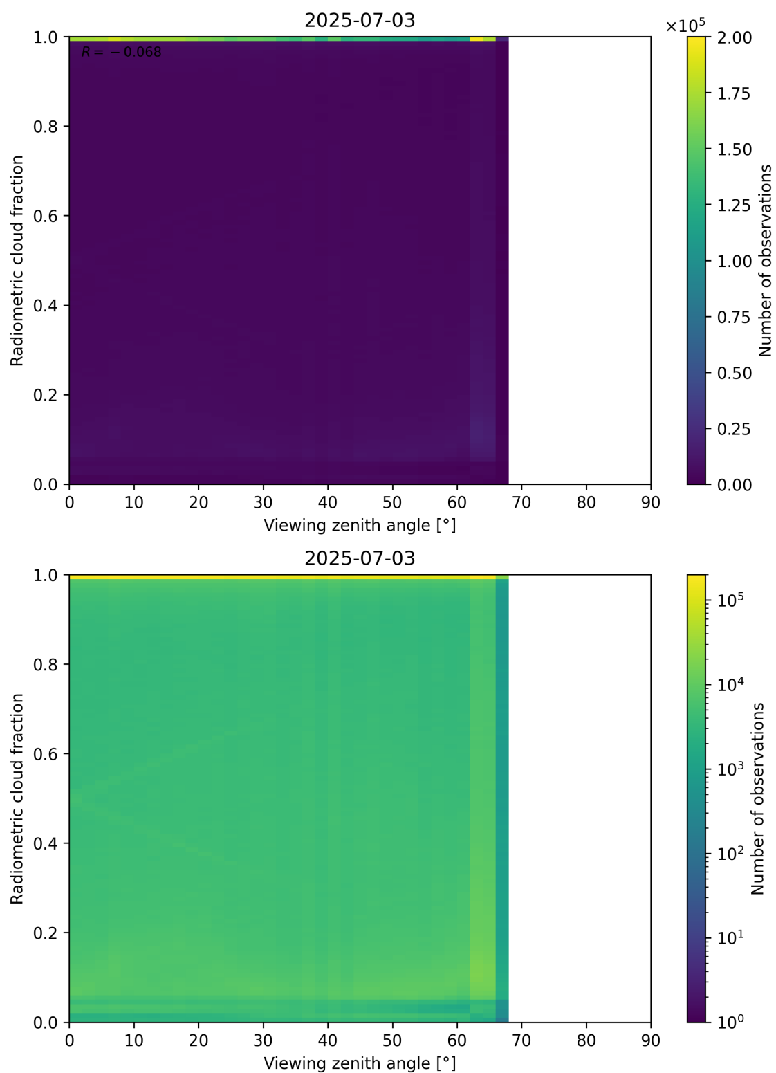
Figure 107: Scatter density plot of “Viewing zenith angle” against “Radiometric cloud fraction” for 2025-07-03 to 2025-07-04.
