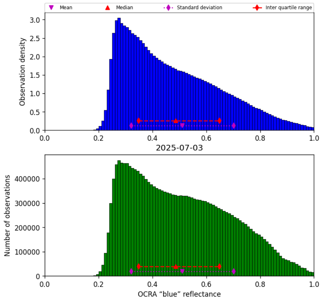
Figure 51: Histogram of “OCRA “blue” reflectance” for 2025-07-03 to 2025-07-04
