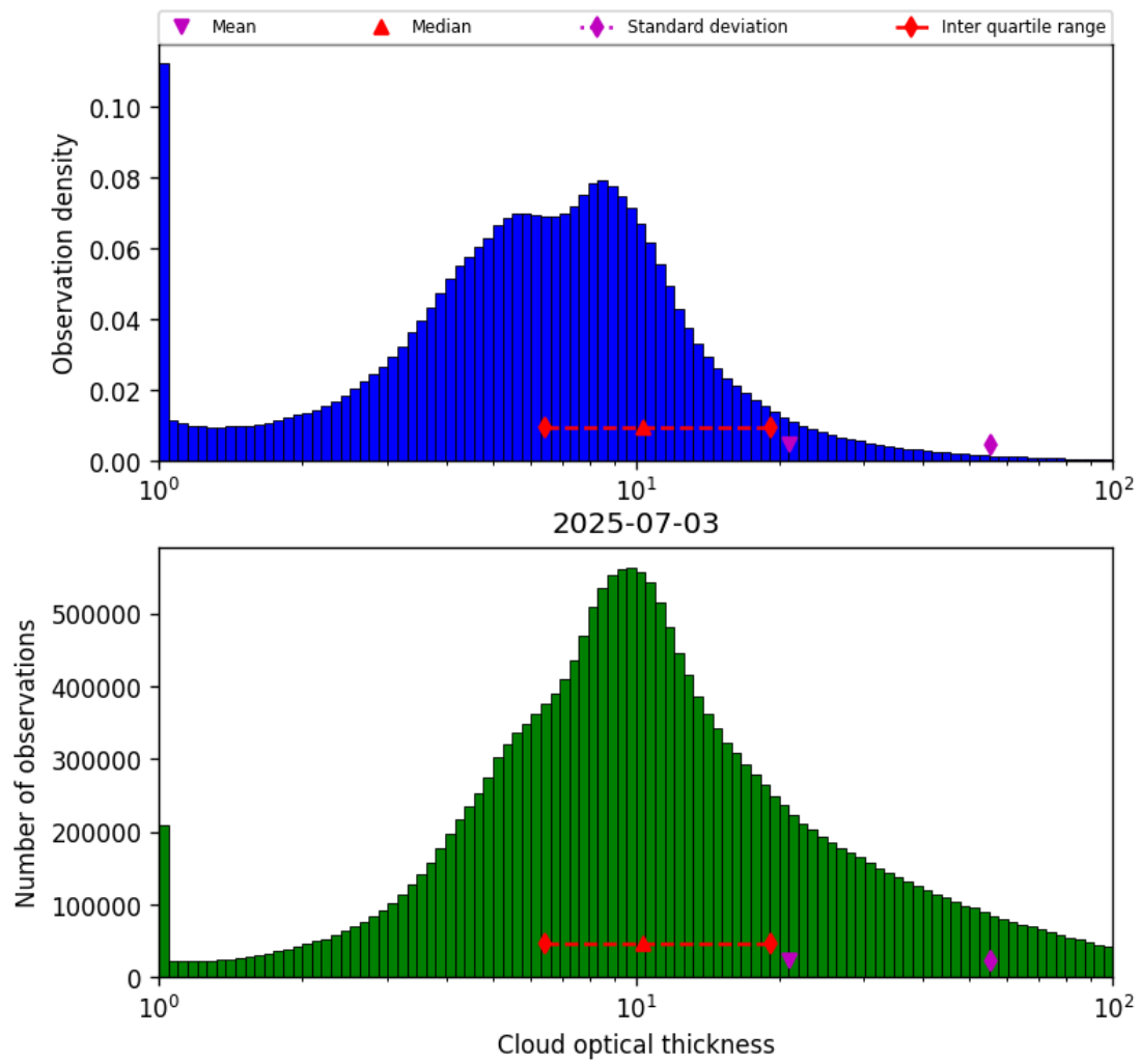
Figure 41: Histogram of “Cloud optical thickness” for 2025-07-03 to 2025-07-04
