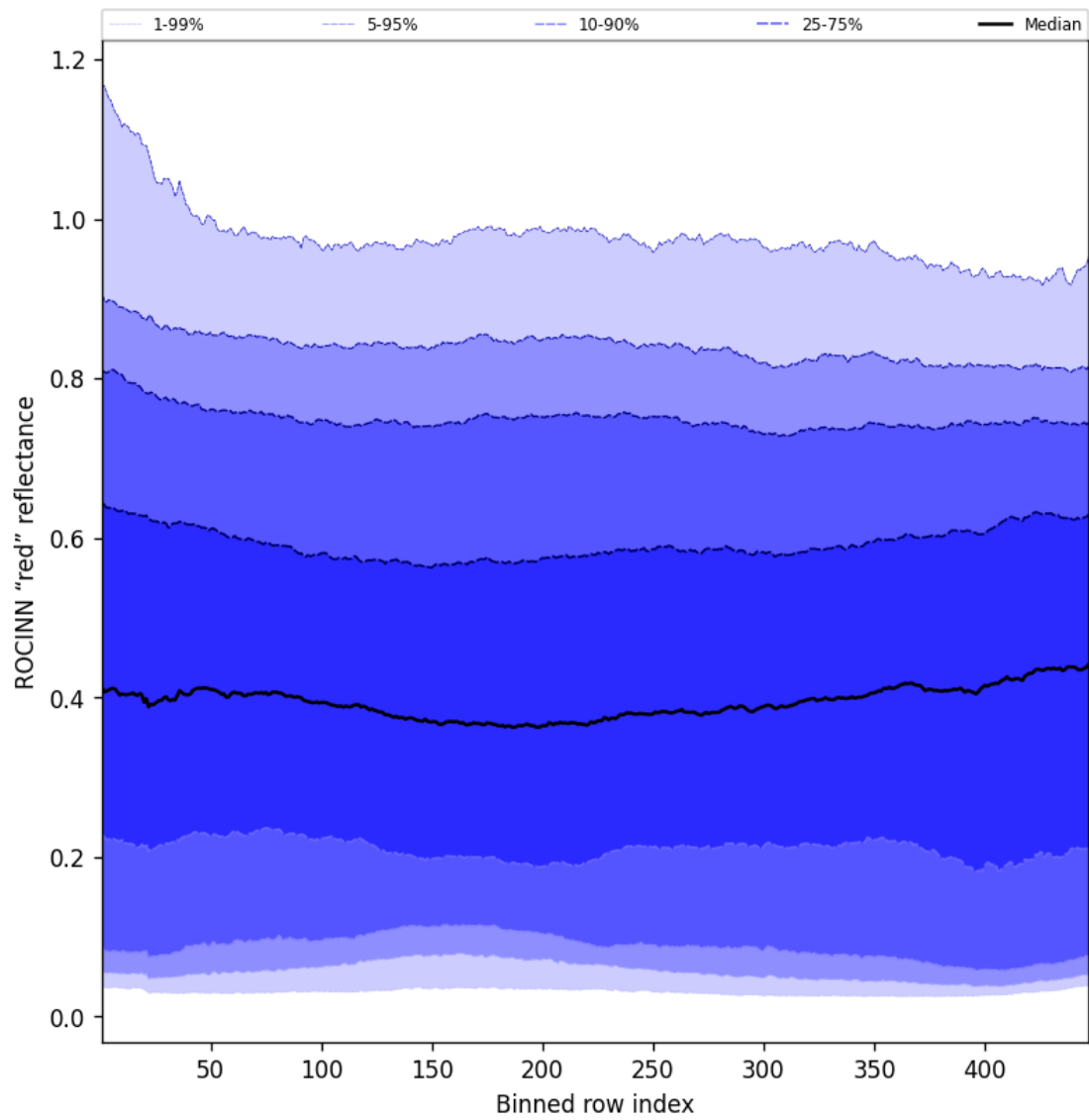
Figure 69: Along track statistics of "ROCINN "red" reflectance" for 2025-07-03 to 2025-07-04
