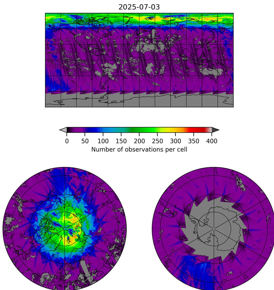
Figure 21: Map of the number of observations for 2025-07-03 to 2025-07-04
