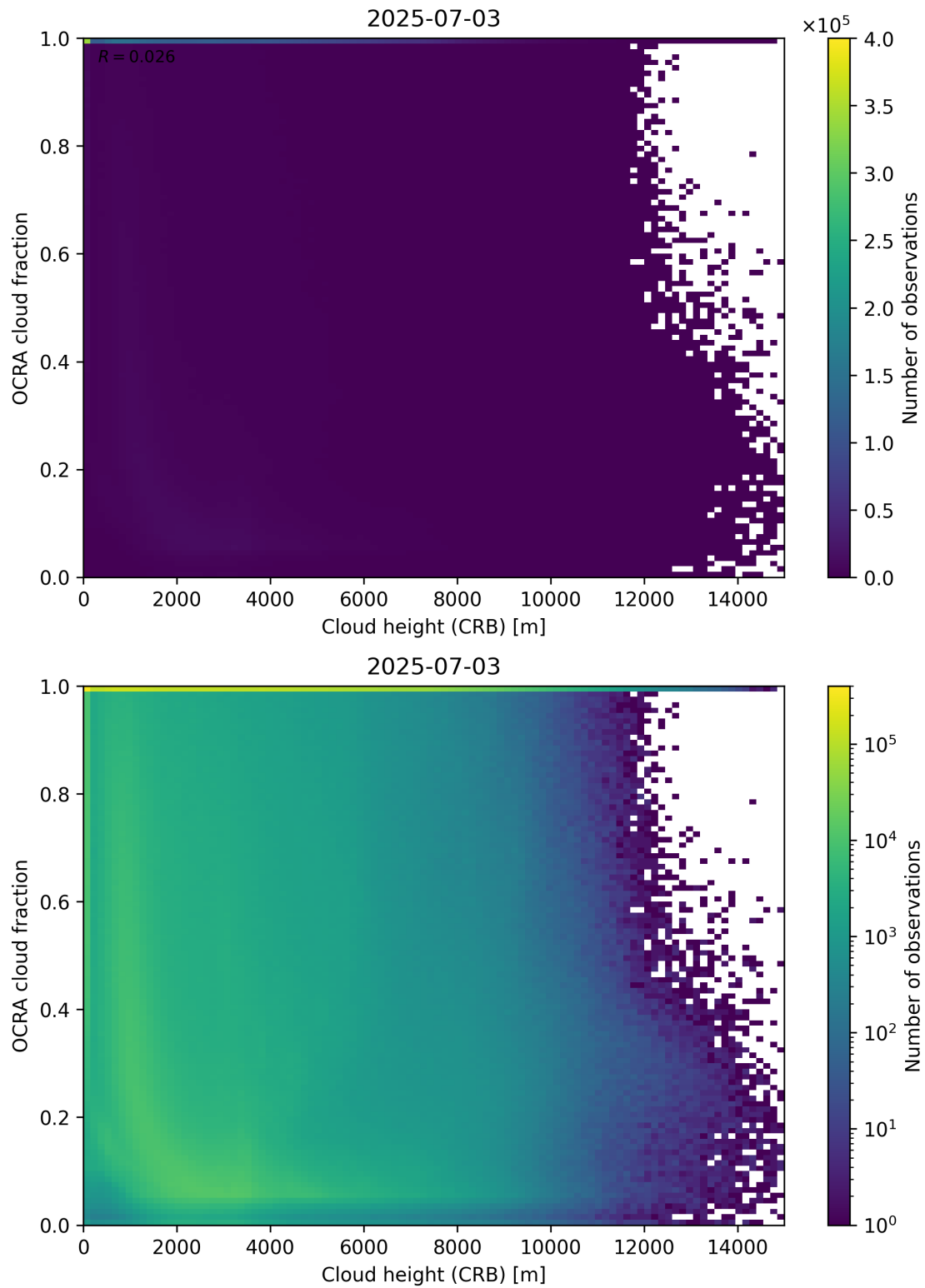
Figure 81: Scatter density plot of “Cloud height (CRB)” against “OCRA cloud fraction” for 2025-07-03 to 2025-07-04.
