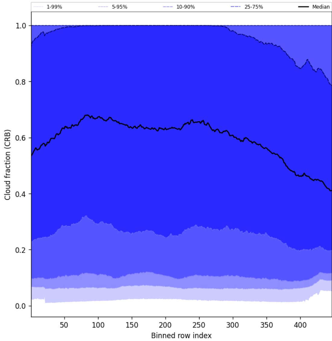
Figure 58: Along track statistics of “Cloud fraction (CRB)” for 2025-07-03 to 2025-07-04
