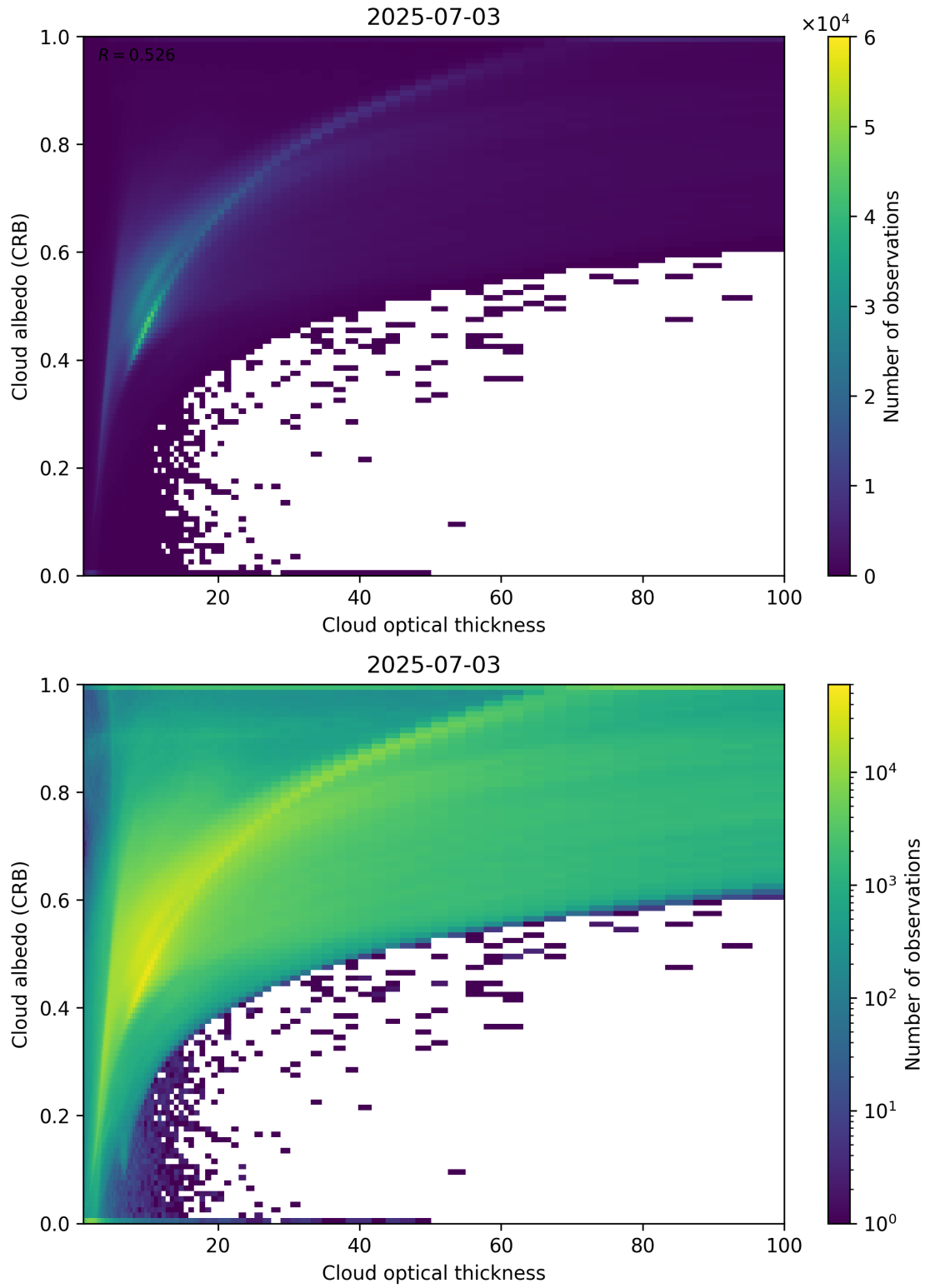
Figure 82: Scatter density plot of “Cloud optical thickness” against “Cloud albedo (CRB)” for 2025-07-03 to 2025-07-04.
