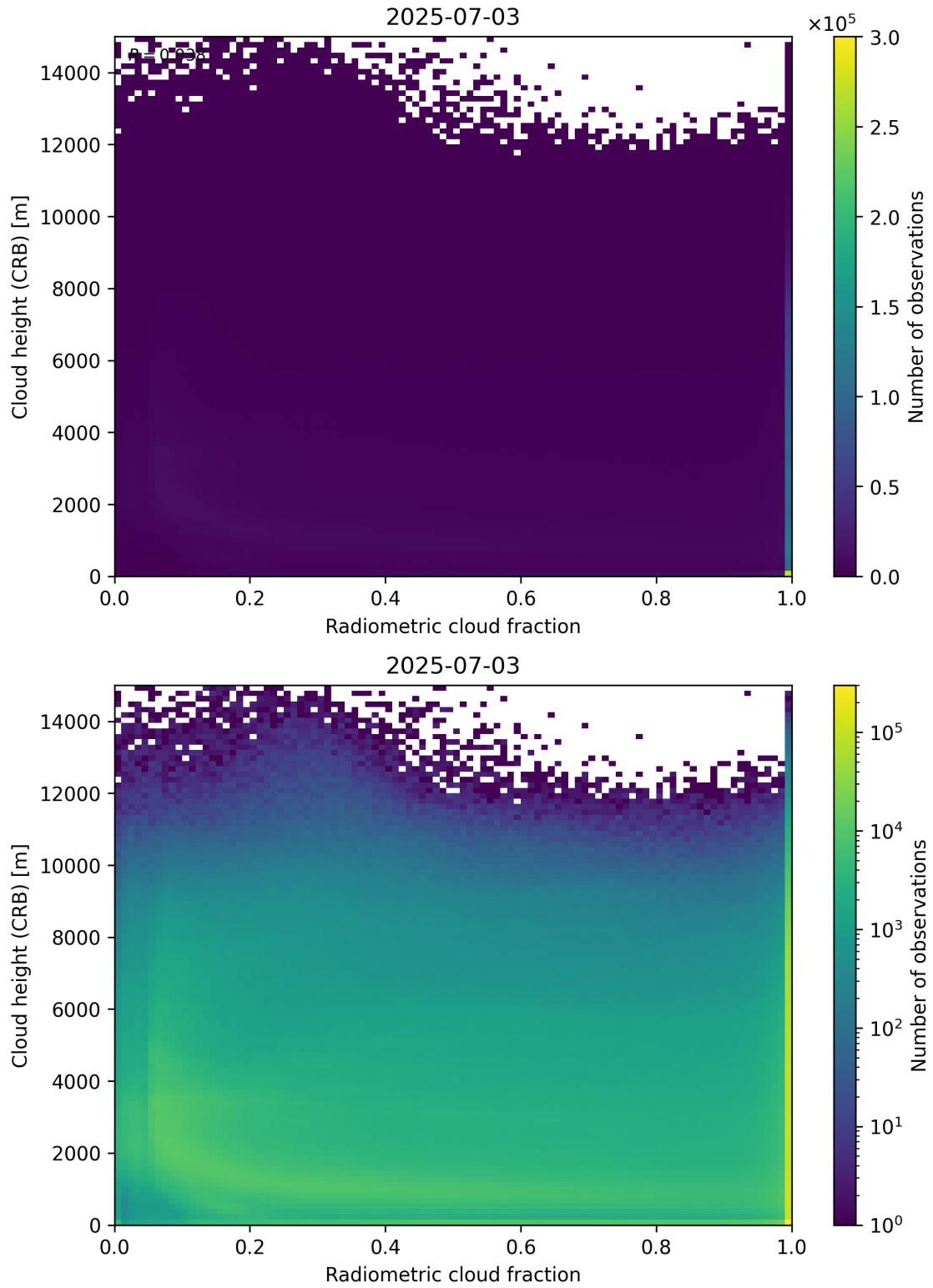
Figure 74: Scatter density plot of “Radiometric cloud fraction” against “Cloud height (CRB)” for 2025-07-03 to 2025-07-04.
