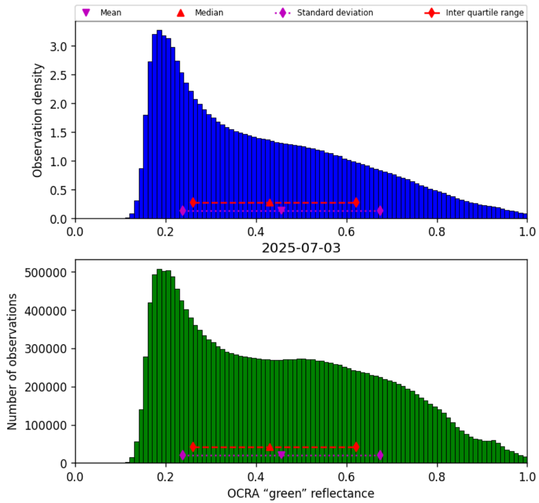
Figure 52: Histogram of “OCRA “green” reflectance” for 2025-07-03 to 2025-07-04
