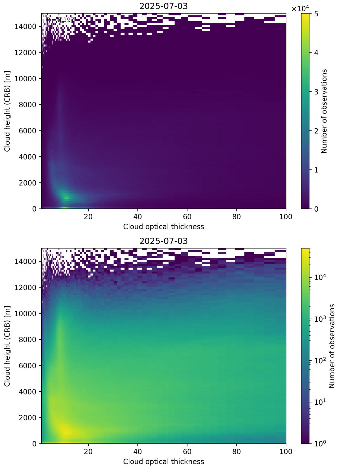
Figure 85: Scatter density plot of “Cloud optical thickness” against “Cloud height (CRB)” for 2025-07-03 to 2025-07-04.
