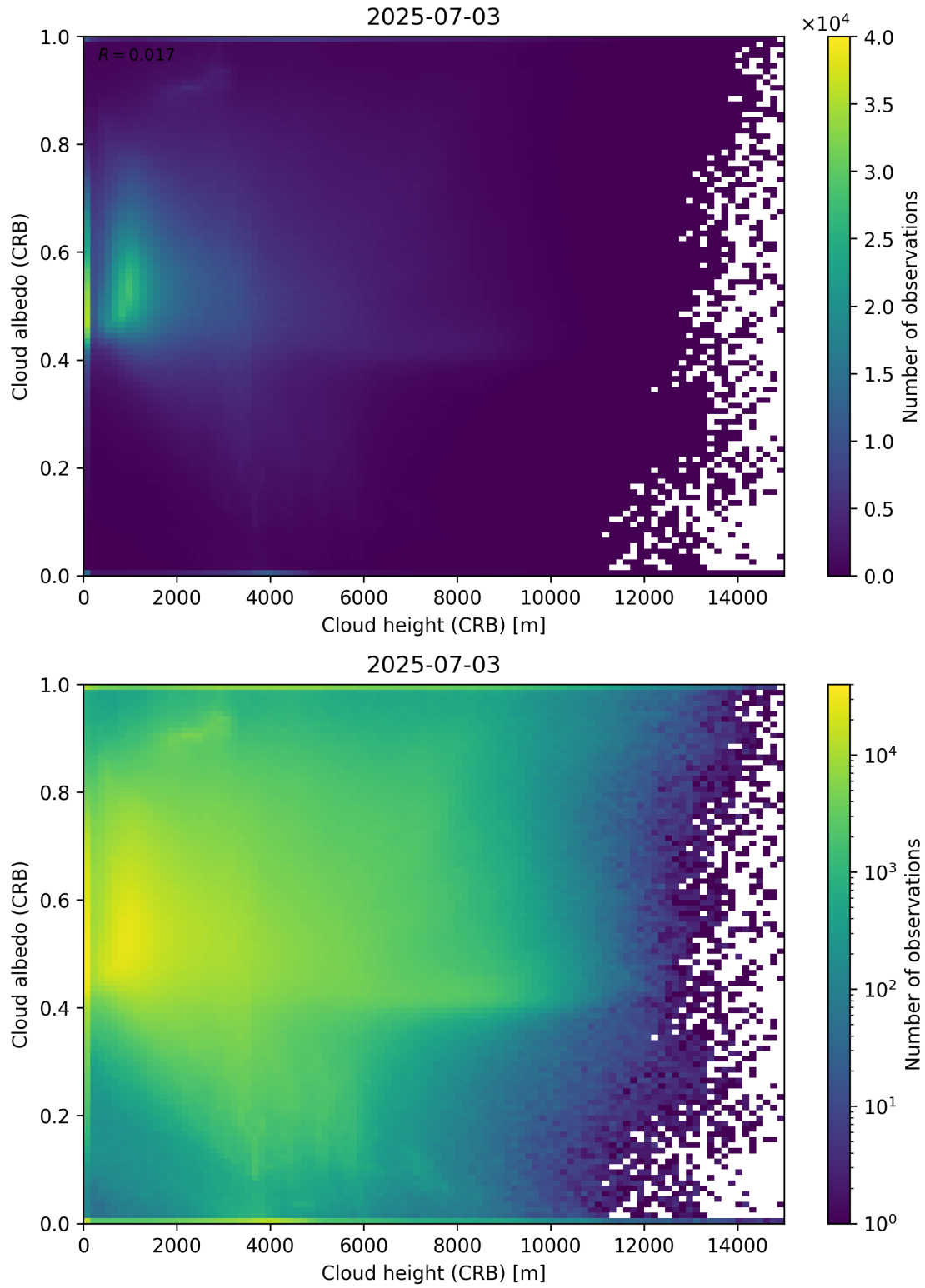
Figure 80: Scatter density plot of “Cloud height (CRB)” against “Cloud albedo (CRB)” for 2025-07-03 to 2025-07-04.
