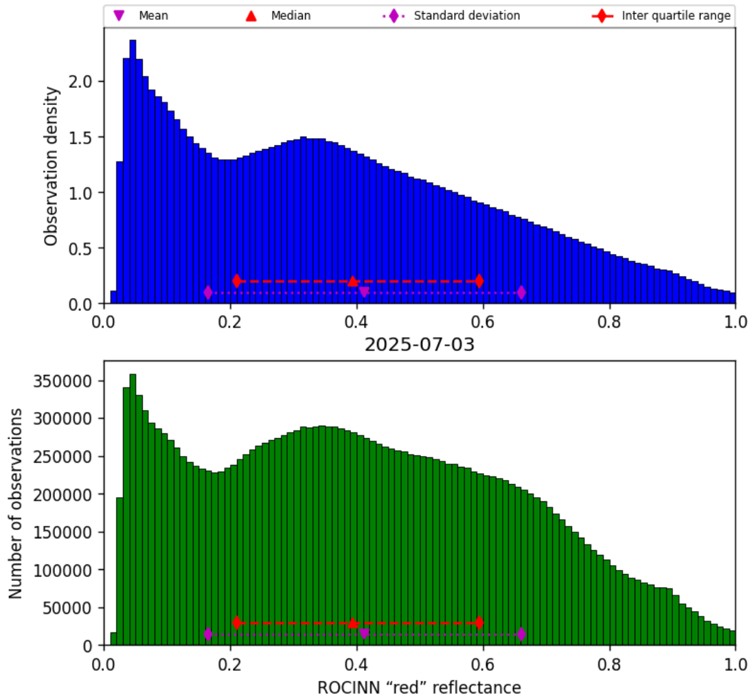
Figure 53: Histogram of "ROCINN "red" reflectance" for 2025-07-03 to 2025-07-04
