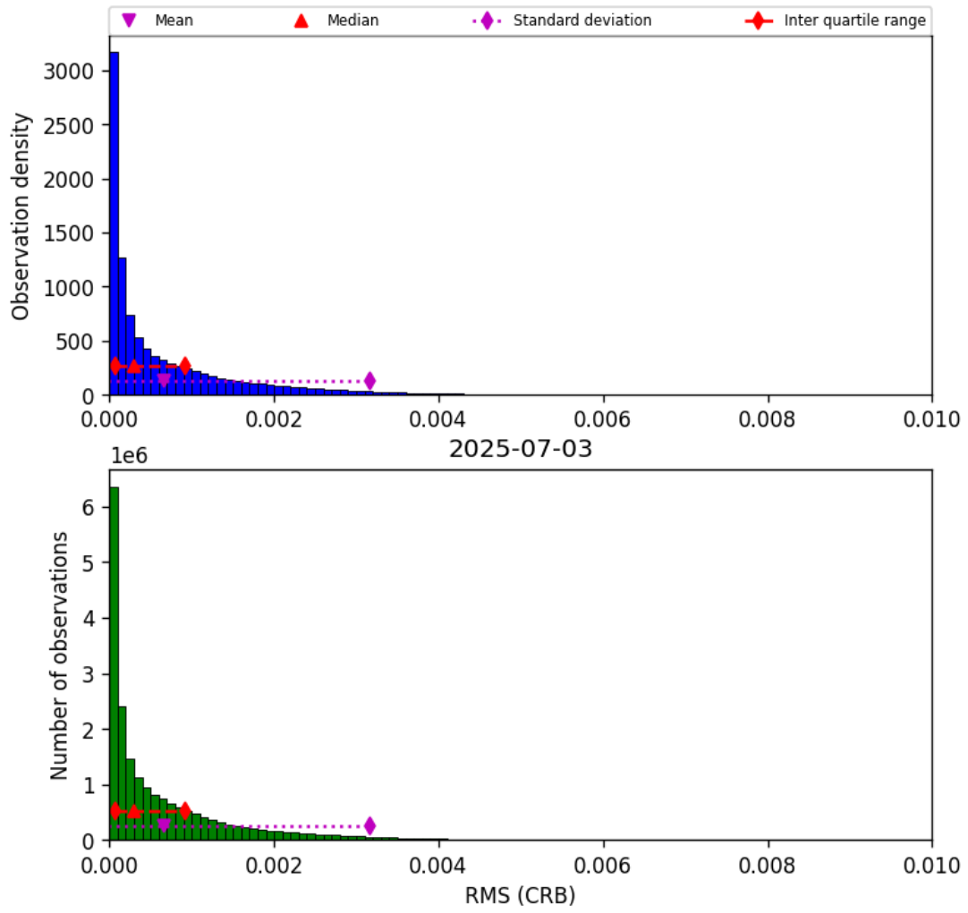
Figure 48: Histogram of “RMS (CRB)” for 2025-07-03 to 2025-07-04
