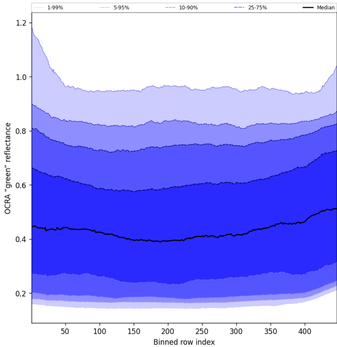
Figure 68: Along track statistics of “OCRA “green” reflectance” for 2025-07-03 to 2025-07-04
