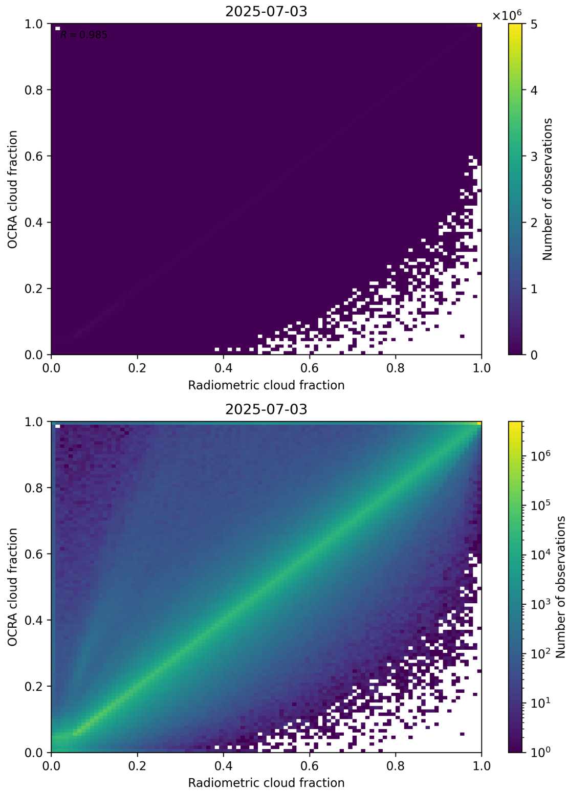
Figure 72: Scatter density plot of “Radiometric cloud fraction” against “OCRA cloud fraction” for 2025-07-03 to 2025-07-04.
