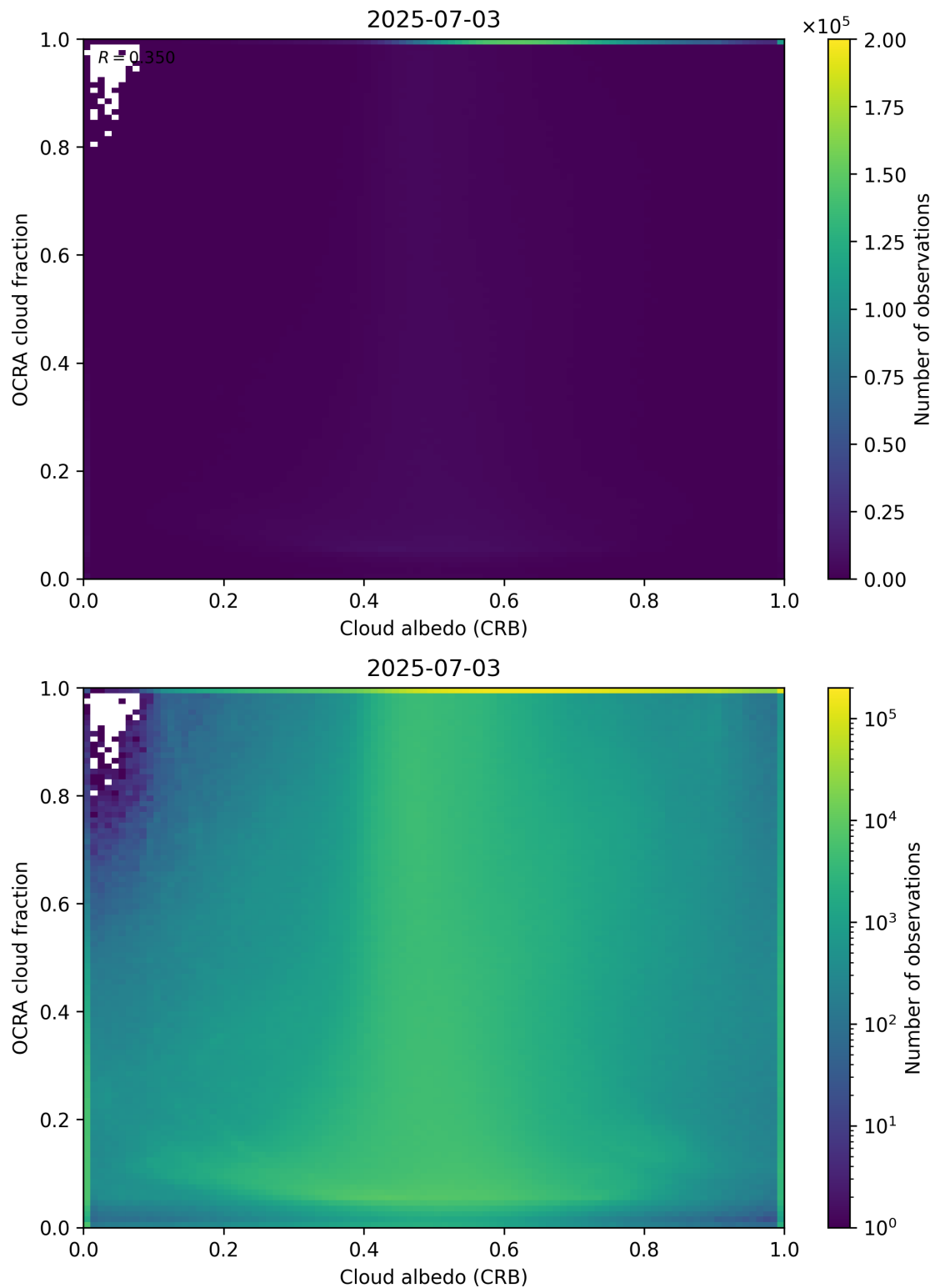
Figure 70: Scatter density plot of “Cloud albedo (CRB)” against “OCRA cloud fraction” for 2025-07-03 to 2025-07-04.
