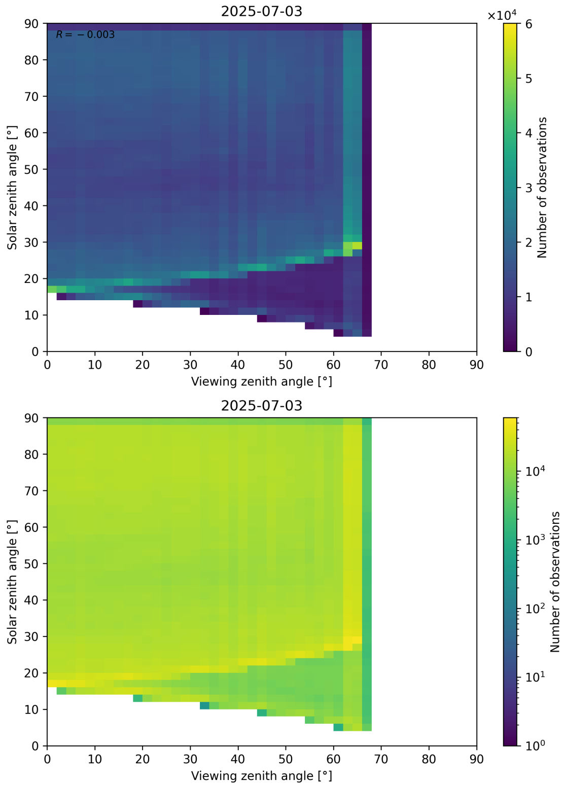
Figure 114: Scatter density plot of “Viewing zenith angle” against “Solar zenith angle” for 2025-07-03 to 2025-07-04.
