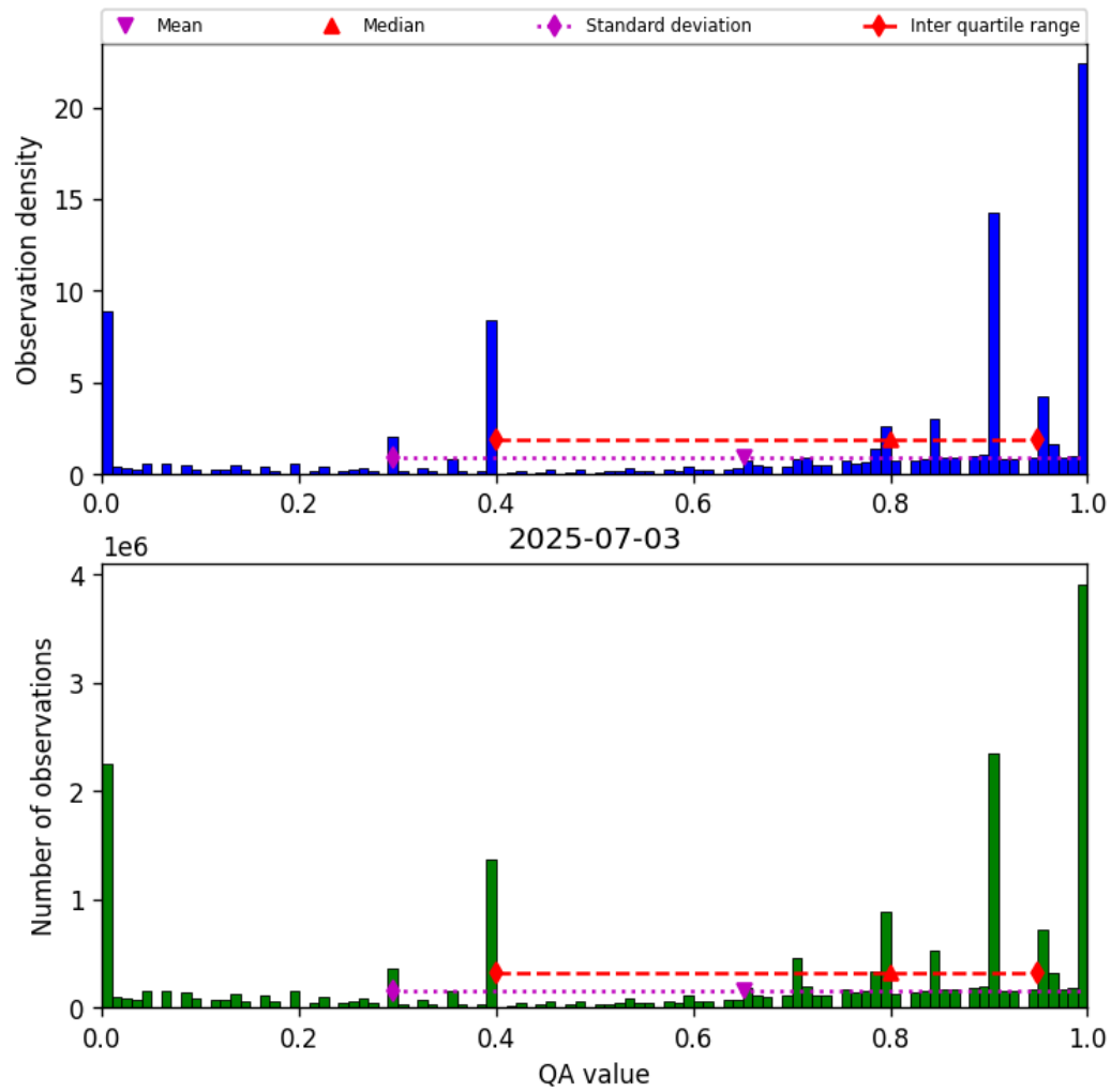
Figure 38: Histogram of “QA value” for 2025-07-03 to 2025-07-04
