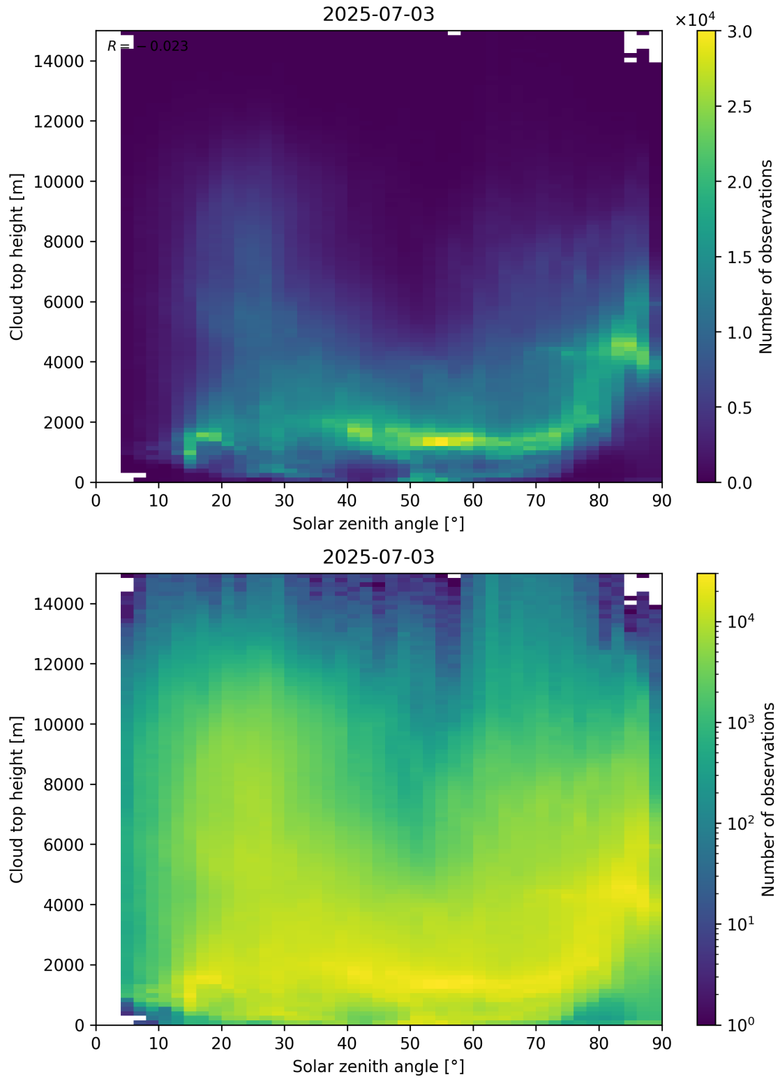
Figure 104: Scatter density plot of “Solar zenith angle” against “Cloud top height” for 2025-07-03 to 2025-07-04.
