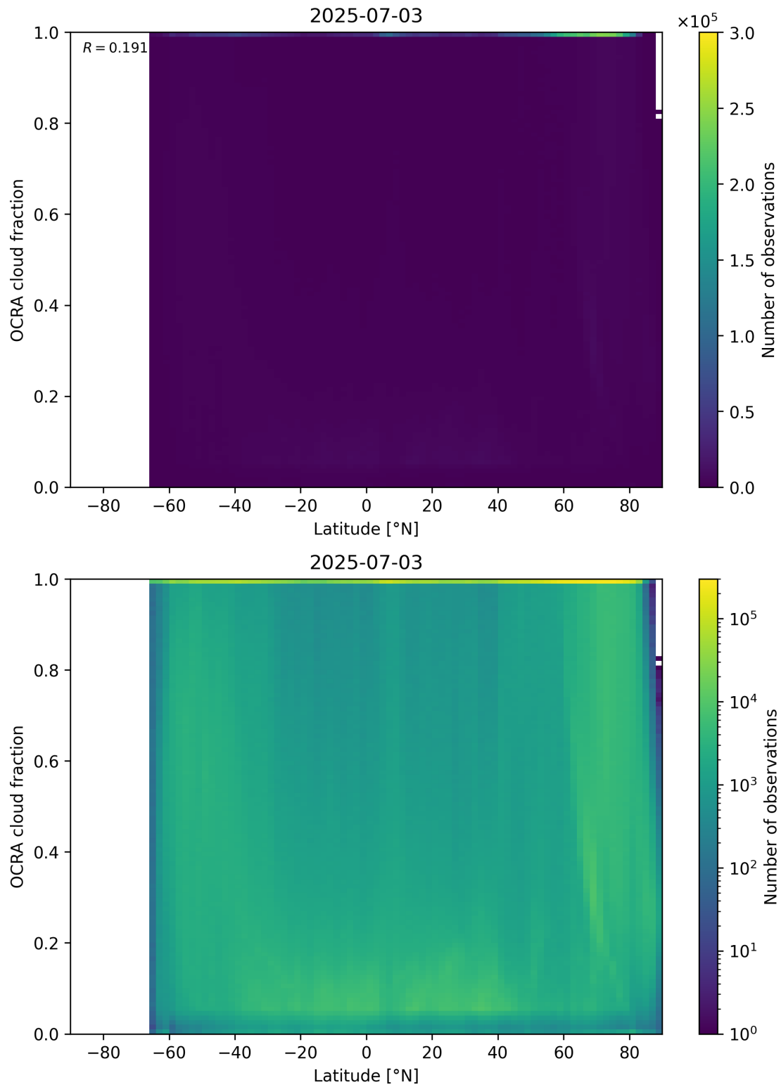
Figure 93: Scatter density plot of “Latitude” against “OCRA cloud fraction” for 2025-07-03 to 2025-07-04.
