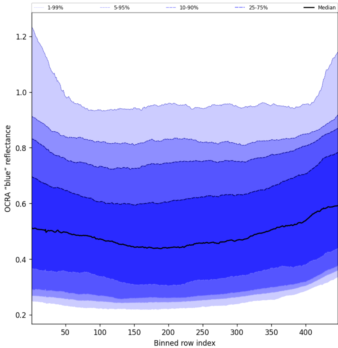
Figure 67: Along track statistics of “OCRA “blue” reflectance” for 2025-07-03 to 2025-07-04
