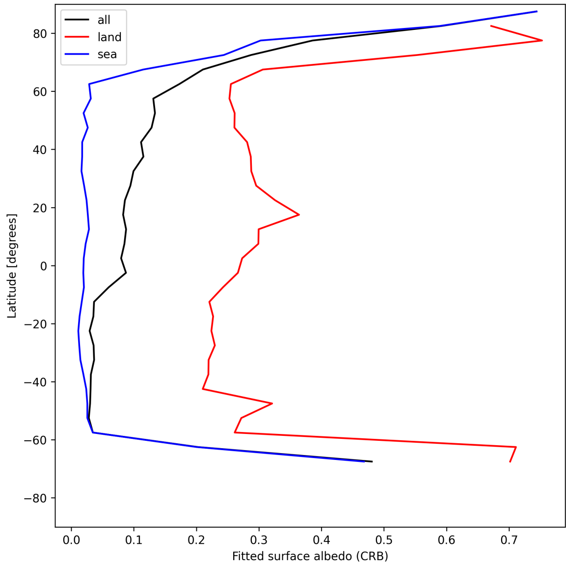
Figure 30: Zonal average of “Fitted surface albedo (CRB)” for 2025-07-03 to 2025-07-04.
