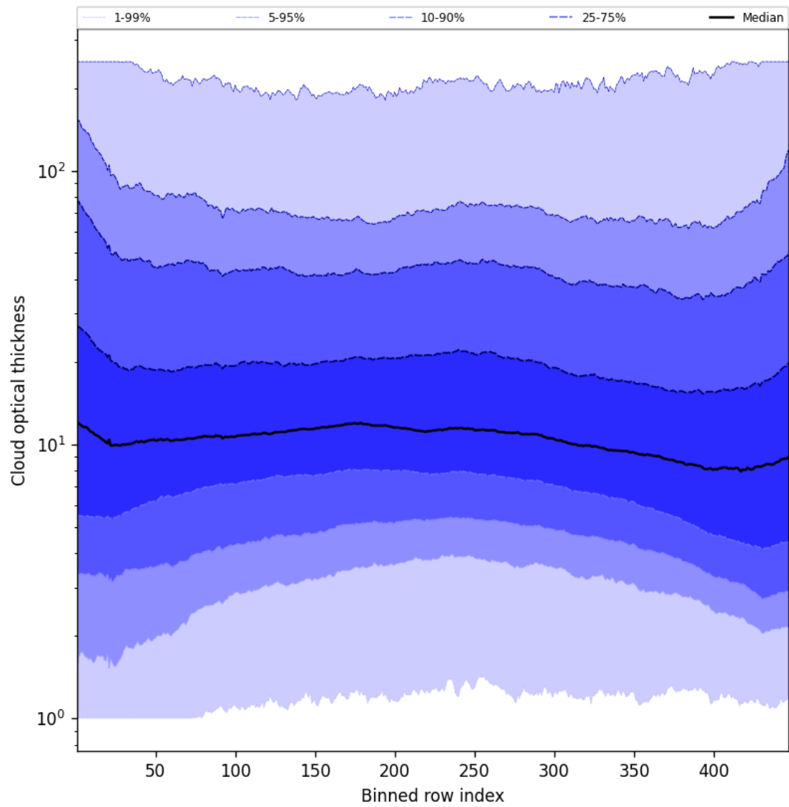
Figure 57: Along track statistics of “Cloud optical thickness” for 2025-07-03 to 2025-07-04
