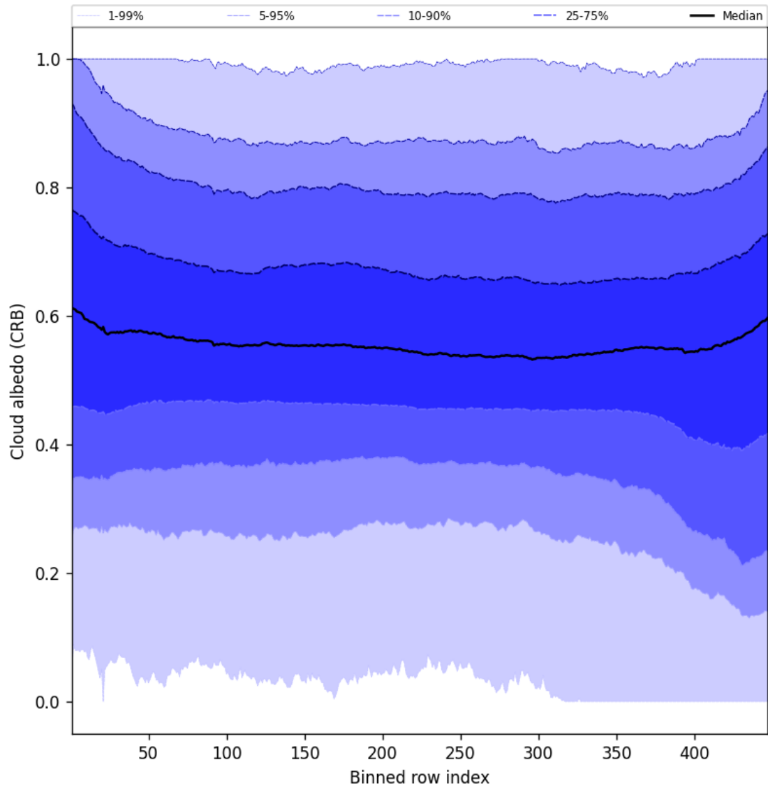
Figure 60: Along track statistics of “Cloud albedo (CRB)” for 2025-07-03 to 2025-07-04
