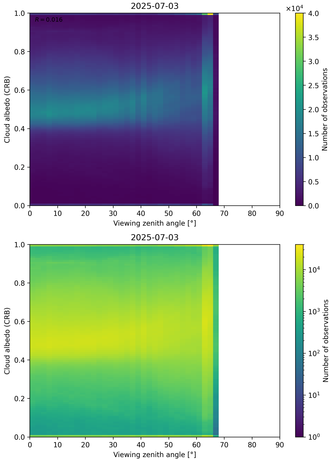
Figure 106: Scatter density plot of “Viewing zenith angle” against “Cloud albedo (CRB)” for 2025-07-03 to 2025-07-04.
