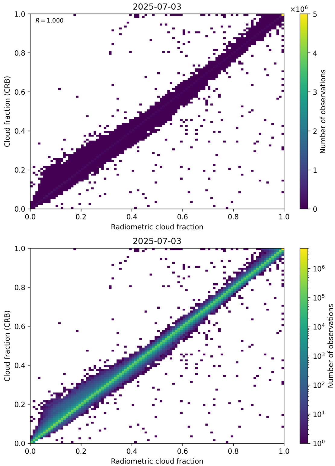
Figure 73: Scatter density plot of “Radiometric cloud fraction” against “Cloud fraction (CRB)” for 2025-07-03 to 2025-07-04.
