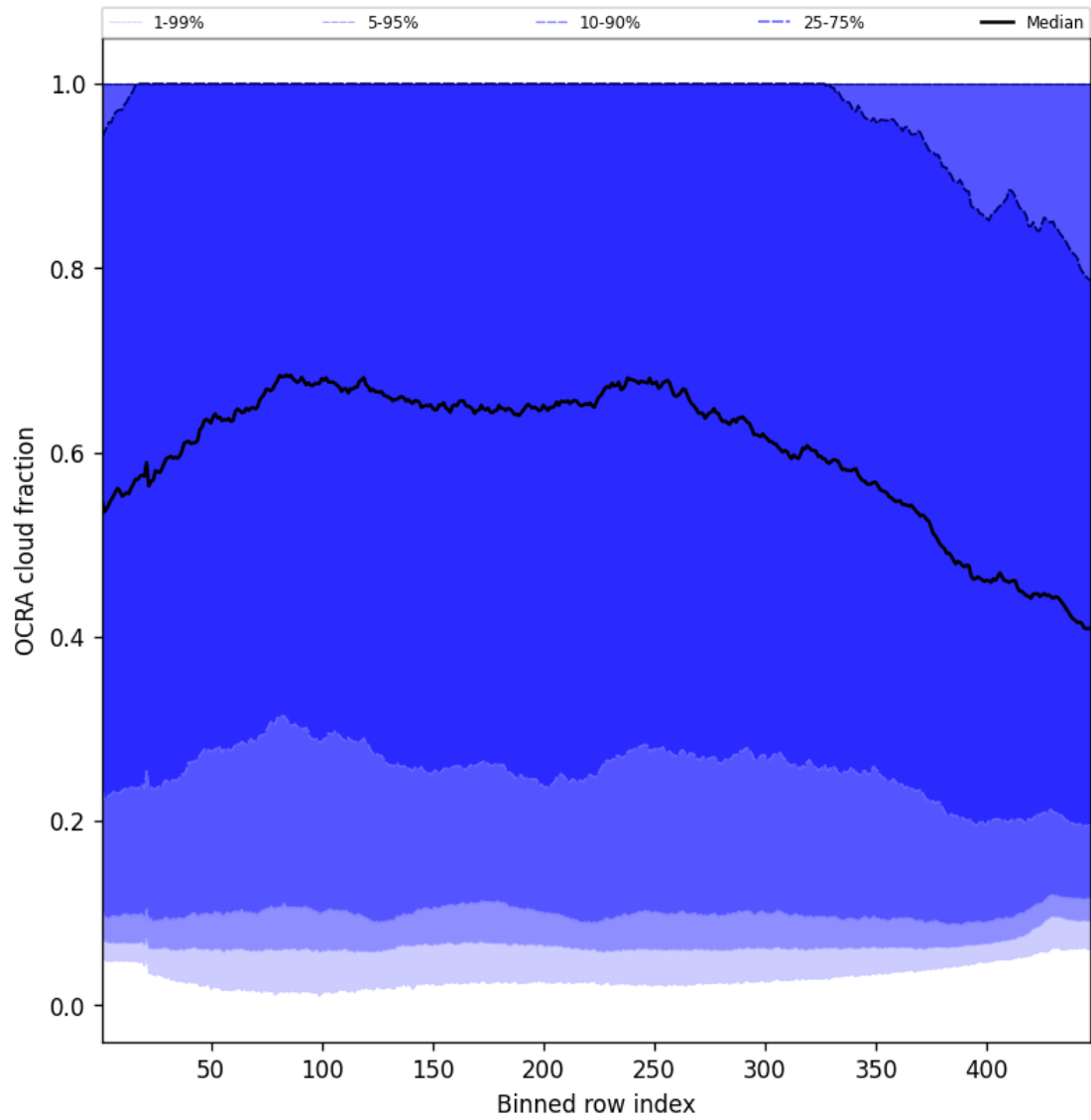
Figure 66: Along track statistics of “OCRA cloud fraction” for 2025-07-03 to 2025-07-04
