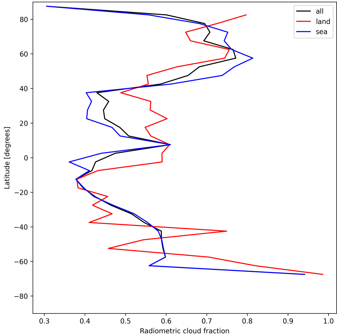
Figure 23: Zonal average of “Radiometric cloud fraction” for 2025-07-03 to 2025-07-04.
