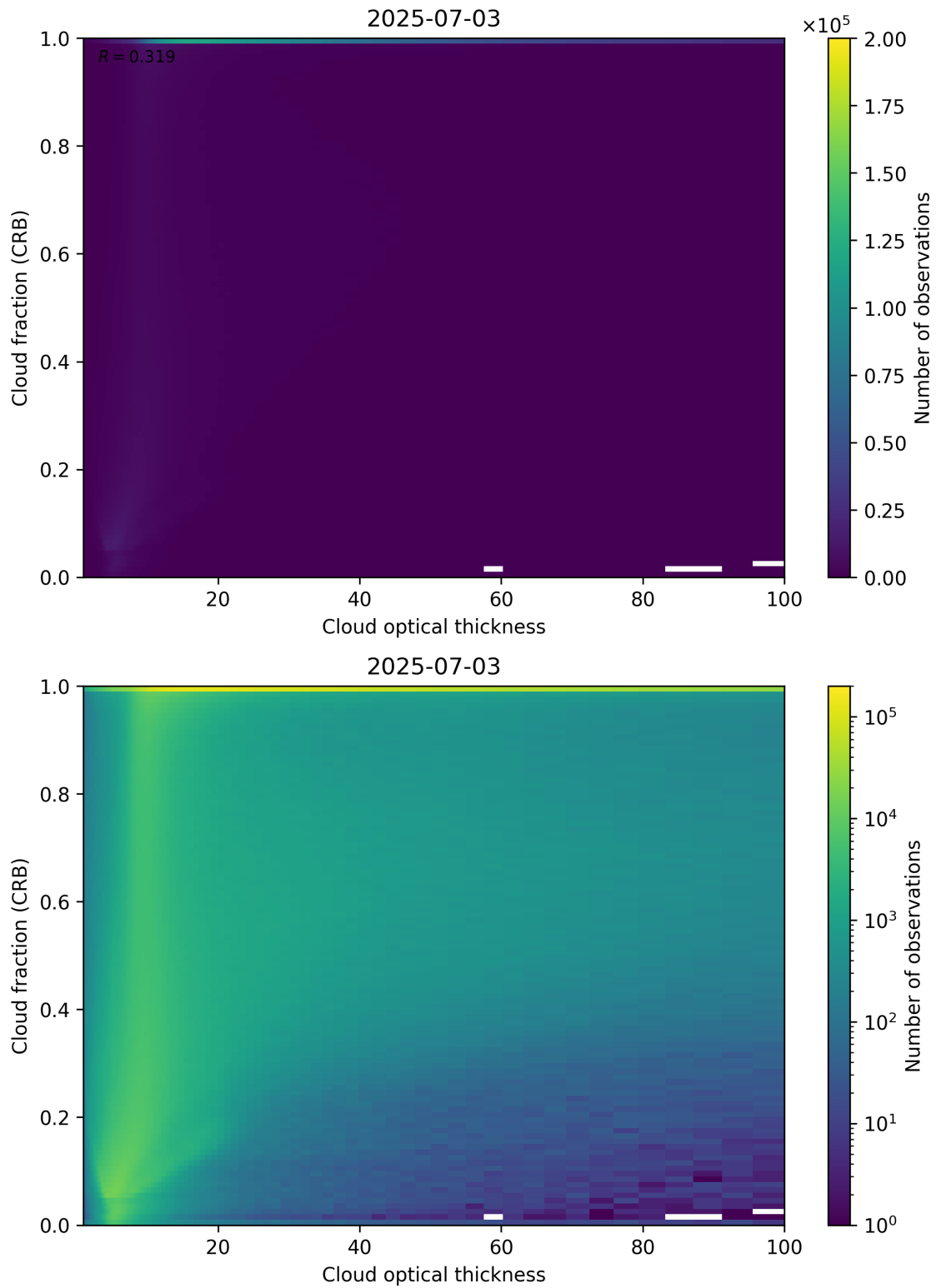
Figure 84: Scatter density plot of “Cloud optical thickness” against “Cloud fraction (CRB)” for 2025-07-03 to 2025-07-04.
