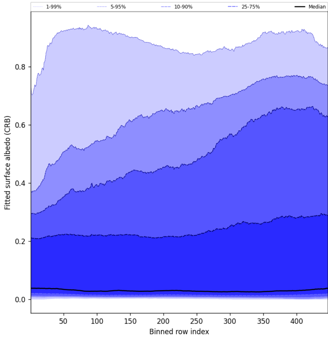
Figure 62: Along track statistics of “Fitted surface albedo (CRB)” for 2025-07-03 to 2025-07-04
