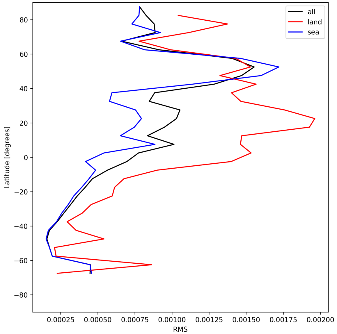
Figure 31: Zonal average of “RMS” for 2025-07-03 to 2025-07-04.
