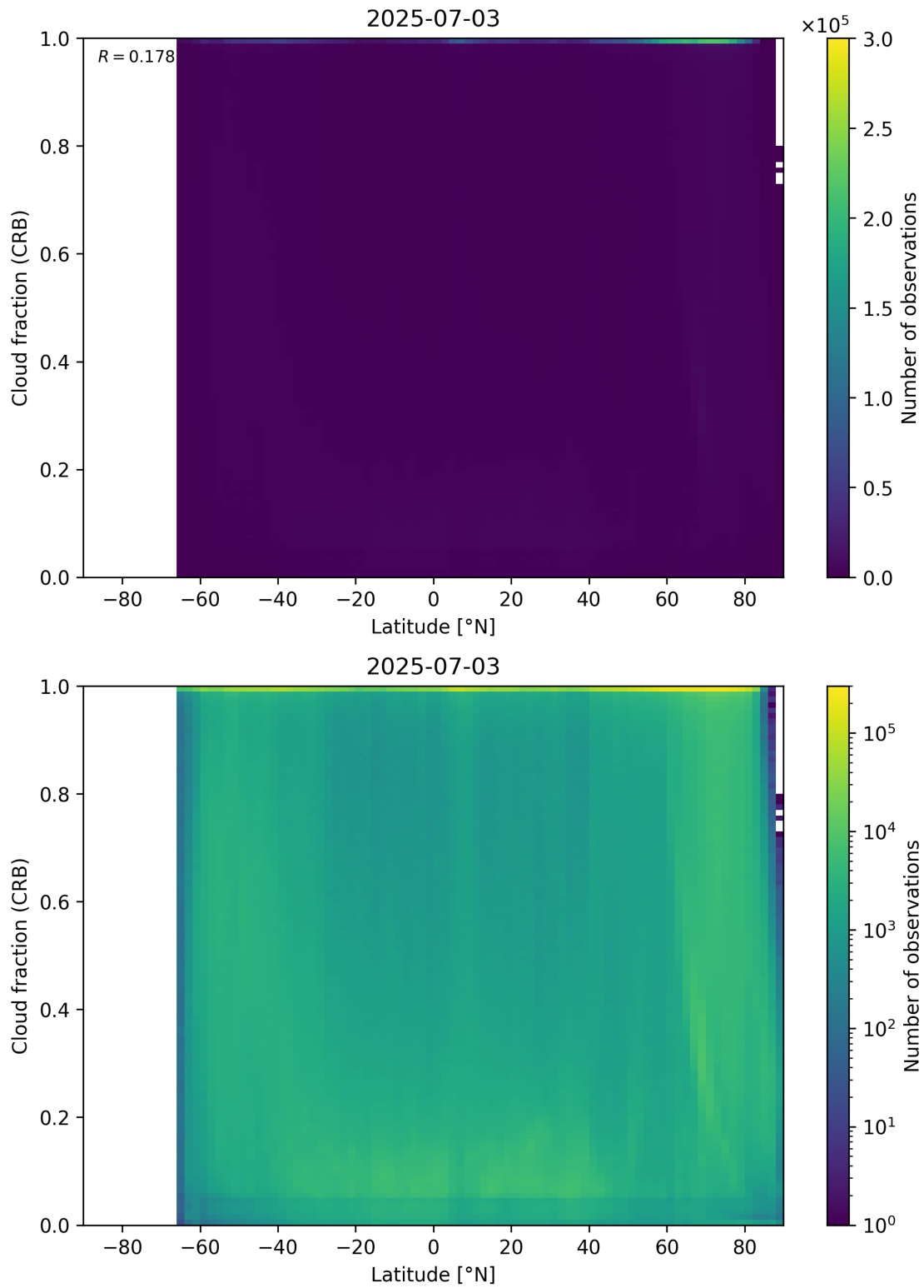
Figure 94: Scatter density plot of “Latitude” against “Cloud fraction (CRB)” for 2025-07-03 to 2025-07-04.
