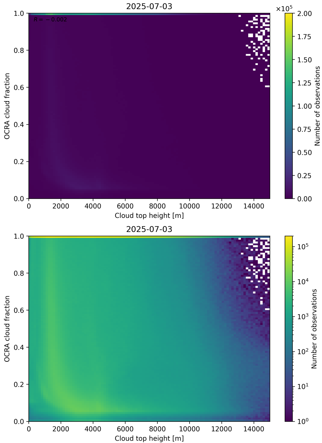
Figure 87: Scatter density plot of “Cloud top height” against “OCRA cloud fraction” for 2025-07-03 to 2025-07-04.
