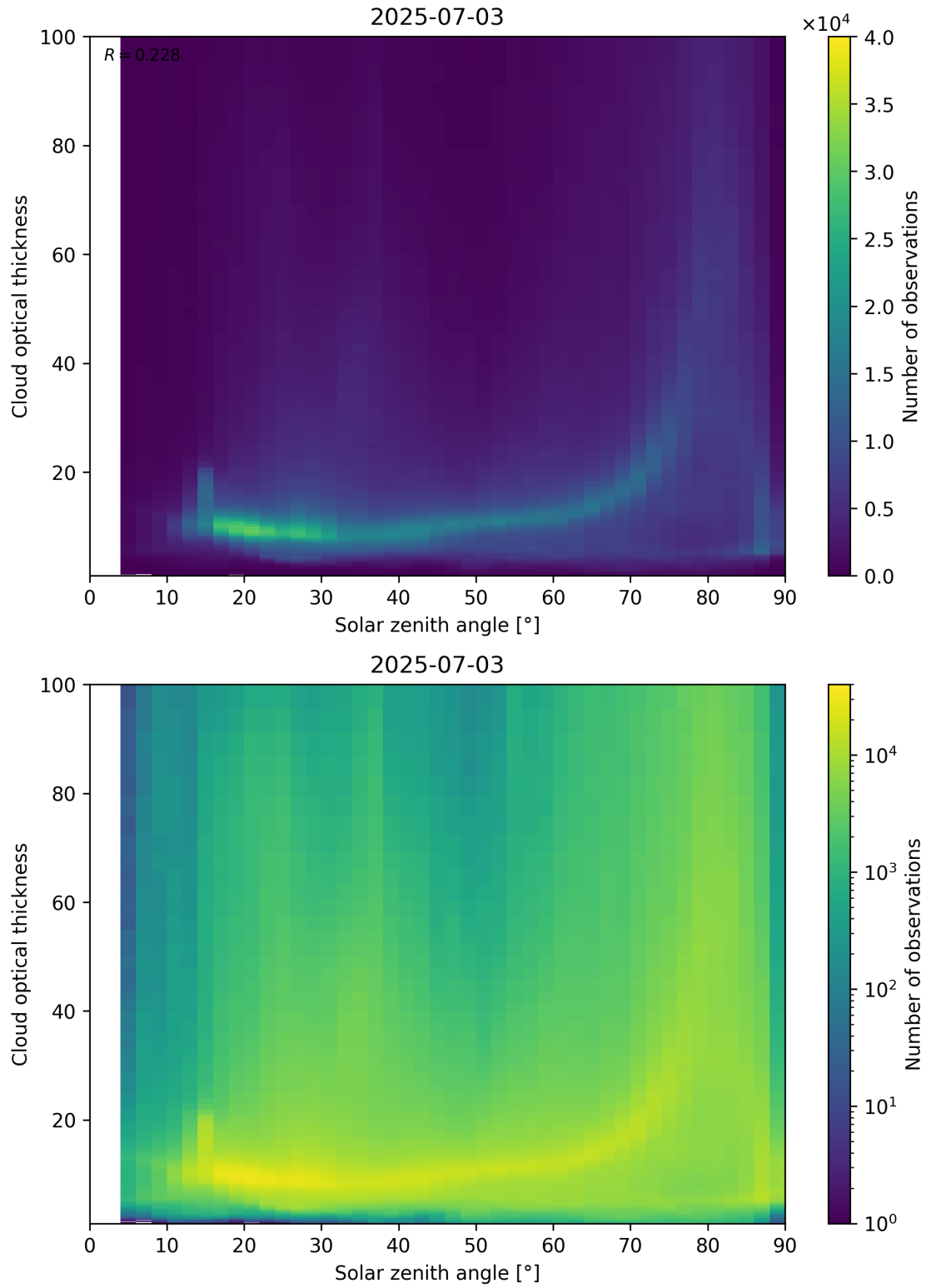
Figure 103: Scatter density plot of “Solar zenith angle” against “Cloud optical thickness” for 2025-07-03 to 2025-07-04.
