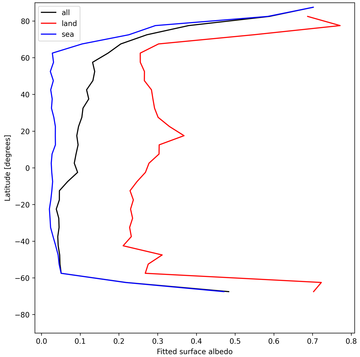
Figure 29: Zonal average of “Fitted surface albedo” for 2025-07-03 to 2025-07-04.
