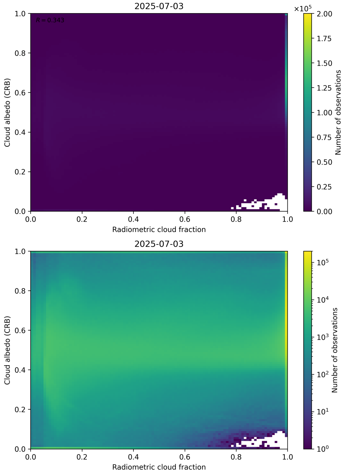
Figure 71: Scatter density plot of “Radiometric cloud fraction” against “Cloud albedo (CRB)” for 2025-07-03 to 2025-07-04.
