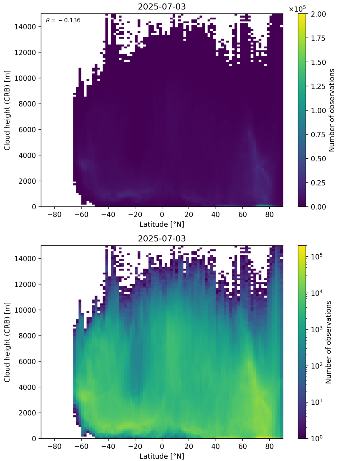
Figure 95: Scatter density plot of “Latitude” against “Cloud height (CRB)” for 2025-07-03 to 2025-07-04.
