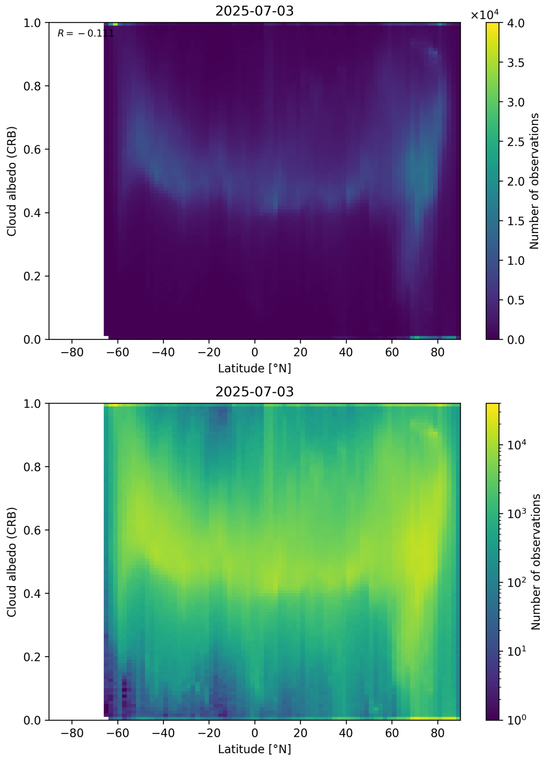
Figure 91: Scatter density plot of “Latitude” against “Cloud albedo (CRB)” for 2025-07-03 to 2025-07-04.
