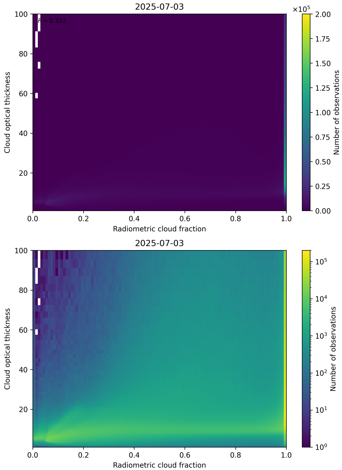
Figure 75: Scatter density plot of “Radiometric cloud fraction” against “Cloud optical thickness” for 2025-07-03 to 2025-07-04.
