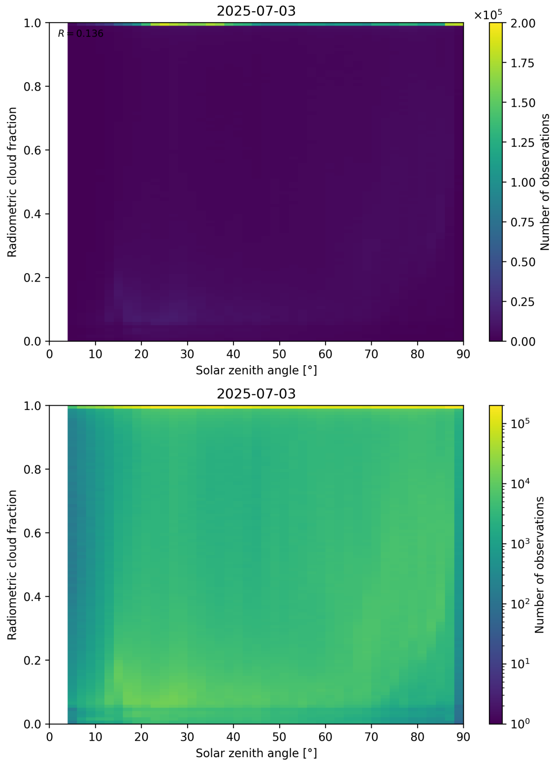
Figure 99: Scatter density plot of “Solar zenith angle” against “Radiometric cloud fraction” for 2025-07-03 to 2025-07-04.
