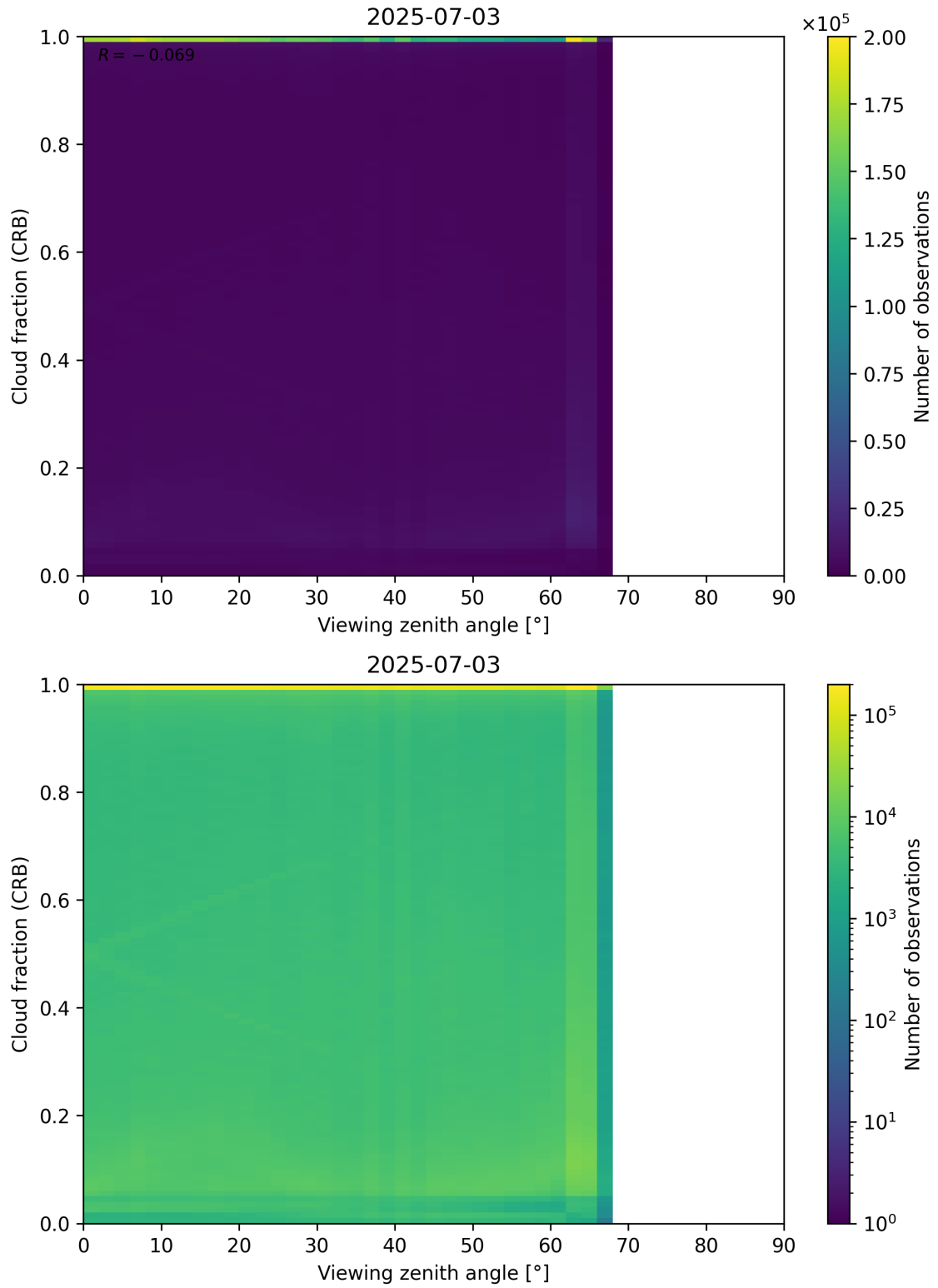
Figure 109: Scatter density plot of “Viewing zenith angle” against “Cloud fraction (CRB)” for 2025-07-03 to 2025-07-04.
