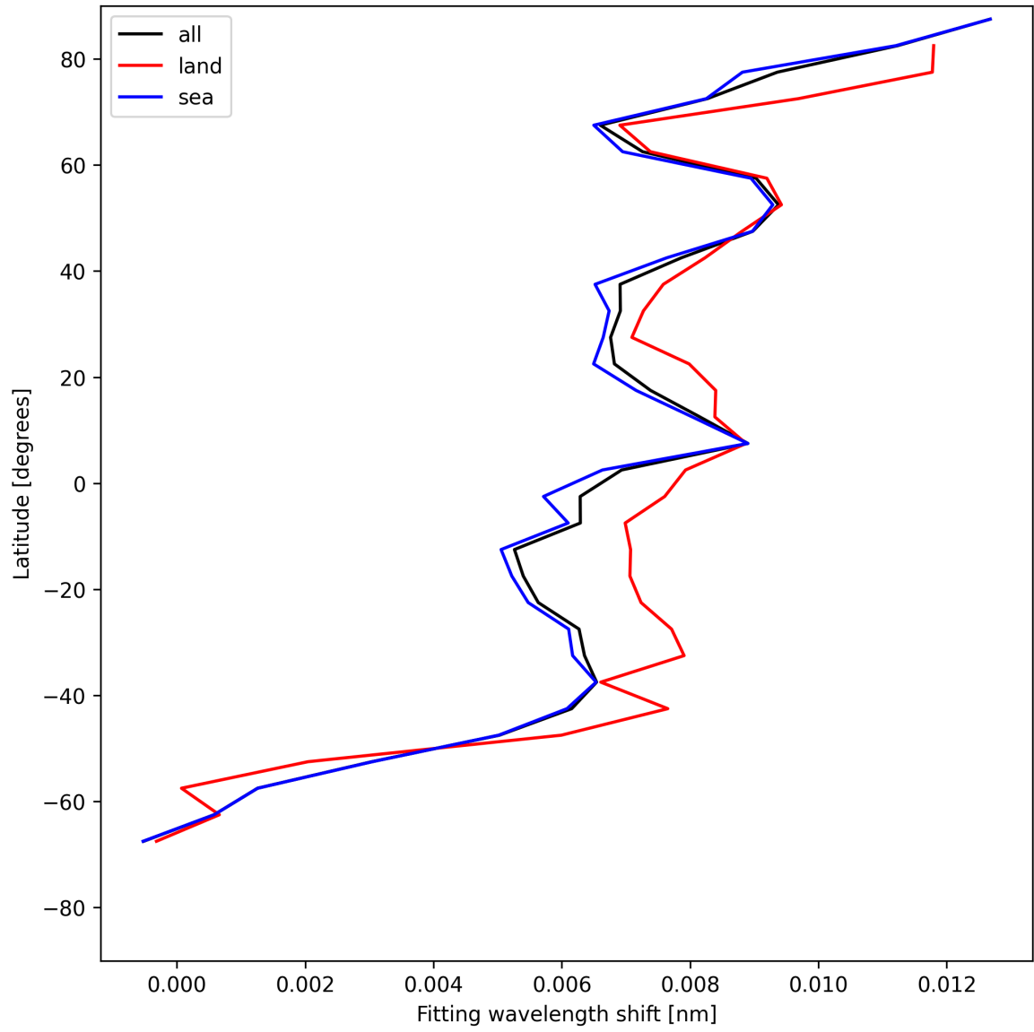
Figure 33: Zonal average of “Fitting wavelength shift” for 2025-07-03 to 2025-07-04.
