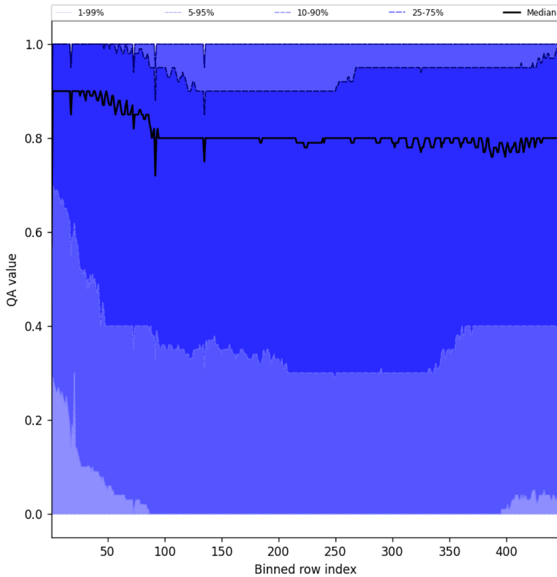
Figure 54: Along track statistics of “QA value” for 2025-07-03 to 2025-07-04
