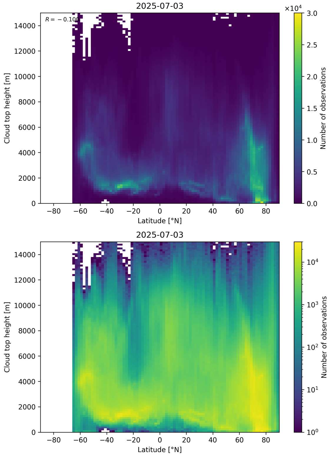
Figure 97: Scatter density plot of “Latitude” against “Cloud top height” for 2025-07-03 to 2025-07-04.
