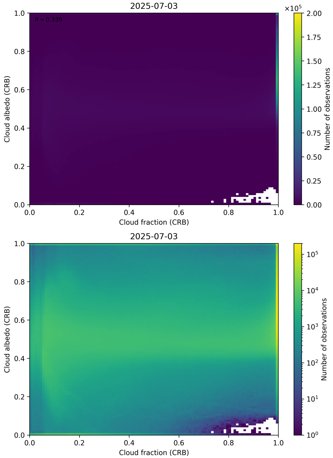
Figure 77: Scatter density plot of “Cloud fraction (CRB)” against “Cloud albedo (CRB)” for 2025-07-03 to 2025-07-04.
