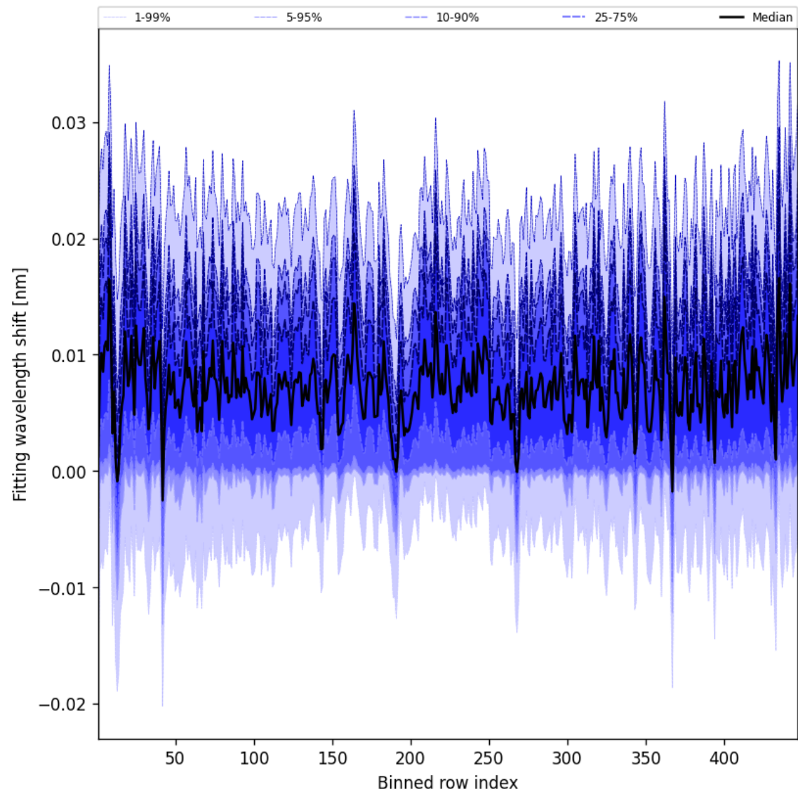
Figure 65: Along track statistics of “Fitting wavelength shift” for 2025-07-03 to 2025-07-04
