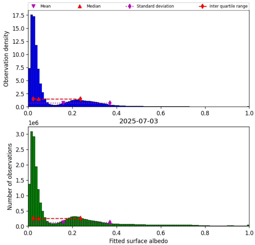
Figure 45: Histogram of “Fitted surface albedo” for 2025-07-03 to 2025-07-04
