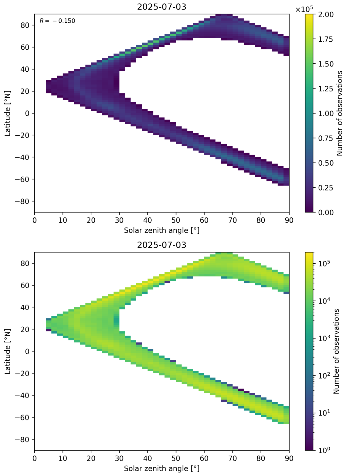
Figure 105: Scatter density plot of “Solar zenith angle” against “Latitude” for 2025-07-03 to 2025-07-04.
