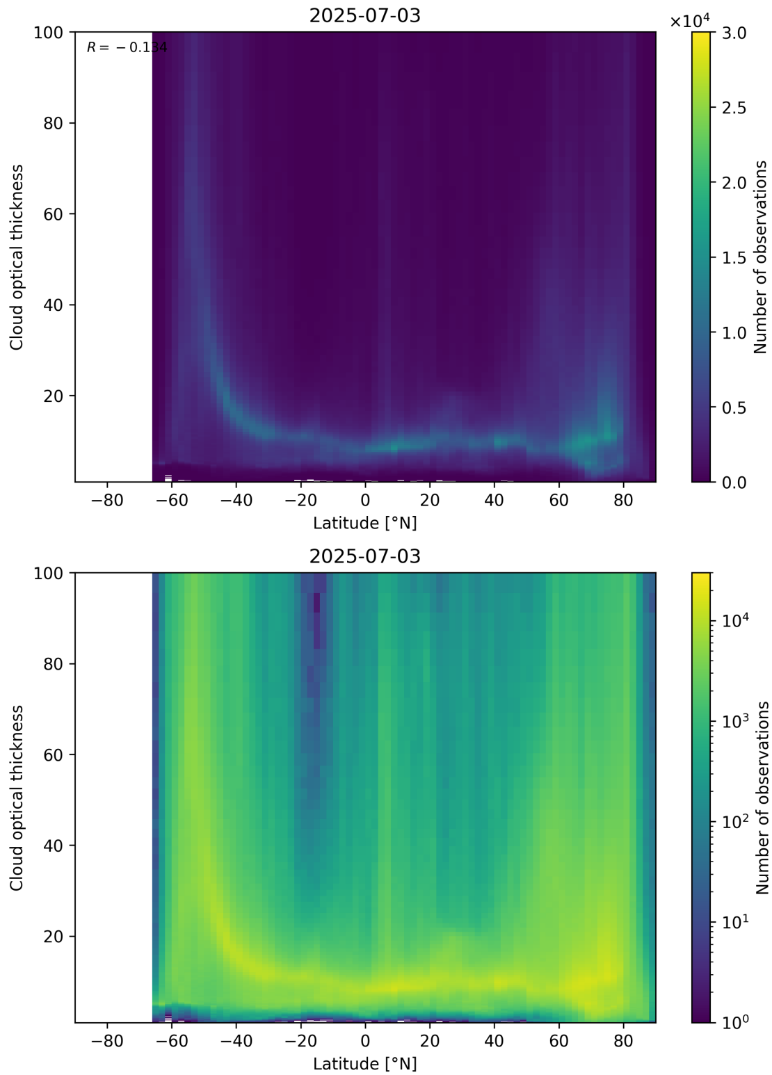
Figure 96: Scatter density plot of “Latitude” against “Cloud optical thickness” for 2025-07-03 to 2025-07-04.
