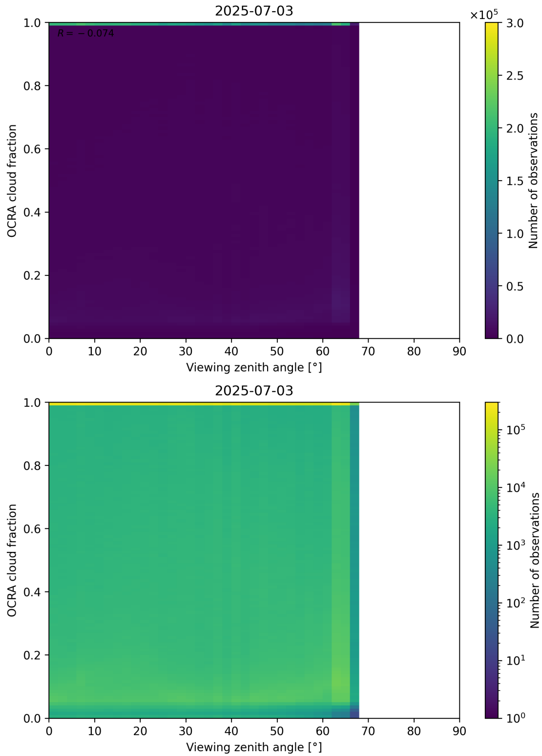
Figure 108: Scatter density plot of “Viewing zenith angle” against “OCRA cloud fraction” for 2025-07-03 to 2025-07-04.
