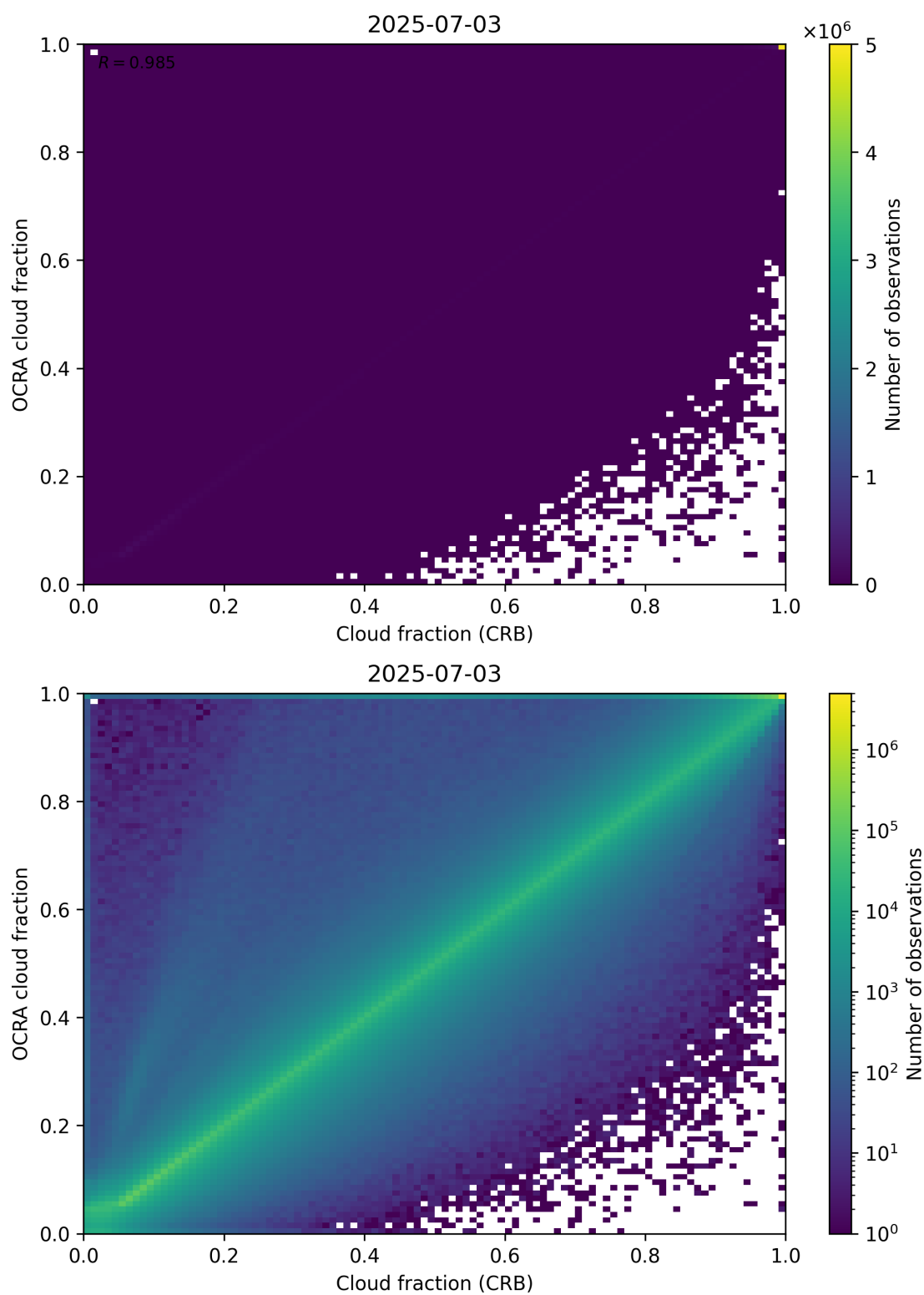
Figure 78: Scatter density plot of “Cloud fraction (CRB)” against “OCRA cloud fraction” for 2025-07-03 to 2025-07-04.
