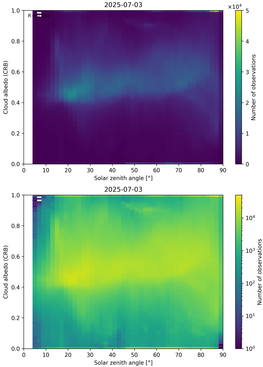
Figure 98: Scatter density plot of “Solar zenith angle” against “Cloud albedo (CRB)” for 2025-07-03 to 2025-07-04.
