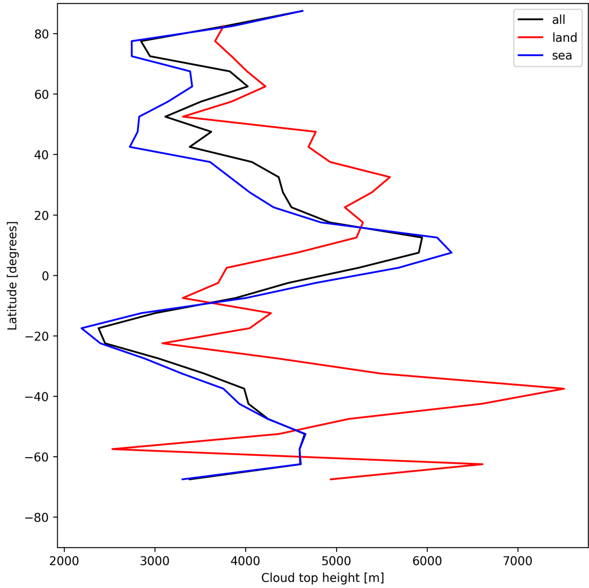
Figure 24: Zonal average of “Cloud top height” for 2025-07-03 to 2025-07-04.
