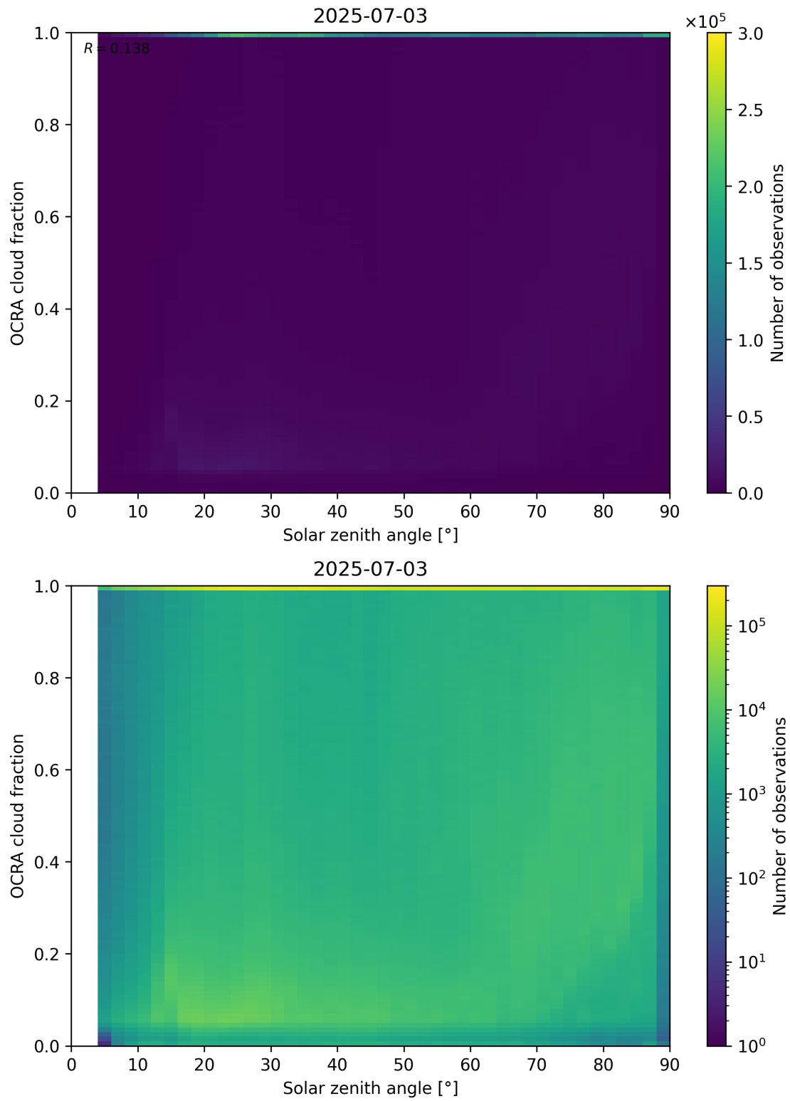
Figure 100: Scatter density plot of “Solar zenith angle” against “OCRA cloud fraction” for 2025-07-03 to 2025-07-04.
