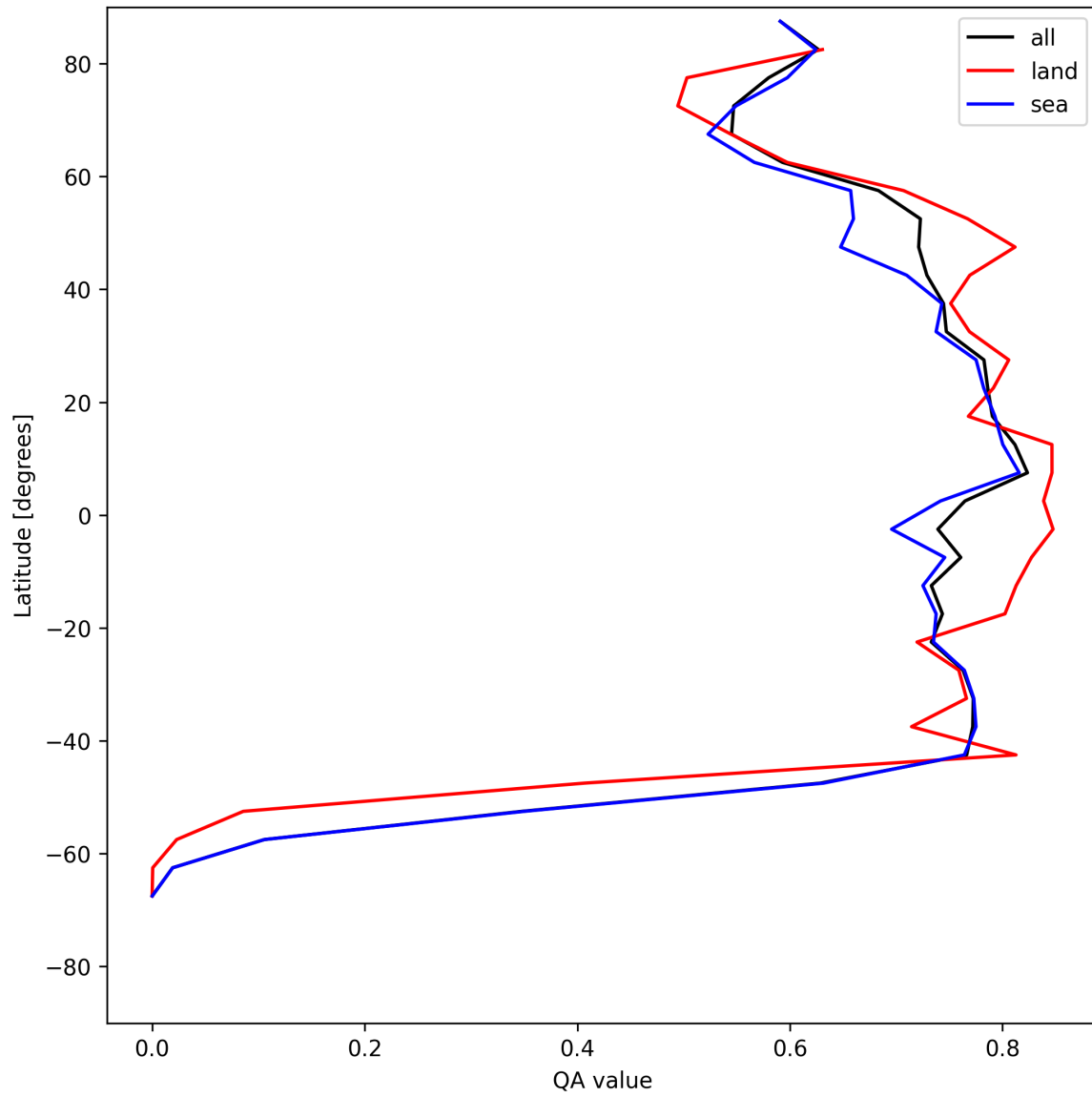
Figure 22: Zonal average of “QA value” for 2025-07-03 to 2025-07-04.
