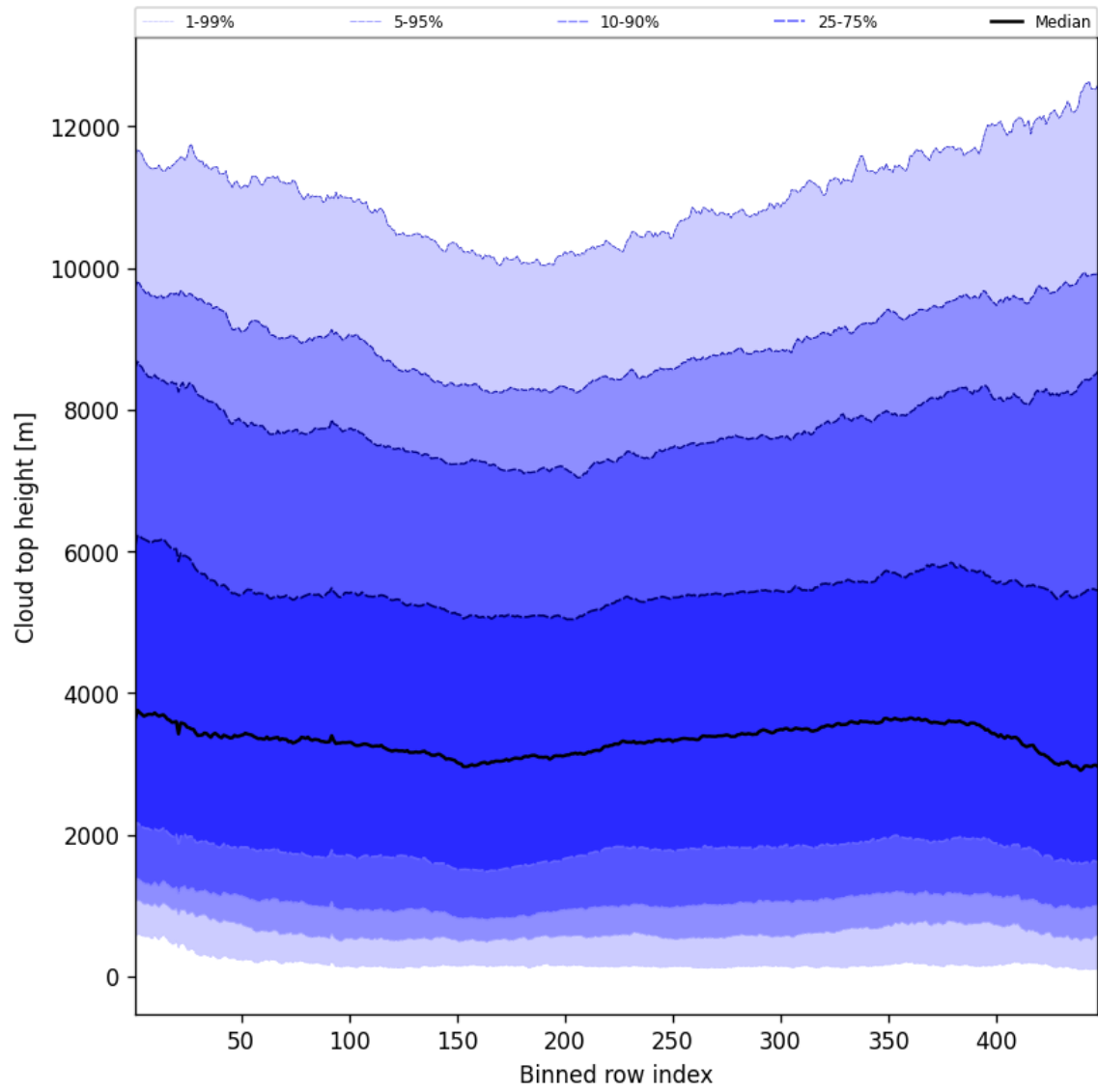
Figure 56: Along track statistics of “Cloud top height” for 2025-07-03 to 2025-07-04
