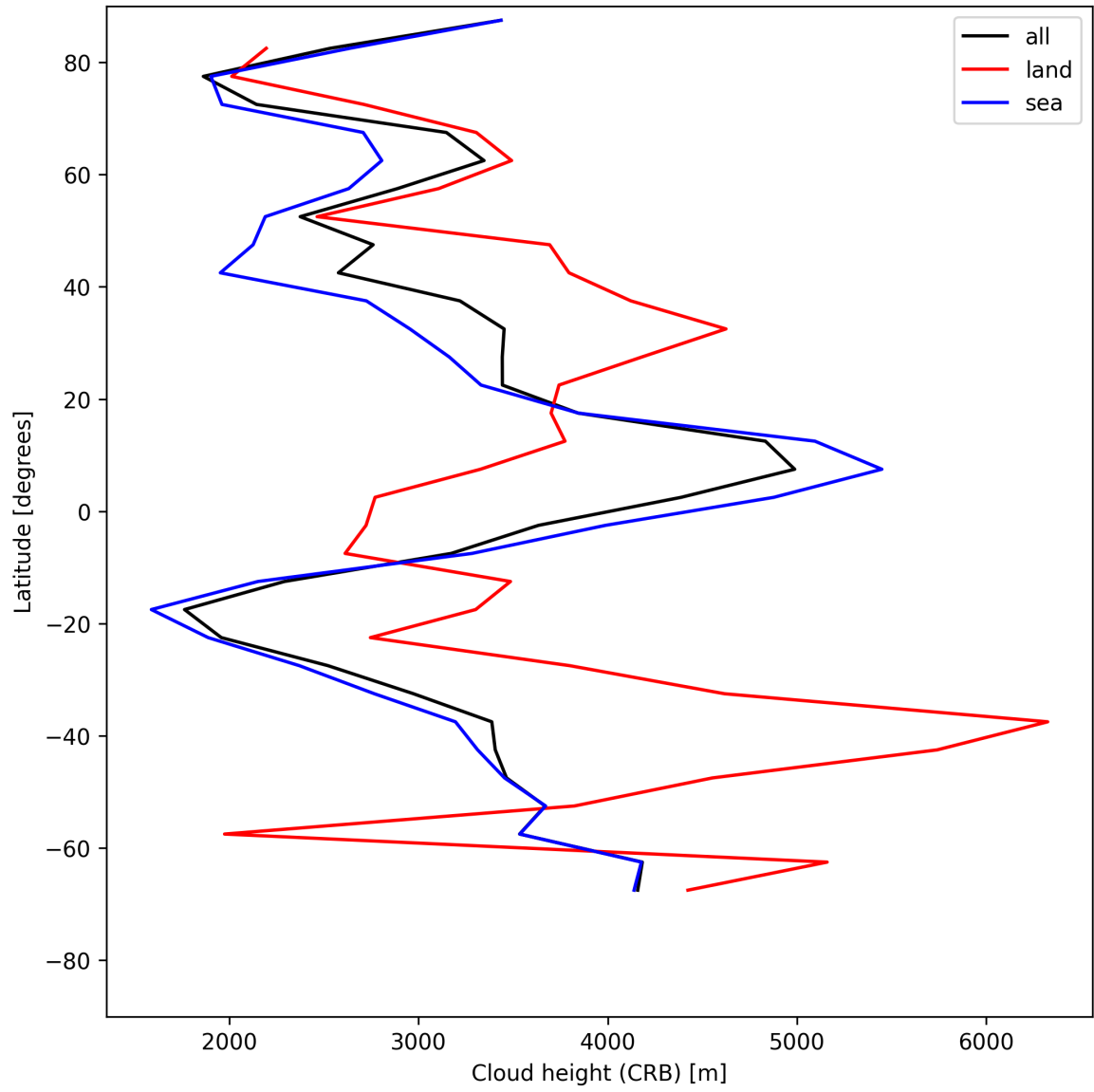
Figure 27: Zonal average of “Cloud height (CRB)” for 2025-07-03 to 2025-07-04.
