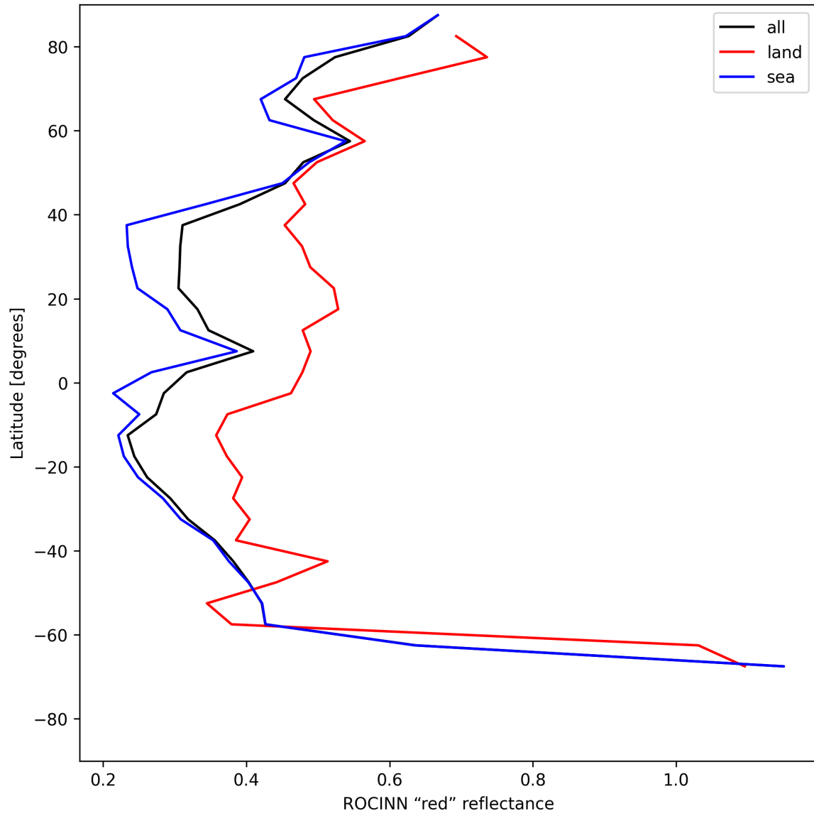
Figure 37: Zonal average of “ROCINN “red” reflectance” for 2025-07-03 to 2025-07-04.
