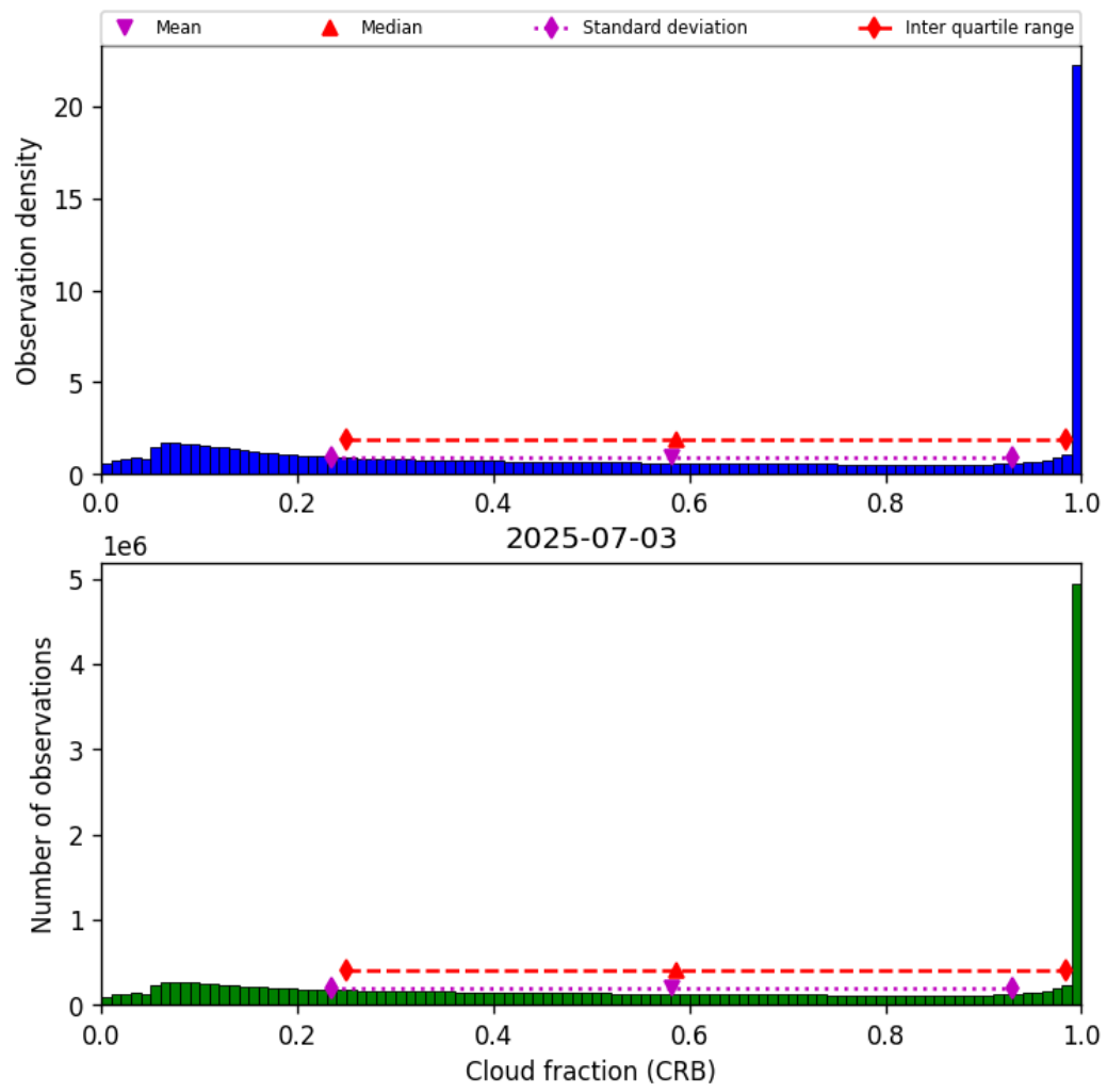
Figure 42: Histogram of “Cloud fraction (CRB)” for 2025-07-03 to 2025-07-04
