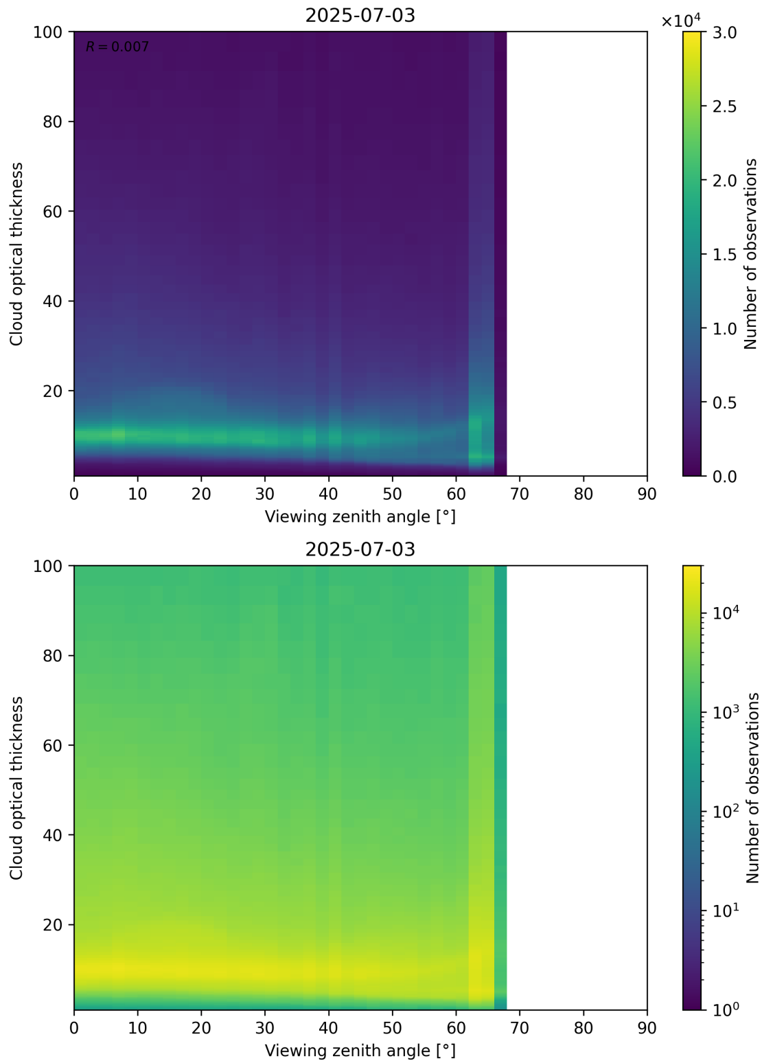
Figure 111: Scatter density plot of “Viewing zenith angle” against “Cloud optical thickness” for 2025-07-03 to 2025-07-04.
