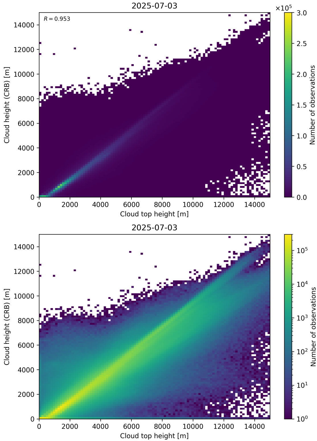
Figure 89: Scatter density plot of “Cloud top height” against “Cloud height (CRB)” for 2025-07-03 to 2025-07-04.
