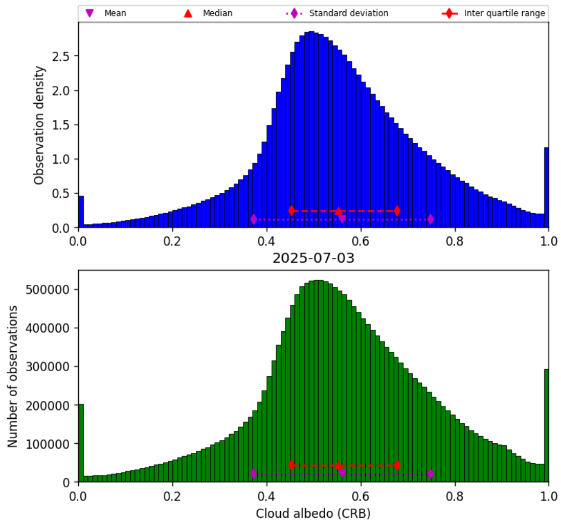
Figure 44: Histogram of “Cloud albedo (CRB)” for 2025-07-03 to 2025-07-04
