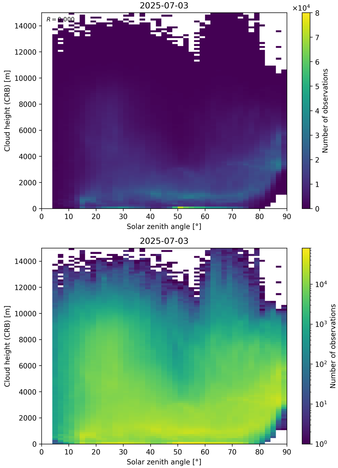
Figure 102: Scatter density plot of “Solar zenith angle” against “Cloud height (CRB)” for 2025-07-03 to 2025-07-04.
