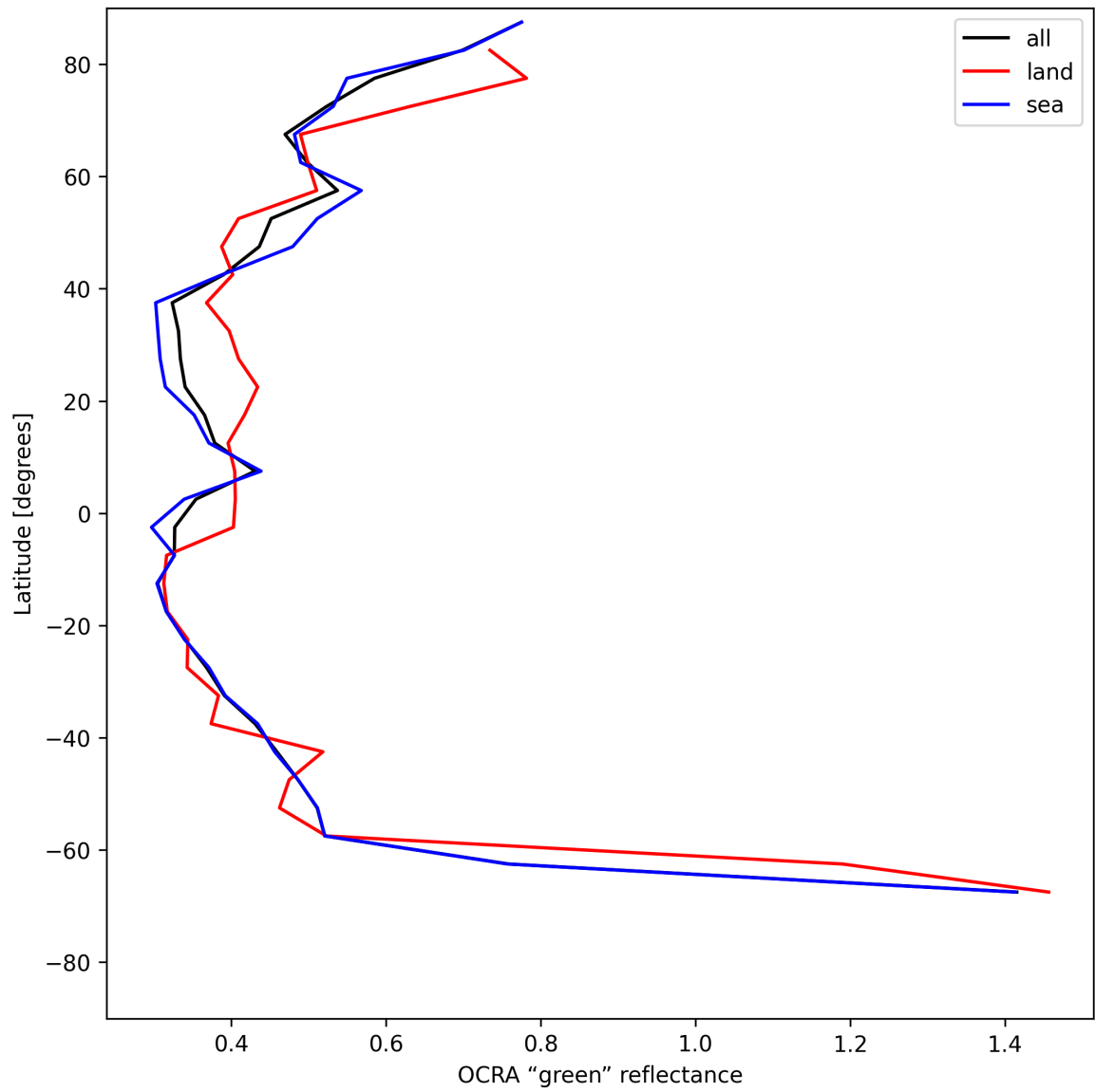
Figure 36: Zonal average of “OCRA “green” reflectance” for 2025-07-03 to 2025-07-04.
