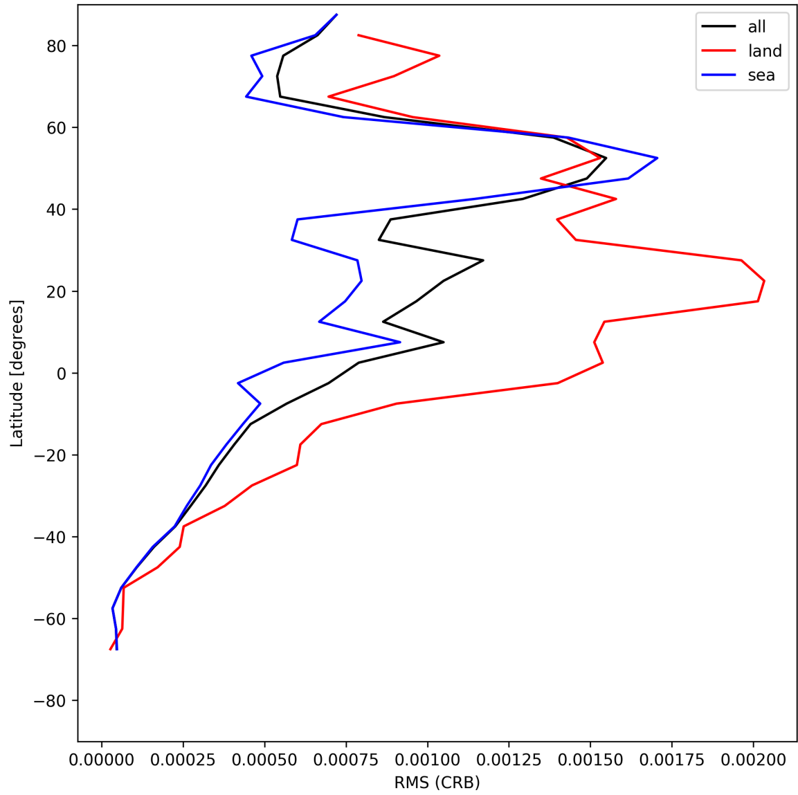
Figure 32: Zonal average of “RMS (CRB)” for 2025-07-03 to 2025-07-04.
