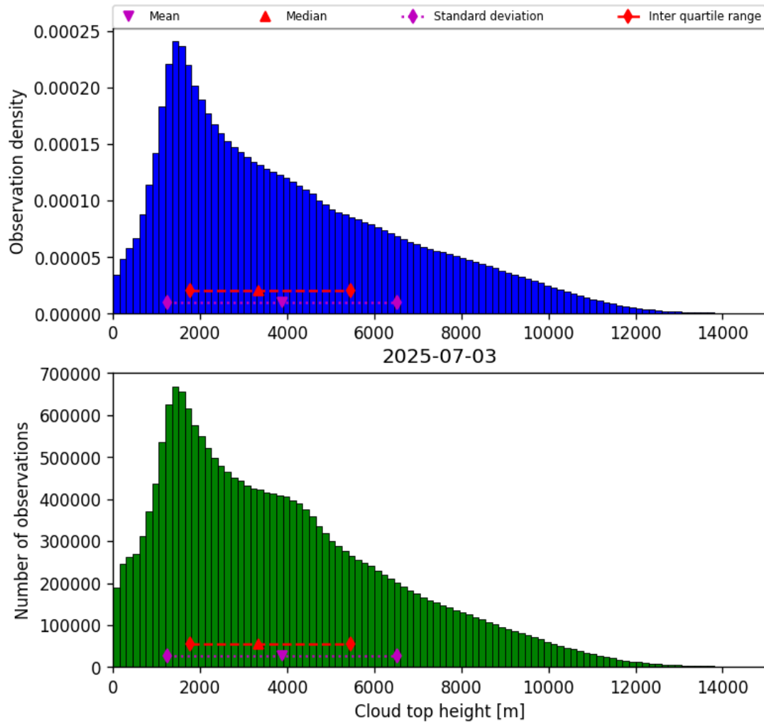
Figure 40: Histogram of “Cloud top height” for 2025-07-03 to 2025-07-04
