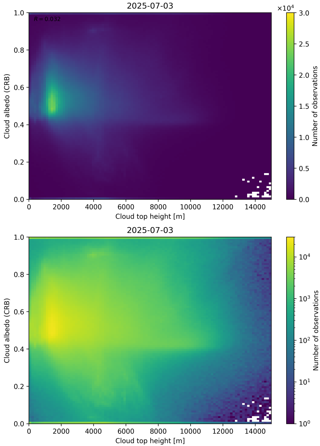
Figure 86: Scatter density plot of “Cloud top height” against “Cloud albedo (CRB)” for 2025-07-03 to 2025-07-04.
