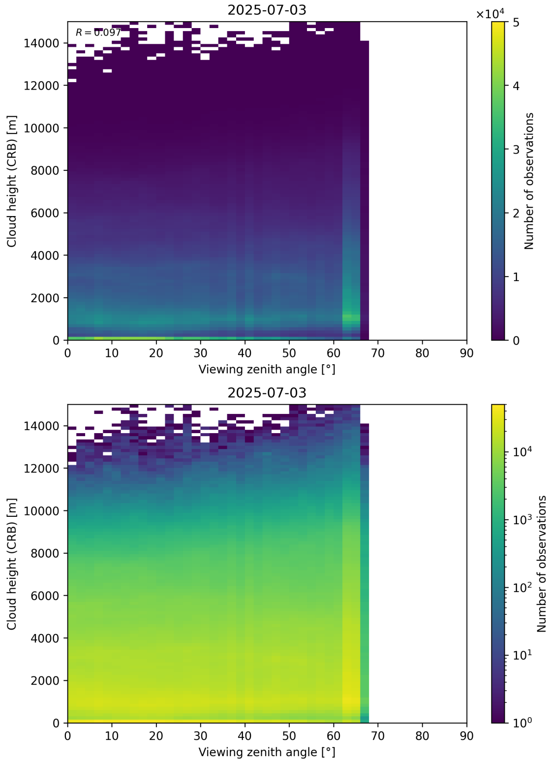
Figure 110: Scatter density plot of “Viewing zenith angle” against “Cloud height (CRB)” for 2025-07-03 to 2025-07-04.
