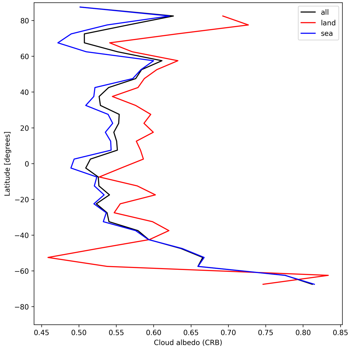
Figure 28: Zonal average of “Cloud albedo (CRB)” for 2025-07-03 to 2025-07-04.
