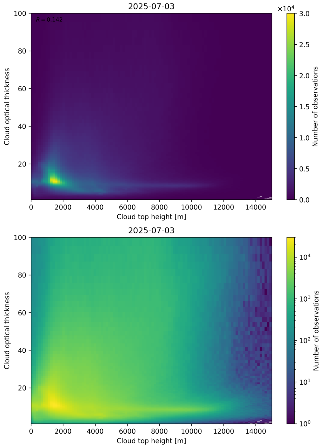
Figure 90: Scatter density plot of “Cloud top height” against “Cloud optical thickness” for 2025-07-03 to 2025-07-04.
