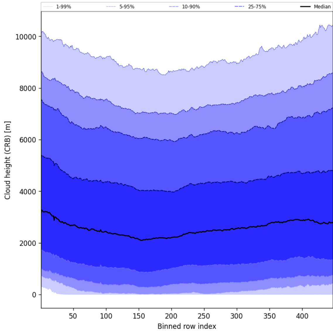
Figure 59: Along track statistics of “Cloud height (CRB)” for 2025-07-03 to 2025-07-04
