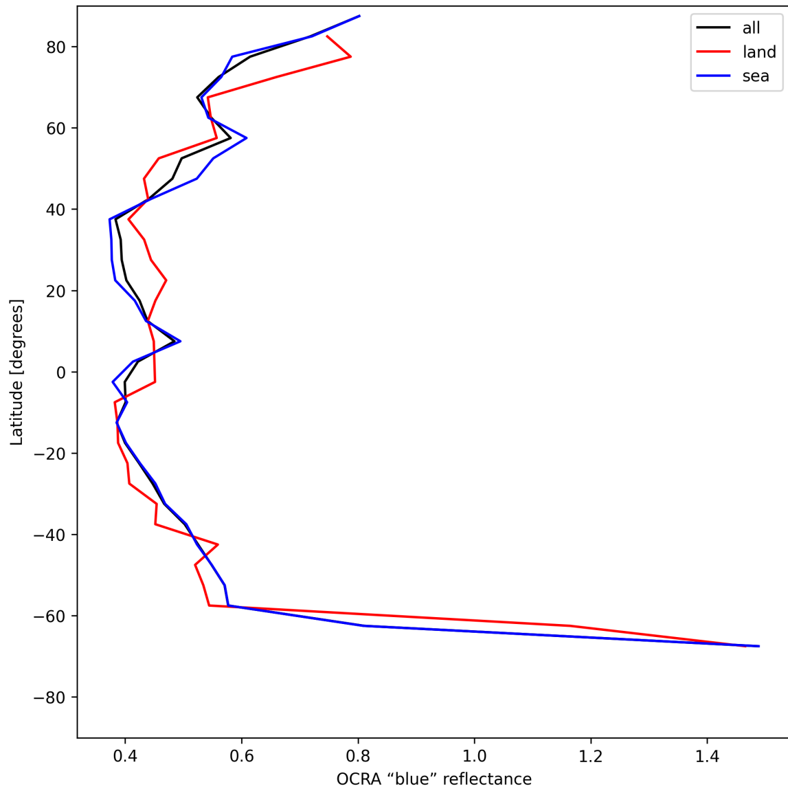
Figure 35: Zonal average of "OCRA "blue" reflectance" for 2025-07-03 to 2025-07-04.
