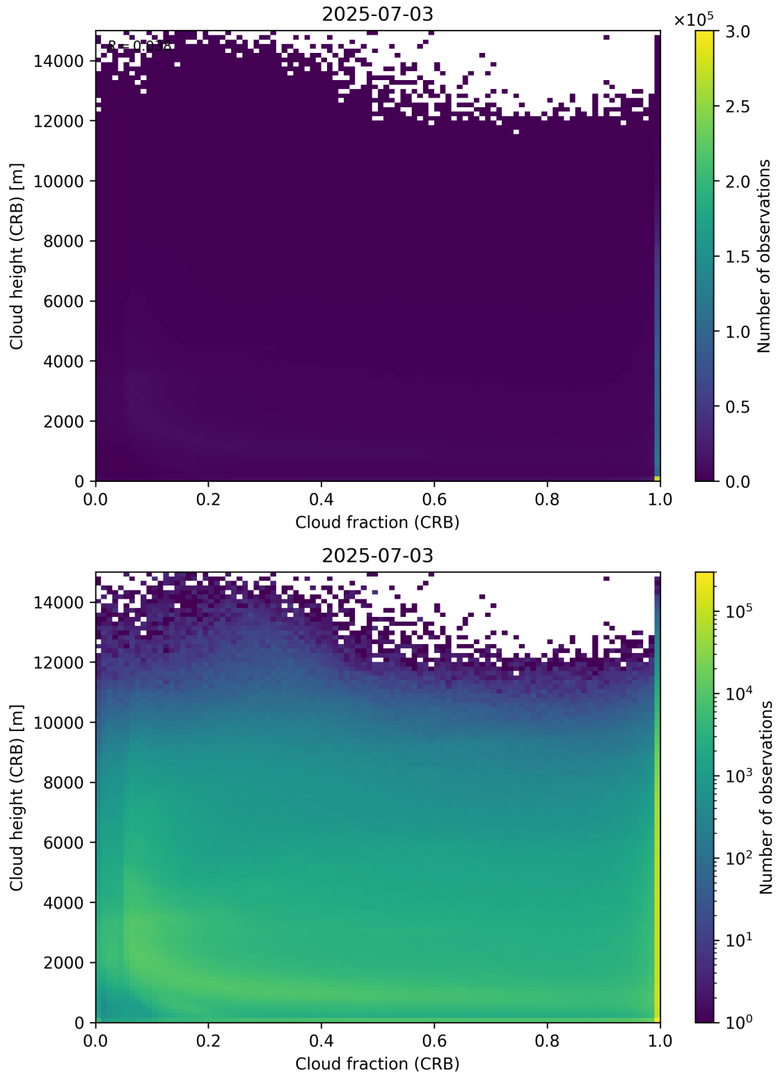
Figure 79: Scatter density plot of “Cloud fraction (CRB)” against “Cloud height (CRB)” for 2025-07-03 to 2025-07-04.
