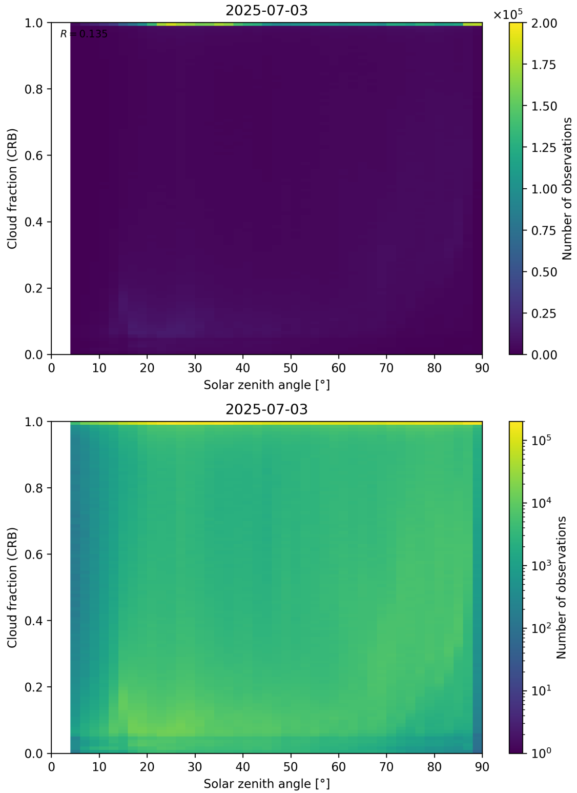
Figure 101: Scatter density plot of “Solar zenith angle” against “Cloud fraction (CRB)” for 2025-07-03 to 2025-07-04.
