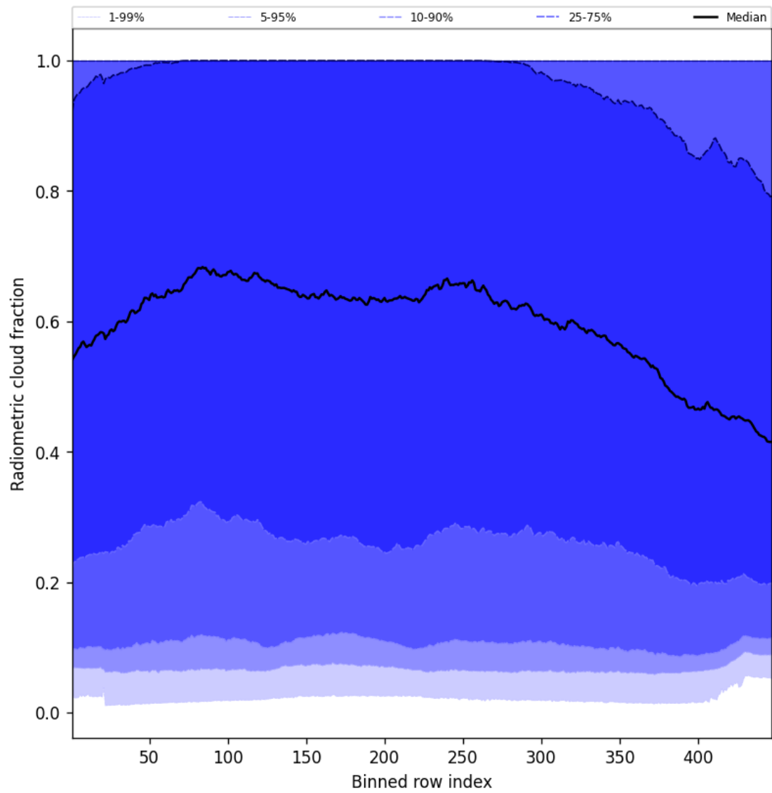
Figure 55: Along track statistics of “Radiometric cloud fraction” for 2025-07-03 to 2025-07-04
