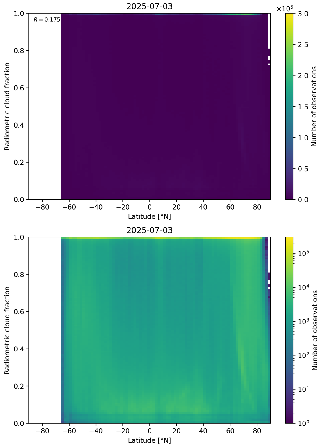
Figure 92: Scatter density plot of “Latitude” against “Radiometric cloud fraction” for 2025-07-03 to 2025-07-04.
