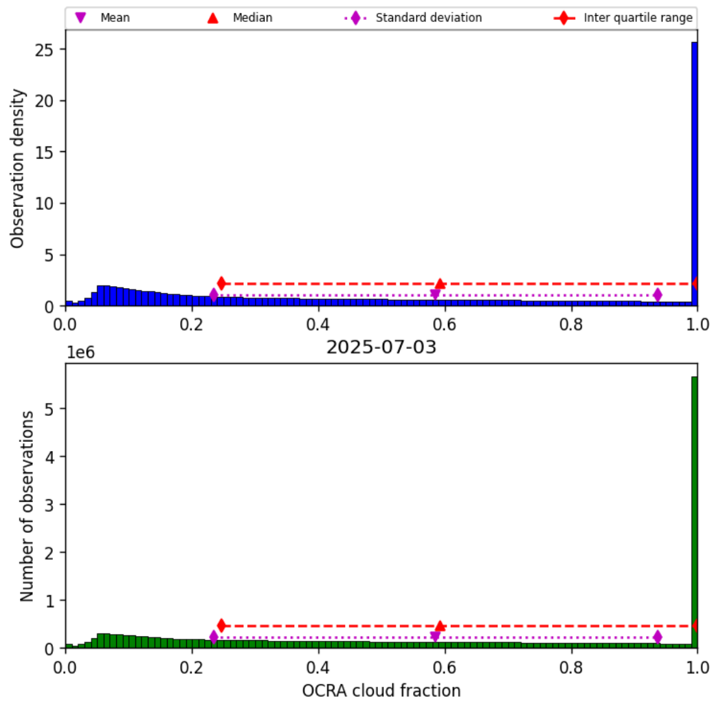
Figure 50: Histogram of “OCRA cloud fraction” for 2025-07-03 to 2025-07-04
