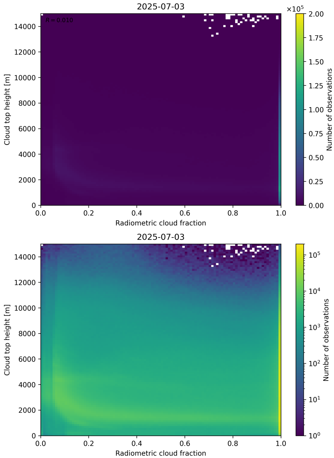
Figure 76: Scatter density plot of “Radiometric cloud fraction” against “Cloud top height” for 2025-07-03 to 2025-07-04.
