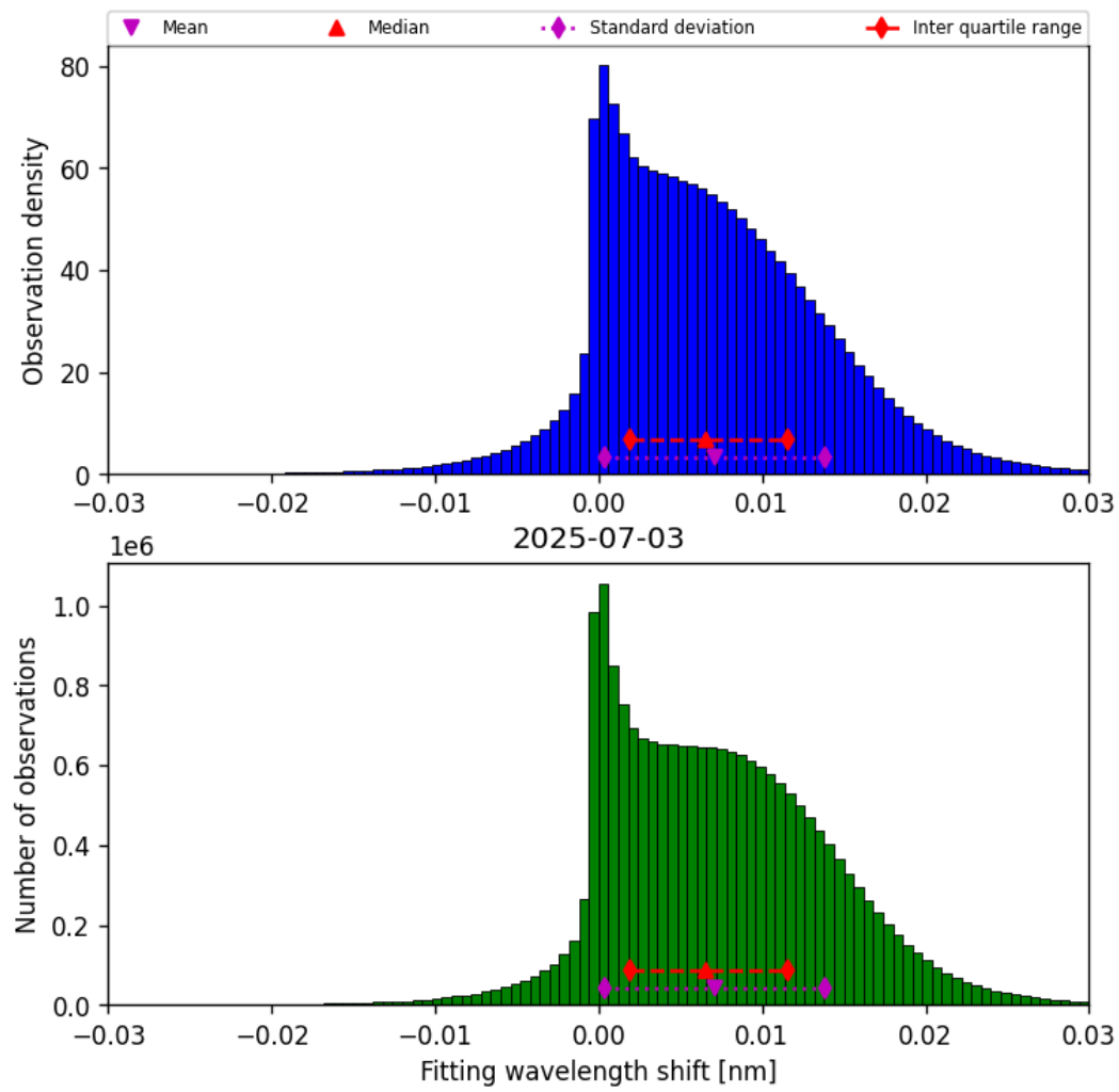
Figure 49: Histogram of “Fitting wavelength shift” for 2025-07-03 to 2025-07-04
