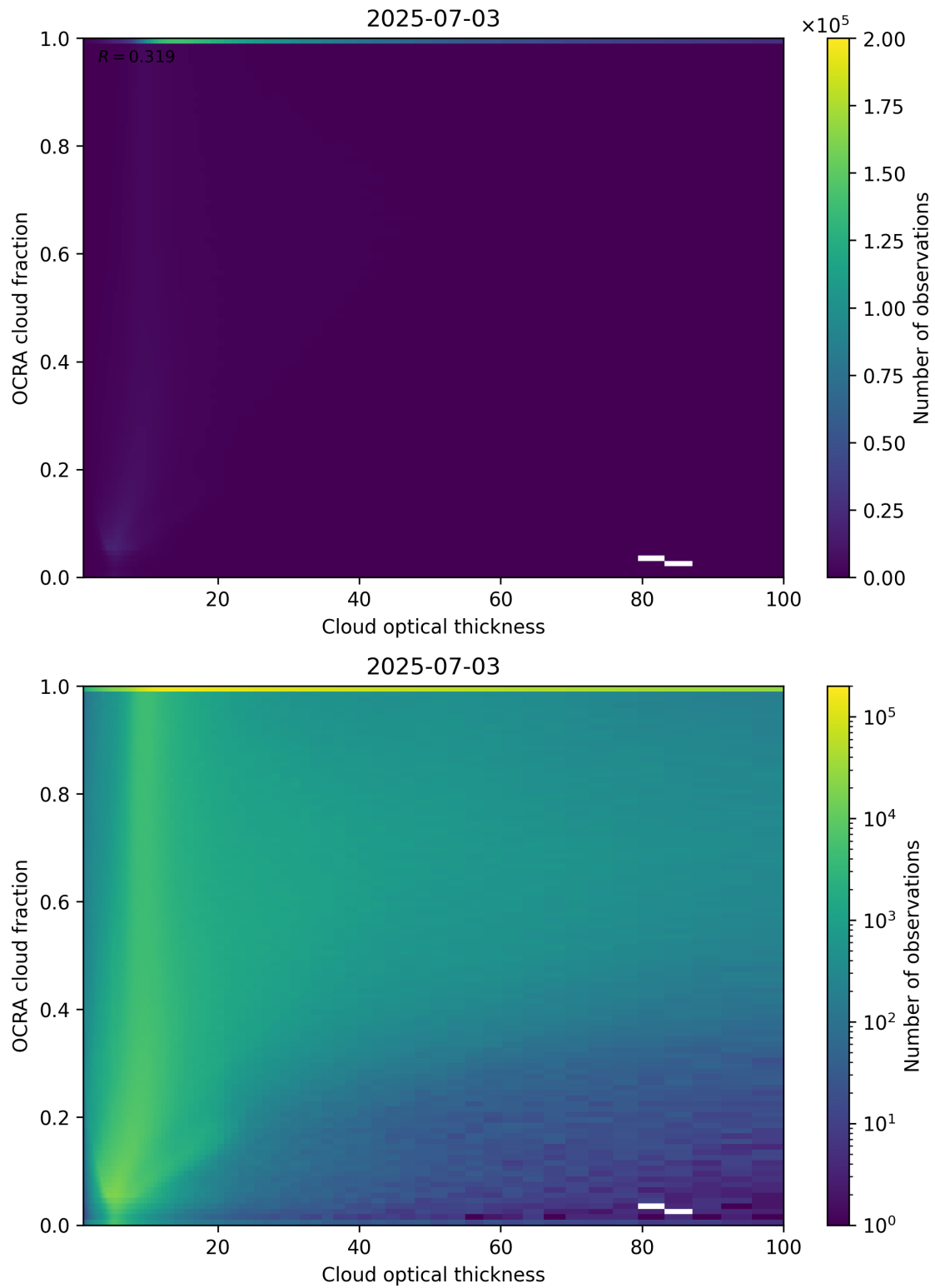
Figure 83: Scatter density plot of “Cloud optical thickness” against “OCRA cloud fraction” for 2025-07-03 to 2025-07-04.
