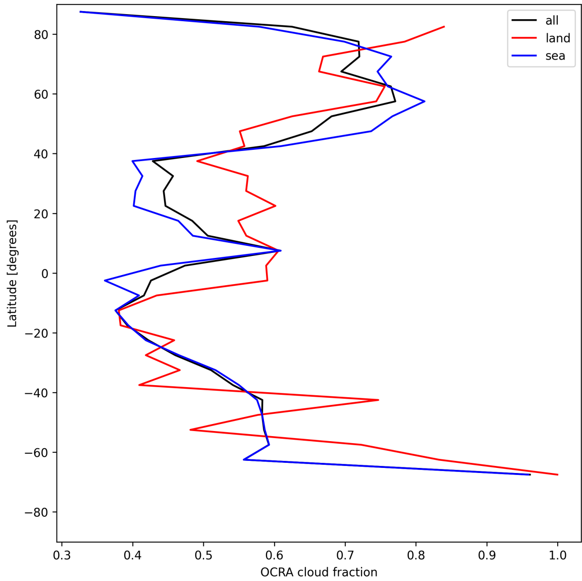
Figure 34: Zonal average of “OCRA cloud fraction” for 2025-07-03 to 2025-07-04.
