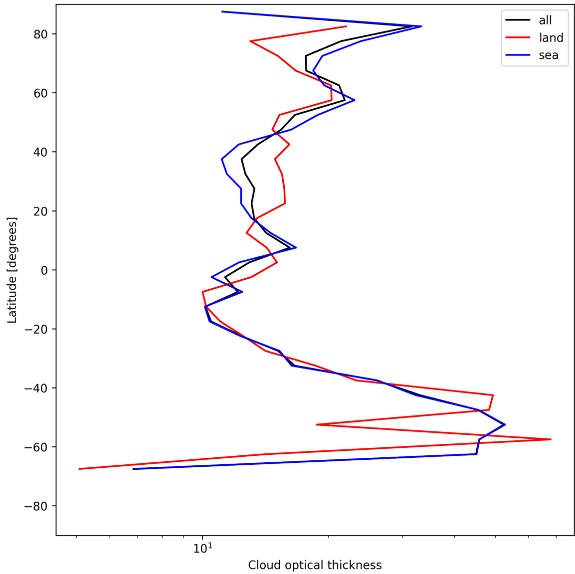
Figure 25: Zonal average of “Cloud optical thickness” for 2025-07-03 to 2025-07-04.
