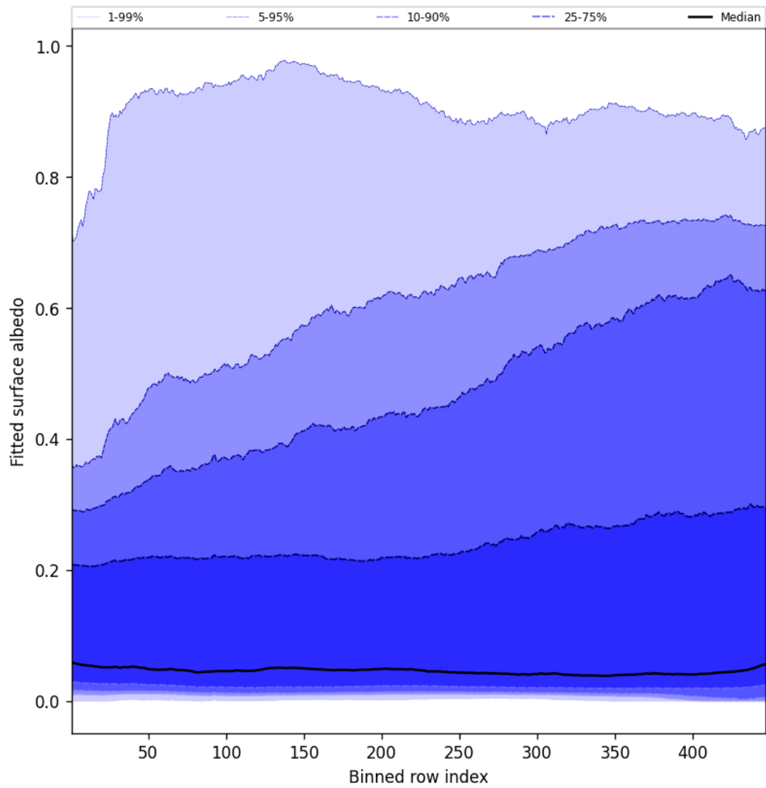
Figure 61: Along track statistics of “Fitted surface albedo” for 2025-07-03 to 2025-07-04
