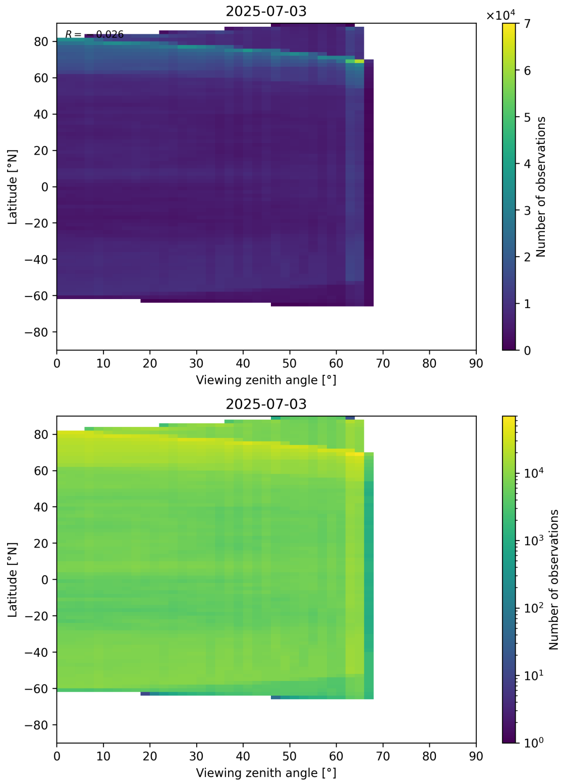
Figure 113: Scatter density plot of “Viewing zenith angle” against “Latitude” for 2025-07-03 to 2025-07-04.
