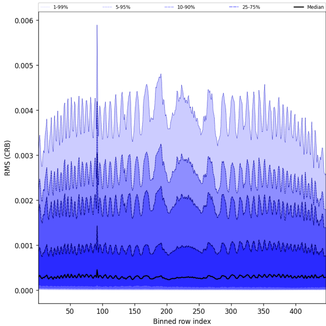
Figure 64: Along track statistics of “RMS (CRB)” for 2025-07-03 to 2025-07-04
