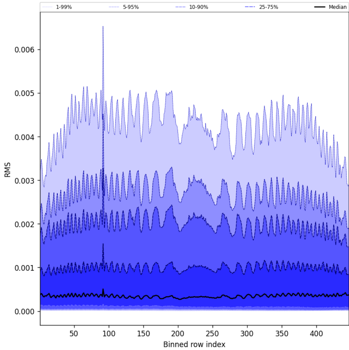
Figure 63: Along track statistics of “RMS” for 2025-07-03 to 2025-07-04
