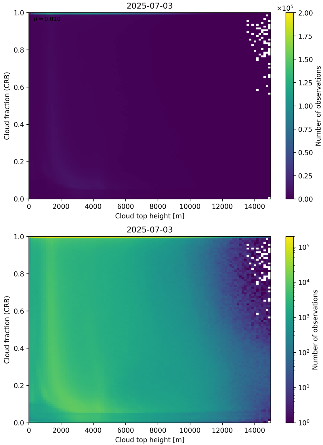
Figure 88: Scatter density plot of “Cloud top height” against “Cloud fraction (CRB)” for 2025-07-03 to 2025-07-04.
