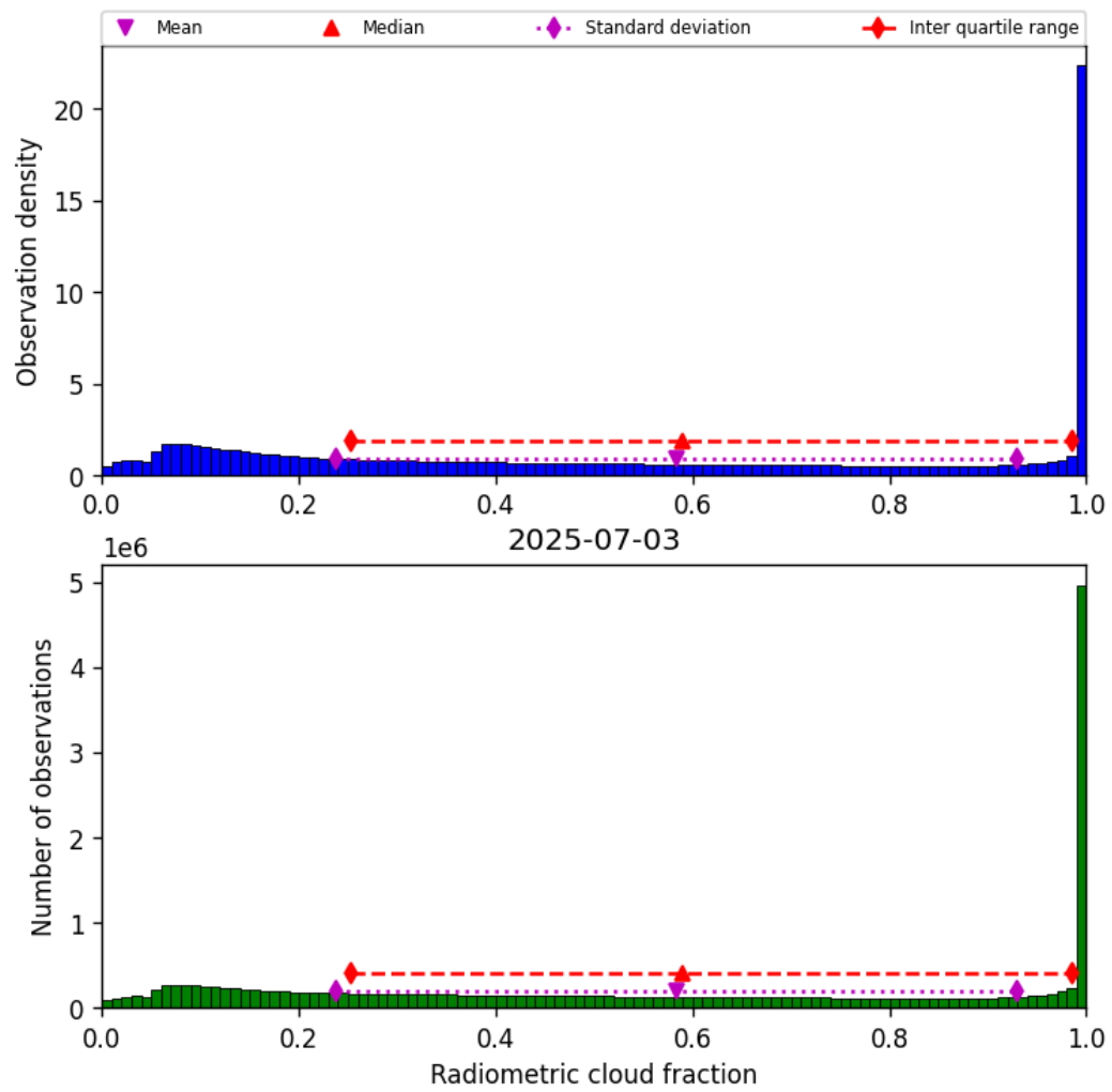
Figure 39: Histogram of “Radiometric cloud fraction” for 2025-07-03 to 2025-07-04
