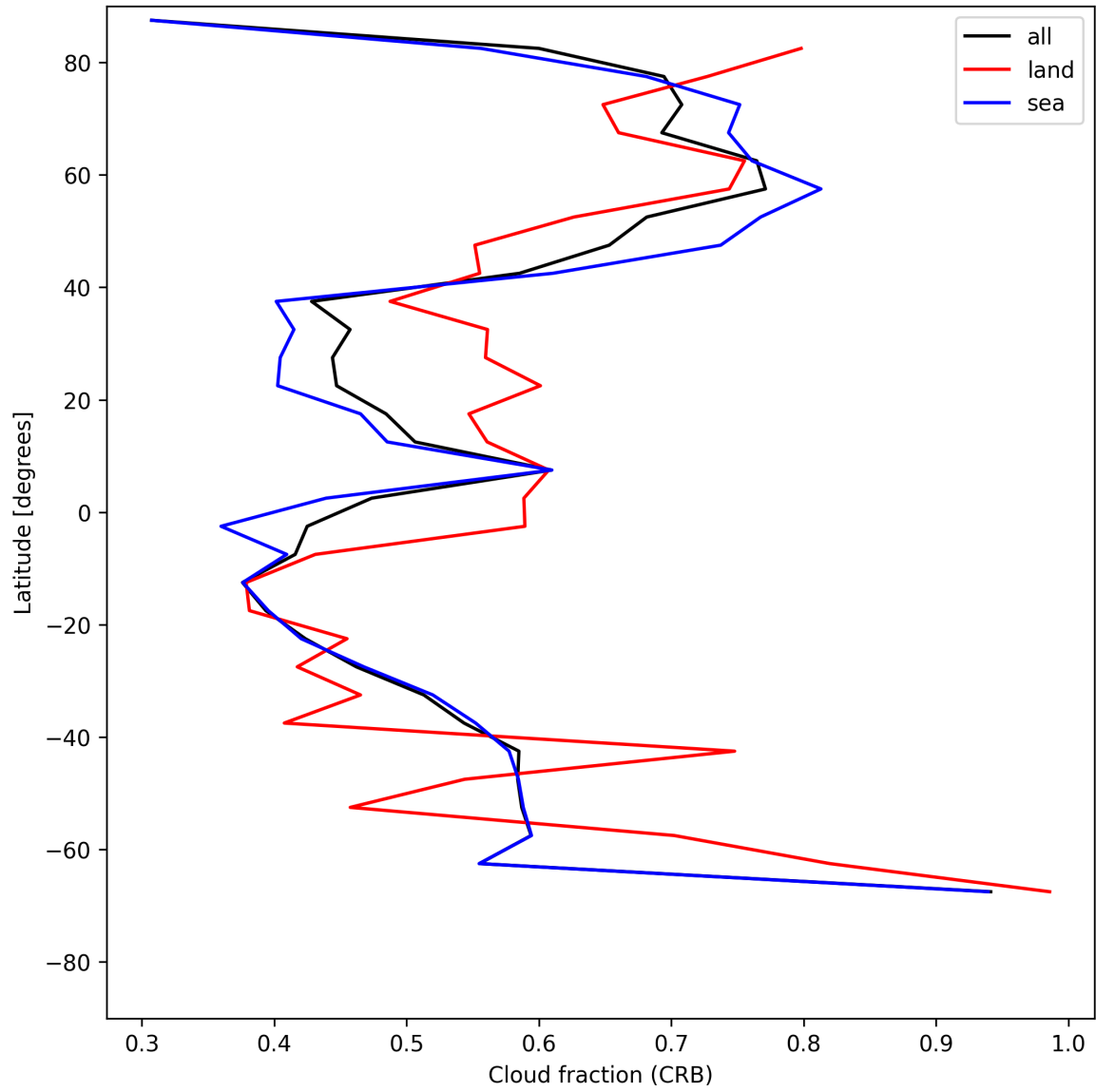
Figure 26: Zonal average of “Cloud fraction (CRB)” for 2025-07-03 to 2025-07-04.
