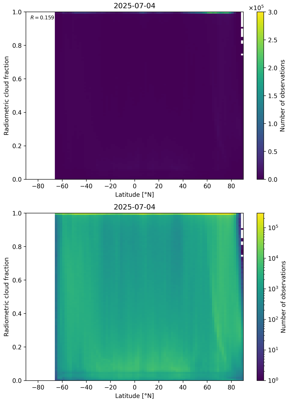
Figure 92: Scatter density plot of “Latitude” against “Radiometric cloud fraction” for 2025-07-03 to 2025-07-05.
