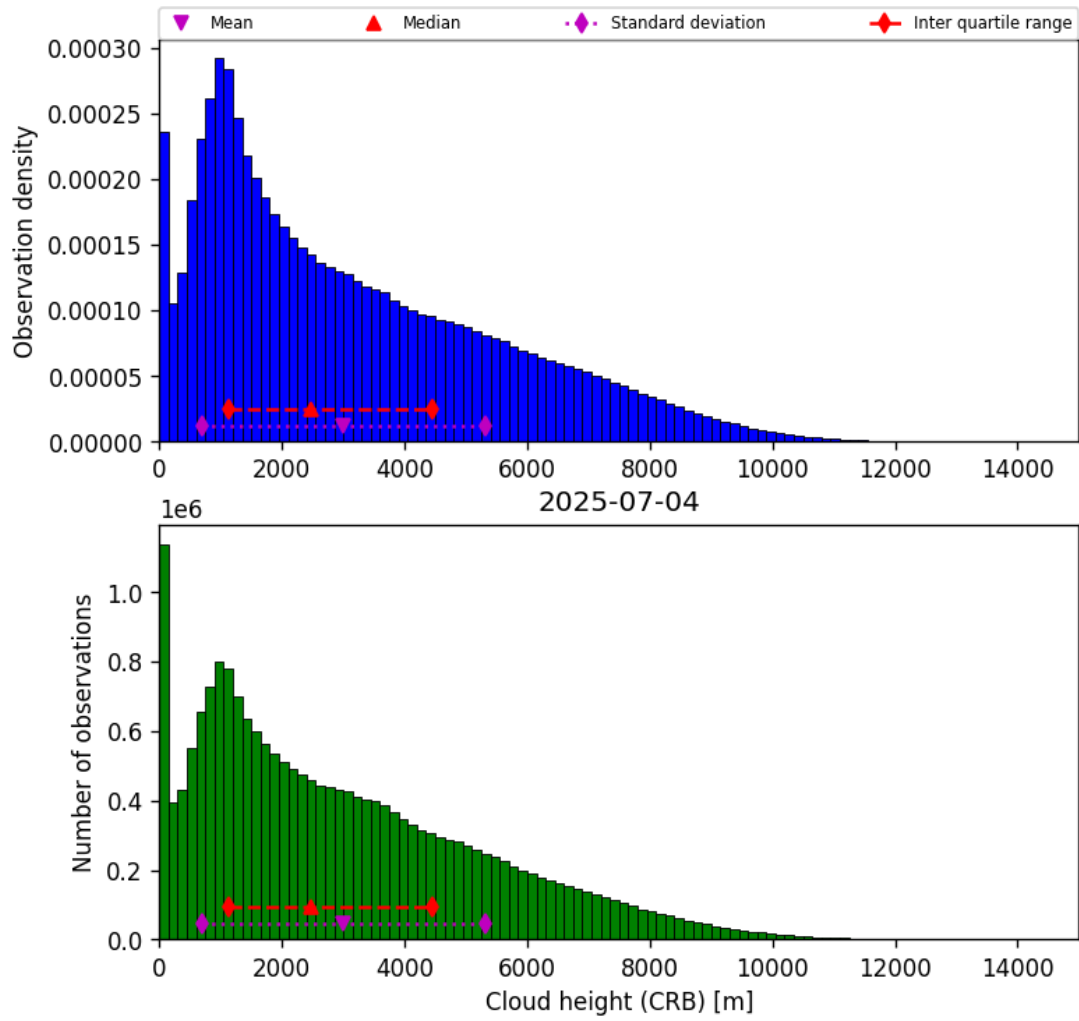
Figure 43: Histogram of “Cloud height (CRB)” for 2025-07-03 to 2025-07-05
