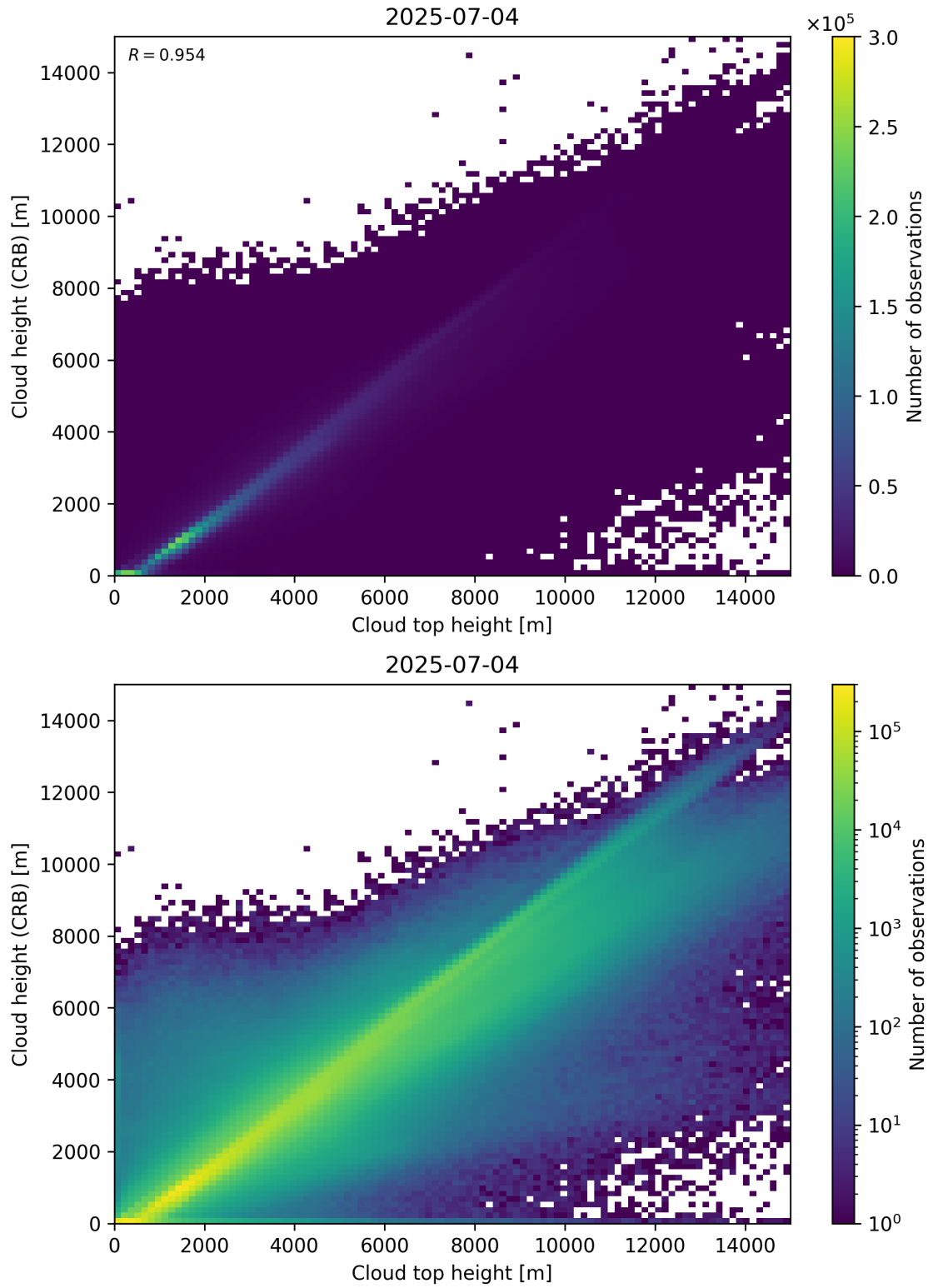
Figure 89: Scatter density plot of “Cloud top height” against “Cloud height (CRB)” for 2025-07-03 to 2025-07-05.
