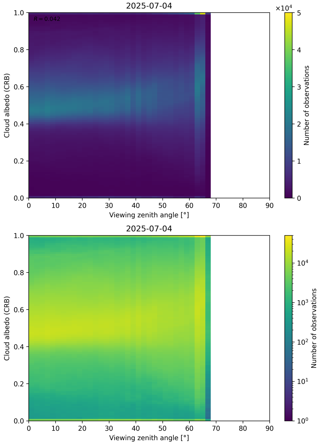
Figure 106: Scatter density plot of “Viewing zenith angle” against “Cloud albedo (CRB)” for 2025-07-03 to 2025-07-05.
