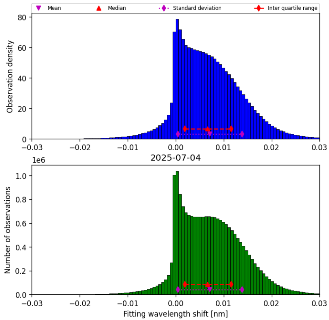
Figure 49: Histogram of “Fitting wavelength shift” for 2025-07-03 to 2025-07-05
