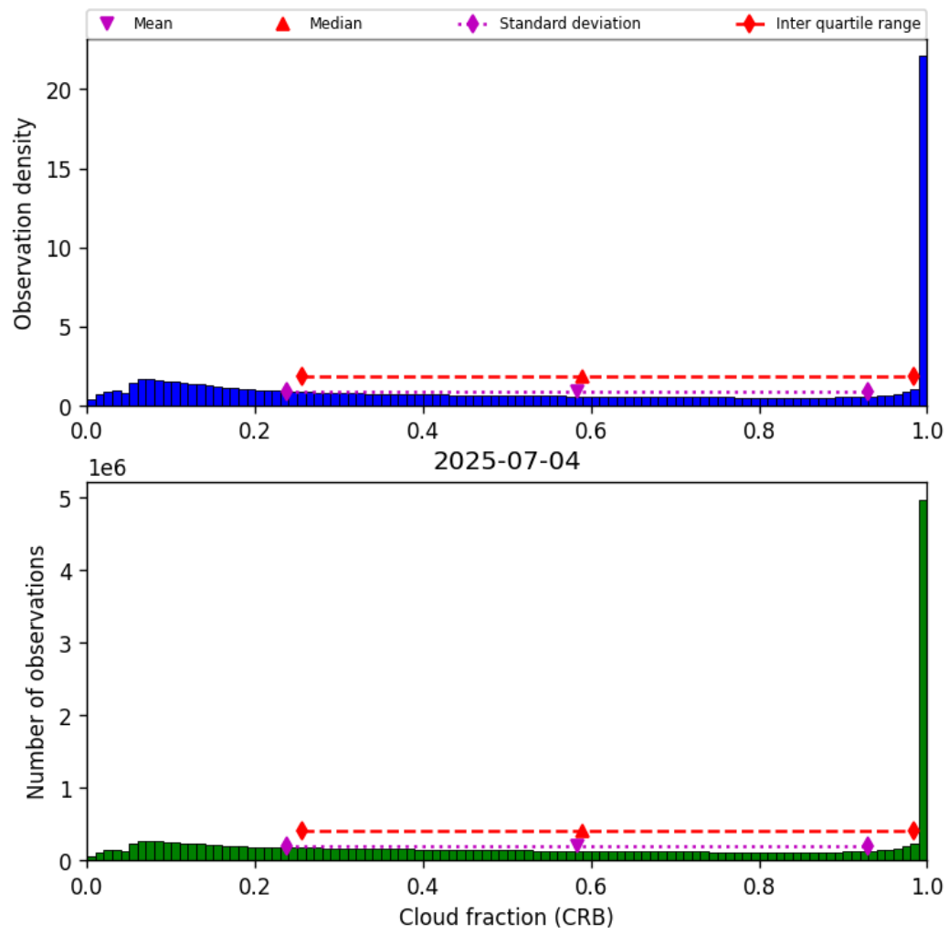
Figure 42: Histogram of “Cloud fraction (CRB)” for 2025-07-03 to 2025-07-05
