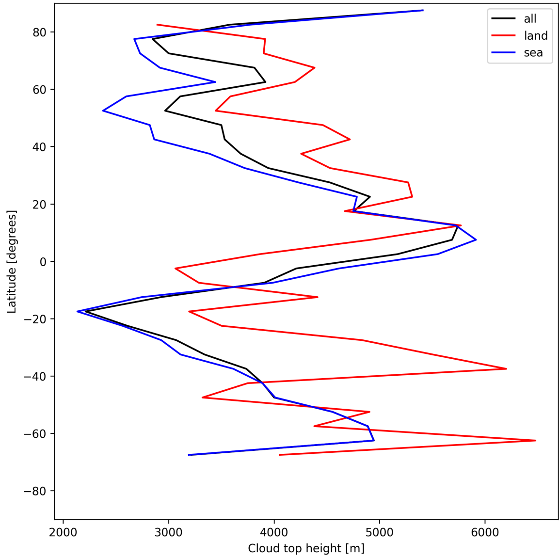
Figure 24: Zonal average of “Cloud top height” for 2025-07-03 to 2025-07-05.
