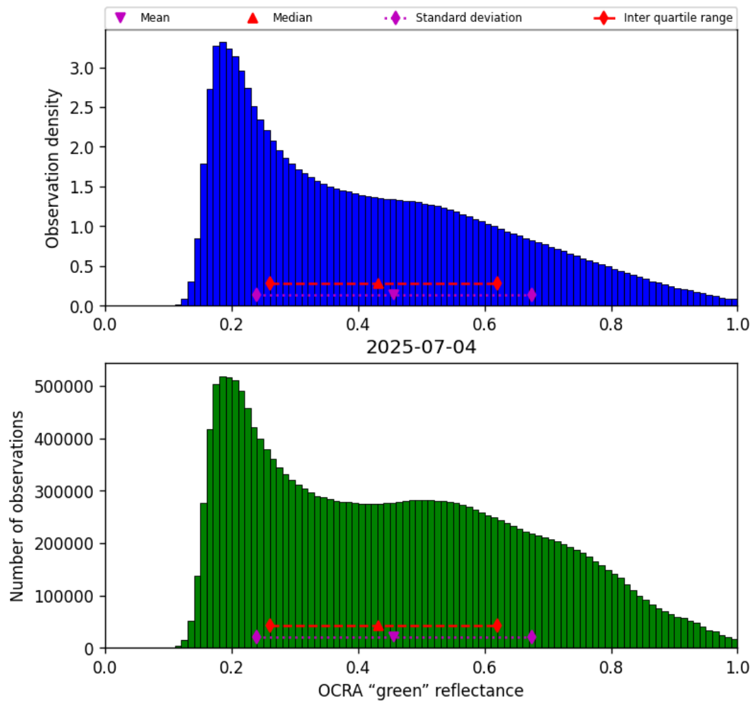
Figure 52: Histogram of “OCRA “green” reflectance” for 2025-07-03 to 2025-07-05
