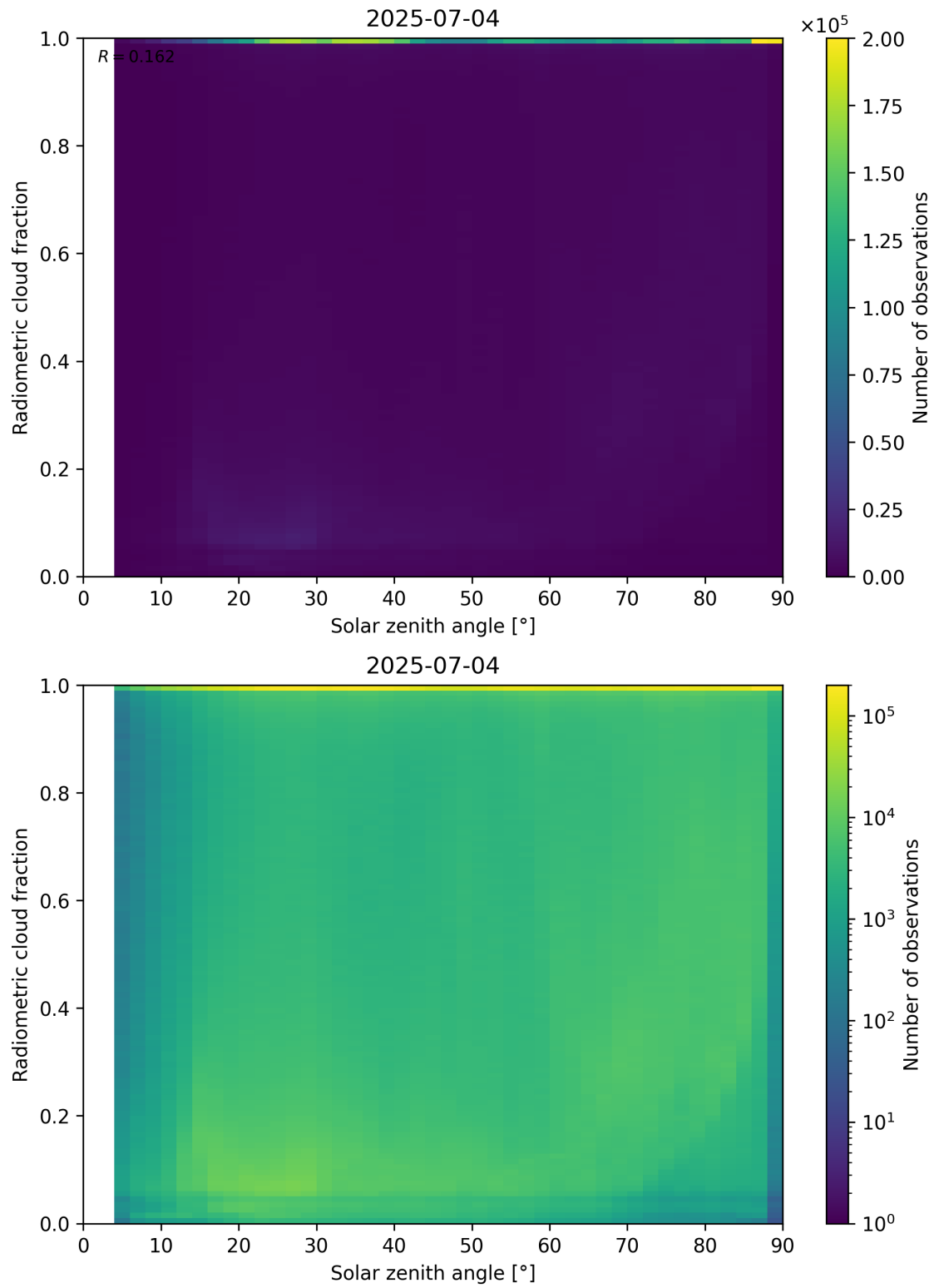
Figure 99: Scatter density plot of “Solar zenith angle” against “Radiometric cloud fraction” for 2025-07-03 to 2025-07-05.
