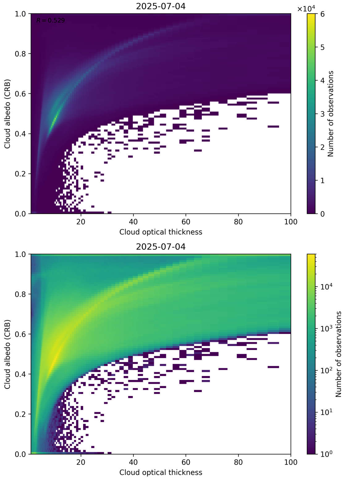
Figure 82: Scatter density plot of “Cloud optical thickness” against “Cloud albedo (CRB)” for 2025-07-03 to 2025-07-05.
