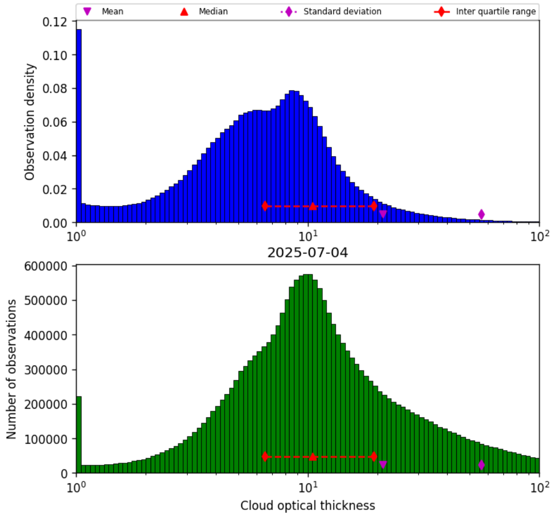
Figure 41: Histogram of “Cloud optical thickness” for 2025-07-03 to 2025-07-05
