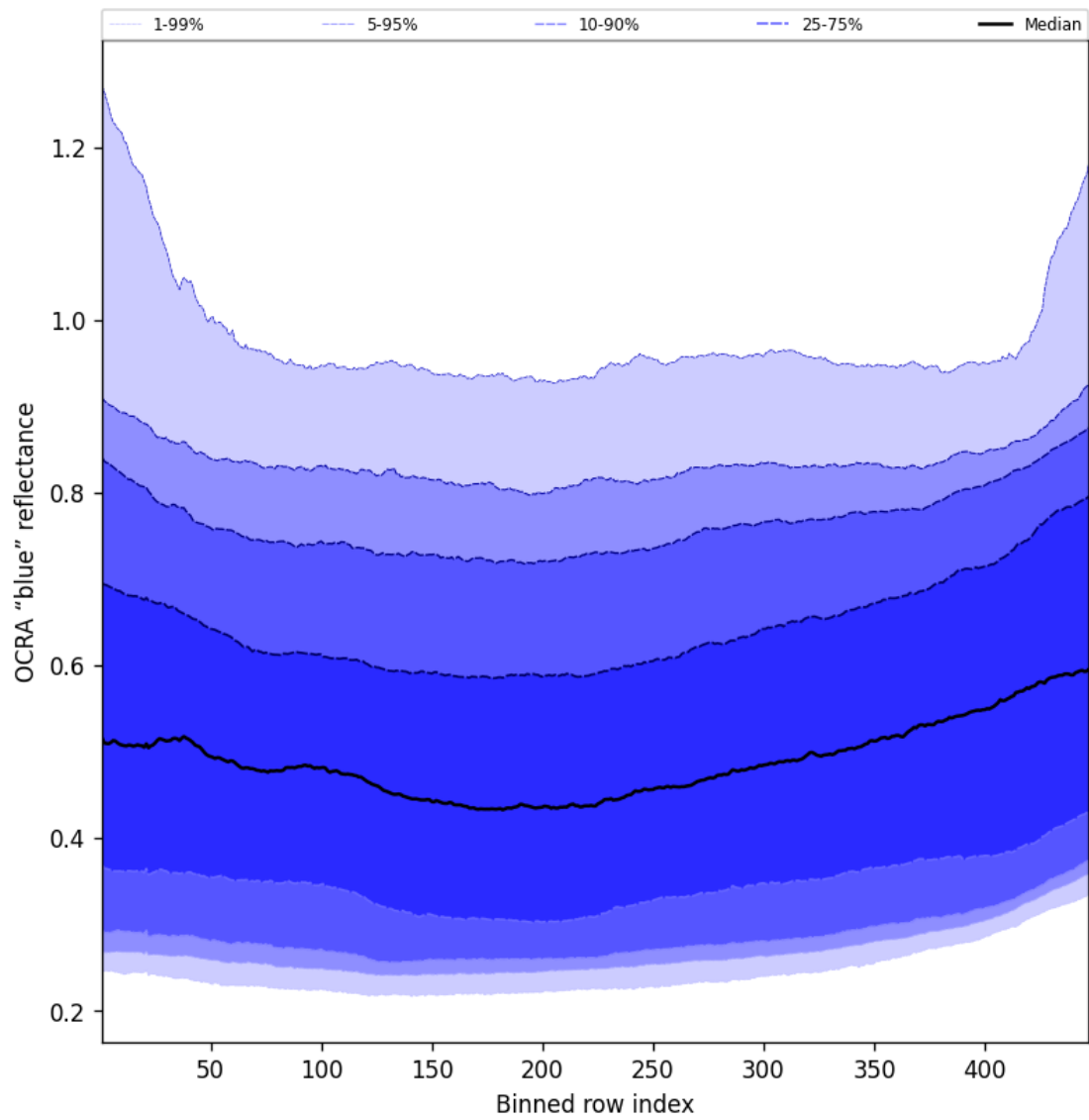
Figure 67: Along track statistics of “OCRA “blue” reflectance” for 2025-07-03 to 2025-07-05
