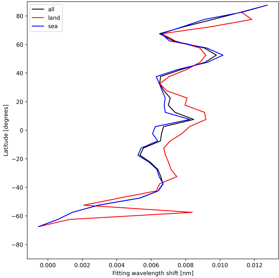
Figure 33: Zonal average of “Fitting wavelength shift” for 2025-07-03 to 2025-07-05.
