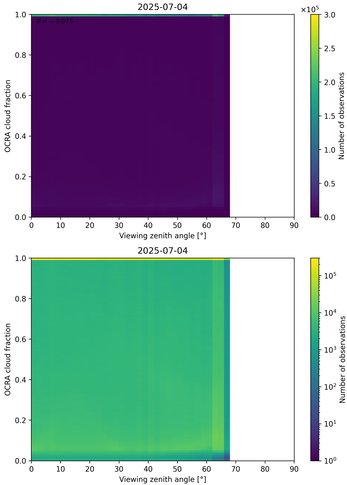
Figure 108: Scatter density plot of “Viewing zenith angle” against “OCRA cloud fraction” for 2025-07-03 to 2025-07-05.
