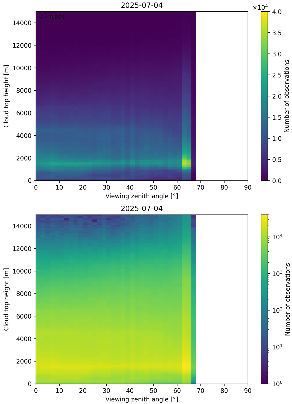
Figure 112: Scatter density plot of “Viewing zenith angle” against “Cloud top height” for 2025-07-03 to 2025-07-05.
