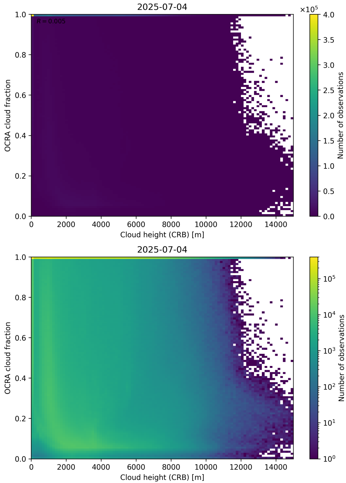
Figure 81: Scatter density plot of “Cloud height (CRB)” against “OCRA cloud fraction” for 2025-07-03 to 2025-07-05.
