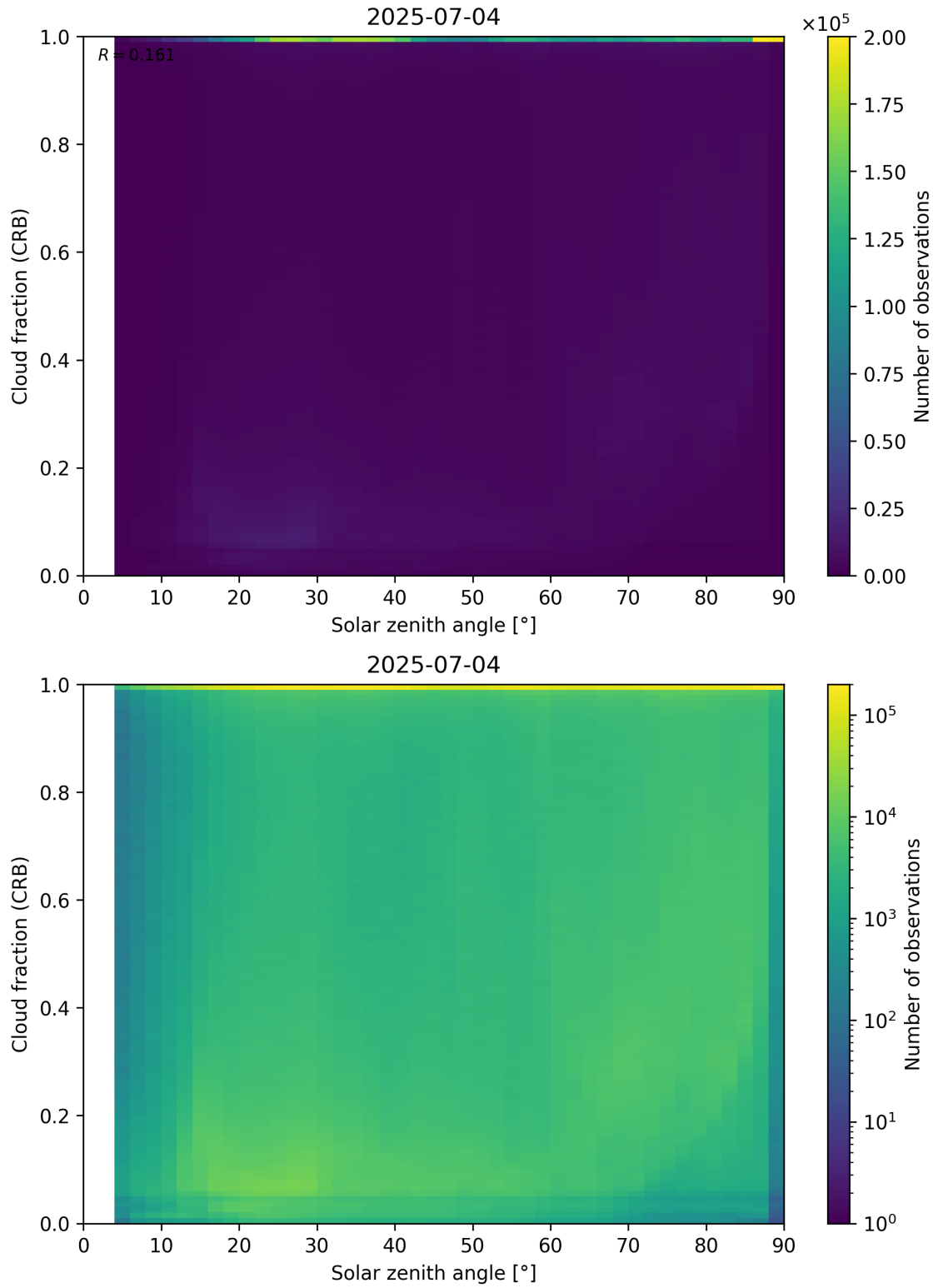
Figure 101: Scatter density plot of “Solar zenith angle” against “Cloud fraction (CRB)” for 2025-07-03 to 2025-07-05.
