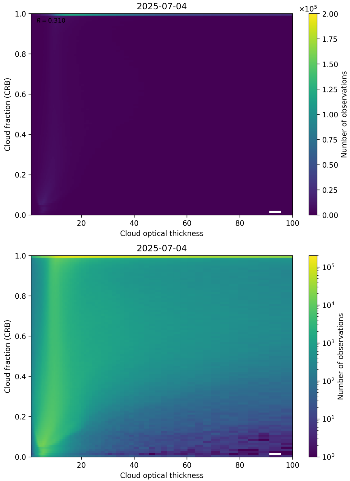
Figure 84: Scatter density plot of “Cloud optical thickness” against “Cloud fraction (CRB)” for 2025-07-03 to 2025-07-05.
