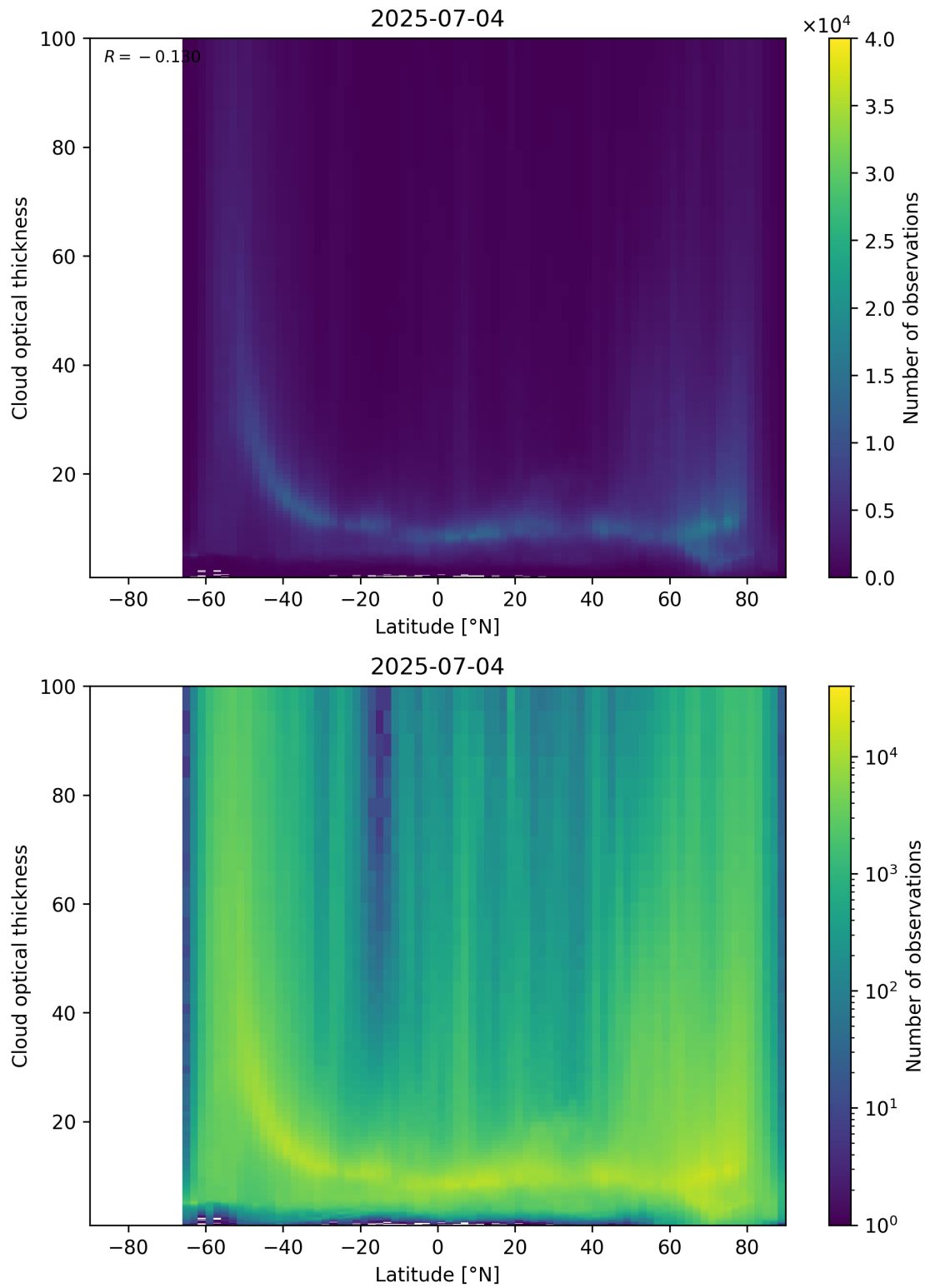
Figure 96: Scatter density plot of “Latitude” against “Cloud optical thickness” for 2025-07-03 to 2025-07-05.
