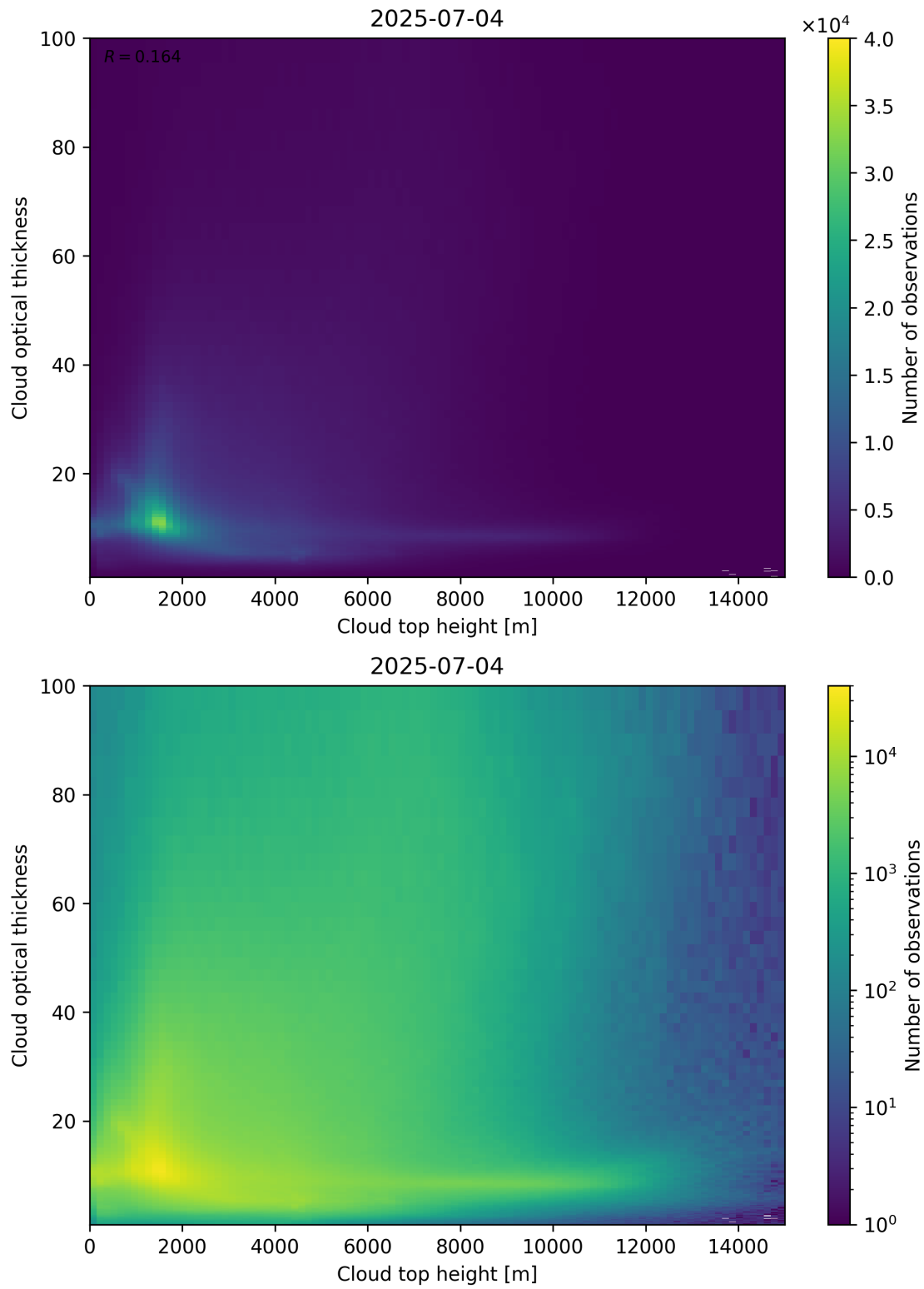
Figure 90: Scatter density plot of “Cloud top height” against “Cloud optical thickness” for 2025-07-03 to 2025-07-05.
