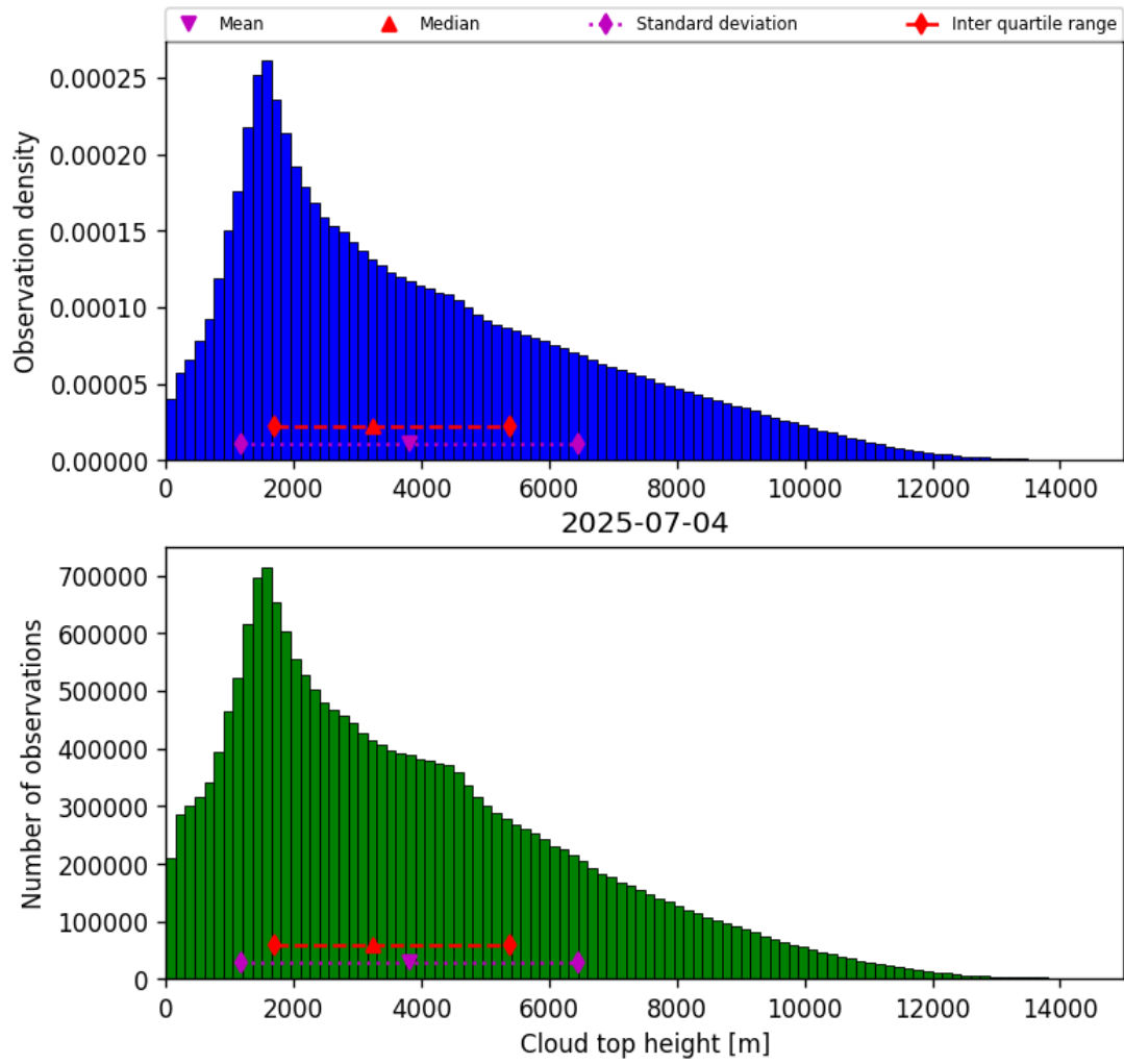
Figure 40: Histogram of “Cloud top height” for 2025-07-03 to 2025-07-05
