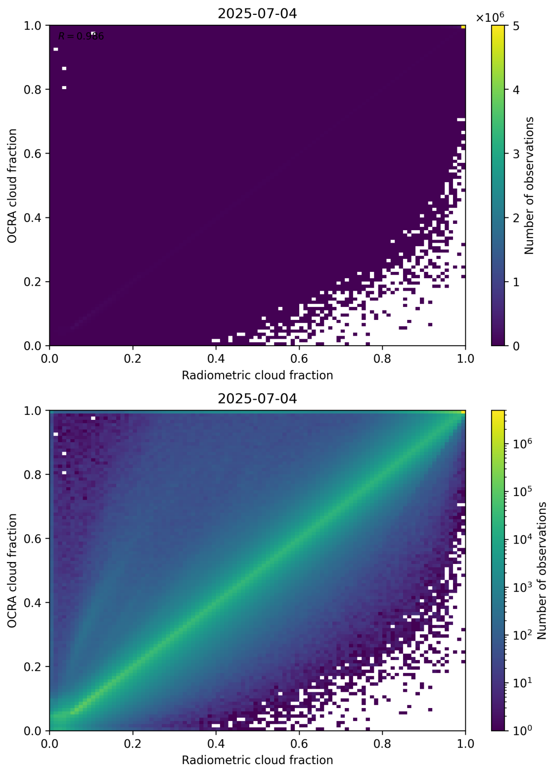
Figure 72: Scatter density plot of “Radiometric cloud fraction” against “OCRA cloud fraction” for 2025-07-03 to 2025-07-05.
