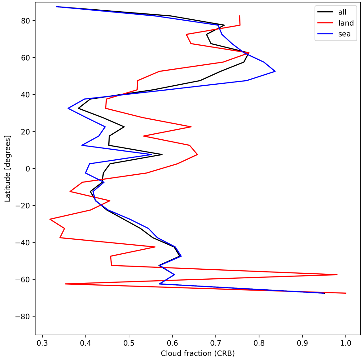
Figure 26: Zonal average of “Cloud fraction (CRB)” for 2025-07-03 to 2025-07-05.
