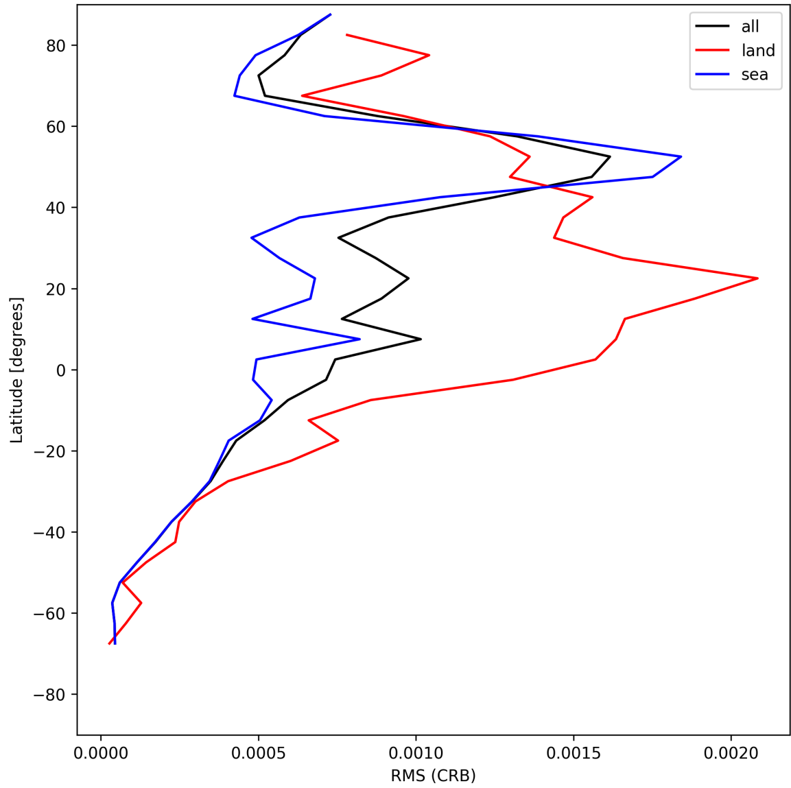
Figure 32: Zonal average of “RMS (CRB)” for 2025-07-03 to 2025-07-05.
