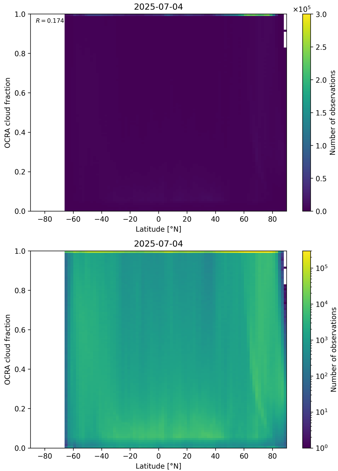
Figure 93: Scatter density plot of “Latitude” against “OCRA cloud fraction” for 2025-07-03 to 2025-07-05.
