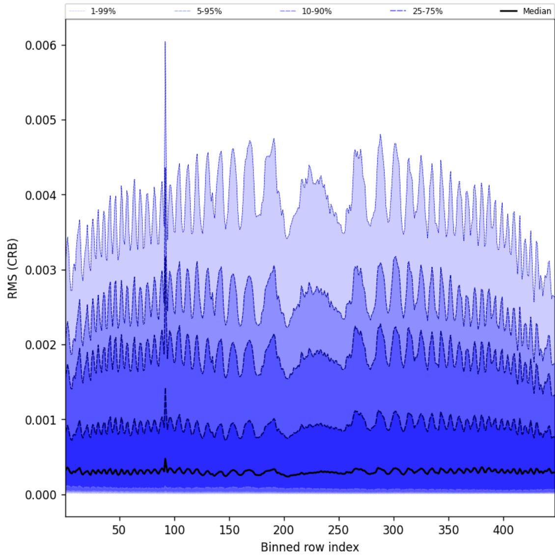
Figure 64: Along track statistics of “RMS (CRB)” for 2025-07-03 to 2025-07-05
