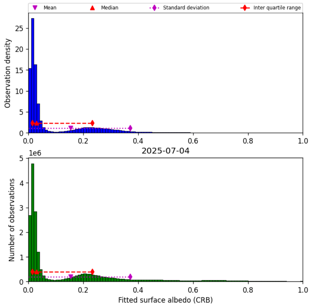
Figure 46: Histogram of “Fitted surface albedo (CRB)” for 2025-07-03 to 2025-07-05
