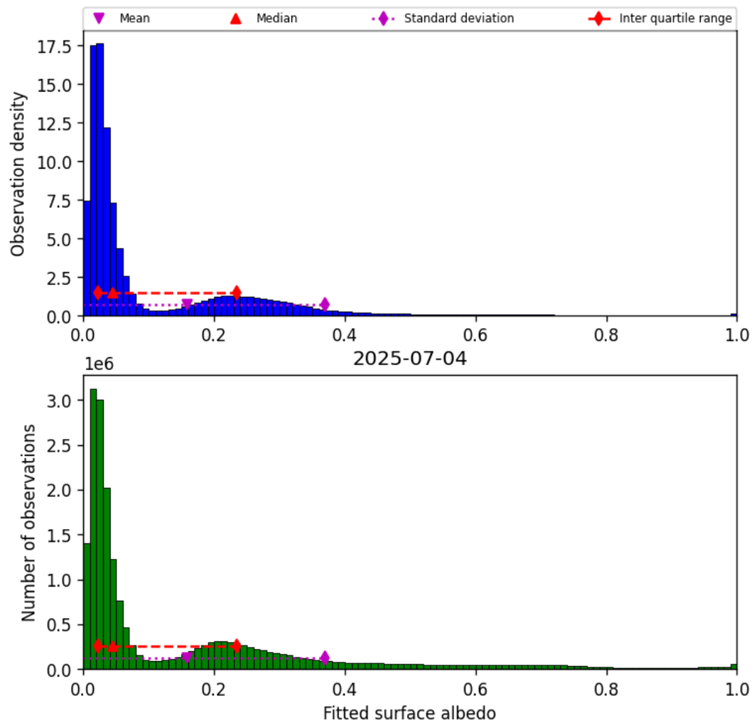
Figure 45: Histogram of “Fitted surface albedo” for 2025-07-03 to 2025-07-05
