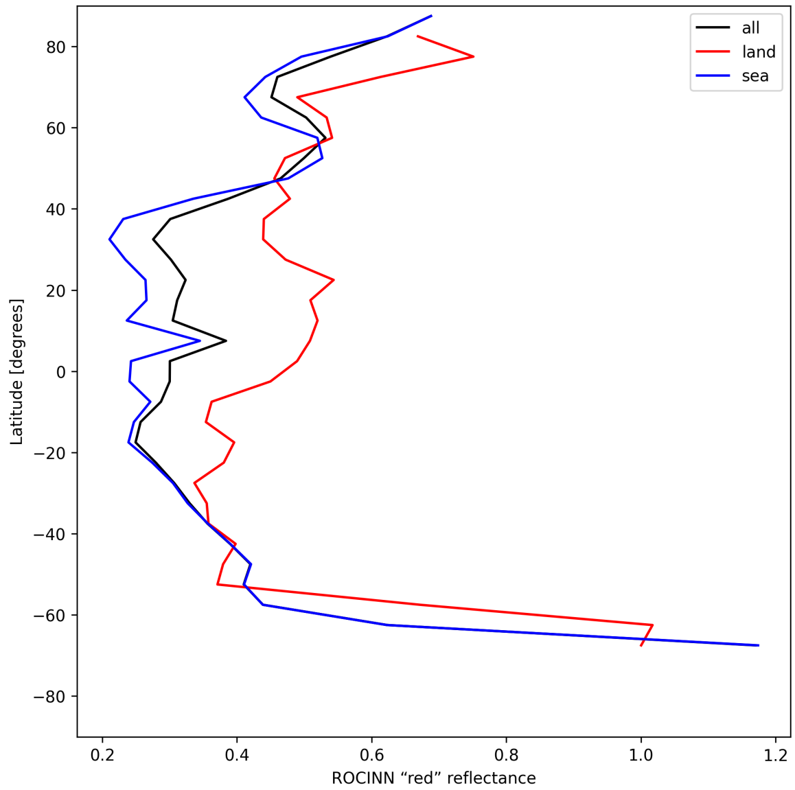
Figure 37: Zonal average of “ROCINN “red” reflectance” for 2025-07-03 to 2025-07-05.
