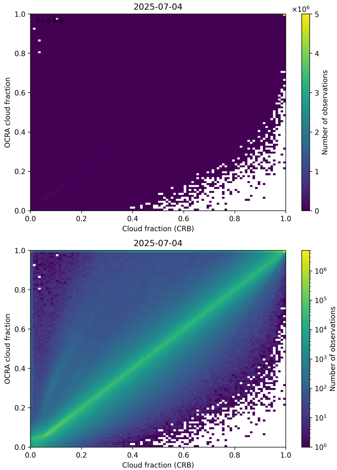
Figure 78: Scatter density plot of “Cloud fraction (CRB)” against “OCRA cloud fraction” for 2025-07-03 to 2025-07-05.
