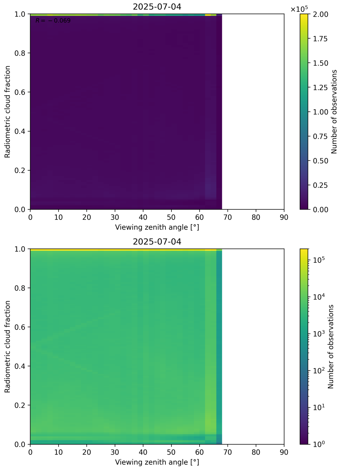
Figure 107: Scatter density plot of “Viewing zenith angle” against “Radiometric cloud fraction” for 2025-07-03 to 2025-07-05.
