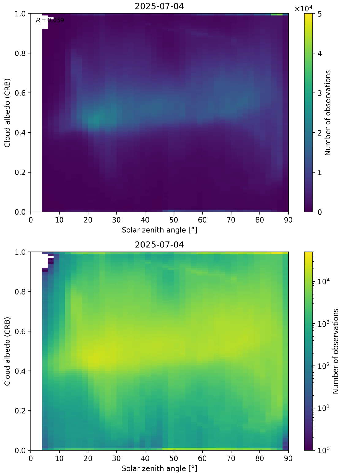
Figure 98: Scatter density plot of “Solar zenith angle” against “Cloud albedo (CRB)” for 2025-07-03 to 2025-07-05.
