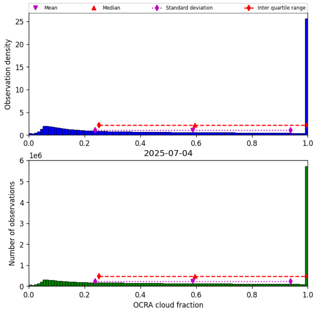
Figure 50: Histogram of “OCRA cloud fraction” for 2025-07-03 to 2025-07-05
