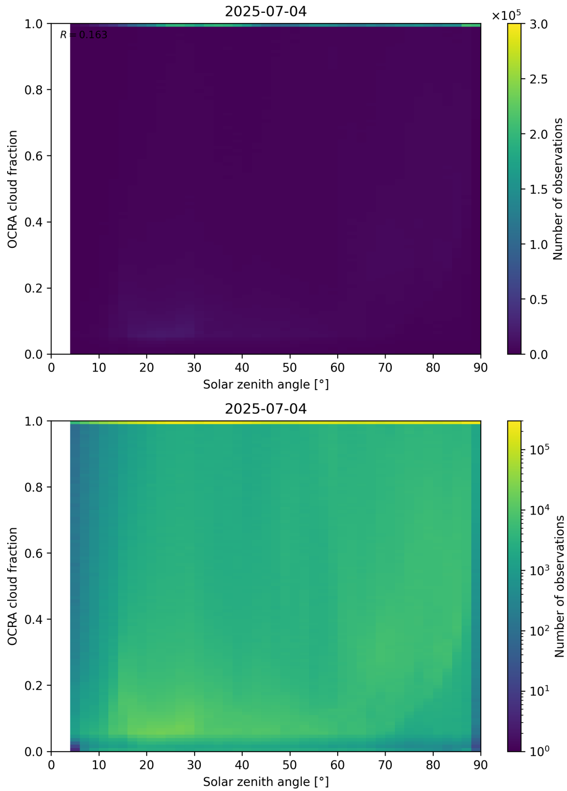
Figure 100: Scatter density plot of “Solar zenith angle” against “OCRA cloud fraction” for 2025-07-03 to 2025-07-05.
