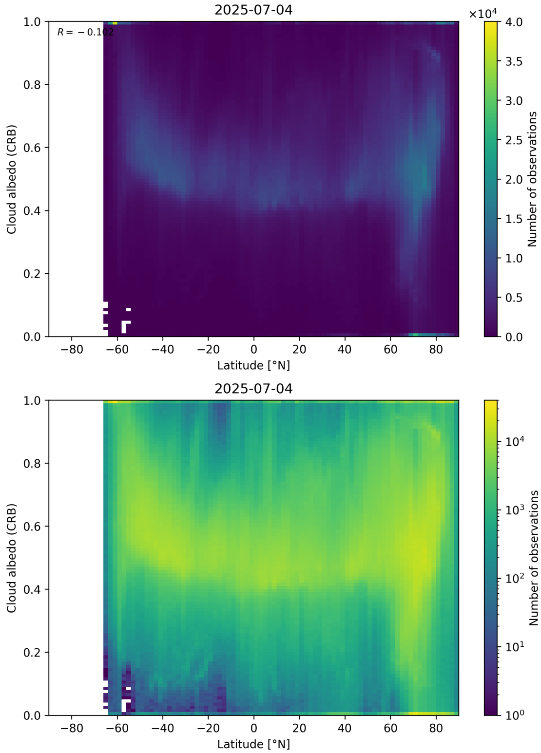
Figure 91: Scatter density plot of “Latitude” against “Cloud albedo (CRB)” for 2025-07-03 to 2025-07-05.
