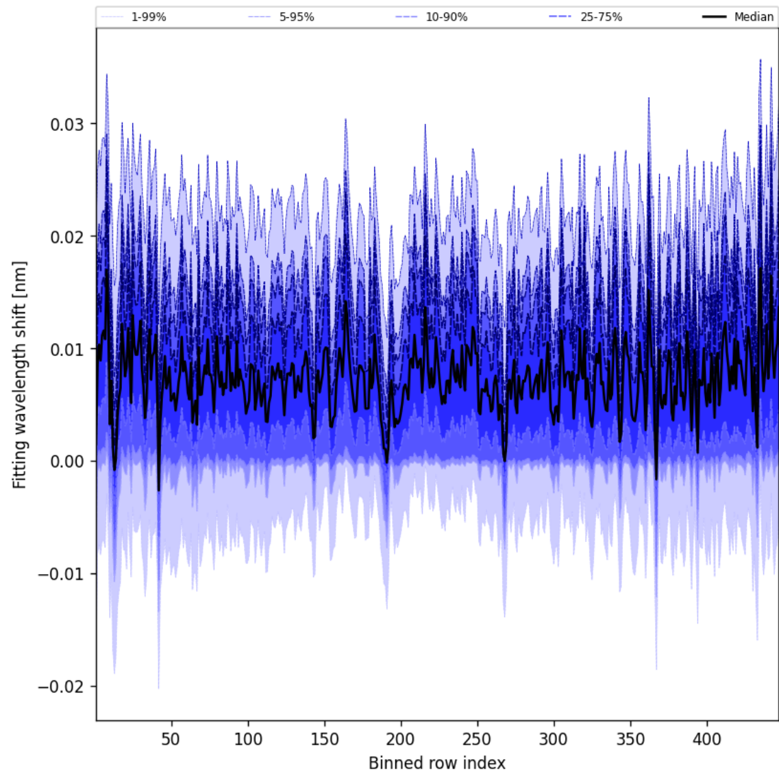
Figure 65: Along track statistics of “Fitting wavelength shift” for 2025-07-03 to 2025-07-05
