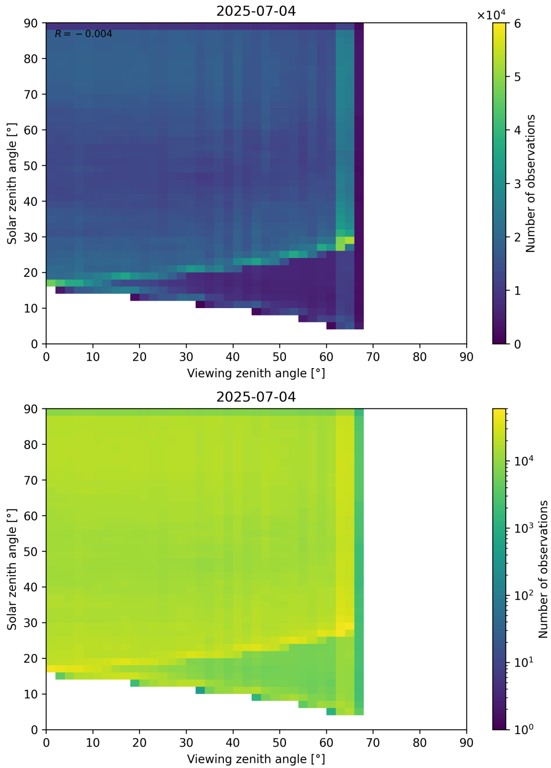
Figure 114: Scatter density plot of “Viewing zenith angle” against “Solar zenith angle” for 2025-07-03 to 2025-07-05.
