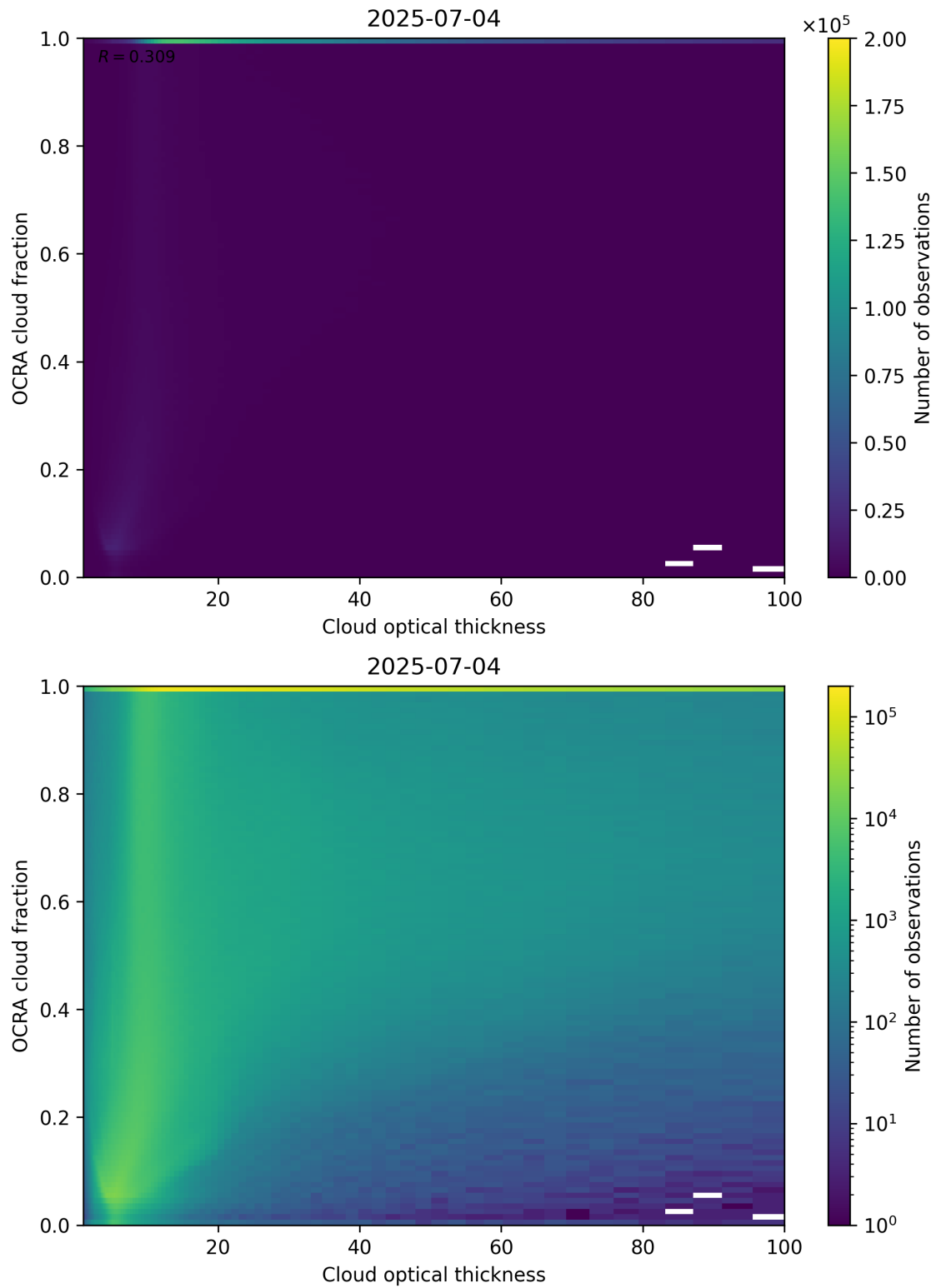
Figure 83: Scatter density plot of “Cloud optical thickness” against “OCRA cloud fraction” for 2025-07-03 to 2025-07-05.
