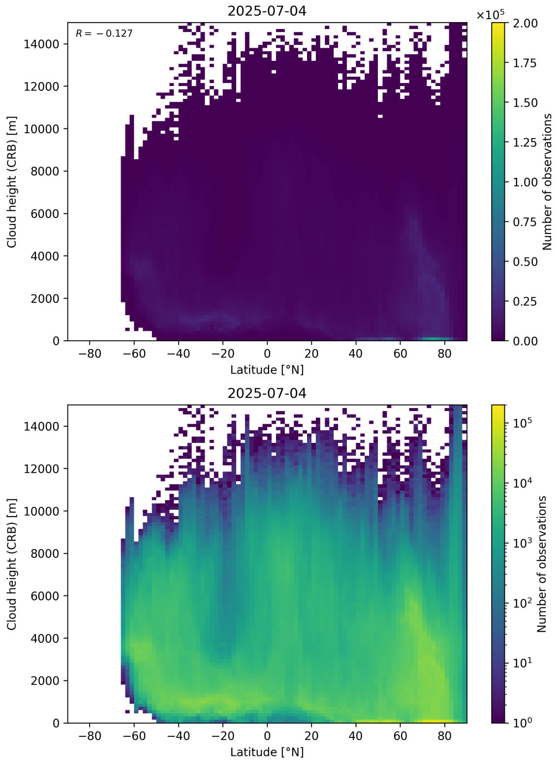
Figure 95: Scatter density plot of “Latitude” against “Cloud height (CRB)” for 2025-07-03 to 2025-07-05.
