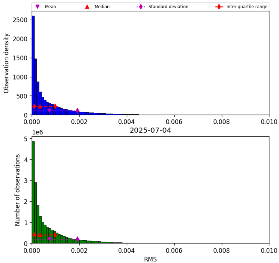
Figure 47: Histogram of “RMS” for 2025-07-03 to 2025-07-05
