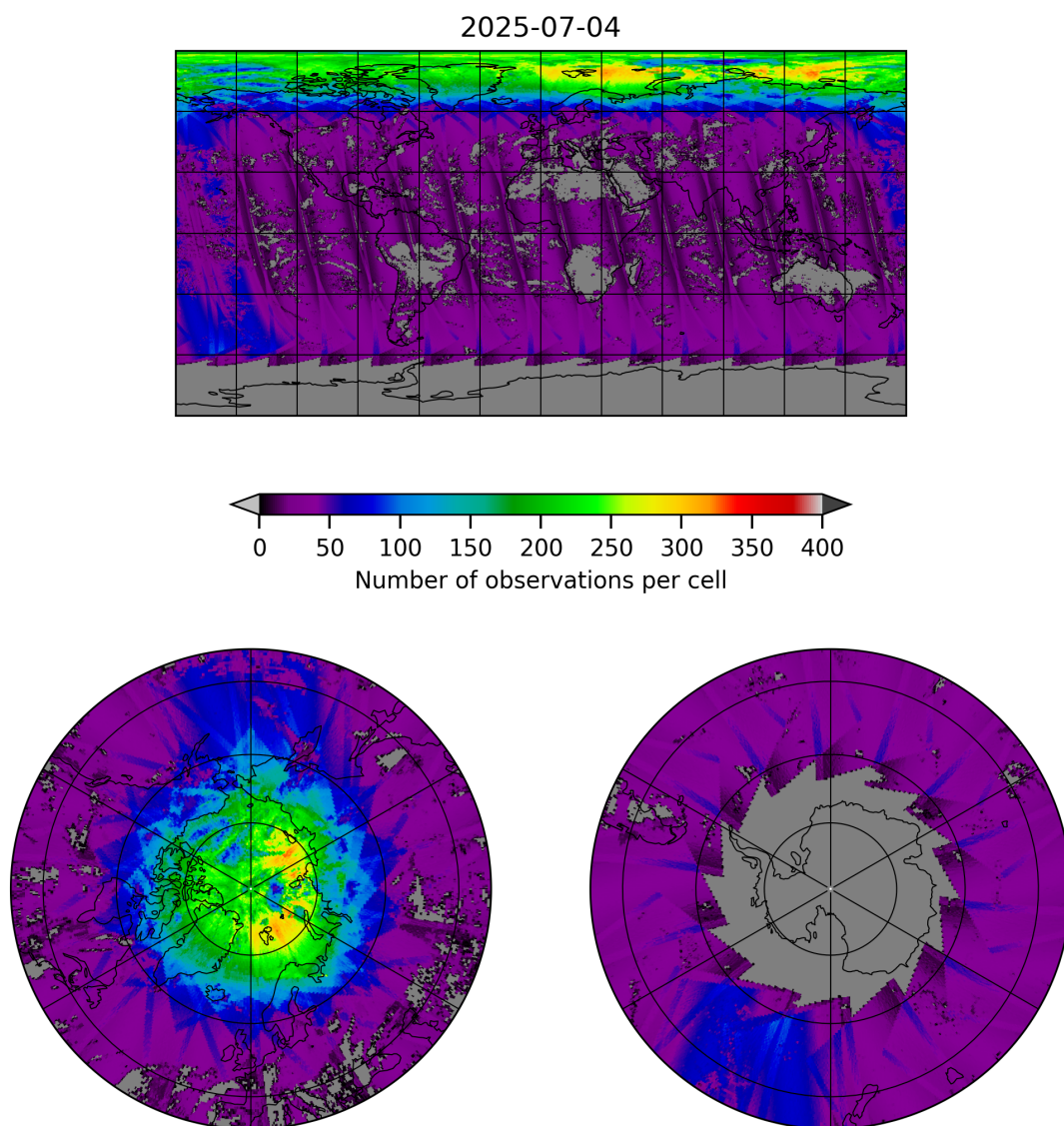
Figure 21: Map of the number of observations for 2025-07-03 to 2025-07-05
