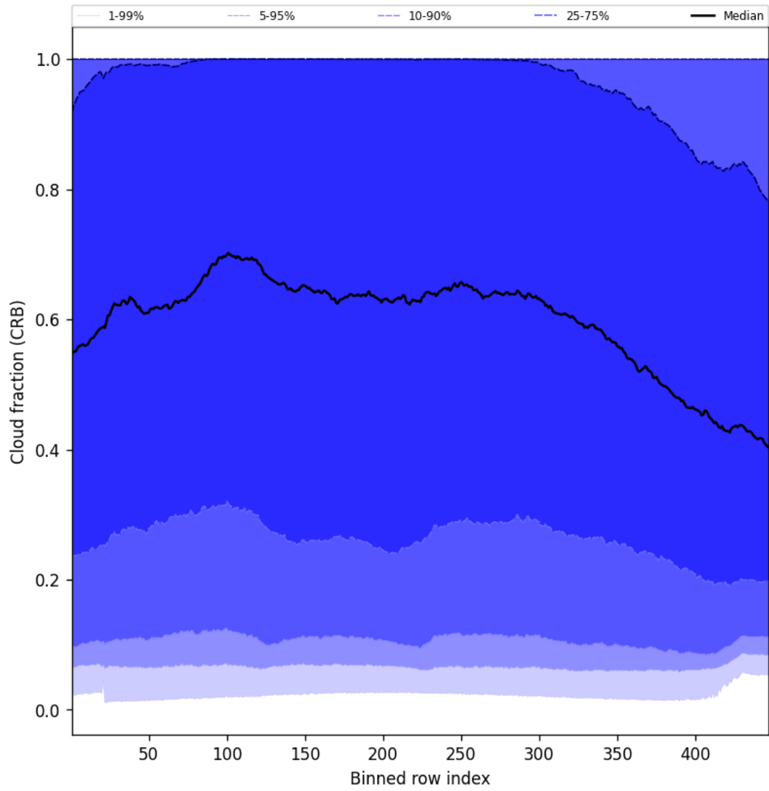
Figure 58: Along track statistics of “Cloud fraction (CRB)” for 2025-07-03 to 2025-07-05
