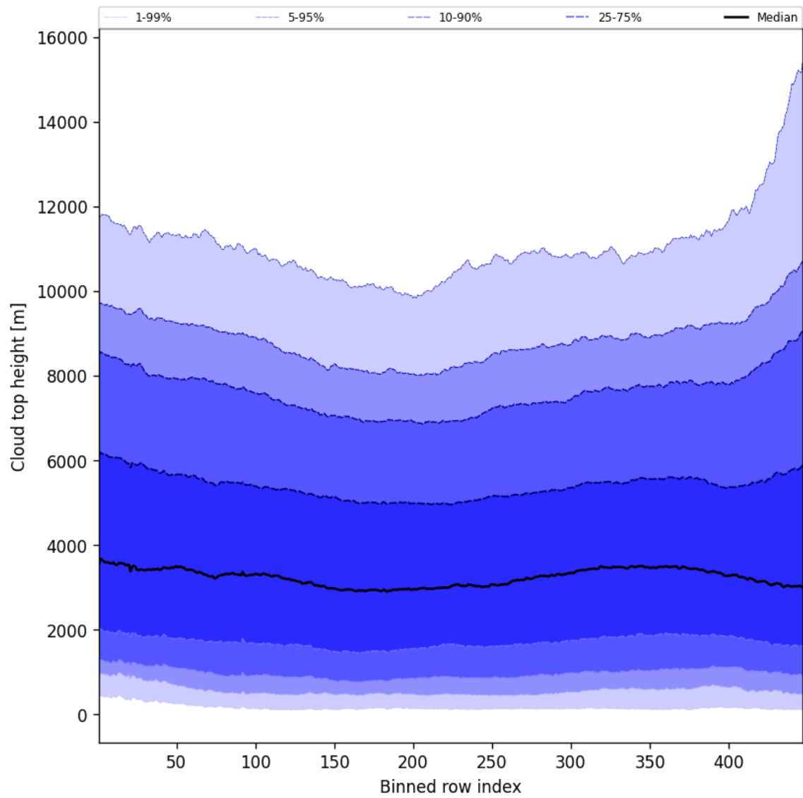
Figure 56: Along track statistics of “Cloud top height” for 2025-07-03 to 2025-07-05
