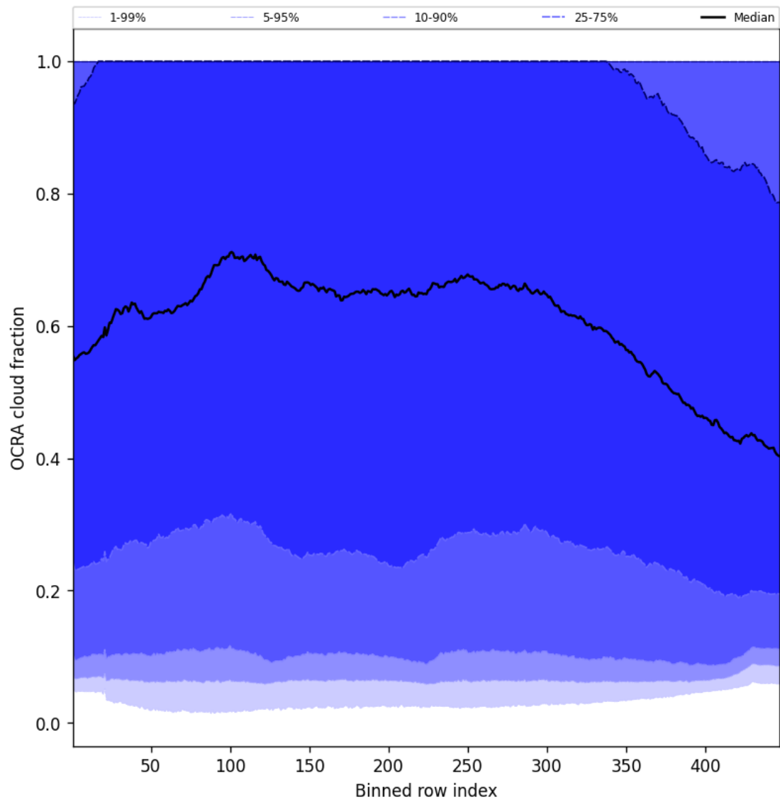
Figure 66: Along track statistics of “OCRA cloud fraction” for 2025-07-03 to 2025-07-05
