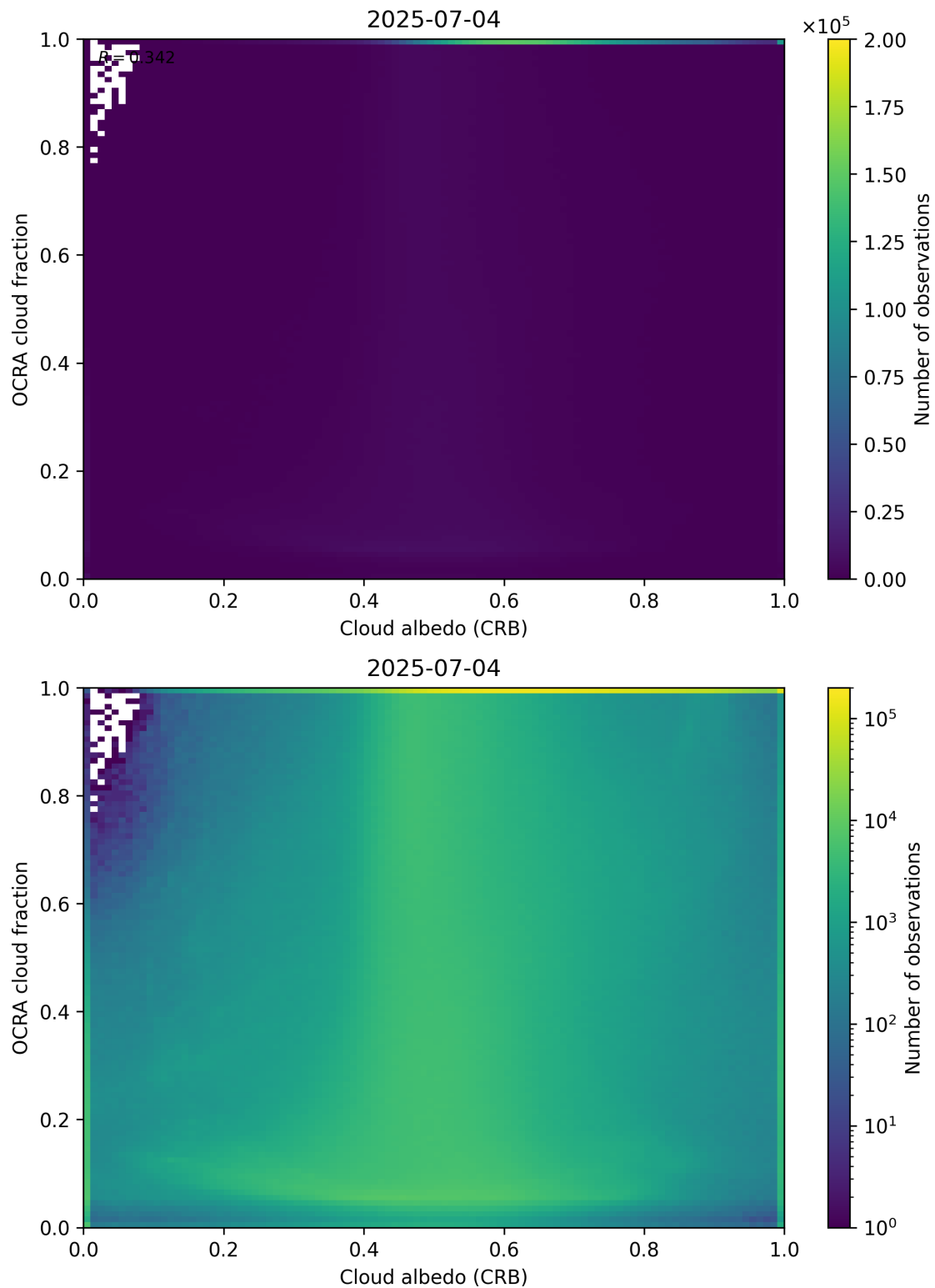
Figure 70: Scatter density plot of “Cloud albedo (CRB)” against “OCRA cloud fraction” for 2025-07-03 to 2025-07-05.
