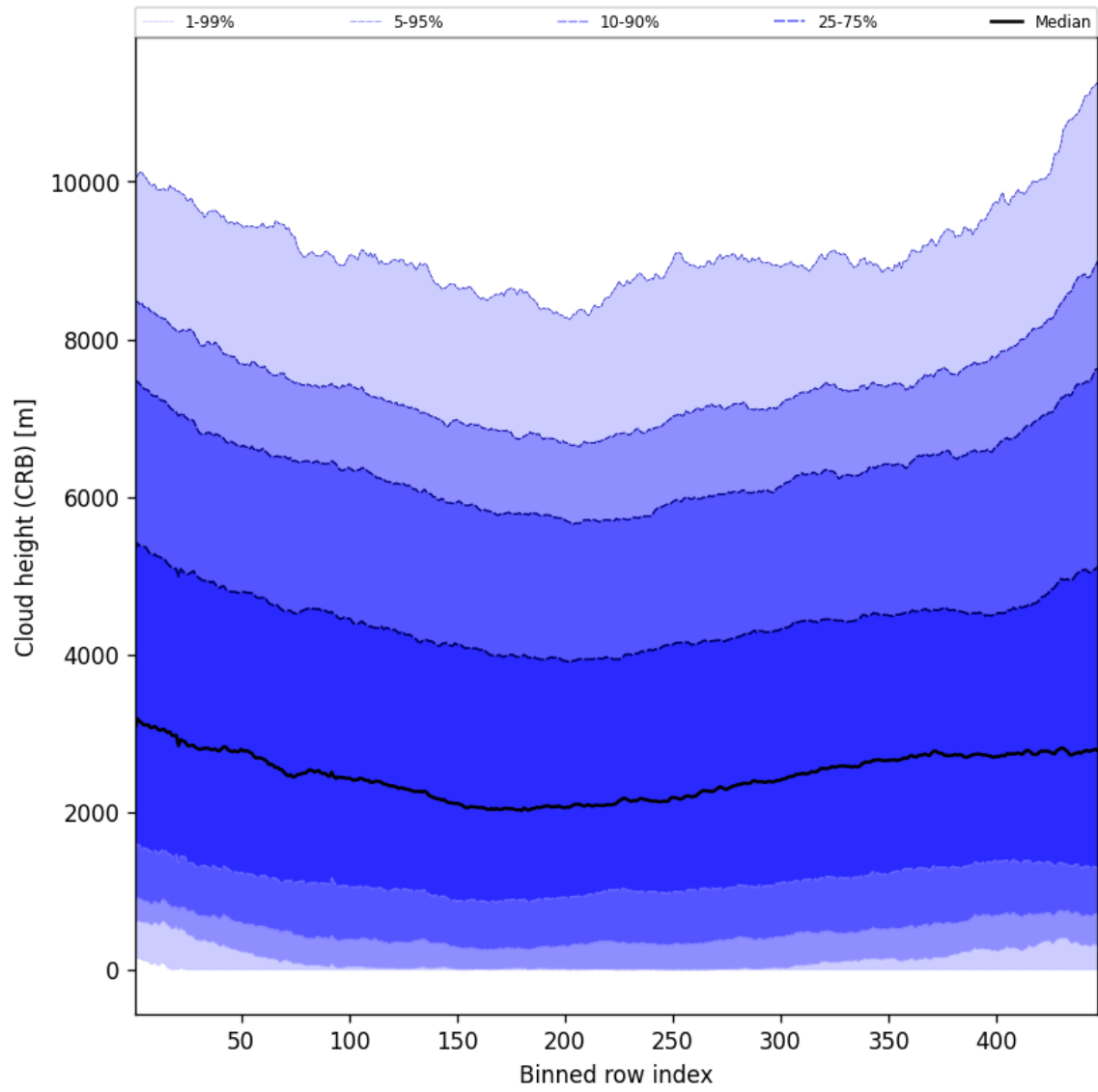
Figure 59: Along track statistics of “Cloud height (CRB)” for 2025-07-03 to 2025-07-05
