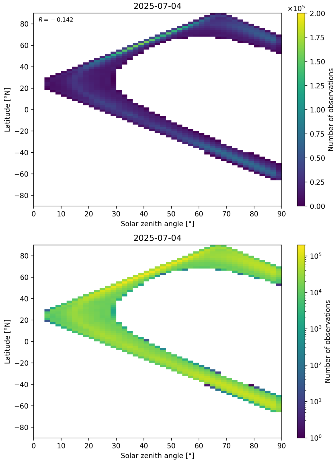
Figure 105: Scatter density plot of “Solar zenith angle” against “Latitude” for 2025-07-03 to 2025-07-05.
