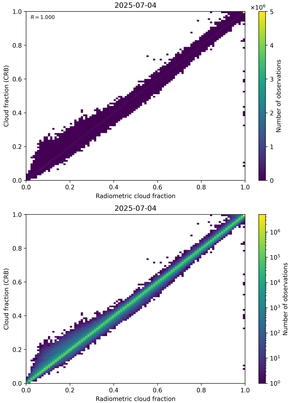
Figure 73: Scatter density plot of “Radiometric cloud fraction” against “Cloud fraction (CRB)” for 2025-07-03 to 2025-07-05.
