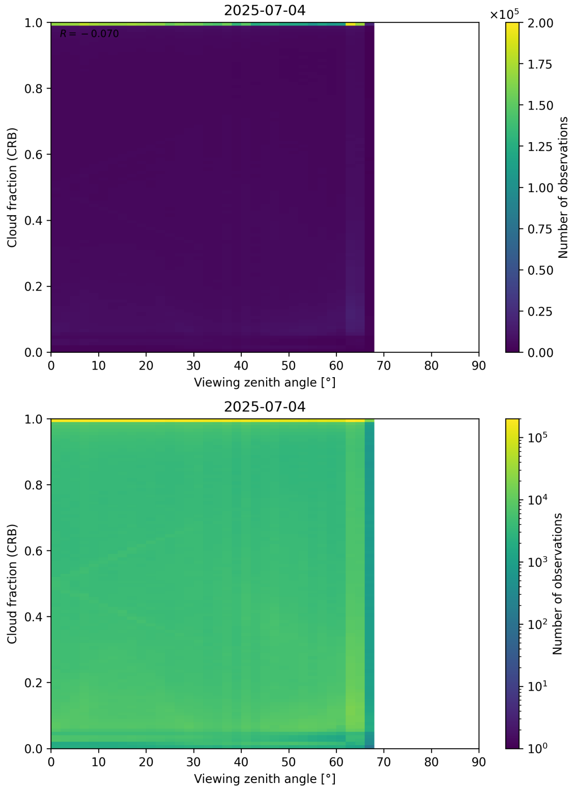
Figure 109: Scatter density plot of “Viewing zenith angle” against “Cloud fraction (CRB)” for 2025-07-03 to 2025-07-05.
