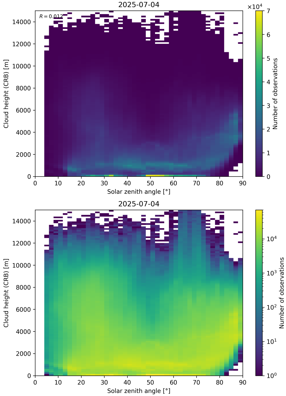
Figure 102: Scatter density plot of “Solar zenith angle” against “Cloud height (CRB)” for 2025-07-03 to 2025-07-05.
