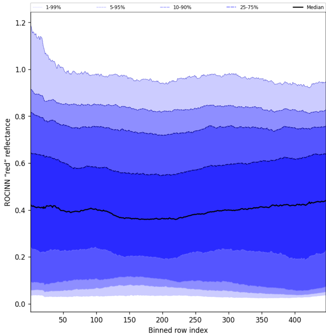
Figure 69: Along track statistics of "ROCINN "red" reflectance" for 2025-07-03 to 2025-07-05
