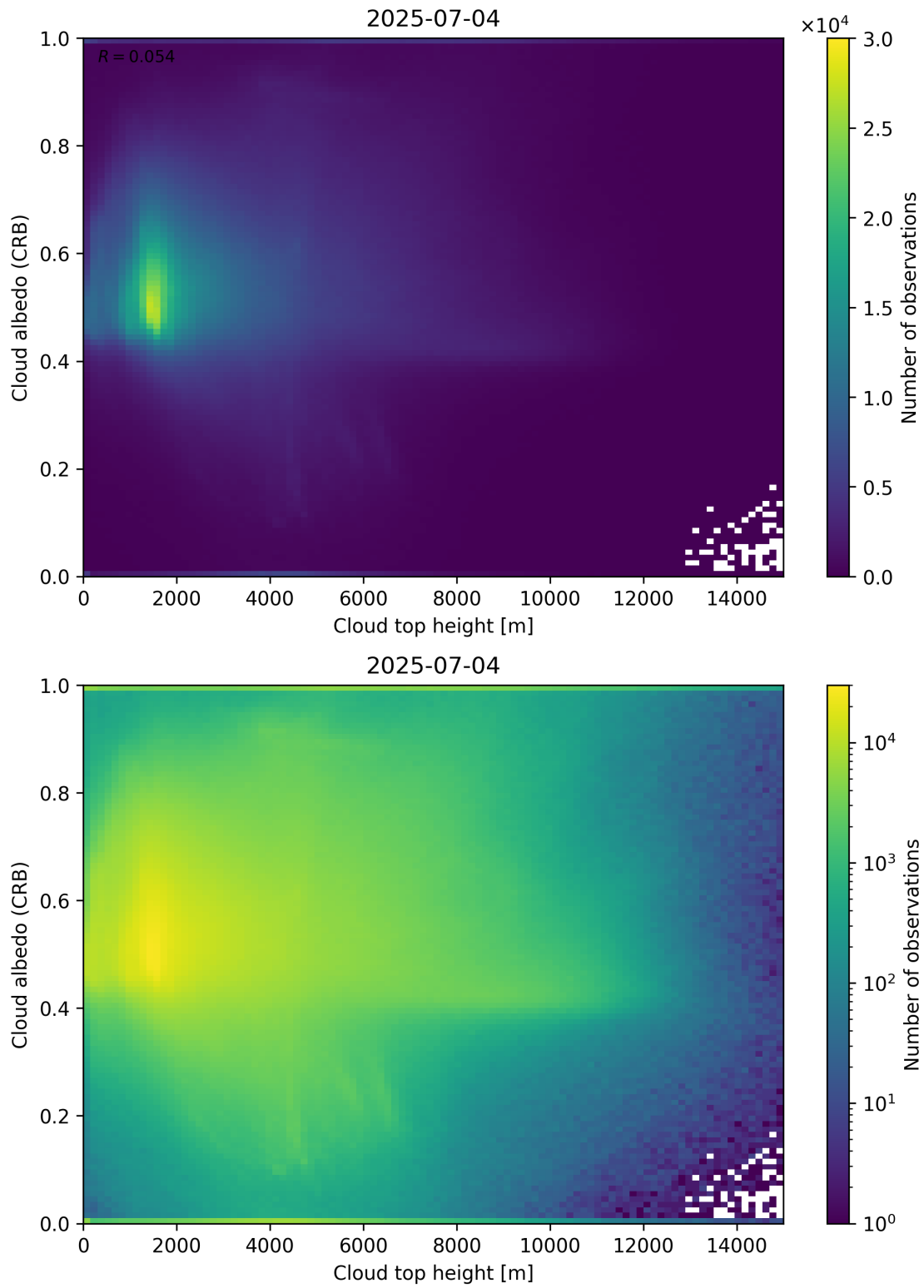
Figure 86: Scatter density plot of “Cloud top height” against “Cloud albedo (CRB)” for 2025-07-03 to 2025-07-05.
