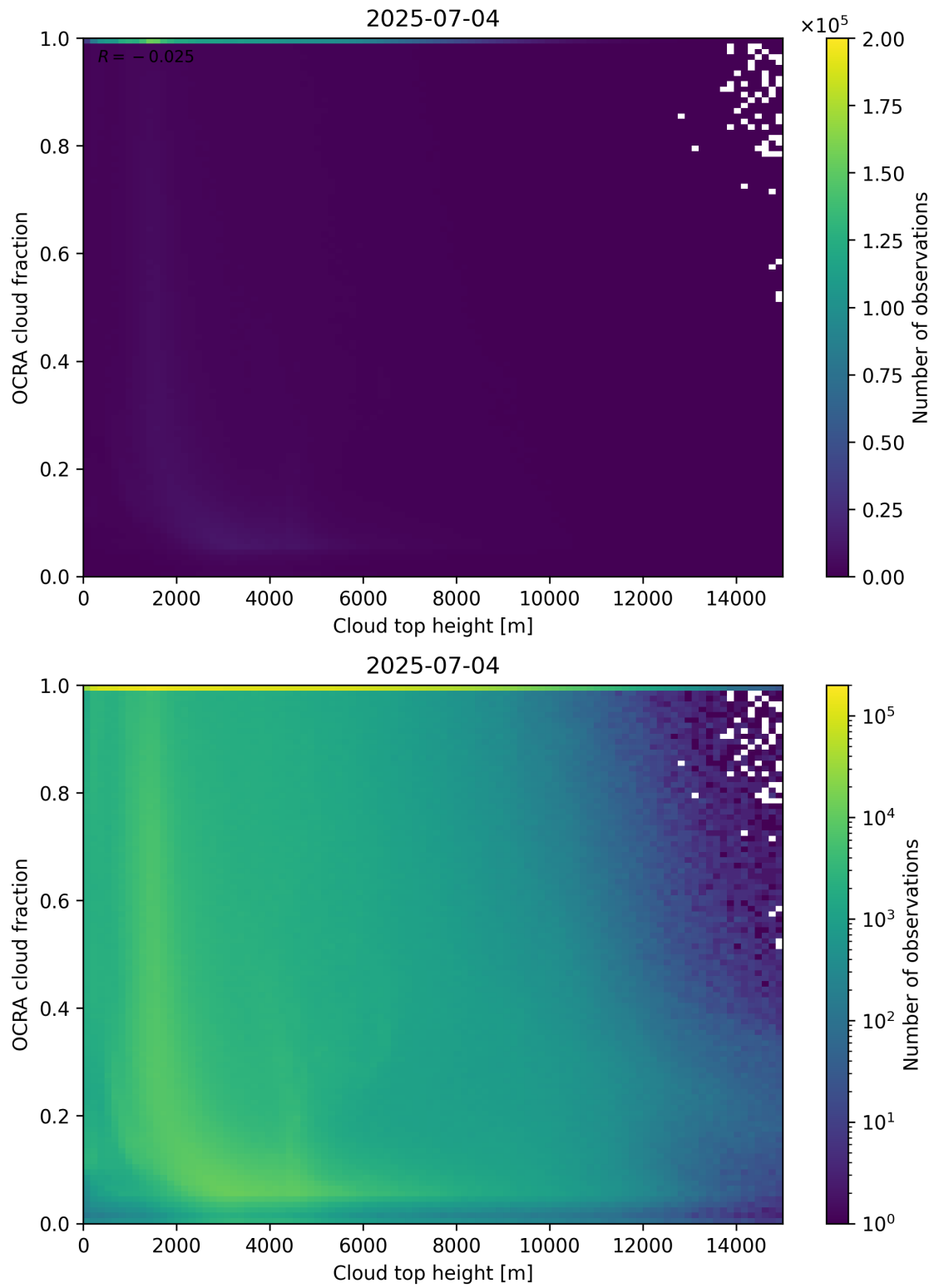
Figure 87: Scatter density plot of “Cloud top height” against “OCRA cloud fraction” for 2025-07-03 to 2025-07-05.
