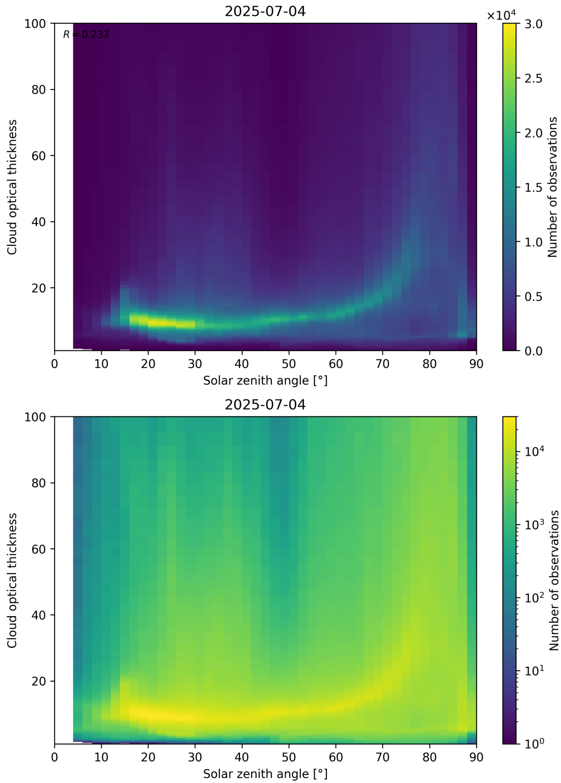
Figure 103: Scatter density plot of “Solar zenith angle” against “Cloud optical thickness” for 2025-07-03 to 2025-07-05.
