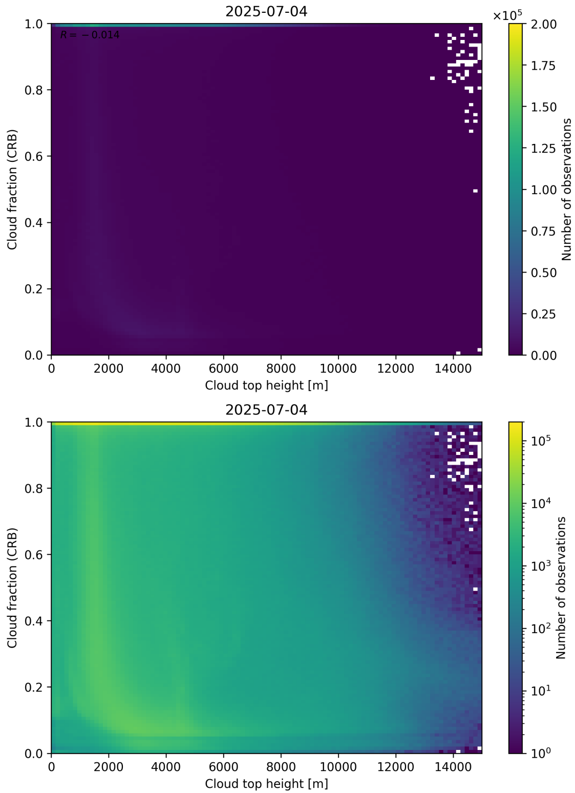
Figure 88: Scatter density plot of “Cloud top height” against “Cloud fraction (CRB)” for 2025-07-03 to 2025-07-05.
