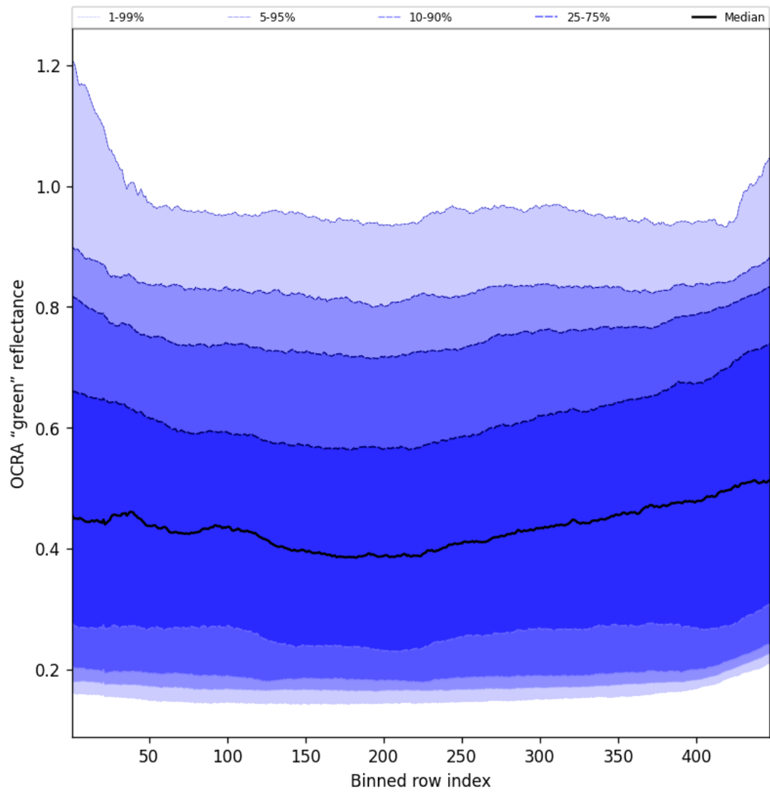
Figure 68: Along track statistics of “OCRA “green” reflectance” for 2025-07-03 to 2025-07-05
