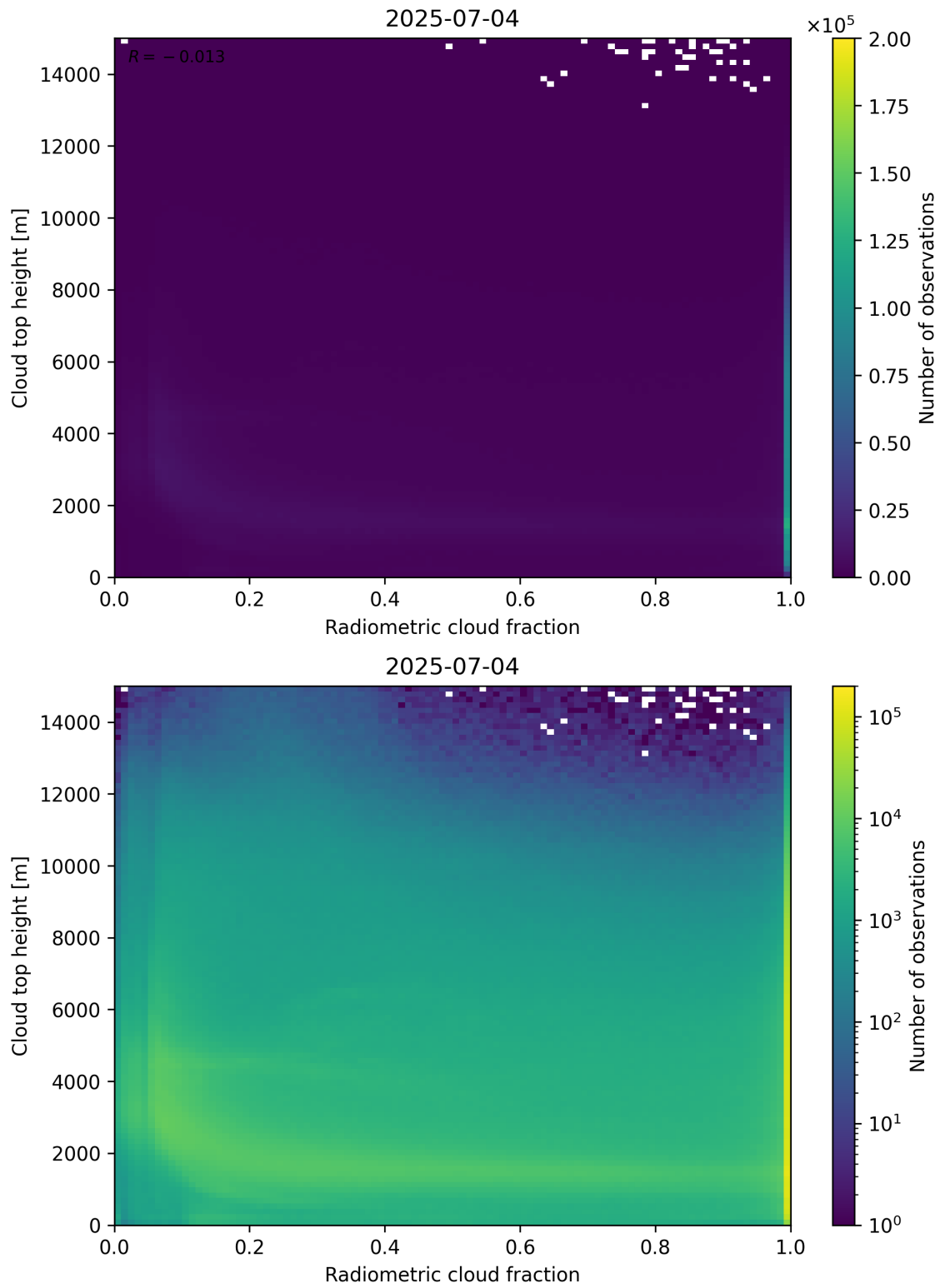
Figure 76: Scatter density plot of “Radiometric cloud fraction” against “Cloud top height” for 2025-07-03 to 2025-07-05.
