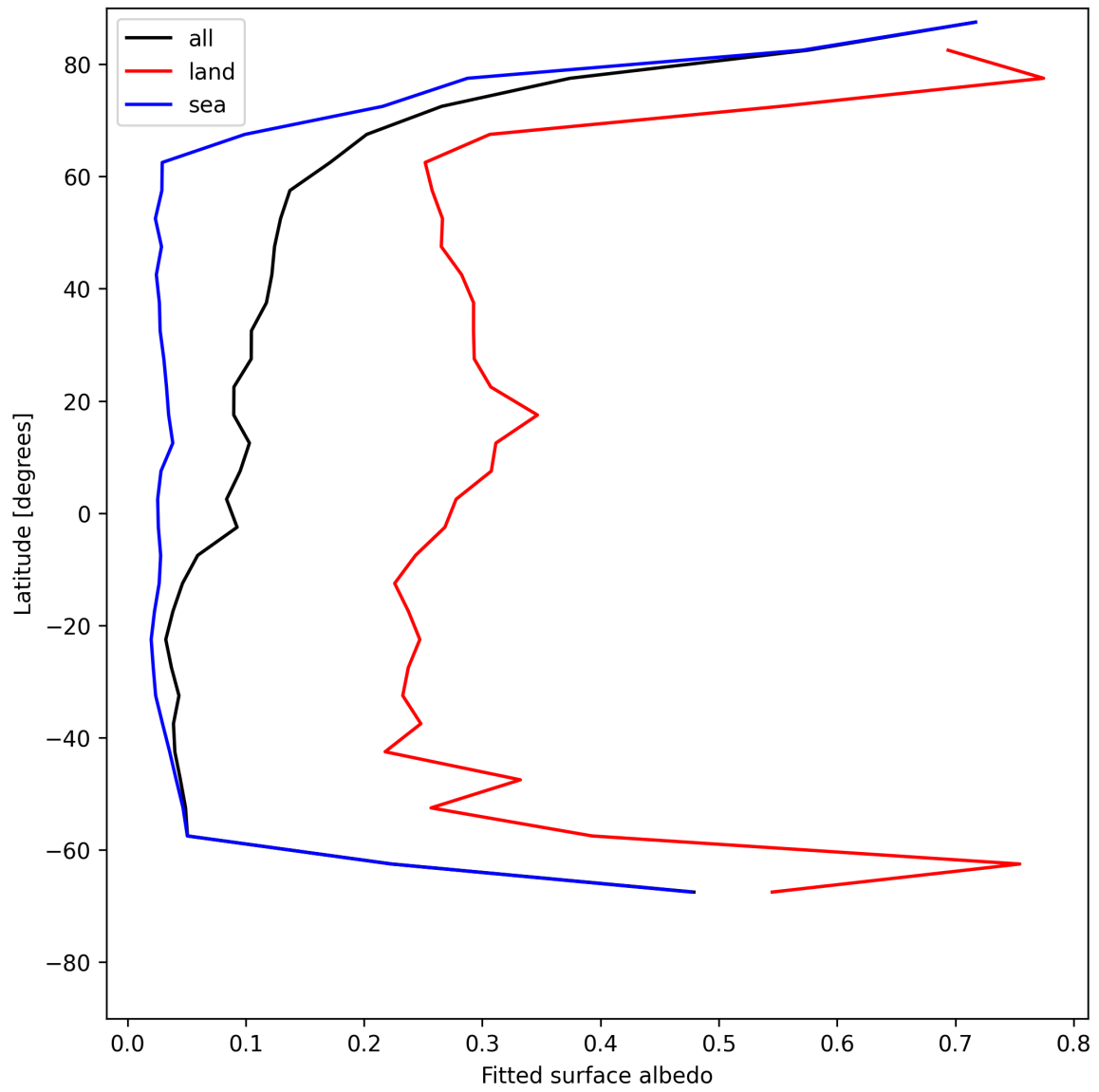
Figure 29: Zonal average of “Fitted surface albedo” for 2025-07-03 to 2025-07-05.
