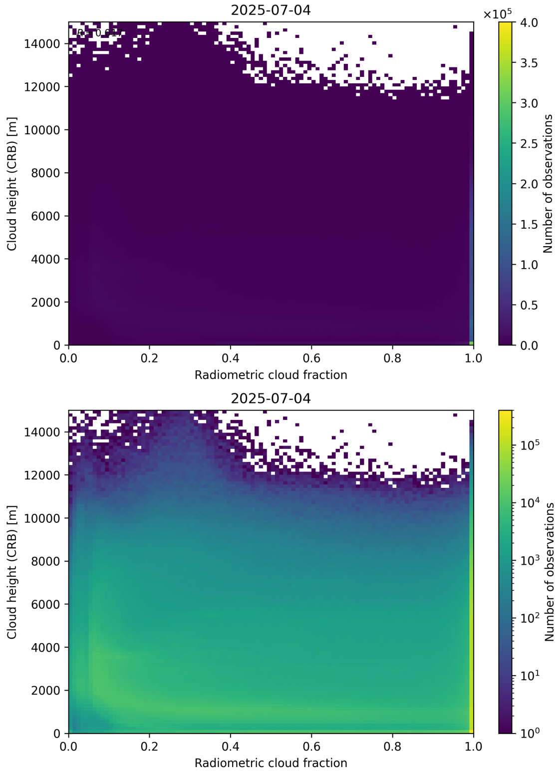
Figure 74: Scatter density plot of “Radiometric cloud fraction” against “Cloud height (CRB)” for 2025-07-03 to 2025-07-05.
