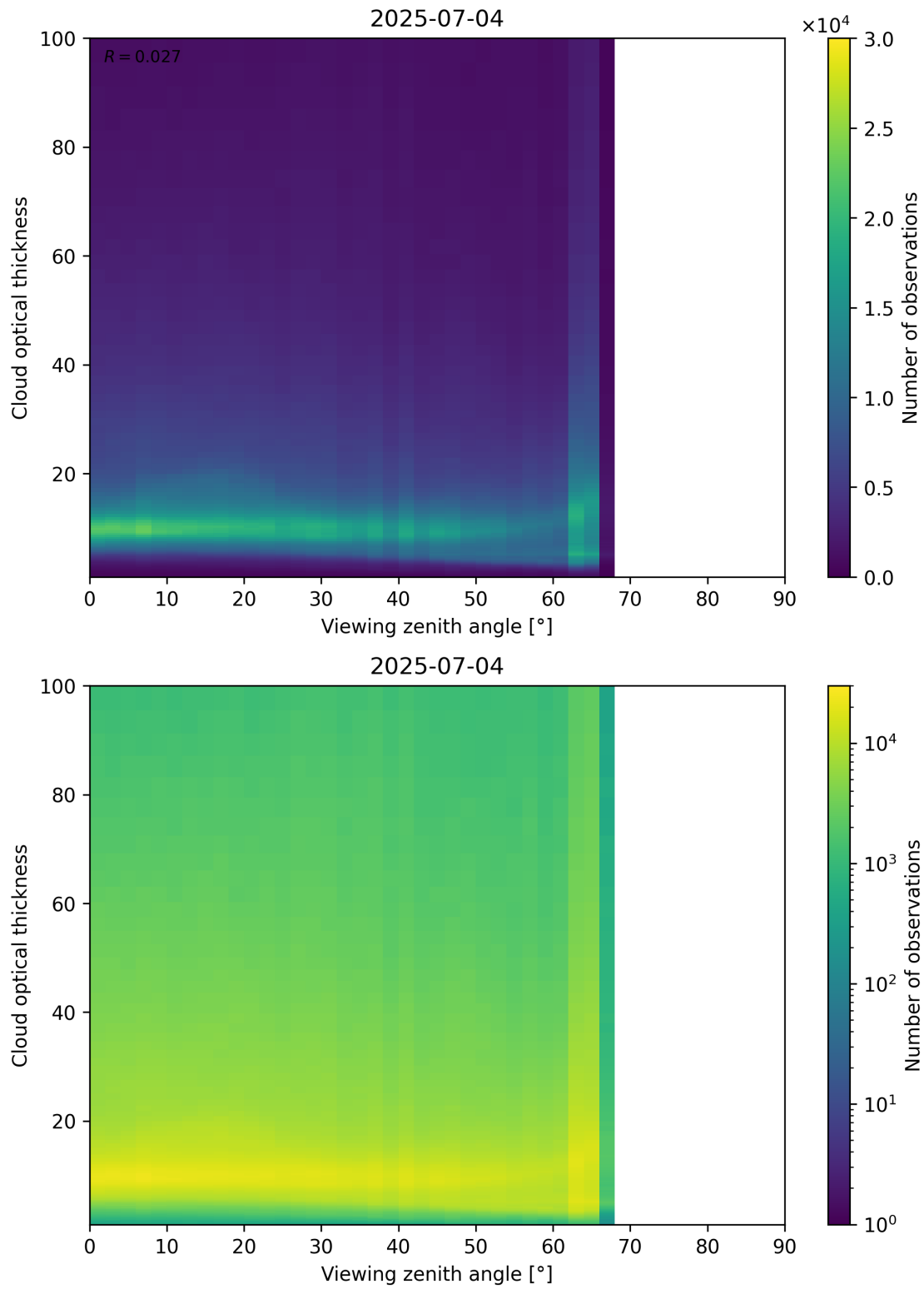
Figure 111: Scatter density plot of “Viewing zenith angle” against “Cloud optical thickness” for 2025-07-03 to 2025-07-05.
