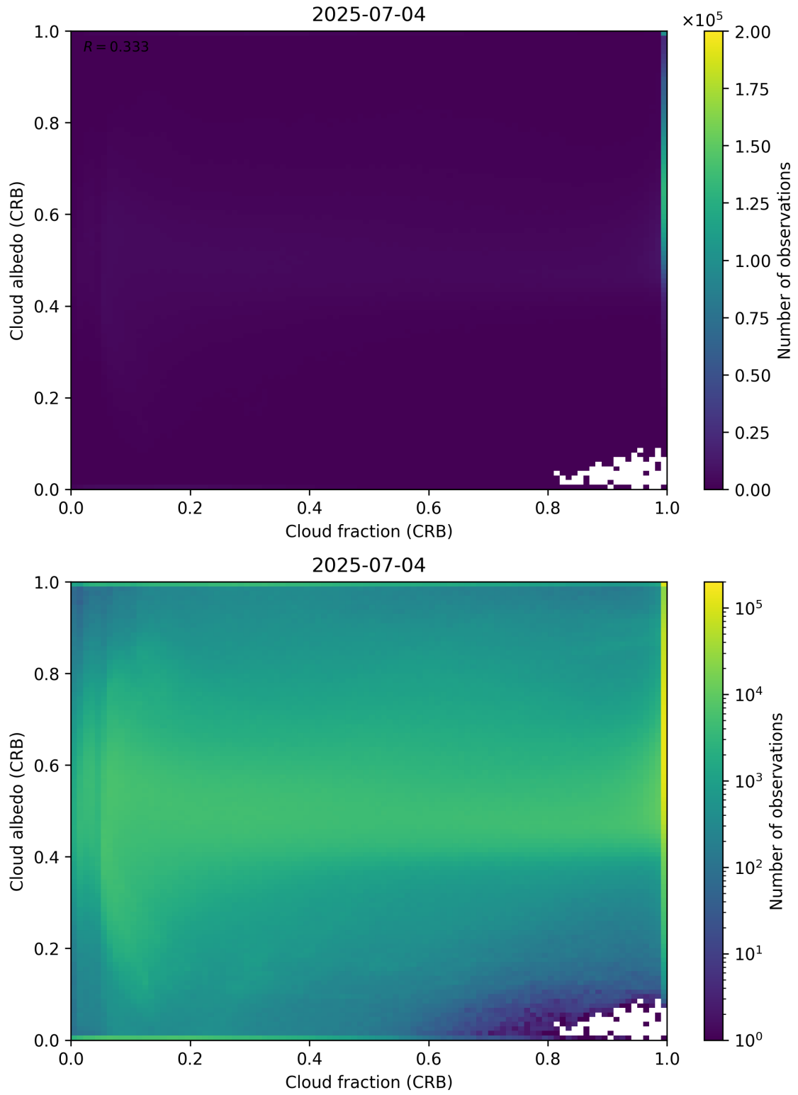
Figure 77: Scatter density plot of “Cloud fraction (CRB)” against “Cloud albedo (CRB)” for 2025-07-03 to 2025-07-05.
