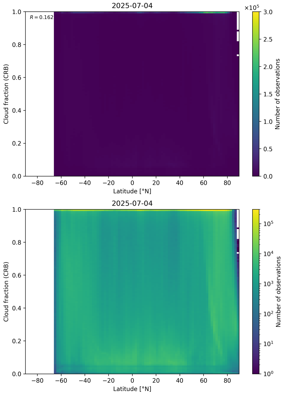
Figure 94: Scatter density plot of “Latitude” against “Cloud fraction (CRB)” for 2025-07-03 to 2025-07-05.
