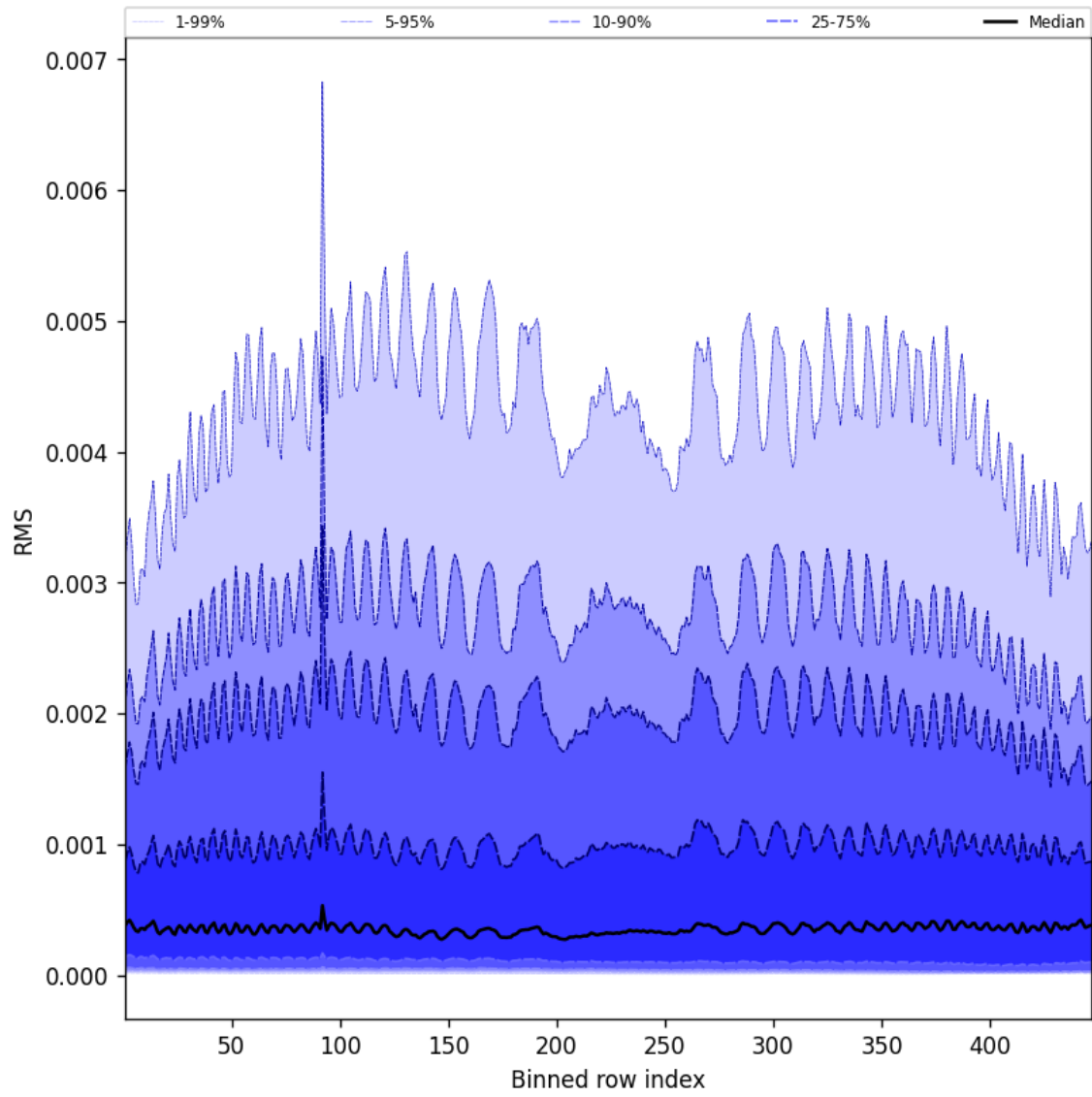
Figure 63: Along track statistics of “RMS” for 2025-07-03 to 2025-07-05
