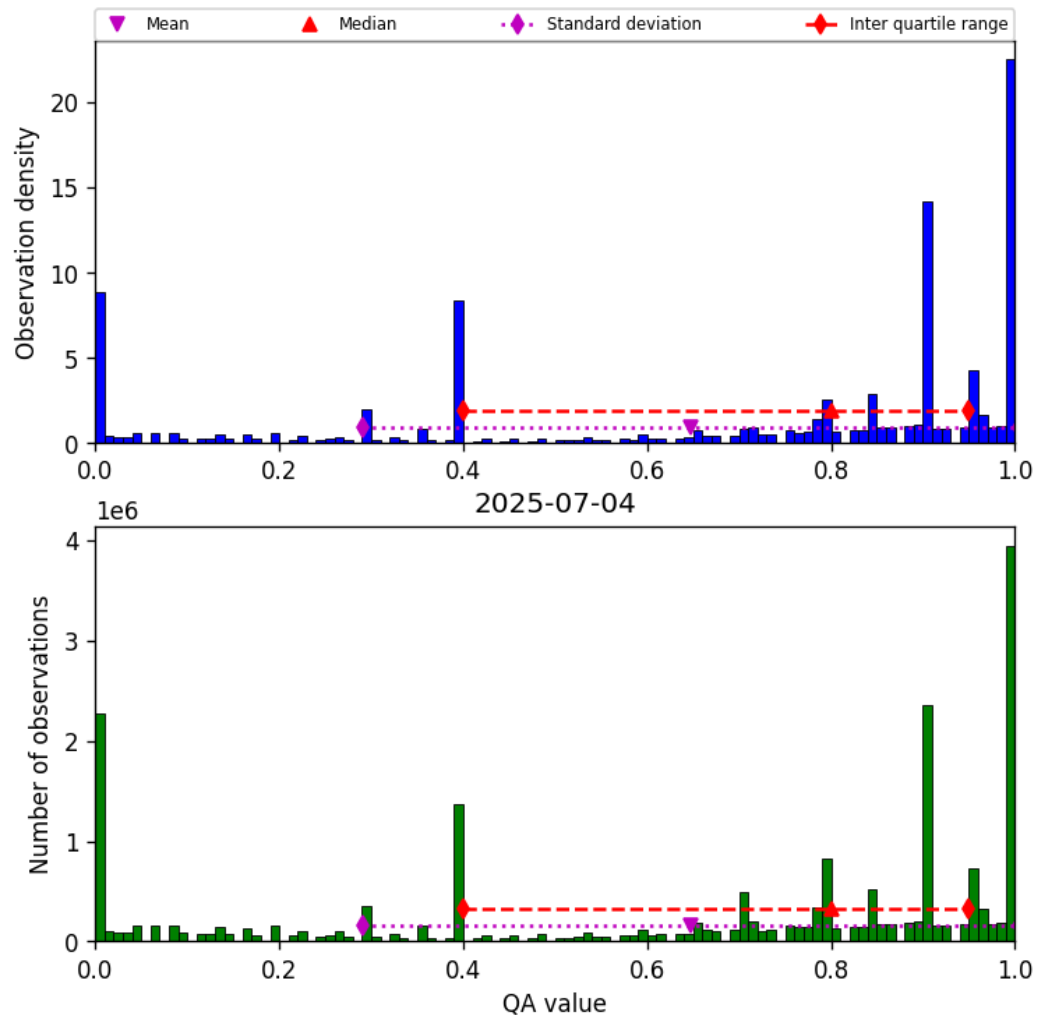
Figure 38: Histogram of “QA value” for 2025-07-03 to 2025-07-05
