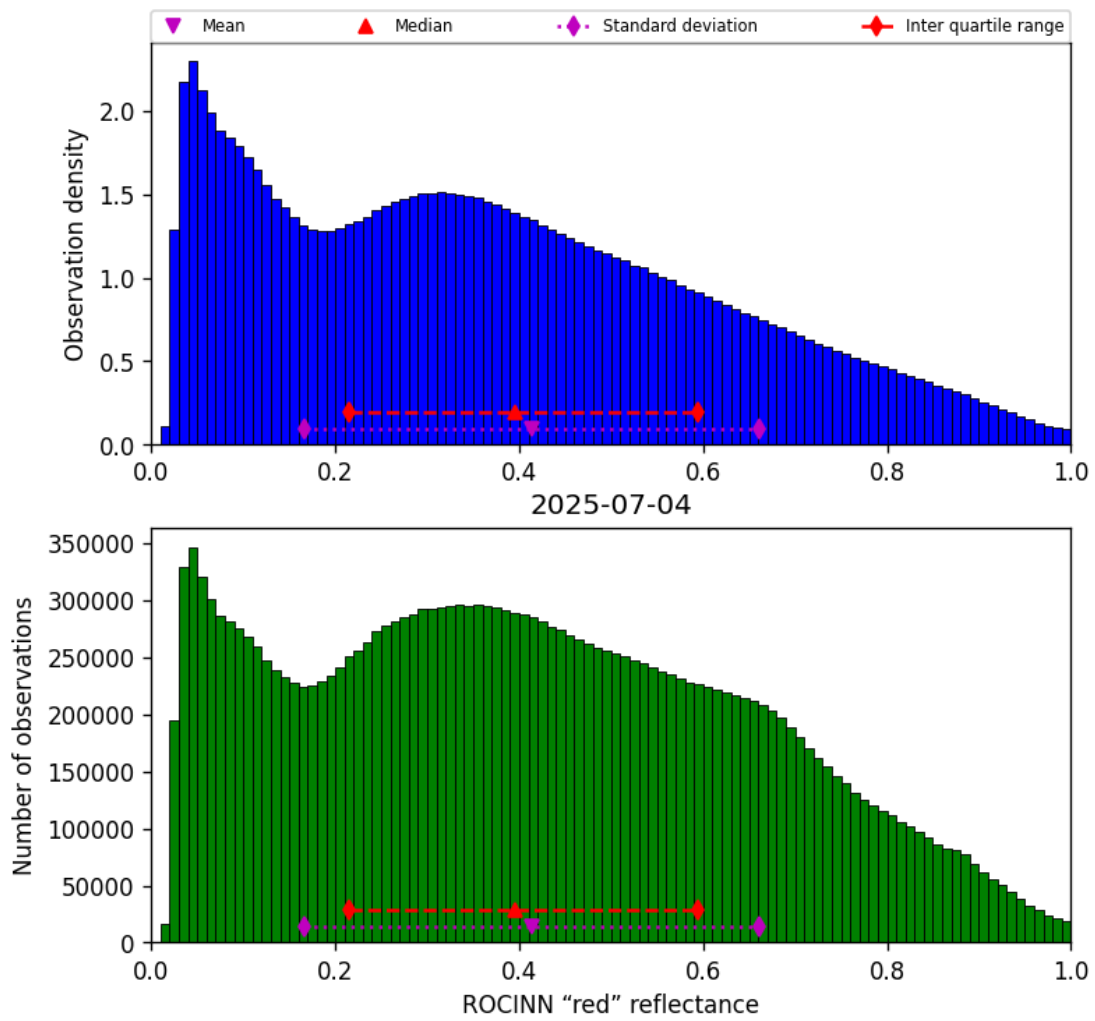
Figure 53: Histogram of “ROCINN “red” reflectance” for 2025-07-03 to 2025-07-05
