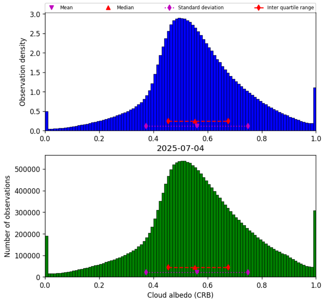
Figure 44: Histogram of “Cloud albedo (CRB)” for 2025-07-03 to 2025-07-05
