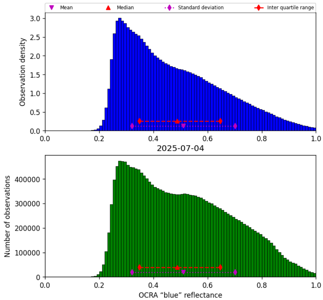
Figure 51: Histogram of “OCRA “blue” reflectance” for 2025-07-03 to 2025-07-05
