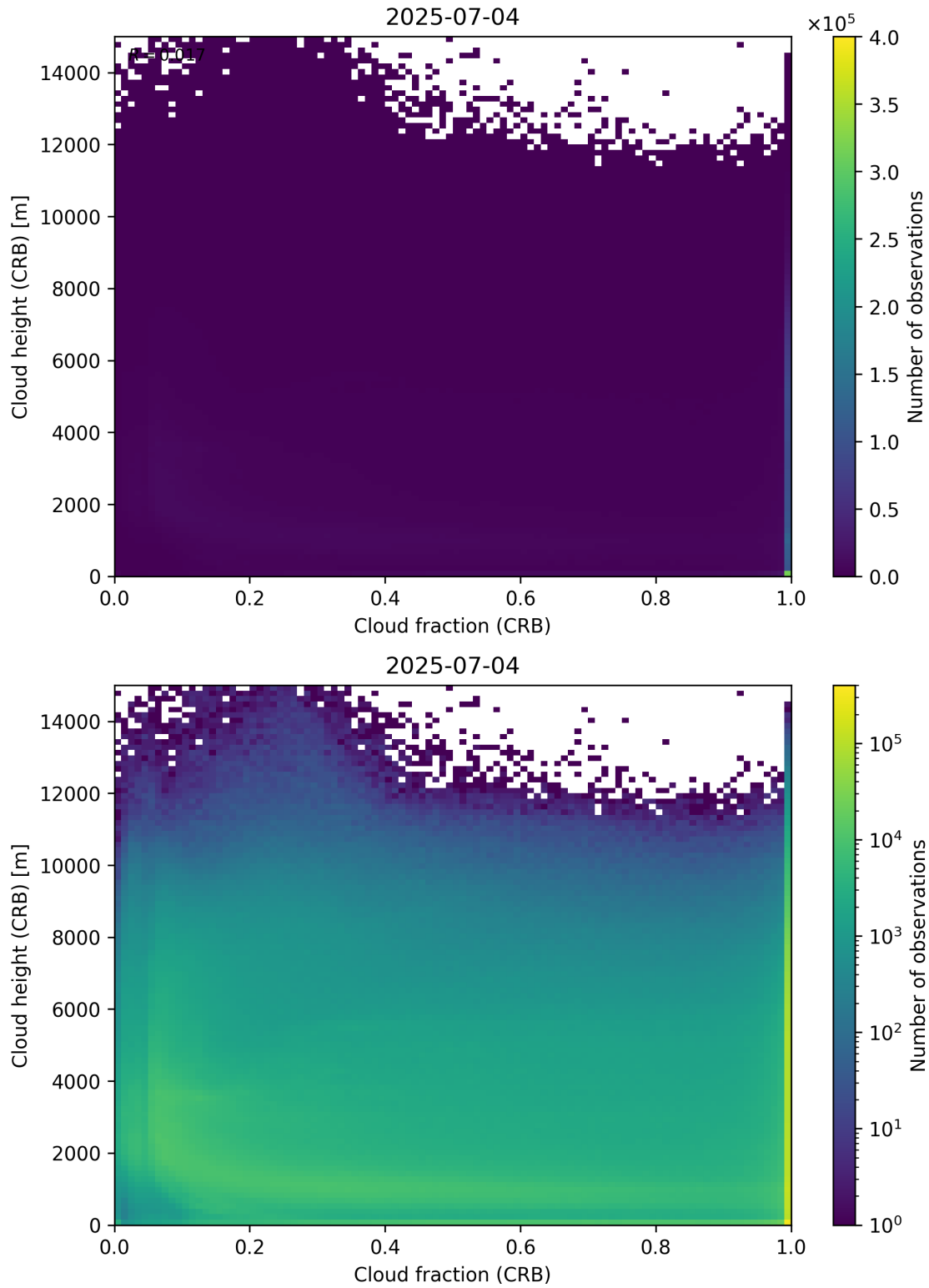
Figure 79: Scatter density plot of “Cloud fraction (CRB)” against “Cloud height (CRB)” for 2025-07-03 to 2025-07-05.
