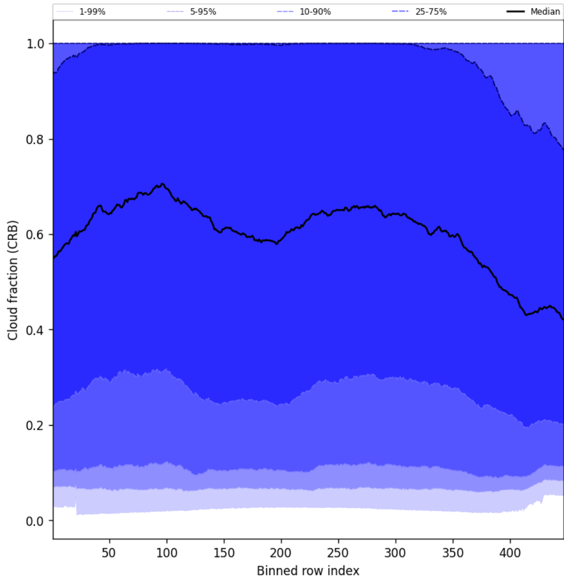
Figure 58: Along track statistics of “Cloud fraction (CRB)” for 2025-07-04 to 2025-07-06
