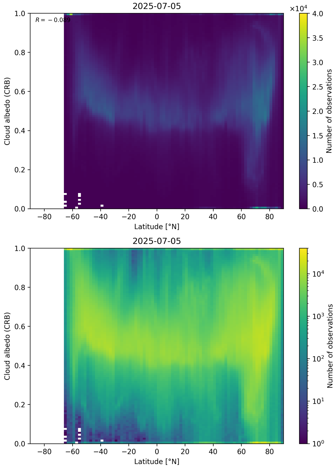
Figure 91: Scatter density plot of “Latitude” against “Cloud albedo (CRB)” for 2025-07-04 to 2025-07-06.
