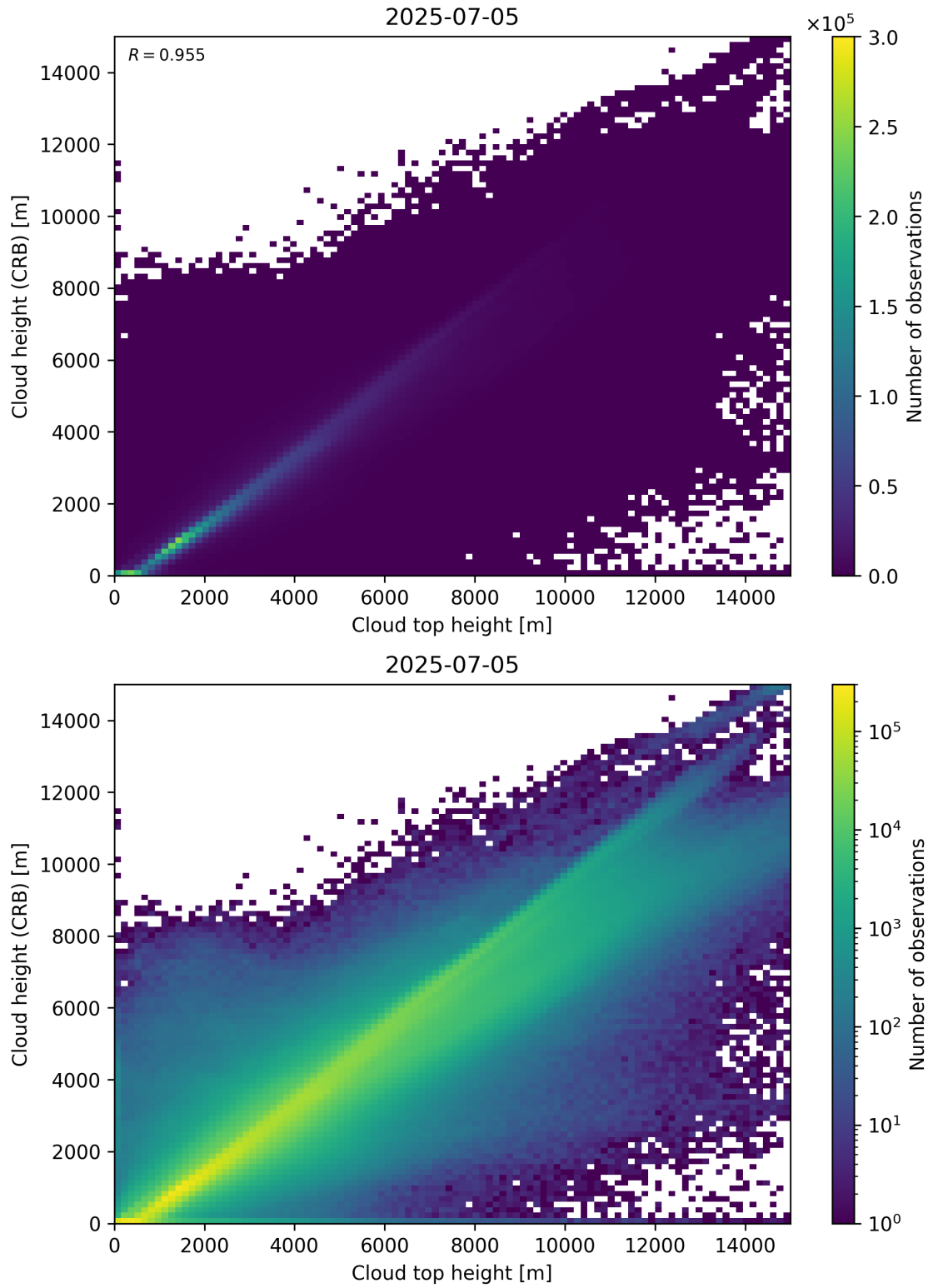
Figure 89: Scatter density plot of “Cloud top height” against “Cloud height (CRB)” for 2025-07-04 to 2025-07-06.
