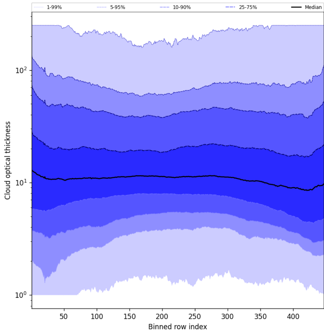
Figure 57: Along track statistics of “Cloud optical thickness” for 2025-07-04 to 2025-07-06
