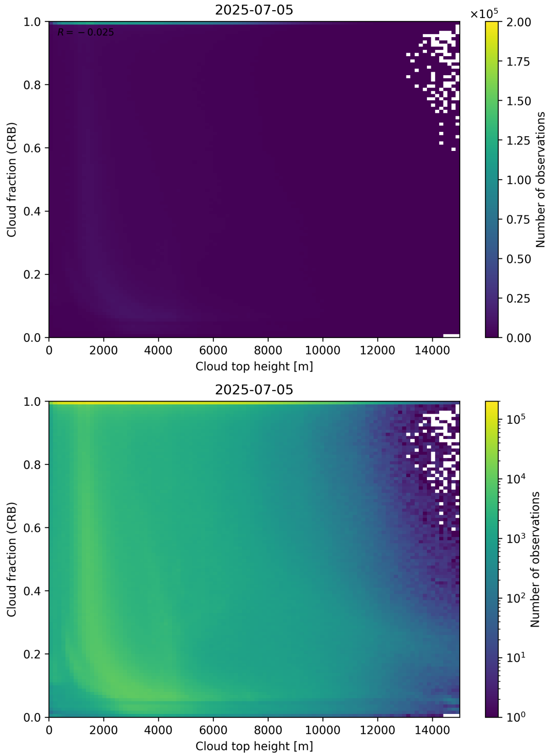
Figure 88: Scatter density plot of “Cloud top height” against “Cloud fraction (CRB)” for 2025-07-04 to 2025-07-06.
