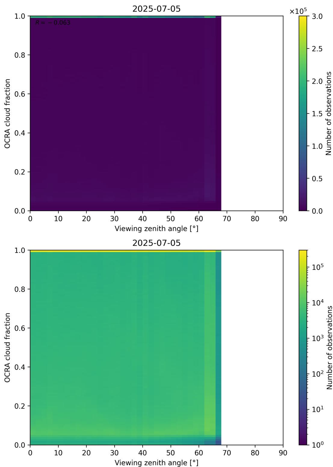
Figure 108: Scatter density plot of “Viewing zenith angle” against “OCRA cloud fraction” for 2025-07-04 to 2025-07-06.
