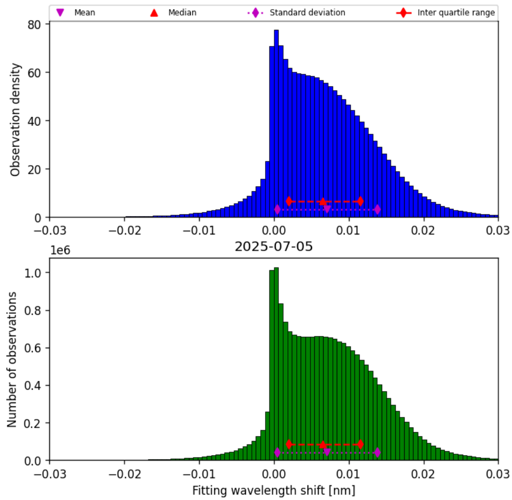
Figure 49: Histogram of “Fitting wavelength shift” for 2025-07-04 to 2025-07-06
