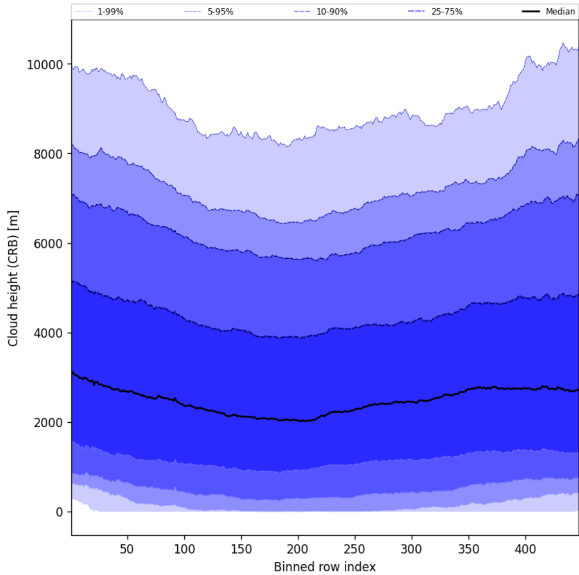
Figure 59: Along track statistics of “Cloud height (CRB)” for 2025-07-04 to 2025-07-06
