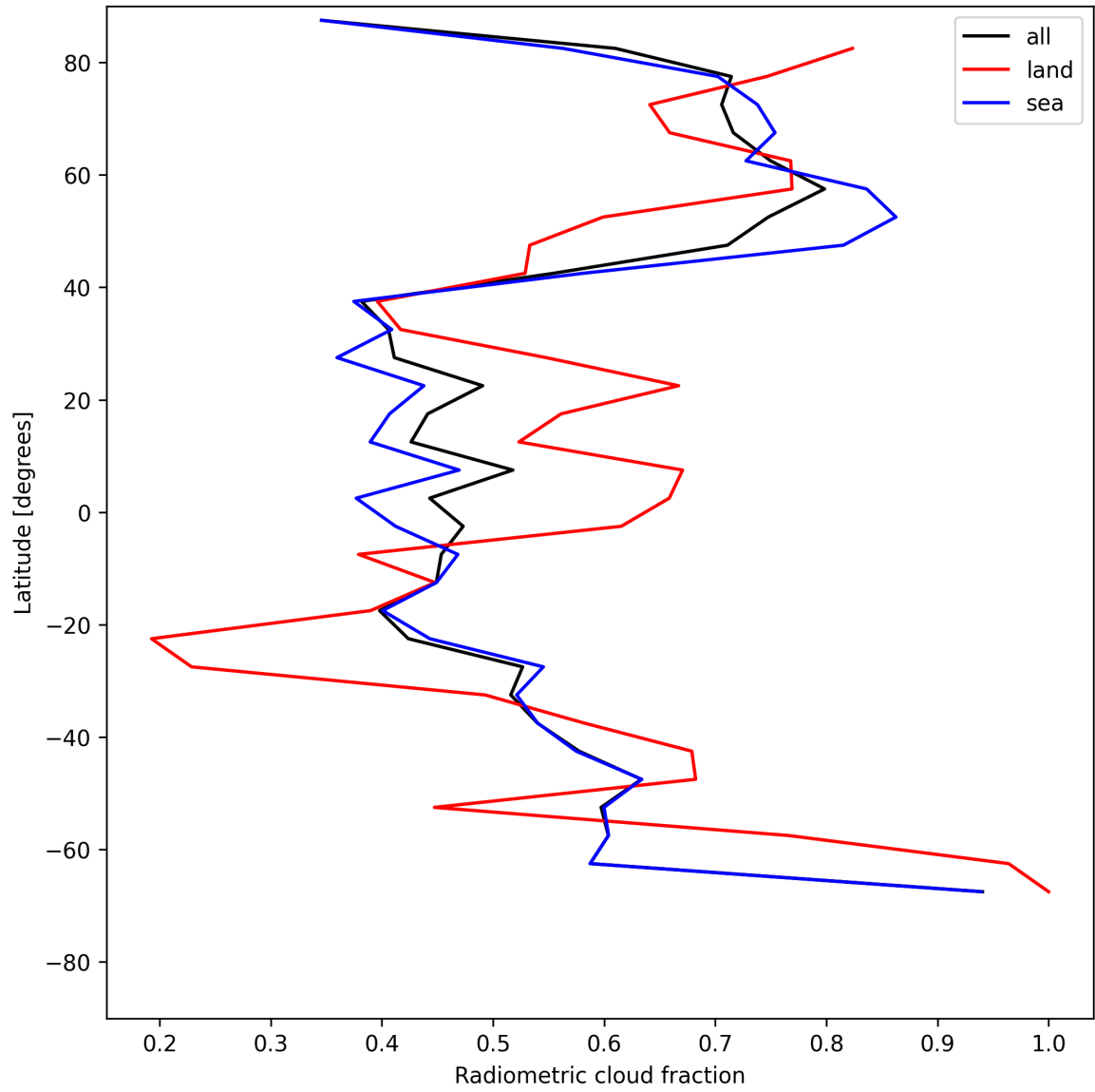
Figure 23: Zonal average of “Radiometric cloud fraction” for 2025-07-04 to 2025-07-06.
