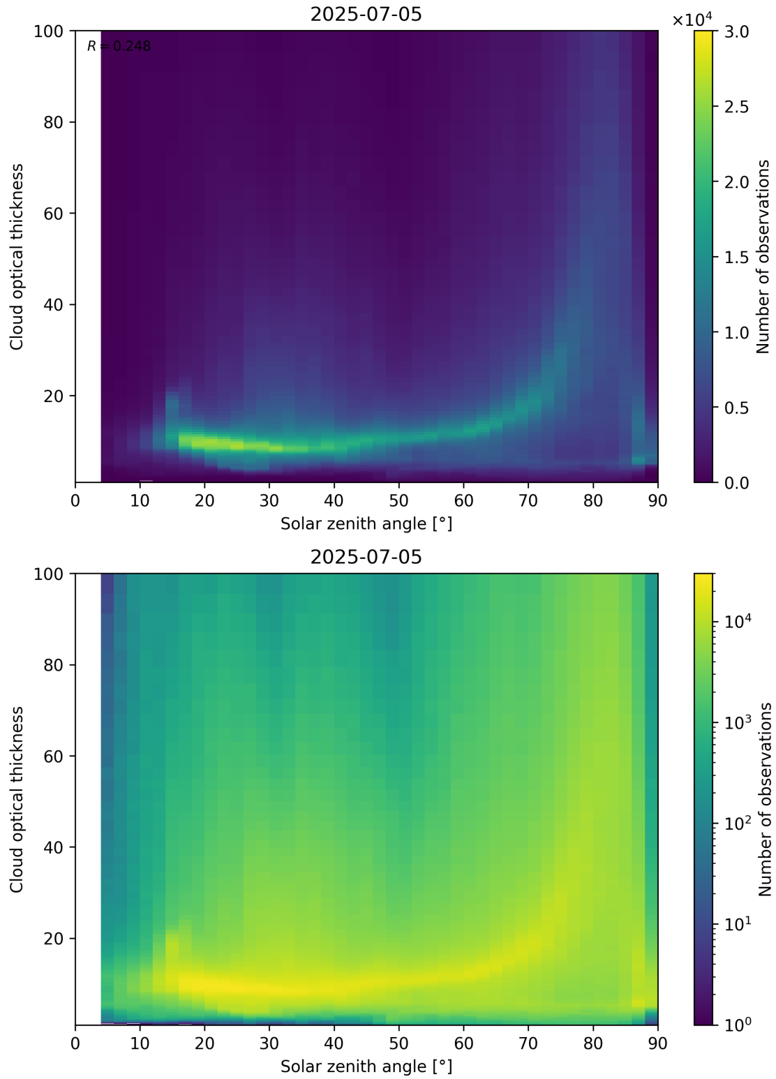
Figure 103: Scatter density plot of “Solar zenith angle” against “Cloud optical thickness” for 2025-07-04 to 2025-07-06.
