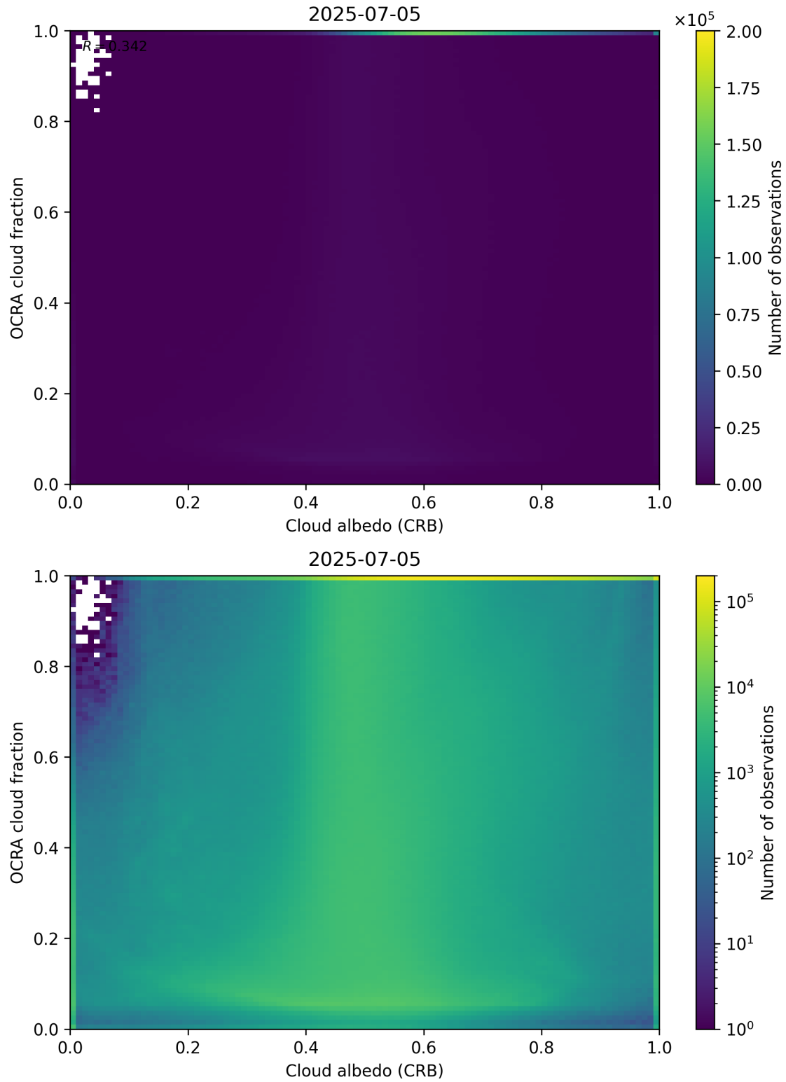
Figure 70: Scatter density plot of “Cloud albedo (CRB)” against “OCRA cloud fraction” for 2025-07-04 to 2025-07-06.
