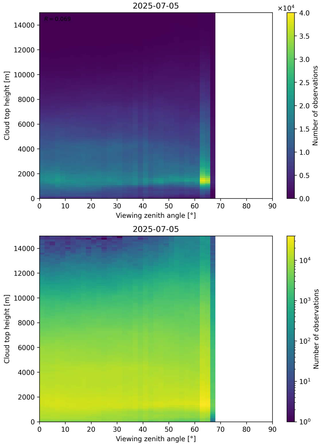
Figure 112: Scatter density plot of “Viewing zenith angle” against “Cloud top height” for 2025-07-04 to 2025-07-06.
