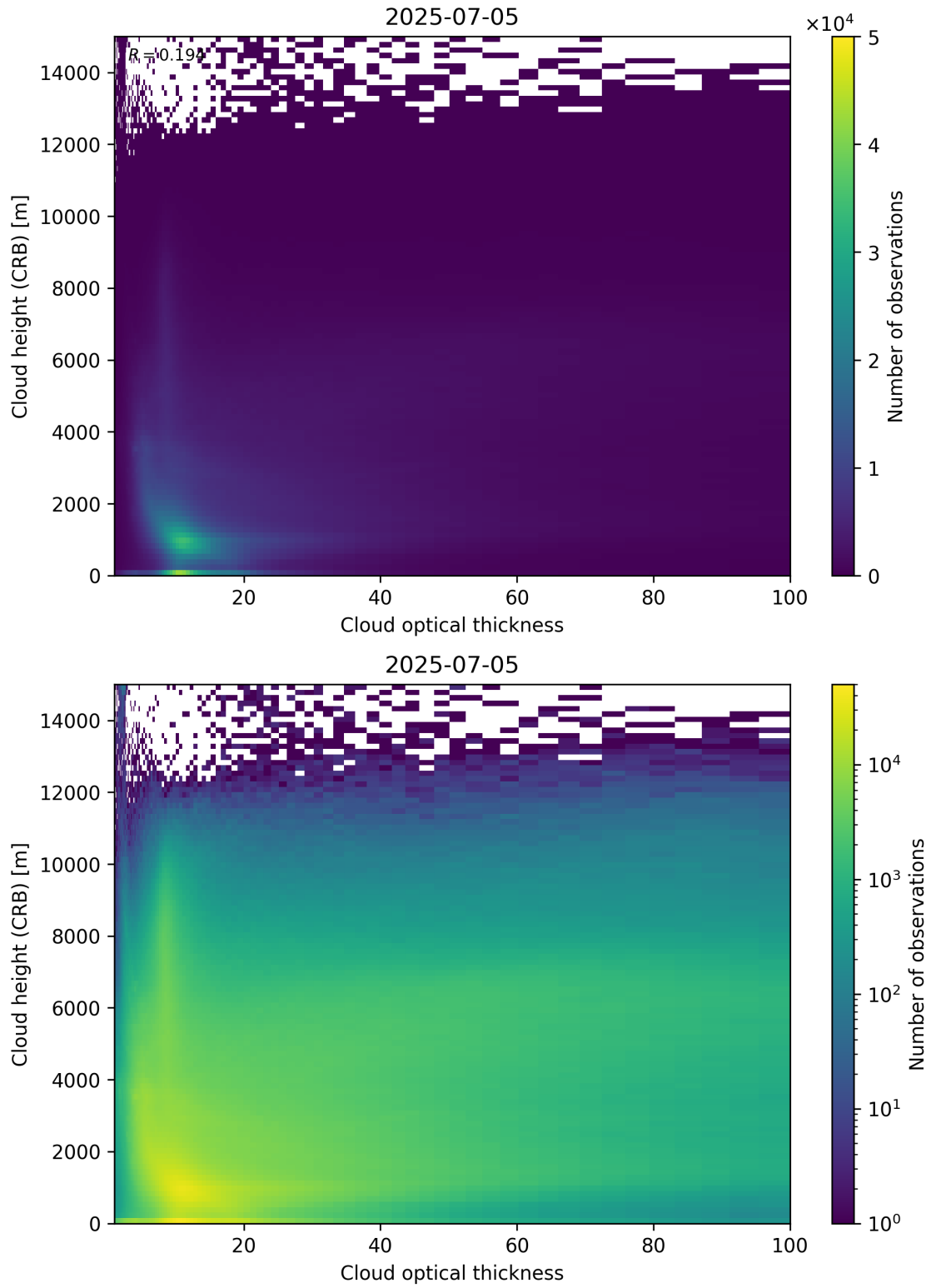
Figure 85: Scatter density plot of “Cloud optical thickness” against “Cloud height (CRB)” for 2025-07-04 to 2025-07-06.
