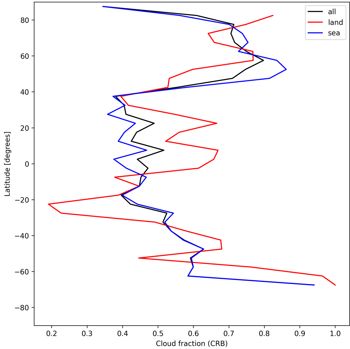
Figure 26: Zonal average of “Cloud fraction (CRB)” for 2025-07-04 to 2025-07-06.
