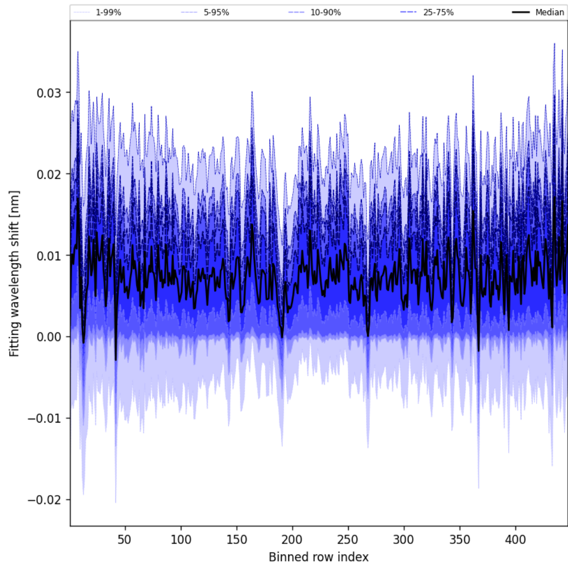
Figure 65: Along track statistics of “Fitting wavelength shift” for 2025-07-04 to 2025-07-06
