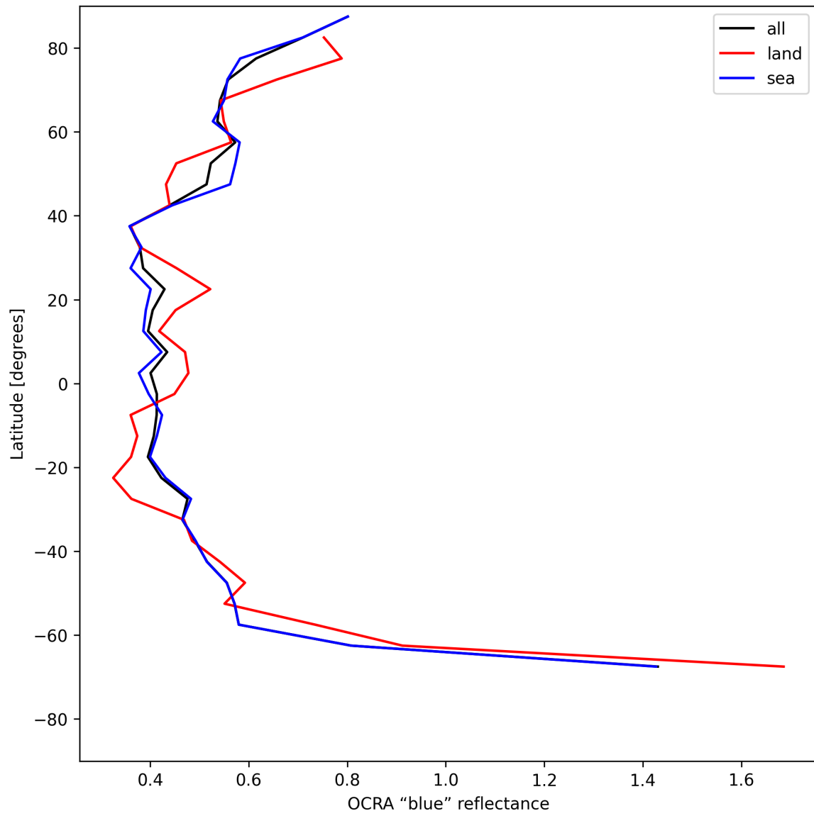
Figure 35: Zonal average of “OCRA “blue” reflectance” for 2025-07-04 to 2025-07-06.
