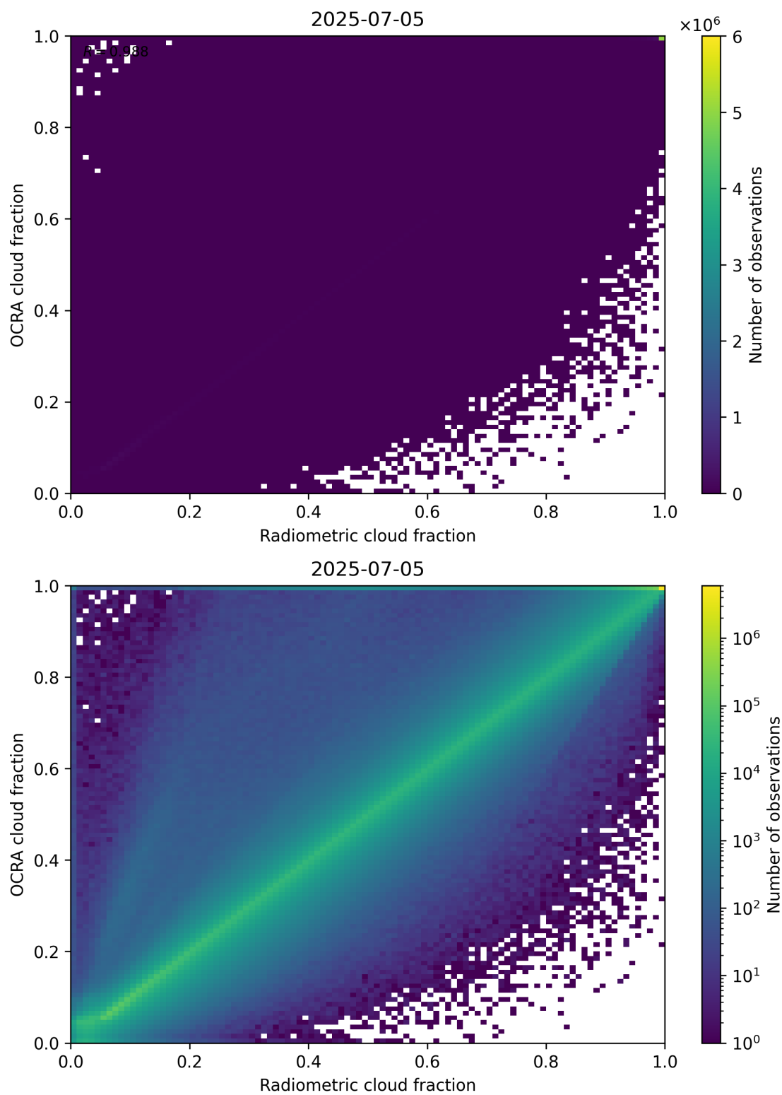
Figure 72: Scatter density plot of “Radiometric cloud fraction” against “OCRA cloud fraction” for 2025-07-04 to 2025-07-06.
