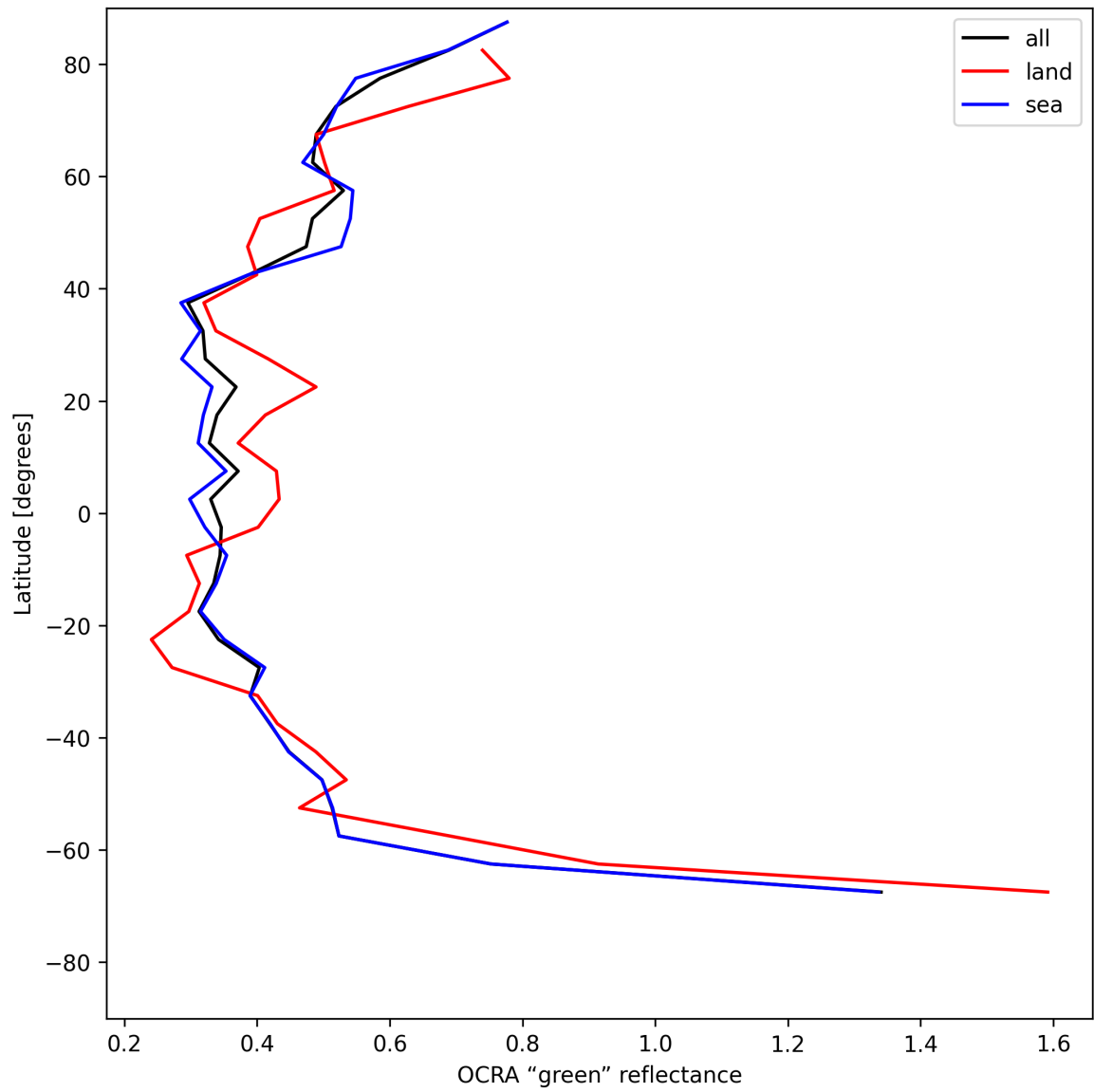
Figure 36: Zonal average of “OCRA “green” reflectance” for 2025-07-04 to 2025-07-06.
