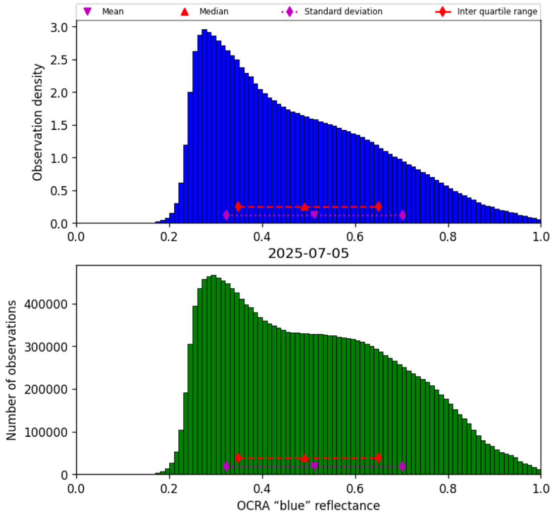
Figure 51: Histogram of “OCRA “blue” reflectance” for 2025-07-04 to 2025-07-06
