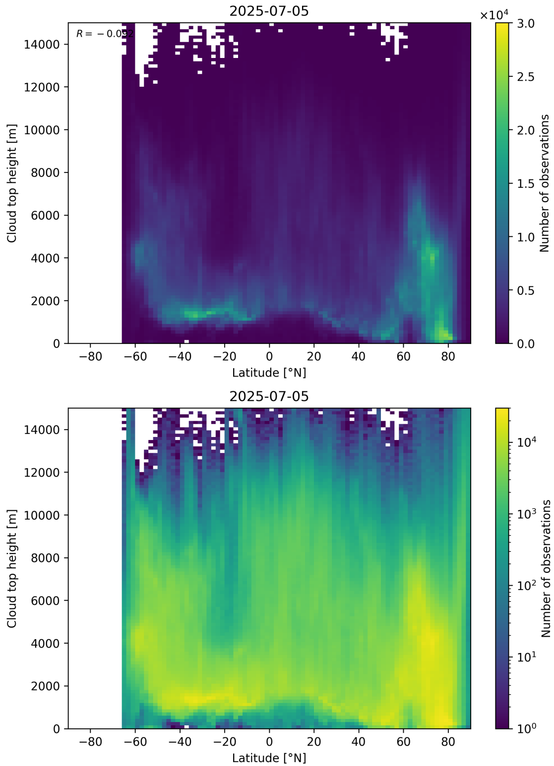
Figure 97: Scatter density plot of “Latitude” against “Cloud top height” for 2025-07-04 to 2025-07-06.
