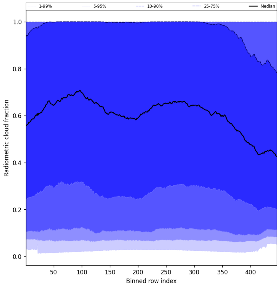
Figure 55: Along track statistics of “Radiometric cloud fraction” for 2025-07-04 to 2025-07-06
