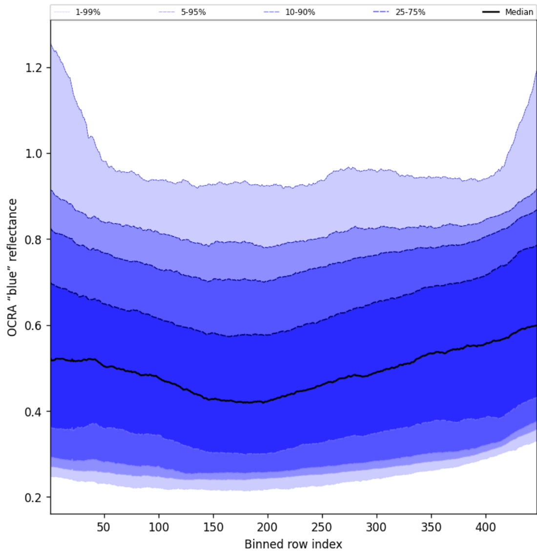
Figure 67: Along track statistics of “OCRA “blue” reflectance” for 2025-07-04 to 2025-07-06
