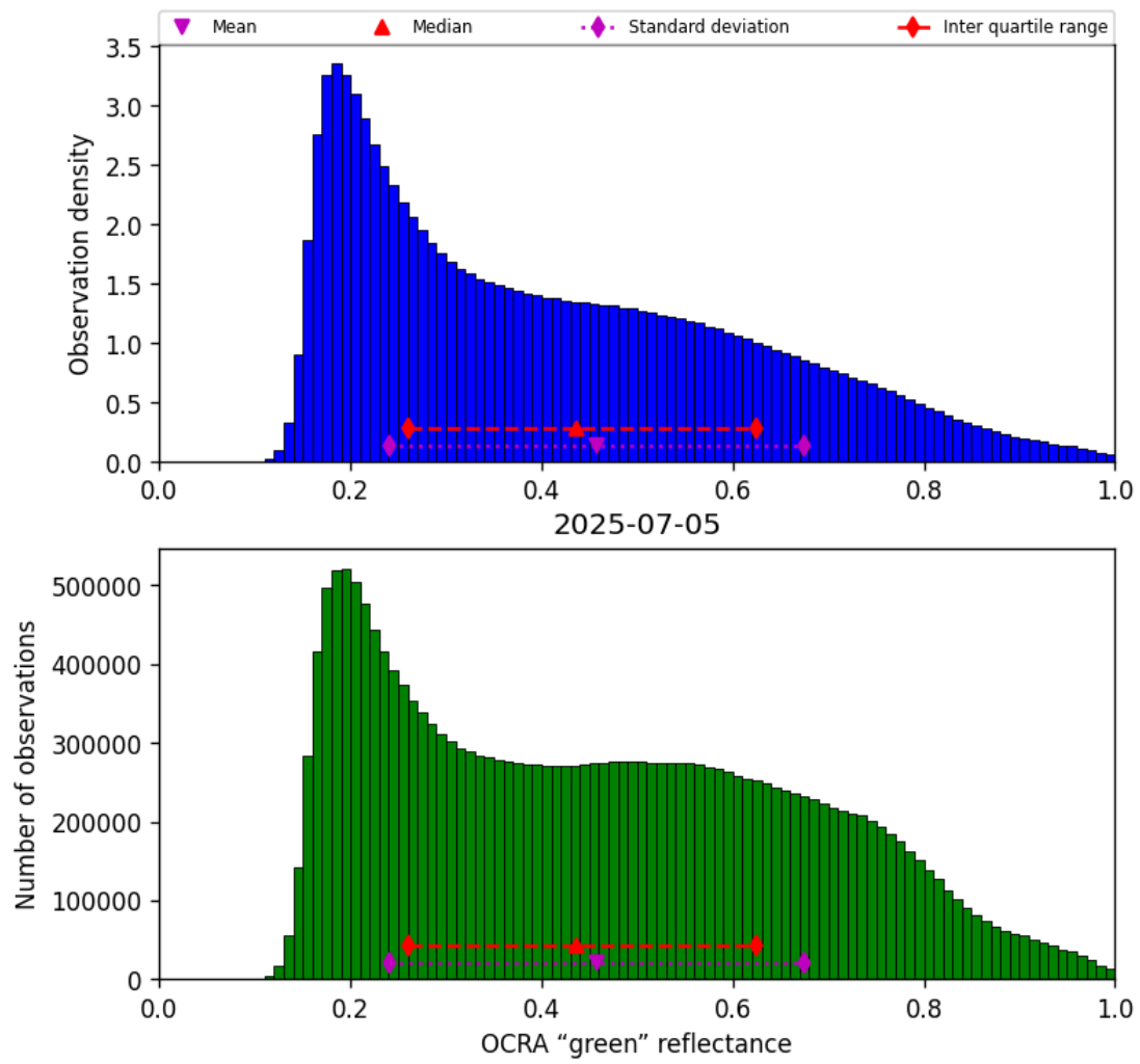
Figure 52: Histogram of “OCRA “green” reflectance” for 2025-07-04 to 2025-07-06
