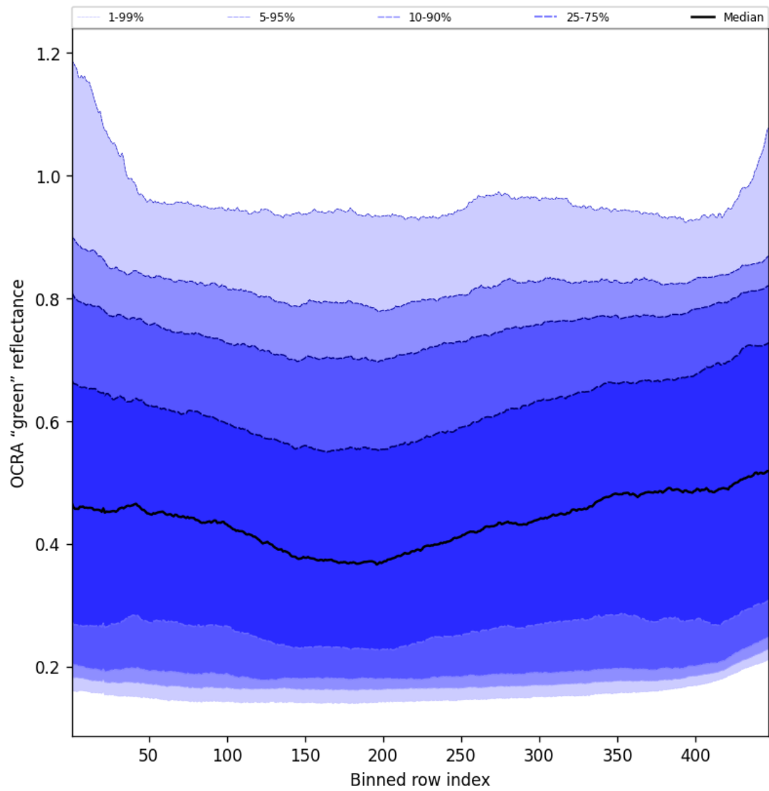
Figure 68: Along track statistics of "OCRA "green" reflectance" for 2025-07-04 to 2025-07-06
