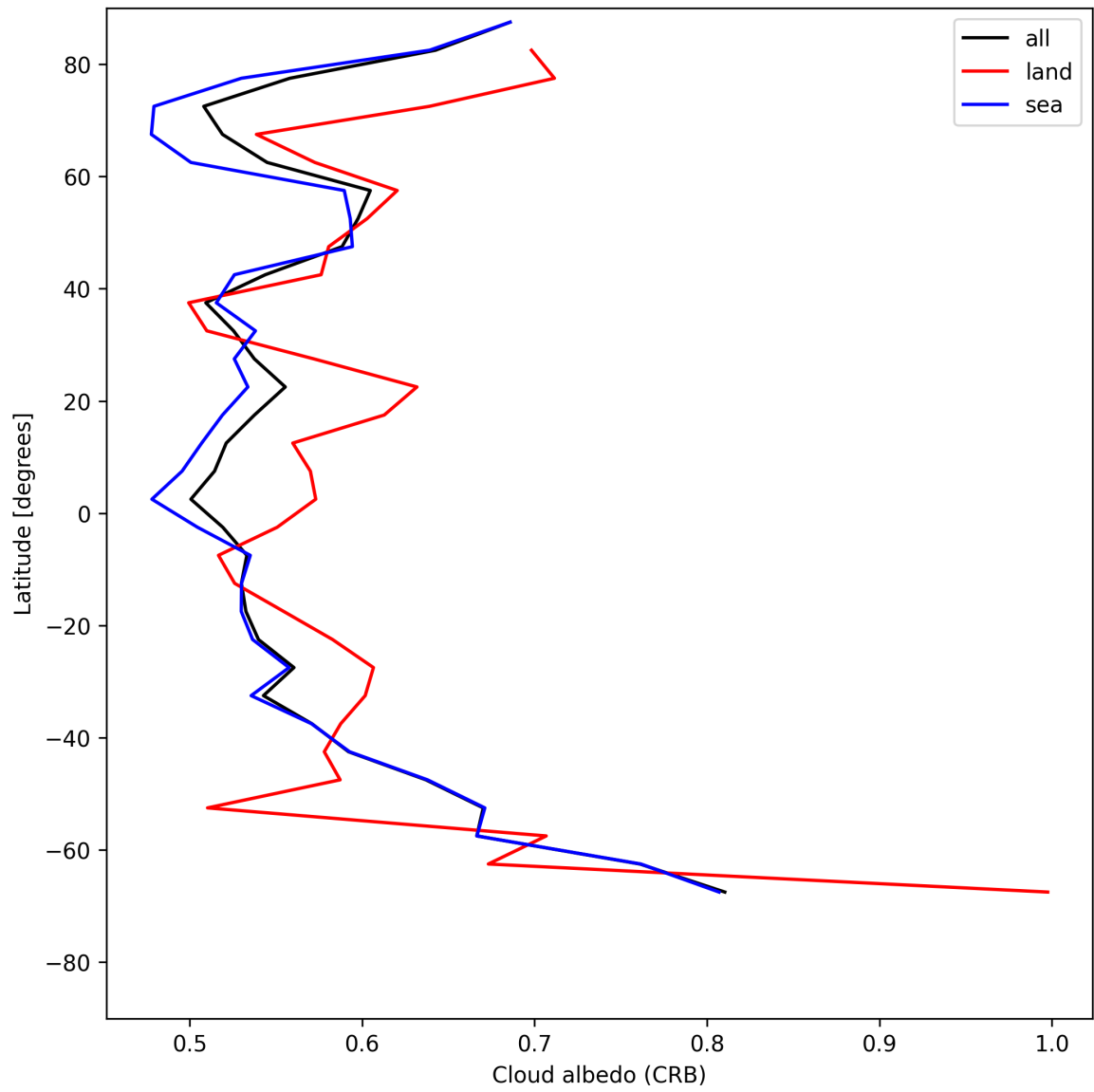
Figure 28: Zonal average of “Cloud albedo (CRB)” for 2025-07-04 to 2025-07-06.
