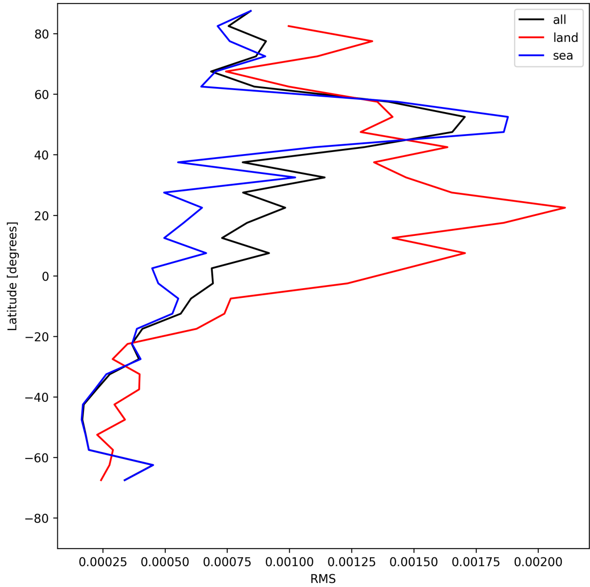
Figure 31: Zonal average of “RMS” for 2025-07-04 to 2025-07-06.
