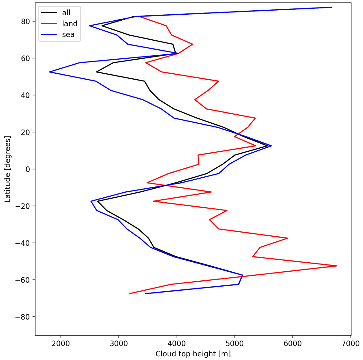
Figure 24: Zonal average of “Cloud top height” for 2025-07-04 to 2025-07-06.
