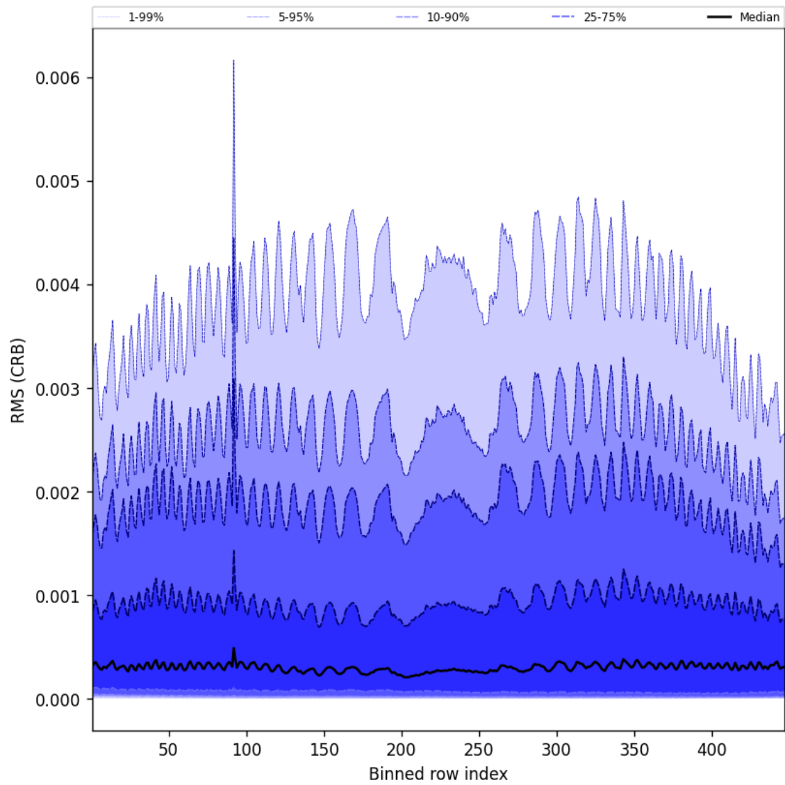
Figure 64: Along track statistics of “RMS (CRB)” for 2025-07-04 to 2025-07-06
