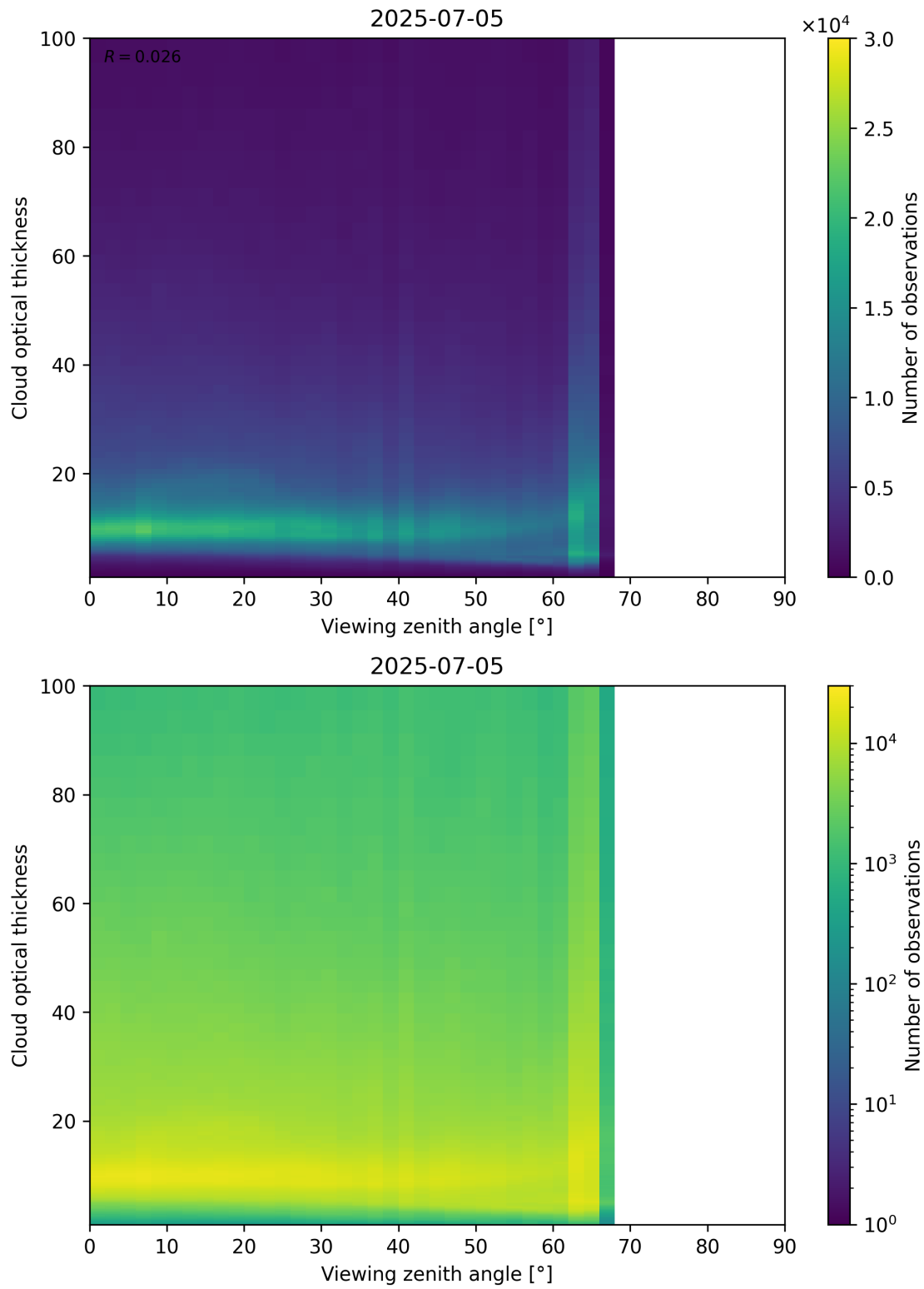
Figure 111: Scatter density plot of “Viewing zenith angle” against “Cloud optical thickness” for 2025-07-04 to 2025-07-06.
