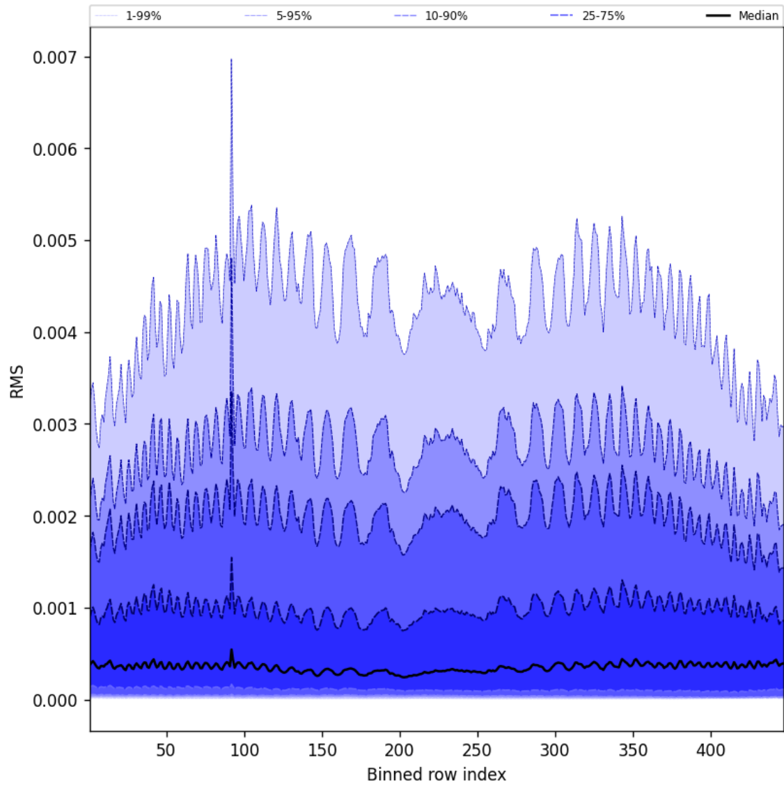
Figure 63: Along track statistics of “RMS” for 2025-07-04 to 2025-07-06
