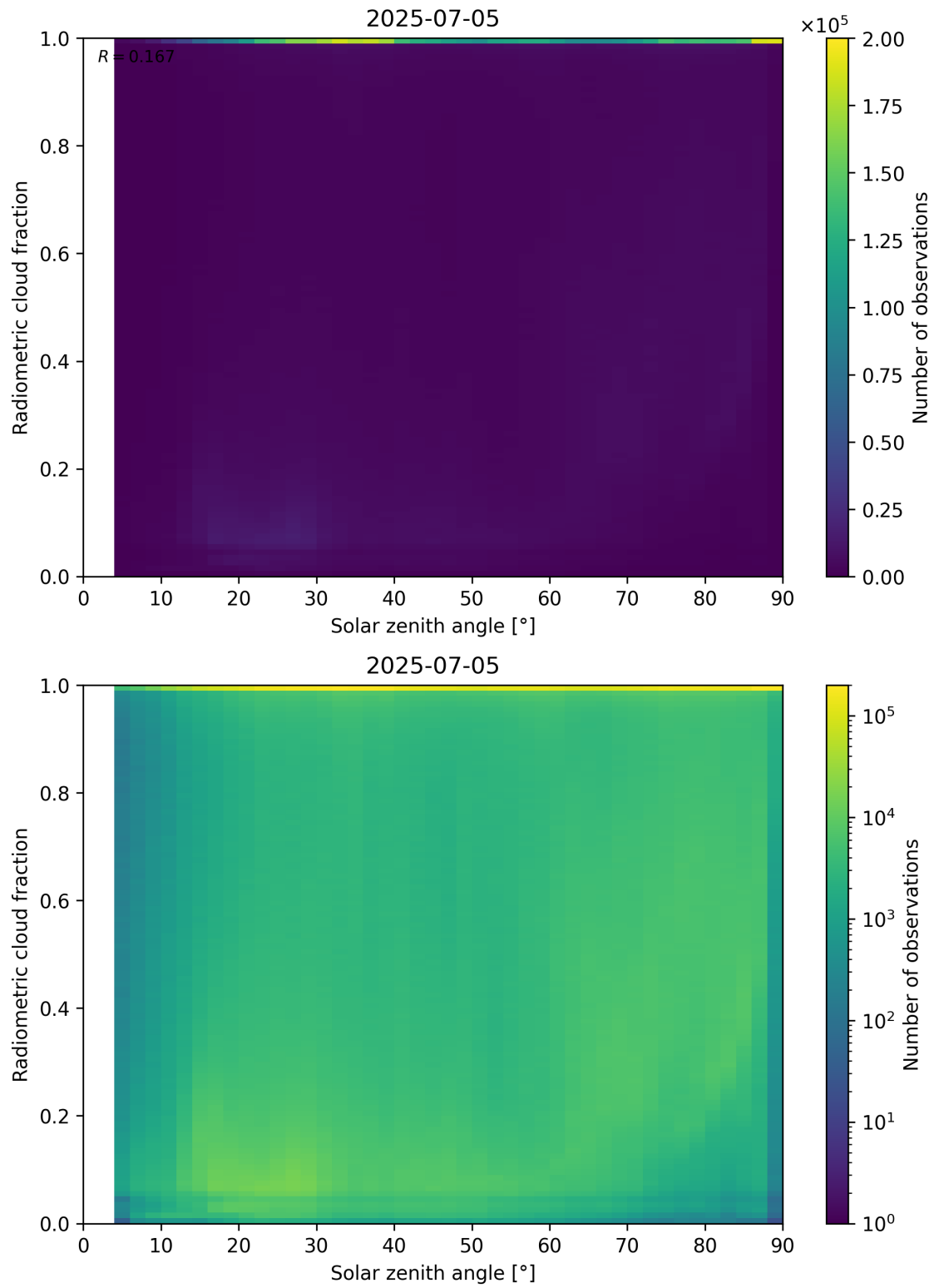
Figure 99: Scatter density plot of “Solar zenith angle” against “Radiometric cloud fraction” for 2025-07-04 to 2025-07-06.
