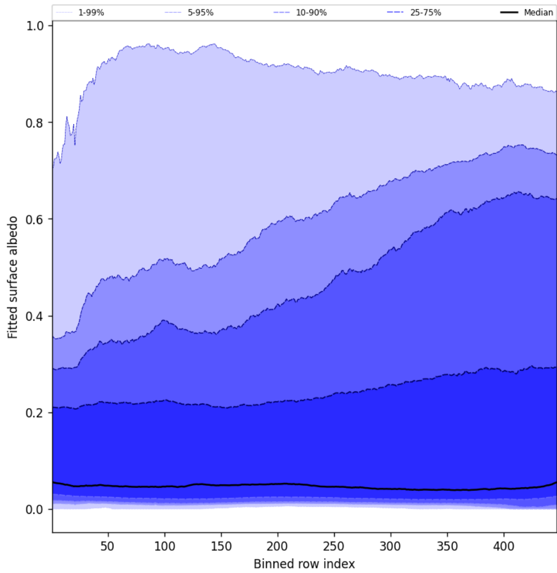
Figure 61: Along track statistics of “Fitted surface albedo” for 2025-07-04 to 2025-07-06
