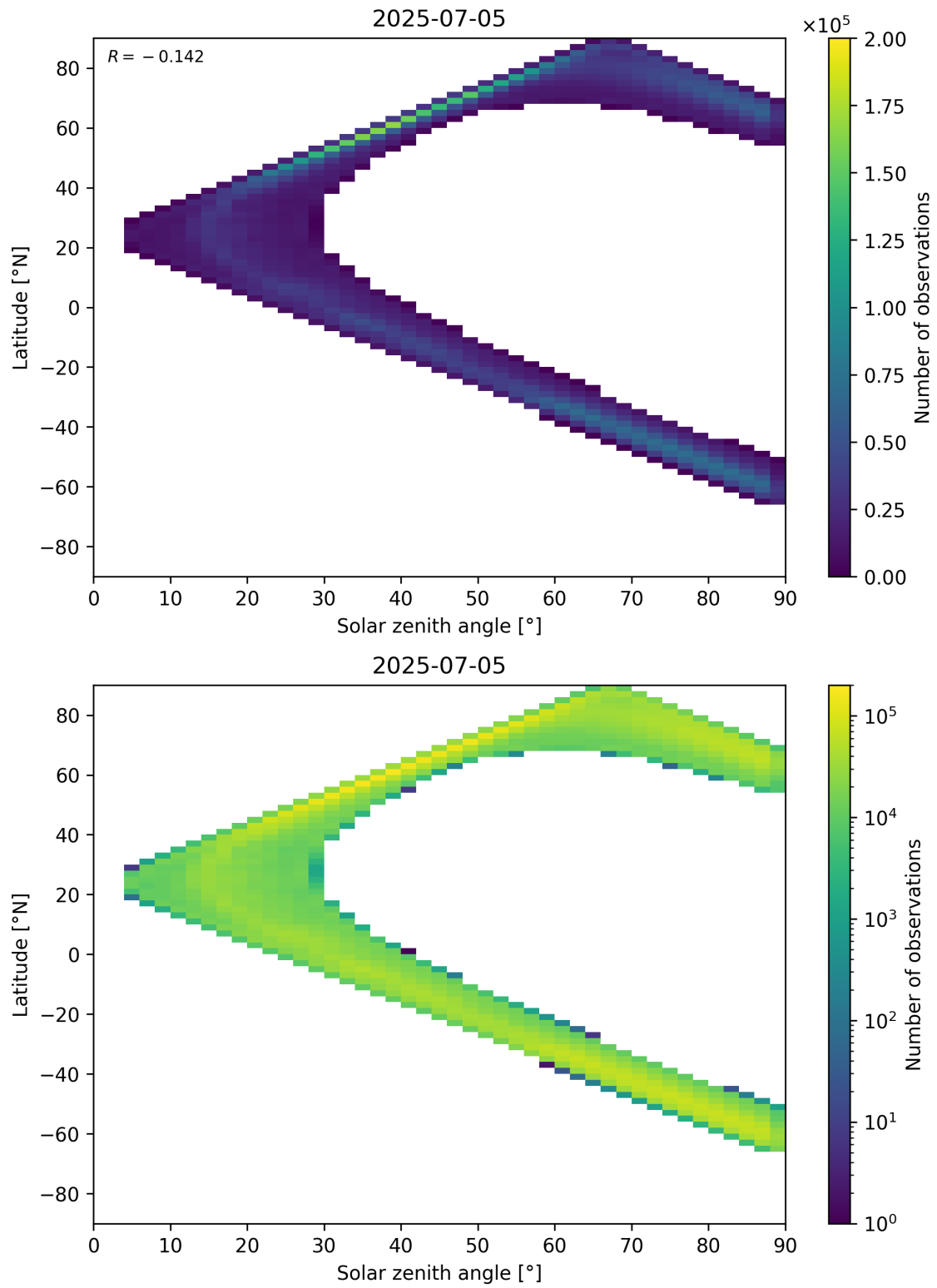
Figure 105: Scatter density plot of “Solar zenith angle” against “Latitude” for 2025-07-04 to 2025-07-06.
