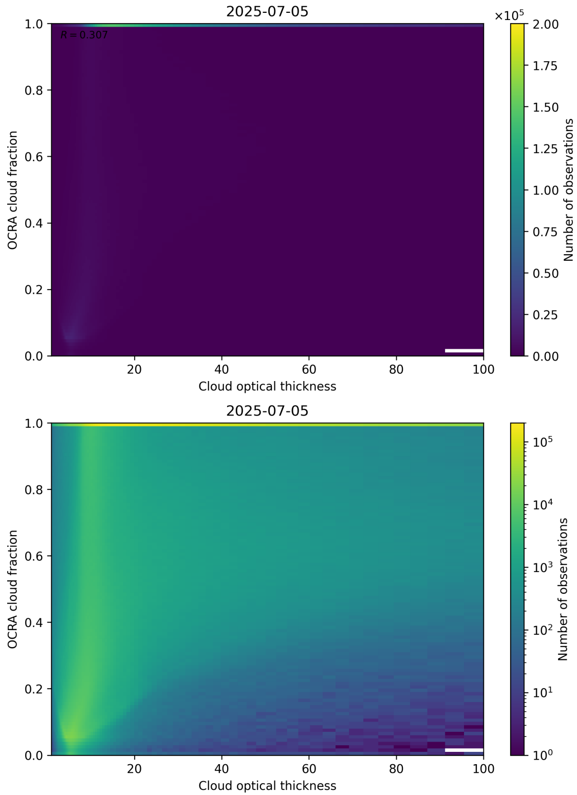
Figure 83: Scatter density plot of “Cloud optical thickness” against “OCRA cloud fraction” for 2025-07-04 to 2025-07-06.
