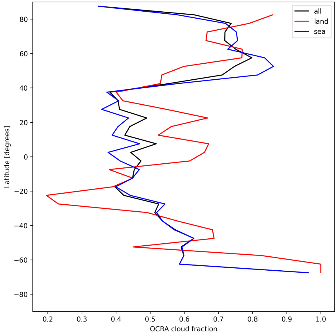
Figure 34: Zonal average of “OCRA cloud fraction” for 2025-07-04 to 2025-07-06.
