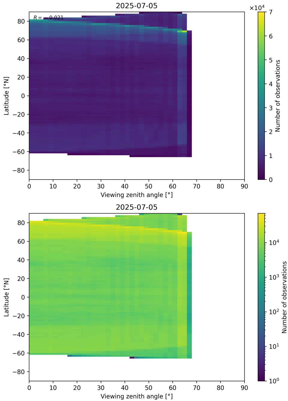
Figure 113: Scatter density plot of “Viewing zenith angle” against “Latitude” for 2025-07-04 to 2025-07-06.
