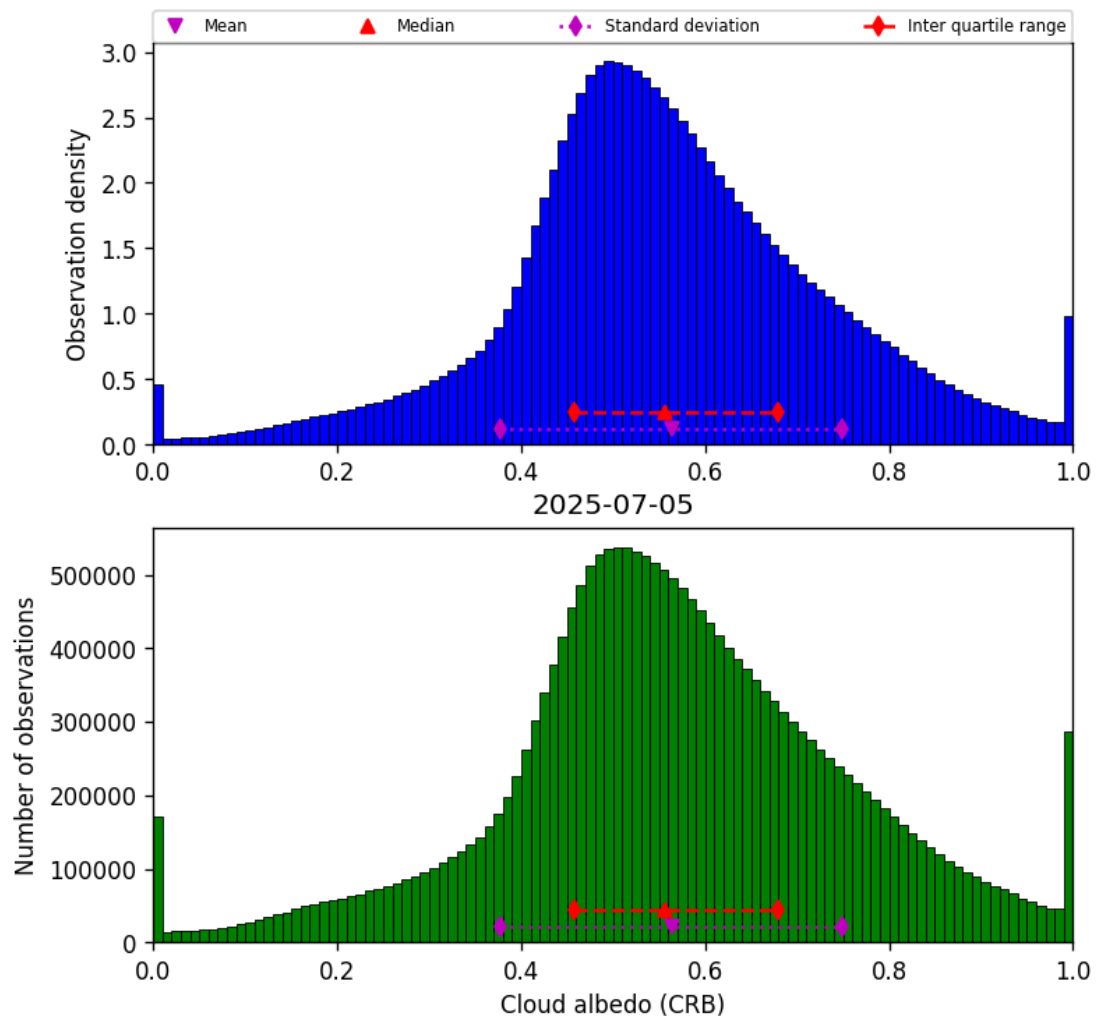
Figure 44: Histogram of “Cloud albedo (CRB)” for 2025-07-04 to 2025-07-06
