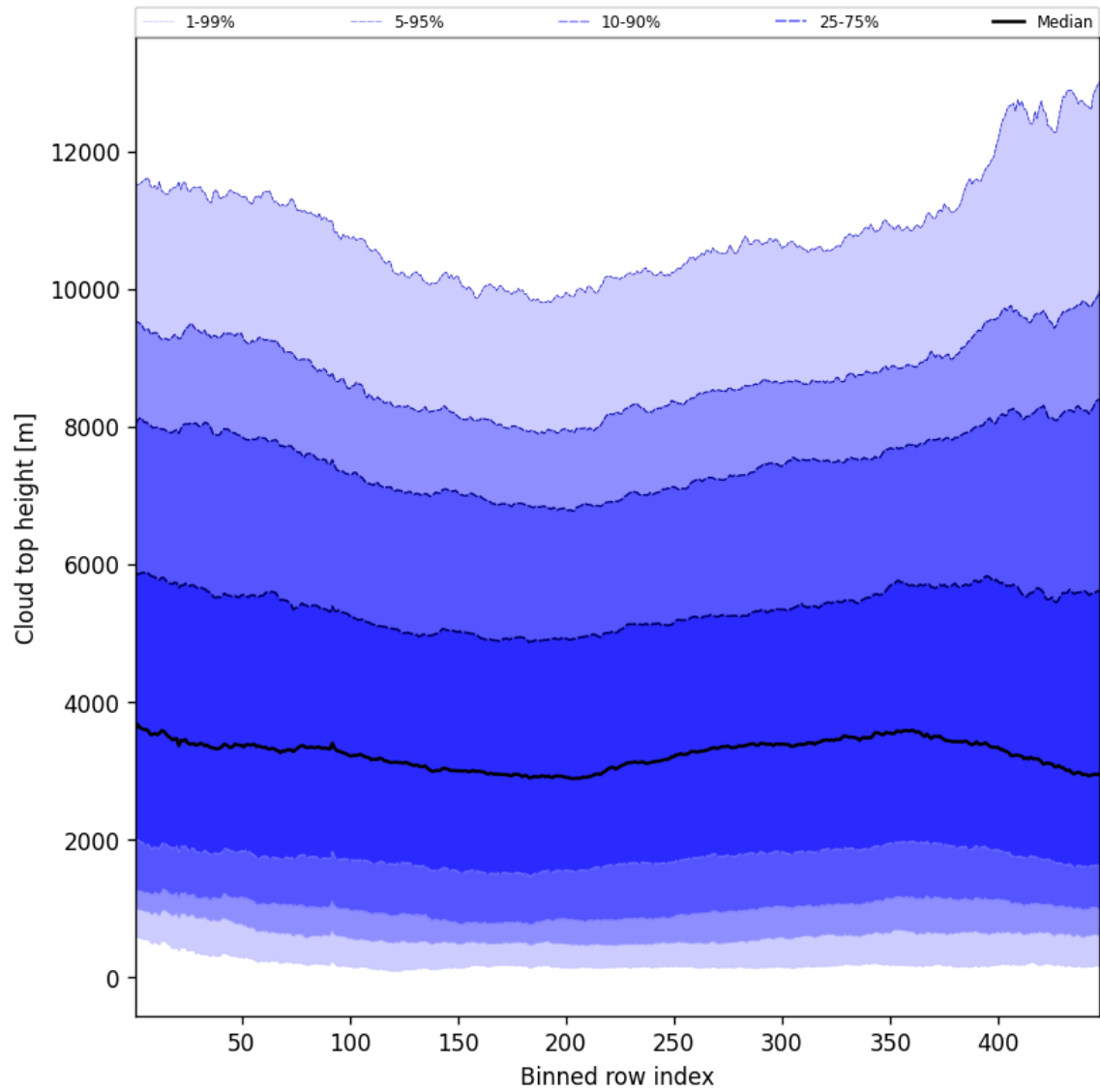
Figure 56: Along track statistics of “Cloud top height” for 2025-07-04 to 2025-07-06
