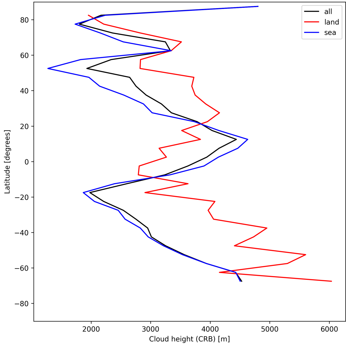
Figure 27: Zonal average of “Cloud height (CRB)” for 2025-07-04 to 2025-07-06.
