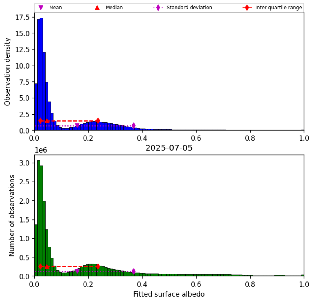
Figure 45: Histogram of “Fitted surface albedo” for 2025-07-04 to 2025-07-06
