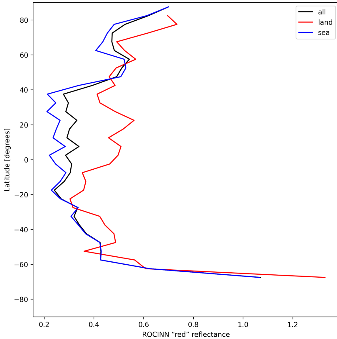
Figure 37: Zonal average of “ROCINN “red” reflectance” for 2025-07-04 to 2025-07-06.
