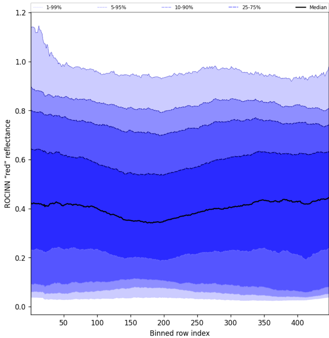
Figure 69: Along track statistics of "ROCINN "red" reflectance" for 2025-07-04 to 2025-07-06
