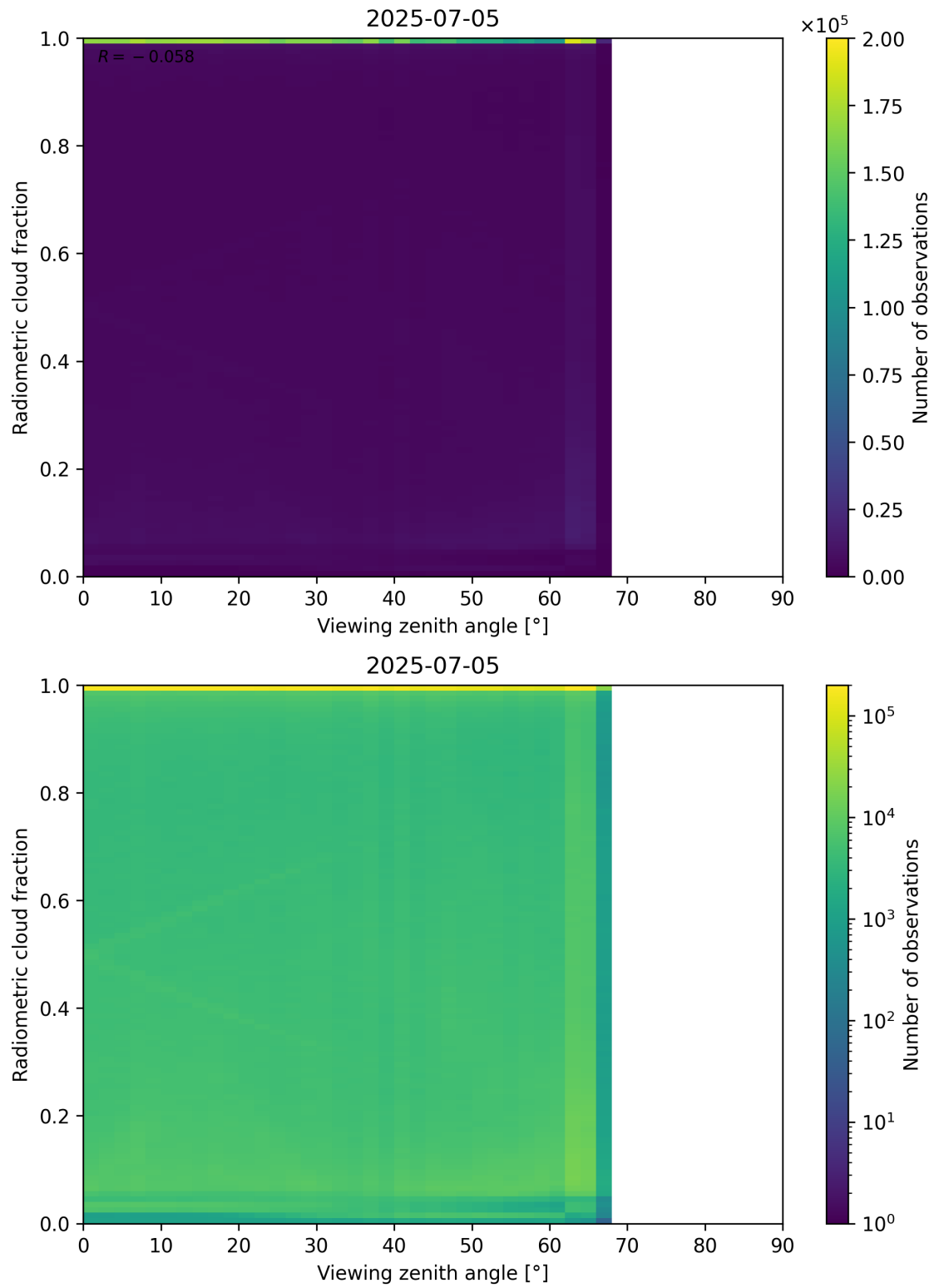
Figure 107: Scatter density plot of “Viewing zenith angle” against “Radiometric cloud fraction” for 2025-07-04 to 2025-07-06.
