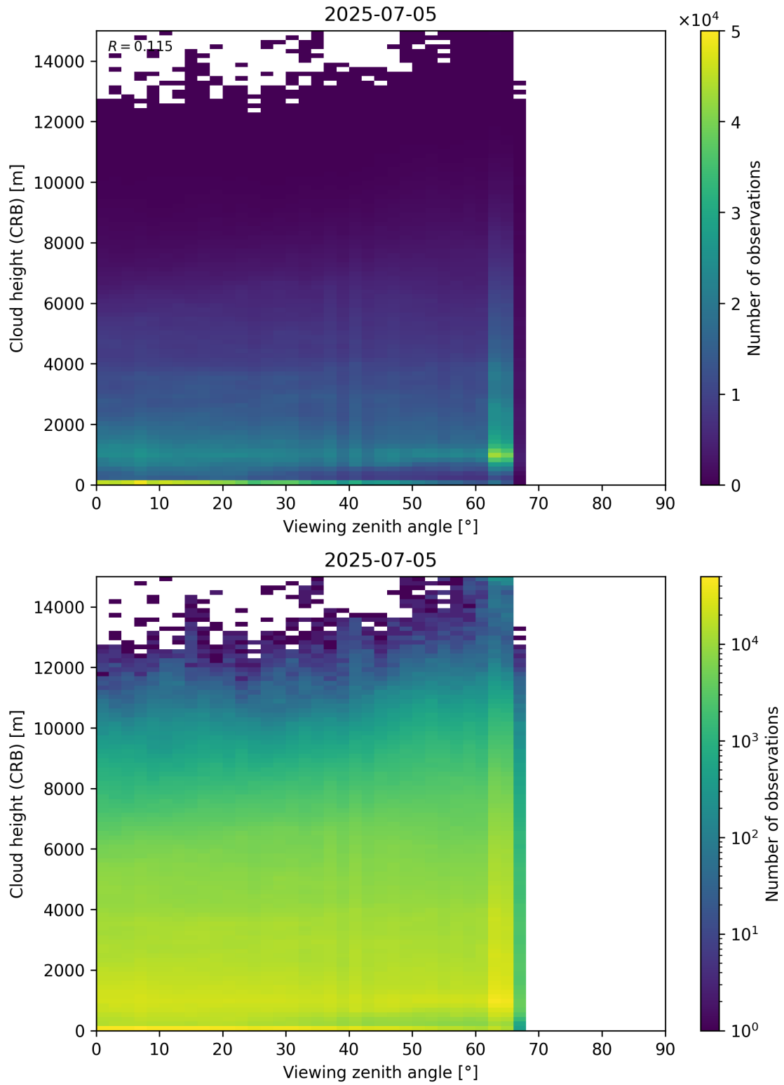
Figure 110: Scatter density plot of “Viewing zenith angle” against “Cloud height (CRB)” for 2025-07-04 to 2025-07-06.
