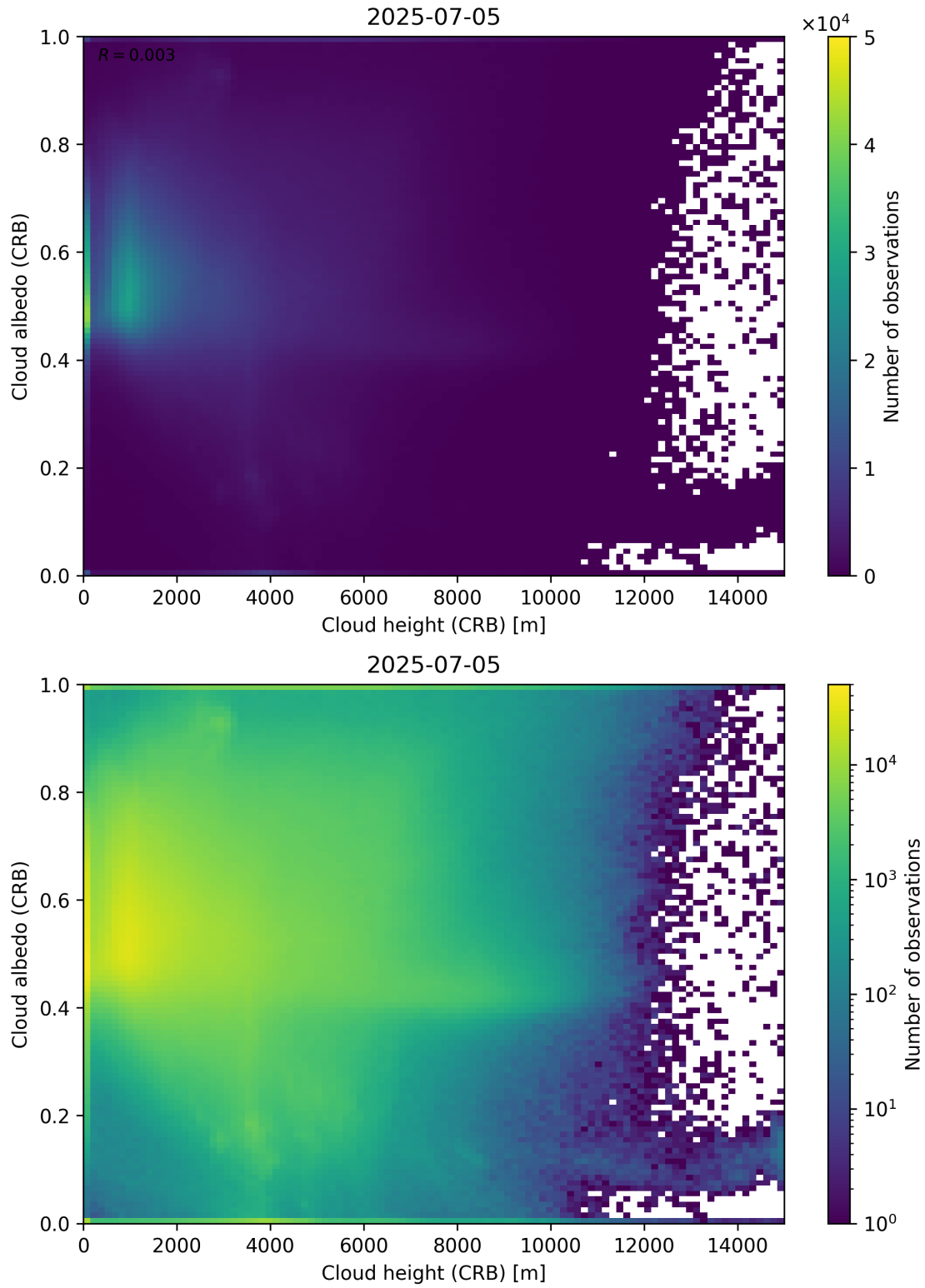
Figure 80: Scatter density plot of “Cloud height (CRB)” against “Cloud albedo (CRB)” for 2025-07-04 to 2025-07-06.
