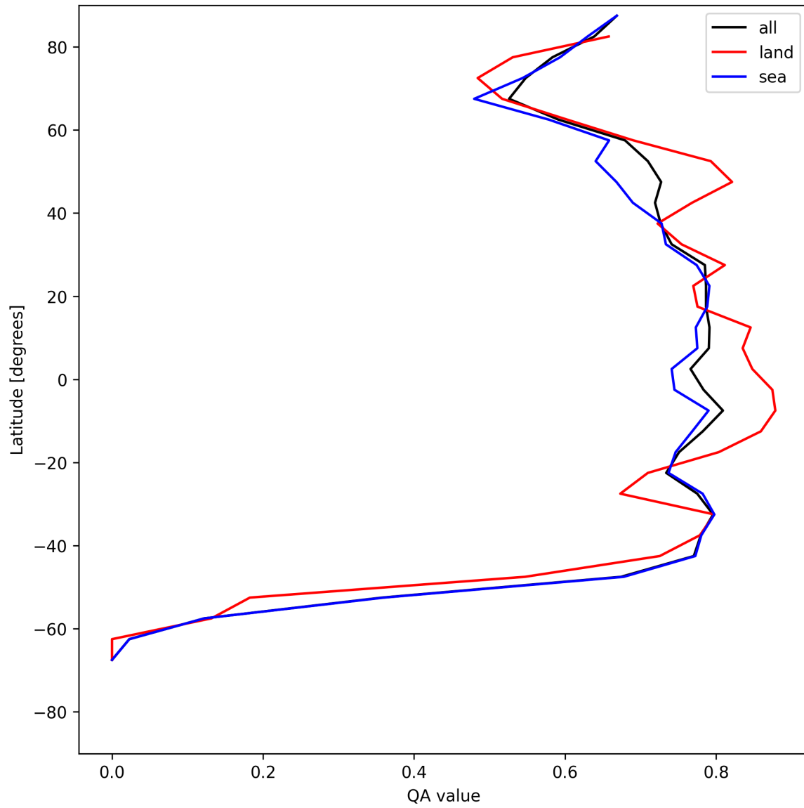
Figure 22: Zonal average of “QA value” for 2025-07-04 to 2025-07-06.
