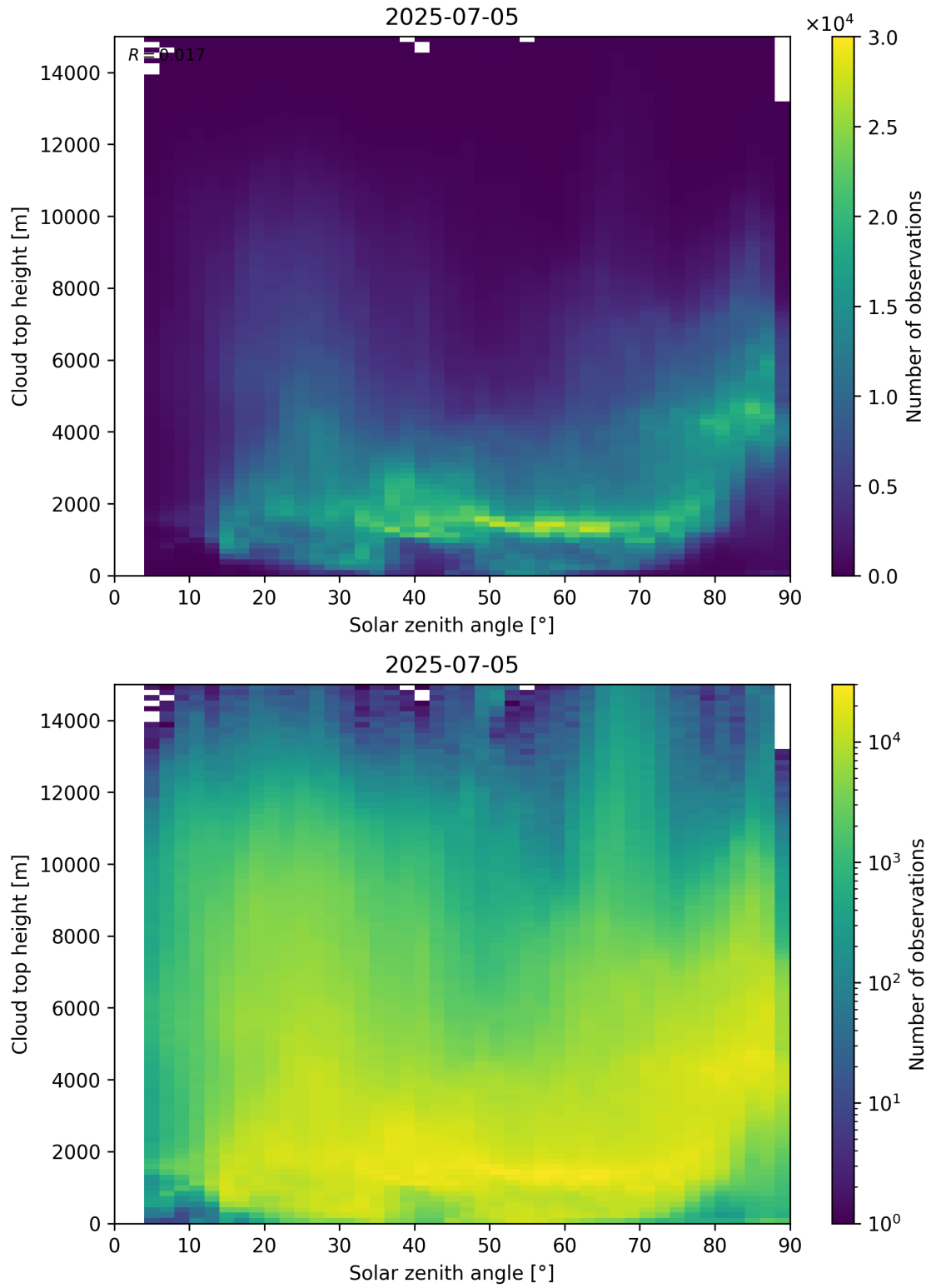
Figure 104: Scatter density plot of “Solar zenith angle” against “Cloud top height” for 2025-07-04 to 2025-07-06.
