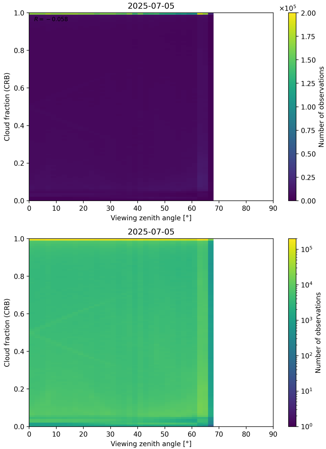
Figure 109: Scatter density plot of “Viewing zenith angle” against “Cloud fraction (CRB)” for 2025-07-04 to 2025-07-06.
