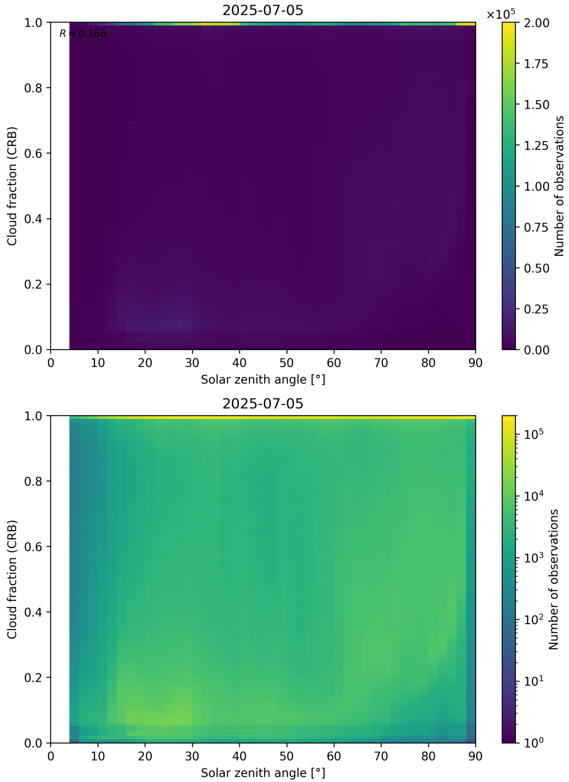
Figure 101: Scatter density plot of “Solar zenith angle” against “Cloud fraction (CRB)” for 2025-07-04 to 2025-07-06.
