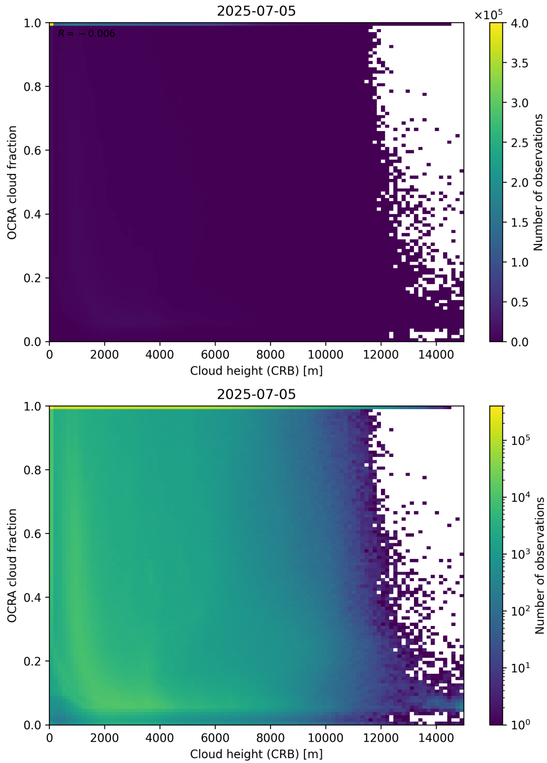
Figure 81: Scatter density plot of “Cloud height (CRB)” against “OCRA cloud fraction” for 2025-07-04 to 2025-07-06.
