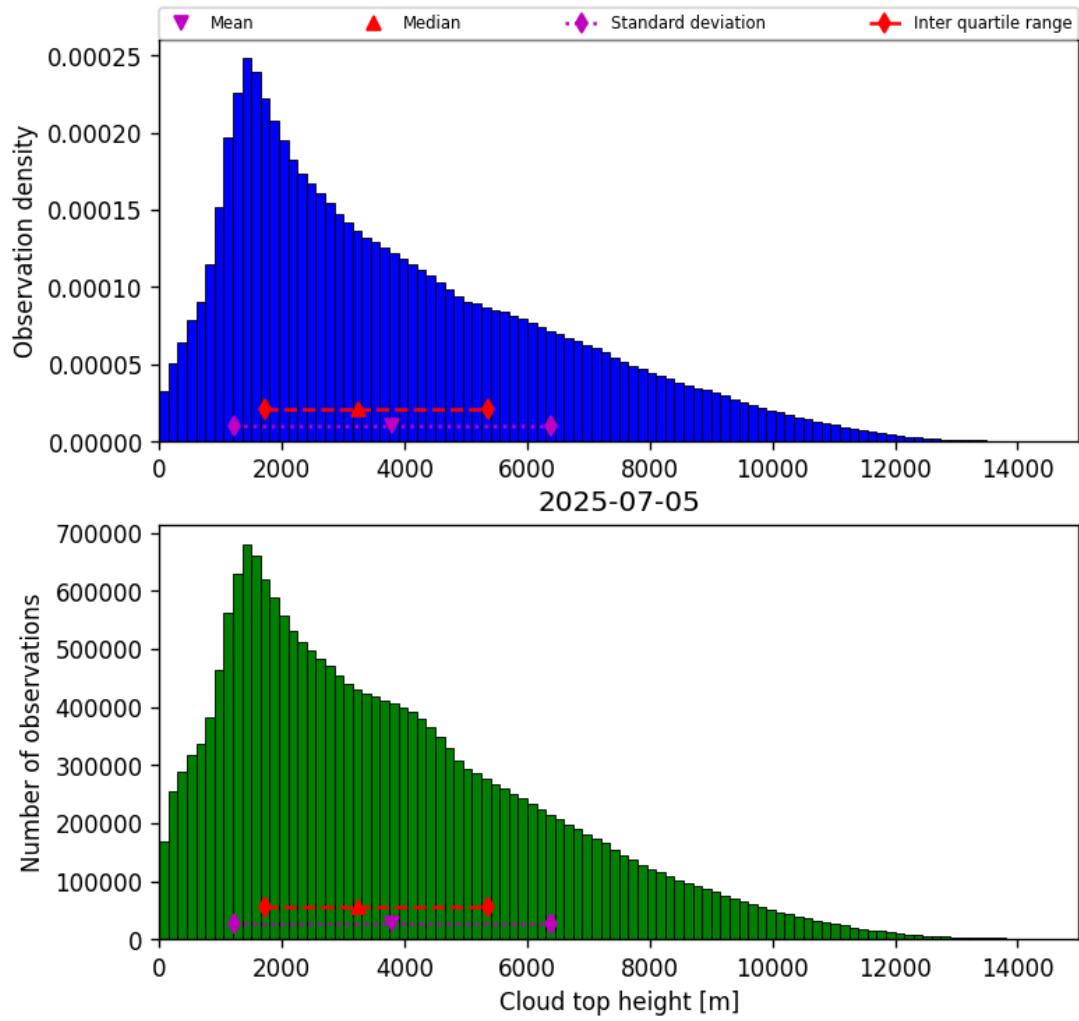
Figure 40: Histogram of “Cloud top height” for 2025-07-04 to 2025-07-06
