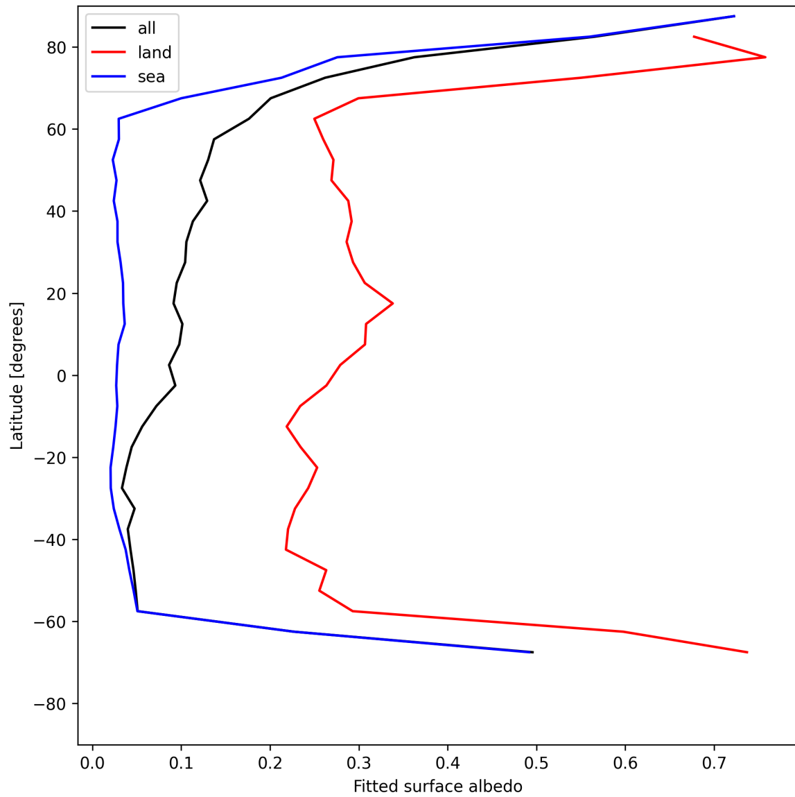
Figure 29: Zonal average of “Fitted surface albedo” for 2025-07-04 to 2025-07-06.
