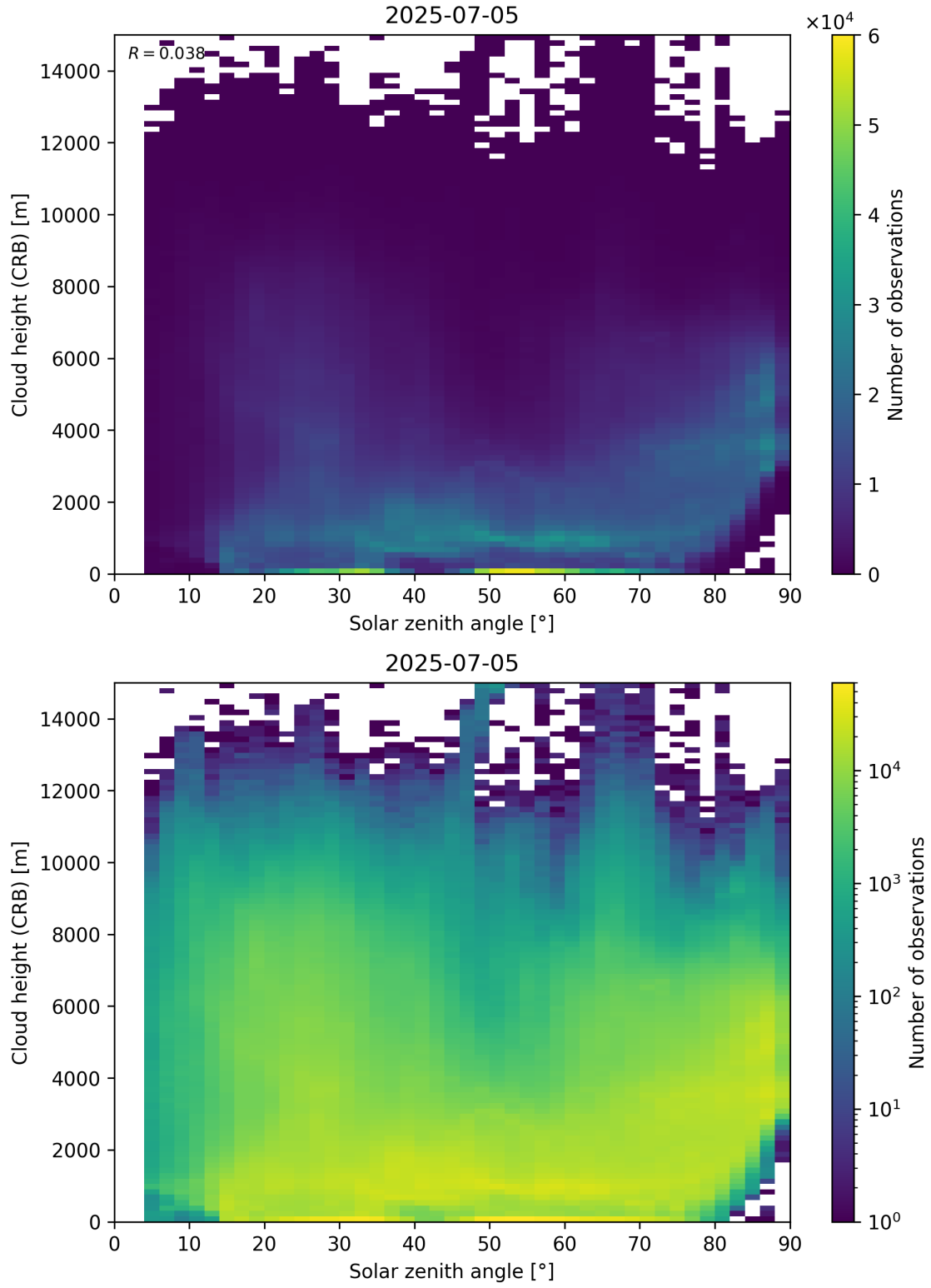
Figure 102: Scatter density plot of “Solar zenith angle” against “Cloud height (CRB)” for 2025-07-04 to 2025-07-06.
