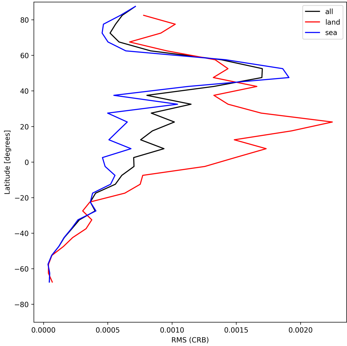
Figure 32: Zonal average of “RMS (CRB)” for 2025-07-04 to 2025-07-06.
