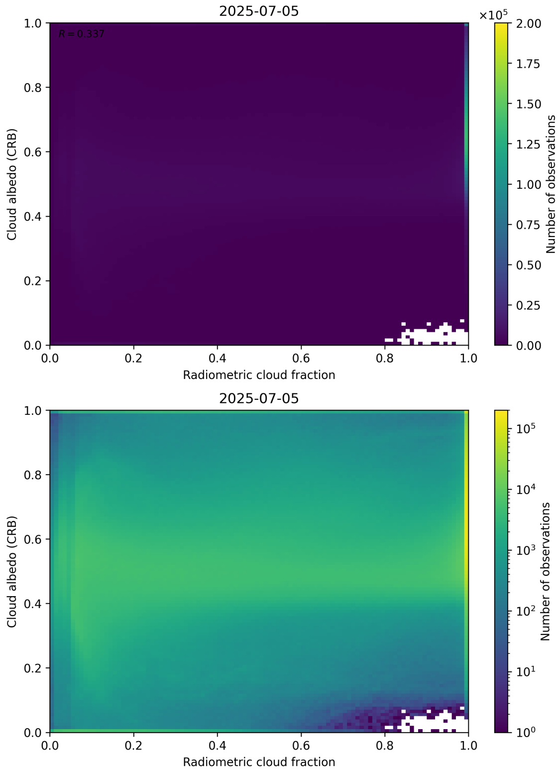
Figure 71: Scatter density plot of “Radiometric cloud fraction” against “Cloud albedo (CRB)” for 2025-07-04 to 2025-07-06.
