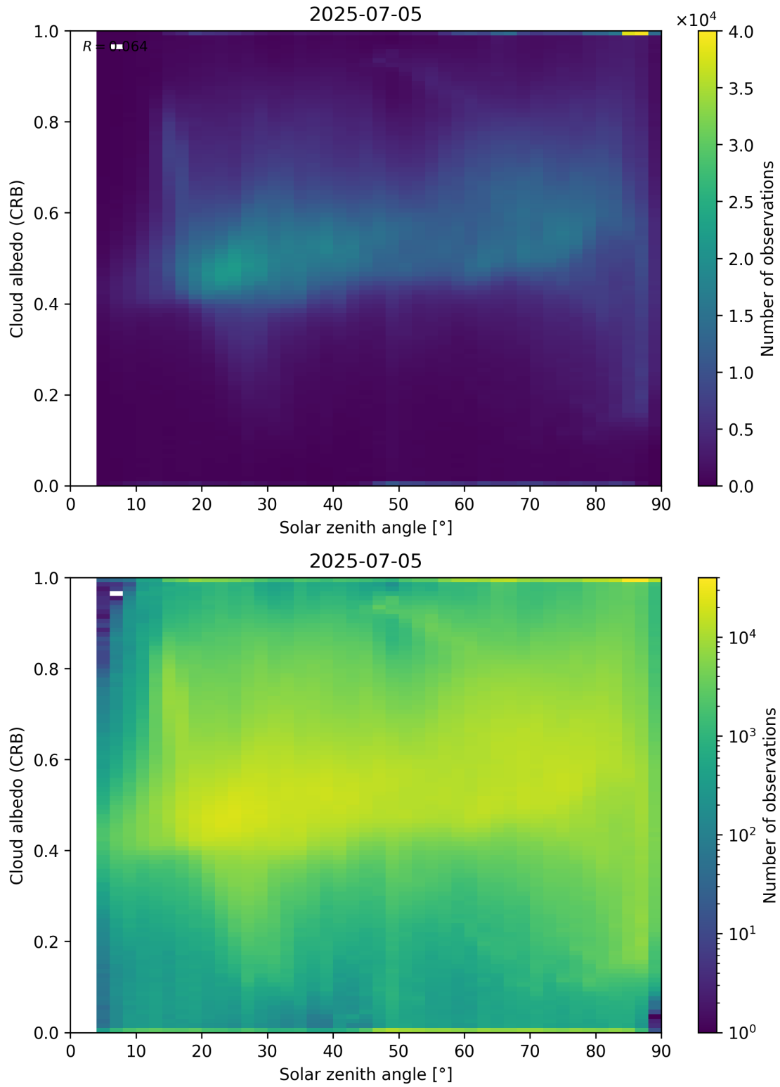
Figure 98: Scatter density plot of “Solar zenith angle” against “Cloud albedo (CRB)” for 2025-07-04 to 2025-07-06.
