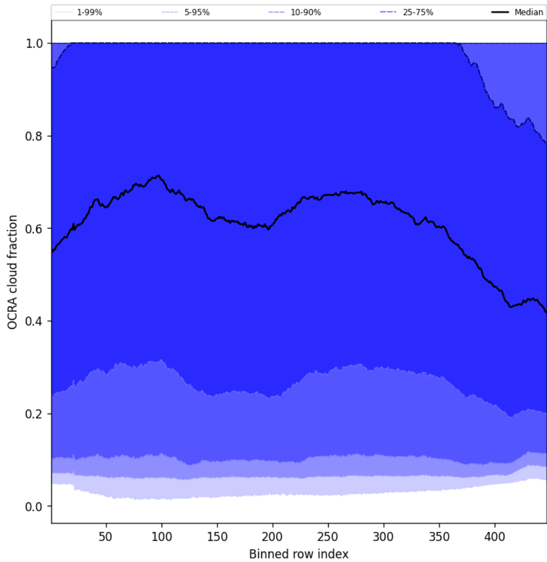
Figure 66: Along track statistics of “OCRA cloud fraction” for 2025-07-04 to 2025-07-06
