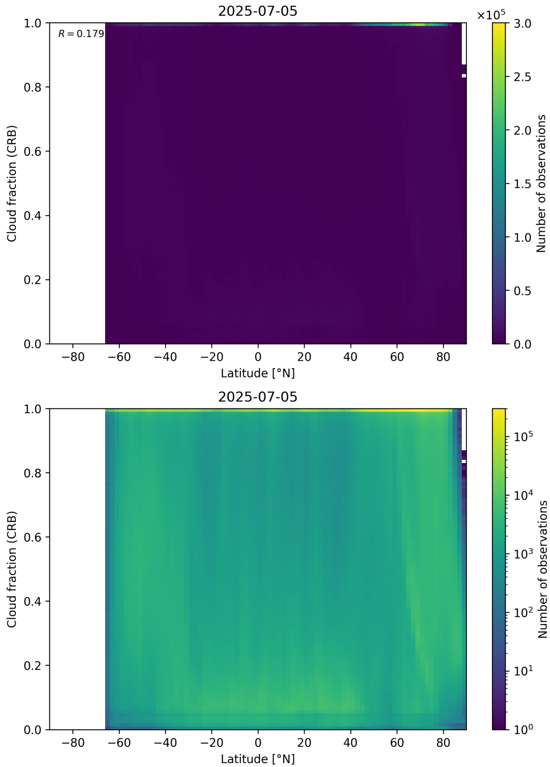
Figure 94: Scatter density plot of “Latitude” against “Cloud fraction (CRB)” for 2025-07-04 to 2025-07-06.
