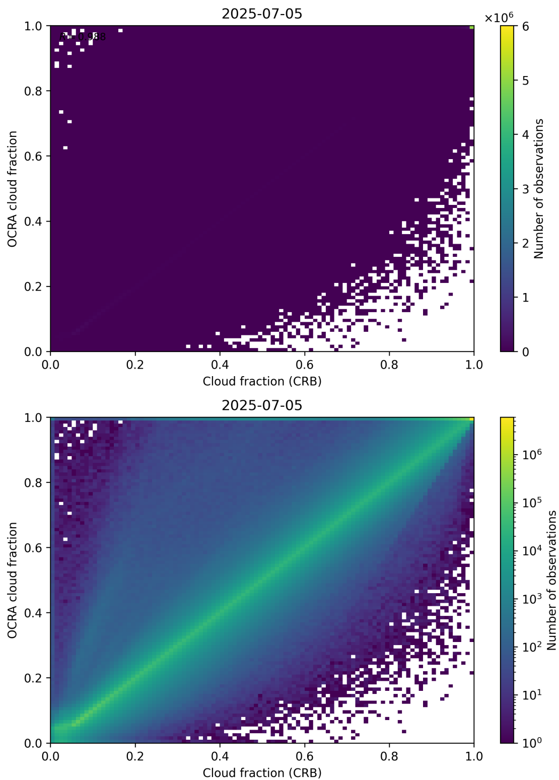
Figure 78: Scatter density plot of “Cloud fraction (CRB)” against “OCRA cloud fraction” for 2025-07-04 to 2025-07-06.
