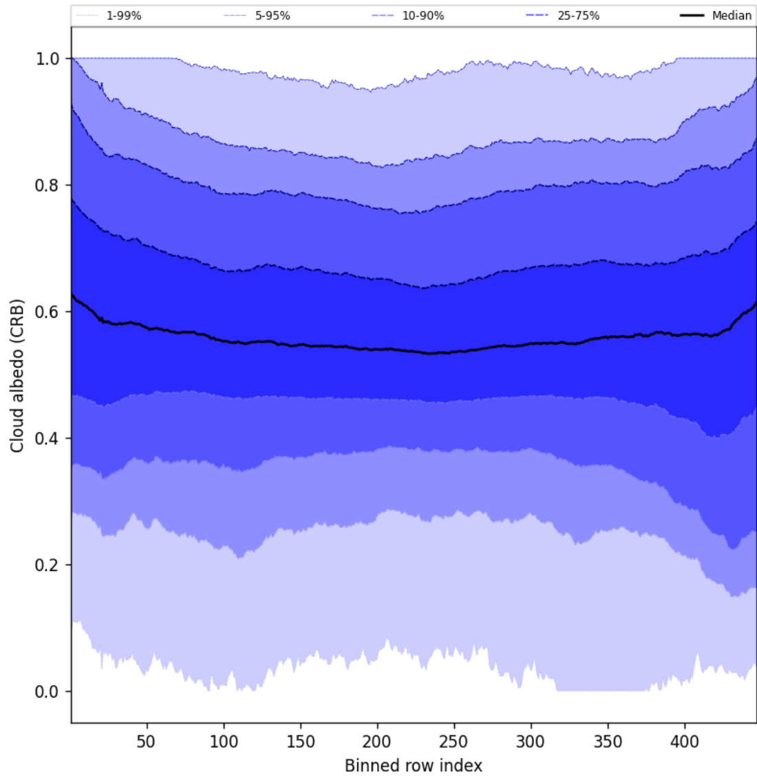
Figure 60: Along track statistics of “Cloud albedo (CRB)” for 2025-07-04 to 2025-07-06
