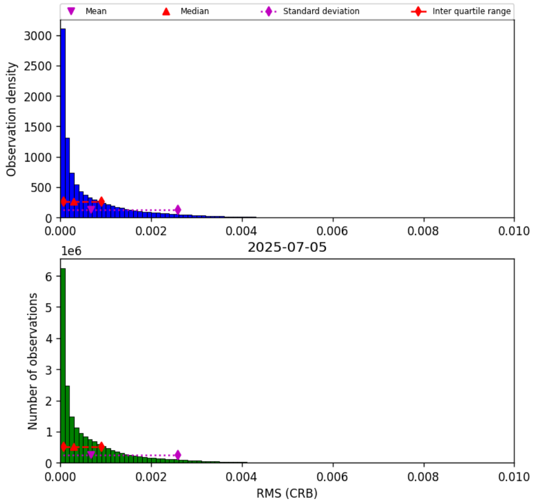
Figure 48: Histogram of “RMS (CRB)” for 2025-07-04 to 2025-07-06
