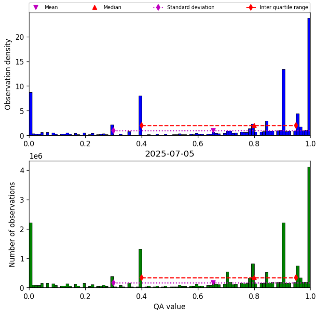
Figure 38: Histogram of “QA value” for 2025-07-04 to 2025-07-06
