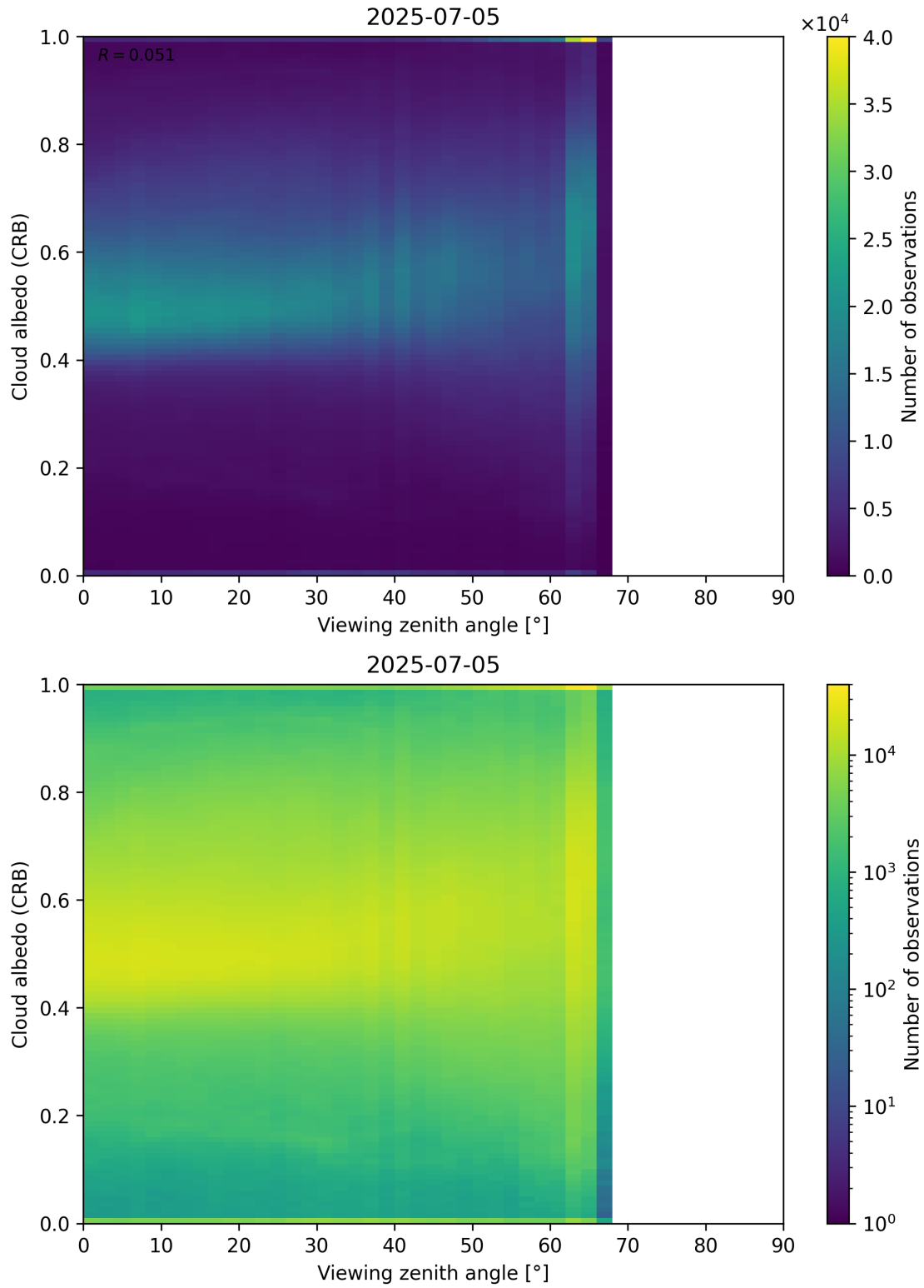
Figure 106: Scatter density plot of “Viewing zenith angle” against “Cloud albedo (CRB)” for 2025-07-04 to 2025-07-06.
