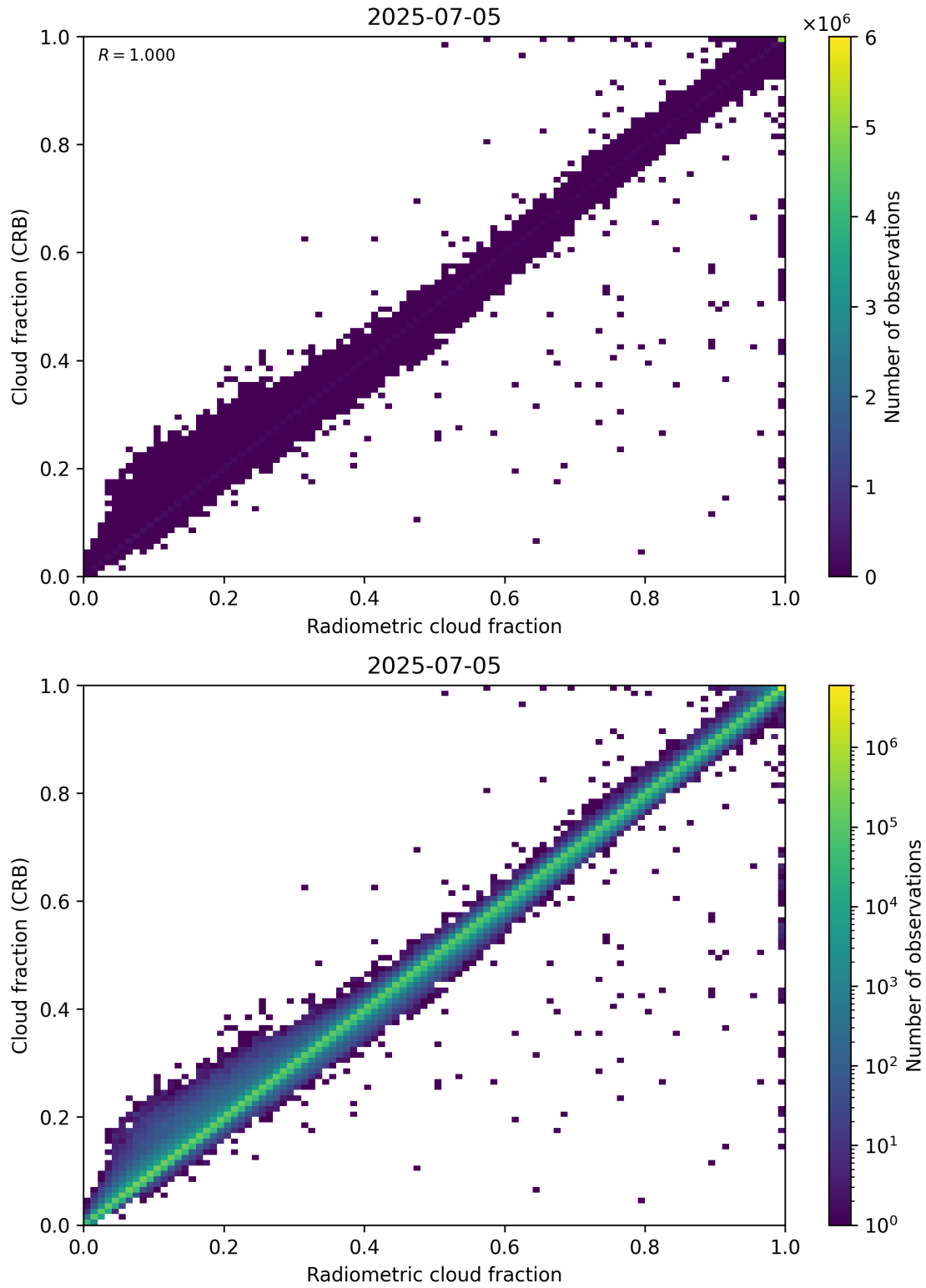
Figure 73: Scatter density plot of “Radiometric cloud fraction” against “Cloud fraction (CRB)” for 2025-07-04 to 2025-07-06.
