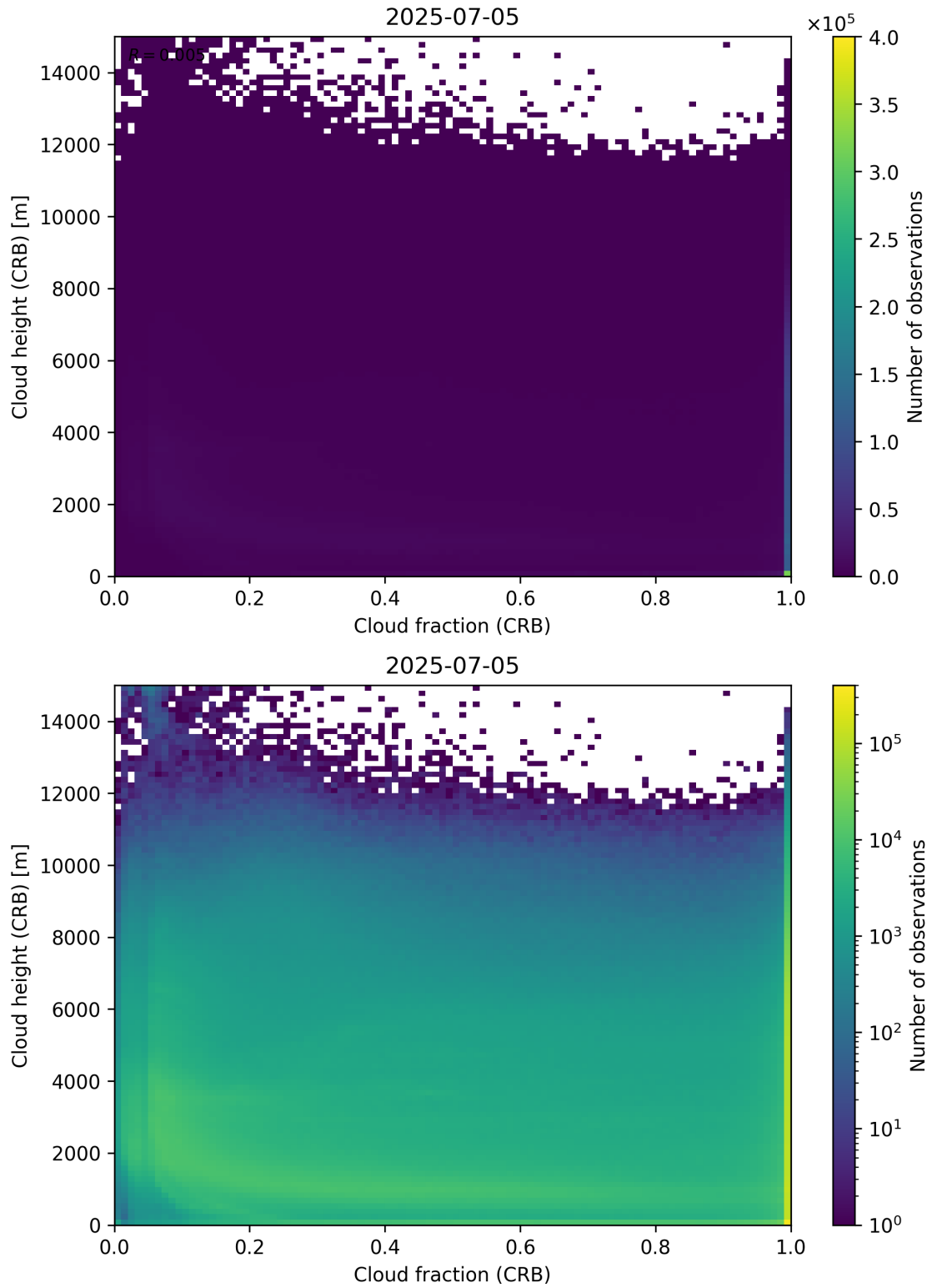
Figure 79: Scatter density plot of “Cloud fraction (CRB)” against “Cloud height (CRB)” for 2025-07-04 to 2025-07-06.
