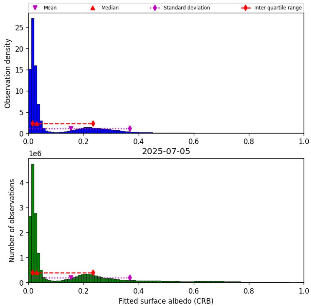
Figure 46: Histogram of “Fitted surface albedo (CRB)” for 2025-07-04 to 2025-07-06
