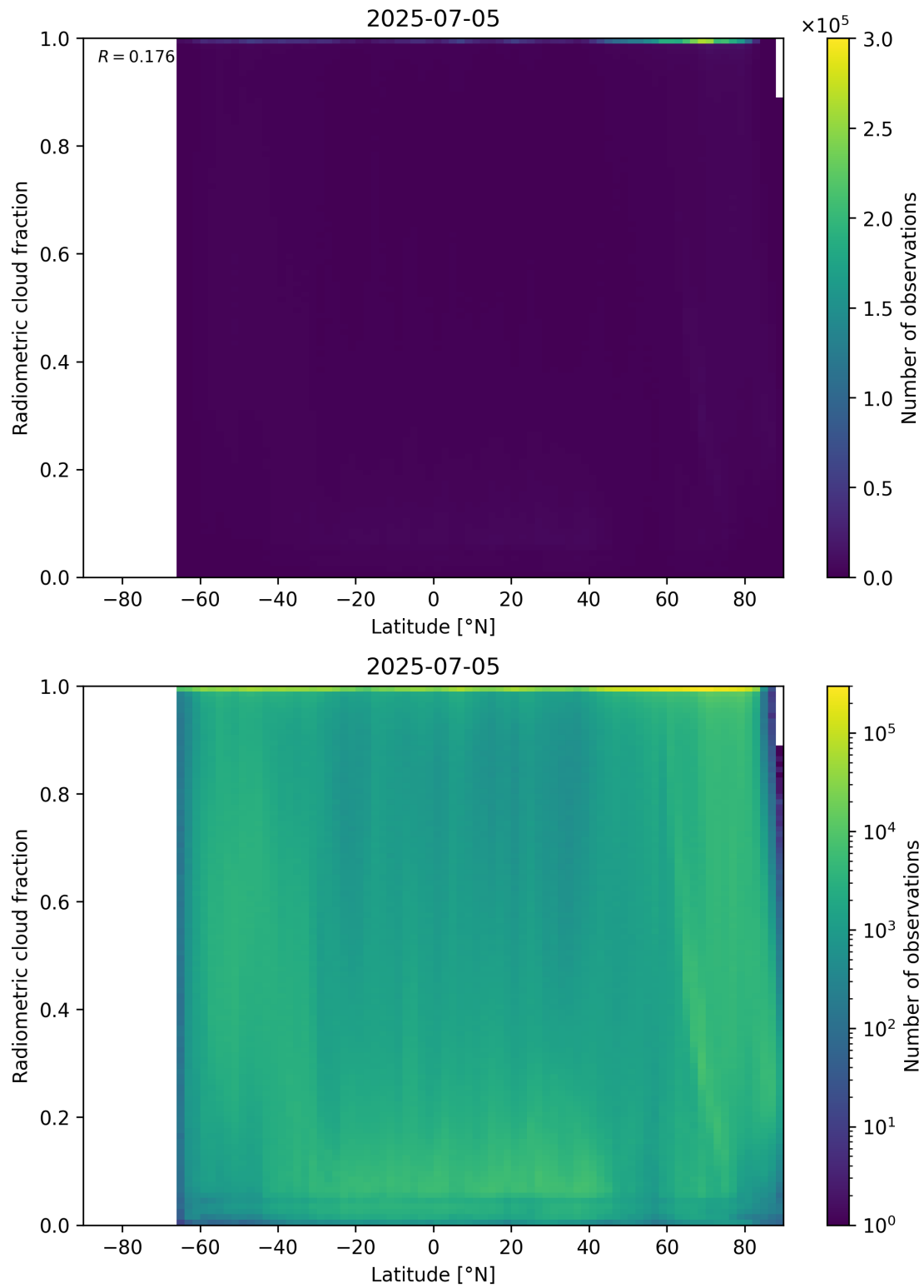
Figure 92: Scatter density plot of “Latitude” against “Radiometric cloud fraction” for 2025-07-04 to 2025-07-06.
