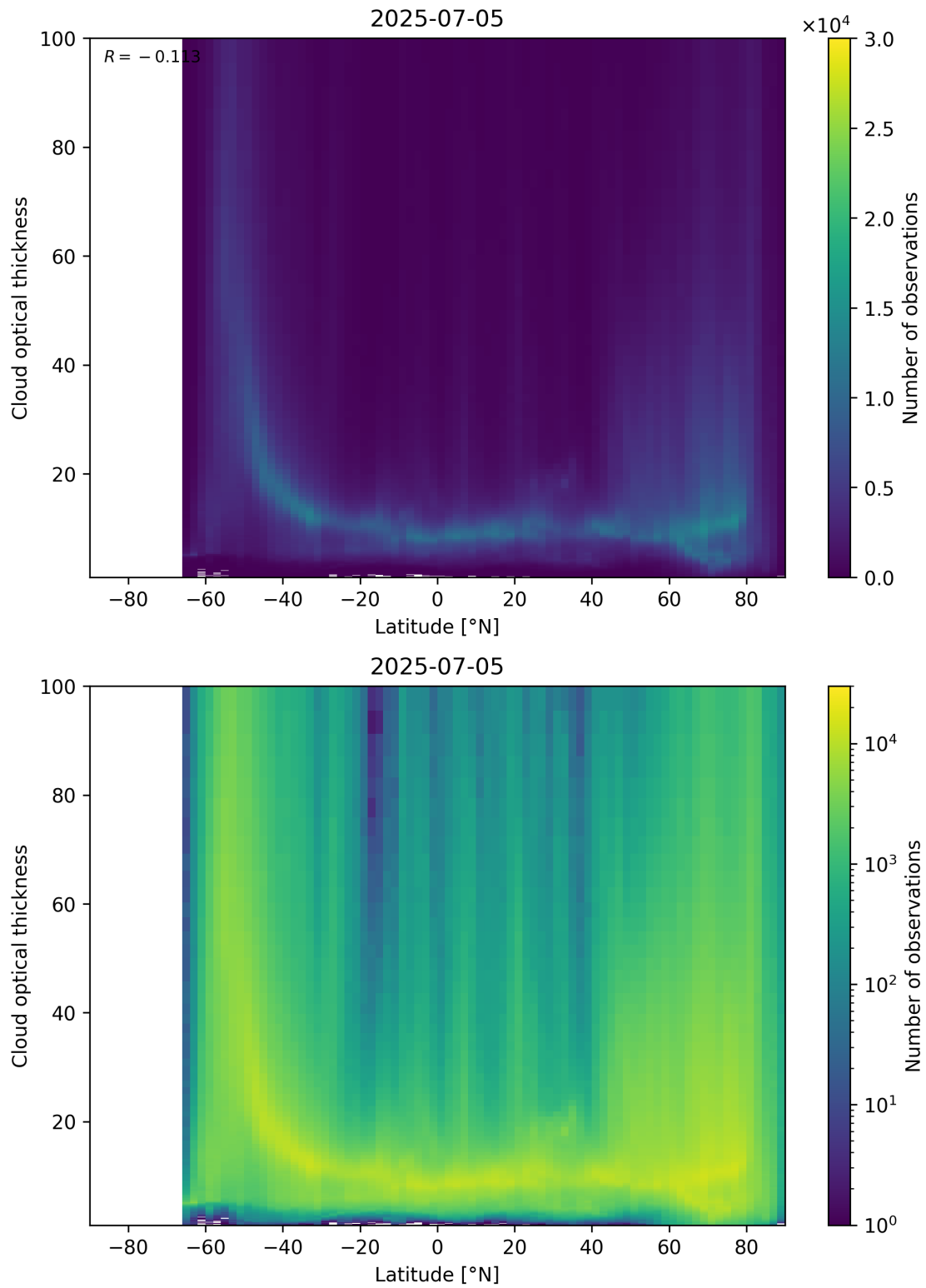
Figure 96: Scatter density plot of “Latitude” against “Cloud optical thickness” for 2025-07-04 to 2025-07-06.
