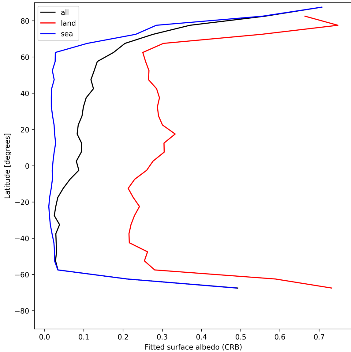
Figure 30: Zonal average of “Fitted surface albedo (CRB)” for 2025-07-04 to 2025-07-06.
