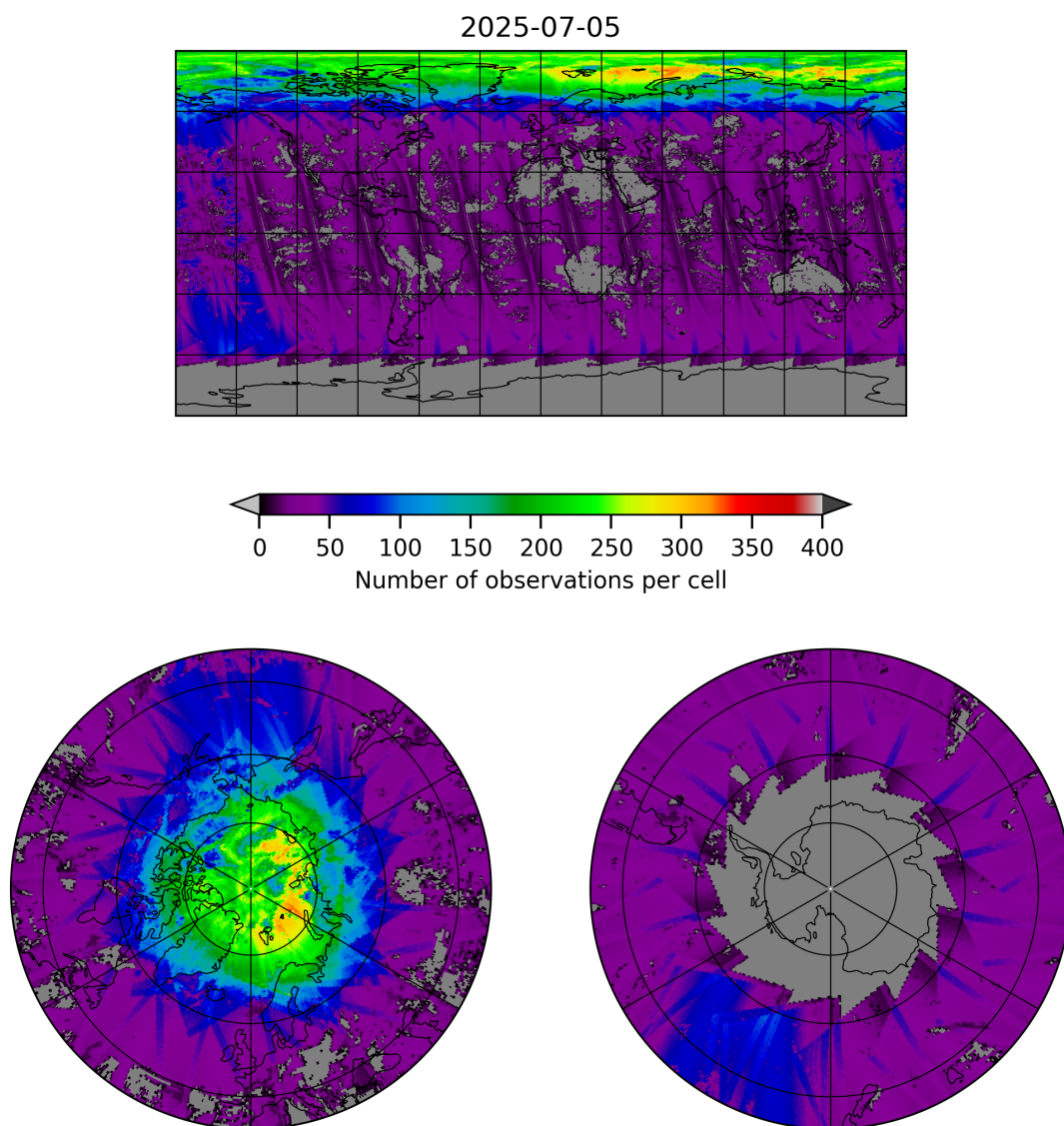
Figure 21: Map of the number of observations for 2025-07-04 to 2025-07-06
