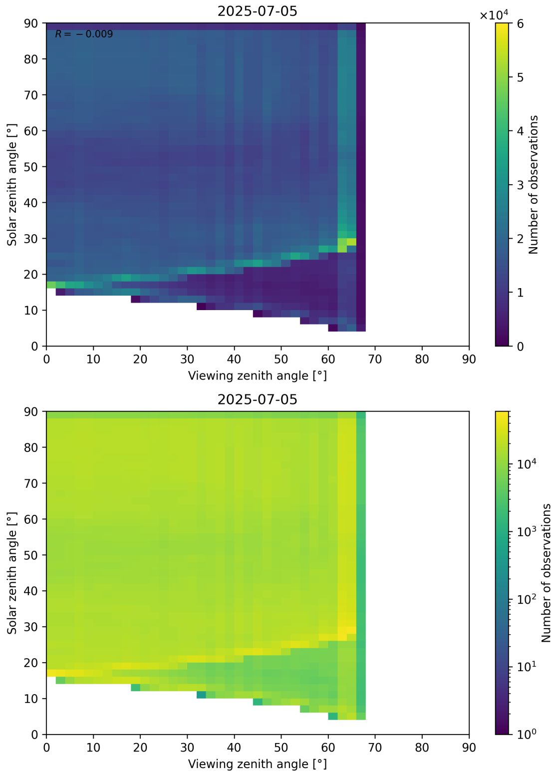
Figure 114: Scatter density plot of “Viewing zenith angle” against “Solar zenith angle” for 2025-07-04 to 2025-07-06.
