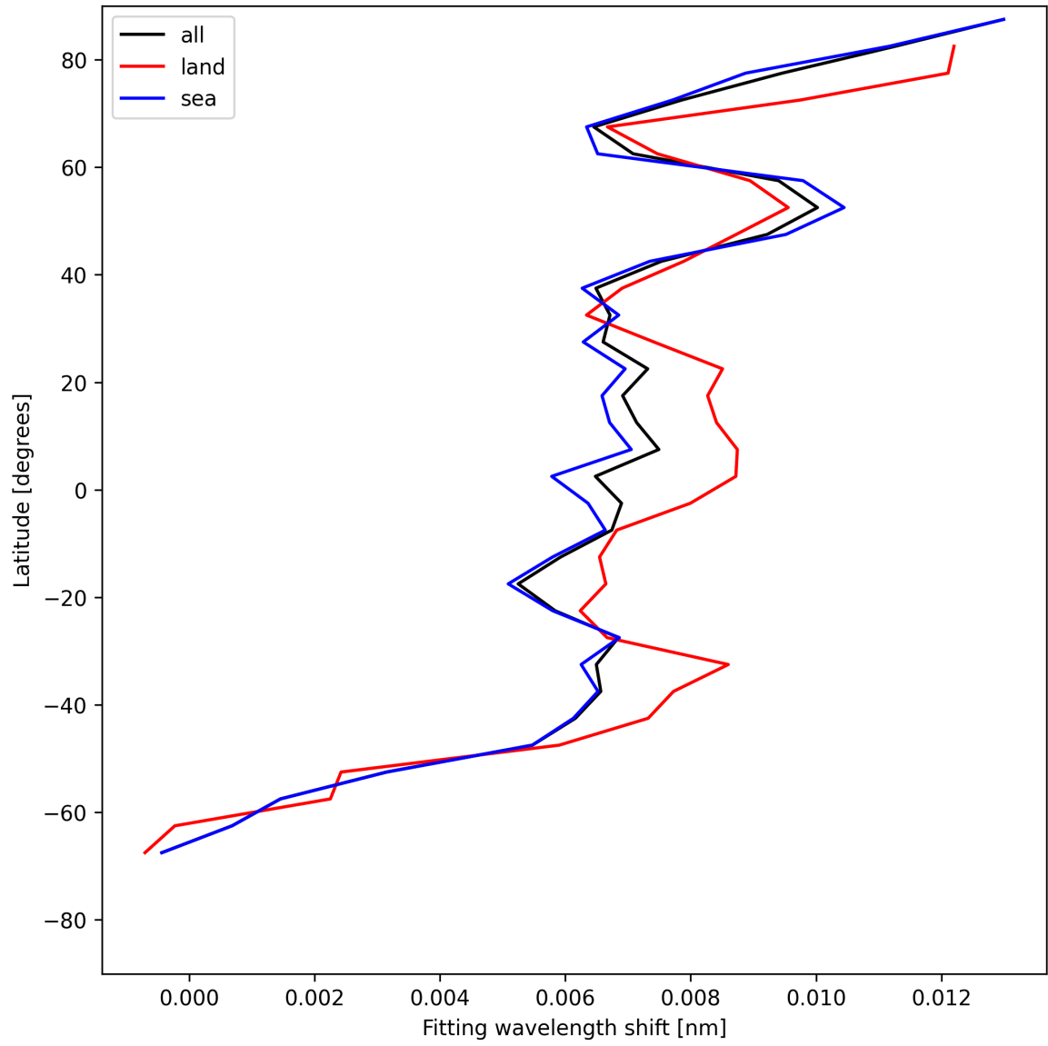
Figure 33: Zonal average of “Fitting wavelength shift” for 2025-07-04 to 2025-07-06.
