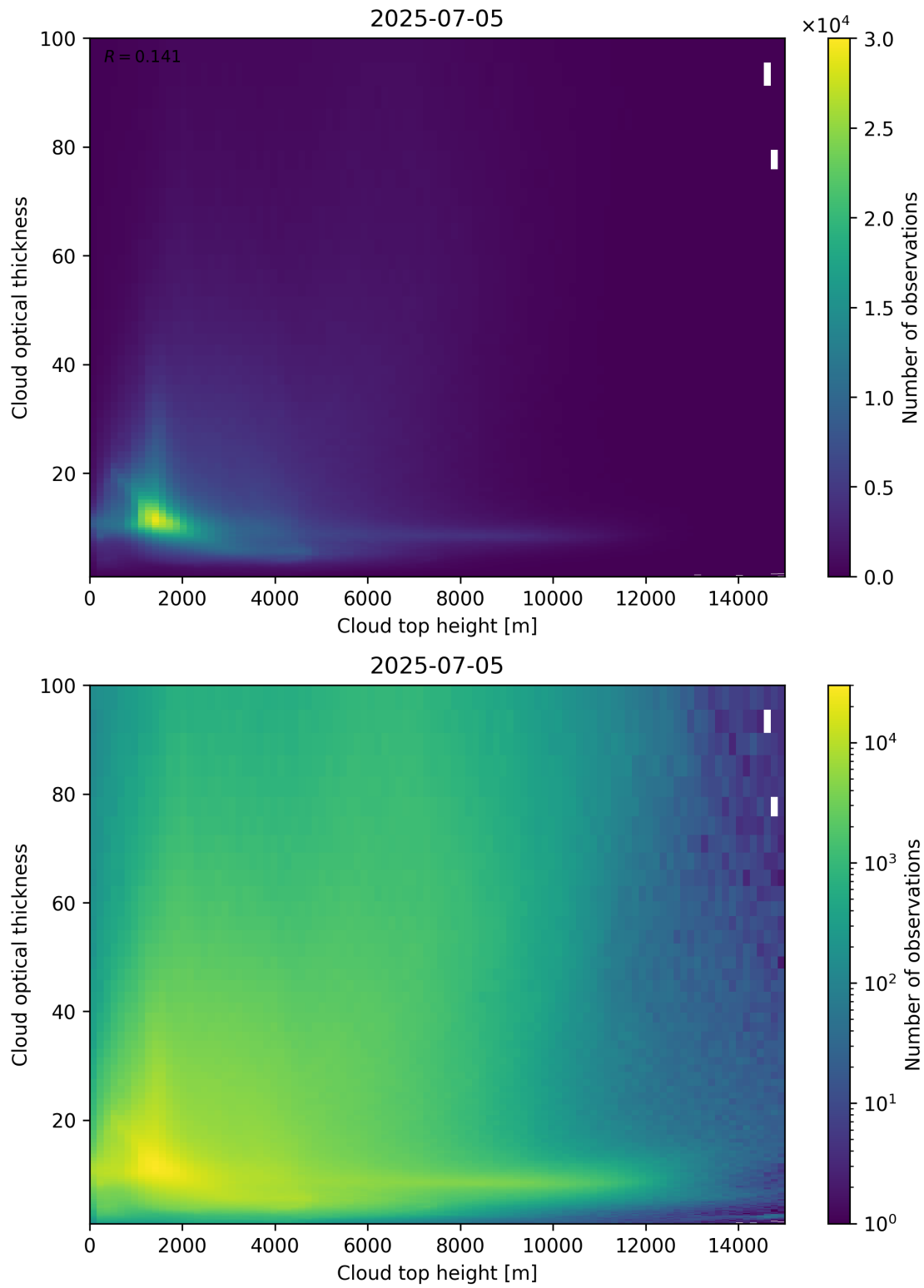
Figure 90: Scatter density plot of “Cloud top height” against “Cloud optical thickness” for 2025-07-04 to 2025-07-06.
