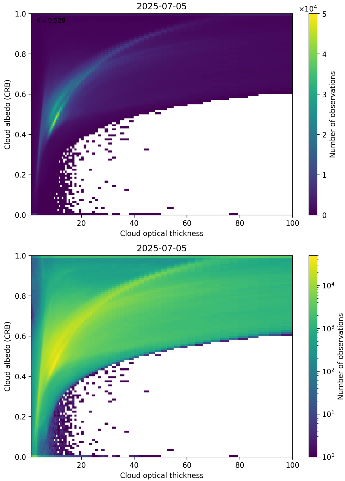
Figure 82: Scatter density plot of “Cloud optical thickness” against “Cloud albedo (CRB)” for 2025-07-04 to 2025-07-06.
