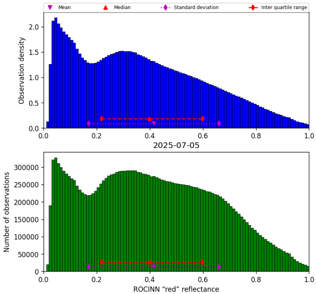
Figure 53: Histogram of “ROCINN “red” reflectance” for 2025-07-04 to 2025-07-06
