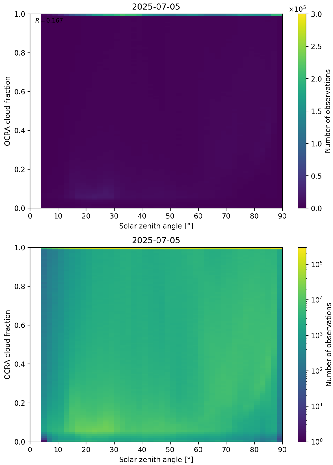
Figure 100: Scatter density plot of “Solar zenith angle” against “OCRA cloud fraction” for 2025-07-04 to 2025-07-06.
