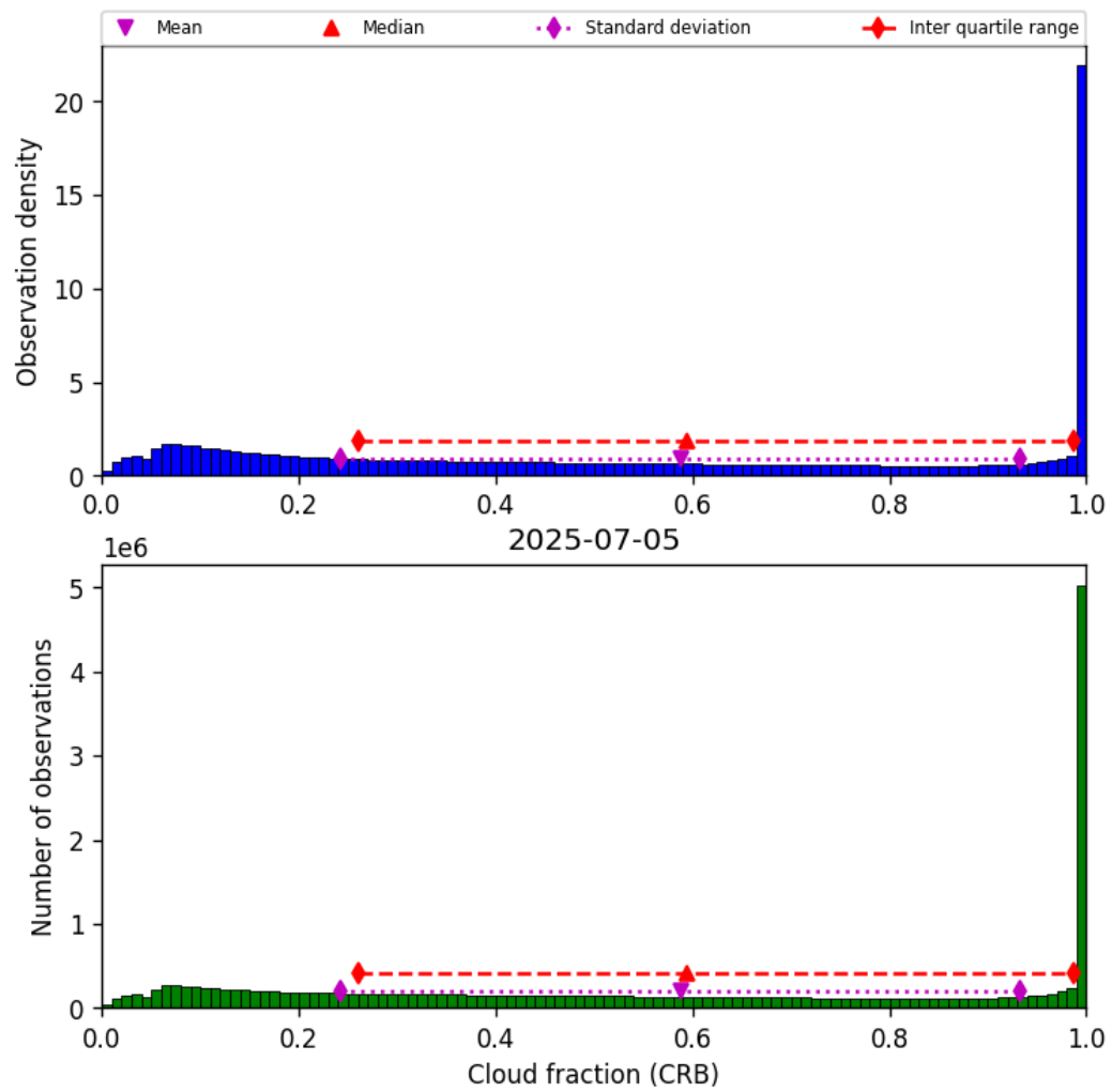
Figure 42: Histogram of “Cloud fraction (CRB)” for 2025-07-04 to 2025-07-06
