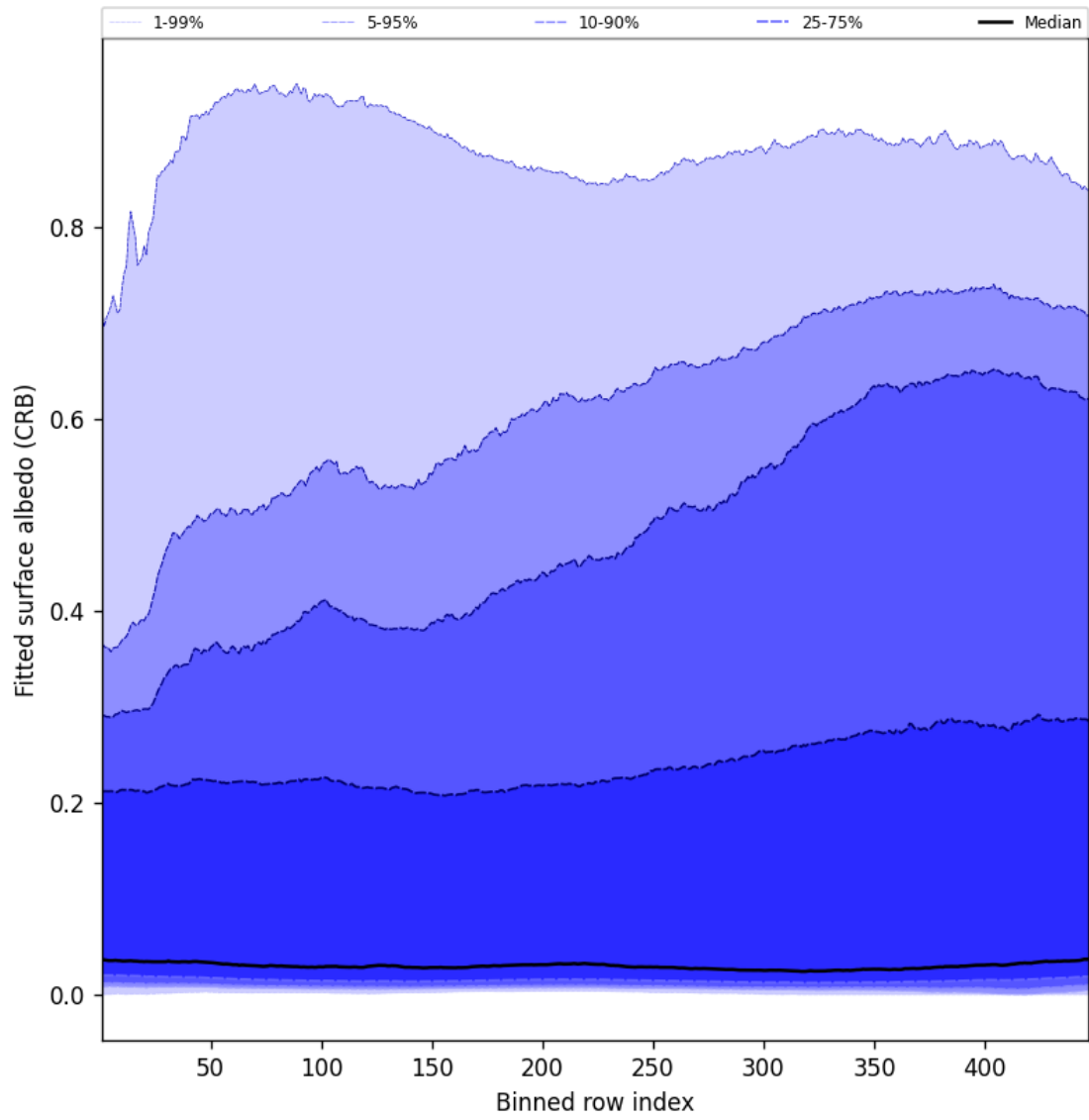
Figure 62: Along track statistics of “Fitted surface albedo (CRB)” for 2025-07-04 to 2025-07-06
