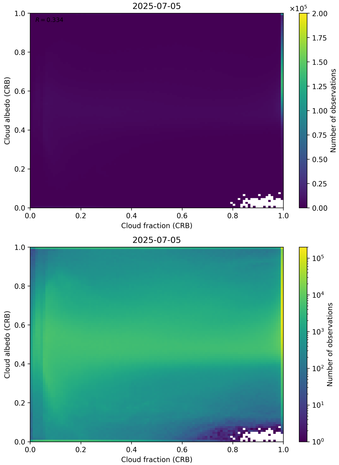
Figure 77: Scatter density plot of “Cloud fraction (CRB)” against “Cloud albedo (CRB)” for 2025-07-04 to 2025-07-06.
