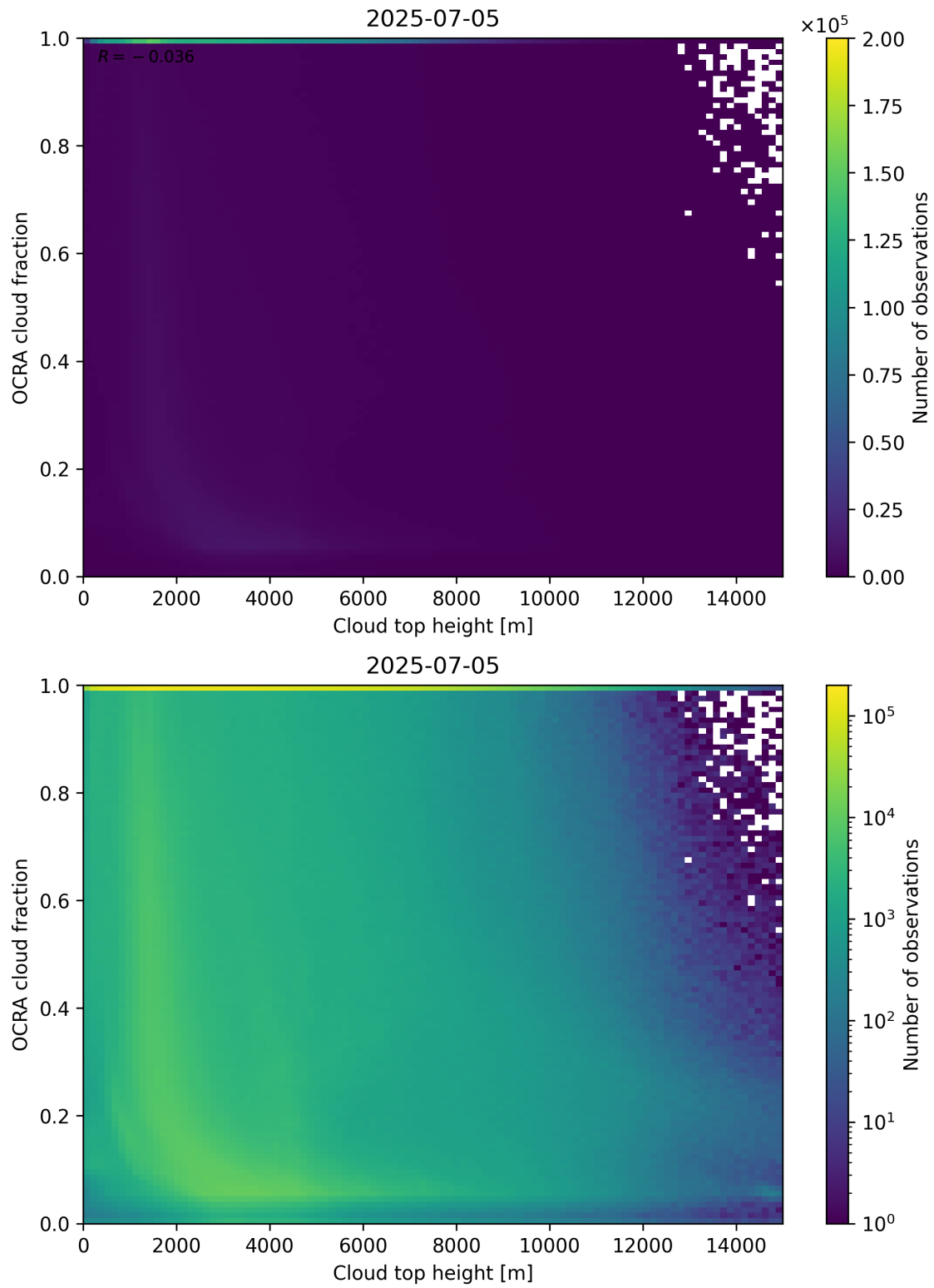
Figure 87: Scatter density plot of “Cloud top height” against “OCRA cloud fraction” for 2025-07-04 to 2025-07-06.
