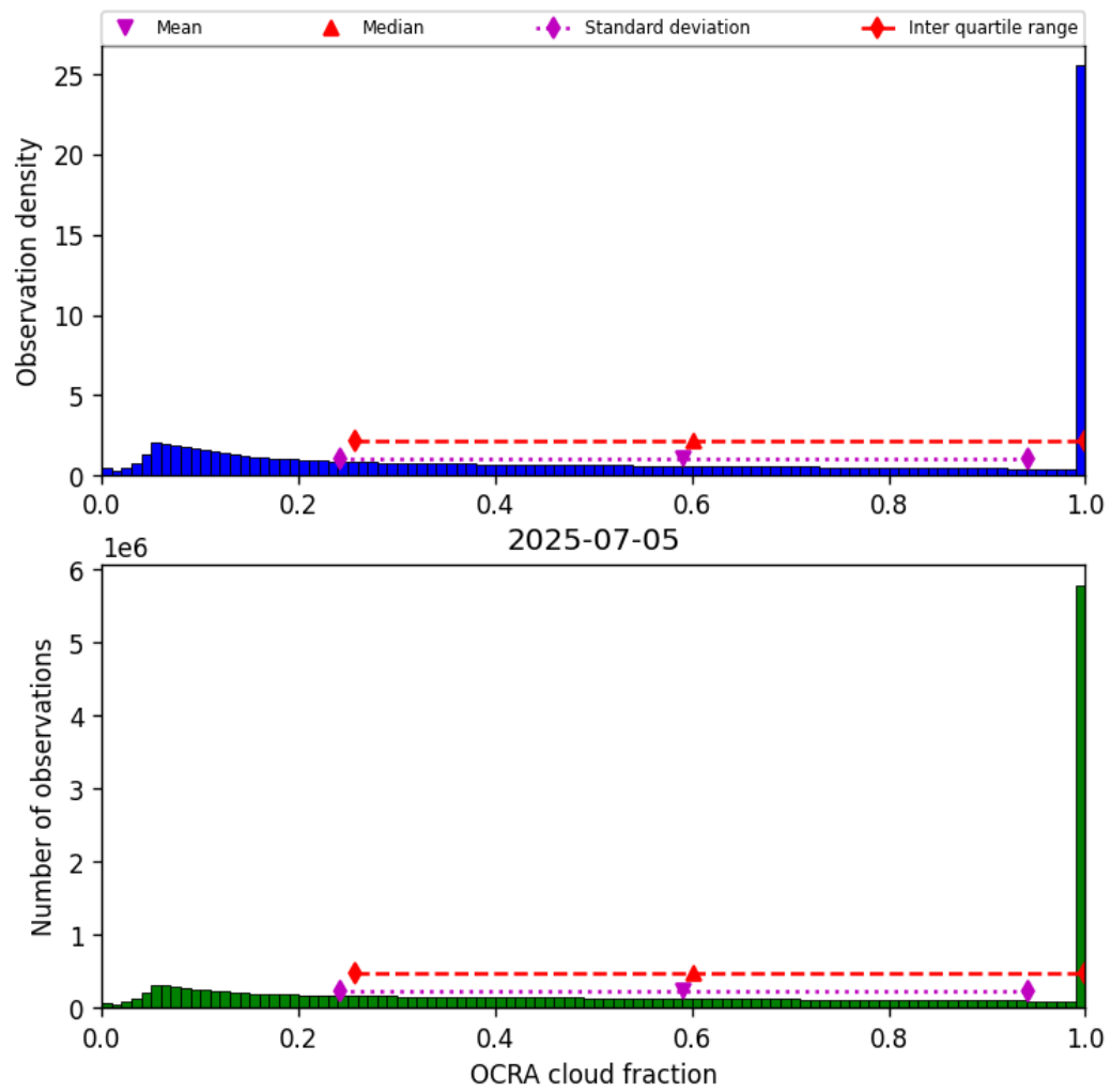
Figure 50: Histogram of “OCRA cloud fraction” for 2025-07-04 to 2025-07-06
