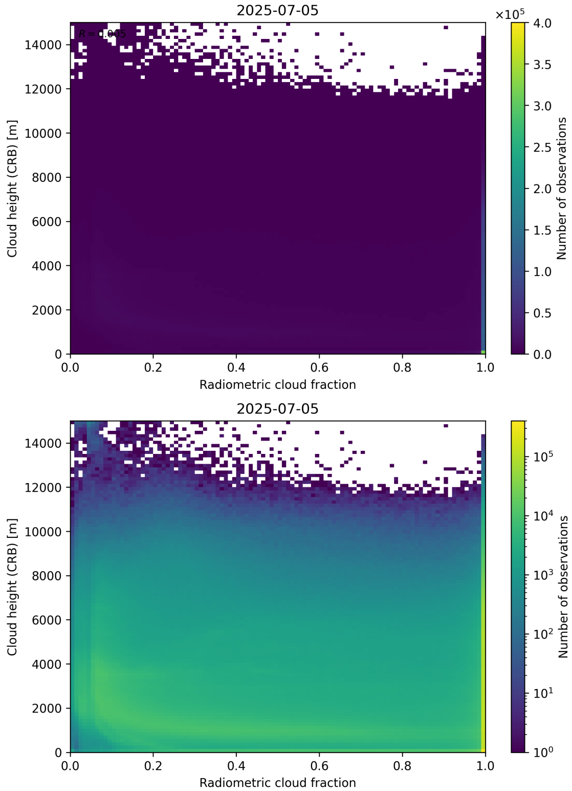
Figure 74: Scatter density plot of “Radiometric cloud fraction” against “Cloud height (CRB)” for 2025-07-04 to 2025-07-06.
