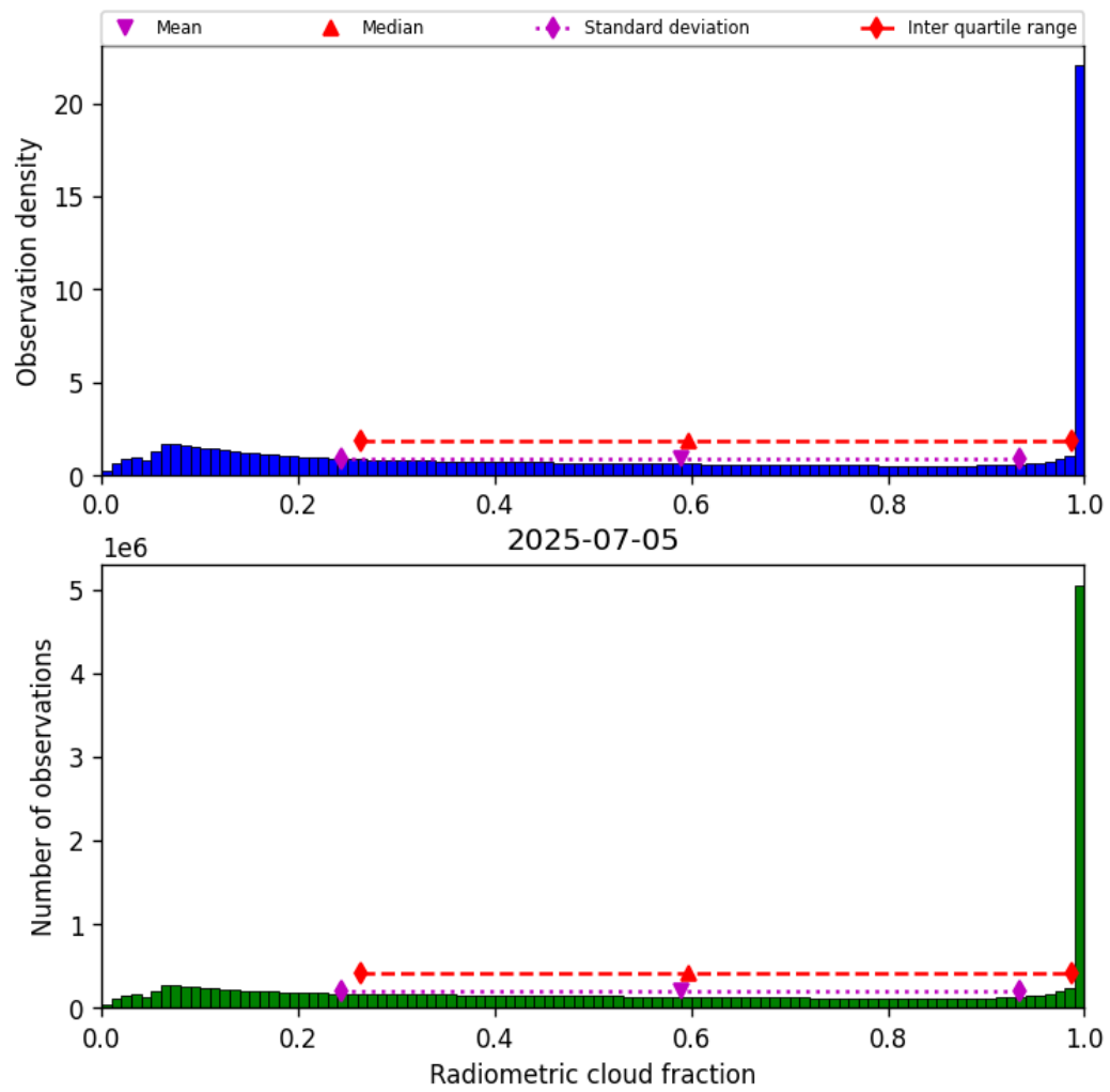
Figure 39: Histogram of “Radiometric cloud fraction” for 2025-07-04 to 2025-07-06
