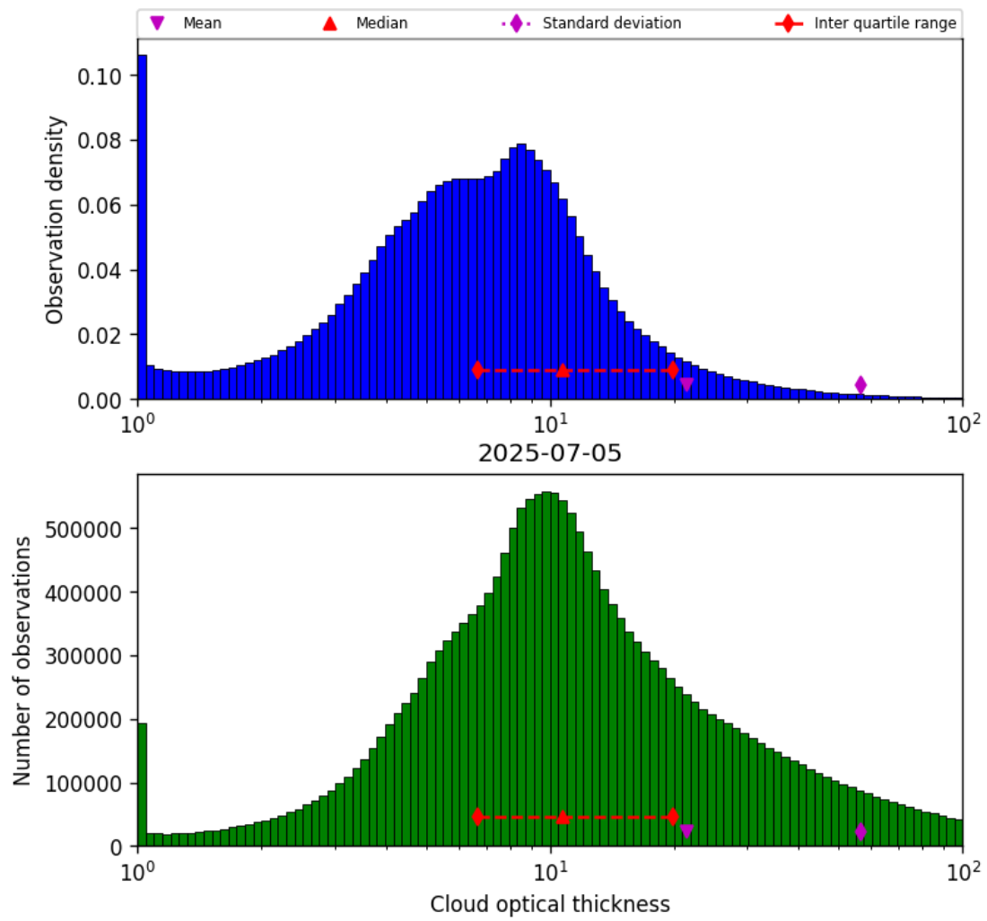
Figure 41: Histogram of “Cloud optical thickness” for 2025-07-04 to 2025-07-06
