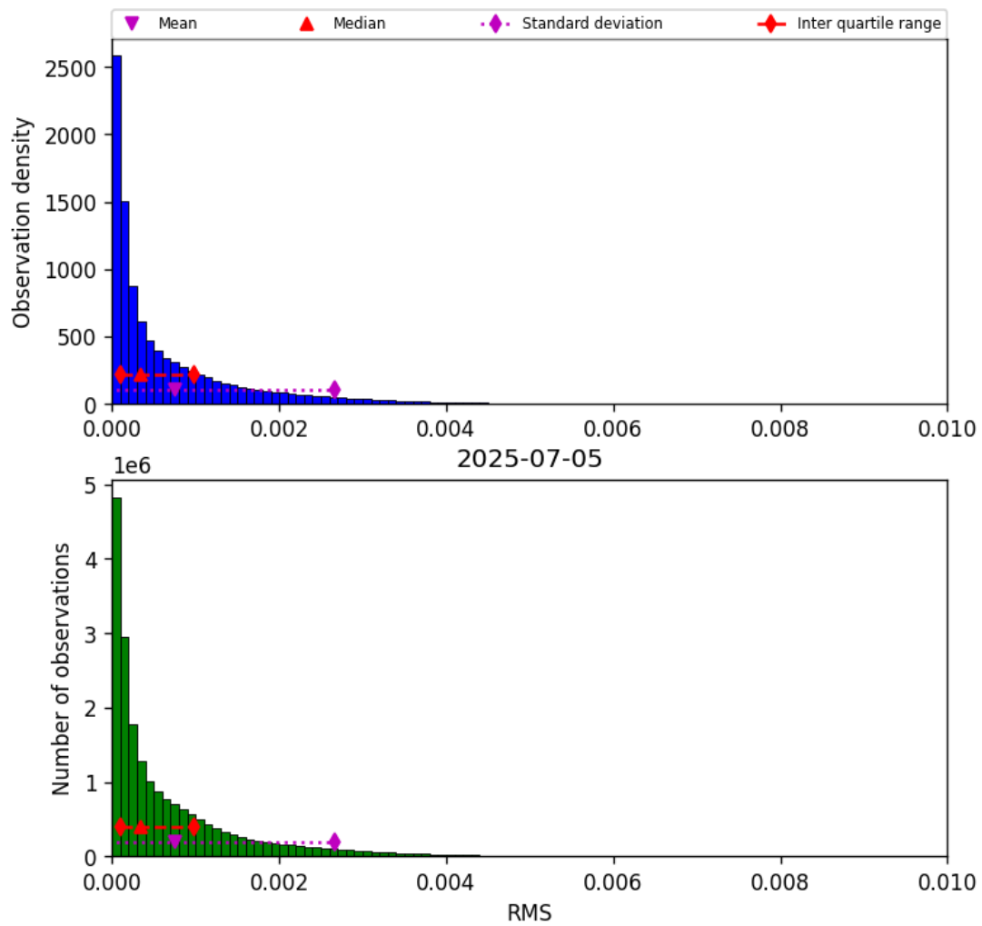
Figure 47: Histogram of “RMS” for 2025-07-04 to 2025-07-06
