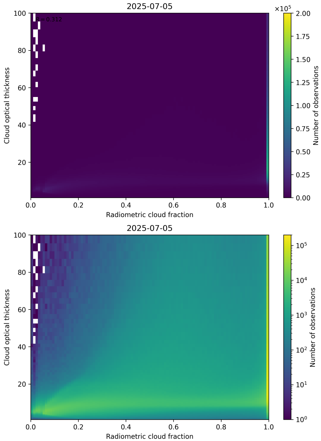
Figure 75: Scatter density plot of “Radiometric cloud fraction” against “Cloud optical thickness” for 2025-07-04 to 2025-07-06.
