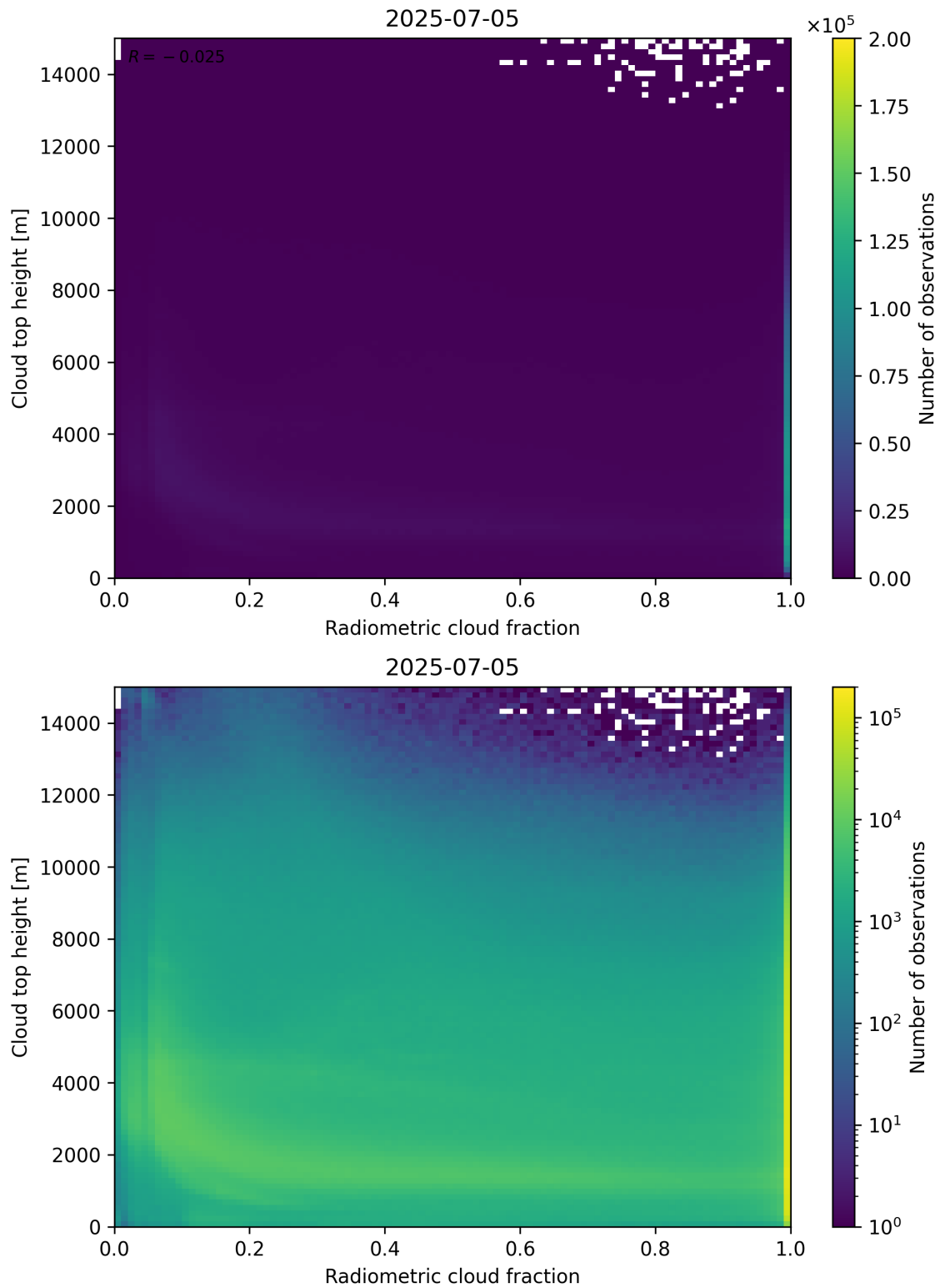
Figure 76: Scatter density plot of “Radiometric cloud fraction” against “Cloud top height” for 2025-07-04 to 2025-07-06.
