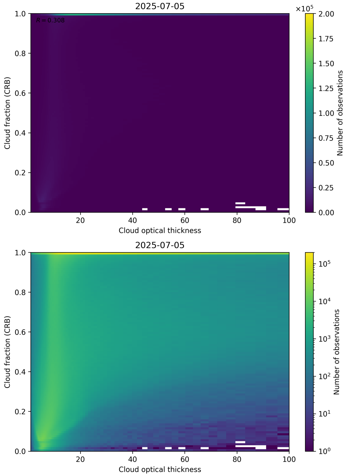
Figure 84: Scatter density plot of “Cloud optical thickness” against “Cloud fraction (CRB)” for 2025-07-04 to 2025-07-06.
