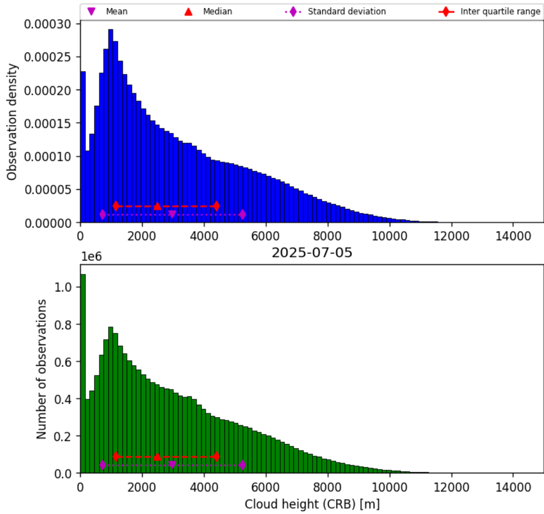
Figure 43: Histogram of “Cloud height (CRB)” for 2025-07-04 to 2025-07-06
