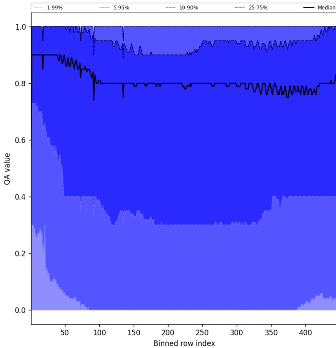
Figure 54: Along track statistics of “QA value” for 2025-07-04 to 2025-07-06
