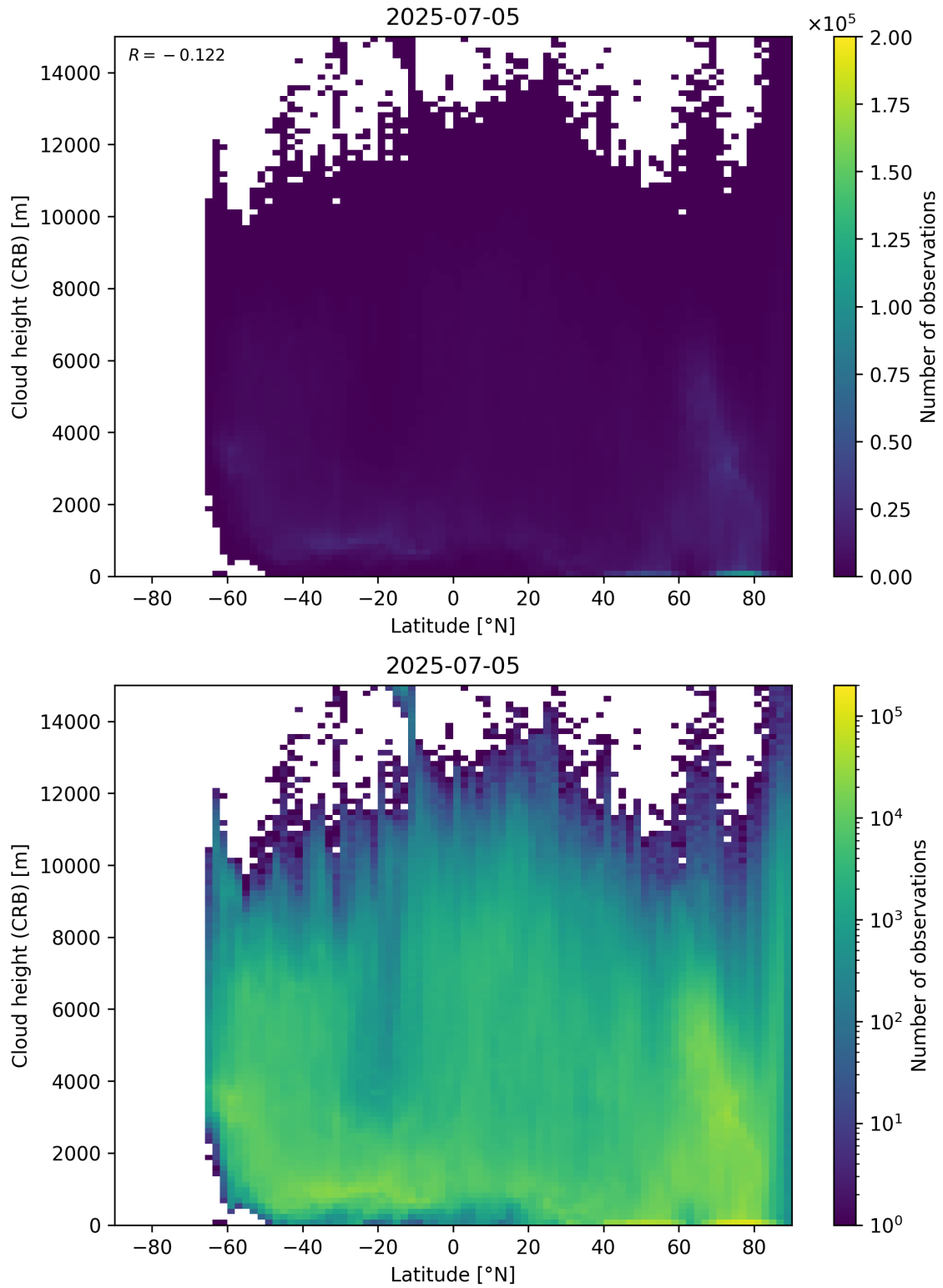
Figure 95: Scatter density plot of “Latitude” against “Cloud height (CRB)” for 2025-07-04 to 2025-07-06.
