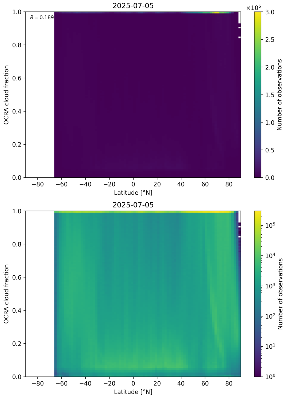
Figure 93: Scatter density plot of “Latitude” against “OCRA cloud fraction” for 2025-07-04 to 2025-07-06.
