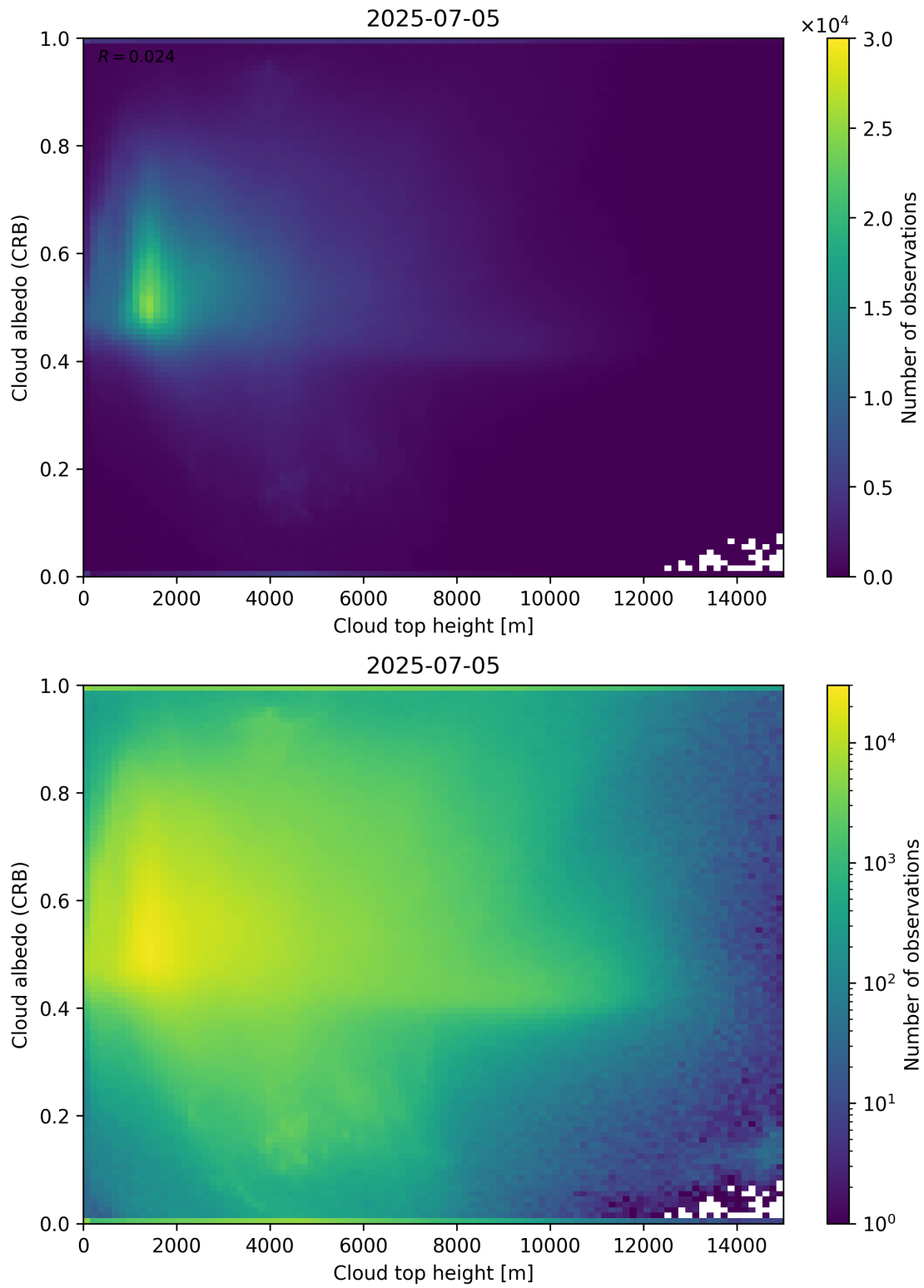
Figure 86: Scatter density plot of “Cloud top height” against “Cloud albedo (CRB)” for 2025-07-04 to 2025-07-06.
