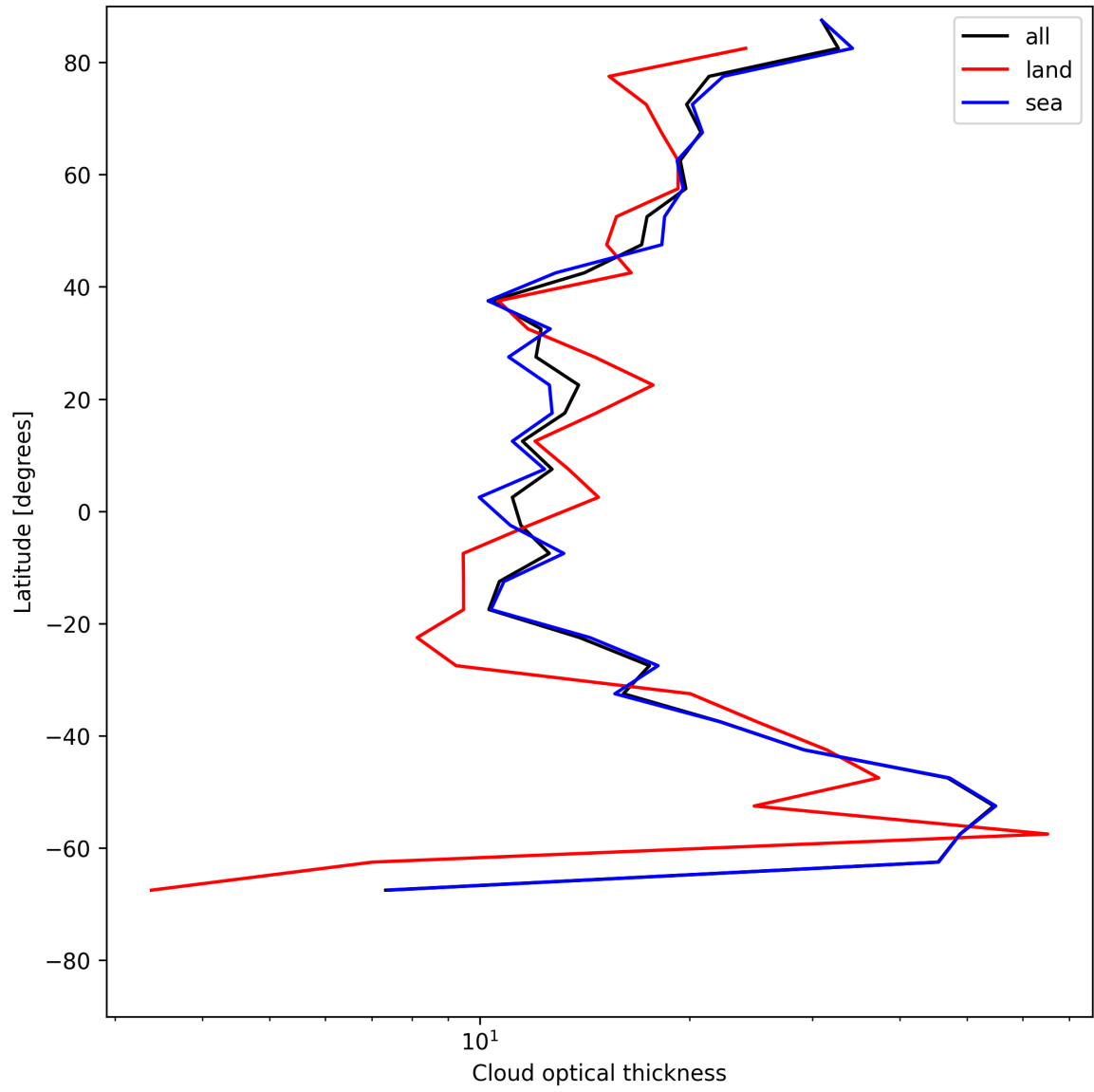
Figure 25: Zonal average of “Cloud optical thickness” for 2025-07-04 to 2025-07-06.
