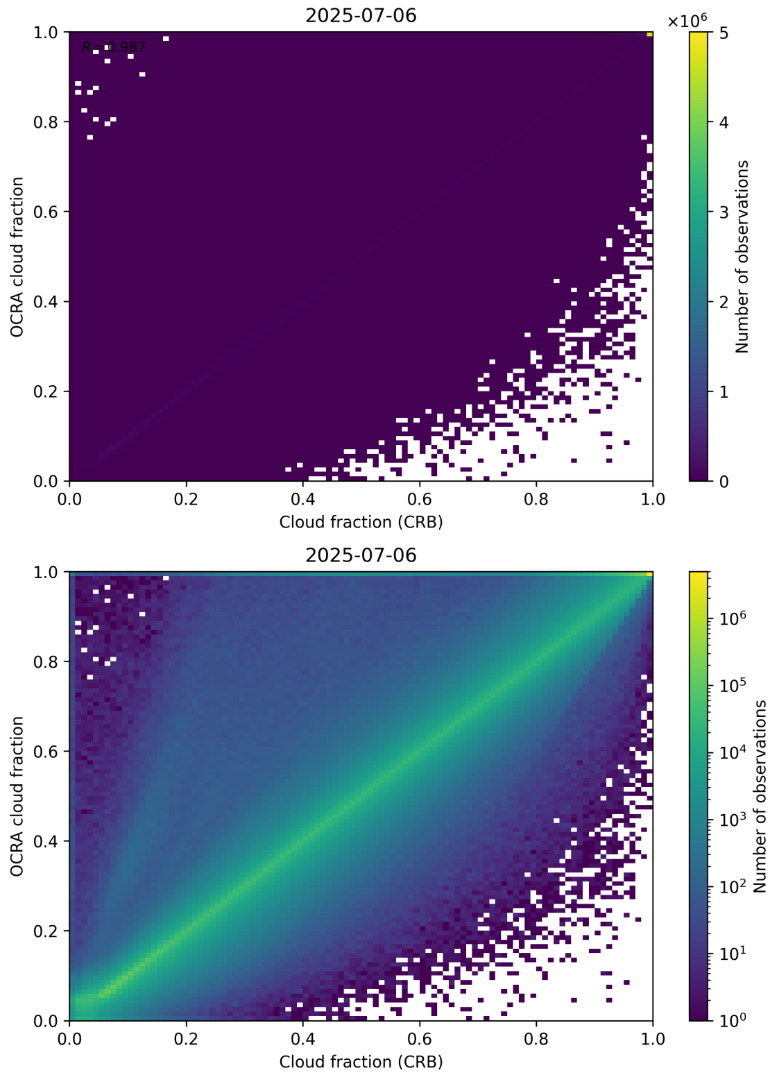
Figure 78: Scatter density plot of “Cloud fraction (CRB)” against “OCRA cloud fraction” for 2025-07-05 to 2025-07-07.
