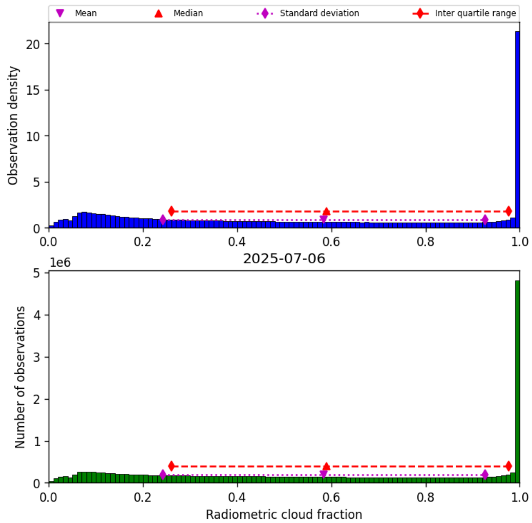
Figure 39: Histogram of “Radiometric cloud fraction” for 2025-07-05 to 2025-07-07
