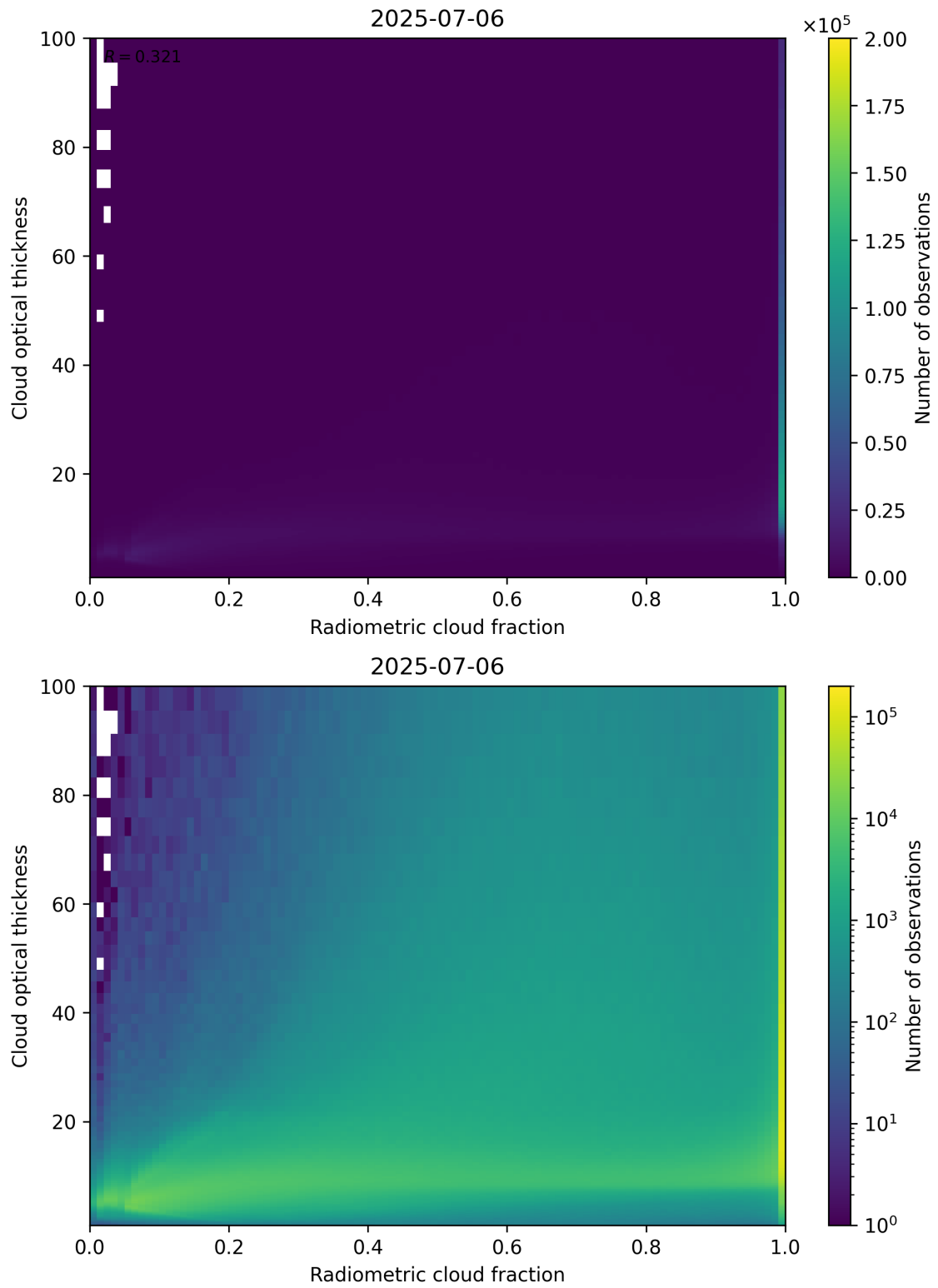
Figure 75: Scatter density plot of “Radiometric cloud fraction” against “Cloud optical thickness” for 2025-07-05 to 2025-07-07.
