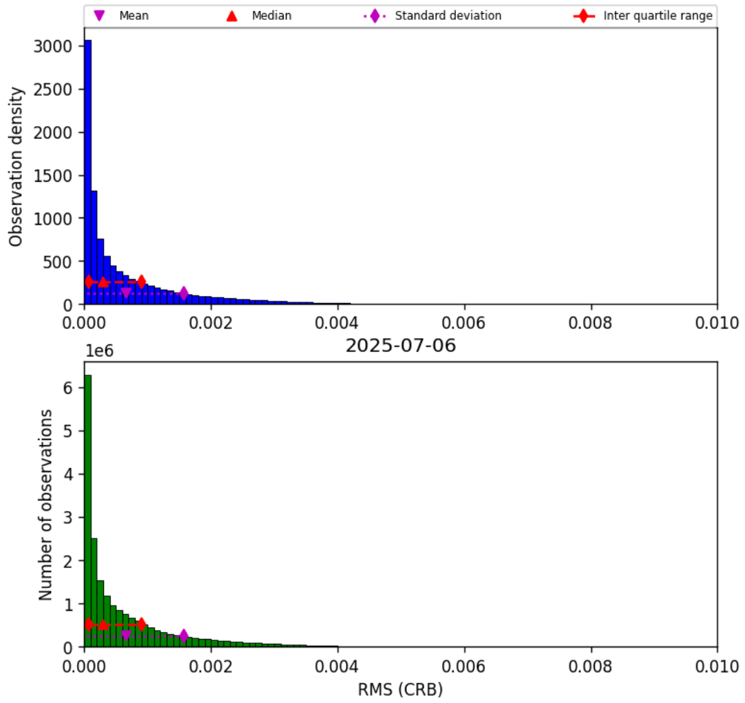
Figure 48: Histogram of “RMS (CRB)” for 2025-07-05 to 2025-07-07
