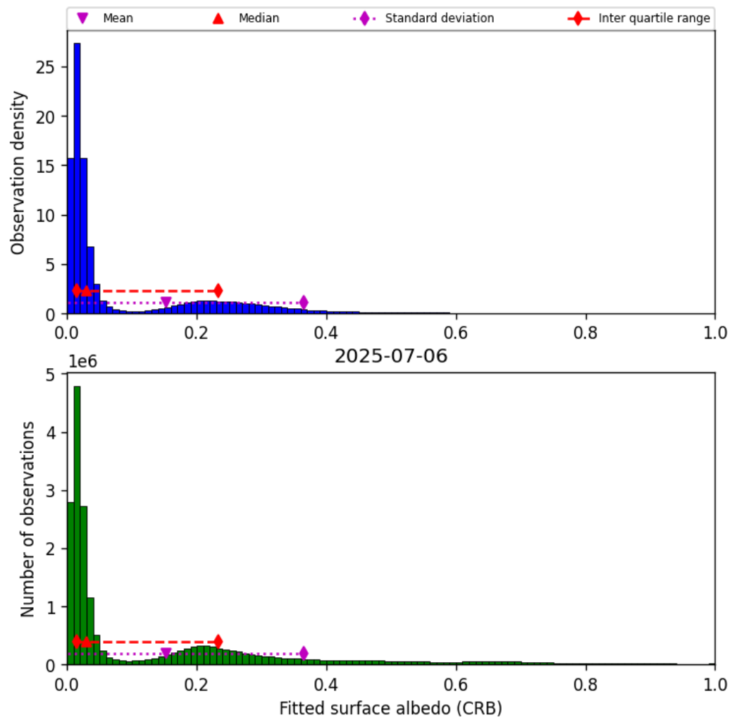
Figure 46: Histogram of “Fitted surface albedo (CRB)” for 2025-07-05 to 2025-07-07
