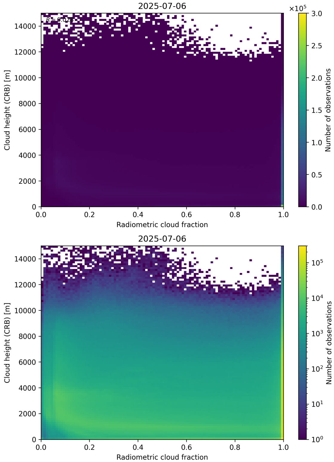
Figure 74: Scatter density plot of “Radiometric cloud fraction” against “Cloud height (CRB)” for 2025-07-05 to 2025-07-07.
