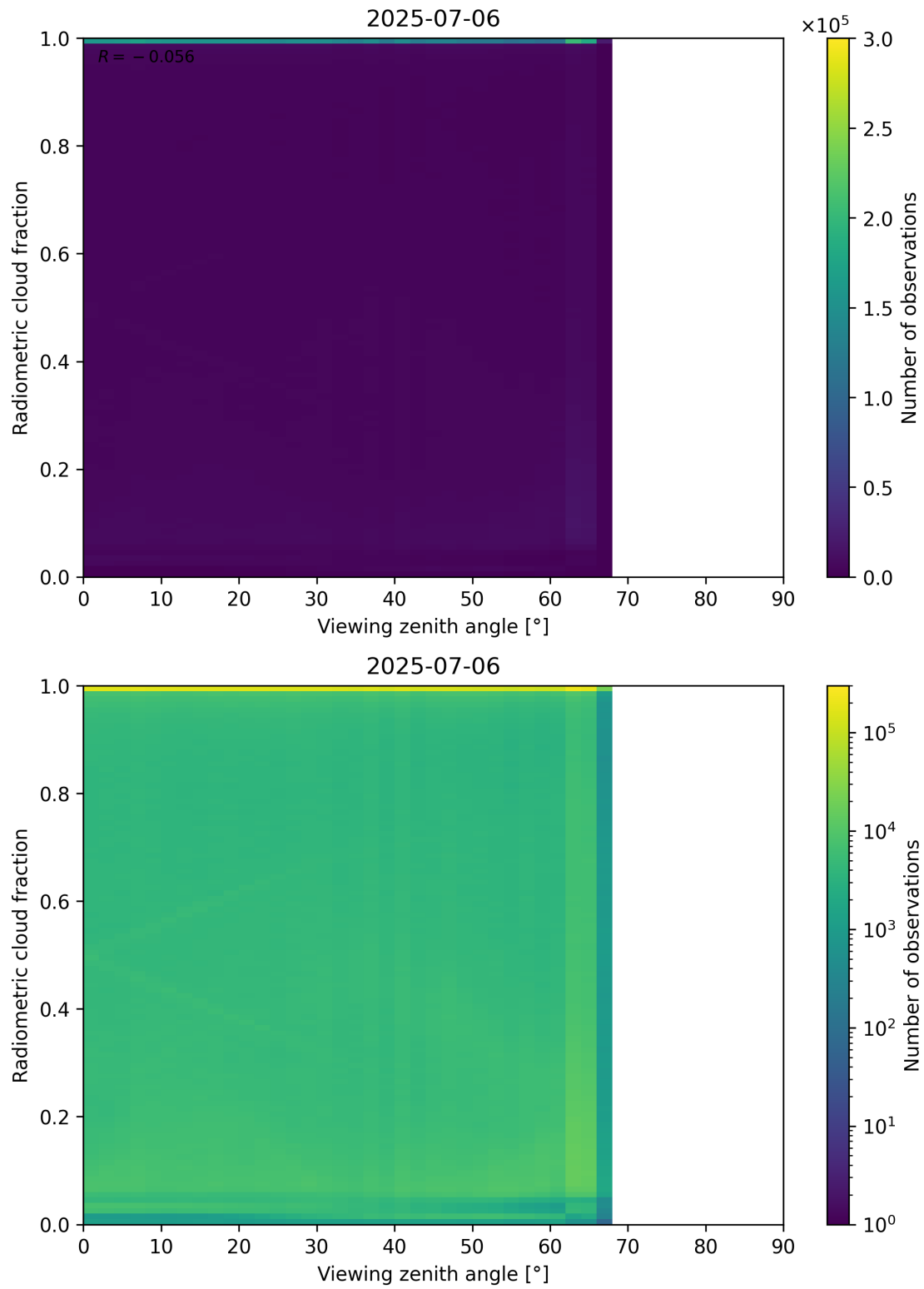
Figure 107: Scatter density plot of “Viewing zenith angle” against “Radiometric cloud fraction” for 2025-07-05 to 2025-07-07.
