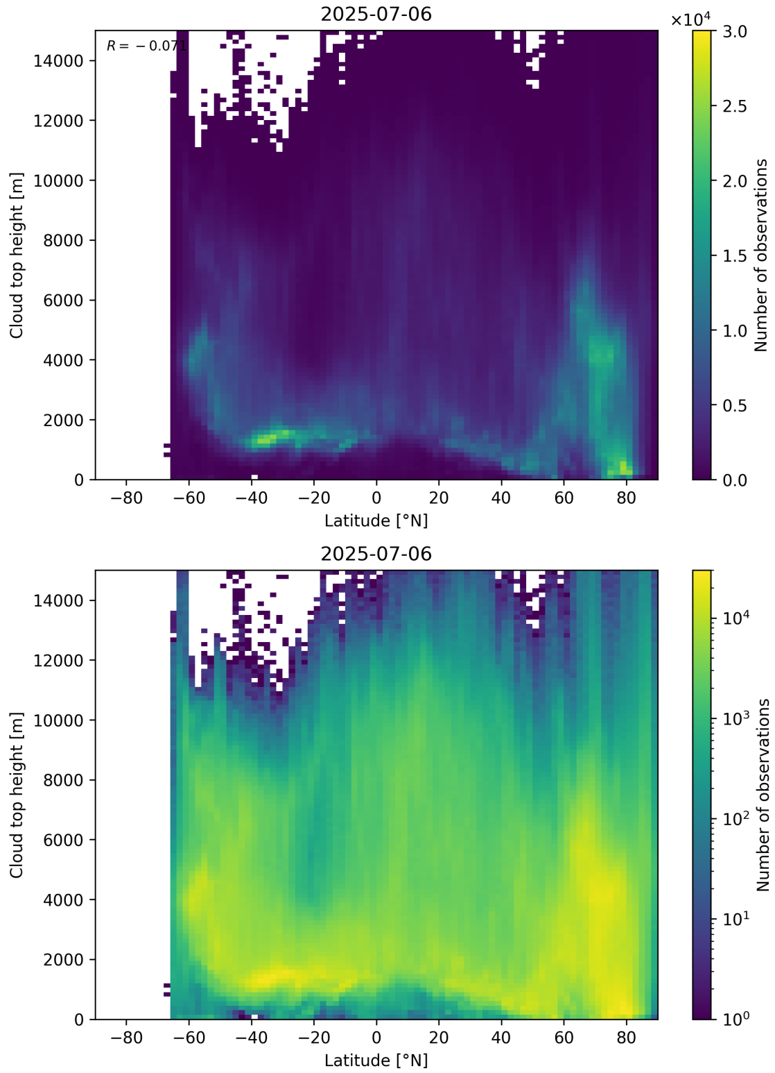
Figure 97: Scatter density plot of “Latitude” against “Cloud top height” for 2025-07-05 to 2025-07-07.
