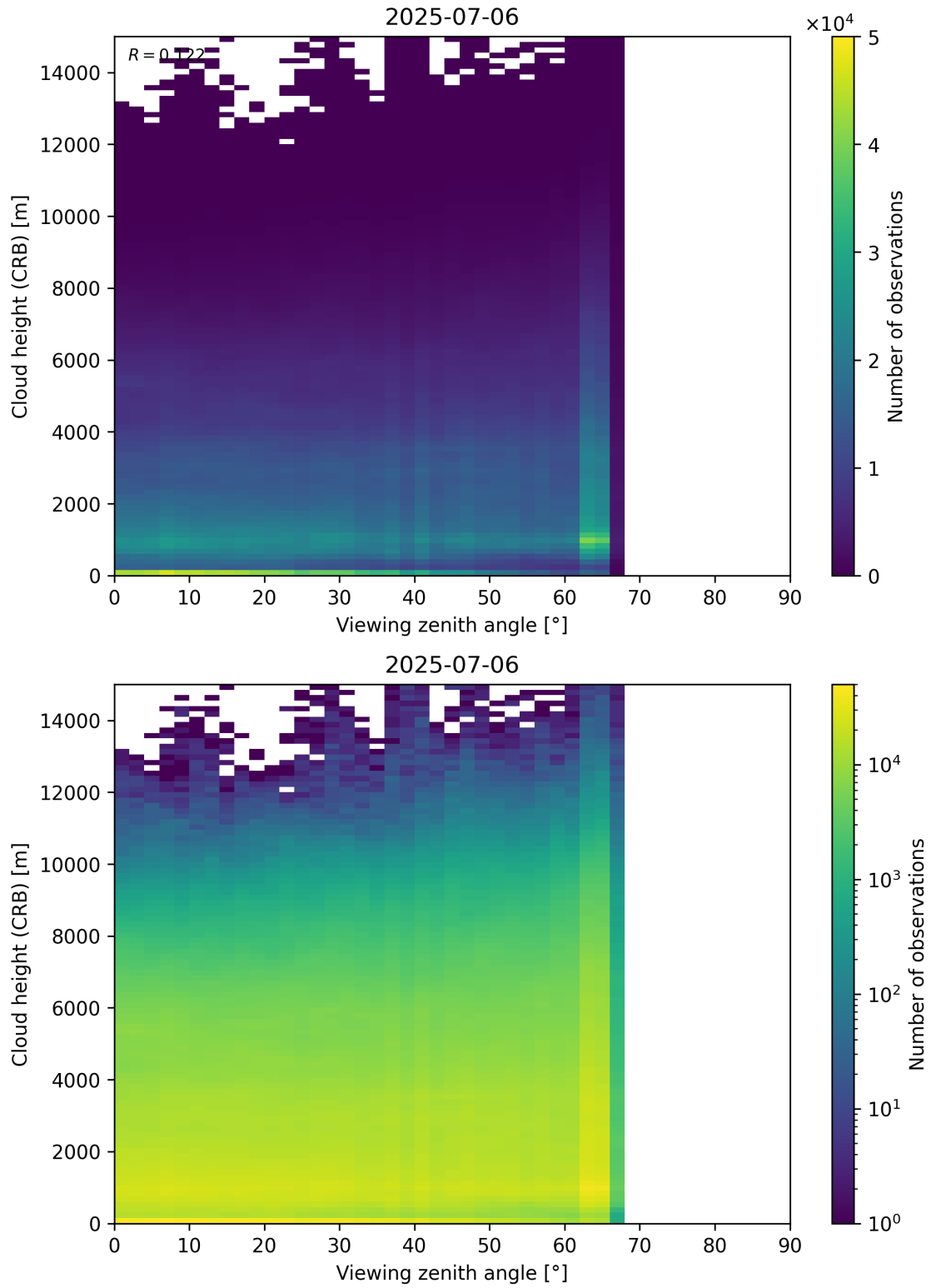
Figure 110: Scatter density plot of “Viewing zenith angle” against “Cloud height (CRB)” for 2025-07-05 to 2025-07-07.
