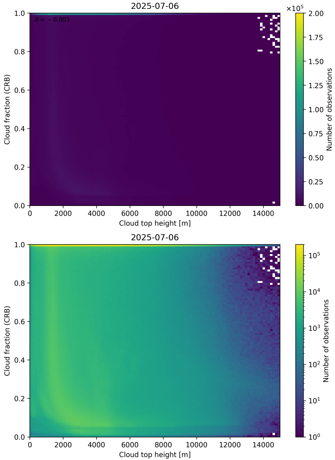
Figure 88: Scatter density plot of “Cloud top height” against “Cloud fraction (CRB)” for 2025-07-05 to 2025-07-07.
