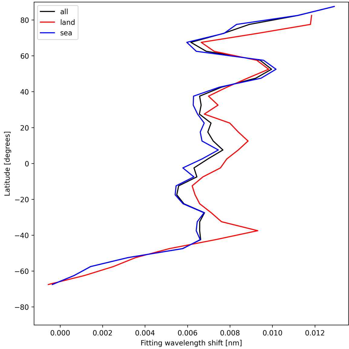
Figure 33: Zonal average of “Fitting wavelength shift” for 2025-07-05 to 2025-07-07.
