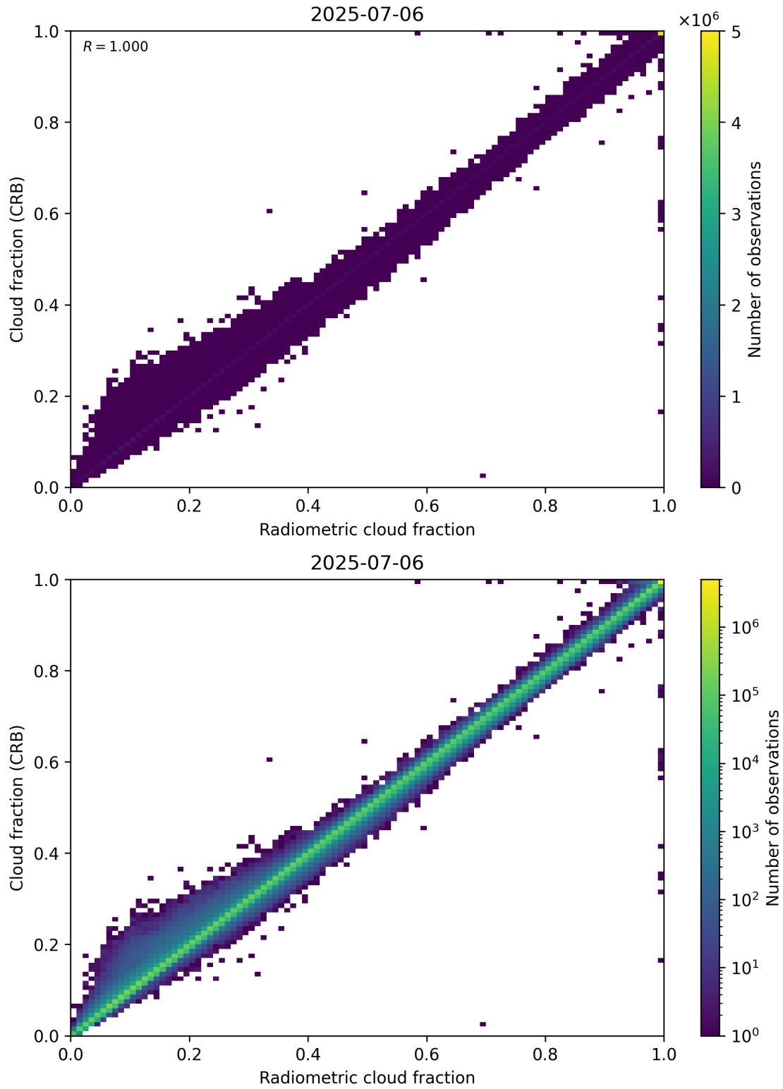
Figure 73: Scatter density plot of “Radiometric cloud fraction” against “Cloud fraction (CRB)” for 2025-07-05 to 2025-07-07.
