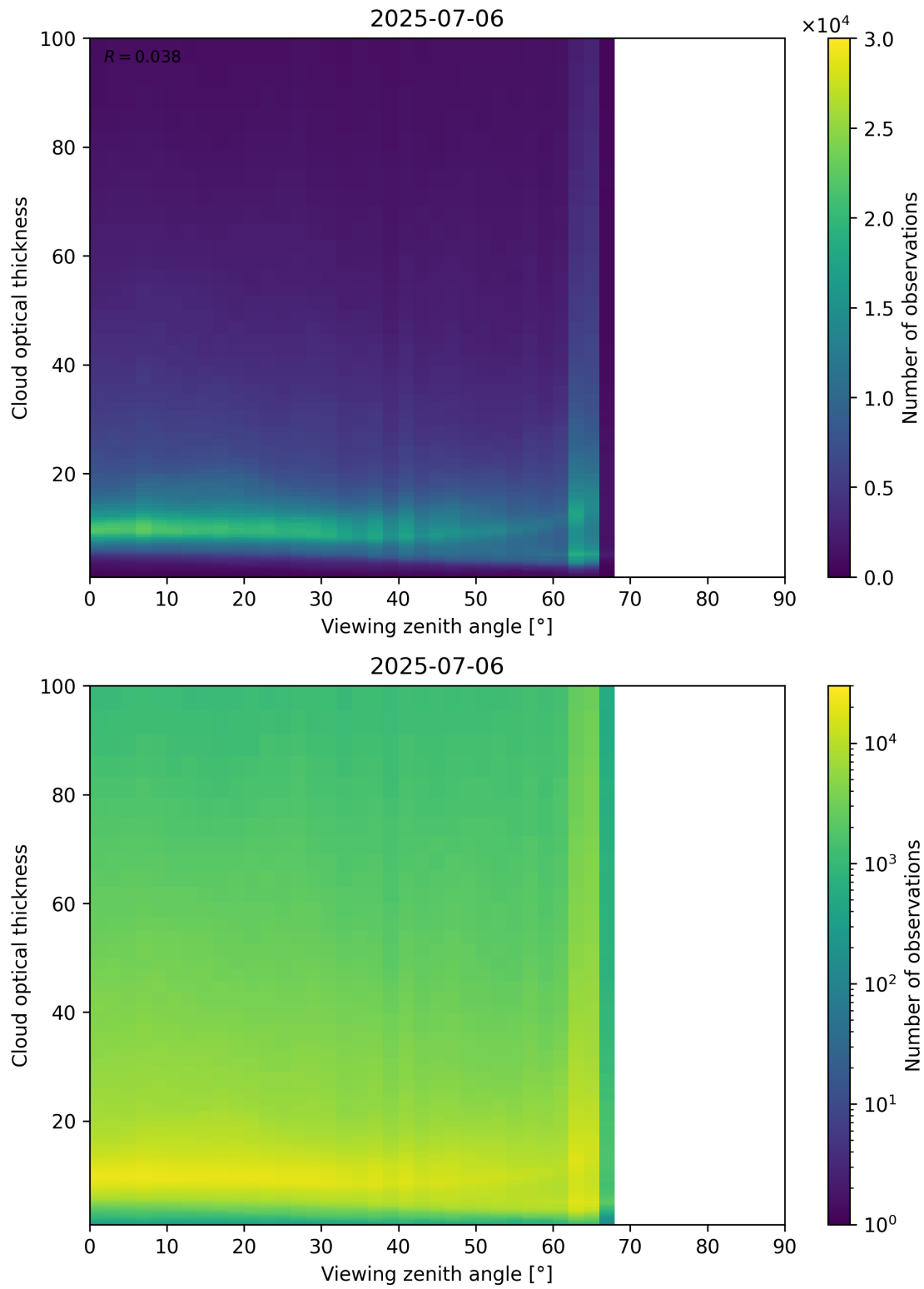
Figure 111: Scatter density plot of “Viewing zenith angle” against “Cloud optical thickness” for 2025-07-05 to 2025-07-07.
