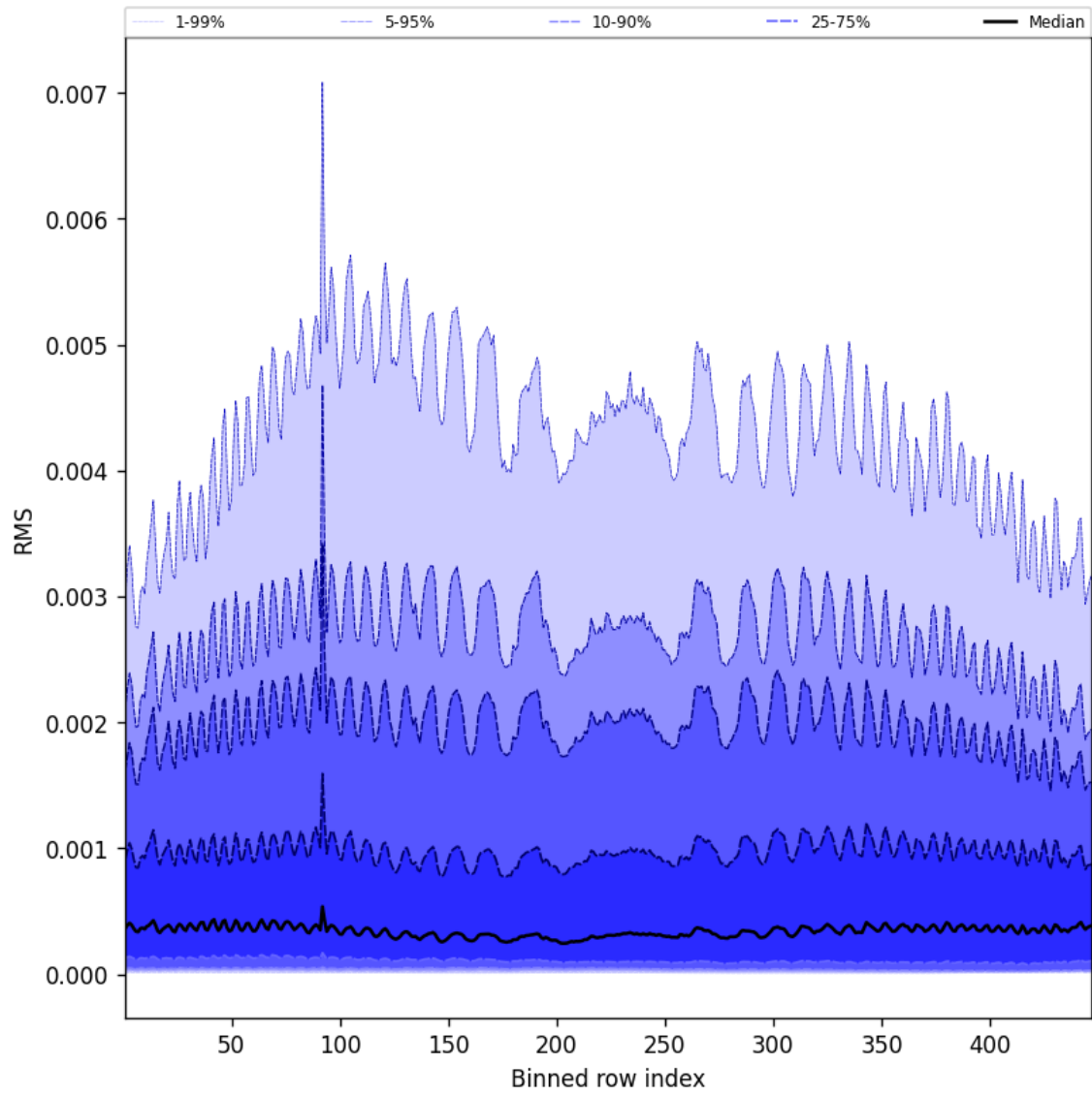
Figure 63: Along track statistics of “RMS” for 2025-07-05 to 2025-07-07
