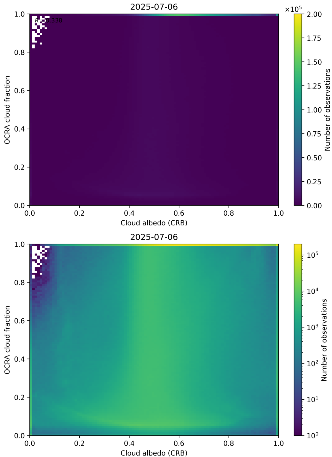
Figure 70: Scatter density plot of “Cloud albedo (CRB)” against “OCRA cloud fraction” for 2025-07-05 to 2025-07-07.
