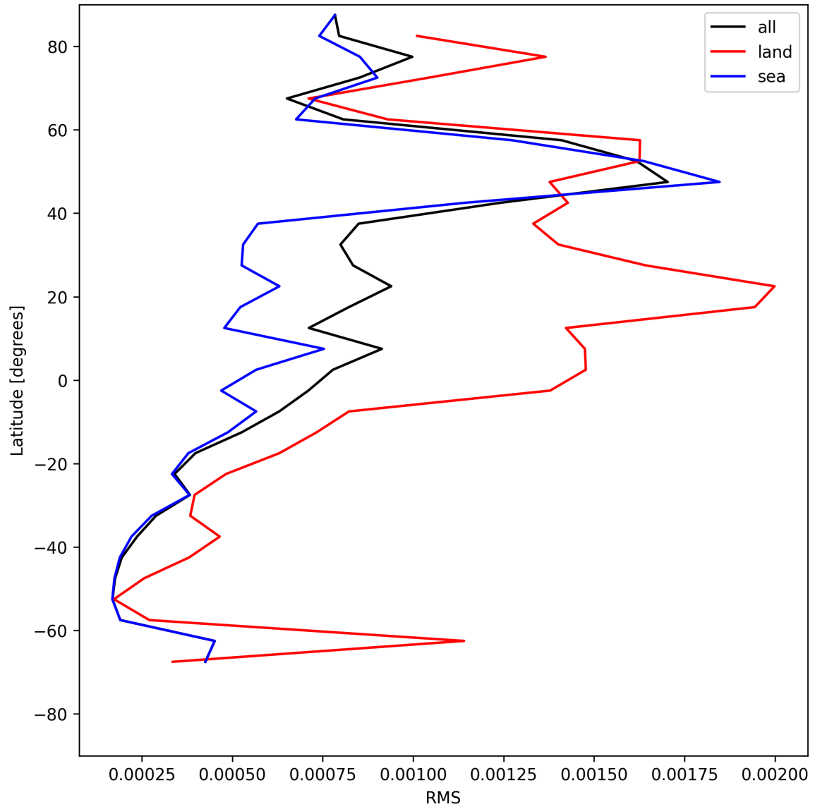
Figure 31: Zonal average of “RMS” for 2025-07-05 to 2025-07-07.
