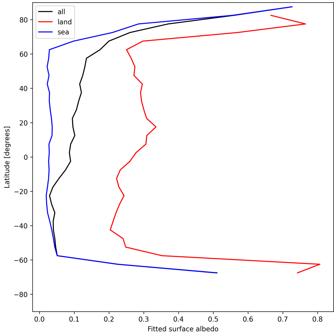
Figure 29: Zonal average of “Fitted surface albedo” for 2025-07-05 to 2025-07-07.
