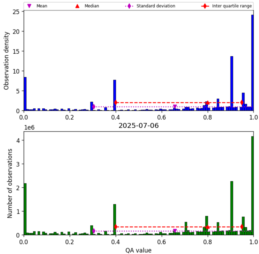
Figure 38: Histogram of “QA value” for 2025-07-05 to 2025-07-07
