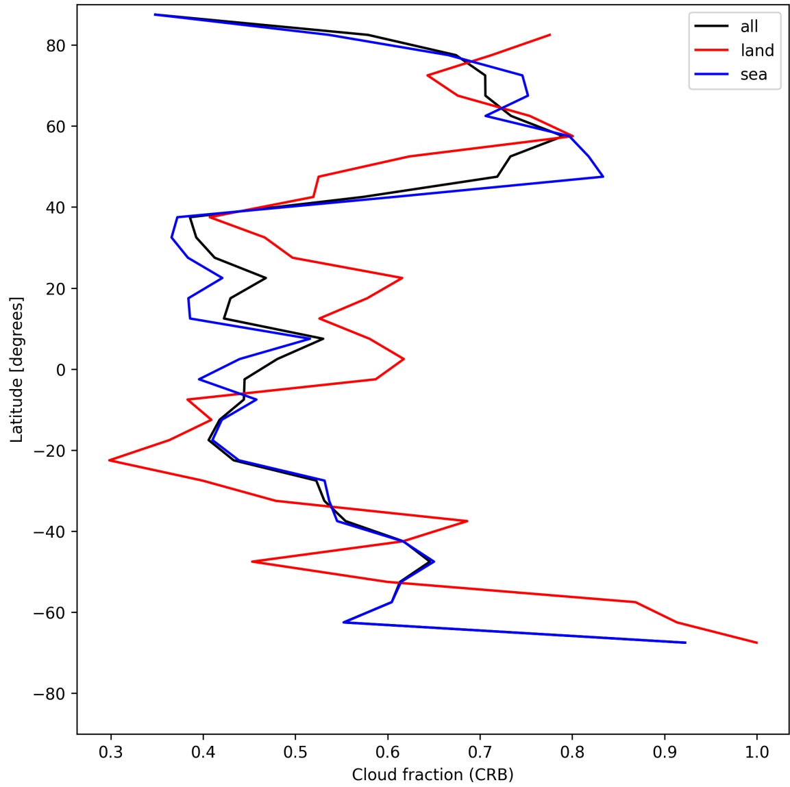
Figure 26: Zonal average of “Cloud fraction (CRB)” for 2025-07-05 to 2025-07-07.
