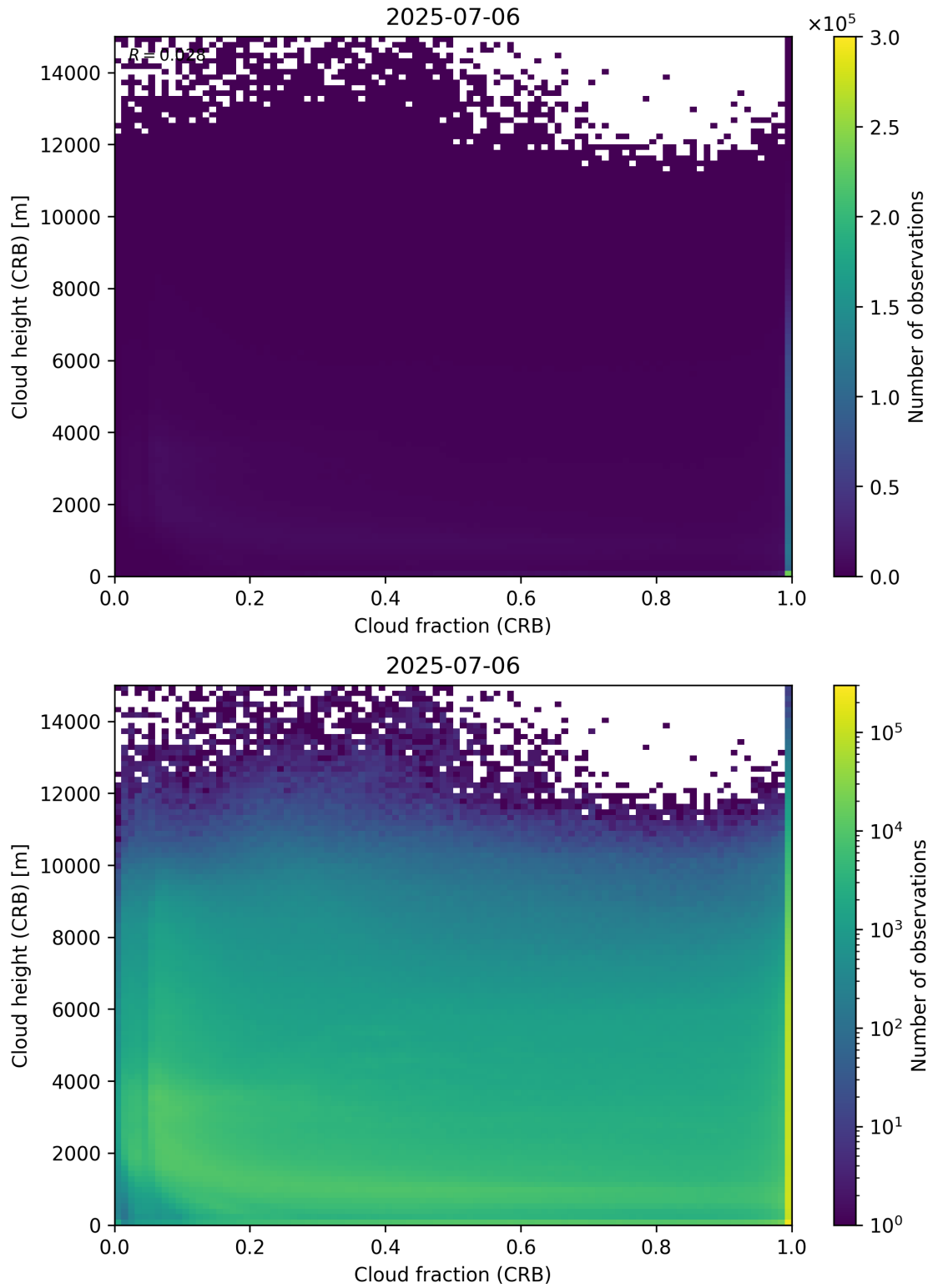
Figure 79: Scatter density plot of “Cloud fraction (CRB)” against “Cloud height (CRB)” for 2025-07-05 to 2025-07-07.
