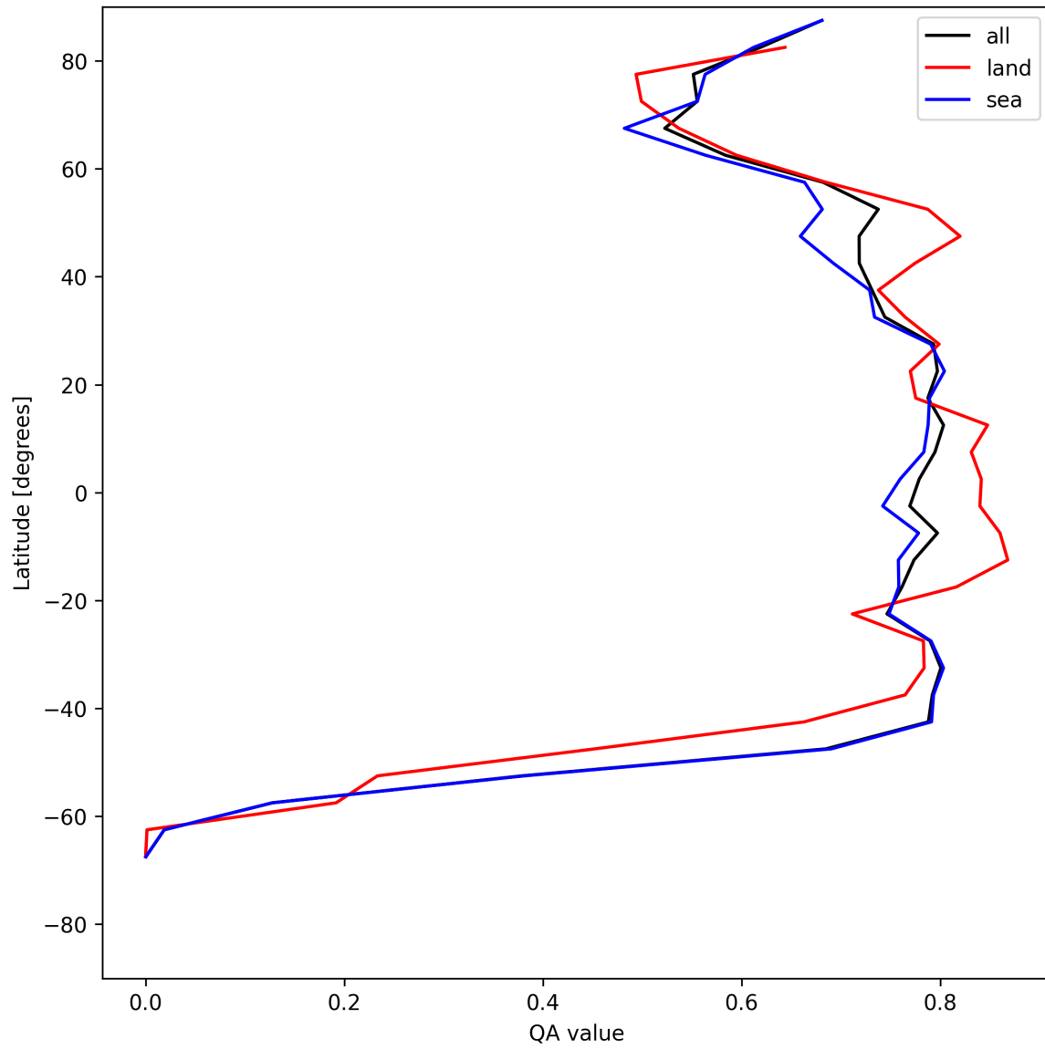
Figure 22: Zonal average of “QA value” for 2025-07-05 to 2025-07-07.
