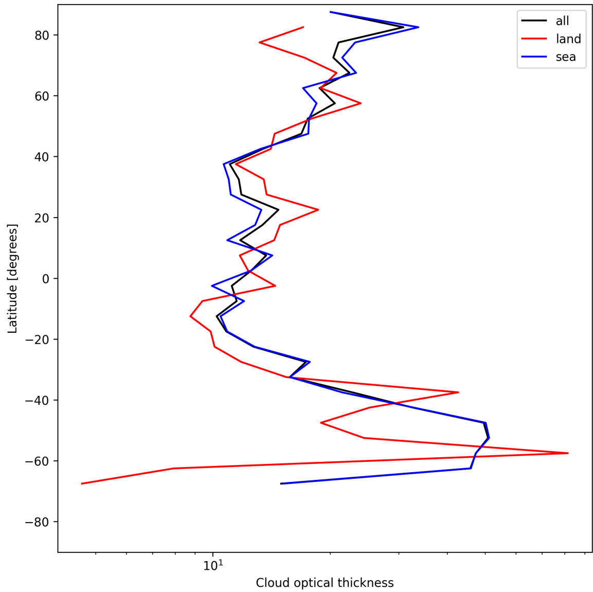
Figure 25: Zonal average of “Cloud optical thickness” for 2025-07-05 to 2025-07-07.
