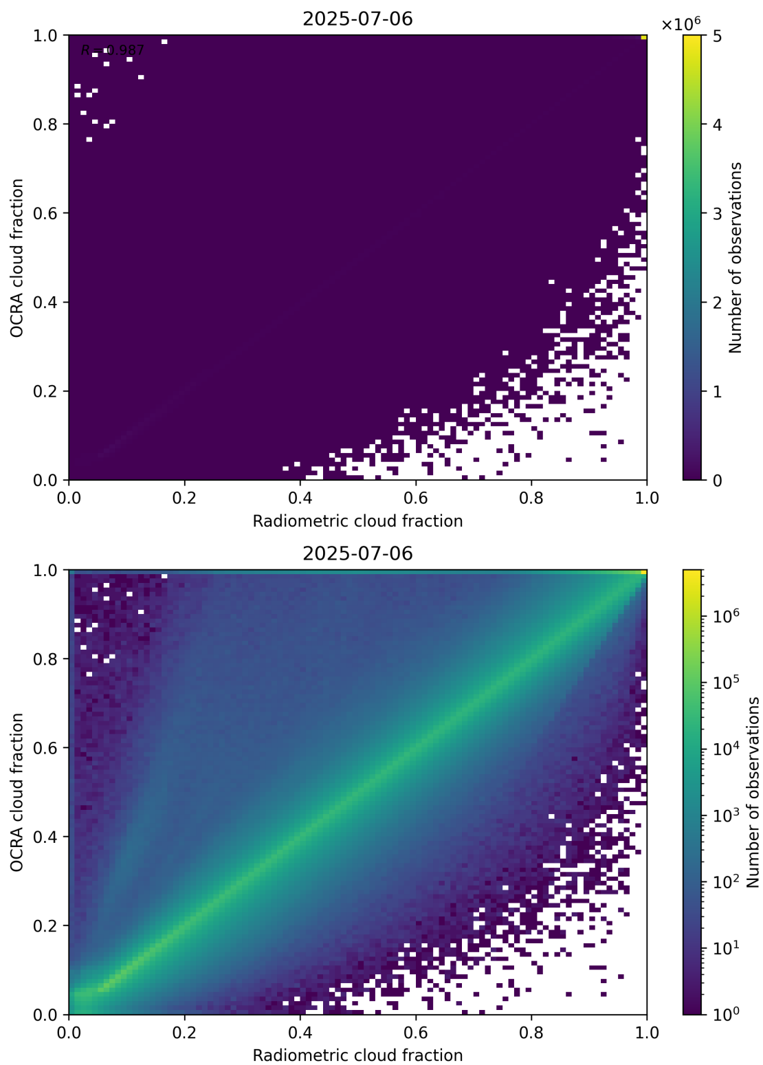
Figure 72: Scatter density plot of “Radiometric cloud fraction” against “OCRA cloud fraction” for 2025-07-05 to 2025-07-07.
