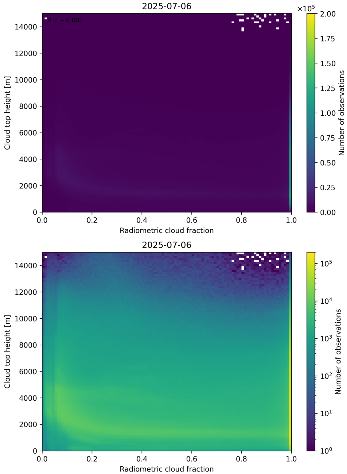
Figure 76: Scatter density plot of “Radiometric cloud fraction” against “Cloud top height” for 2025-07-05 to 2025-07-07.
