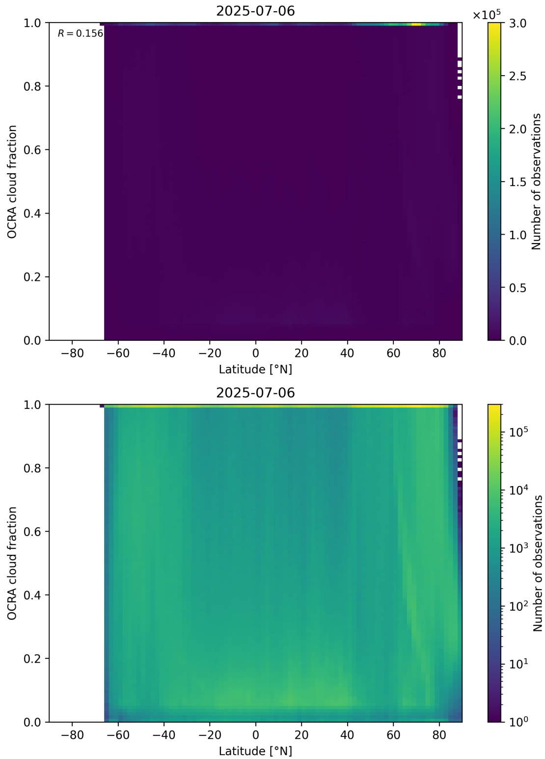
Figure 93: Scatter density plot of “Latitude” against “OCRA cloud fraction” for 2025-07-05 to 2025-07-07.
