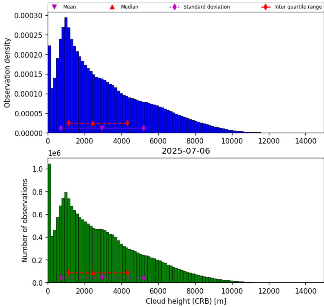
Figure 43: Histogram of “Cloud height (CRB)” for 2025-07-05 to 2025-07-07
