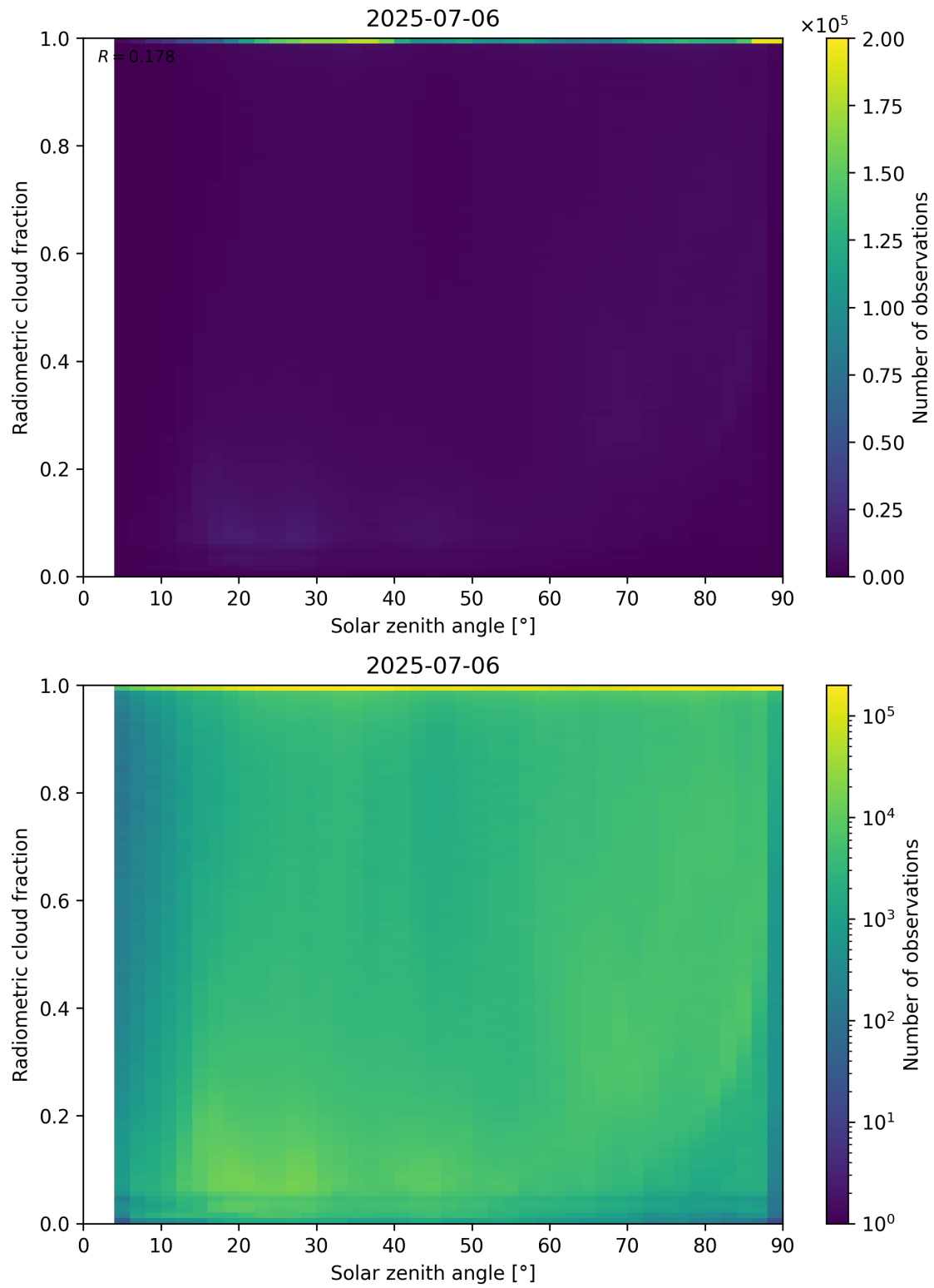
Figure 99: Scatter density plot of “Solar zenith angle” against “Radiometric cloud fraction” for 2025-07-05 to 2025-07-07.
