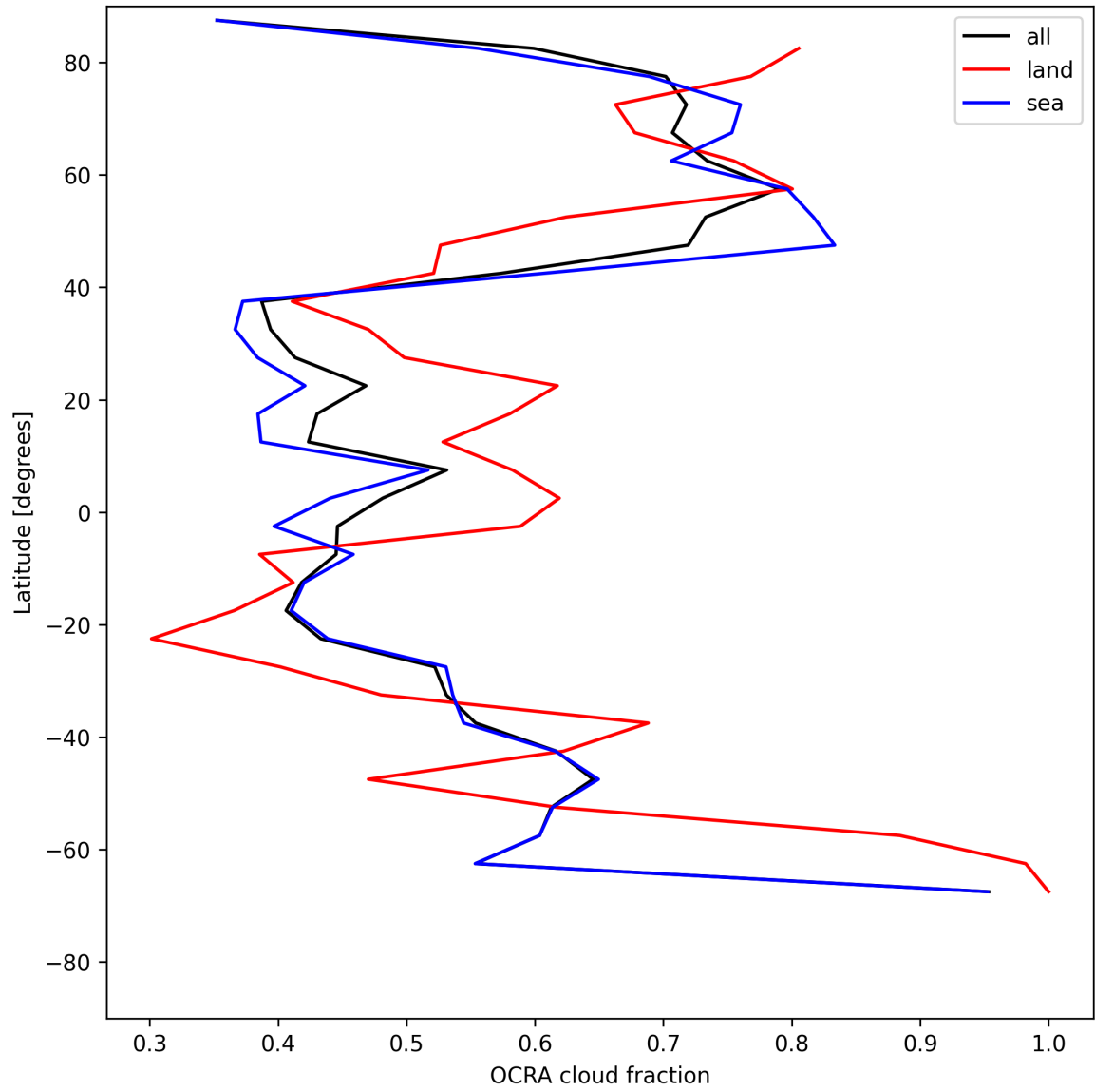
Figure 34: Zonal average of “OCRA cloud fraction” for 2025-07-05 to 2025-07-07.
