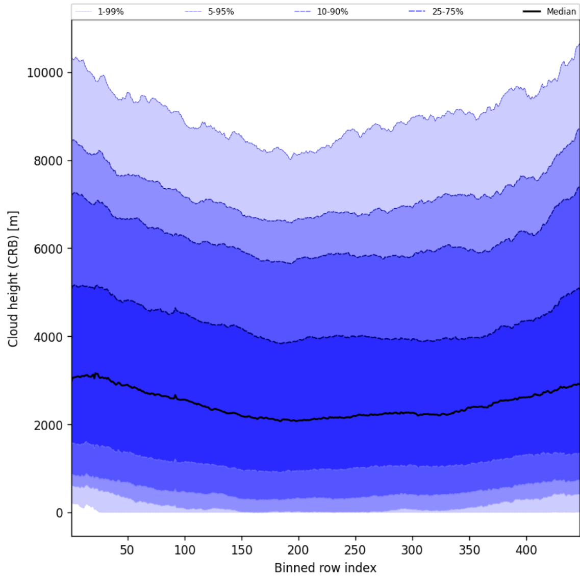
Figure 59: Along track statistics of “Cloud height (CRB)” for 2025-07-05 to 2025-07-07
