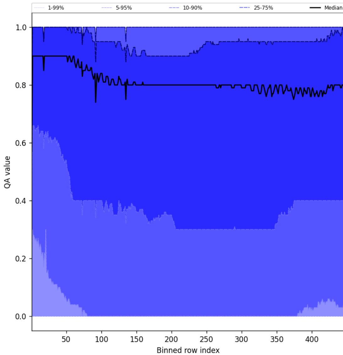
Figure 54: Along track statistics of “QA value” for 2025-07-05 to 2025-07-07
