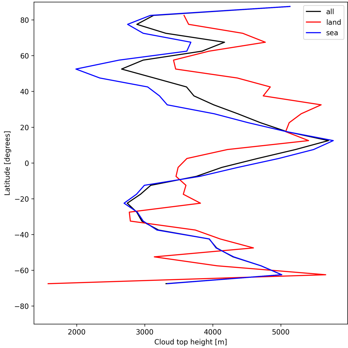
Figure 24: Zonal average of “Cloud top height” for 2025-07-05 to 2025-07-07.
