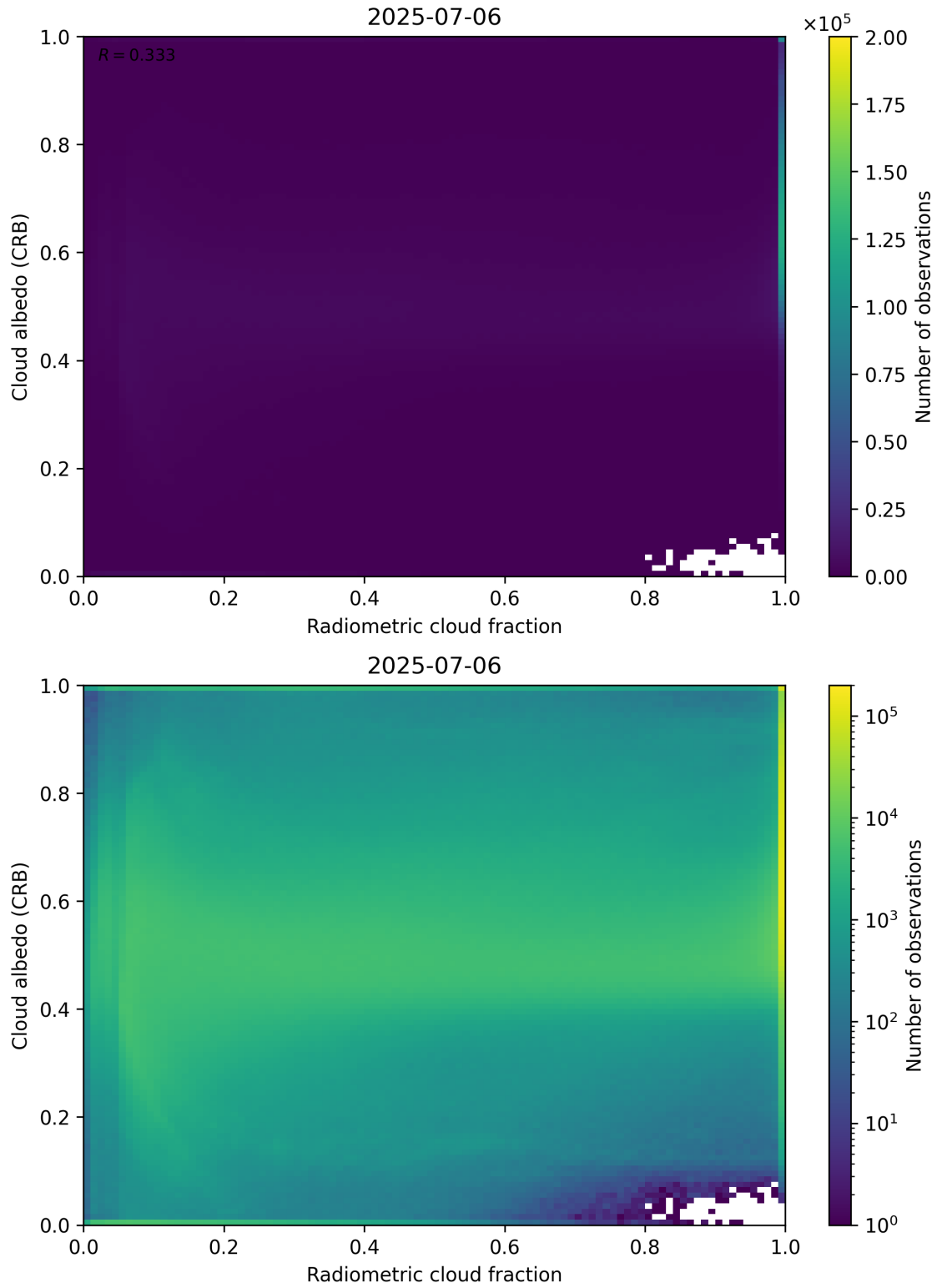
Figure 71: Scatter density plot of “Radiometric cloud fraction” against “Cloud albedo (CRB)” for 2025-07-05 to 2025-07-07.
