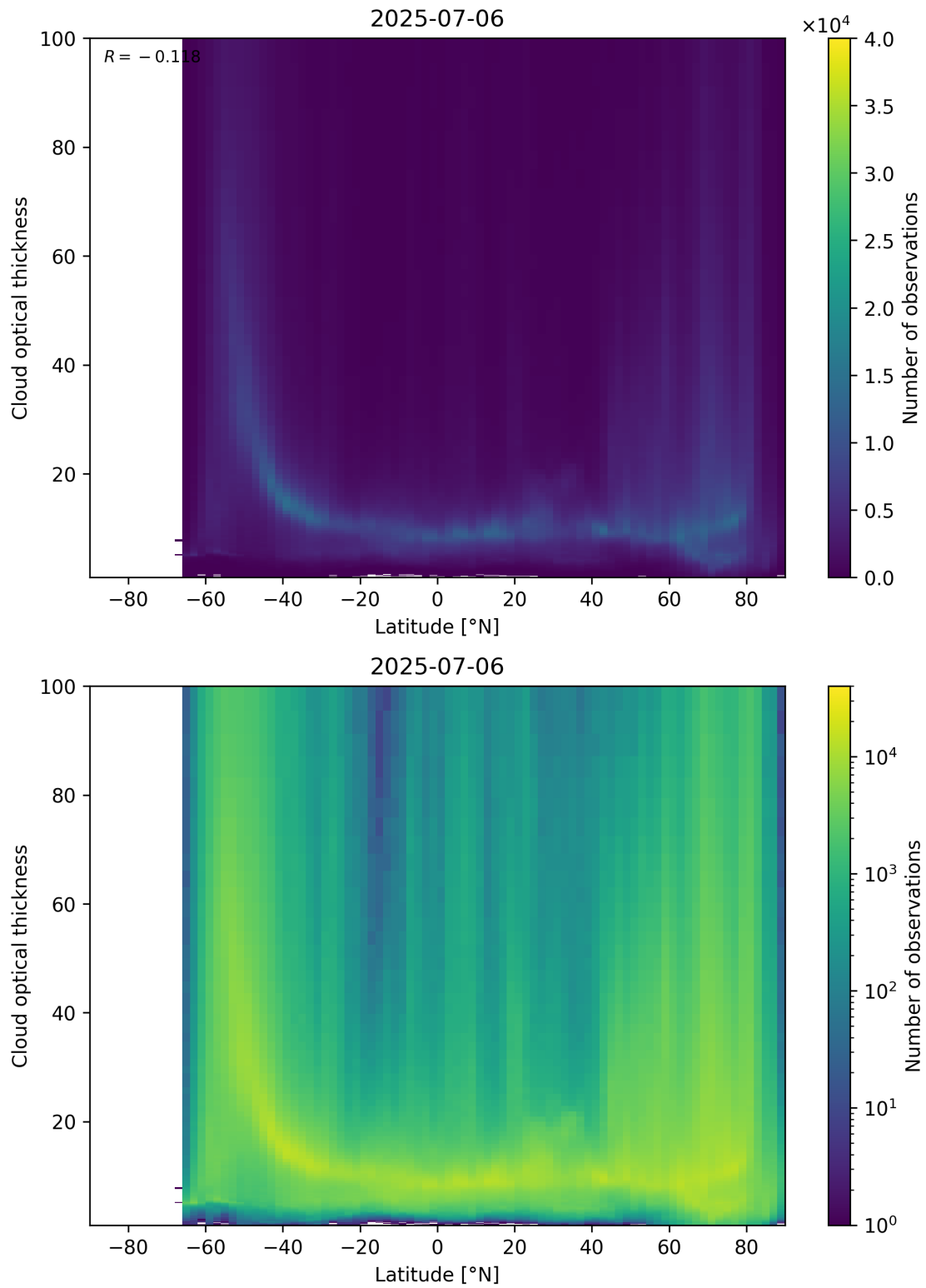
Figure 96: Scatter density plot of “Latitude” against “Cloud optical thickness” for 2025-07-05 to 2025-07-07.
