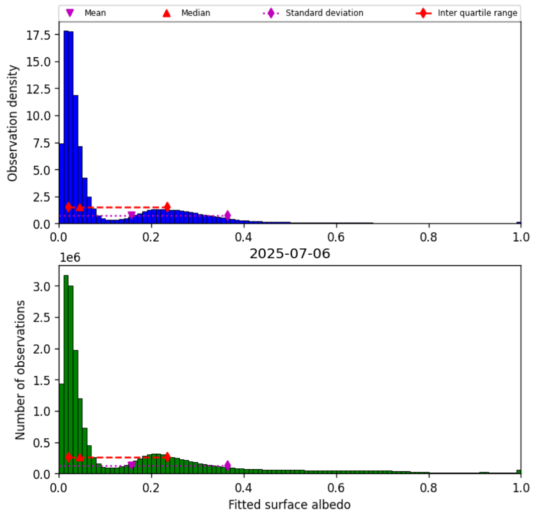
Figure 45: Histogram of “Fitted surface albedo” for 2025-07-05 to 2025-07-07
