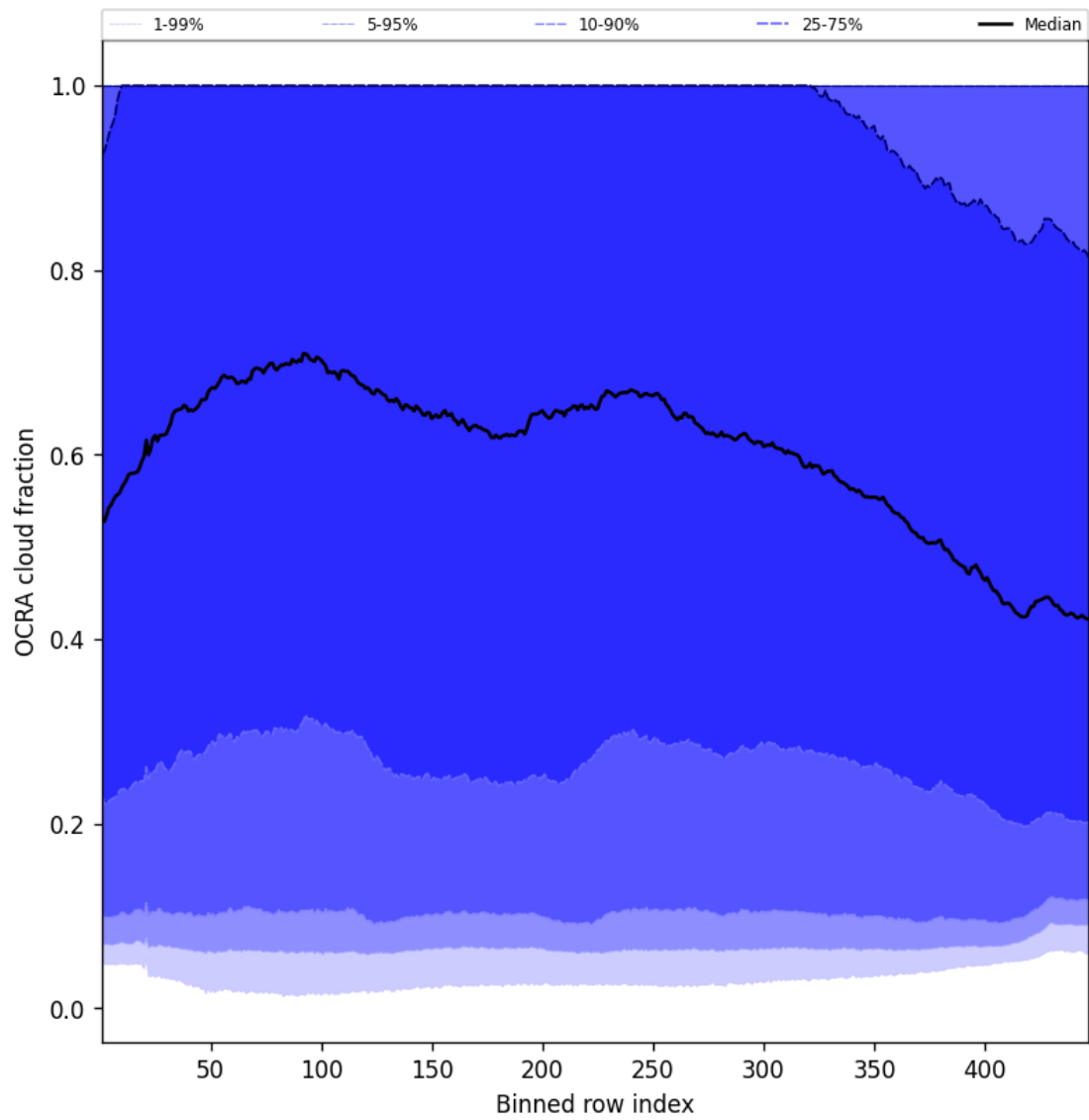
Figure 66: Along track statistics of “OCRA cloud fraction” for 2025-07-05 to 2025-07-07
