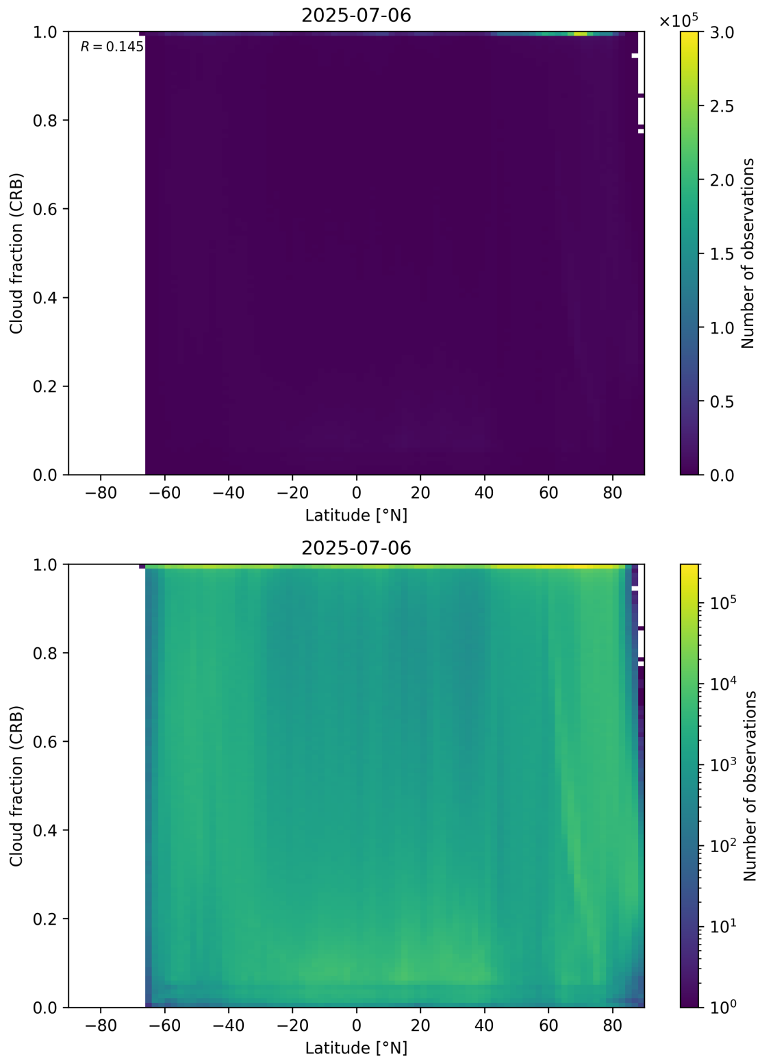
Figure 94: Scatter density plot of “Latitude” against “Cloud fraction (CRB)” for 2025-07-05 to 2025-07-07.
