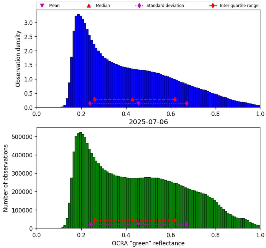
Figure 52: Histogram of “OCRA “green” reflectance” for 2025-07-05 to 2025-07-07
