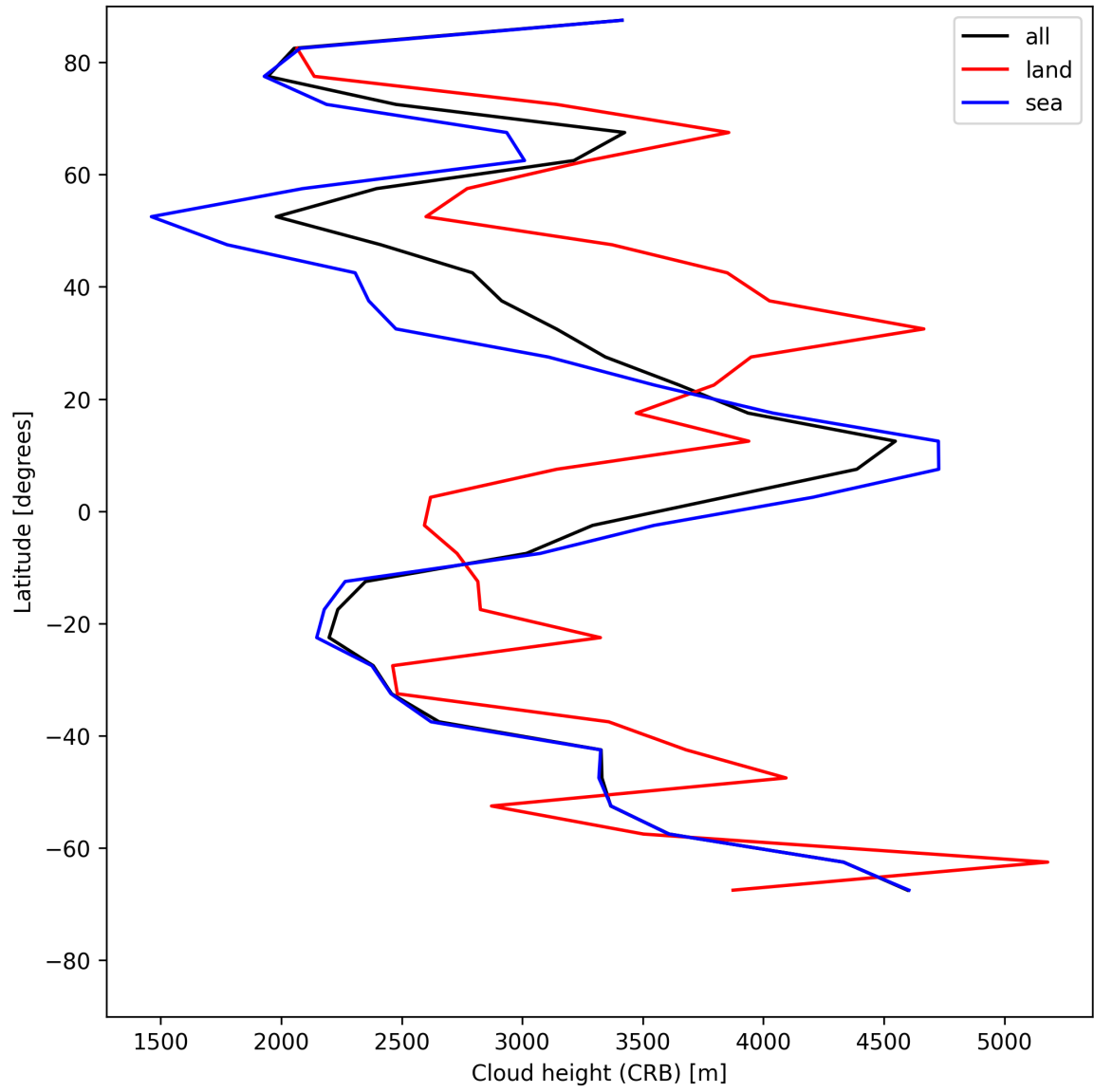
Figure 27: Zonal average of “Cloud height (CRB)” for 2025-07-05 to 2025-07-07.
