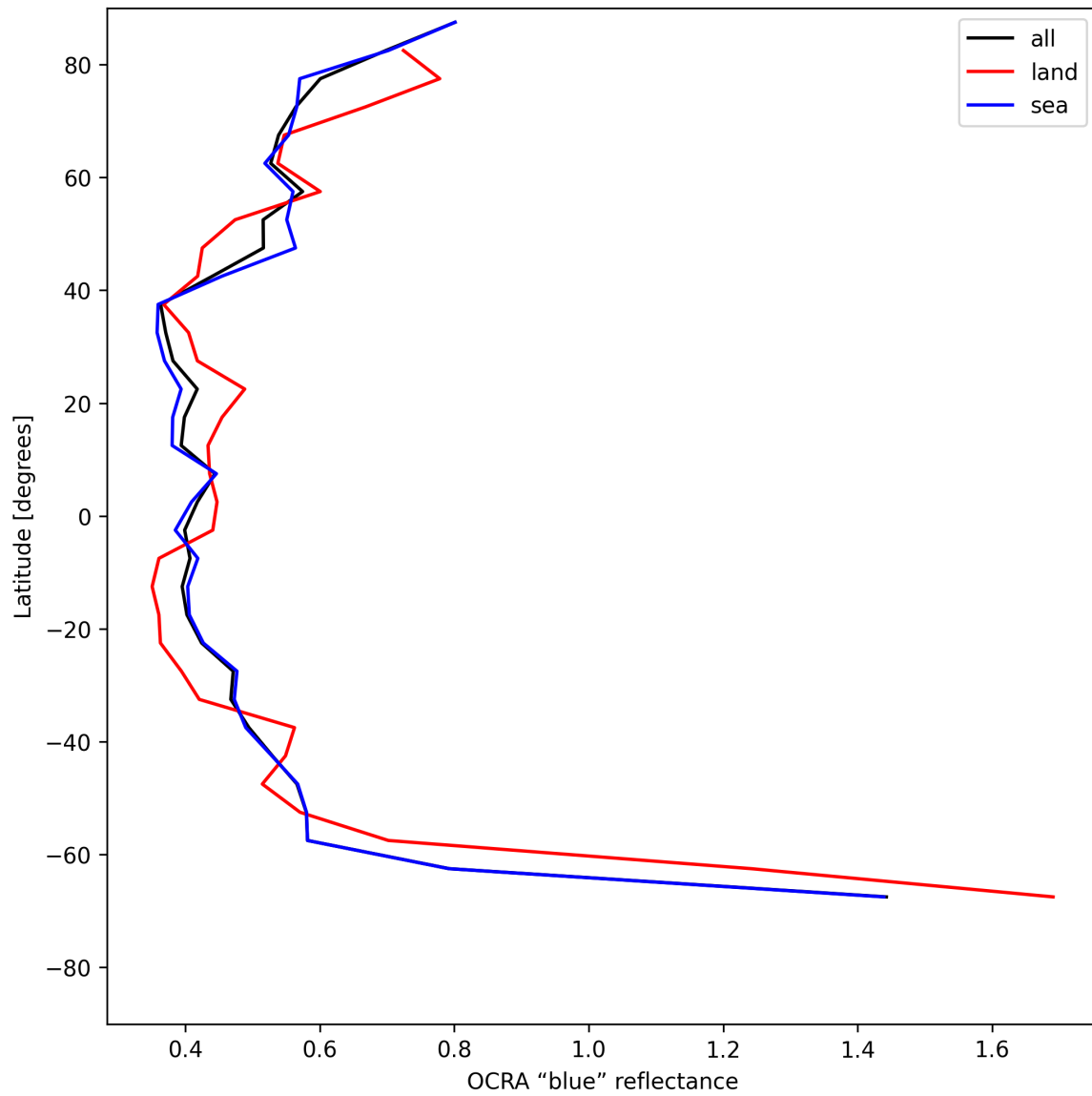
Figure 35: Zonal average of “OCRA “blue” reflectance” for 2025-07-05 to 2025-07-07.
