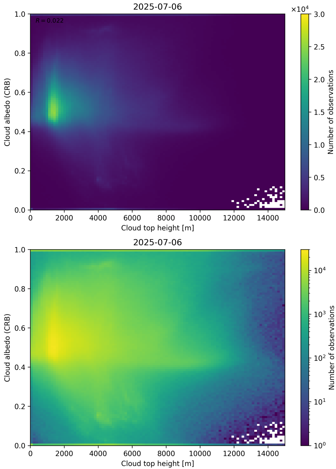
Figure 86: Scatter density plot of “Cloud top height” against “Cloud albedo (CRB)” for 2025-07-05 to 2025-07-07.
