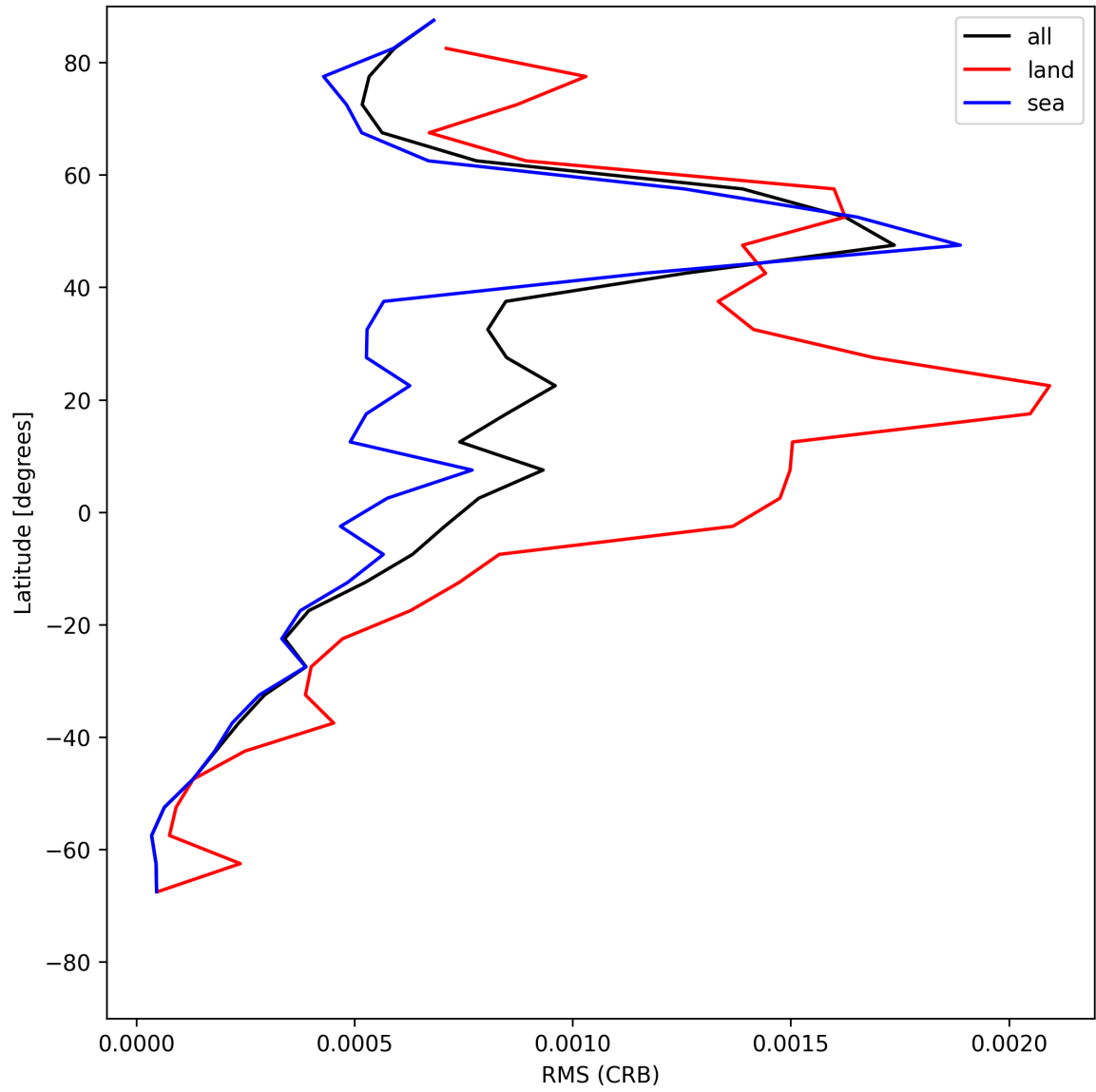
Figure 32: Zonal average of “RMS (CRB)” for 2025-07-05 to 2025-07-07.
