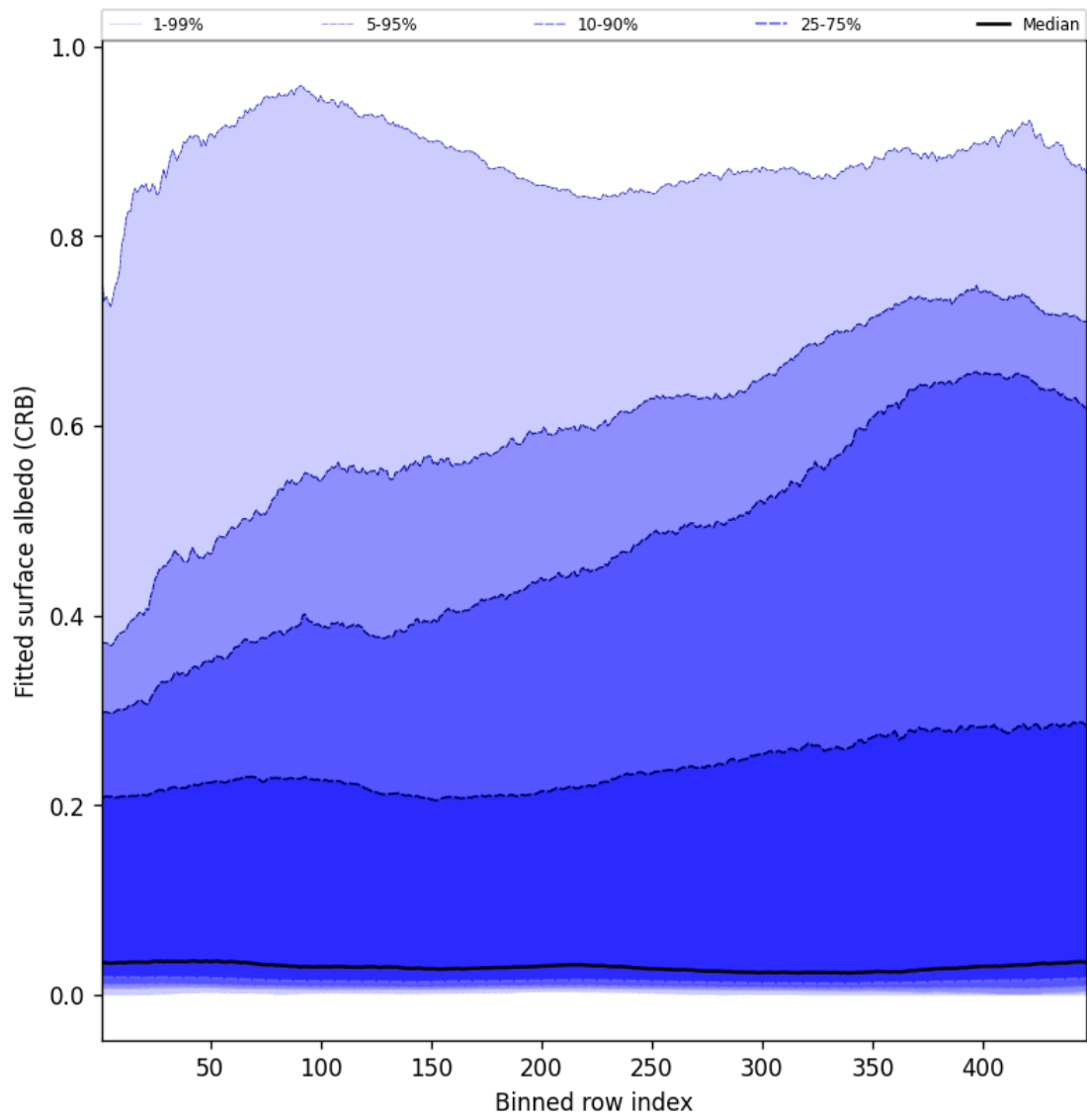
Figure 62: Along track statistics of “Fitted surface albedo (CRB)” for 2025-07-05 to 2025-07-07
