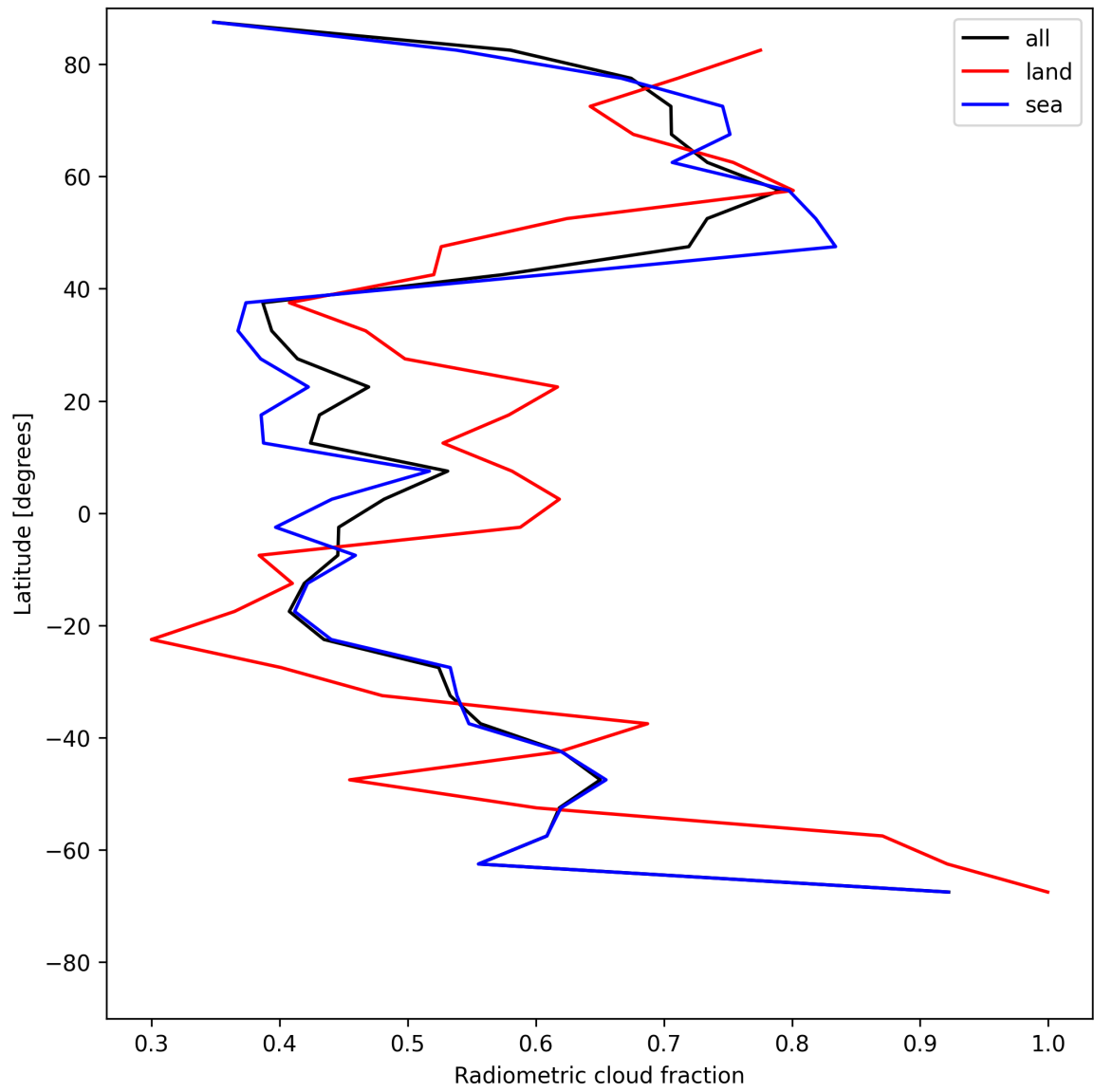
Figure 23: Zonal average of “Radiometric cloud fraction” for 2025-07-05 to 2025-07-07.
