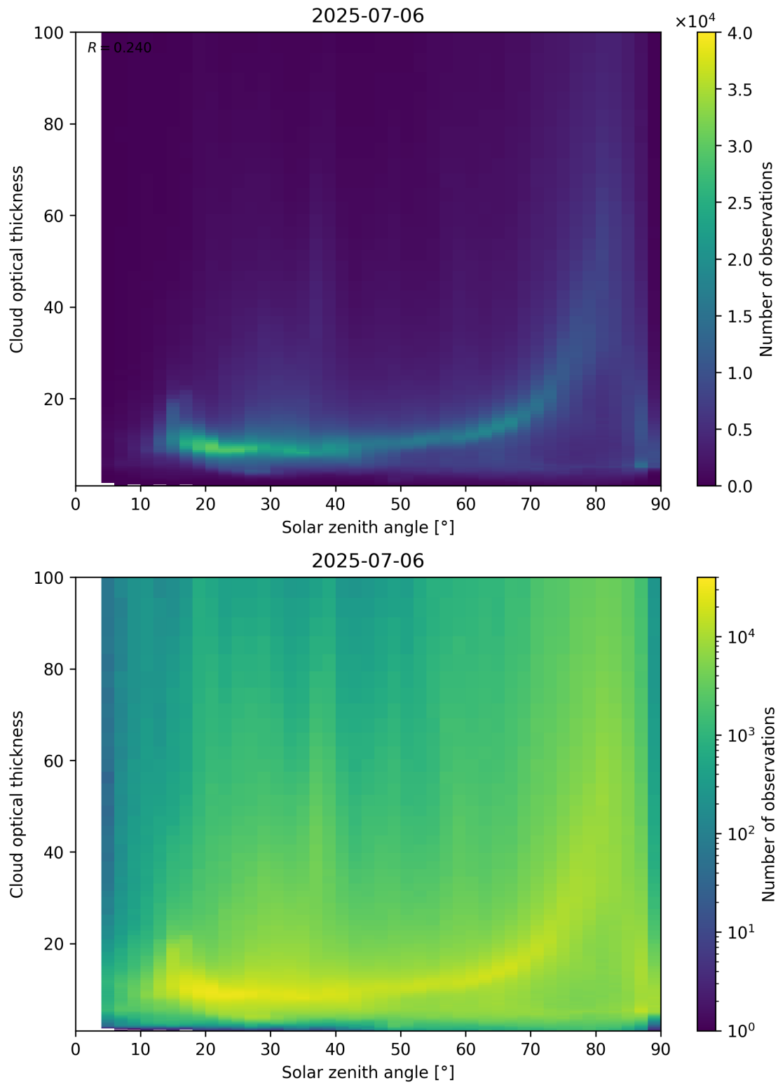
Figure 103: Scatter density plot of “Solar zenith angle” against “Cloud optical thickness” for 2025-07-05 to 2025-07-07.
