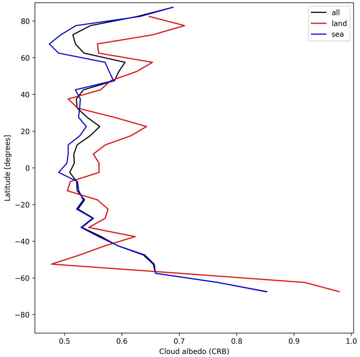
Figure 28: Zonal average of “Cloud albedo (CRB)” for 2025-07-05 to 2025-07-07.
