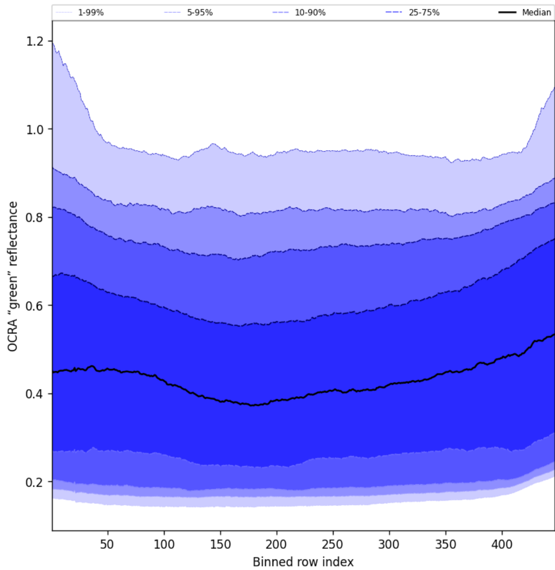
Figure 68: Along track statistics of “OCRA “green” reflectance” for 2025-07-05 to 2025-07-07
