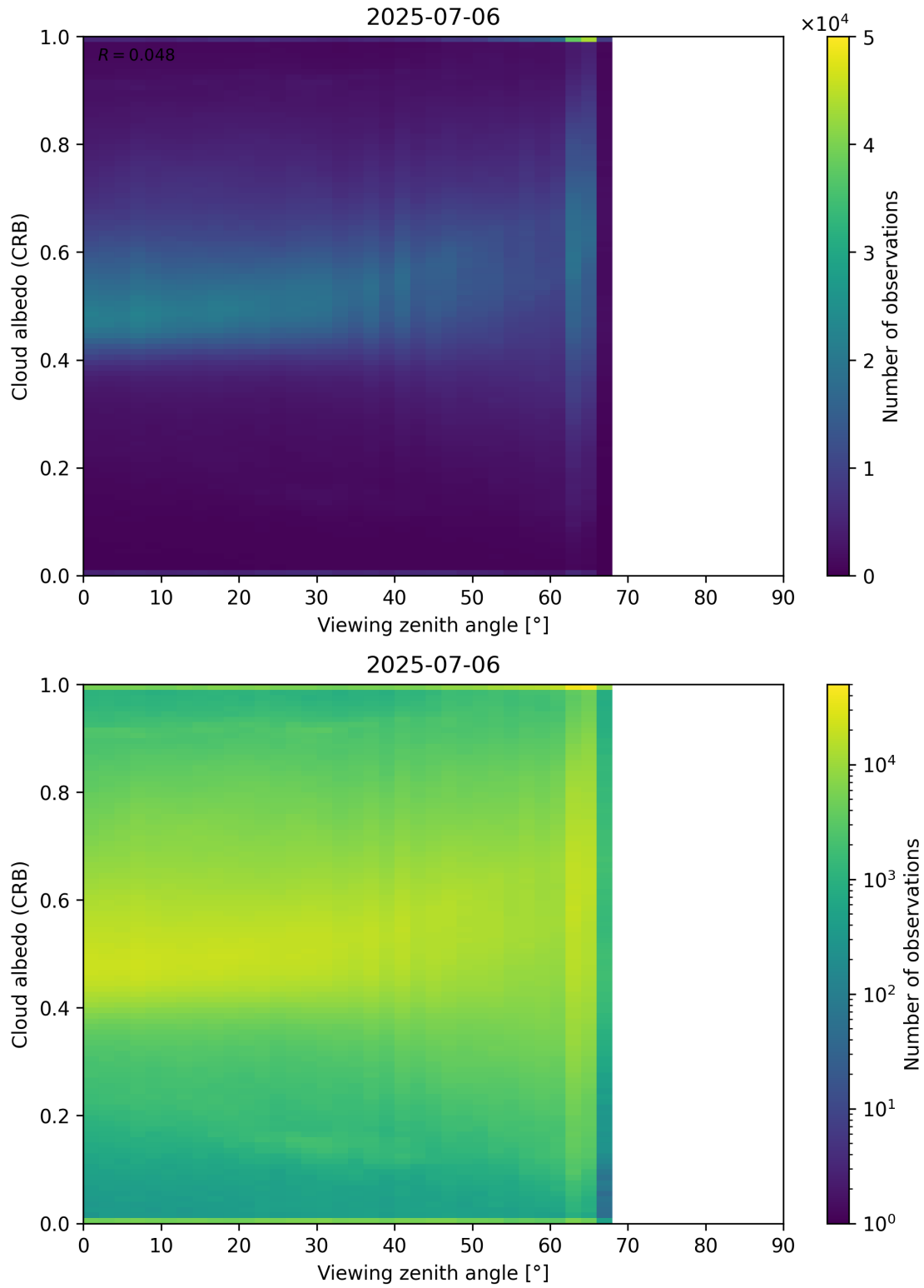
Figure 106: Scatter density plot of “Viewing zenith angle” against “Cloud albedo (CRB)” for 2025-07-05 to 2025-07-07.
