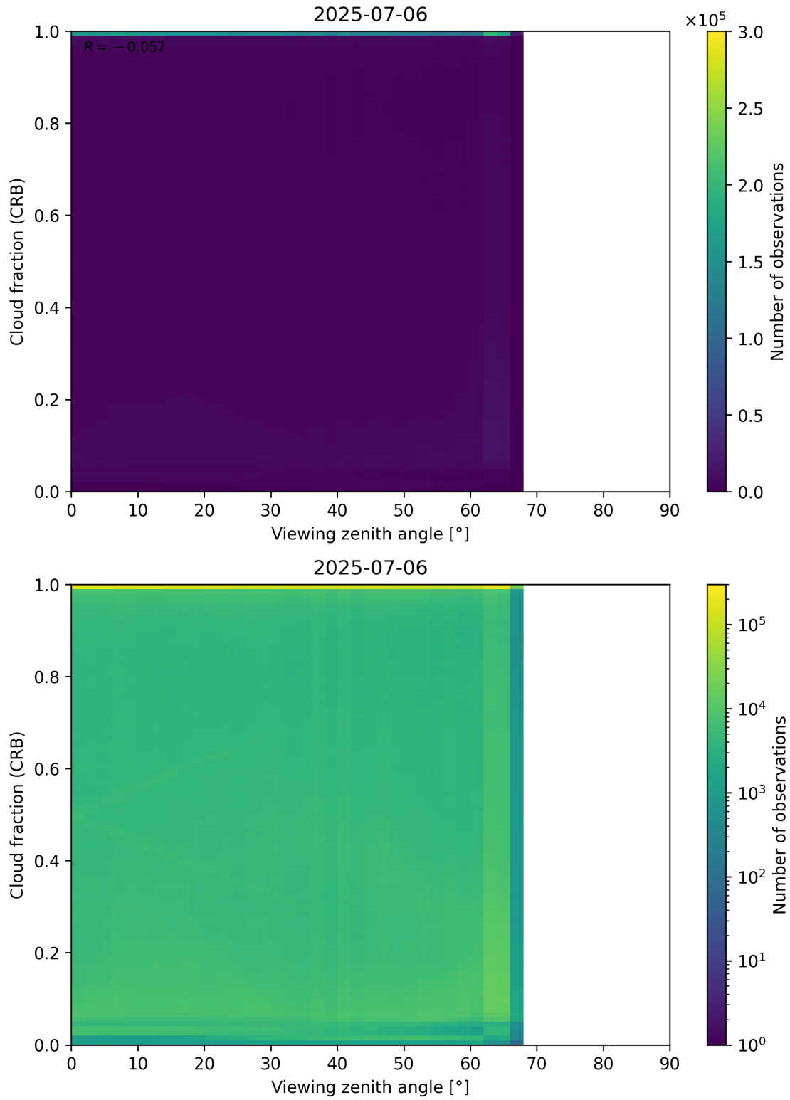
Figure 109: Scatter density plot of “Viewing zenith angle” against “Cloud fraction (CRB)” for 2025-07-05 to 2025-07-07.
