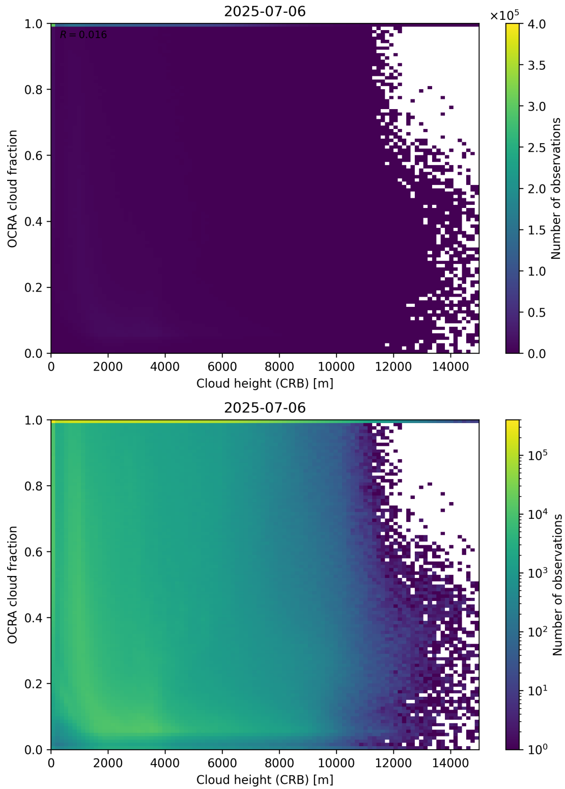
Figure 81: Scatter density plot of “Cloud height (CRB)” against “OCRA cloud fraction” for 2025-07-05 to 2025-07-07.
