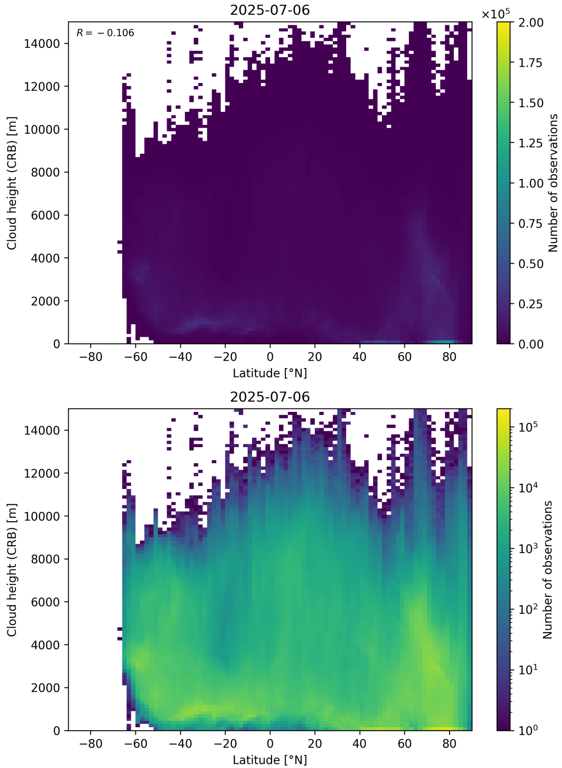
Figure 95: Scatter density plot of “Latitude” against “Cloud height (CRB)” for 2025-07-05 to 2025-07-07.
