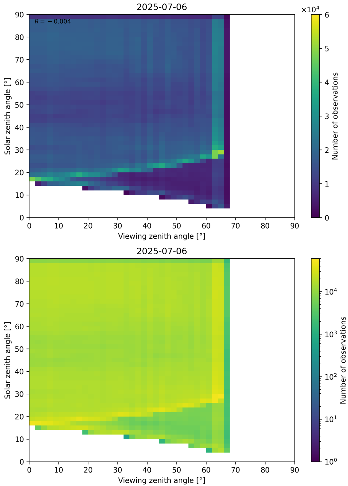
Figure 114: Scatter density plot of “Viewing zenith angle” against “Solar zenith angle” for 2025-07-05 to 2025-07-07.
