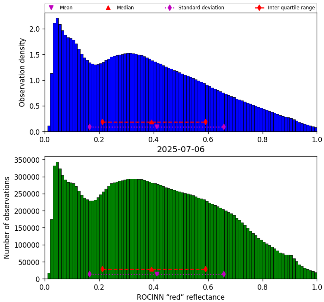
Figure 53: Histogram of “ROCINN “red” reflectance” for 2025-07-05 to 2025-07-07
