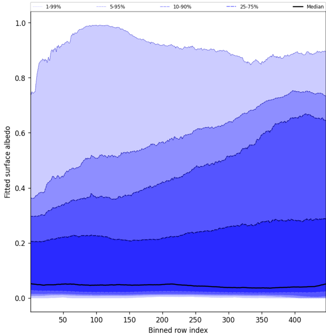
Figure 61: Along track statistics of “Fitted surface albedo” for 2025-07-05 to 2025-07-07
