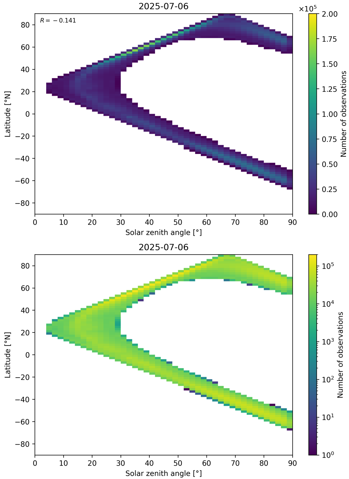
Figure 105: Scatter density plot of “Solar zenith angle” against “Latitude” for 2025-07-05 to 2025-07-07.
