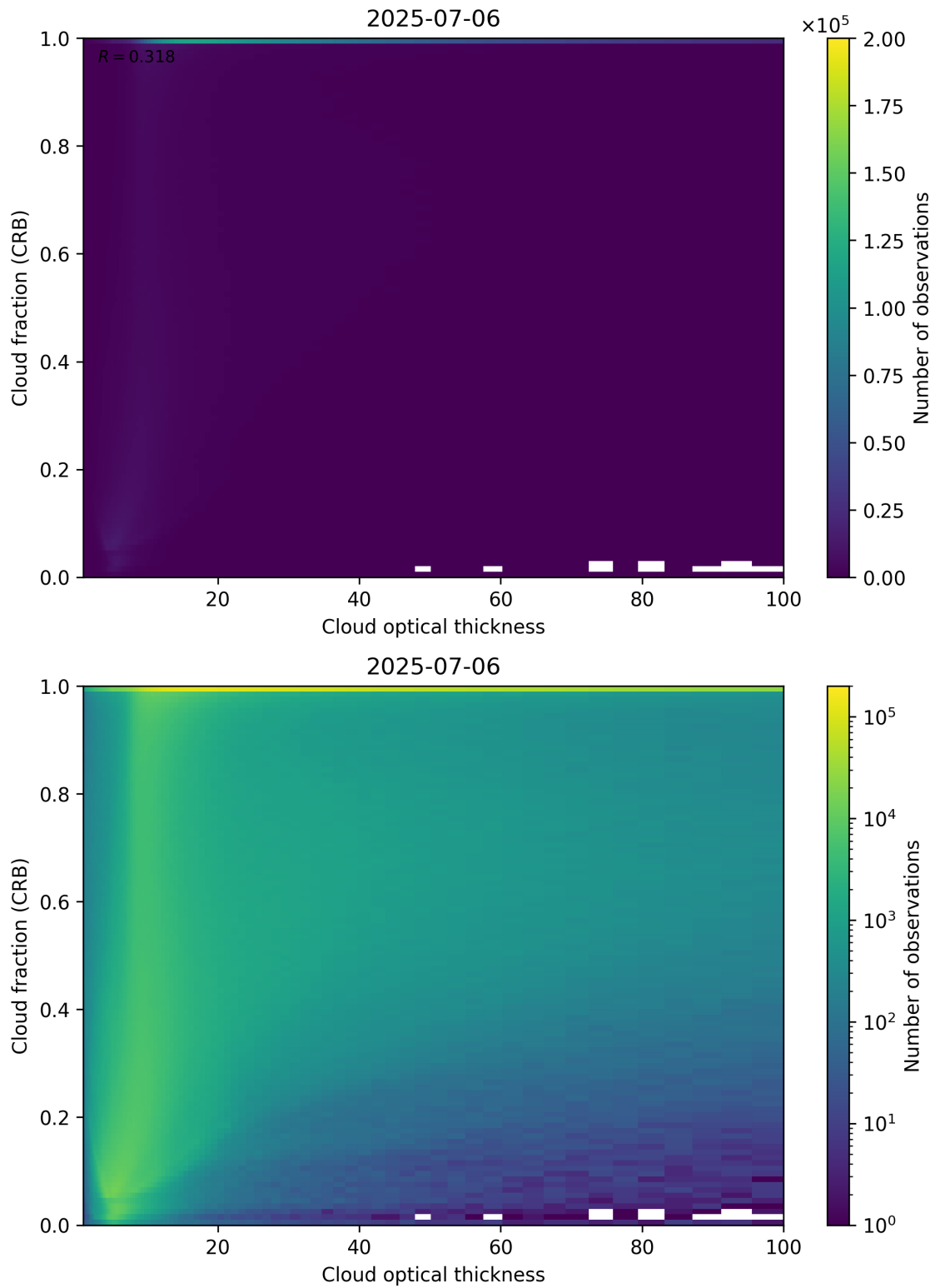
Figure 84: Scatter density plot of “Cloud optical thickness” against “Cloud fraction (CRB)” for 2025-07-05 to 2025-07-07.
