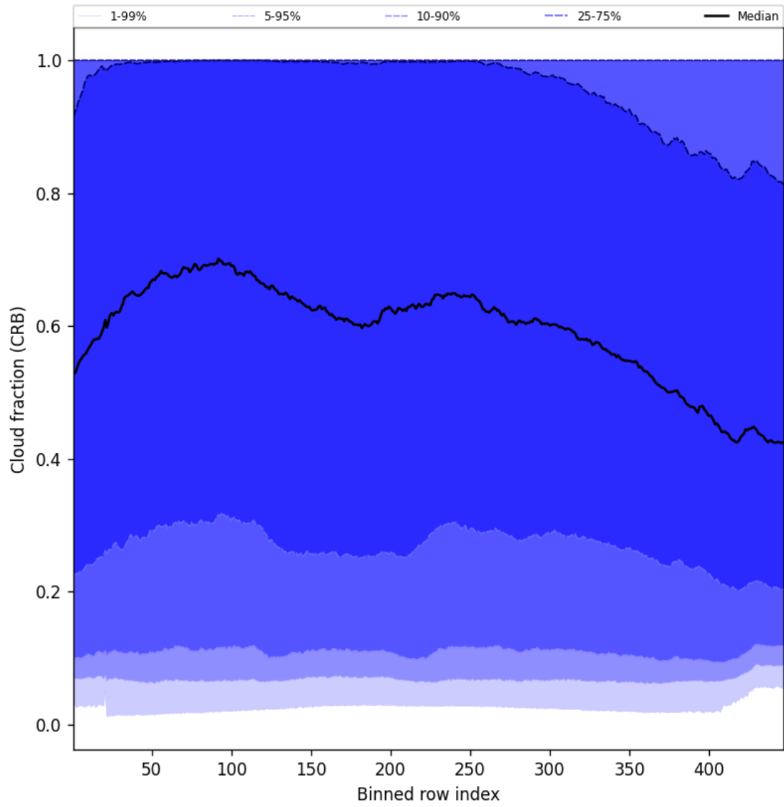
Figure 58: Along track statistics of “Cloud fraction (CRB)” for 2025-07-05 to 2025-07-07
