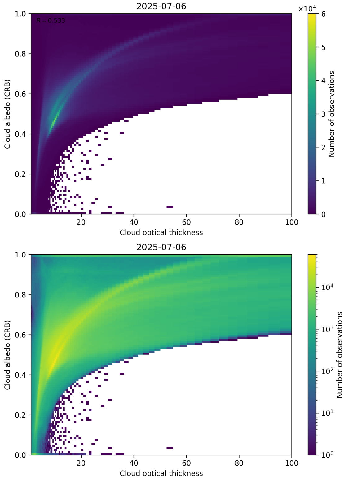
Figure 82: Scatter density plot of “Cloud optical thickness” against “Cloud albedo (CRB)” for 2025-07-05 to 2025-07-07.
