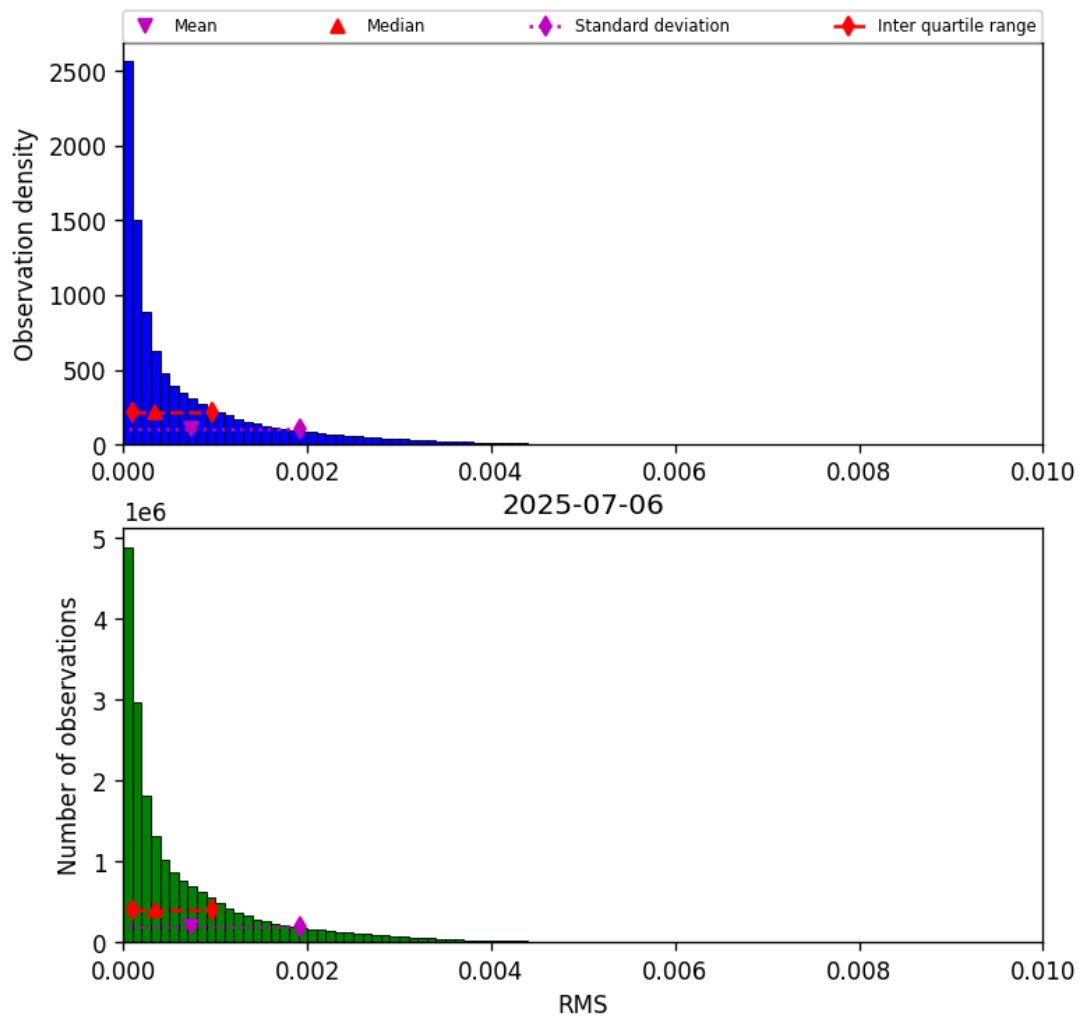
Figure 47: Histogram of “RMS” for 2025-07-05 to 2025-07-07
