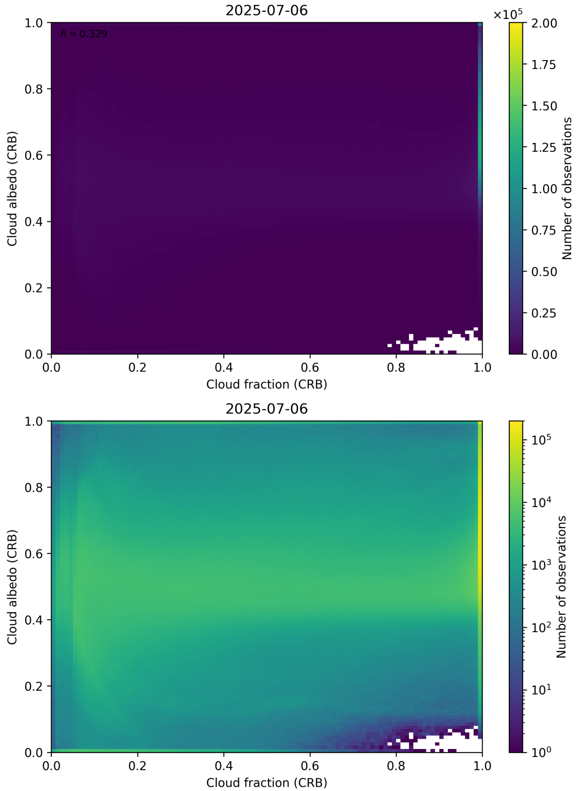
Figure 77: Scatter density plot of “Cloud fraction (CRB)” against “Cloud albedo (CRB)” for 2025-07-05 to 2025-07-07.
