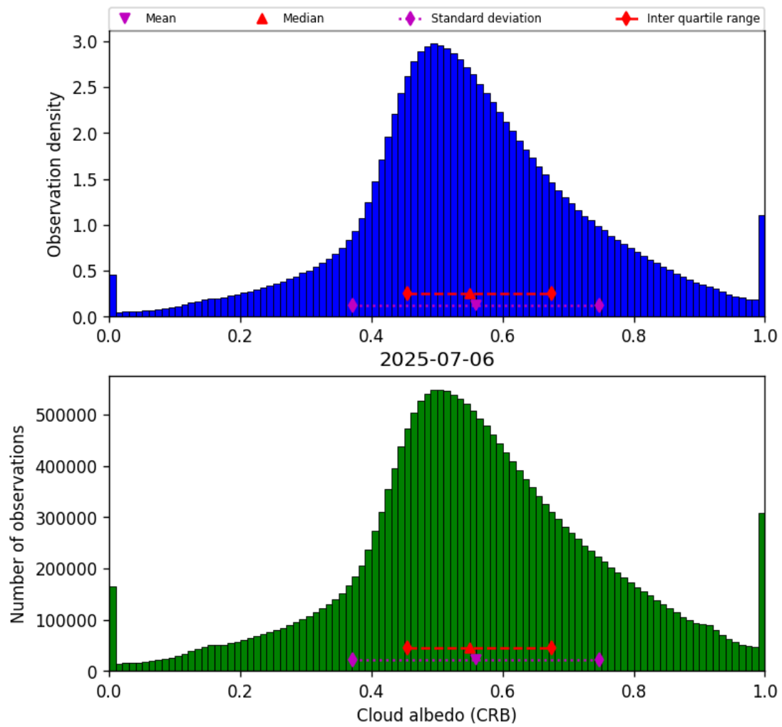
Figure 44: Histogram of “Cloud albedo (CRB)” for 2025-07-05 to 2025-07-07
