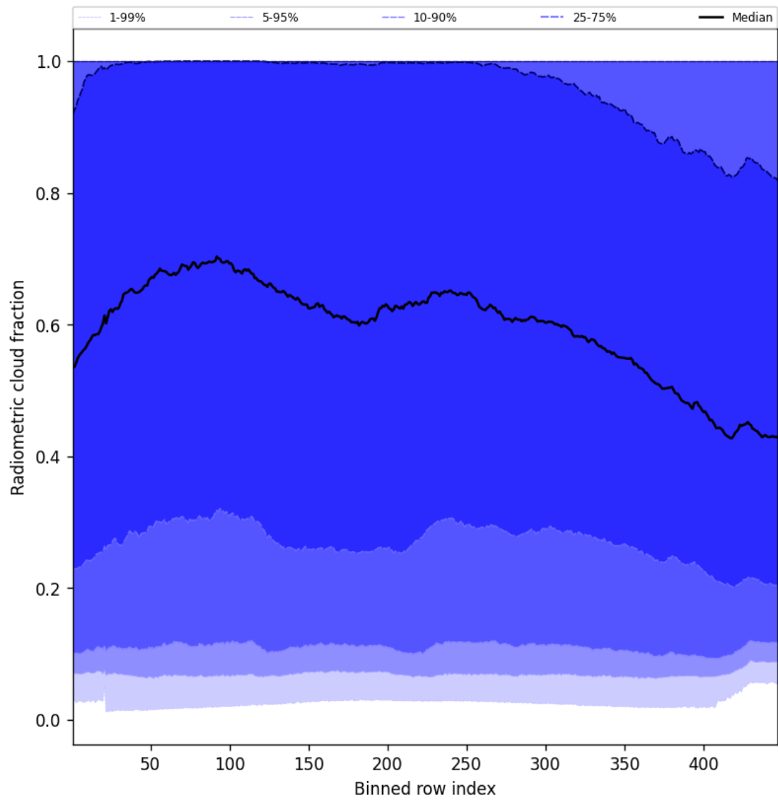
Figure 55: Along track statistics of “Radiometric cloud fraction” for 2025-07-05 to 2025-07-07
