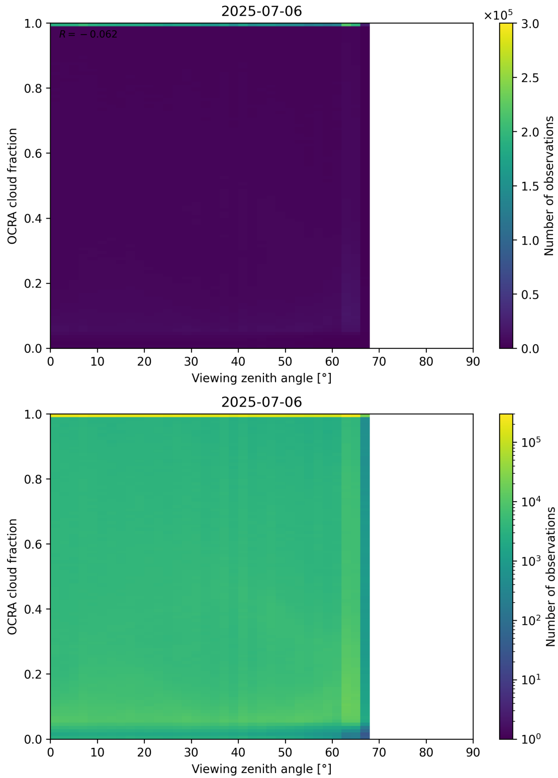
Figure 108: Scatter density plot of “Viewing zenith angle” against “OCRA cloud fraction” for 2025-07-05 to 2025-07-07.
