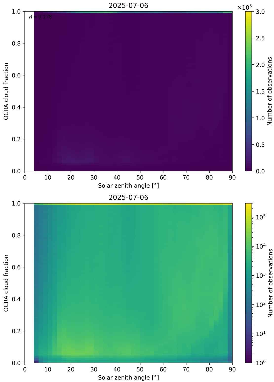
Figure 100: Scatter density plot of “Solar zenith angle” against “OCRA cloud fraction” for 2025-07-05 to 2025-07-07.
