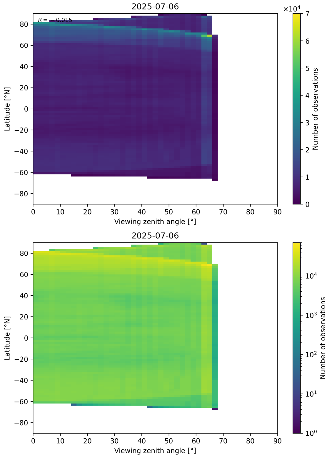
Figure 113: Scatter density plot of “Viewing zenith angle” against “Latitude” for 2025-07-05 to 2025-07-07.
