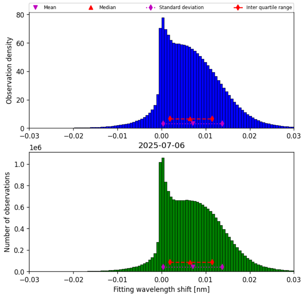
Figure 49: Histogram of “Fitting wavelength shift” for 2025-07-05 to 2025-07-07
