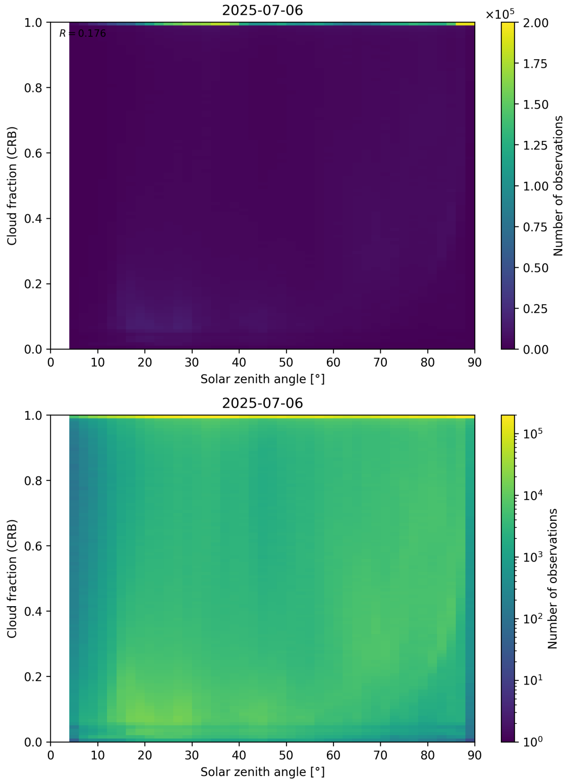
Figure 101: Scatter density plot of “Solar zenith angle” against “Cloud fraction (CRB)” for 2025-07-05 to 2025-07-07.
