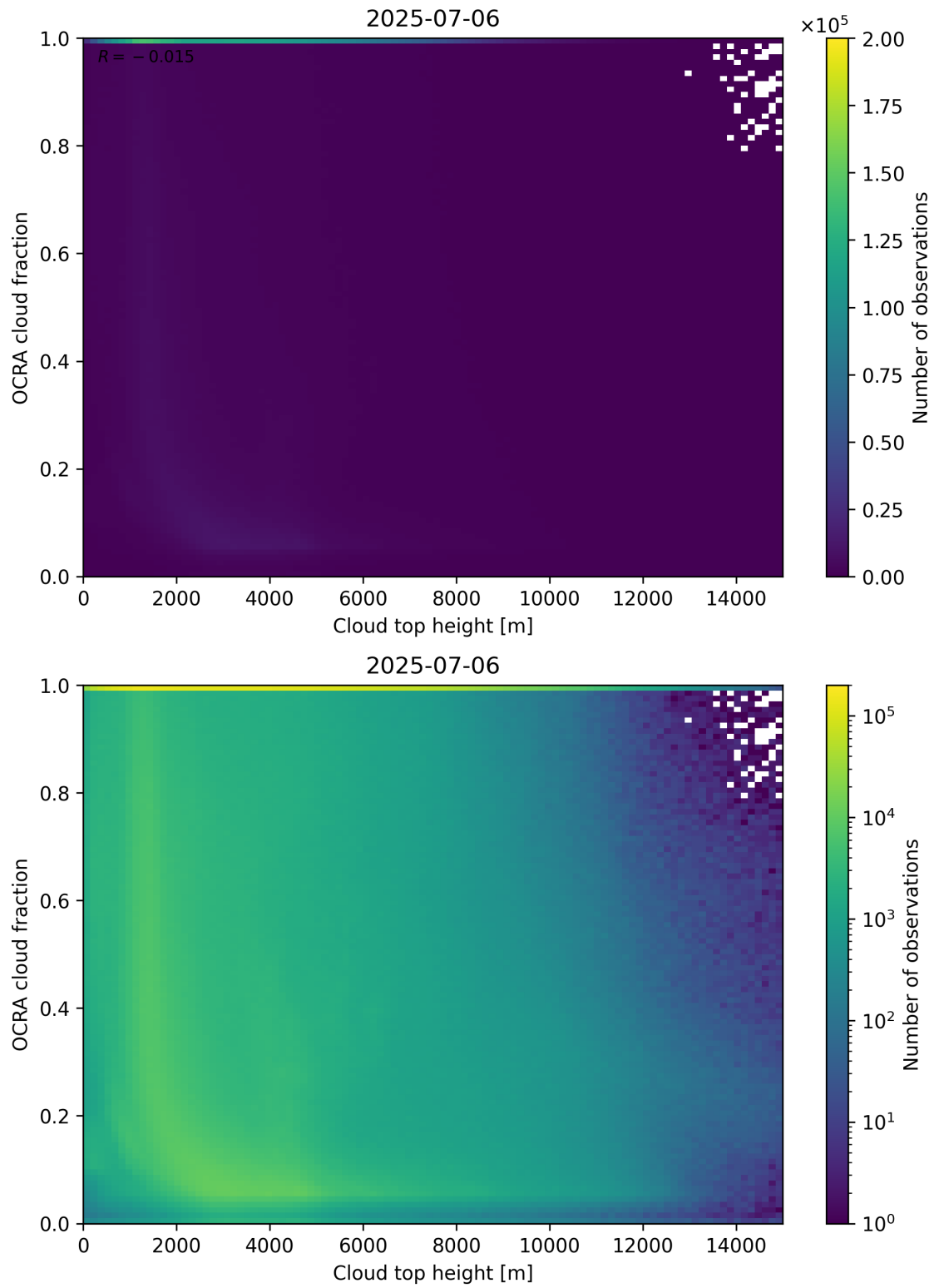
Figure 87: Scatter density plot of “Cloud top height” against “OCRA cloud fraction” for 2025-07-05 to 2025-07-07.
