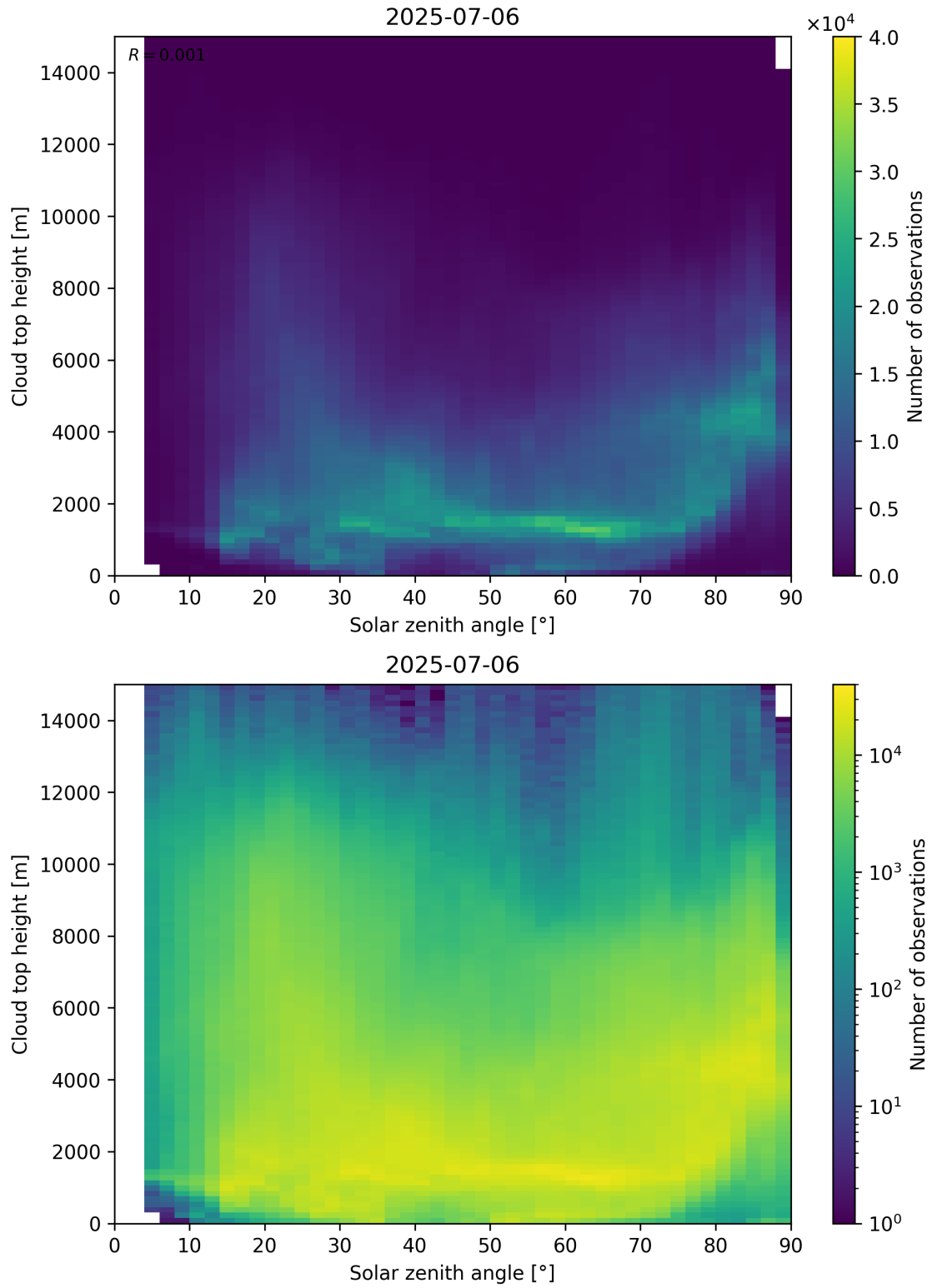
Figure 104: Scatter density plot of “Solar zenith angle” against “Cloud top height” for 2025-07-05 to 2025-07-07.
