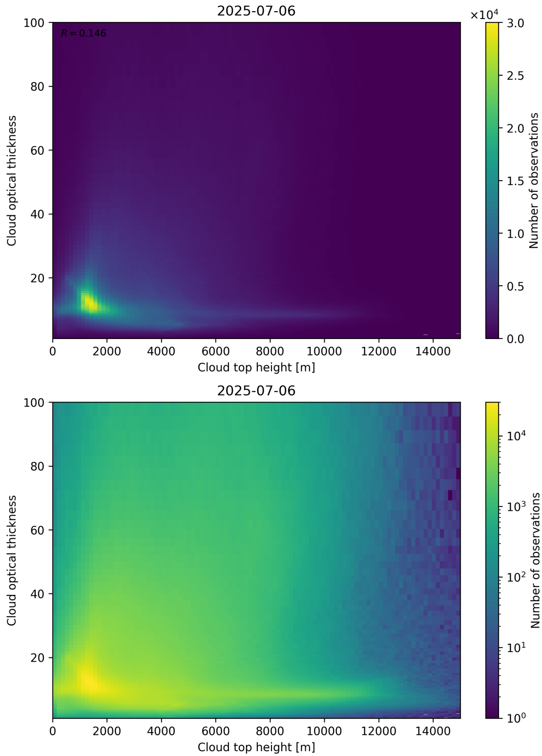
Figure 90: Scatter density plot of “Cloud top height” against “Cloud optical thickness” for 2025-07-05 to 2025-07-07.
