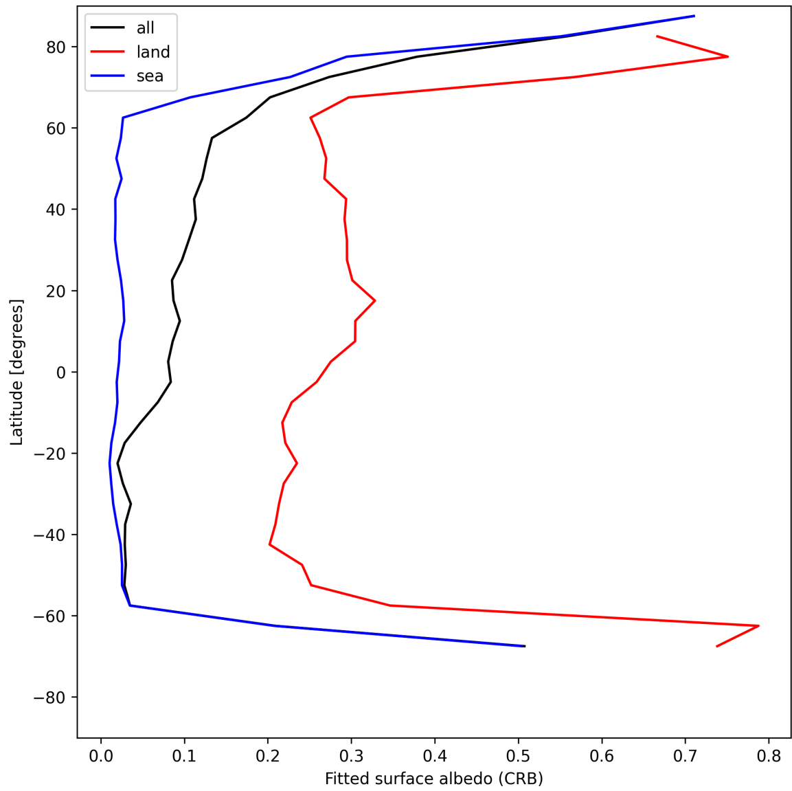
Figure 30: Zonal average of “Fitted surface albedo (CRB)” for 2025-07-05 to 2025-07-07.
