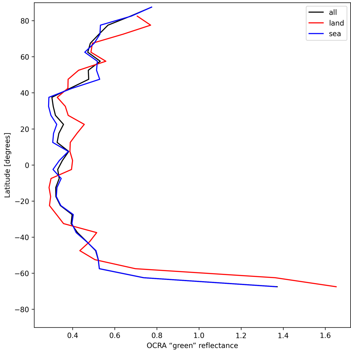
Figure 36: Zonal average of “OCRA “green” reflectance” for 2025-07-05 to 2025-07-07.
