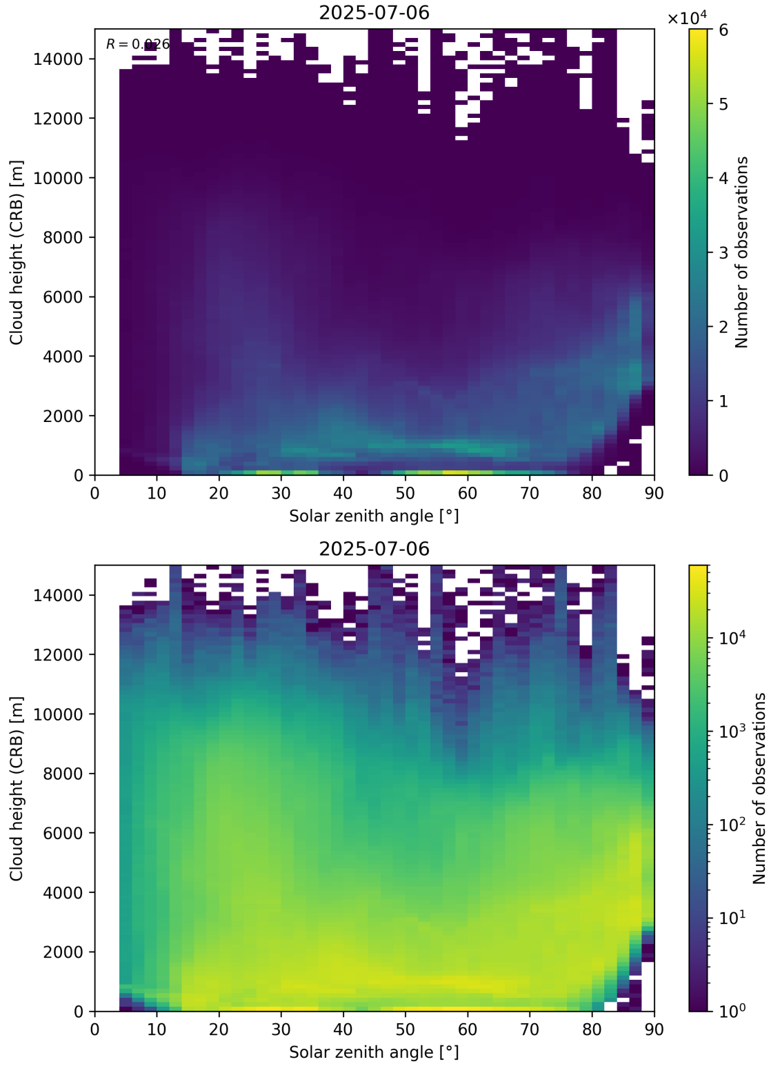
Figure 102: Scatter density plot of “Solar zenith angle” against “Cloud height (CRB)” for 2025-07-05 to 2025-07-07.
