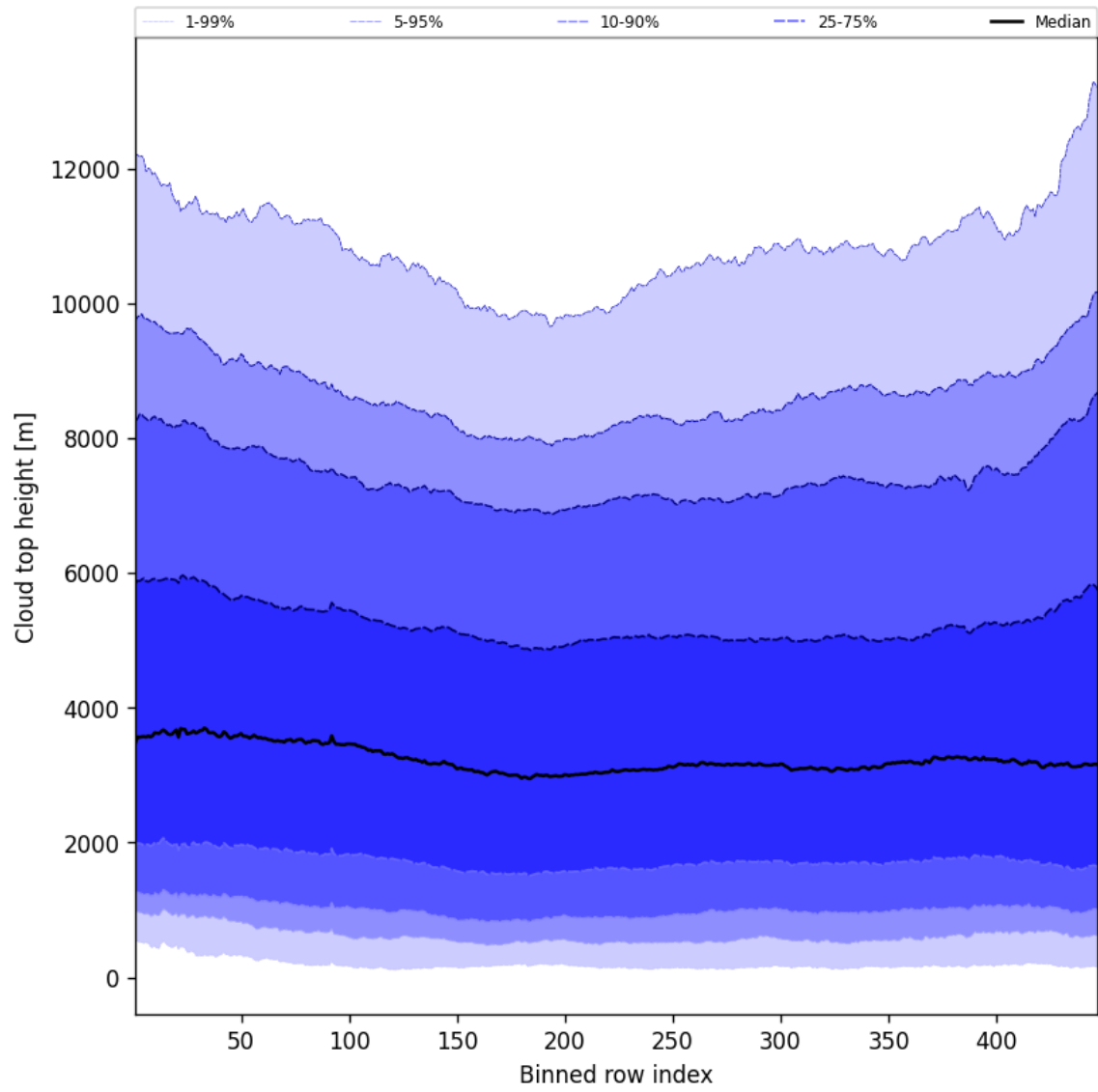
Figure 56: Along track statistics of “Cloud top height” for 2025-07-05 to 2025-07-07
