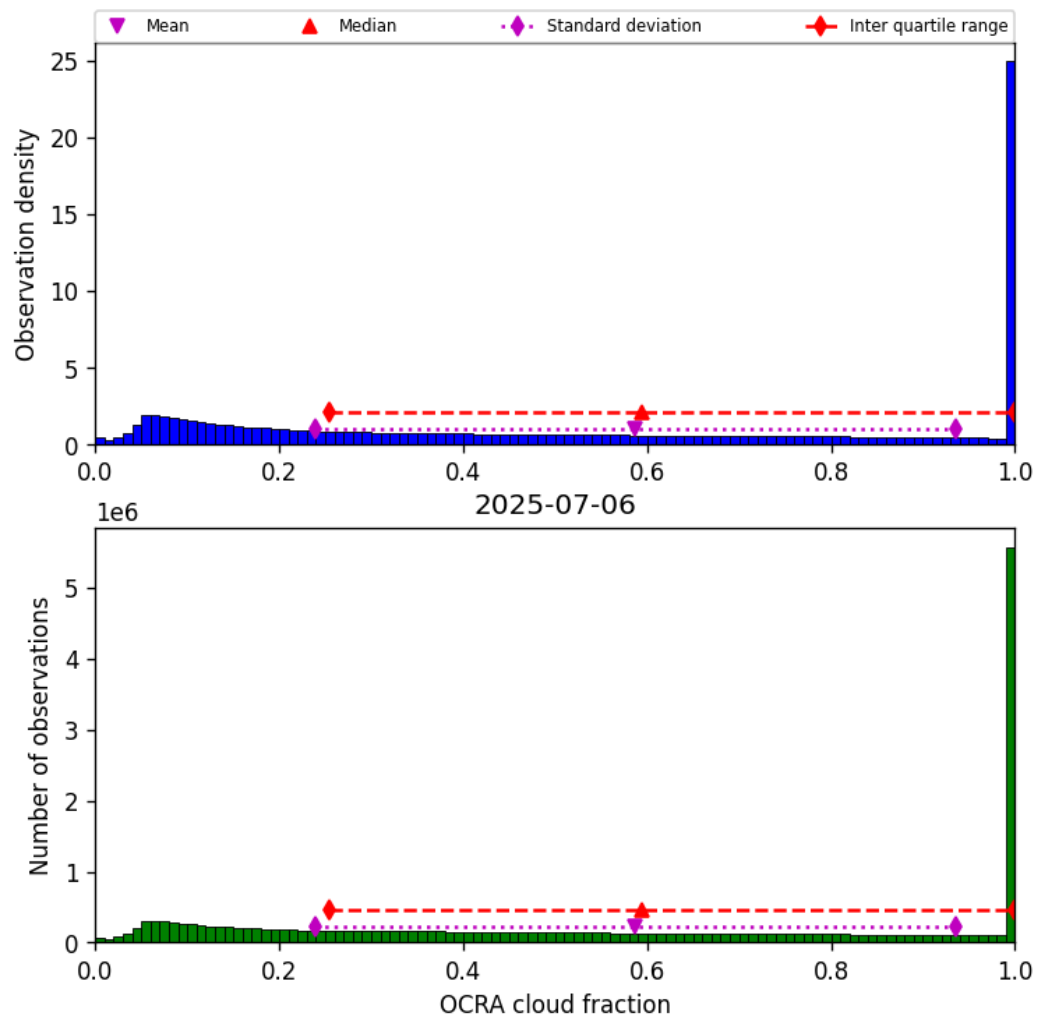
Figure 50: Histogram of “OCRA cloud fraction” for 2025-07-05 to 2025-07-07
