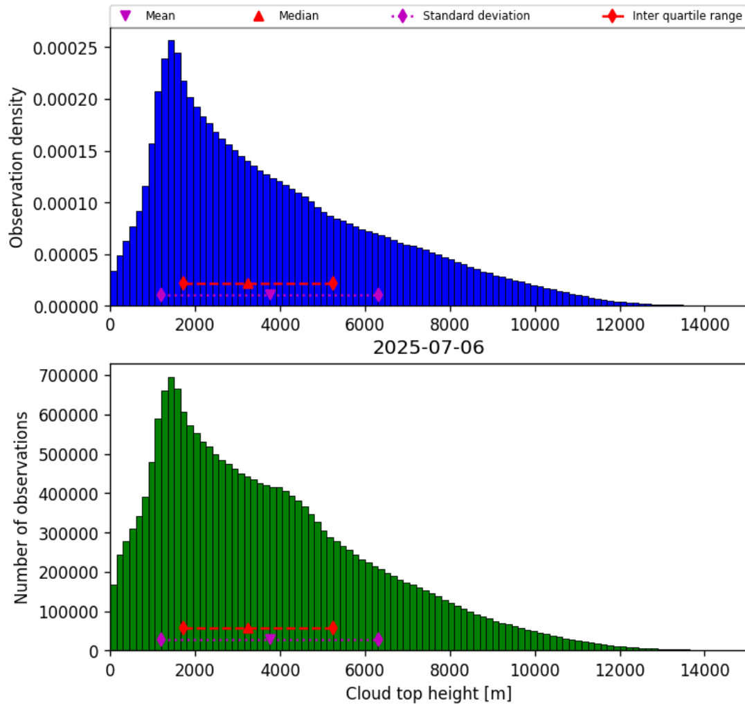
Figure 40: Histogram of “Cloud top height” for 2025-07-05 to 2025-07-07
