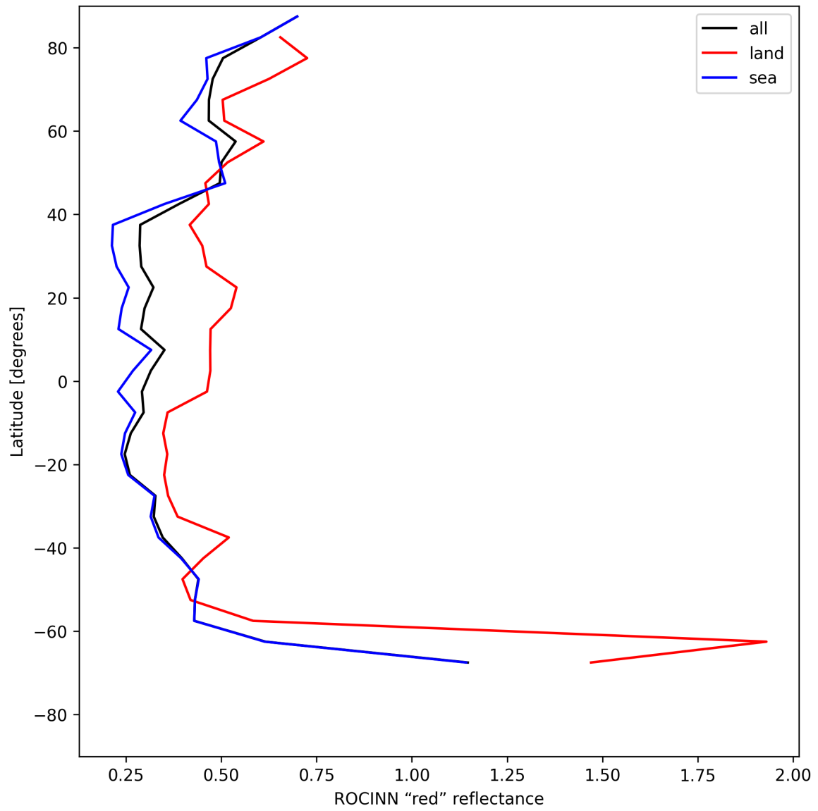
Figure 37: Zonal average of “ROCINN “red” reflectance” for 2025-07-05 to 2025-07-07.
