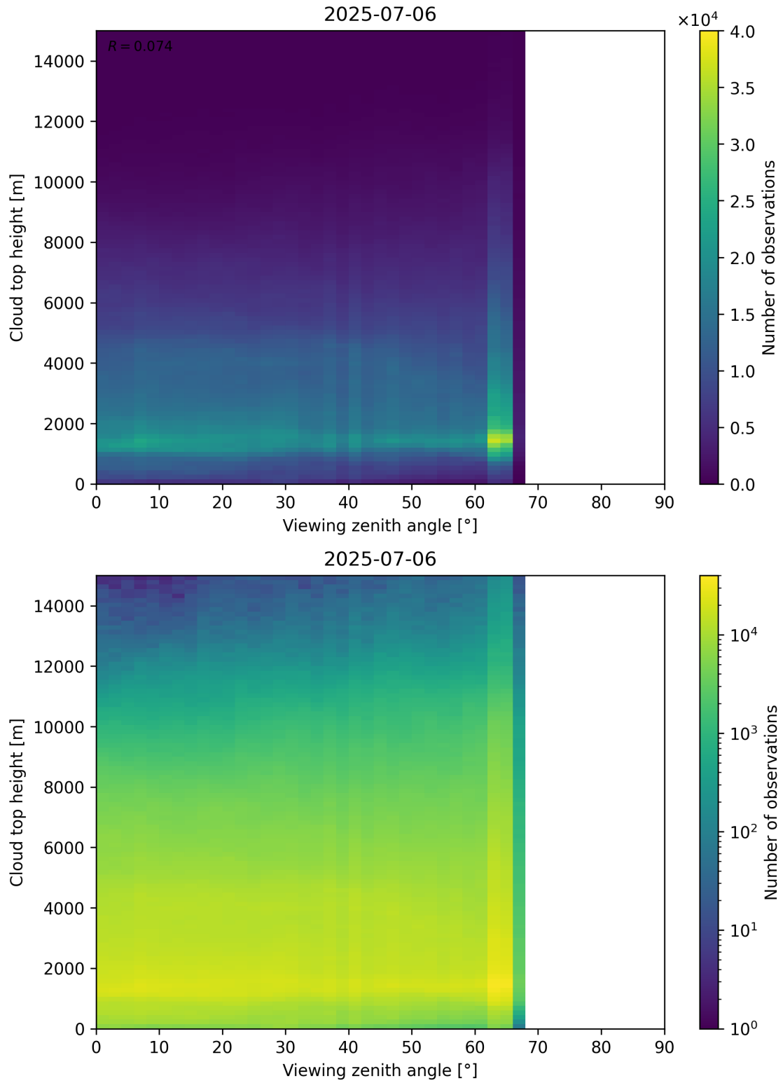
Figure 112: Scatter density plot of “Viewing zenith angle” against “Cloud top height” for 2025-07-05 to 2025-07-07.
