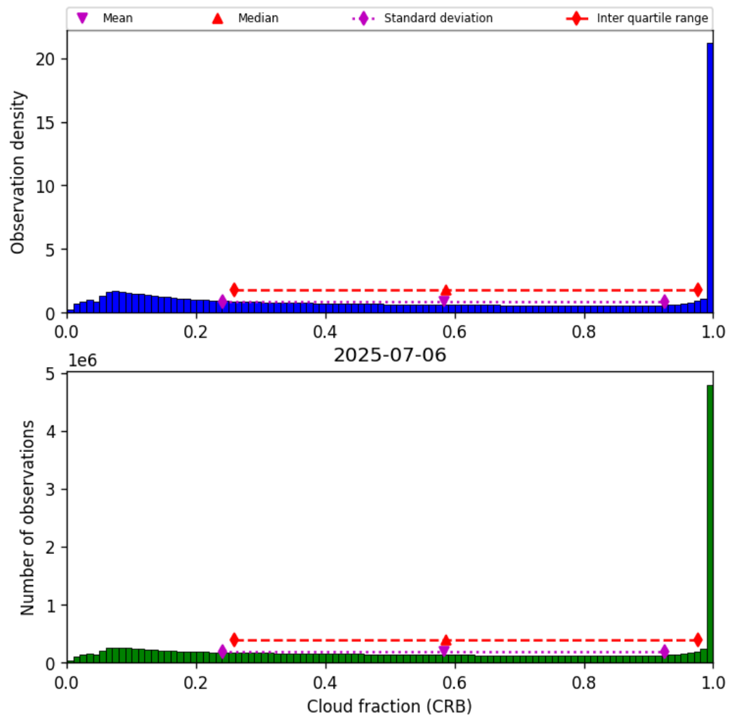
Figure 42: Histogram of “Cloud fraction (CRB)” for 2025-07-05 to 2025-07-07
