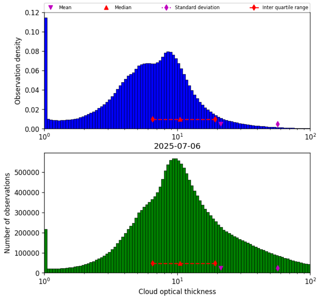
Figure 41: Histogram of “Cloud optical thickness” for 2025-07-05 to 2025-07-07
