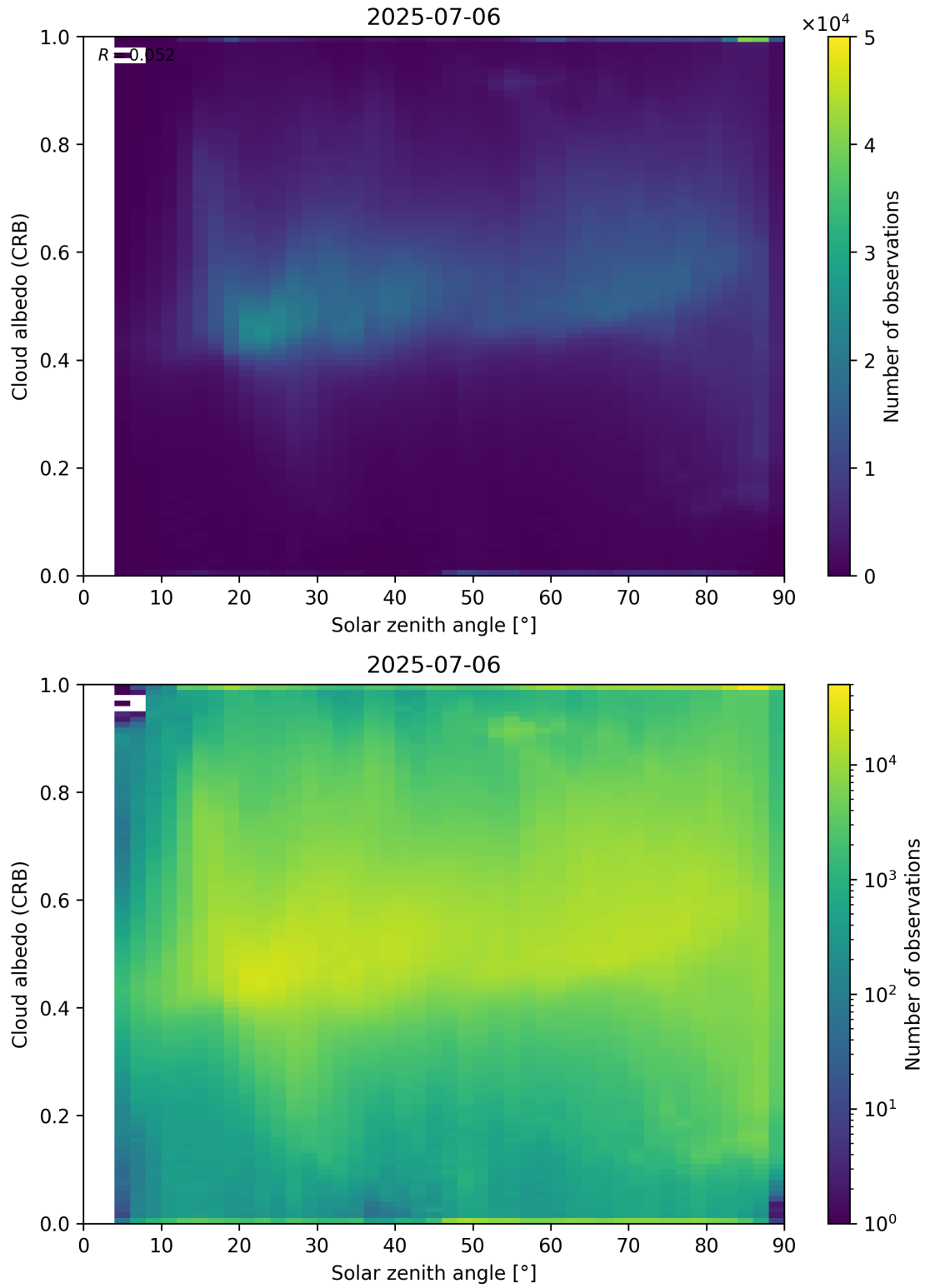
Figure 98: Scatter density plot of “Solar zenith angle” against “Cloud albedo (CRB)” for 2025-07-05 to 2025-07-07.
