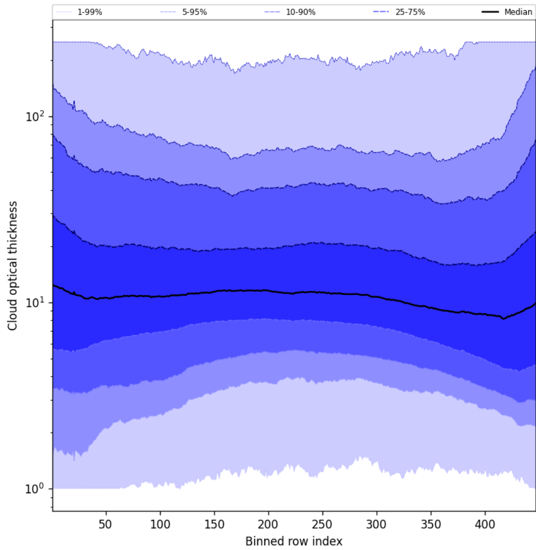
Figure 57: Along track statistics of “Cloud optical thickness” for 2025-07-05 to 2025-07-07
