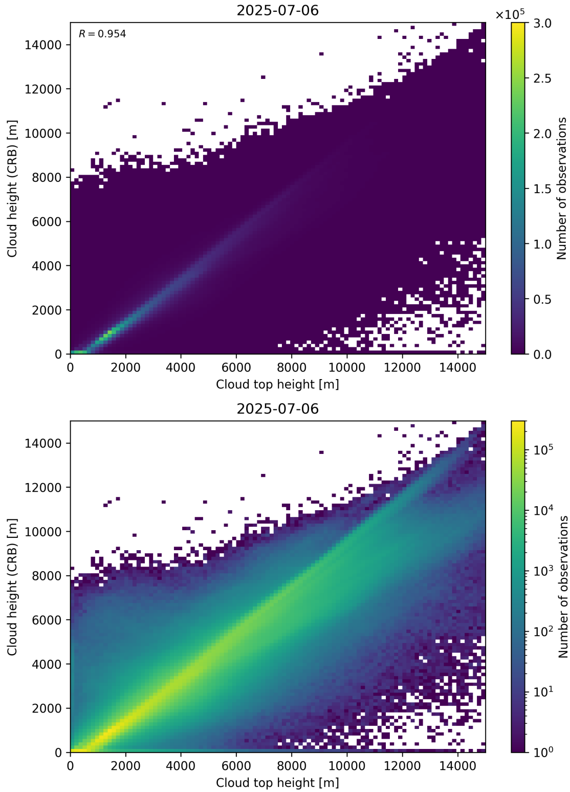
Figure 89: Scatter density plot of “Cloud top height” against “Cloud height (CRB)” for 2025-07-05 to 2025-07-07.
