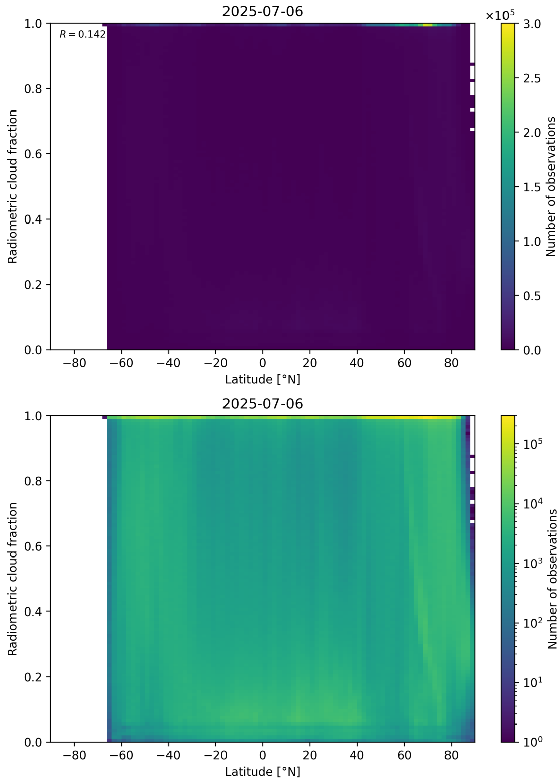
Figure 92: Scatter density plot of “Latitude” against “Radiometric cloud fraction” for 2025-07-05 to 2025-07-07.
