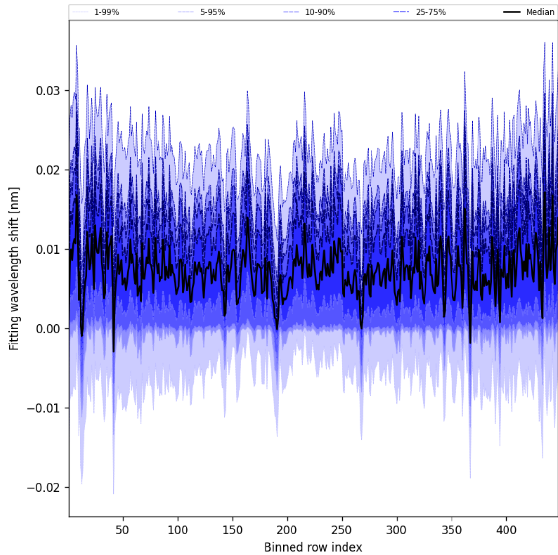
Figure 65: Along track statistics of “Fitting wavelength shift” for 2025-07-05 to 2025-07-07
