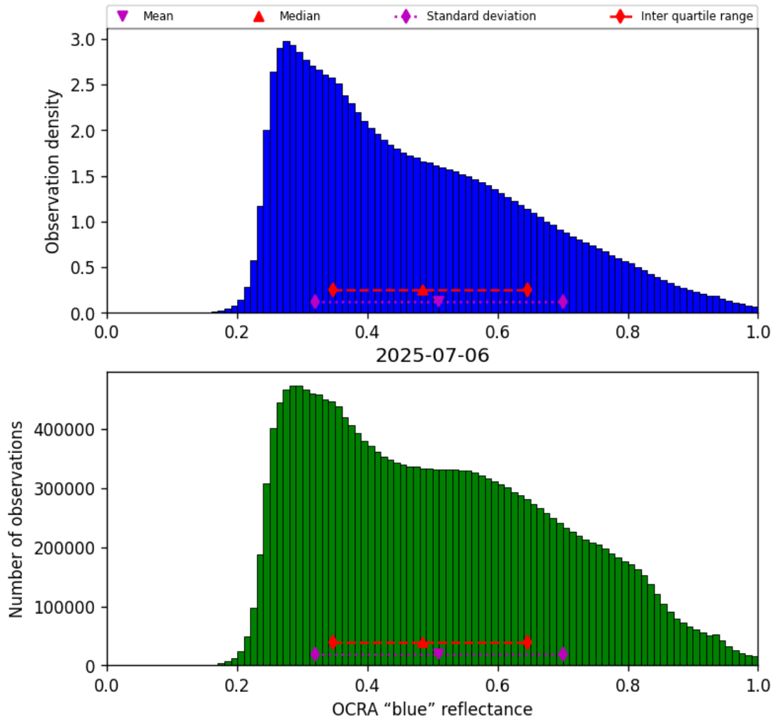
Figure 51: Histogram of “OCRA “blue” reflectance” for 2025-07-05 to 2025-07-07
