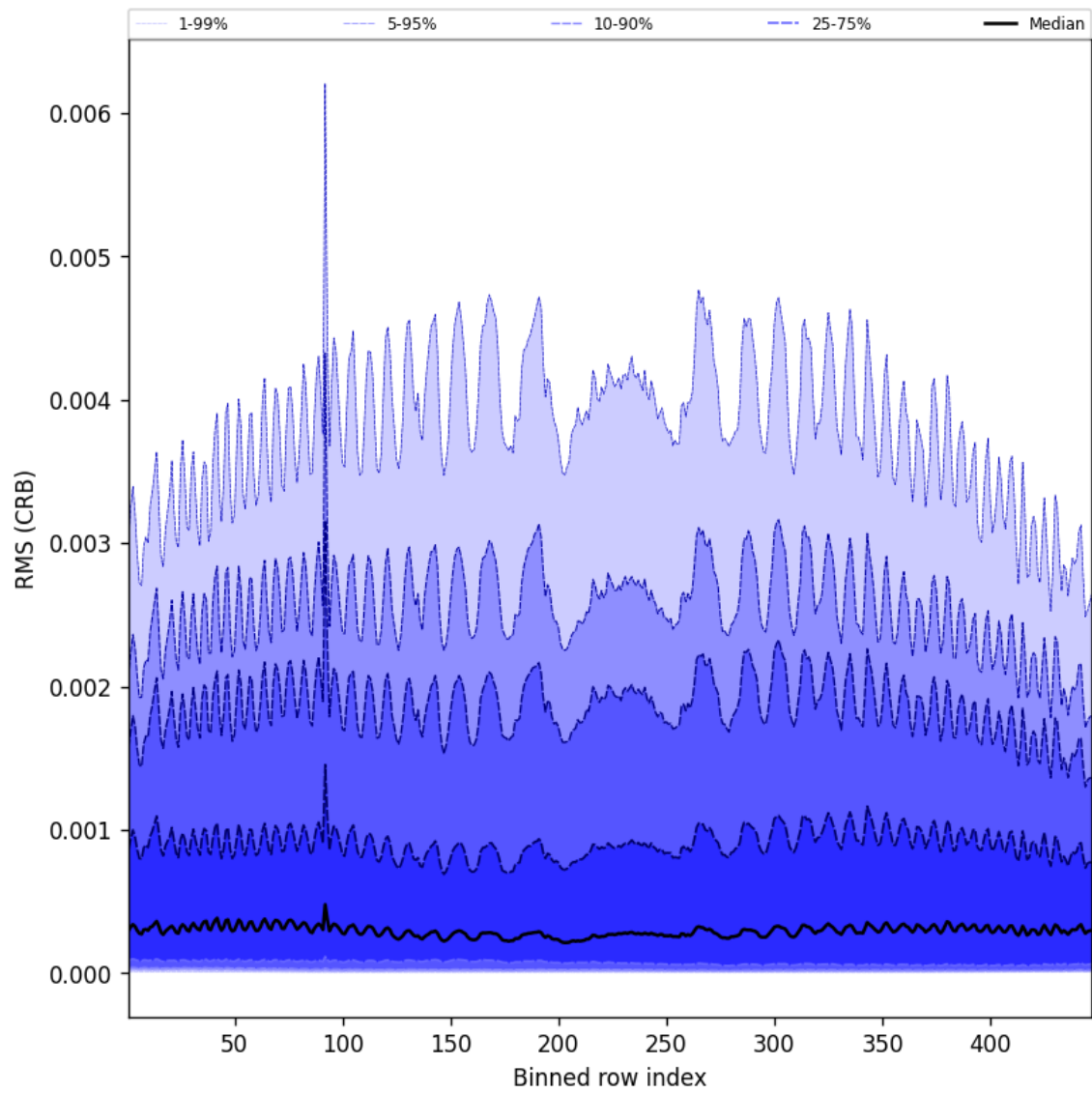
Figure 64: Along track statistics of “RMS (CRB)” for 2025-07-05 to 2025-07-07
