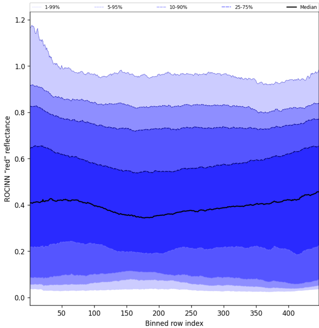
Figure 69: Along track statistics of "ROCINN "red" reflectance" for 2025-07-05 to 2025-07-07
