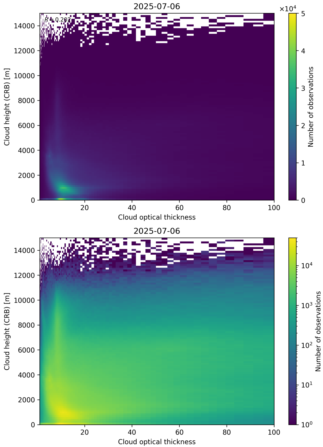
Figure 85: Scatter density plot of “Cloud optical thickness” against “Cloud height (CRB)” for 2025-07-05 to 2025-07-07.
