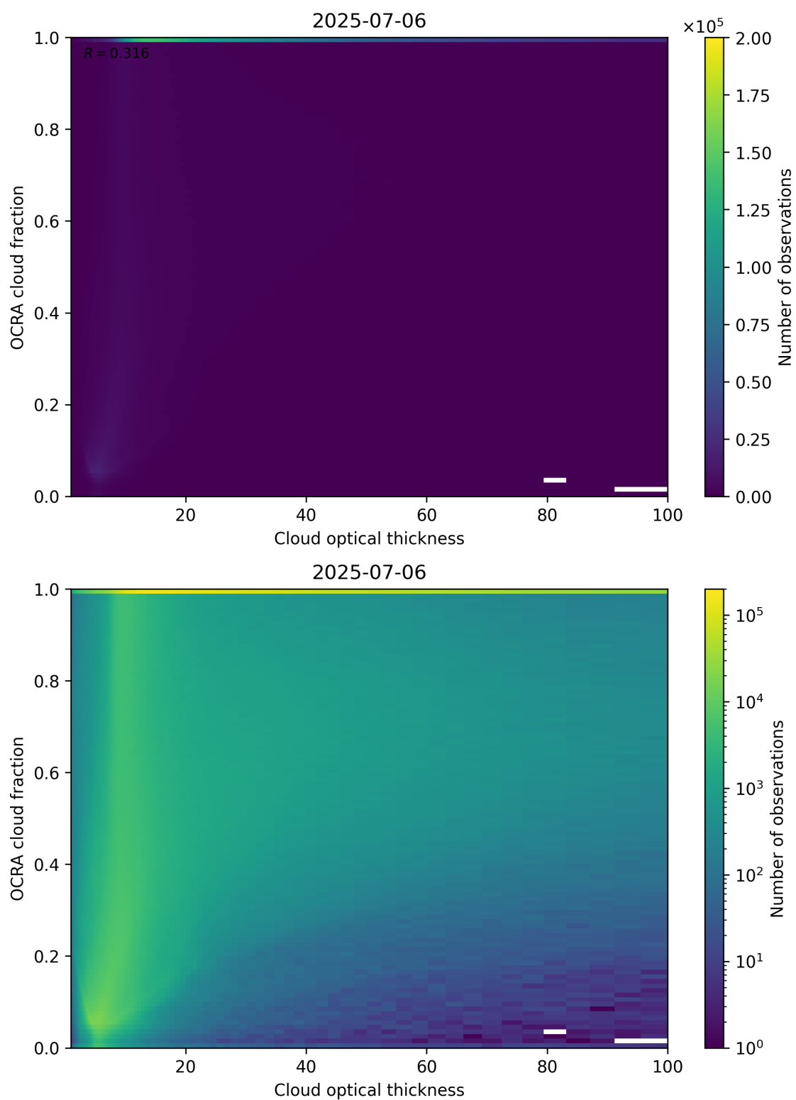
Figure 83: Scatter density plot of “Cloud optical thickness” against “OCRA cloud fraction” for 2025-07-05 to 2025-07-07.
