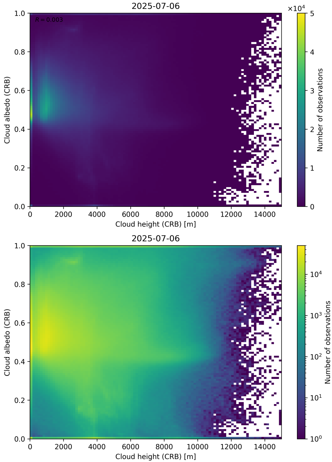
Figure 80: Scatter density plot of “Cloud height (CRB)” against “Cloud albedo (CRB)” for 2025-07-05 to 2025-07-07.
