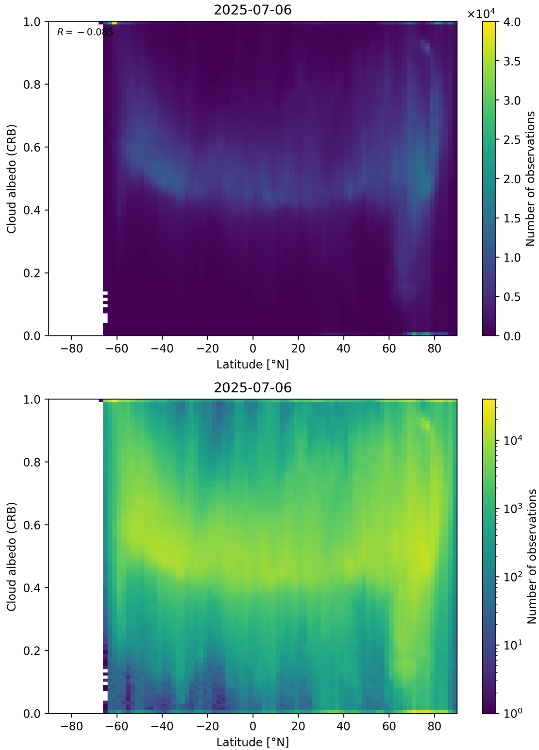
Figure 91: Scatter density plot of “Latitude” against “Cloud albedo (CRB)” for 2025-07-05 to 2025-07-07.
