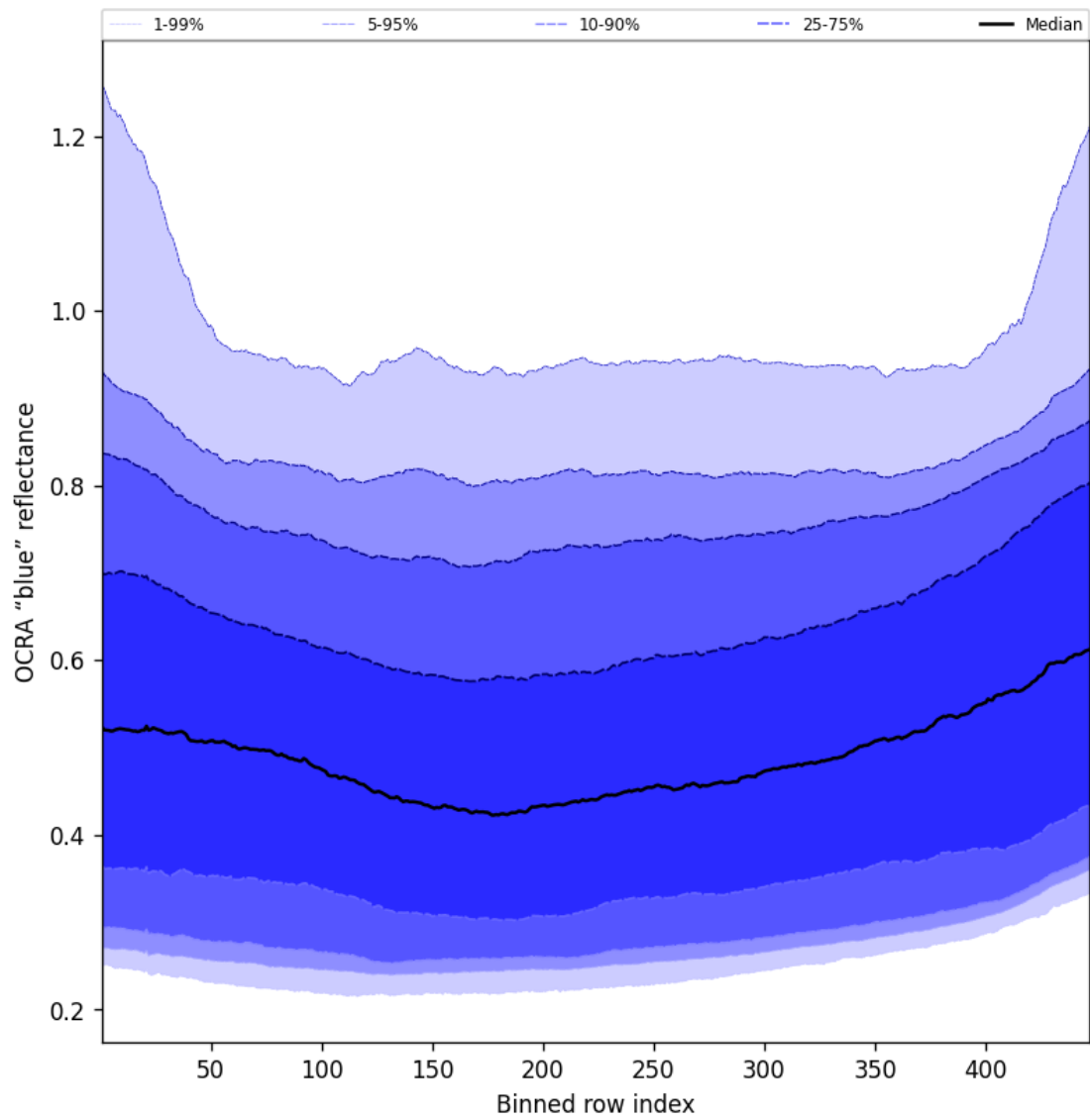
Figure 67: Along track statistics of “OCRA “blue” reflectance” for 2025-07-05 to 2025-07-07
