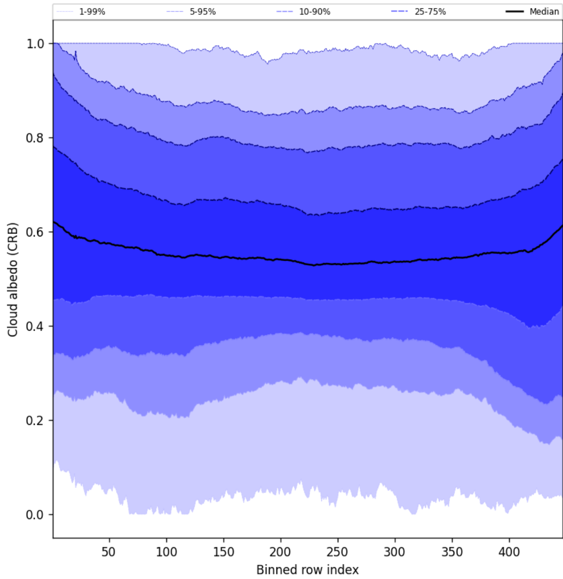
Figure 60: Along track statistics of “Cloud albedo (CRB)” for 2025-07-05 to 2025-07-07
