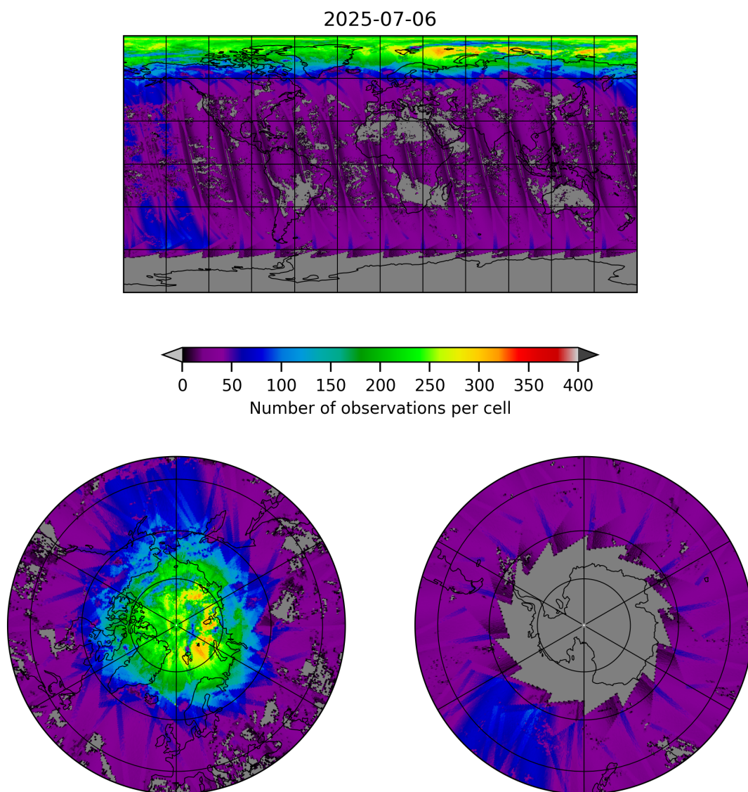
Figure 21: Map of the number of observations for 2025-07-05 to 2025-07-07
