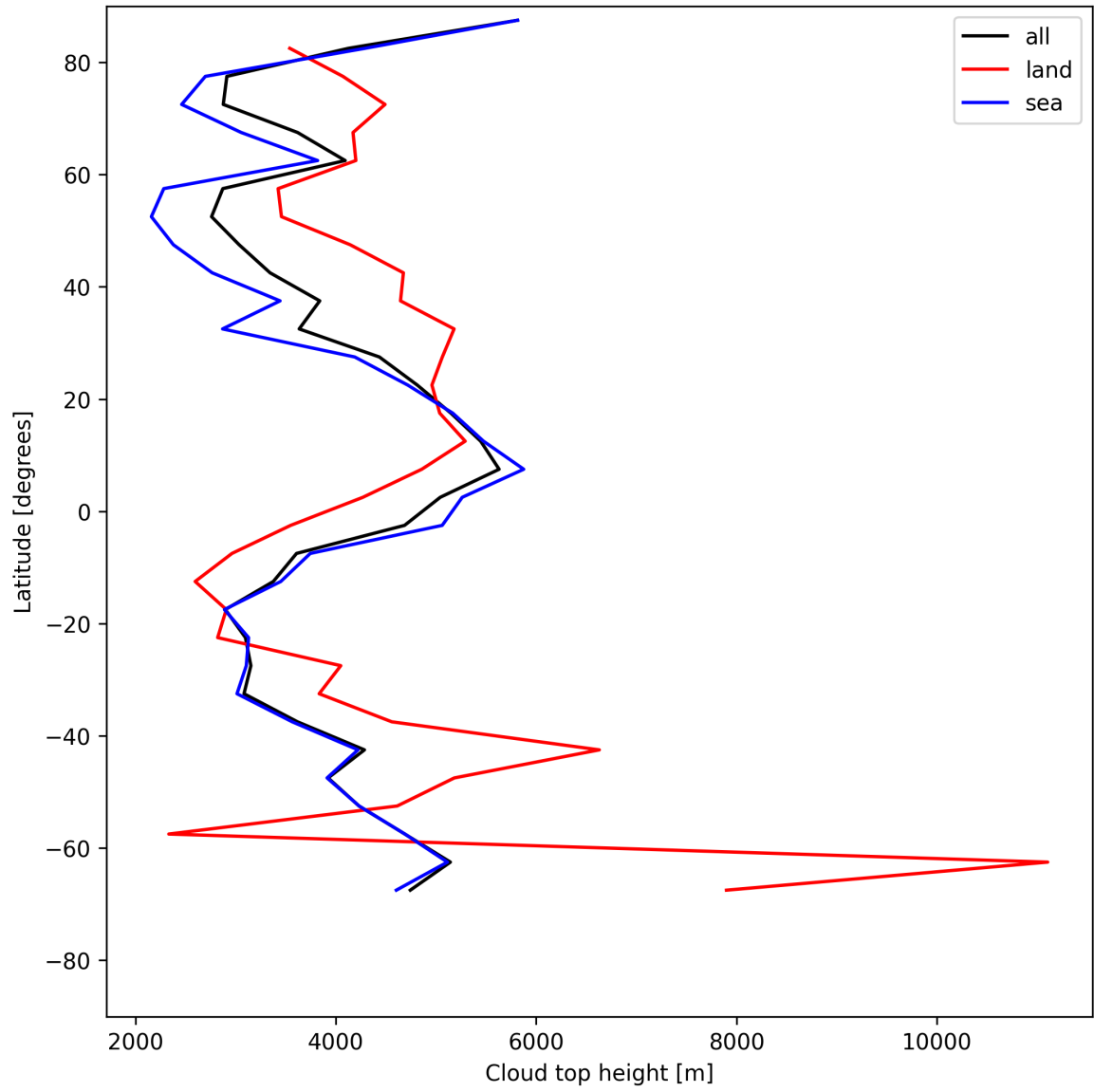
Figure 24: Zonal average of “Cloud top height” for 2025-07-08 to 2025-07-09.
