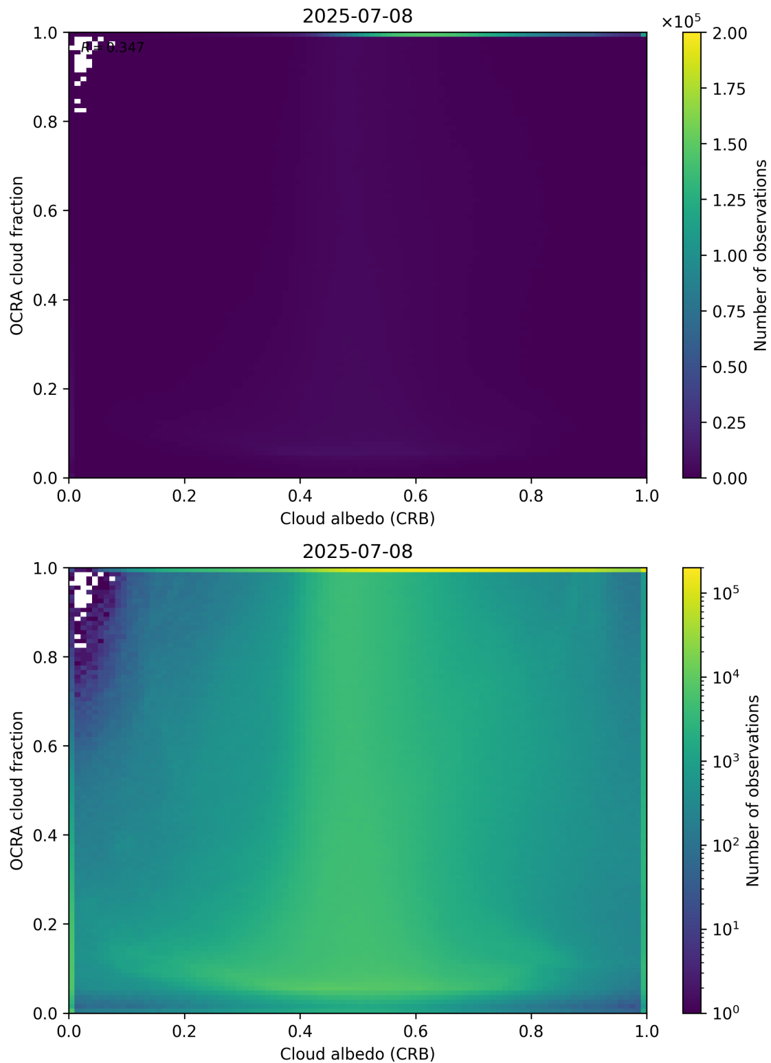
Figure 70: Scatter density plot of “Cloud albedo (CRB)” against “OCRA cloud fraction” for 2025-07-08 to 2025-07-09.
