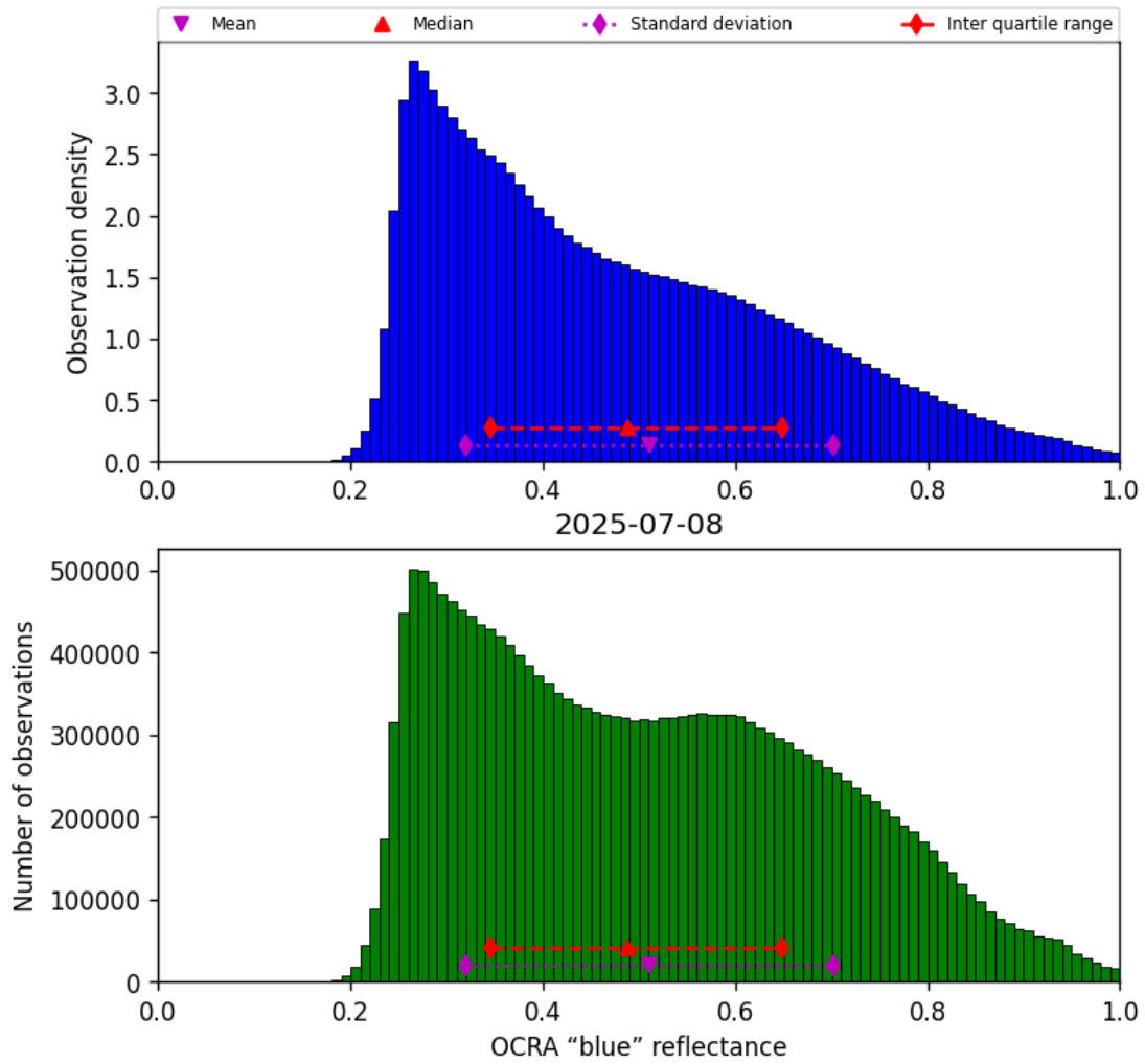
Figure 51: Histogram of “OCRA “blue” reflectance” for 2025-07-08 to 2025-07-09
