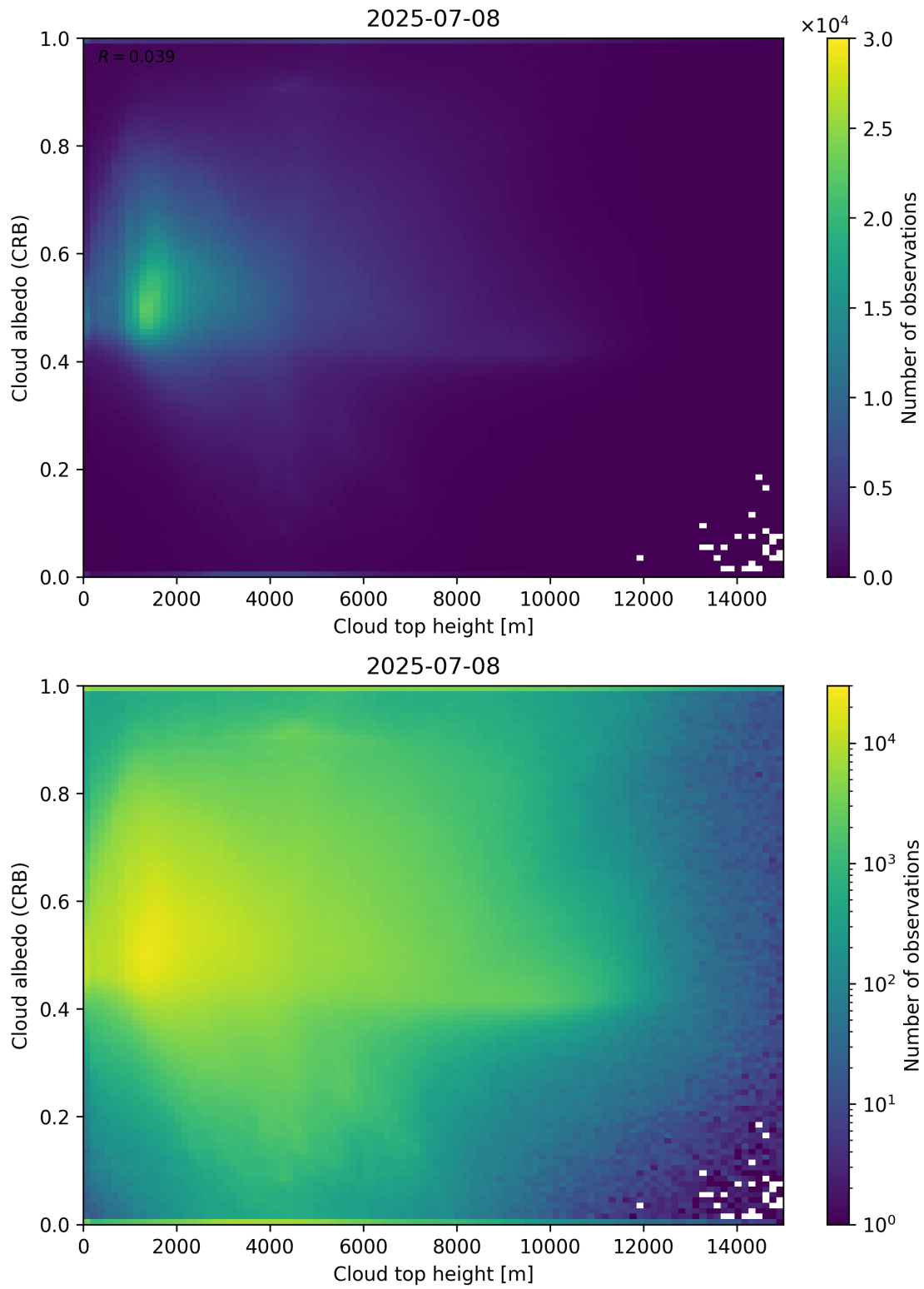
Figure 86: Scatter density plot of “Cloud top height” against “Cloud albedo (CRB)” for 2025-07-08 to 2025-07-09.
