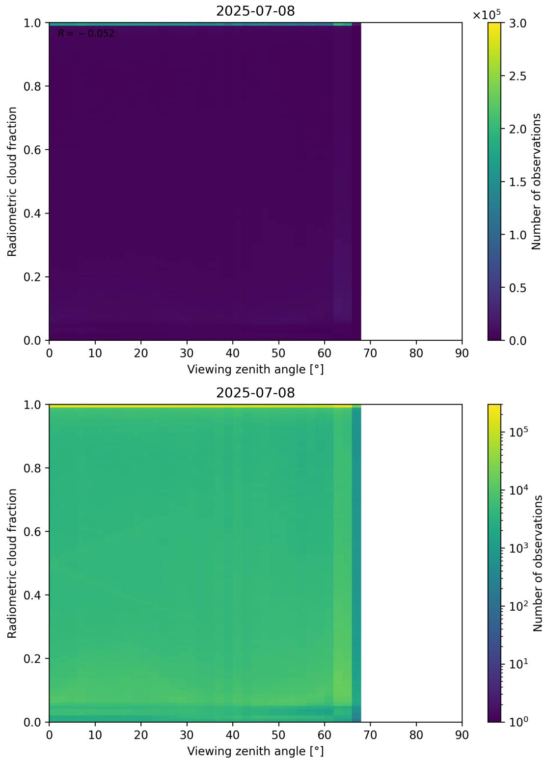
Figure 107: Scatter density plot of “Viewing zenith angle” against “Radiometric cloud fraction” for 2025-07-08 to 2025-07-09.
