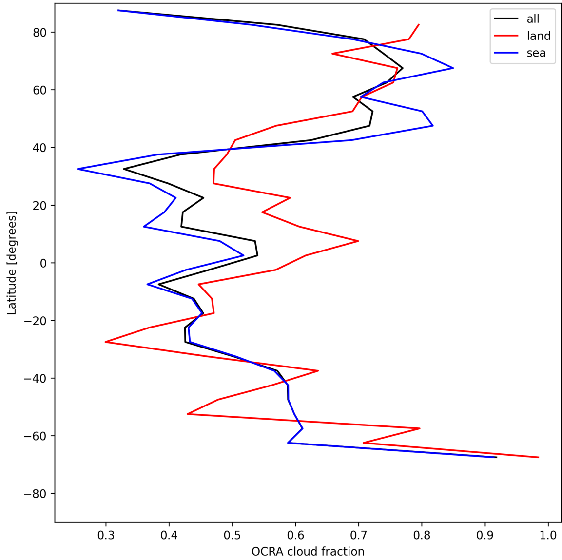
Figure 34: Zonal average of “OCRA cloud fraction” for 2025-07-08 to 2025-07-09.
