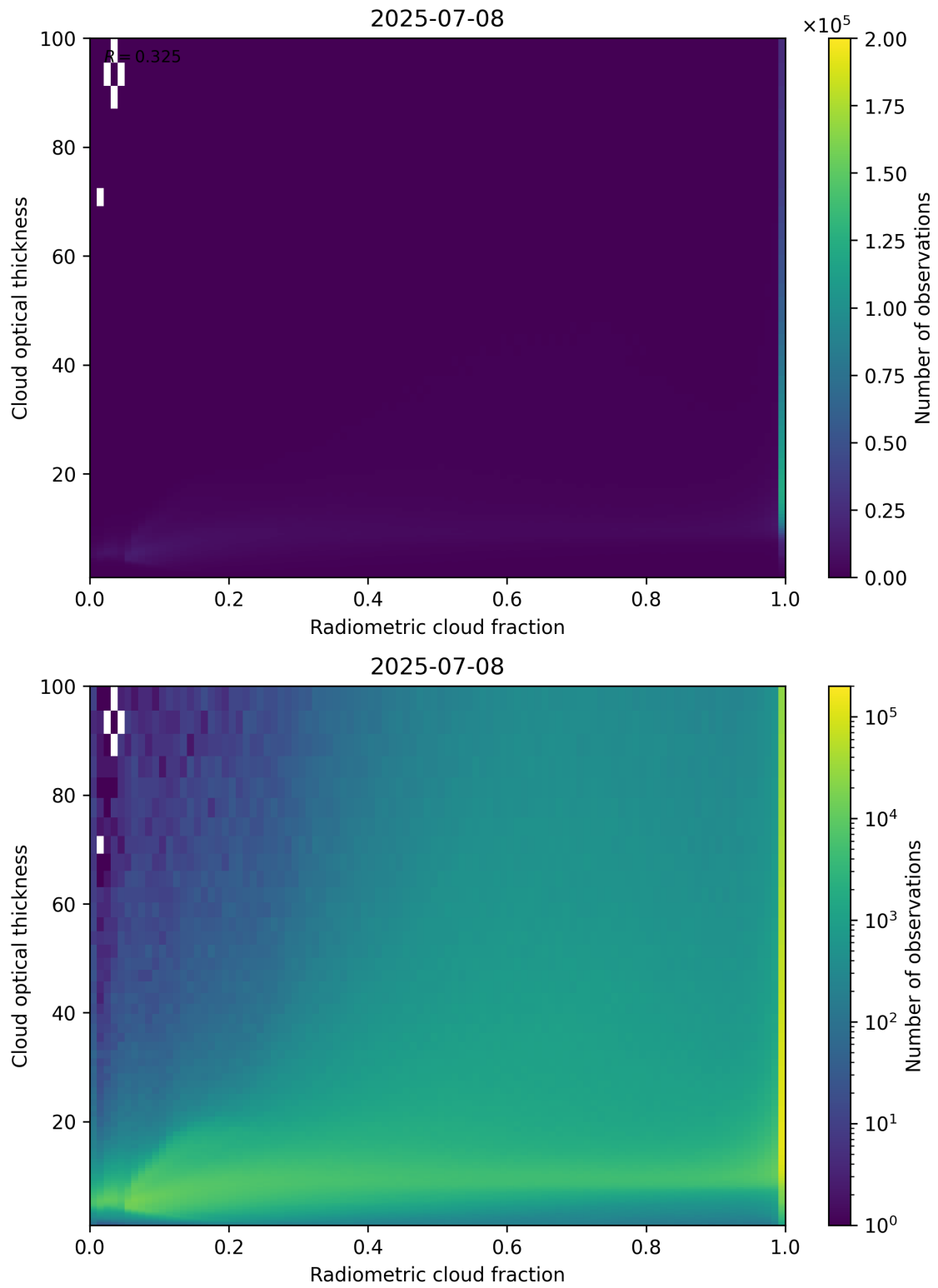
Figure 75: Scatter density plot of “Radiometric cloud fraction” against “Cloud optical thickness” for 2025-07-08 to 2025-07-09.
