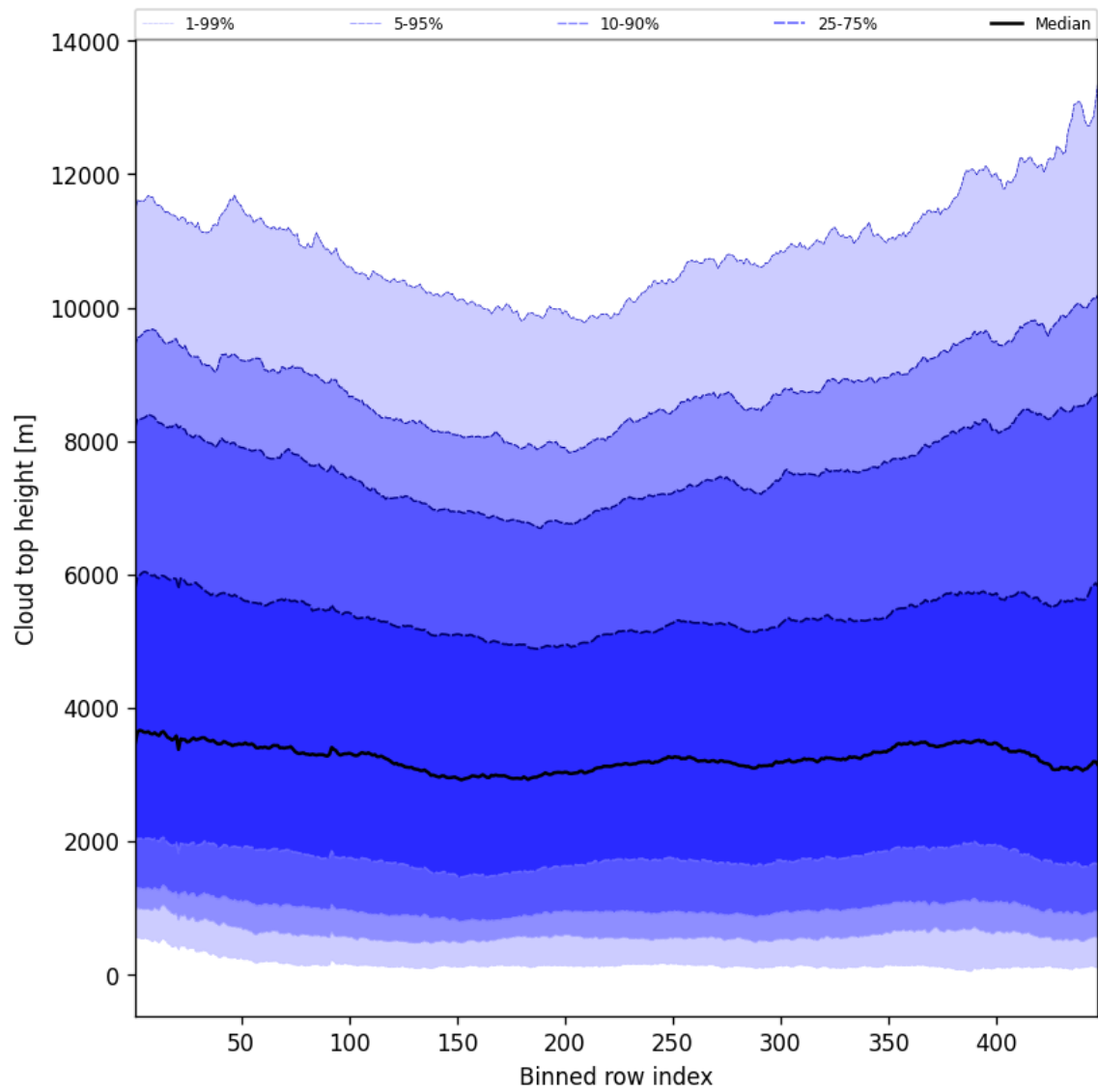
Figure 56: Along track statistics of “Cloud top height” for 2025-07-08 to 2025-07-09
