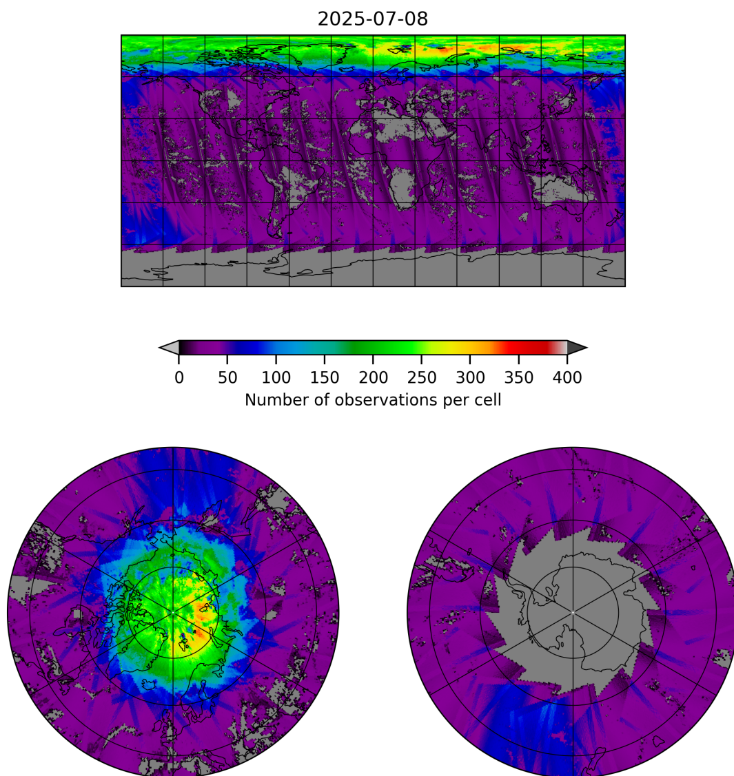
Figure 21: Map of the number of observations for 2025-07-08 to 2025-07-09
