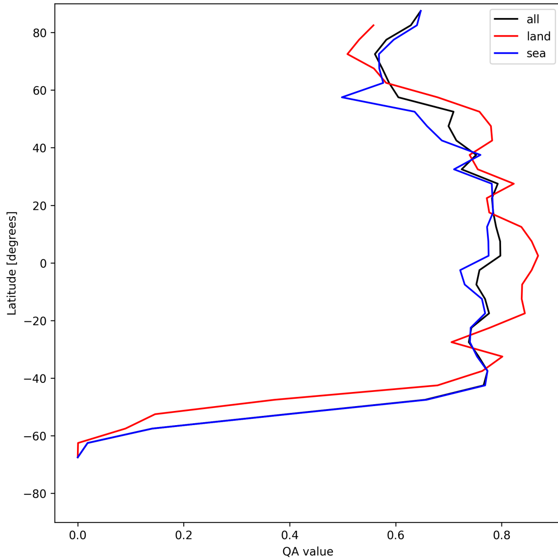
Figure 22: Zonal average of “QA value” for 2025-07-08 to 2025-07-09.
