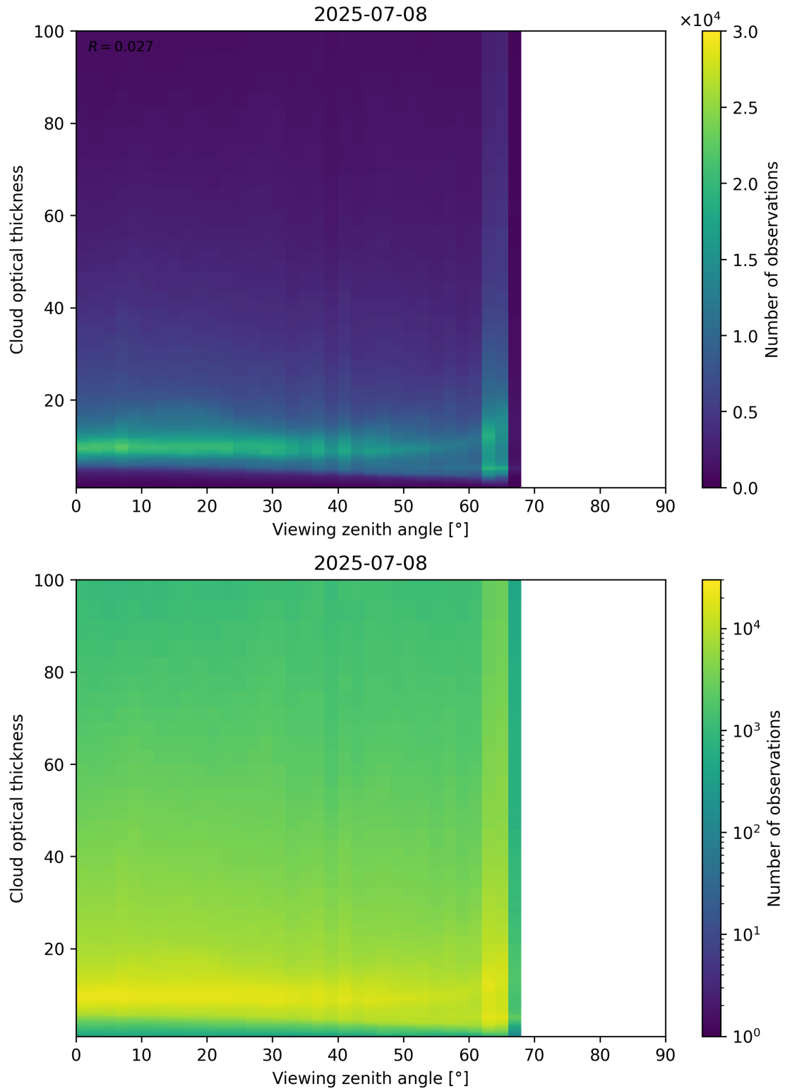
Figure 111: Scatter density plot of “Viewing zenith angle” against “Cloud optical thickness” for 2025-07-08 to 2025-07-09.
