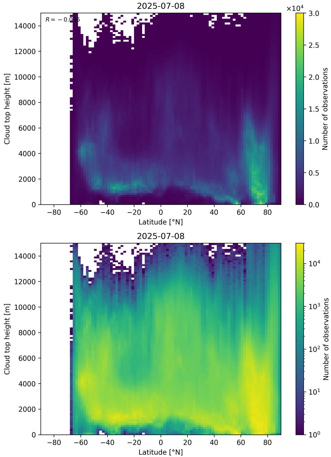
Figure 97: Scatter density plot of “Latitude” against “Cloud top height” for 2025-07-08 to 2025-07-09.
