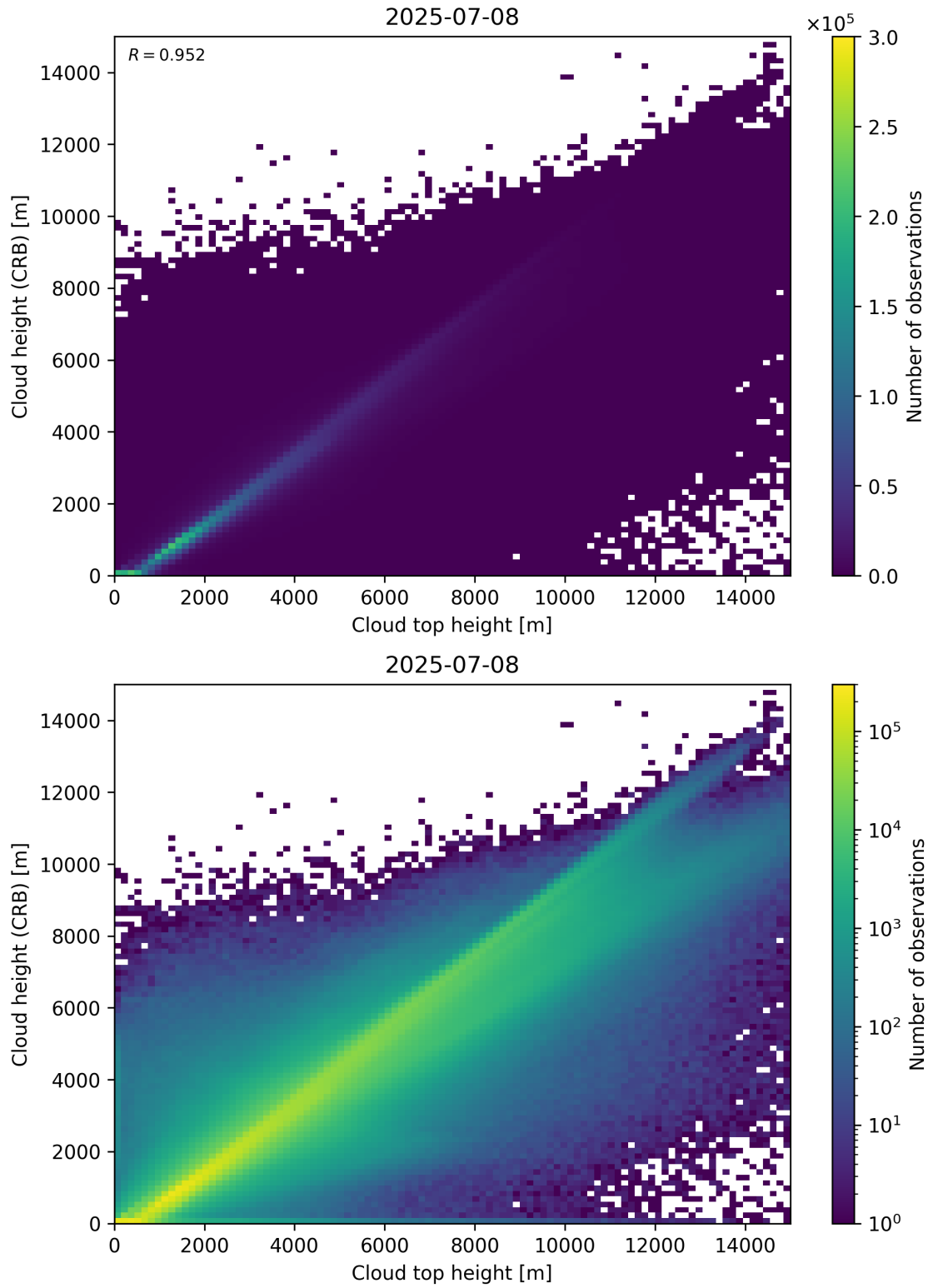
Figure 89: Scatter density plot of “Cloud top height” against “Cloud height (CRB)” for 2025-07-08 to 2025-07-09.
