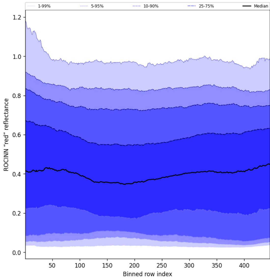
Figure 69: Along track statistics of "ROCINN "red" reflectance" for 2025-07-08 to 2025-07-09
