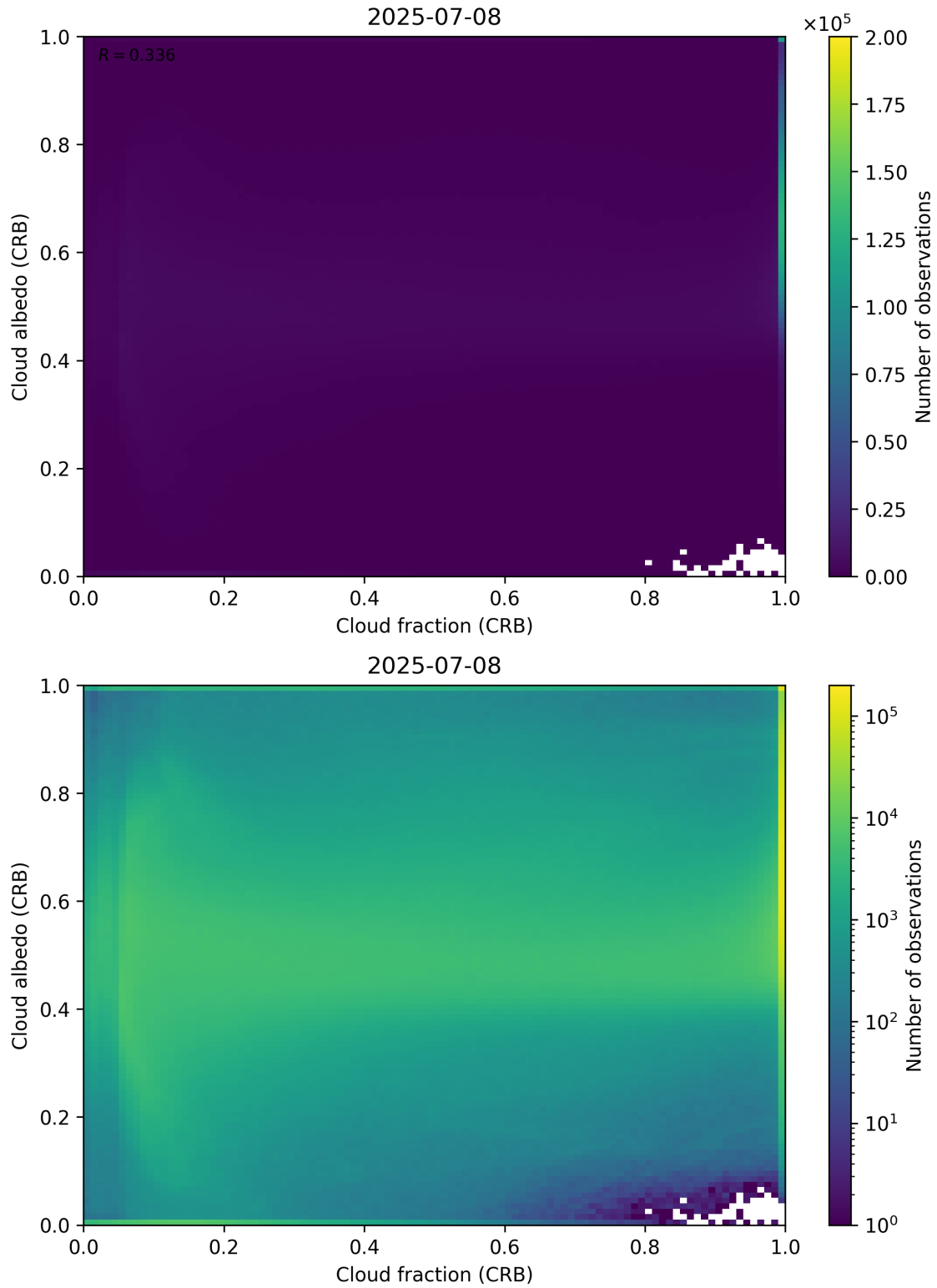
Figure 77: Scatter density plot of “Cloud fraction (CRB)” against “Cloud albedo (CRB)” for 2025-07-08 to 2025-07-09.
