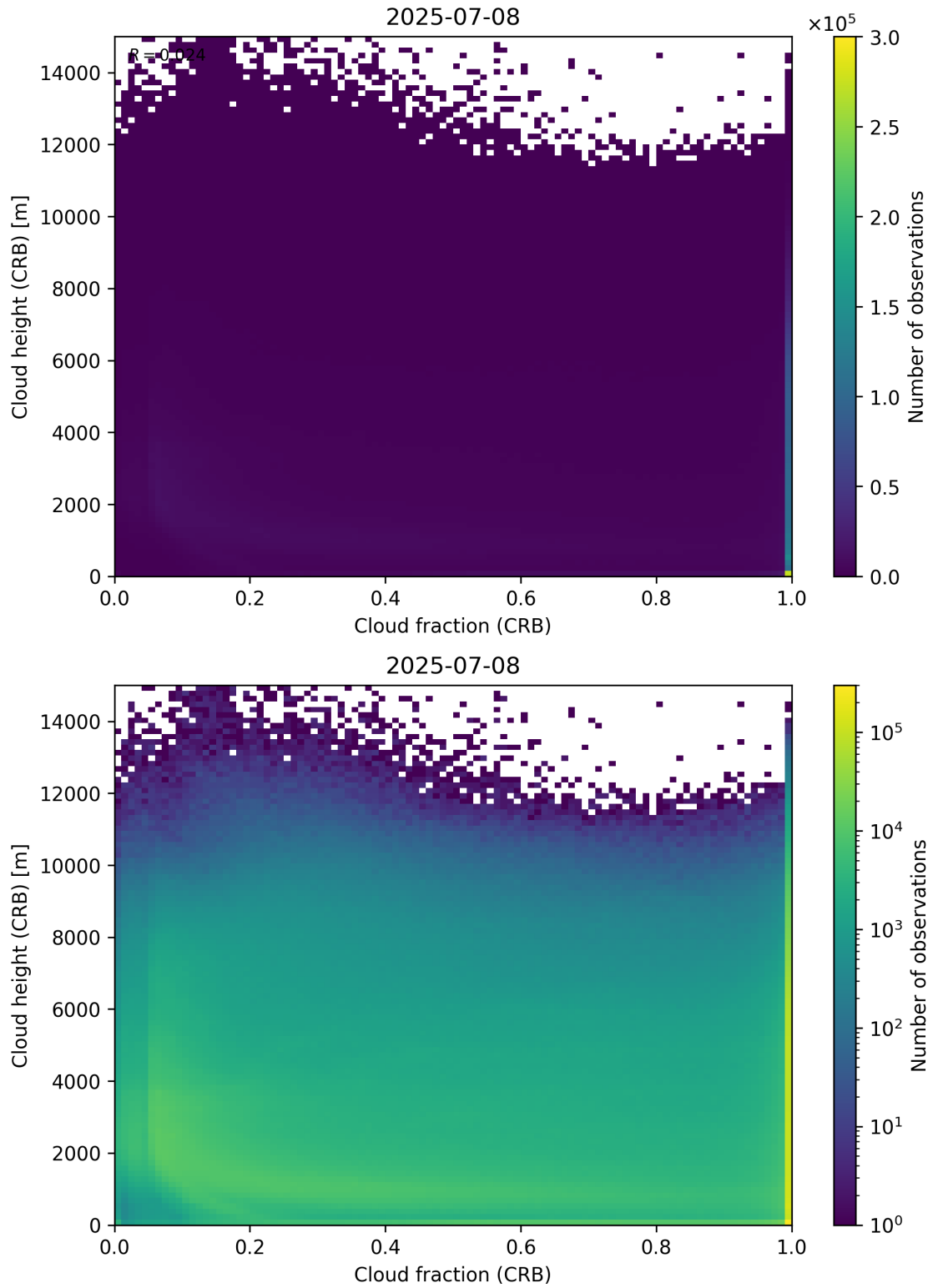
Figure 79: Scatter density plot of “Cloud fraction (CRB)” against “Cloud height (CRB)” for 2025-07-08 to 2025-07-09.
