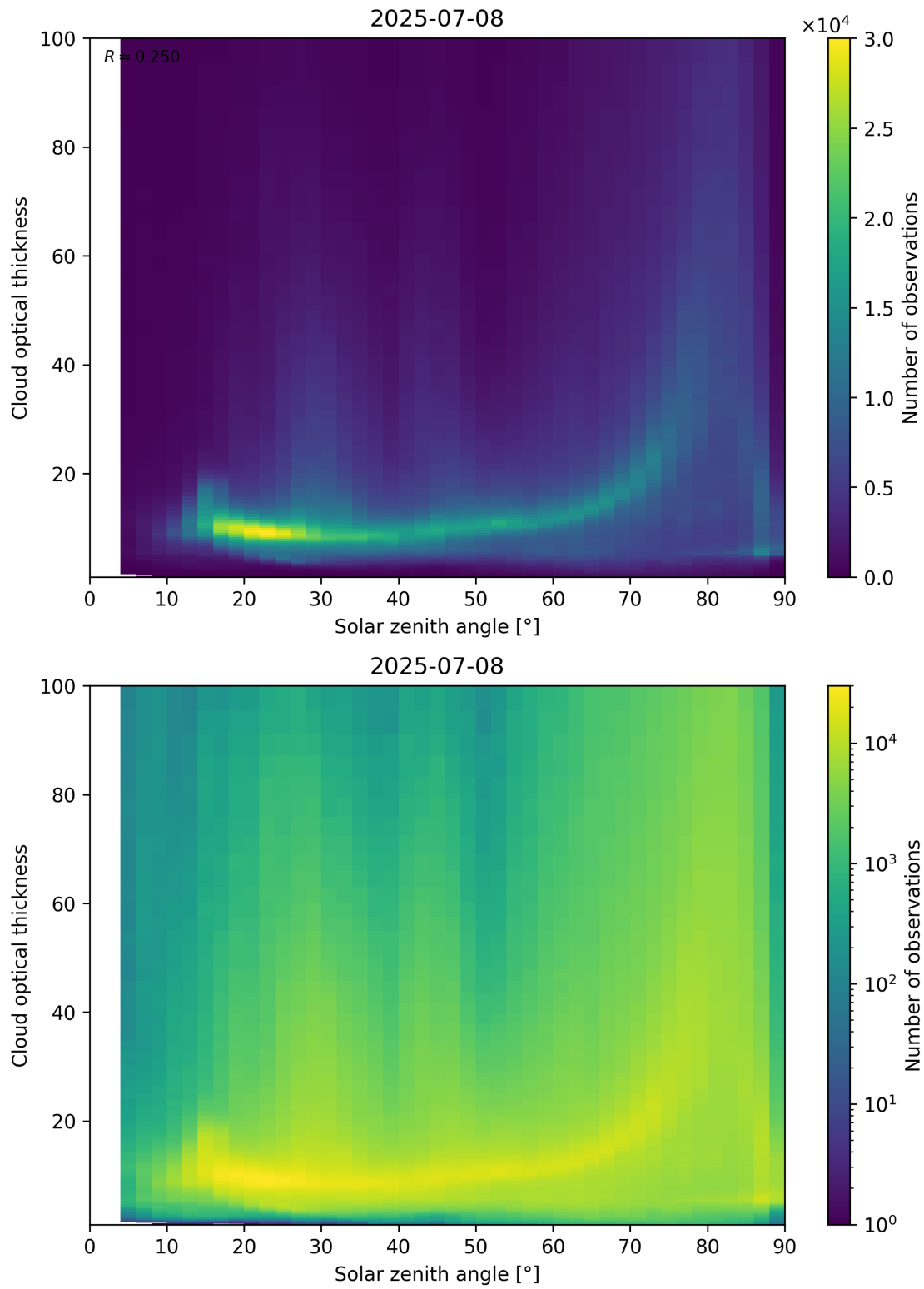
Figure 103: Scatter density plot of “Solar zenith angle” against “Cloud optical thickness” for 2025-07-08 to 2025-07-09.
