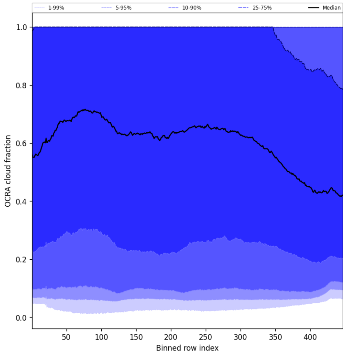
Figure 66: Along track statistics of “OCRA cloud fraction” for 2025-07-08 to 2025-07-09
