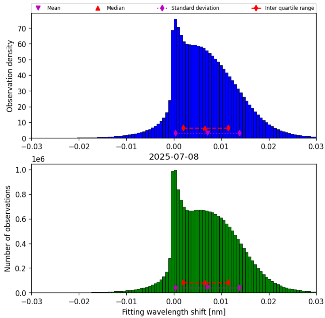
Figure 49: Histogram of “Fitting wavelength shift” for 2025-07-08 to 2025-07-09
