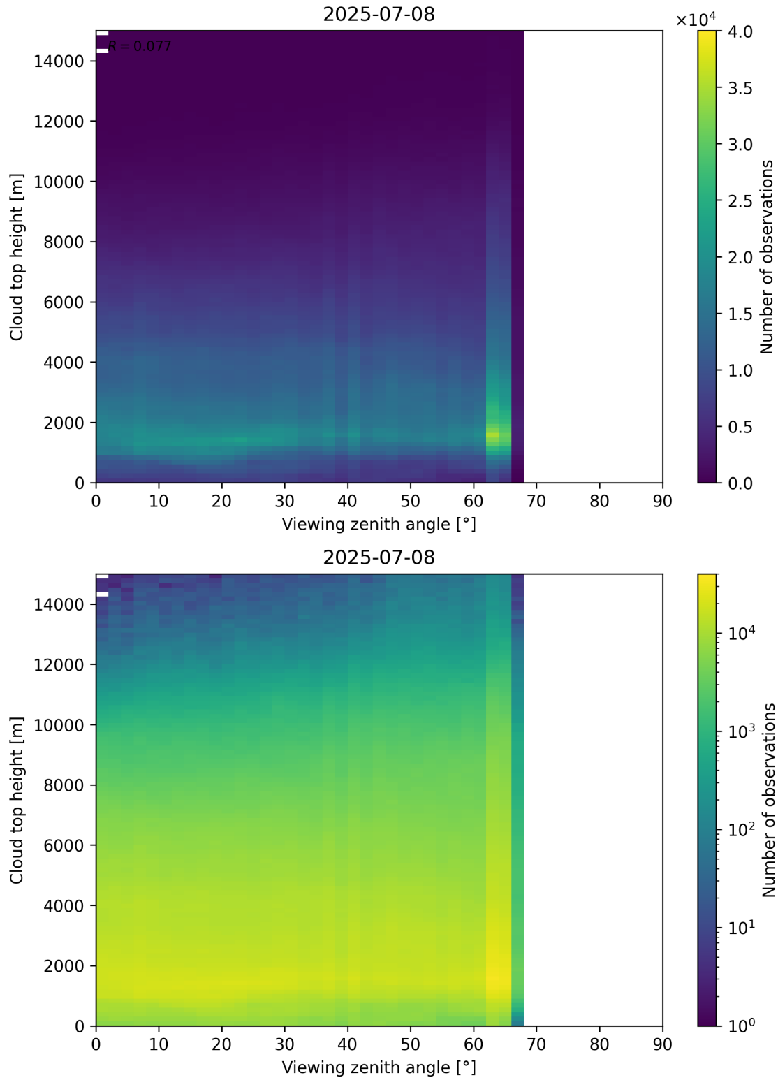
Figure 112: Scatter density plot of “Viewing zenith angle” against “Cloud top height” for 2025-07-08 to 2025-07-09.
