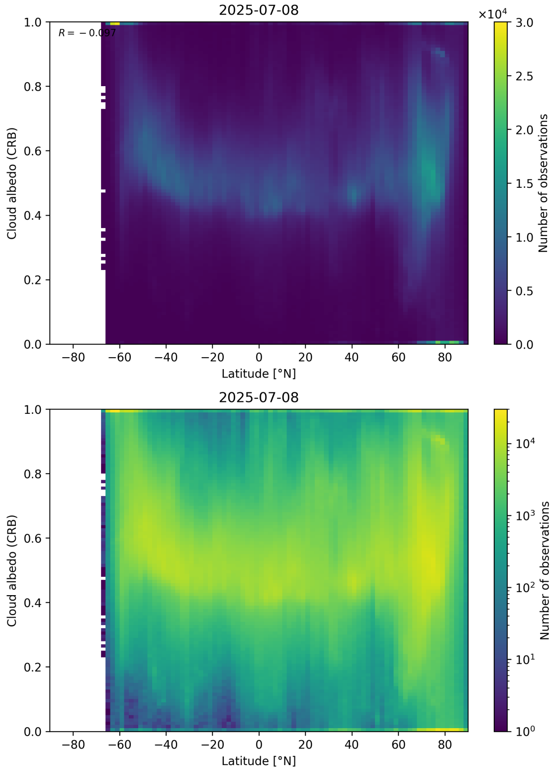
Figure 91: Scatter density plot of “Latitude” against “Cloud albedo (CRB)” for 2025-07-08 to 2025-07-09.
