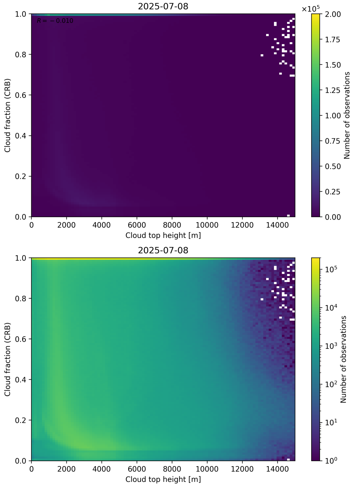
Figure 88: Scatter density plot of “Cloud top height” against “Cloud fraction (CRB)” for 2025-07-08 to 2025-07-09.
