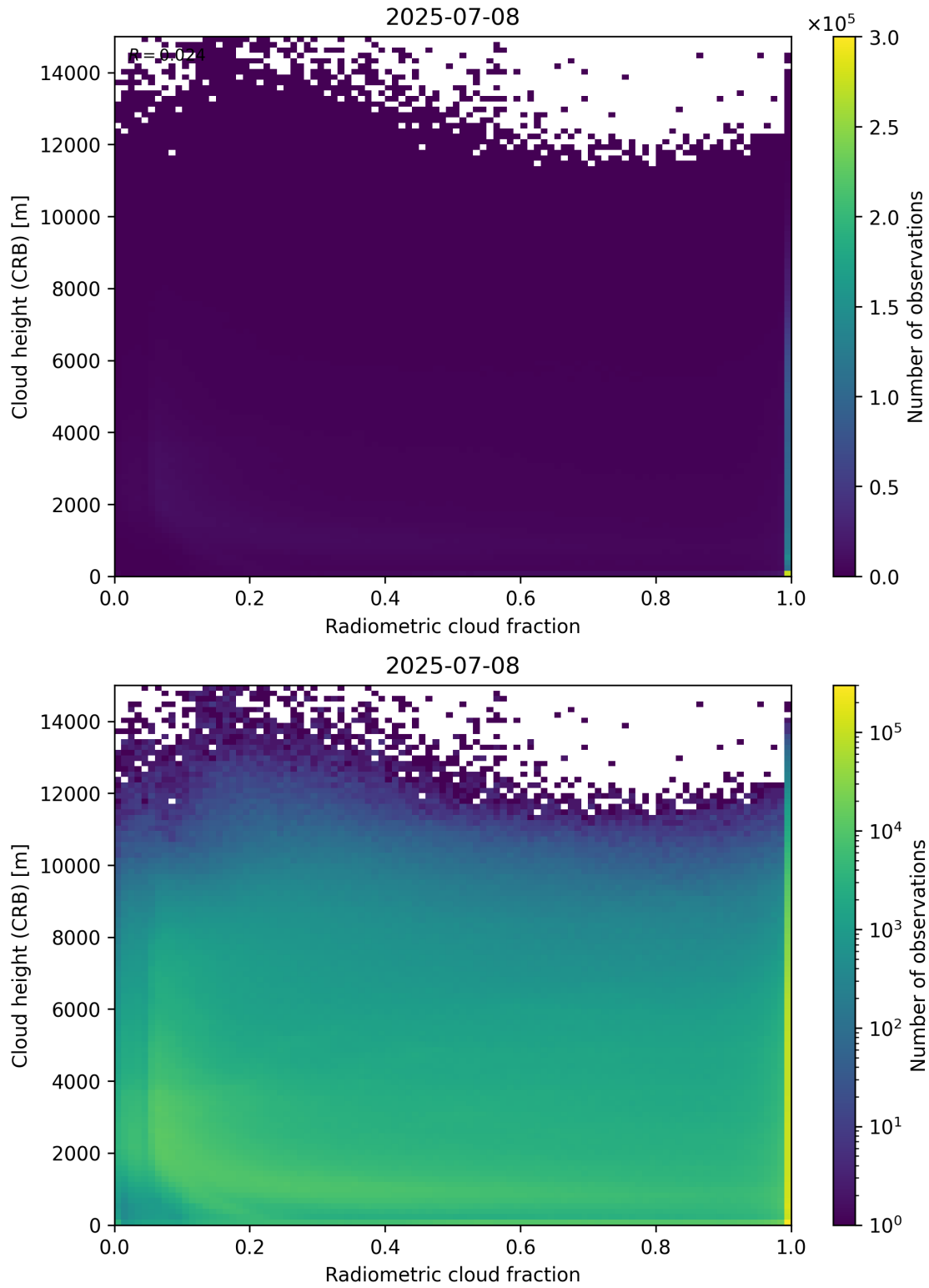
Figure 74: Scatter density plot of “Radiometric cloud fraction” against “Cloud height (CRB)” for 2025-07-08 to 2025-07-09.
