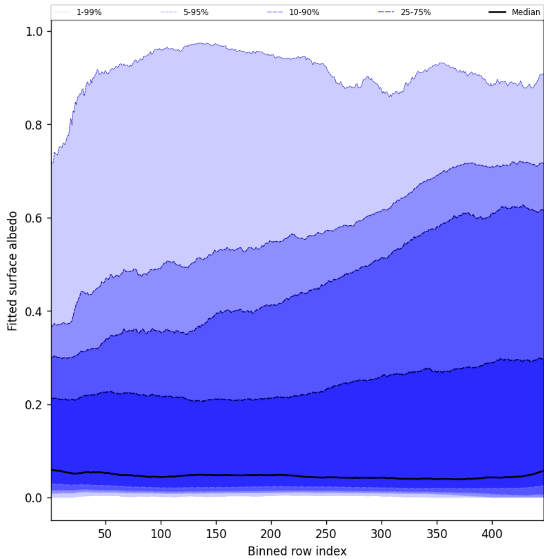
Figure 61: Along track statistics of “Fitted surface albedo” for 2025-07-08 to 2025-07-09
