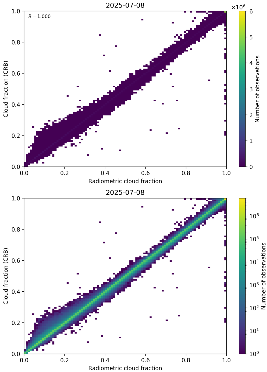
Figure 73: Scatter density plot of “Radiometric cloud fraction” against “Cloud fraction (CRB)” for 2025-07-08 to 2025-07-09.
