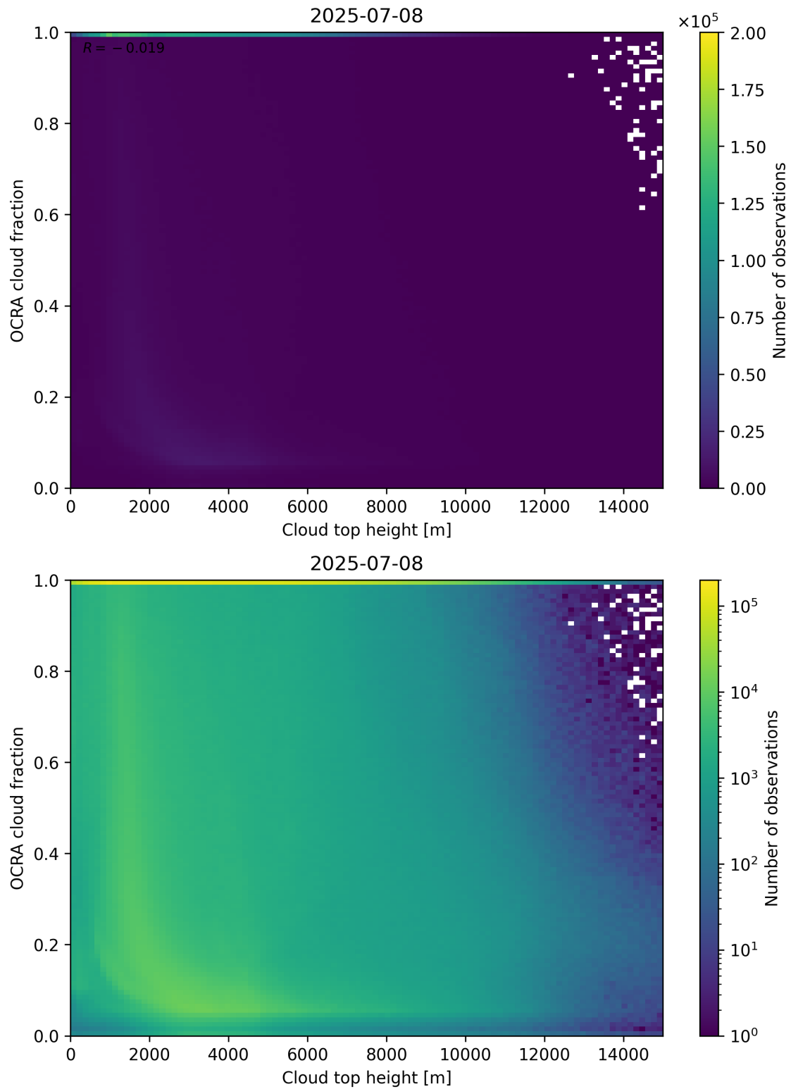
Figure 87: Scatter density plot of “Cloud top height” against “OCRA cloud fraction” for 2025-07-08 to 2025-07-09.
