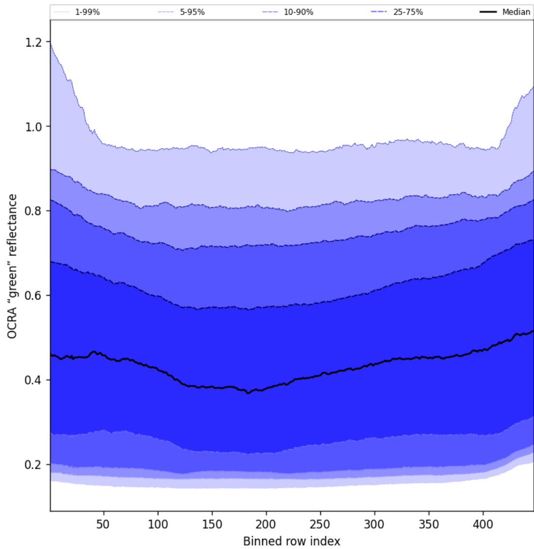
Figure 68: Along track statistics of “OCRA “green” reflectance” for 2025-07-08 to 2025-07-09
