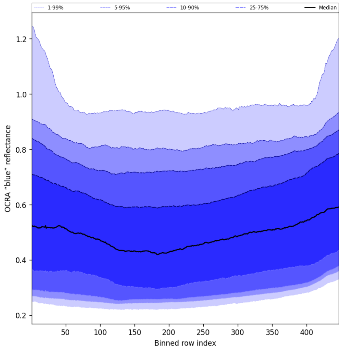
Figure 67: Along track statistics of “OCRA “blue” reflectance” for 2025-07-08 to 2025-07-09
