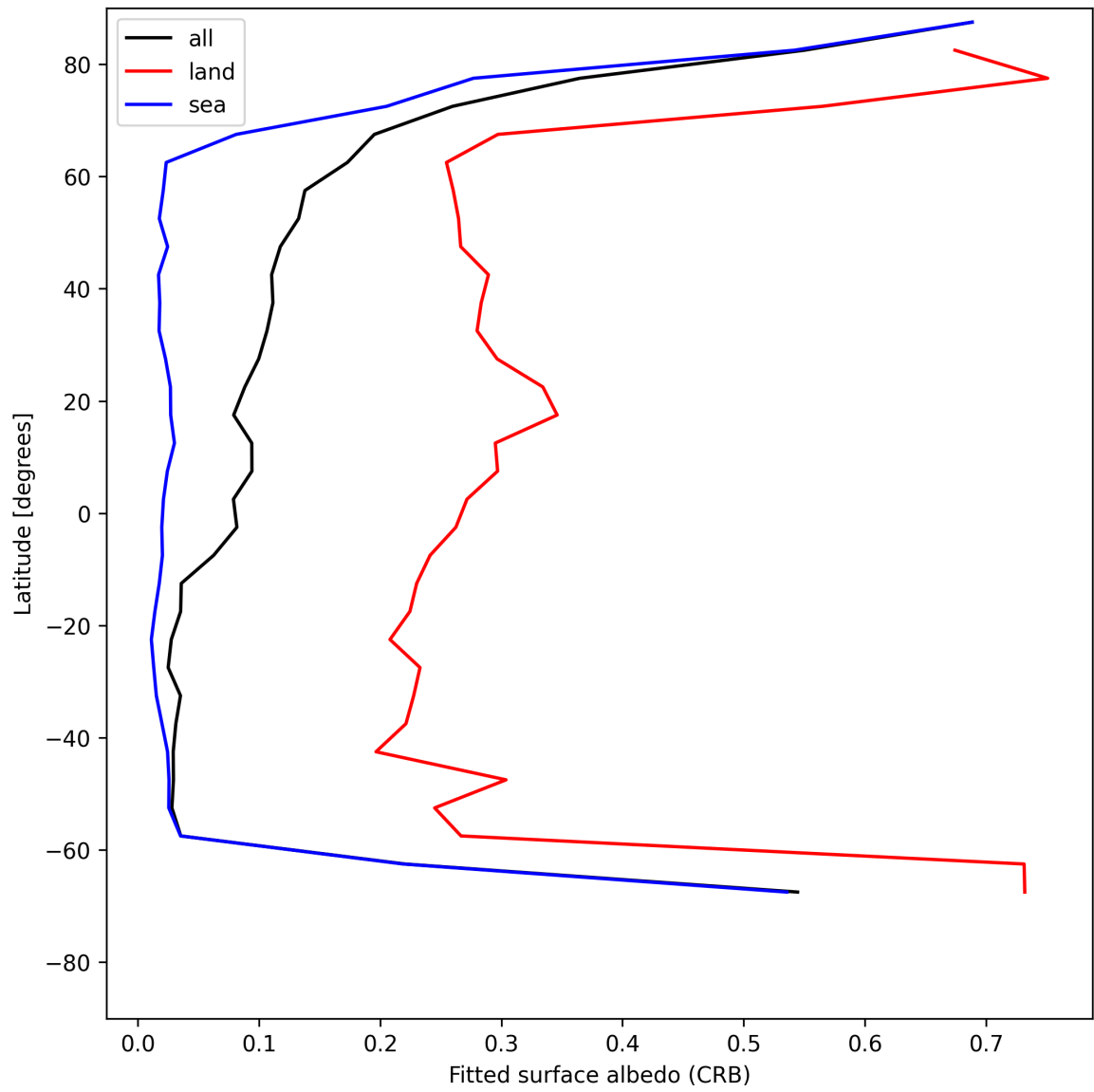
Figure 30: Zonal average of “Fitted surface albedo (CRB)” for 2025-07-08 to 2025-07-09.
