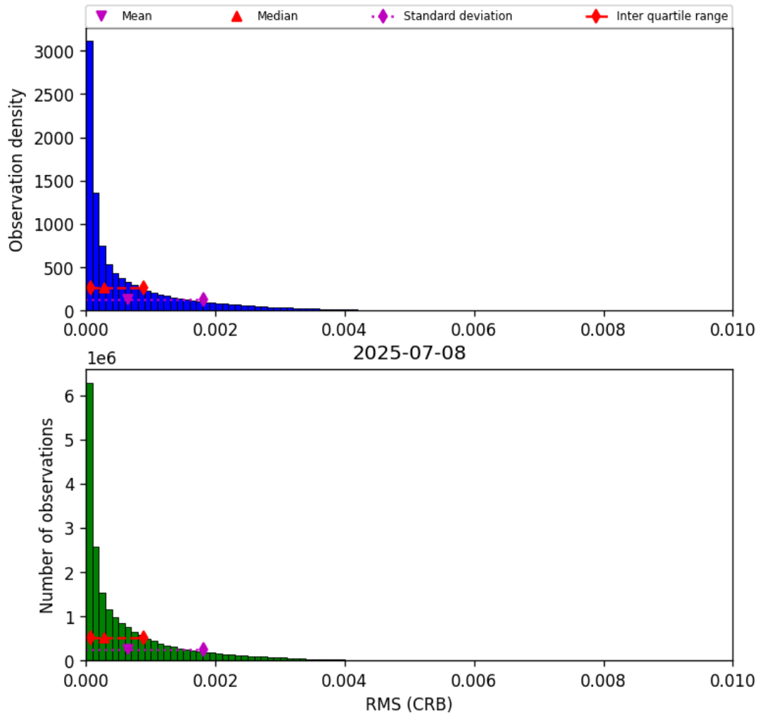
Figure 48: Histogram of “RMS (CRB)” for 2025-07-08 to 2025-07-09
