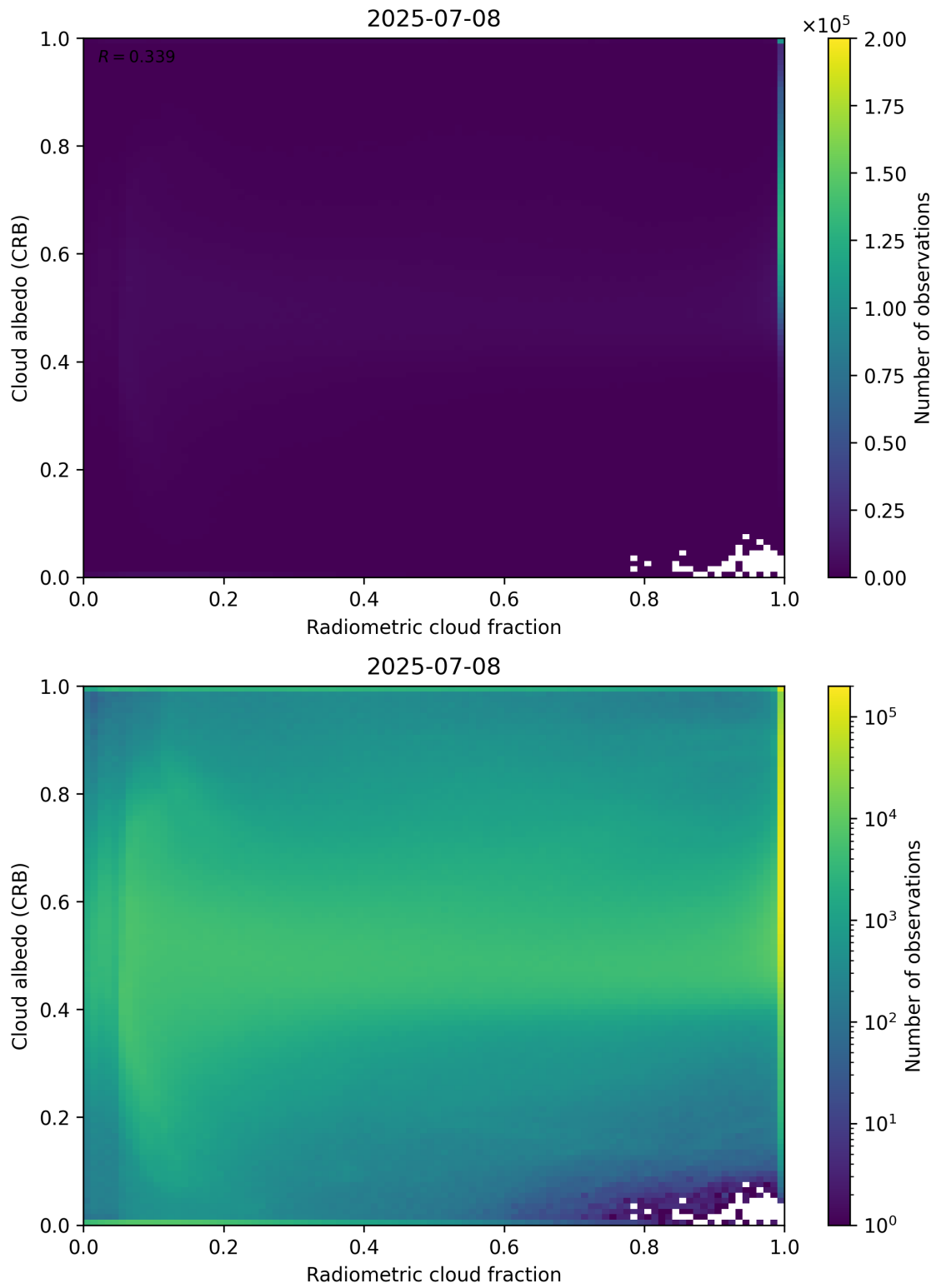
Figure 71: Scatter density plot of “Radiometric cloud fraction” against “Cloud albedo (CRB)” for 2025-07-08 to 2025-07-09.
