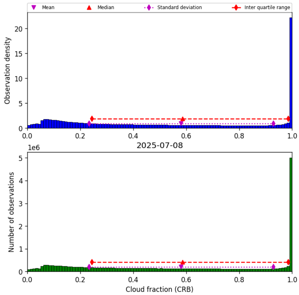
Figure 42: Histogram of “Cloud fraction (CRB)” for 2025-07-08 to 2025-07-09
