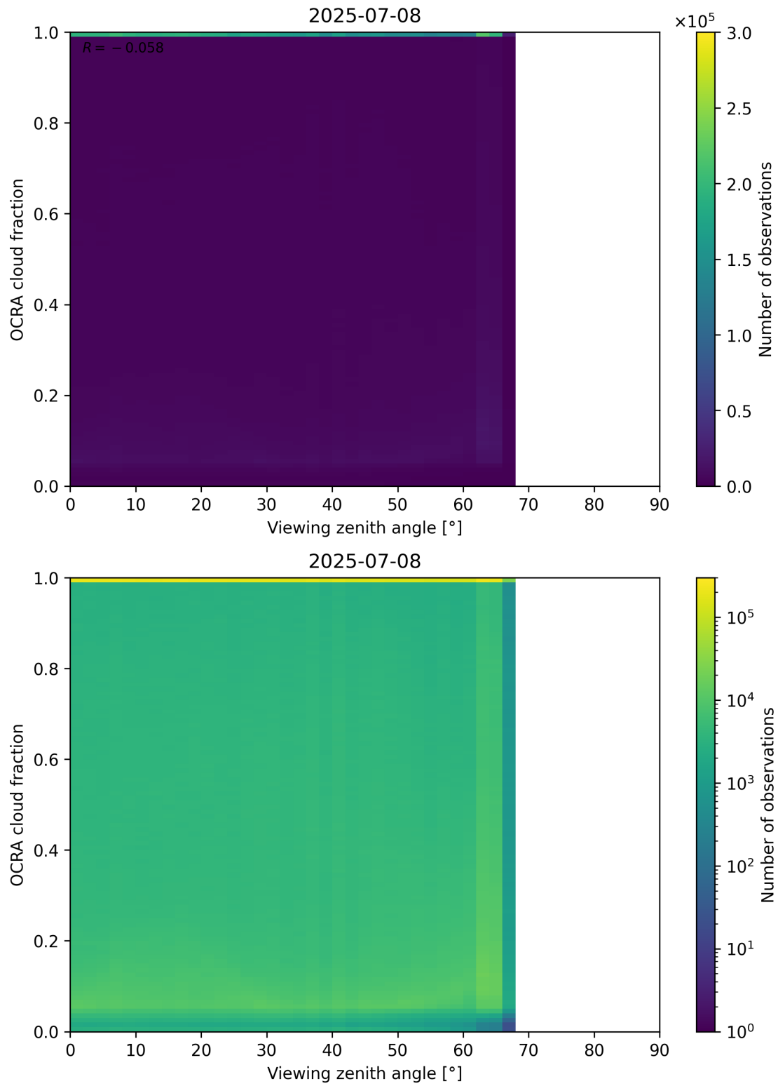
Figure 108: Scatter density plot of “Viewing zenith angle” against “OCRA cloud fraction” for 2025-07-08 to 2025-07-09.
