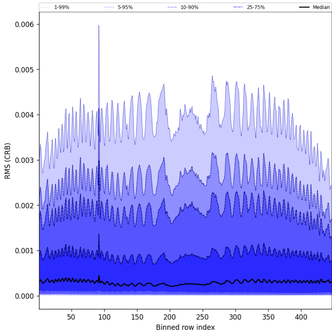
Figure 64: Along track statistics of “RMS (CRB)” for 2025-07-08 to 2025-07-09
