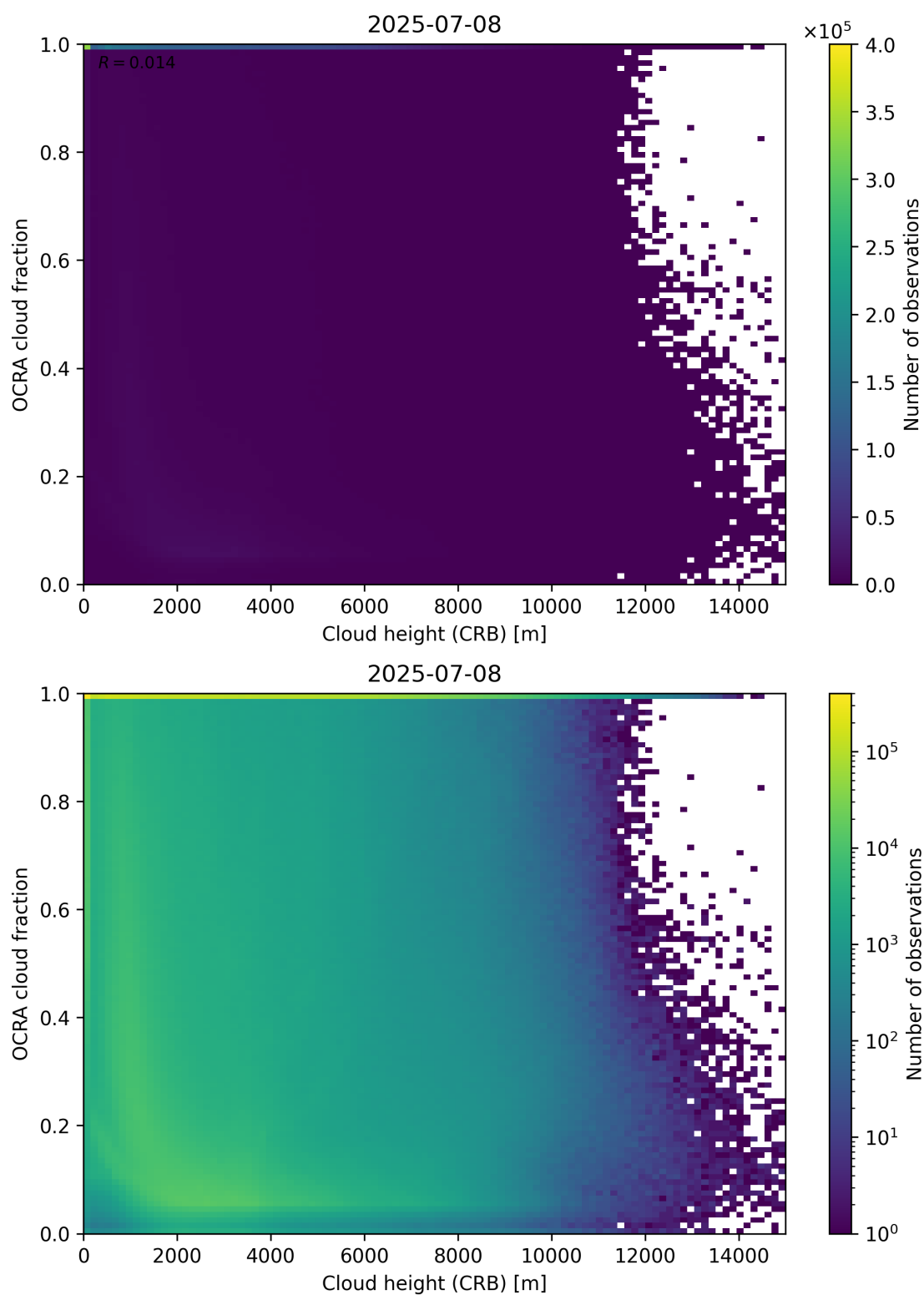
Figure 81: Scatter density plot of “Cloud height (CRB)” against “OCRA cloud fraction” for 2025-07-08 to 2025-07-09.
