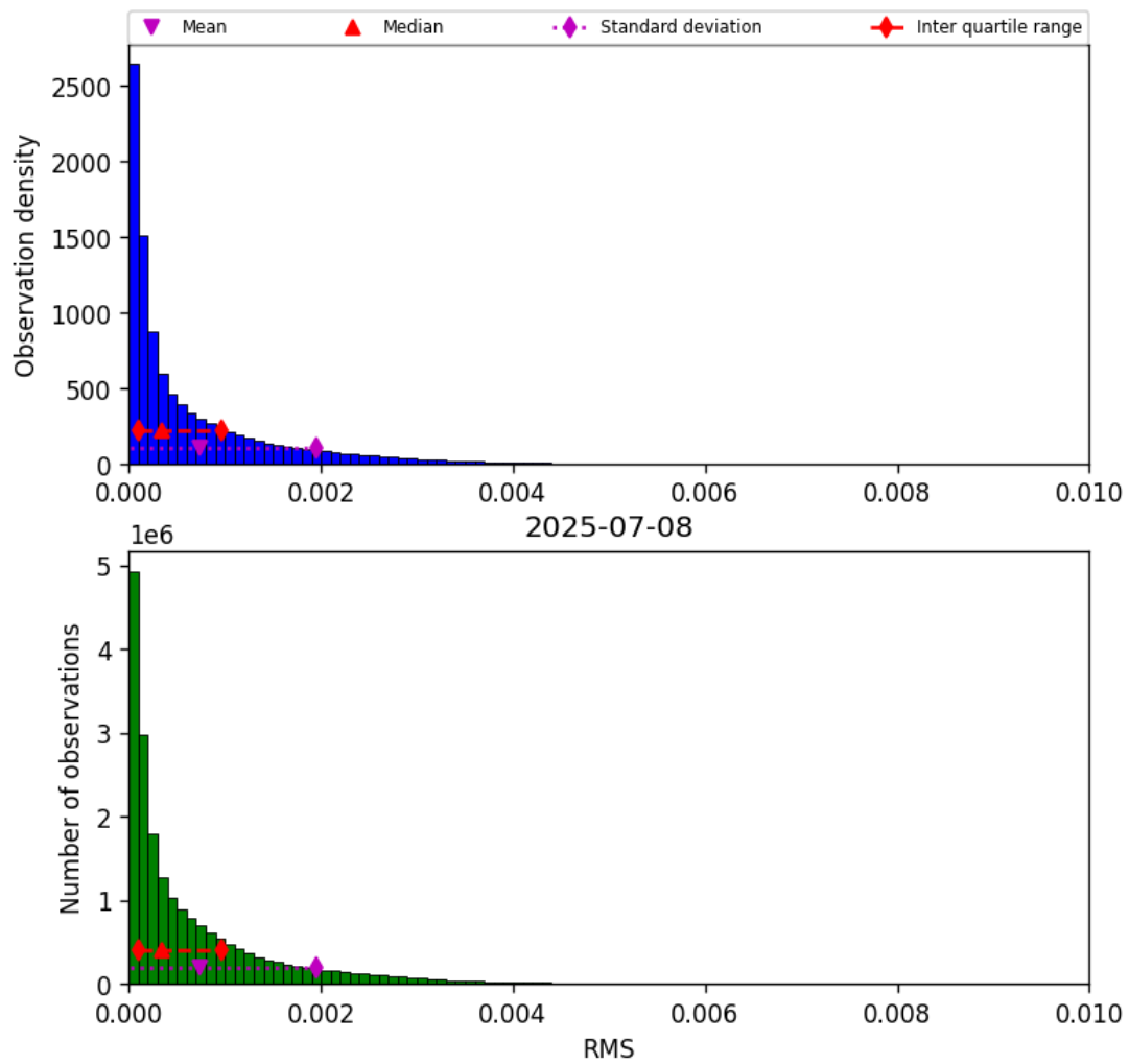
Figure 47: Histogram of “RMS” for 2025-07-08 to 2025-07-09
