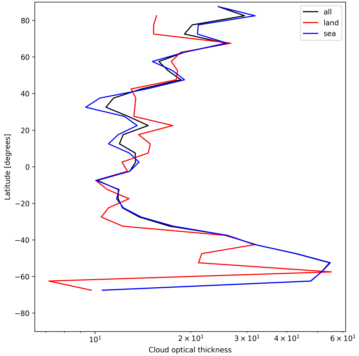
Figure 25: Zonal average of “Cloud optical thickness” for 2025-07-08 to 2025-07-09.
