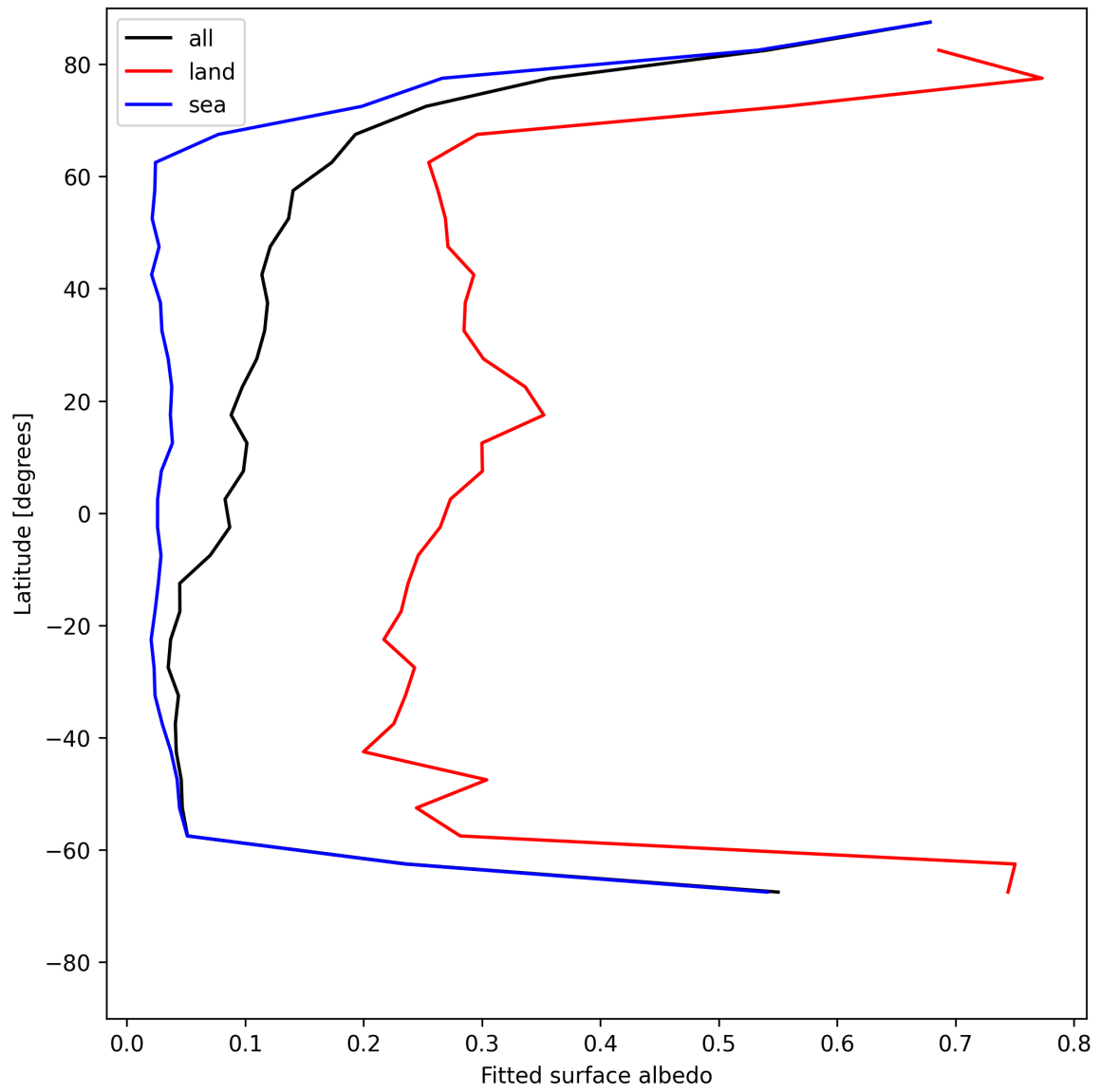
Figure 29: Zonal average of “Fitted surface albedo” for 2025-07-08 to 2025-07-09.
