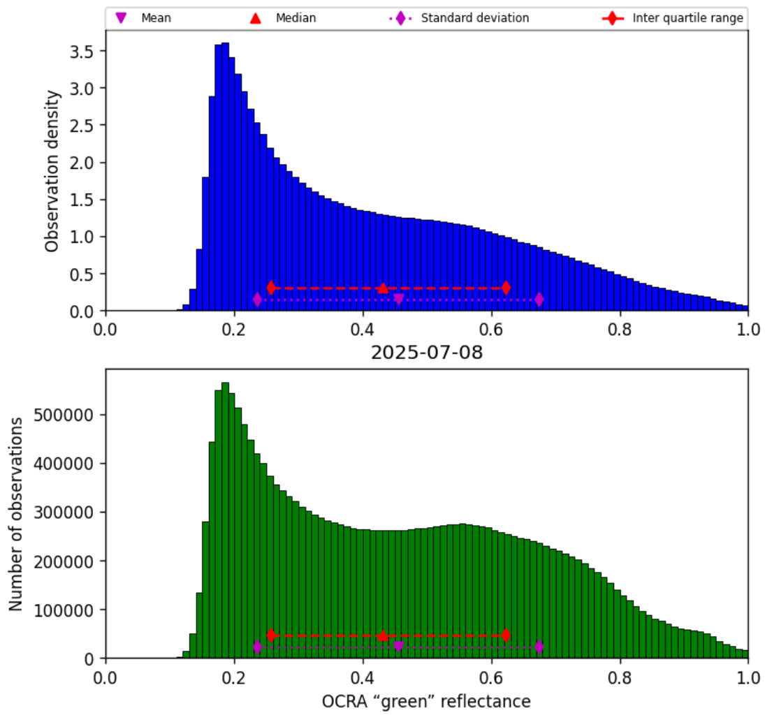
Figure 52: Histogram of “OCRA “green” reflectance” for 2025-07-08 to 2025-07-09
