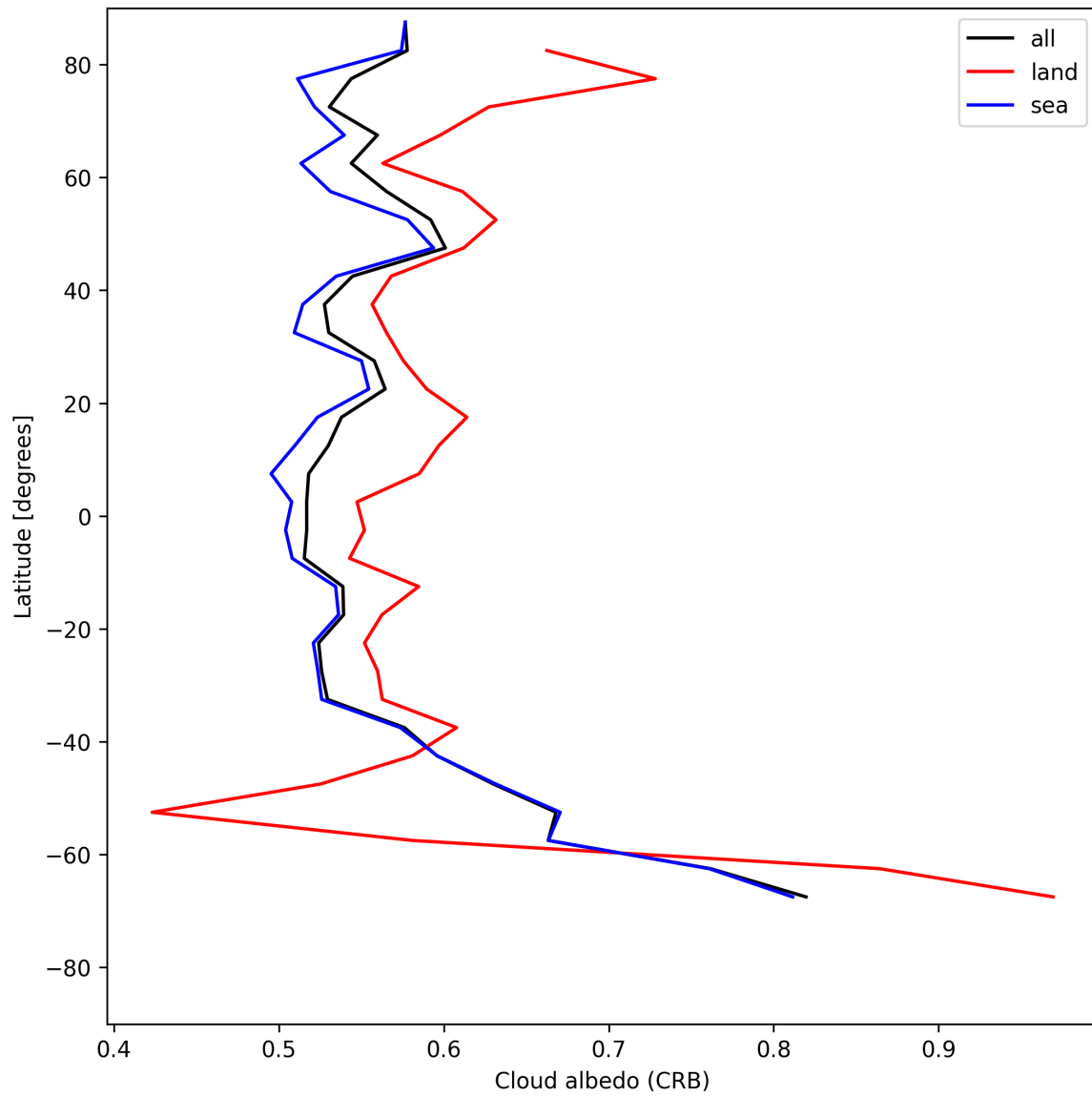
Figure 28: Zonal average of “Cloud albedo (CRB)” for 2025-07-08 to 2025-07-09.
