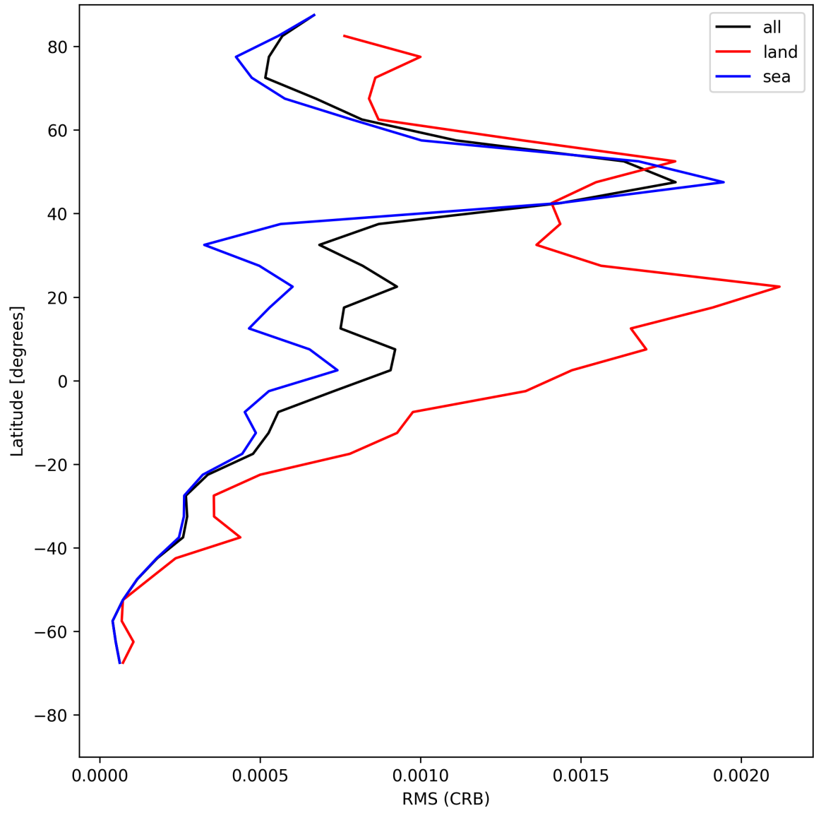
Figure 32: Zonal average of “RMS (CRB)” for 2025-07-08 to 2025-07-09.
