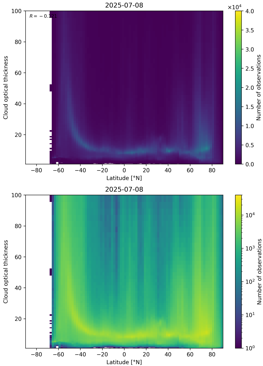
Figure 96: Scatter density plot of “Latitude” against “Cloud optical thickness” for 2025-07-08 to 2025-07-09.
