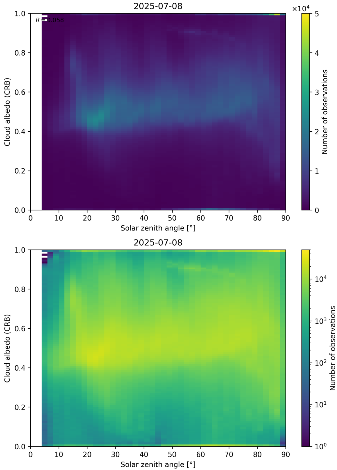
Figure 98: Scatter density plot of “Solar zenith angle” against “Cloud albedo (CRB)” for 2025-07-08 to 2025-07-09.
