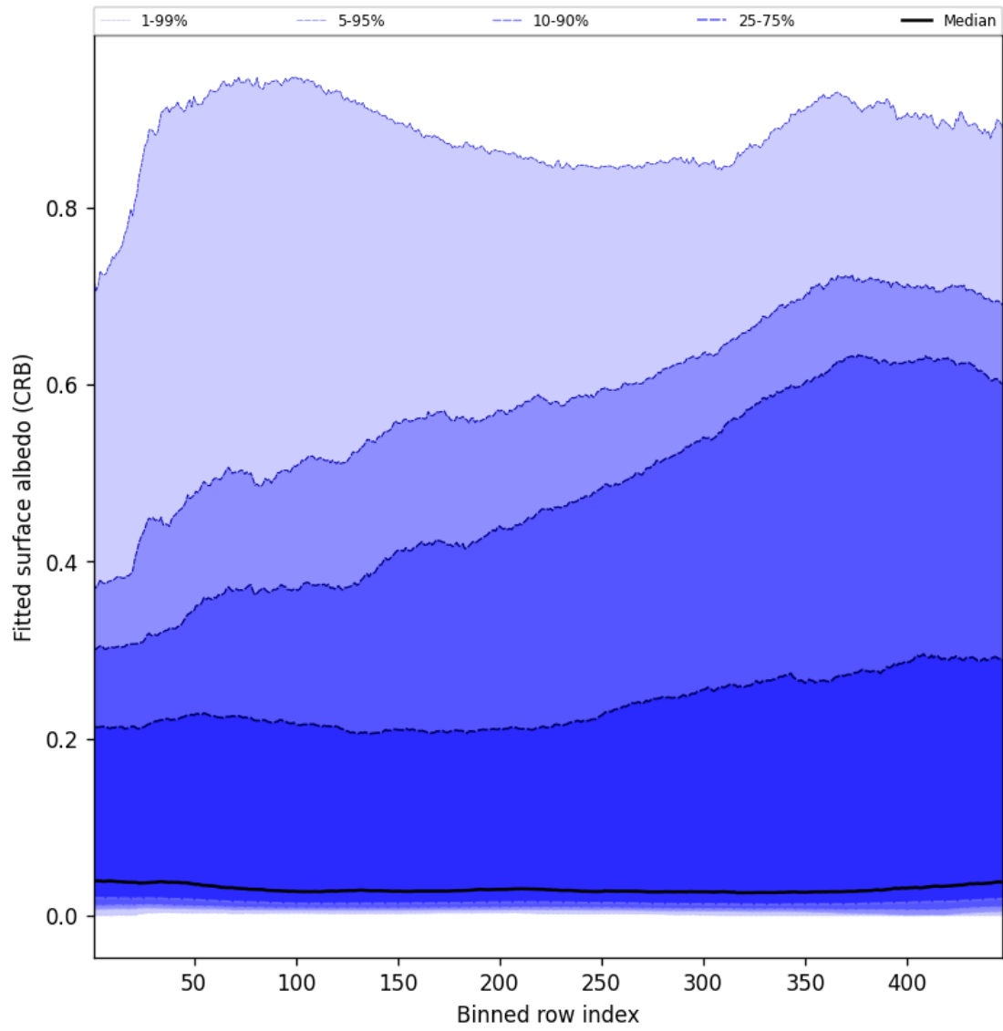
Figure 62: Along track statistics of “Fitted surface albedo (CRB)” for 2025-07-08 to 2025-07-09
