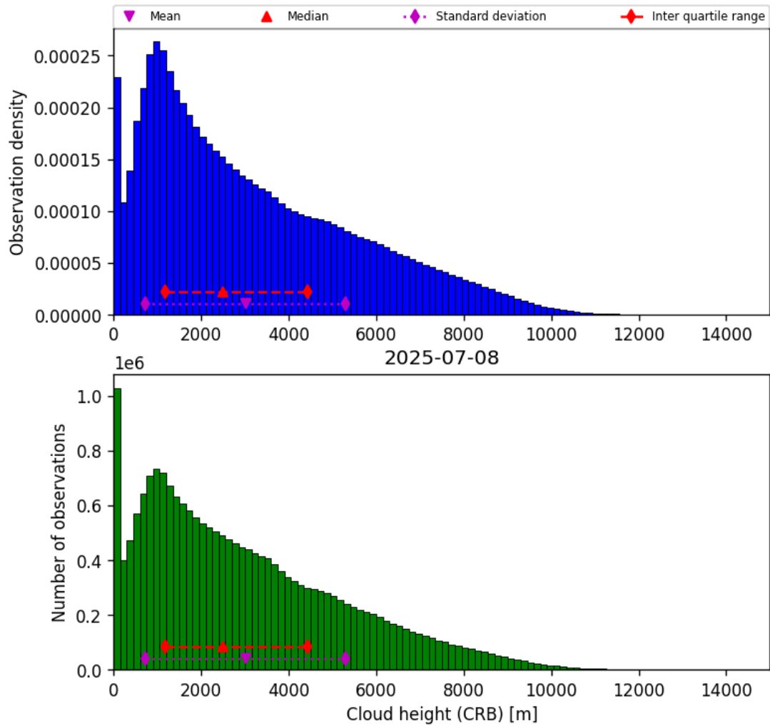
Figure 43: Histogram of “Cloud height (CRB)” for 2025-07-08 to 2025-07-09
