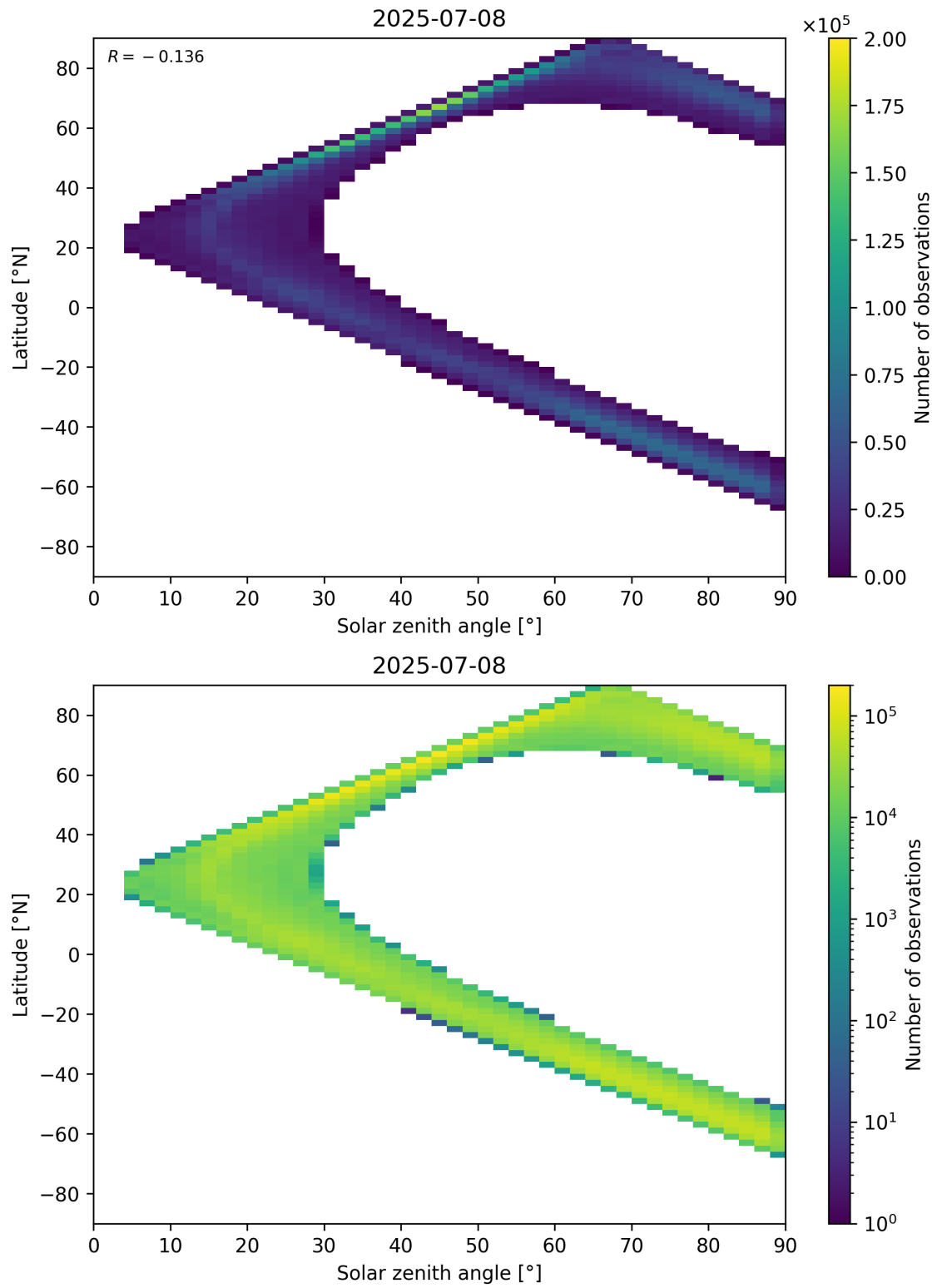
Figure 105: Scatter density plot of “Solar zenith angle” against “Latitude” for 2025-07-08 to 2025-07-09.
