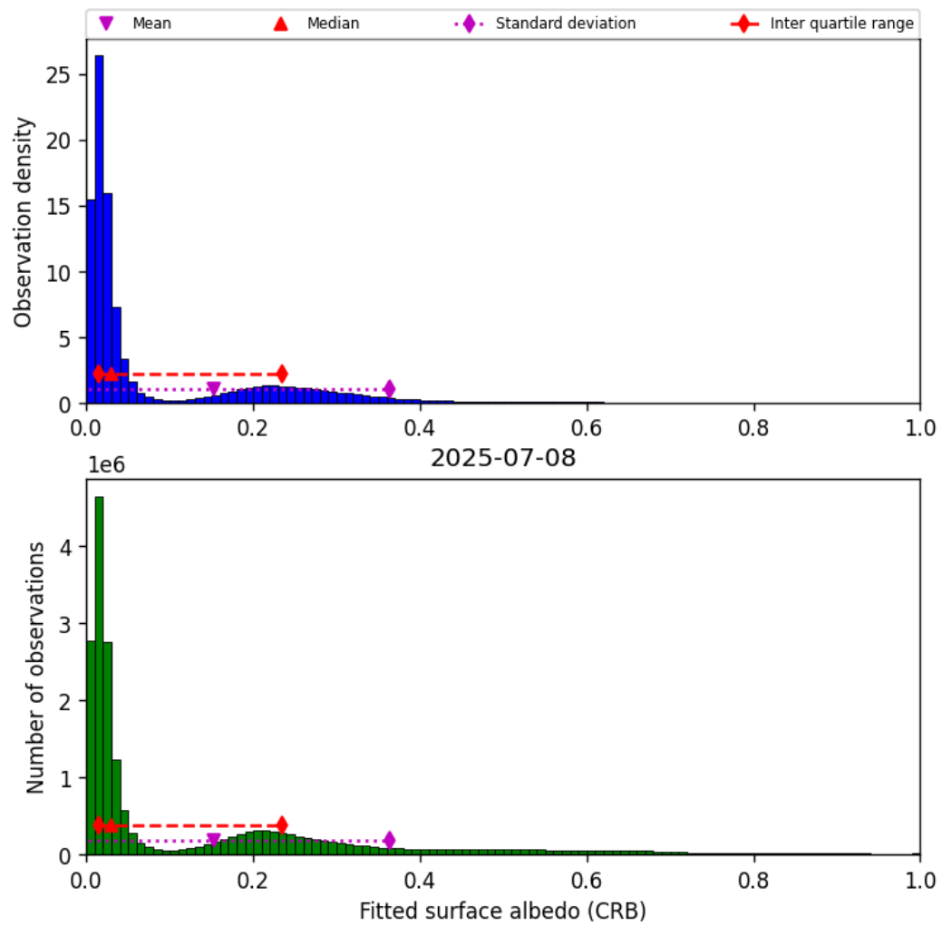
Figure 46: Histogram of “Fitted surface albedo (CRB)” for 2025-07-08 to 2025-07-09
