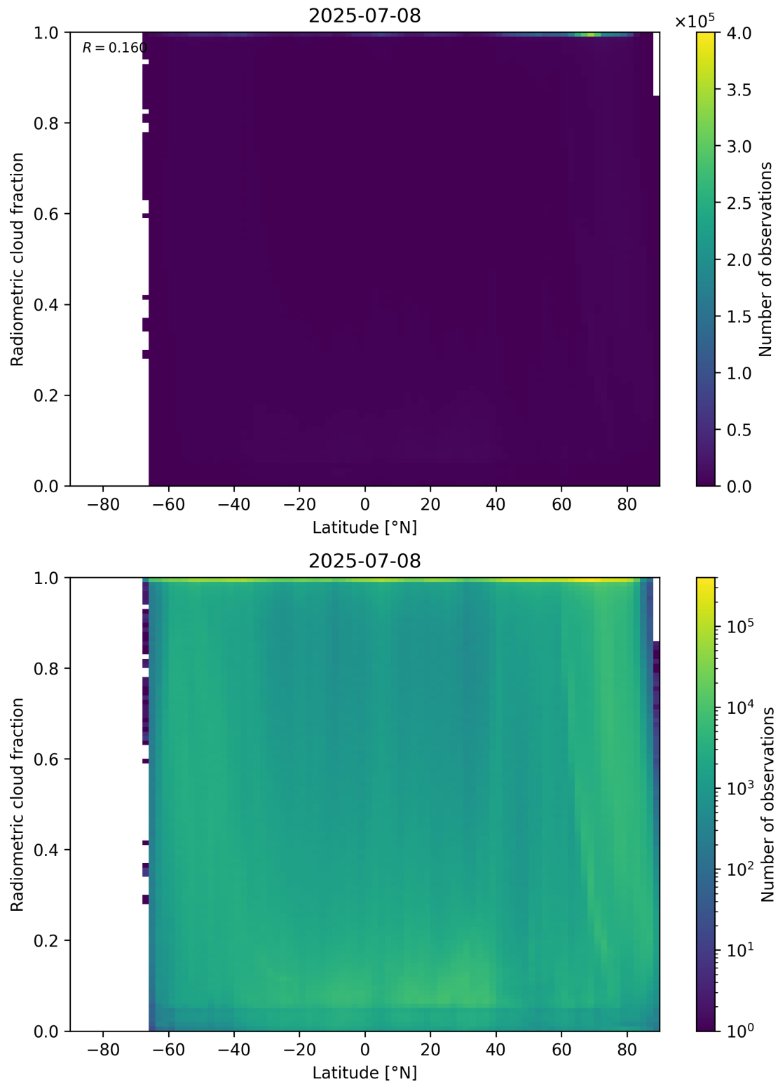
Figure 92: Scatter density plot of “Latitude” against “Radiometric cloud fraction” for 2025-07-08 to 2025-07-09.
