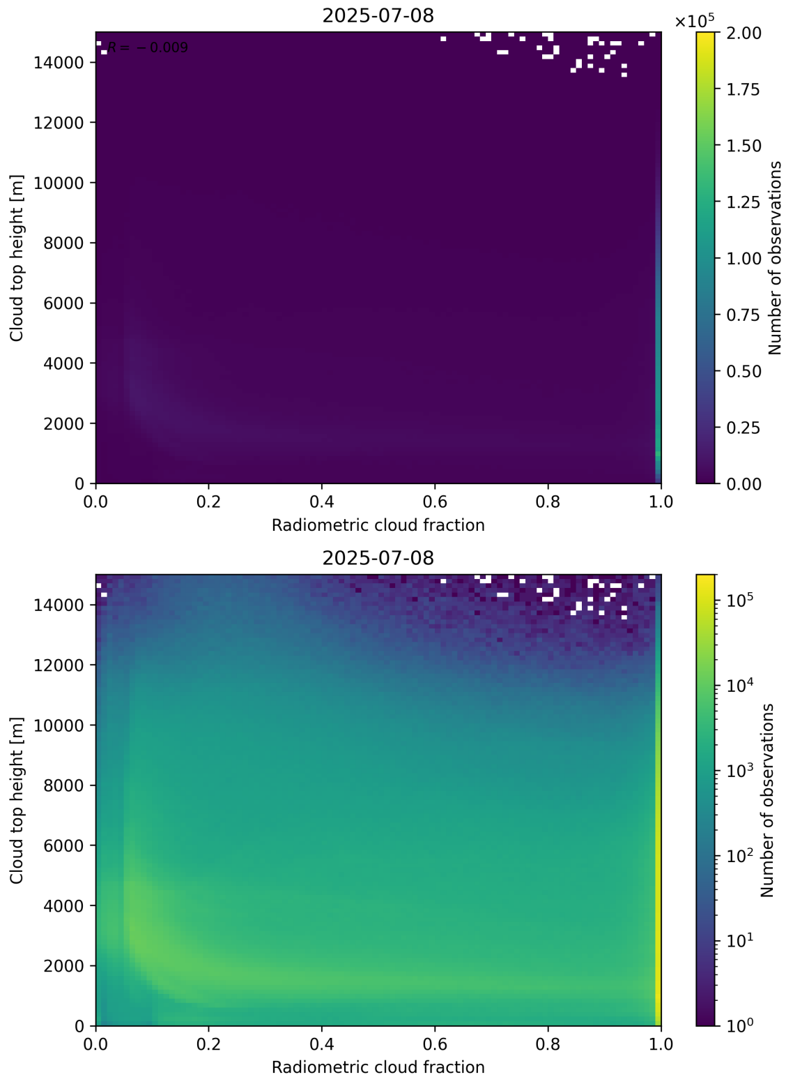
Figure 76: Scatter density plot of “Radiometric cloud fraction” against “Cloud top height” for 2025-07-08 to 2025-07-09.
