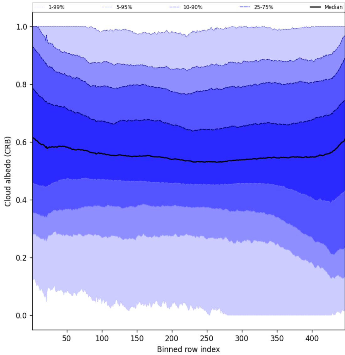
Figure 60: Along track statistics of “Cloud albedo (CRB)” for 2025-07-08 to 2025-07-09
