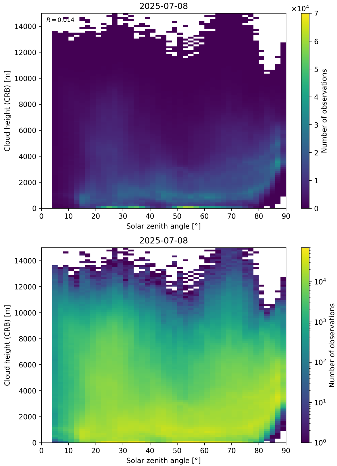
Figure 102: Scatter density plot of “Solar zenith angle” against “Cloud height (CRB)” for 2025-07-08 to 2025-07-09.
