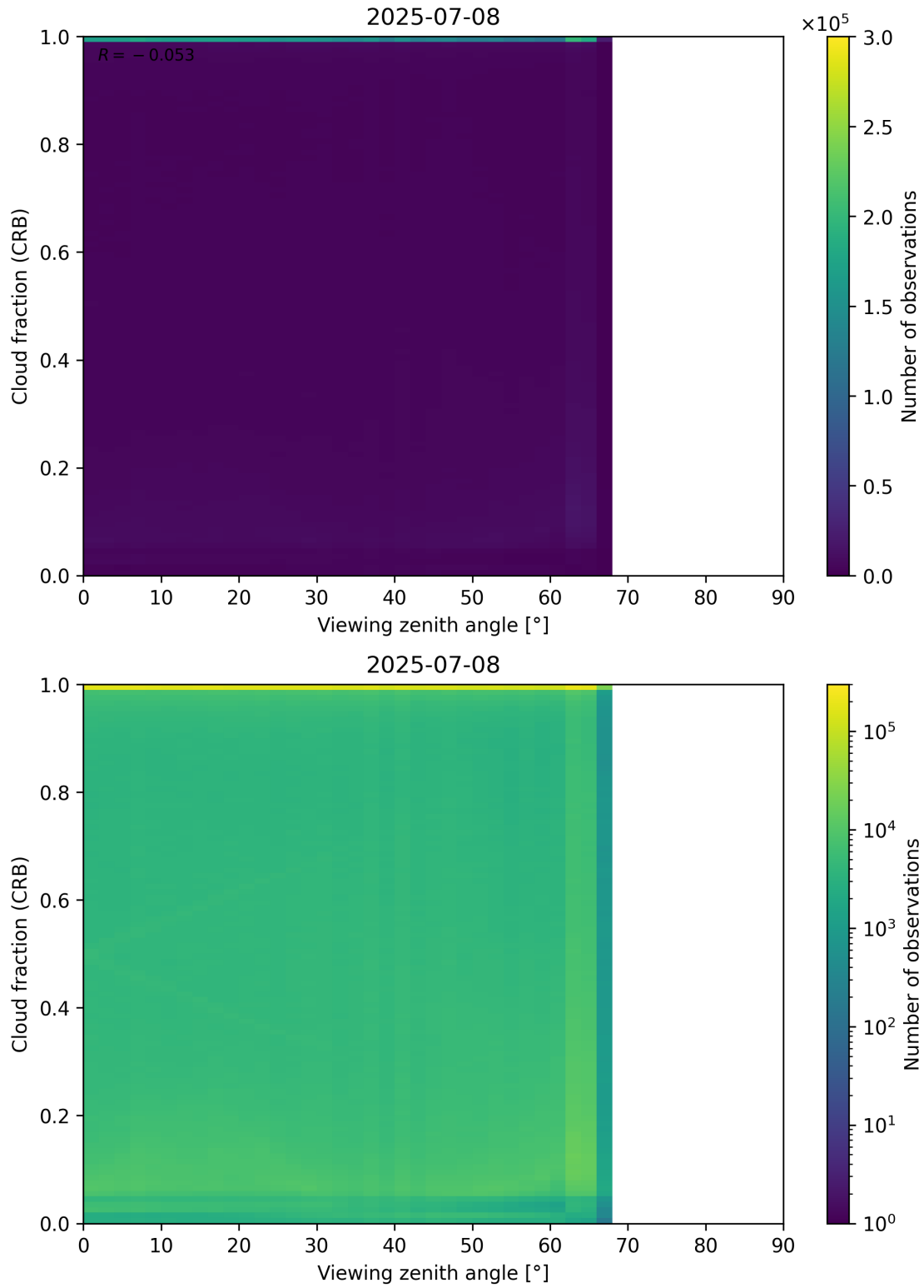
Figure 109: Scatter density plot of “Viewing zenith angle” against “Cloud fraction (CRB)” for 2025-07-08 to 2025-07-09.
