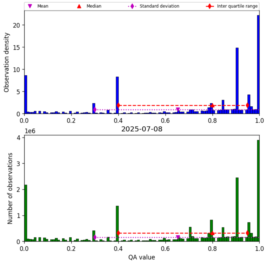
Figure 38: Histogram of “QA value” for 2025-07-08 to 2025-07-09
