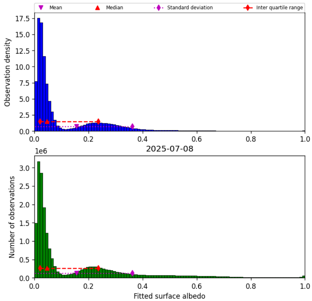
Figure 45: Histogram of “Fitted surface albedo” for 2025-07-08 to 2025-07-09
