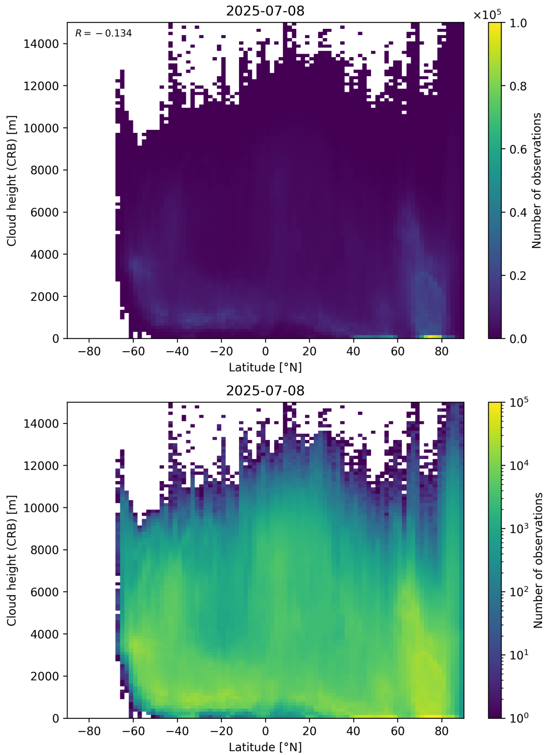
Figure 95: Scatter density plot of “Latitude” against “Cloud height (CRB)” for 2025-07-08 to 2025-07-09.
