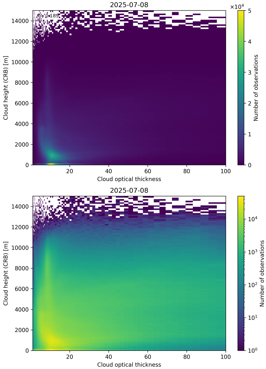
Figure 85: Scatter density plot of “Cloud optical thickness” against “Cloud height (CRB)” for 2025-07-08 to 2025-07-09.
