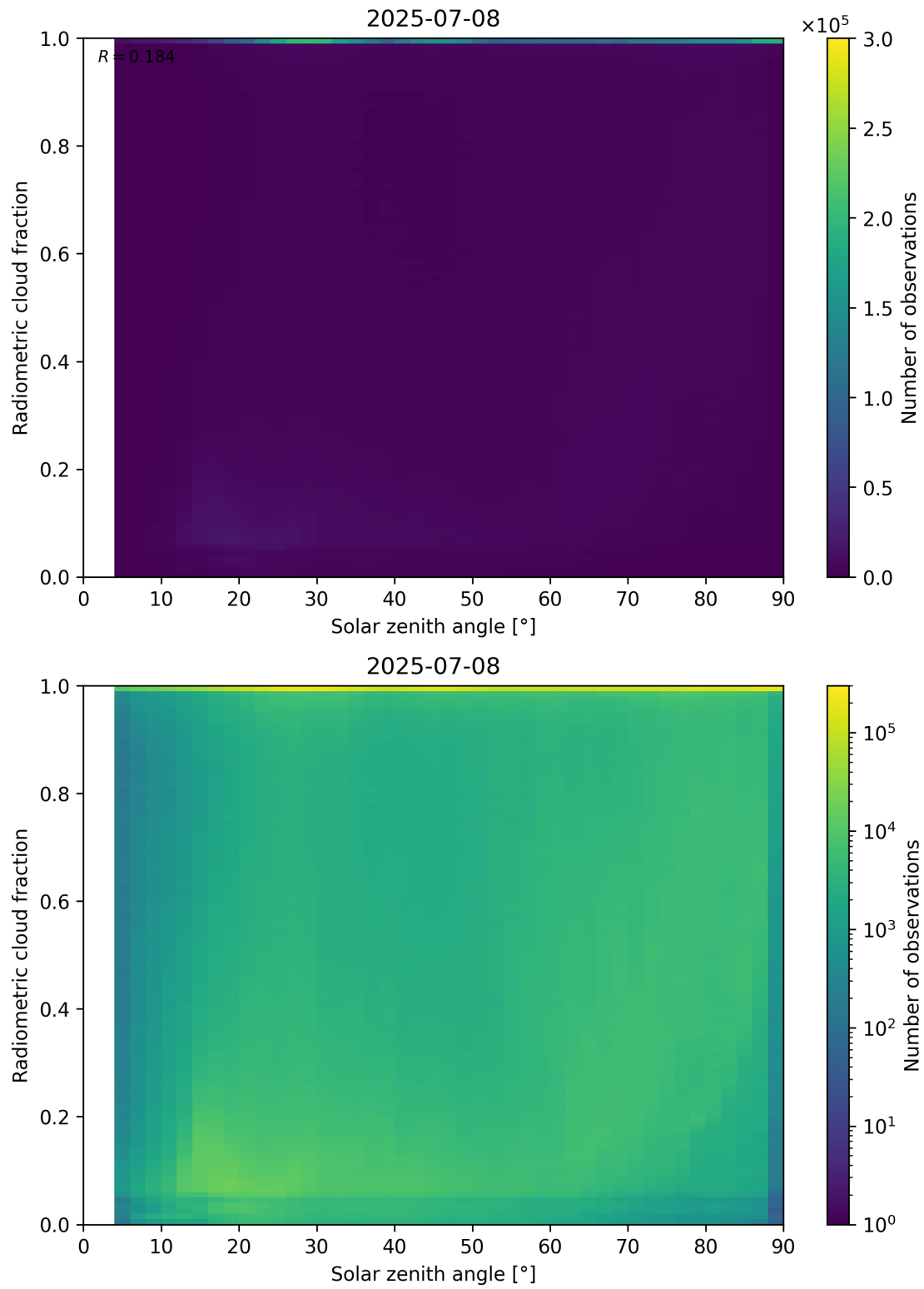
Figure 99: Scatter density plot of “Solar zenith angle” against “Radiometric cloud fraction” for 2025-07-08 to 2025-07-09.
