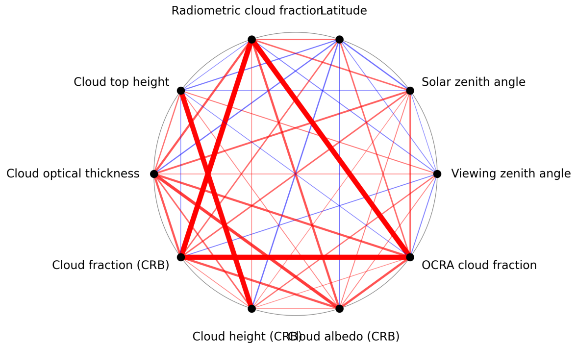
Figure 1: Map of correlation graph for 2025-07-08 to 2025-07-09.
