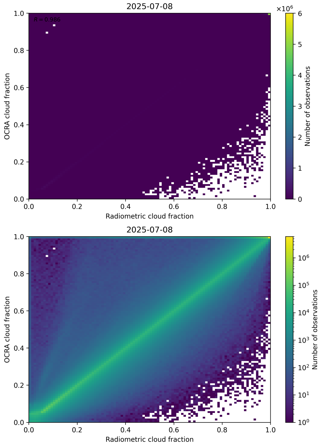
Figure 72: Scatter density plot of “Radiometric cloud fraction” against “OCRA cloud fraction” for 2025-07-08 to 2025-07-09.
