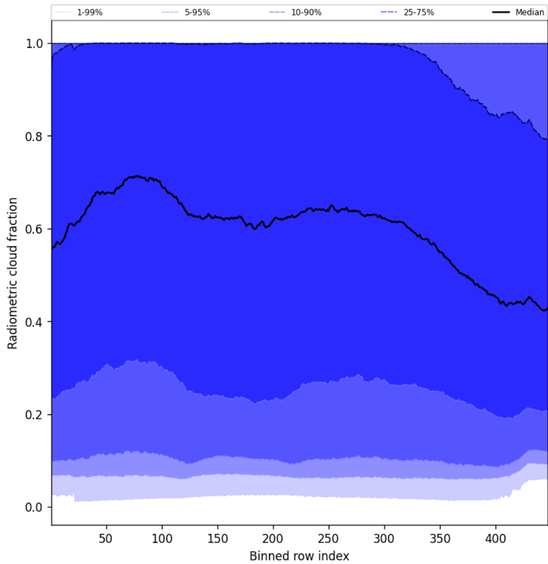
Figure 55: Along track statistics of “Radiometric cloud fraction” for 2025-07-08 to 2025-07-09
