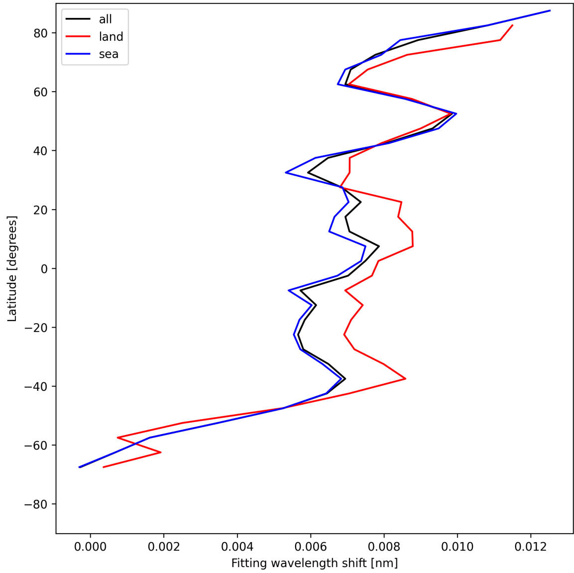
Figure 33: Zonal average of “Fitting wavelength shift” for 2025-07-08 to 2025-07-09.
