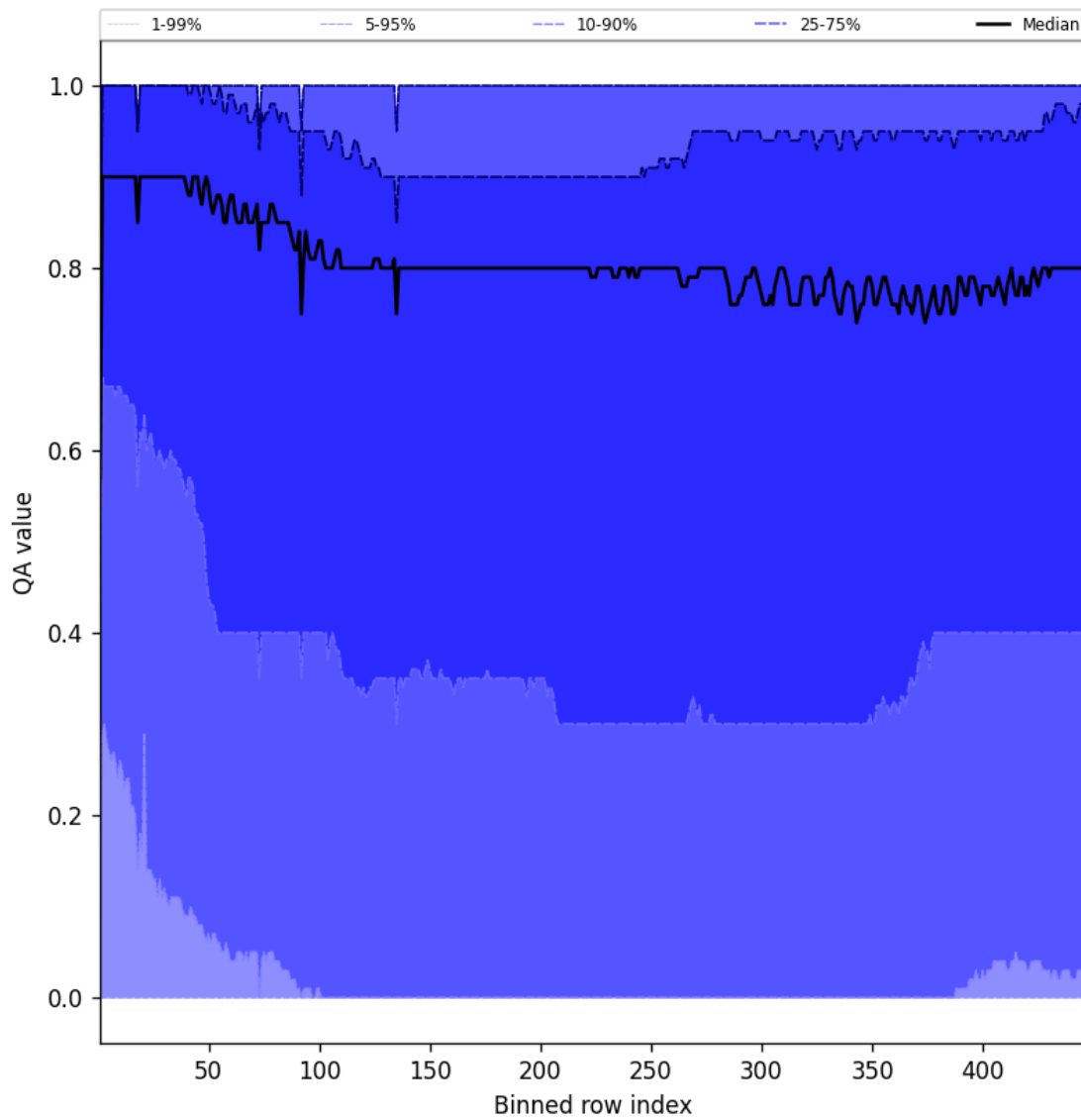
Figure 54: Along track statistics of “QA value” for 2025-07-08 to 2025-07-09
