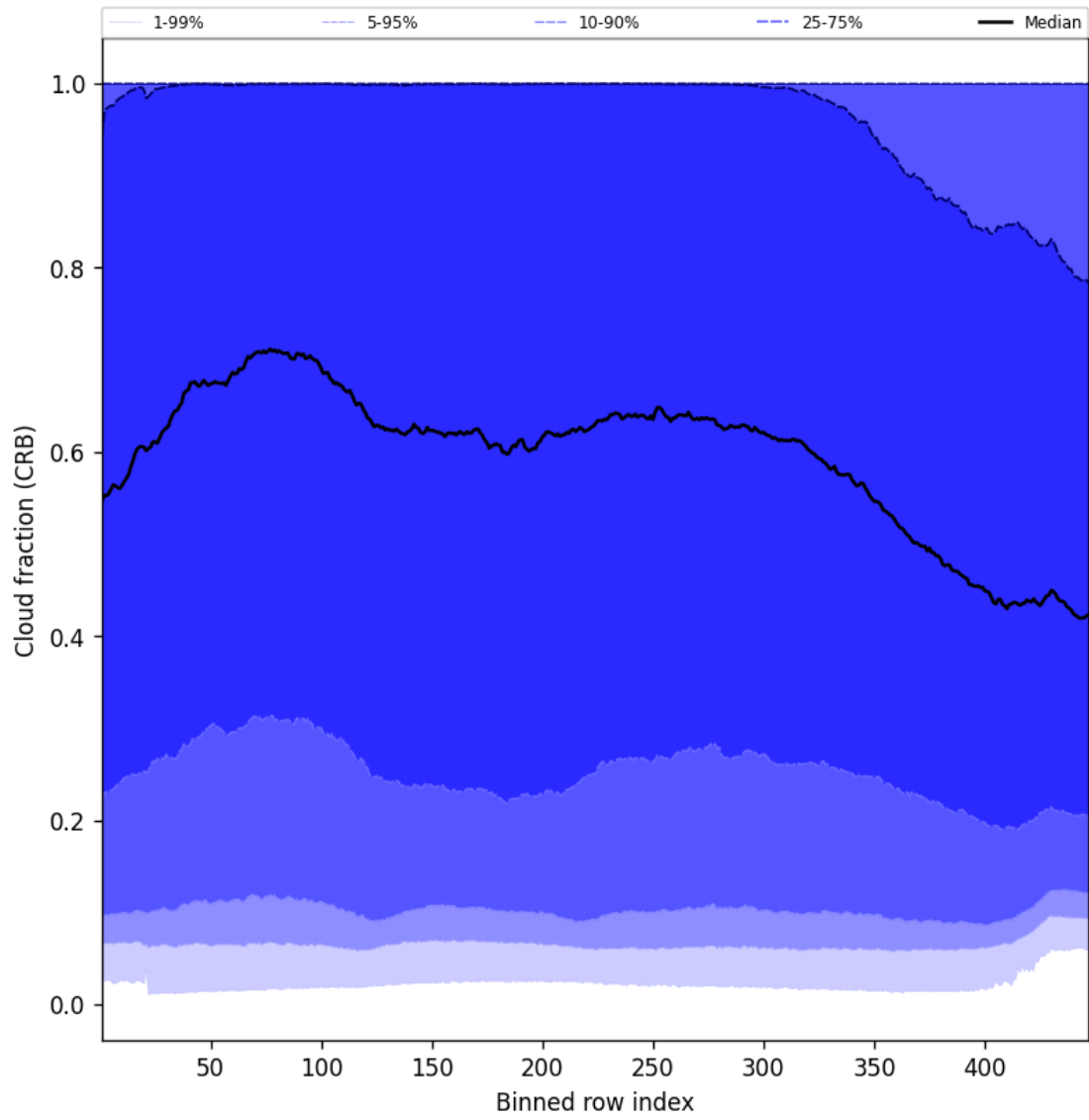
Figure 58: Along track statistics of “Cloud fraction (CRB)” for 2025-07-08 to 2025-07-09
