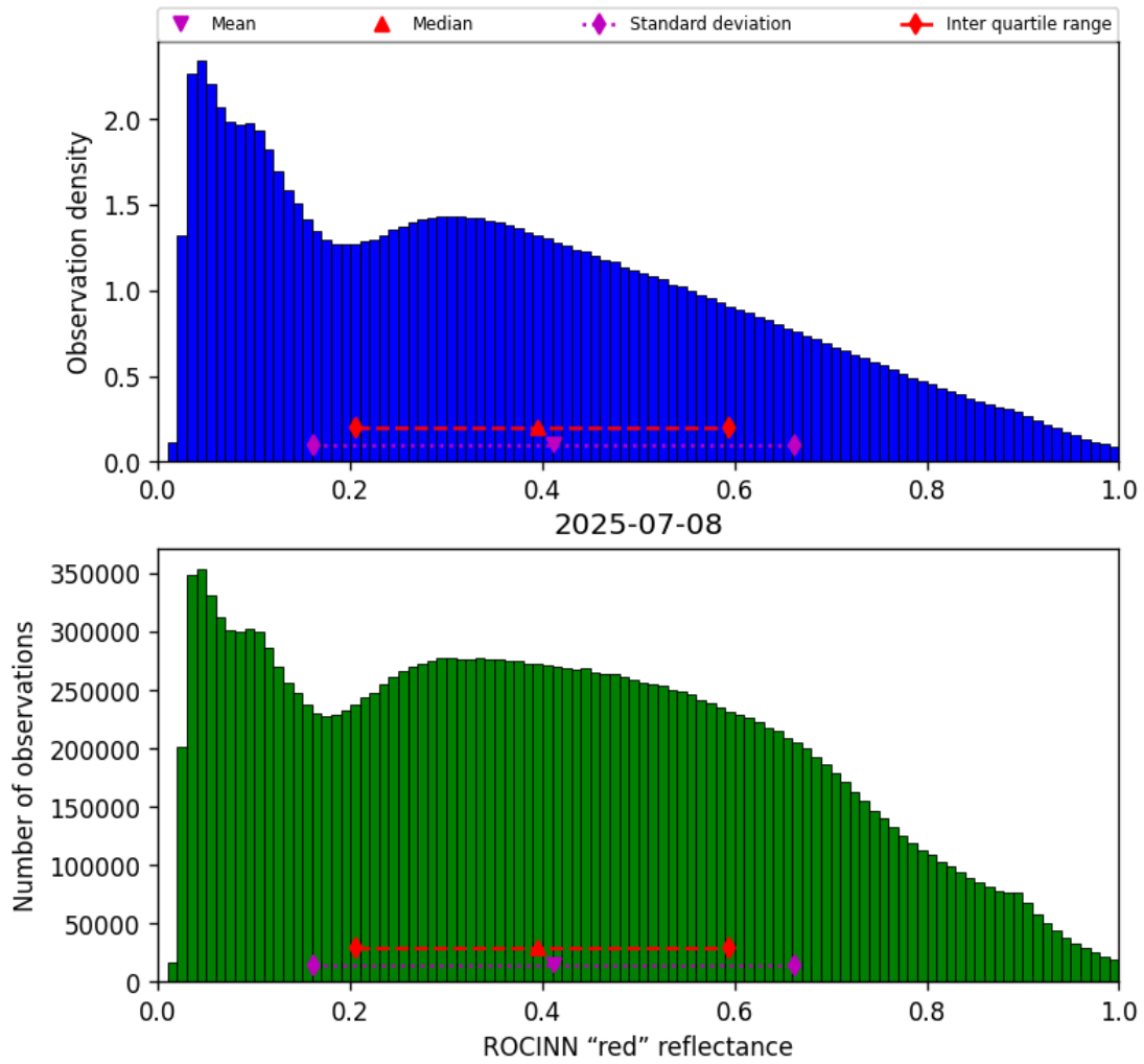
Figure 53: Histogram of “ROCINN “red” reflectance” for 2025-07-08 to 2025-07-09
