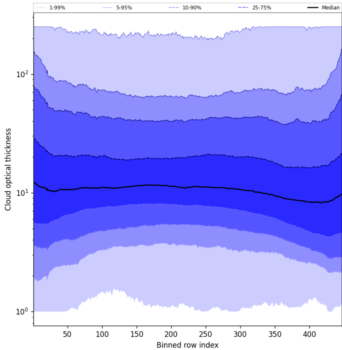
Figure 57: Along track statistics of “Cloud optical thickness” for 2025-07-08 to 2025-07-09
