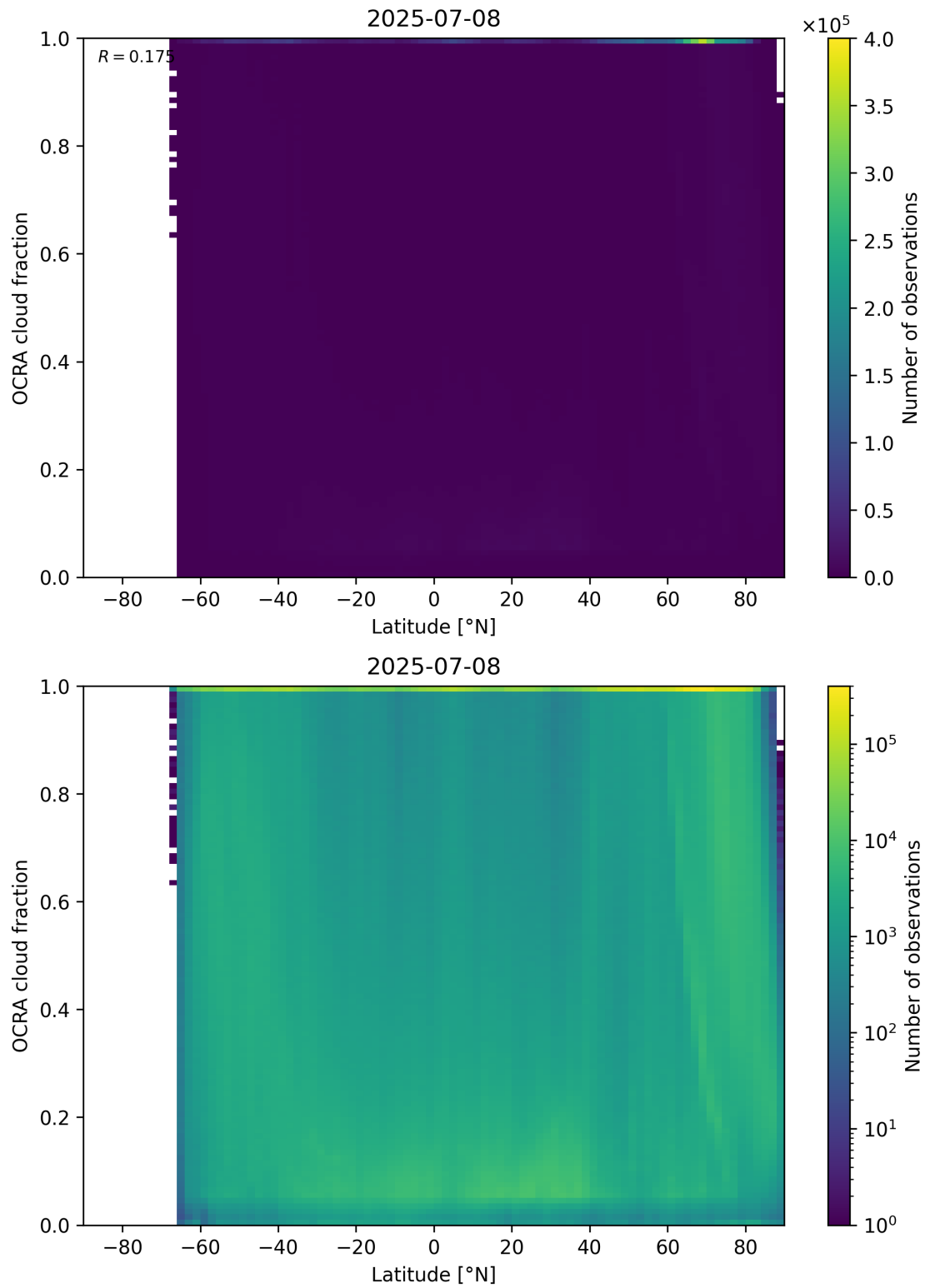
Figure 93: Scatter density plot of “Latitude” against “OCRA cloud fraction” for 2025-07-08 to 2025-07-09.
