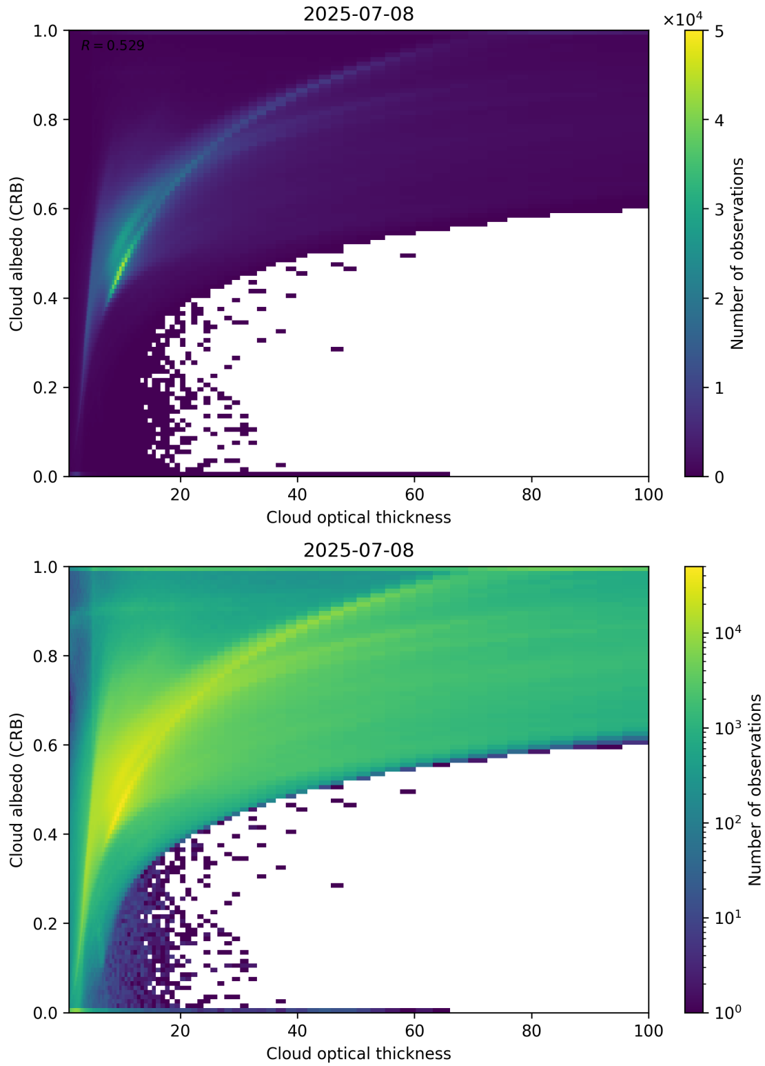
Figure 82: Scatter density plot of “Cloud optical thickness” against “Cloud albedo (CRB)” for 2025-07-08 to 2025-07-09.
