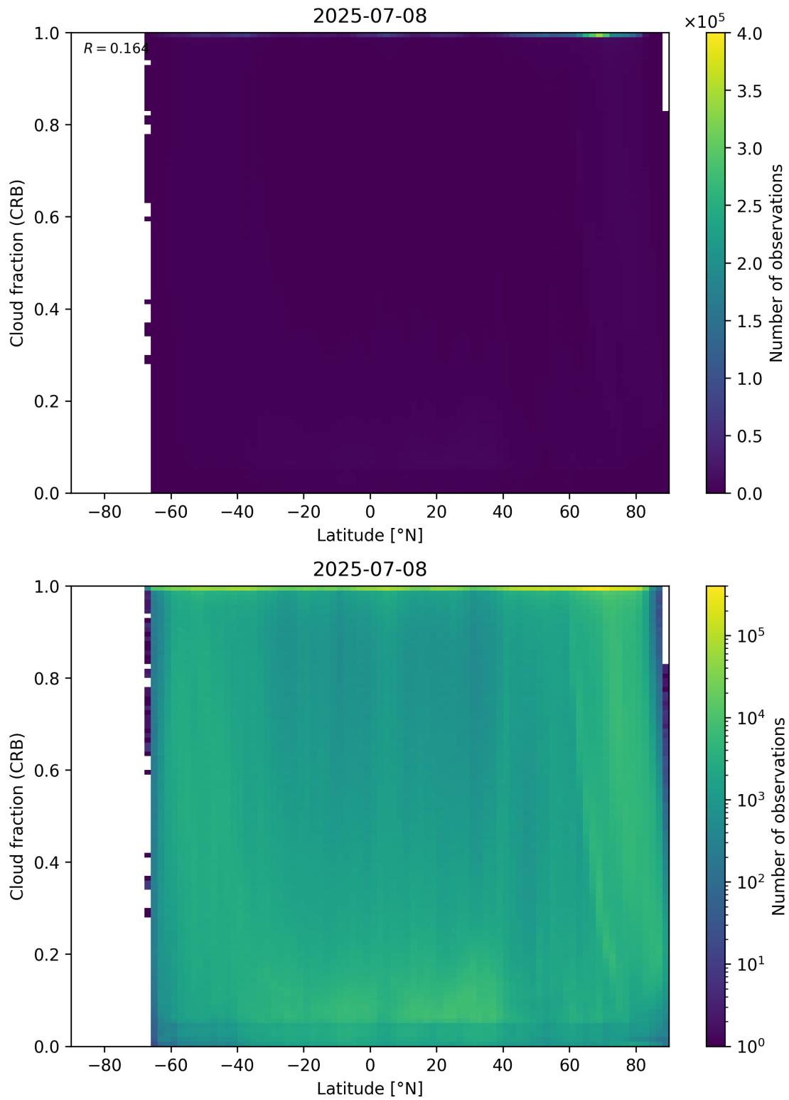
Figure 94: Scatter density plot of “Latitude” against “Cloud fraction (CRB)” for 2025-07-08 to 2025-07-09.
