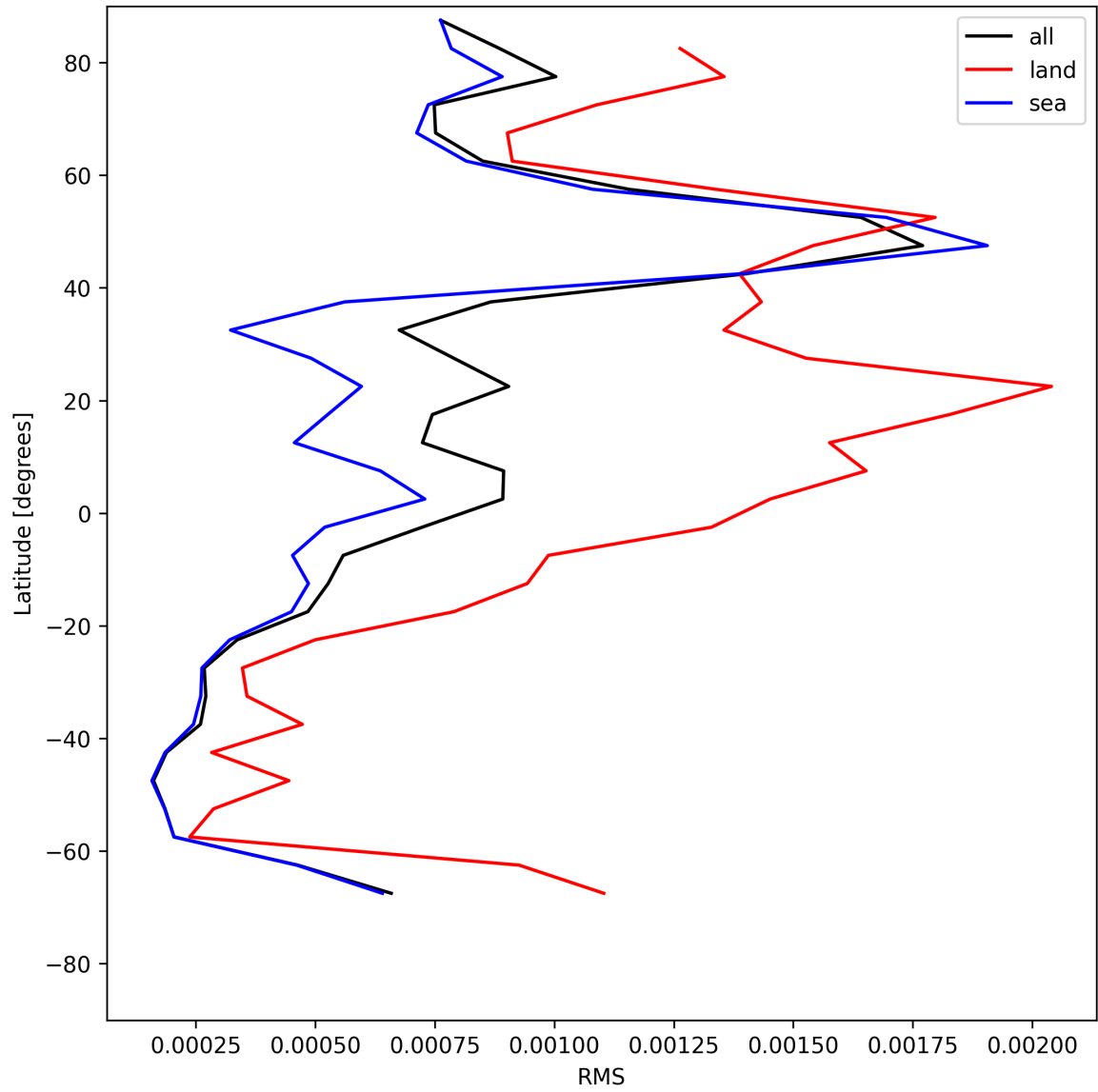
Figure 31: Zonal average of “RMS” for 2025-07-08 to 2025-07-09.
