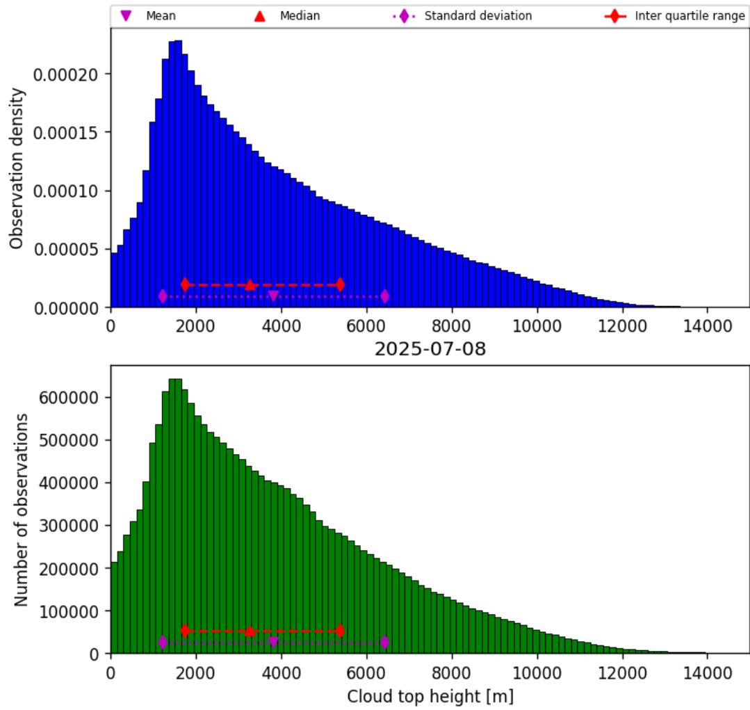
Figure 40: Histogram of “Cloud top height” for 2025-07-08 to 2025-07-09
