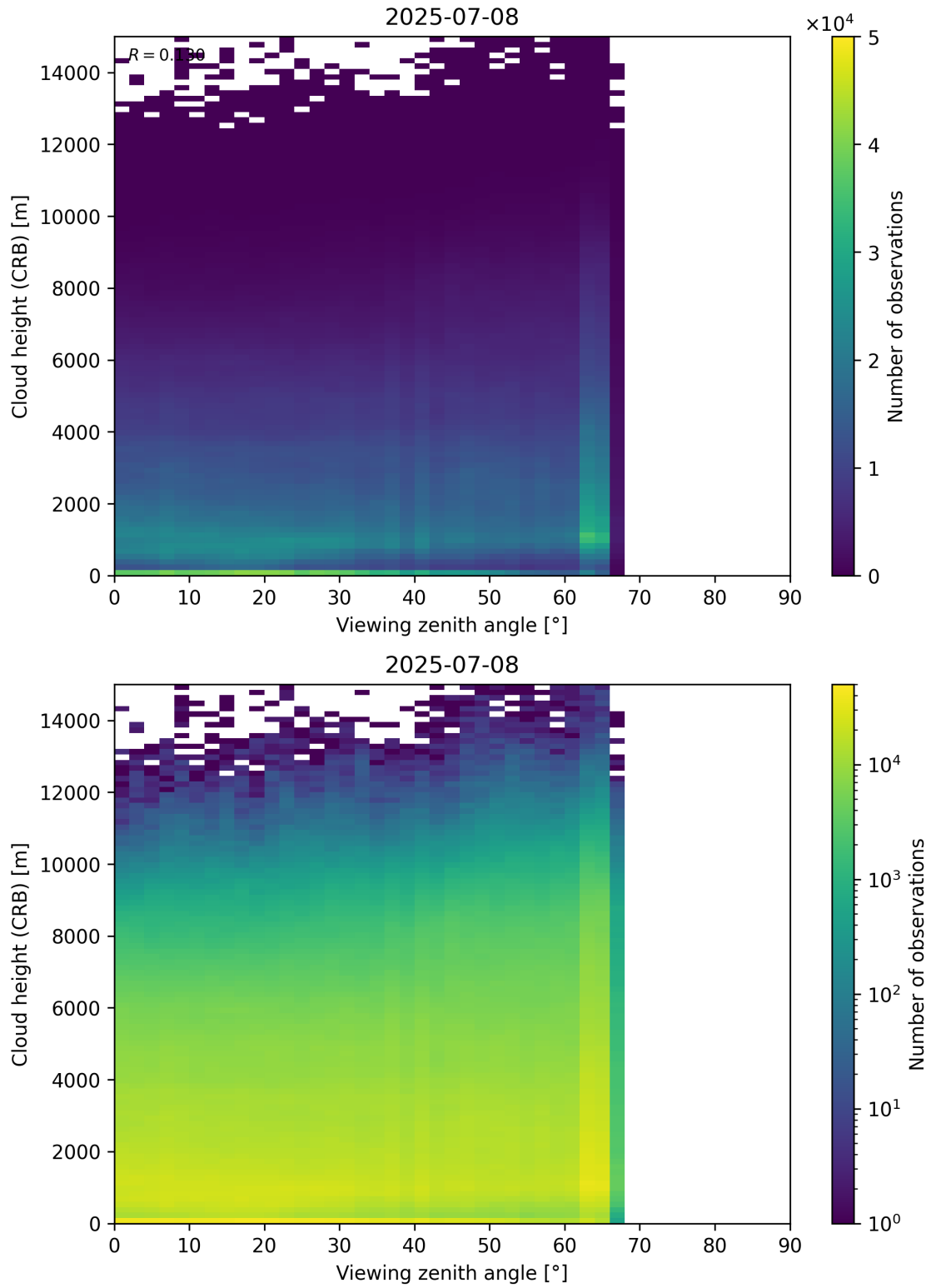
Figure 110: Scatter density plot of “Viewing zenith angle” against “Cloud height (CRB)” for 2025-07-08 to 2025-07-09.
