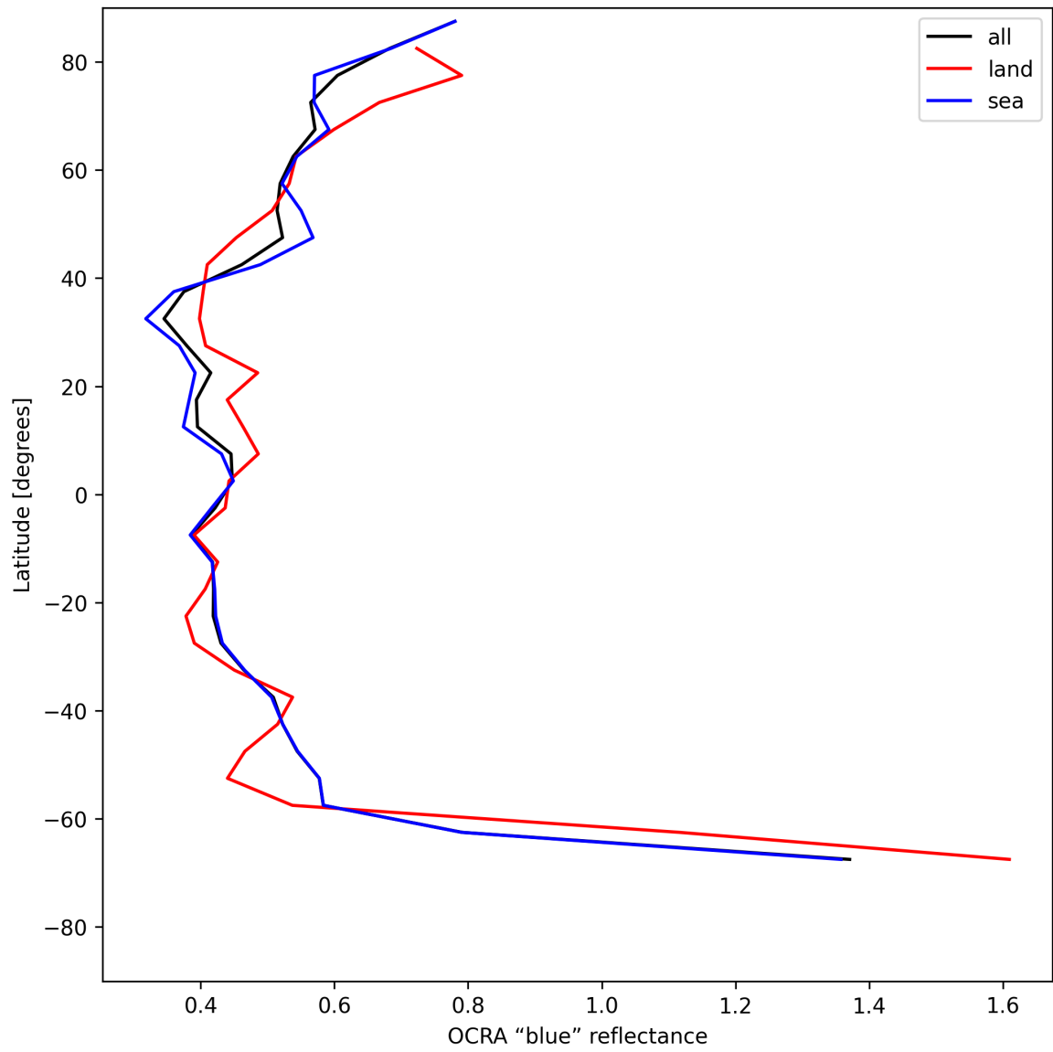
Figure 35: Zonal average of “OCRA “blue” reflectance” for 2025-07-08 to 2025-07-09.
