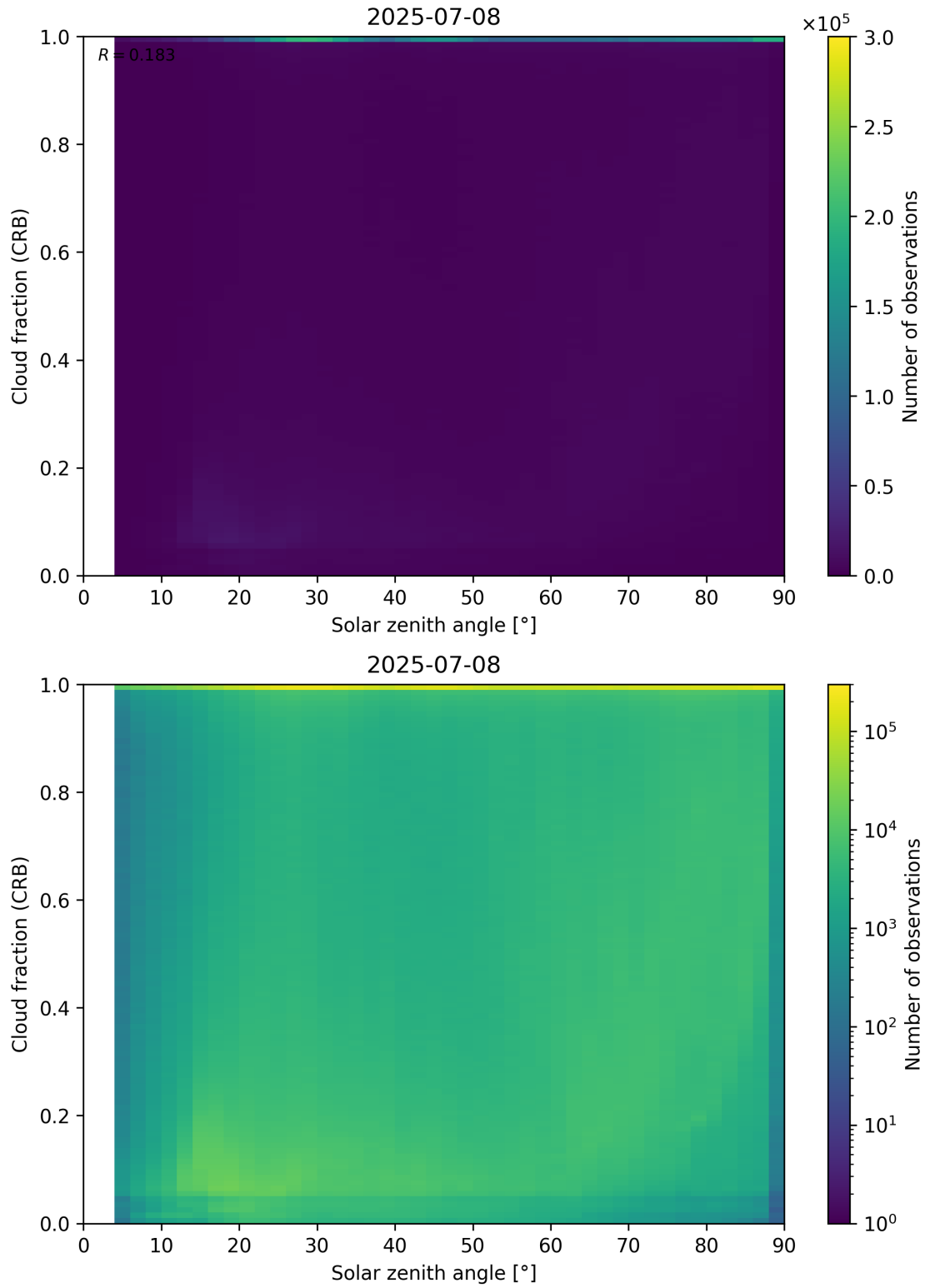
Figure 101: Scatter density plot of “Solar zenith angle” against “Cloud fraction (CRB)” for 2025-07-08 to 2025-07-09.
