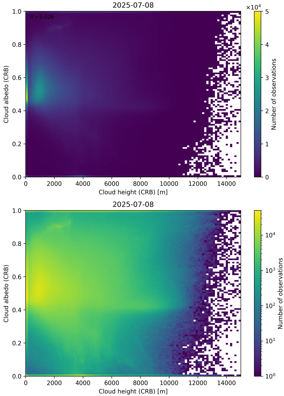
Figure 80: Scatter density plot of “Cloud height (CRB)” against “Cloud albedo (CRB)” for 2025-07-08 to 2025-07-09.
