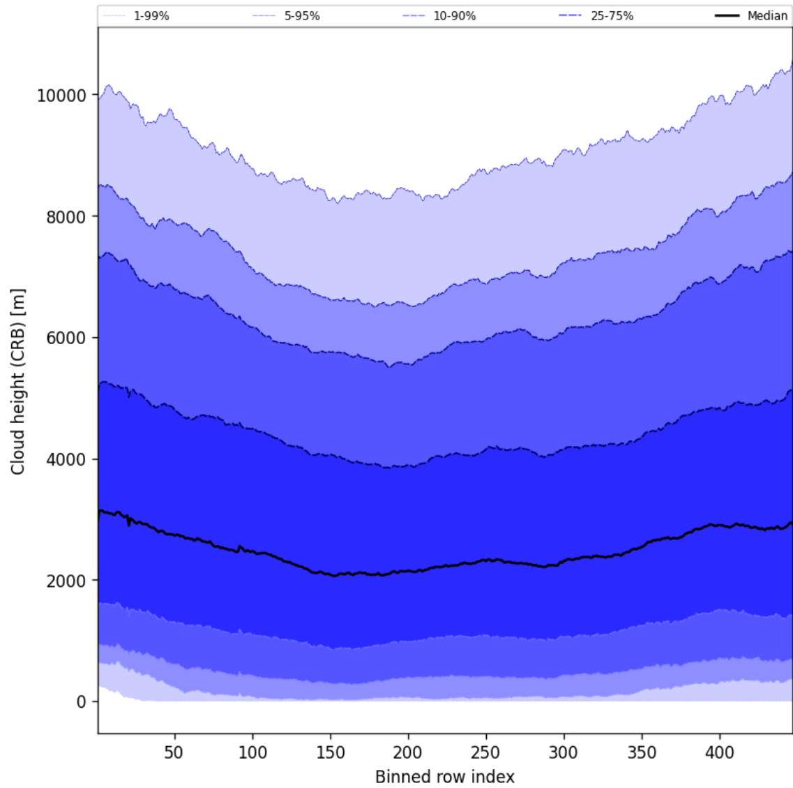
Figure 59: Along track statistics of “Cloud height (CRB)” for 2025-07-08 to 2025-07-09
