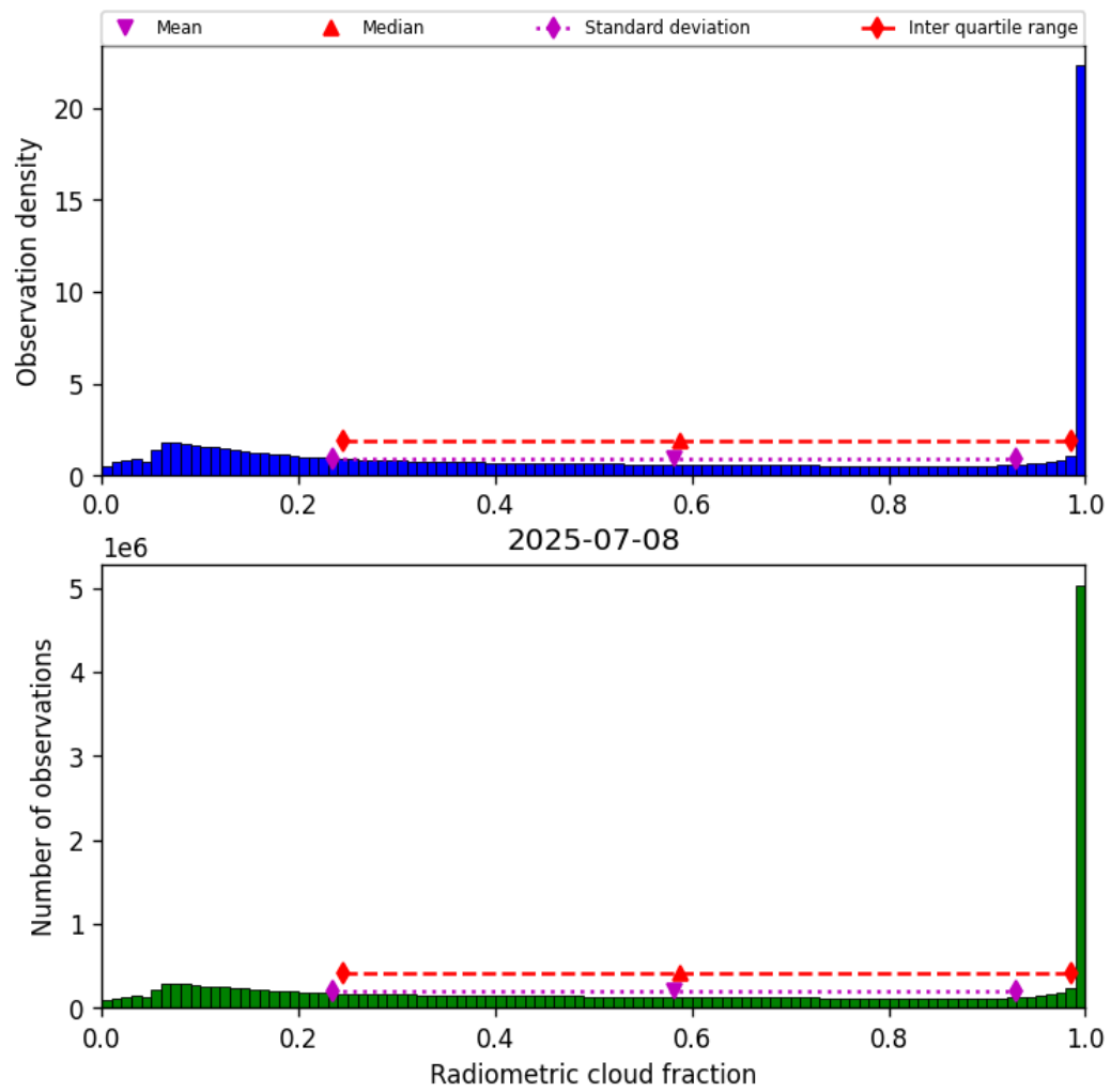
Figure 39: Histogram of “Radiometric cloud fraction” for 2025-07-08 to 2025-07-09
