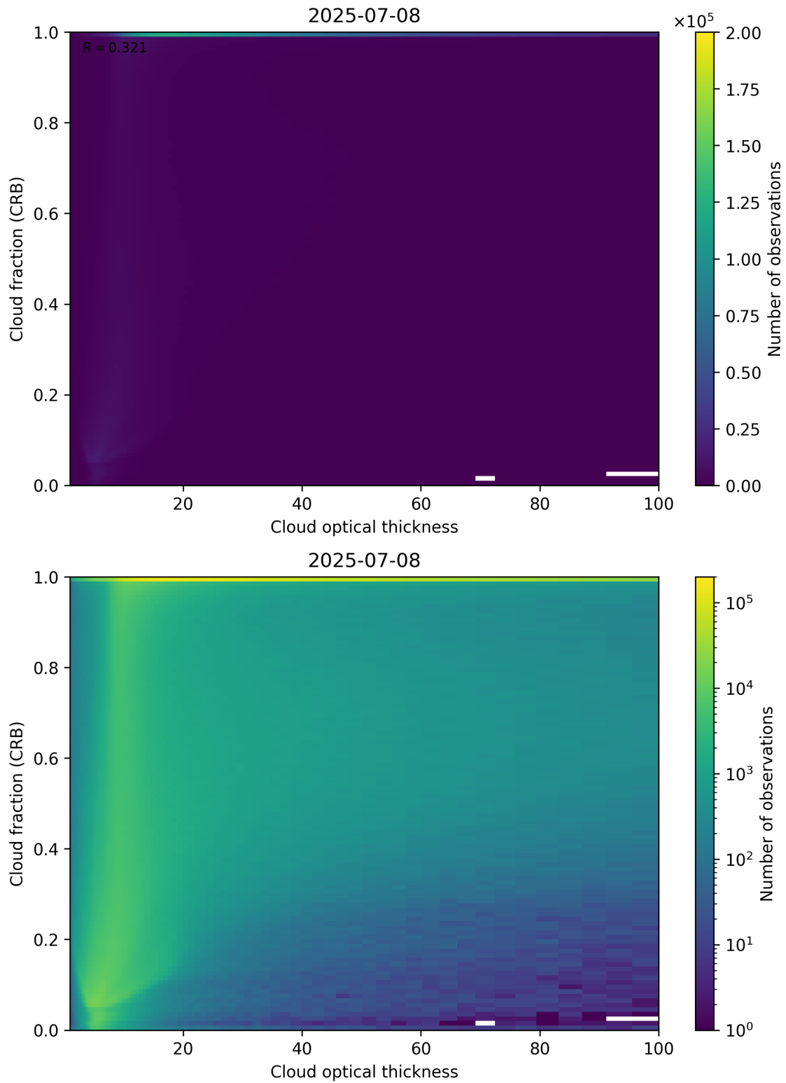
Figure 84: Scatter density plot of “Cloud optical thickness” against “Cloud fraction (CRB)” for 2025-07-08 to 2025-07-09.
