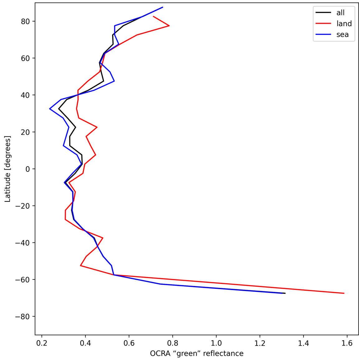
Figure 36: Zonal average of “OCRA “green” reflectance” for 2025-07-08 to 2025-07-09.
