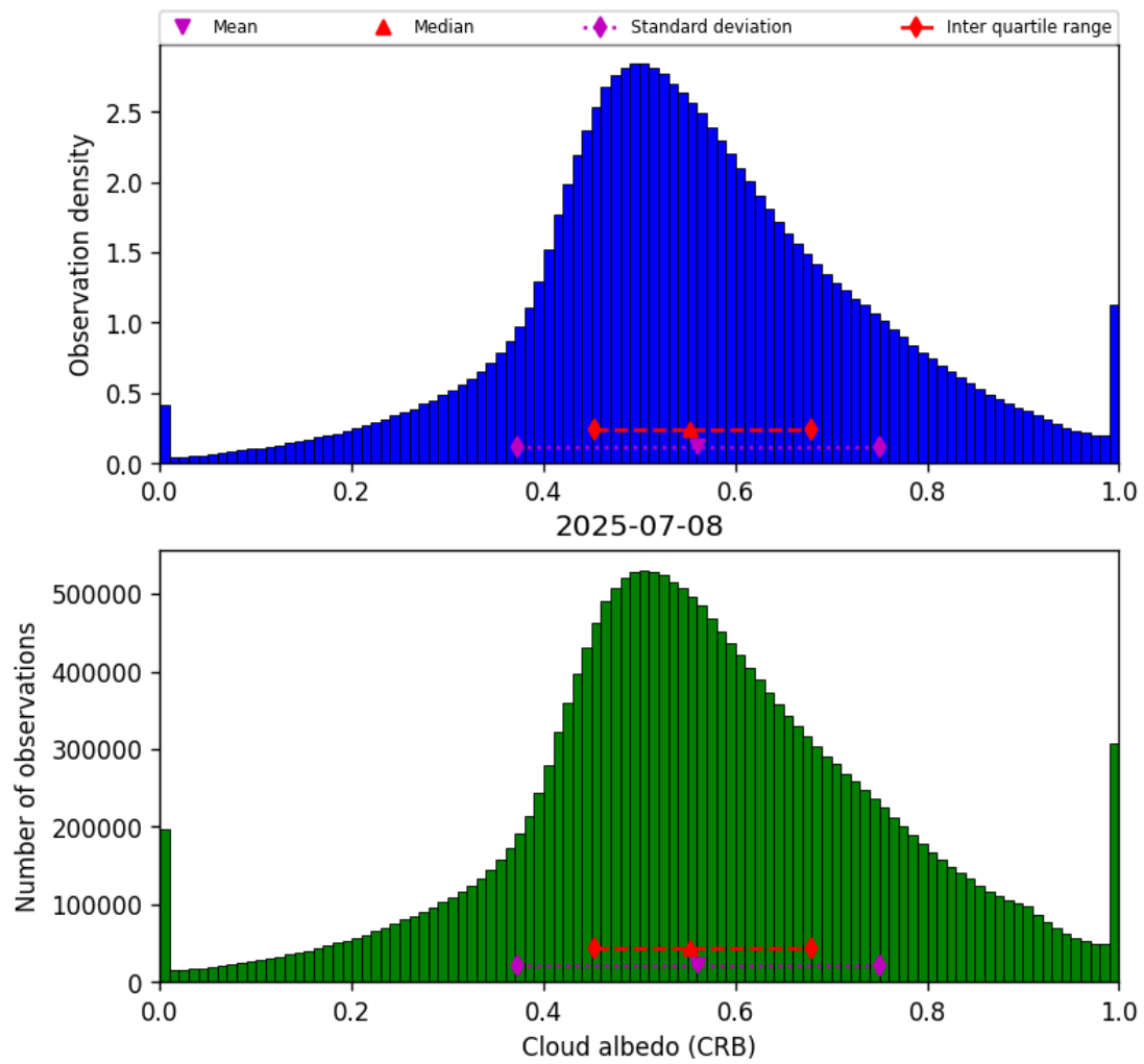
Figure 44: Histogram of “Cloud albedo (CRB)” for 2025-07-08 to 2025-07-09
