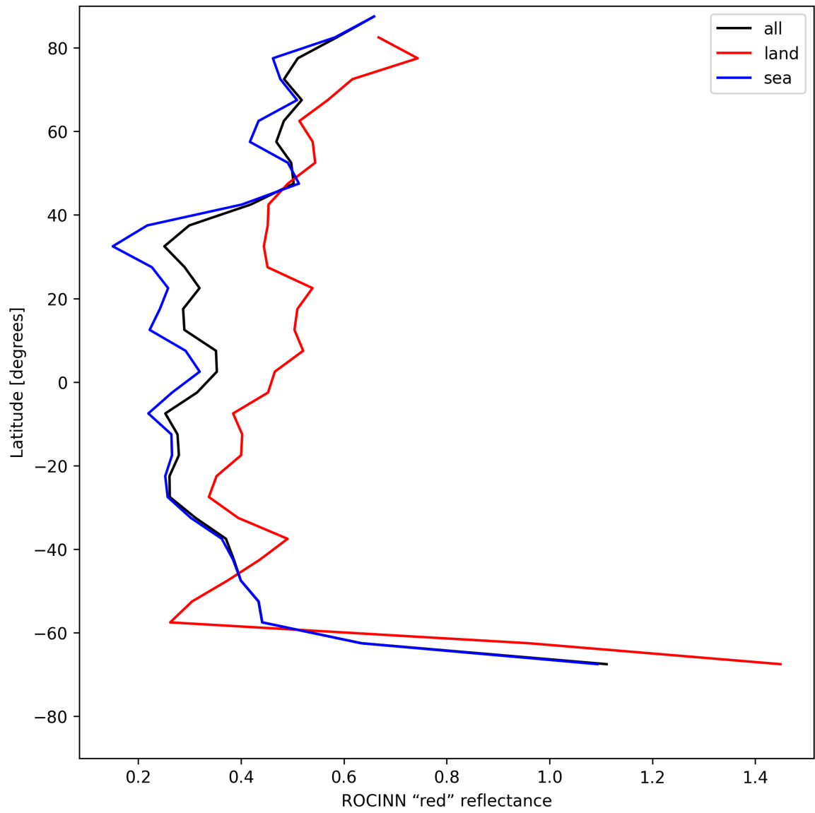
Figure 37: Zonal average of “ROCINN “red” reflectance” for 2025-07-08 to 2025-07-09.
