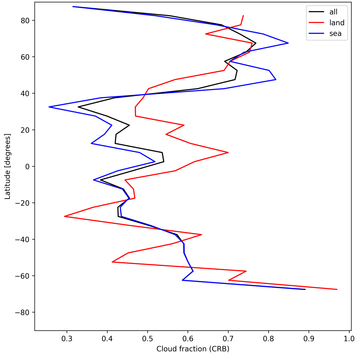
Figure 26: Zonal average of “Cloud fraction (CRB)” for 2025-07-08 to 2025-07-09.
