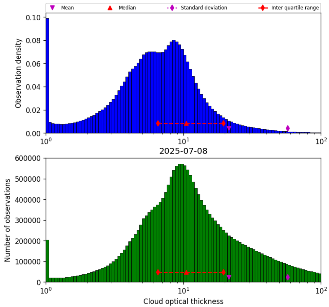
Figure 41: Histogram of “Cloud optical thickness” for 2025-07-08 to 2025-07-09
