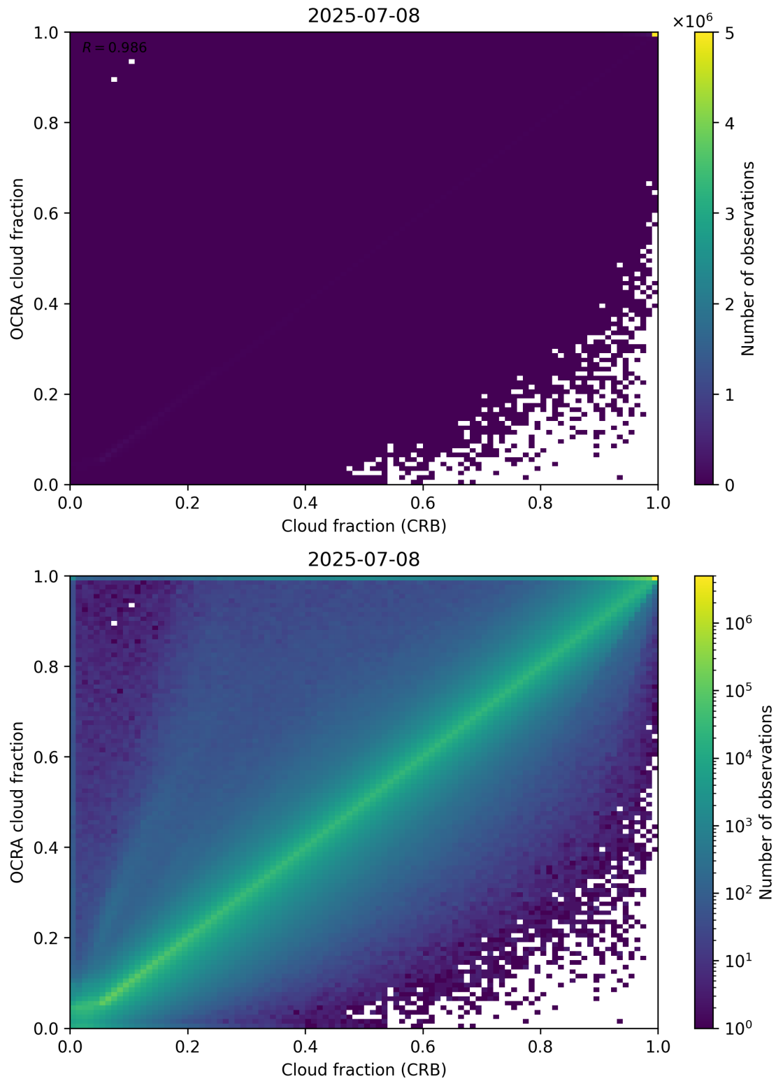
Figure 78: Scatter density plot of “Cloud fraction (CRB)” against “OCRA cloud fraction” for 2025-07-08 to 2025-07-09.
