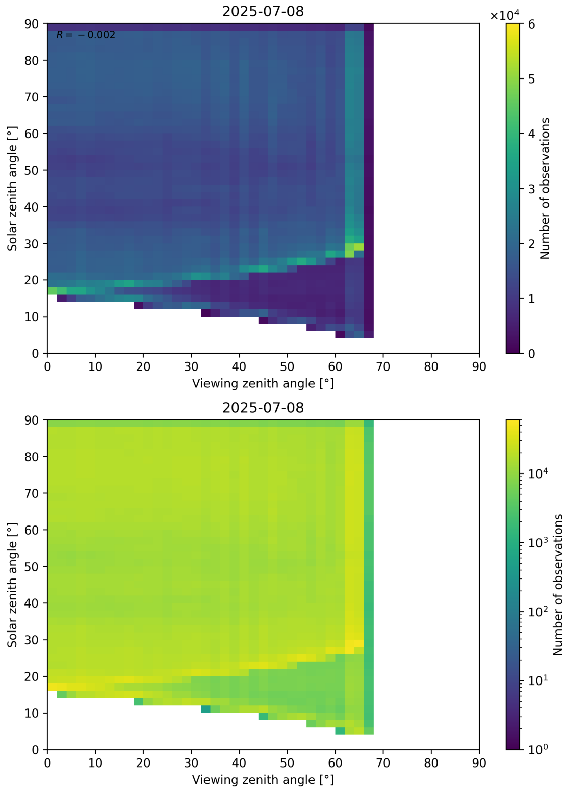
Figure 114: Scatter density plot of “Viewing zenith angle” against “Solar zenith angle” for 2025-07-08 to 2025-07-09.
