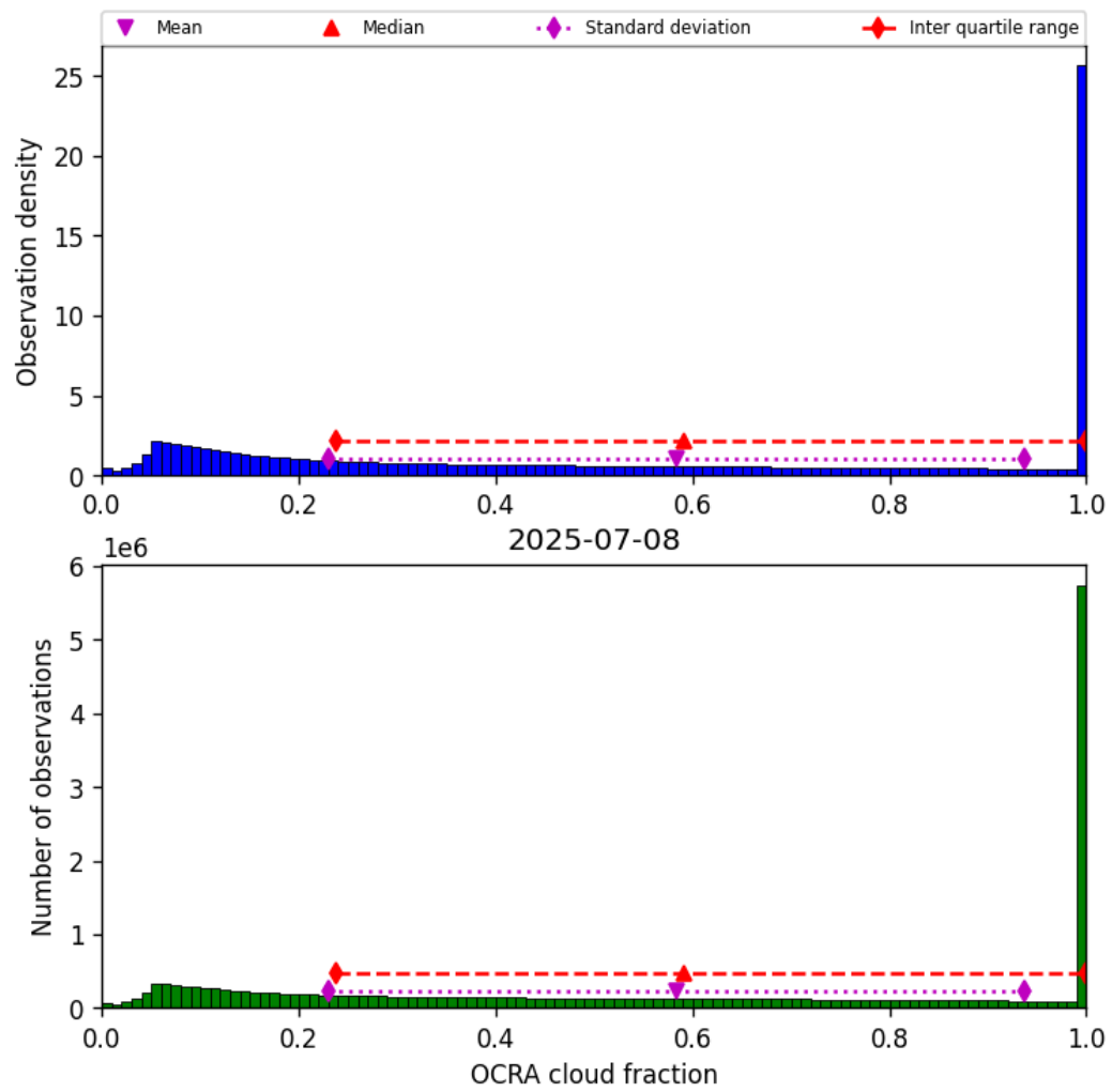
Figure 50: Histogram of “OCRA cloud fraction” for 2025-07-08 to 2025-07-09
