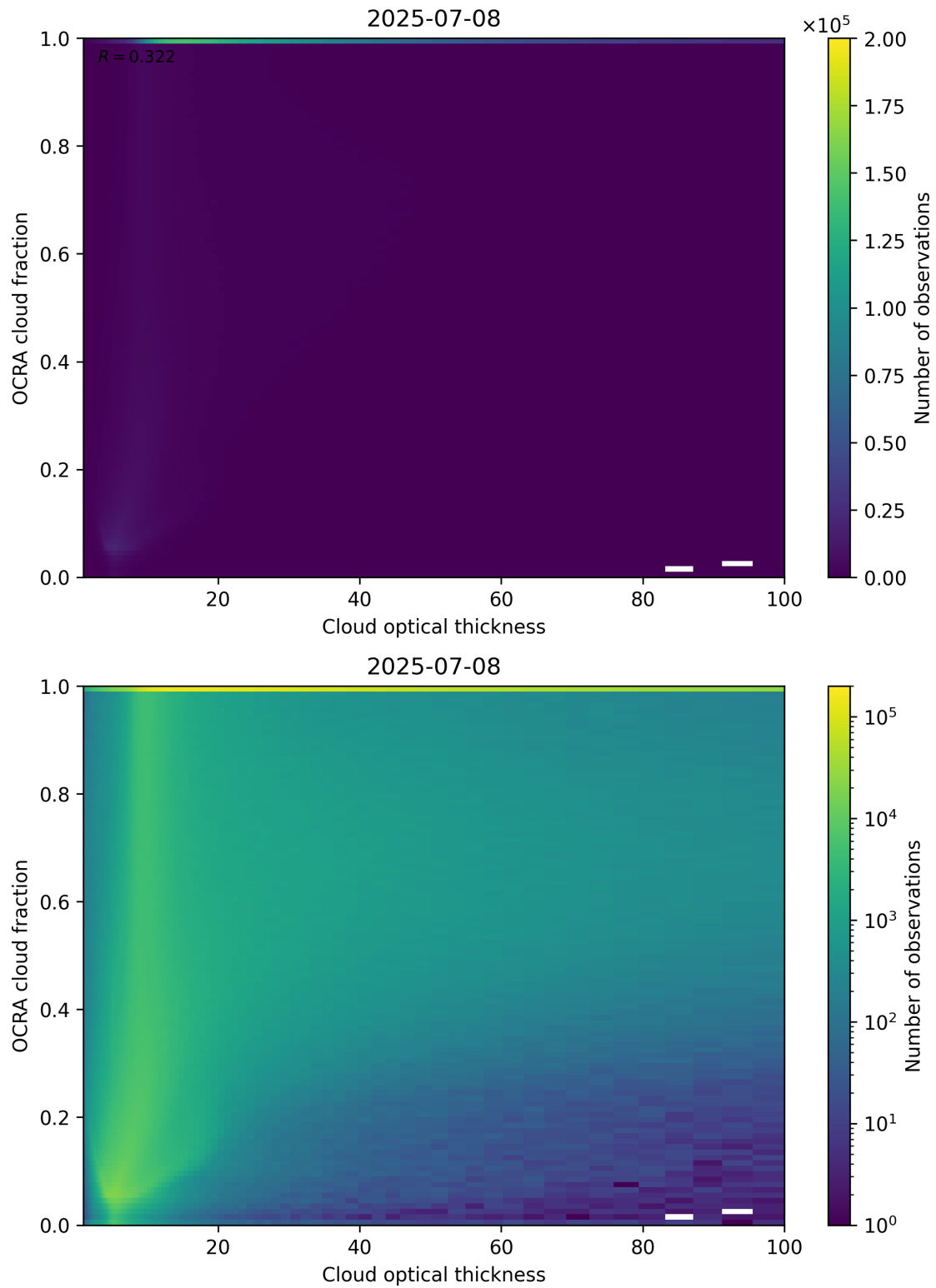
Figure 83: Scatter density plot of “Cloud optical thickness” against “OCRA cloud fraction” for 2025-07-08 to 2025-07-09.
