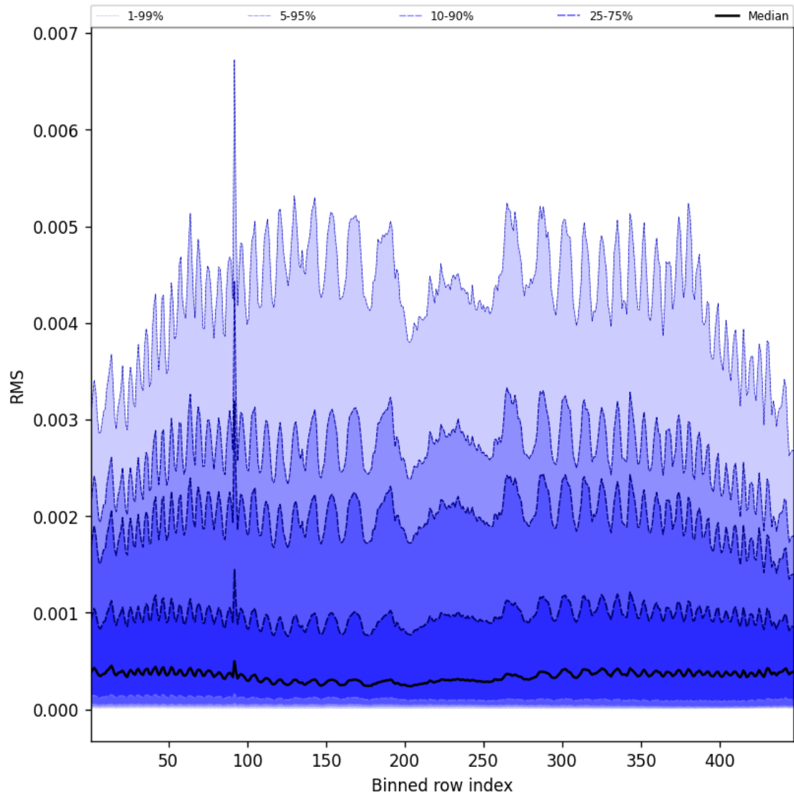
Figure 63: Along track statistics of “RMS” for 2025-07-08 to 2025-07-09
