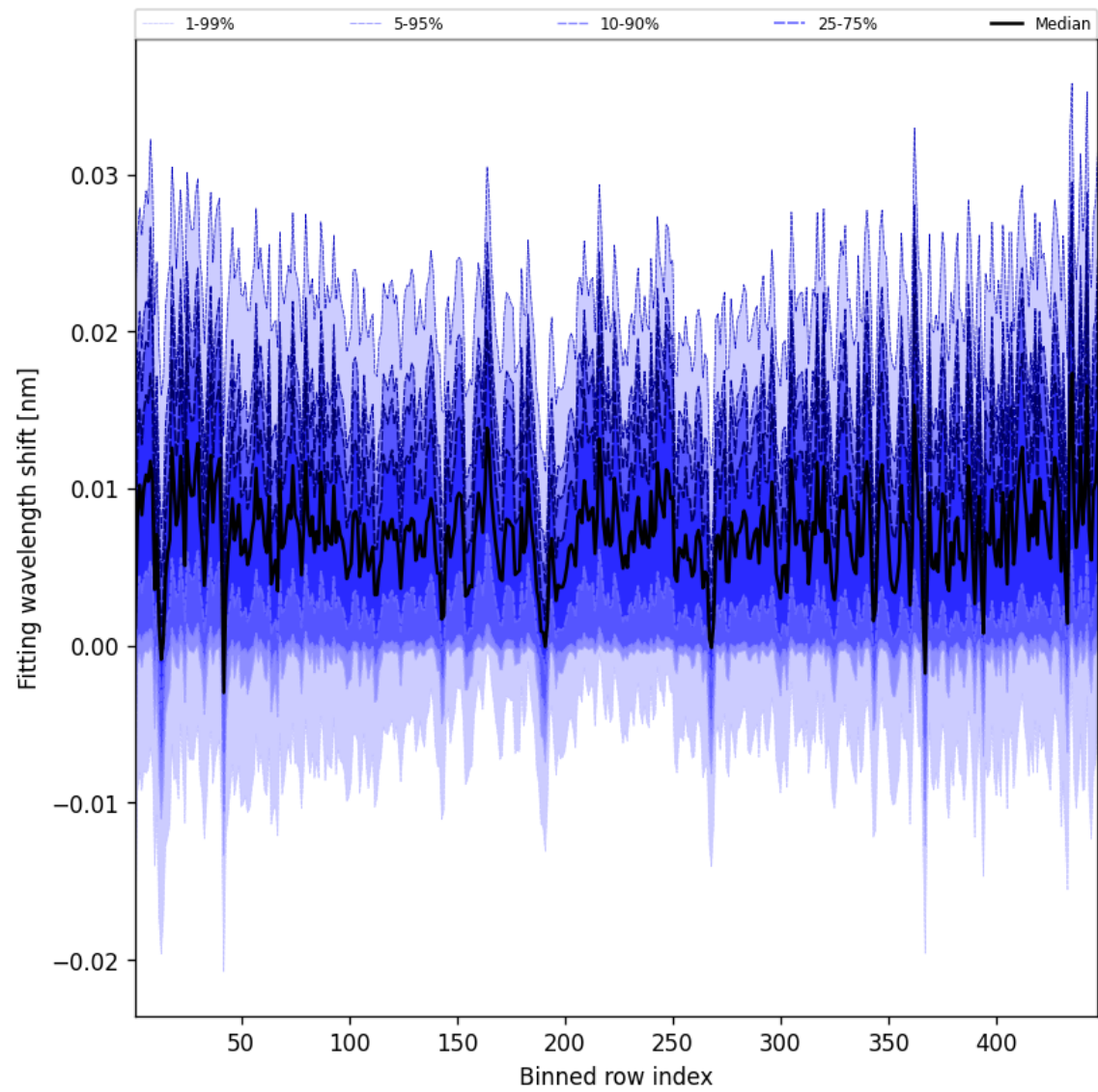
Figure 65: Along track statistics of “Fitting wavelength shift” for 2025-07-08 to 2025-07-09
