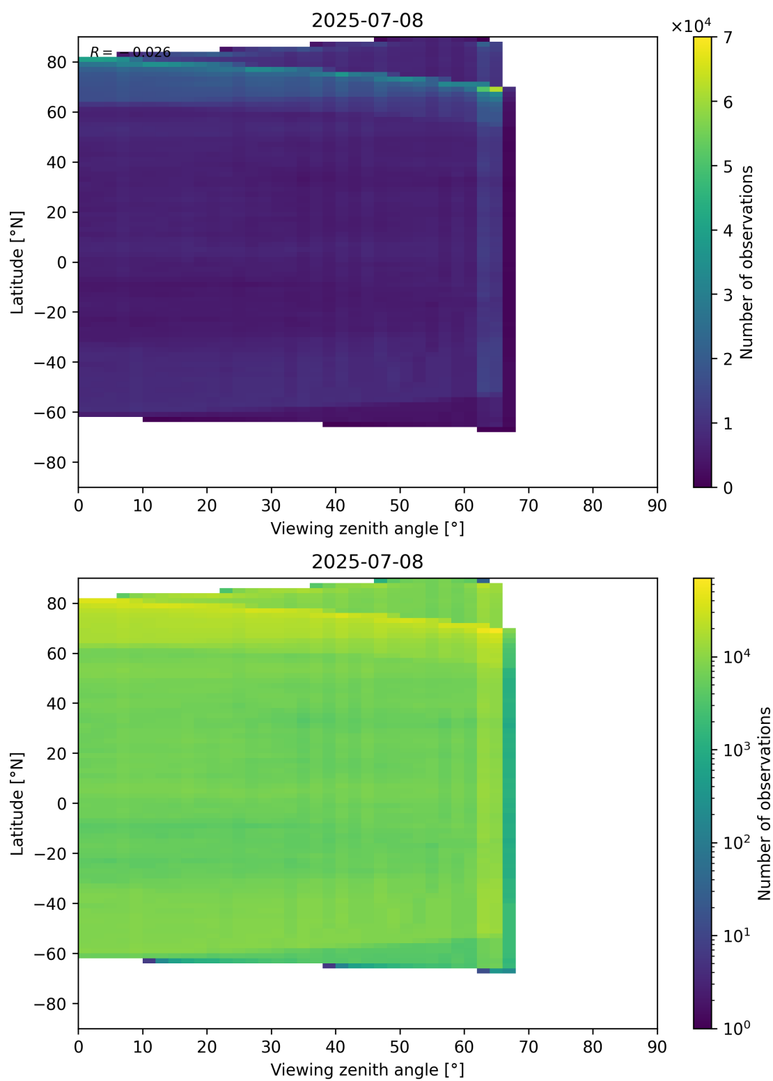
Figure 113: Scatter density plot of “Viewing zenith angle” against “Latitude” for 2025-07-08 to 2025-07-09.
