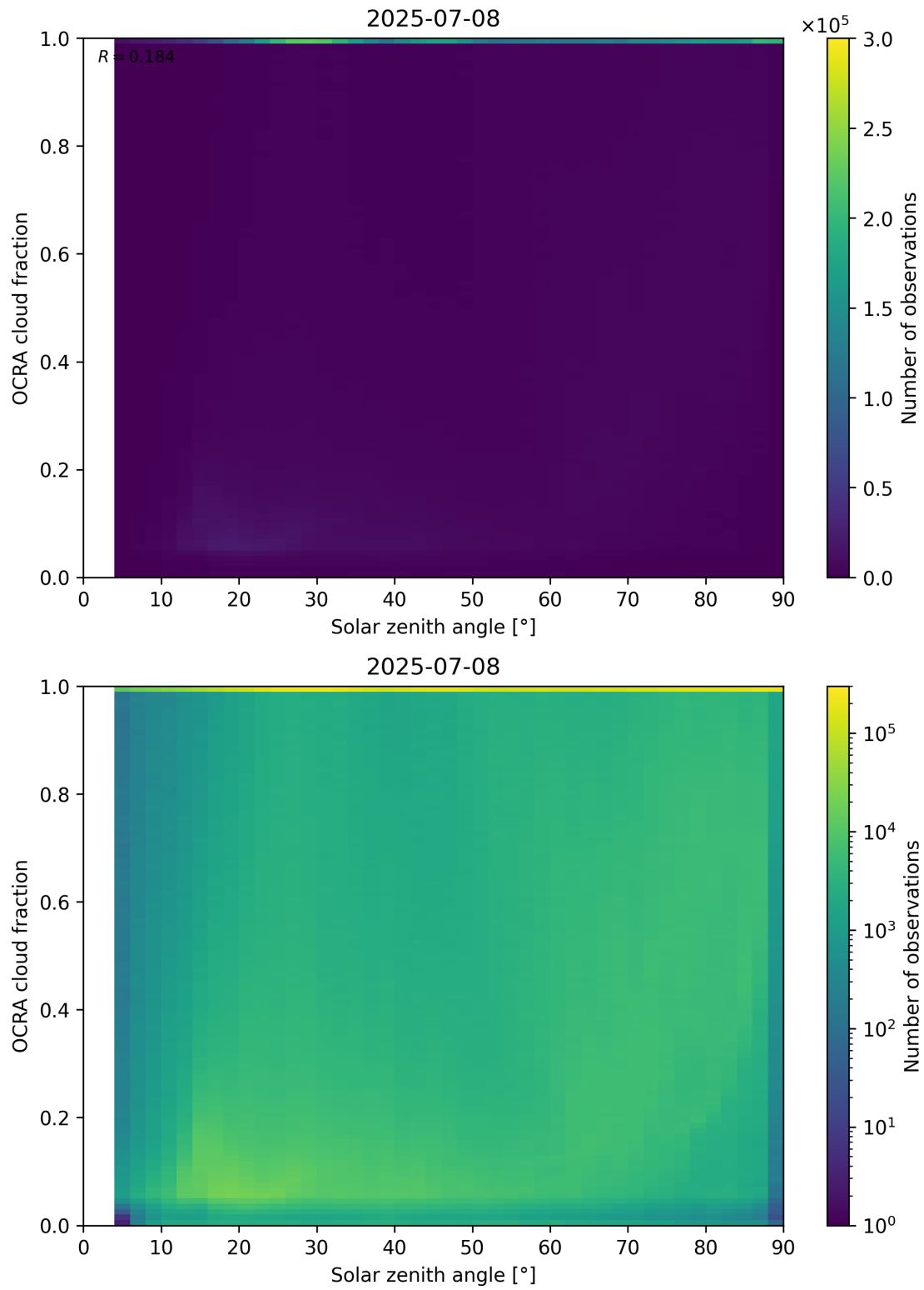
Figure 100: Scatter density plot of “Solar zenith angle” against “OCRA cloud fraction” for 2025-07-08 to 2025-07-09.
