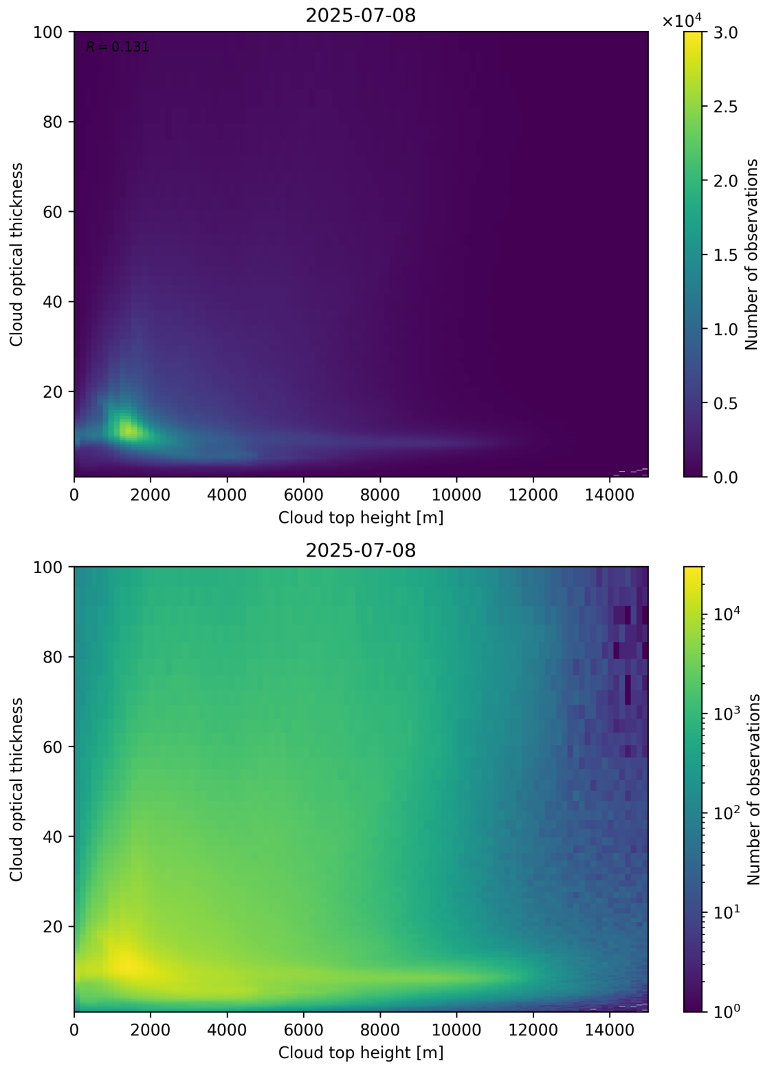
Figure 90: Scatter density plot of “Cloud top height” against “Cloud optical thickness” for 2025-07-08 to 2025-07-09.
