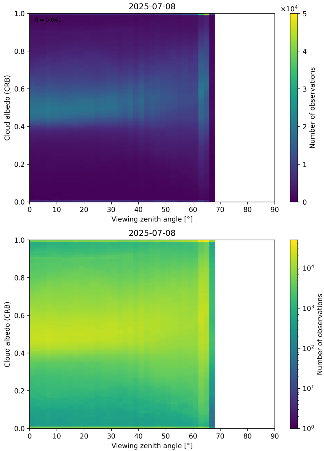
Figure 106: Scatter density plot of “Viewing zenith angle” against “Cloud albedo (CRB)” for 2025-07-08 to 2025-07-09.
