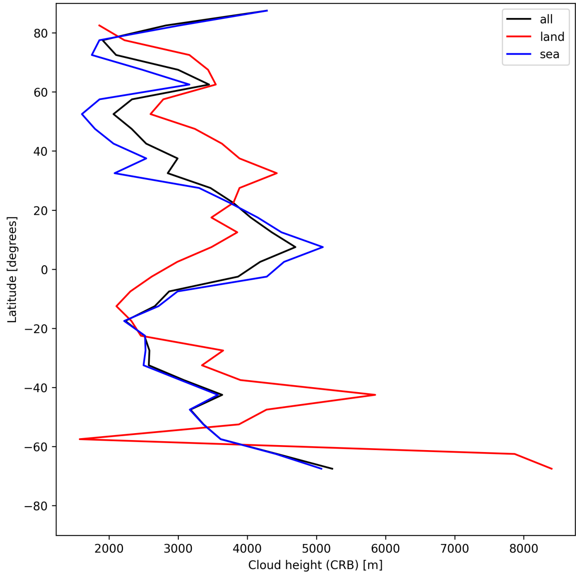
Figure 27: Zonal average of “Cloud height (CRB)” for 2025-07-08 to 2025-07-09.
