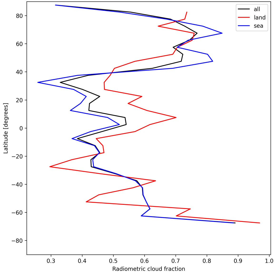
Figure 23: Zonal average of “Radiometric cloud fraction” for 2025-07-08 to 2025-07-09.
