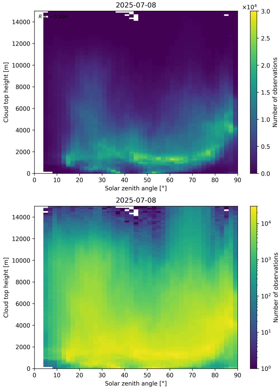
Figure 104: Scatter density plot of “Solar zenith angle” against “Cloud top height” for 2025-07-08 to 2025-07-09.
