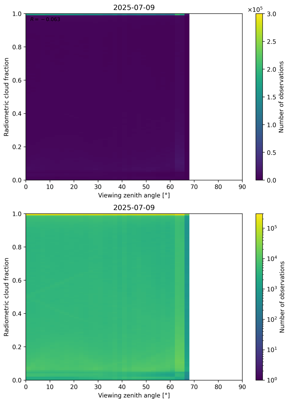
Figure 107: Scatter density plot of “Viewing zenith angle” against “Radiometric cloud fraction” for 2025-07-08 to 2025-07-10.
