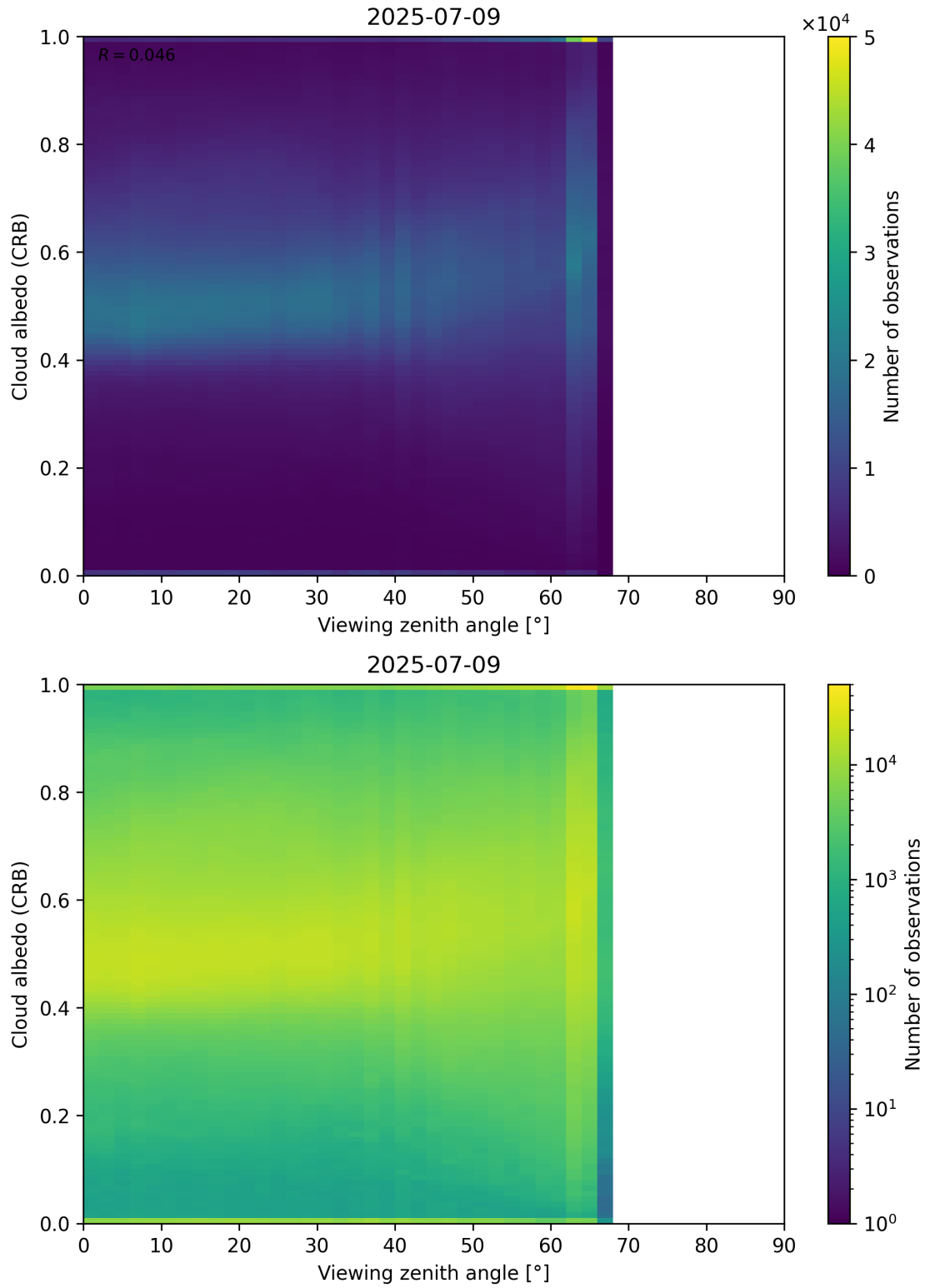
Figure 106: Scatter density plot of “Viewing zenith angle” against “Cloud albedo (CRB)” for 2025-07-08 to 2025-07-10.
