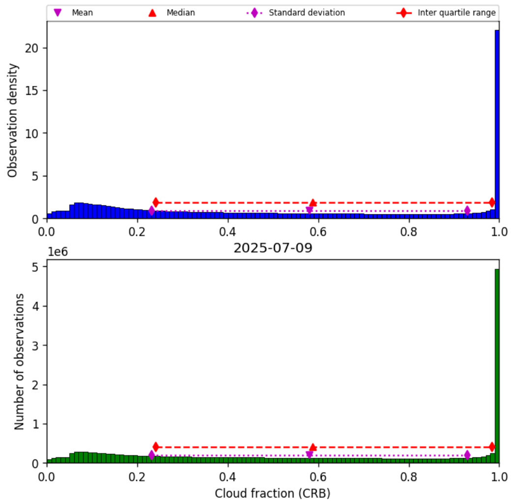
Figure 42: Histogram of “Cloud fraction (CRB)” for 2025-07-08 to 2025-07-10
