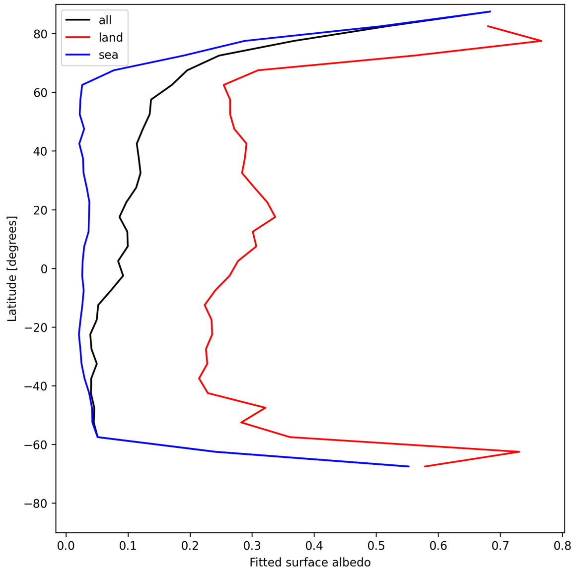
Figure 29: Zonal average of “Fitted surface albedo” for 2025-07-08 to 2025-07-10.
