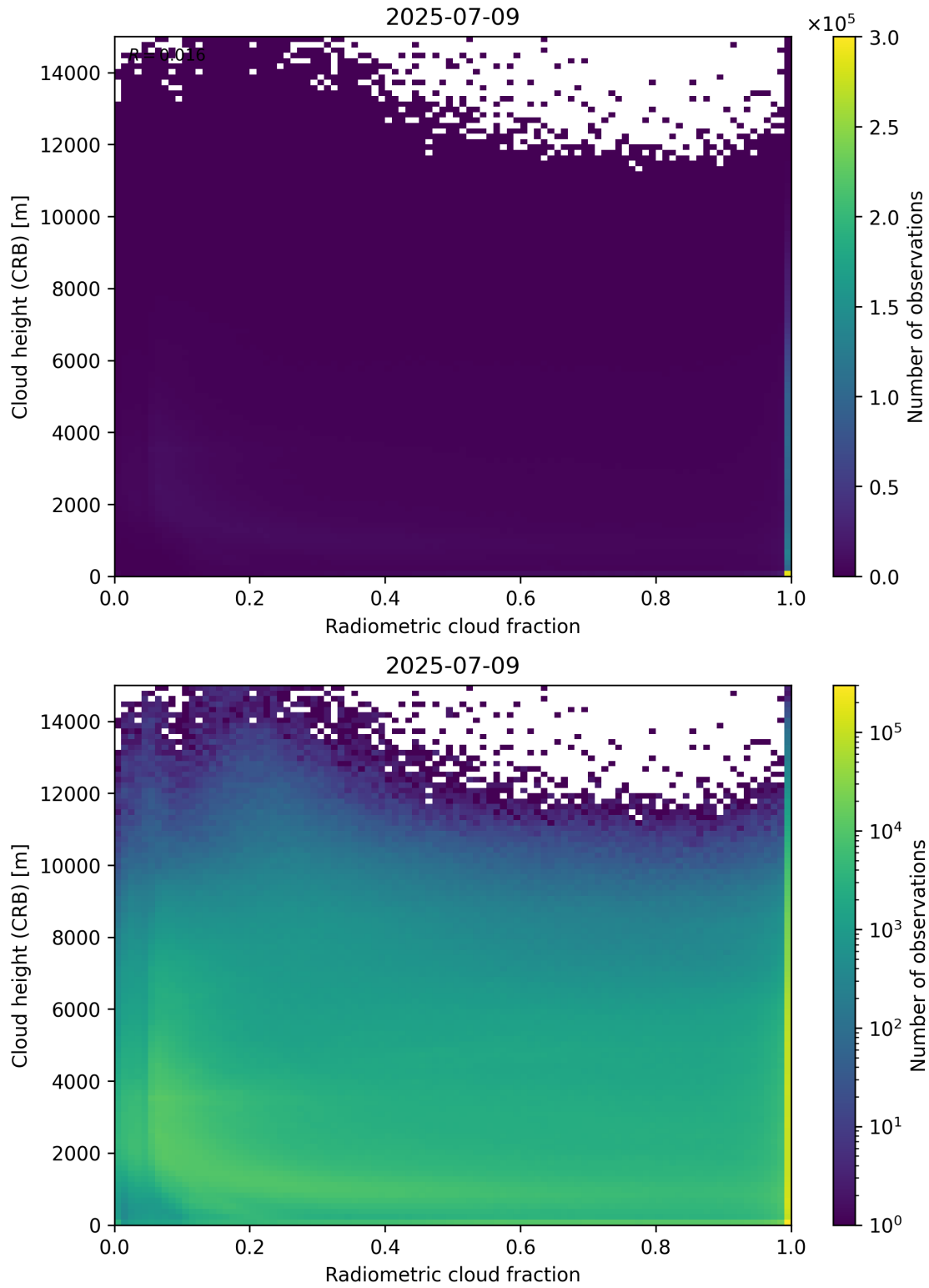
Figure 74: Scatter density plot of “Radiometric cloud fraction” against “Cloud height (CRB)” for 2025-07-08 to 2025-07-10.
