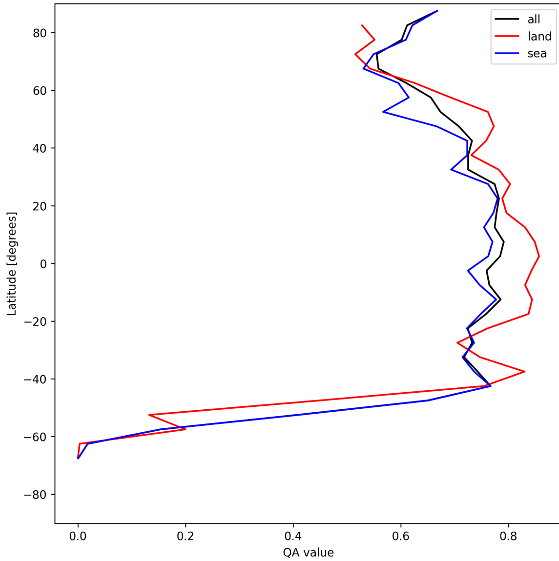
Figure 22: Zonal average of “QA value” for 2025-07-08 to 2025-07-10.
