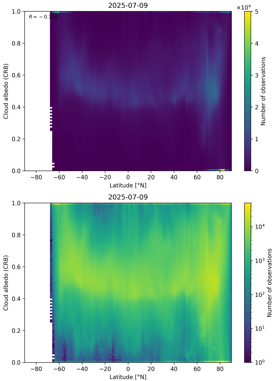
Figure 91: Scatter density plot of “Latitude” against “Cloud albedo (CRB)” for 2025-07-08 to 2025-07-10.
