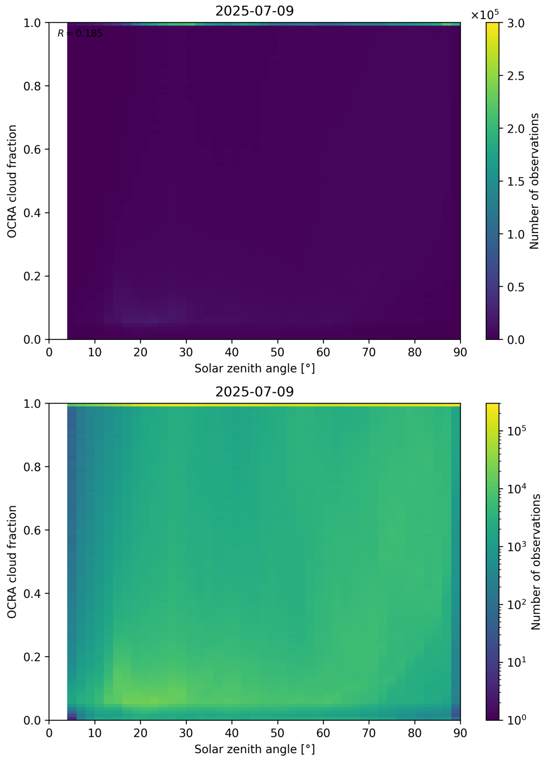
Figure 100: Scatter density plot of “Solar zenith angle” against “OCRA cloud fraction” for 2025-07-08 to 2025-07-10.
