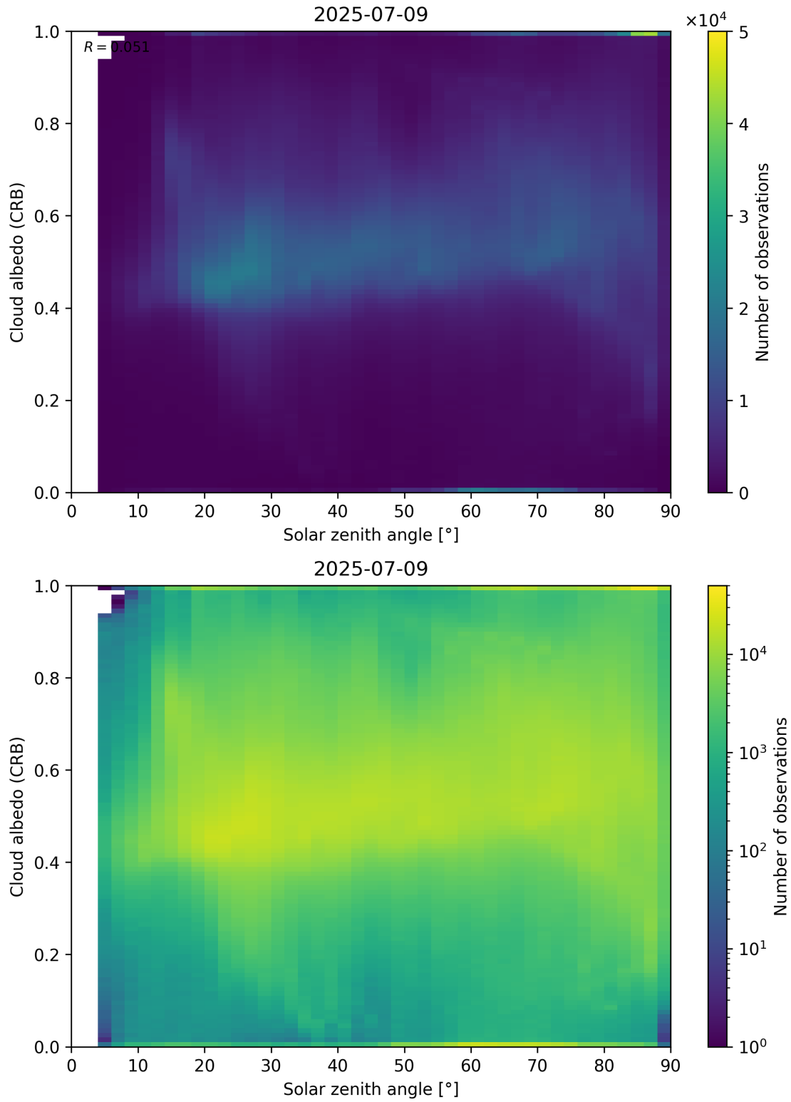
Figure 98: Scatter density plot of “Solar zenith angle” against “Cloud albedo (CRB)” for 2025-07-08 to 2025-07-10.
