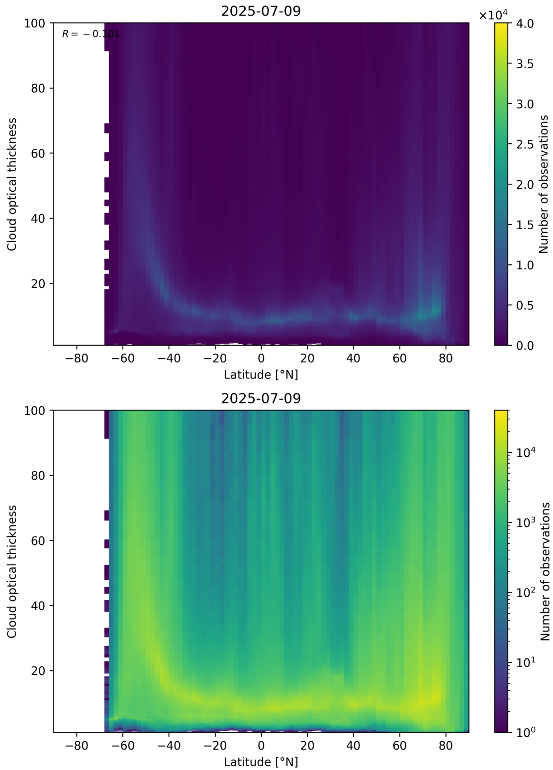
Figure 96: Scatter density plot of “Latitude” against “Cloud optical thickness” for 2025-07-08 to 2025-07-10.
