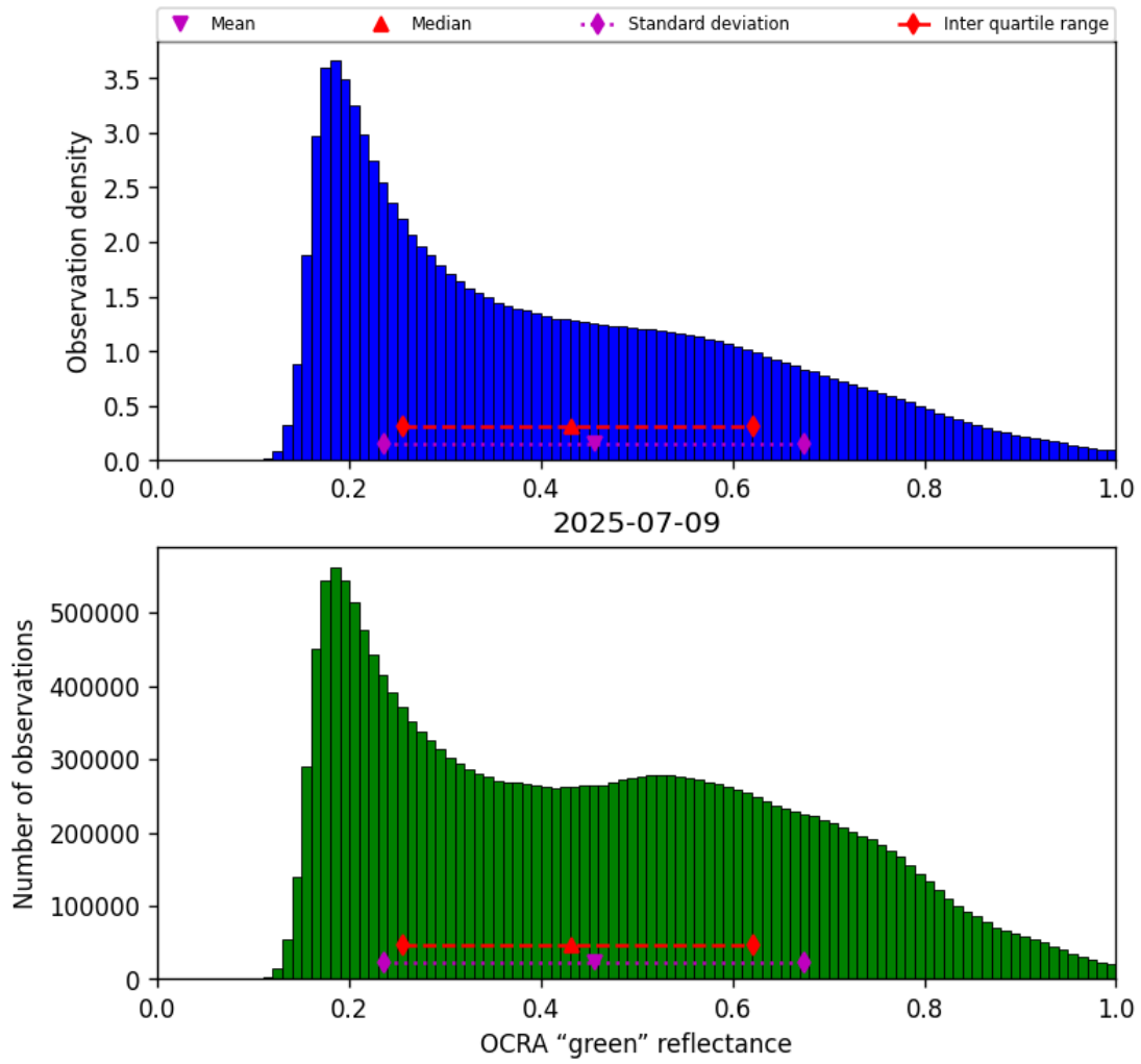
Figure 52: Histogram of “OCRA “green” reflectance” for 2025-07-08 to 2025-07-10
