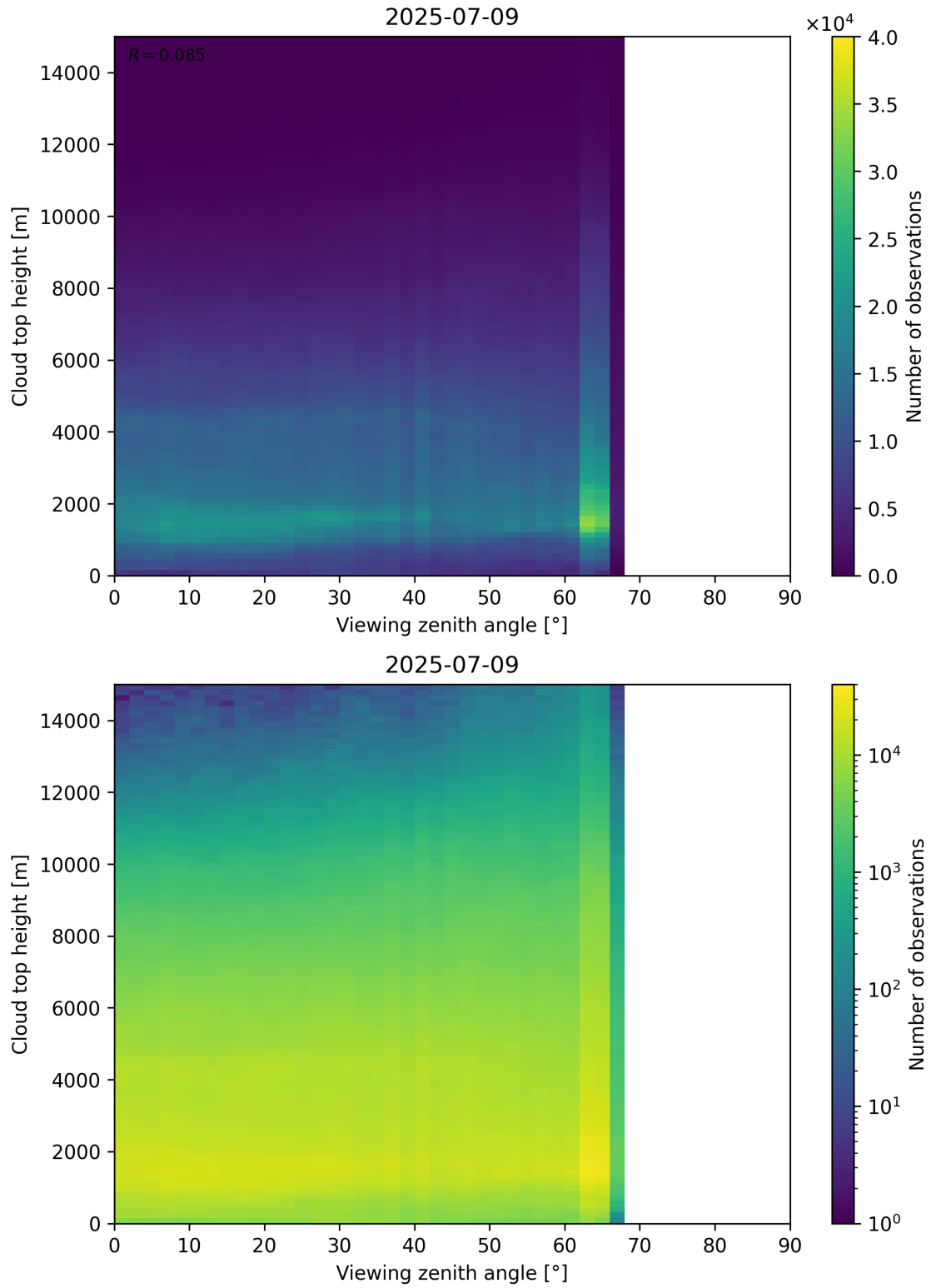
Figure 112: Scatter density plot of “Viewing zenith angle” against “Cloud top height” for 2025-07-08 to 2025-07-10.
