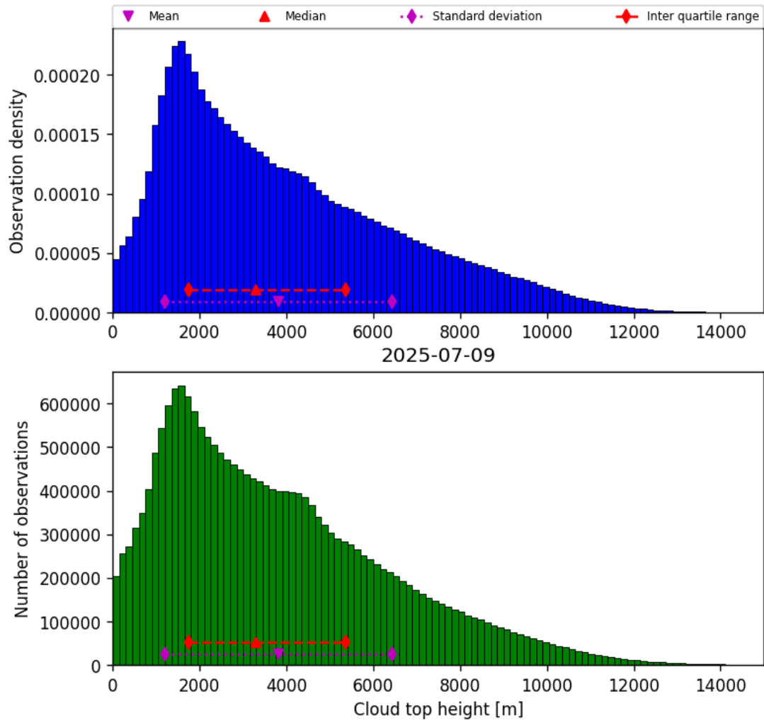
Figure 40: Histogram of “Cloud top height” for 2025-07-08 to 2025-07-10
