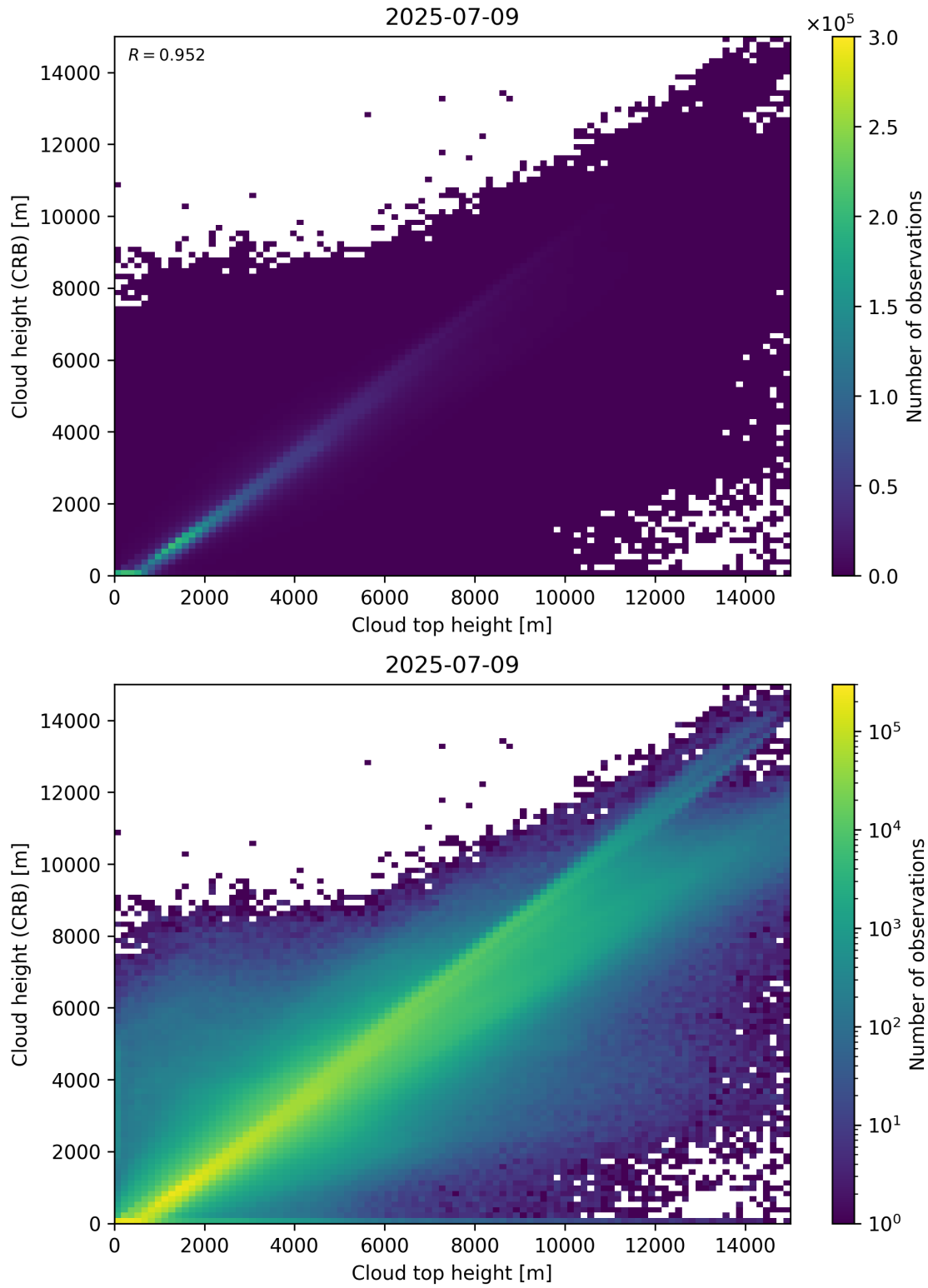
Figure 89: Scatter density plot of “Cloud top height” against “Cloud height (CRB)” for 2025-07-08 to 2025-07-10.
