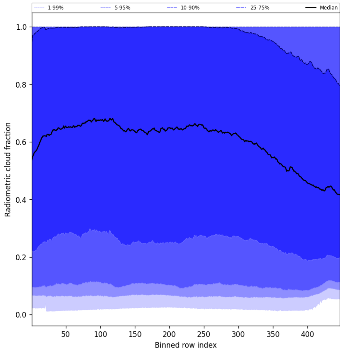
Figure 55: Along track statistics of “Radiometric cloud fraction” for 2025-07-08 to 2025-07-10
