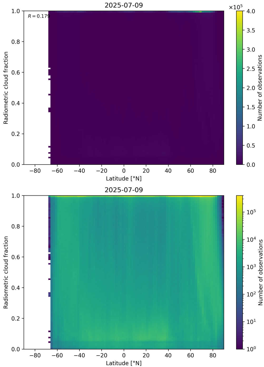
Figure 92: Scatter density plot of “Latitude” against “Radiometric cloud fraction” for 2025-07-08 to 2025-07-10.
