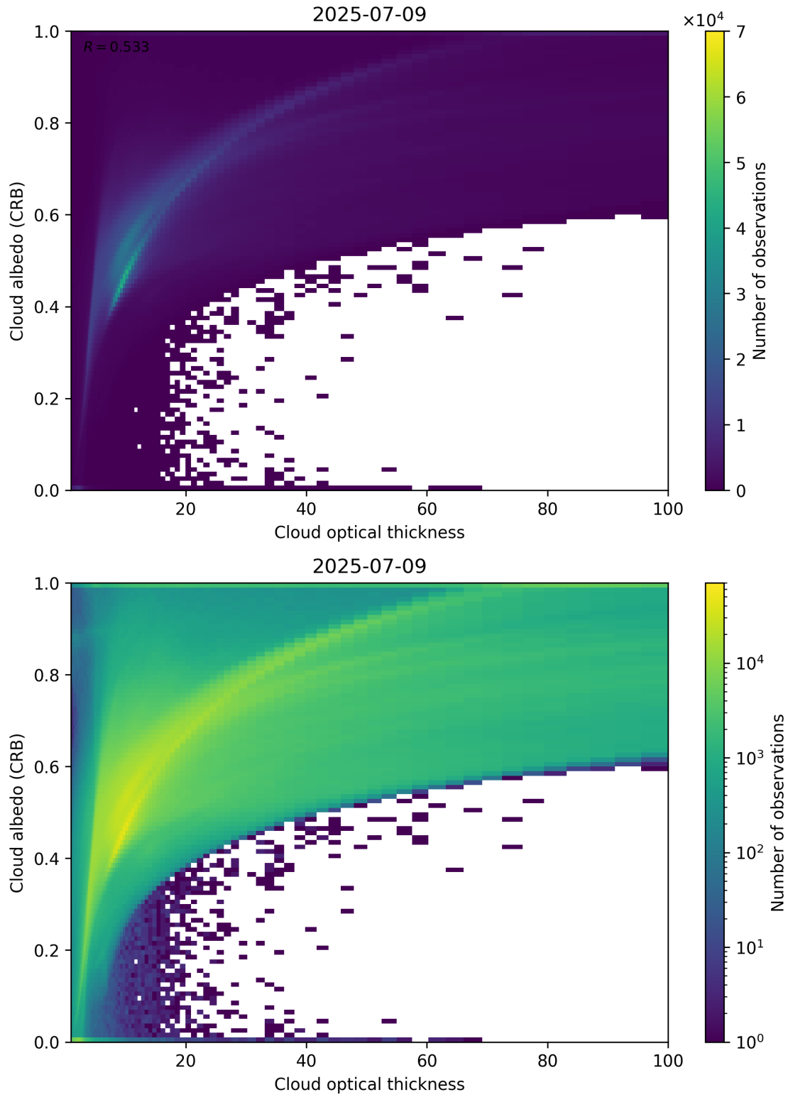
Figure 82: Scatter density plot of “Cloud optical thickness” against “Cloud albedo (CRB)” for 2025-07-08 to 2025-07-10.
