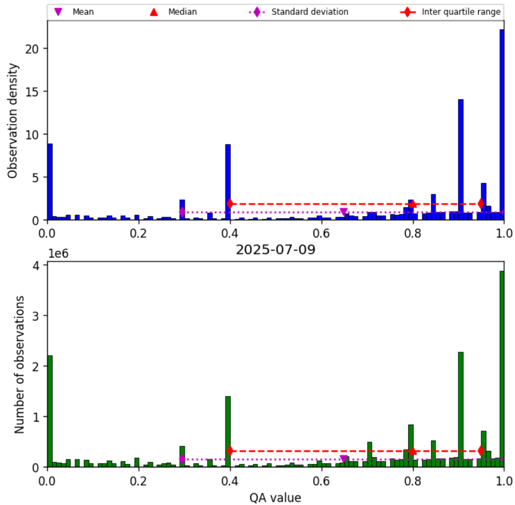
Figure 38: Histogram of “QA value” for 2025-07-08 to 2025-07-10
