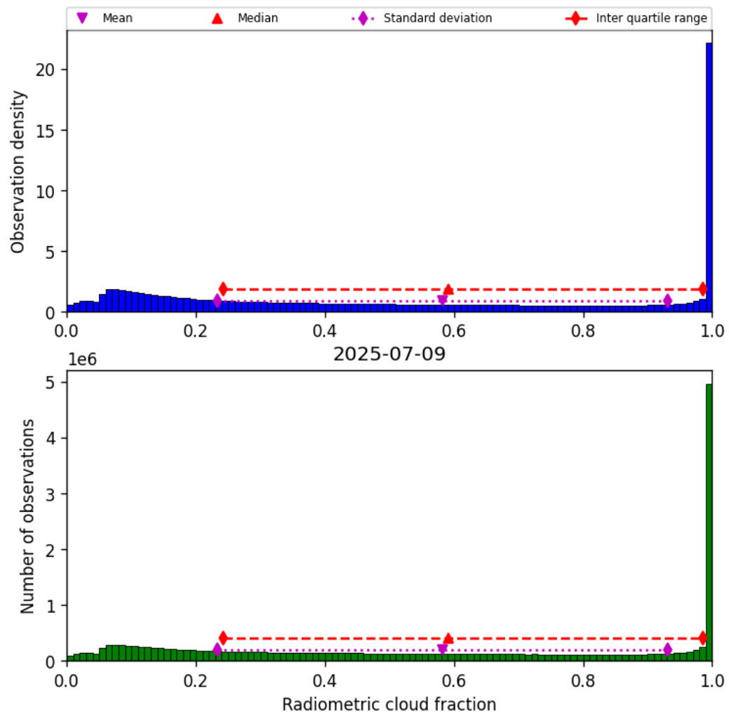
Figure 39: Histogram of “Radiometric cloud fraction” for 2025-07-08 to 2025-07-10
