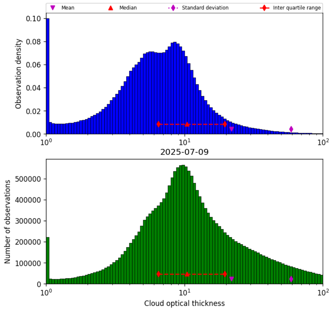
Figure 41: Histogram of “Cloud optical thickness” for 2025-07-08 to 2025-07-10
