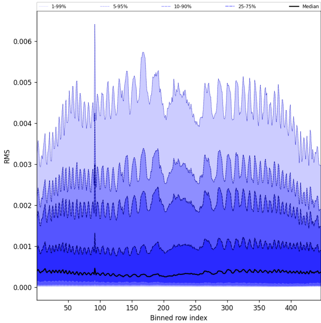
Figure 63: Along track statistics of “RMS” for 2025-07-08 to 2025-07-10
