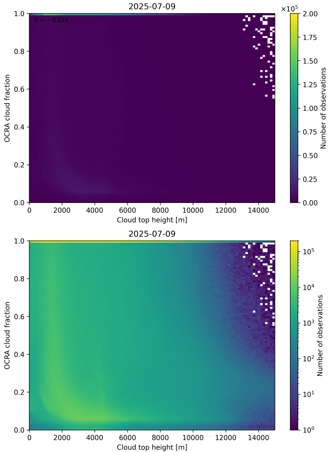
Figure 87: Scatter density plot of “Cloud top height” against “OCRA cloud fraction” for 2025-07-08 to 2025-07-10.
