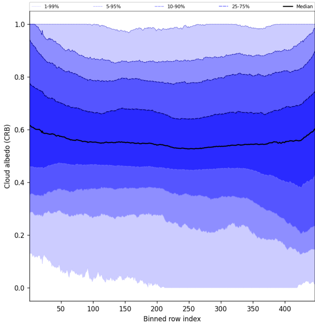
Figure 60: Along track statistics of “Cloud albedo (CRB)” for 2025-07-08 to 2025-07-10
