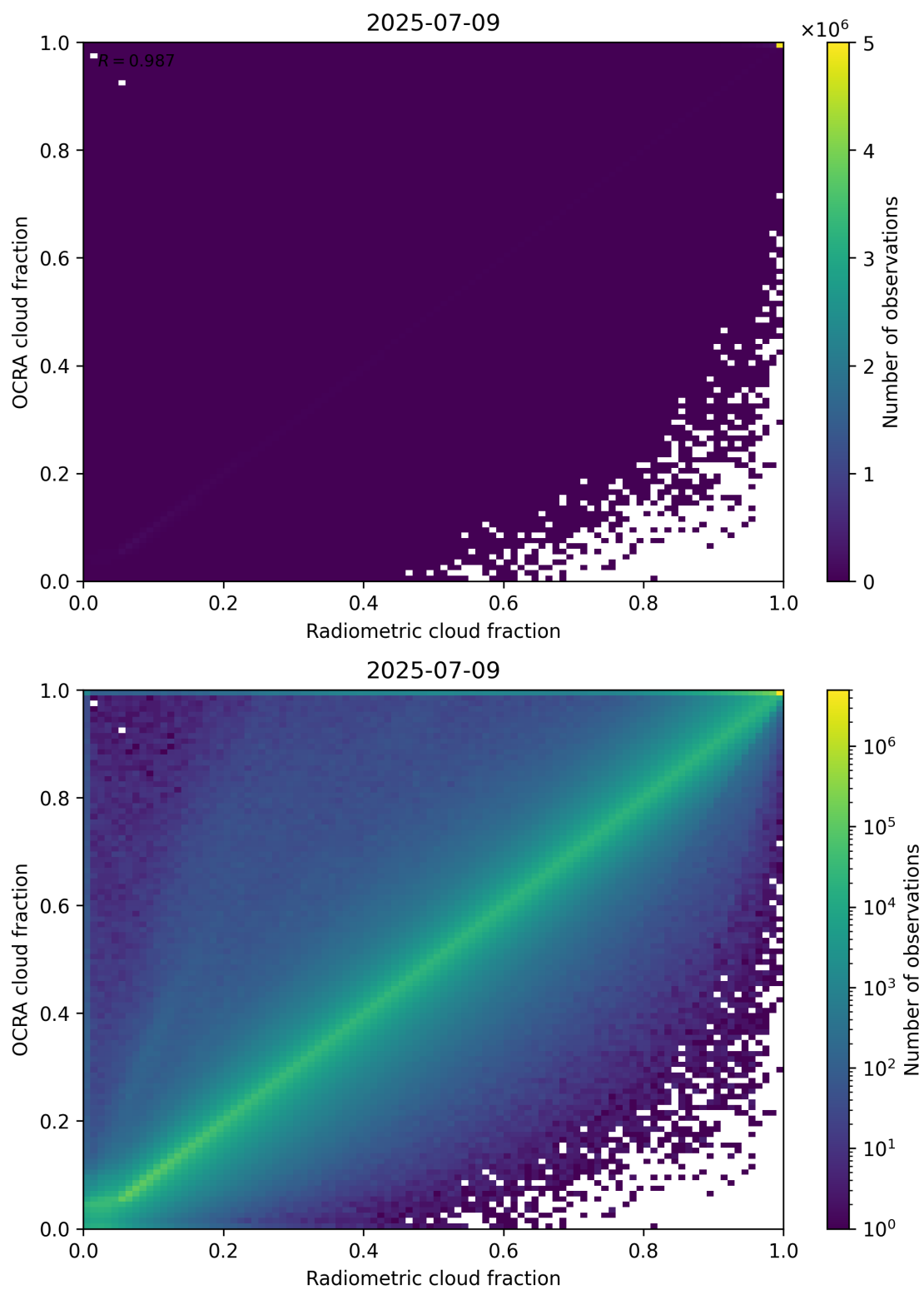
Figure 72: Scatter density plot of “Radiometric cloud fraction” against “OCRA cloud fraction” for 2025-07-08 to 2025-07-10.
