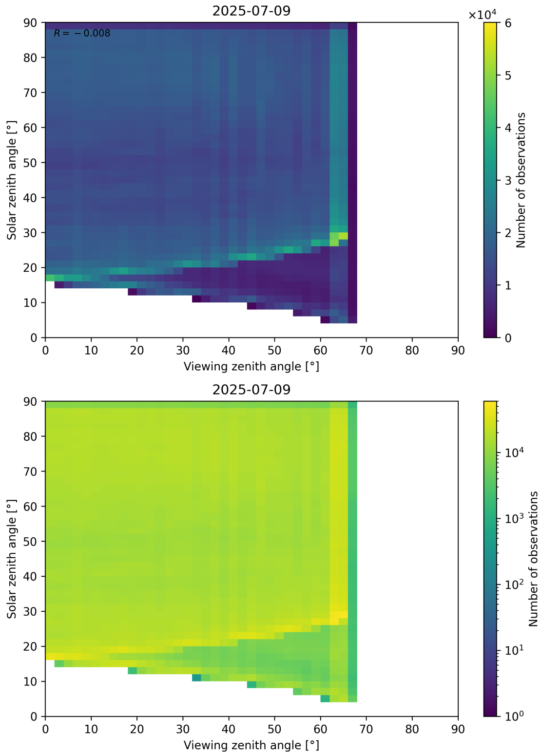
Figure 114: Scatter density plot of “Viewing zenith angle” against “Solar zenith angle” for 2025-07-08 to 2025-07-10.
