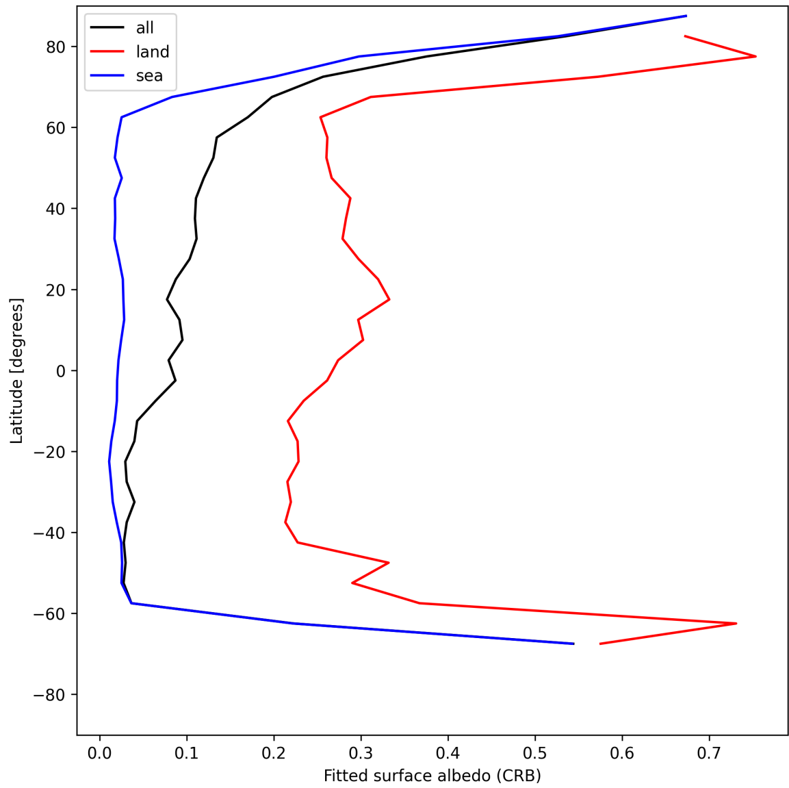
Figure 30: Zonal average of “Fitted surface albedo (CRB)” for 2025-07-08 to 2025-07-10.
