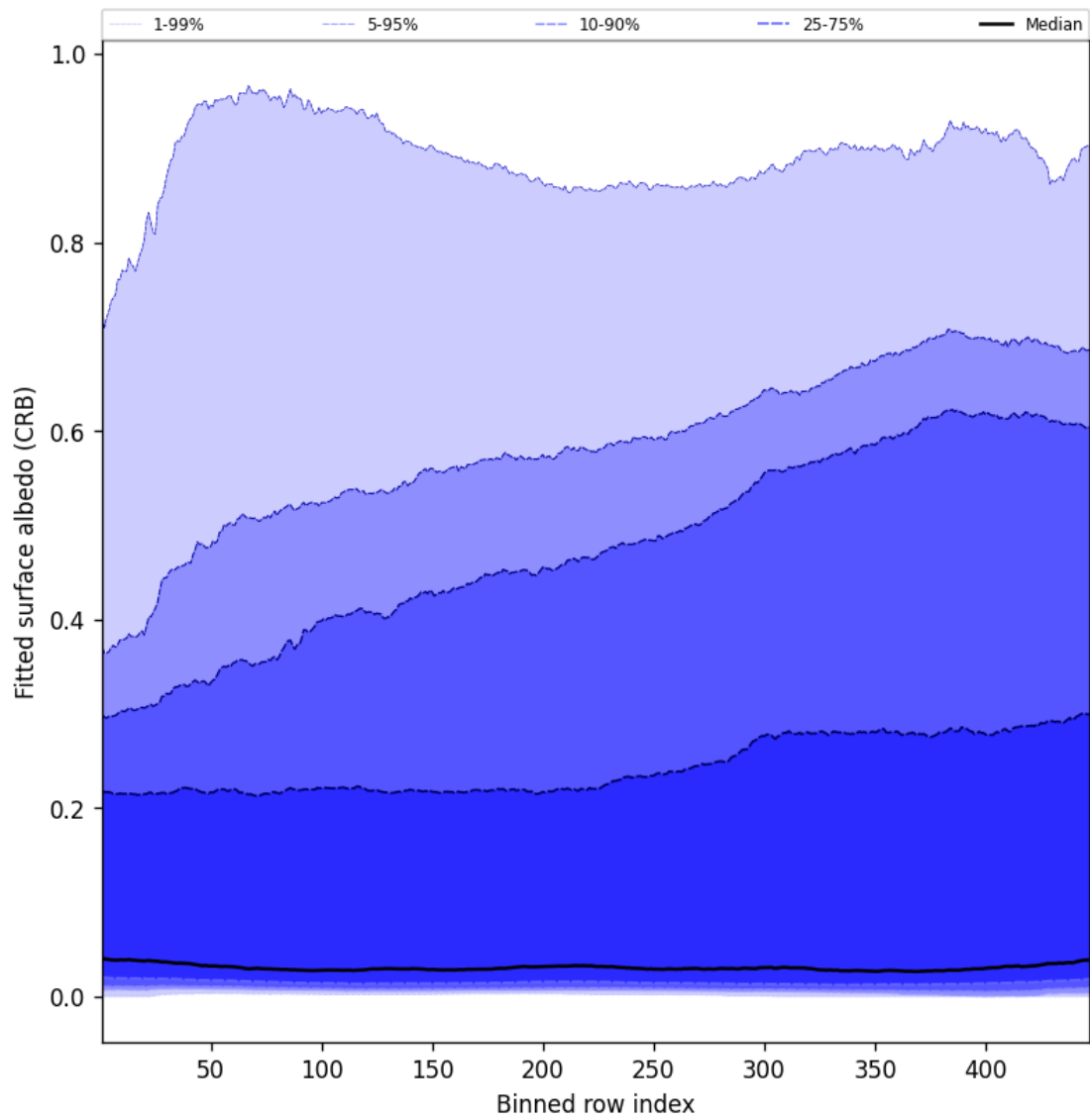
Figure 62: Along track statistics of “Fitted surface albedo (CRB)” for 2025-07-08 to 2025-07-10
