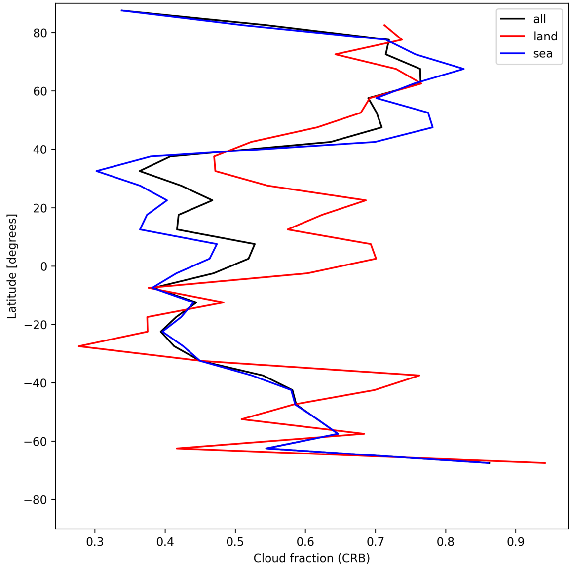
Figure 26: Zonal average of “Cloud fraction (CRB)” for 2025-07-08 to 2025-07-10.
