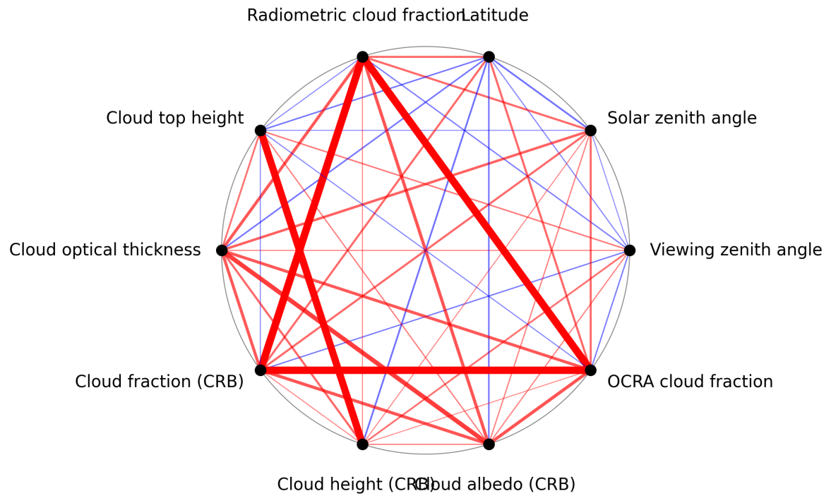
Figure 1: Map of correlation graph for 2025-07-08 to 2025-07-10.
