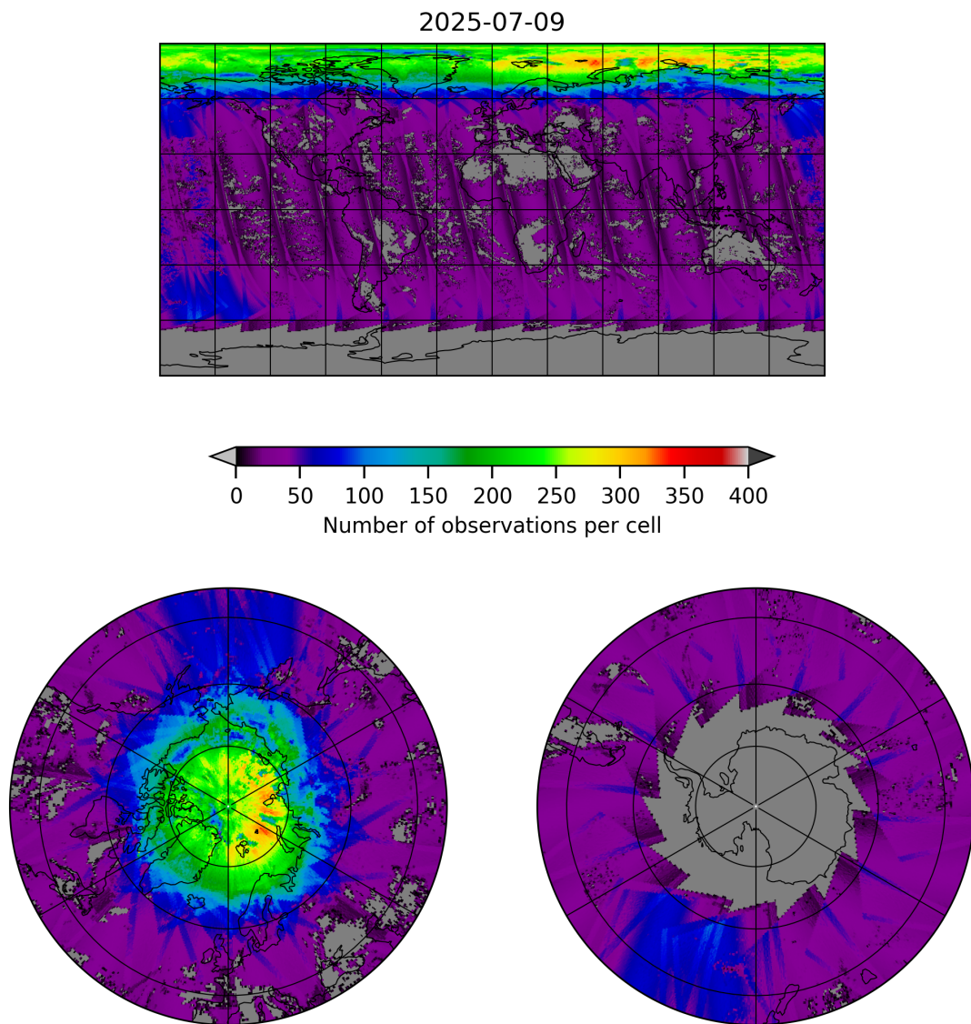
Figure 21: Map of the number of observations for 2025-07-08 to 2025-07-10
