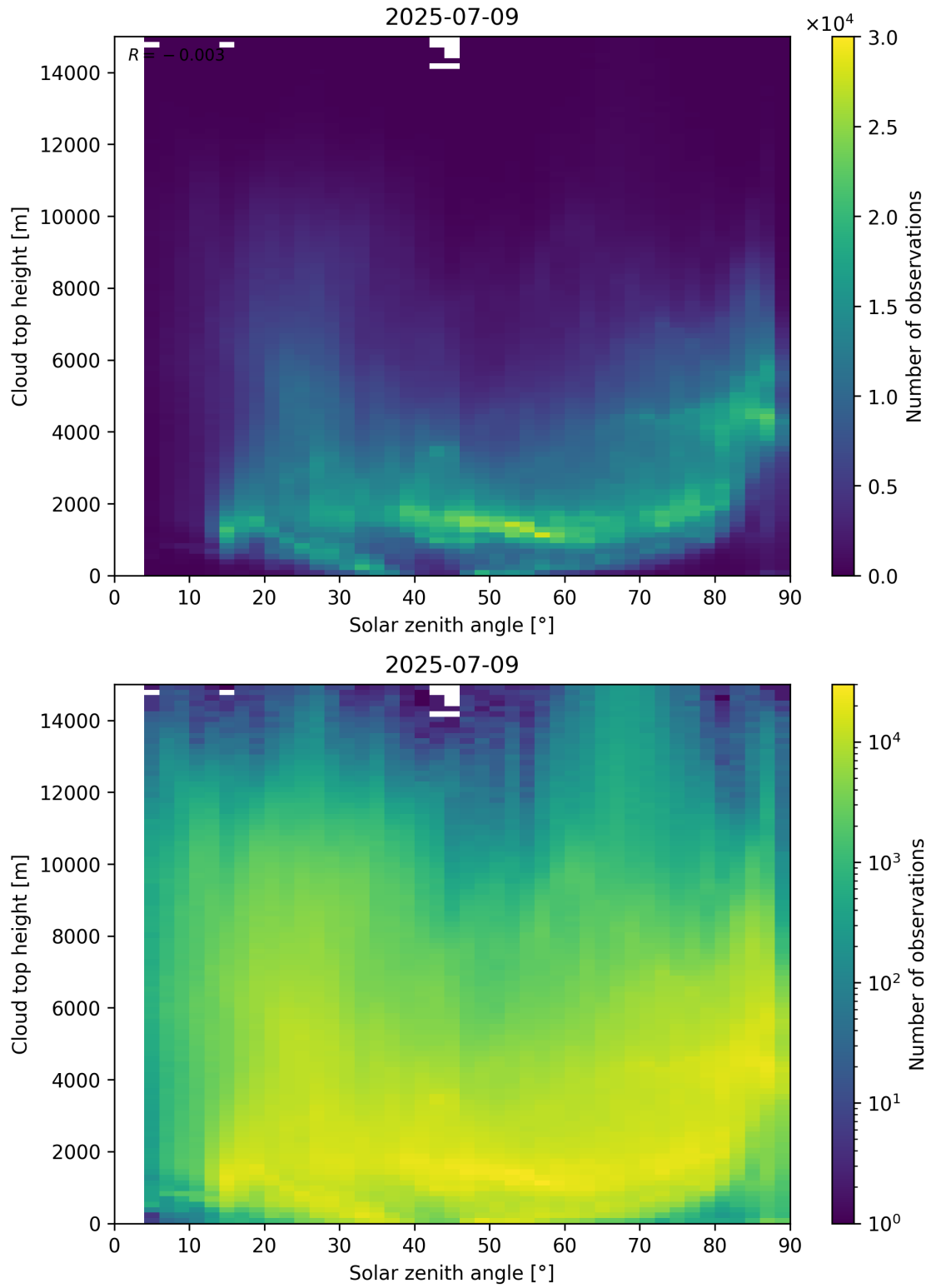
Figure 104: Scatter density plot of “Solar zenith angle” against “Cloud top height” for 2025-07-08 to 2025-07-10.
