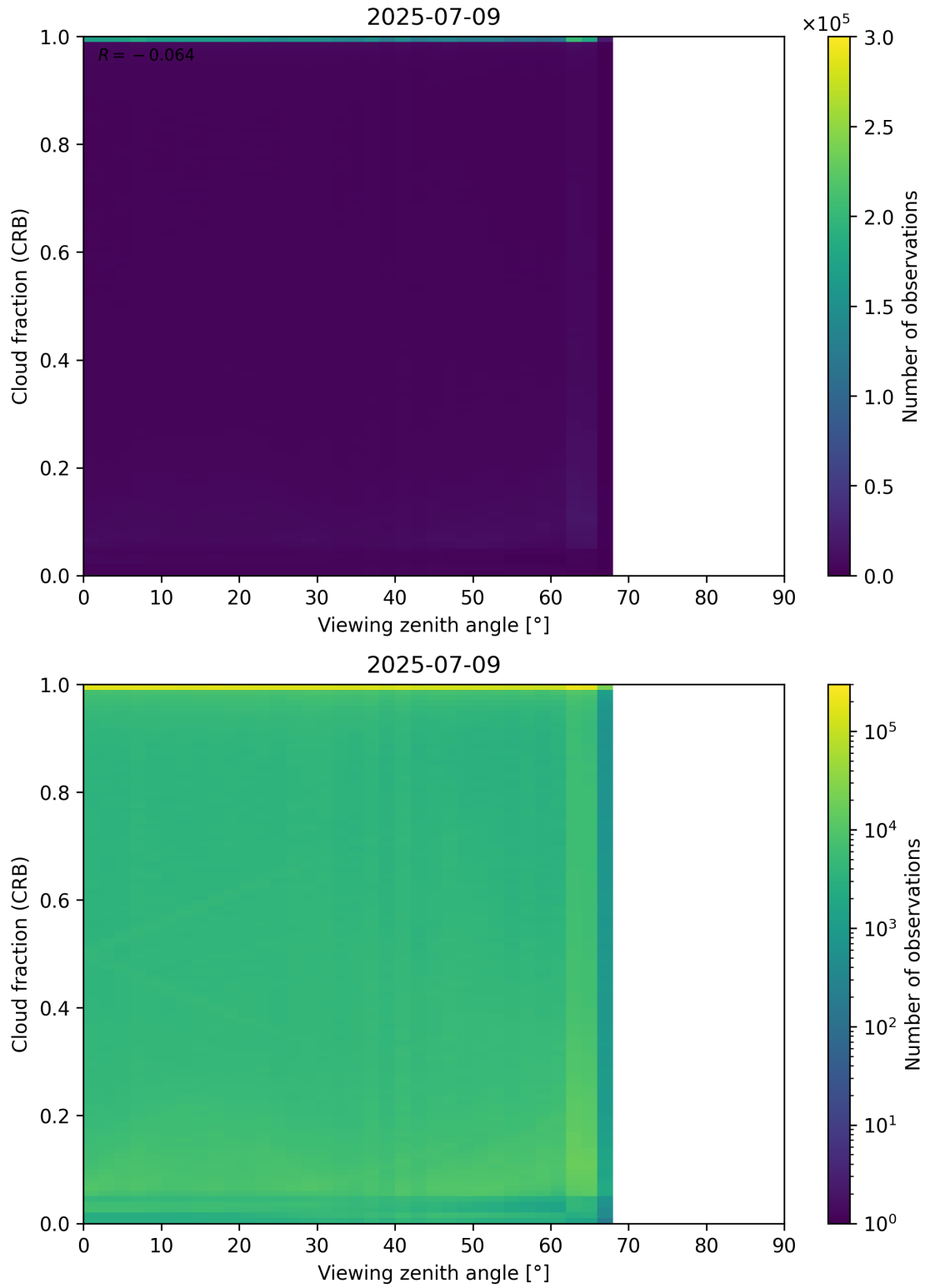
Figure 109: Scatter density plot of “Viewing zenith angle” against “Cloud fraction (CRB)” for 2025-07-08 to 2025-07-10.
