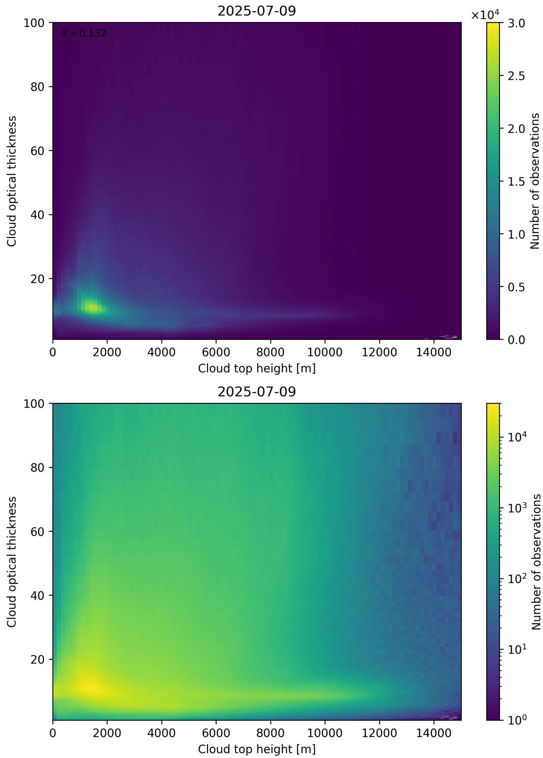
Figure 90: Scatter density plot of “Cloud top height” against “Cloud optical thickness” for 2025-07-08 to 2025-07-10.
