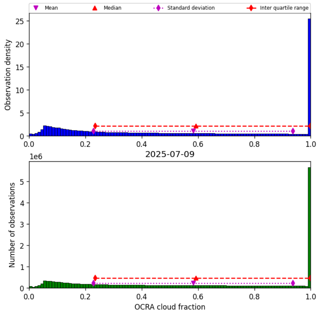
Figure 50: Histogram of “OCRA cloud fraction” for 2025-07-08 to 2025-07-10
