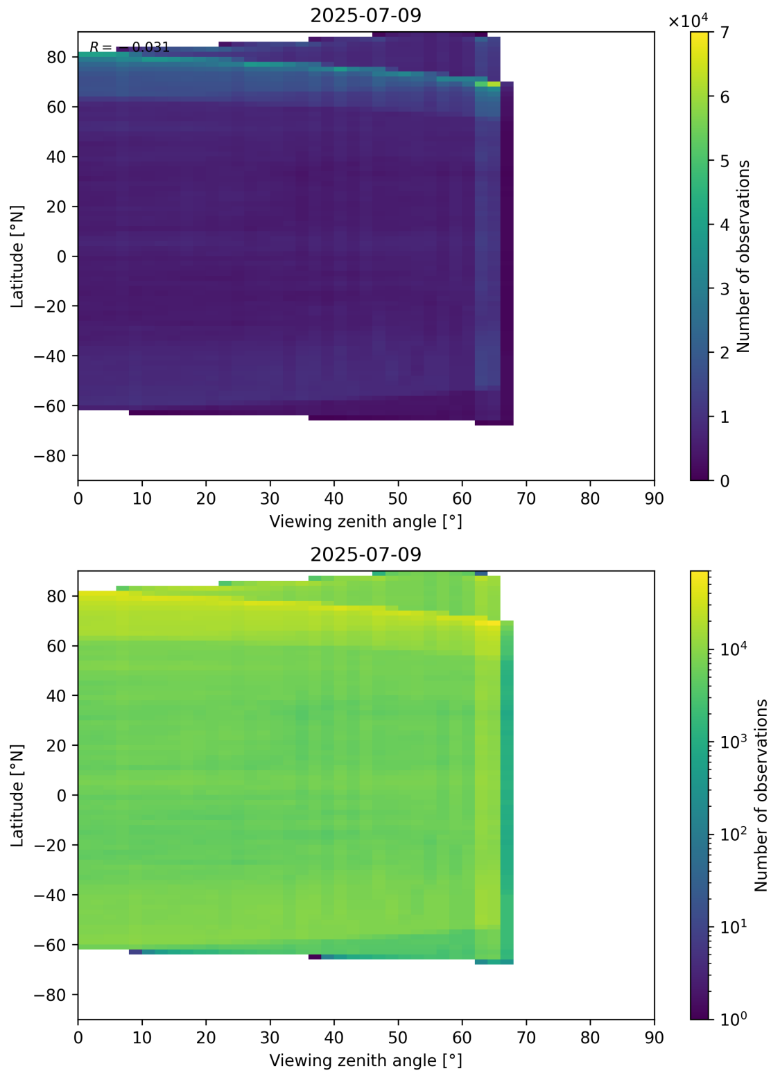
Figure 113: Scatter density plot of “Viewing zenith angle” against “Latitude” for 2025-07-08 to 2025-07-10.
