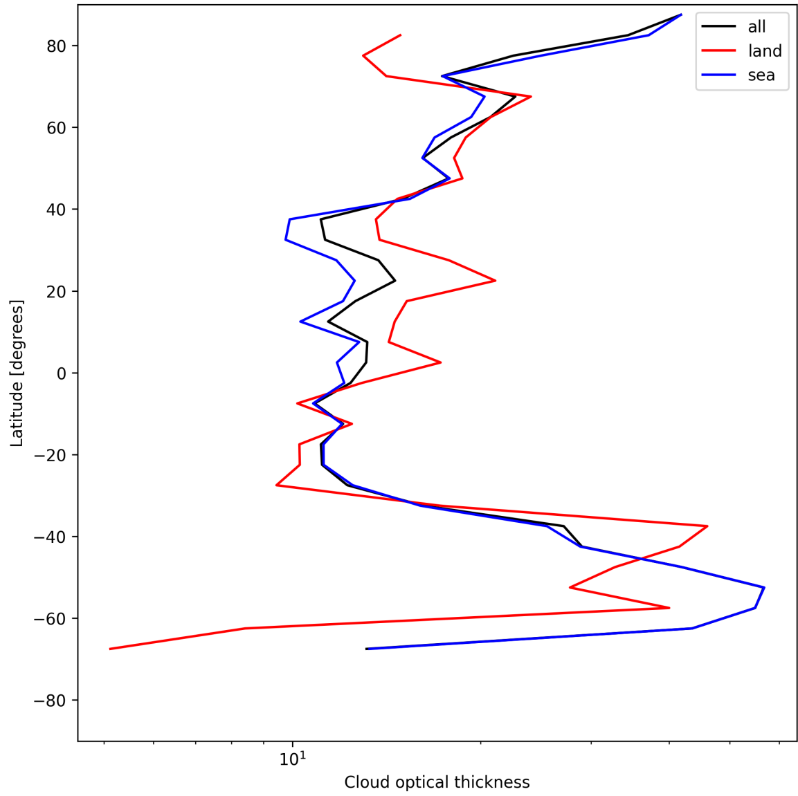
Figure 25: Zonal average of “Cloud optical thickness” for 2025-07-08 to 2025-07-10.
