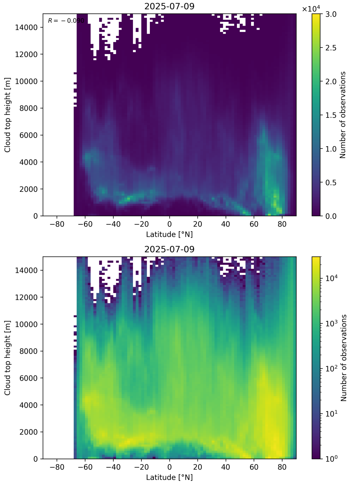
Figure 97: Scatter density plot of “Latitude” against “Cloud top height” for 2025-07-08 to 2025-07-10.
