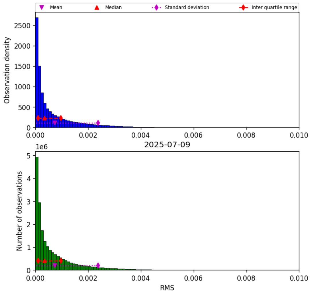
Figure 47: Histogram of “RMS” for 2025-07-08 to 2025-07-10
