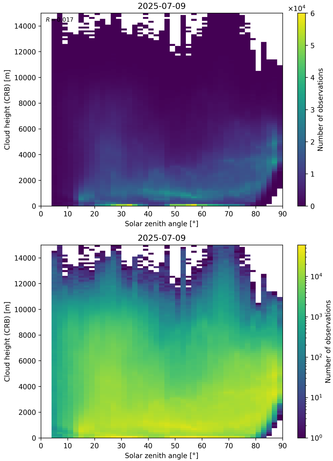
Figure 102: Scatter density plot of “Solar zenith angle” against “Cloud height (CRB)” for 2025-07-08 to 2025-07-10.
