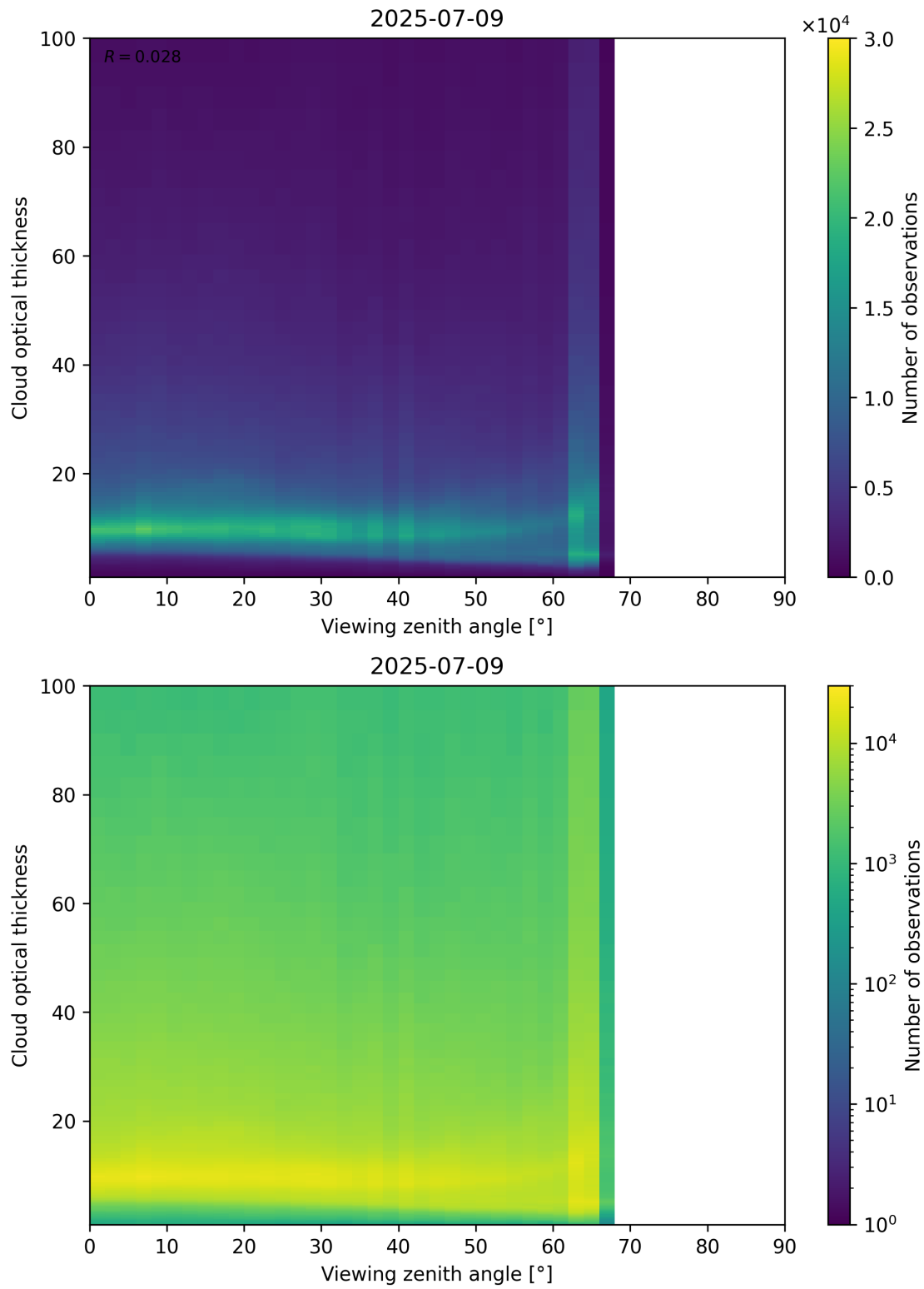
Figure 111: Scatter density plot of “Viewing zenith angle” against “Cloud optical thickness” for 2025-07-08 to 2025-07-10.
