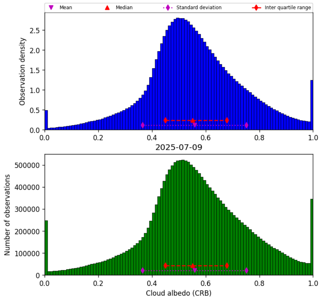
Figure 44: Histogram of “Cloud albedo (CRB)” for 2025-07-08 to 2025-07-10
