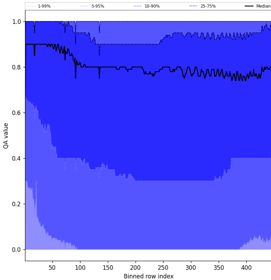
Figure 54: Along track statistics of “QA value” for 2025-07-08 to 2025-07-10
