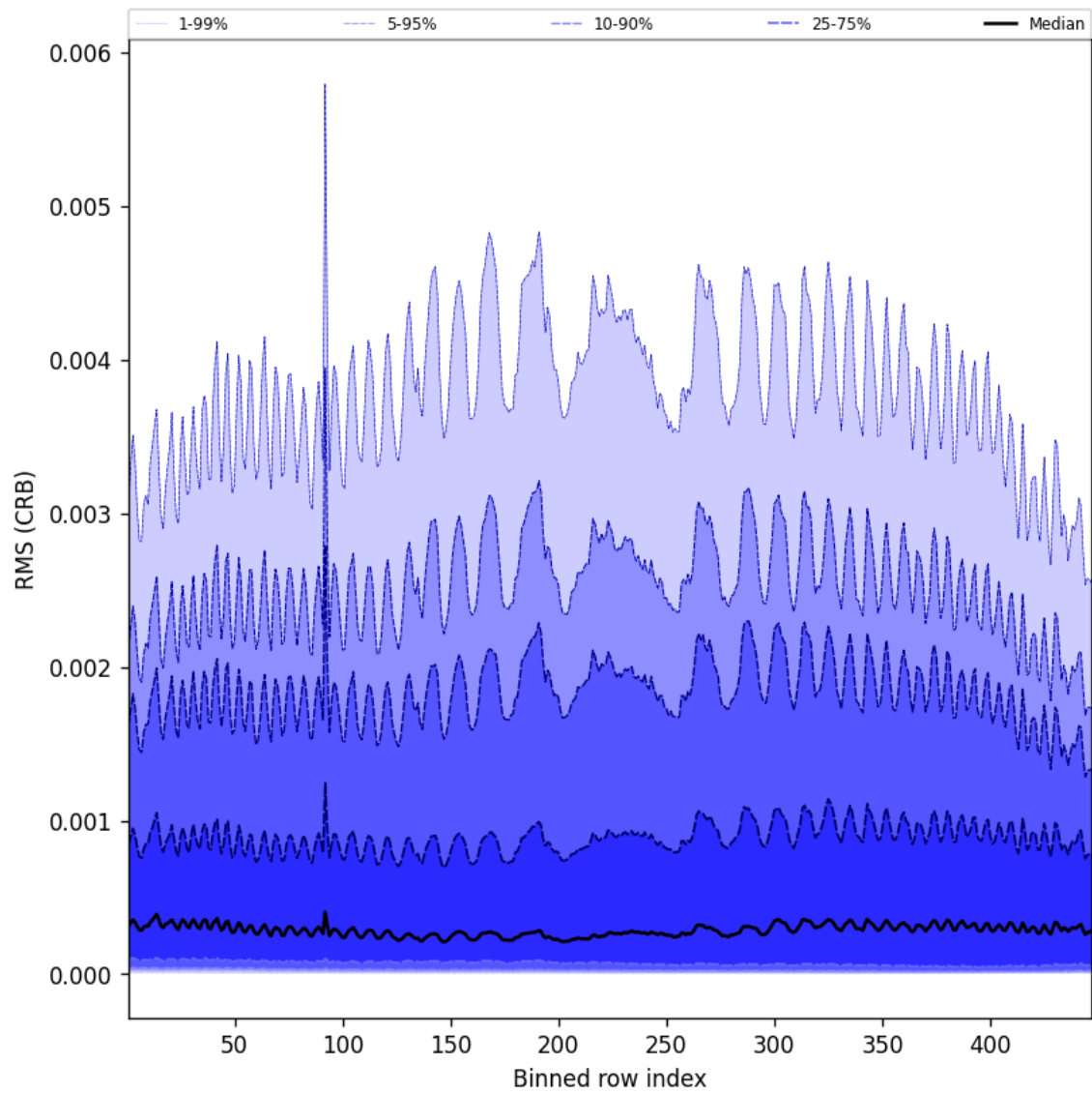
Figure 64: Along track statistics of “RMS (CRB)” for 2025-07-08 to 2025-07-10
