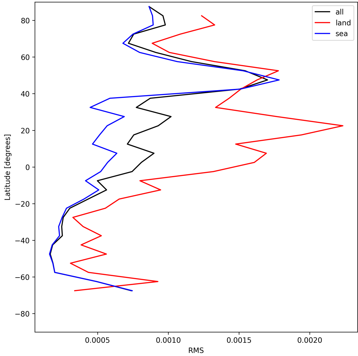
Figure 31: Zonal average of “RMS” for 2025-07-08 to 2025-07-10.
