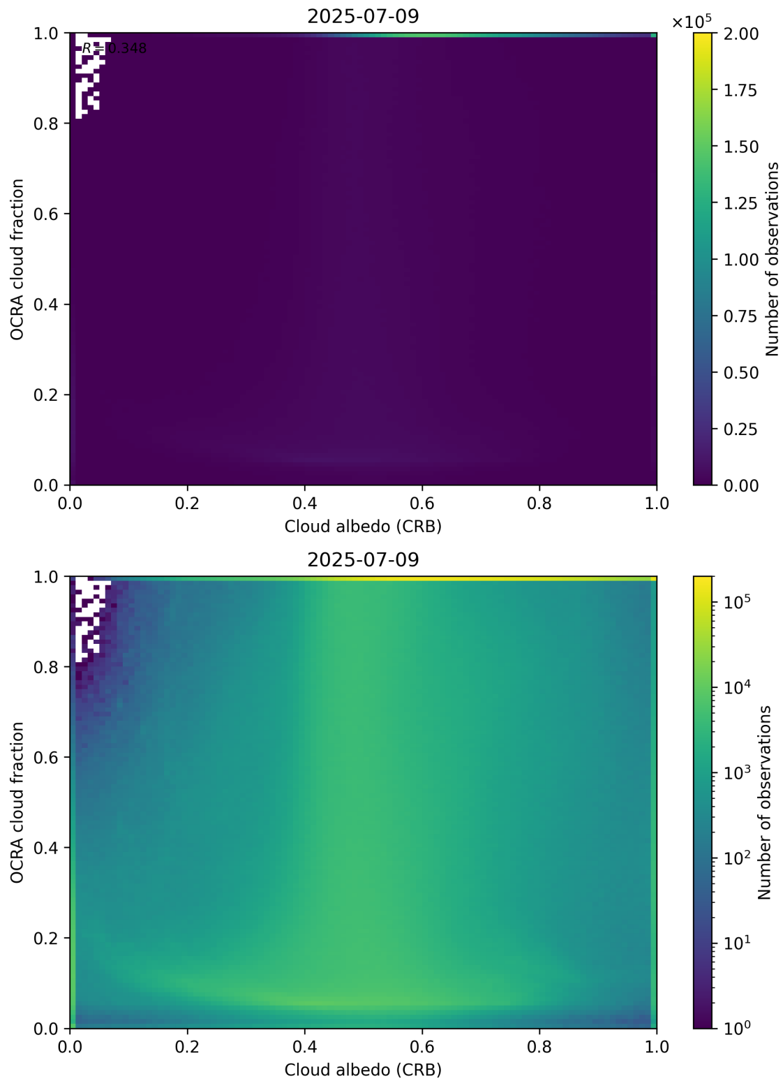
Figure 70: Scatter density plot of “Cloud albedo (CRB)” against “OCRA cloud fraction” for 2025-07-08 to 2025-07-10.
