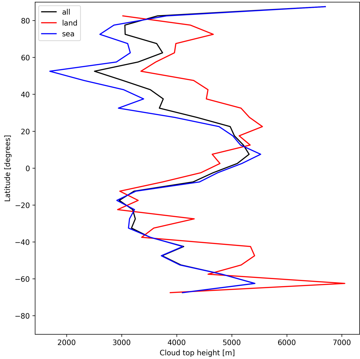
Figure 24: Zonal average of “Cloud top height” for 2025-07-08 to 2025-07-10.
