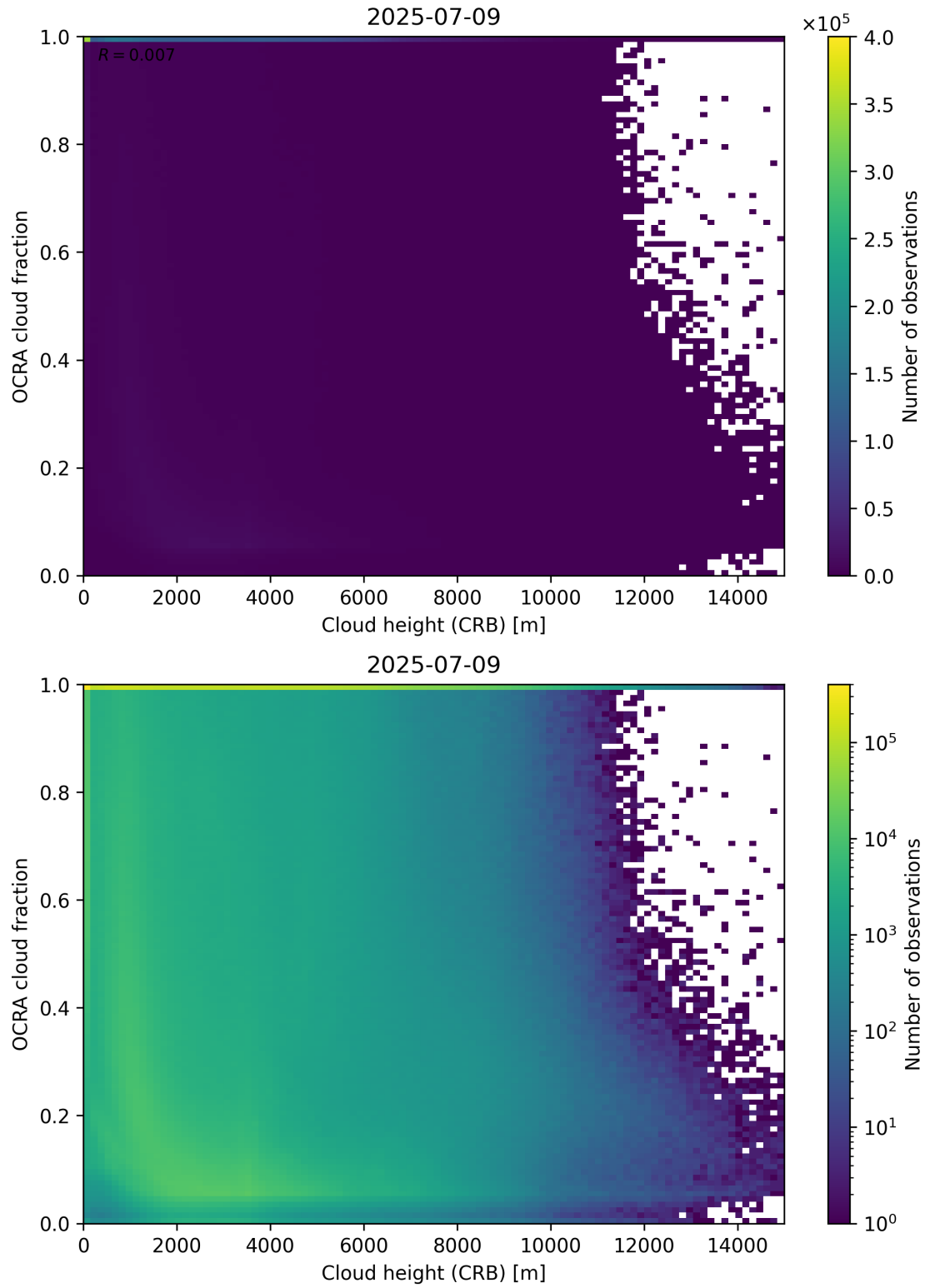
Figure 81: Scatter density plot of “Cloud height (CRB)” against “OCRA cloud fraction” for 2025-07-08 to 2025-07-10.
