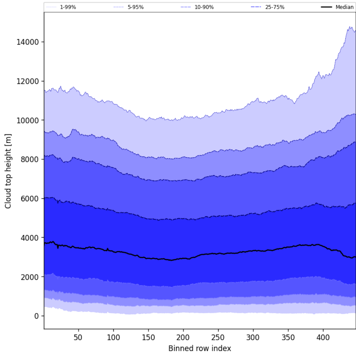
Figure 56: Along track statistics of “Cloud top height” for 2025-07-08 to 2025-07-10
