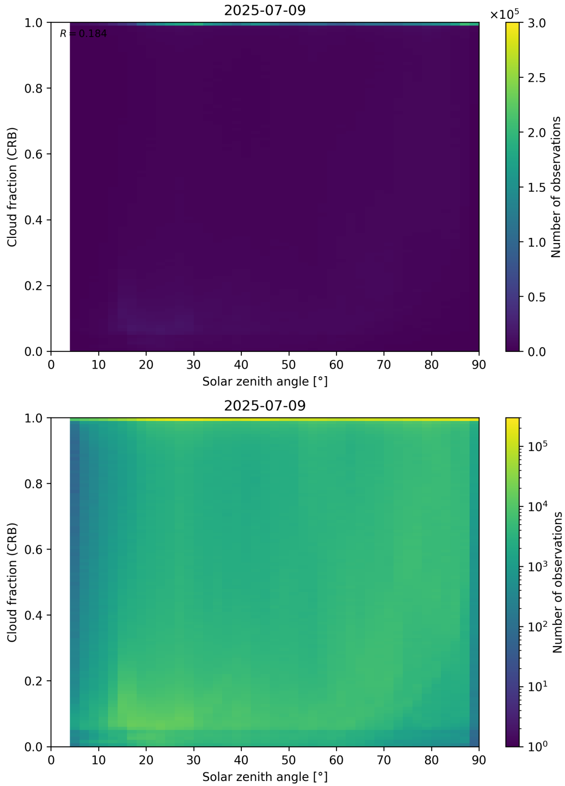
Figure 101: Scatter density plot of “Solar zenith angle” against “Cloud fraction (CRB)” for 2025-07-08 to 2025-07-10.
