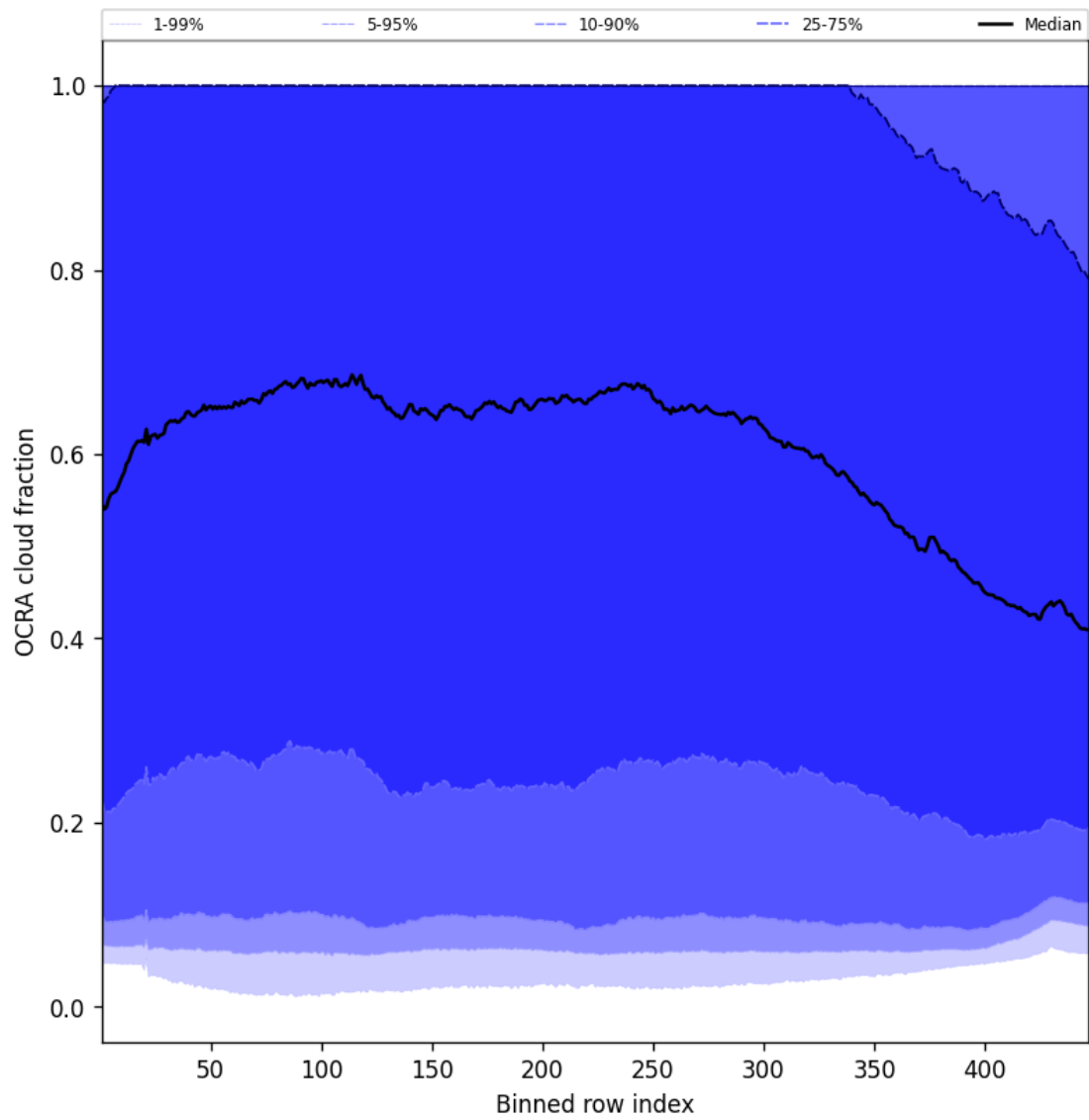
Figure 66: Along track statistics of “OCRA cloud fraction” for 2025-07-08 to 2025-07-10
