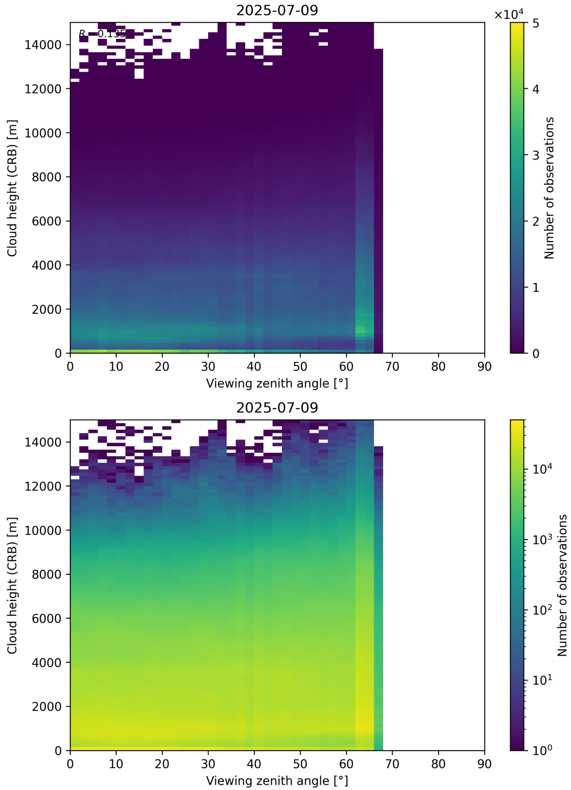
Figure 110: Scatter density plot of “Viewing zenith angle” against “Cloud height (CRB)” for 2025-07-08 to 2025-07-10.
