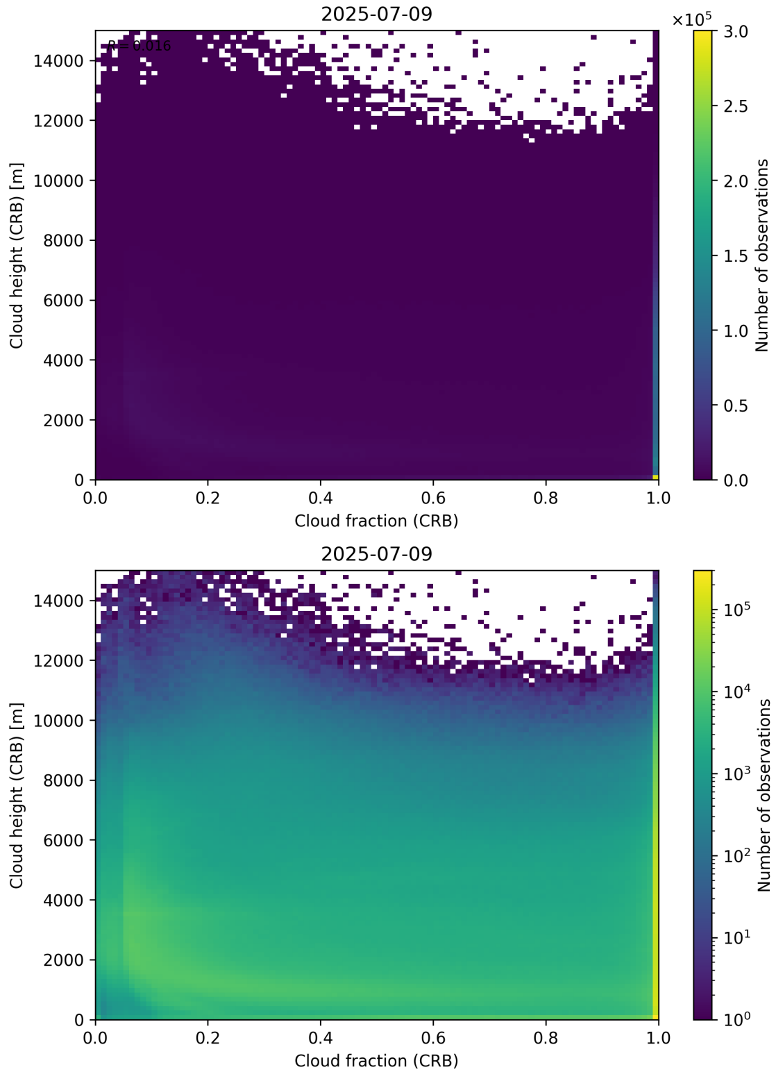
Figure 79: Scatter density plot of “Cloud fraction (CRB)” against “Cloud height (CRB)” for 2025-07-08 to 2025-07-10.
