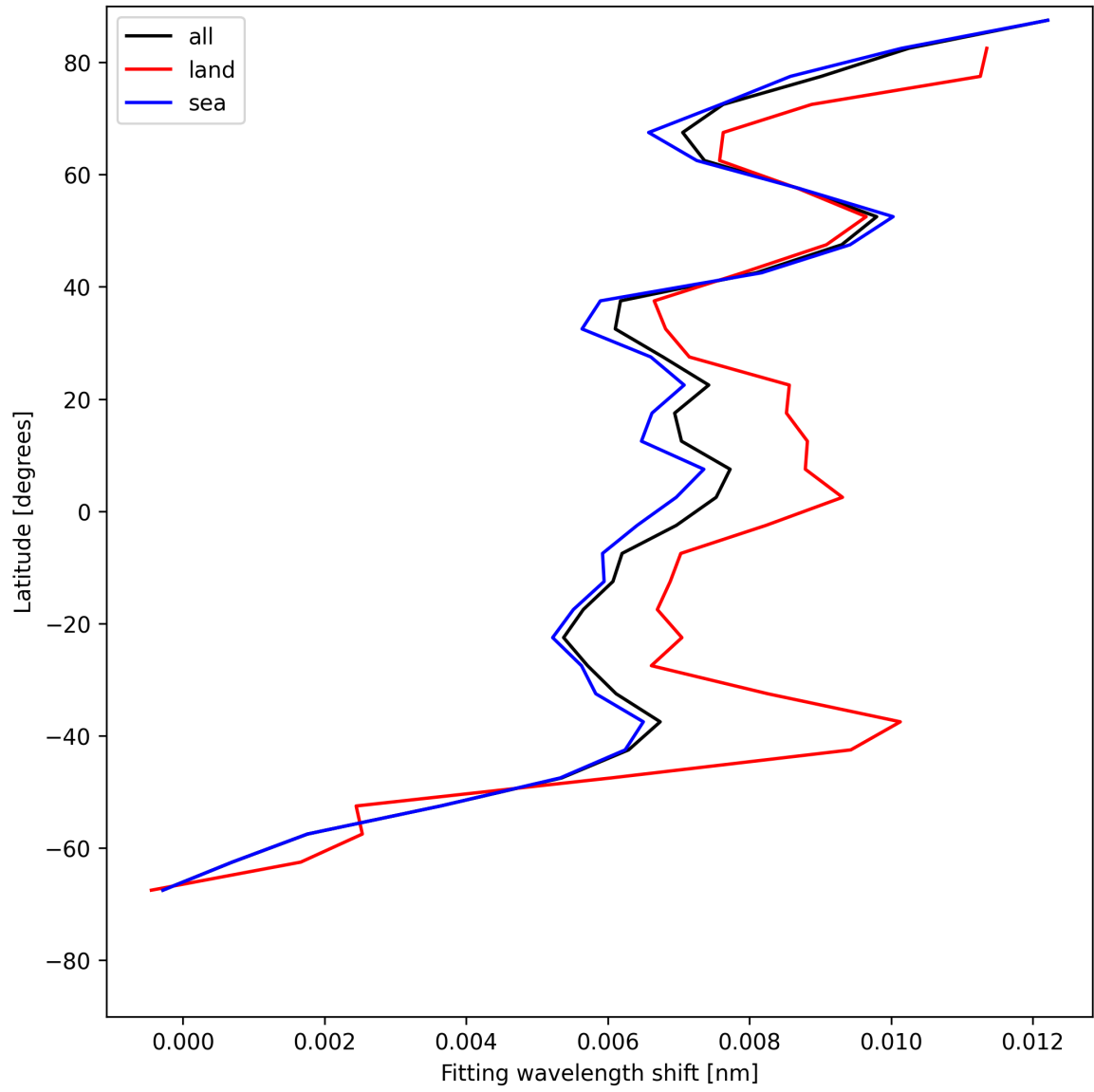
Figure 33: Zonal average of “Fitting wavelength shift” for 2025-07-08 to 2025-07-10.
