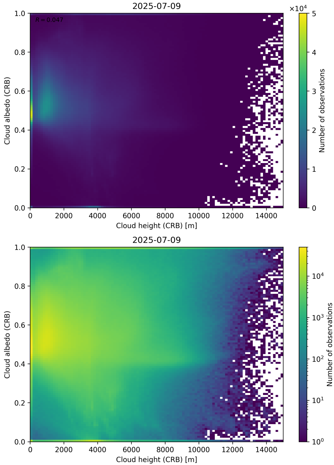
Figure 80: Scatter density plot of “Cloud height (CRB)” against “Cloud albedo (CRB)” for 2025-07-08 to 2025-07-10.
