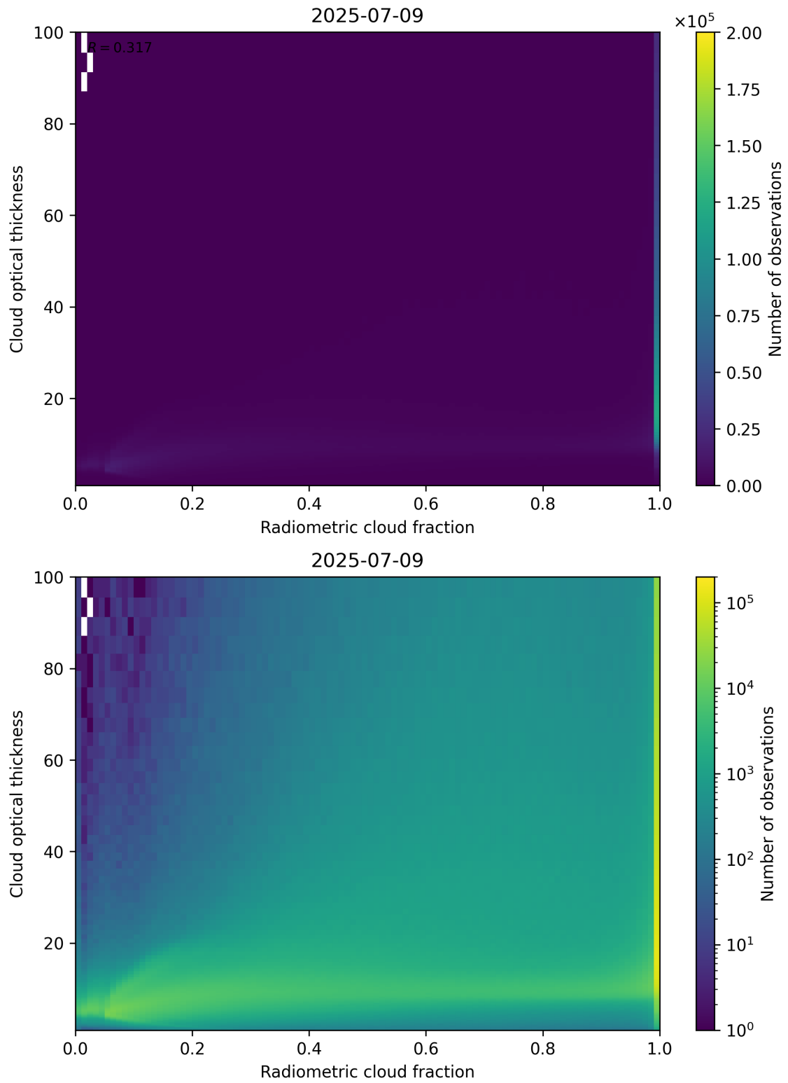
Figure 75: Scatter density plot of “Radiometric cloud fraction” against “Cloud optical thickness” for 2025-07-08 to 2025-07-10.
