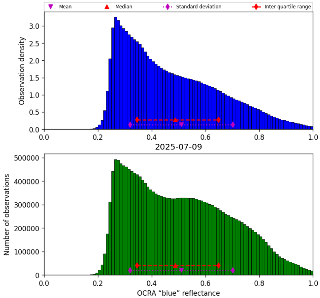
Figure 51: Histogram of “OCRA “blue” reflectance” for 2025-07-08 to 2025-07-10
