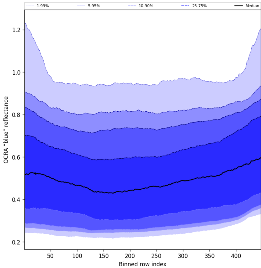
Figure 67: Along track statistics of “OCRA “blue” reflectance” for 2025-07-08 to 2025-07-10
