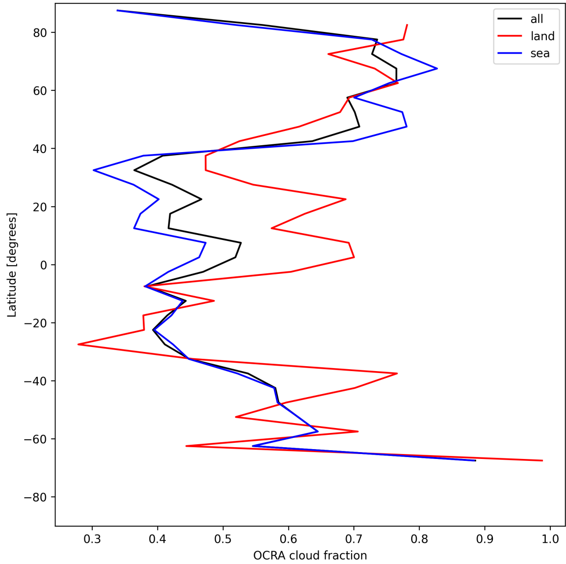
Figure 34: Zonal average of “OCRA cloud fraction” for 2025-07-08 to 2025-07-10.
