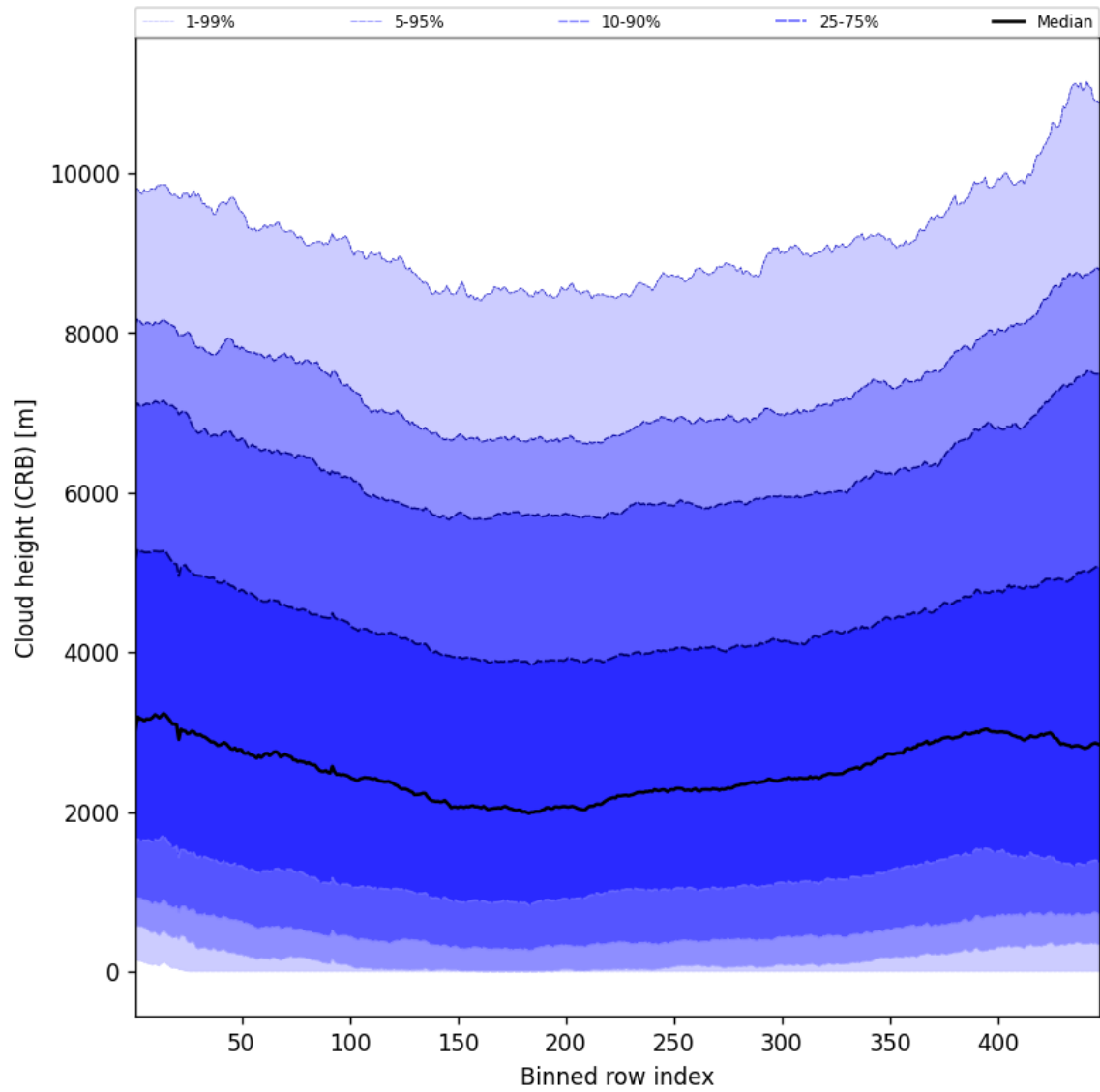
Figure 59: Along track statistics of “Cloud height (CRB)” for 2025-07-08 to 2025-07-10
