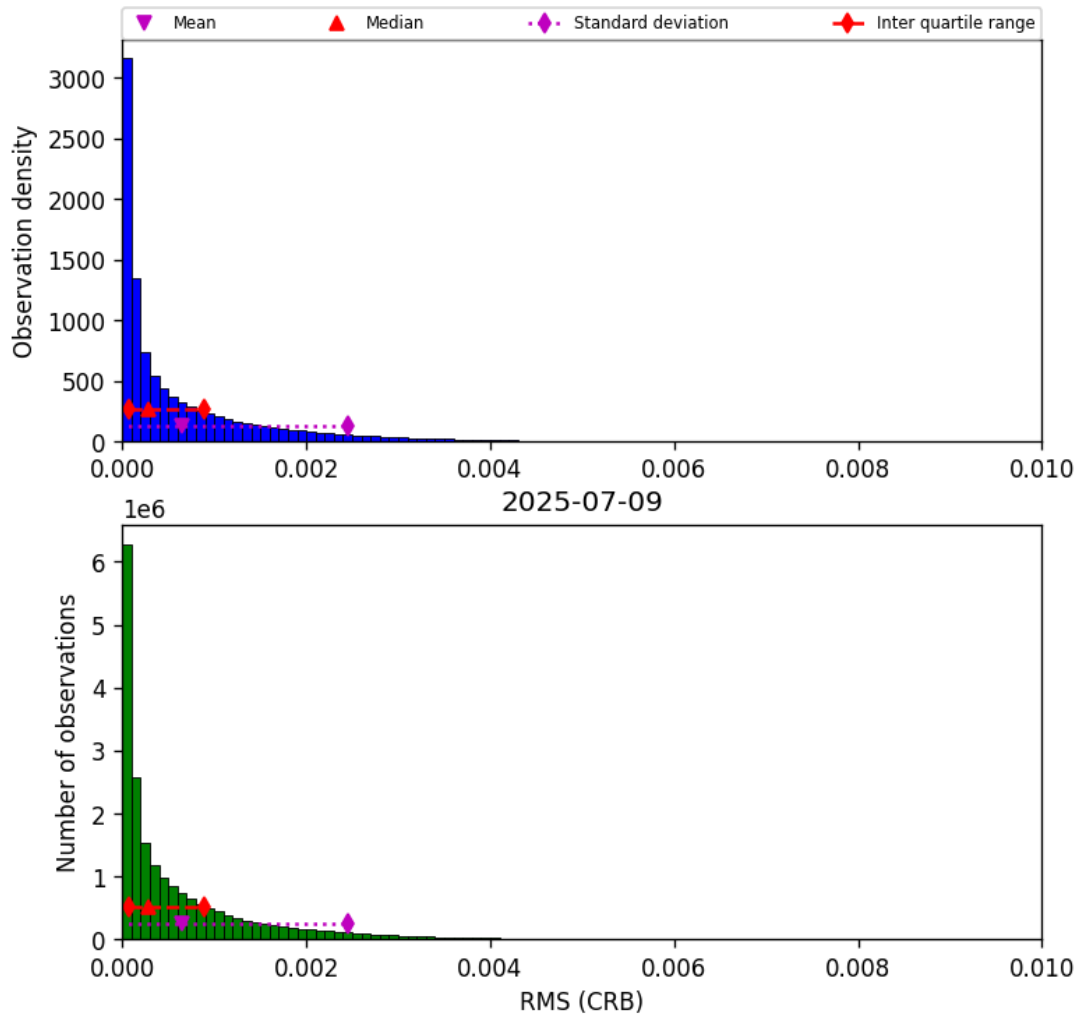
Figure 48: Histogram of “RMS (CRB)” for 2025-07-08 to 2025-07-10
