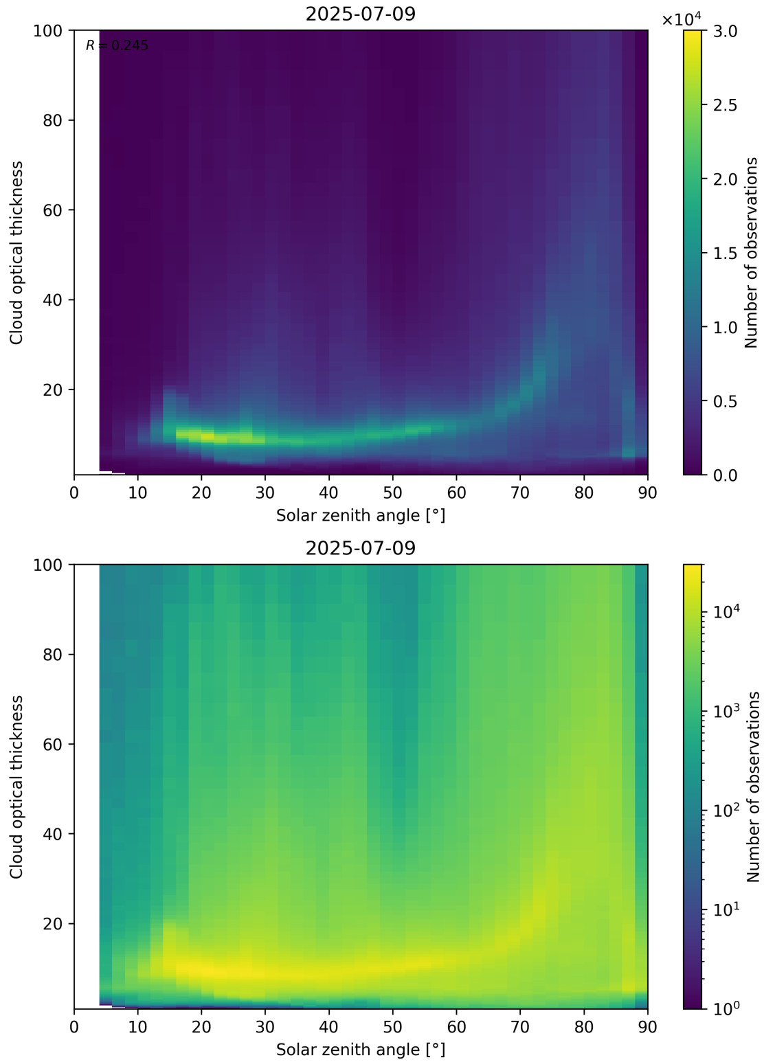
Figure 103: Scatter density plot of “Solar zenith angle” against “Cloud optical thickness” for 2025-07-08 to 2025-07-10.
