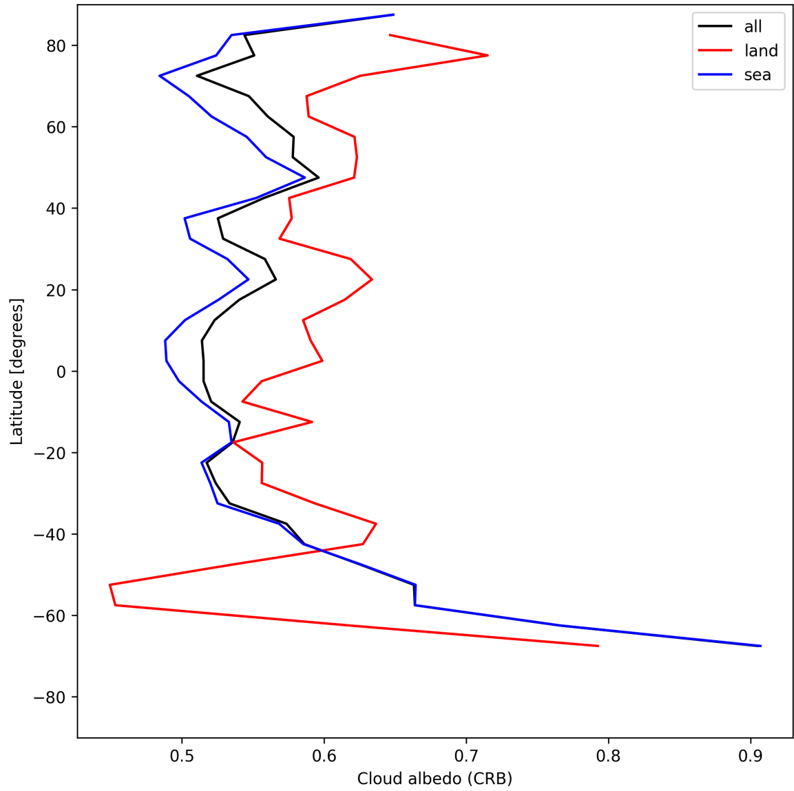
Figure 28: Zonal average of “Cloud albedo (CRB)” for 2025-07-08 to 2025-07-10.
