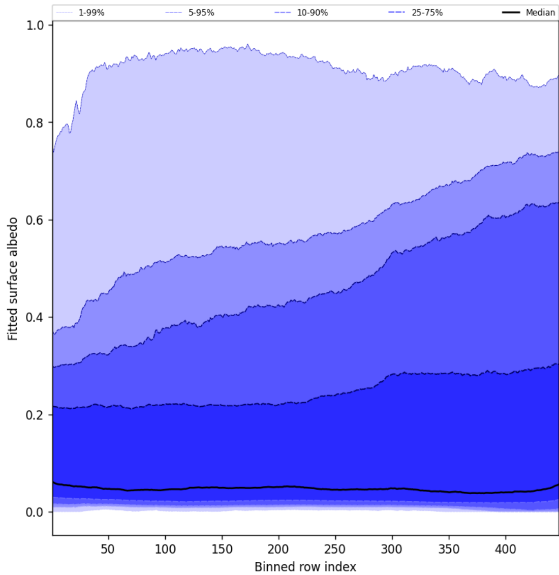
Figure 61: Along track statistics of “Fitted surface albedo” for 2025-07-08 to 2025-07-10
