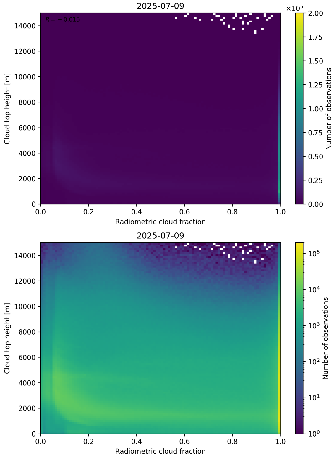
Figure 76: Scatter density plot of “Radiometric cloud fraction” against “Cloud top height” for 2025-07-08 to 2025-07-10.
