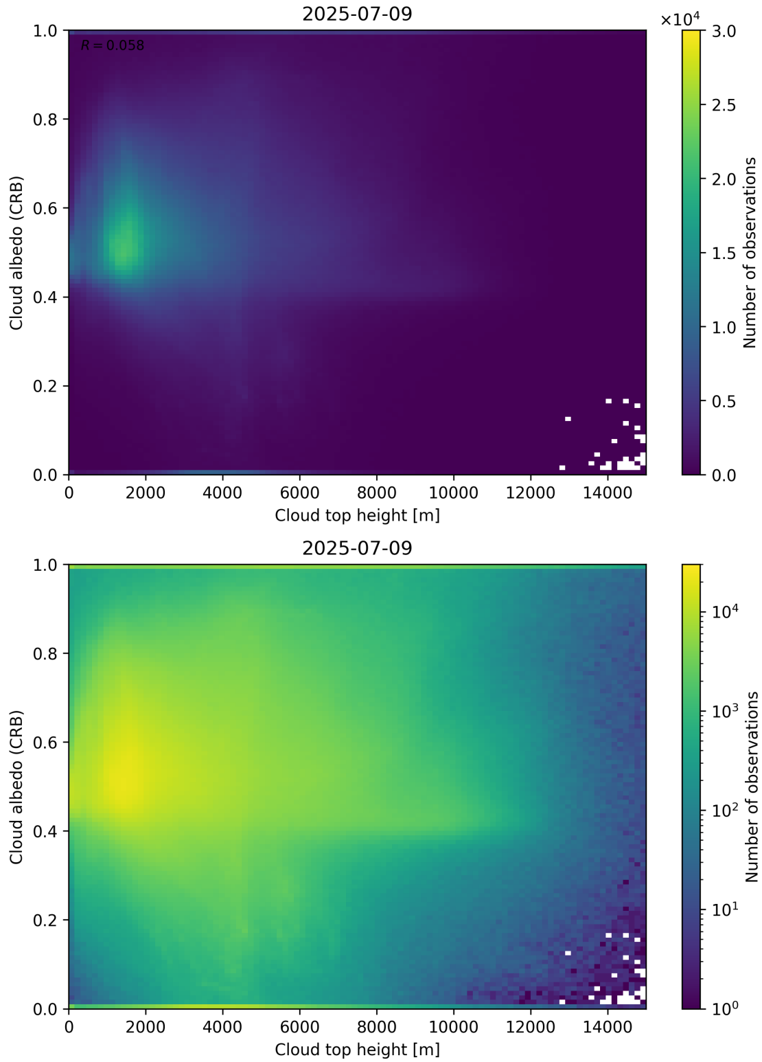
Figure 86: Scatter density plot of “Cloud top height” against “Cloud albedo (CRB)” for 2025-07-08 to 2025-07-10.
