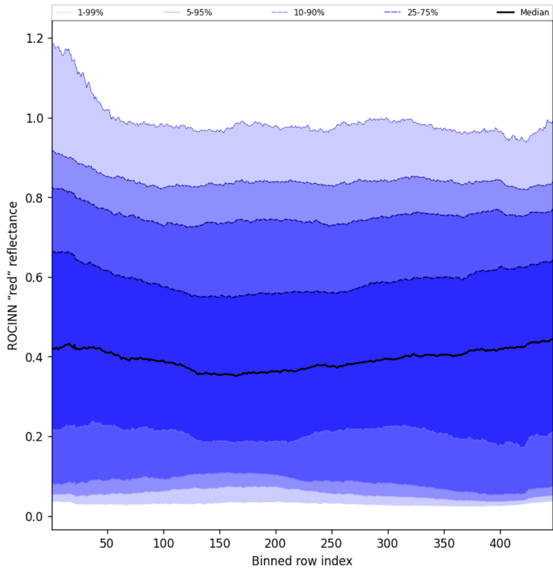
Figure 69: Along track statistics of “ROCINN “red” reflectance” for 2025-07-08 to 2025-07-10
