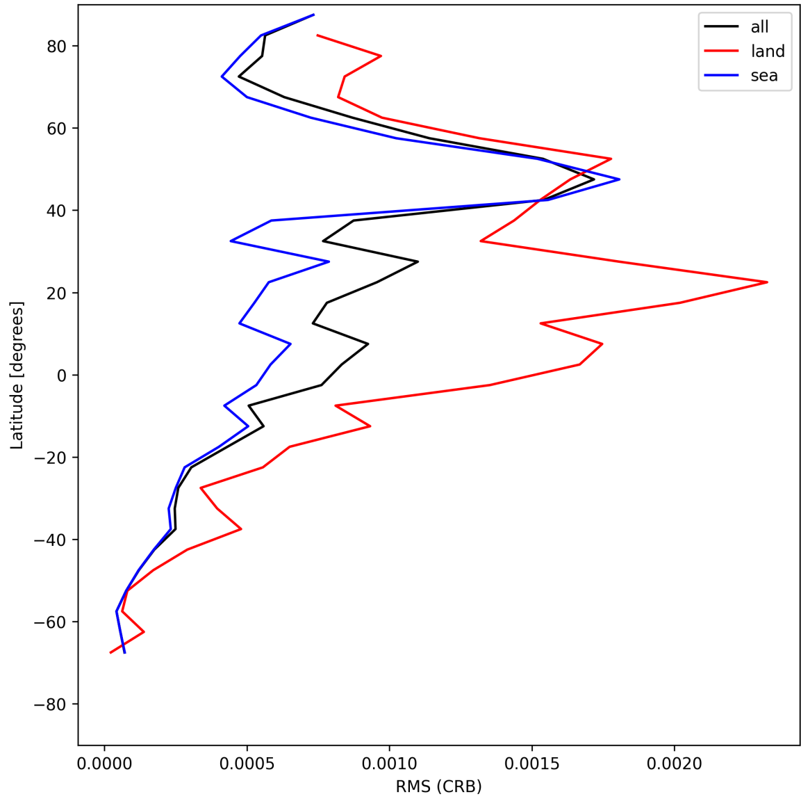
Figure 32: Zonal average of “RMS (CRB)” for 2025-07-08 to 2025-07-10.
