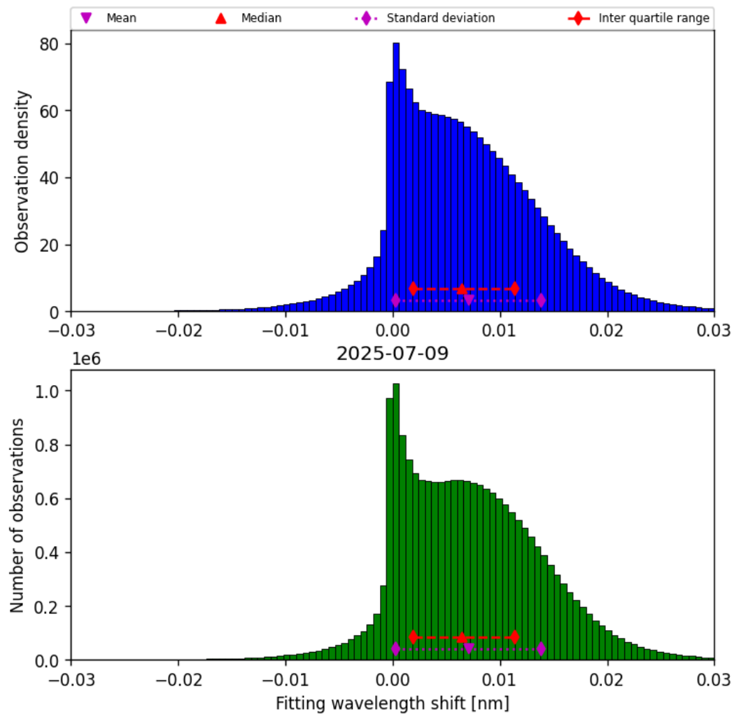
Figure 49: Histogram of “Fitting wavelength shift” for 2025-07-08 to 2025-07-10
