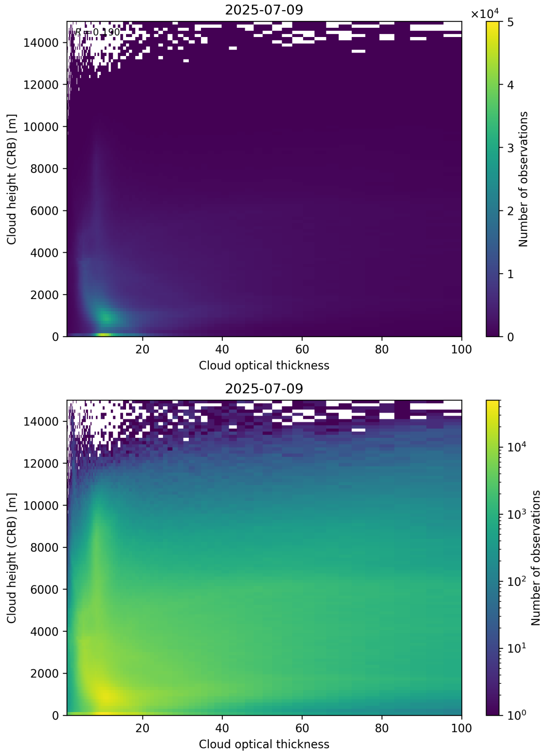
Figure 85: Scatter density plot of “Cloud optical thickness” against “Cloud height (CRB)” for 2025-07-08 to 2025-07-10.
