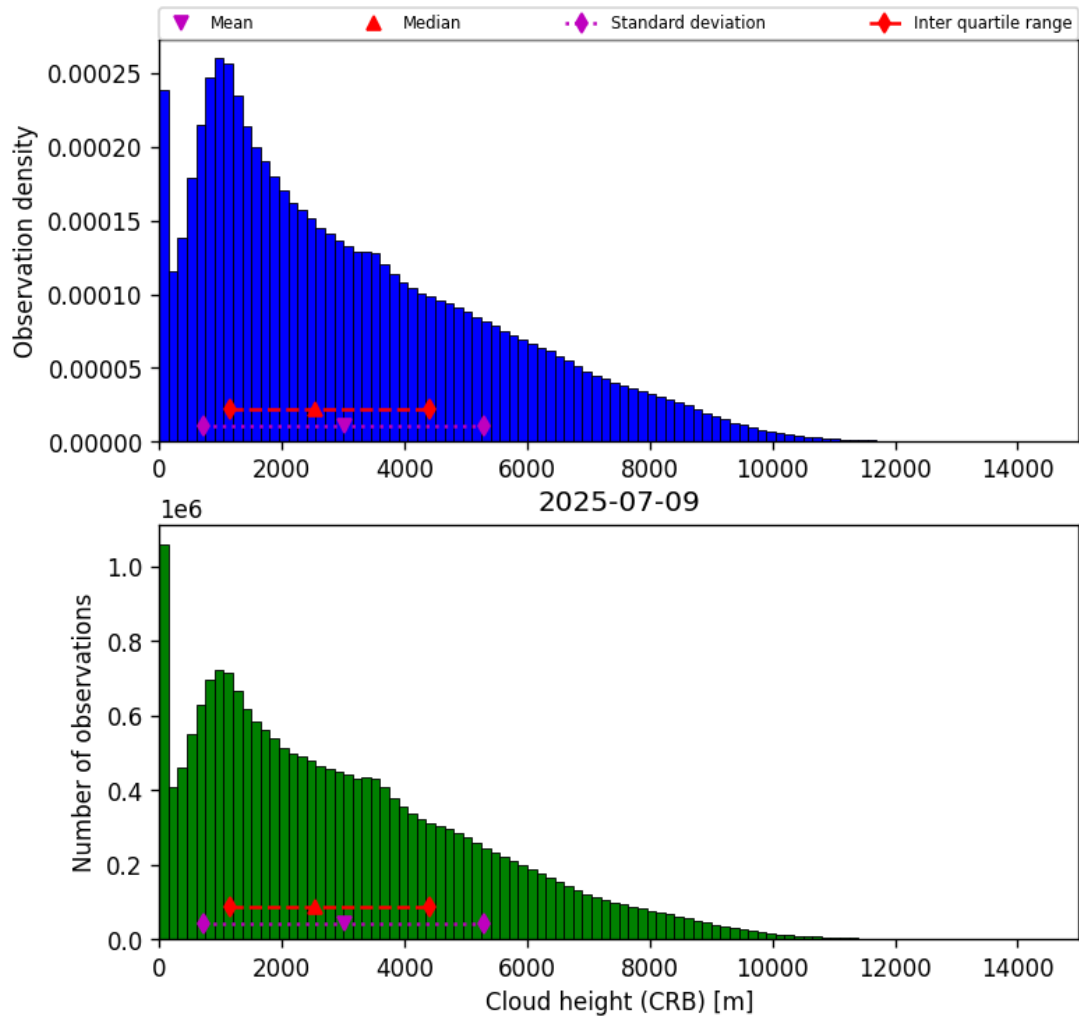
Figure 43: Histogram of “Cloud height (CRB)” for 2025-07-08 to 2025-07-10
