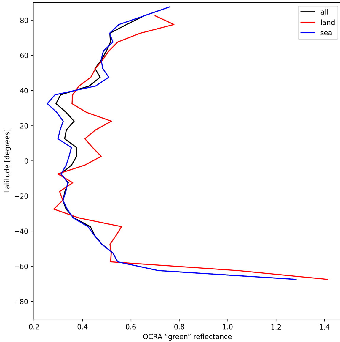
Figure 36: Zonal average of “OCRA “green” reflectance” for 2025-07-08 to 2025-07-10.
