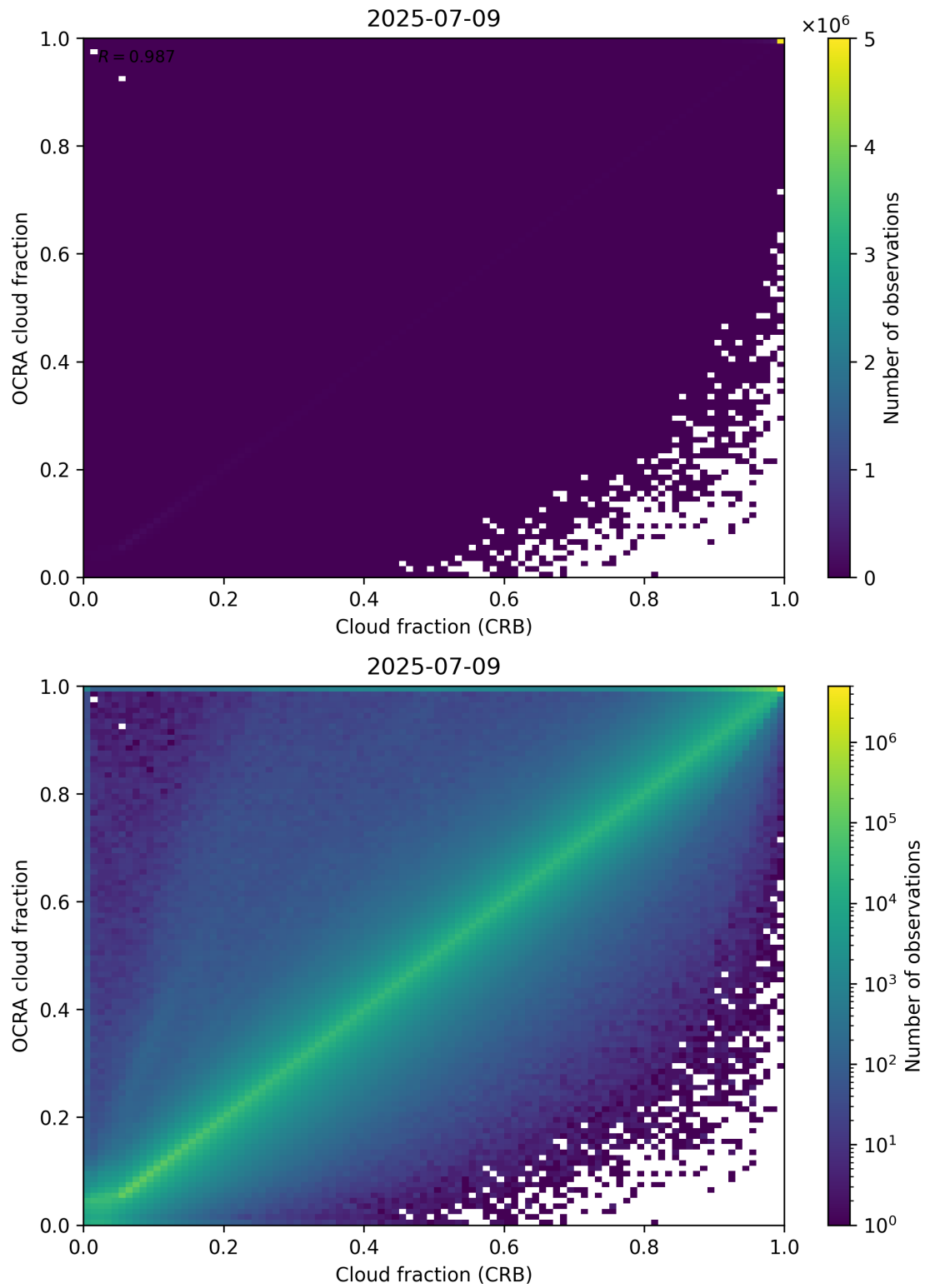
Figure 78: Scatter density plot of “Cloud fraction (CRB)” against “OCRA cloud fraction” for 2025-07-08 to 2025-07-10.
