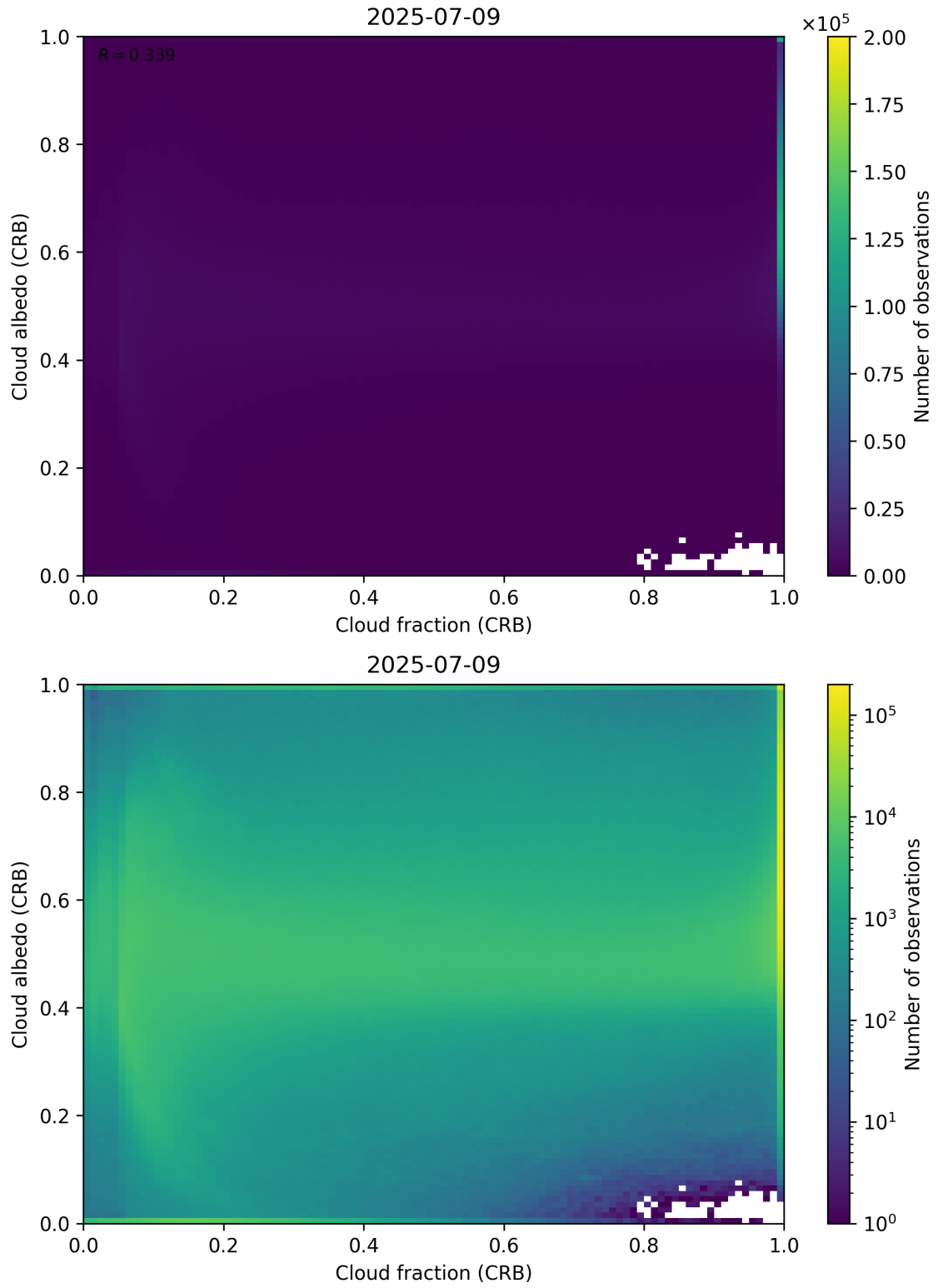
Figure 77: Scatter density plot of “Cloud fraction (CRB)” against “Cloud albedo (CRB)” for 2025-07-08 to 2025-07-10.
