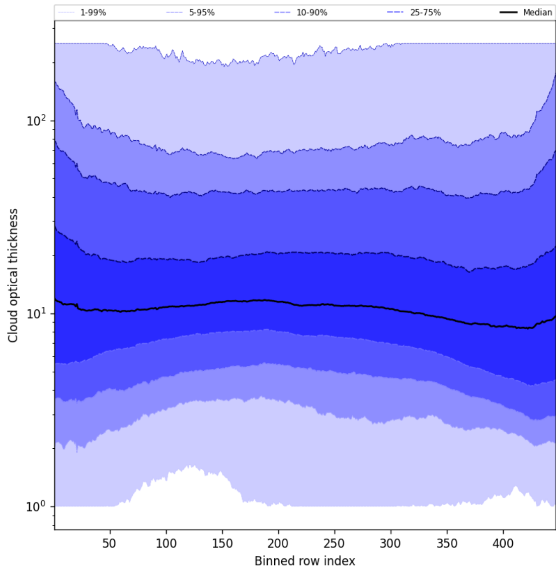
Figure 57: Along track statistics of “Cloud optical thickness” for 2025-07-08 to 2025-07-10
