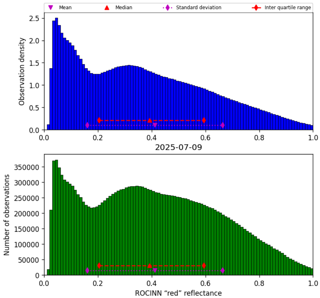
Figure 53: Histogram of “ROCINN “red” reflectance” for 2025-07-08 to 2025-07-10
