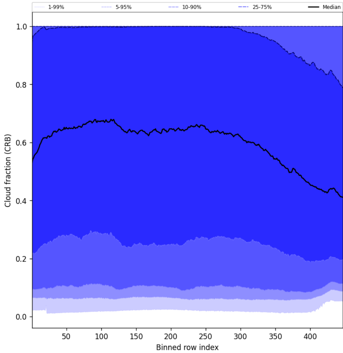
Figure 58: Along track statistics of “Cloud fraction (CRB)” for 2025-07-08 to 2025-07-10
