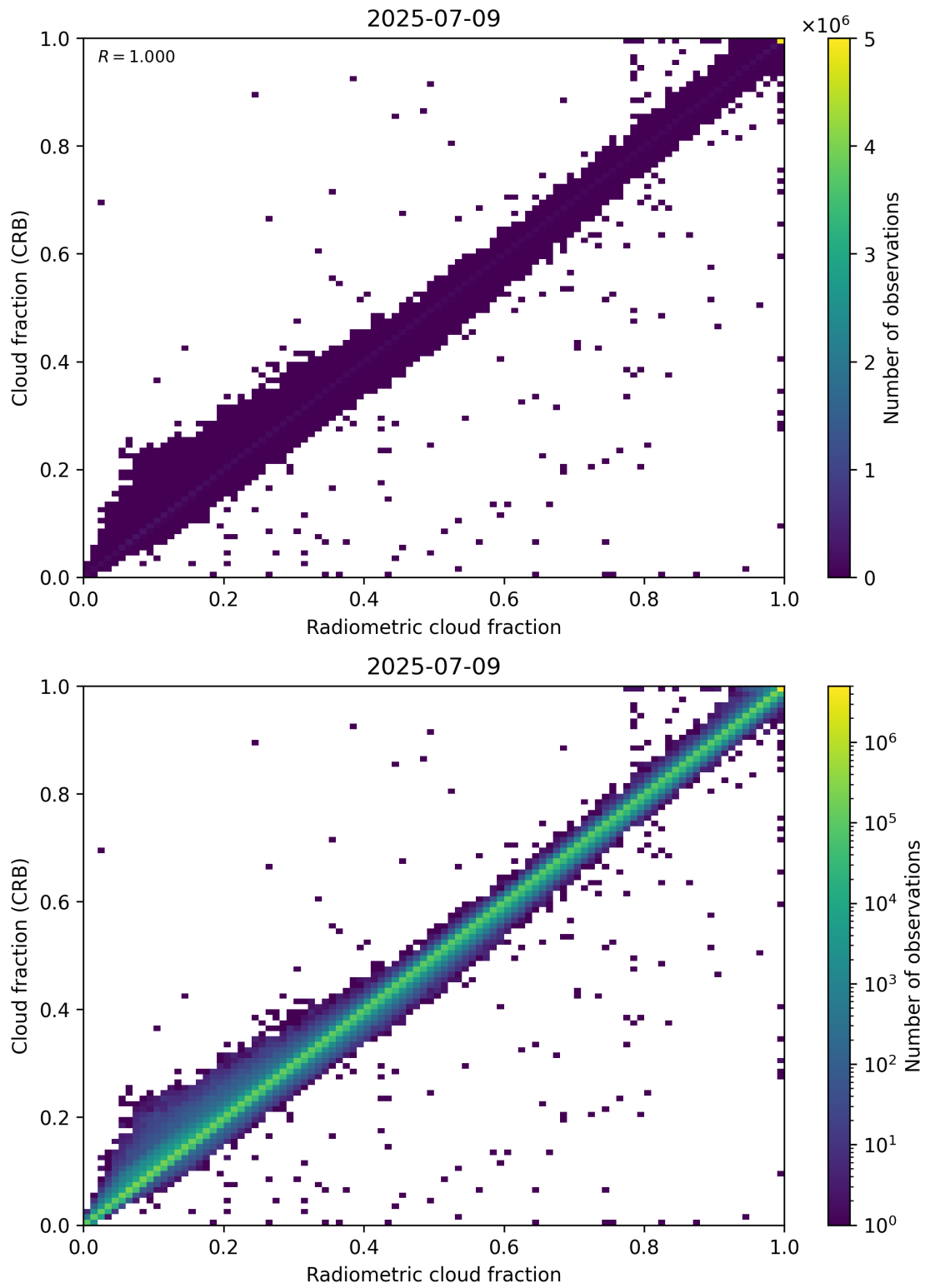
Figure 73: Scatter density plot of “Radiometric cloud fraction” against “Cloud fraction (CRB)” for 2025-07-08 to 2025-07-10.
