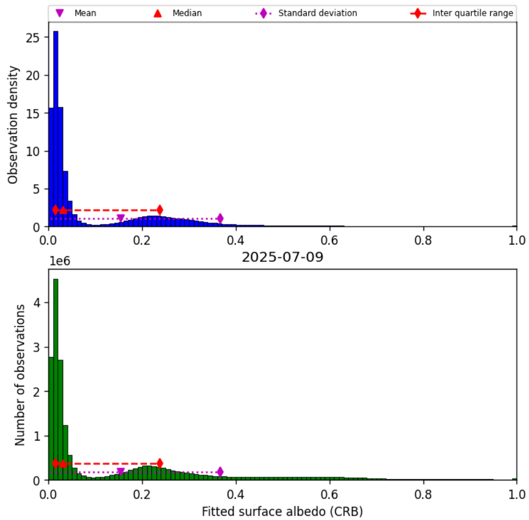
Figure 46: Histogram of “Fitted surface albedo (CRB)” for 2025-07-08 to 2025-07-10
