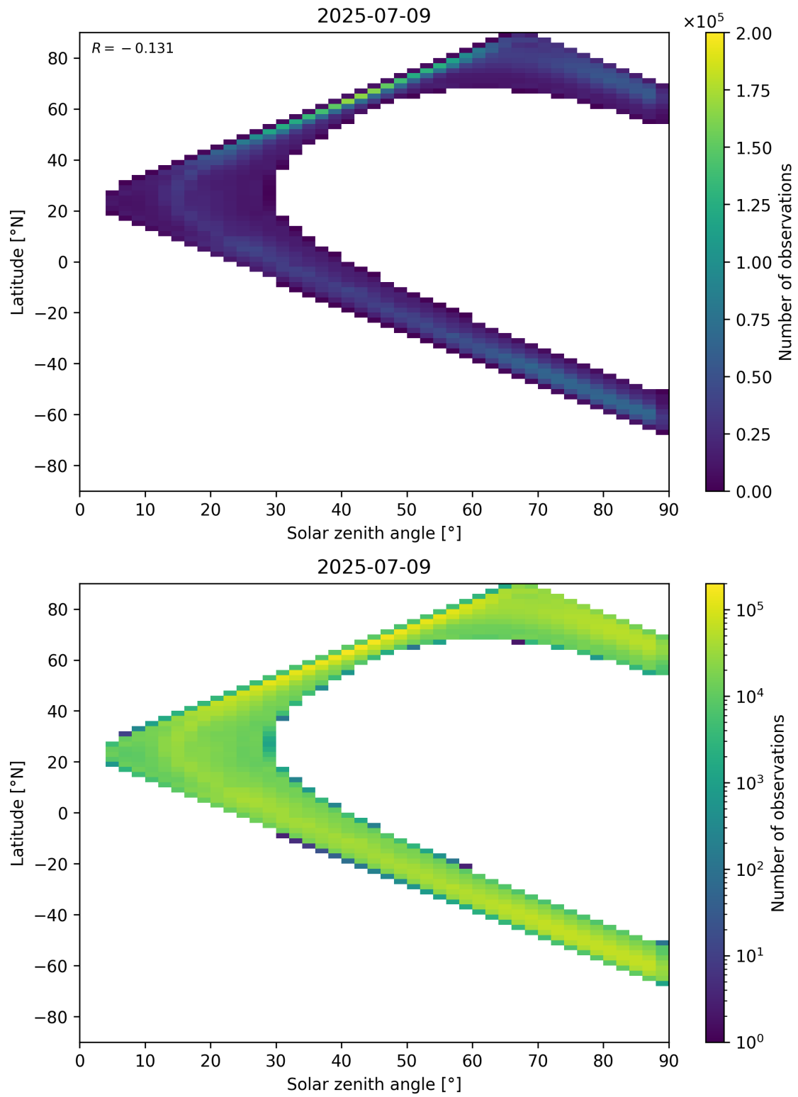
Figure 105: Scatter density plot of “Solar zenith angle” against “Latitude” for 2025-07-08 to 2025-07-10.
