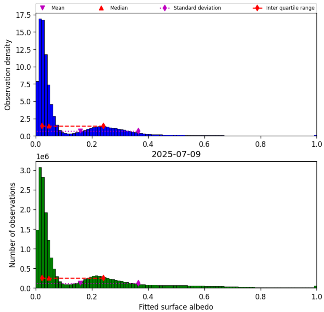
Figure 45: Histogram of “Fitted surface albedo” for 2025-07-08 to 2025-07-10
