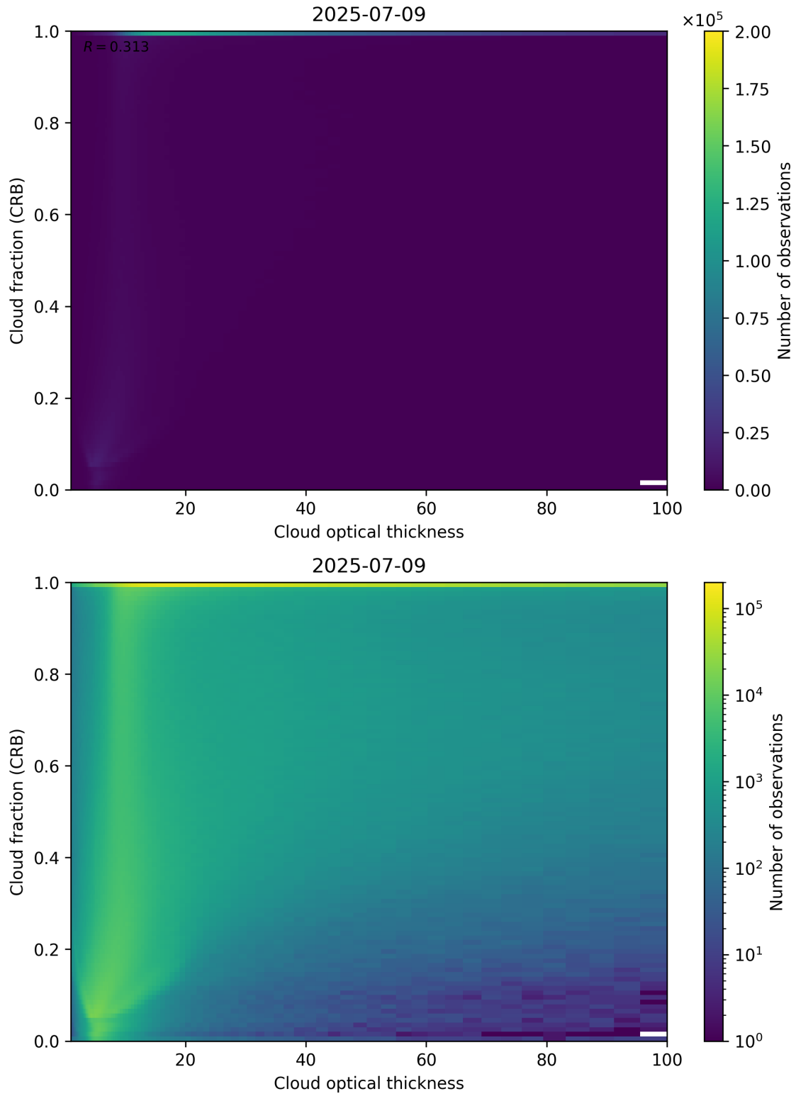
Figure 84: Scatter density plot of “Cloud optical thickness” against “Cloud fraction (CRB)” for 2025-07-08 to 2025-07-10.
