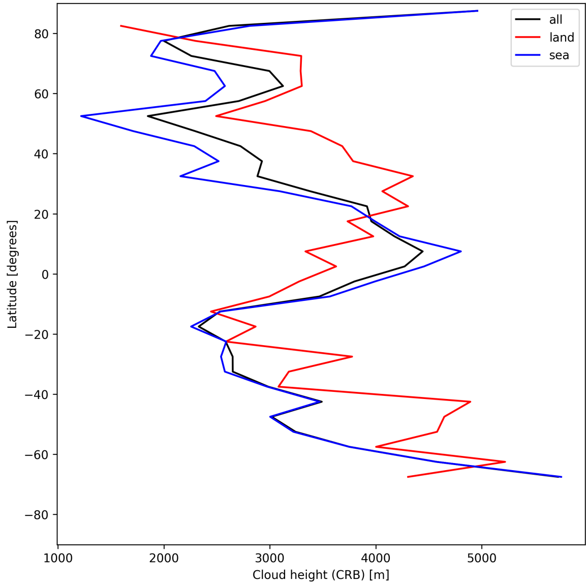
Figure 27: Zonal average of “Cloud height (CRB)” for 2025-07-08 to 2025-07-10.
