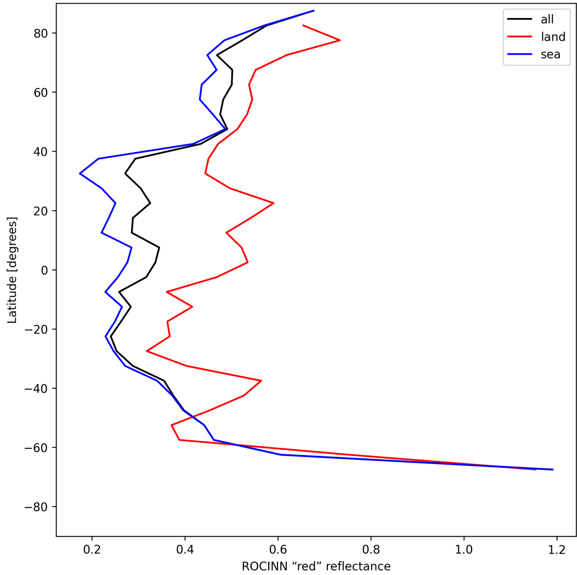
Figure 37: Zonal average of “ROCINN “red” reflectance” for 2025-07-08 to 2025-07-10.
