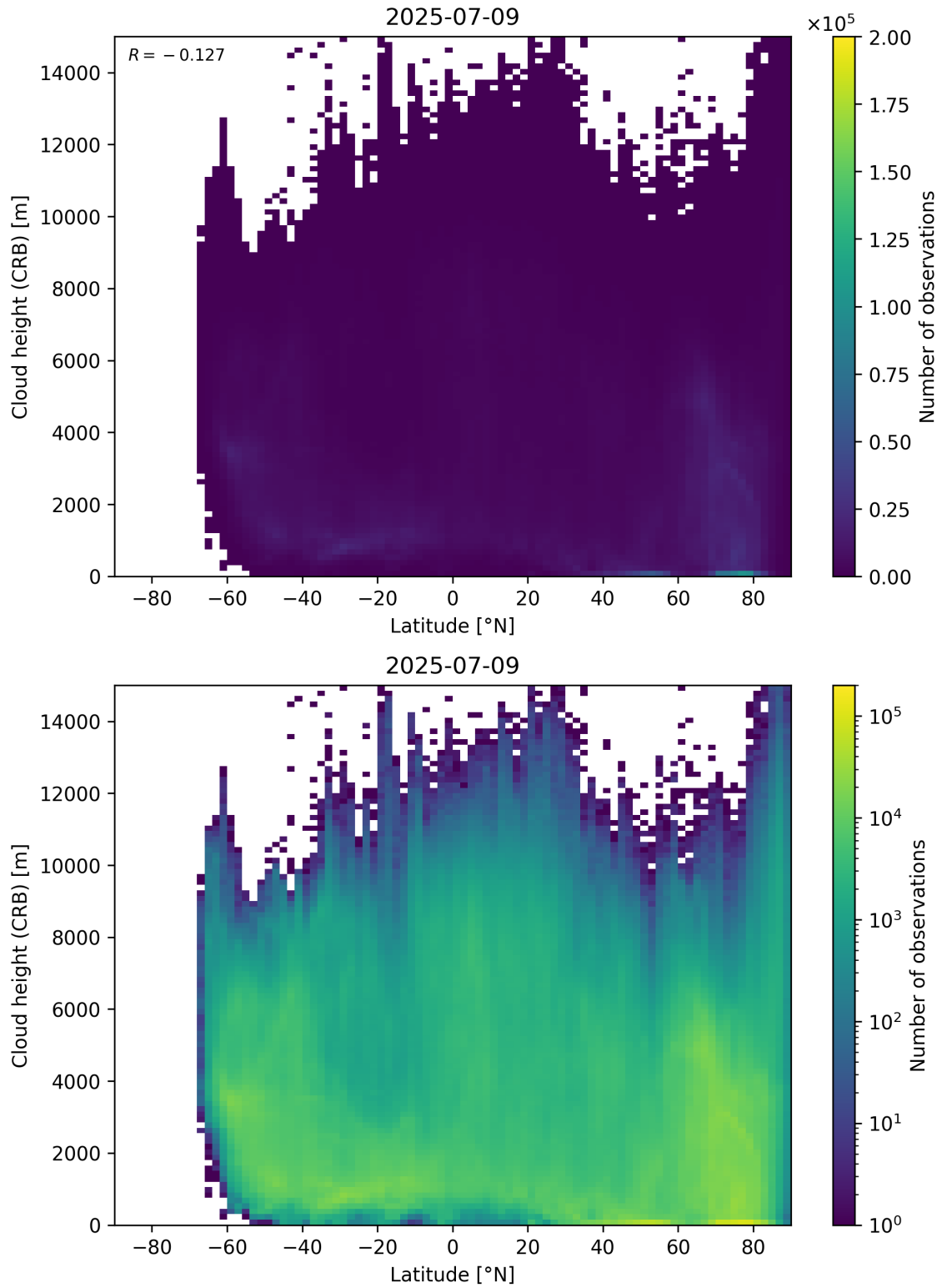
Figure 95: Scatter density plot of “Latitude” against “Cloud height (CRB)” for 2025-07-08 to 2025-07-10.
