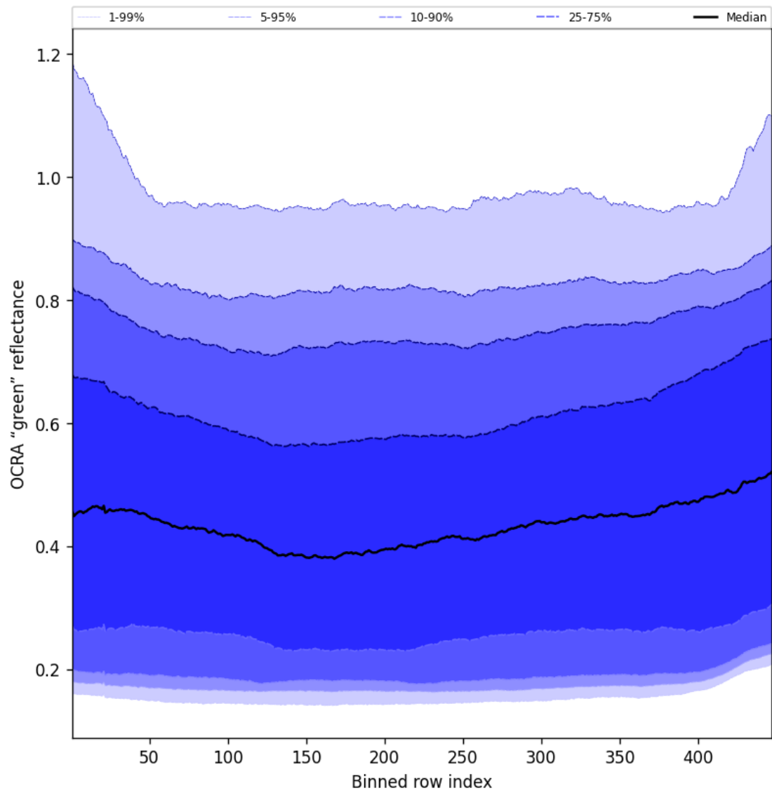
Figure 68: Along track statistics of “OCRA “green” reflectance” for 2025-07-08 to 2025-07-10
