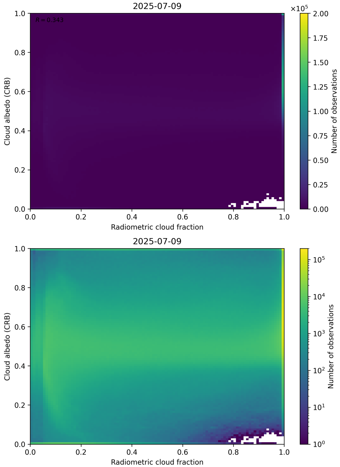
Figure 71: Scatter density plot of “Radiometric cloud fraction” against “Cloud albedo (CRB)” for 2025-07-08 to 2025-07-10.
