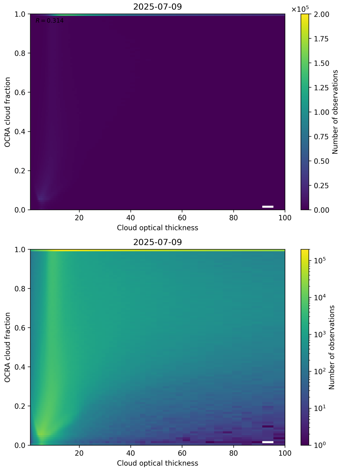
Figure 83: Scatter density plot of “Cloud optical thickness” against “OCRA cloud fraction” for 2025-07-08 to 2025-07-10.
