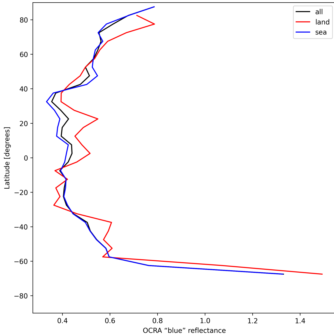
Figure 35: Zonal average of "OCRA "blue" reflectance" for 2025-07-08 to 2025-07-10.
