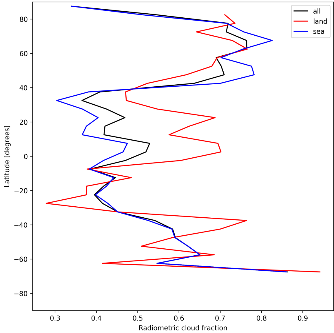
Figure 23: Zonal average of “Radiometric cloud fraction” for 2025-07-08 to 2025-07-10.
