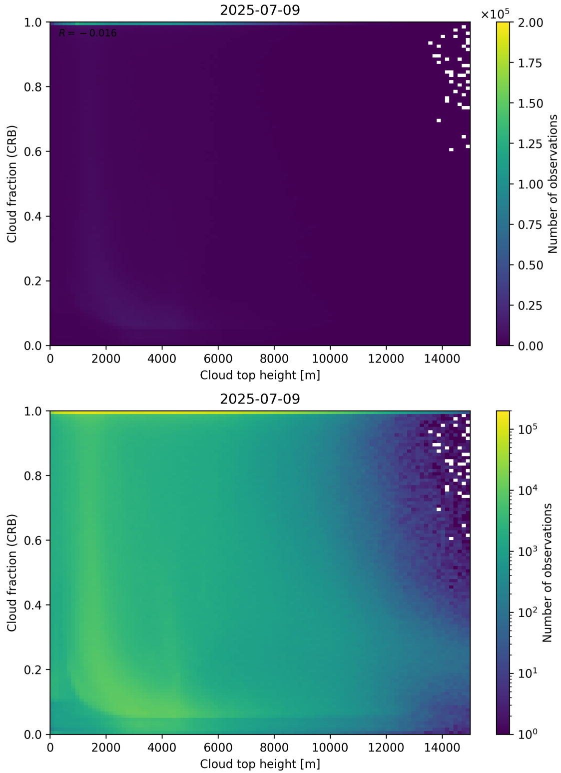
Figure 88: Scatter density plot of “Cloud top height” against “Cloud fraction (CRB)” for 2025-07-08 to 2025-07-10.
