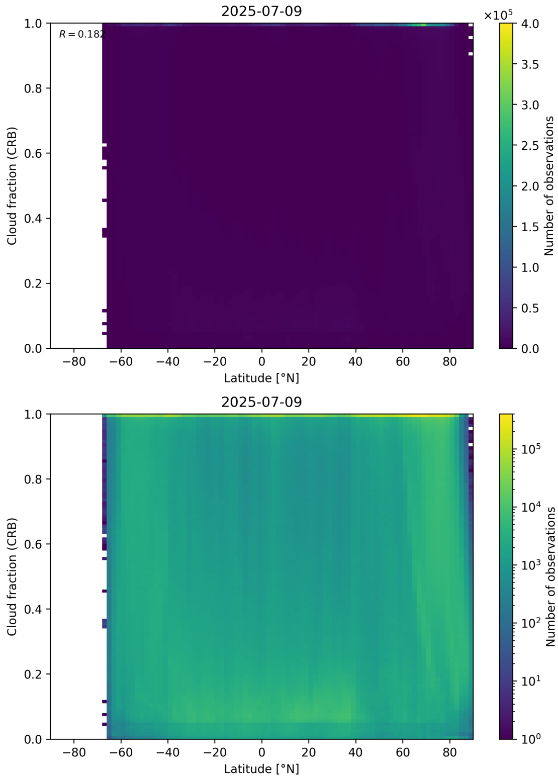
Figure 94: Scatter density plot of “Latitude” against “Cloud fraction (CRB)” for 2025-07-08 to 2025-07-10.
