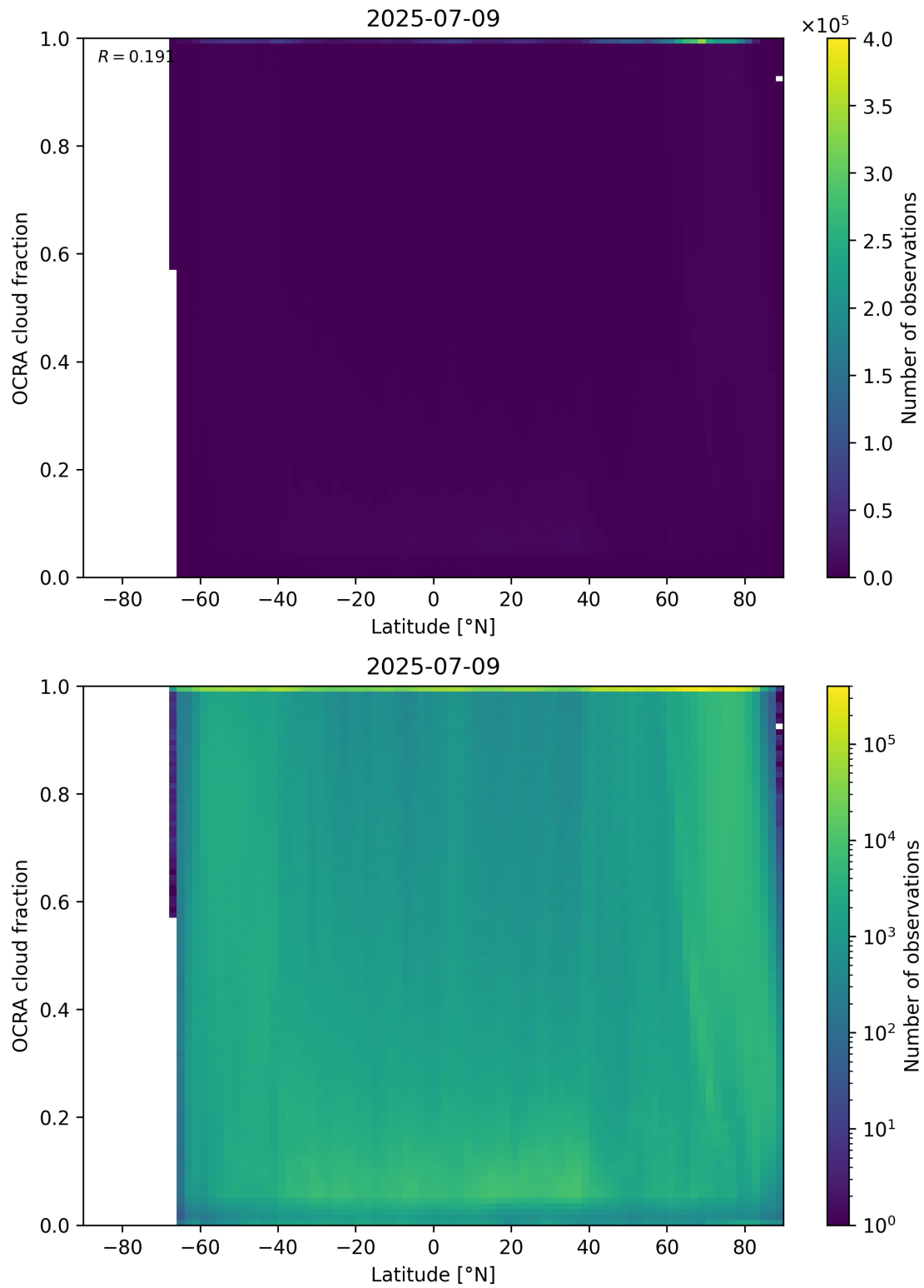
Figure 93: Scatter density plot of “Latitude” against “OCRA cloud fraction” for 2025-07-08 to 2025-07-10.
