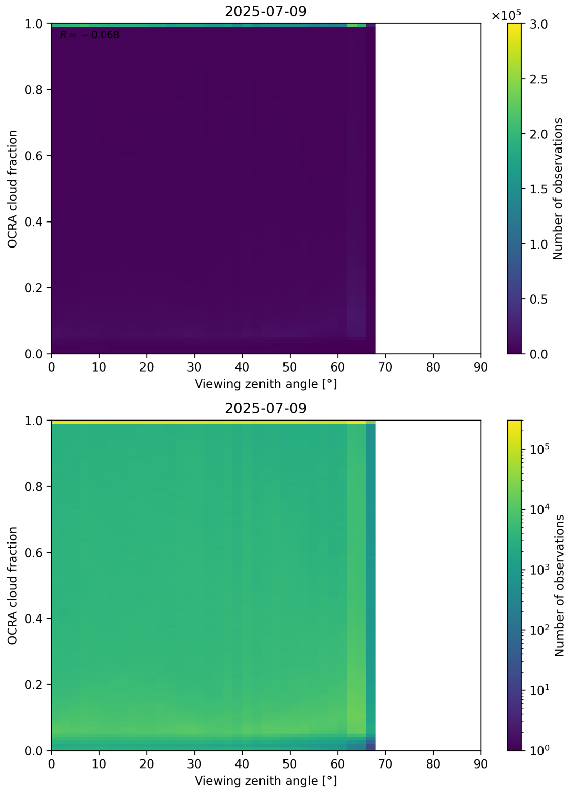
Figure 108: Scatter density plot of “Viewing zenith angle” against “OCRA cloud fraction” for 2025-07-08 to 2025-07-10.
