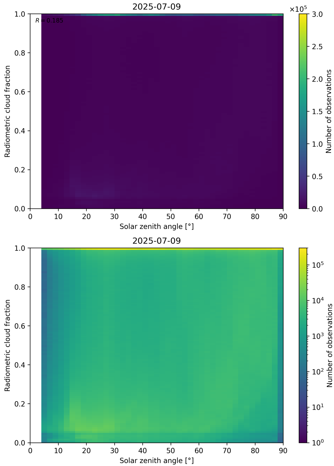
Figure 99: Scatter density plot of “Solar zenith angle” against “Radiometric cloud fraction” for 2025-07-08 to 2025-07-10.
