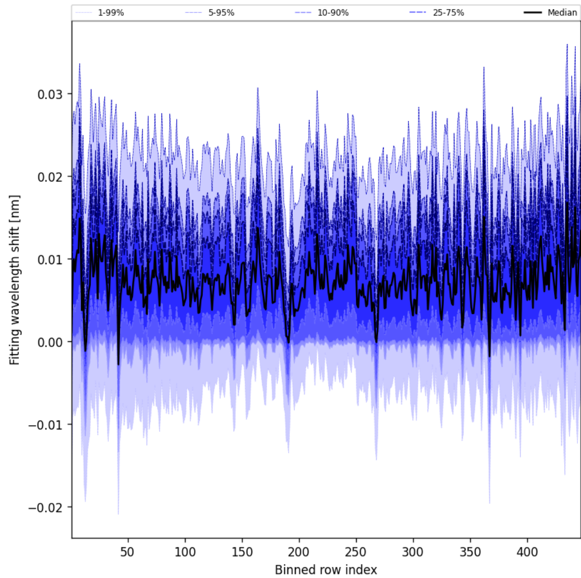
Figure 65: Along track statistics of “Fitting wavelength shift” for 2025-07-08 to 2025-07-10
