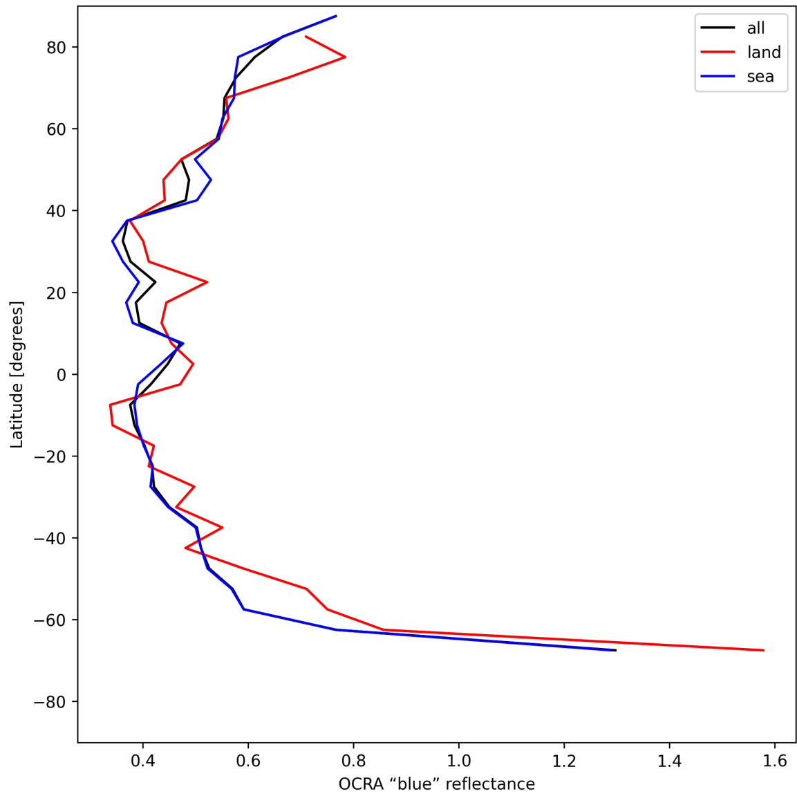
Figure 35: Zonal average of “OCRA “blue” reflectance” for 2025-07-09 to 2025-07-11.
