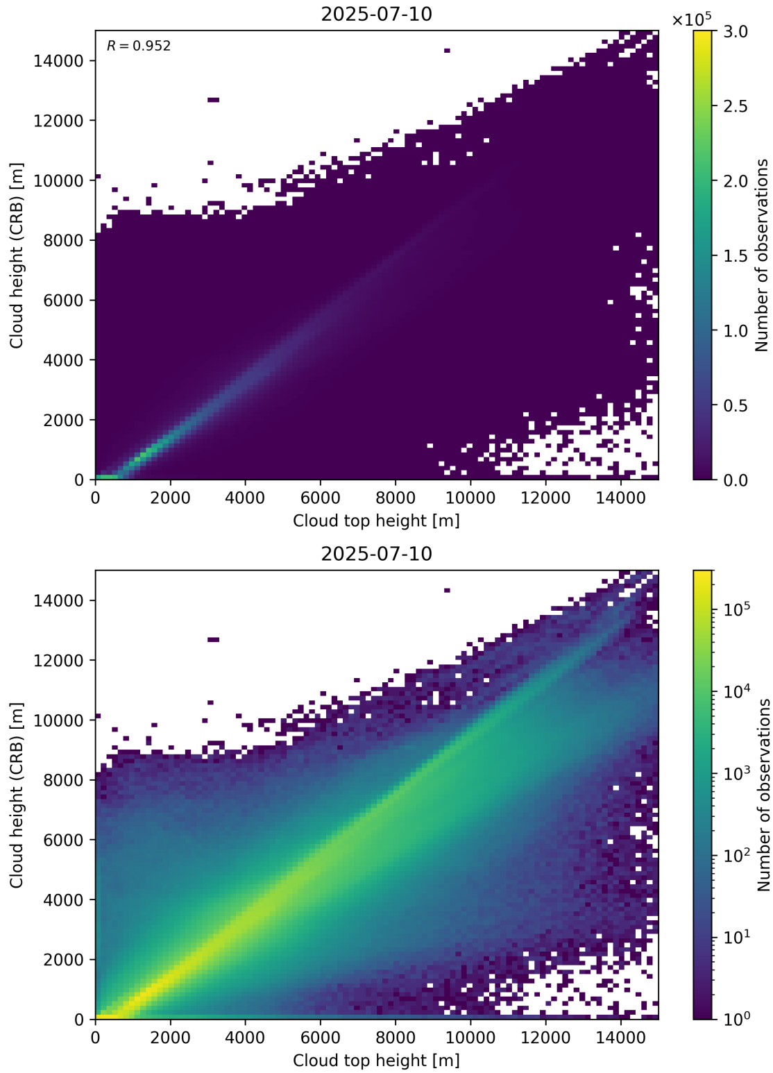
Figure 89: Scatter density plot of “Cloud top height” against “Cloud height (CRB)” for 2025-07-09 to 2025-07-11.
