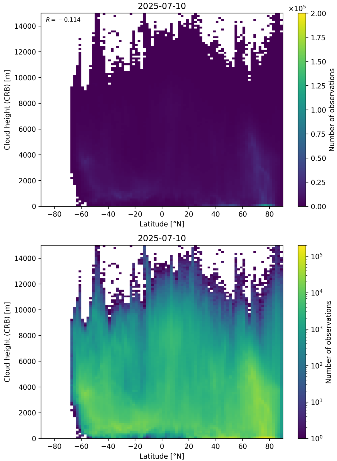
Figure 95: Scatter density plot of “Latitude” against “Cloud height (CRB)” for 2025-07-09 to 2025-07-11.
