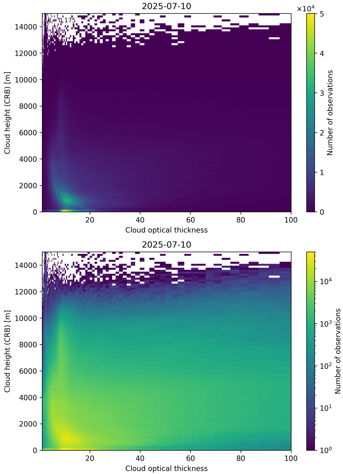
Figure 85: Scatter density plot of “Cloud optical thickness” against “Cloud height (CRB)” for 2025-07-09 to 2025-07-11.
