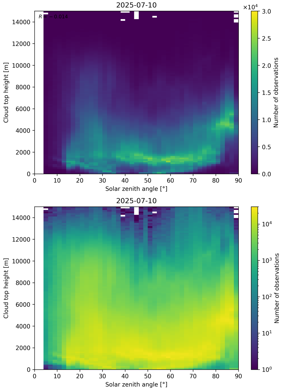
Figure 104: Scatter density plot of “Solar zenith angle” against “Cloud top height” for 2025-07-09 to 2025-07-11.
