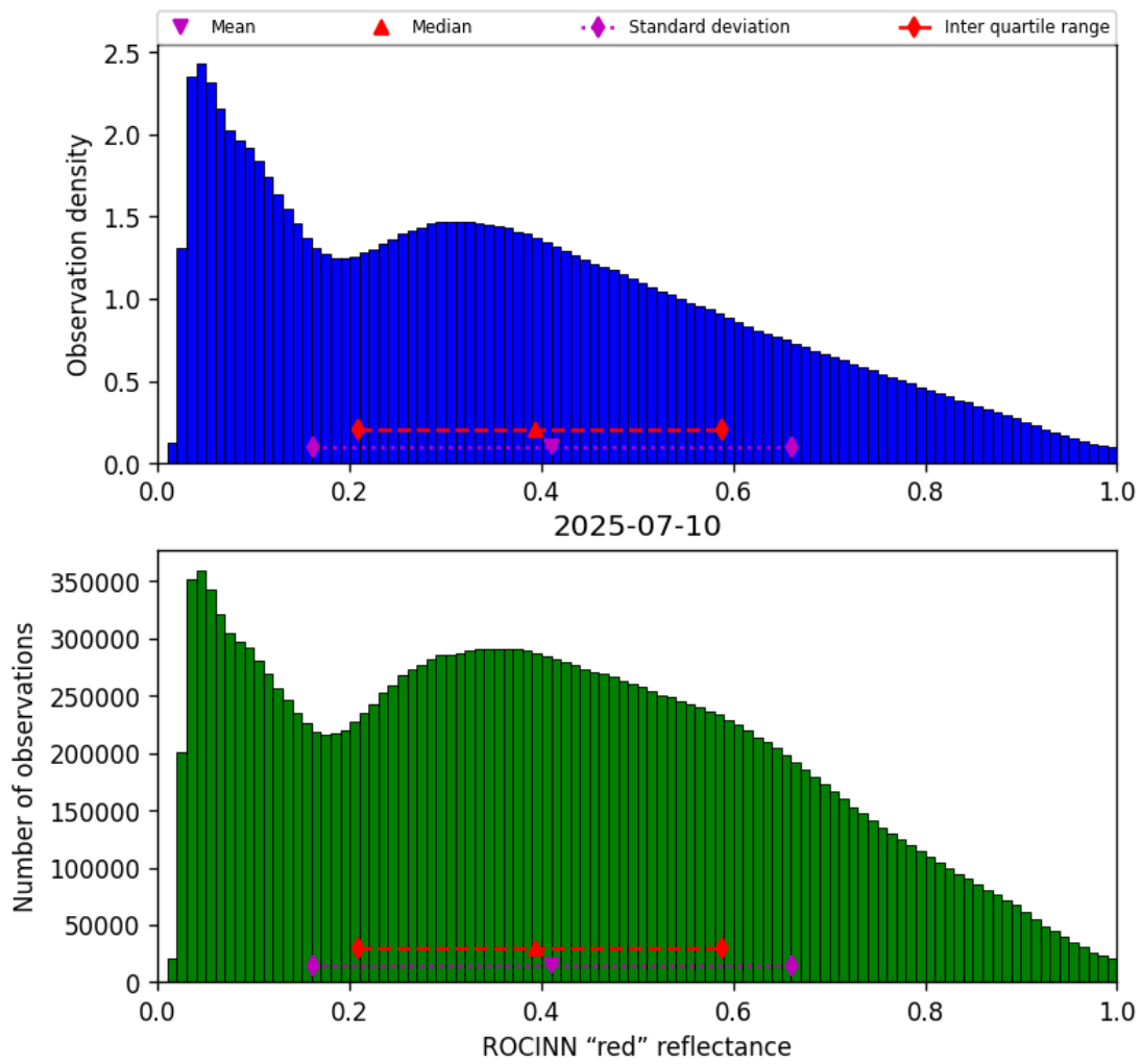
Figure 53: Histogram of “ROCINN “red” reflectance” for 2025-07-09 to 2025-07-11
