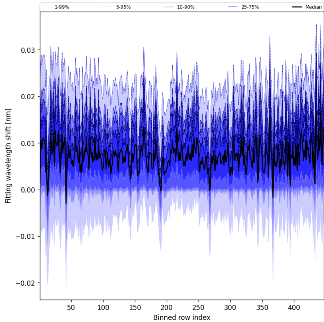
Figure 65: Along track statistics of “Fitting wavelength shift” for 2025-07-09 to 2025-07-11
