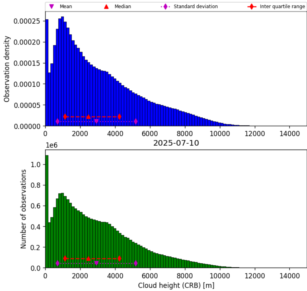
Figure 43: Histogram of “Cloud height (CRB)” for 2025-07-09 to 2025-07-11
