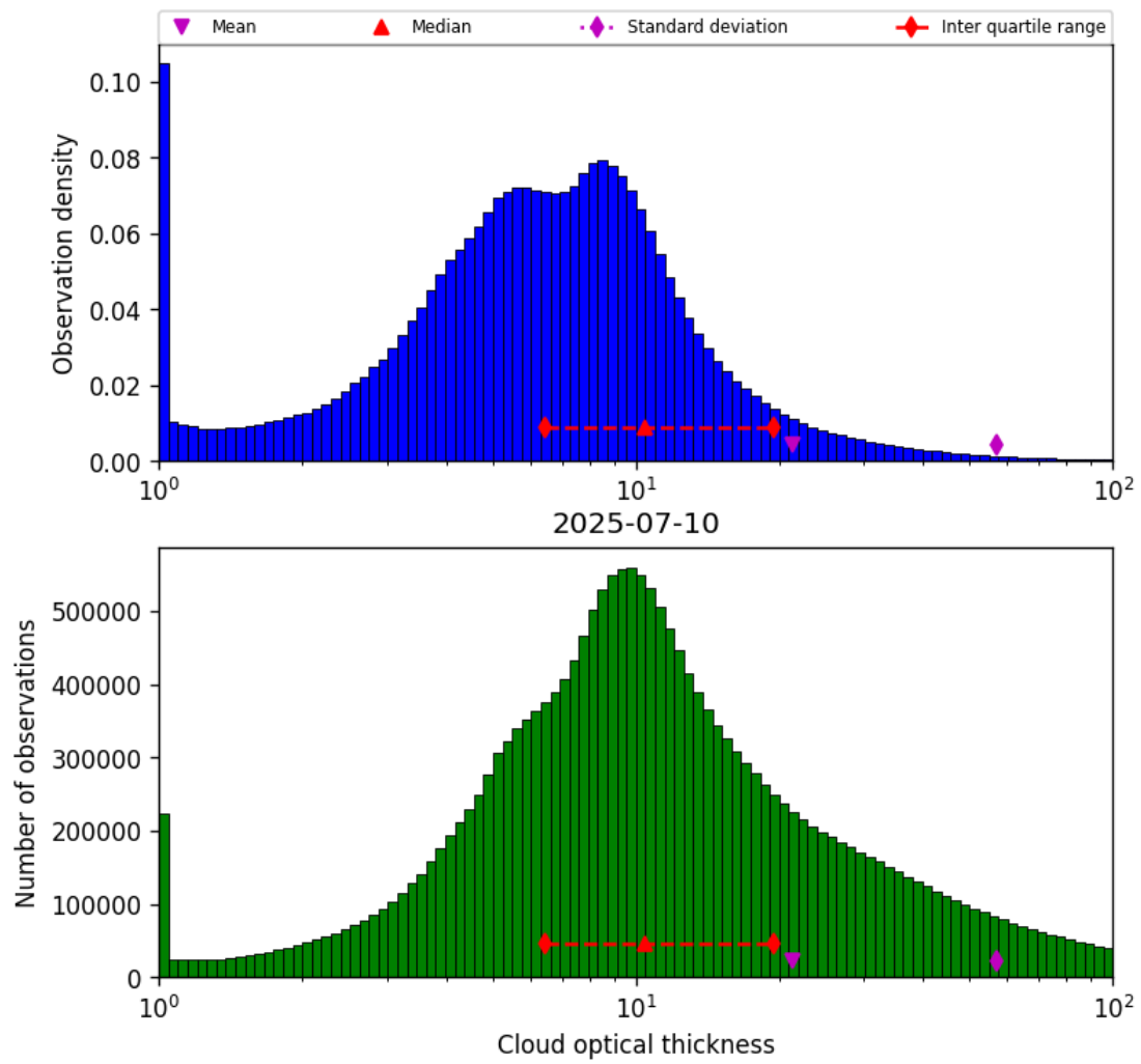
Figure 41: Histogram of “Cloud optical thickness” for 2025-07-09 to 2025-07-11
