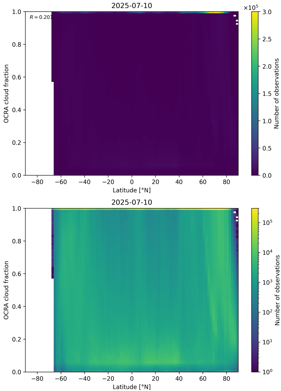
Figure 93: Scatter density plot of “Latitude” against “OCRA cloud fraction” for 2025-07-09 to 2025-07-11.
