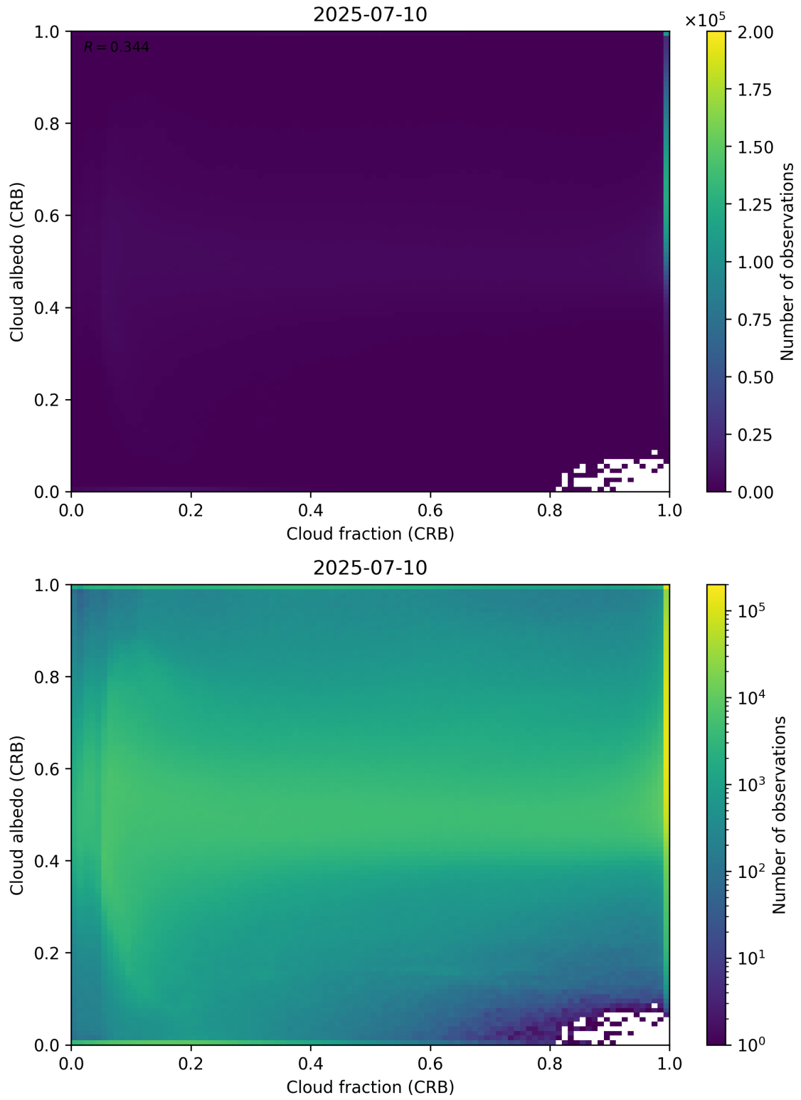
Figure 77: Scatter density plot of “Cloud fraction (CRB)” against “Cloud albedo (CRB)” for 2025-07-09 to 2025-07-11.
