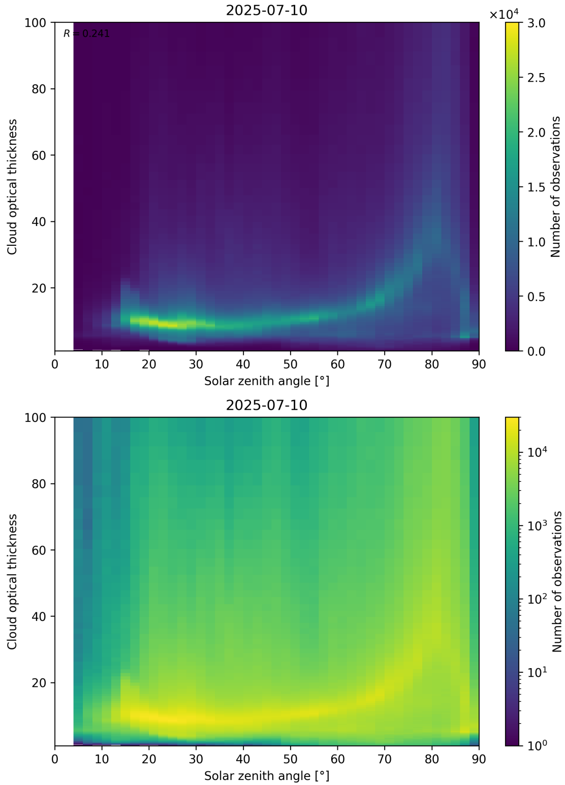
Figure 103: Scatter density plot of “Solar zenith angle” against “Cloud optical thickness” for 2025-07-09 to 2025-07-11.
