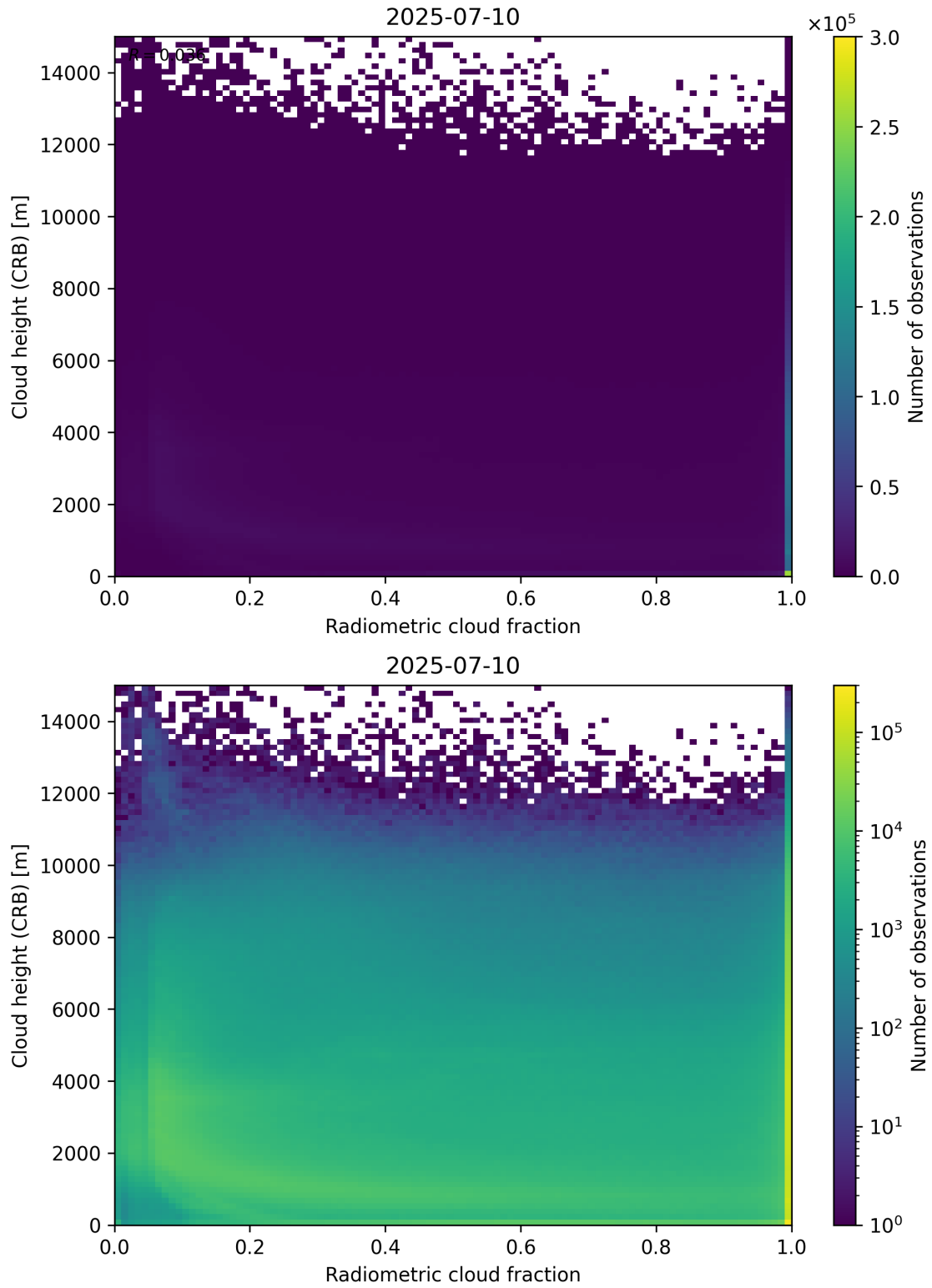
Figure 74: Scatter density plot of “Radiometric cloud fraction” against “Cloud height (CRB)” for 2025-07-09 to 2025-07-11.
