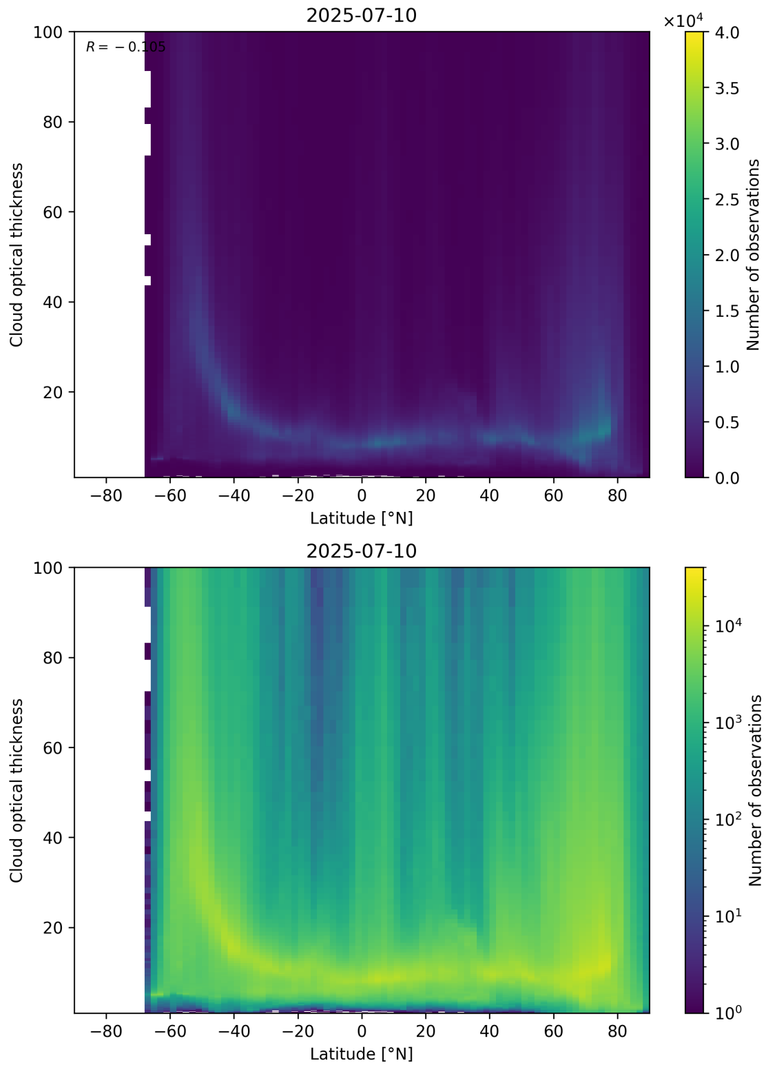
Figure 96: Scatter density plot of “Latitude” against “Cloud optical thickness” for 2025-07-09 to 2025-07-11.
