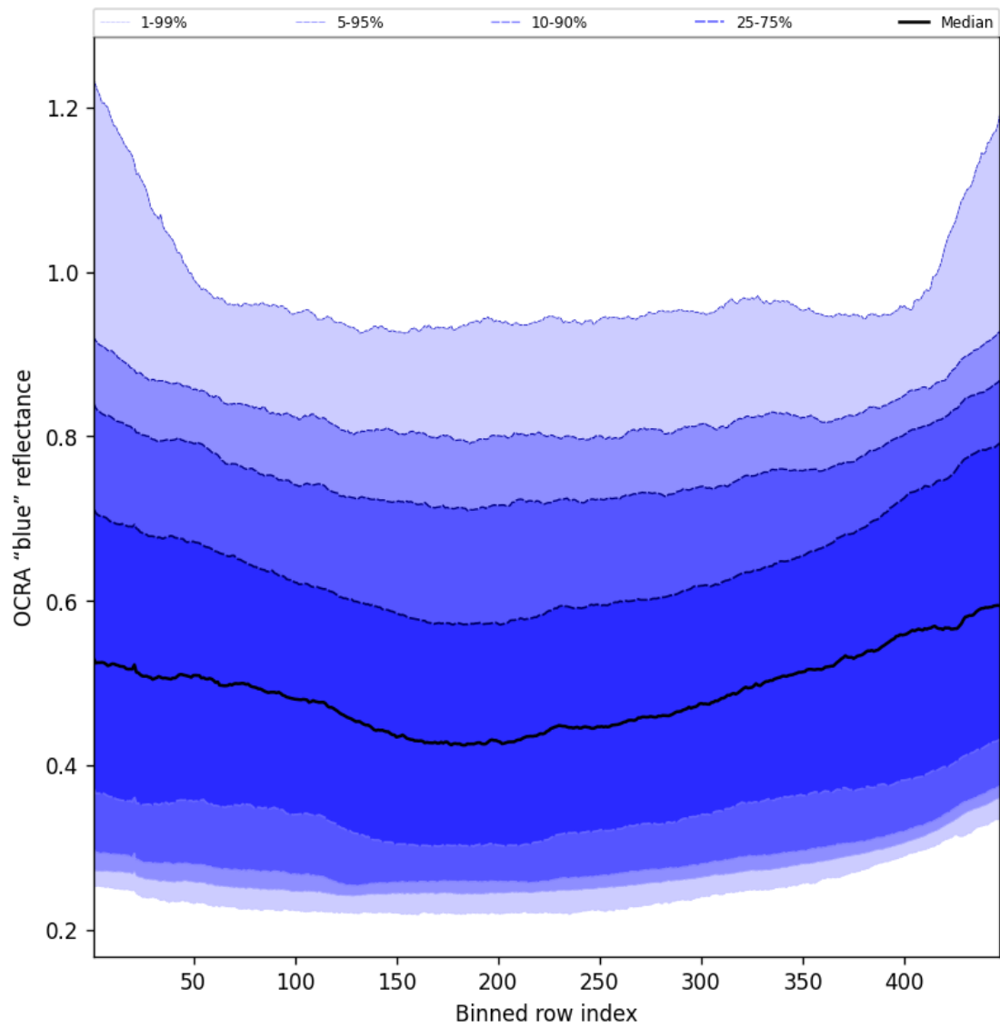
Figure 67: Along track statistics of “OCRA “blue” reflectance” for 2025-07-09 to 2025-07-11
