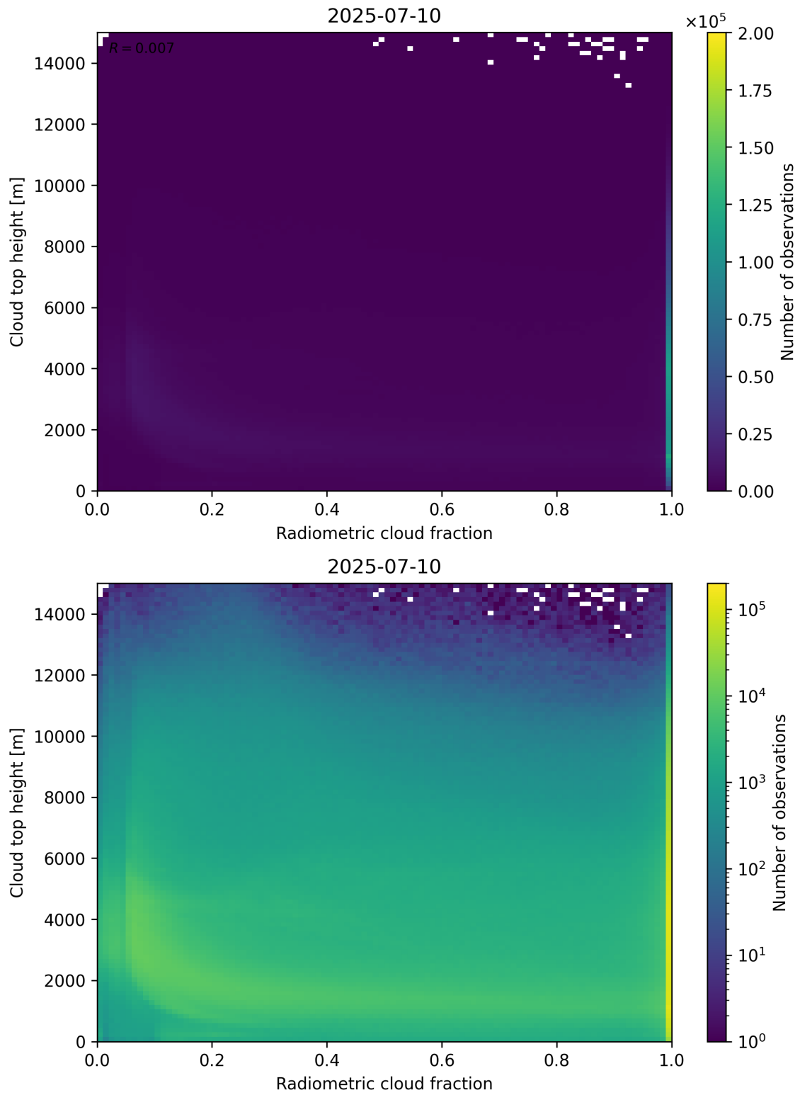
Figure 76: Scatter density plot of “Radiometric cloud fraction” against “Cloud top height” for 2025-07-09 to 2025-07-11.
