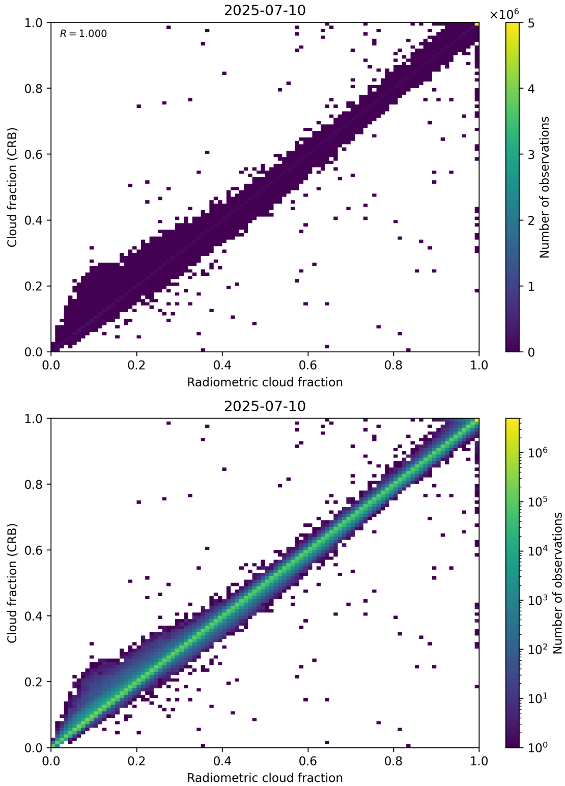
Figure 73: Scatter density plot of “Radiometric cloud fraction” against “Cloud fraction (CRB)” for 2025-07-09 to 2025-07-11.
