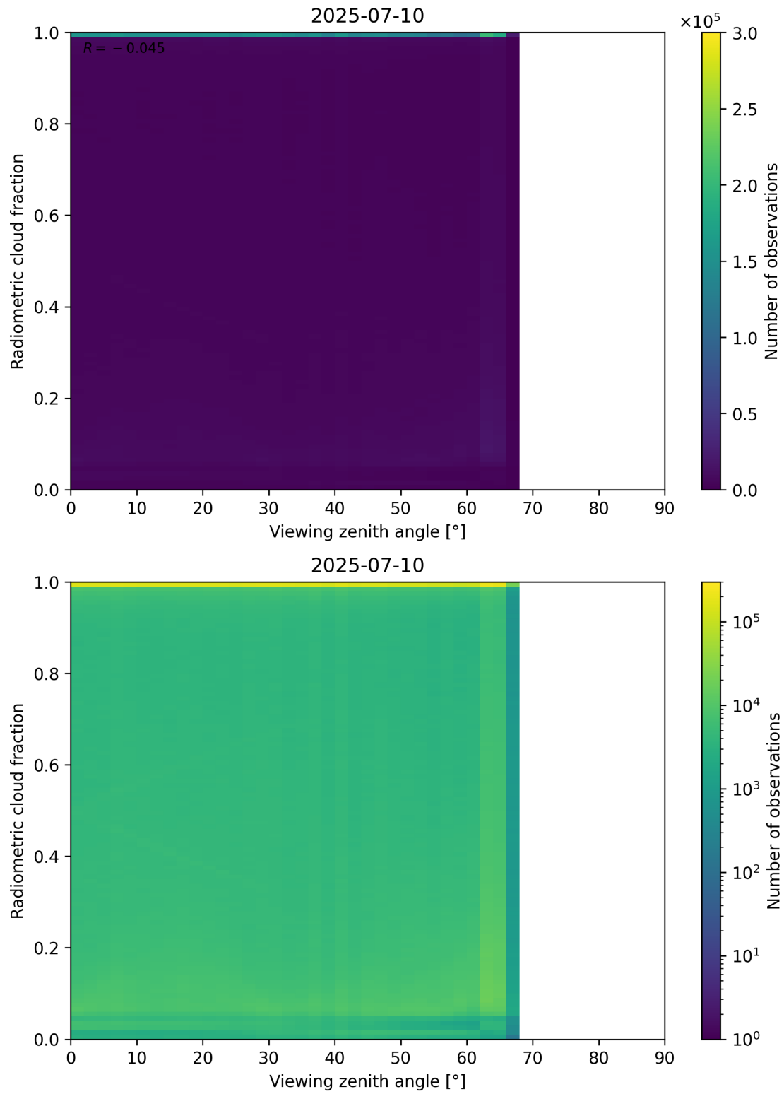
Figure 107: Scatter density plot of “Viewing zenith angle” against “Radiometric cloud fraction” for 2025-07-09 to 2025-07-11.
