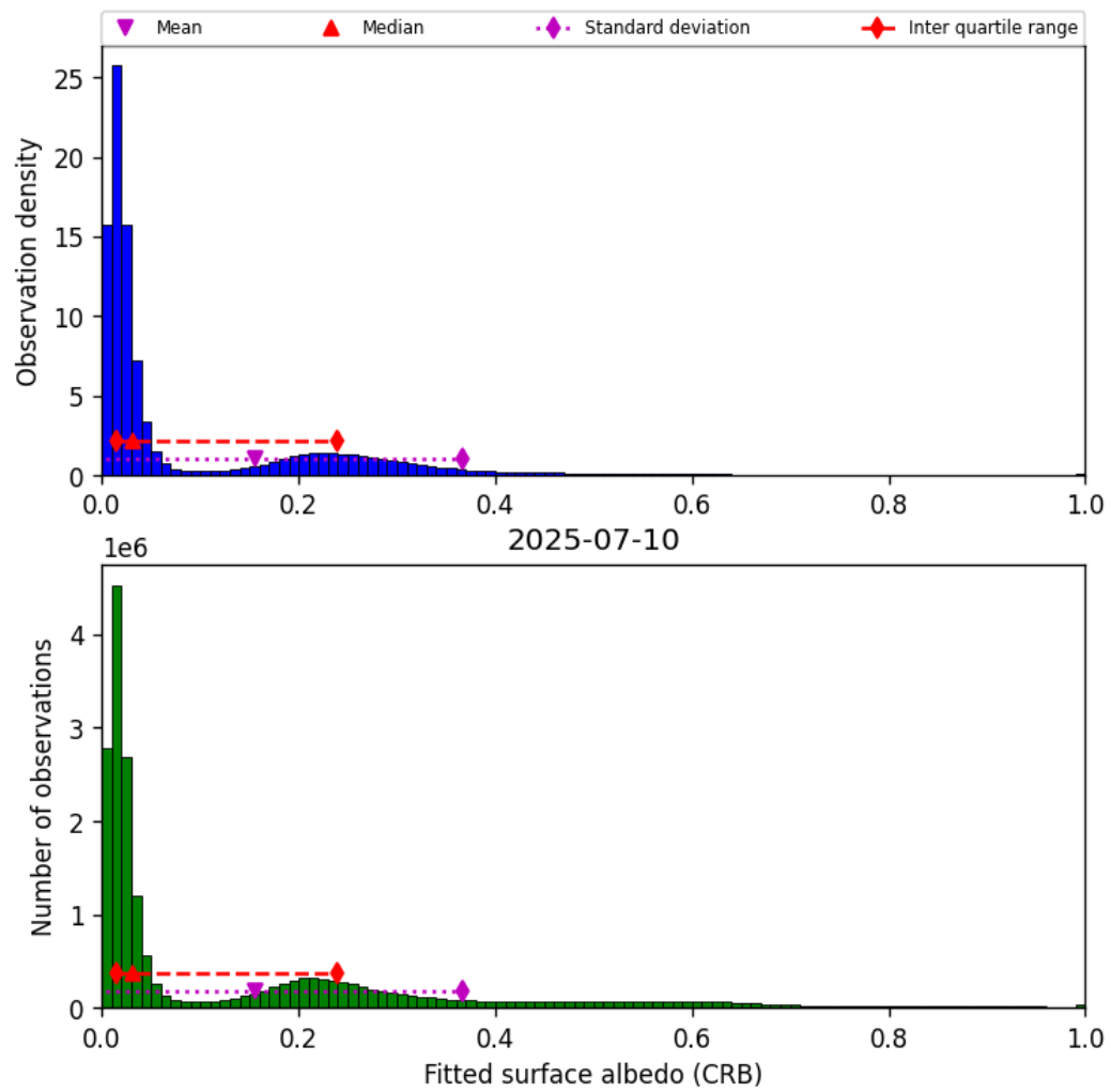
Figure 46: Histogram of “Fitted surface albedo (CRB)” for 2025-07-09 to 2025-07-11
