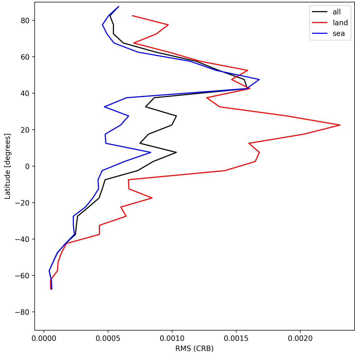
Figure 32: Zonal average of “RMS (CRB)” for 2025-07-09 to 2025-07-11.
