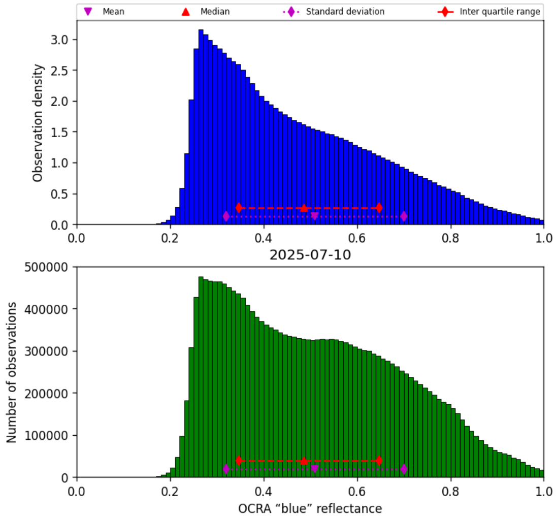
Figure 51: Histogram of “OCRA “blue” reflectance” for 2025-07-09 to 2025-07-11
