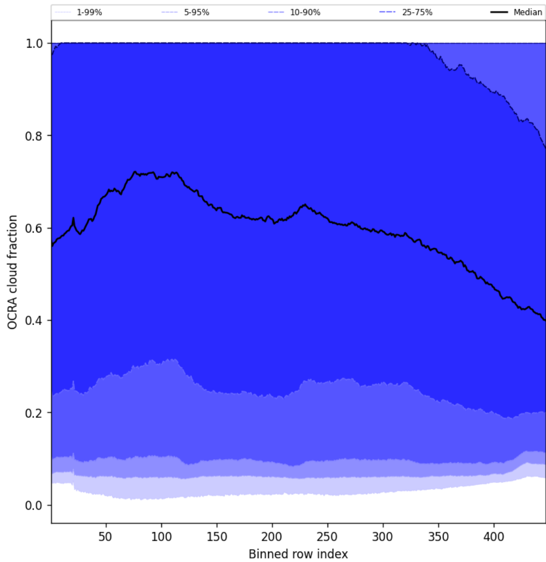
Figure 66: Along track statistics of “OCRA cloud fraction” for 2025-07-09 to 2025-07-11
