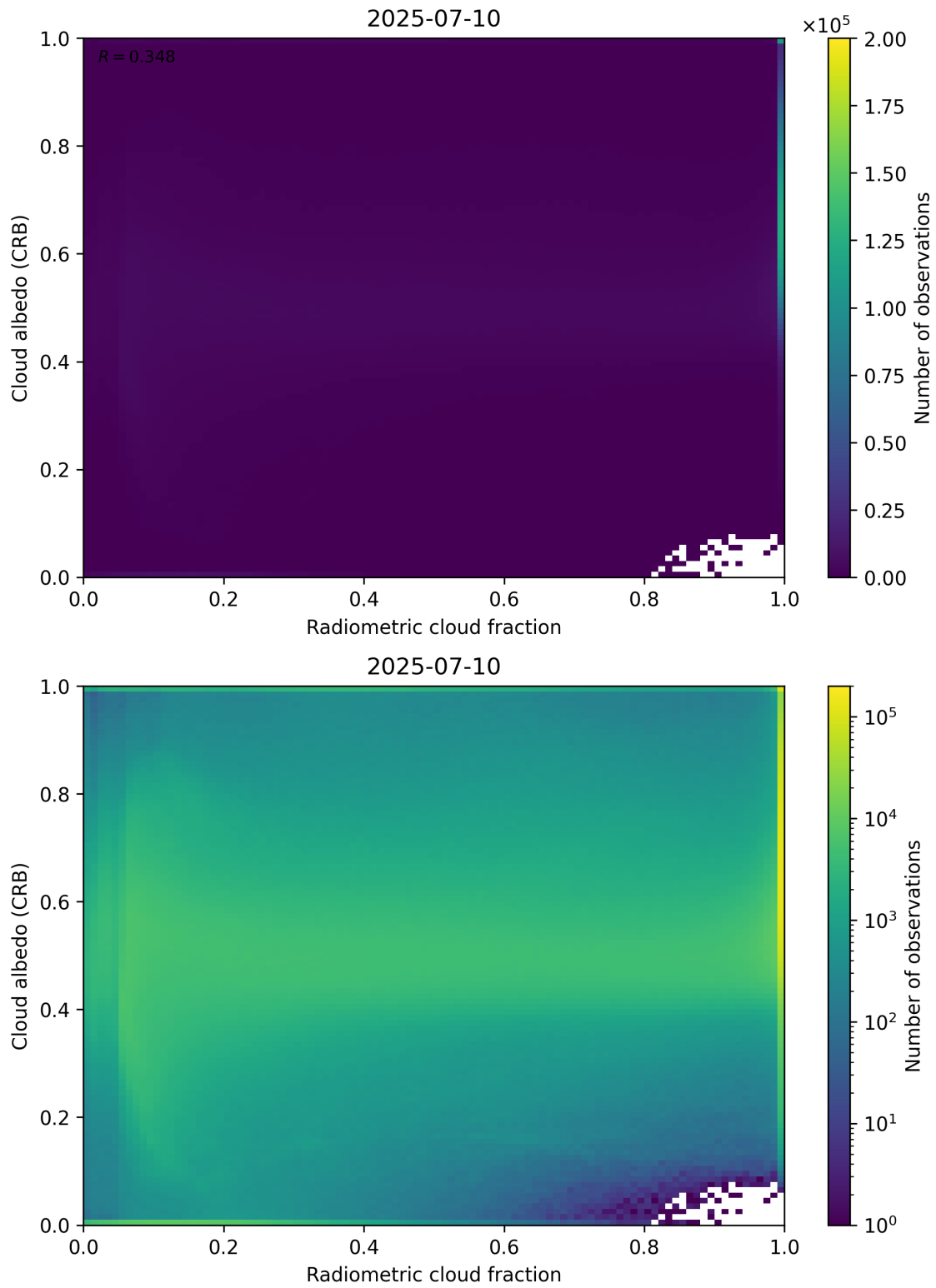
Figure 71: Scatter density plot of “Radiometric cloud fraction” against “Cloud albedo (CRB)” for 2025-07-09 to 2025-07-11.
