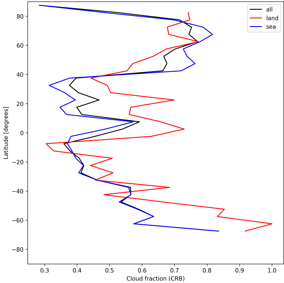
Figure 26: Zonal average of “Cloud fraction (CRB)” for 2025-07-09 to 2025-07-11.
