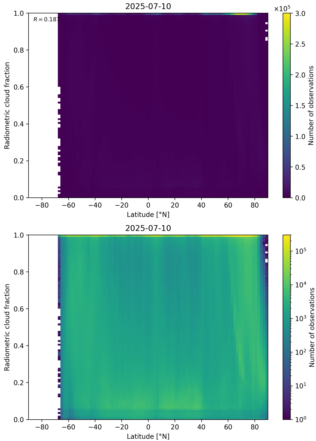
Figure 92: Scatter density plot of “Latitude” against “Radiometric cloud fraction” for 2025-07-09 to 2025-07-11.
