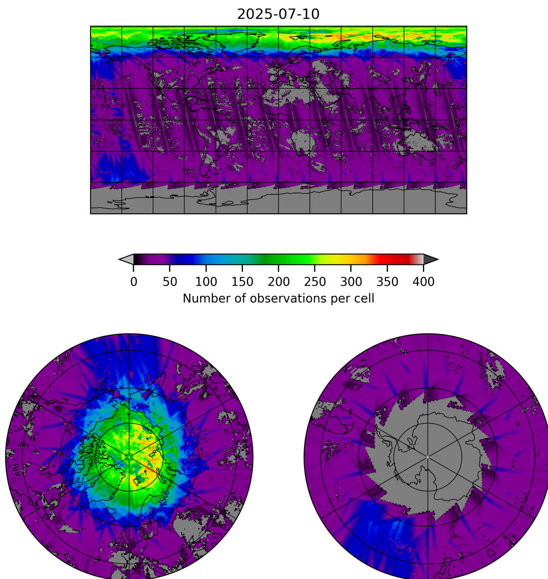
Figure 21: Map of the number of observations for 2025-07-09 to 2025-07-11
