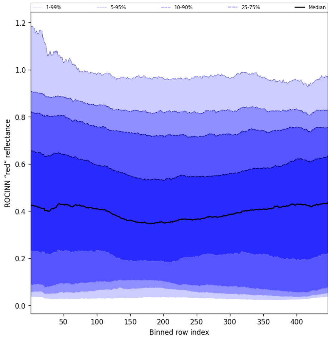
Figure 69: Along track statistics of “ROCINN “red” reflectance” for 2025-07-09 to 2025-07-11
