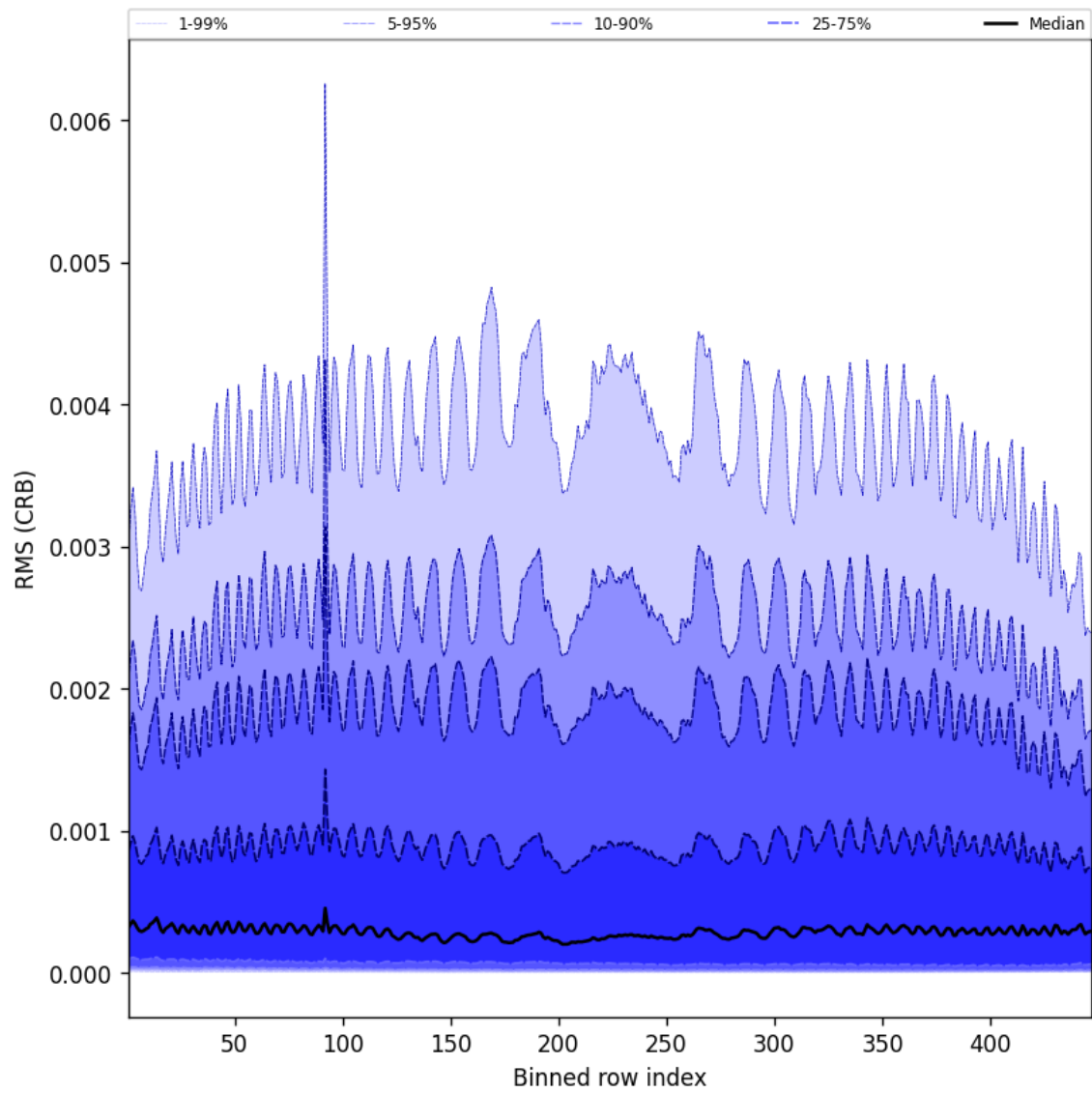
Figure 64: Along track statistics of “RMS (CRB)” for 2025-07-09 to 2025-07-11
