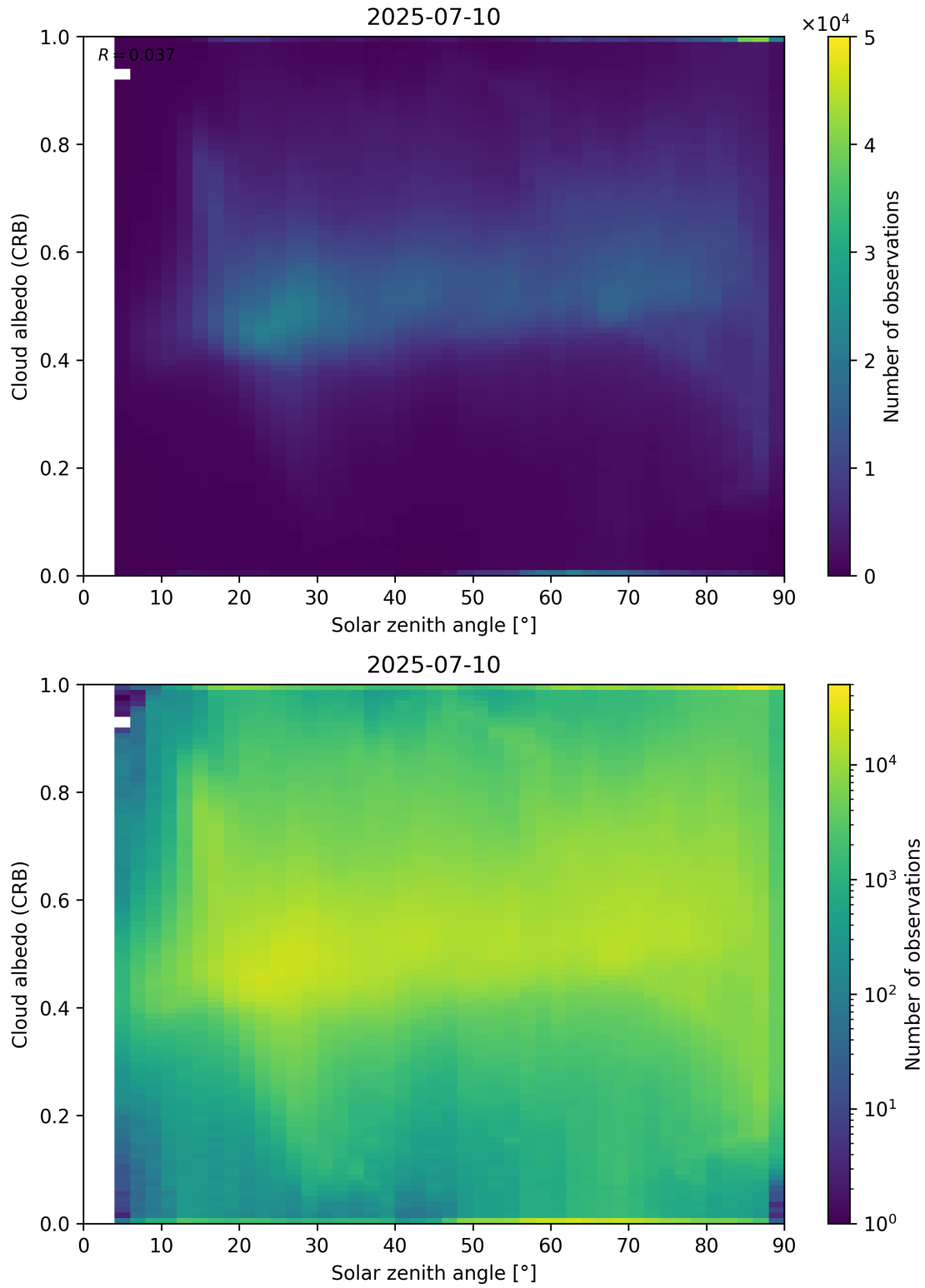
Figure 98: Scatter density plot of “Solar zenith angle” against “Cloud albedo (CRB)” for 2025-07-09 to 2025-07-11.
