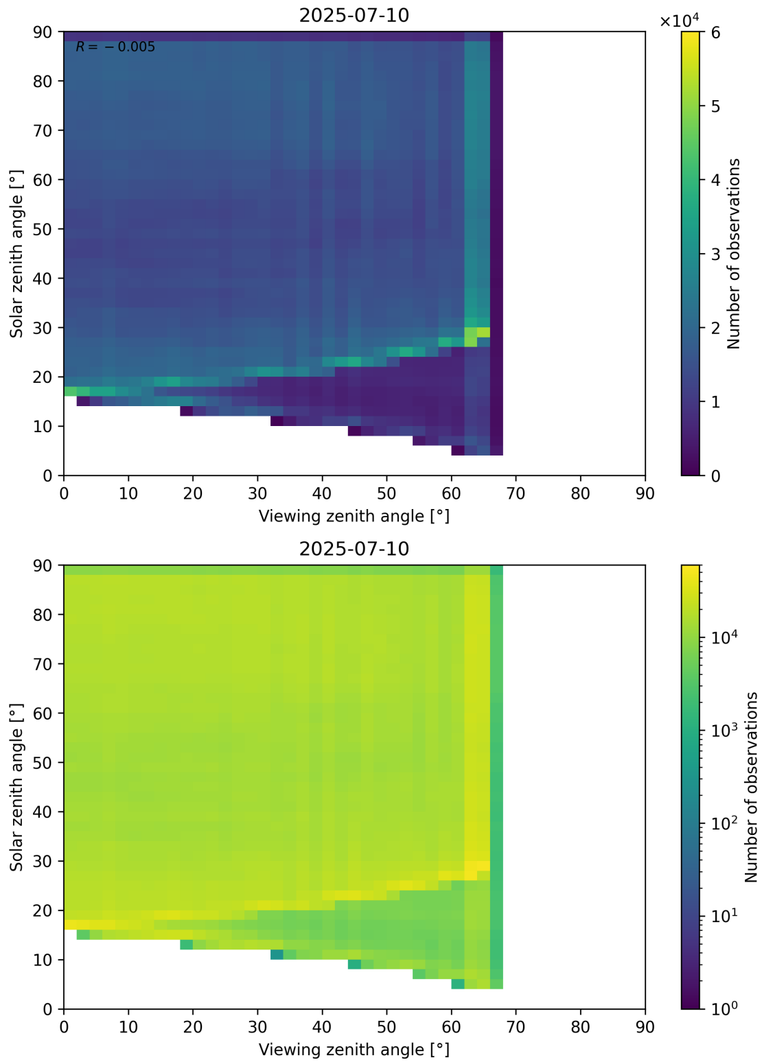
Figure 114: Scatter density plot of “Viewing zenith angle” against “Solar zenith angle” for 2025-07-09 to 2025-07-11.
