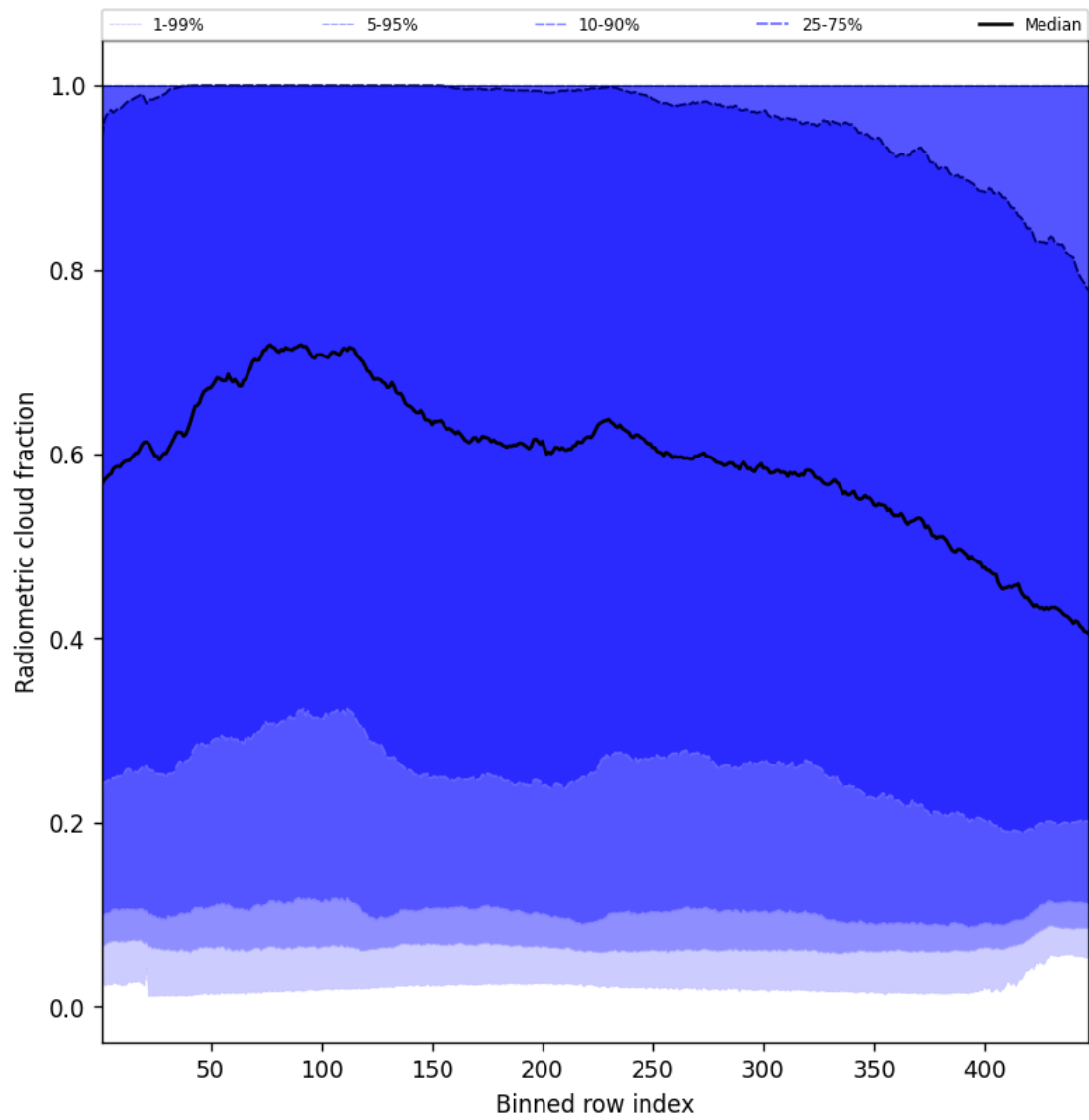
Figure 55: Along track statistics of “Radiometric cloud fraction” for 2025-07-09 to 2025-07-11
