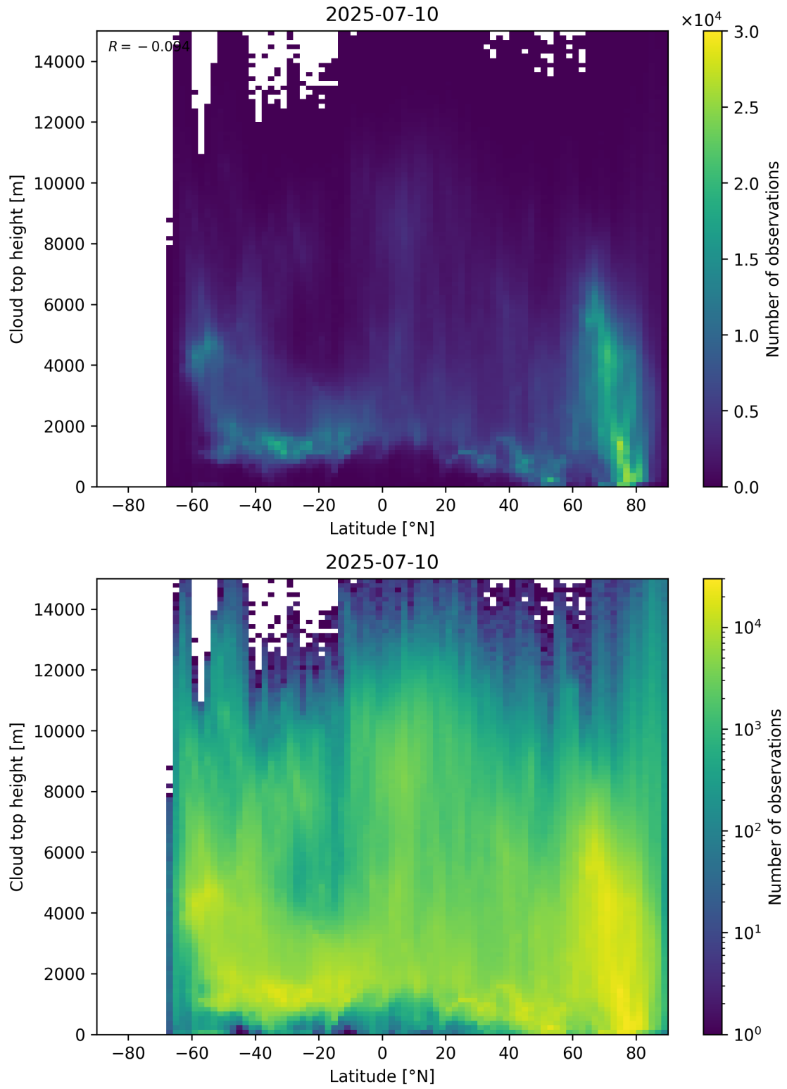
Figure 97: Scatter density plot of “Latitude” against “Cloud top height” for 2025-07-09 to 2025-07-11.
