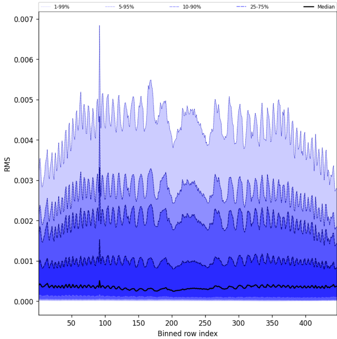
Figure 63: Along track statistics of “RMS” for 2025-07-09 to 2025-07-11
