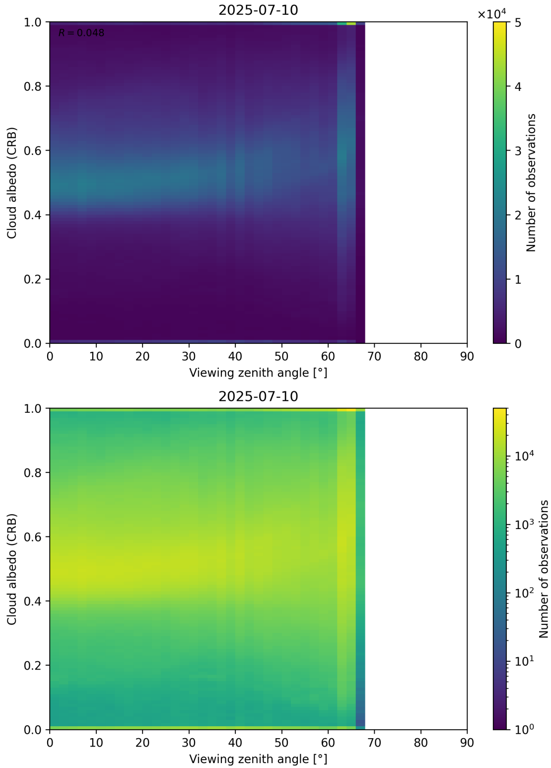
Figure 106: Scatter density plot of “Viewing zenith angle” against “Cloud albedo (CRB)” for 2025-07-09 to 2025-07-11.
