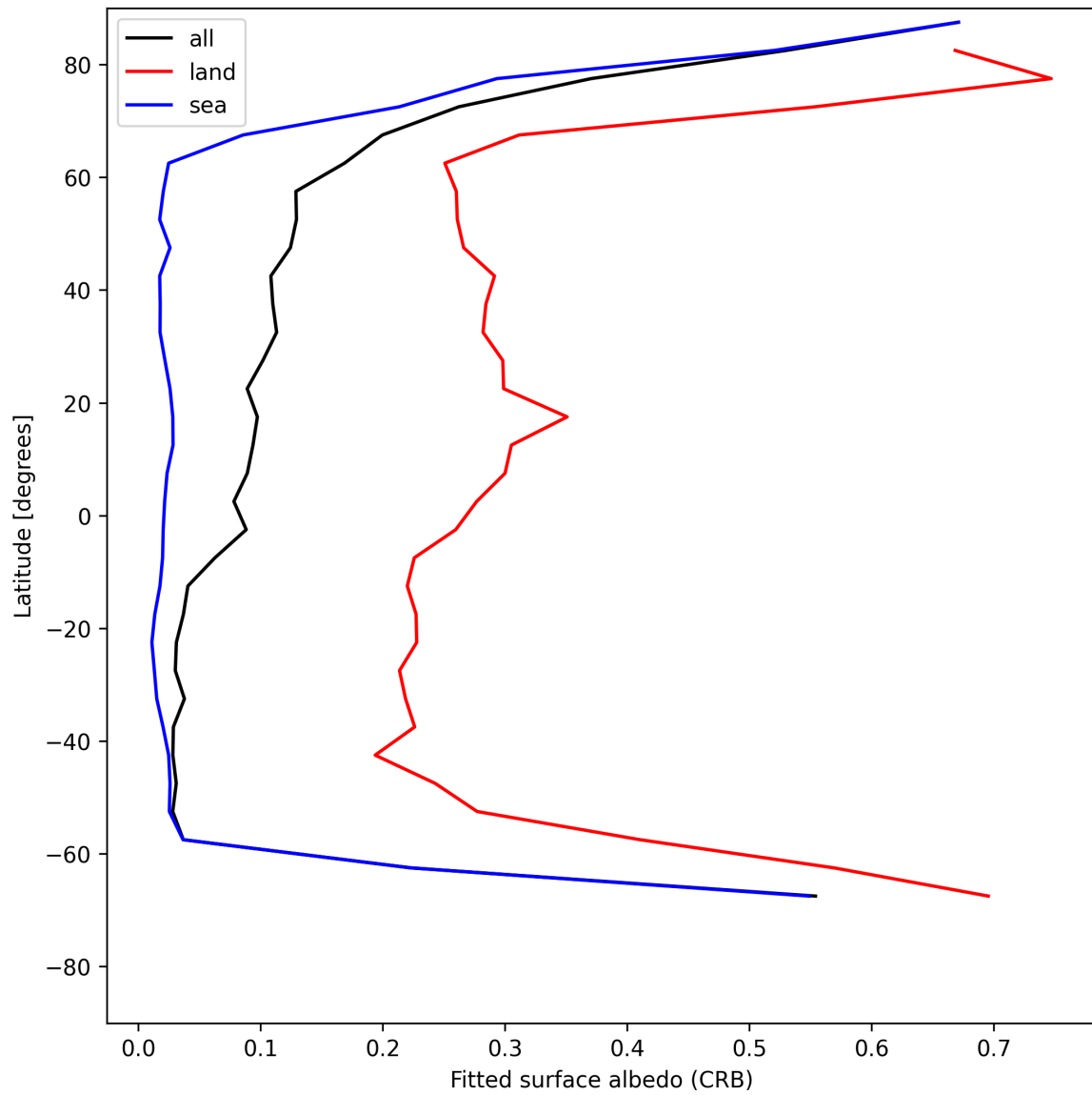
Figure 30: Zonal average of “Fitted surface albedo (CRB)” for 2025-07-09 to 2025-07-11.
