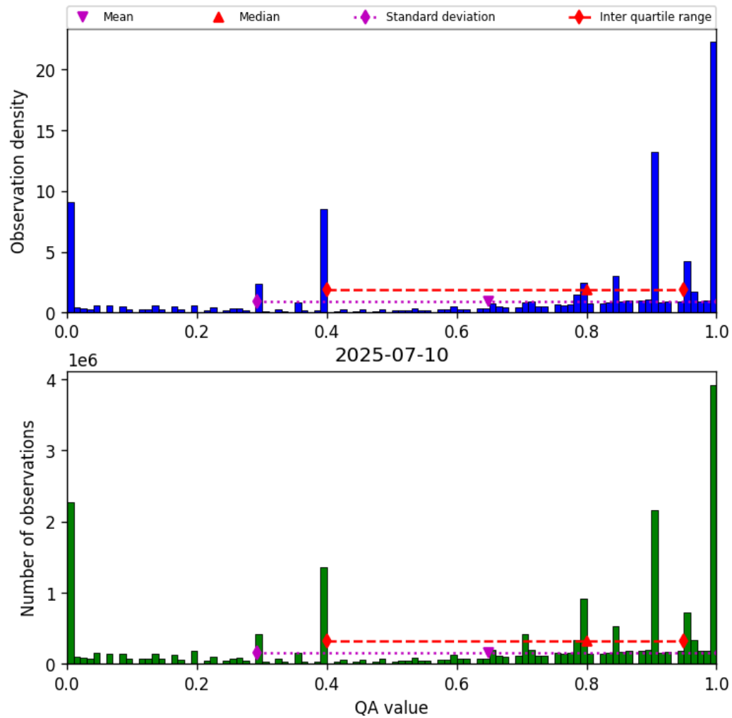
Figure 38: Histogram of “QA value” for 2025-07-09 to 2025-07-11
