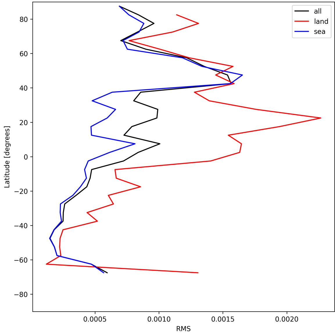
Figure 31: Zonal average of “RMS” for 2025-07-09 to 2025-07-11.
