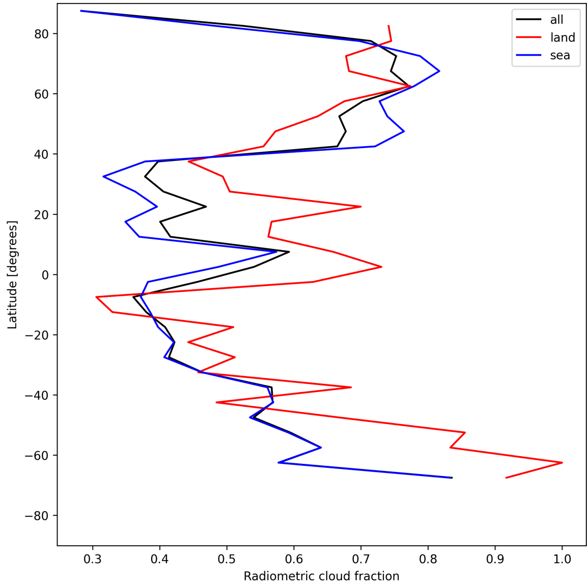
Figure 23: Zonal average of “Radiometric cloud fraction” for 2025-07-09 to 2025-07-11.
