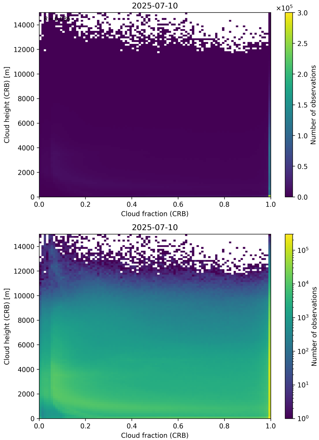
Figure 79: Scatter density plot of “Cloud fraction (CRB)” against “Cloud height (CRB)” for 2025-07-09 to 2025-07-11.
