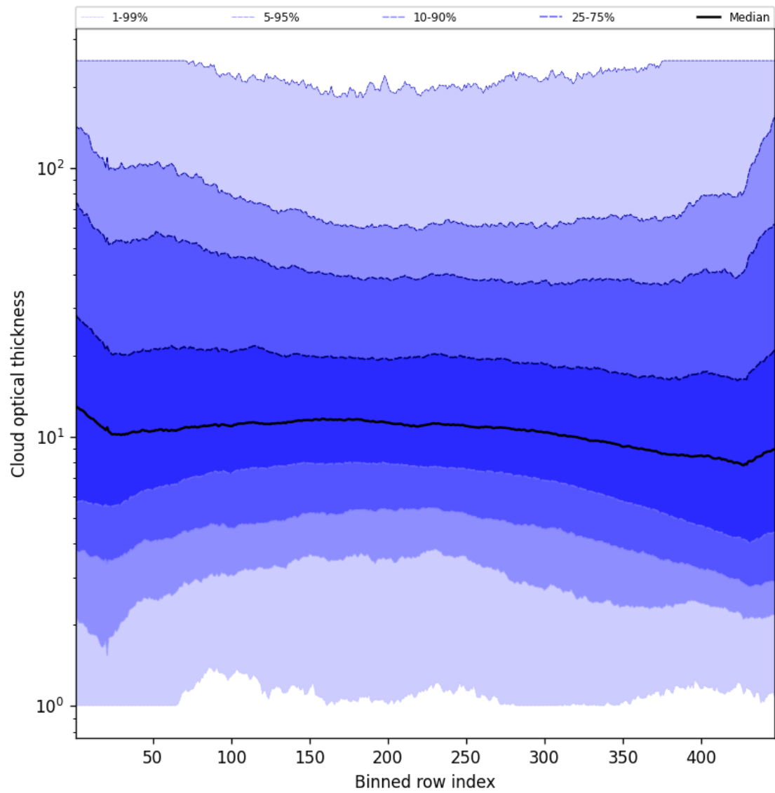
Figure 57: Along track statistics of “Cloud optical thickness” for 2025-07-09 to 2025-07-11
