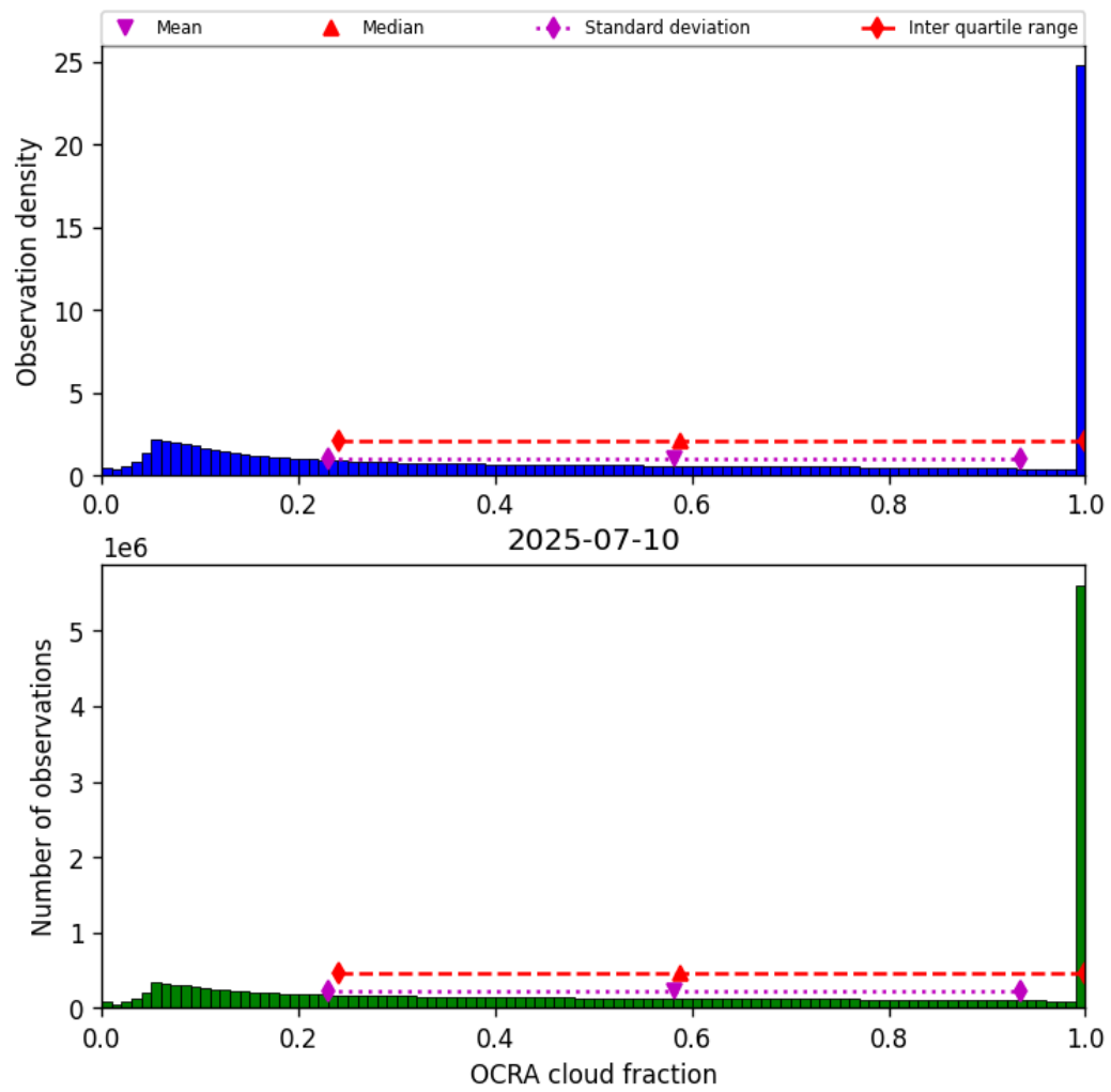
Figure 50: Histogram of “OCRA cloud fraction” for 2025-07-09 to 2025-07-11
