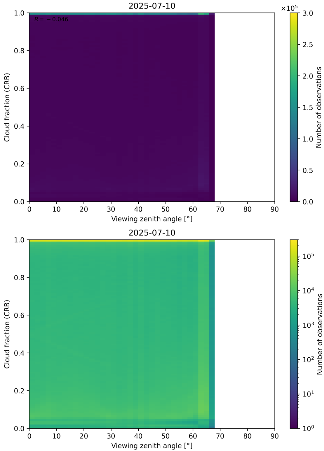
Figure 109: Scatter density plot of “Viewing zenith angle” against “Cloud fraction (CRB)” for 2025-07-09 to 2025-07-11.
