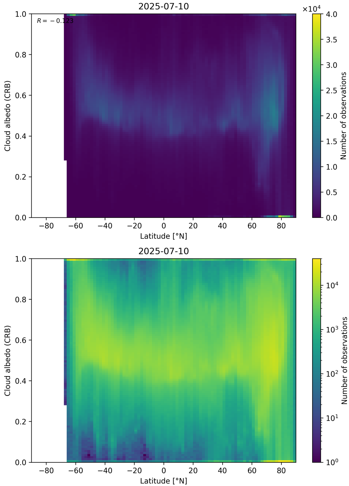
Figure 91: Scatter density plot of “Latitude” against “Cloud albedo (CRB)” for 2025-07-09 to 2025-07-11.
