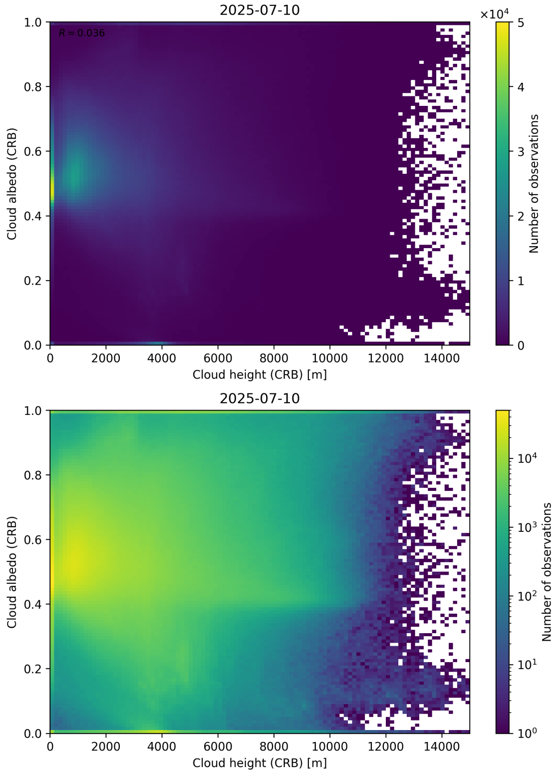
Figure 80: Scatter density plot of “Cloud height (CRB)” against “Cloud albedo (CRB)” for 2025-07-09 to 2025-07-11.
