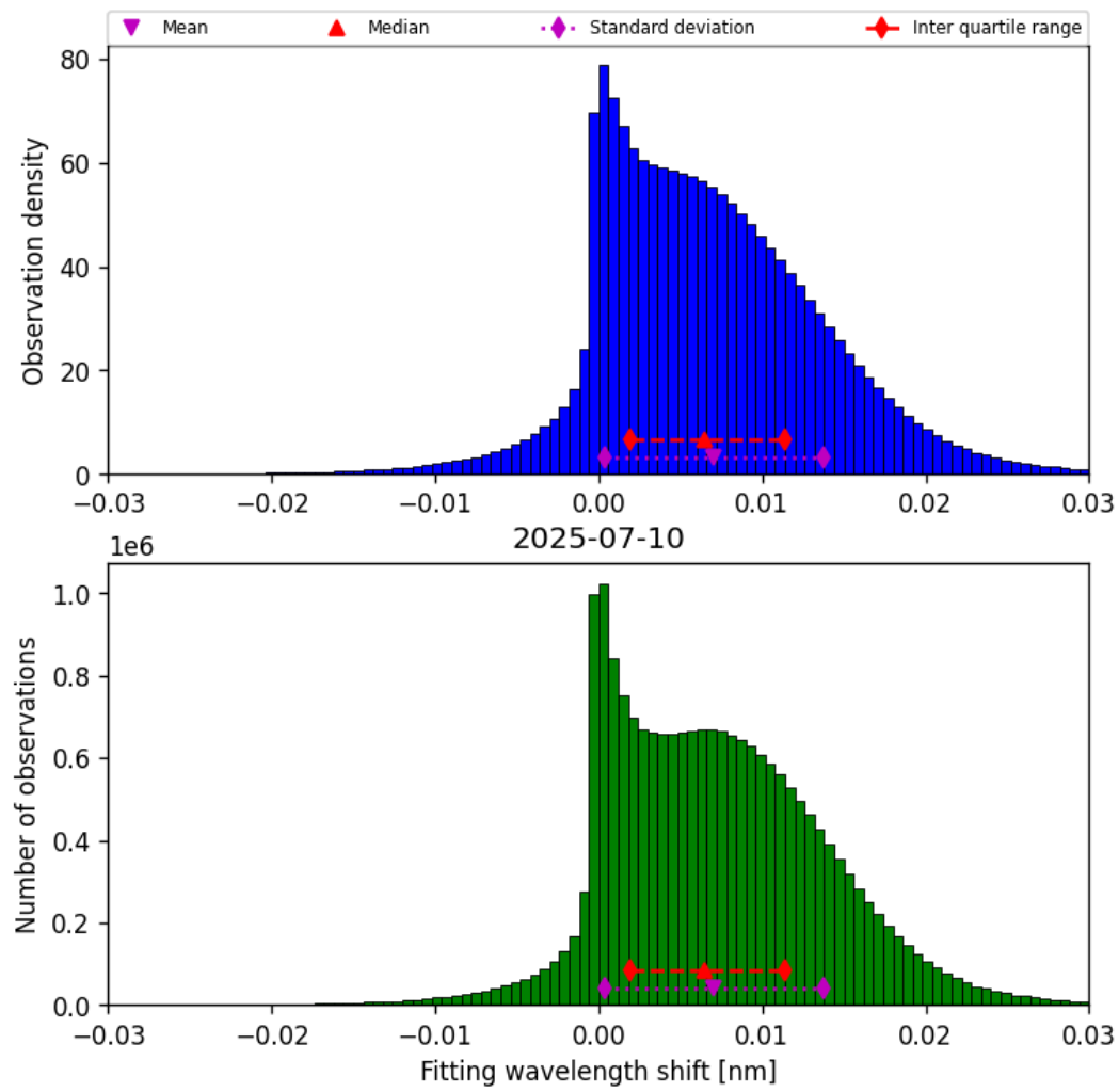
Figure 49: Histogram of “Fitting wavelength shift” for 2025-07-09 to 2025-07-11
