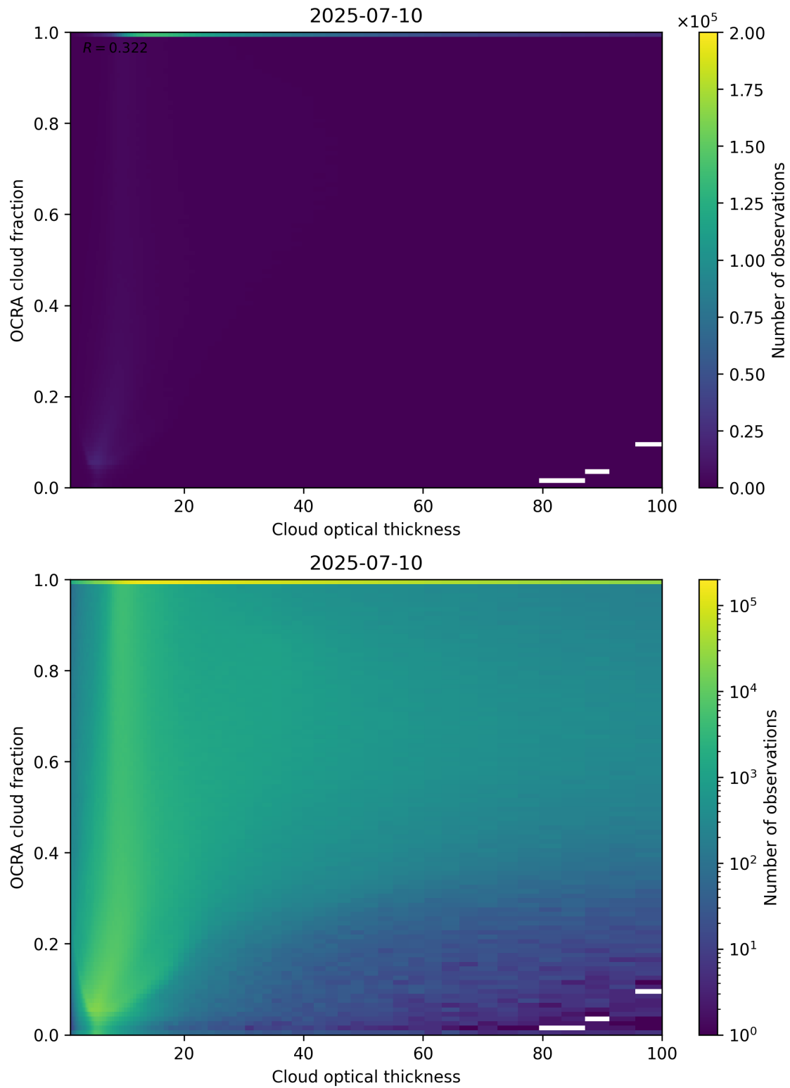
Figure 83: Scatter density plot of “Cloud optical thickness” against “OCRA cloud fraction” for 2025-07-09 to 2025-07-11.
