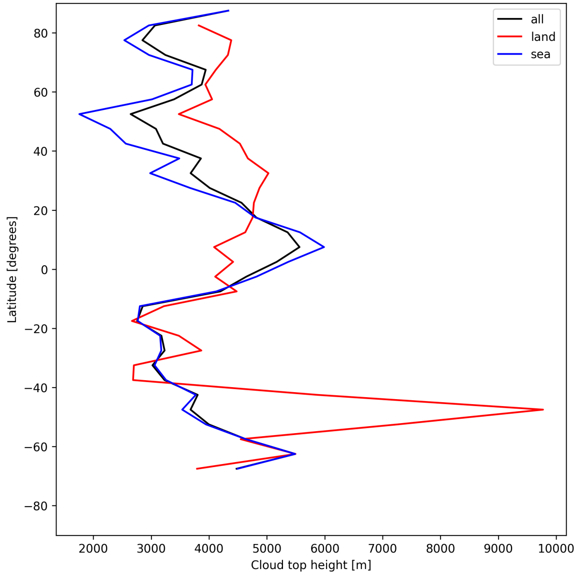
Figure 24: Zonal average of “Cloud top height” for 2025-07-09 to 2025-07-11.
