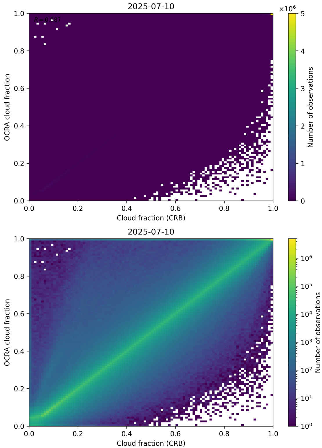
Figure 78: Scatter density plot of “Cloud fraction (CRB)” against “OCRA cloud fraction” for 2025-07-09 to 2025-07-11.
