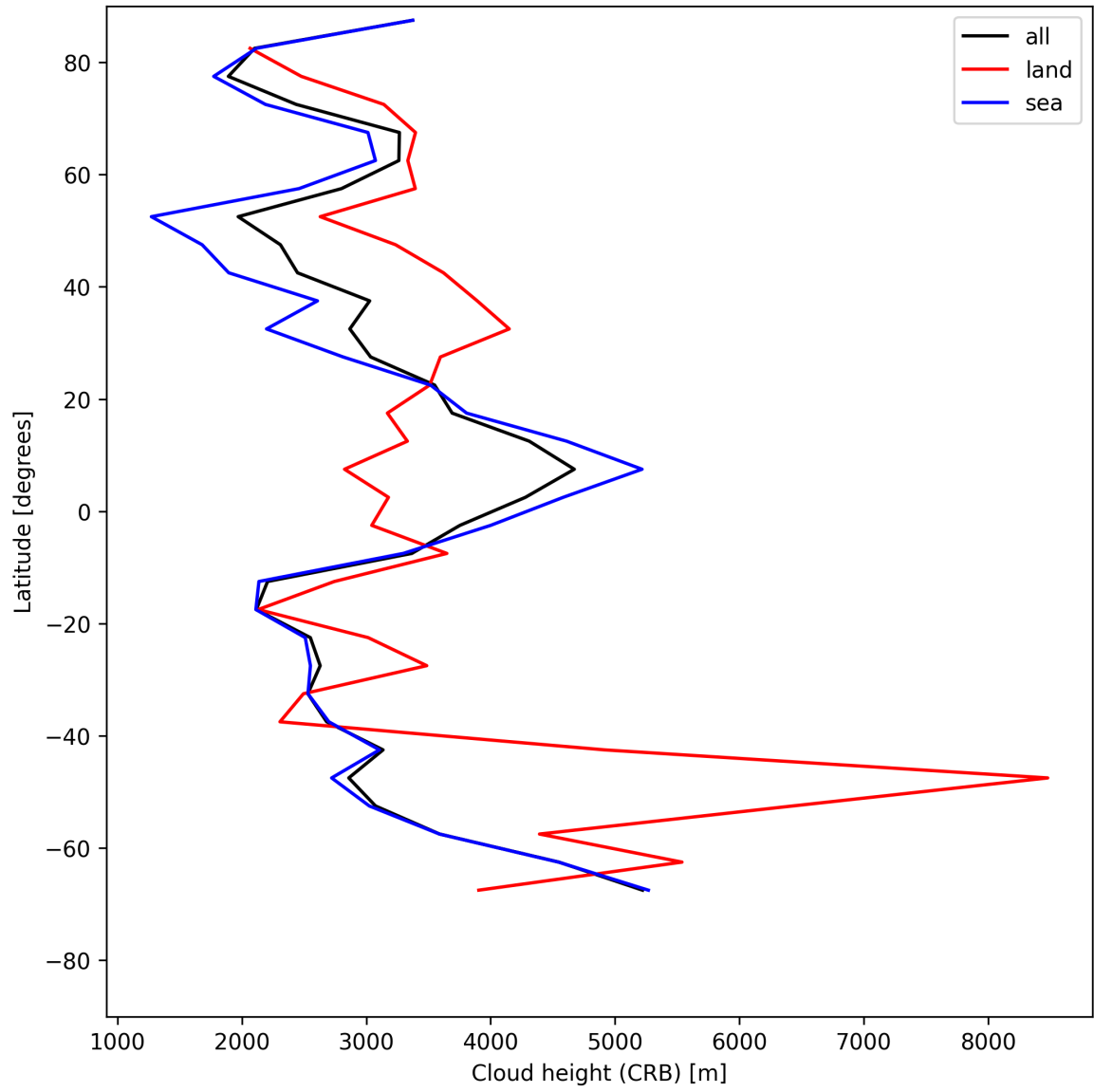
Figure 27: Zonal average of “Cloud height (CRB)” for 2025-07-09 to 2025-07-11.
