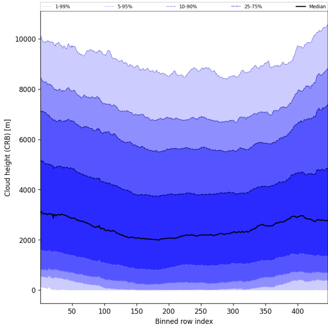
Figure 59: Along track statistics of “Cloud height (CRB)” for 2025-07-09 to 2025-07-11
