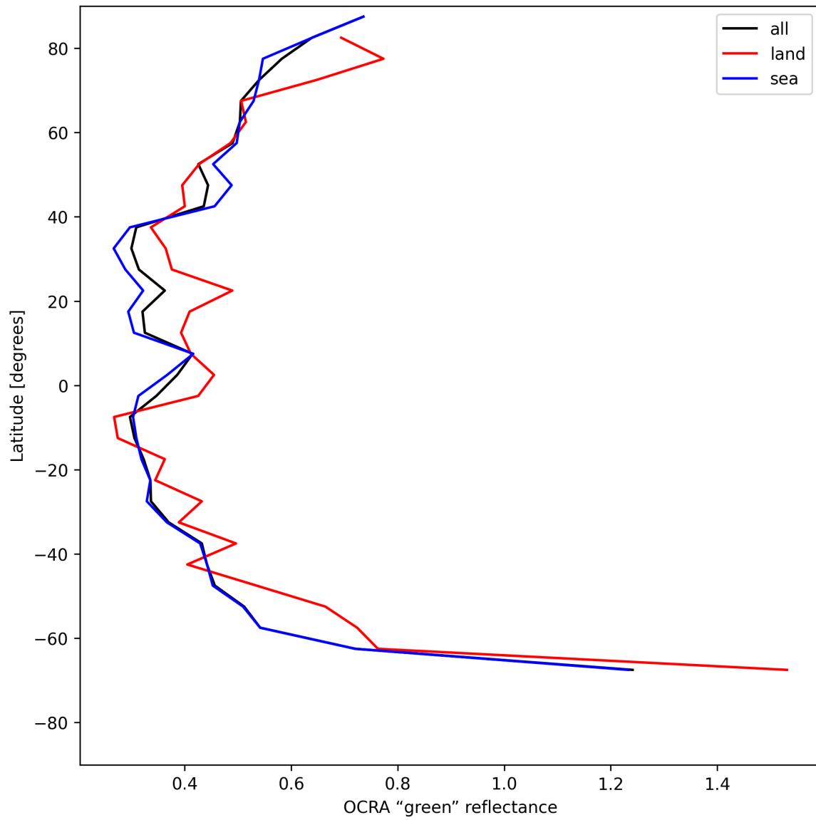
Figure 36: Zonal average of “OCRA “green” reflectance” for 2025-07-09 to 2025-07-11.
