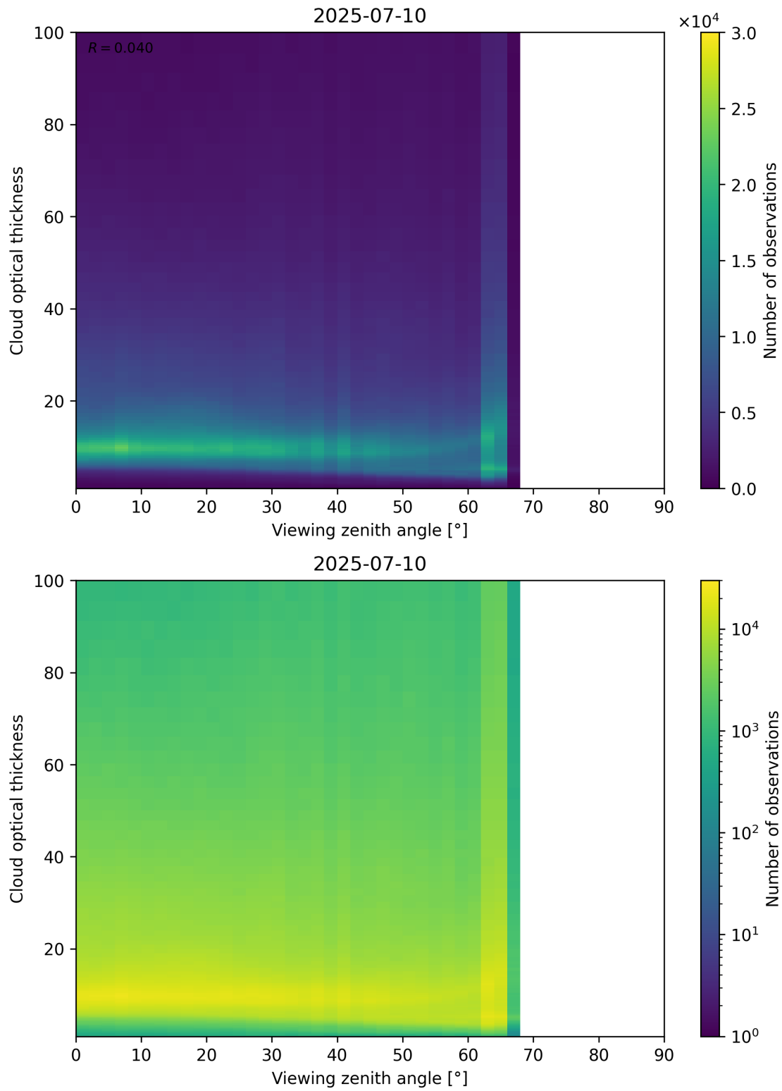
Figure 111: Scatter density plot of “Viewing zenith angle” against “Cloud optical thickness” for 2025-07-09 to 2025-07-11.
