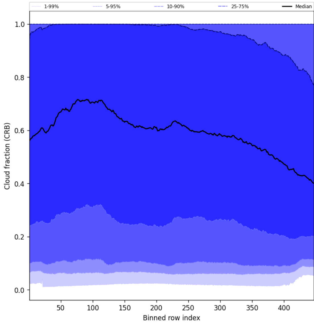
Figure 58: Along track statistics of “Cloud fraction (CRB)” for 2025-07-09 to 2025-07-11
