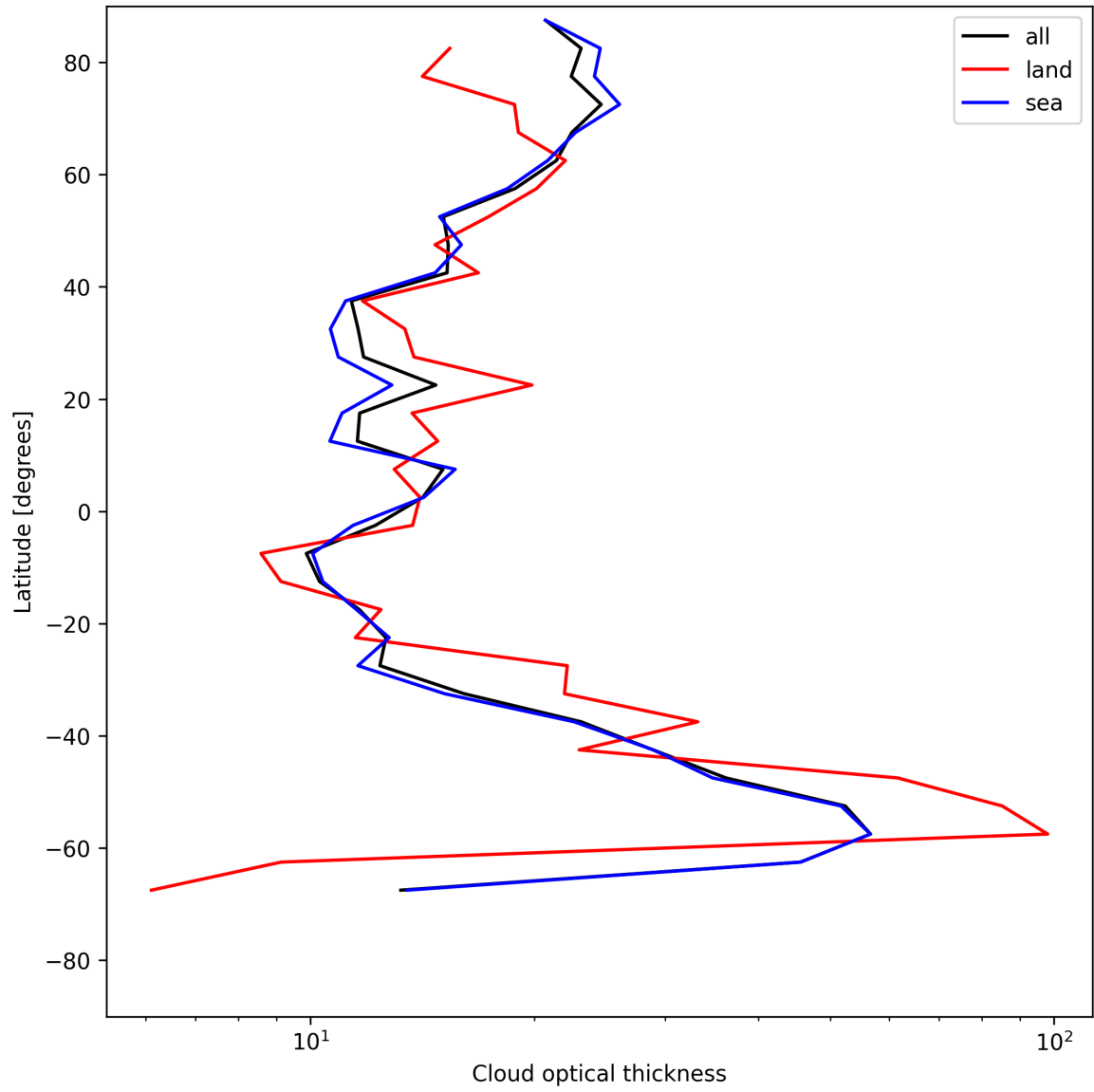
Figure 25: Zonal average of “Cloud optical thickness” for 2025-07-09 to 2025-07-11.
