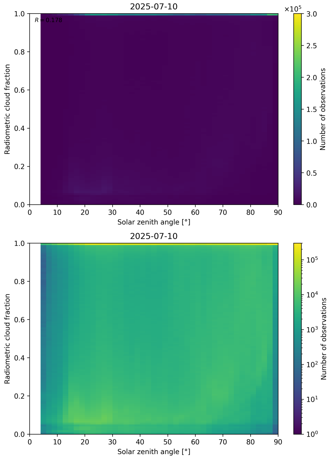
Figure 99: Scatter density plot of “Solar zenith angle” against “Radiometric cloud fraction” for 2025-07-09 to 2025-07-11.
