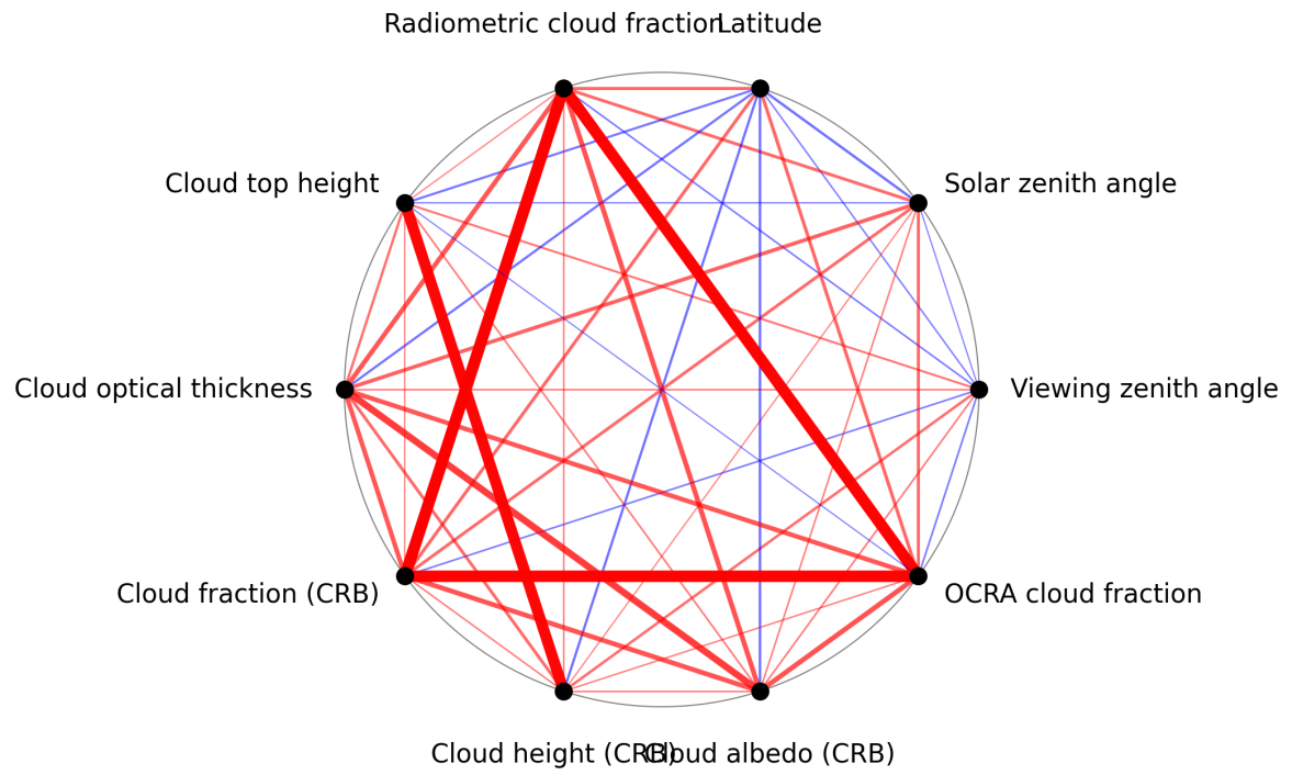
Figure 1: Map of correlation graph for 2025-07-09 to 2025-07-11.
