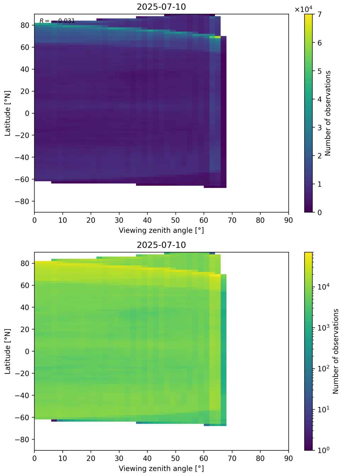
Figure 113: Scatter density plot of “Viewing zenith angle” against “Latitude” for 2025-07-09 to 2025-07-11.
