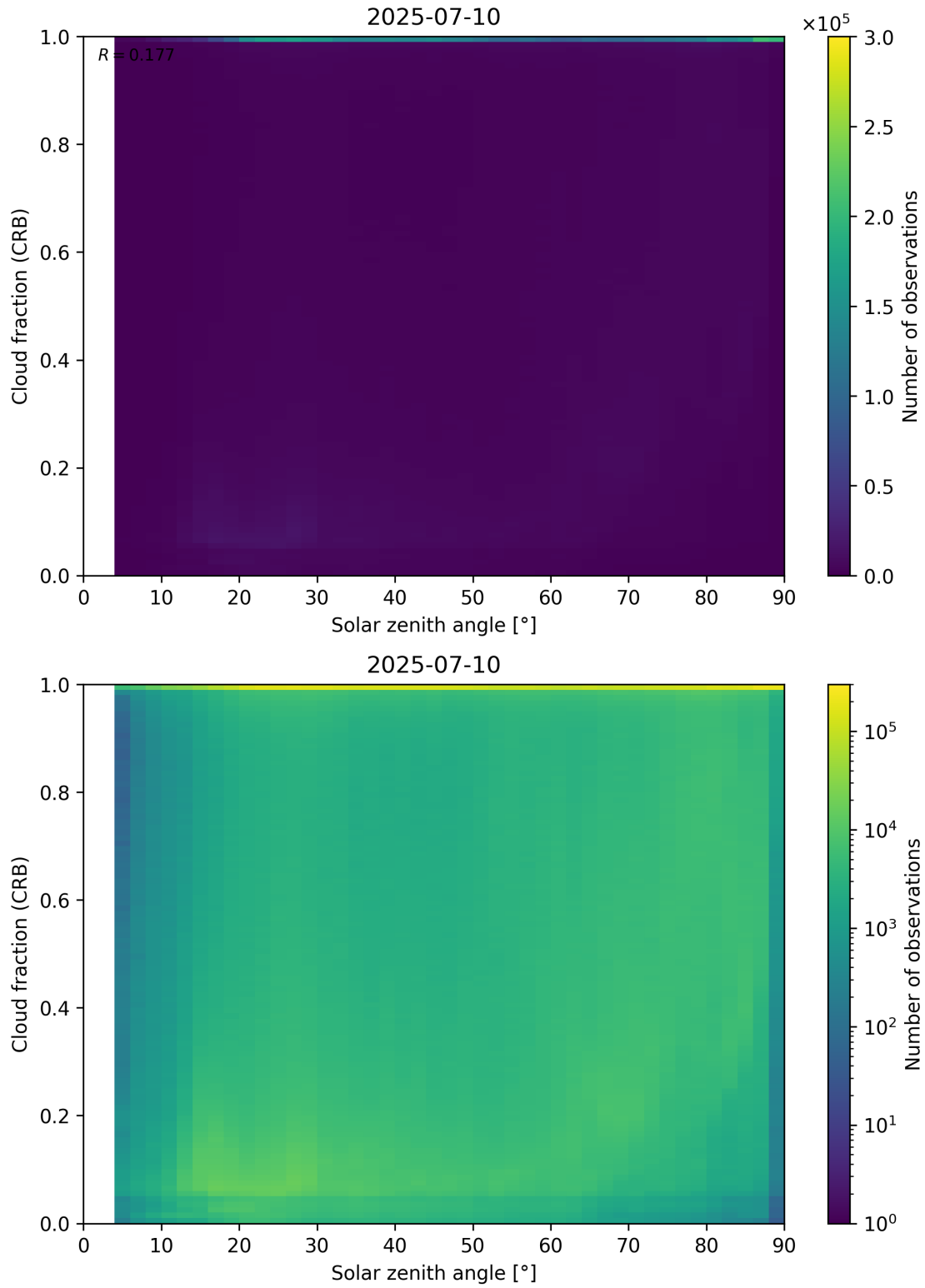
Figure 101: Scatter density plot of “Solar zenith angle” against “Cloud fraction (CRB)” for 2025-07-09 to 2025-07-11.
