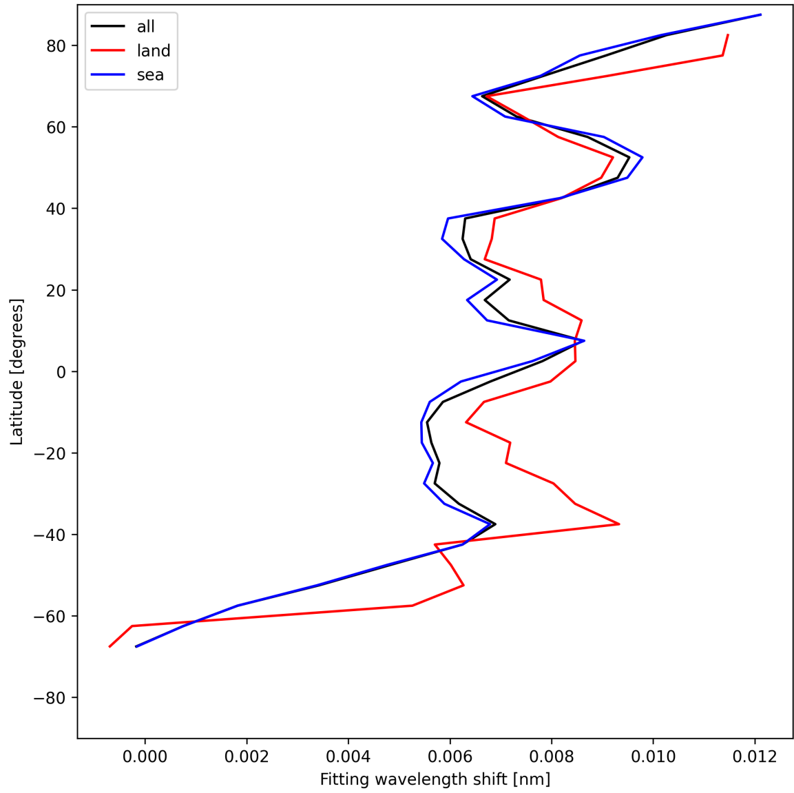
Figure 33: Zonal average of “Fitting wavelength shift” for 2025-07-09 to 2025-07-11.
