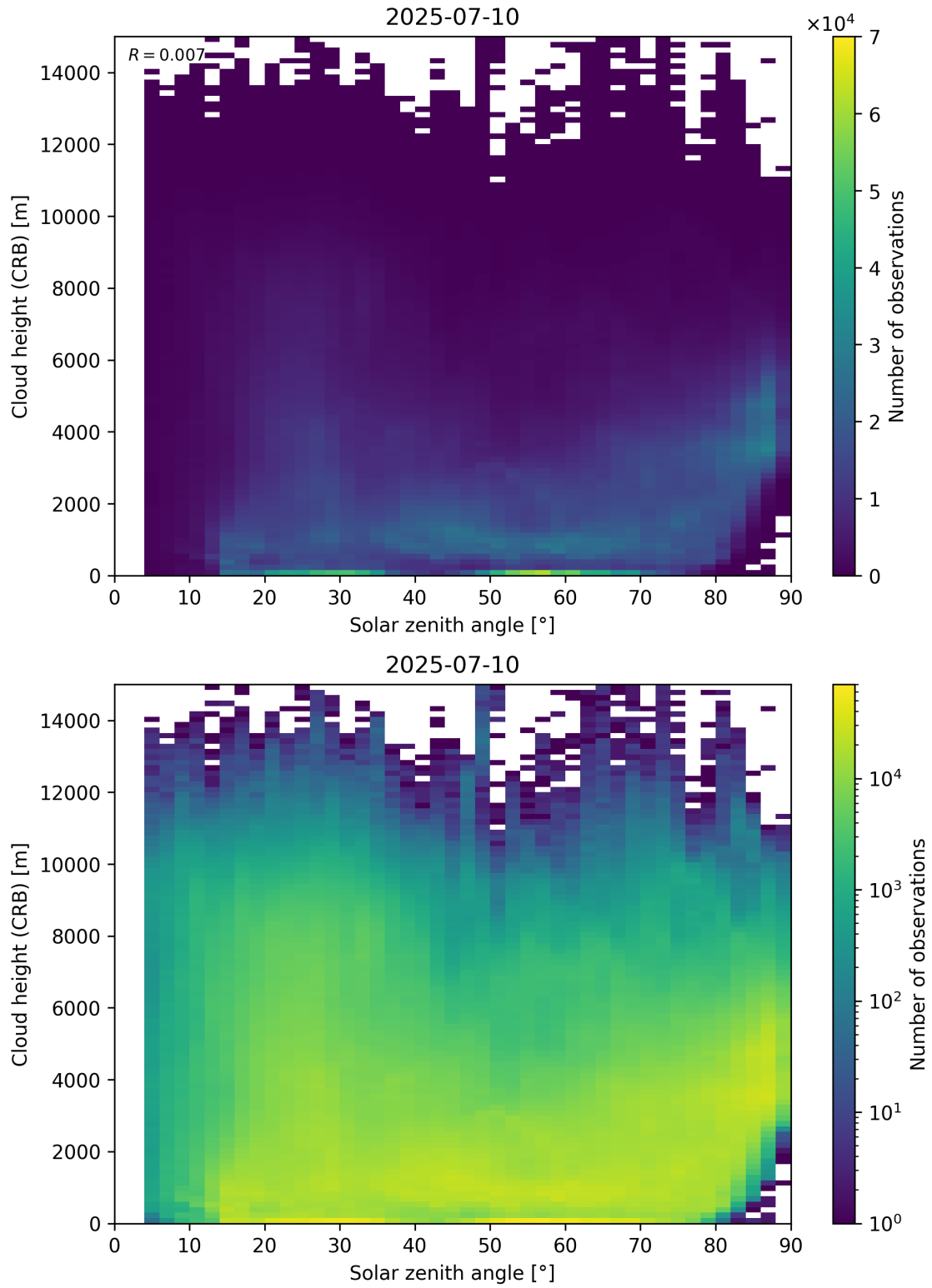
Figure 102: Scatter density plot of “Solar zenith angle” against “Cloud height (CRB)” for 2025-07-09 to 2025-07-11.
