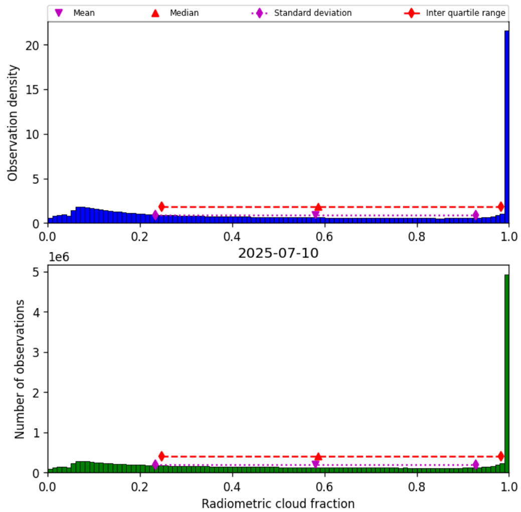
Figure 39: Histogram of “Radiometric cloud fraction” for 2025-07-09 to 2025-07-11
