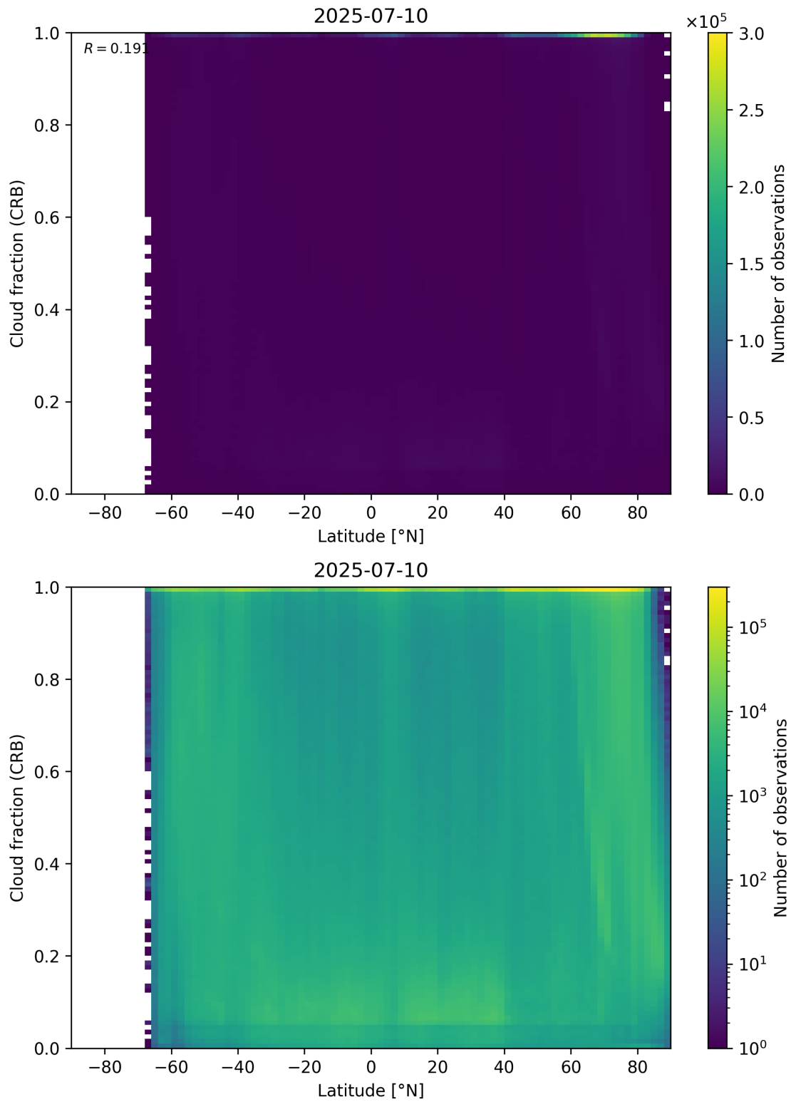
Figure 94: Scatter density plot of “Latitude” against “Cloud fraction (CRB)” for 2025-07-09 to 2025-07-11.
