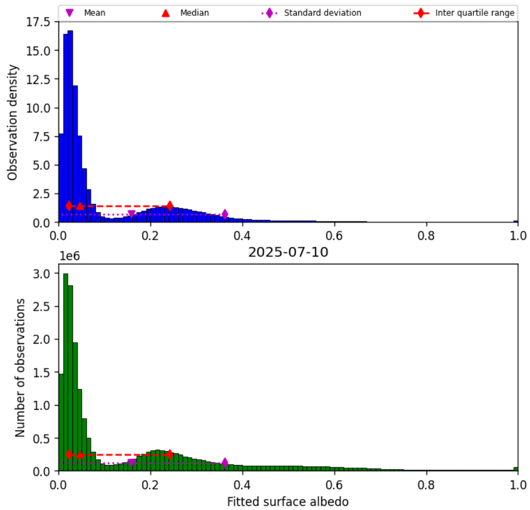
Figure 45: Histogram of “Fitted surface albedo” for 2025-07-09 to 2025-07-11
