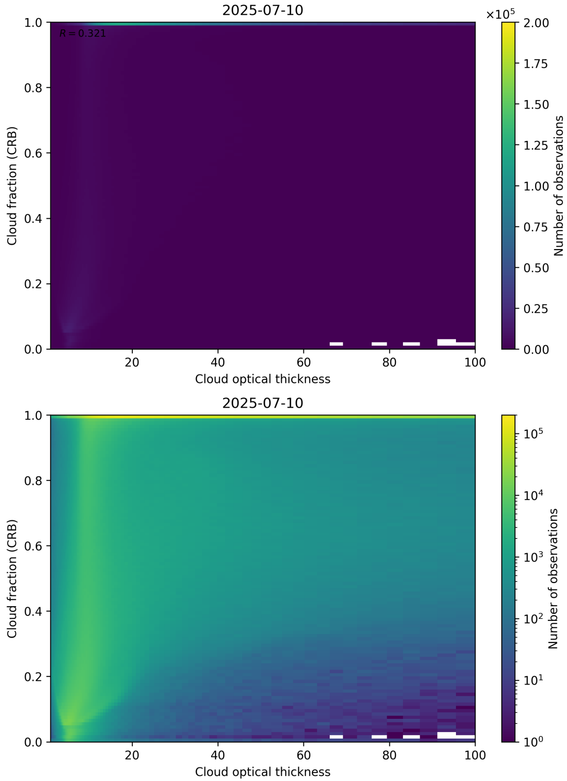
Figure 84: Scatter density plot of “Cloud optical thickness” against “Cloud fraction (CRB)” for 2025-07-09 to 2025-07-11.
