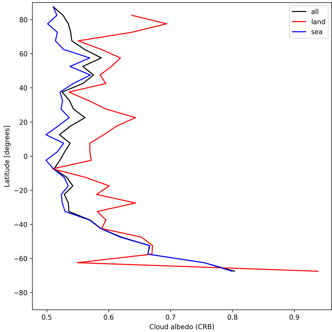
Figure 28: Zonal average of “Cloud albedo (CRB)” for 2025-07-09 to 2025-07-11.
