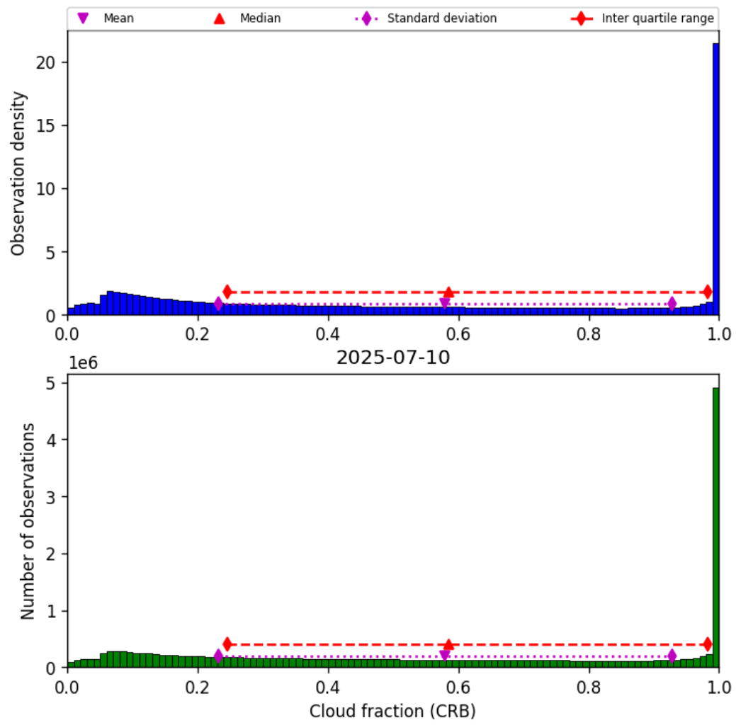
Figure 42: Histogram of “Cloud fraction (CRB)” for 2025-07-09 to 2025-07-11
