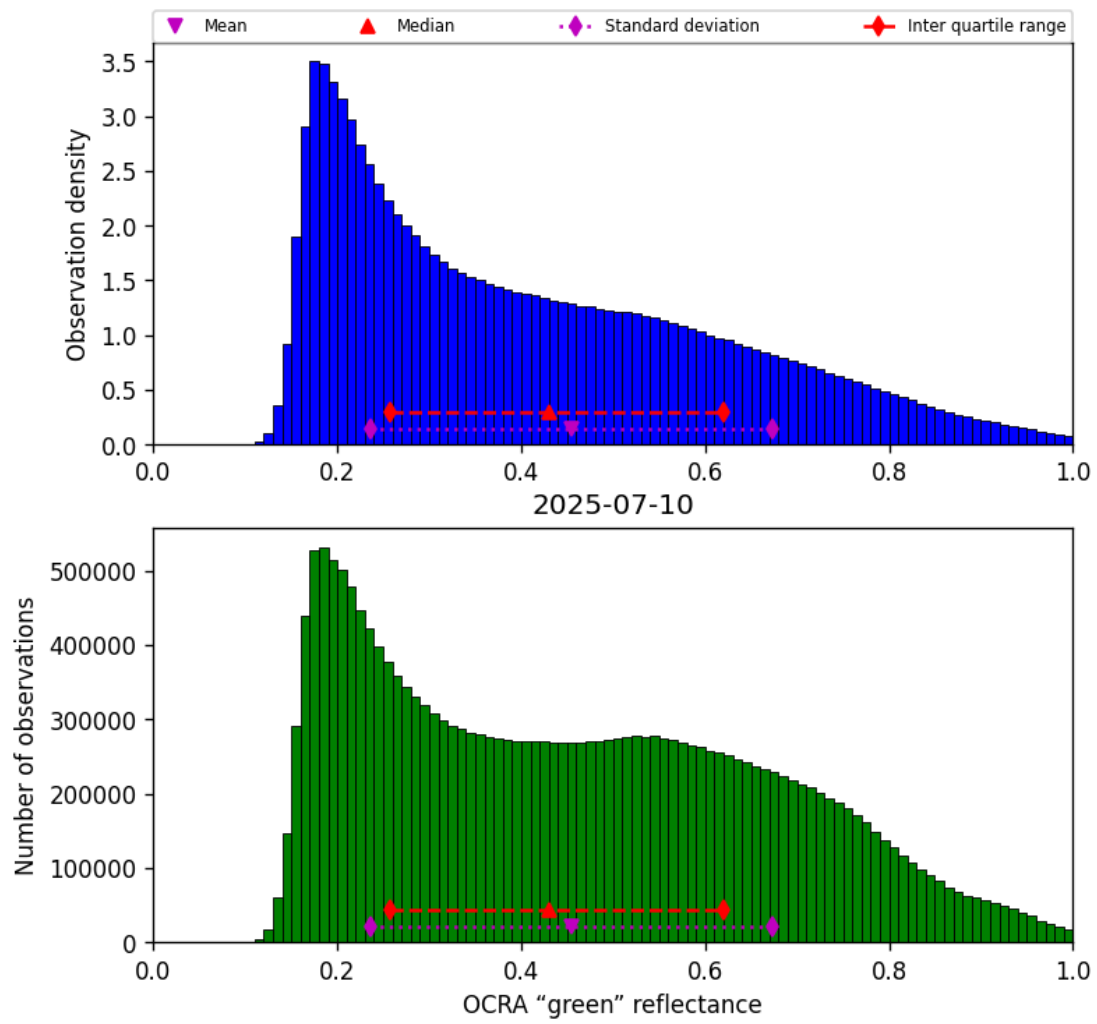
Figure 52: Histogram of “OCRA “green” reflectance” for 2025-07-09 to 2025-07-11
