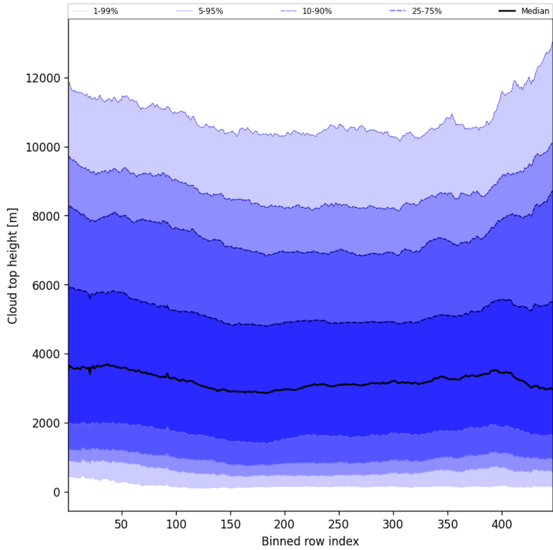
Figure 56: Along track statistics of “Cloud top height” for 2025-07-09 to 2025-07-11
