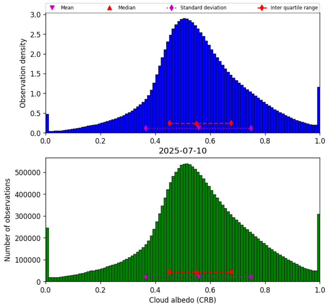
Figure 44: Histogram of “Cloud albedo (CRB)” for 2025-07-09 to 2025-07-11
