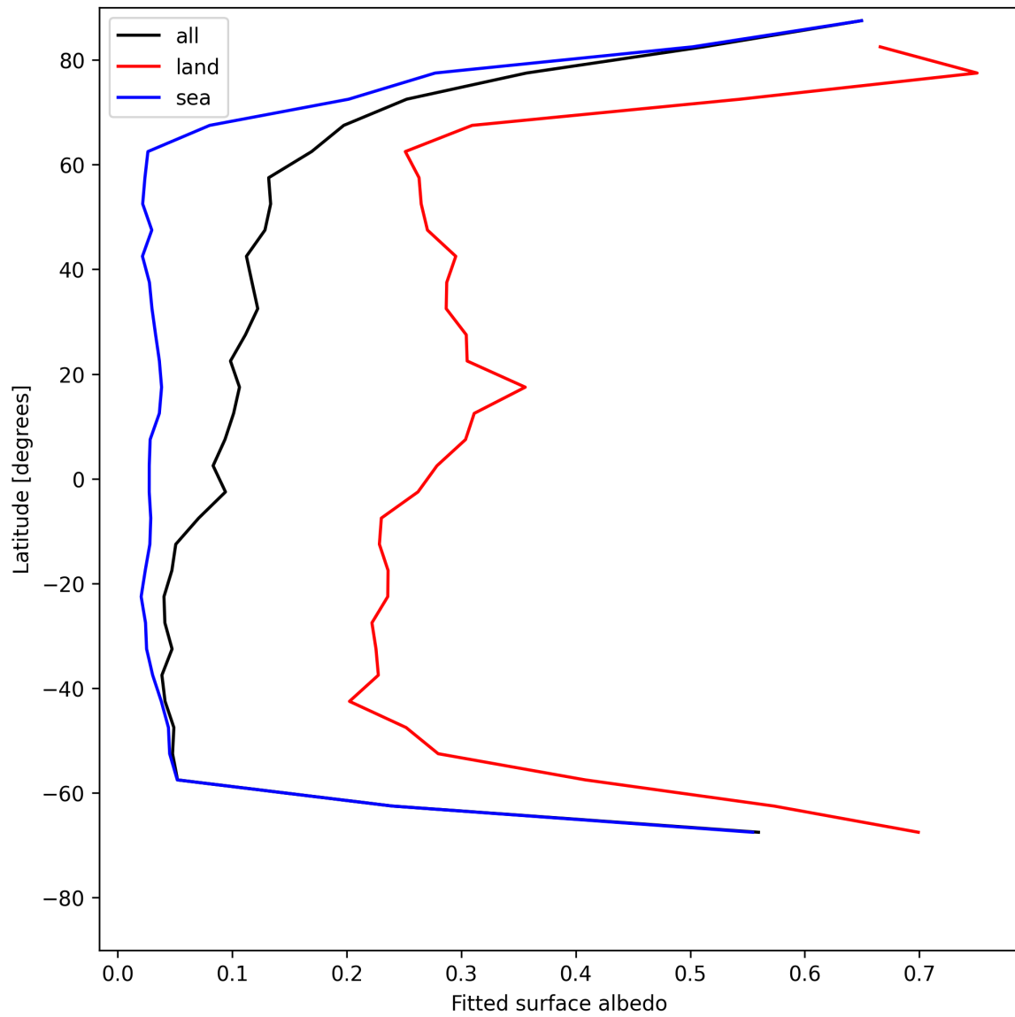
Figure 29: Zonal average of “Fitted surface albedo” for 2025-07-09 to 2025-07-11.
