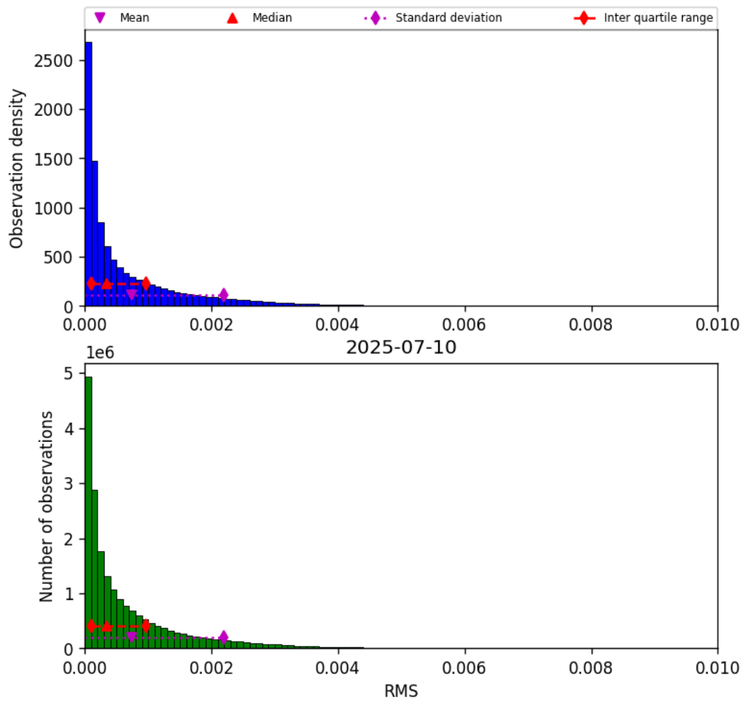
Figure 47: Histogram of “RMS” for 2025-07-09 to 2025-07-11
