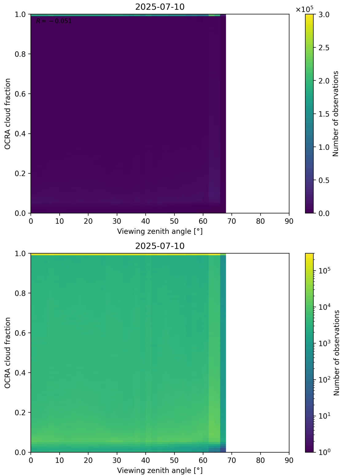
Figure 108: Scatter density plot of “Viewing zenith angle” against “OCRA cloud fraction” for 2025-07-09 to 2025-07-11.
