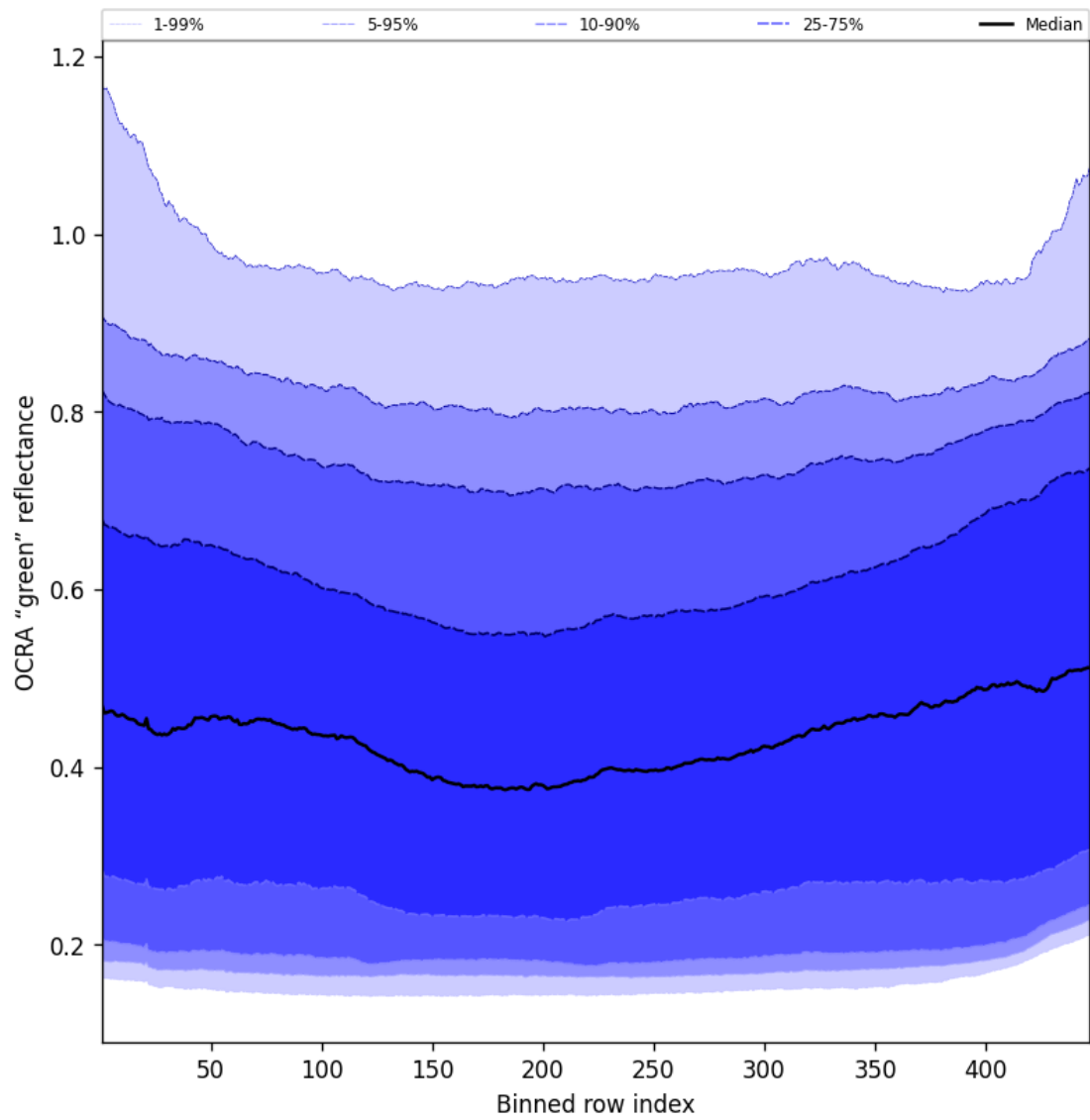
Figure 68: Along track statistics of “OCRA “green” reflectance” for 2025-07-09 to 2025-07-11
