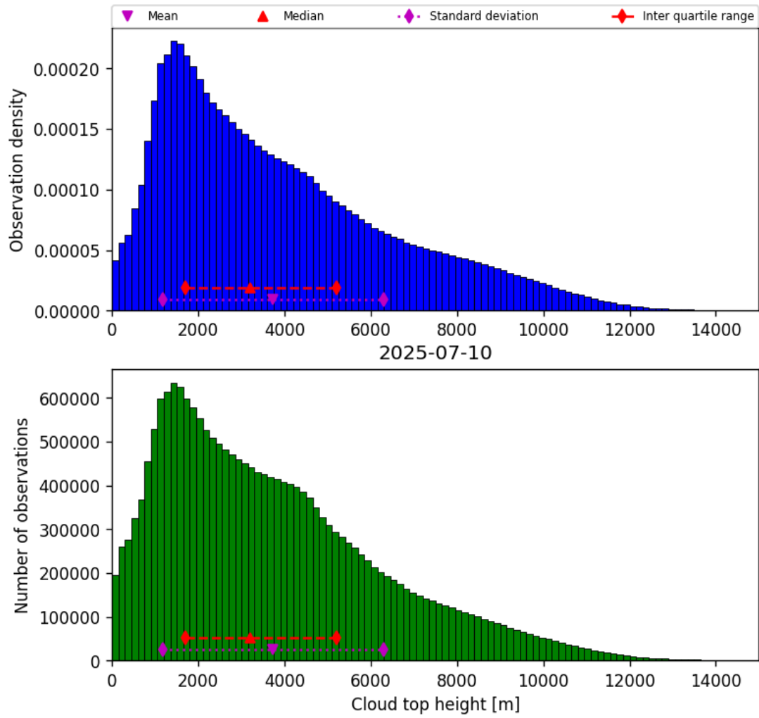
Figure 40: Histogram of “Cloud top height” for 2025-07-09 to 2025-07-11
