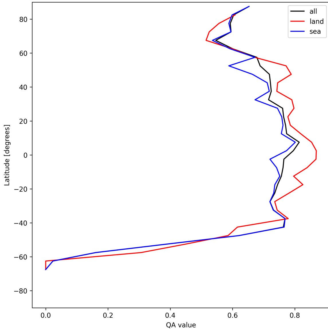
Figure 22: Zonal average of “QA value” for 2025-07-09 to 2025-07-11.
