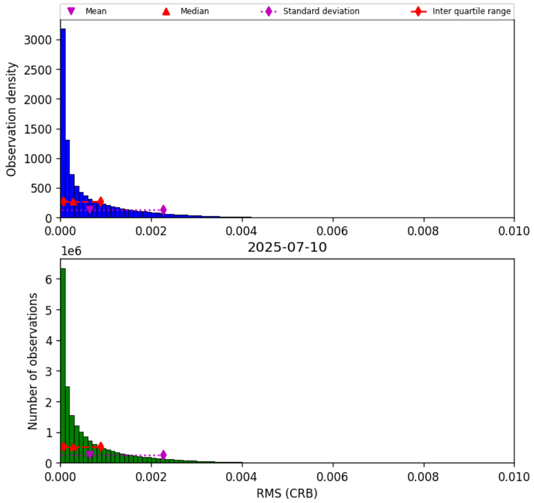
Figure 48: Histogram of “RMS (CRB)” for 2025-07-09 to 2025-07-11
