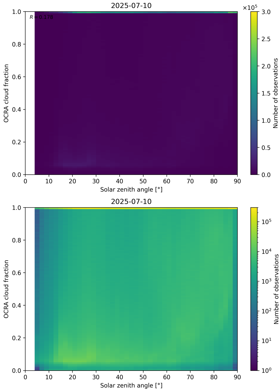
Figure 100: Scatter density plot of “Solar zenith angle” against “OCRA cloud fraction” for 2025-07-09 to 2025-07-11.
