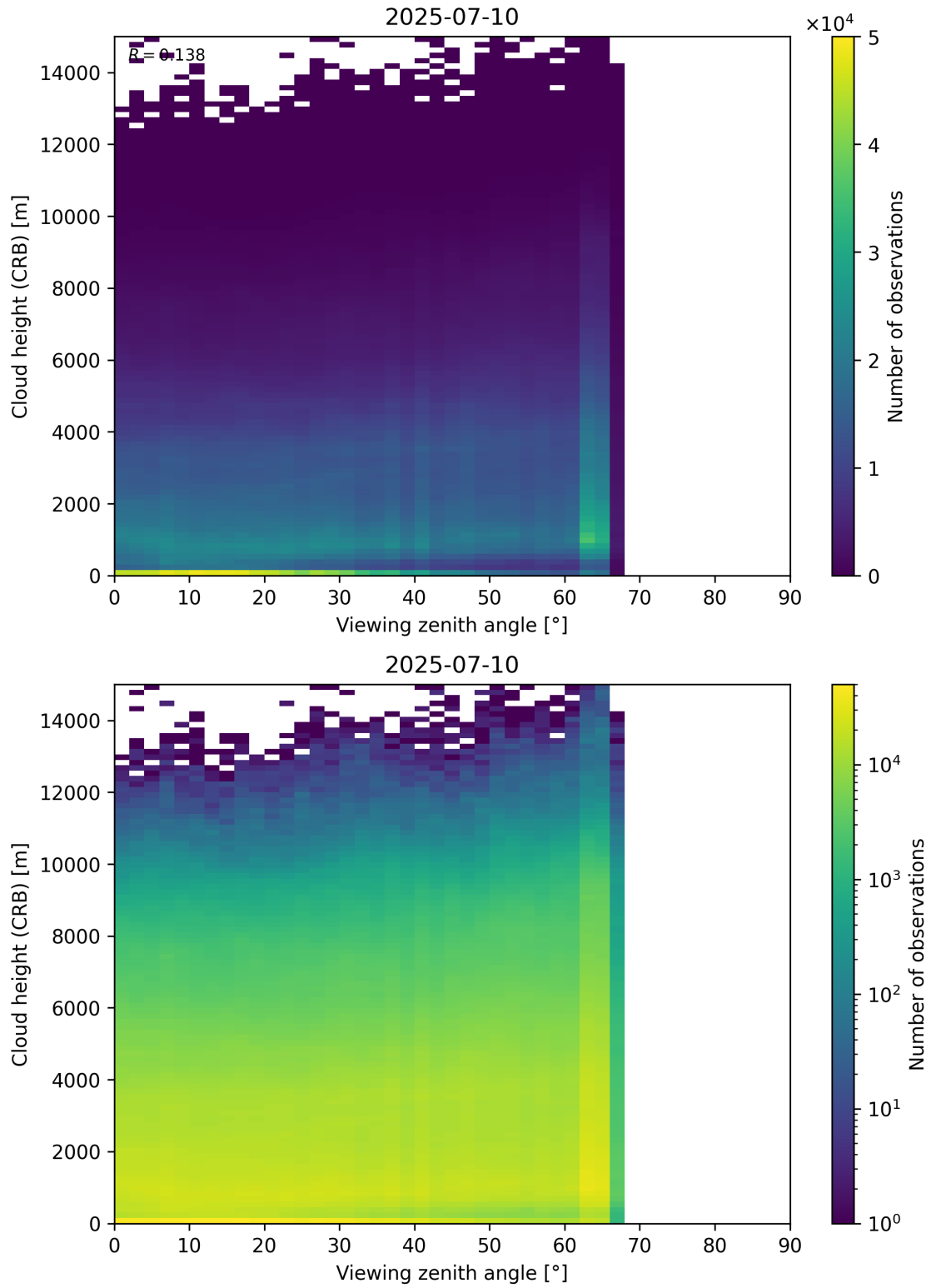
Figure 110: Scatter density plot of “Viewing zenith angle” against “Cloud height (CRB)” for 2025-07-09 to 2025-07-11.
