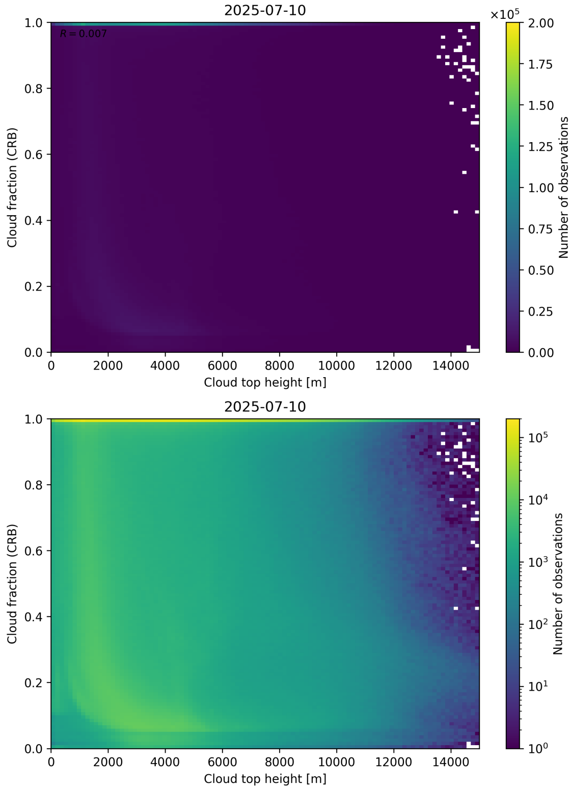
Figure 88: Scatter density plot of “Cloud top height” against “Cloud fraction (CRB)” for 2025-07-09 to 2025-07-11.
