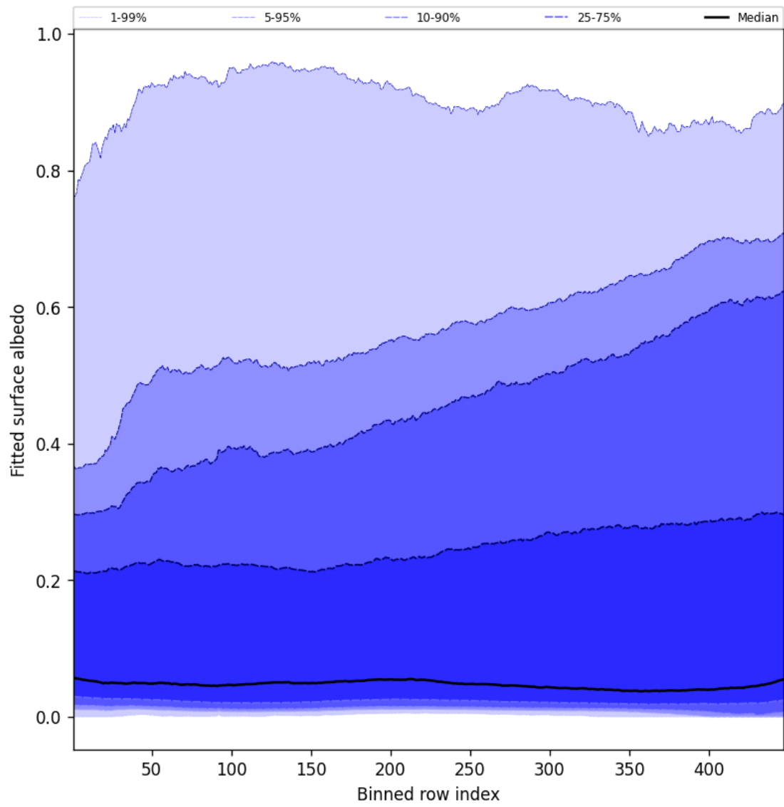
Figure 61: Along track statistics of “Fitted surface albedo” for 2025-07-09 to 2025-07-11
