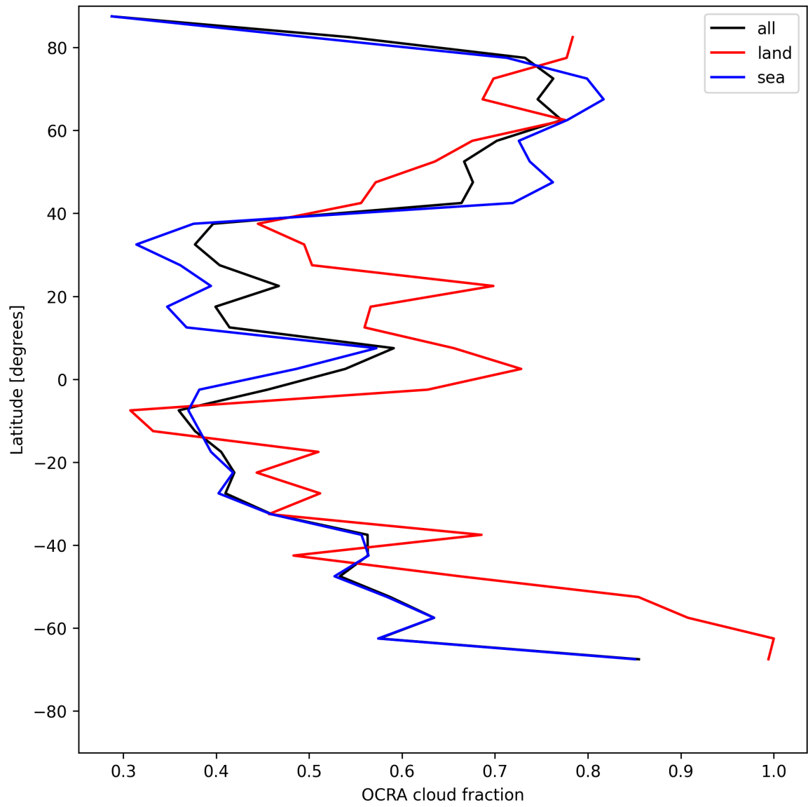
Figure 34: Zonal average of “OCRA cloud fraction” for 2025-07-09 to 2025-07-11.
