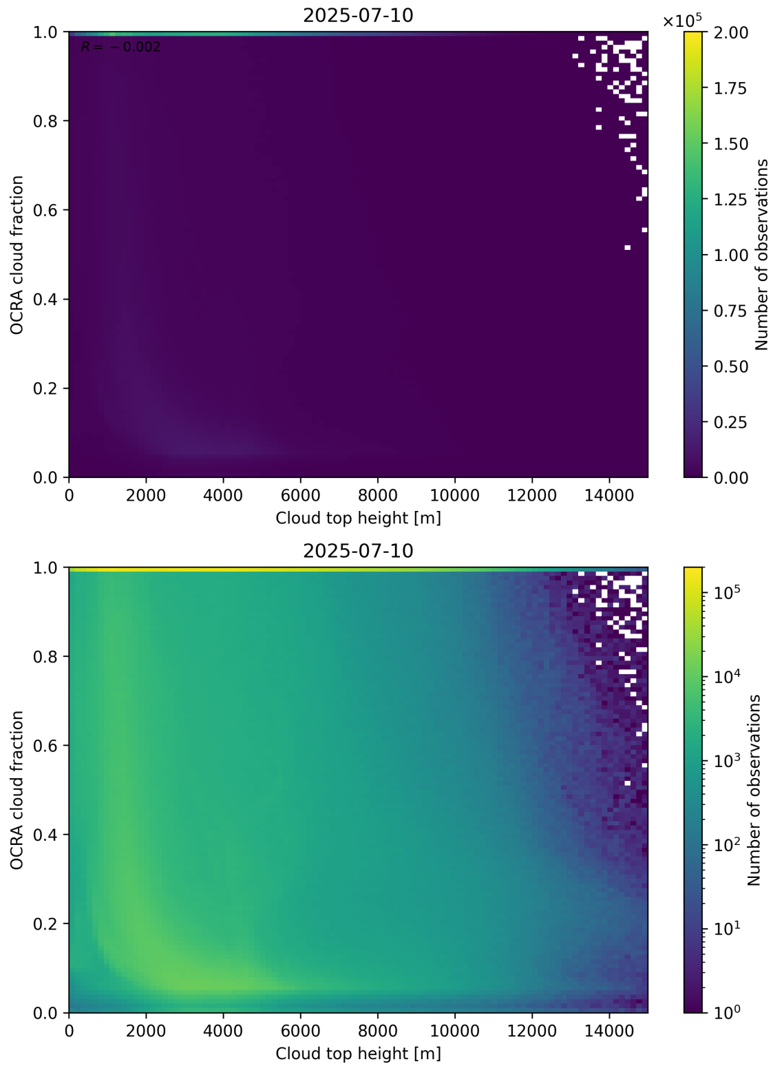
Figure 87: Scatter density plot of “Cloud top height” against “OCRA cloud fraction” for 2025-07-09 to 2025-07-11.
