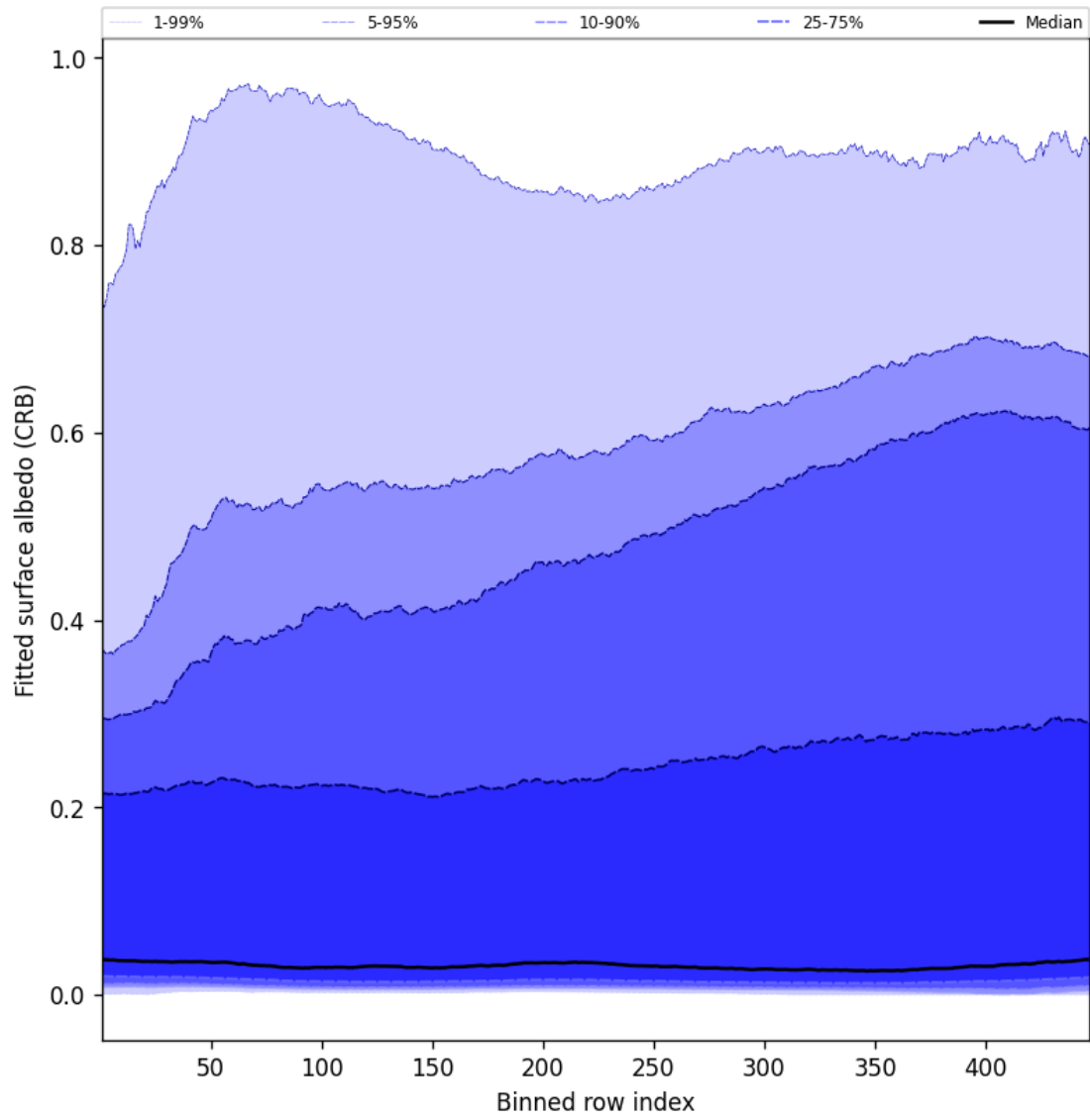
Figure 62: Along track statistics of “Fitted surface albedo (CRB)” for 2025-07-09 to 2025-07-11
