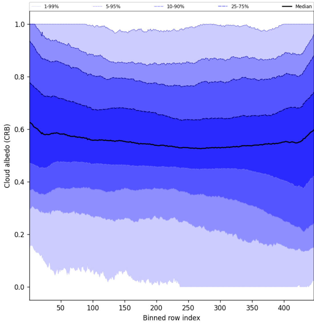
Figure 60: Along track statistics of “Cloud albedo (CRB)” for 2025-07-09 to 2025-07-11
