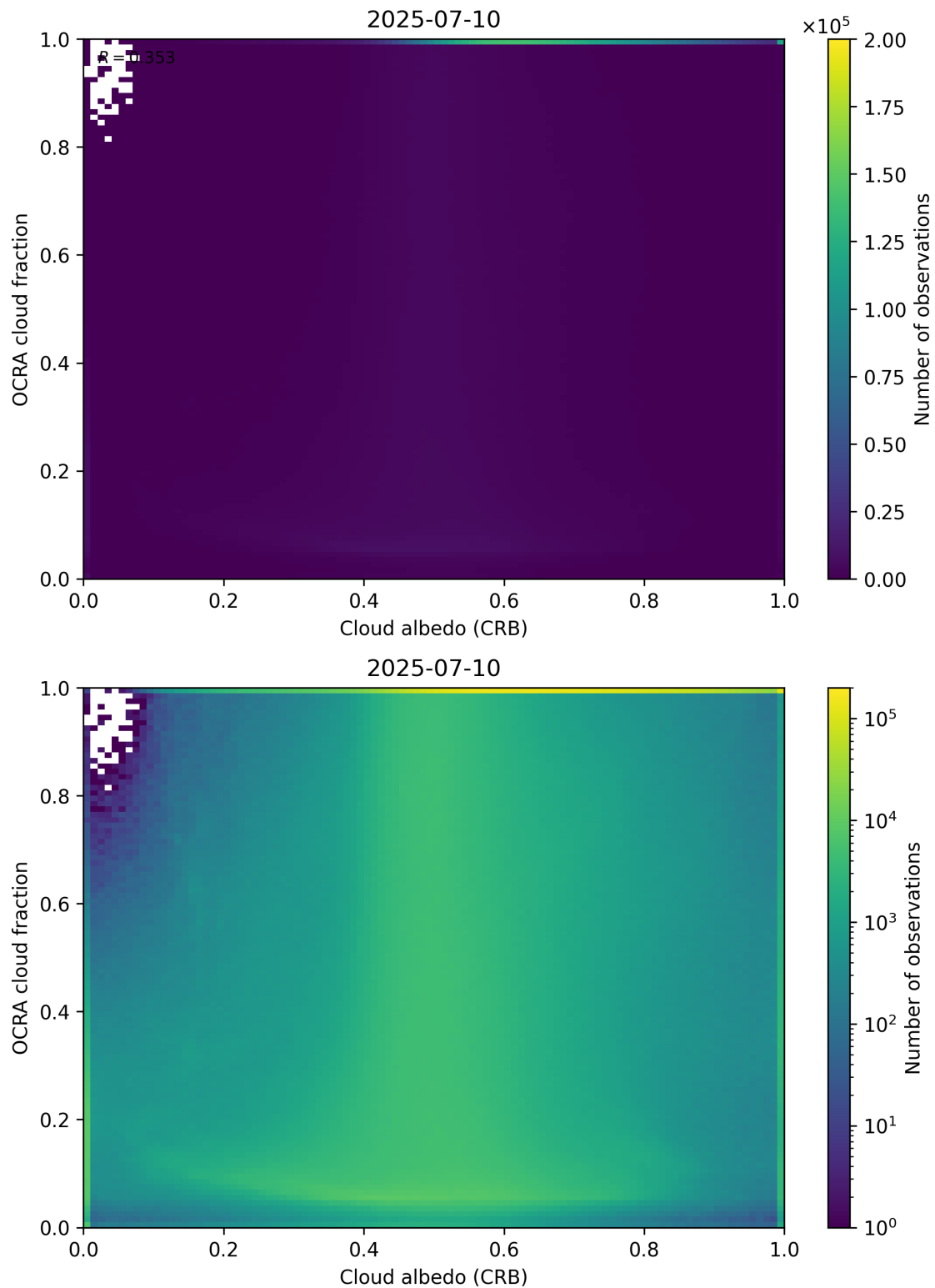
Figure 70: Scatter density plot of “Cloud albedo (CRB)” against “OCRA cloud fraction” for 2025-07-09 to 2025-07-11.
