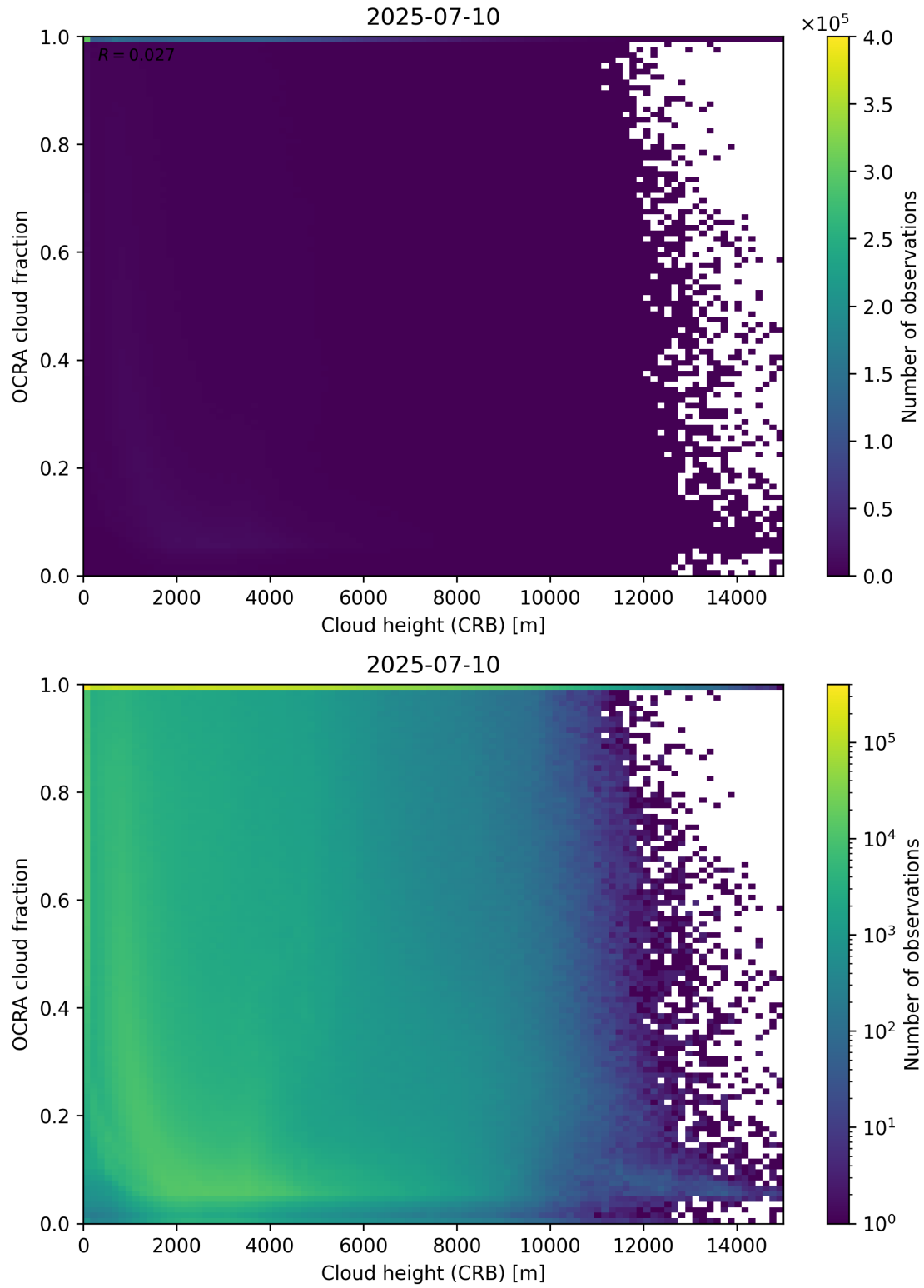
Figure 81: Scatter density plot of “Cloud height (CRB)” against “OCRA cloud fraction” for 2025-07-09 to 2025-07-11.
