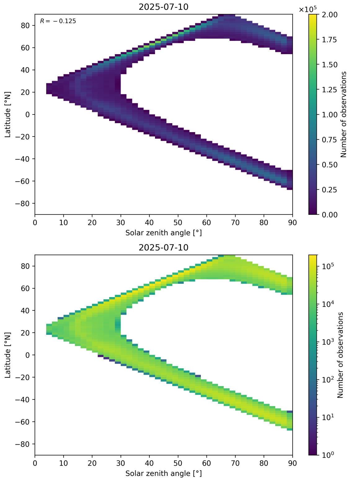
Figure 105: Scatter density plot of “Solar zenith angle” against “Latitude” for 2025-07-09 to 2025-07-11.
