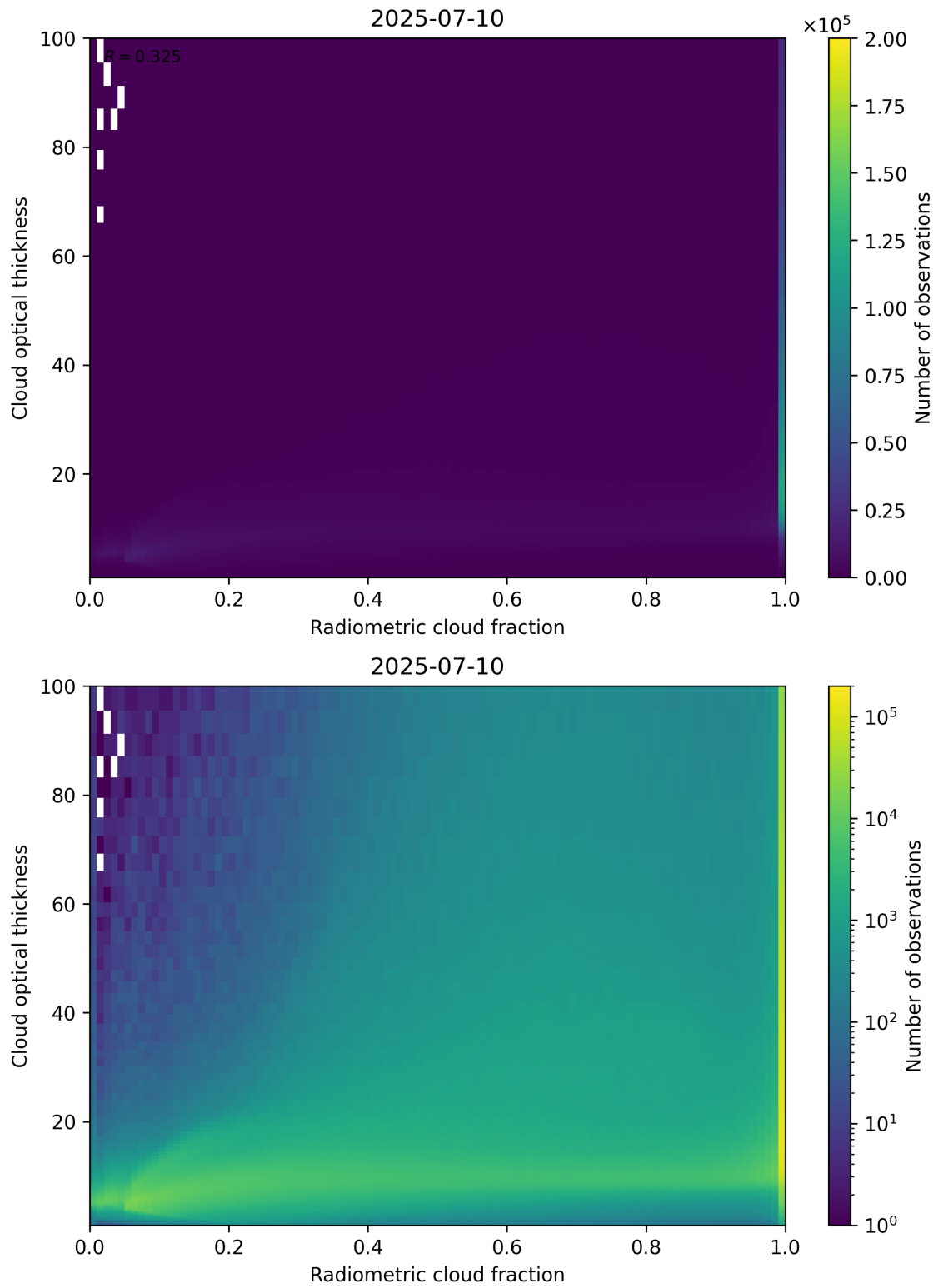
Figure 75: Scatter density plot of “Radiometric cloud fraction” against “Cloud optical thickness” for 2025-07-09 to 2025-07-11.
