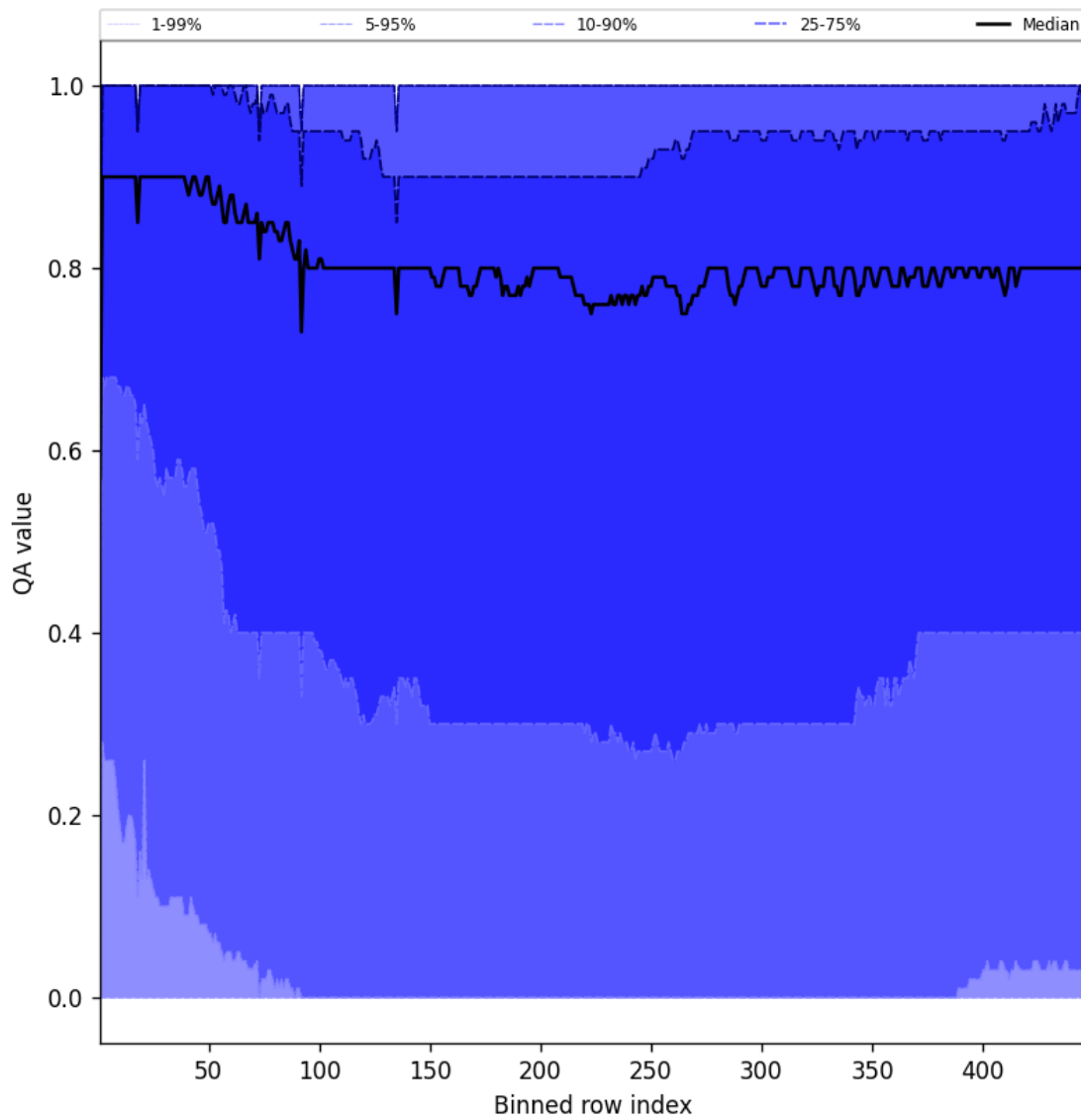
Figure 54: Along track statistics of “QA value” for 2025-07-09 to 2025-07-11
