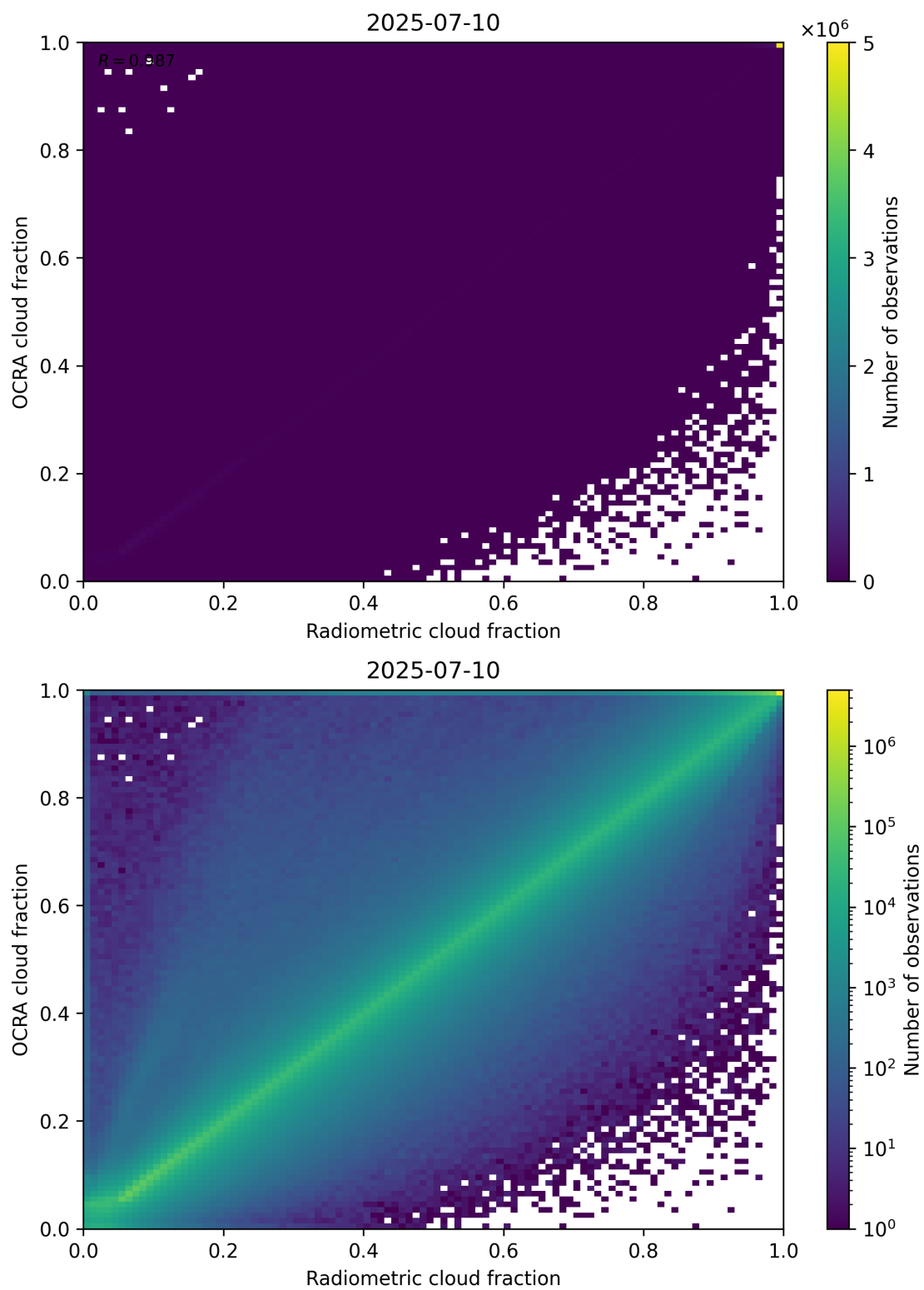
Figure 72: Scatter density plot of “Radiometric cloud fraction” against “OCRA cloud fraction” for 2025-07-09 to 2025-07-11.
