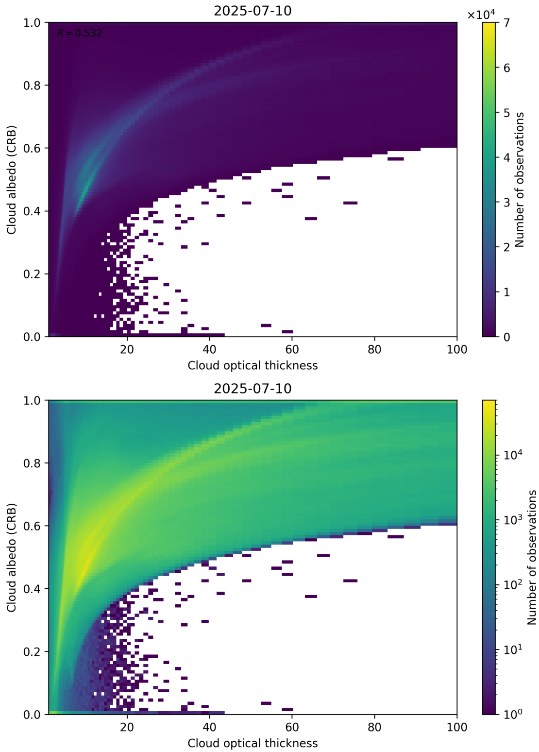
Figure 82: Scatter density plot of “Cloud optical thickness” against “Cloud albedo (CRB)” for 2025-07-09 to 2025-07-11.
