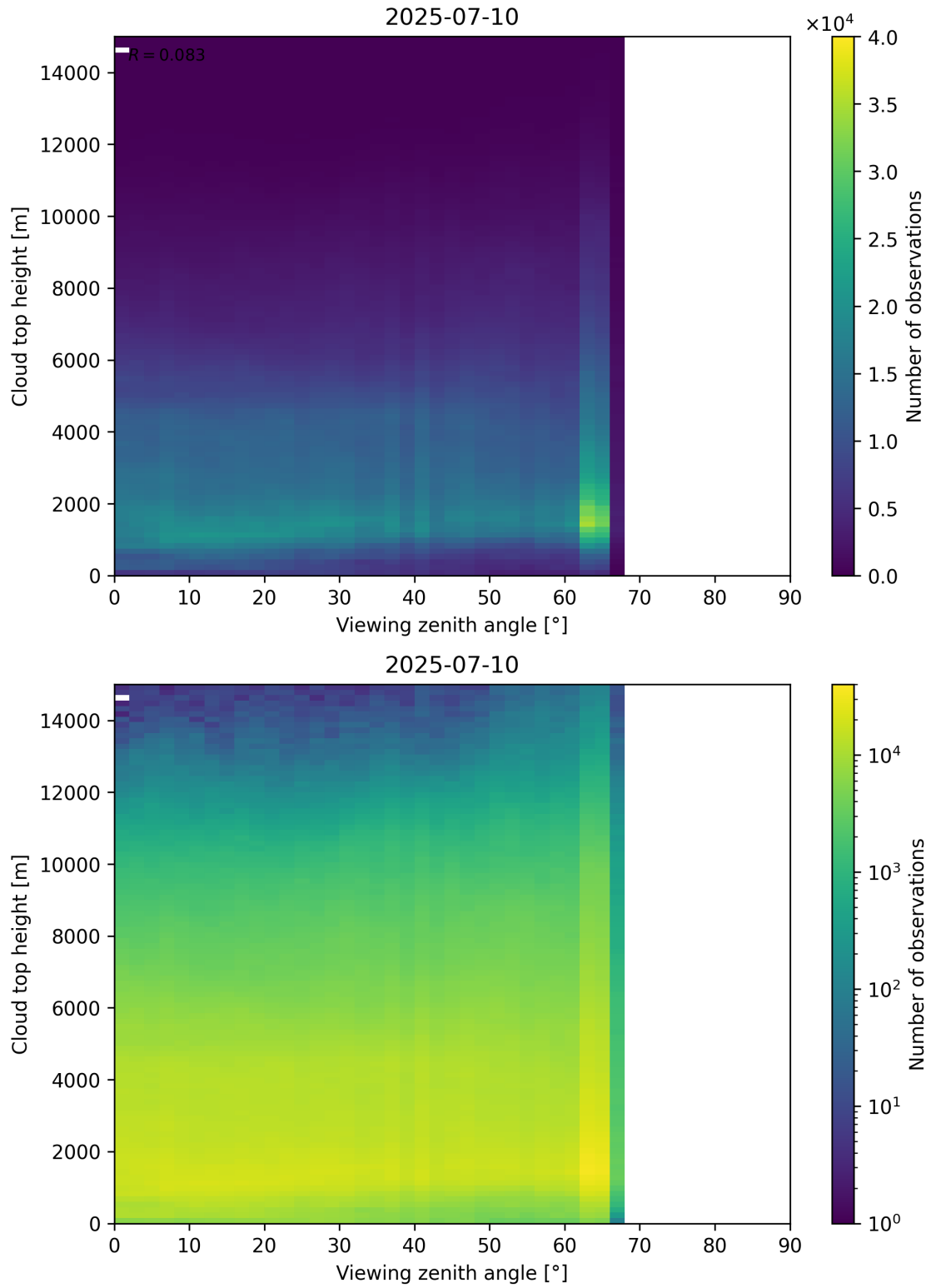
Figure 112: Scatter density plot of “Viewing zenith angle” against “Cloud top height” for 2025-07-09 to 2025-07-11.
