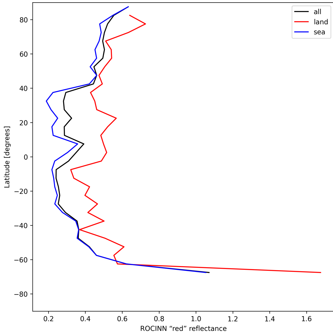
Figure 37: Zonal average of “ROCINN “red” reflectance” for 2025-07-09 to 2025-07-11.
