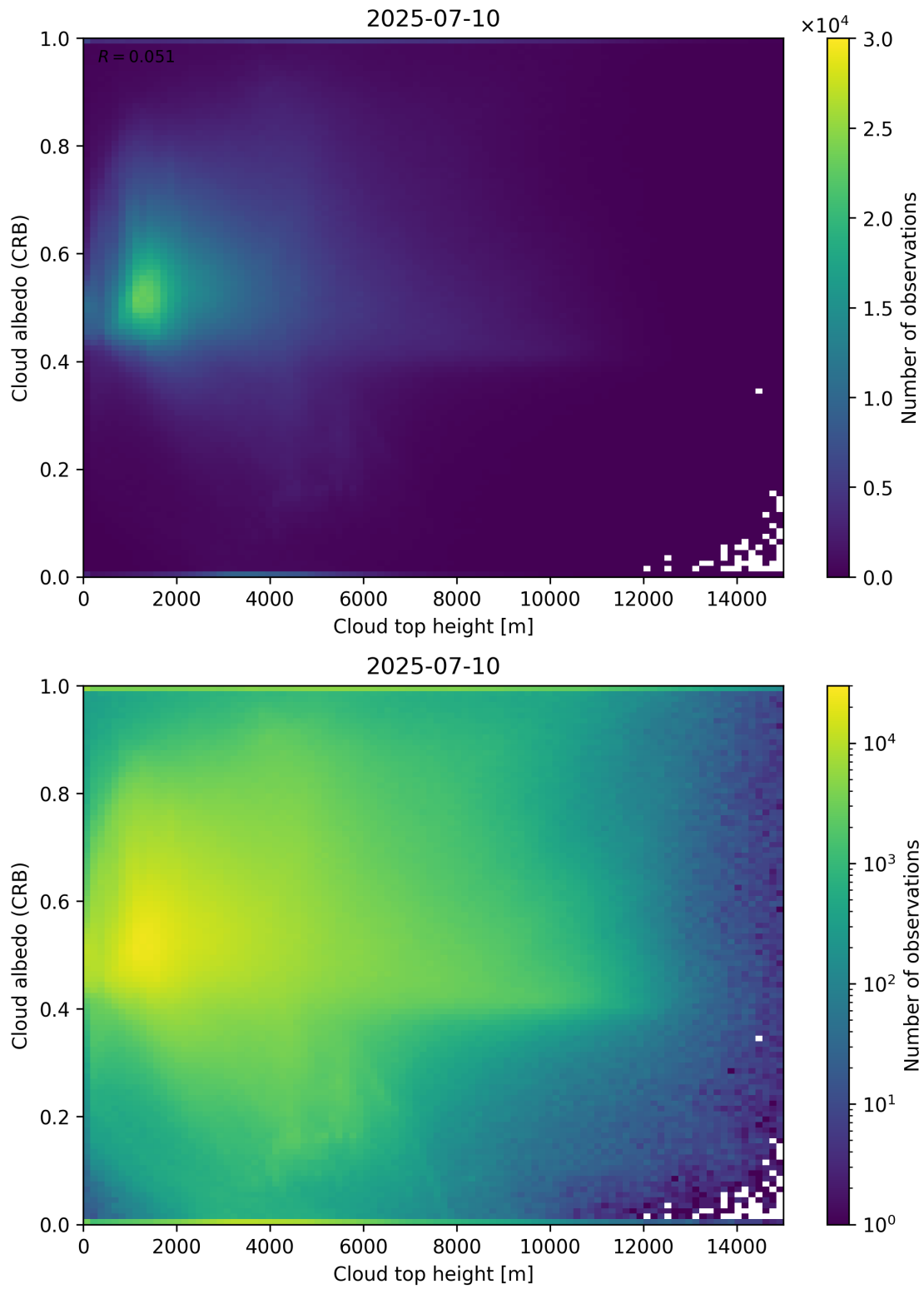
Figure 86: Scatter density plot of “Cloud top height” against “Cloud albedo (CRB)” for 2025-07-09 to 2025-07-11.
