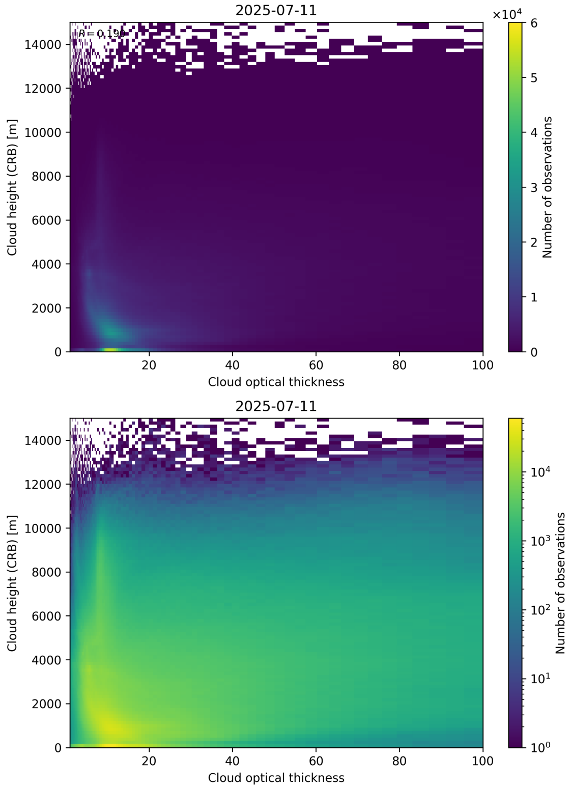
Figure 85: Scatter density plot of “Cloud optical thickness” against “Cloud height (CRB)” for 2025-07-10 to 2025-07-12.
