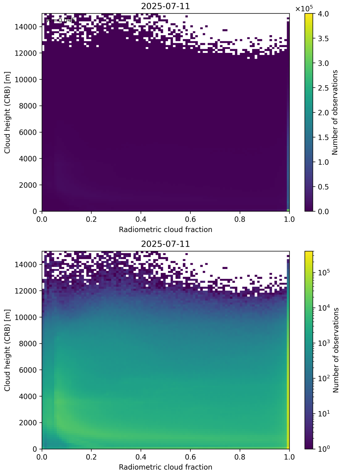
Figure 74: Scatter density plot of “Radiometric cloud fraction” against “Cloud height (CRB)” for 2025-07-10 to 2025-07-12.
