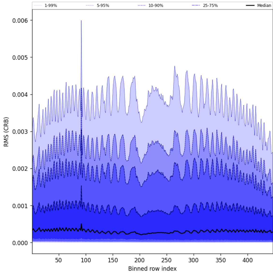
Figure 64: Along track statistics of “RMS (CRB)” for 2025-07-10 to 2025-07-12
