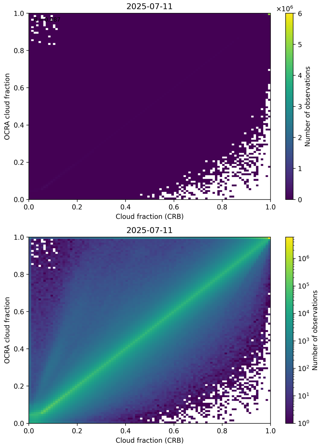
Figure 78: Scatter density plot of “Cloud fraction (CRB)” against “OCRA cloud fraction” for 2025-07-10 to 2025-07-12.
