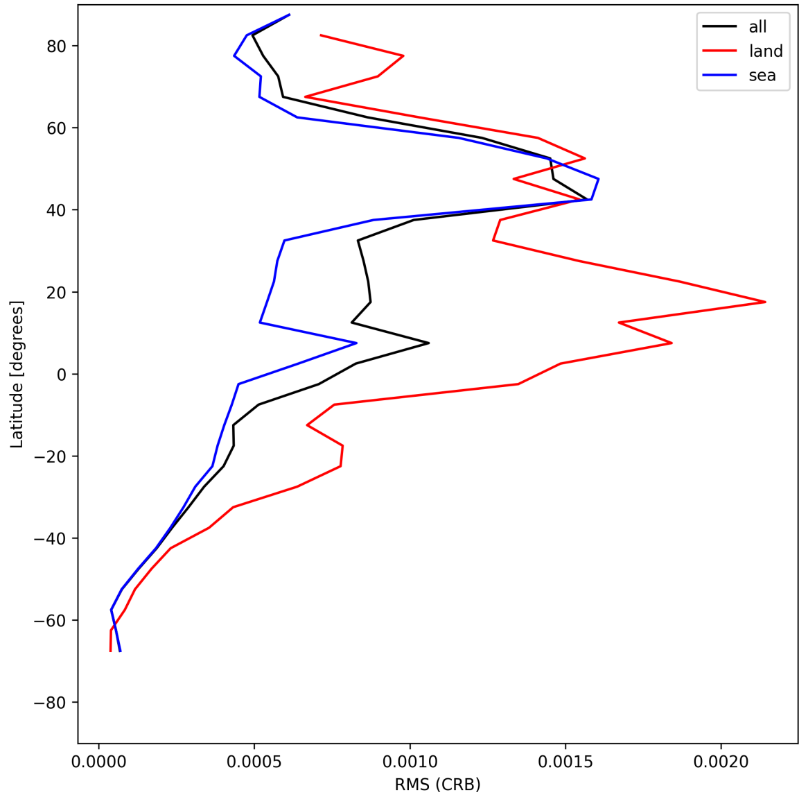
Figure 32: Zonal average of “RMS (CRB)” for 2025-07-10 to 2025-07-12.
