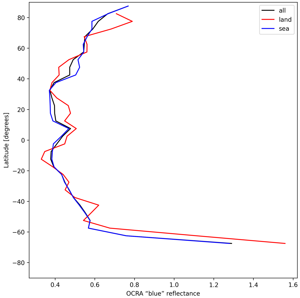
Figure 35: Zonal average of "OCRA "blue" reflectance" for 2025-07-10 to 2025-07-12.
