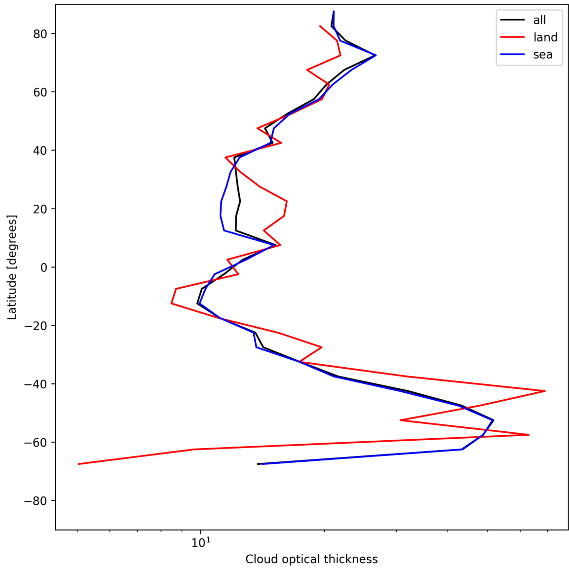
Figure 25: Zonal average of “Cloud optical thickness” for 2025-07-10 to 2025-07-12.
