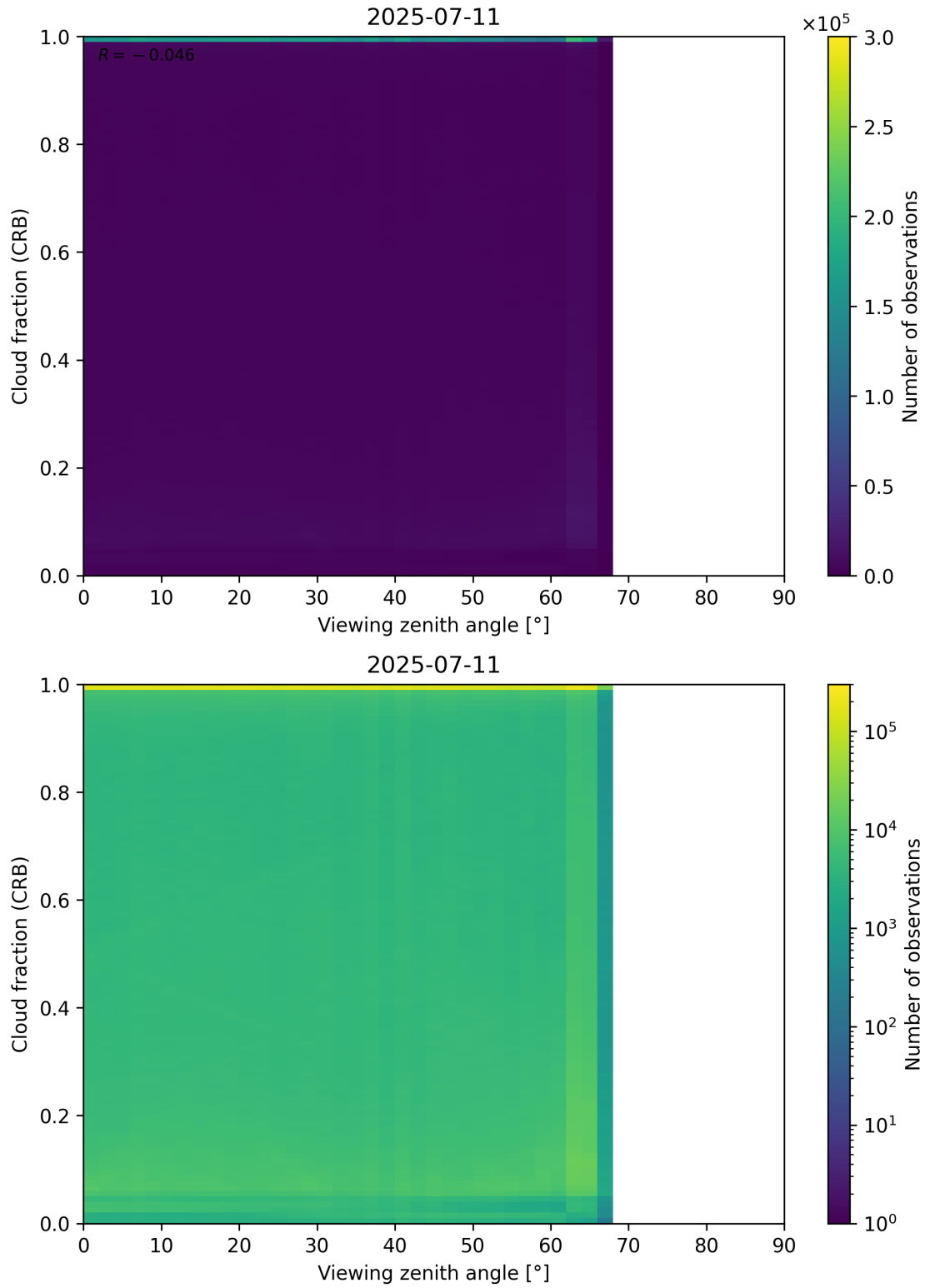
Figure 109: Scatter density plot of “Viewing zenith angle” against “Cloud fraction (CRB)” for 2025-07-10 to 2025-07-12.
