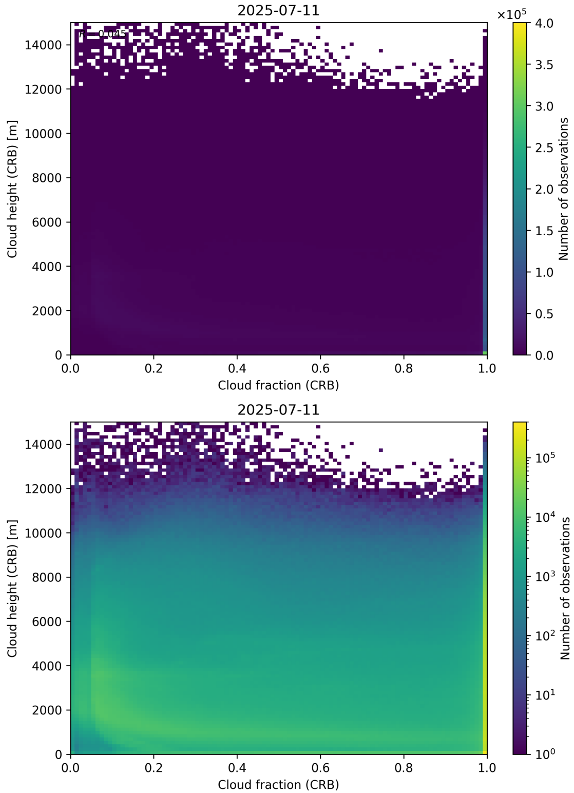
Figure 79: Scatter density plot of “Cloud fraction (CRB)” against “Cloud height (CRB)” for 2025-07-10 to 2025-07-12.
