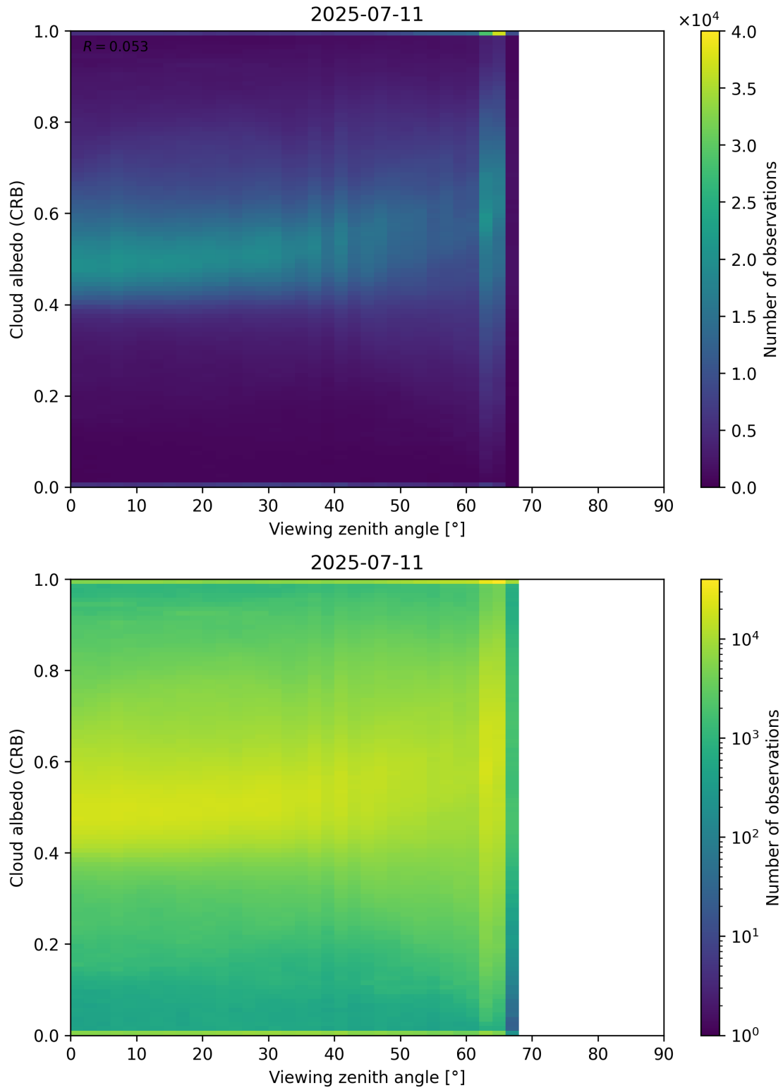
Figure 106: Scatter density plot of “Viewing zenith angle” against “Cloud albedo (CRB)” for 2025-07-10 to 2025-07-12.
