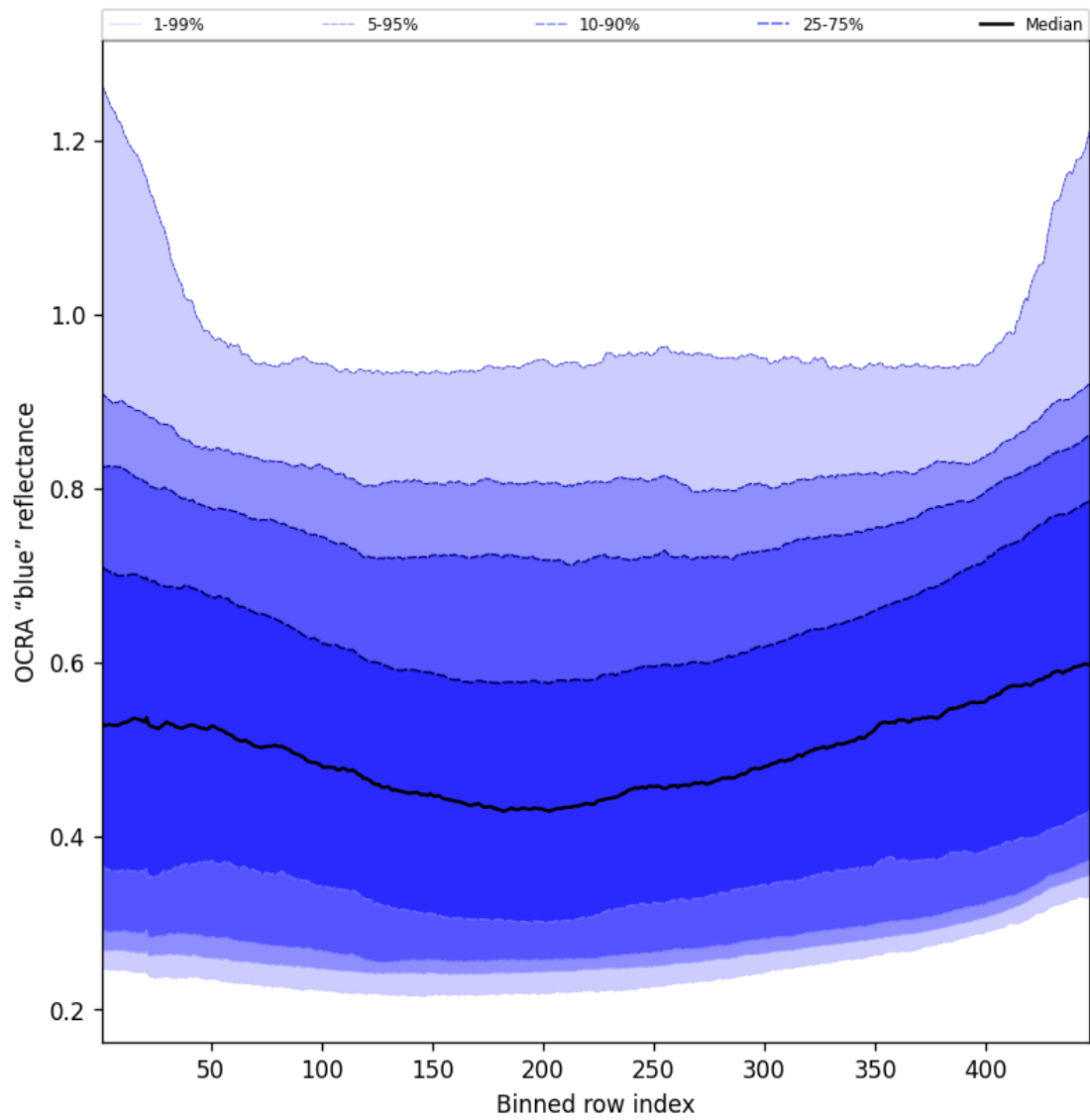
Figure 67: Along track statistics of “OCRA “blue” reflectance” for 2025-07-10 to 2025-07-12
