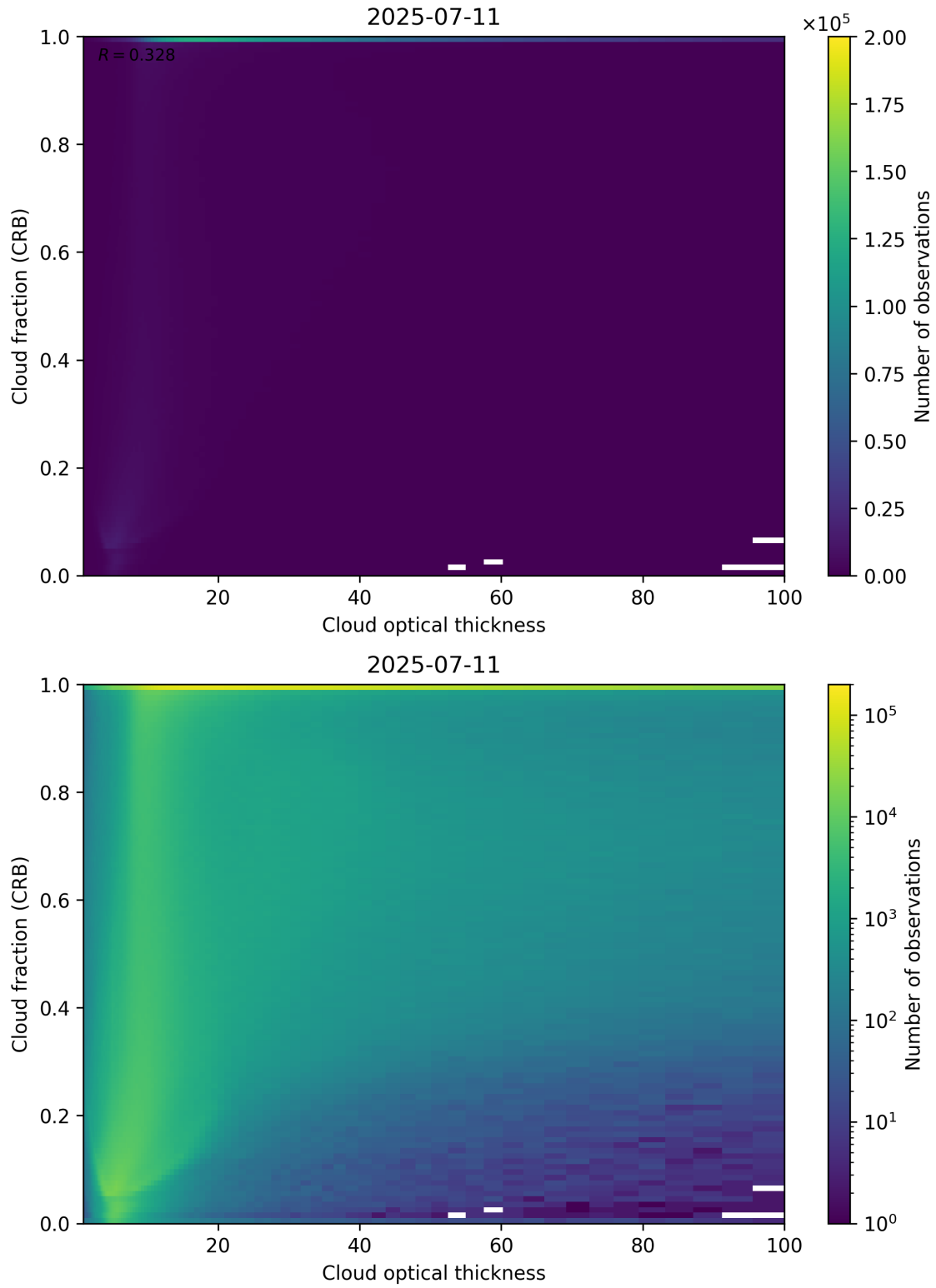
Figure 84: Scatter density plot of “Cloud optical thickness” against “Cloud fraction (CRB)” for 2025-07-10 to 2025-07-12.
