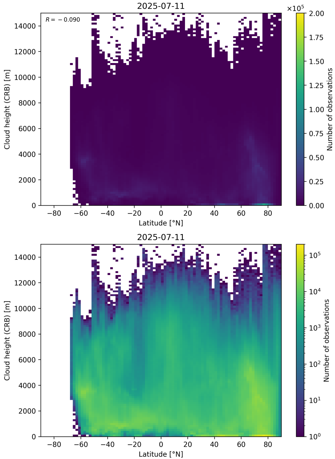
Figure 95: Scatter density plot of “Latitude” against “Cloud height (CRB)” for 2025-07-10 to 2025-07-12.
