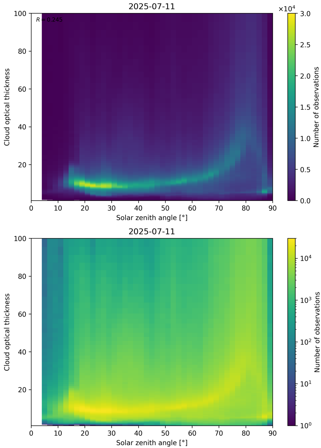
Figure 103: Scatter density plot of “Solar zenith angle” against “Cloud optical thickness” for 2025-07-10 to 2025-07-12.
