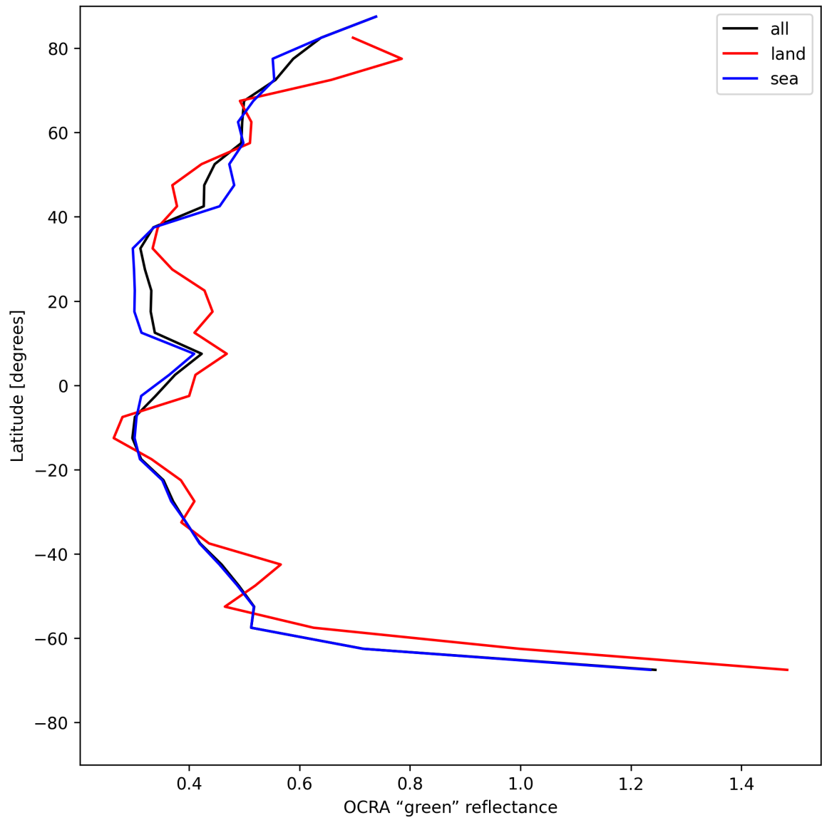
Figure 36: Zonal average of “OCRA “green” reflectance” for 2025-07-10 to 2025-07-12.
