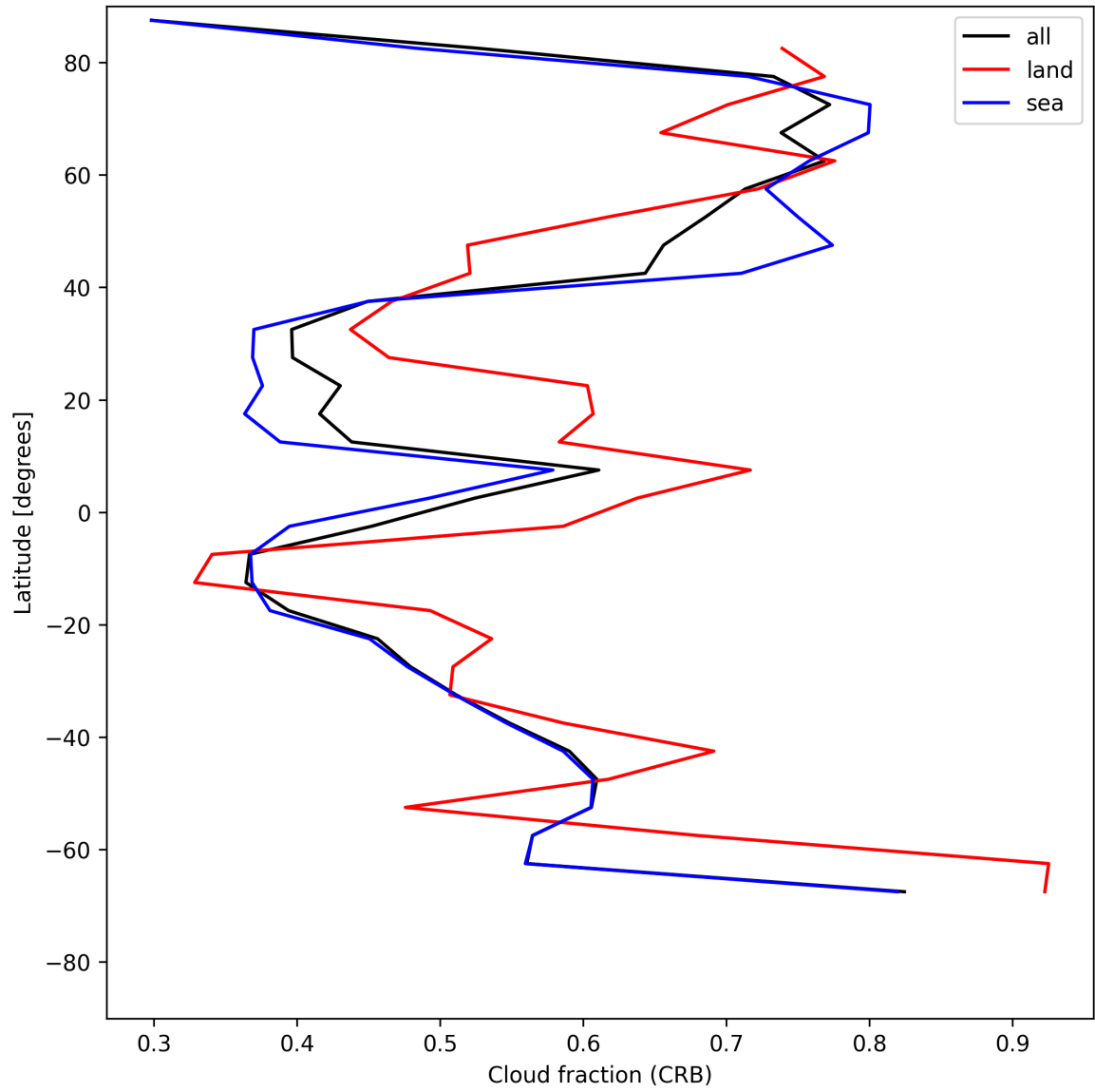
Figure 26: Zonal average of “Cloud fraction (CRB)” for 2025-07-10 to 2025-07-12.
