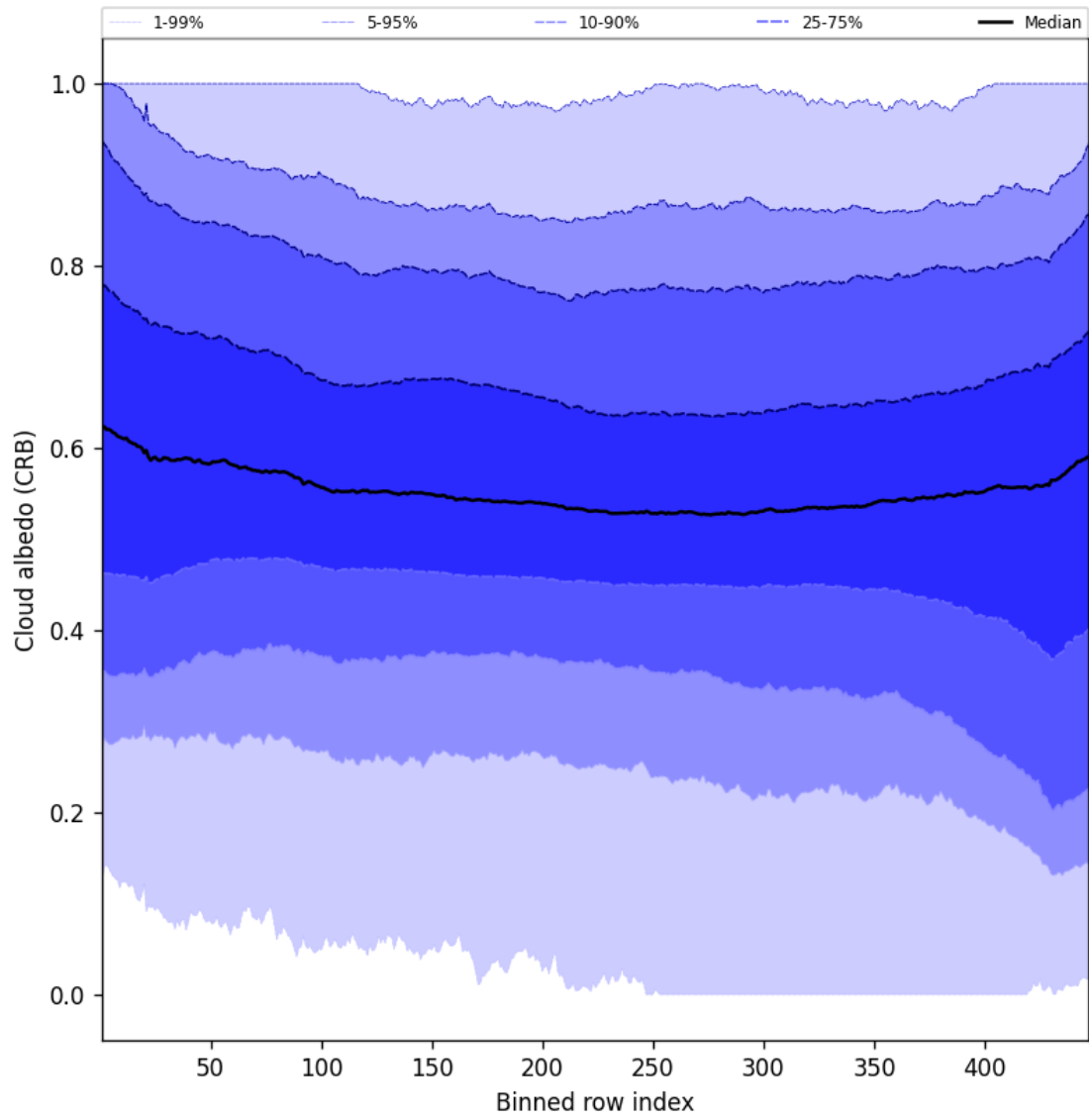
Figure 60: Along track statistics of “Cloud albedo (CRB)” for 2025-07-10 to 2025-07-12
