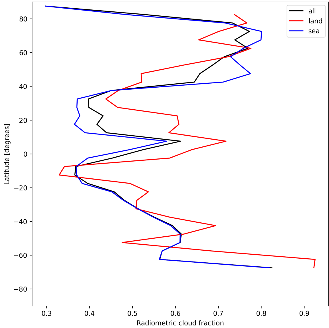
Figure 23: Zonal average of “Radiometric cloud fraction” for 2025-07-10 to 2025-07-12.
