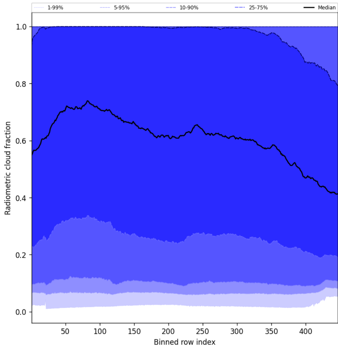
Figure 55: Along track statistics of “Radiometric cloud fraction” for 2025-07-10 to 2025-07-12
