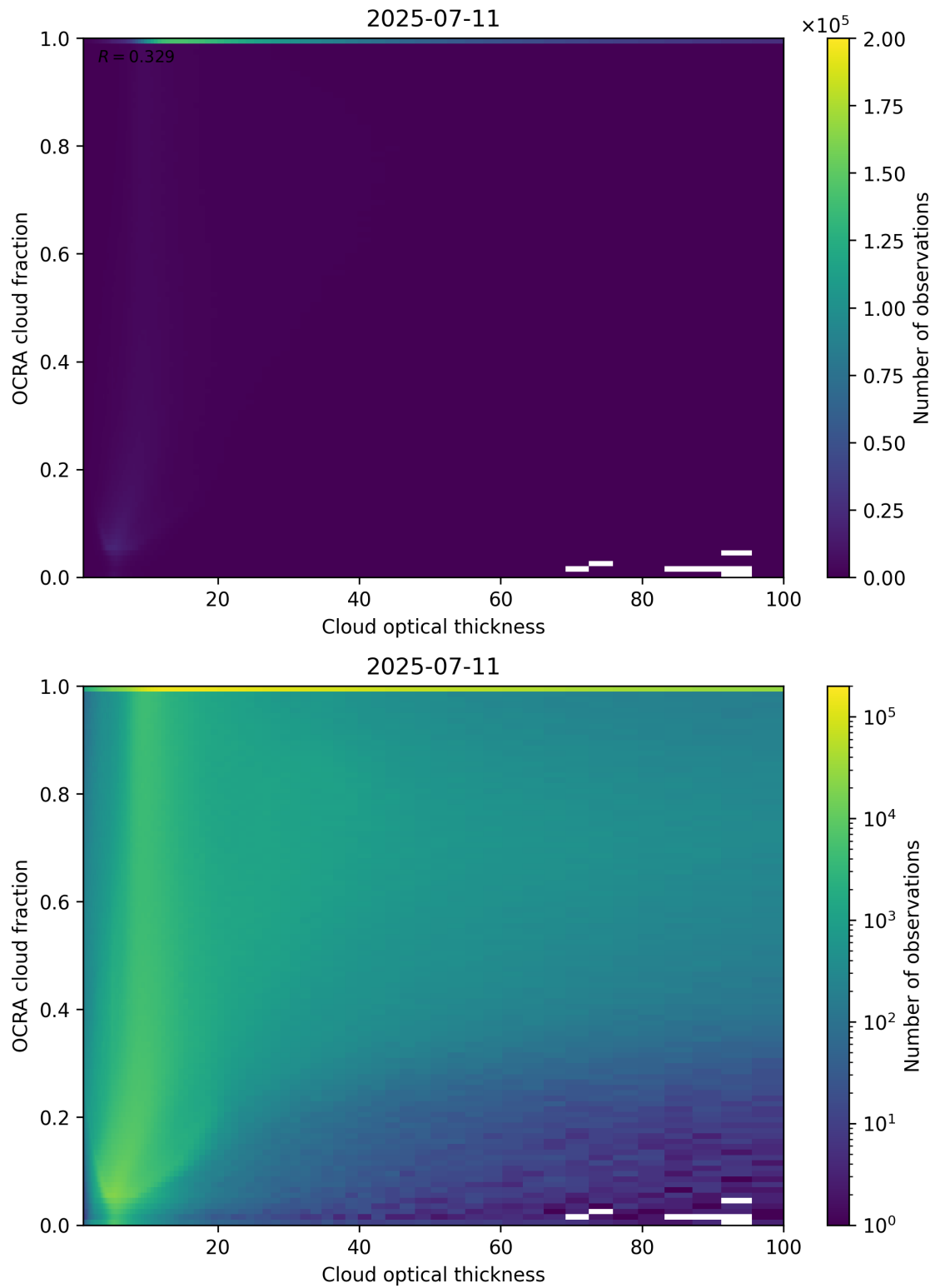
Figure 83: Scatter density plot of “Cloud optical thickness” against “OCRA cloud fraction” for 2025-07-10 to 2025-07-12.
