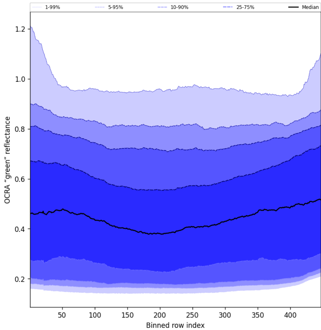
Figure 68: Along track statistics of “OCRA “green” reflectance” for 2025-07-10 to 2025-07-12
