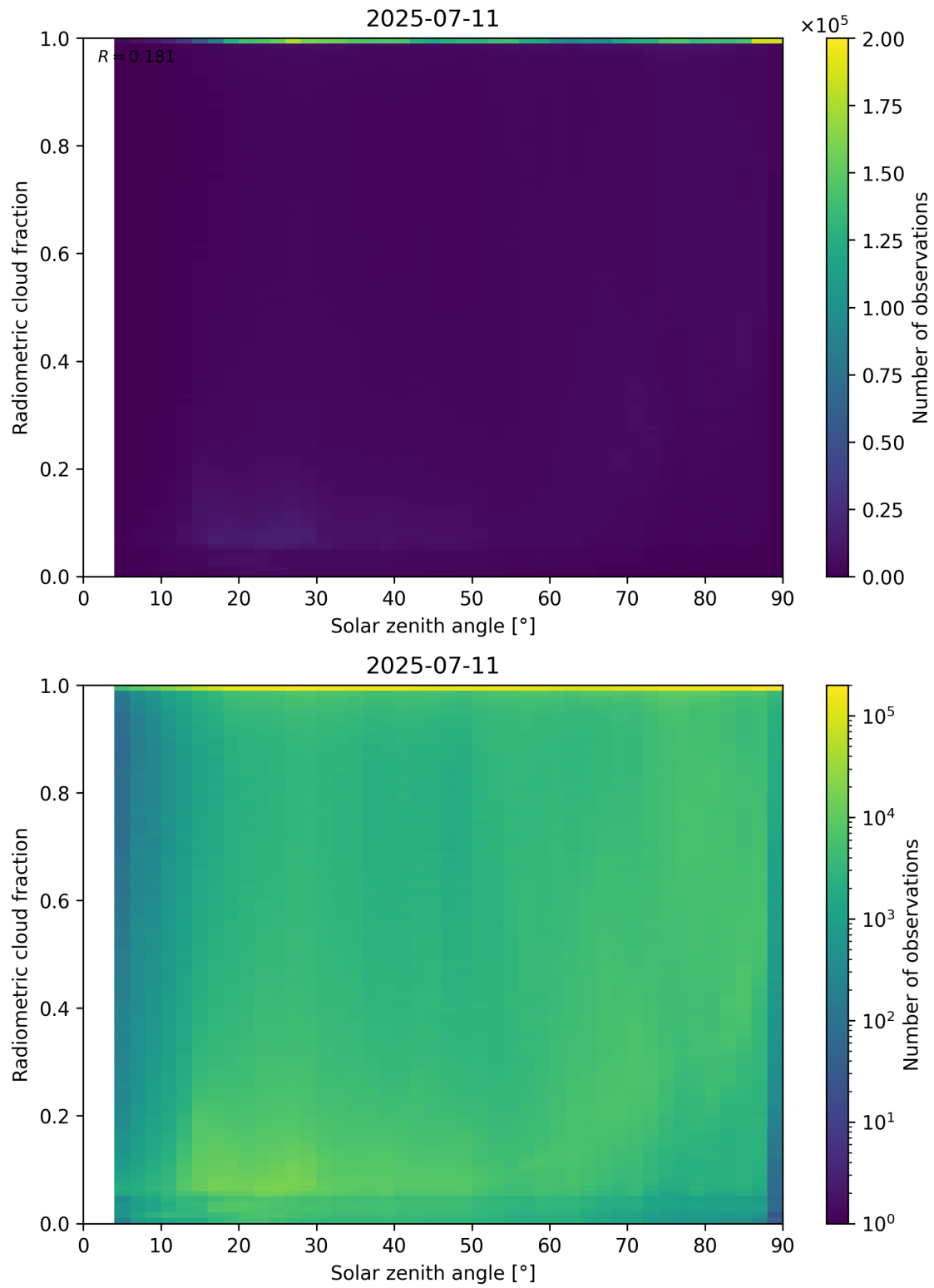
Figure 99: Scatter density plot of “Solar zenith angle” against “Radiometric cloud fraction” for 2025-07-10 to 2025-07-12.
