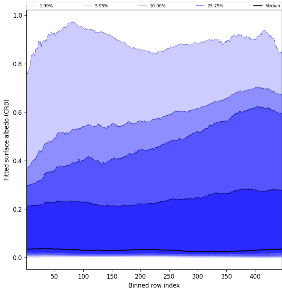
Figure 62: Along track statistics of “Fitted surface albedo (CRB)” for 2025-07-10 to 2025-07-12
