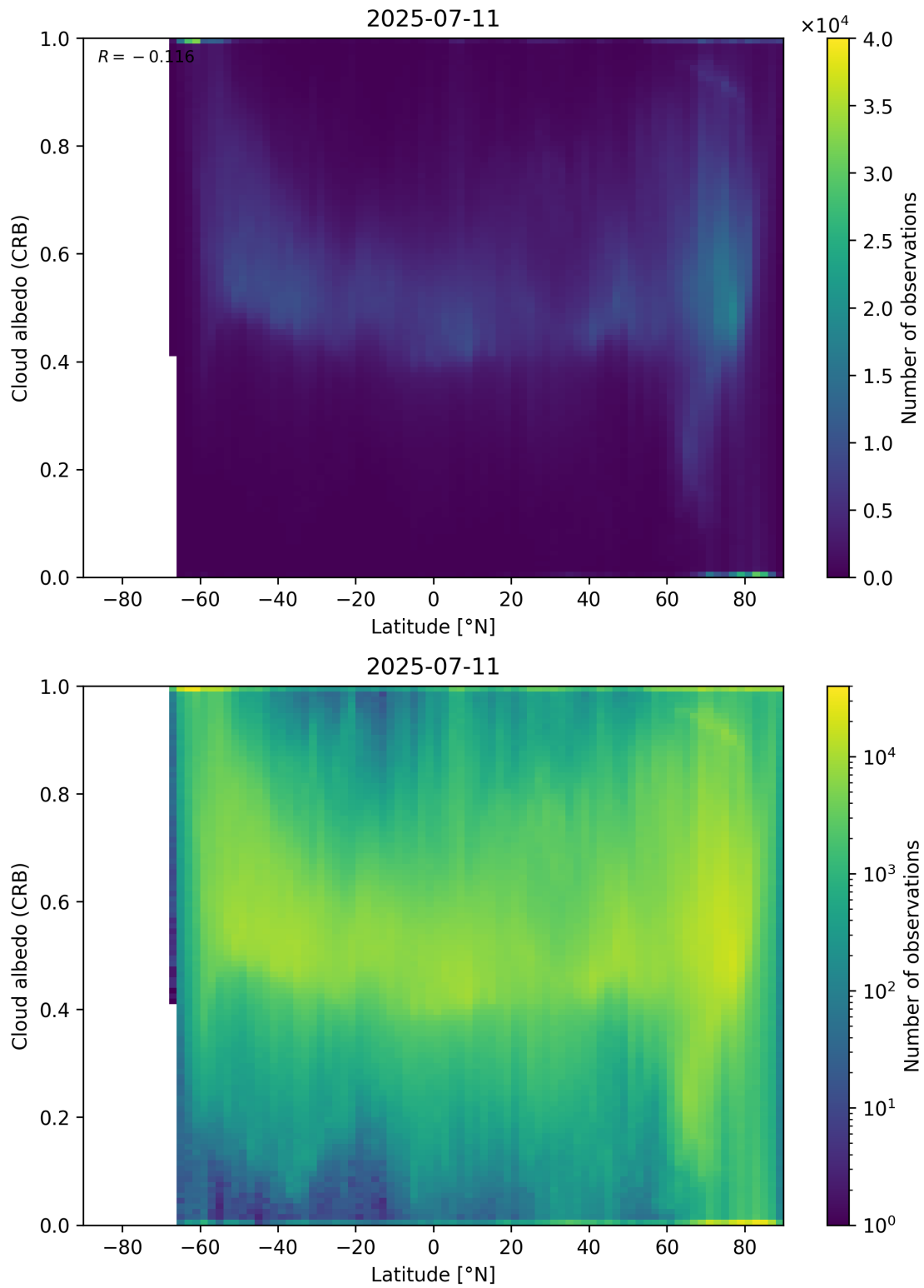
Figure 91: Scatter density plot of “Latitude” against “Cloud albedo (CRB)” for 2025-07-10 to 2025-07-12.
