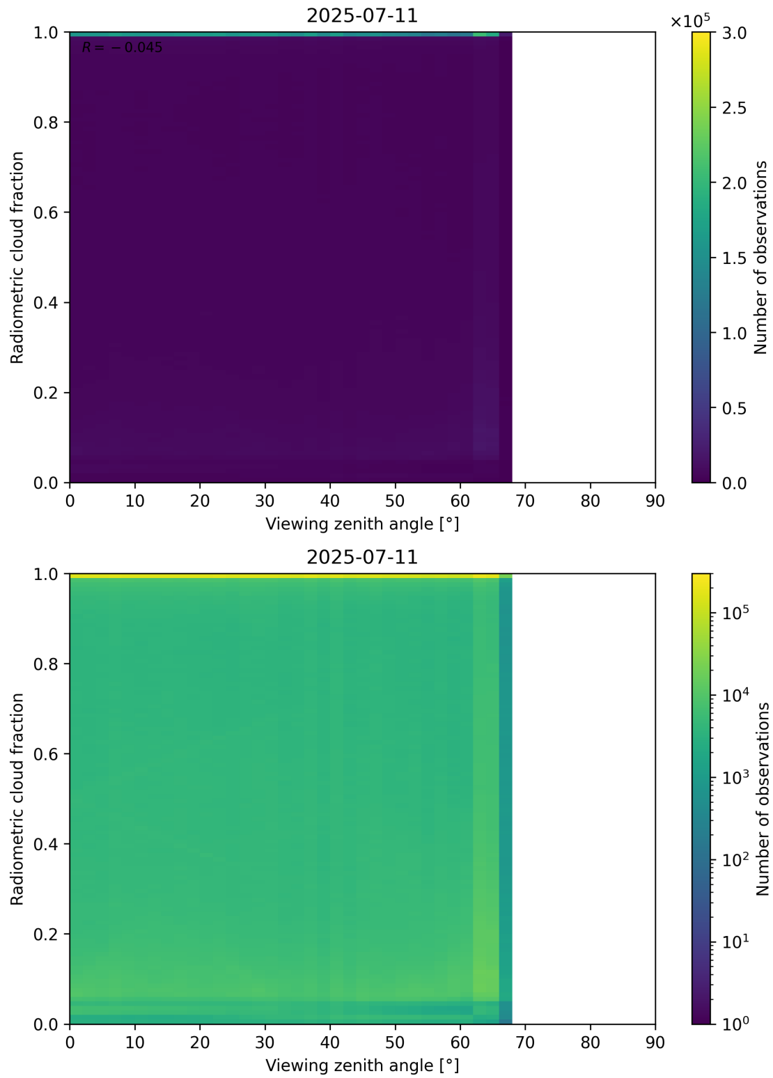
Figure 107: Scatter density plot of “Viewing zenith angle” against “Radiometric cloud fraction” for 2025-07-10 to 2025-07-12.
