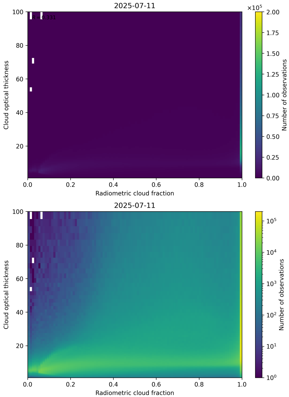
Figure 75: Scatter density plot of “Radiometric cloud fraction” against “Cloud optical thickness” for 2025-07-10 to 2025-07-12.
