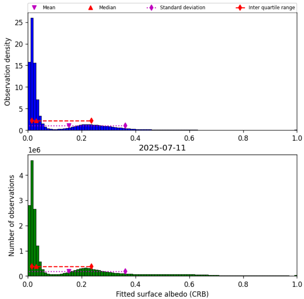
Figure 46: Histogram of “Fitted surface albedo (CRB)” for 2025-07-10 to 2025-07-12
