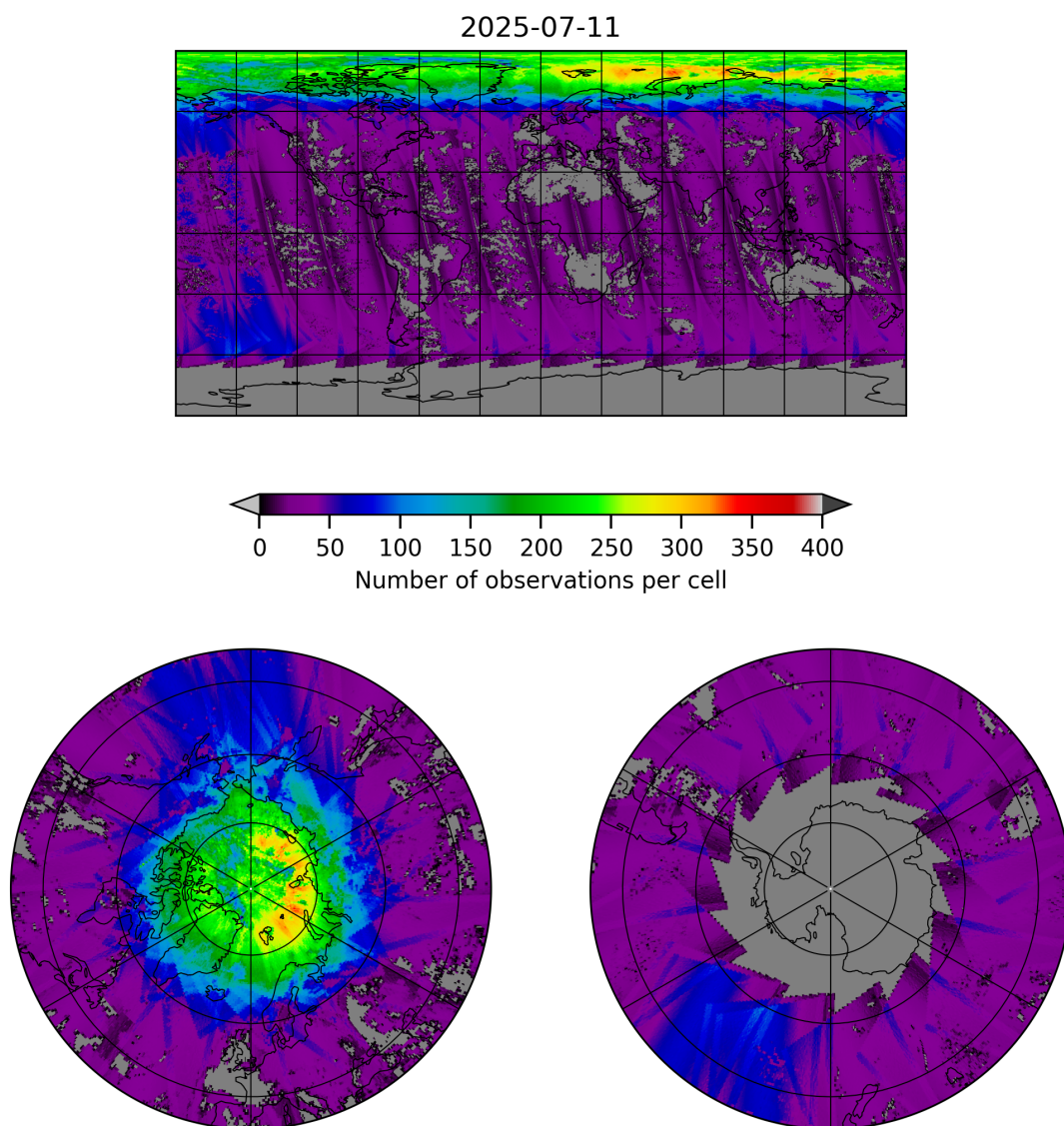
Figure 21: Map of the number of observations for 2025-07-10 to 2025-07-12
