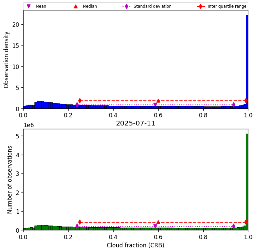
Figure 42: Histogram of “Cloud fraction (CRB)” for 2025-07-10 to 2025-07-12
