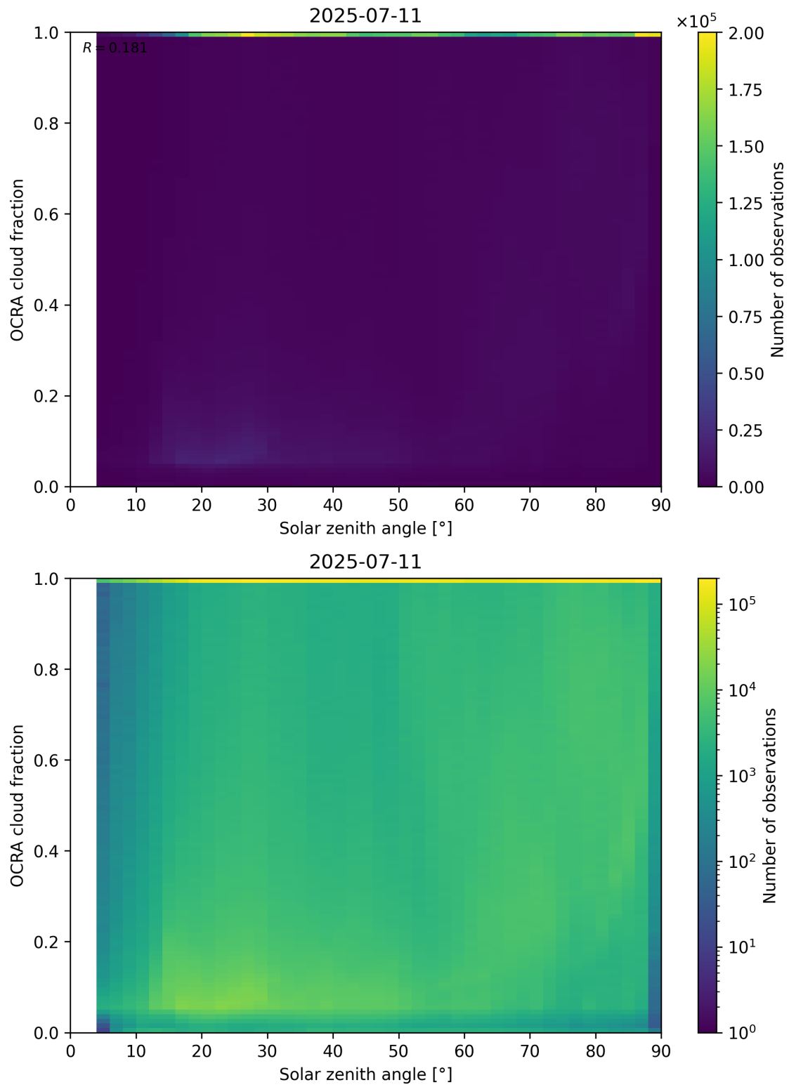
Figure 100: Scatter density plot of “Solar zenith angle” against “OCRA cloud fraction” for 2025-07-10 to 2025-07-12.
