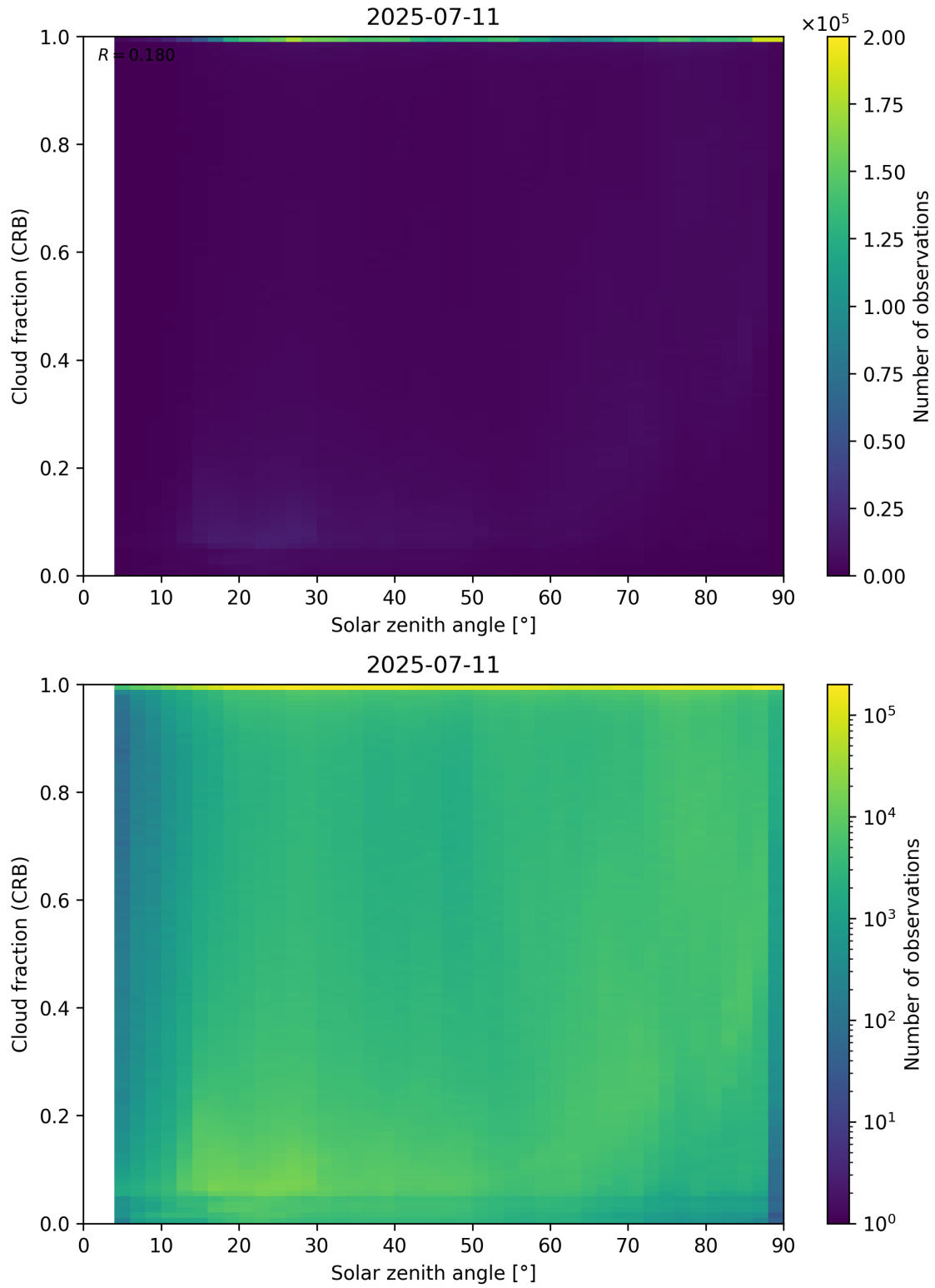
Figure 101: Scatter density plot of “Solar zenith angle” against “Cloud fraction (CRB)” for 2025-07-10 to 2025-07-12.
