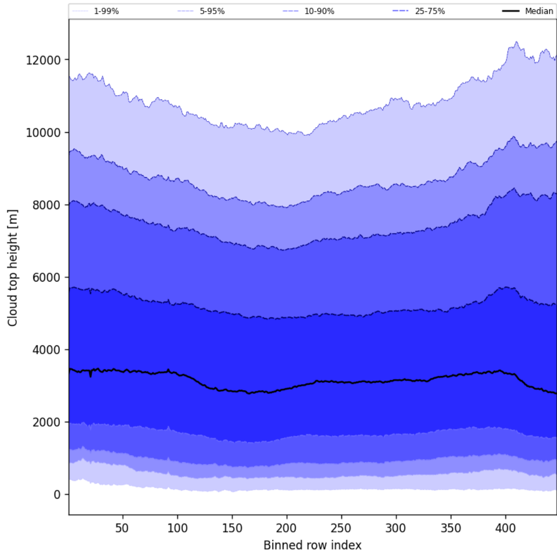
Figure 56: Along track statistics of “Cloud top height” for 2025-07-10 to 2025-07-12
