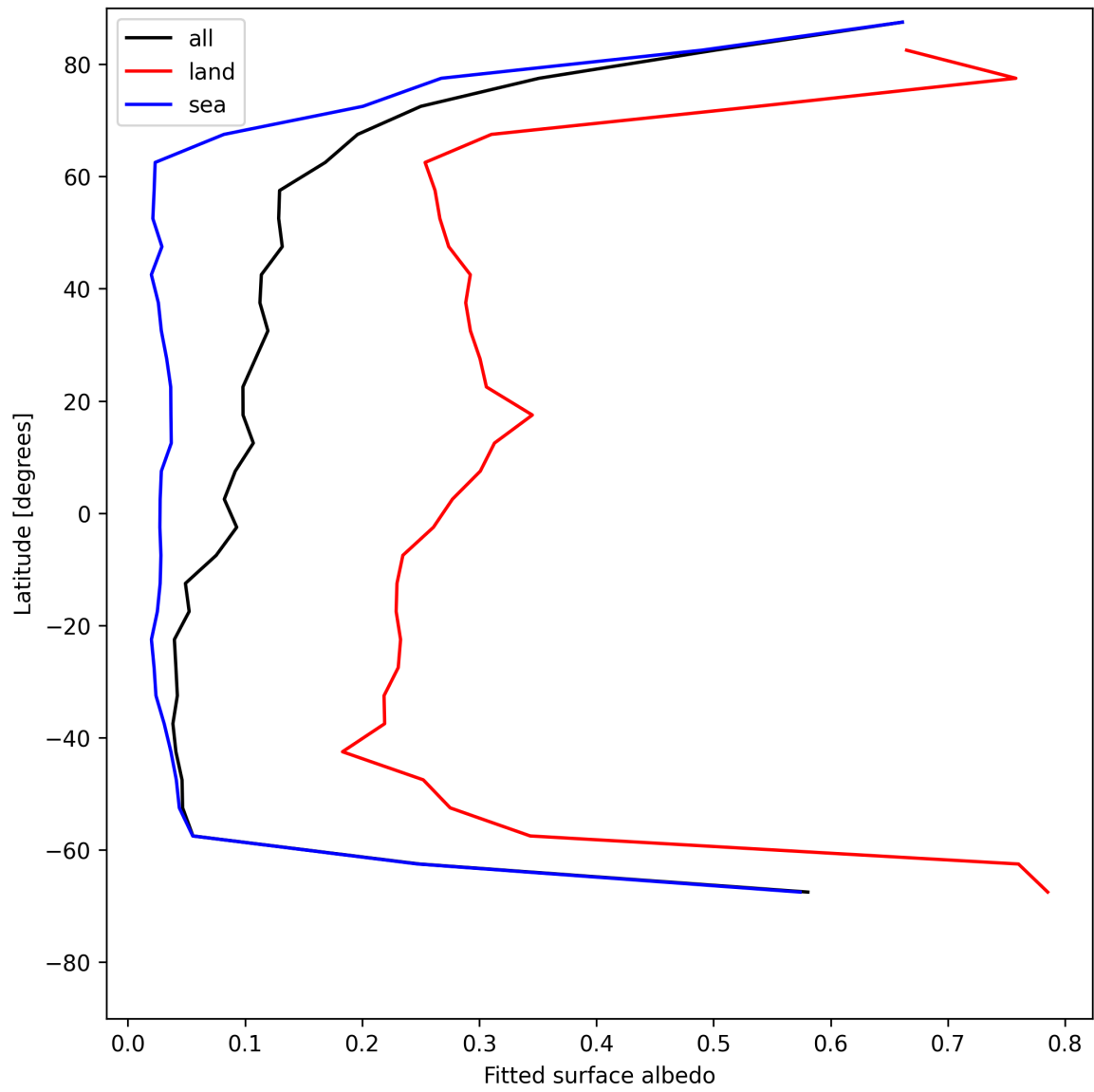
Figure 29: Zonal average of “Fitted surface albedo” for 2025-07-10 to 2025-07-12.
