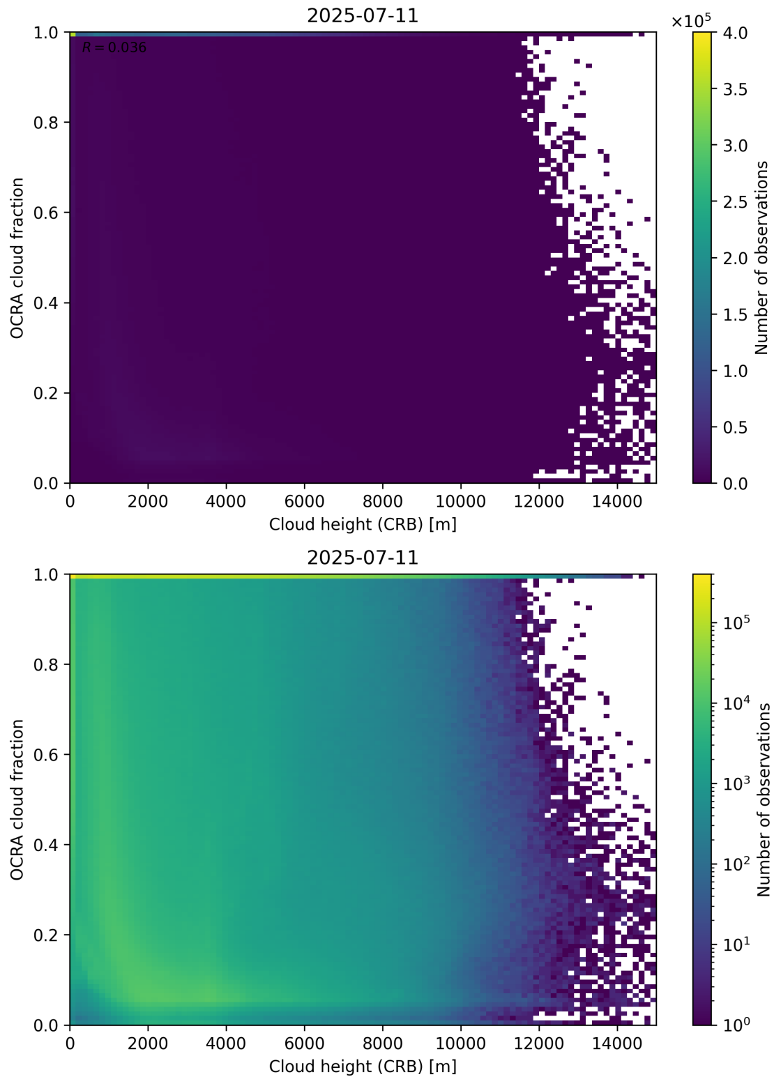
Figure 81: Scatter density plot of “Cloud height (CRB)” against “OCRA cloud fraction” for 2025-07-10 to 2025-07-12.
