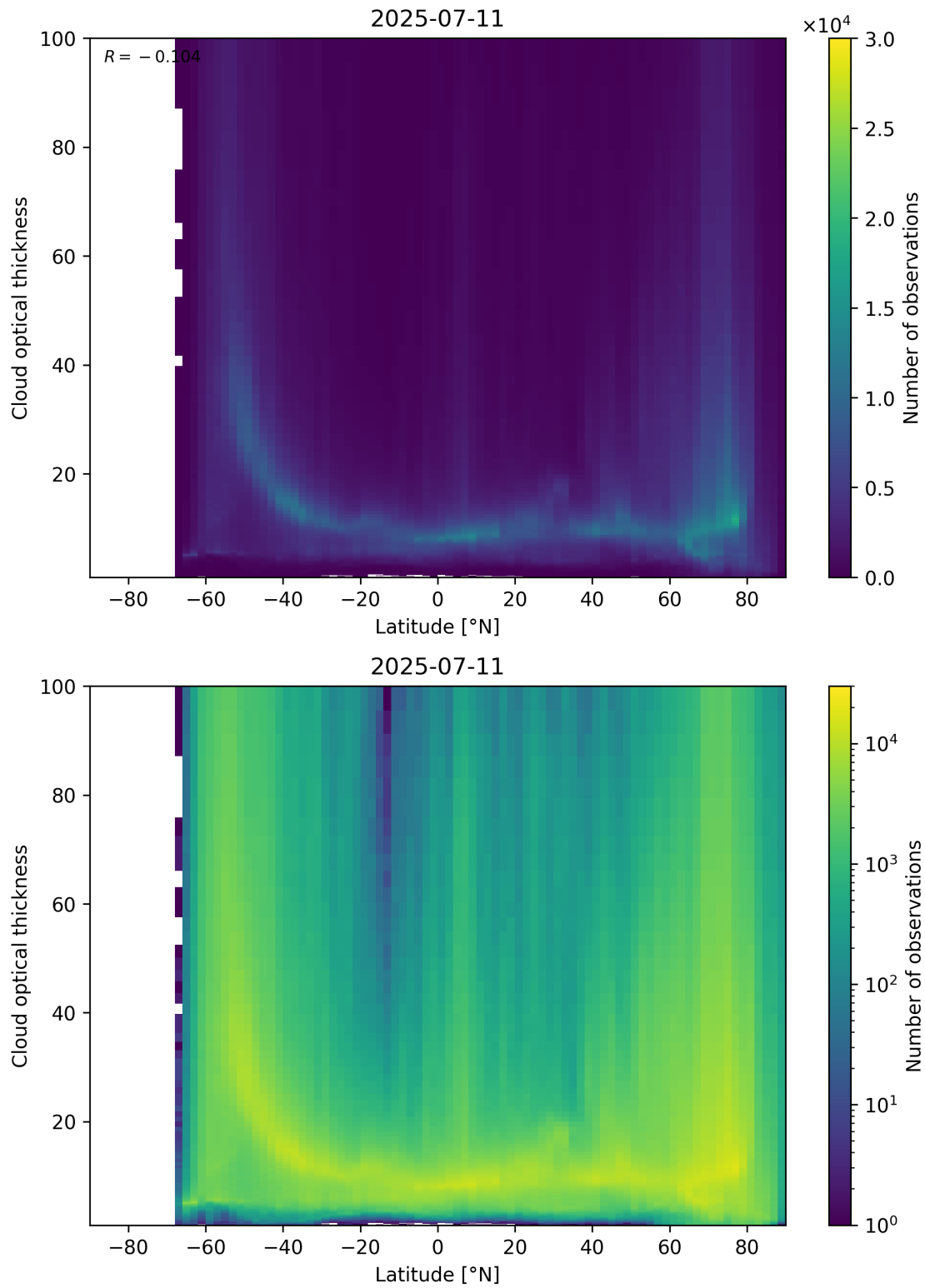
Figure 96: Scatter density plot of “Latitude” against “Cloud optical thickness” for 2025-07-10 to 2025-07-12.
