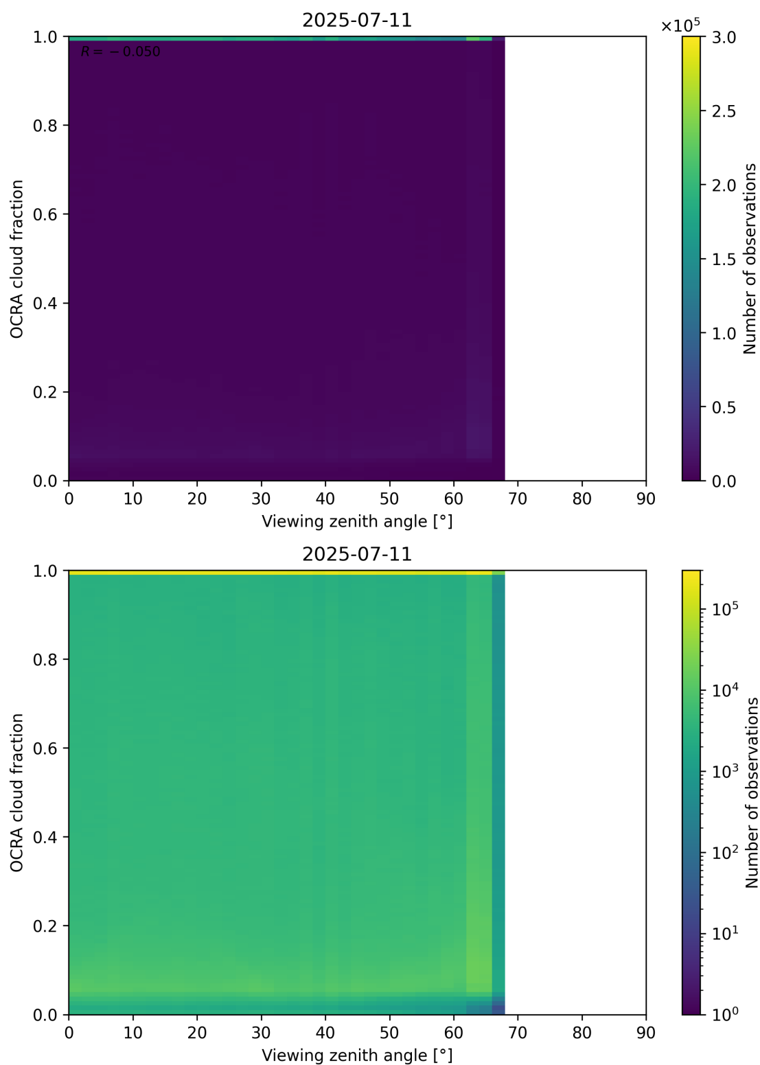
Figure 108: Scatter density plot of “Viewing zenith angle” against “OCRA cloud fraction” for 2025-07-10 to 2025-07-12.
