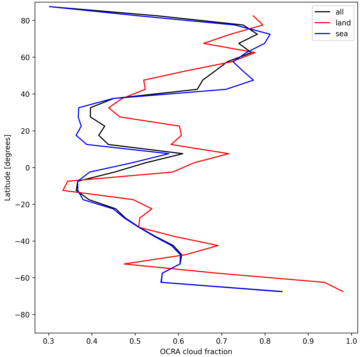
Figure 34: Zonal average of “OCRA cloud fraction” for 2025-07-10 to 2025-07-12.
