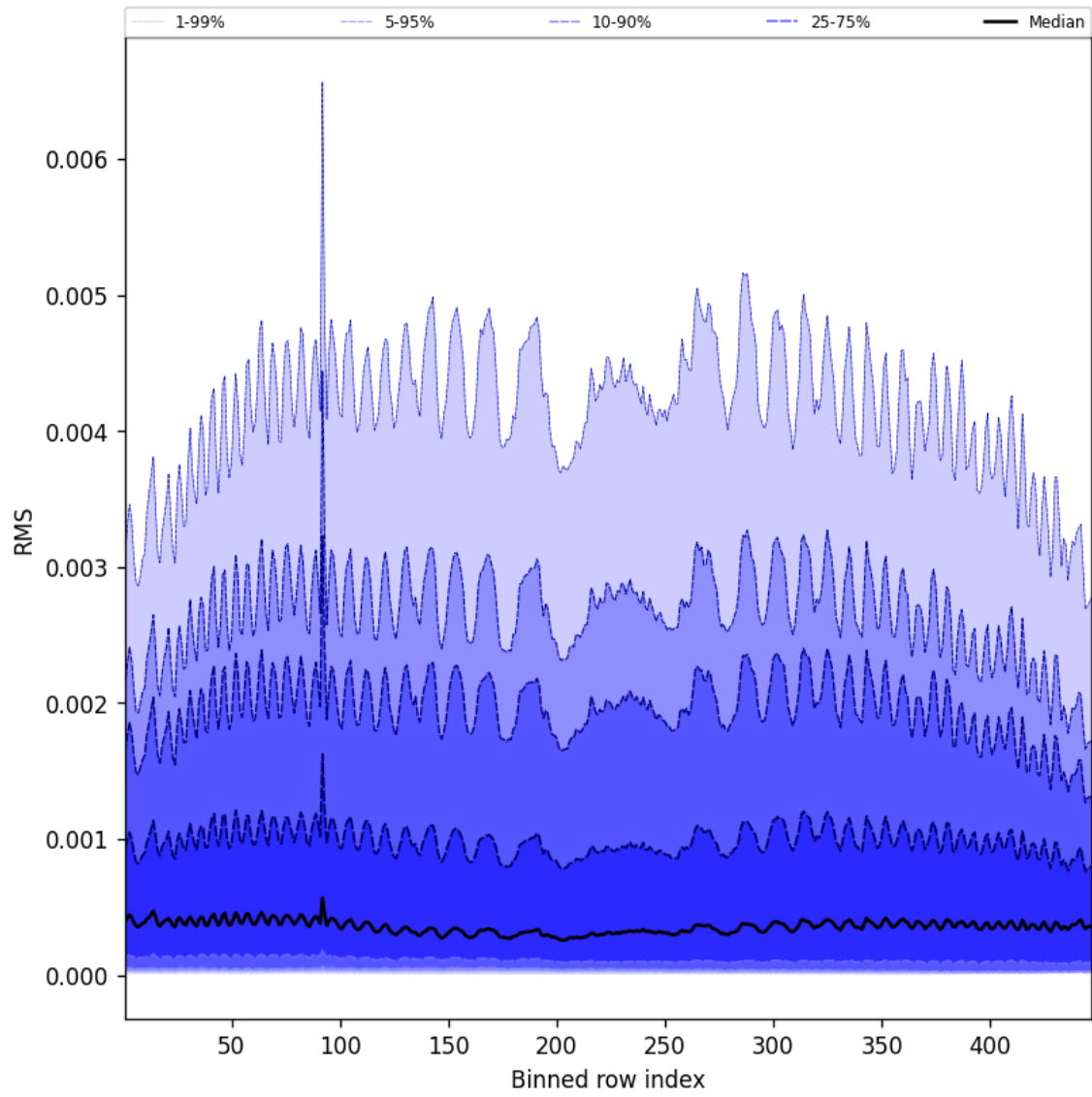
Figure 63: Along track statistics of “RMS” for 2025-07-10 to 2025-07-12
