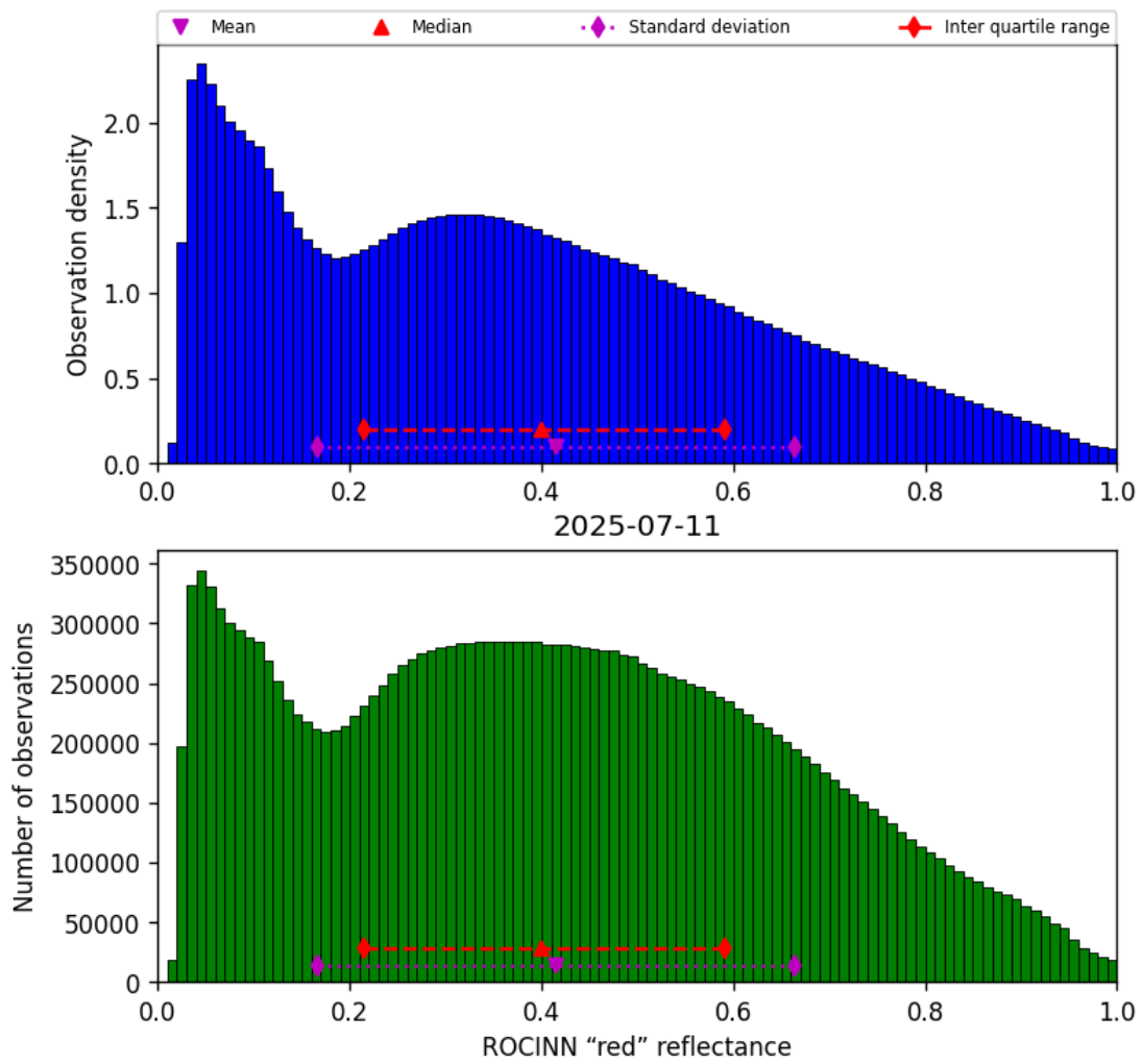
Figure 53: Histogram of “ROCINN “red” reflectance” for 2025-07-10 to 2025-07-12
