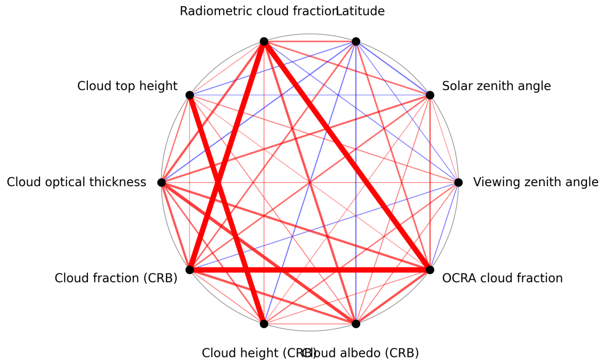
Figure 1: Map of correlation graph for 2025-07-10 to 2025-07-12.
