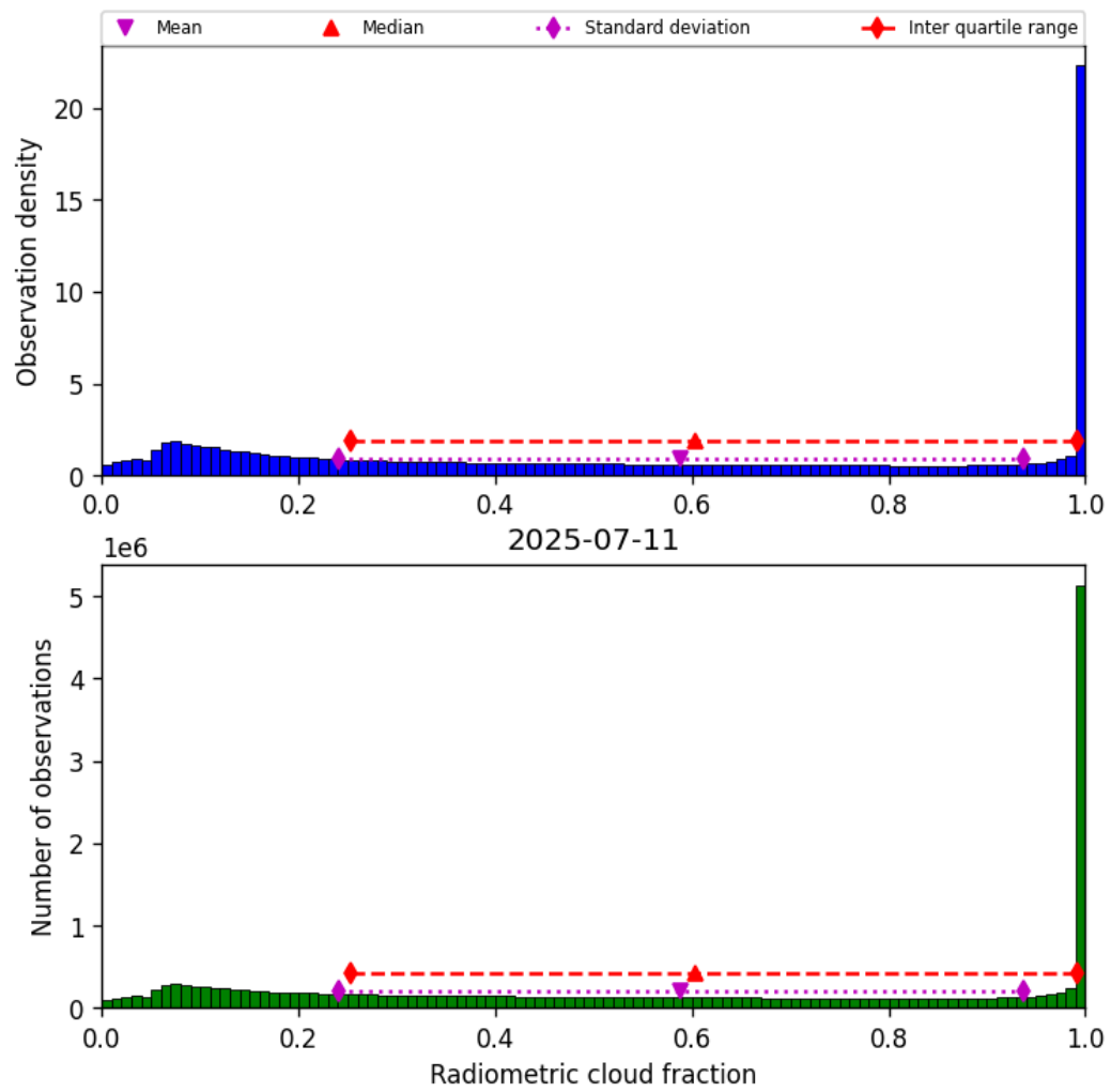
Figure 39: Histogram of “Radiometric cloud fraction” for 2025-07-10 to 2025-07-12
