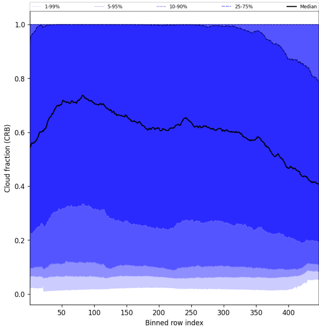
Figure 58: Along track statistics of "Cloud fraction (CRB)" for 2025-07-10 to 2025-07-12
