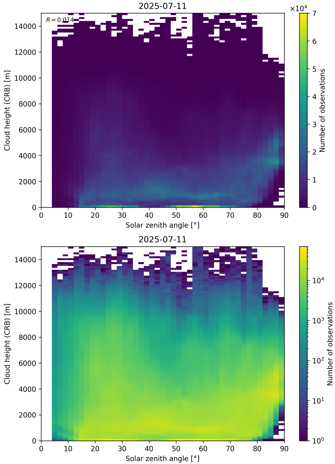
Figure 102: Scatter density plot of “Solar zenith angle” against “Cloud height (CRB)” for 2025-07-10 to 2025-07-12.
