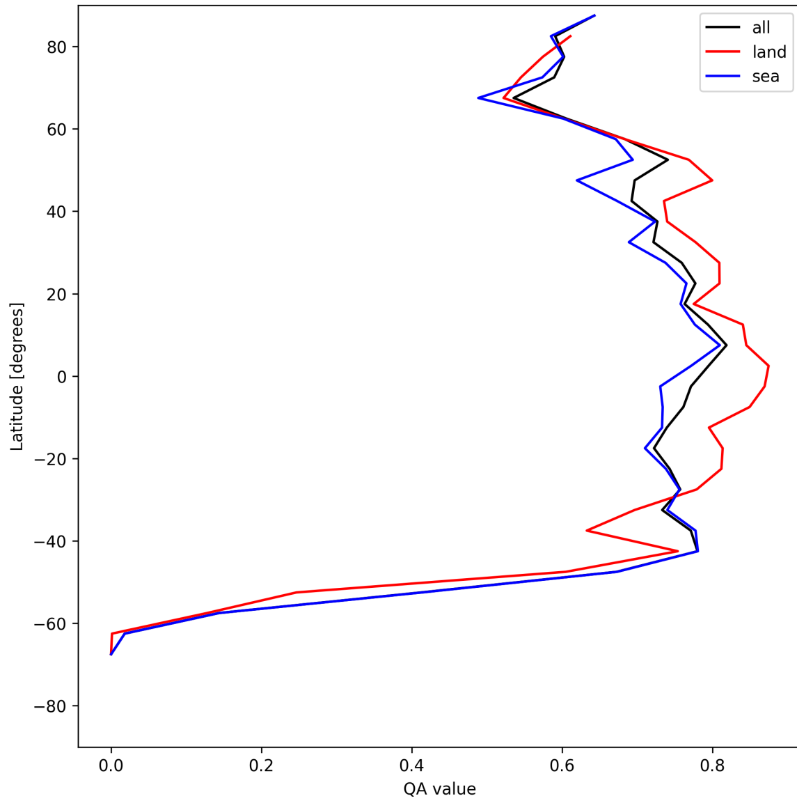
Figure 22: Zonal average of “QA value” for 2025-07-10 to 2025-07-12.
