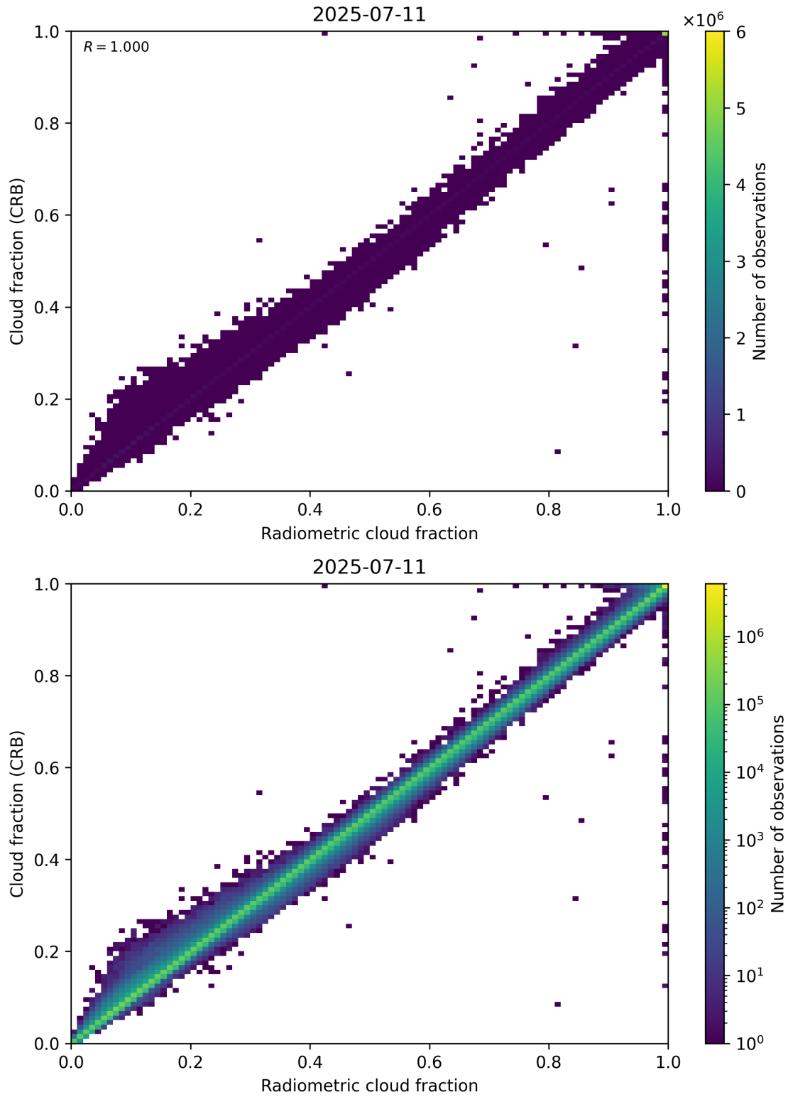
Figure 73: Scatter density plot of “Radiometric cloud fraction” against “Cloud fraction (CRB)” for 2025-07-10 to 2025-07-12.
