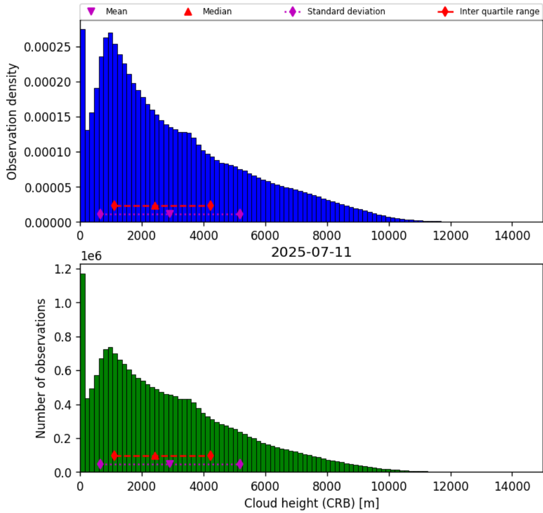
Figure 43: Histogram of “Cloud height (CRB)” for 2025-07-10 to 2025-07-12
