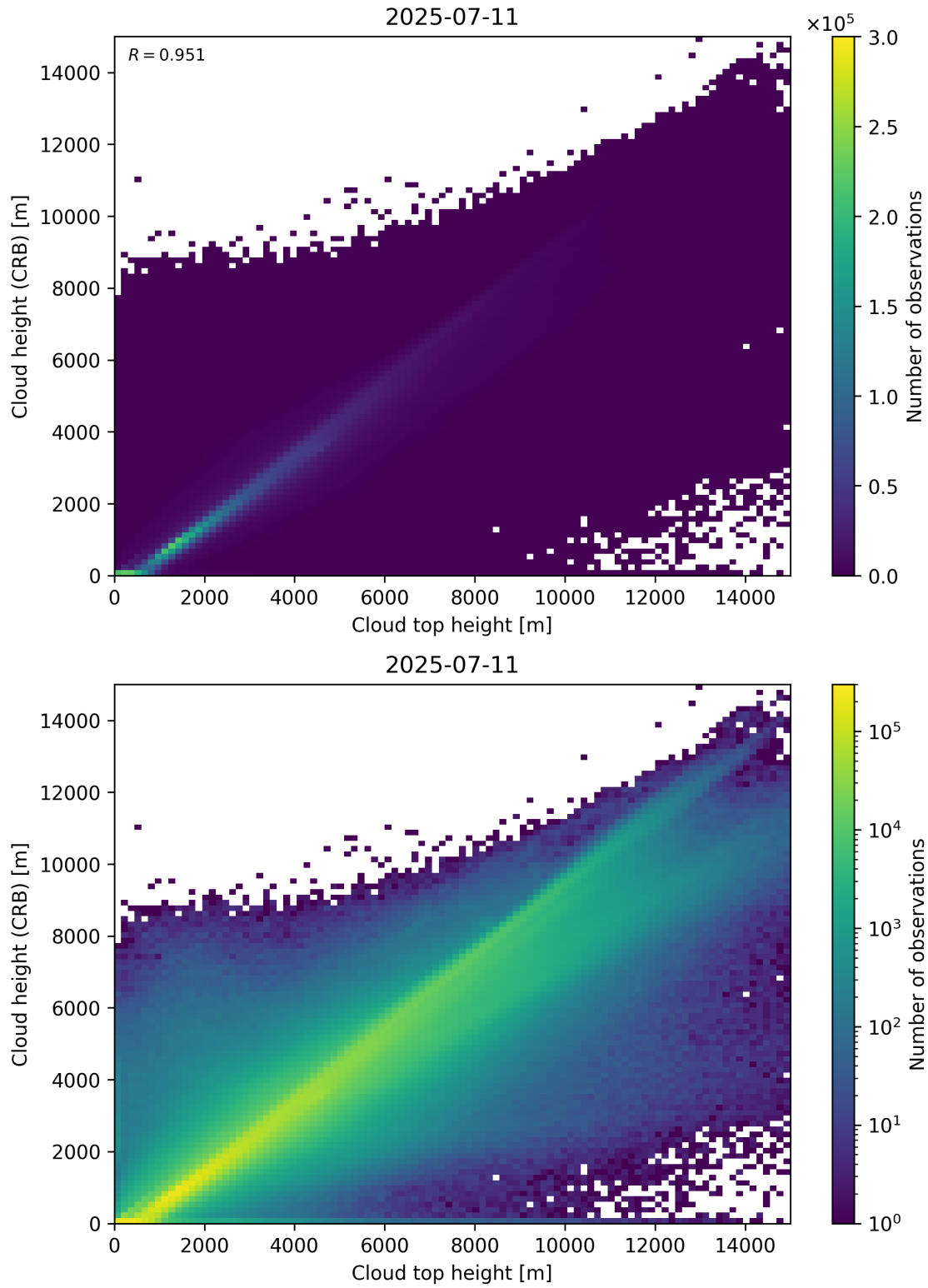
Figure 89: Scatter density plot of “Cloud top height” against “Cloud height (CRB)” for 2025-07-10 to 2025-07-12.
