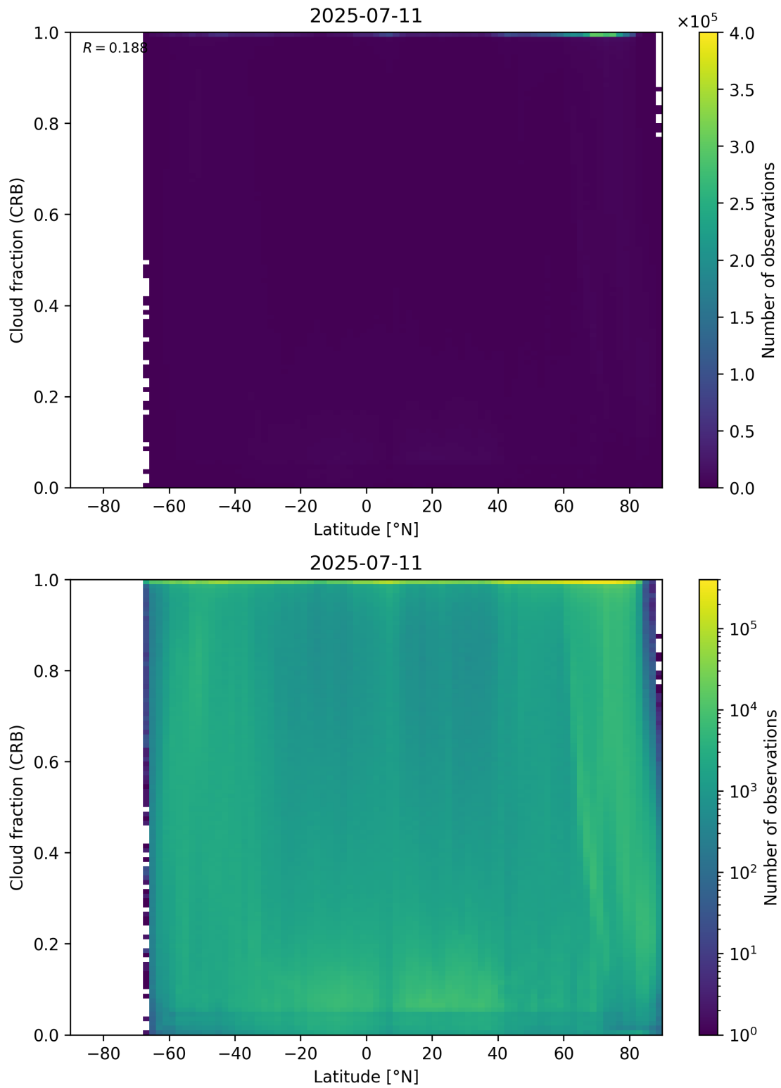
Figure 94: Scatter density plot of “Latitude” against “Cloud fraction (CRB)” for 2025-07-10 to 2025-07-12.
