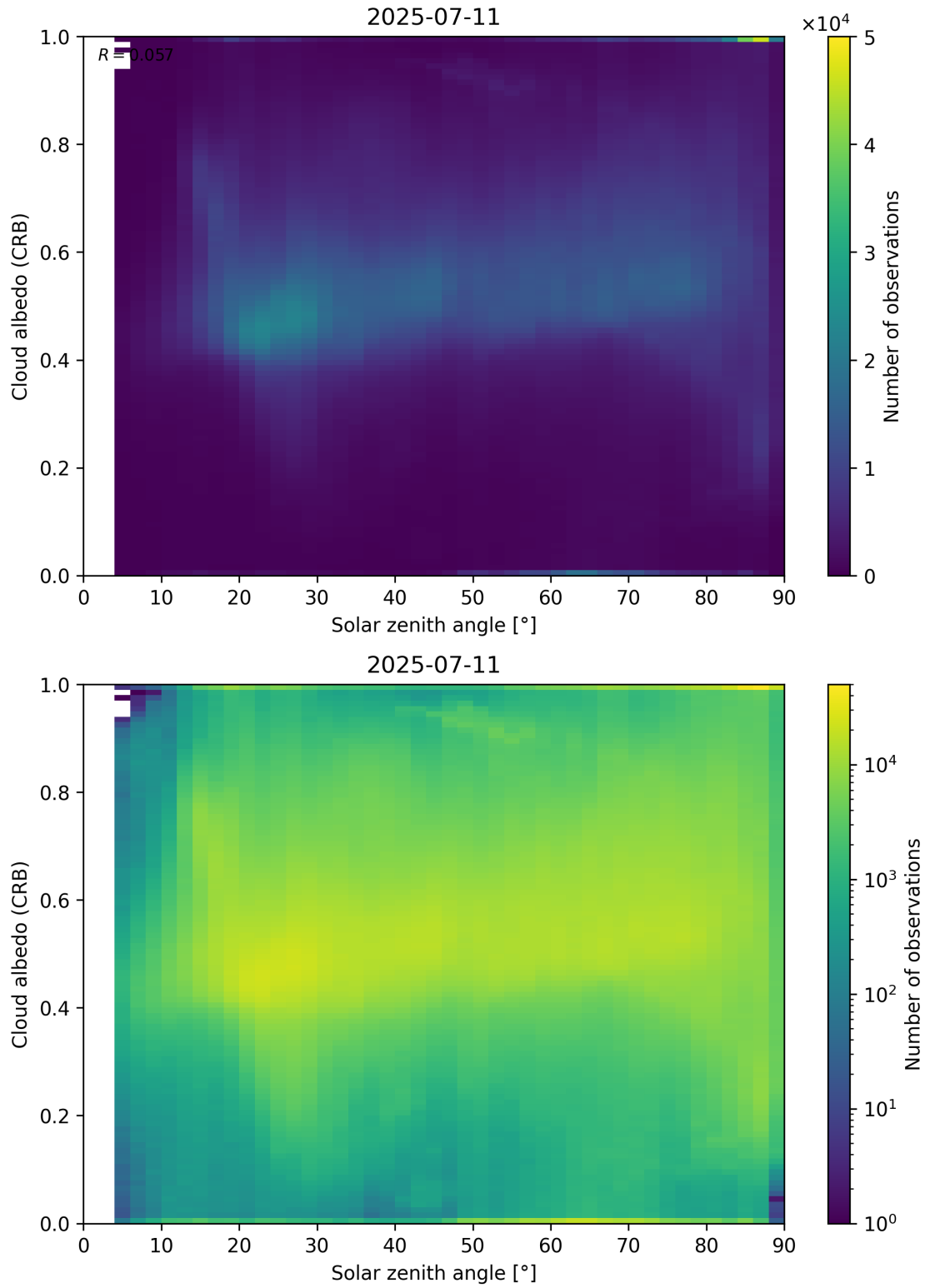
Figure 98: Scatter density plot of “Solar zenith angle” against “Cloud albedo (CRB)” for 2025-07-10 to 2025-07-12.
