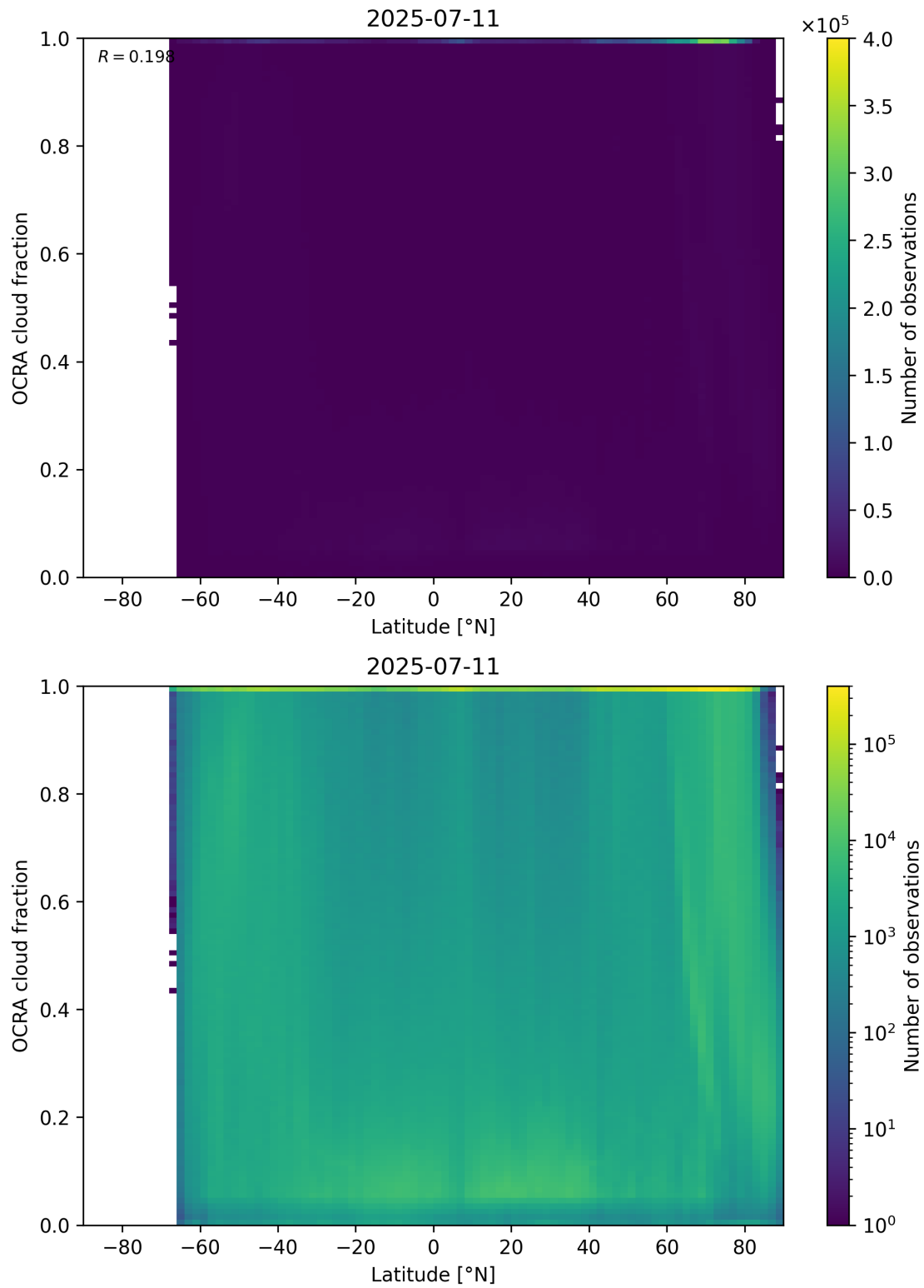
Figure 93: Scatter density plot of “Latitude” against “OCRA cloud fraction” for 2025-07-10 to 2025-07-12.
