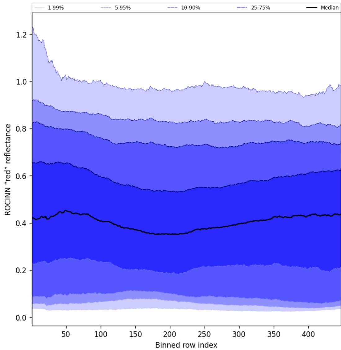
Figure 69: Along track statistics of “ROCINN “red” reflectance” for 2025-07-10 to 2025-07-12
