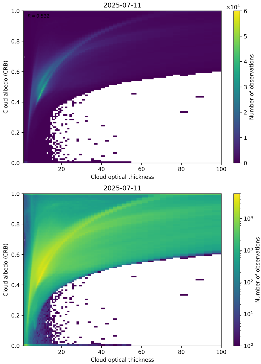
Figure 82: Scatter density plot of “Cloud optical thickness” against “Cloud albedo (CRB)” for 2025-07-10 to 2025-07-12.
