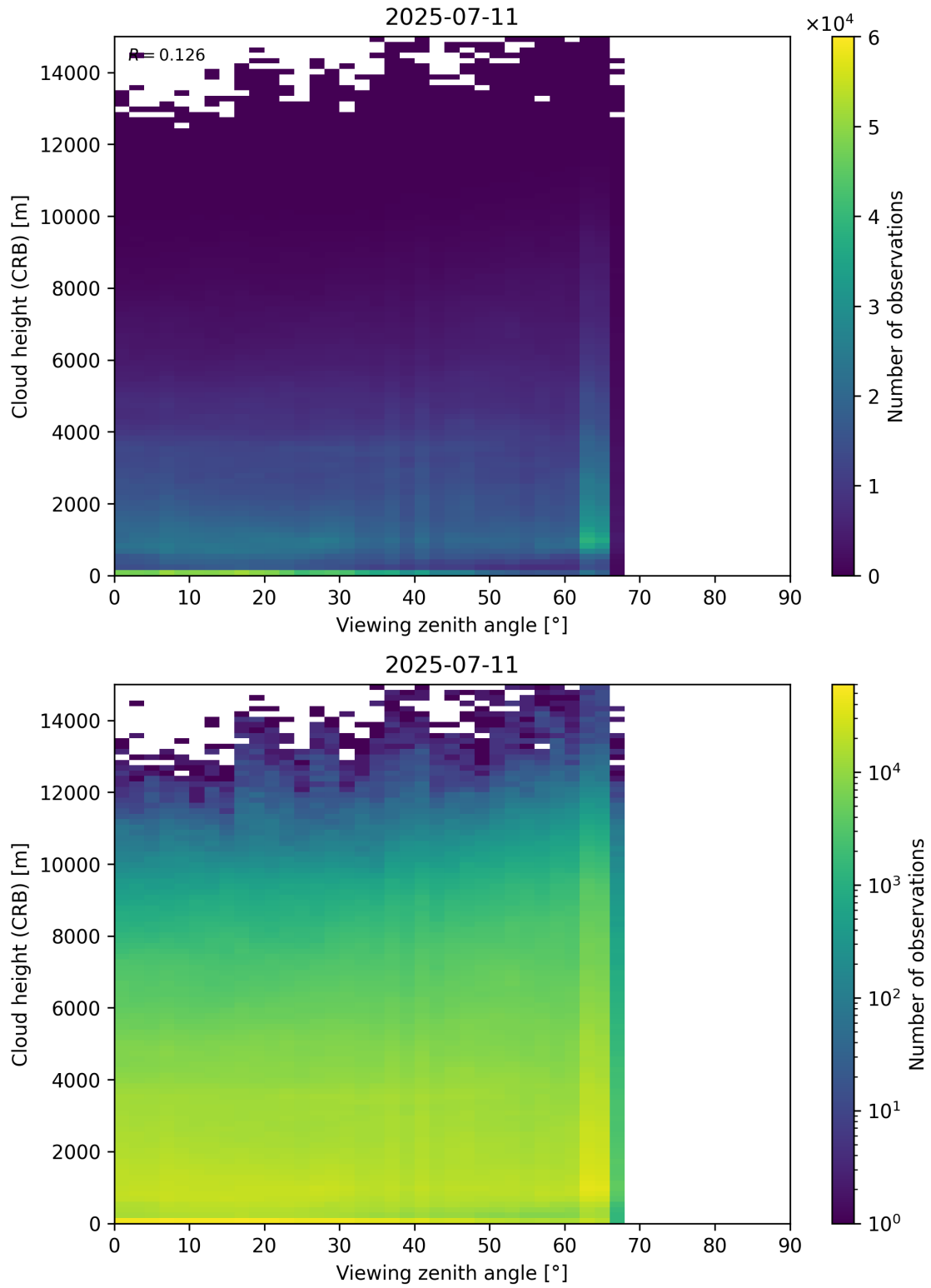
Figure 110: Scatter density plot of “Viewing zenith angle” against “Cloud height (CRB)” for 2025-07-10 to 2025-07-12.
