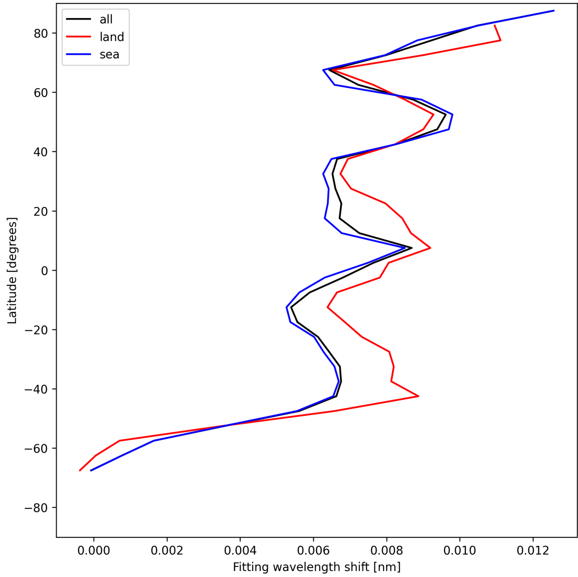
Figure 33: Zonal average of “Fitting wavelength shift” for 2025-07-10 to 2025-07-12.
