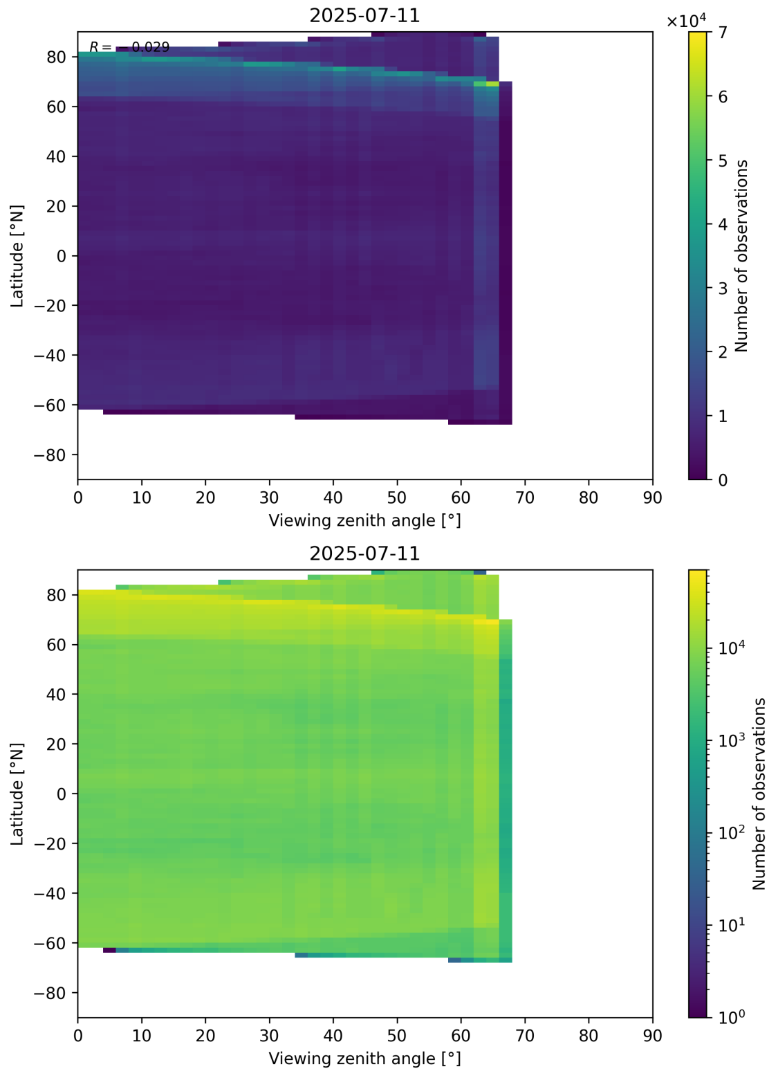
Figure 113: Scatter density plot of “Viewing zenith angle” against “Latitude” for 2025-07-10 to 2025-07-12.
