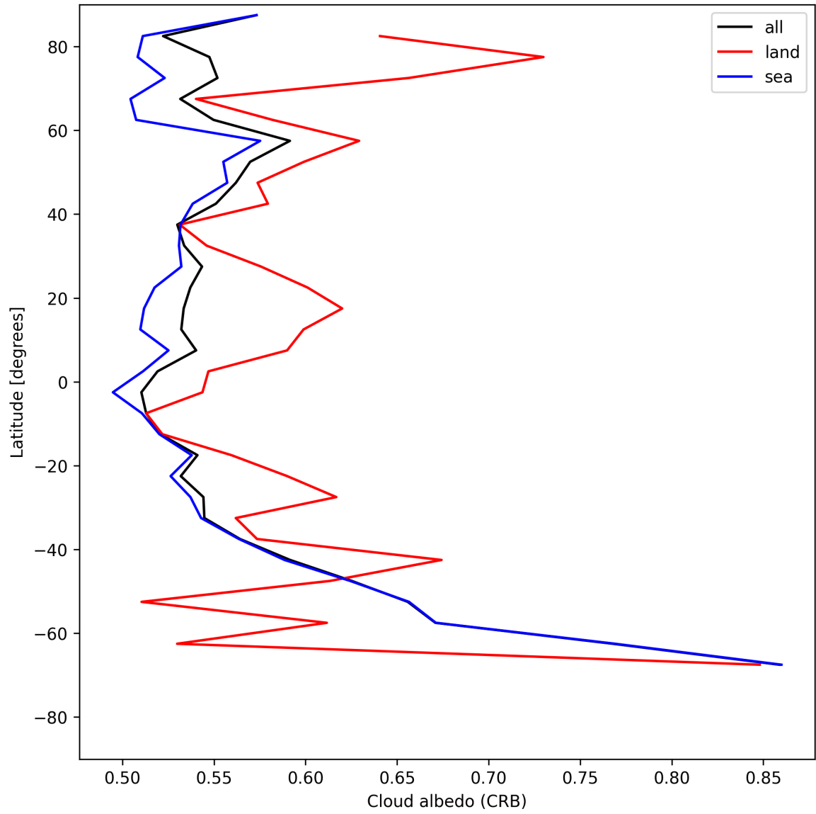
Figure 28: Zonal average of “Cloud albedo (CRB)” for 2025-07-10 to 2025-07-12.
