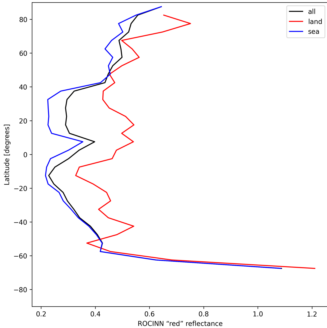
Figure 37: Zonal average of “ROCINN “red” reflectance” for 2025-07-10 to 2025-07-12.
