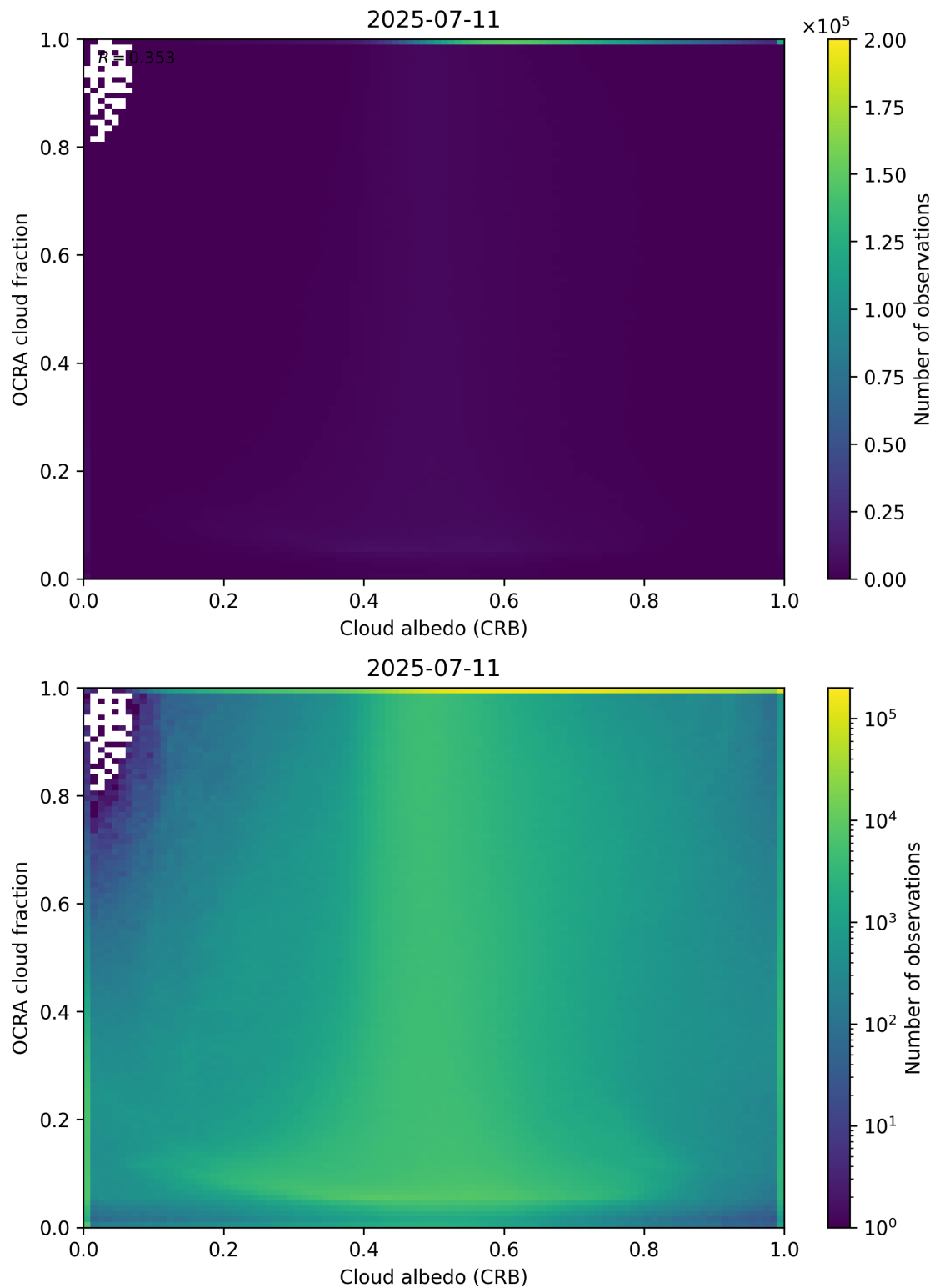
Figure 70: Scatter density plot of “Cloud albedo (CRB)” against “OCRA cloud fraction” for 2025-07-10 to 2025-07-12.
