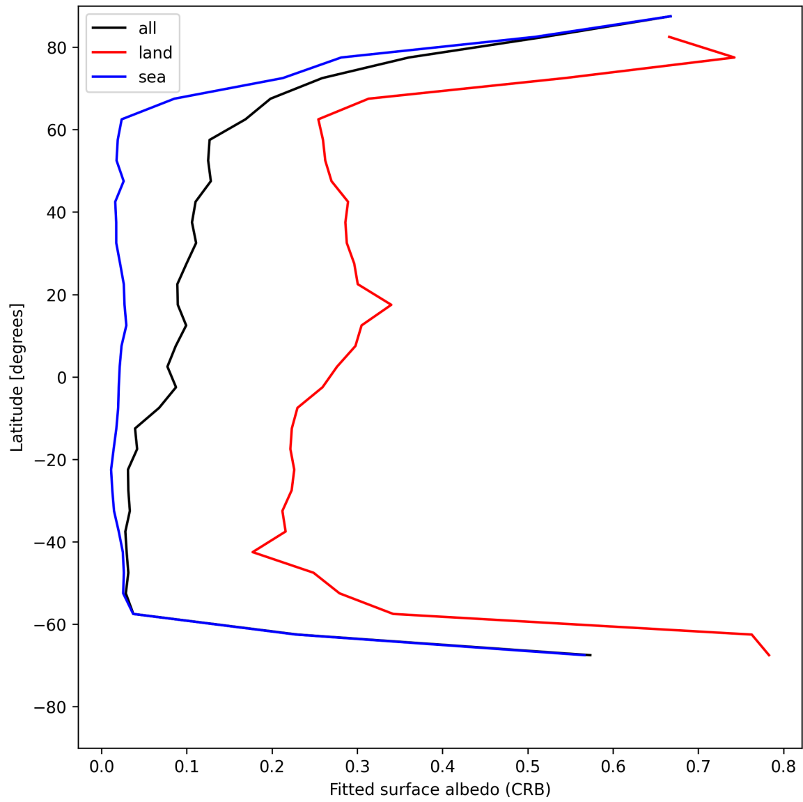
Figure 30: Zonal average of “Fitted surface albedo (CRB)” for 2025-07-10 to 2025-07-12.
