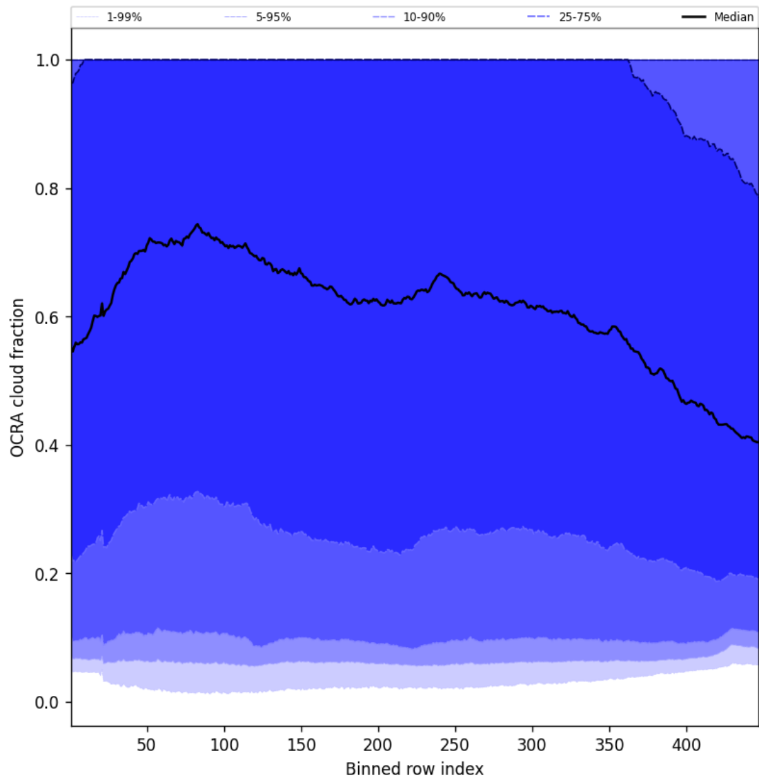
Figure 66: Along track statistics of “OCRA cloud fraction” for 2025-07-10 to 2025-07-12
