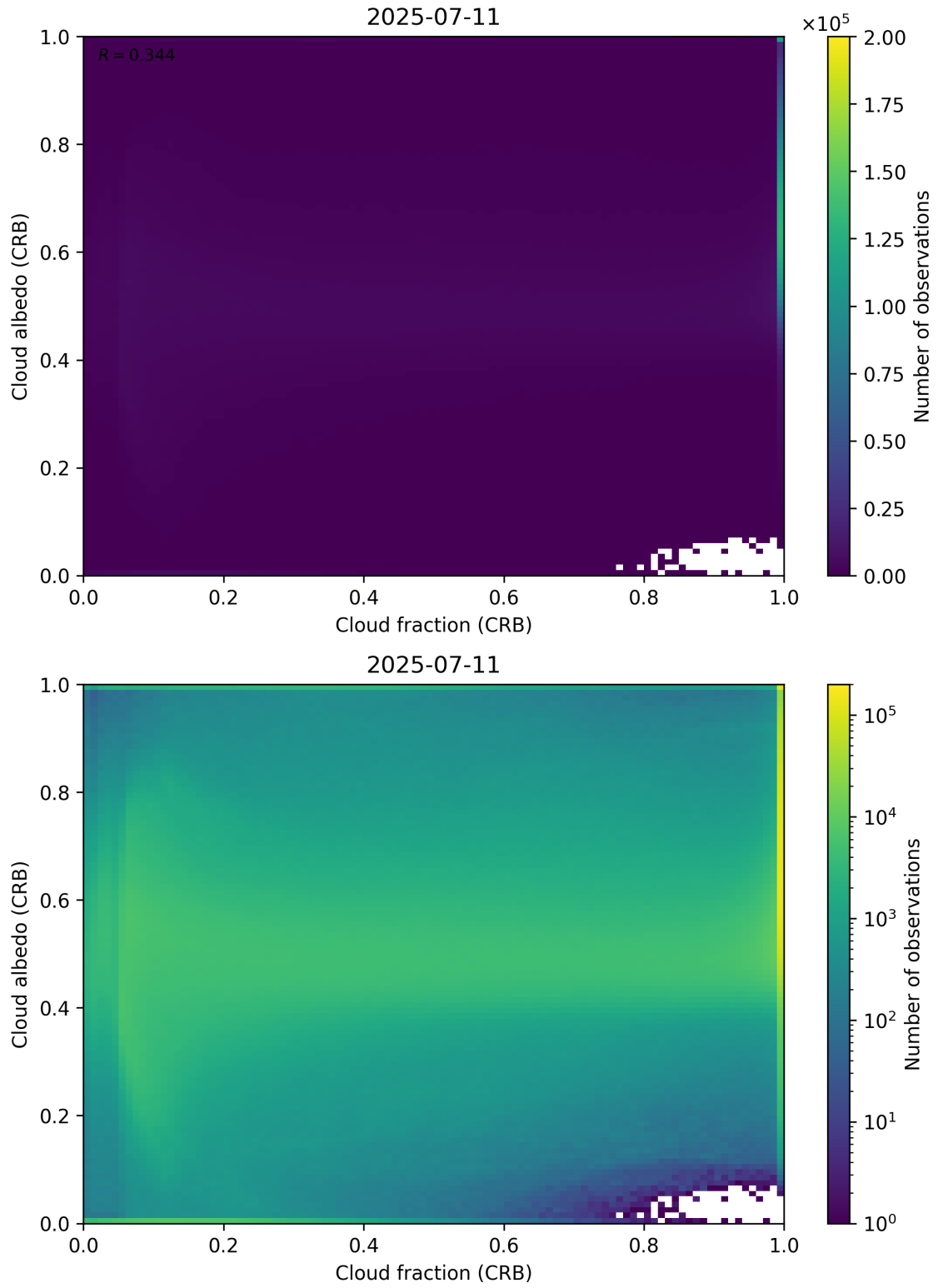
Figure 77: Scatter density plot of “Cloud fraction (CRB)” against “Cloud albedo (CRB)” for 2025-07-10 to 2025-07-12.
