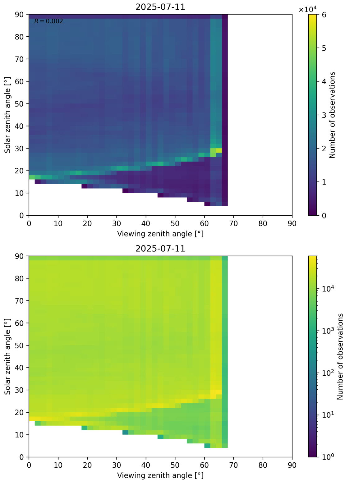
Figure 114: Scatter density plot of “Viewing zenith angle” against “Solar zenith angle” for 2025-07-10 to 2025-07-12.
