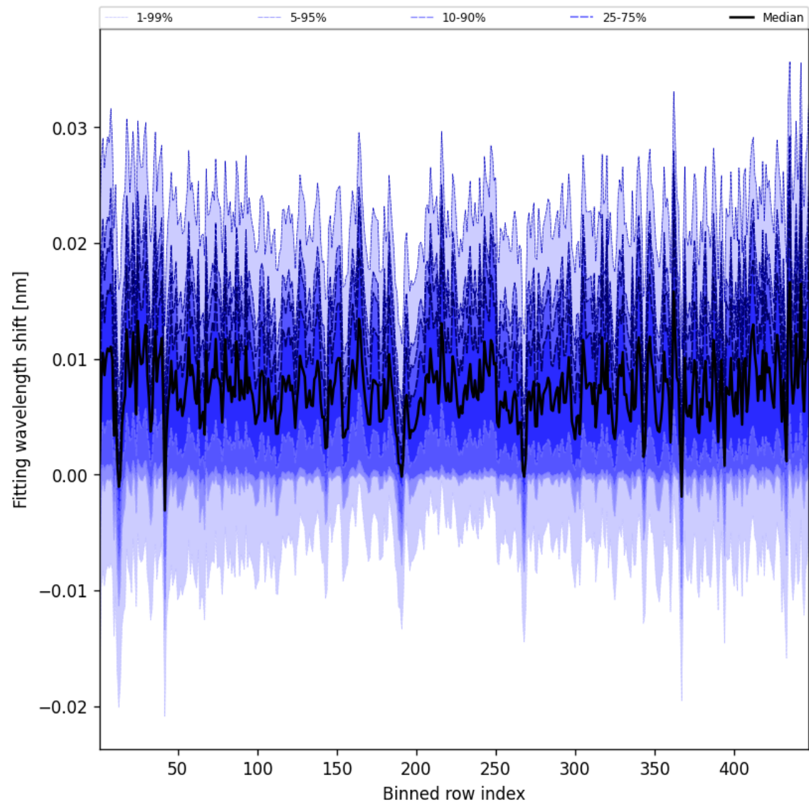
Figure 65: Along track statistics of “Fitting wavelength shift” for 2025-07-10 to 2025-07-12
