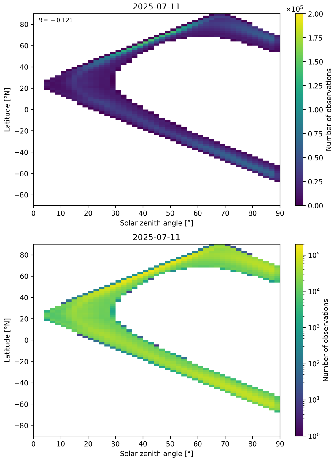
Figure 105: Scatter density plot of “Solar zenith angle” against “Latitude” for 2025-07-10 to 2025-07-12.
