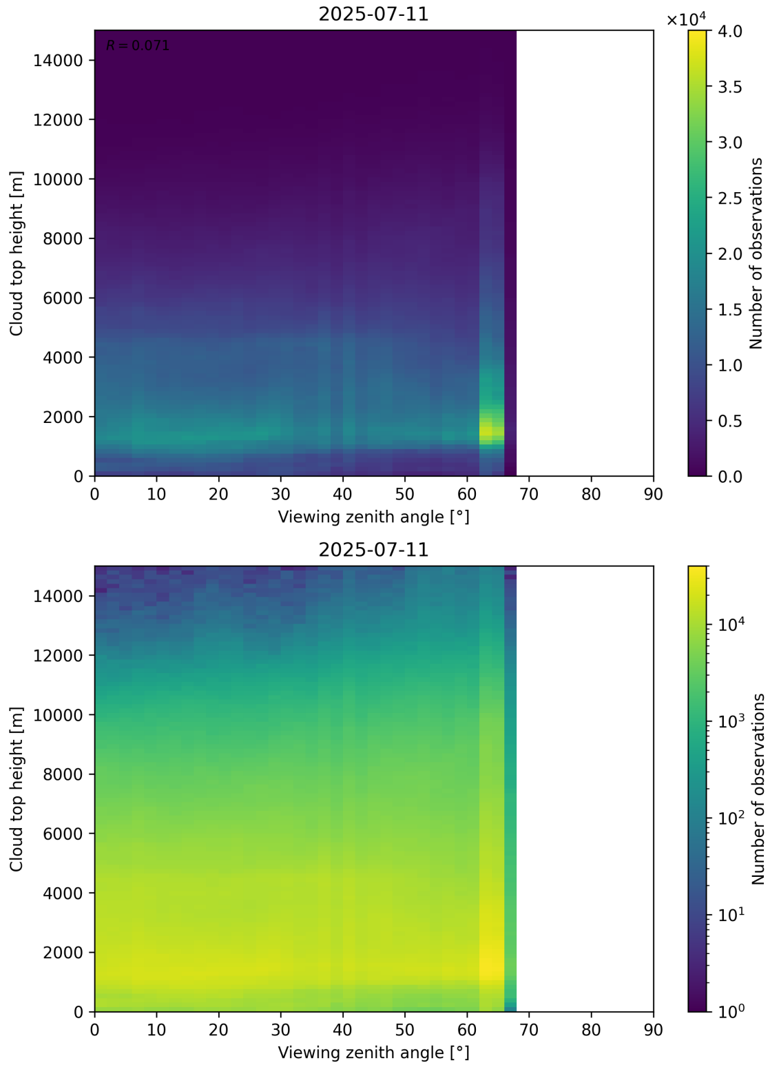
Figure 112: Scatter density plot of “Viewing zenith angle” against “Cloud top height” for 2025-07-10 to 2025-07-12.
