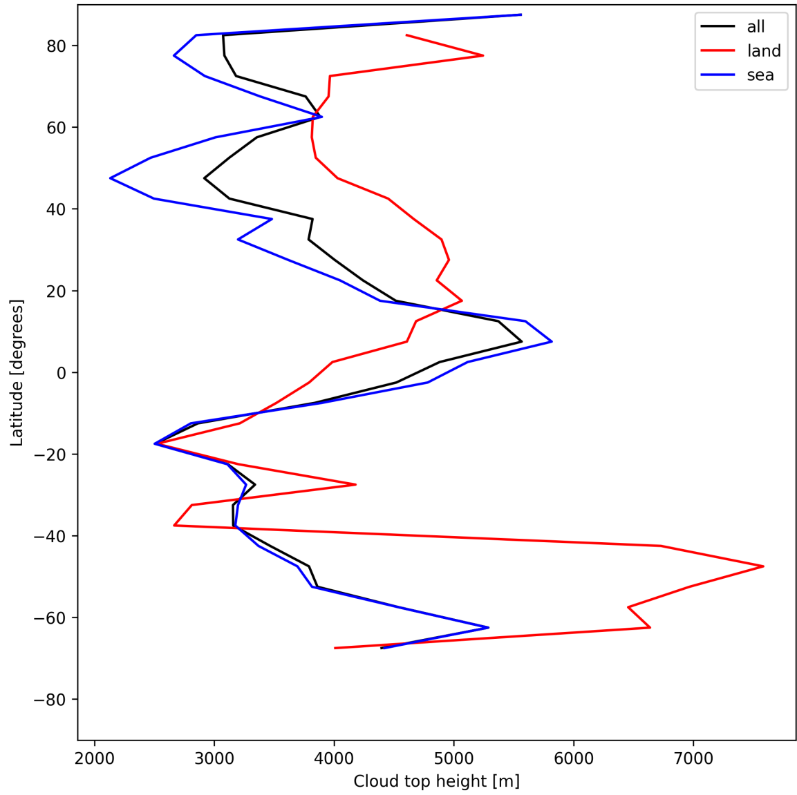
Figure 24: Zonal average of “Cloud top height” for 2025-07-10 to 2025-07-12.
