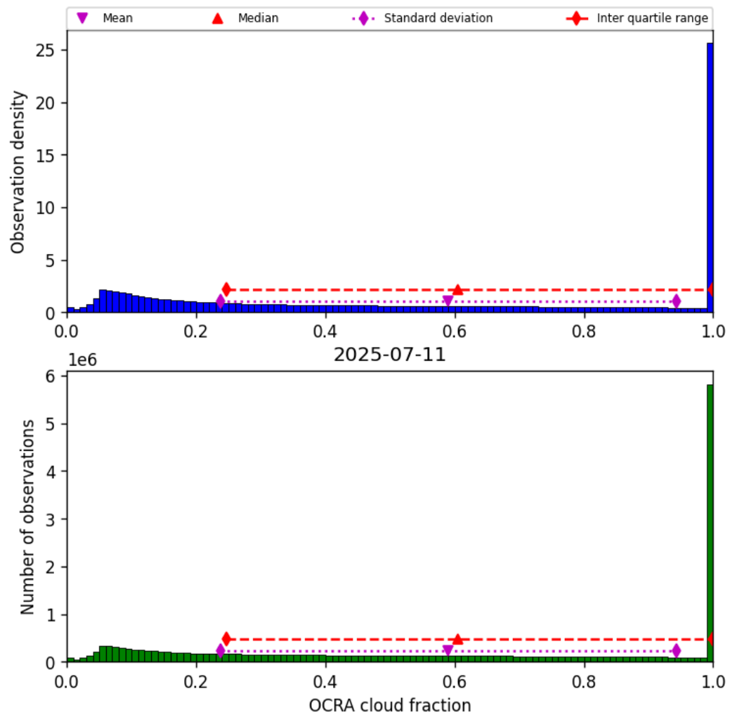
Figure 50: Histogram of “OCRA cloud fraction” for 2025-07-10 to 2025-07-12
