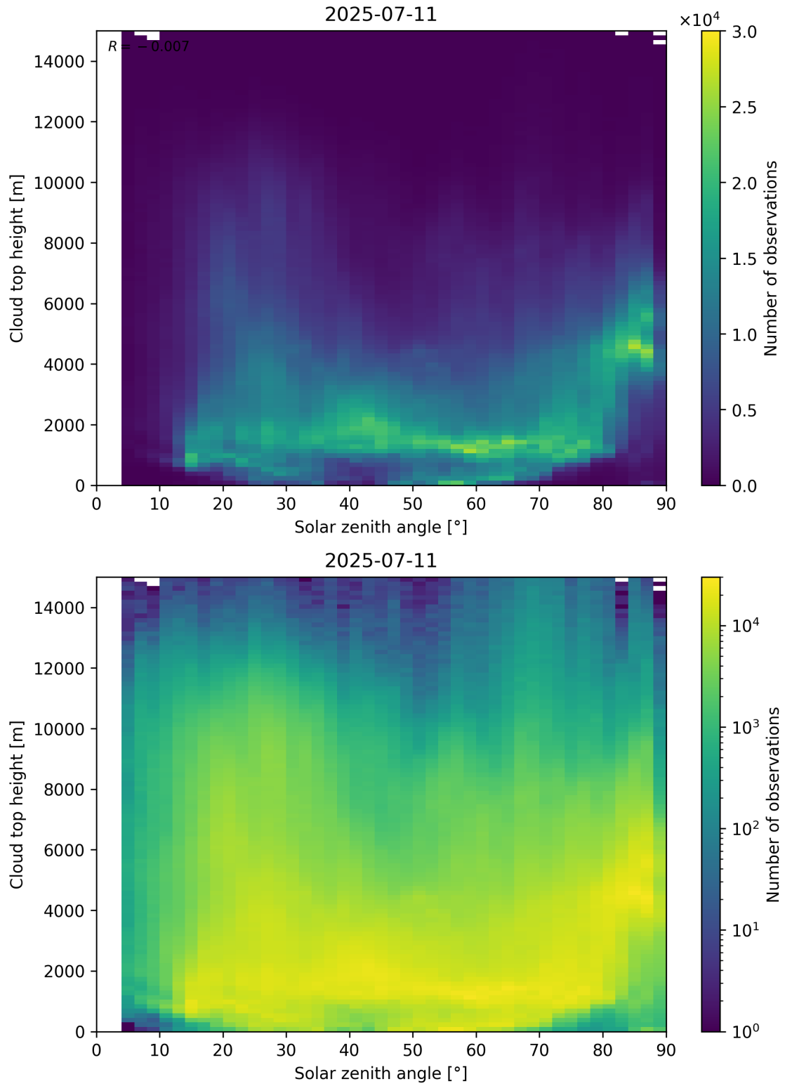
Figure 104: Scatter density plot of “Solar zenith angle” against “Cloud top height” for 2025-07-10 to 2025-07-12.
