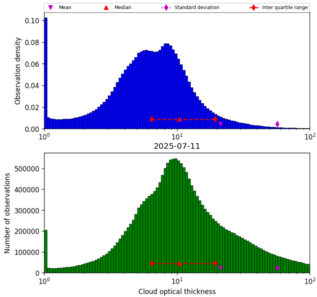
Figure 41: Histogram of “Cloud optical thickness” for 2025-07-10 to 2025-07-12
