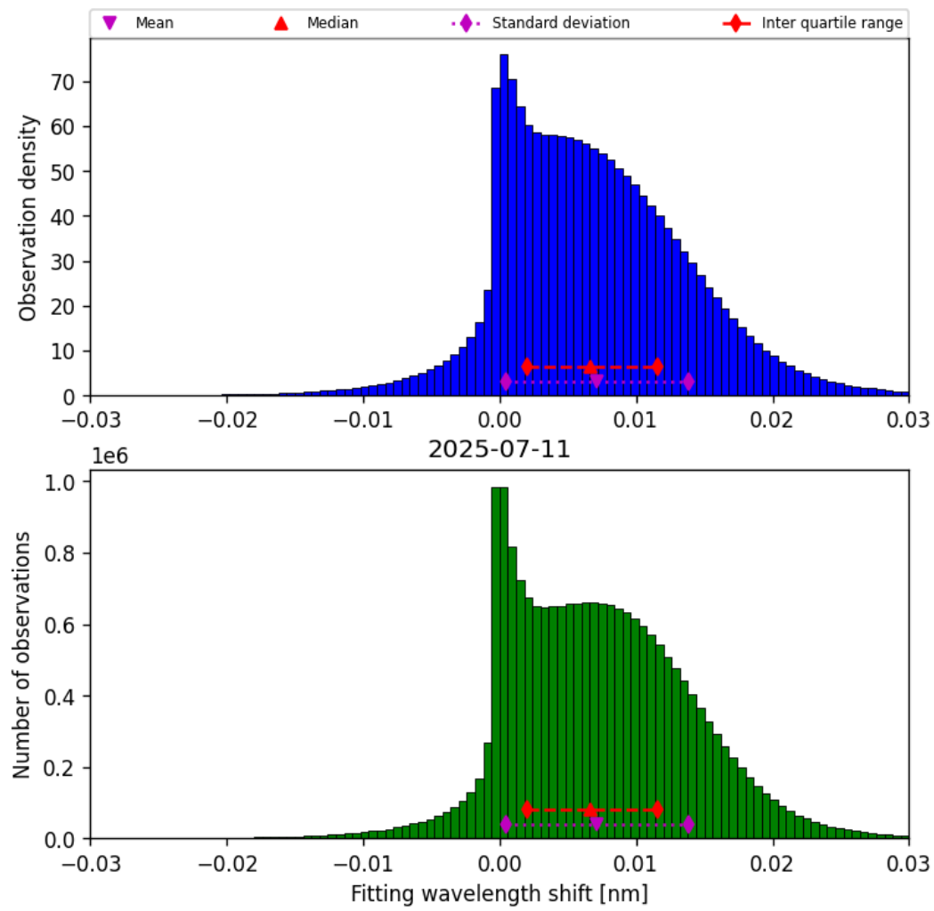
Figure 49: Histogram of “Fitting wavelength shift” for 2025-07-10 to 2025-07-12
