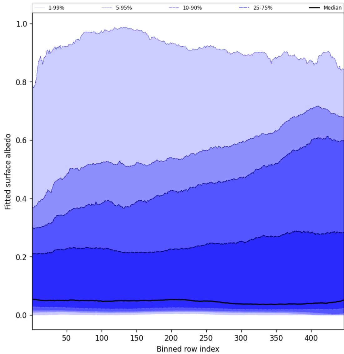
Figure 61: Along track statistics of “Fitted surface albedo” for 2025-07-10 to 2025-07-12
