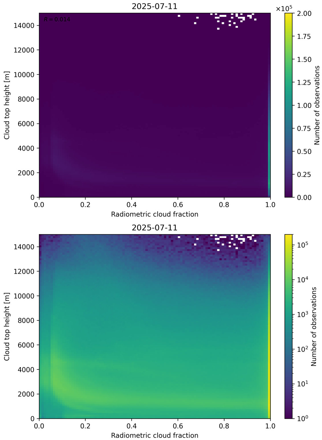
Figure 76: Scatter density plot of “Radiometric cloud fraction” against “Cloud top height” for 2025-07-10 to 2025-07-12.
