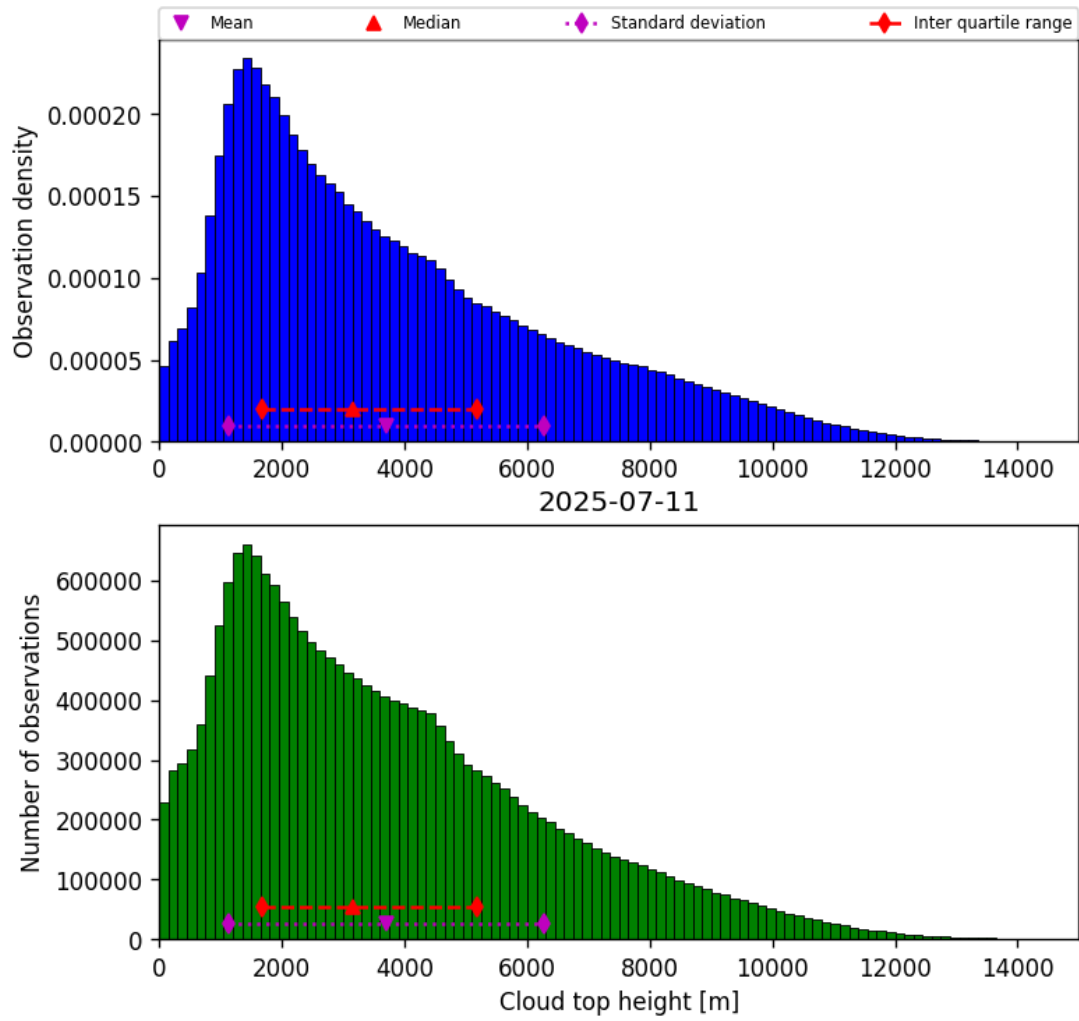
Figure 40: Histogram of “Cloud top height” for 2025-07-10 to 2025-07-12
