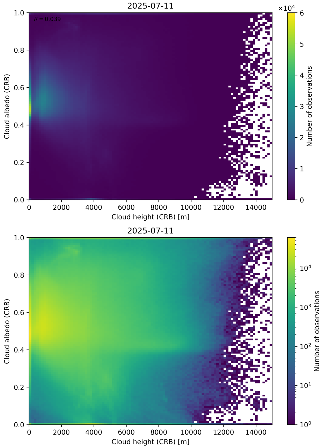
Figure 80: Scatter density plot of “Cloud height (CRB)” against “Cloud albedo (CRB)” for 2025-07-10 to 2025-07-12.
