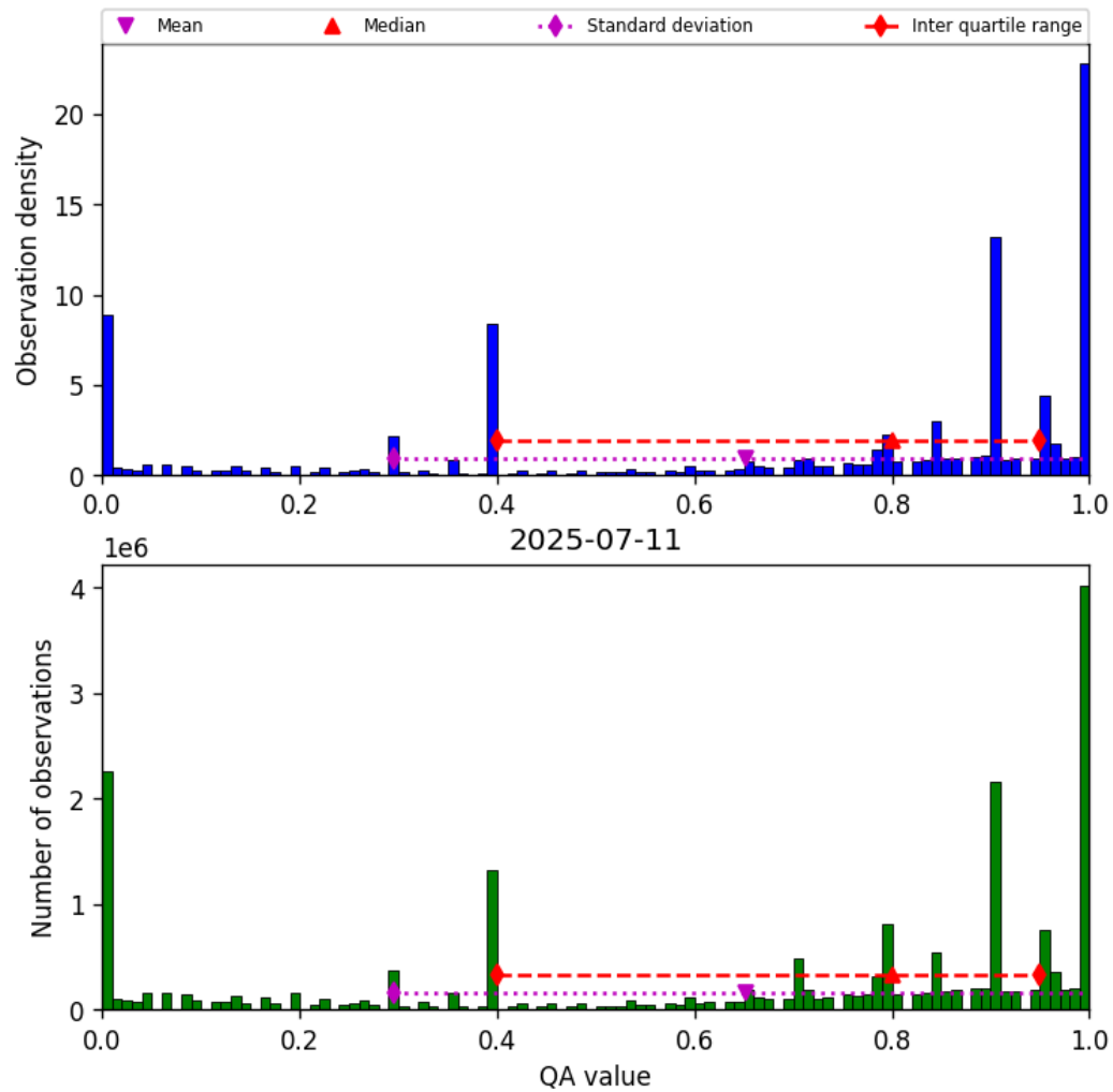
Figure 38: Histogram of “QA value” for 2025-07-10 to 2025-07-12
