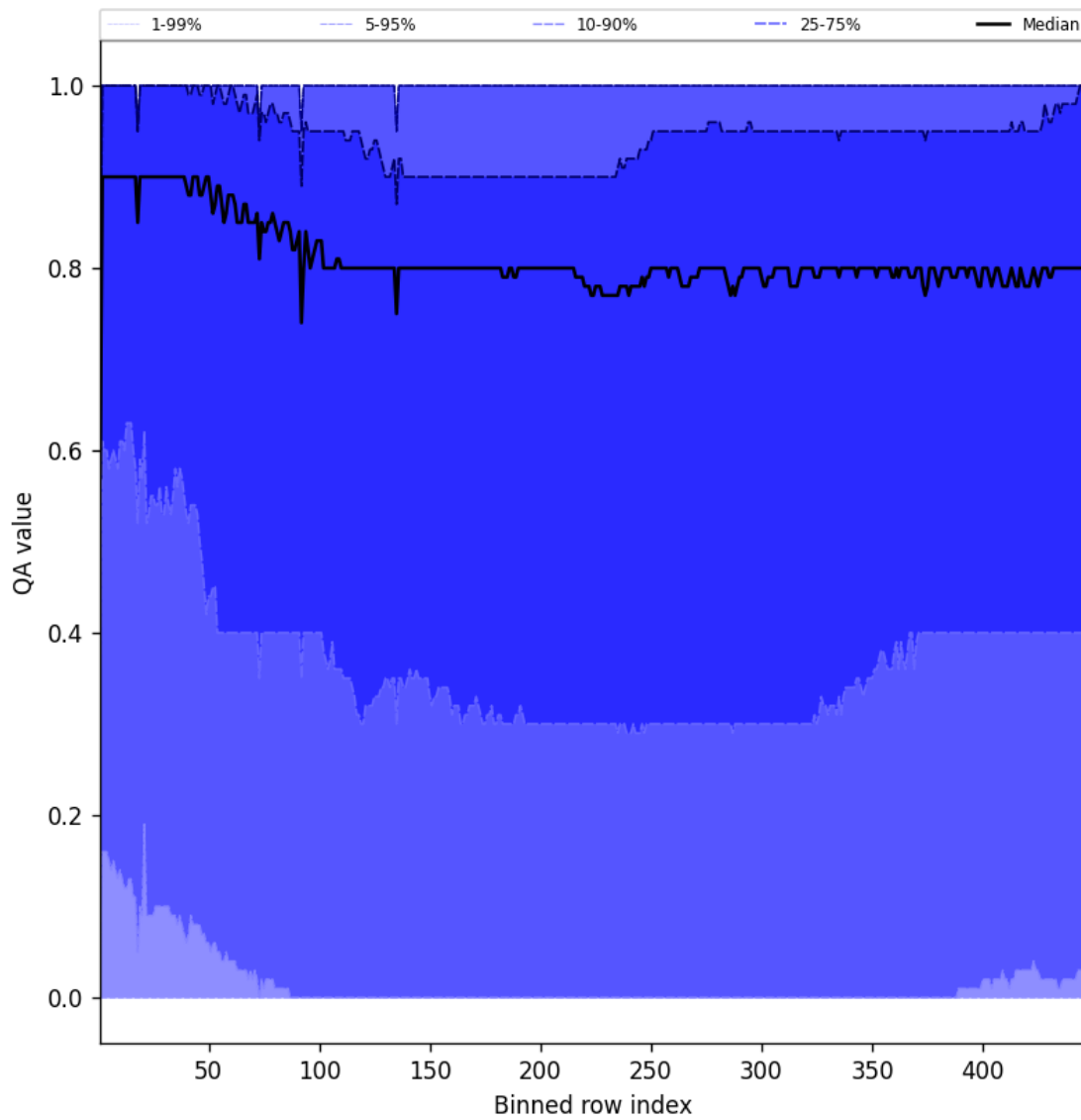
Figure 54: Along track statistics of “QA value” for 2025-07-10 to 2025-07-12
