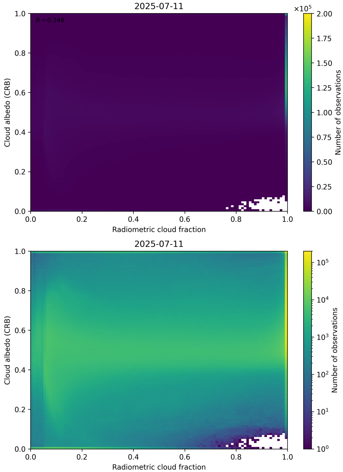
Figure 71: Scatter density plot of “Radiometric cloud fraction” against “Cloud albedo (CRB)” for 2025-07-10 to 2025-07-12.
