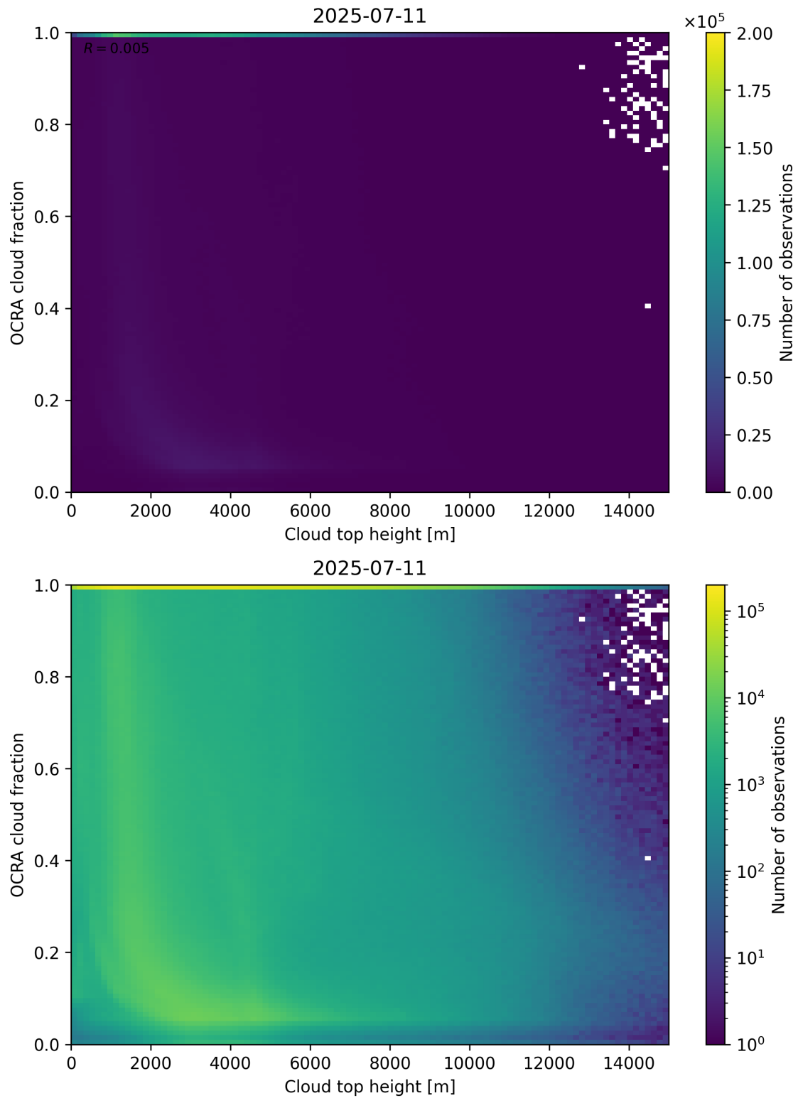
Figure 87: Scatter density plot of “Cloud top height” against “OCRA cloud fraction” for 2025-07-10 to 2025-07-12.
