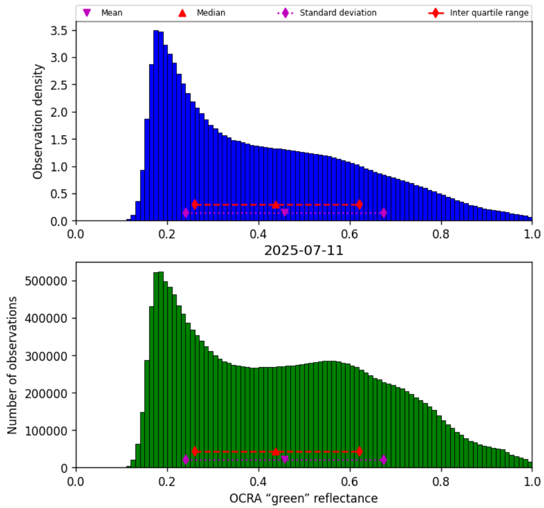
Figure 52: Histogram of “OCRA “green” reflectance” for 2025-07-10 to 2025-07-12
