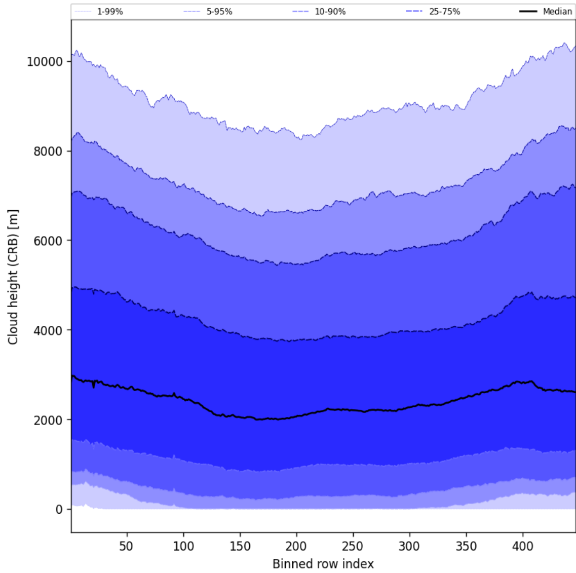
Figure 59: Along track statistics of “Cloud height (CRB)” for 2025-07-10 to 2025-07-12
