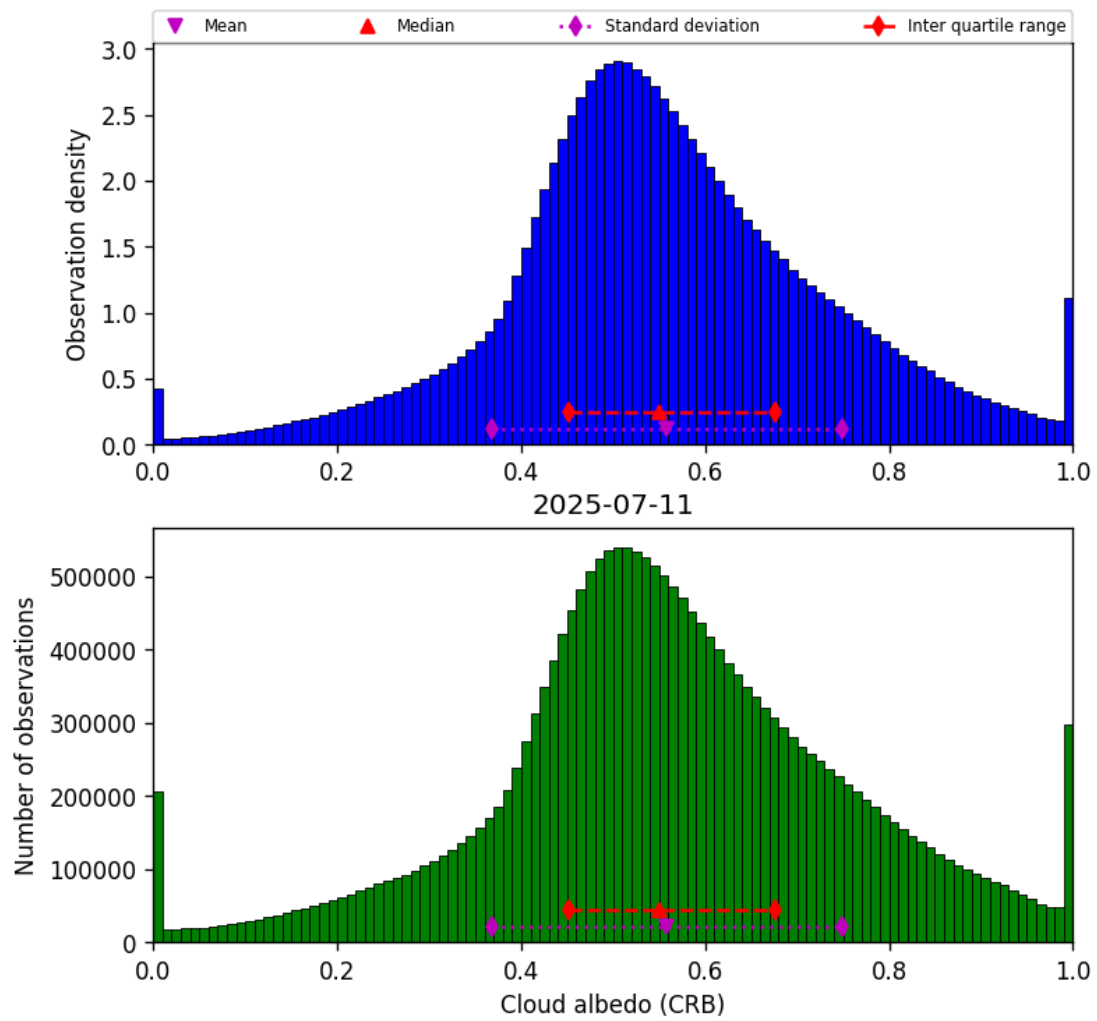
Figure 44: Histogram of “Cloud albedo (CRB)” for 2025-07-10 to 2025-07-12
