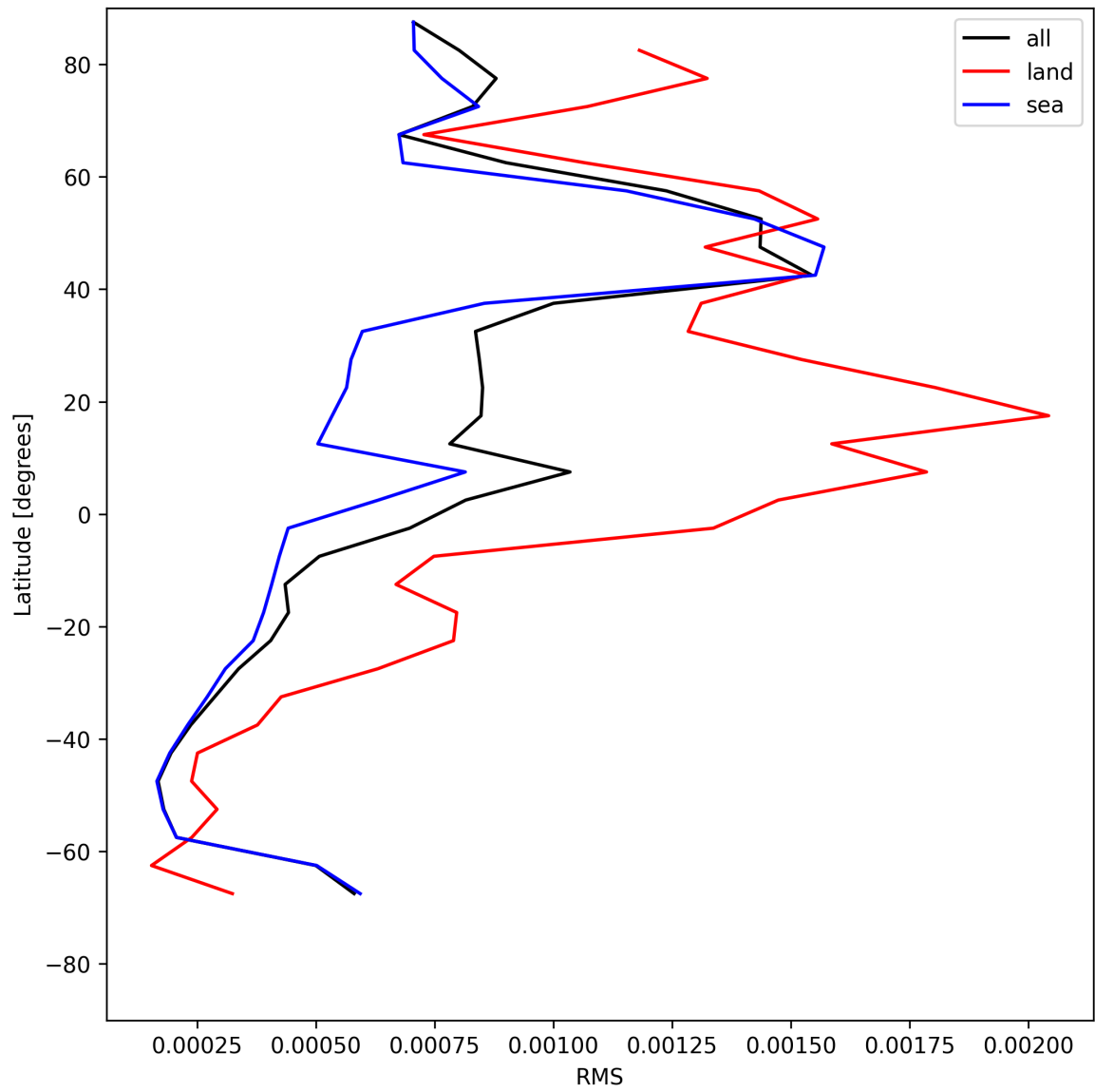
Figure 31: Zonal average of “RMS” for 2025-07-10 to 2025-07-12.
