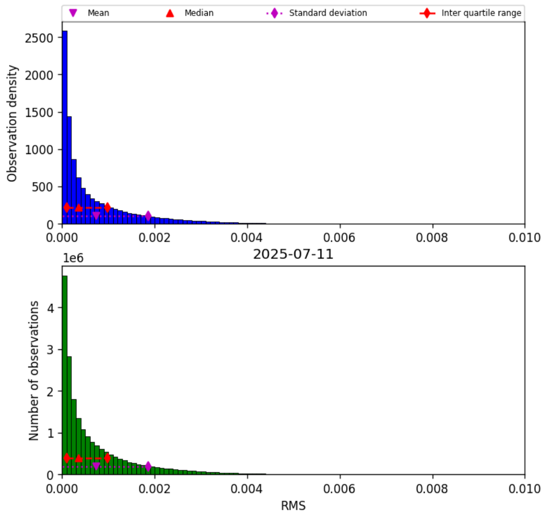
Figure 47: Histogram of “RMS” for 2025-07-10 to 2025-07-12
