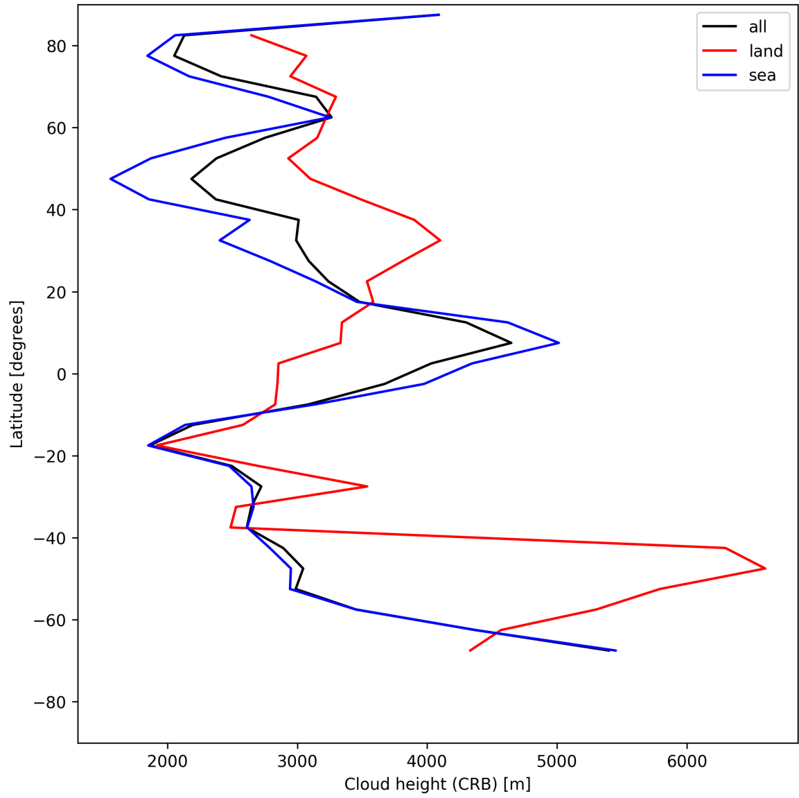
Figure 27: Zonal average of “Cloud height (CRB)” for 2025-07-10 to 2025-07-12.
