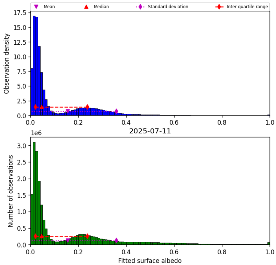
Figure 45: Histogram of “Fitted surface albedo” for 2025-07-10 to 2025-07-12
