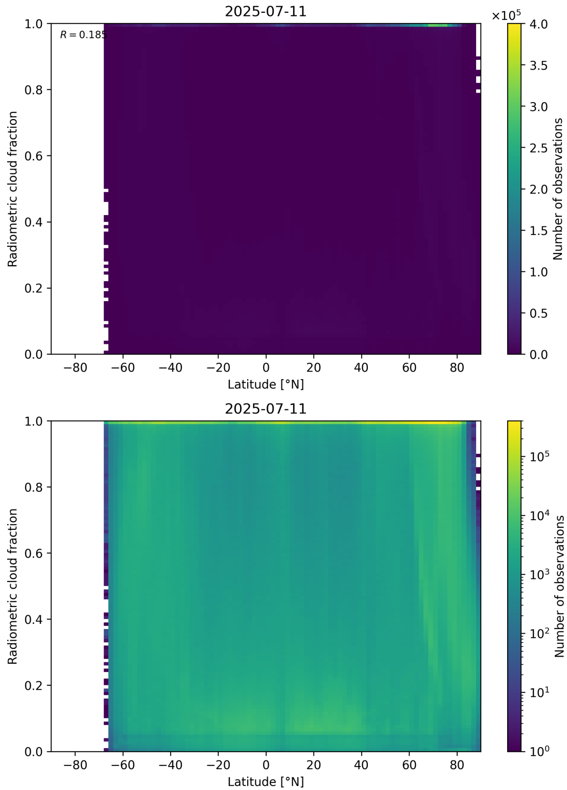
Figure 92: Scatter density plot of “Latitude” against “Radiometric cloud fraction” for 2025-07-10 to 2025-07-12.
