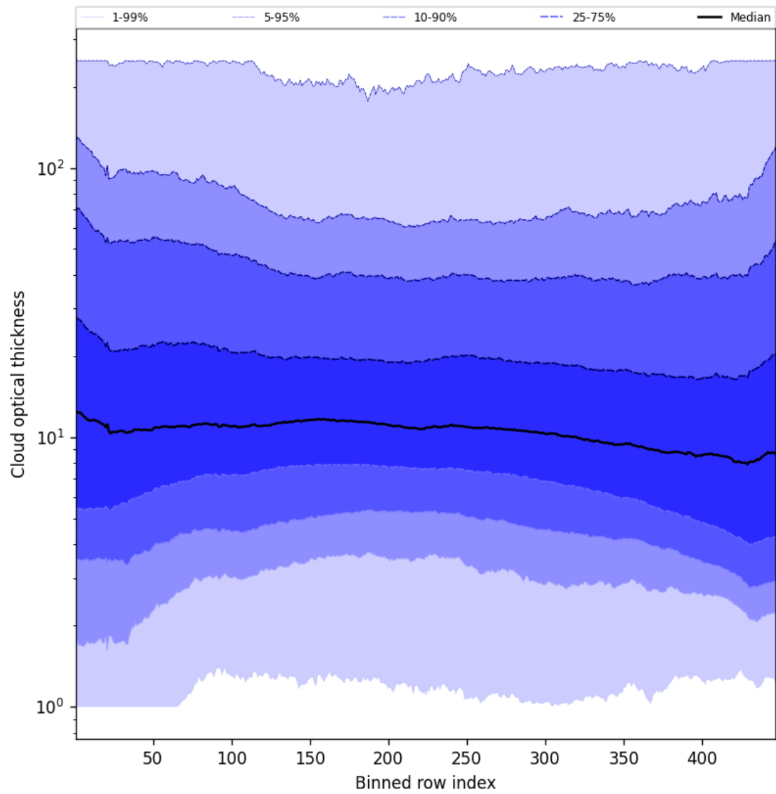
Figure 57: Along track statistics of “Cloud optical thickness” for 2025-07-10 to 2025-07-12
