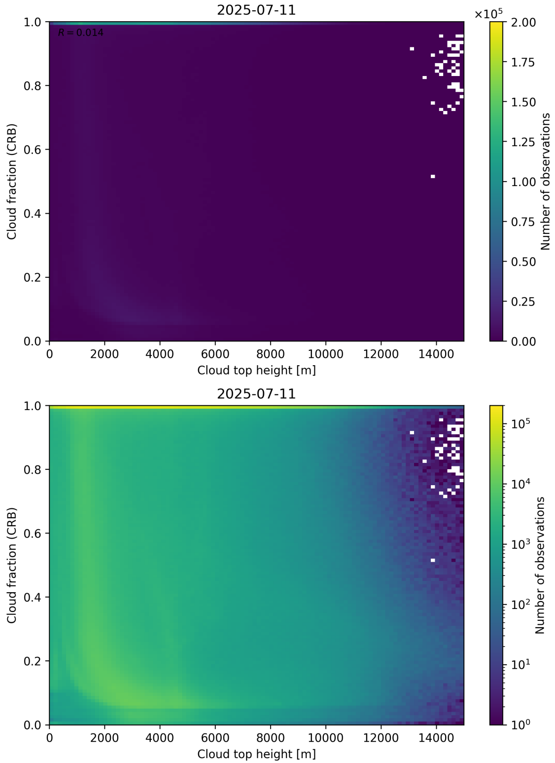
Figure 88: Scatter density plot of “Cloud top height” against “Cloud fraction (CRB)” for 2025-07-10 to 2025-07-12.
