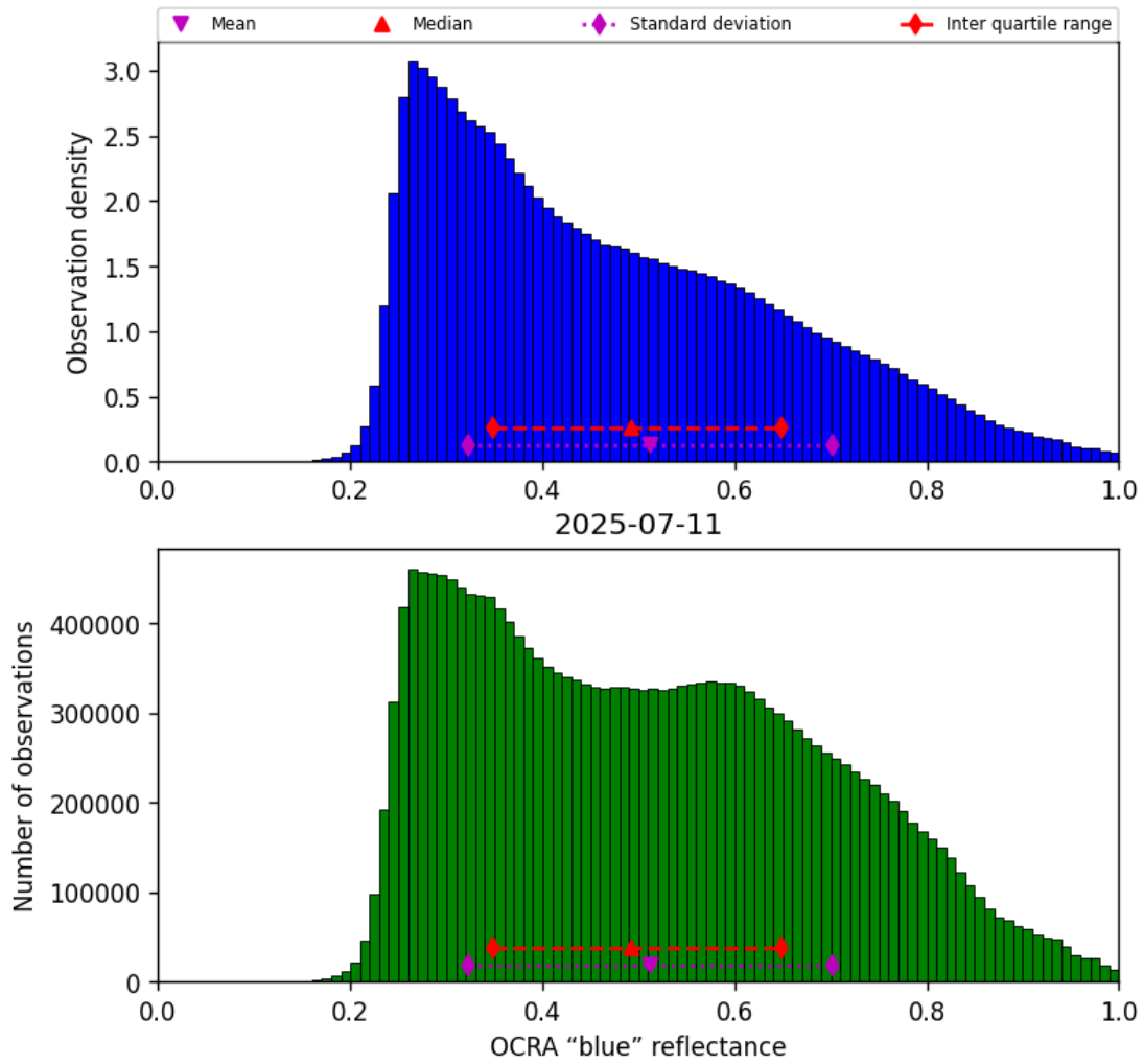
Figure 51: Histogram of “OCRA “blue” reflectance” for 2025-07-10 to 2025-07-12
