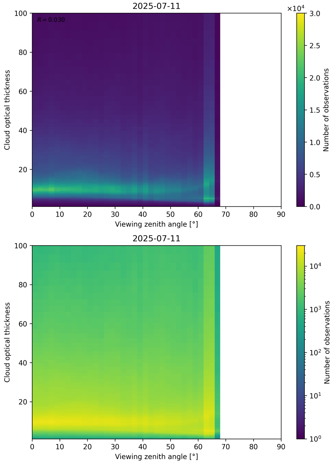
Figure 111: Scatter density plot of “Viewing zenith angle” against “Cloud optical thickness” for 2025-07-10 to 2025-07-12.
