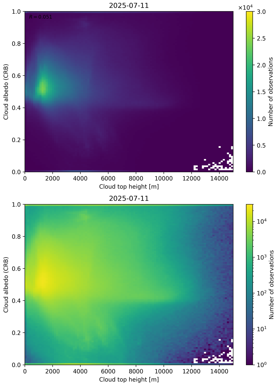
Figure 86: Scatter density plot of “Cloud top height” against “Cloud albedo (CRB)” for 2025-07-10 to 2025-07-12.
