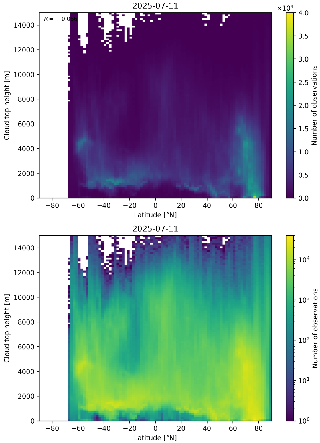
Figure 97: Scatter density plot of “Latitude” against “Cloud top height” for 2025-07-10 to 2025-07-12.
