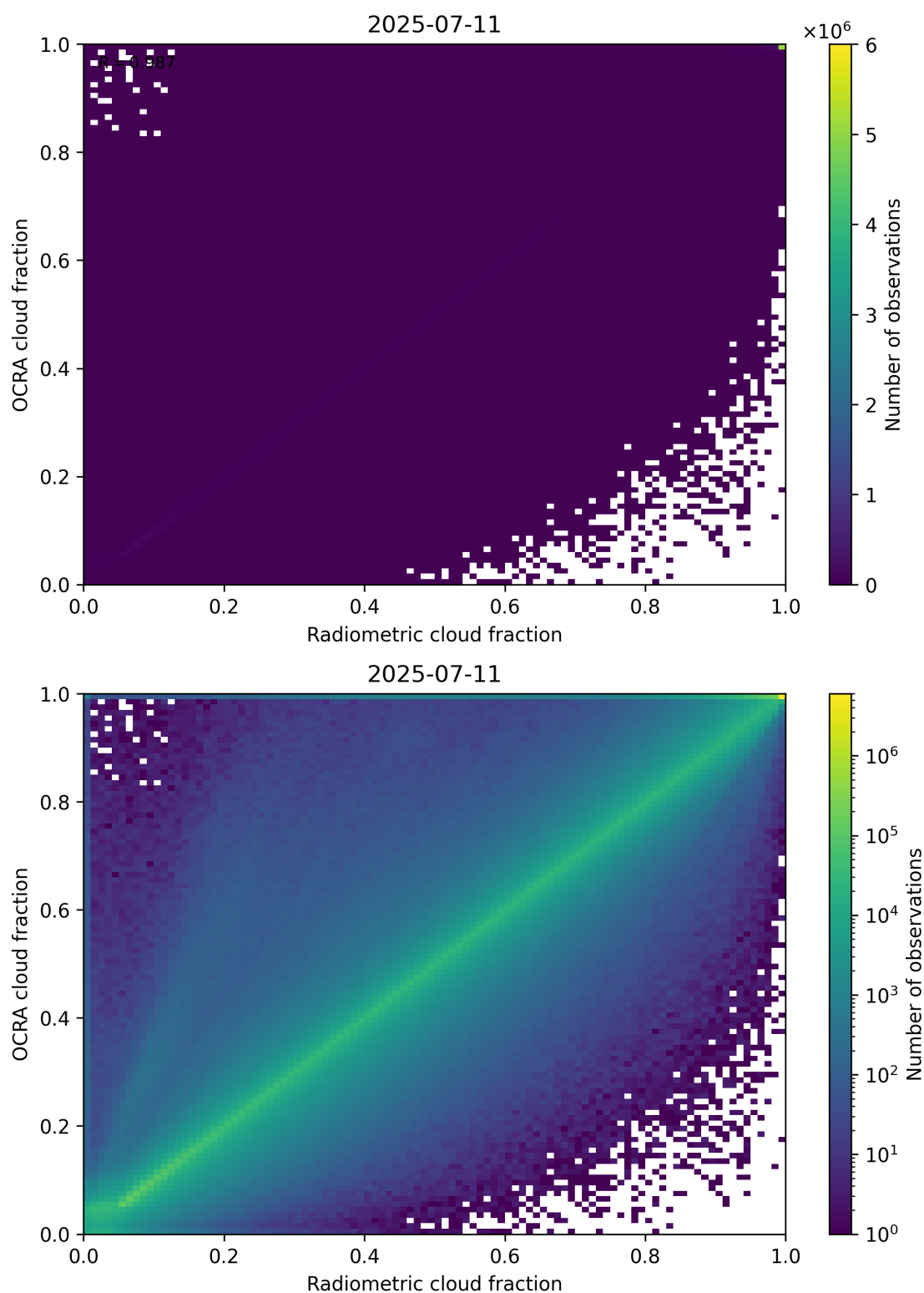
Figure 72: Scatter density plot of “Radiometric cloud fraction” against “OCRA cloud fraction” for 2025-07-10 to 2025-07-12.
