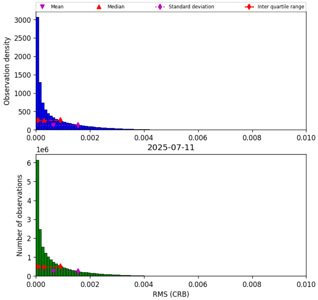
Figure 48: Histogram of “RMS (CRB)” for 2025-07-10 to 2025-07-12
