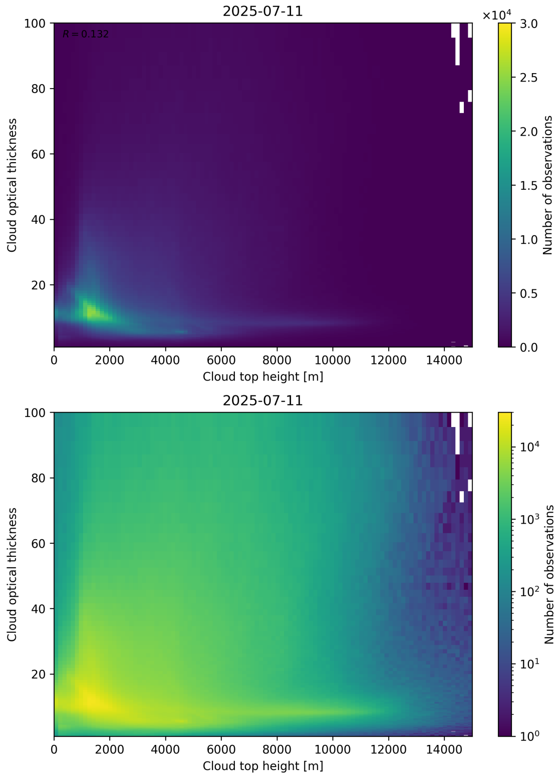
Figure 90: Scatter density plot of “Cloud top height” against “Cloud optical thickness” for 2025-07-10 to 2025-07-12.
