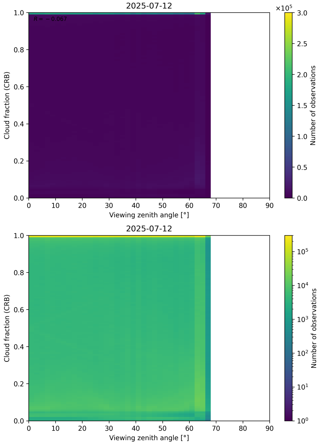
Figure 109: Scatter density plot of “Viewing zenith angle” against “Cloud fraction (CRB)” for 2025-07-11 to 2025-07-13.
