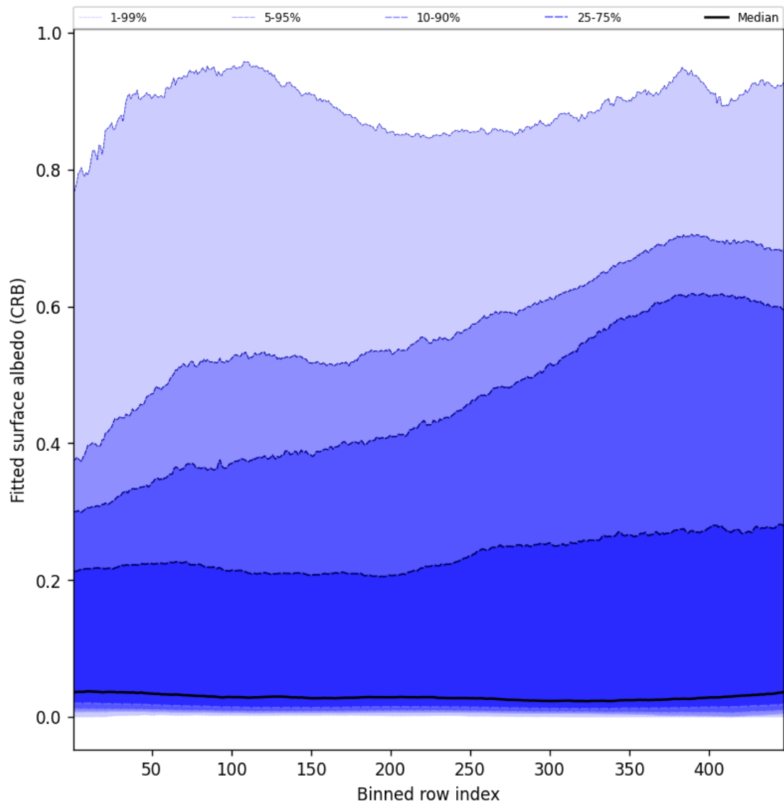
Figure 62: Along track statistics of “Fitted surface albedo (CRB)” for 2025-07-11 to 2025-07-13
