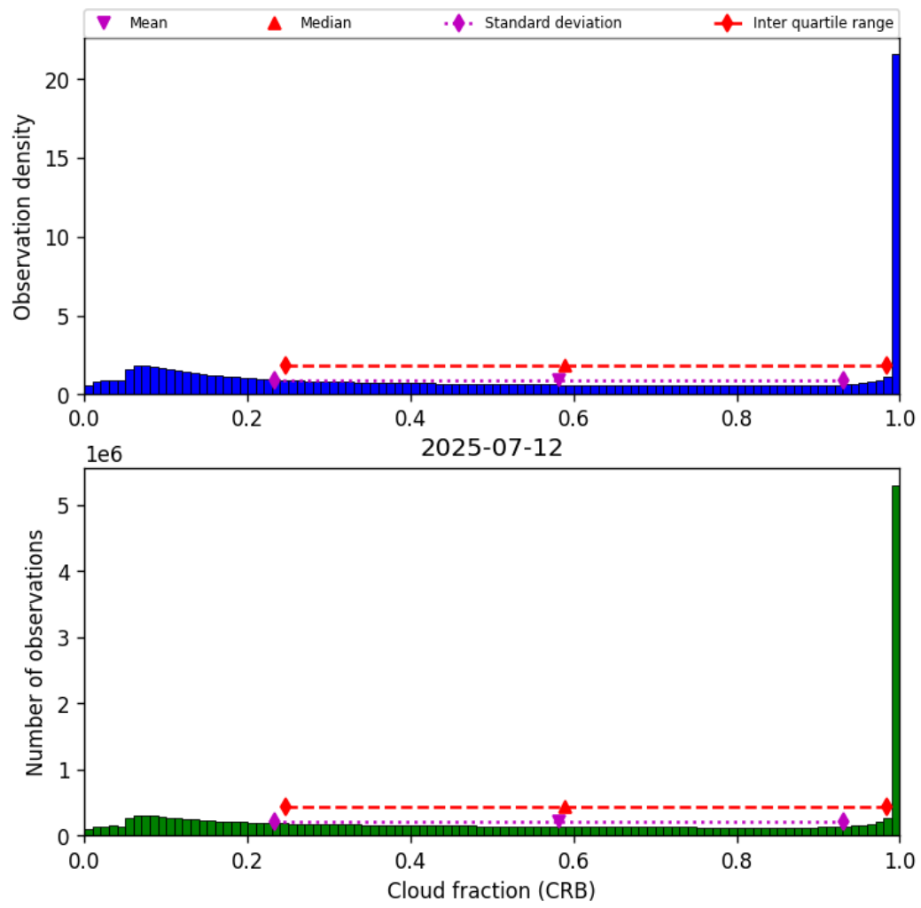
Figure 42: Histogram of “Cloud fraction (CRB)” for 2025-07-11 to 2025-07-13
