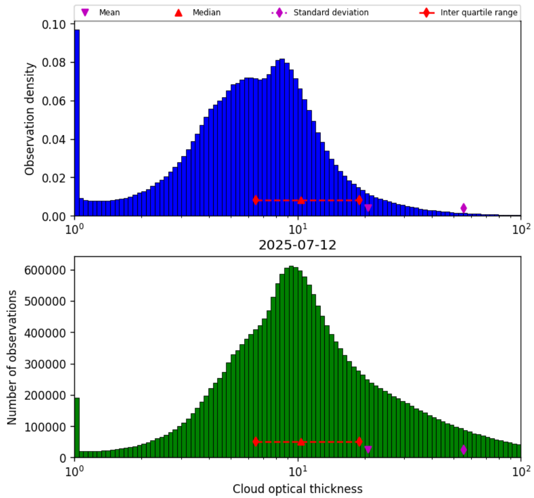
Figure 41: Histogram of “Cloud optical thickness” for 2025-07-11 to 2025-07-13
