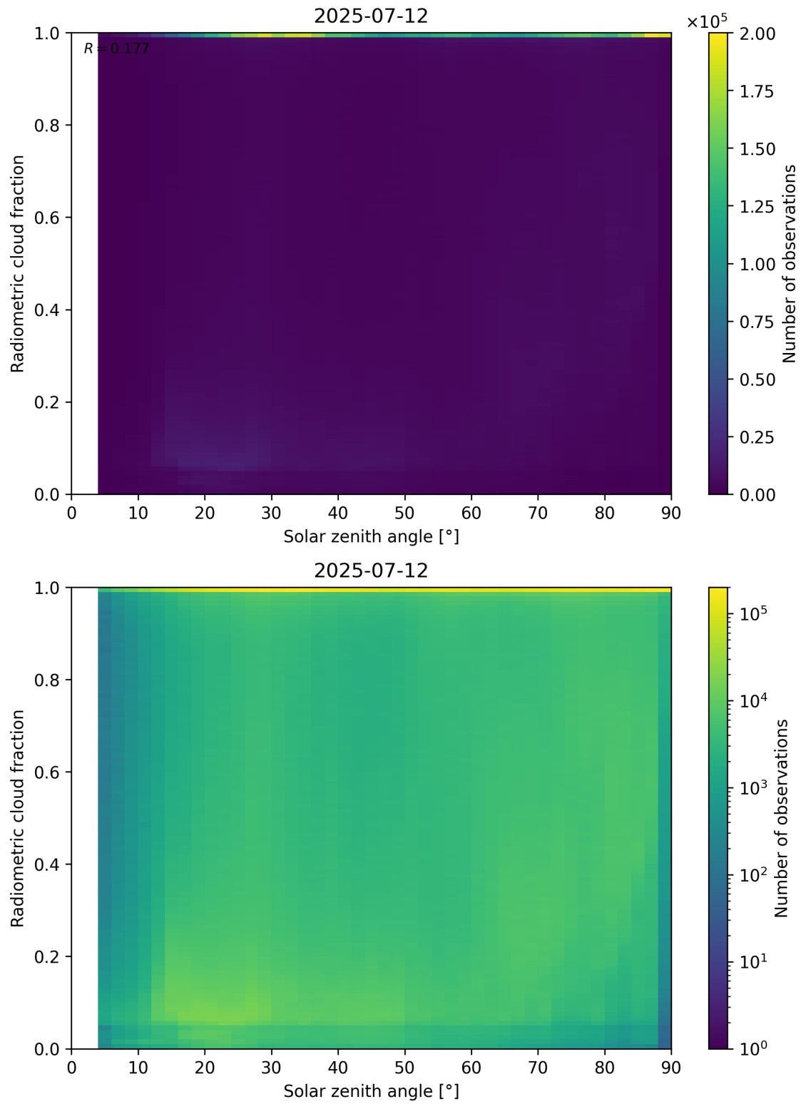
Figure 99: Scatter density plot of “Solar zenith angle” against “Radiometric cloud fraction” for 2025-07-11 to 2025-07-13.
