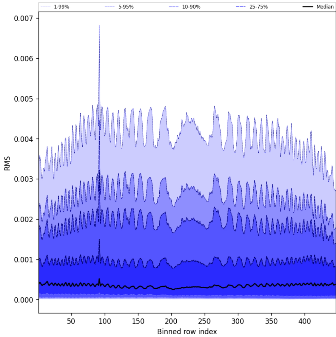
Figure 63: Along track statistics of “RMS” for 2025-07-11 to 2025-07-13
