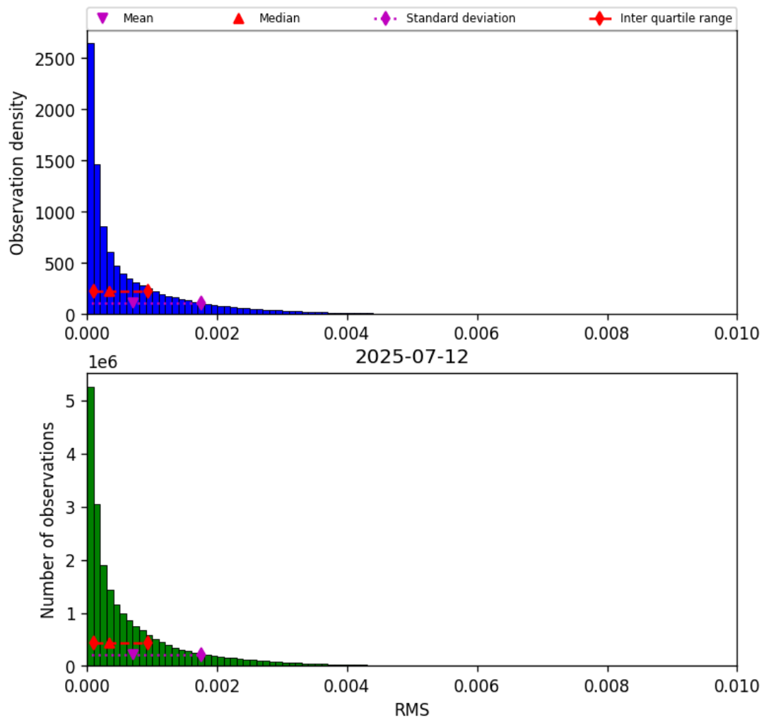
Figure 47: Histogram of “RMS” for 2025-07-11 to 2025-07-13
