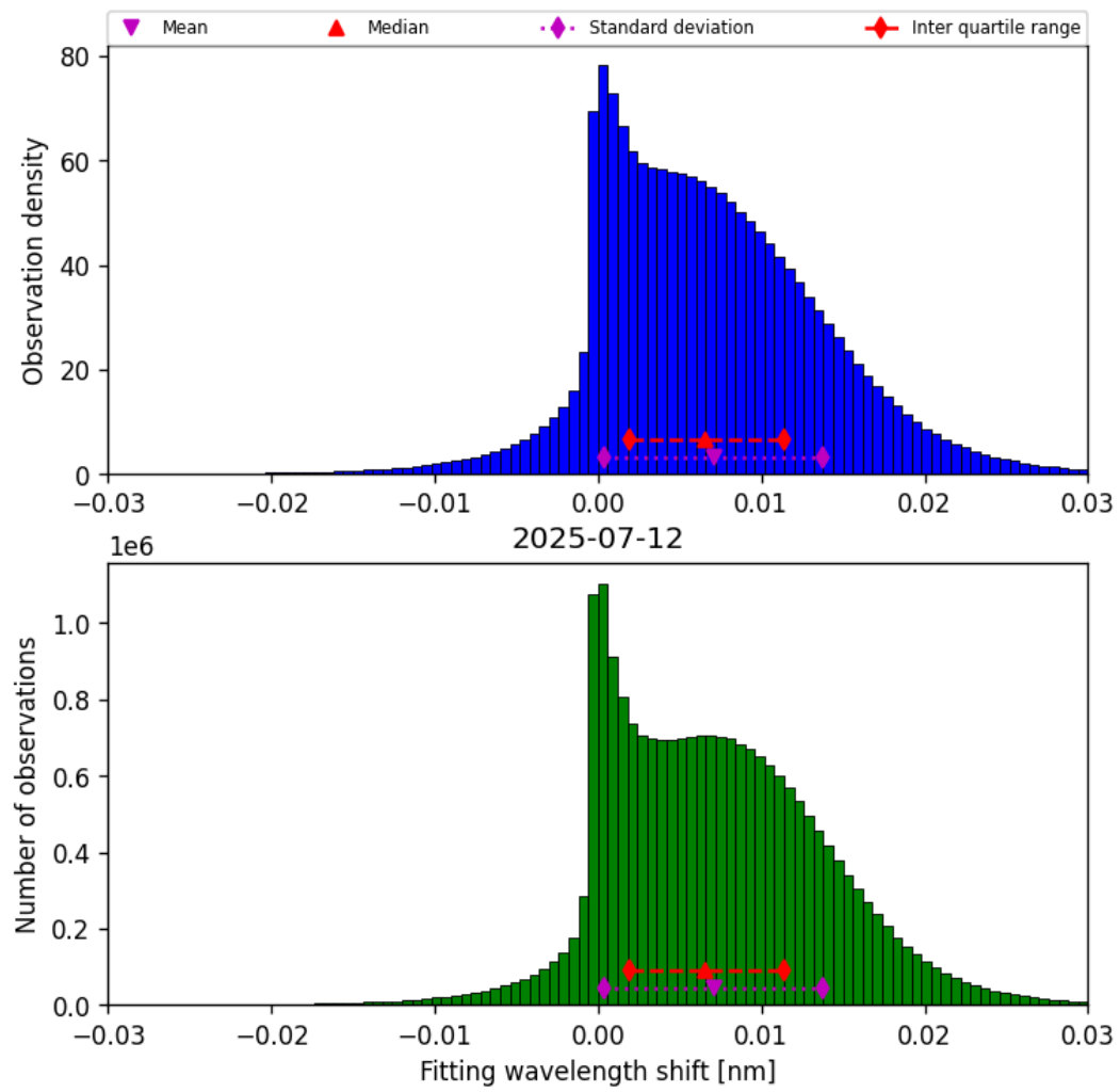
Figure 49: Histogram of “Fitting wavelength shift” for 2025-07-11 to 2025-07-13
