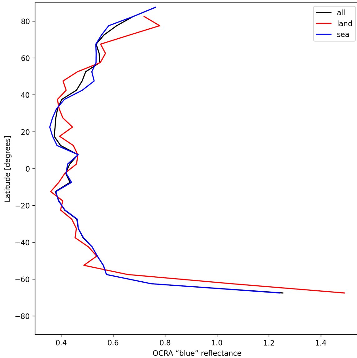
Figure 35: Zonal average of “OCRA “blue” reflectance” for 2025-07-11 to 2025-07-13.
