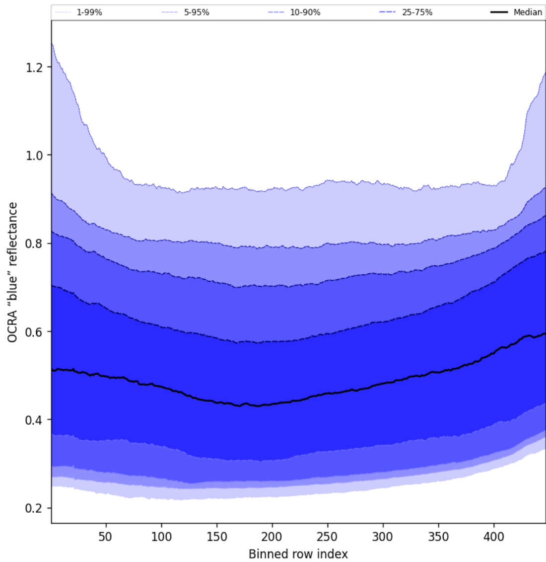
Figure 67: Along track statistics of “OCRA “blue” reflectance” for 2025-07-11 to 2025-07-13
