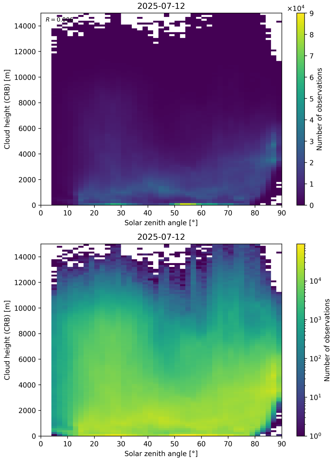
Figure 102: Scatter density plot of “Solar zenith angle” against “Cloud height (CRB)” for 2025-07-11 to 2025-07-13.
