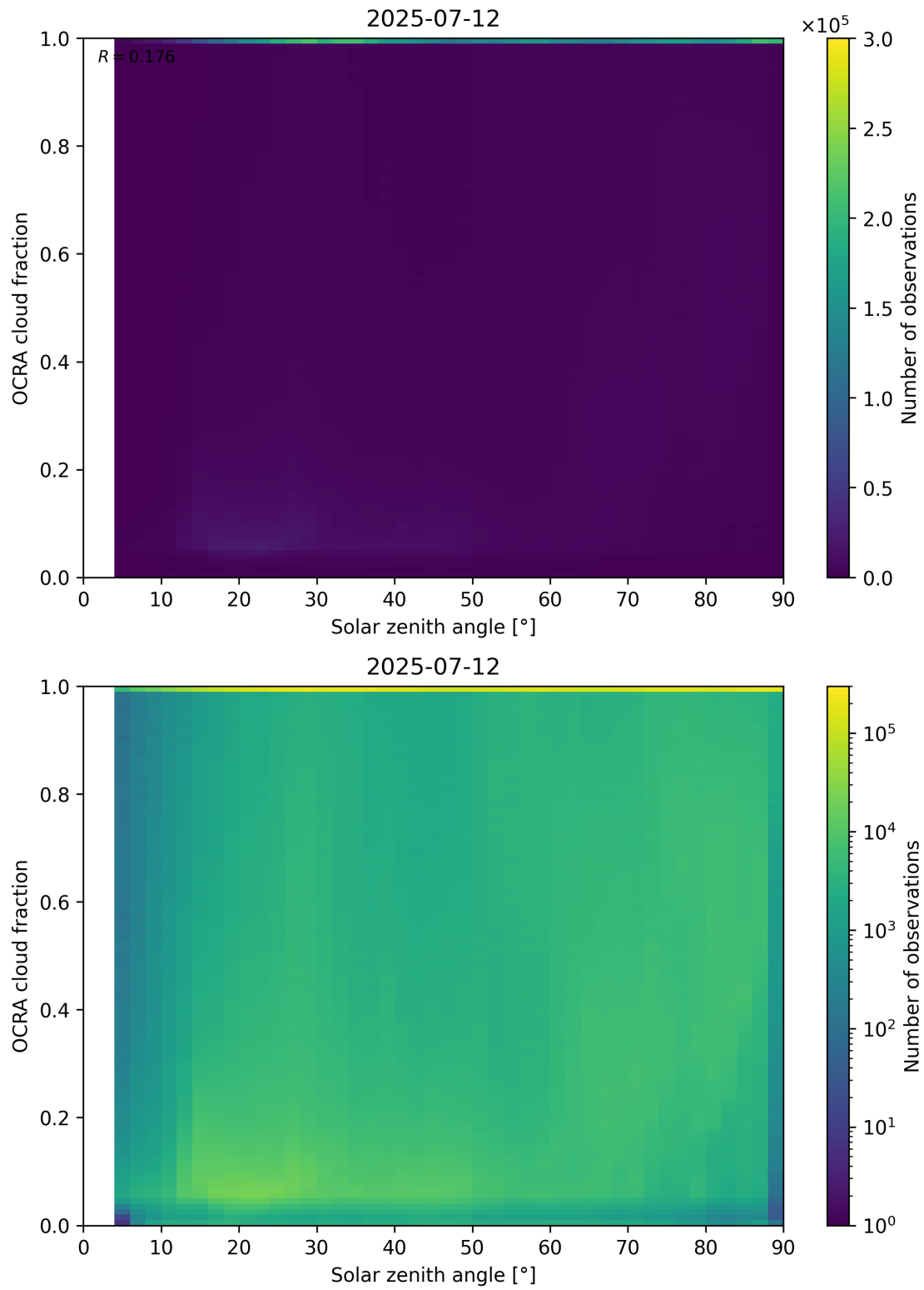
Figure 100: Scatter density plot of “Solar zenith angle” against “OCRA cloud fraction” for 2025-07-11 to 2025-07-13.
