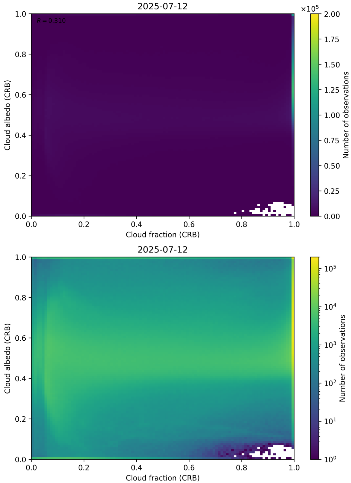
Figure 77: Scatter density plot of “Cloud fraction (CRB)” against “Cloud albedo (CRB)” for 2025-07-11 to 2025-07-13.
