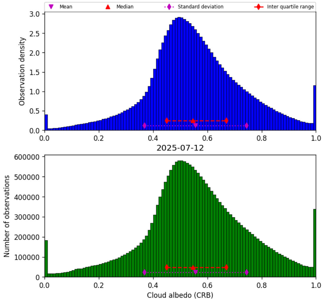
Figure 44: Histogram of “Cloud albedo (CRB)” for 2025-07-11 to 2025-07-13
