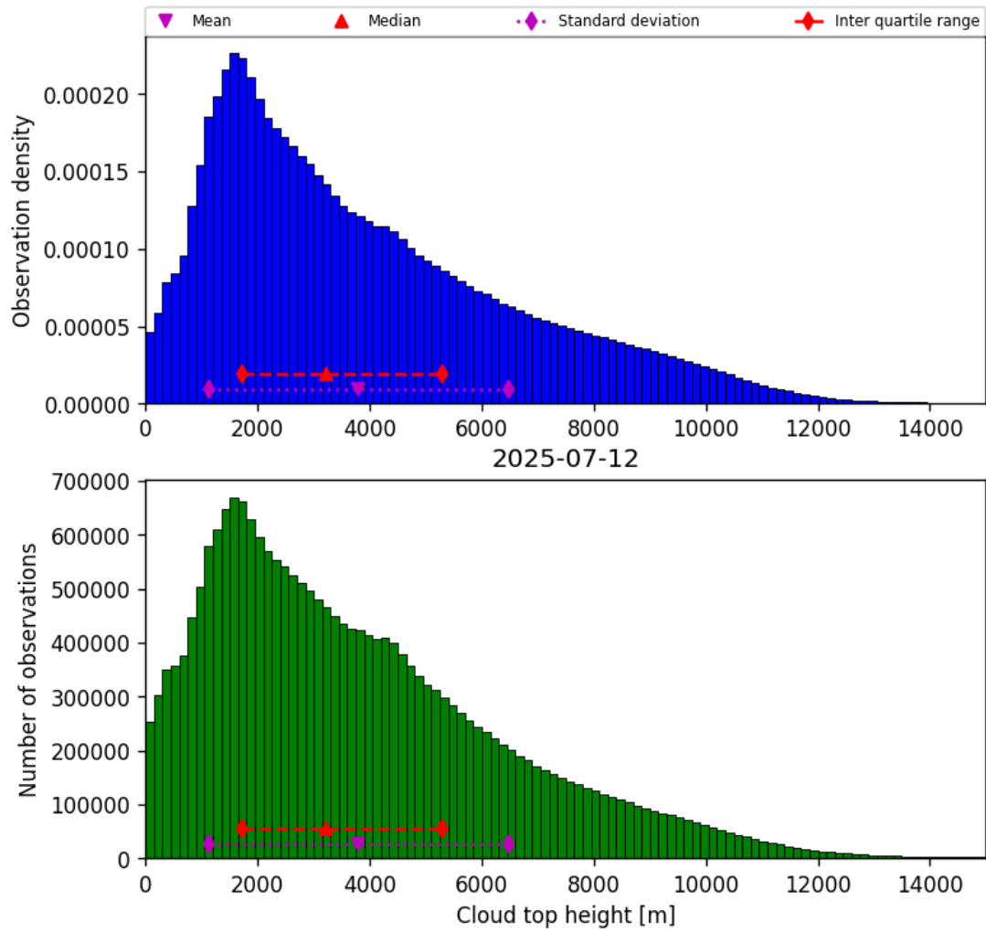
Figure 40: Histogram of “Cloud top height” for 2025-07-11 to 2025-07-13
