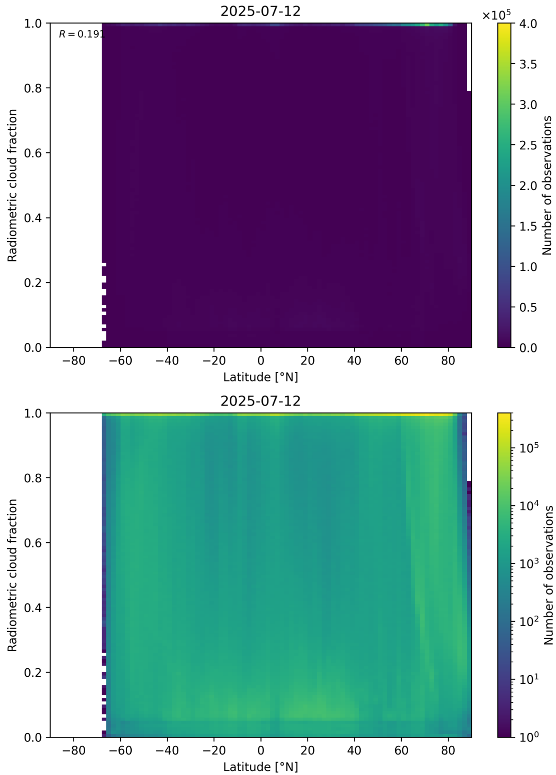
Figure 92: Scatter density plot of “Latitude” against “Radiometric cloud fraction” for 2025-07-11 to 2025-07-13.
