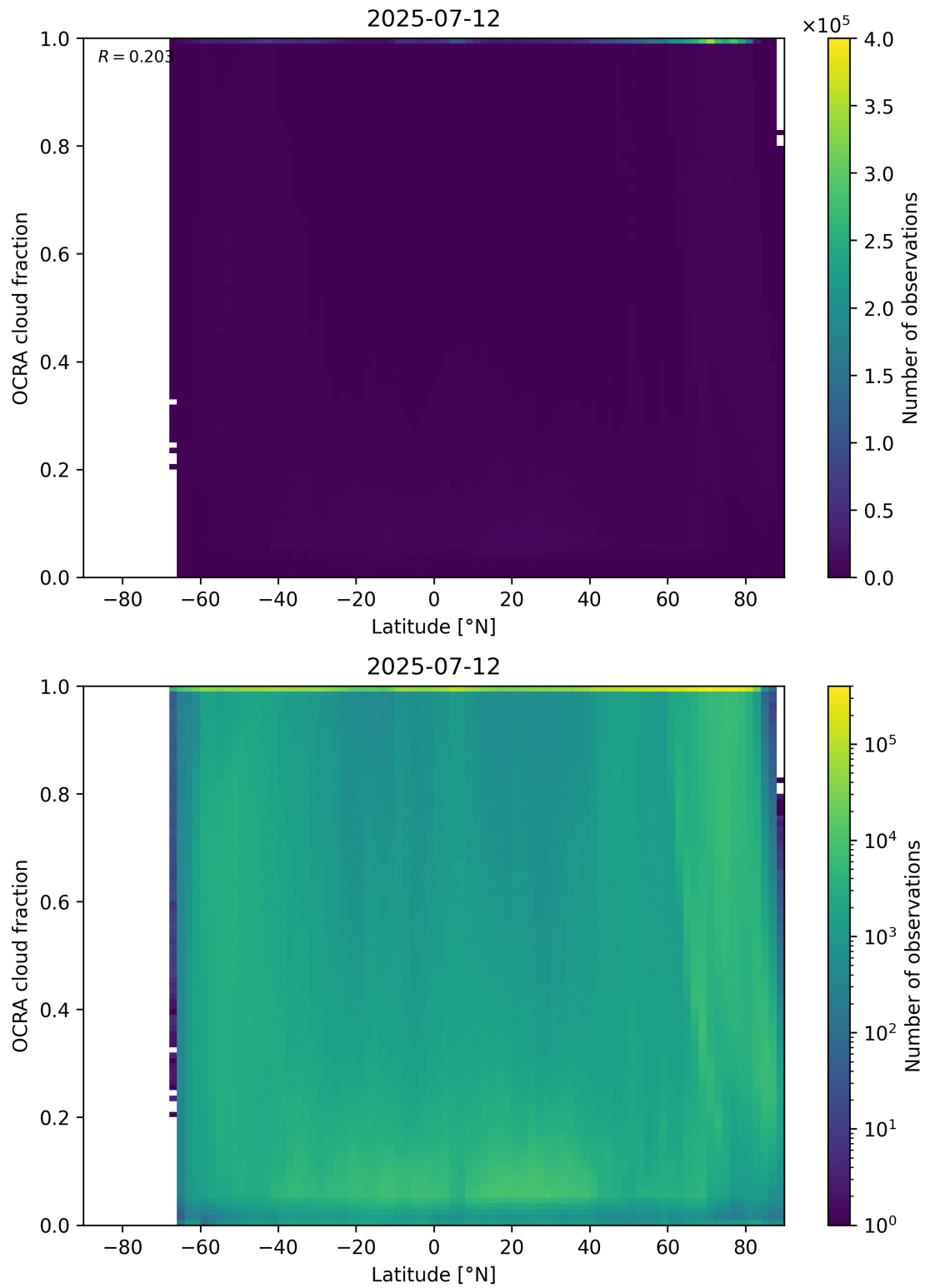
Figure 93: Scatter density plot of “Latitude” against “OCRA cloud fraction” for 2025-07-11 to 2025-07-13.
