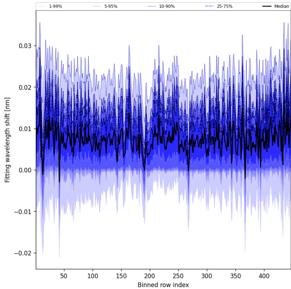
Figure 65: Along track statistics of “Fitting wavelength shift” for 2025-07-11 to 2025-07-13
