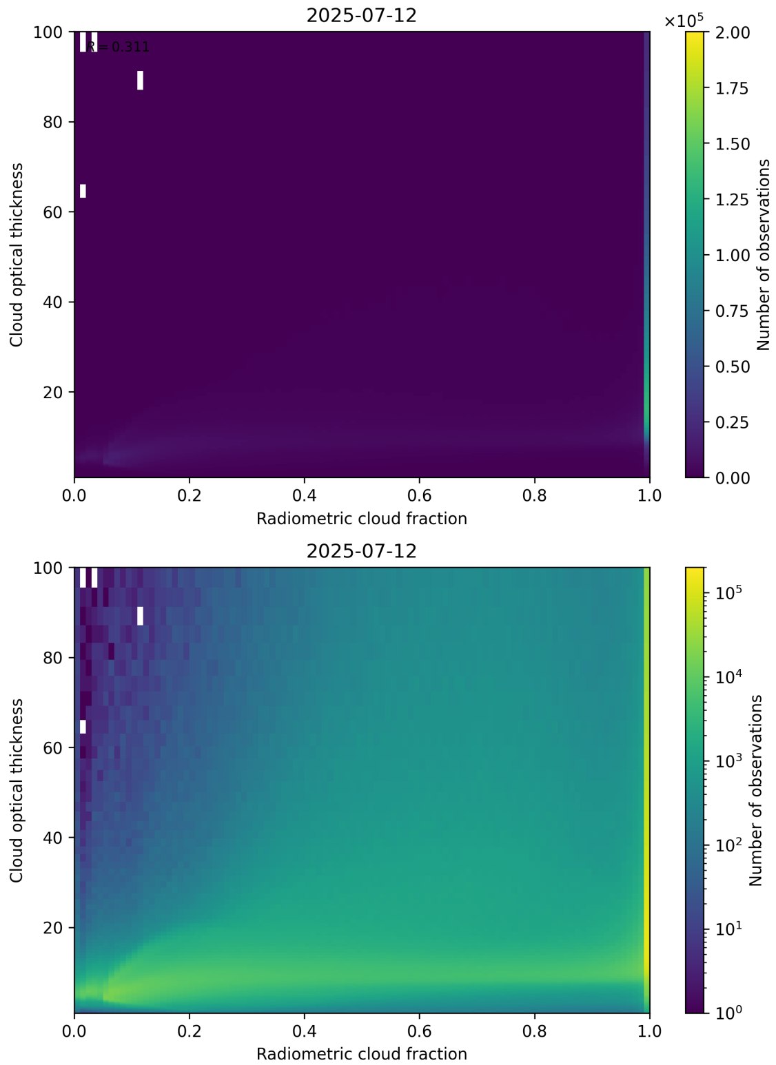
Figure 75: Scatter density plot of “Radiometric cloud fraction” against “Cloud optical thickness” for 2025-07-11 to 2025-07-13.
