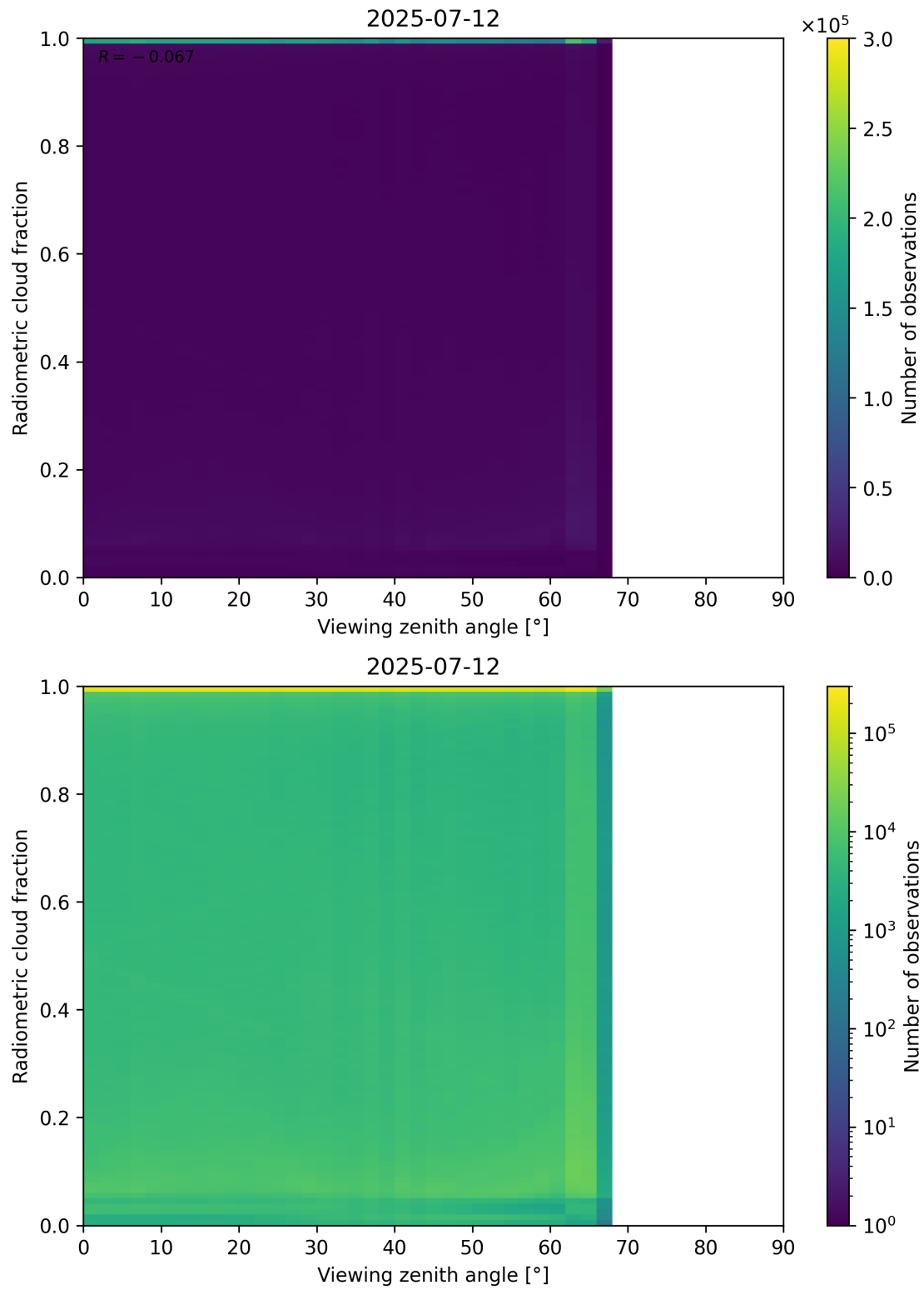
Figure 107: Scatter density plot of “Viewing zenith angle” against “Radiometric cloud fraction” for 2025-07-11 to 2025-07-13.
