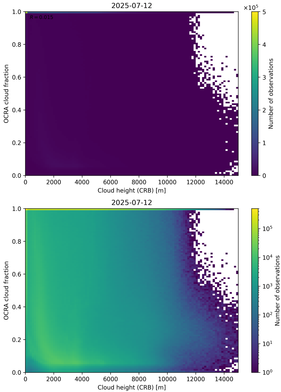
Figure 81: Scatter density plot of “Cloud height (CRB)” against “OCRA cloud fraction” for 2025-07-11 to 2025-07-13.
