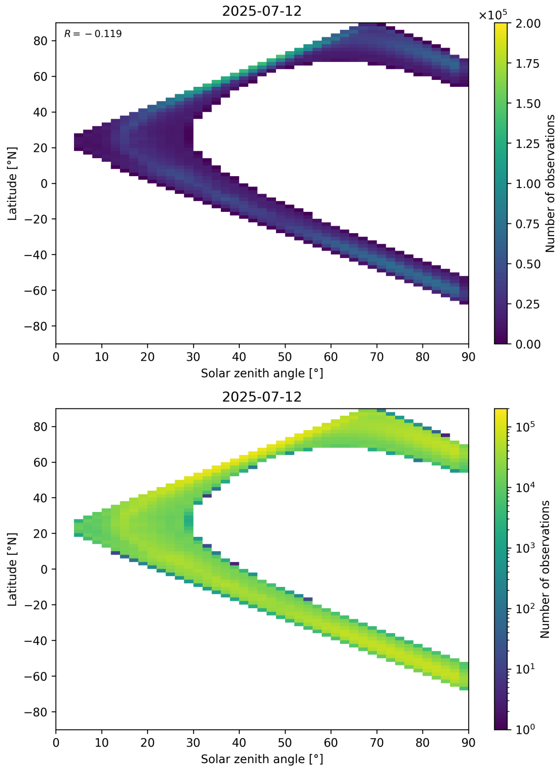
Figure 105: Scatter density plot of “Solar zenith angle” against “Latitude” for 2025-07-11 to 2025-07-13.
