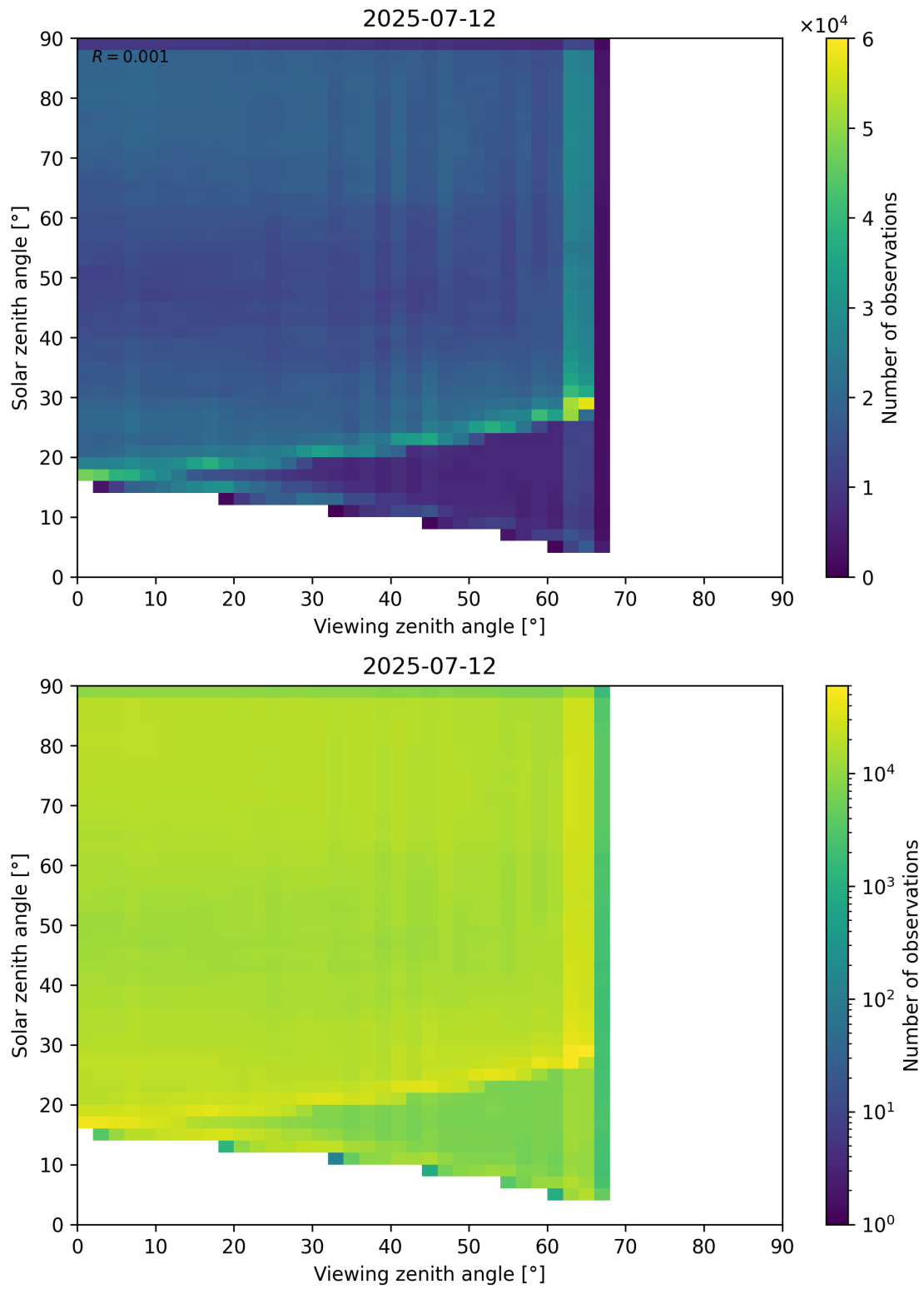
Figure 114: Scatter density plot of “Viewing zenith angle” against “Solar zenith angle” for 2025-07-11 to 2025-07-13.
