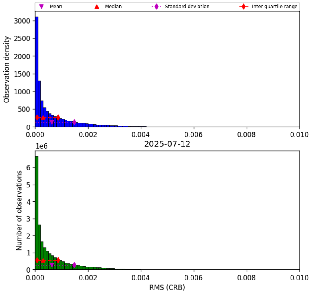
Figure 48: Histogram of “RMS (CRB)” for 2025-07-11 to 2025-07-13
