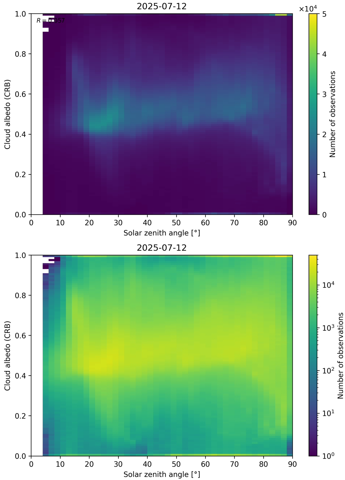
Figure 98: Scatter density plot of “Solar zenith angle” against “Cloud albedo (CRB)” for 2025-07-11 to 2025-07-13.
