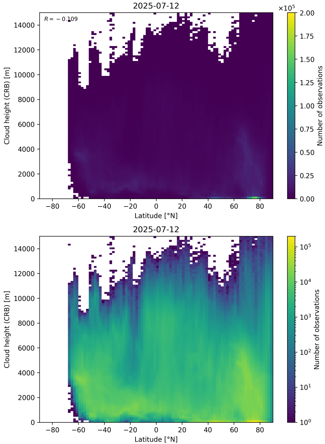
Figure 95: Scatter density plot of “Latitude” against “Cloud height (CRB)” for 2025-07-11 to 2025-07-13.
