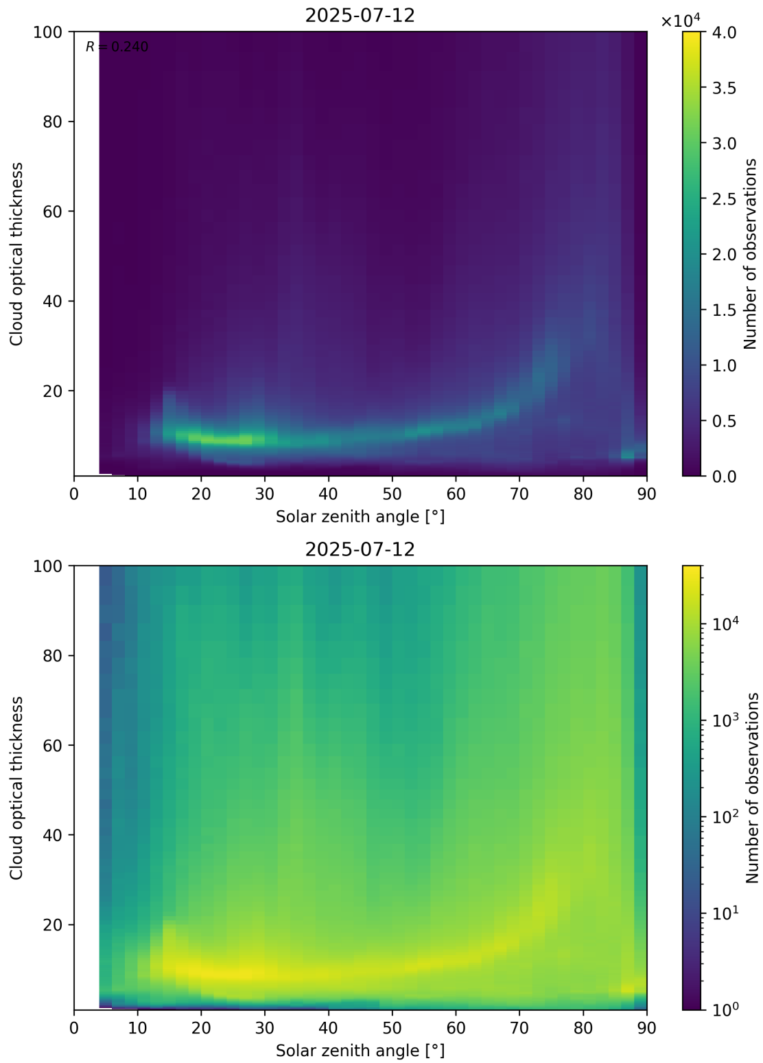
Figure 103: Scatter density plot of “Solar zenith angle” against “Cloud optical thickness” for 2025-07-11 to 2025-07-13.
