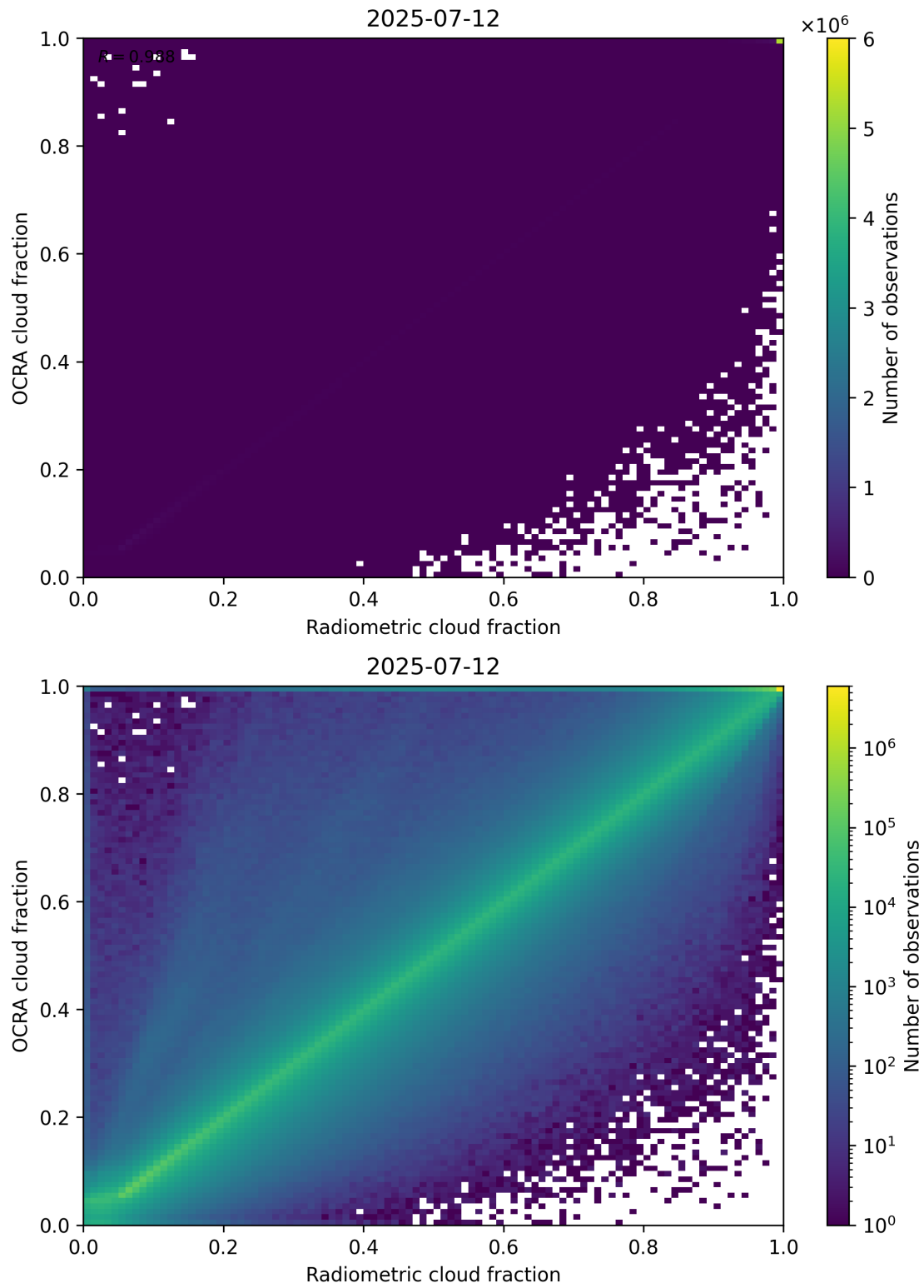
Figure 72: Scatter density plot of “Radiometric cloud fraction” against “OCRA cloud fraction” for 2025-07-11 to 2025-07-13.
