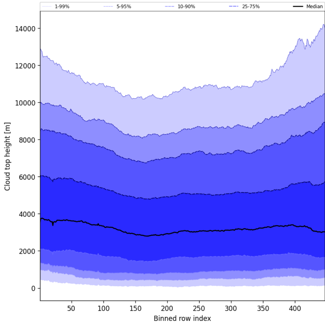
Figure 56: Along track statistics of “Cloud top height” for 2025-07-11 to 2025-07-13
