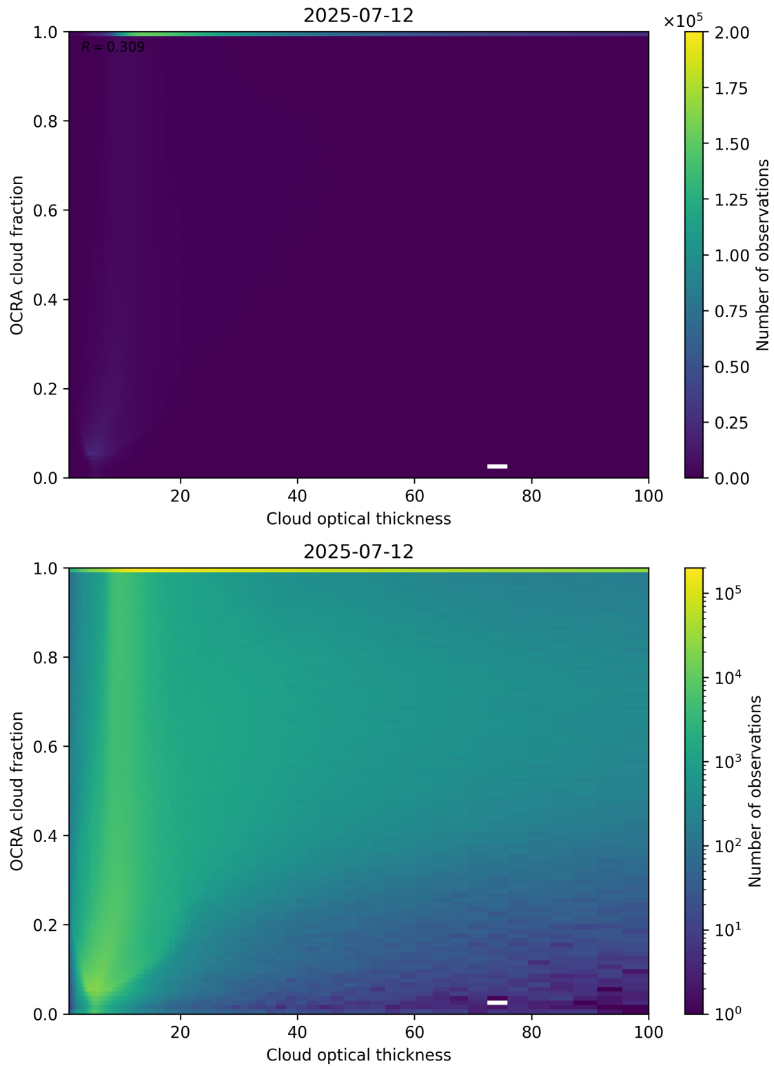
Figure 83: Scatter density plot of “Cloud optical thickness” against “OCRA cloud fraction” for 2025-07-11 to 2025-07-13.
