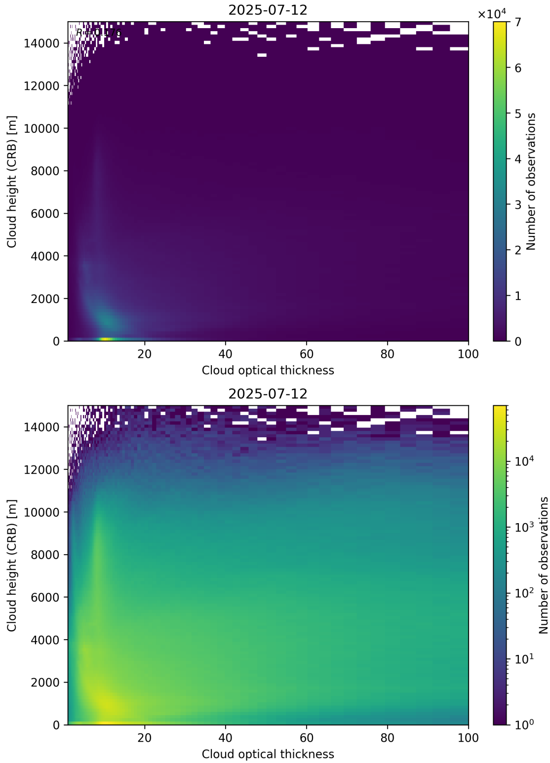
Figure 85: Scatter density plot of “Cloud optical thickness” against “Cloud height (CRB)” for 2025-07-11 to 2025-07-13.
