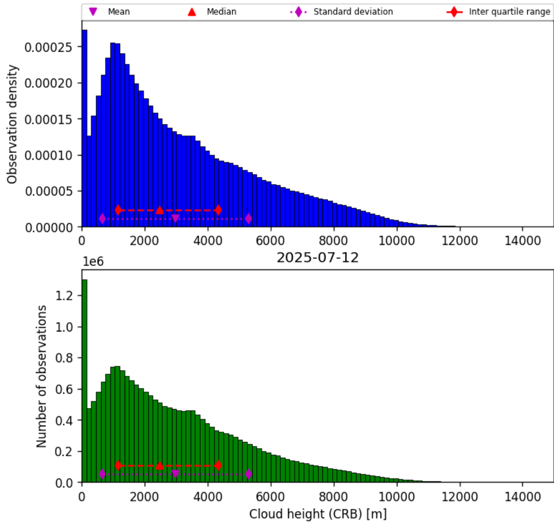
Figure 43: Histogram of “Cloud height (CRB)” for 2025-07-11 to 2025-07-13
