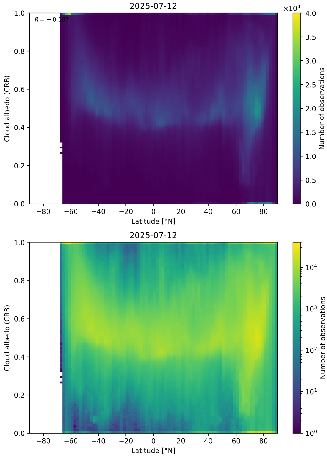
Figure 91: Scatter density plot of “Latitude” against “Cloud albedo (CRB)” for 2025-07-11 to 2025-07-13.
