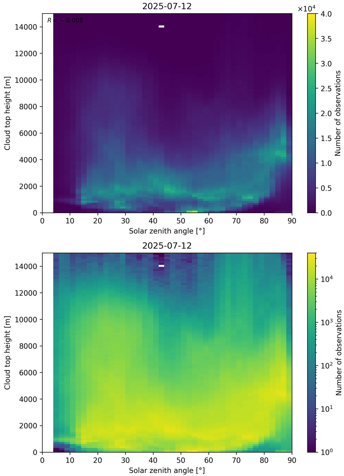
Figure 104: Scatter density plot of “Solar zenith angle” against “Cloud top height” for 2025-07-11 to 2025-07-13.
