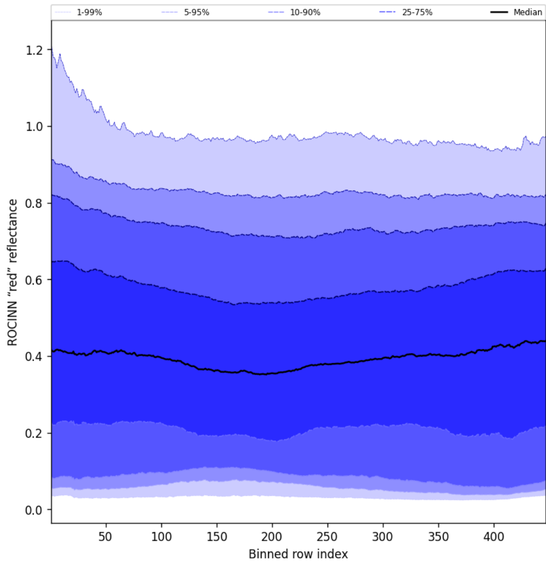
Figure 69: Along track statistics of “ROCINN “red” reflectance” for 2025-07-11 to 2025-07-13
