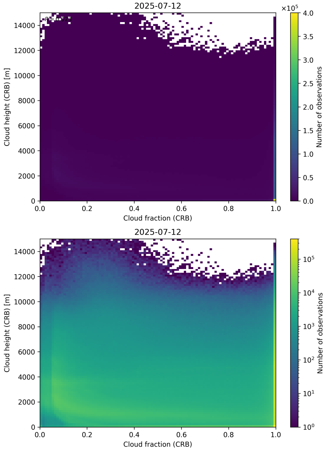
Figure 79: Scatter density plot of “Cloud fraction (CRB)” against “Cloud height (CRB)” for 2025-07-11 to 2025-07-13.
