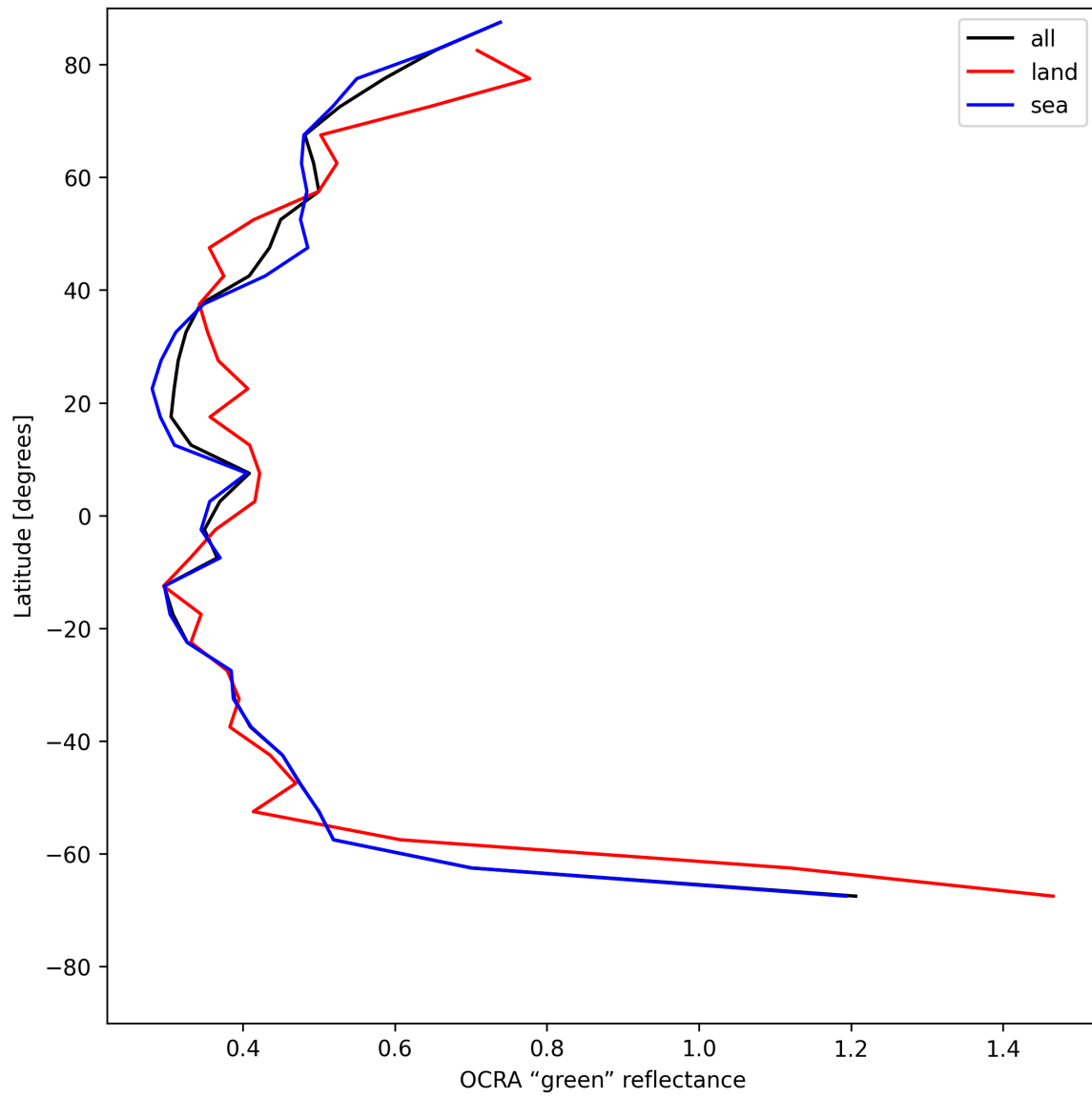
Figure 36: Zonal average of “OCRA “green” reflectance” for 2025-07-11 to 2025-07-13.
