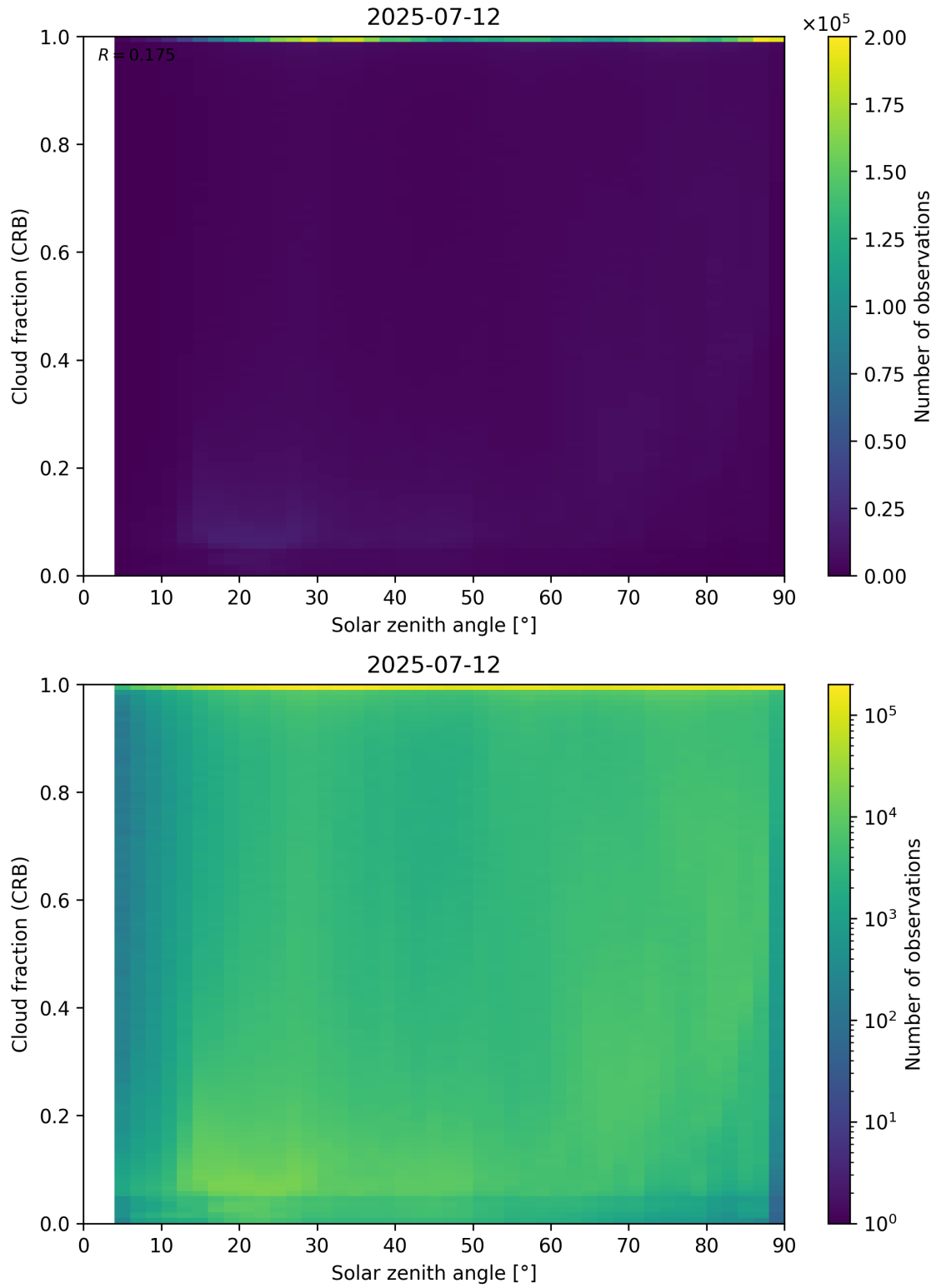
Figure 101: Scatter density plot of “Solar zenith angle” against “Cloud fraction (CRB)” for 2025-07-11 to 2025-07-13.
