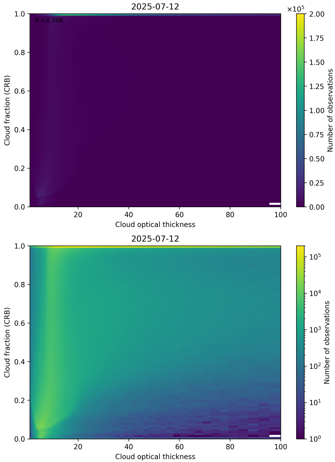
Figure 84: Scatter density plot of “Cloud optical thickness” against “Cloud fraction (CRB)” for 2025-07-11 to 2025-07-13.
