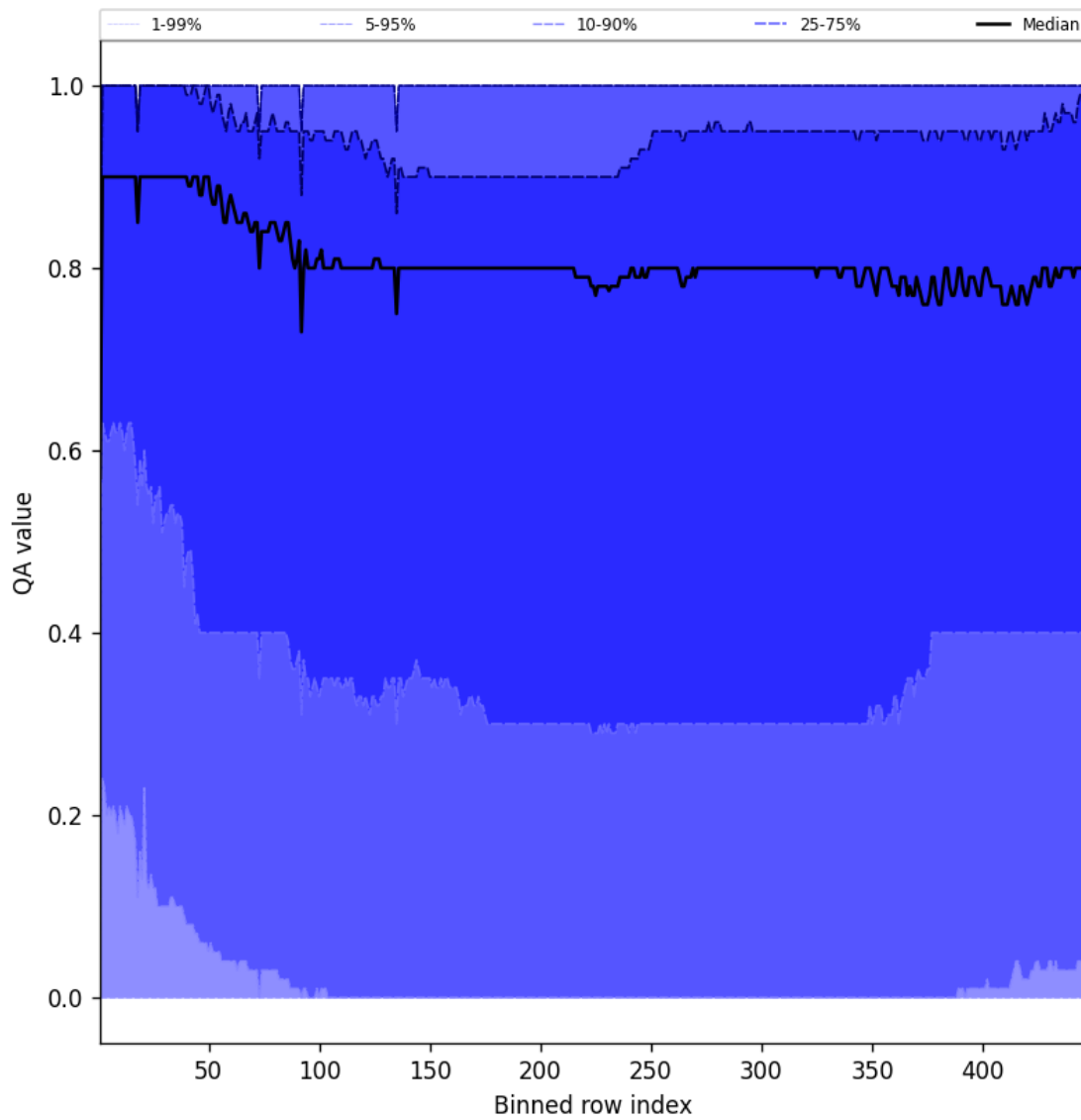
Figure 54: Along track statistics of “QA value” for 2025-07-11 to 2025-07-13
