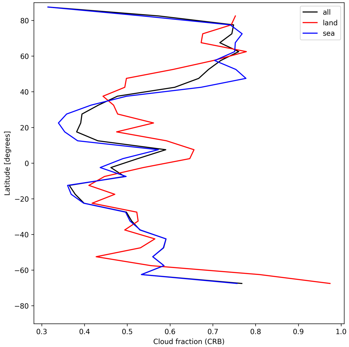
Figure 26: Zonal average of “Cloud fraction (CRB)” for 2025-07-11 to 2025-07-13.
