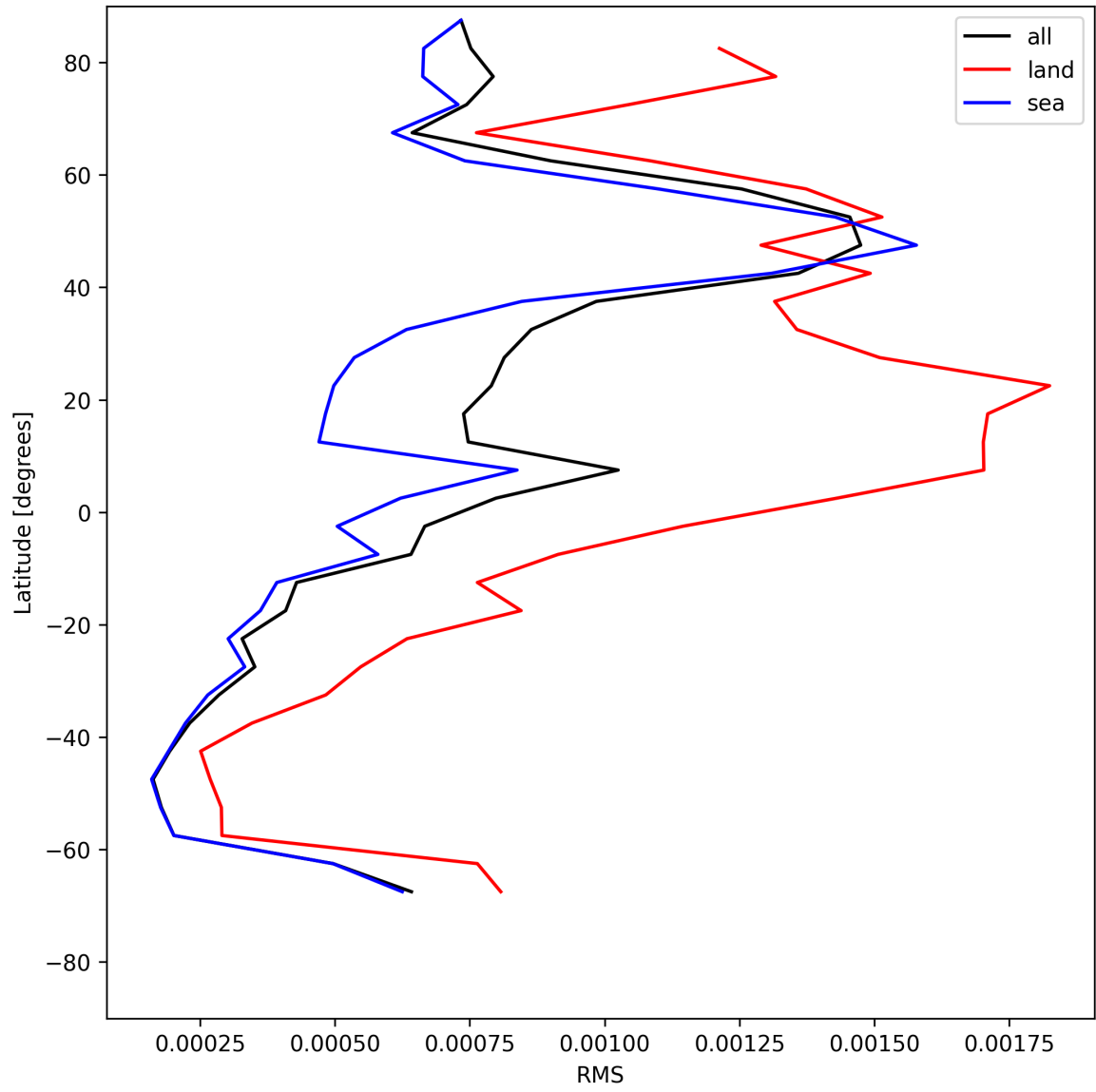
Figure 31: Zonal average of “RMS” for 2025-07-11 to 2025-07-13.
