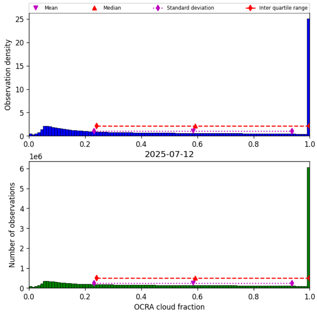
Figure 50: Histogram of “OCRA cloud fraction” for 2025-07-11 to 2025-07-13
