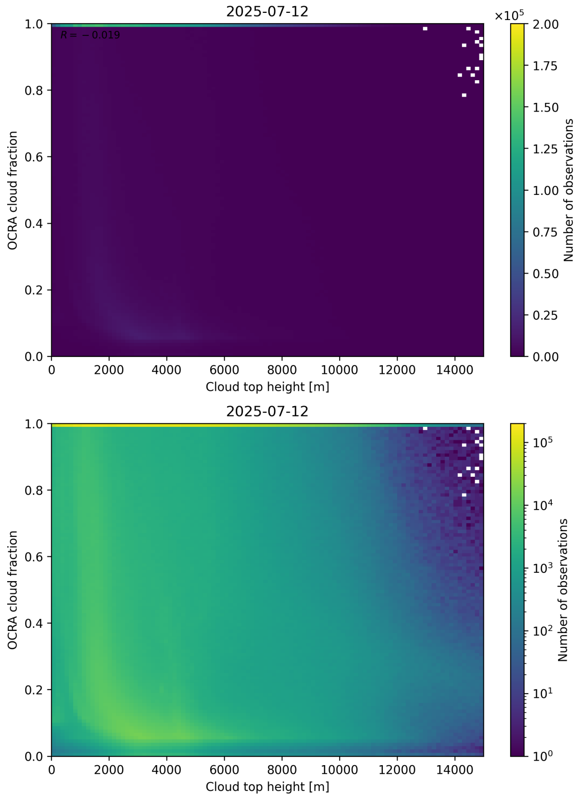
Figure 87: Scatter density plot of “Cloud top height” against “OCRA cloud fraction” for 2025-07-11 to 2025-07-13.
