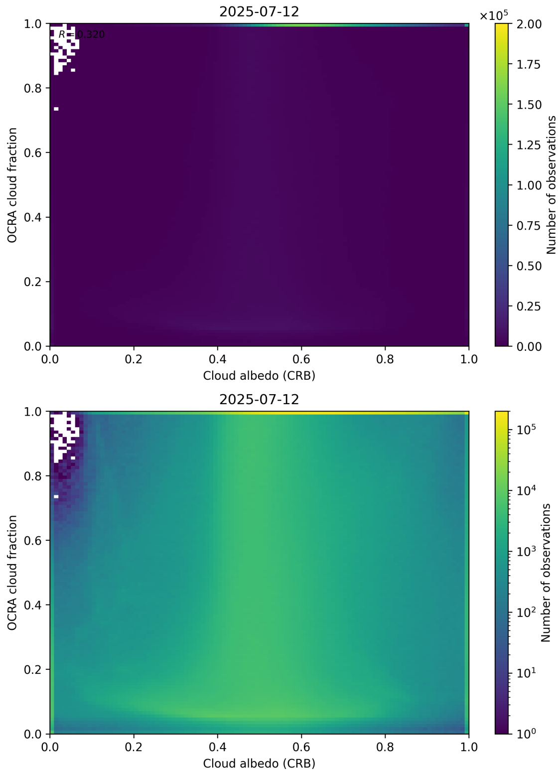
Figure 70: Scatter density plot of “Cloud albedo (CRB)” against “OCRA cloud fraction” for 2025-07-11 to 2025-07-13.
