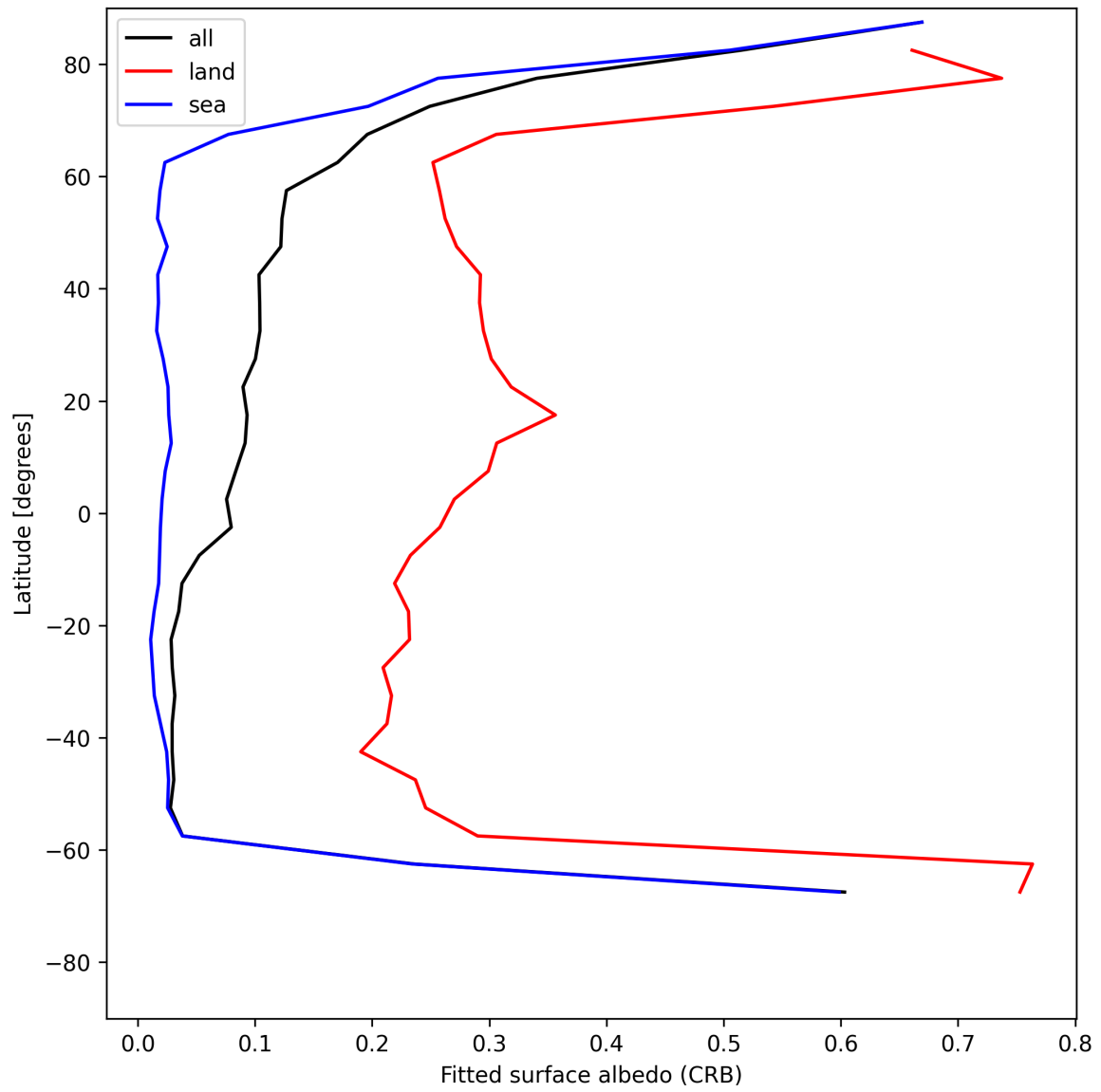
Figure 30: Zonal average of “Fitted surface albedo (CRB)” for 2025-07-11 to 2025-07-13.
