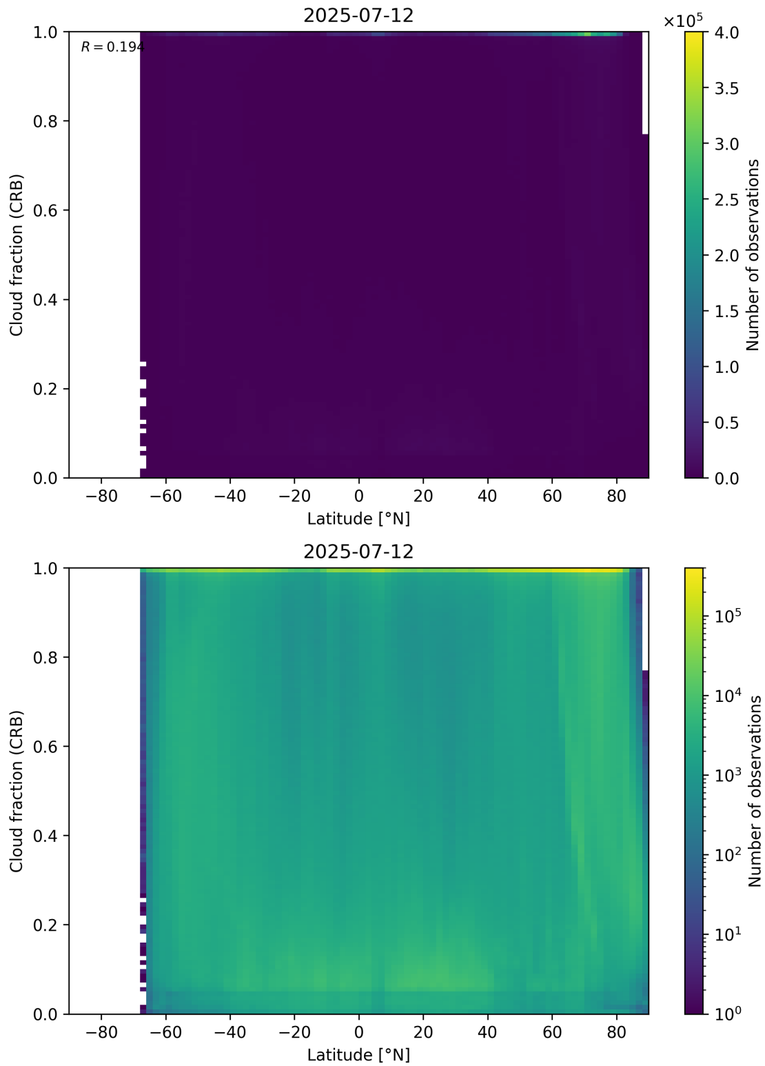
Figure 94: Scatter density plot of “Latitude” against “Cloud fraction (CRB)” for 2025-07-11 to 2025-07-13.
