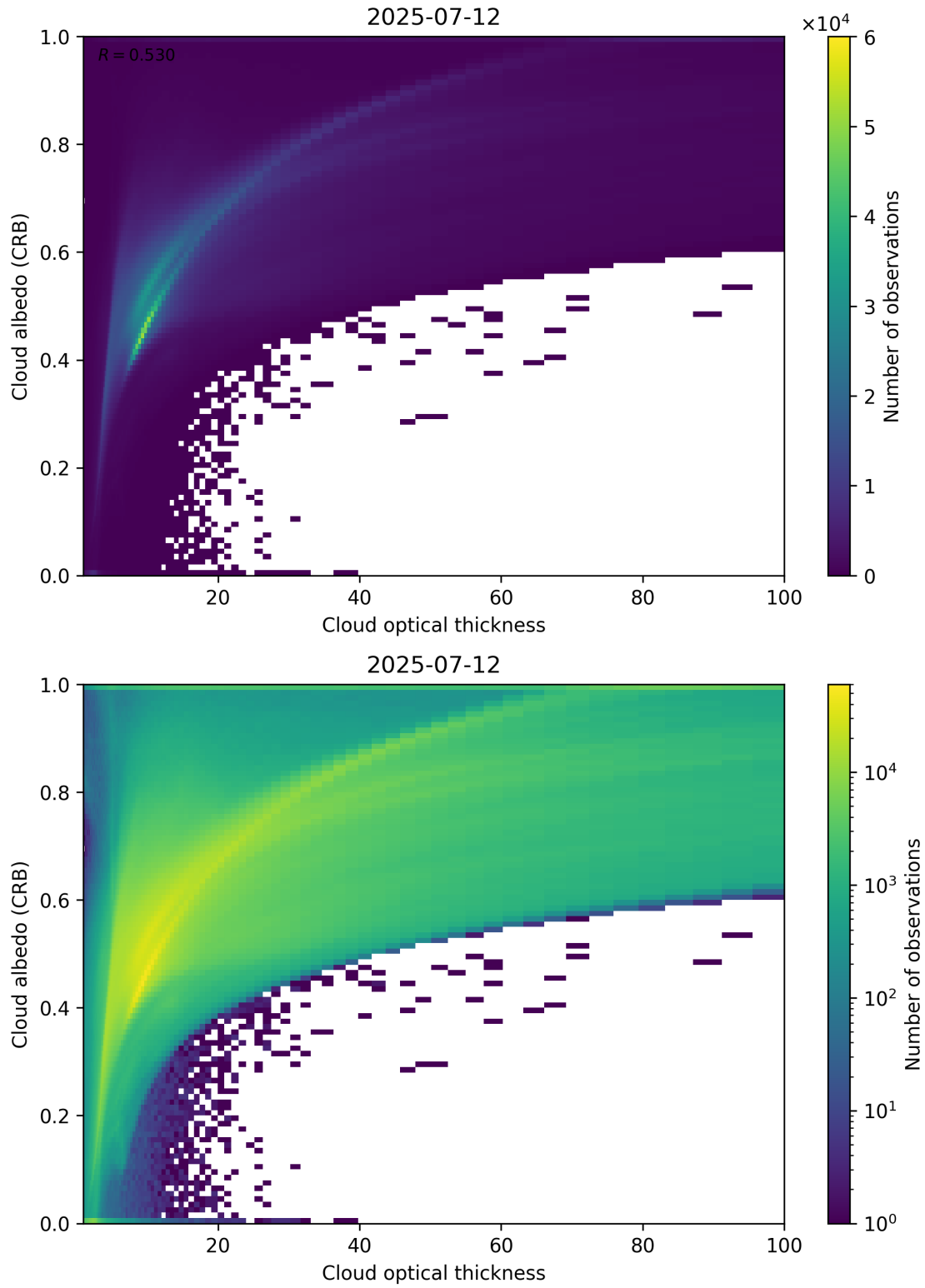
Figure 82: Scatter density plot of “Cloud optical thickness” against “Cloud albedo (CRB)” for 2025-07-11 to 2025-07-13.
