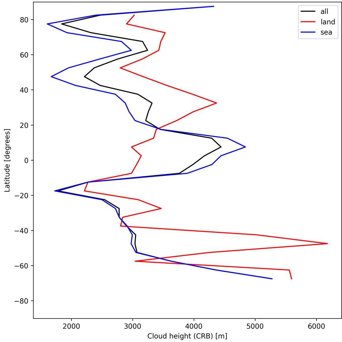
Figure 27: Zonal average of “Cloud height (CRB)” for 2025-07-11 to 2025-07-13.
