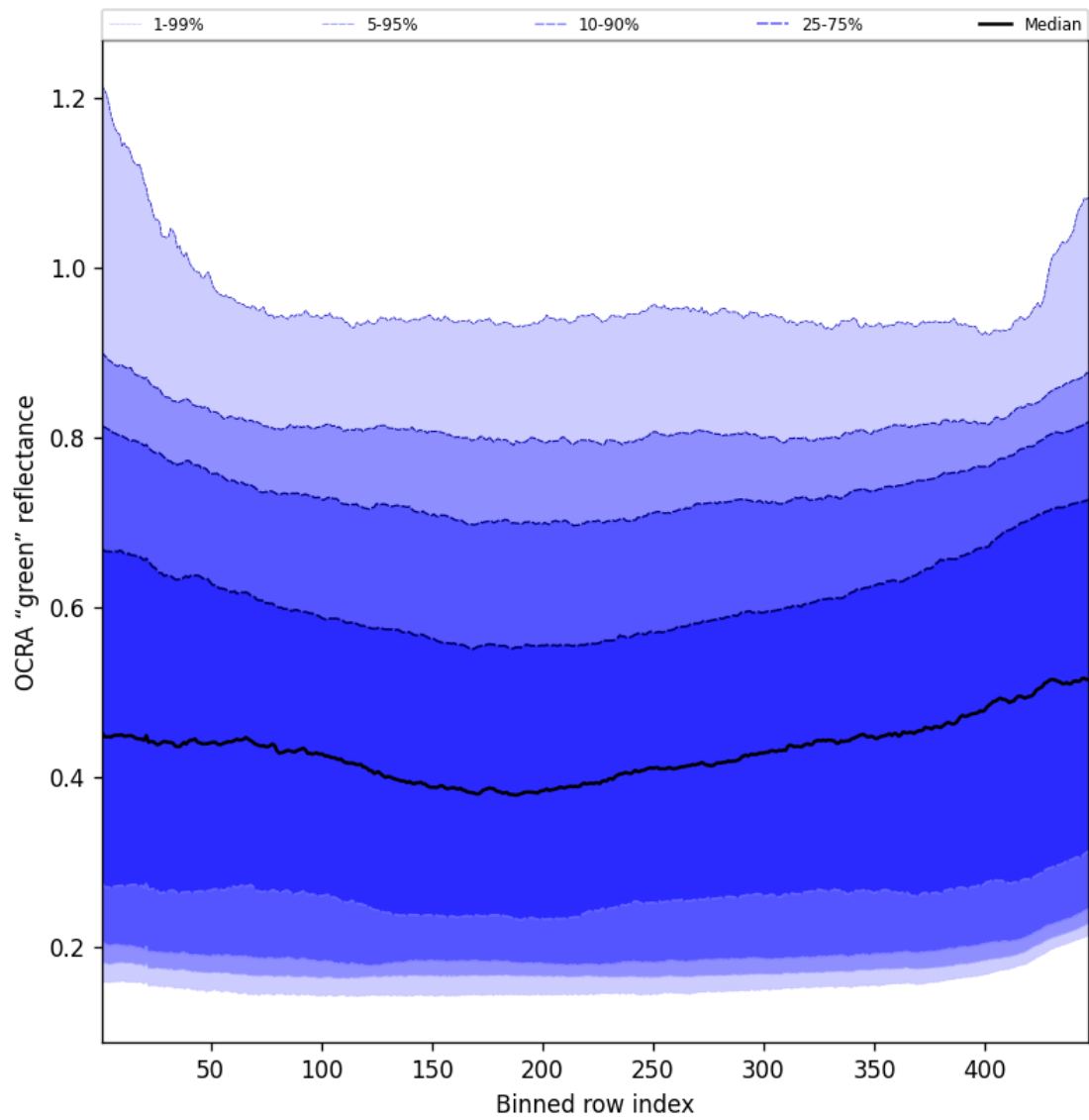
Figure 68: Along track statistics of “OCRA “green” reflectance” for 2025-07-11 to 2025-07-13
