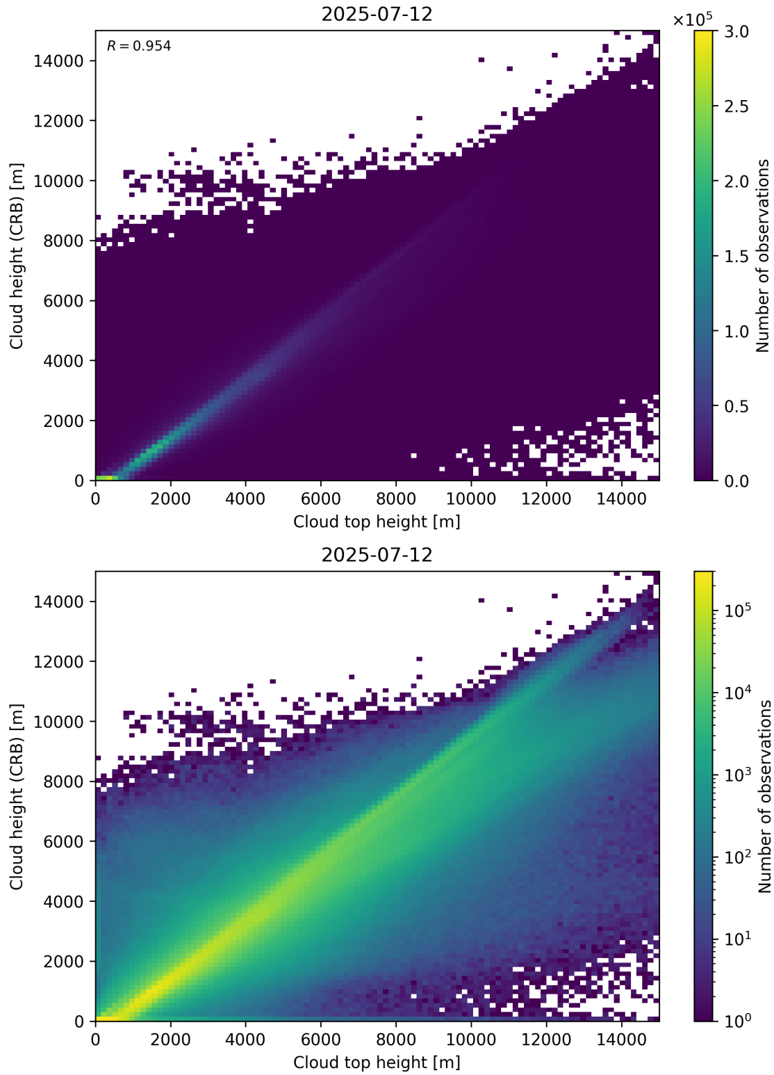
Figure 89: Scatter density plot of “Cloud top height” against “Cloud height (CRB)” for 2025-07-11 to 2025-07-13.
