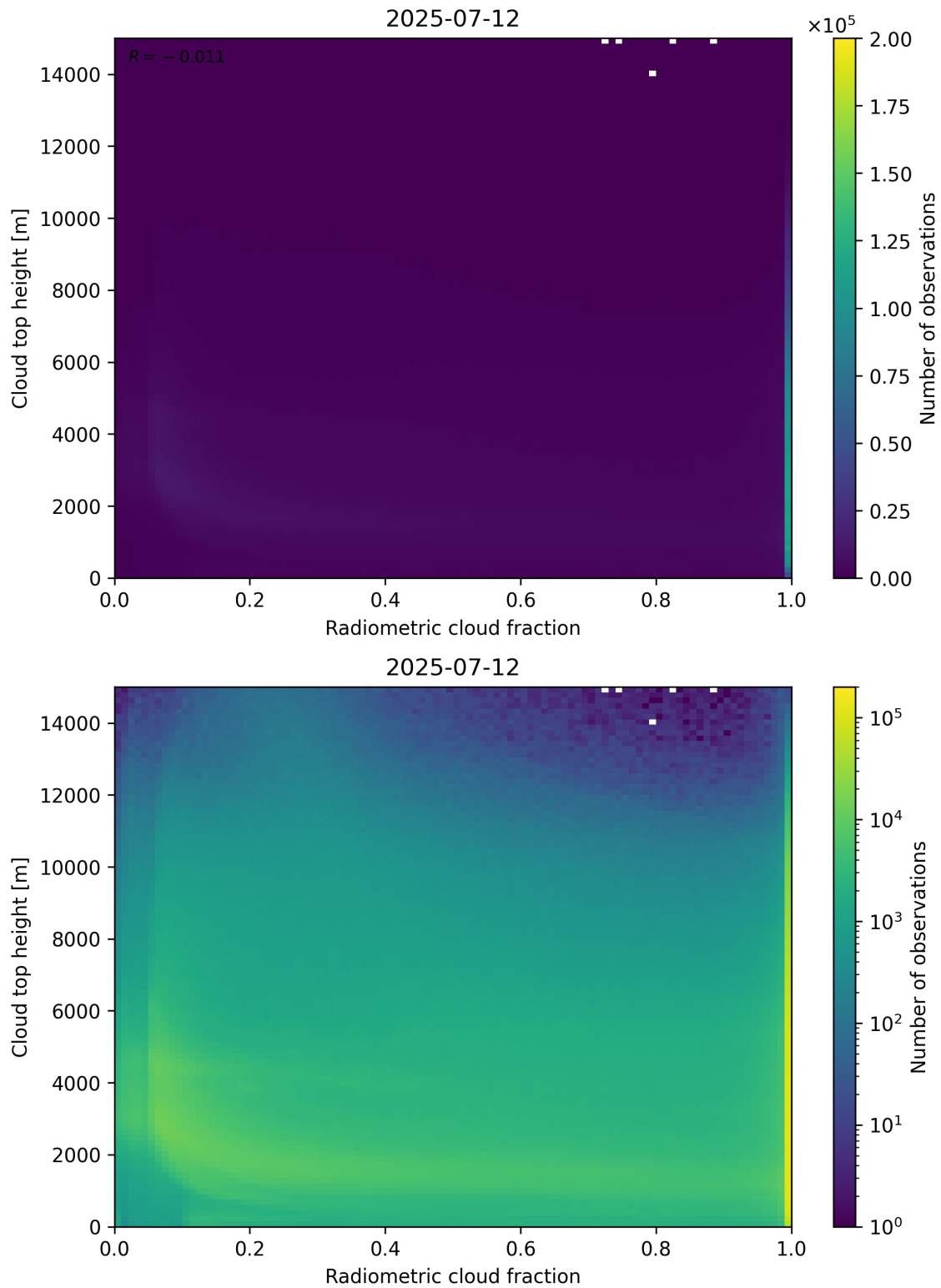
Figure 76: Scatter density plot of “Radiometric cloud fraction” against “Cloud top height” for 2025-07-11 to 2025-07-13.
