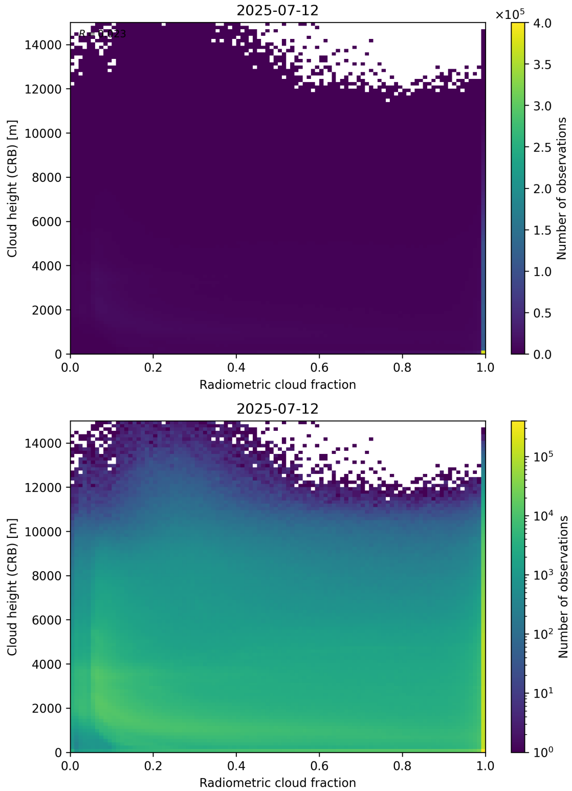
Figure 74: Scatter density plot of “Radiometric cloud fraction” against “Cloud height (CRB)” for 2025-07-11 to 2025-07-13.
