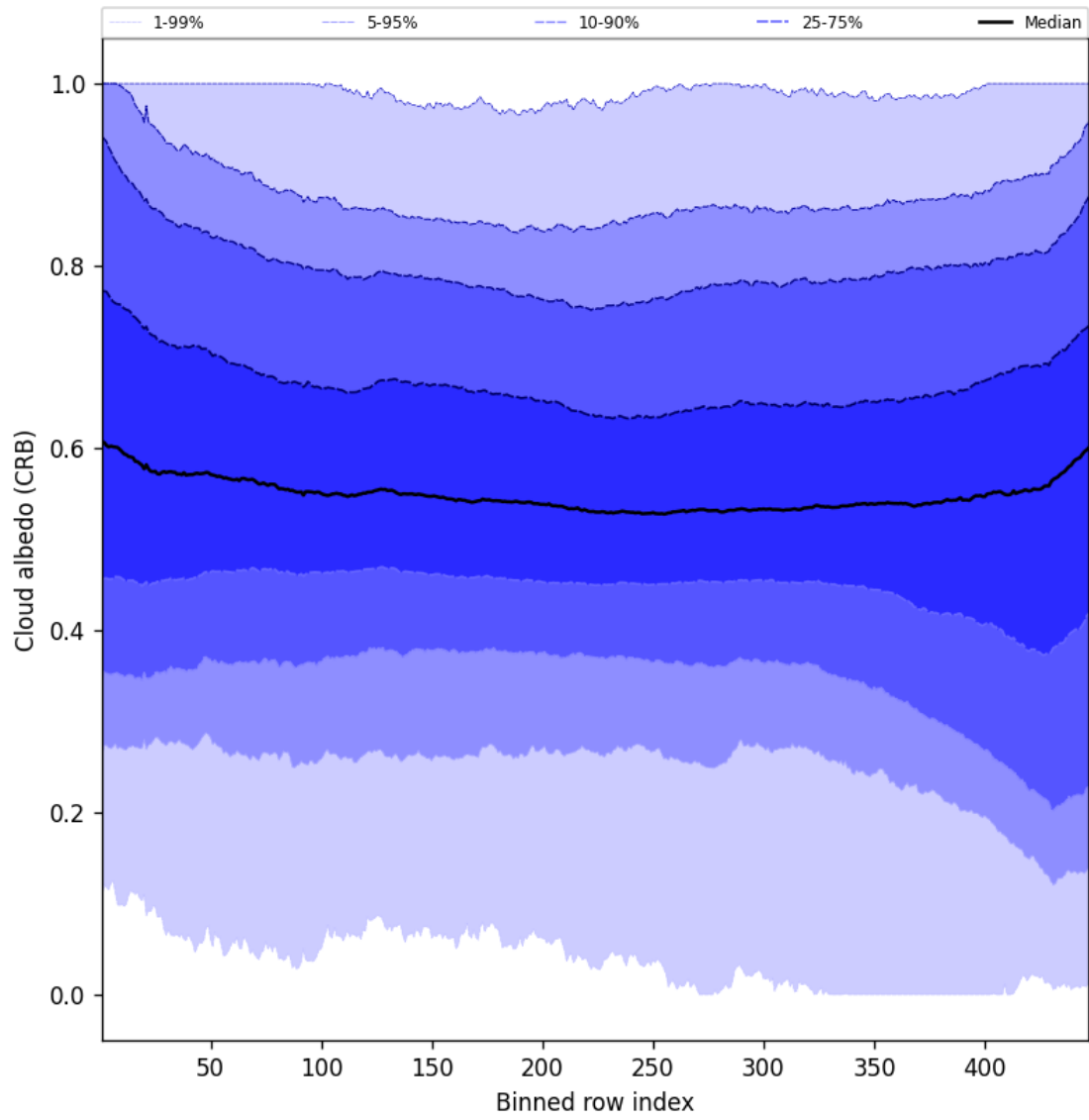
Figure 60: Along track statistics of “Cloud albedo (CRB)” for 2025-07-11 to 2025-07-13
