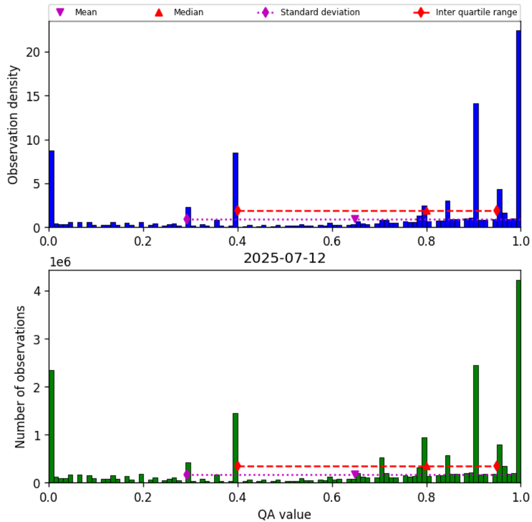
Figure 38: Histogram of “QA value” for 2025-07-11 to 2025-07-13
