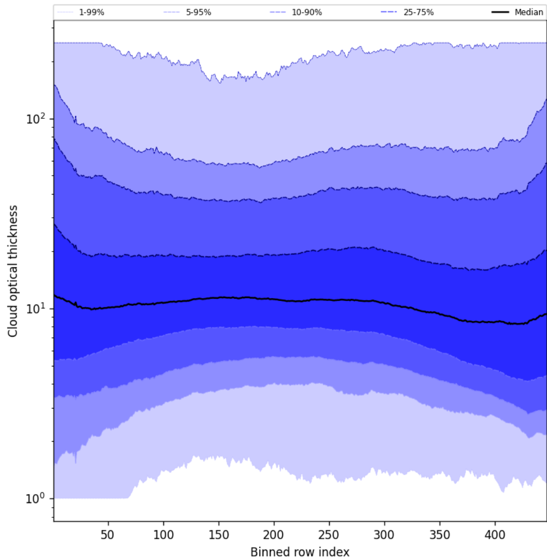
Figure 57: Along track statistics of “Cloud optical thickness” for 2025-07-11 to 2025-07-13
