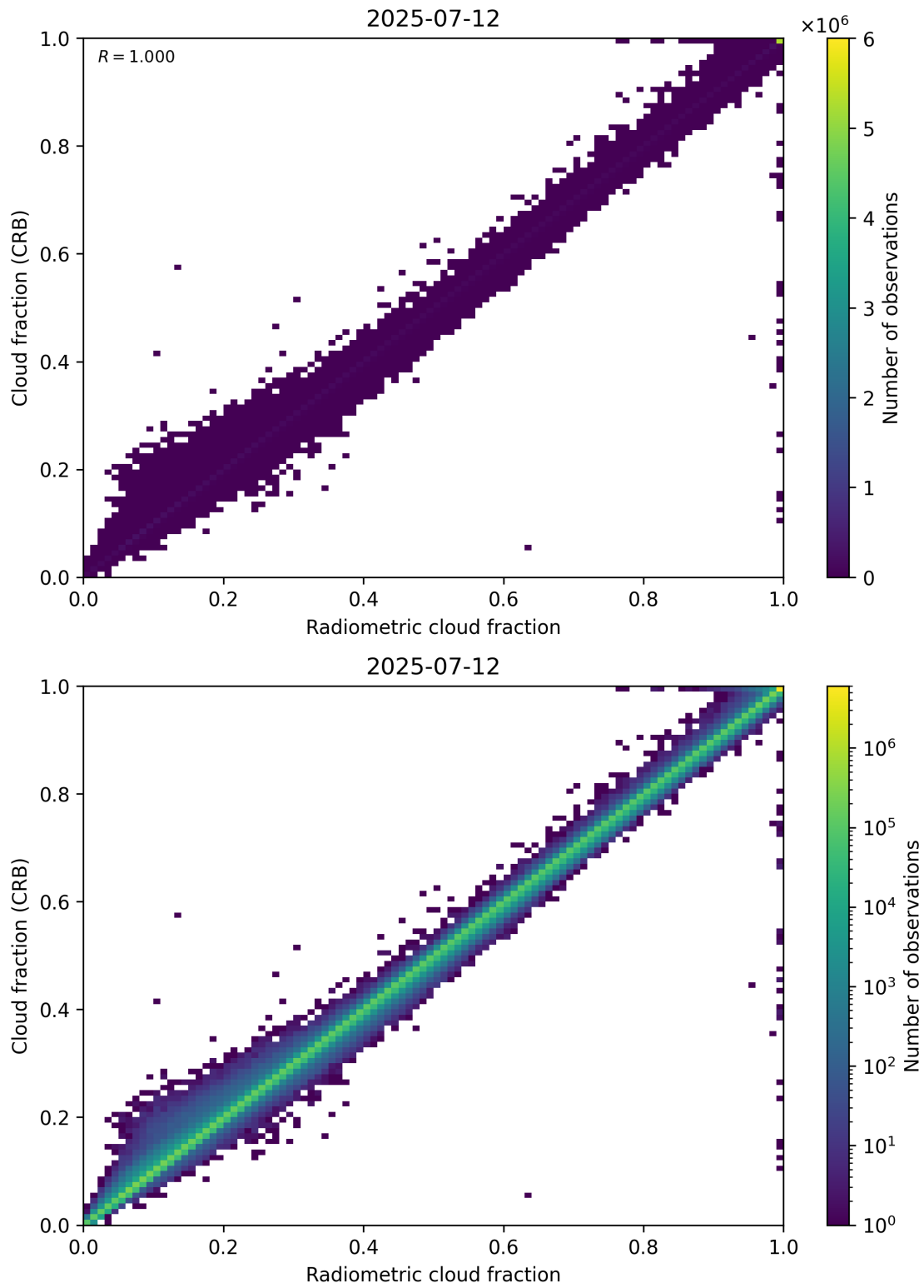
Figure 73: Scatter density plot of “Radiometric cloud fraction” against “Cloud fraction (CRB)” for 2025-07-11 to 2025-07-13.
