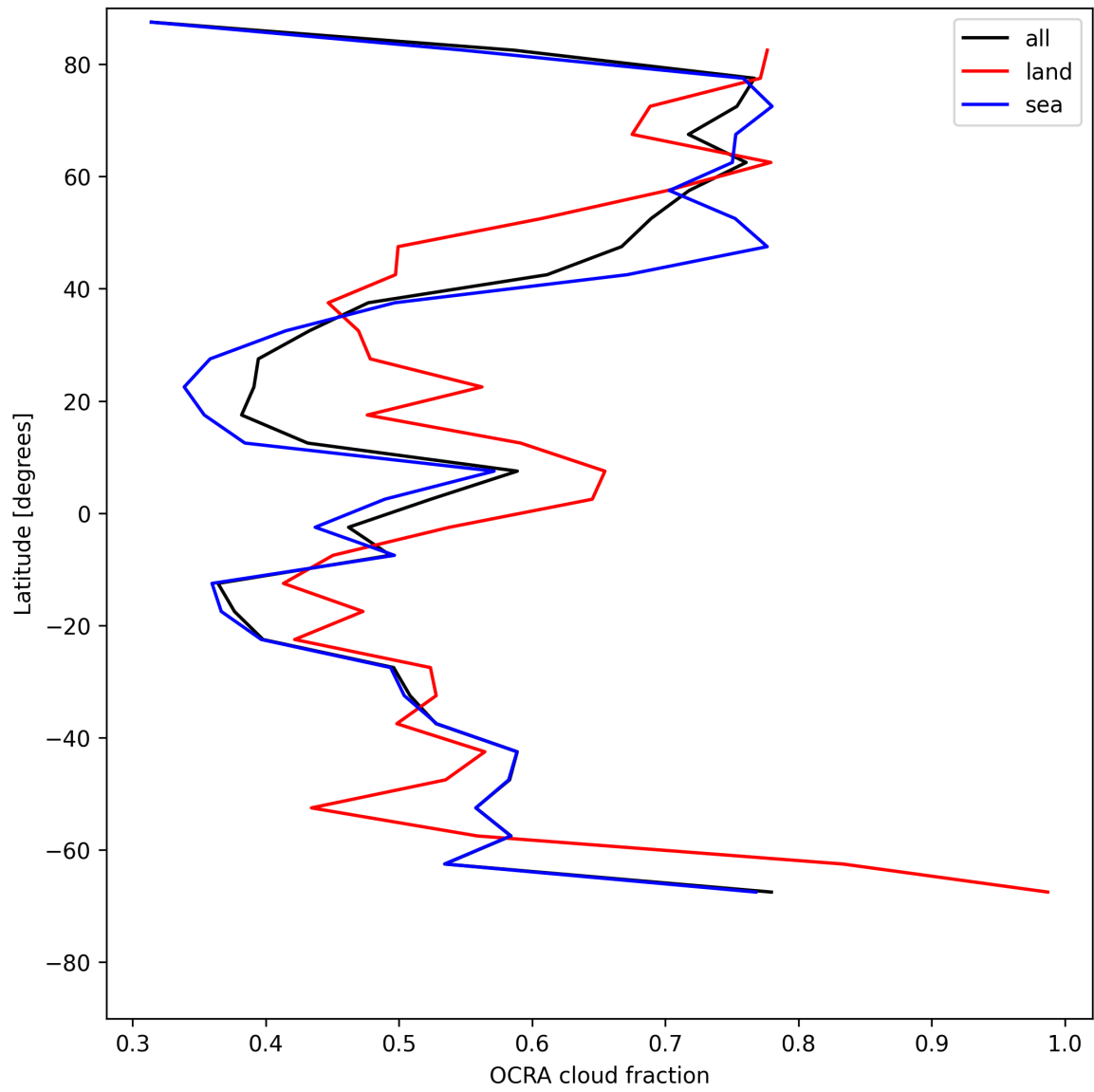
Figure 34: Zonal average of “OCRA cloud fraction” for 2025-07-11 to 2025-07-13.
