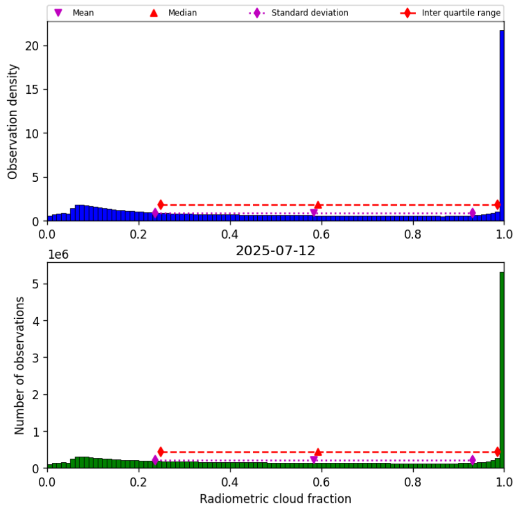
Figure 39: Histogram of “Radiometric cloud fraction” for 2025-07-11 to 2025-07-13
