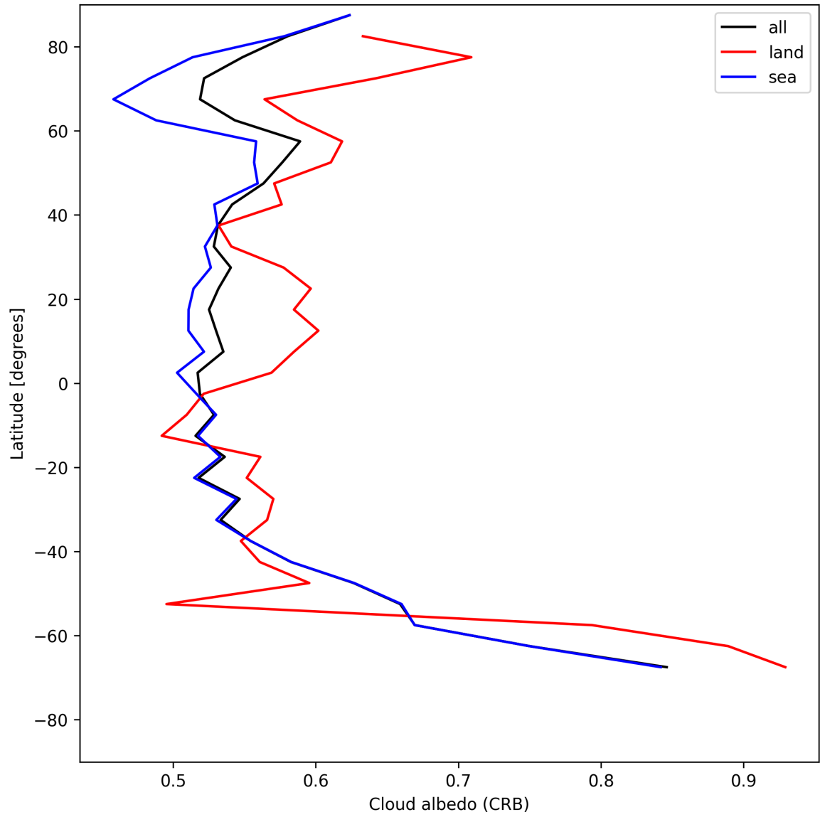
Figure 28: Zonal average of “Cloud albedo (CRB)” for 2025-07-11 to 2025-07-13.
