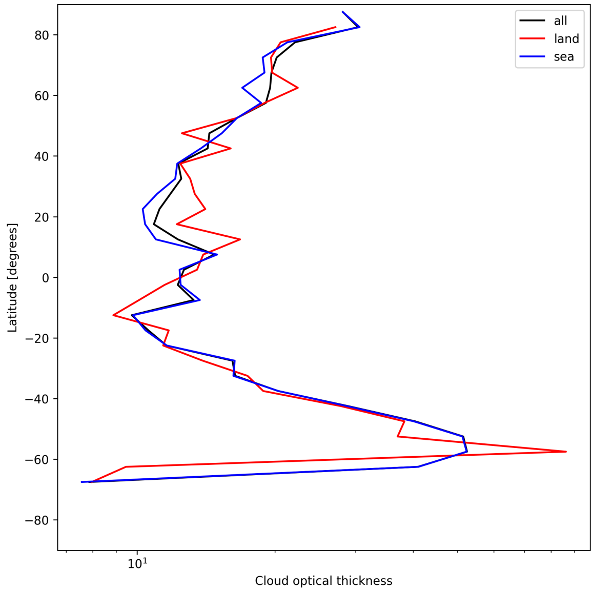
Figure 25: Zonal average of “Cloud optical thickness” for 2025-07-11 to 2025-07-13.
