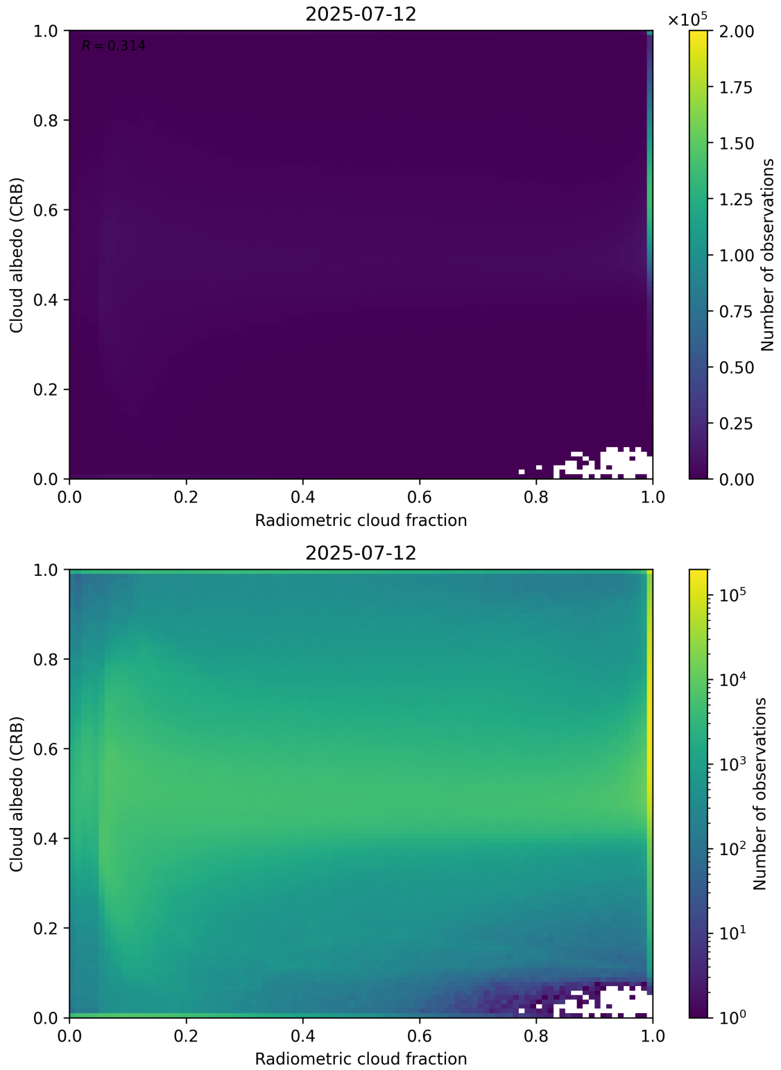
Figure 71: Scatter density plot of “Radiometric cloud fraction” against “Cloud albedo (CRB)” for 2025-07-11 to 2025-07-13.
