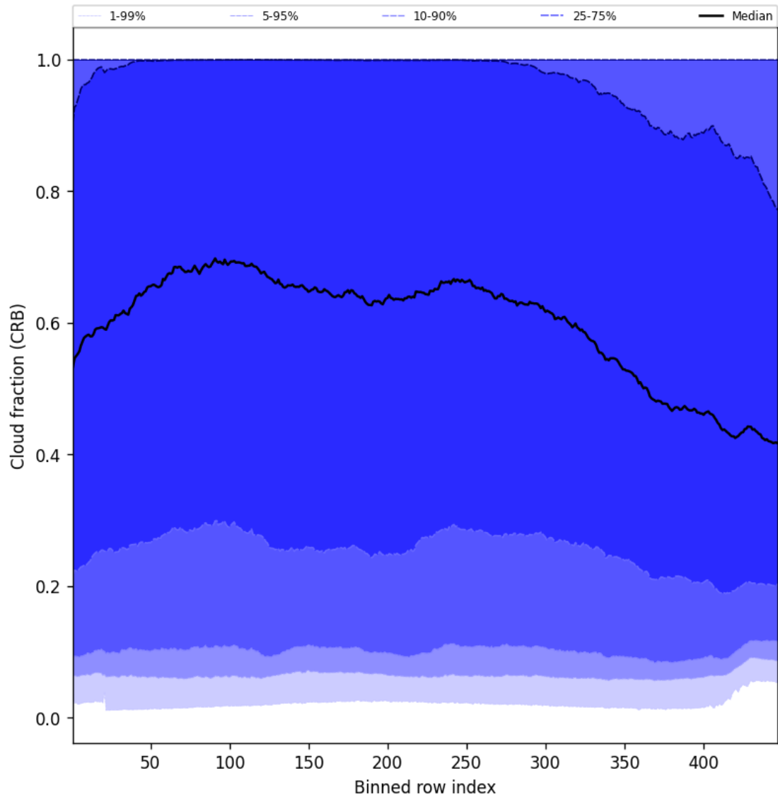
Figure 58: Along track statistics of “Cloud fraction (CRB)” for 2025-07-11 to 2025-07-13
