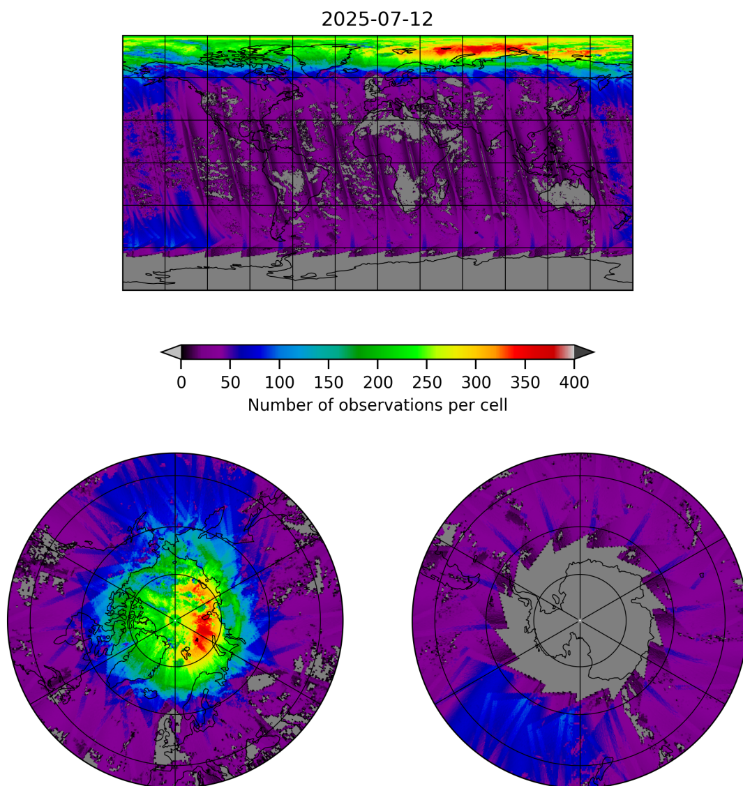
Figure 21: Map of the number of observations for 2025-07-11 to 2025-07-13
