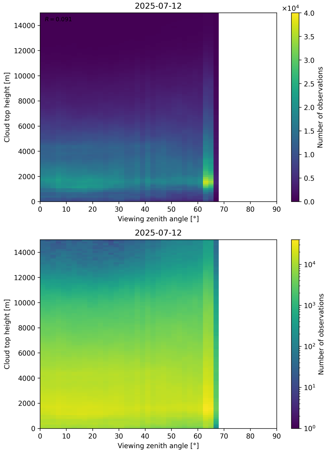
Figure 112: Scatter density plot of “Viewing zenith angle” against “Cloud top height” for 2025-07-11 to 2025-07-13.
