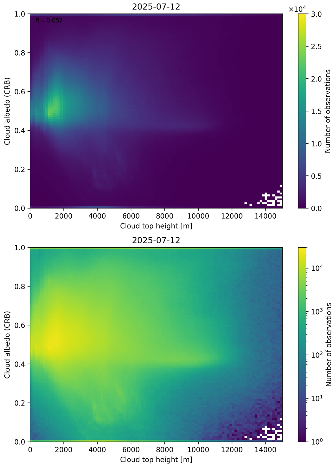
Figure 86: Scatter density plot of “Cloud top height” against “Cloud albedo (CRB)” for 2025-07-11 to 2025-07-13.
