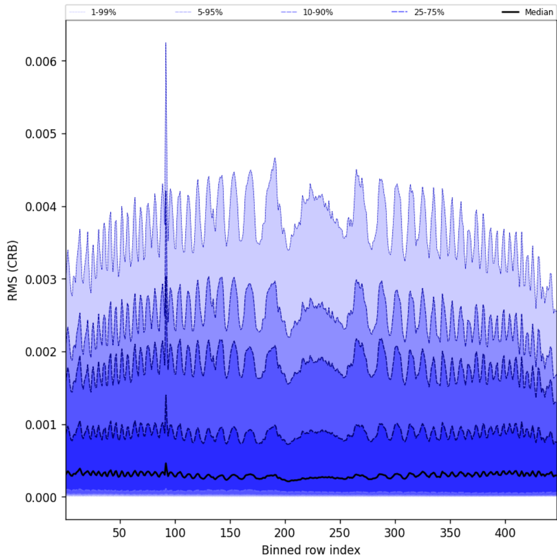
Figure 64: Along track statistics of “RMS (CRB)” for 2025-07-11 to 2025-07-13
