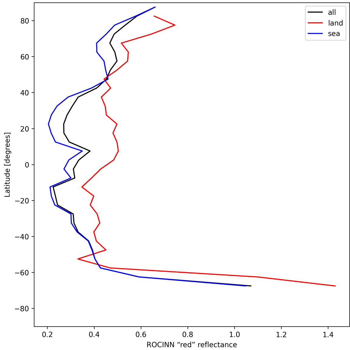
Figure 37: Zonal average of “ROCINN “red” reflectance” for 2025-07-11 to 2025-07-13.
