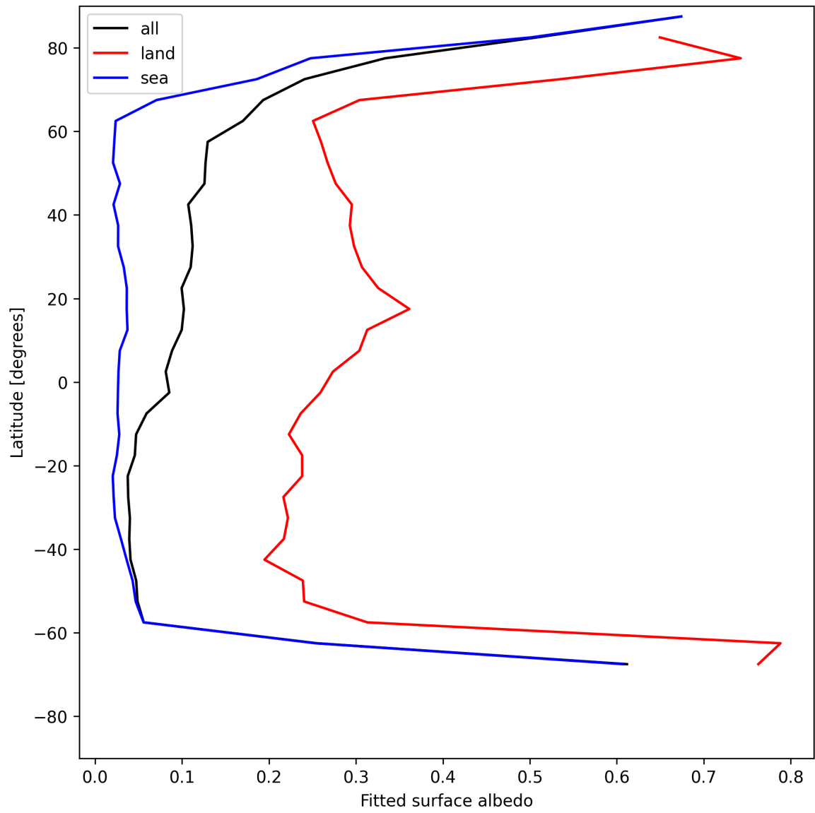
Figure 29: Zonal average of “Fitted surface albedo” for 2025-07-11 to 2025-07-13.
