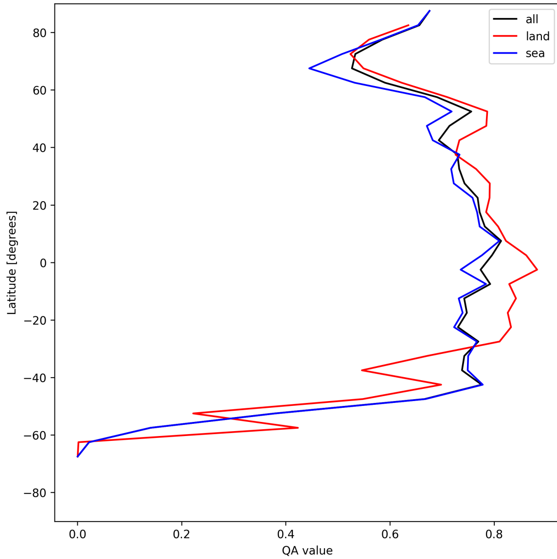
Figure 22: Zonal average of “QA value” for 2025-07-11 to 2025-07-13.
