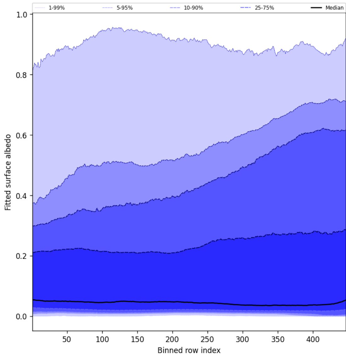
Figure 61: Along track statistics of “Fitted surface albedo” for 2025-07-11 to 2025-07-13
