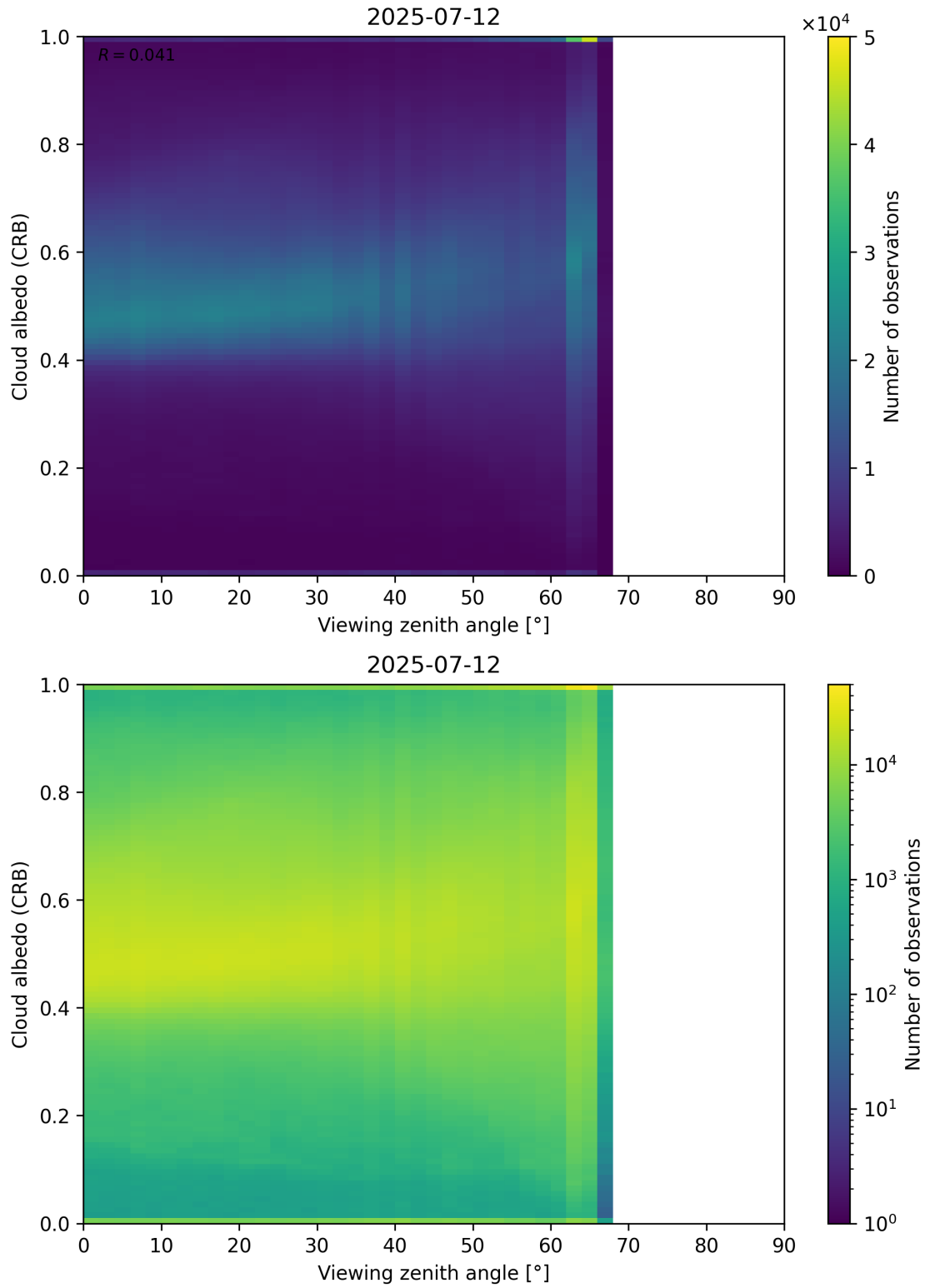
Figure 106: Scatter density plot of “Viewing zenith angle” against “Cloud albedo (CRB)” for 2025-07-11 to 2025-07-13.
