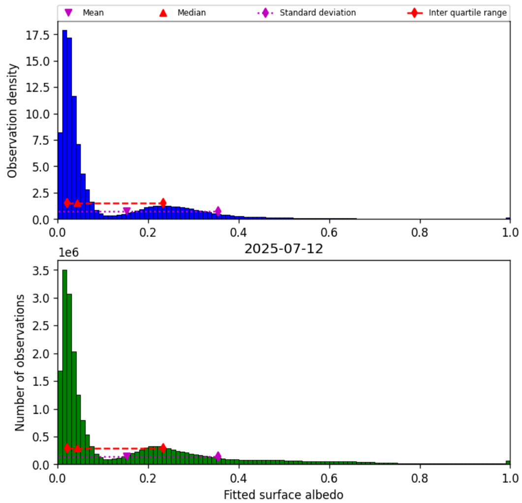
Figure 45: Histogram of “Fitted surface albedo” for 2025-07-11 to 2025-07-13
