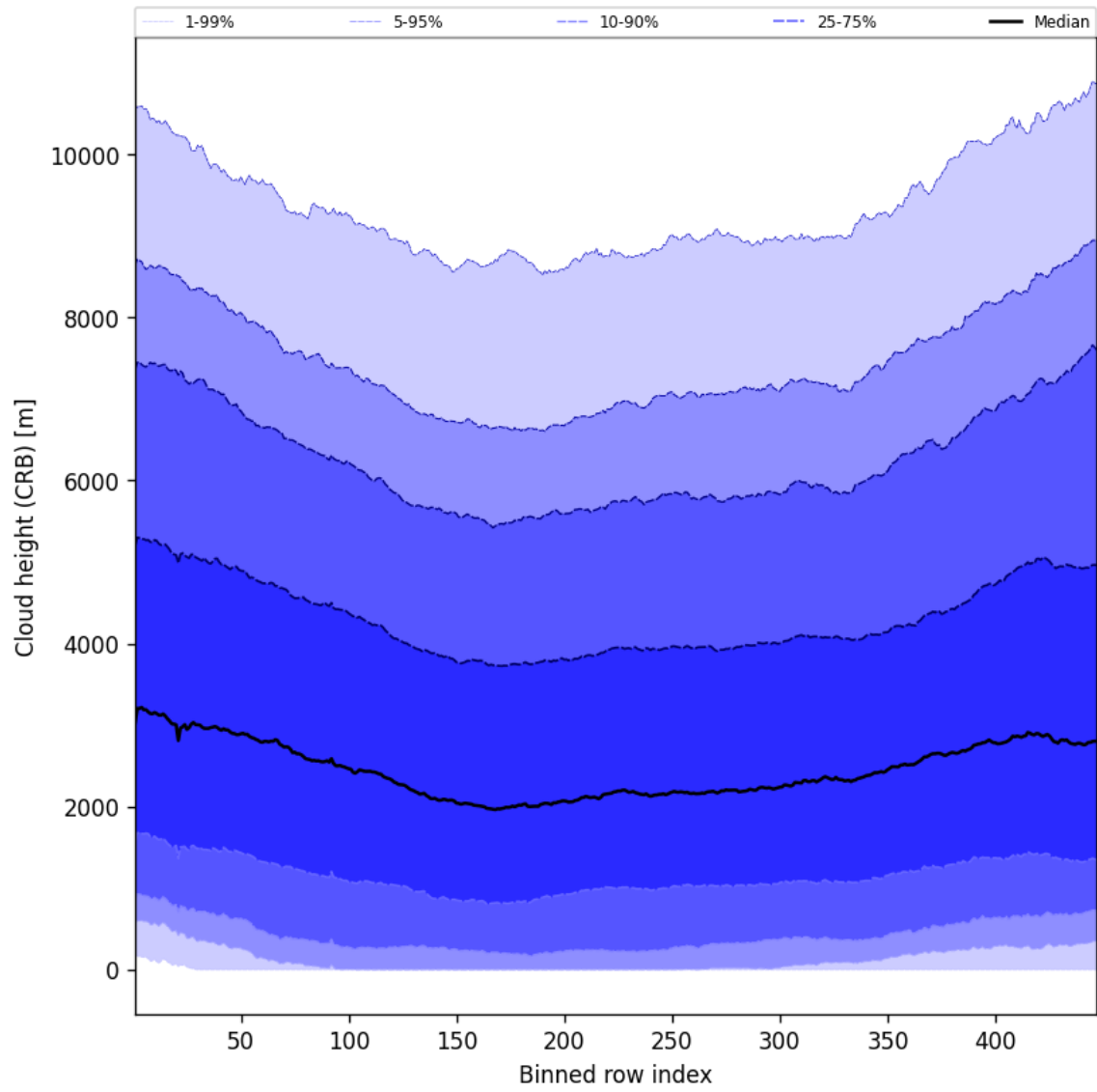
Figure 59: Along track statistics of “Cloud height (CRB)” for 2025-07-11 to 2025-07-13
