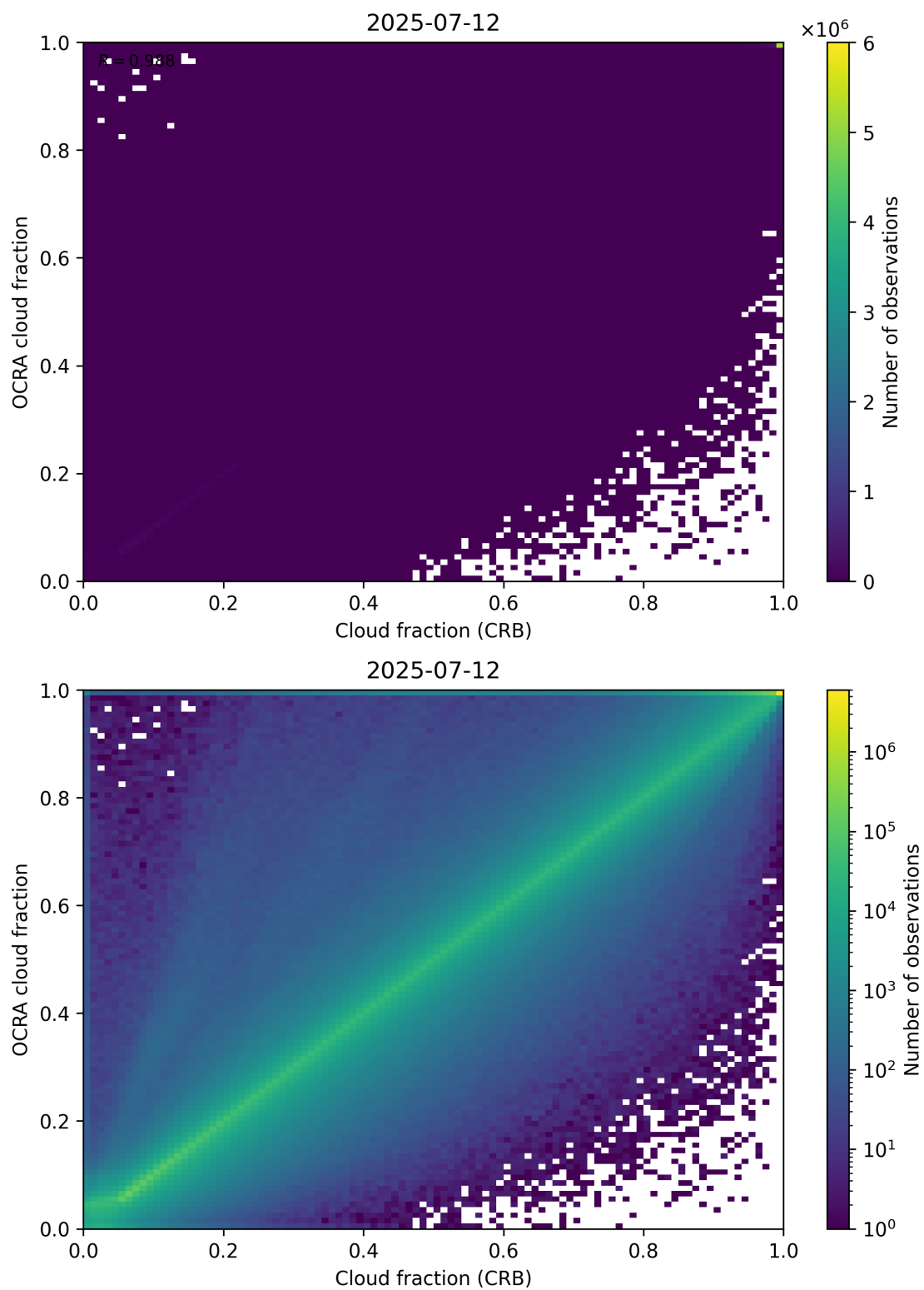
Figure 78: Scatter density plot of “Cloud fraction (CRB)” against “OCRA cloud fraction” for 2025-07-11 to 2025-07-13.
