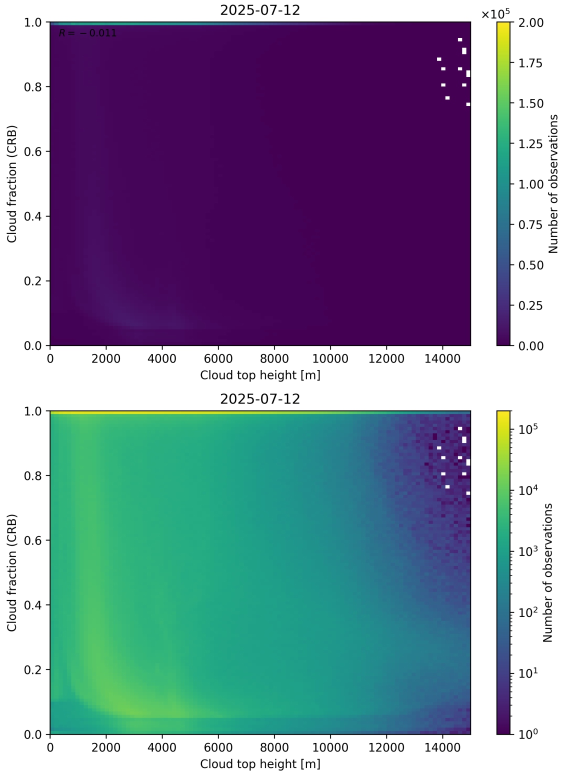
Figure 88: Scatter density plot of “Cloud top height” against “Cloud fraction (CRB)” for 2025-07-11 to 2025-07-13.
