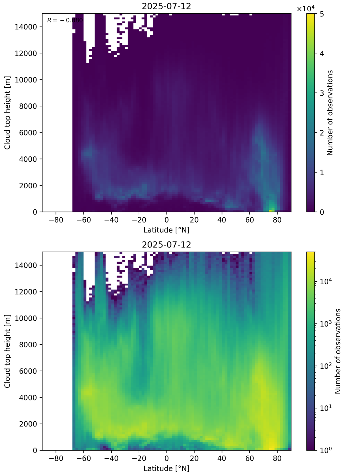
Figure 97: Scatter density plot of “Latitude” against “Cloud top height” for 2025-07-11 to 2025-07-13.
