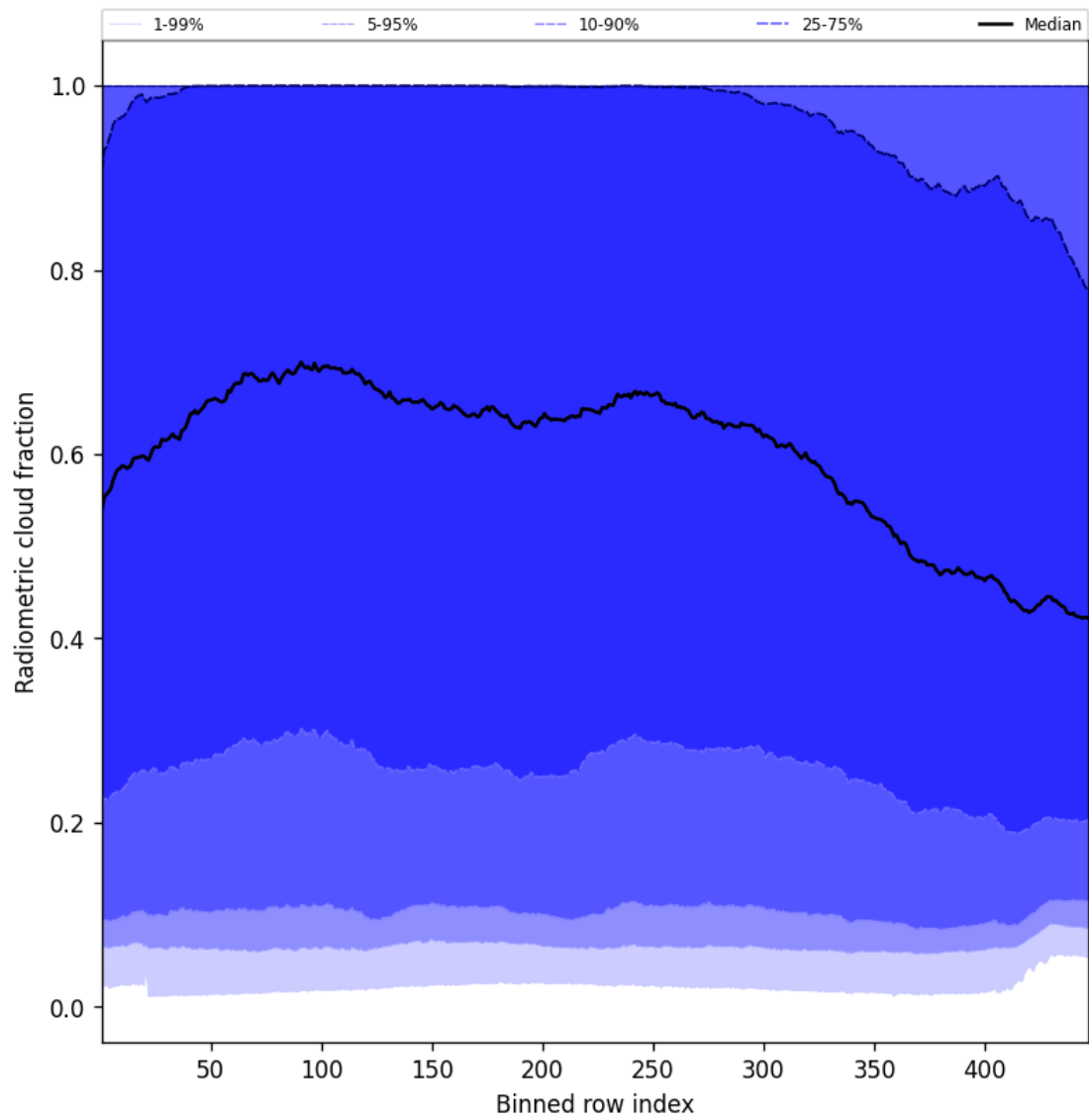
Figure 55: Along track statistics of “Radiometric cloud fraction” for 2025-07-11 to 2025-07-13
