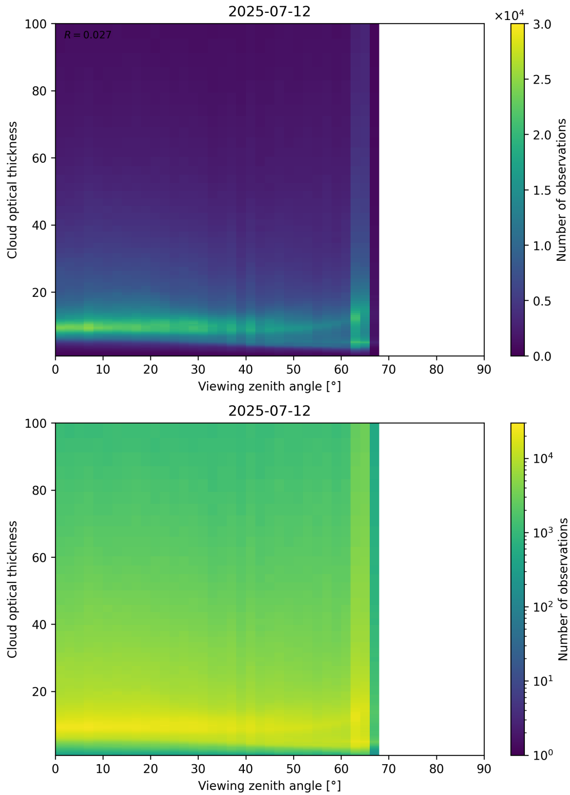
Figure 111: Scatter density plot of “Viewing zenith angle” against “Cloud optical thickness” for 2025-07-11 to 2025-07-13.
