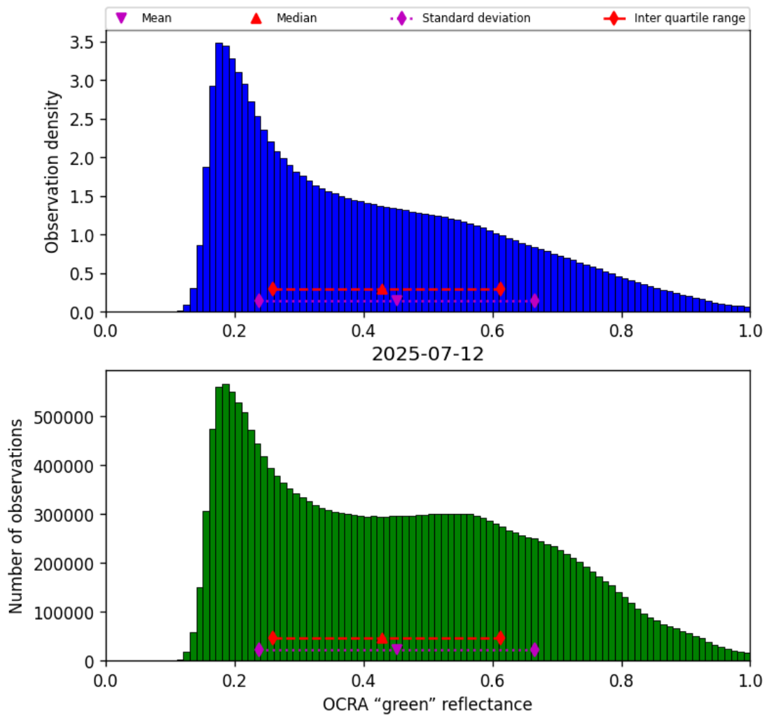
Figure 52: Histogram of “OCRA “green” reflectance” for 2025-07-11 to 2025-07-13
