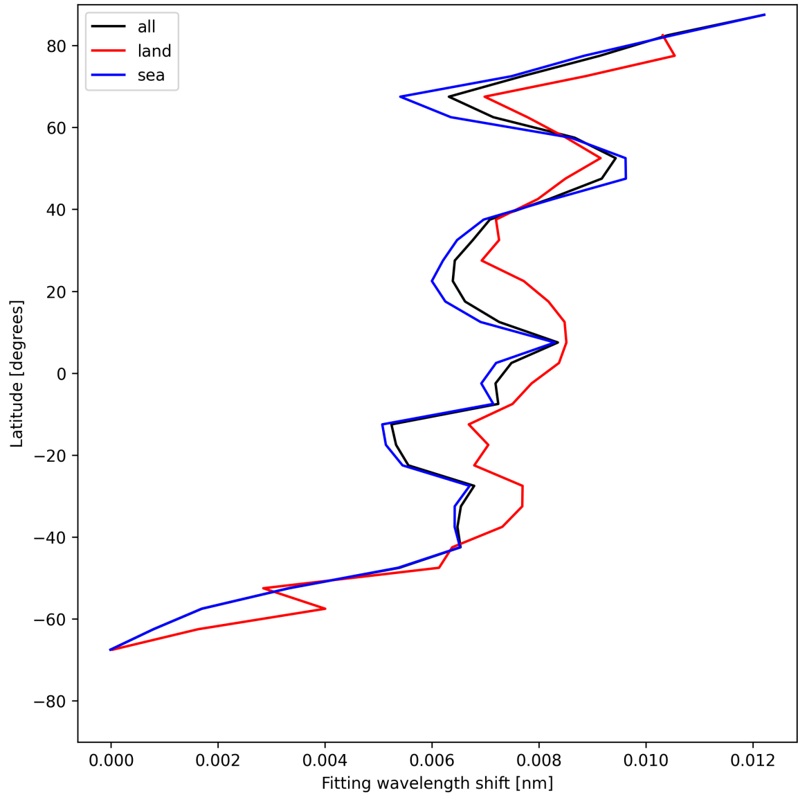
Figure 33: Zonal average of “Fitting wavelength shift” for 2025-07-11 to 2025-07-13.
