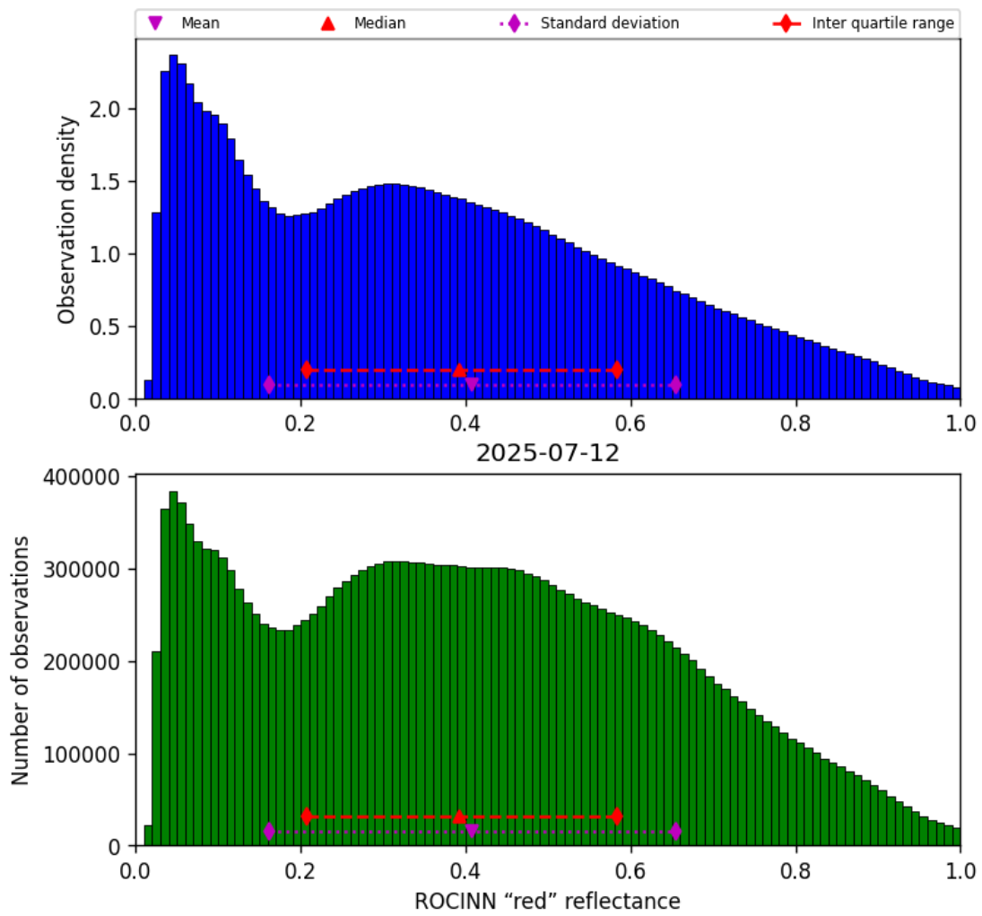
Figure 53: Histogram of "ROCINN "red" reflectance" for 2025-07-11 to 2025-07-13
