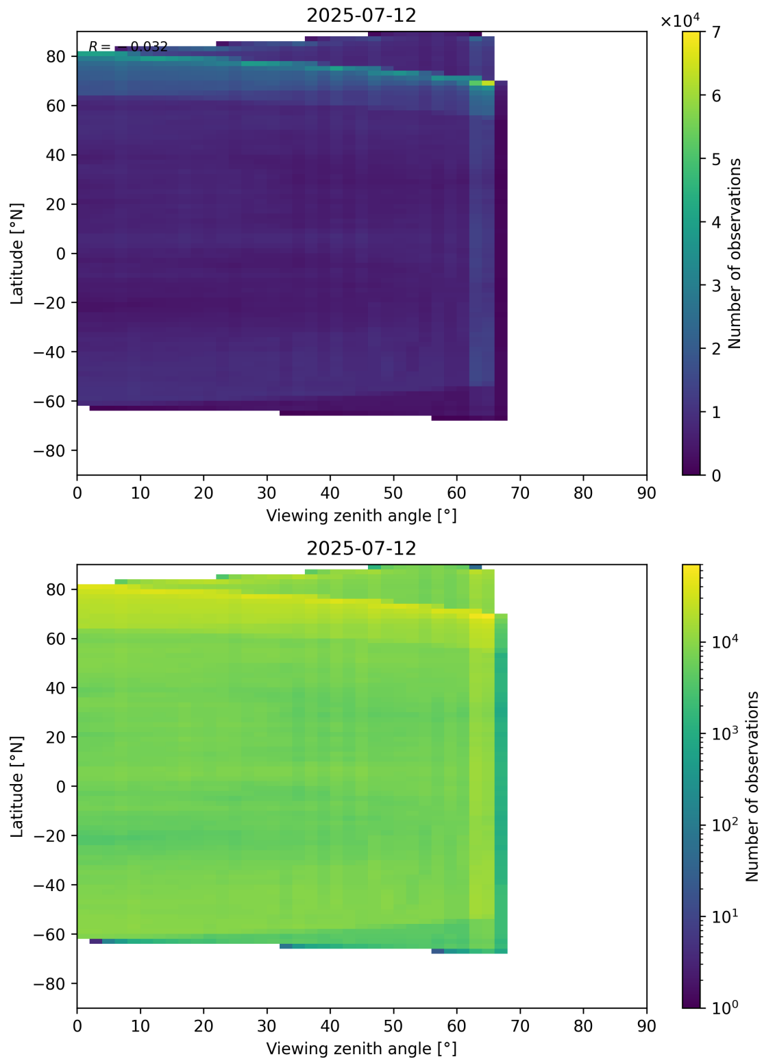
Figure 113: Scatter density plot of “Viewing zenith angle” against “Latitude” for 2025-07-11 to 2025-07-13.
