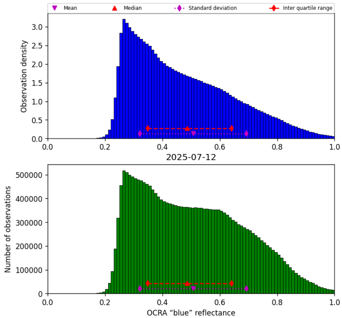
Figure 51: Histogram of “OCRA “blue” reflectance” for 2025-07-11 to 2025-07-13
