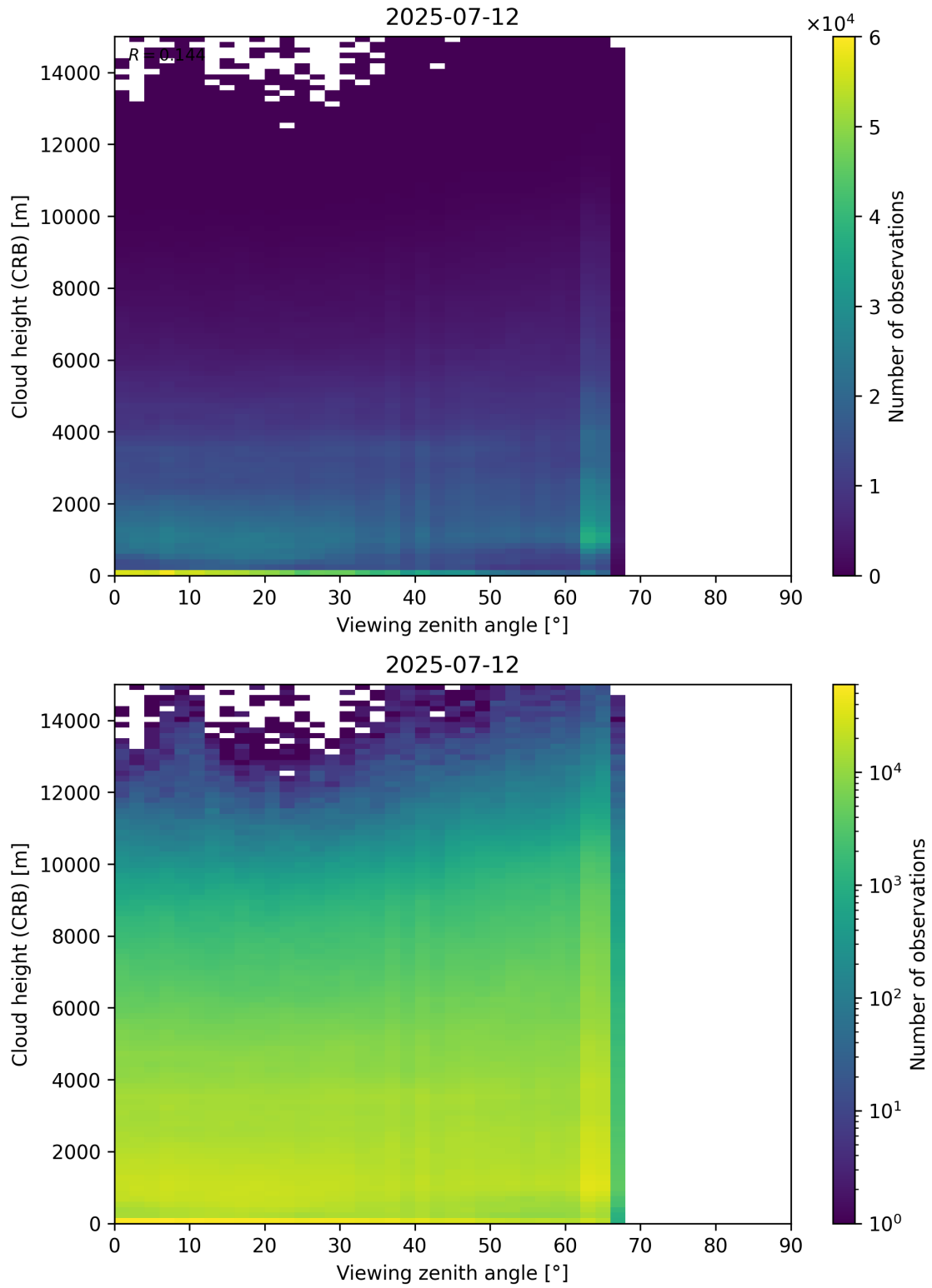
Figure 110: Scatter density plot of “Viewing zenith angle” against “Cloud height (CRB)” for 2025-07-11 to 2025-07-13.
