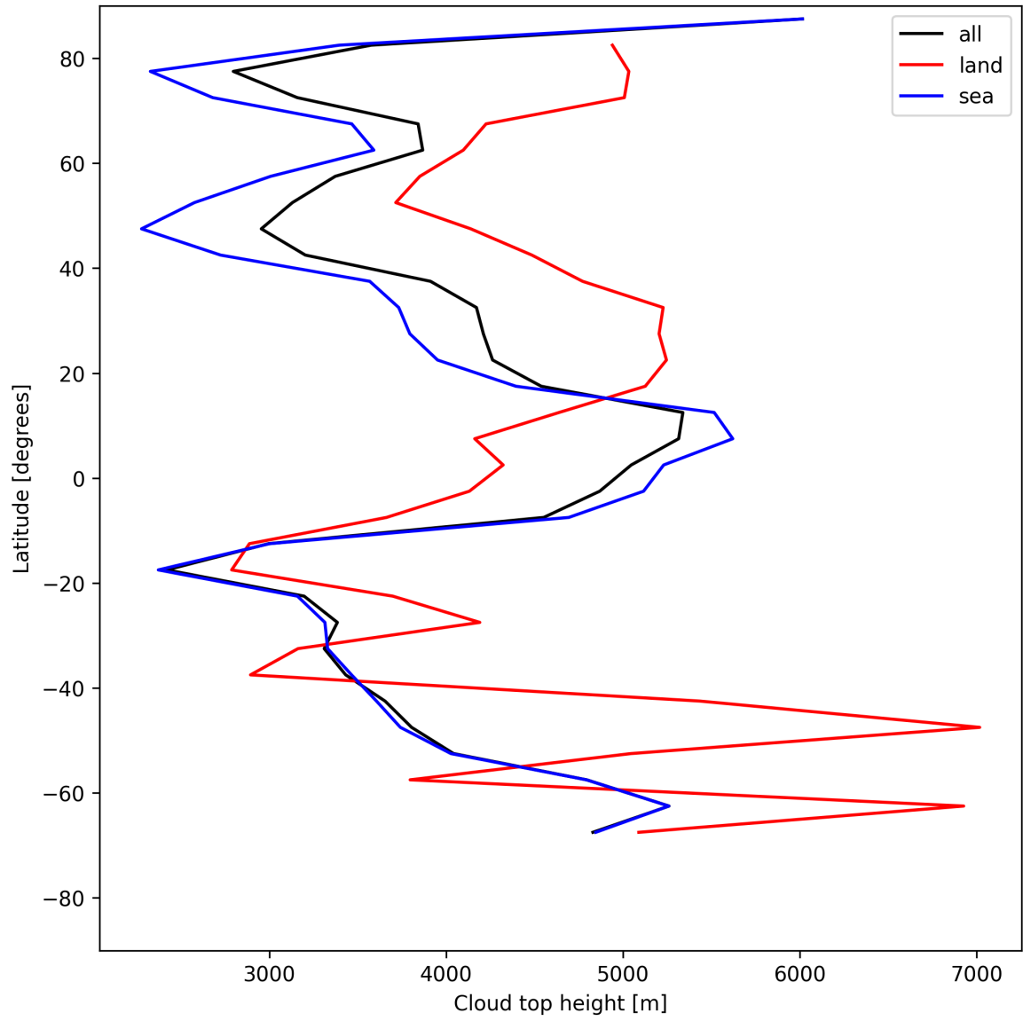
Figure 24: Zonal average of “Cloud top height” for 2025-07-11 to 2025-07-13.
