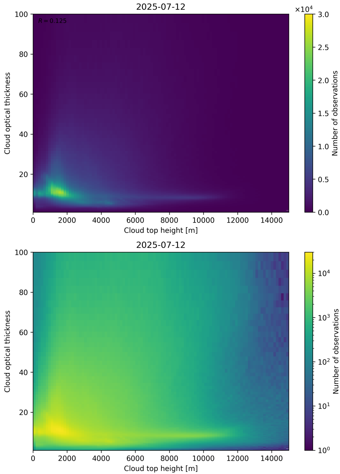
Figure 90: Scatter density plot of “Cloud top height” against “Cloud optical thickness” for 2025-07-11 to 2025-07-13.
