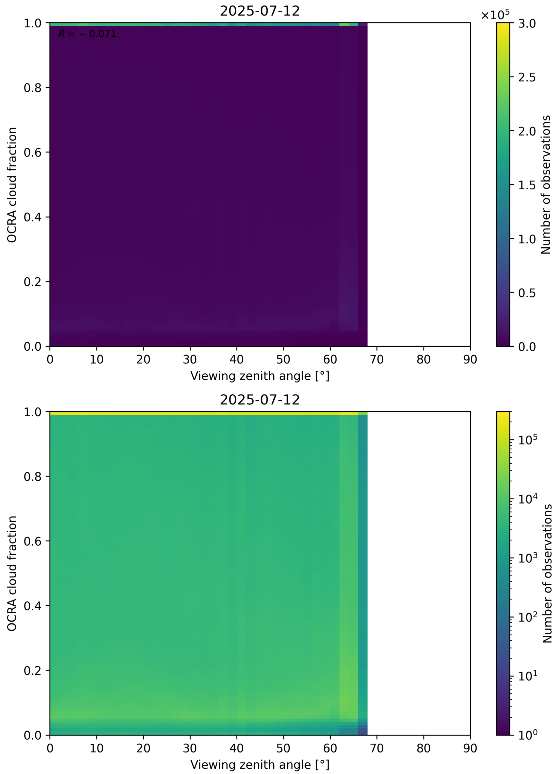
Figure 108: Scatter density plot of “Viewing zenith angle” against “OCRA cloud fraction” for 2025-07-11 to 2025-07-13.
