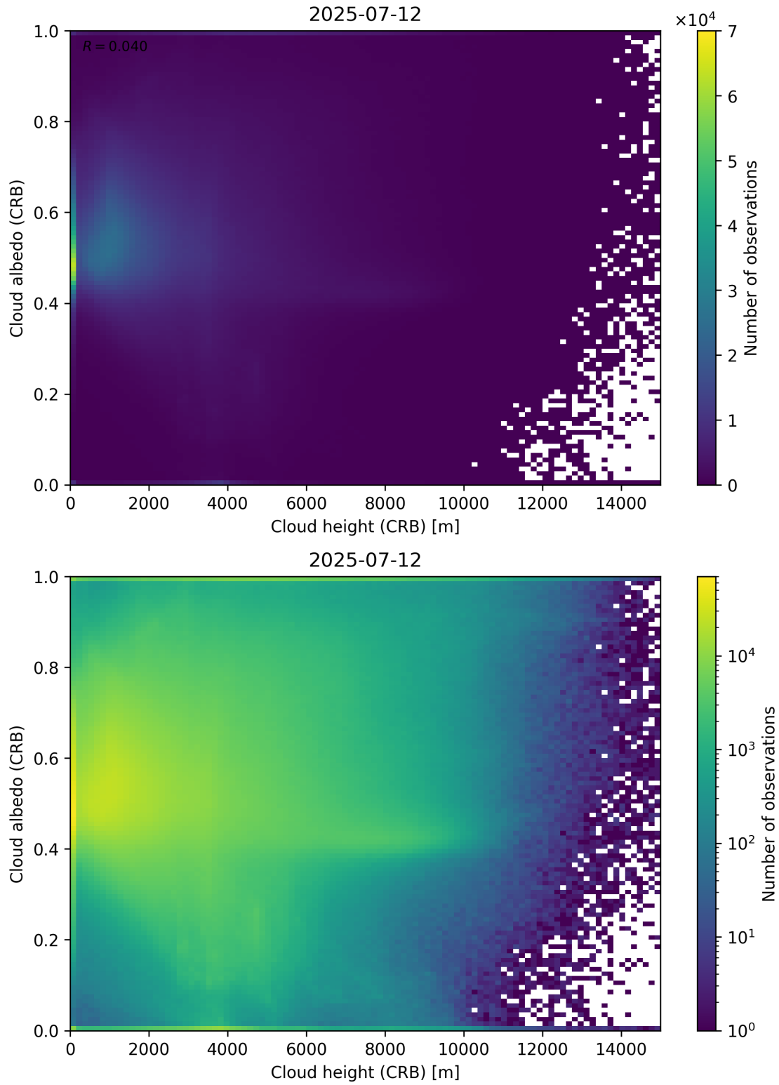
Figure 80: Scatter density plot of “Cloud height (CRB)” against “Cloud albedo (CRB)” for 2025-07-11 to 2025-07-13.
