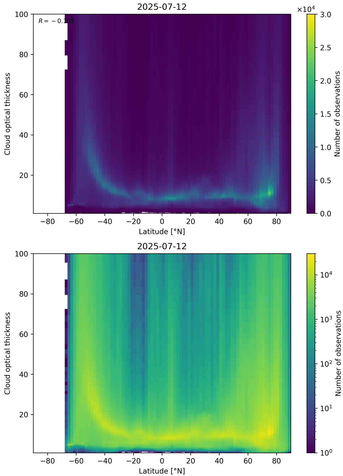
Figure 96: Scatter density plot of “Latitude” against “Cloud optical thickness” for 2025-07-11 to 2025-07-13.
