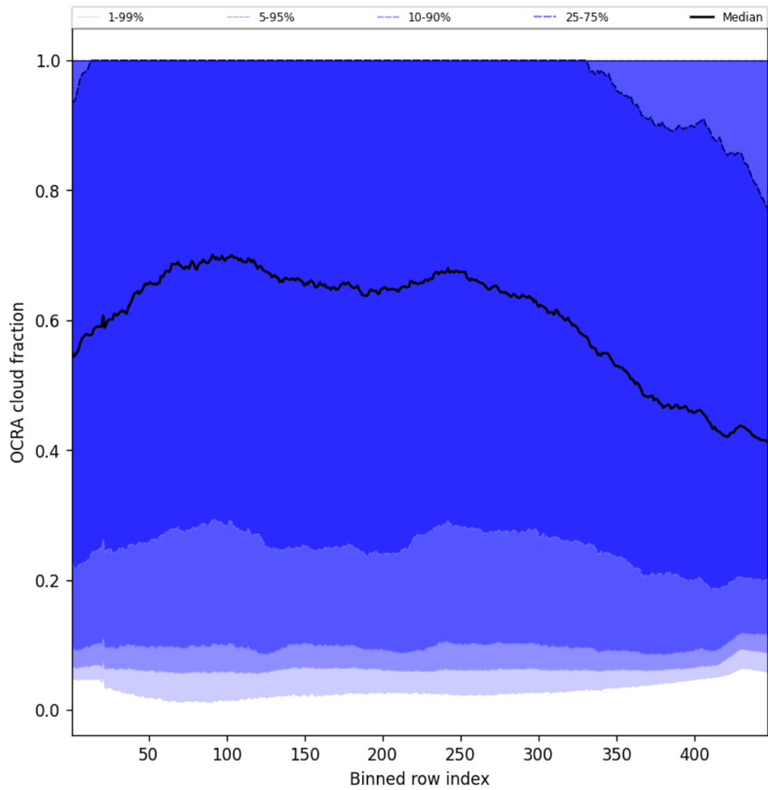
Figure 66: Along track statistics of “OCRA cloud fraction” for 2025-07-11 to 2025-07-13
