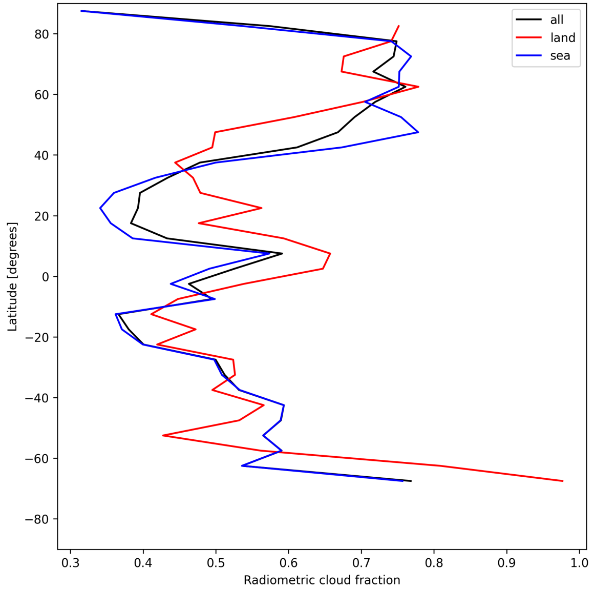
Figure 23: Zonal average of “Radiometric cloud fraction” for 2025-07-11 to 2025-07-13.
