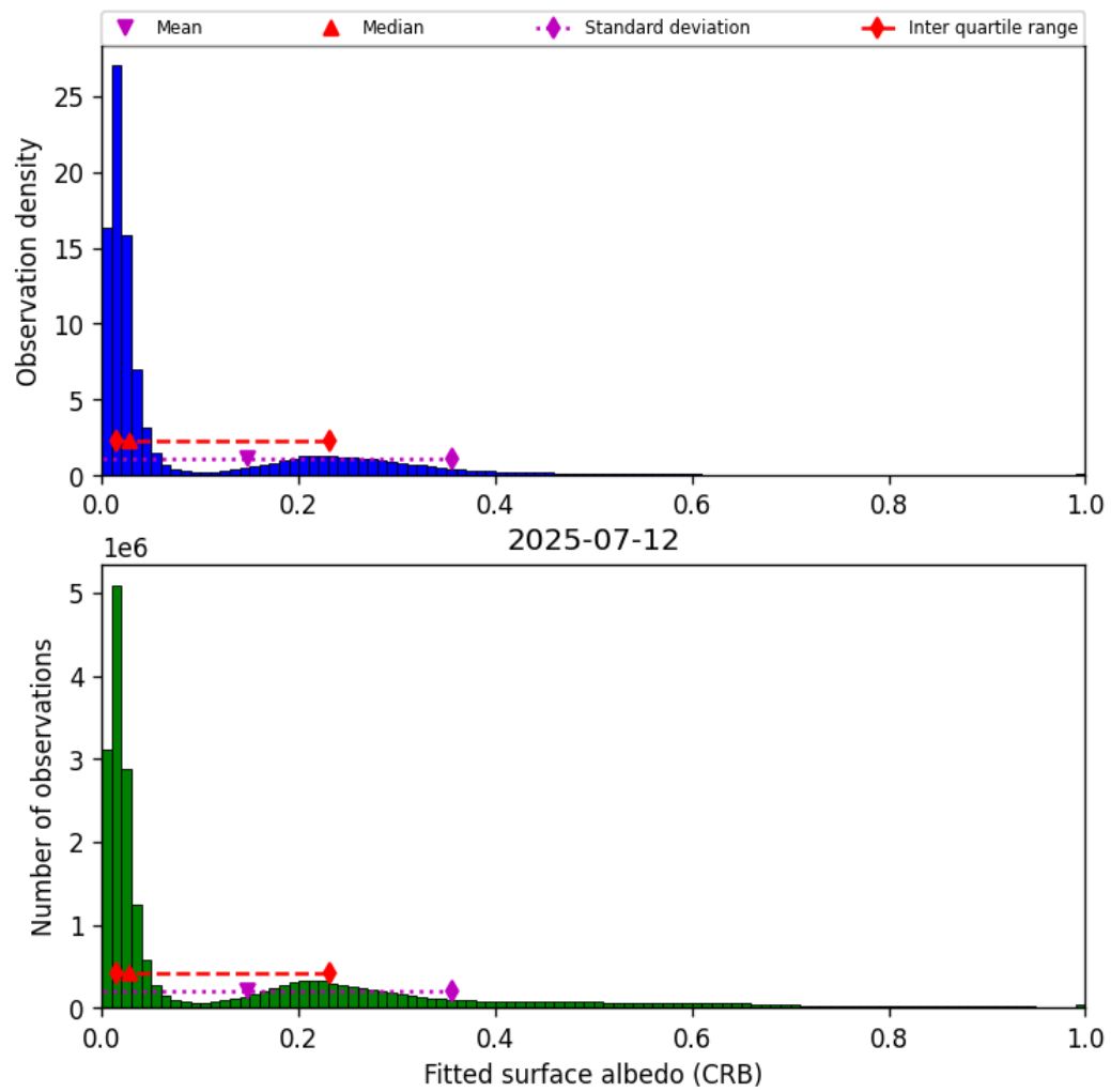
Figure 46: Histogram of "Fitted surface albedo (CRB)" for 2025-07-11 to 2025-07-13
