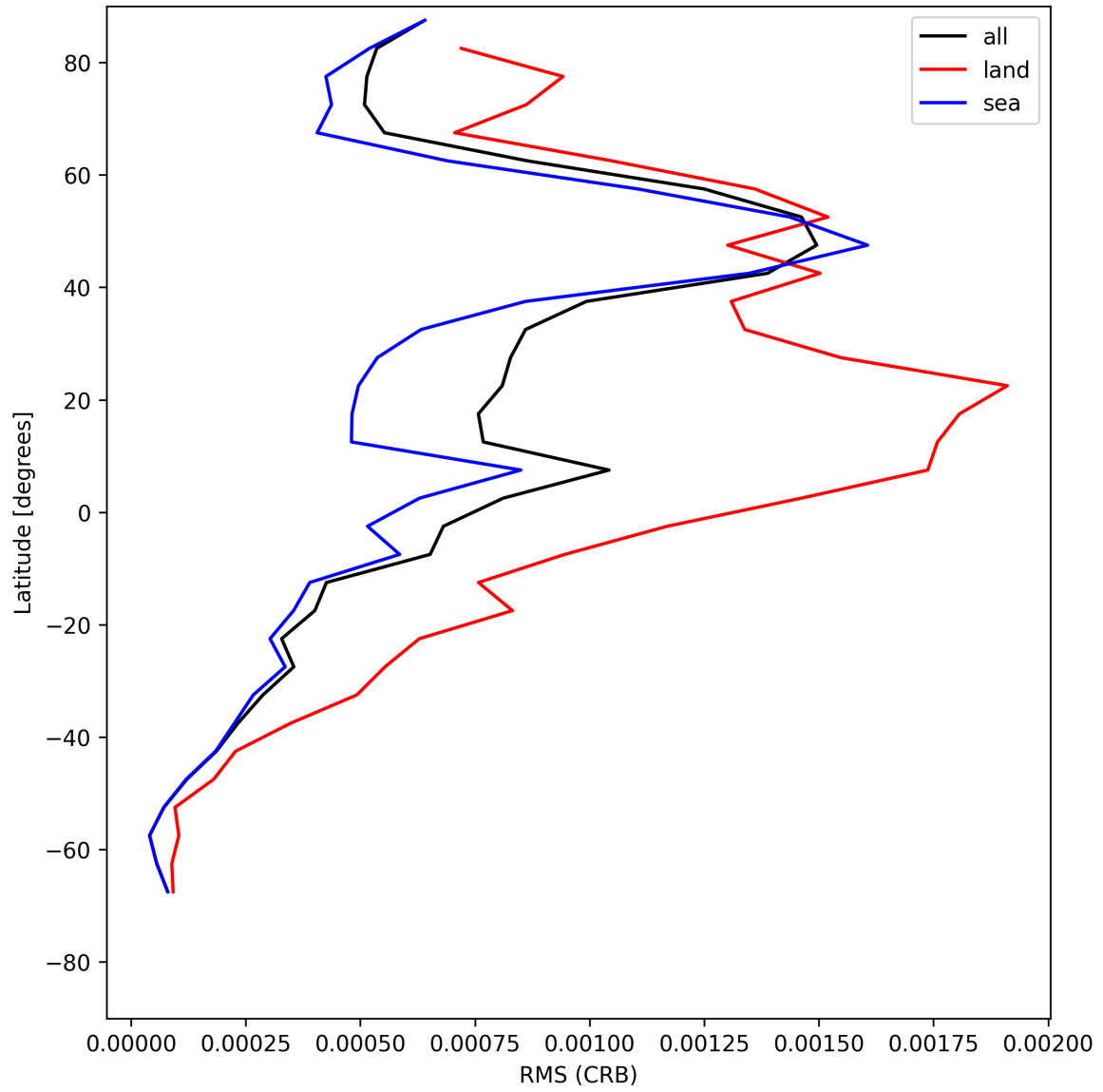
Figure 32: Zonal average of “RMS (CRB)” for 2025-07-11 to 2025-07-13.
