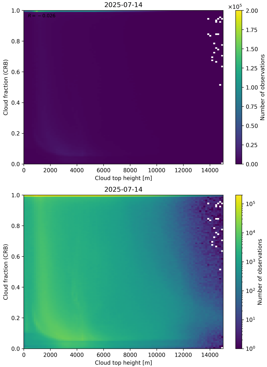
Figure 88: Scatter density plot of “Cloud top height” against “Cloud fraction (CRB)” for 2025-07-13 to 2025-07-15.
