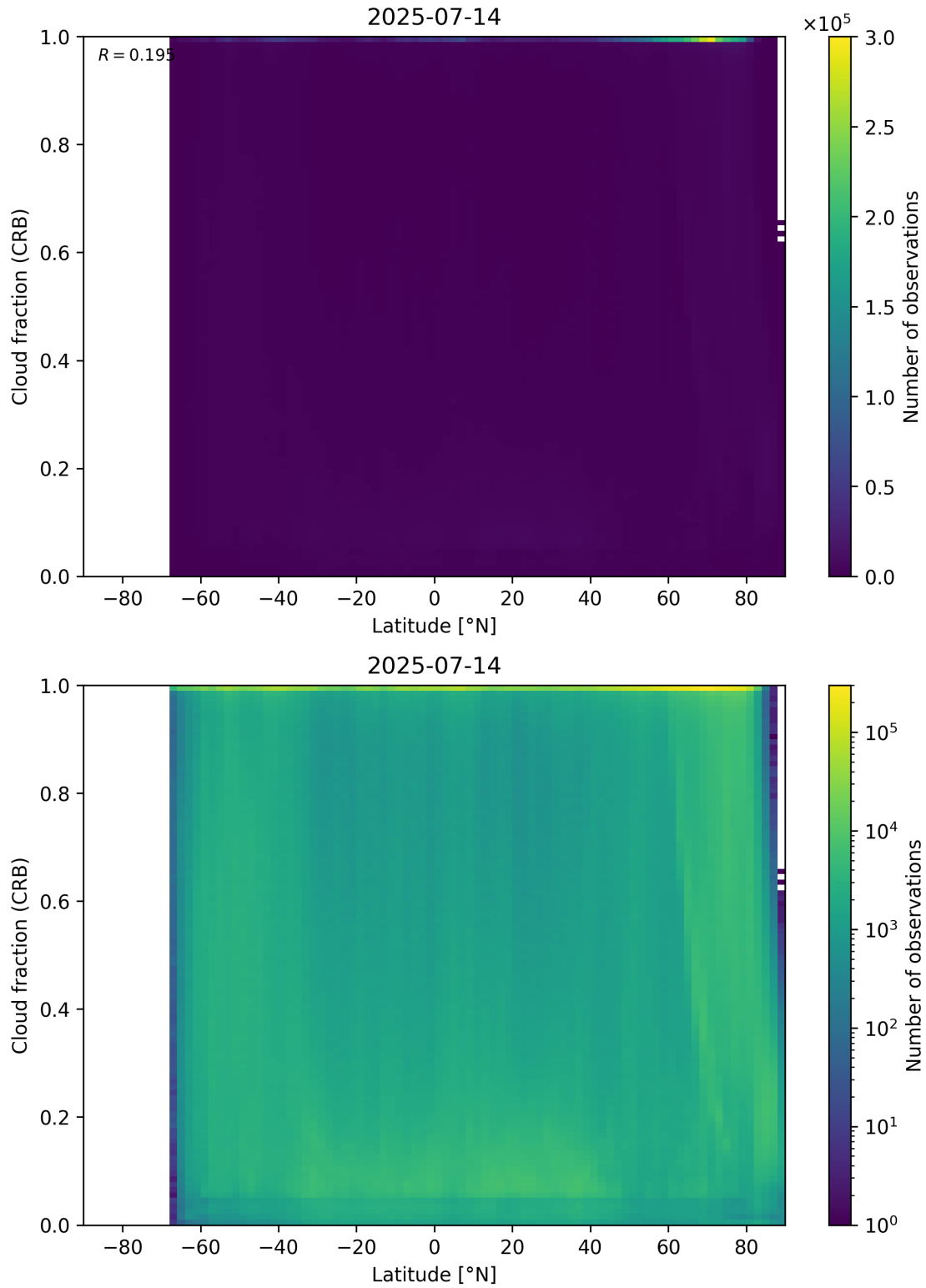
Figure 94: Scatter density plot of “Latitude” against “Cloud fraction (CRB)” for 2025-07-13 to 2025-07-15.
