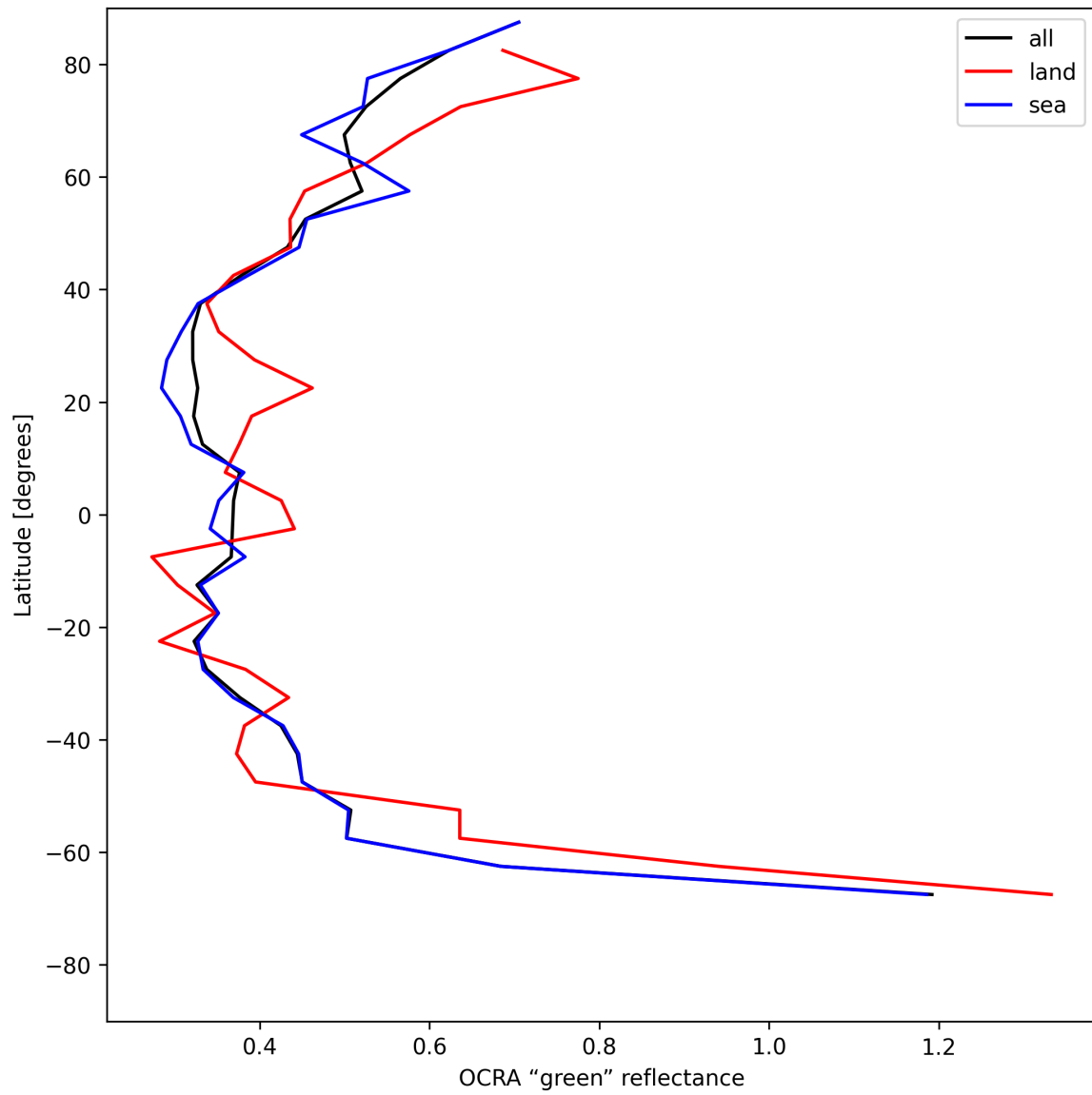
Figure 36: Zonal average of “OCRA “green” reflectance” for 2025-07-13 to 2025-07-15.
