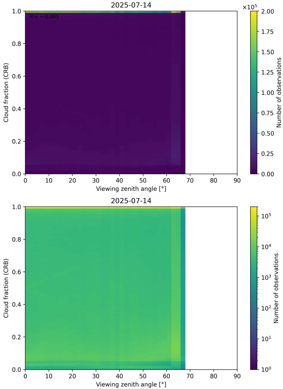
Figure 109: Scatter density plot of “Viewing zenith angle” against “Cloud fraction (CRB)” for 2025-07-13 to 2025-07-15.
