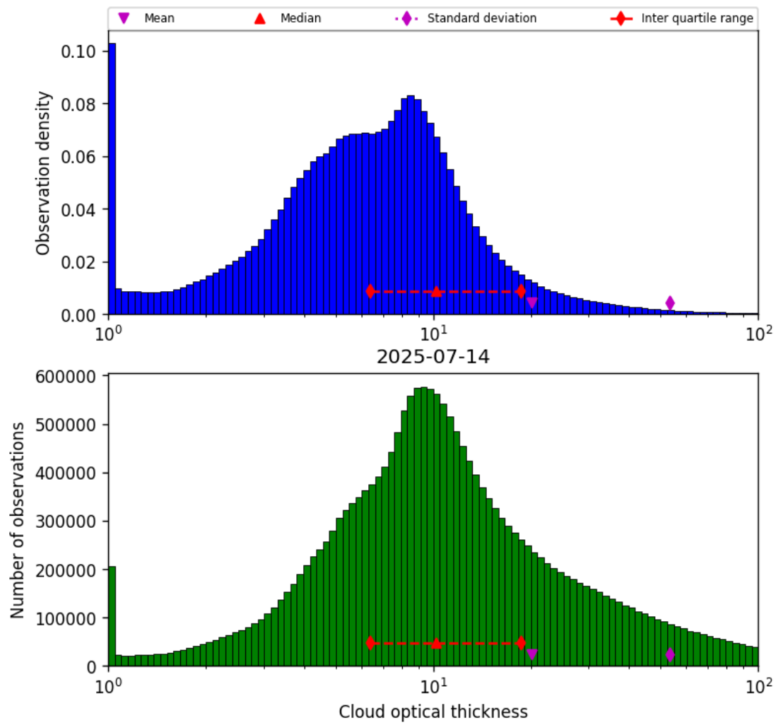
Figure 41: Histogram of “Cloud optical thickness” for 2025-07-13 to 2025-07-15
