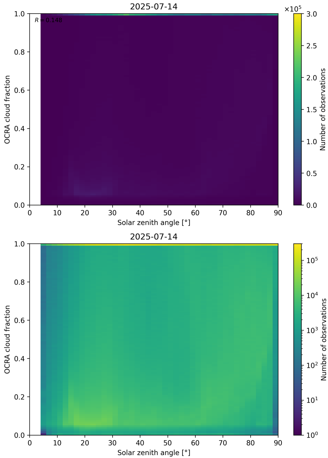
Figure 100: Scatter density plot of “Solar zenith angle” against “OCRA cloud fraction” for 2025-07-13 to 2025-07-15.
