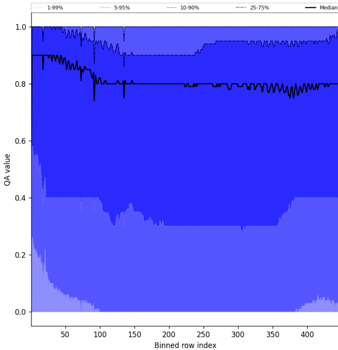
Figure 54: Along track statistics of “QA value” for 2025-07-13 to 2025-07-15
