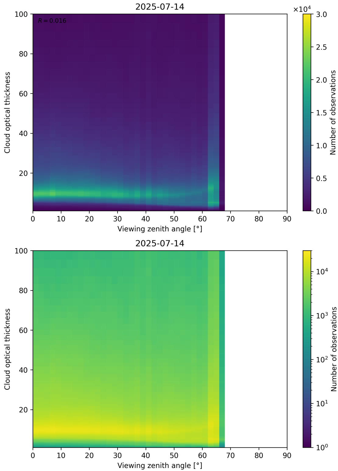
Figure 111: Scatter density plot of “Viewing zenith angle” against “Cloud optical thickness” for 2025-07-13 to 2025-07-15.
