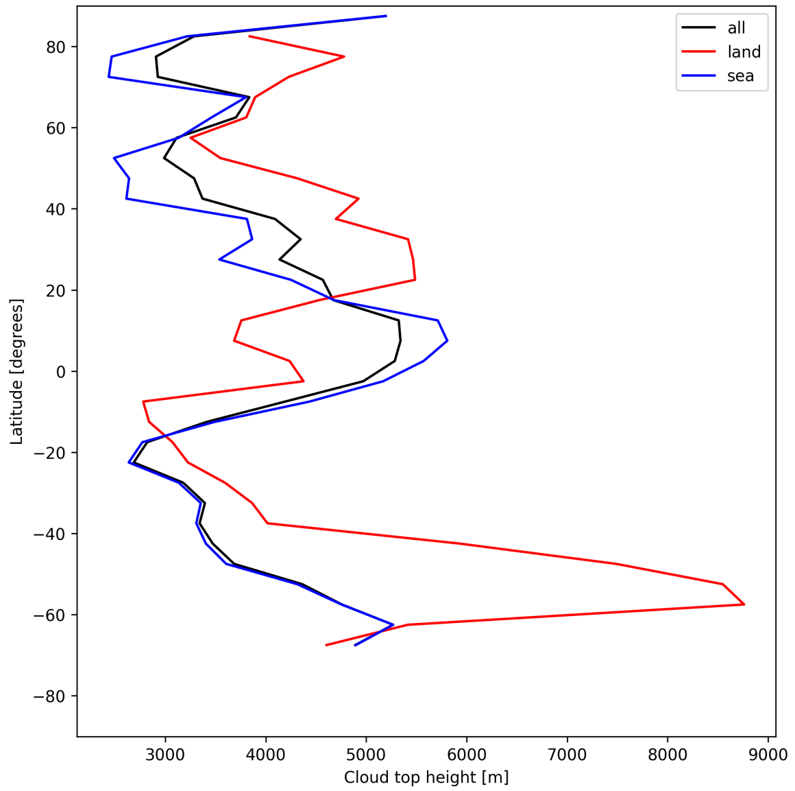
Figure 24: Zonal average of “Cloud top height” for 2025-07-13 to 2025-07-15.
