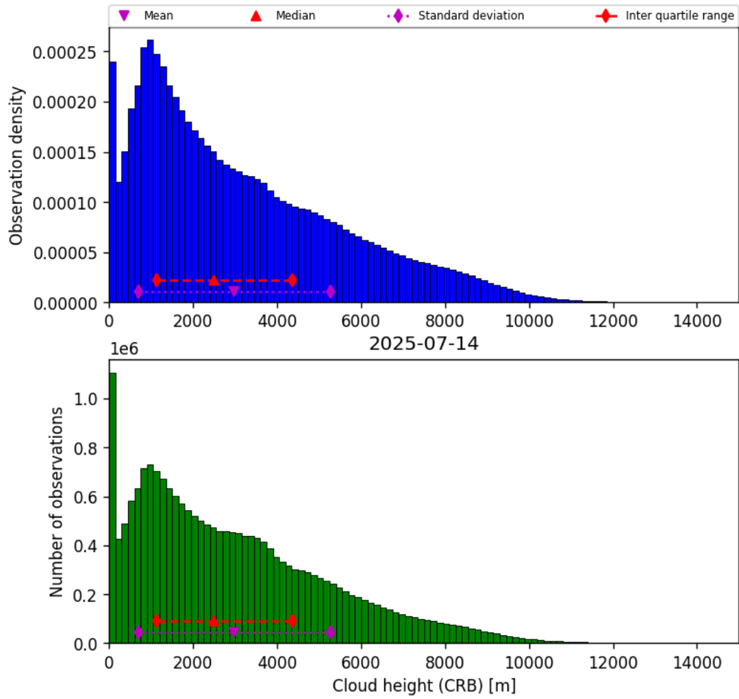
Figure 43: Histogram of “Cloud height (CRB)” for 2025-07-13 to 2025-07-15
