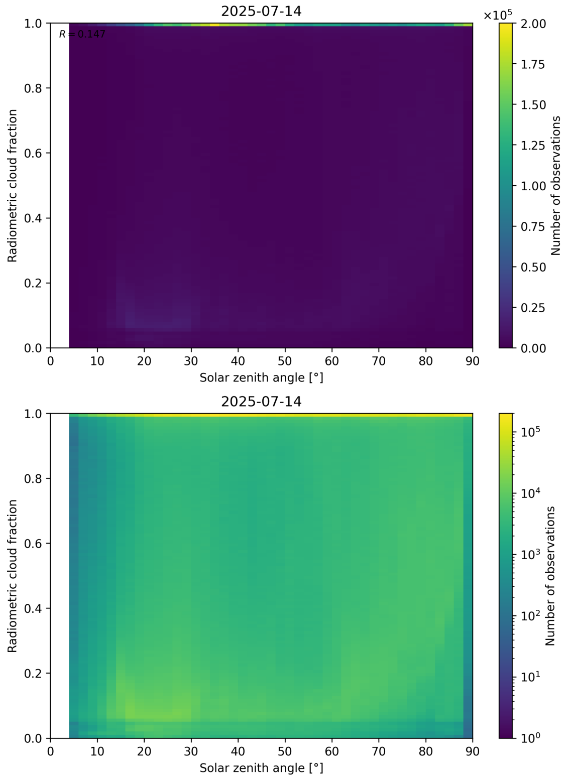
Figure 99: Scatter density plot of “Solar zenith angle” against “Radiometric cloud fraction” for 2025-07-13 to 2025-07-15.
