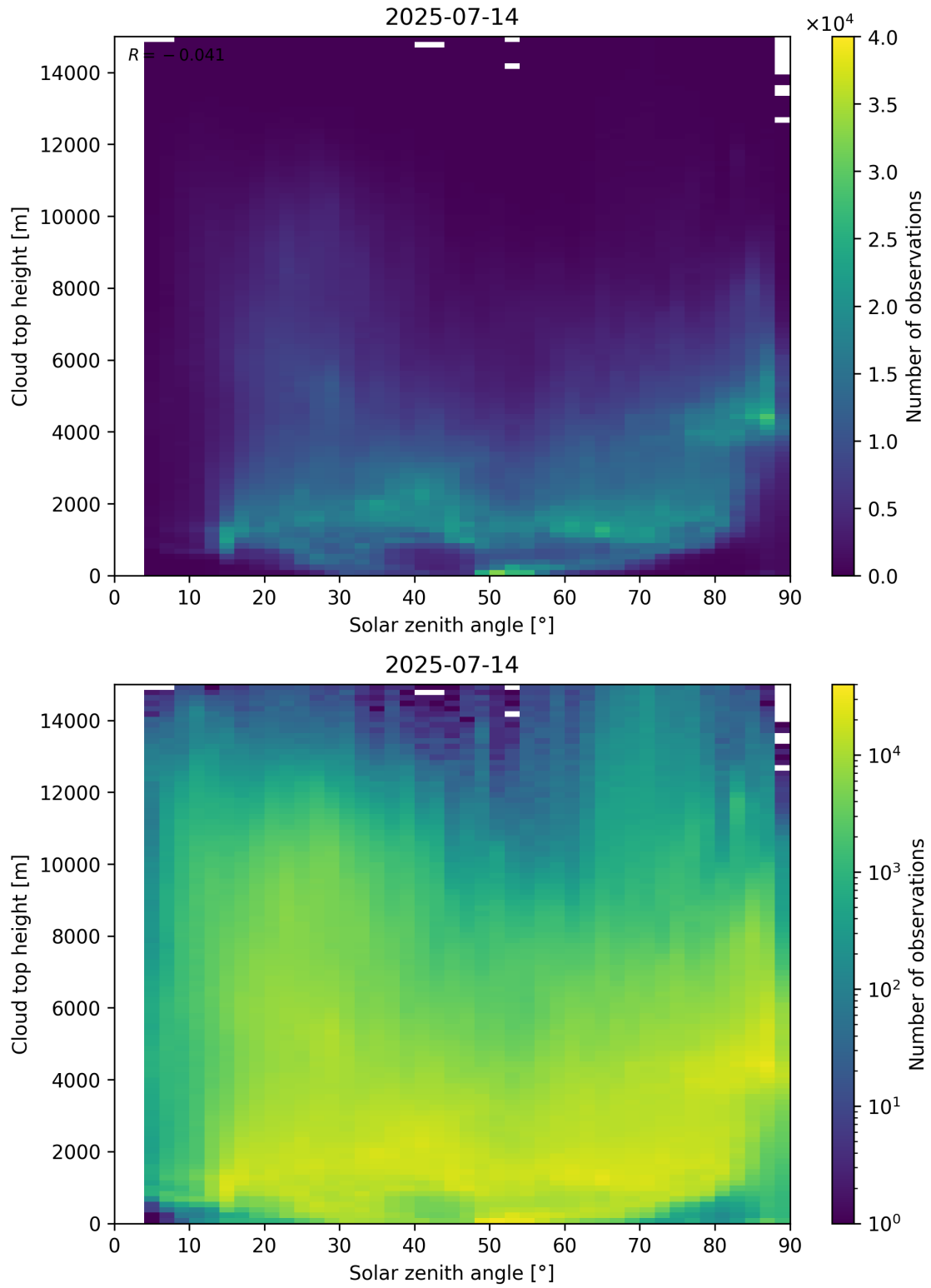
Figure 104: Scatter density plot of “Solar zenith angle” against “Cloud top height” for 2025-07-13 to 2025-07-15.
