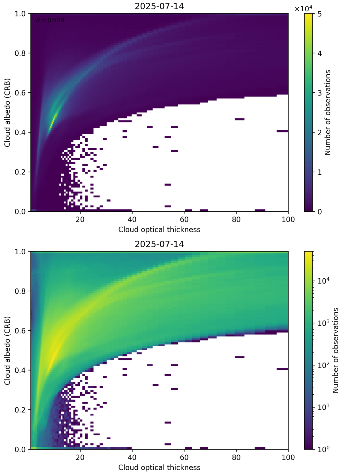
Figure 82: Scatter density plot of “Cloud optical thickness” against “Cloud albedo (CRB)” for 2025-07-13 to 2025-07-15.
