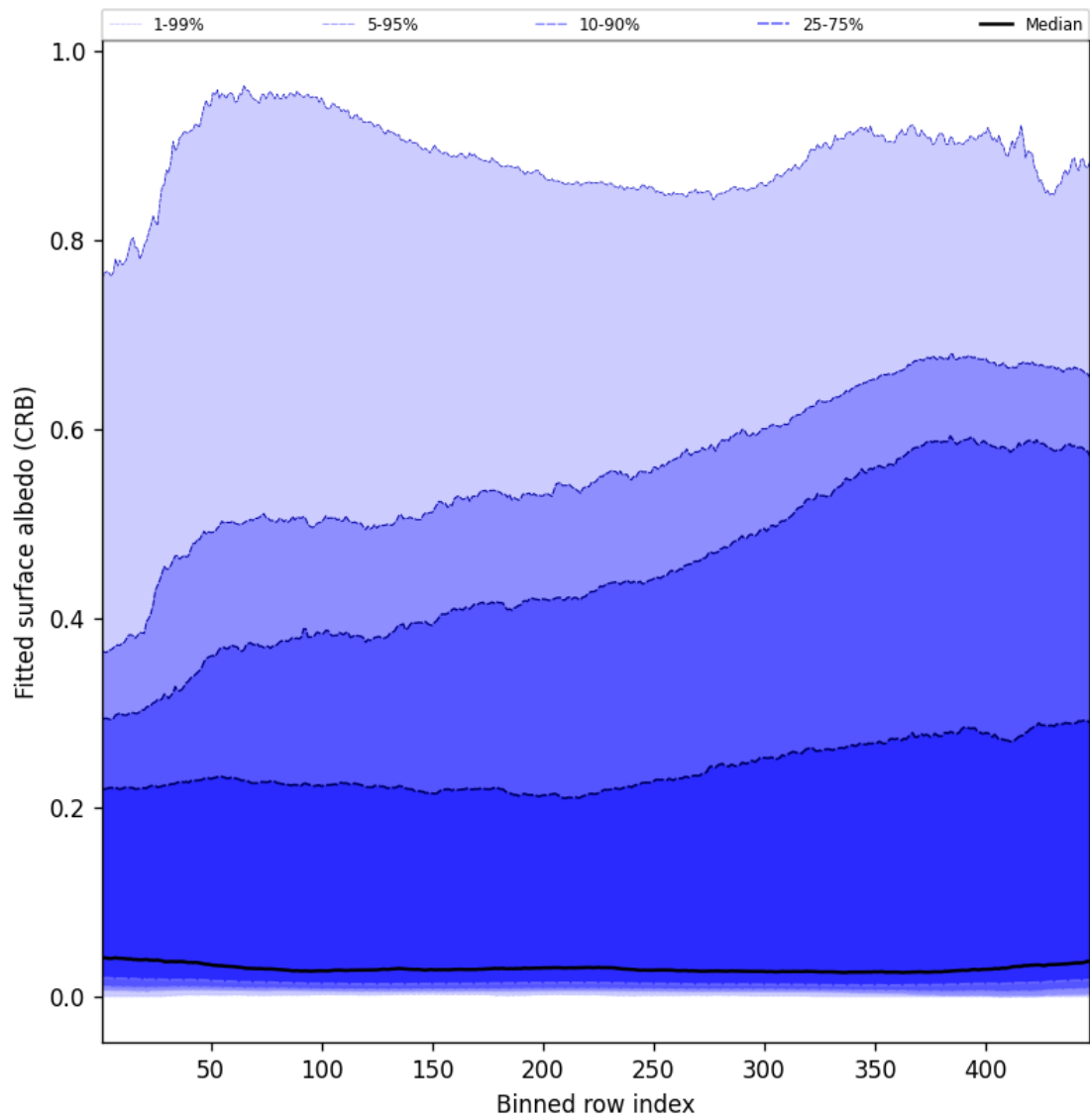
Figure 62: Along track statistics of “Fitted surface albedo (CRB)” for 2025-07-13 to 2025-07-15
