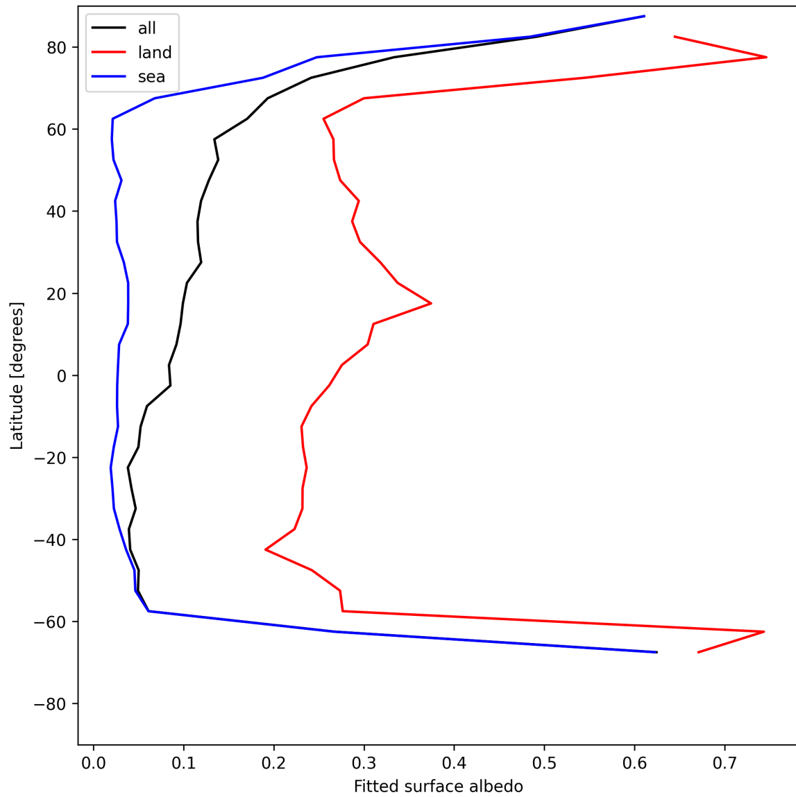
Figure 29: Zonal average of “Fitted surface albedo” for 2025-07-13 to 2025-07-15.
