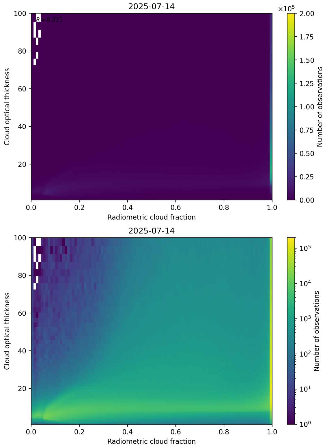
Figure 75: Scatter density plot of “Radiometric cloud fraction” against “Cloud optical thickness” for 2025-07-13 to 2025-07-15.
