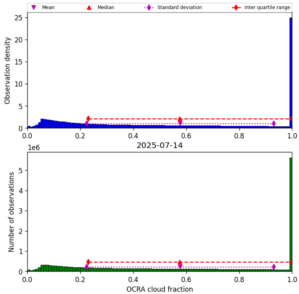
Figure 50: Histogram of “OCRA cloud fraction” for 2025-07-13 to 2025-07-15
