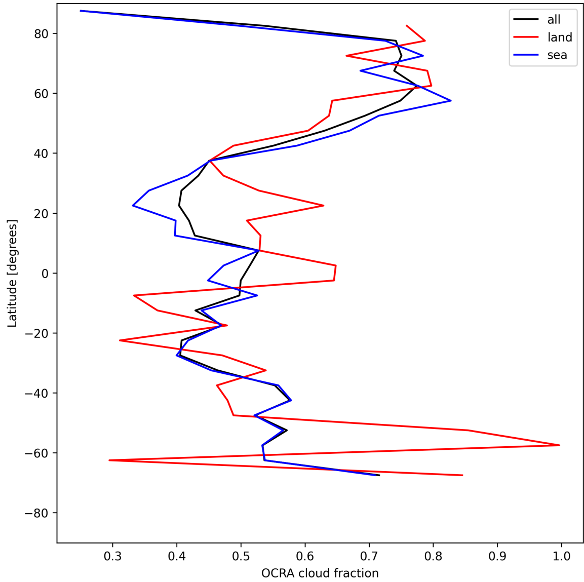
Figure 34: Zonal average of “OCRA cloud fraction” for 2025-07-13 to 2025-07-15.
