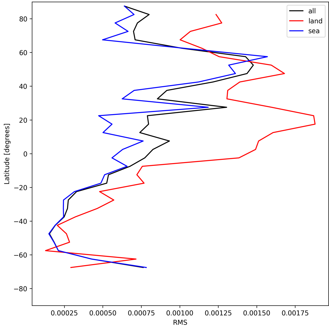
Figure 31: Zonal average of “RMS” for 2025-07-13 to 2025-07-15.
