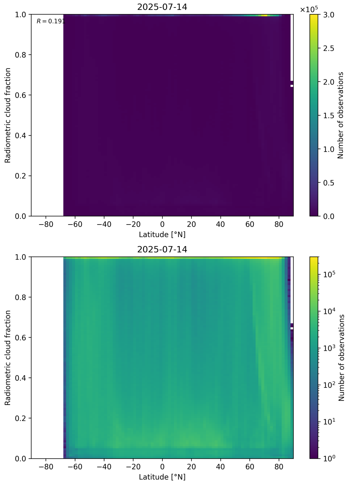
Figure 92: Scatter density plot of “Latitude” against “Radiometric cloud fraction” for 2025-07-13 to 2025-07-15.
