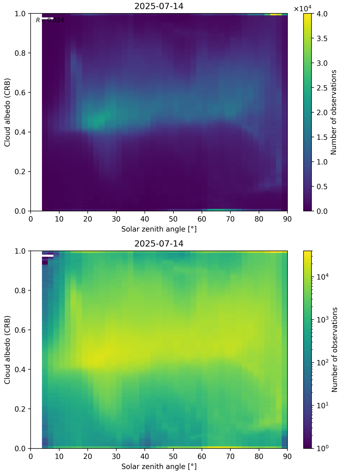
Figure 98: Scatter density plot of “Solar zenith angle” against “Cloud albedo (CRB)” for 2025-07-13 to 2025-07-15.
