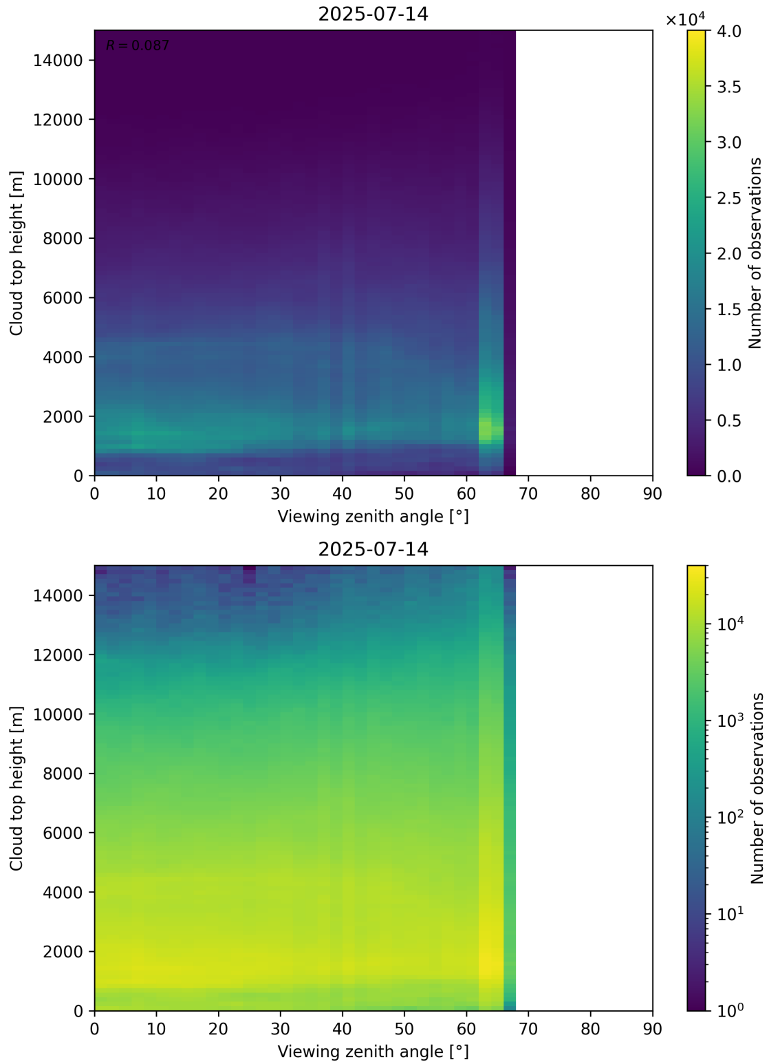
Figure 112: Scatter density plot of “Viewing zenith angle” against “Cloud top height” for 2025-07-13 to 2025-07-15.
