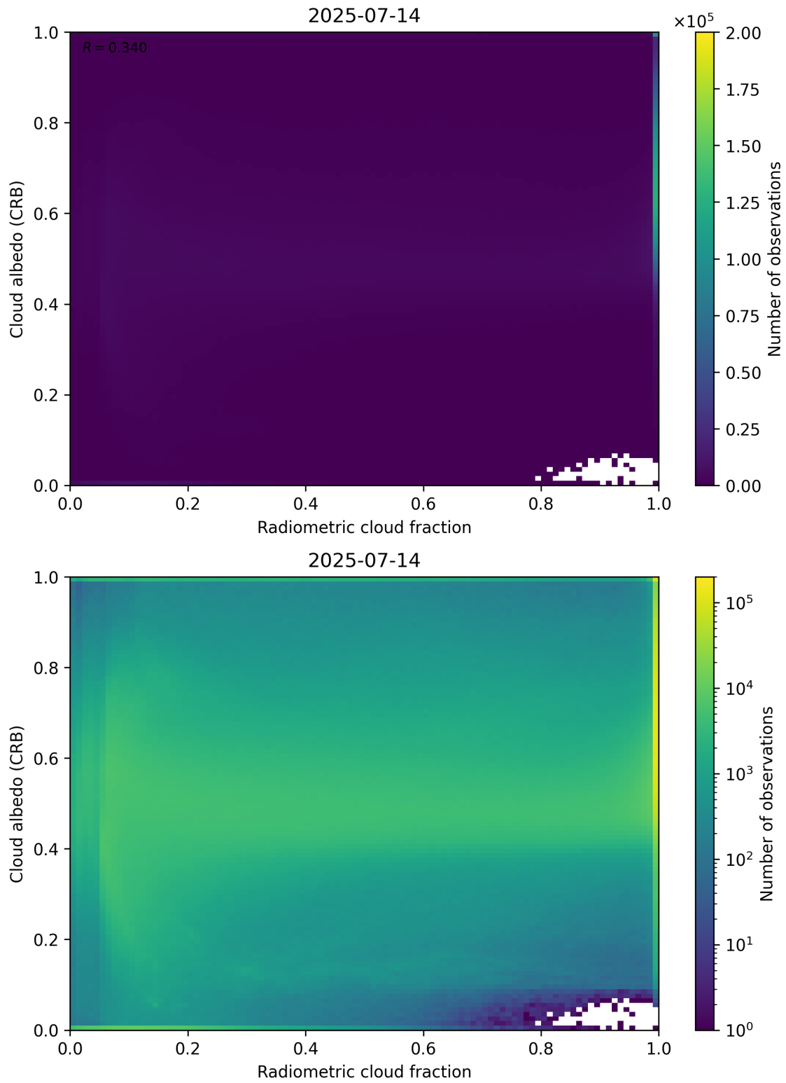
Figure 71: Scatter density plot of “Radiometric cloud fraction” against “Cloud albedo (CRB)” for 2025-07-13 to 2025-07-15.
