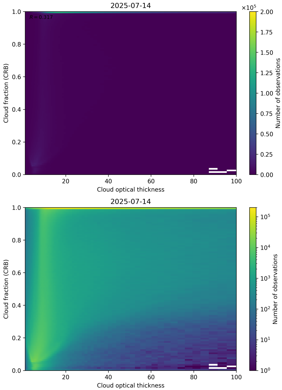
Figure 84: Scatter density plot of “Cloud optical thickness” against “Cloud fraction (CRB)” for 2025-07-13 to 2025-07-15.
