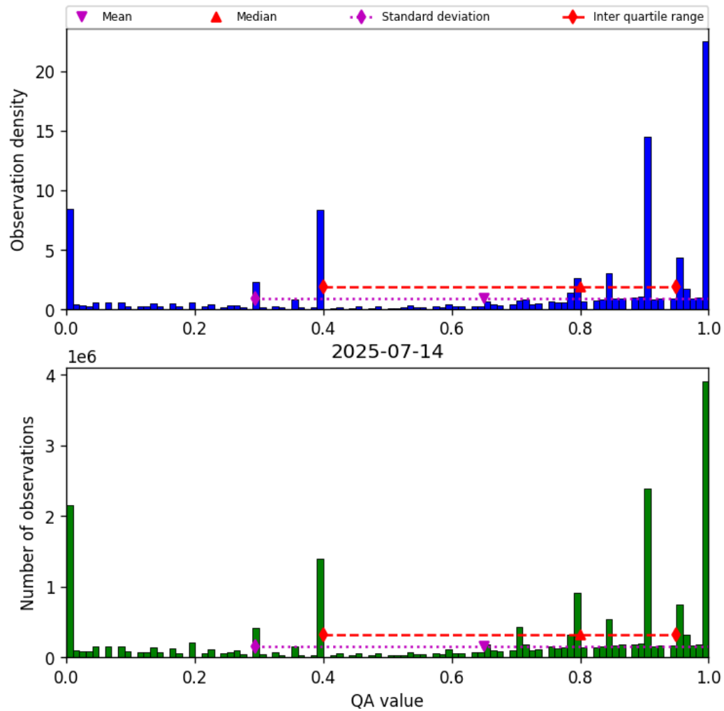
Figure 38: Histogram of “QA value” for 2025-07-13 to 2025-07-15
