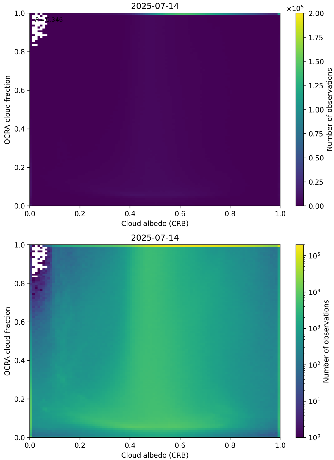
Figure 70: Scatter density plot of “Cloud albedo (CRB)” against “OCRA cloud fraction” for 2025-07-13 to 2025-07-15.
