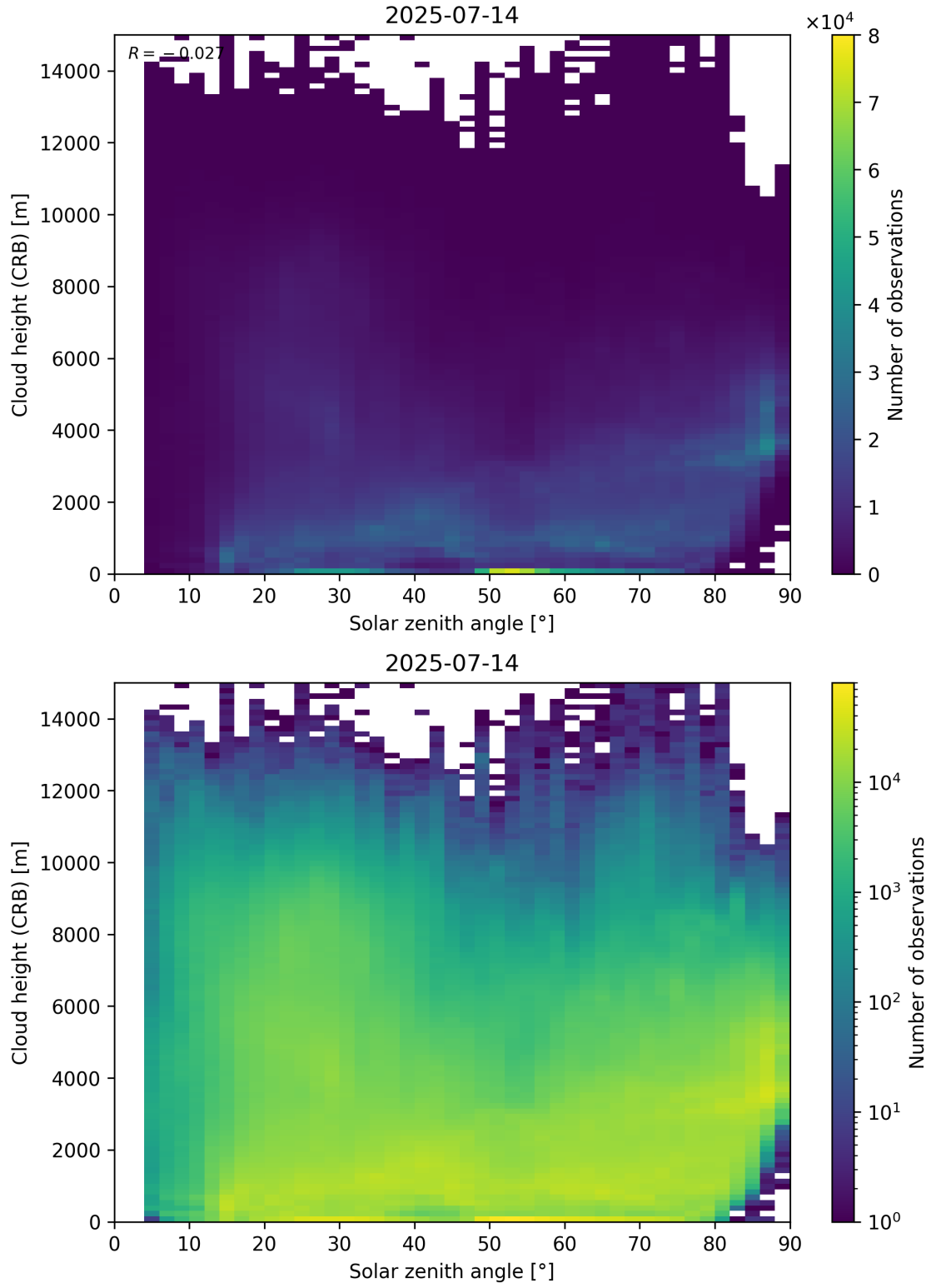
Figure 102: Scatter density plot of “Solar zenith angle” against “Cloud height (CRB)” for 2025-07-13 to 2025-07-15.
