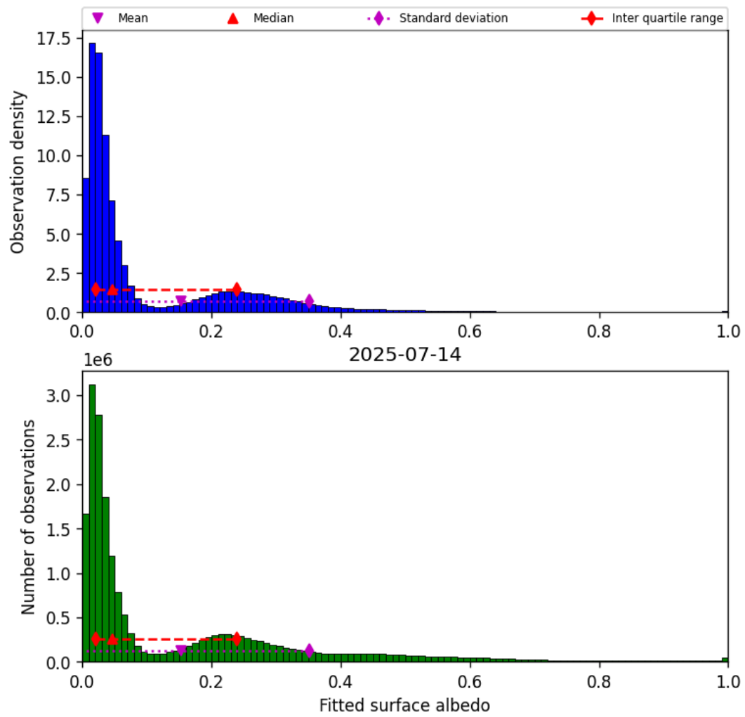
Figure 45: Histogram of “Fitted surface albedo” for 2025-07-13 to 2025-07-15
