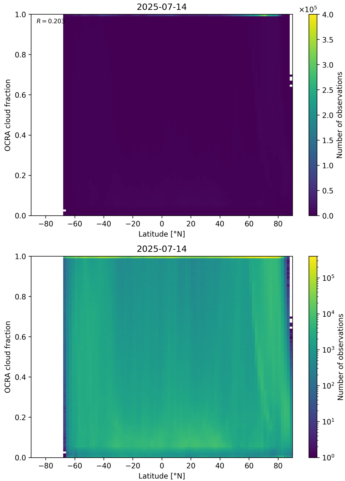
Figure 93: Scatter density plot of “Latitude” against “OCRA cloud fraction” for 2025-07-13 to 2025-07-15.
