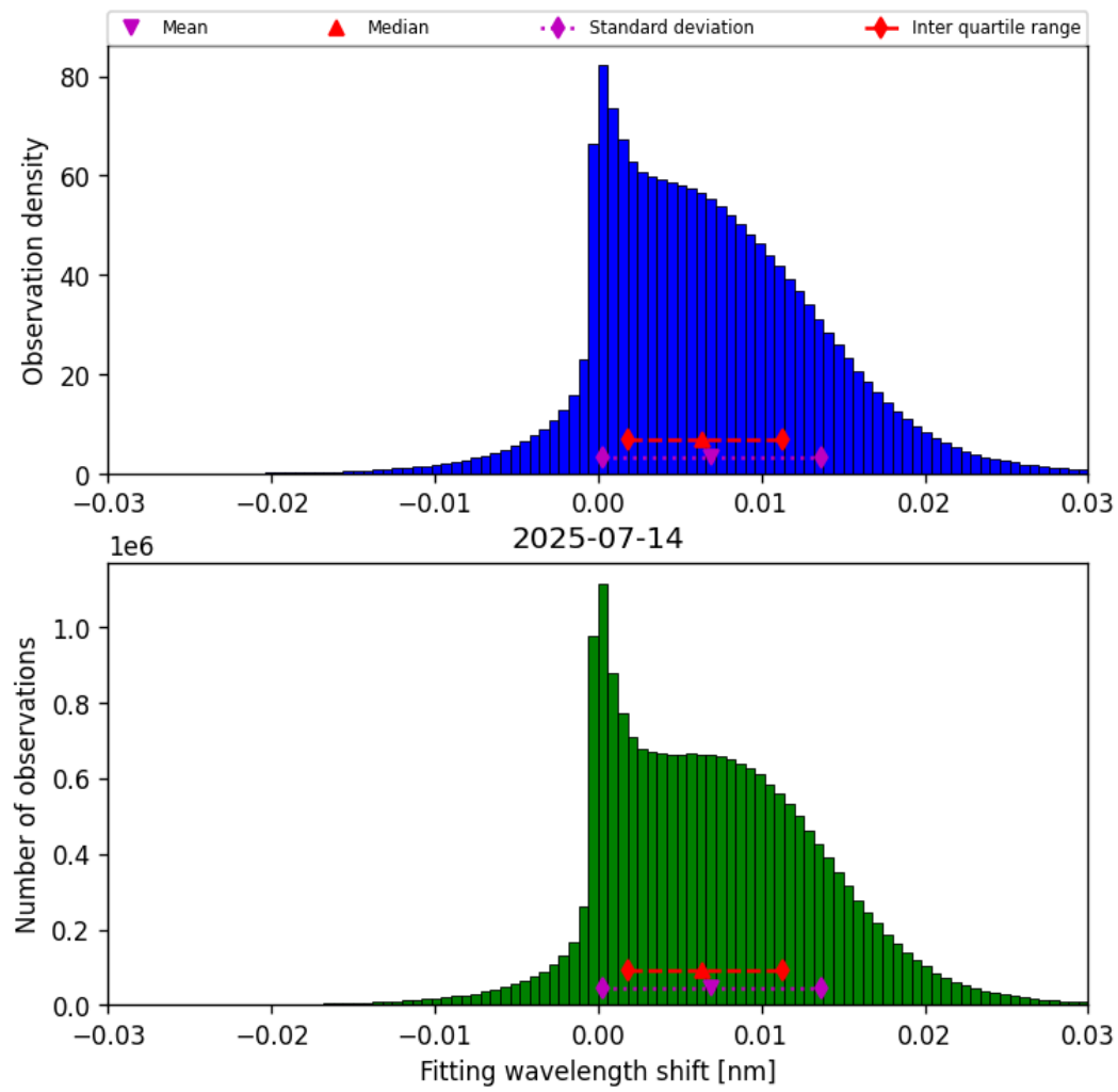
Figure 49: Histogram of “Fitting wavelength shift” for 2025-07-13 to 2025-07-15
