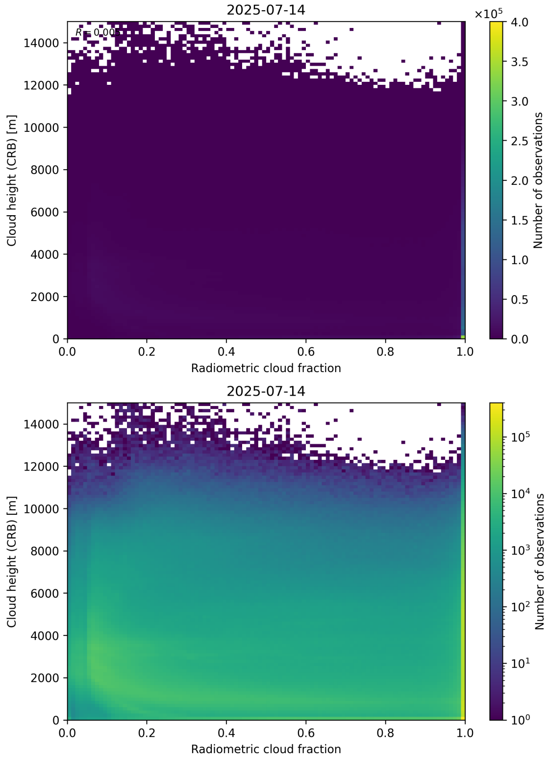
Figure 74: Scatter density plot of “Radiometric cloud fraction” against “Cloud height (CRB)” for 2025-07-13 to 2025-07-15.
