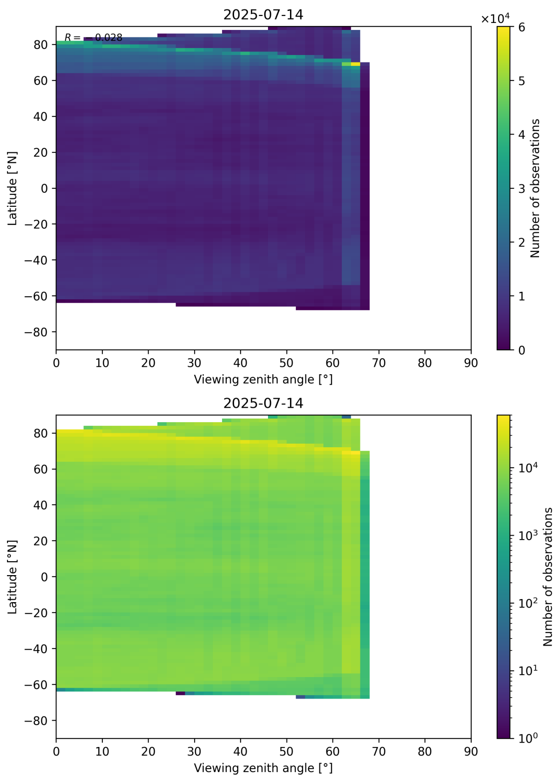
Figure 113: Scatter density plot of “Viewing zenith angle” against “Latitude” for 2025-07-13 to 2025-07-15.
