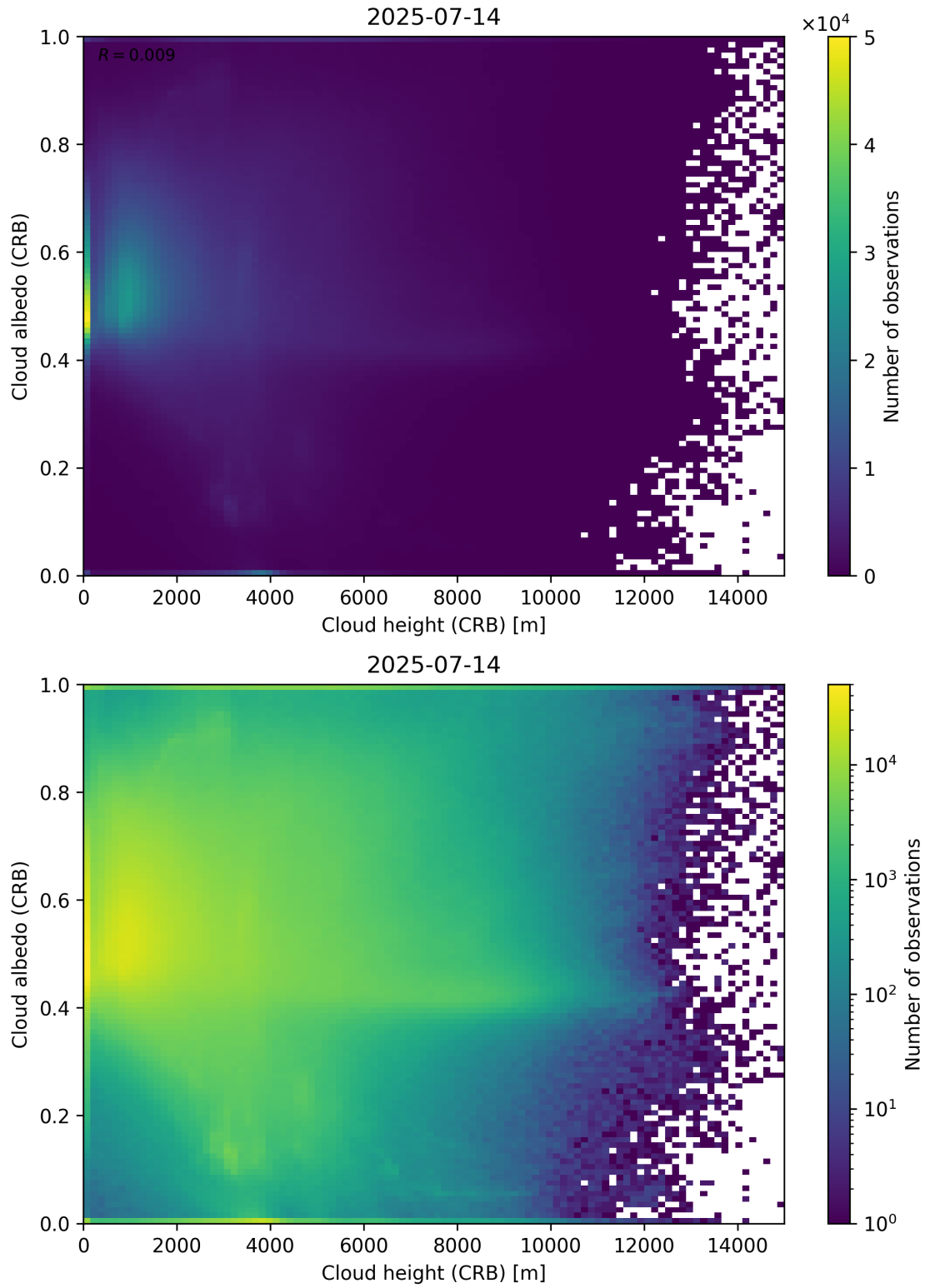
Figure 80: Scatter density plot of “Cloud height (CRB)” against “Cloud albedo (CRB)” for 2025-07-13 to 2025-07-15.
