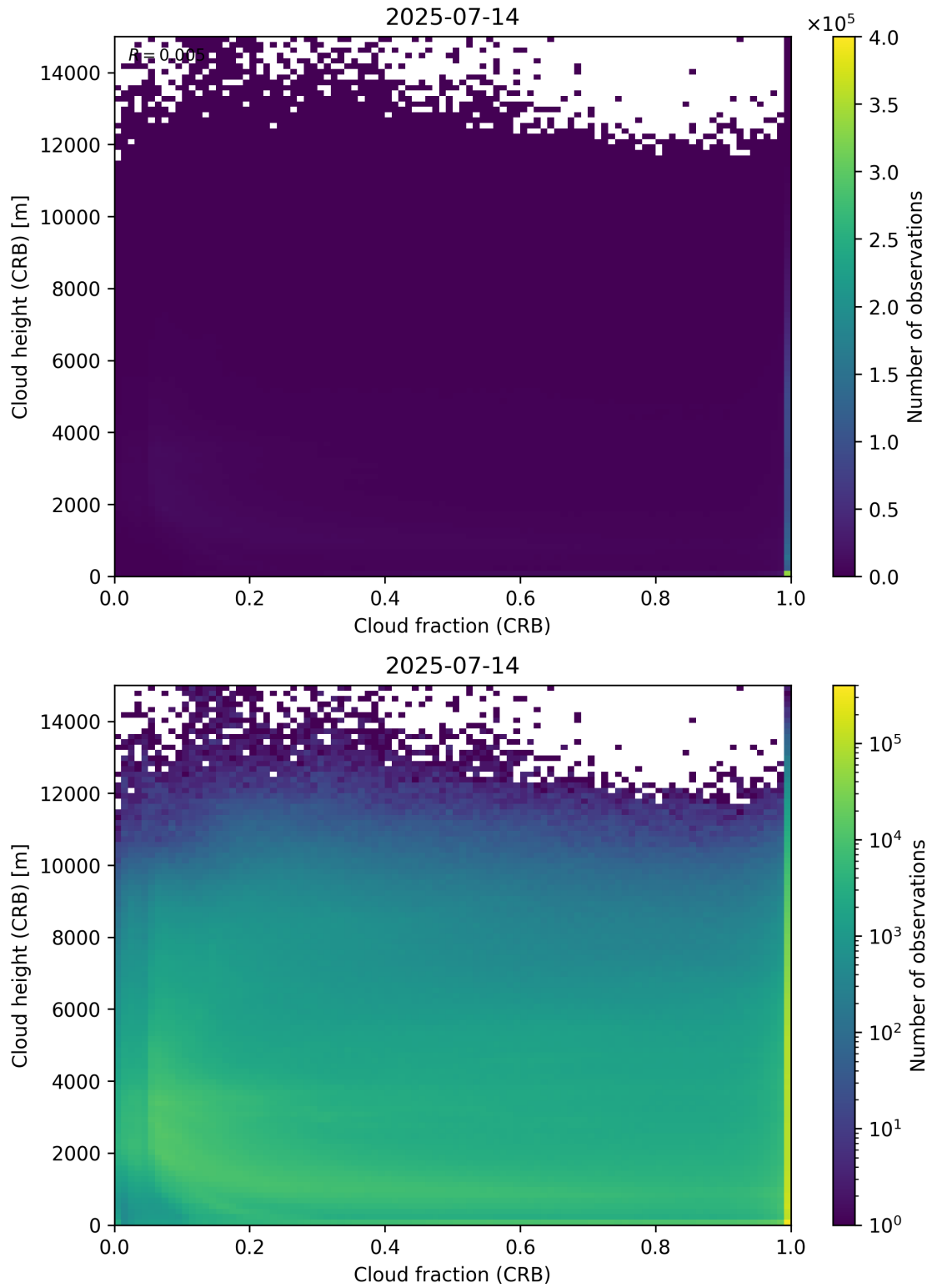
Figure 79: Scatter density plot of “Cloud fraction (CRB)” against “Cloud height (CRB)” for 2025-07-13 to 2025-07-15.
