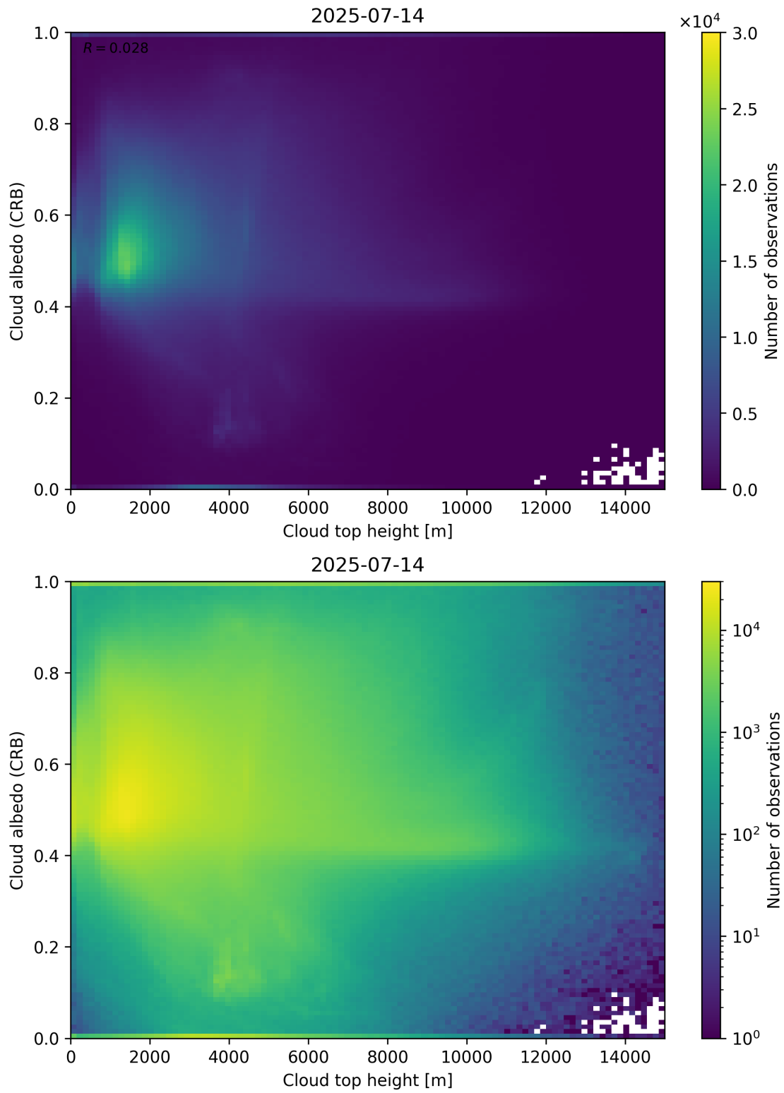
Figure 86: Scatter density plot of “Cloud top height” against “Cloud albedo (CRB)” for 2025-07-13 to 2025-07-15.
