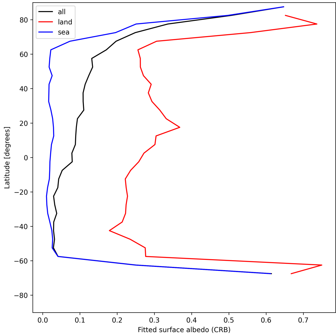
Figure 30: Zonal average of “Fitted surface albedo (CRB)” for 2025-07-13 to 2025-07-15.
