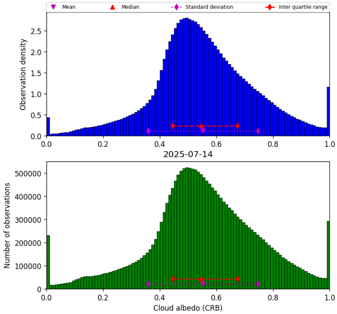
Figure 44: Histogram of “Cloud albedo (CRB)” for 2025-07-13 to 2025-07-15
