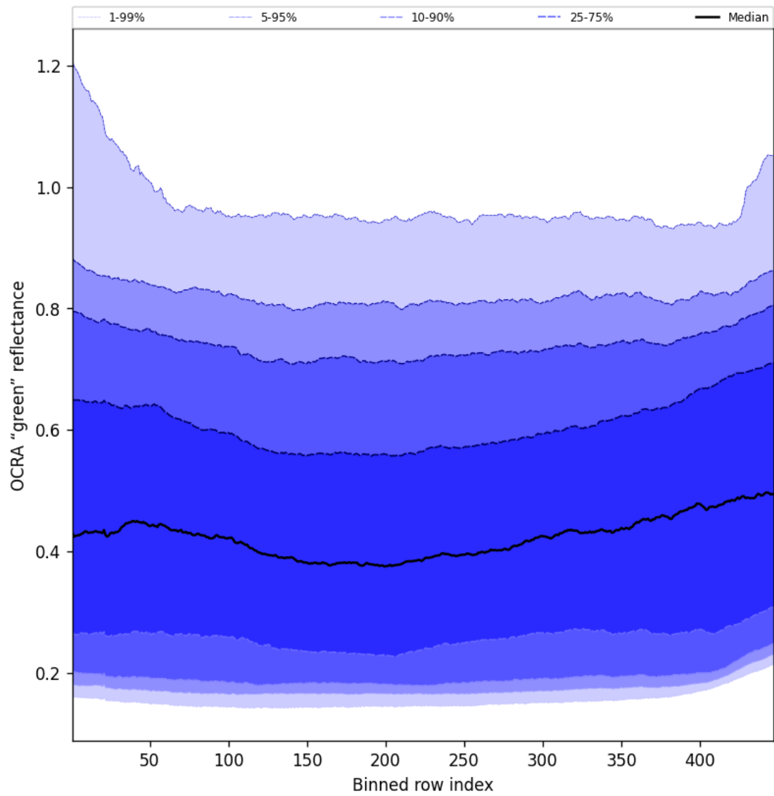
Figure 68: Along track statistics of “OCRA “green” reflectance” for 2025-07-13 to 2025-07-15
