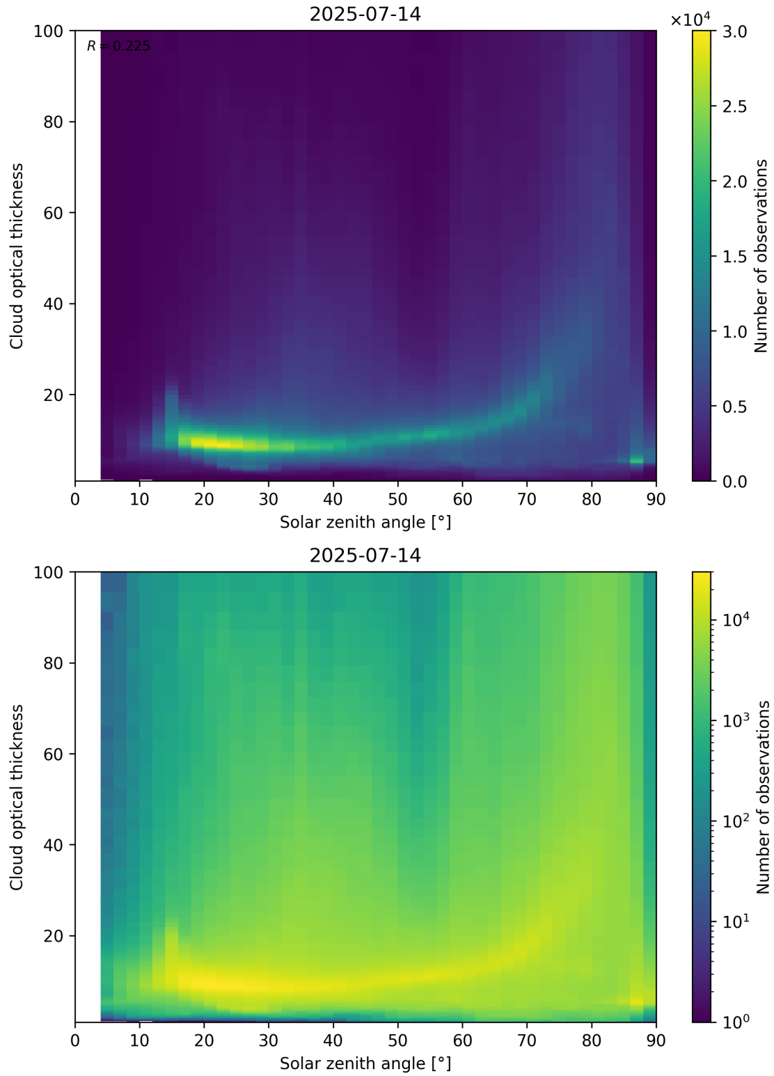
Figure 103: Scatter density plot of “Solar zenith angle” against “Cloud optical thickness” for 2025-07-13 to 2025-07-15.
