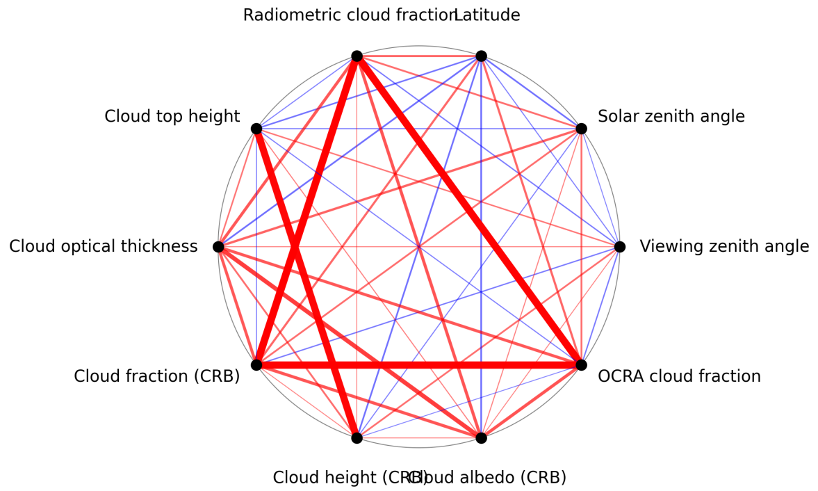
Figure 1: Map of correlation graph for 2025-07-13 to 2025-07-15.
