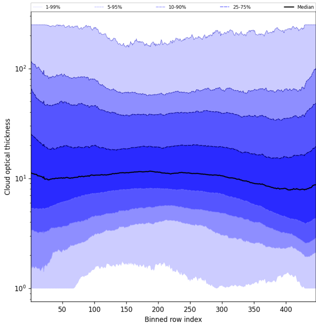
Figure 57: Along track statistics of “Cloud optical thickness” for 2025-07-13 to 2025-07-15
