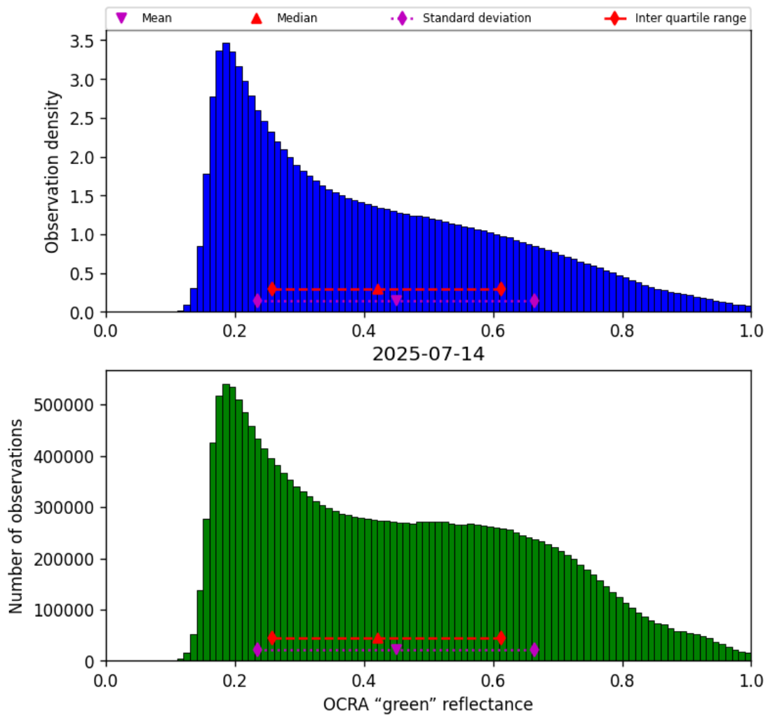
Figure 52: Histogram of “OCRA “green” reflectance” for 2025-07-13 to 2025-07-15
