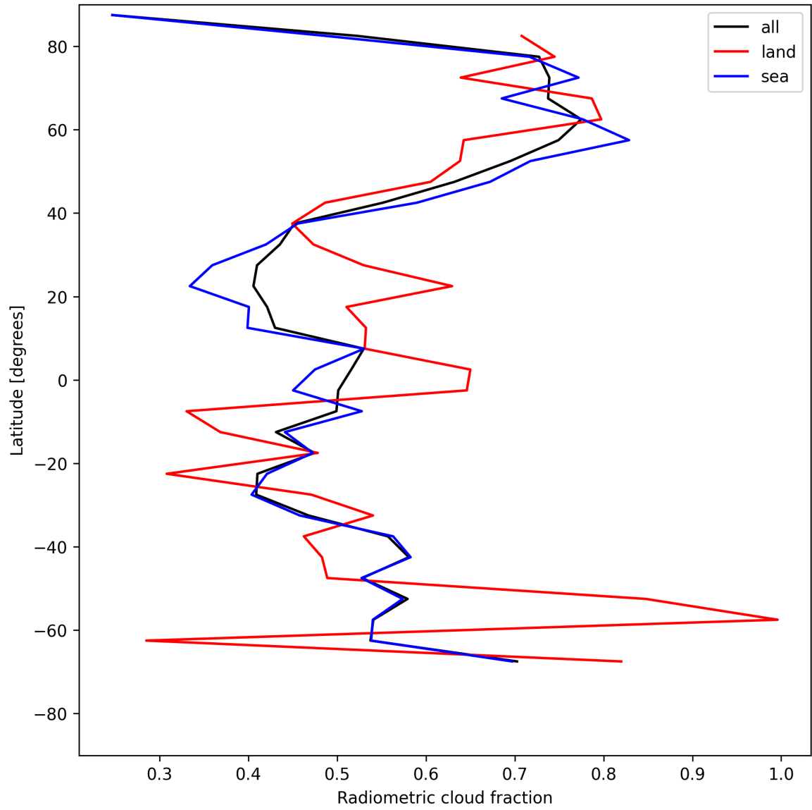
Figure 23: Zonal average of “Radiometric cloud fraction” for 2025-07-13 to 2025-07-15.
