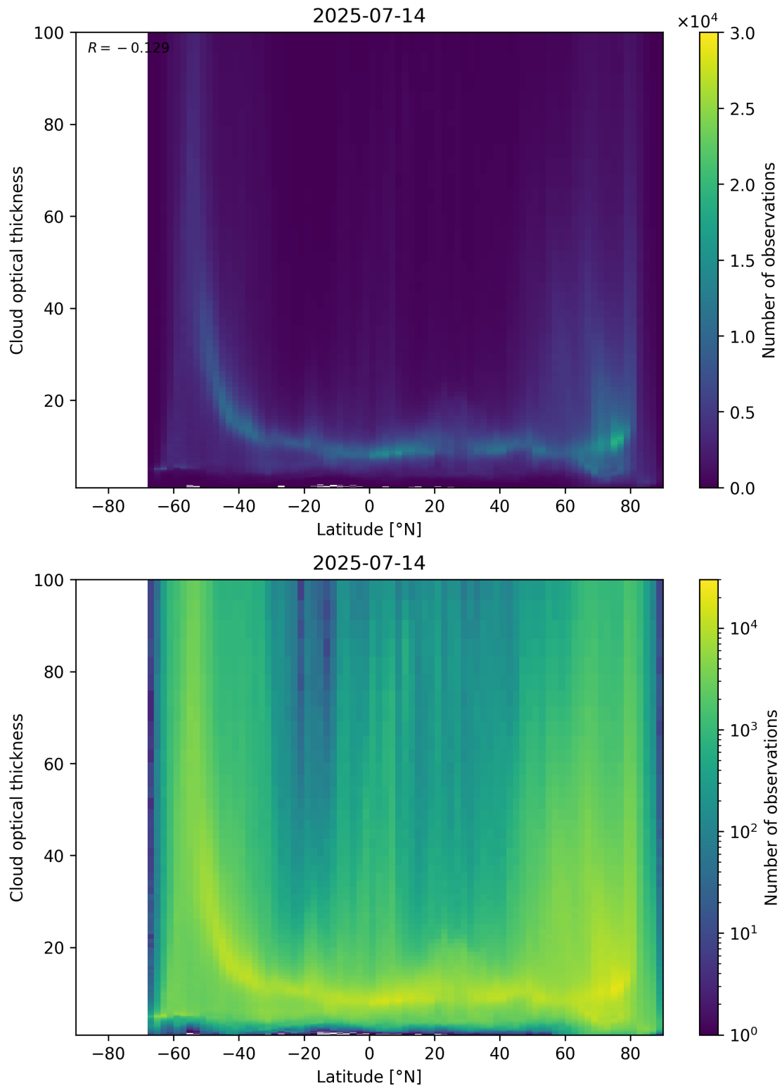
Figure 96: Scatter density plot of “Latitude” against “Cloud optical thickness” for 2025-07-13 to 2025-07-15.
