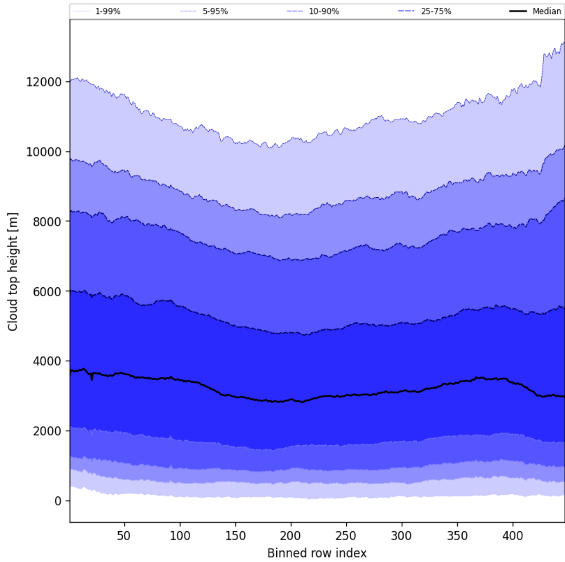
Figure 56: Along track statistics of “Cloud top height” for 2025-07-13 to 2025-07-15
