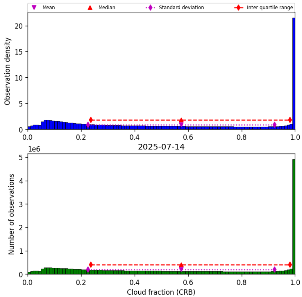
Figure 42: Histogram of “Cloud fraction (CRB)” for 2025-07-13 to 2025-07-15
