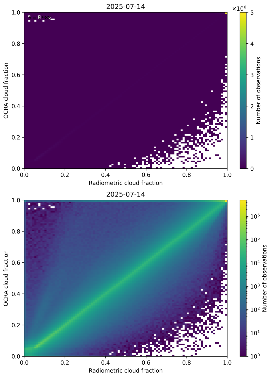
Figure 72: Scatter density plot of “Radiometric cloud fraction” against “OCRA cloud fraction” for 2025-07-13 to 2025-07-15.
