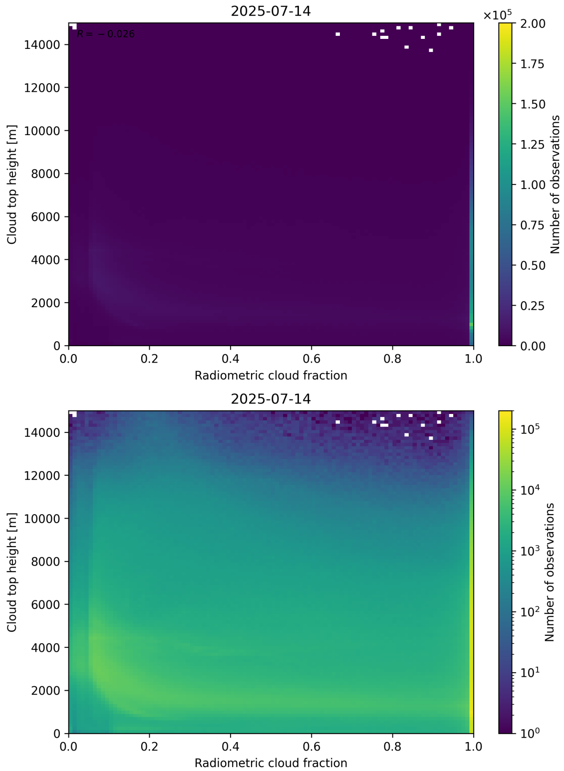
Figure 76: Scatter density plot of “Radiometric cloud fraction” against “Cloud top height” for 2025-07-13 to 2025-07-15.
