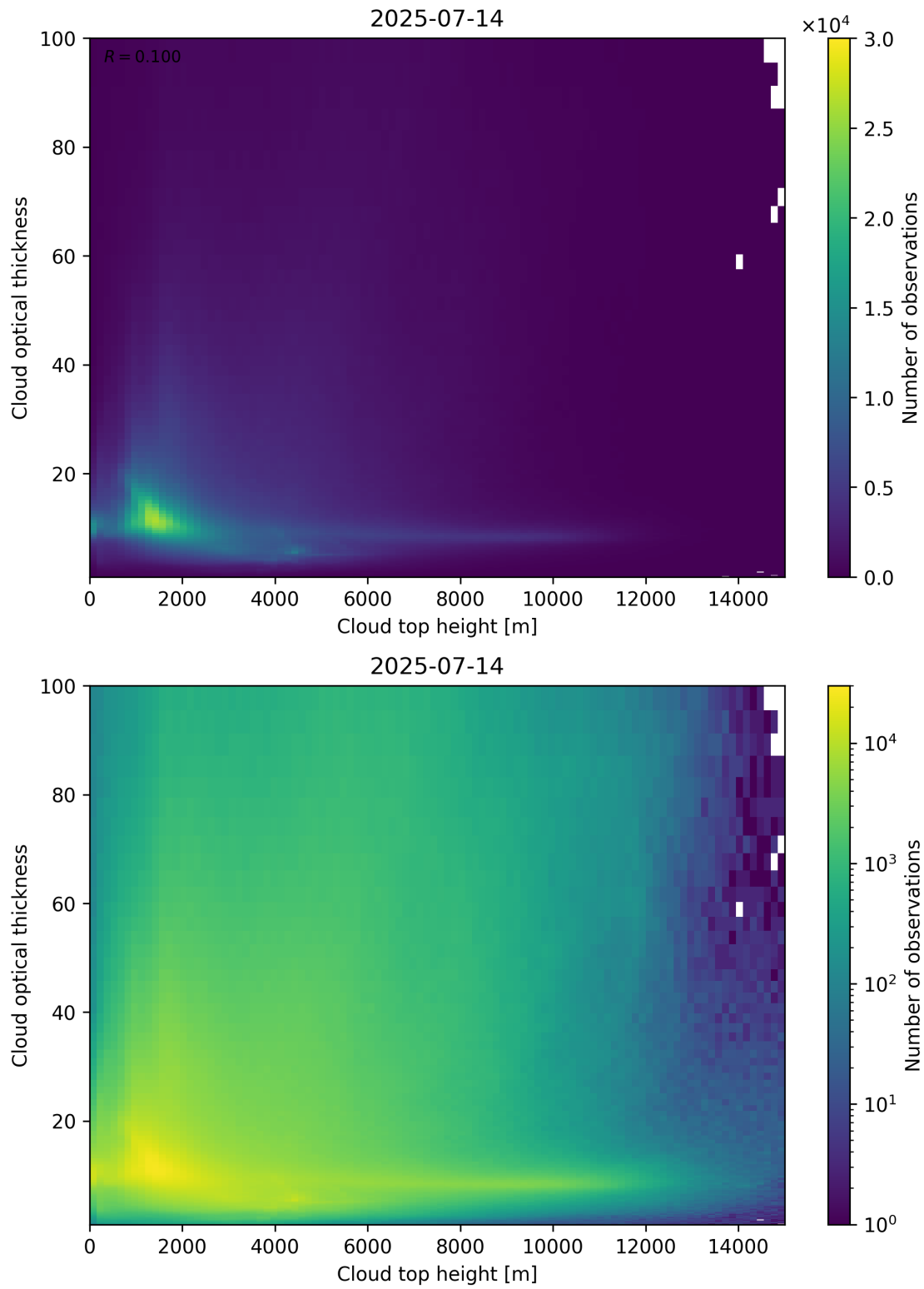
Figure 90: Scatter density plot of “Cloud top height” against “Cloud optical thickness” for 2025-07-13 to 2025-07-15.
