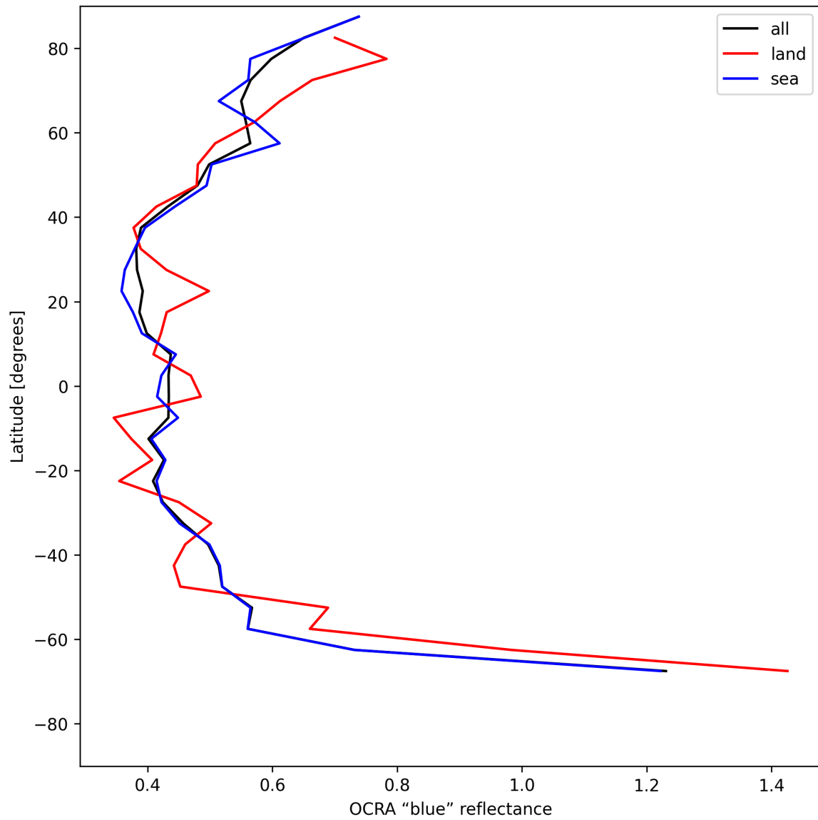
Figure 35: Zonal average of “OCRA “blue” reflectance” for 2025-07-13 to 2025-07-15.
