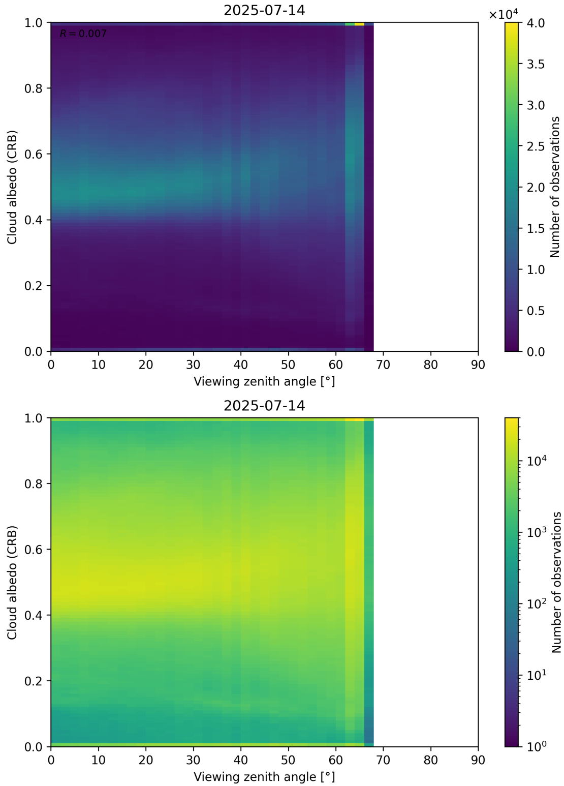
Figure 106: Scatter density plot of “Viewing zenith angle” against “Cloud albedo (CRB)” for 2025-07-13 to 2025-07-15.
