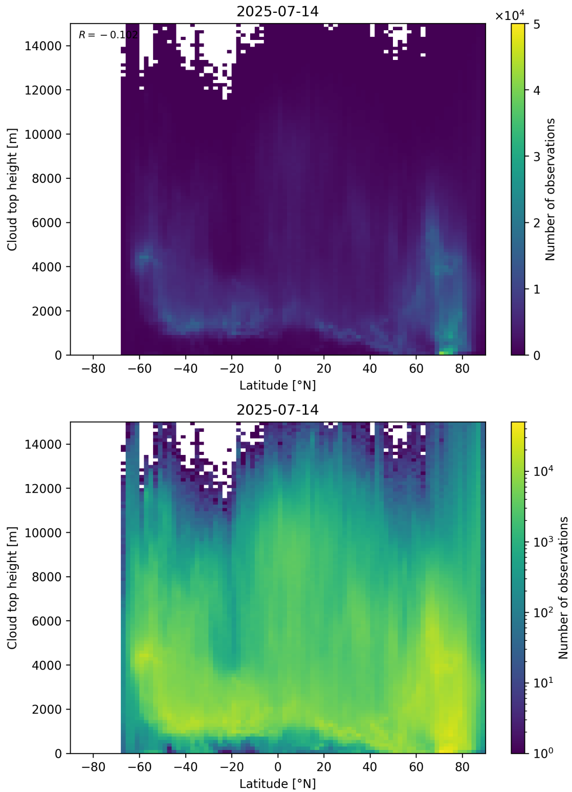
Figure 97: Scatter density plot of “Latitude” against “Cloud top height” for 2025-07-13 to 2025-07-15.
