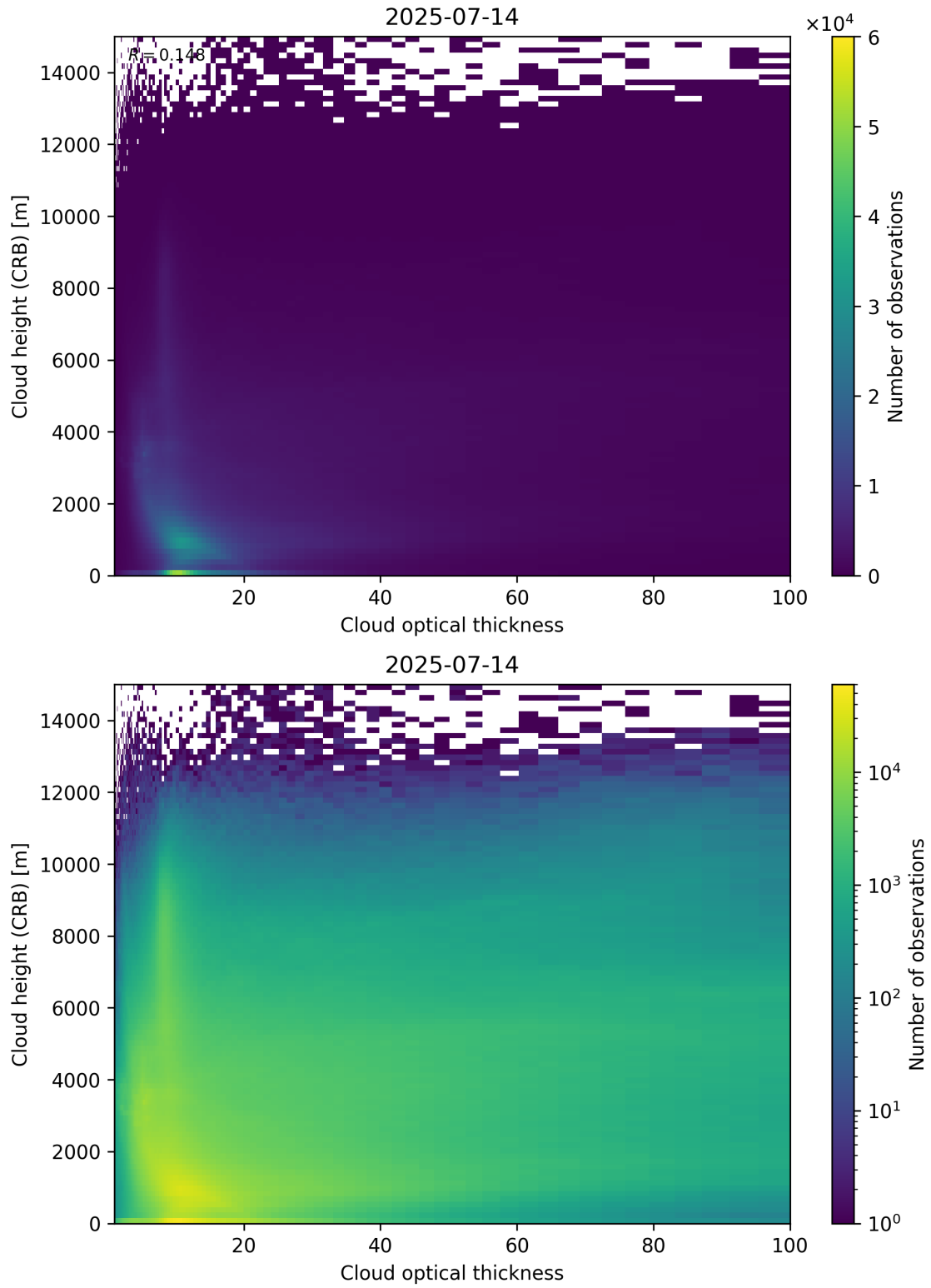
Figure 85: Scatter density plot of “Cloud optical thickness” against “Cloud height (CRB)” for 2025-07-13 to 2025-07-15.
