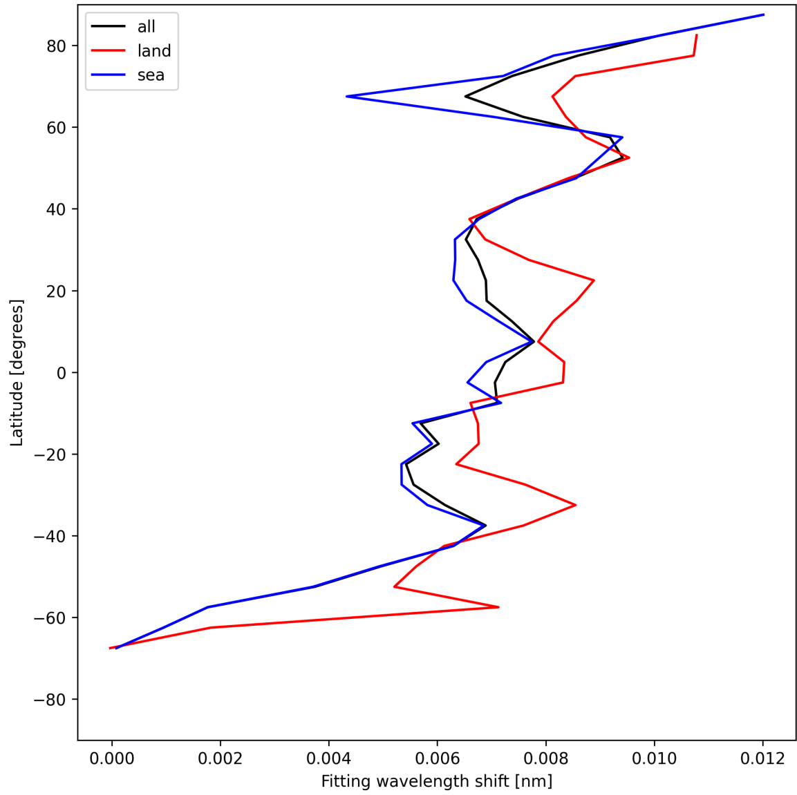
Figure 33: Zonal average of “Fitting wavelength shift” for 2025-07-13 to 2025-07-15.
