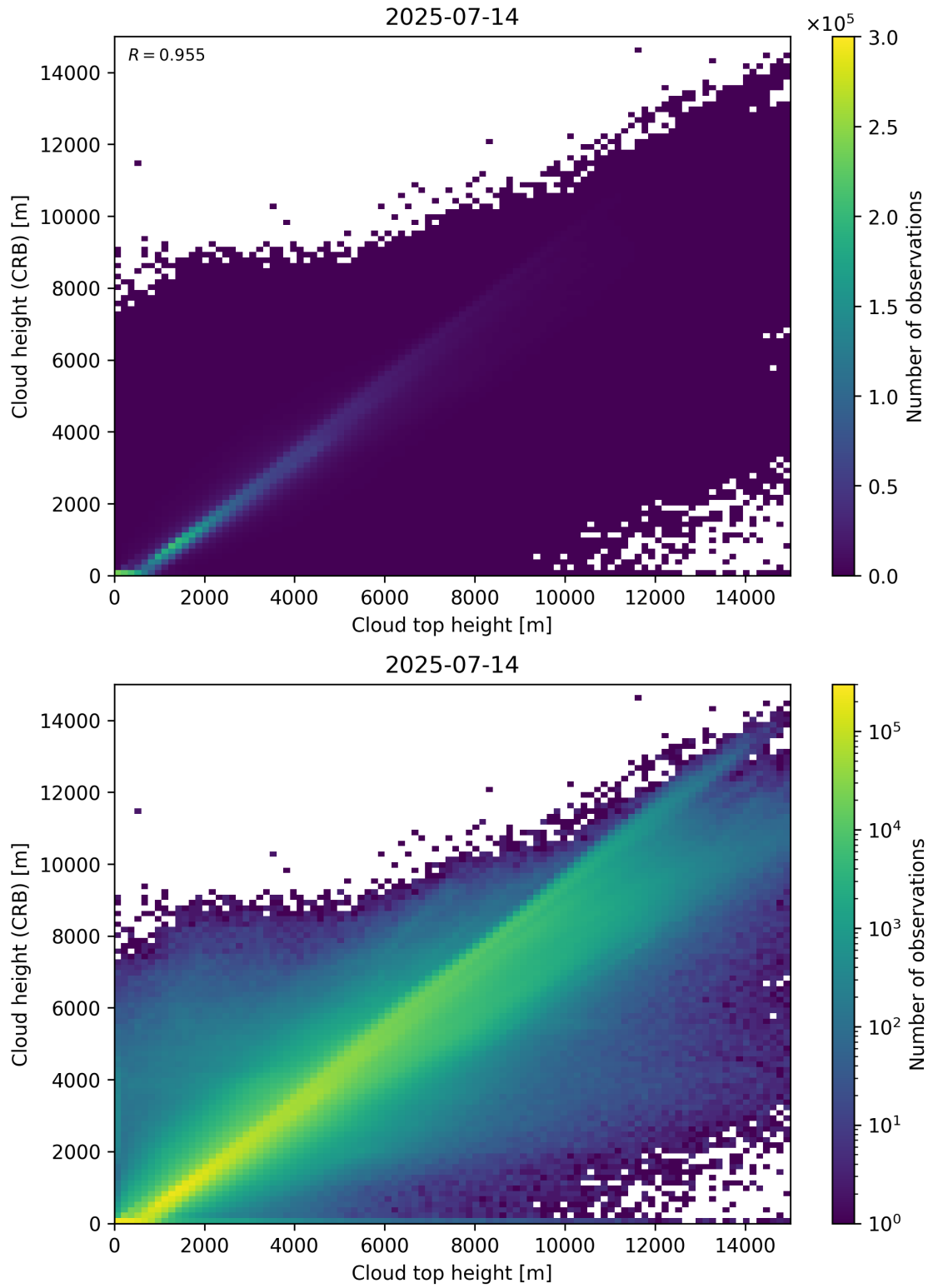
Figure 89: Scatter density plot of “Cloud top height” against “Cloud height (CRB)” for 2025-07-13 to 2025-07-15.
