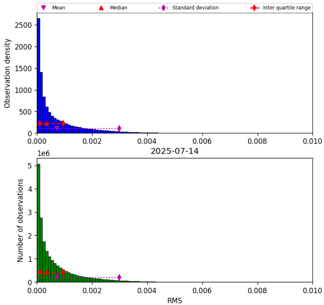
Figure 47: Histogram of “RMS” for 2025-07-13 to 2025-07-15
