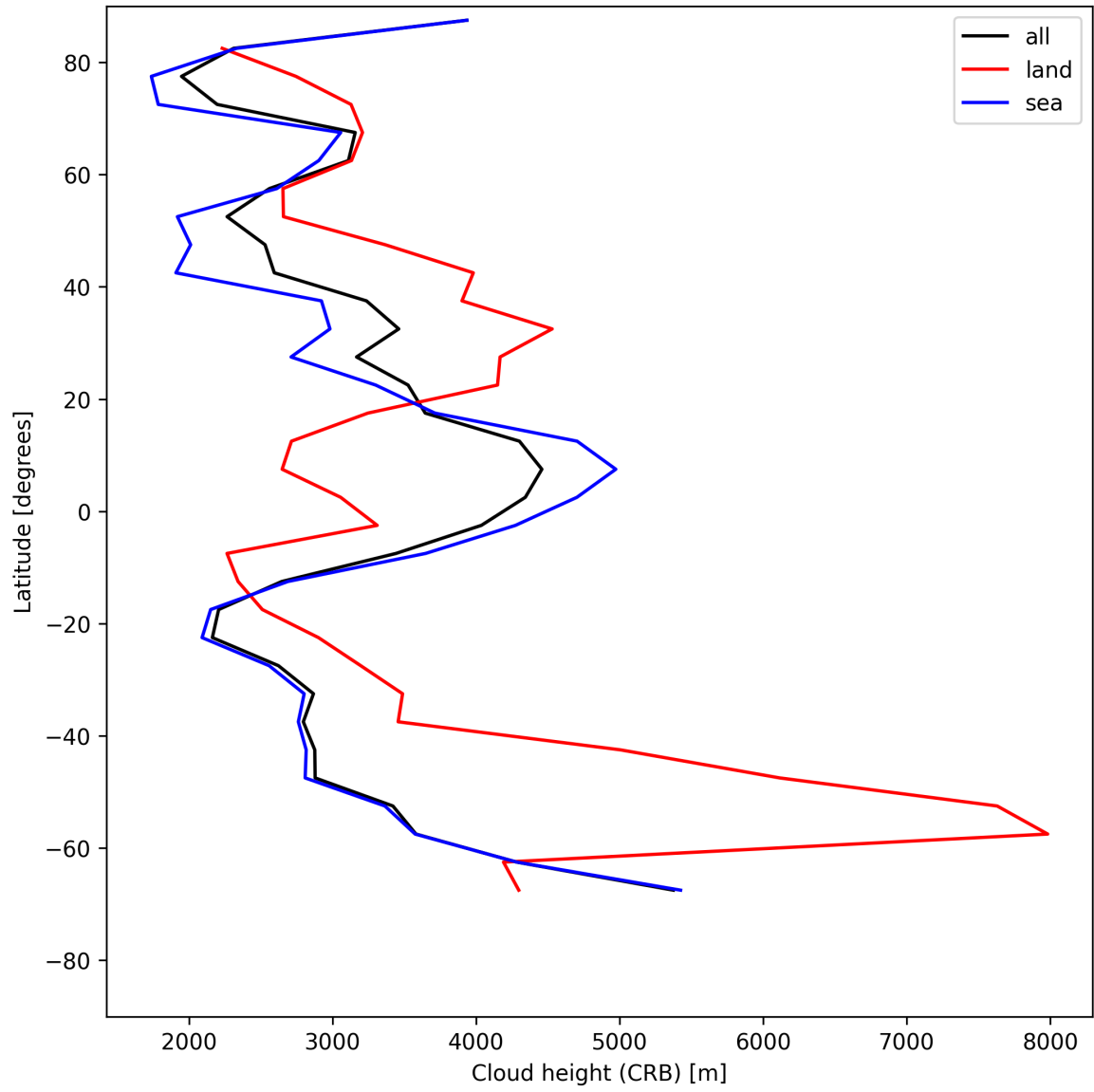
Figure 27: Zonal average of “Cloud height (CRB)” for 2025-07-13 to 2025-07-15.
