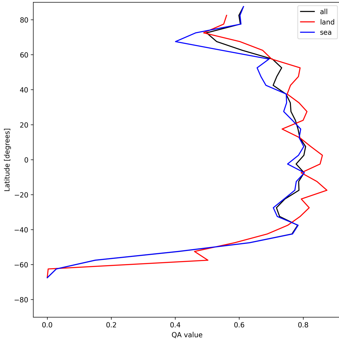
Figure 22: Zonal average of “QA value” for 2025-07-13 to 2025-07-15.
