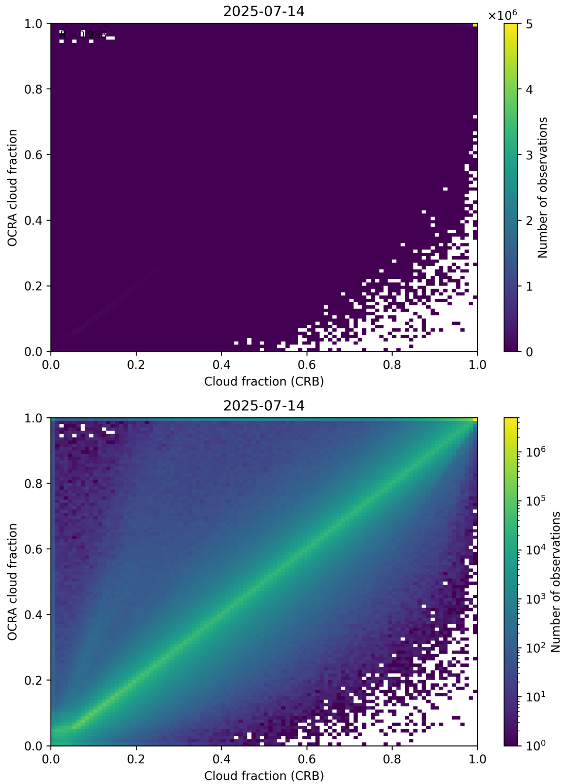
Figure 78: Scatter density plot of “Cloud fraction (CRB)” against “OCRA cloud fraction” for 2025-07-13 to 2025-07-15.
