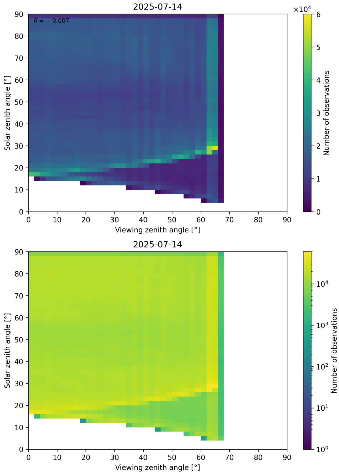
Figure 114: Scatter density plot of “Viewing zenith angle” against “Solar zenith angle” for 2025-07-13 to 2025-07-15.
