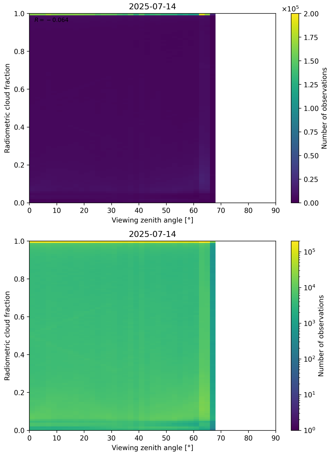
Figure 107: Scatter density plot of “Viewing zenith angle” against “Radiometric cloud fraction” for 2025-07-13 to 2025-07-15.
