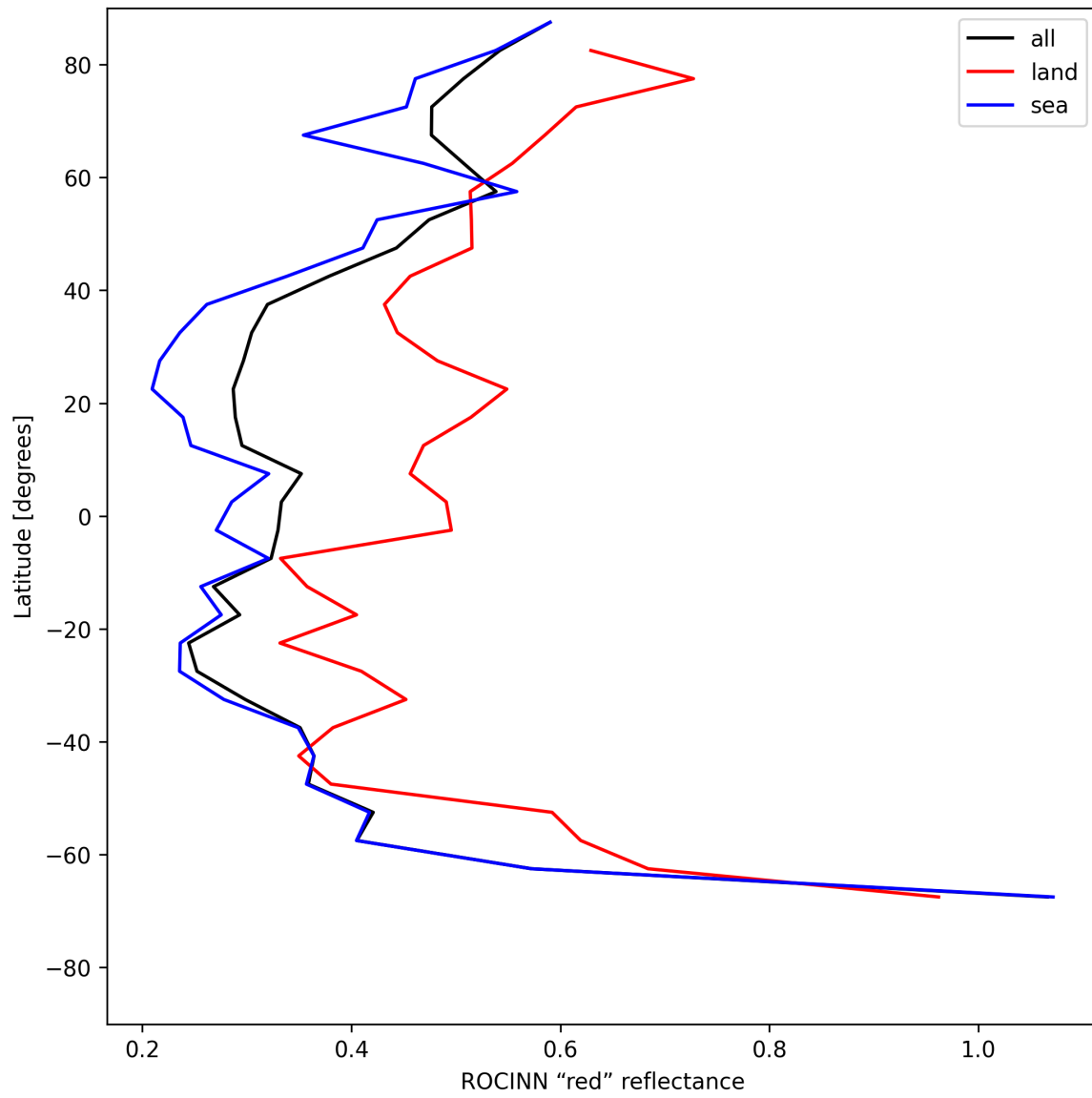
Figure 37: Zonal average of "ROCINN "red" reflectance" for 2025-07-13 to 2025-07-15.
