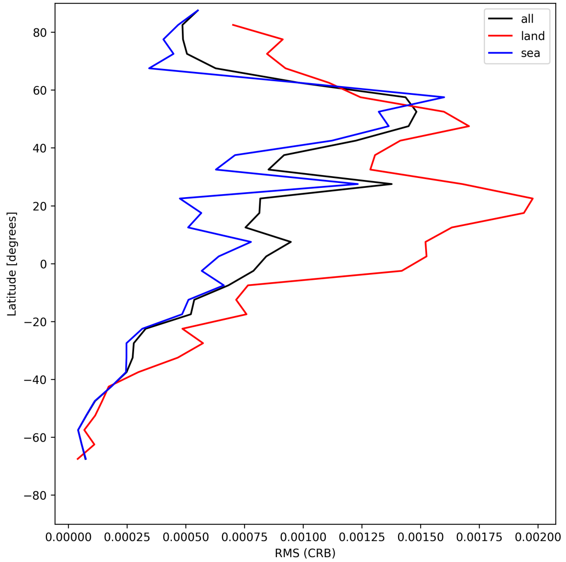
Figure 32: Zonal average of “RMS (CRB)” for 2025-07-13 to 2025-07-15.
