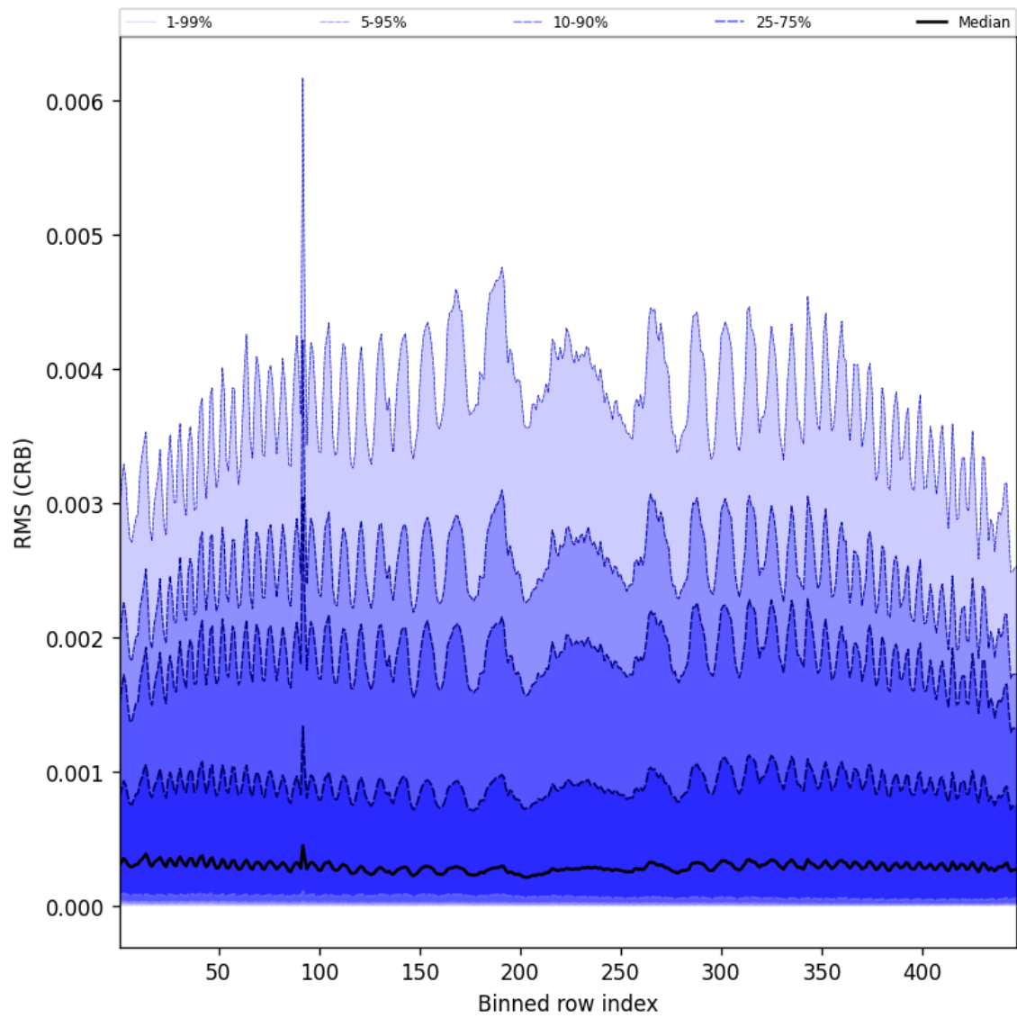
Figure 64: Along track statistics of “RMS (CRB)” for 2025-07-13 to 2025-07-15
