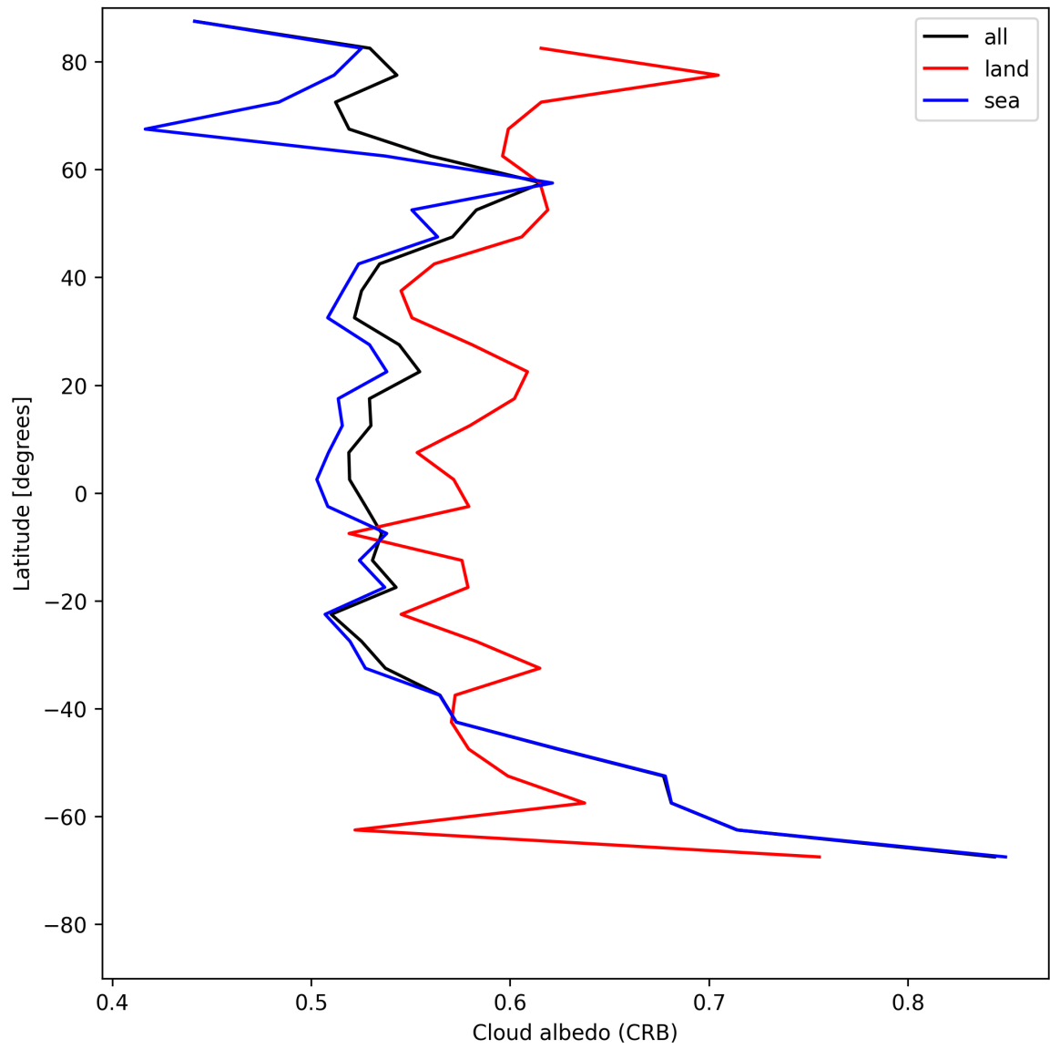
Figure 28: Zonal average of “Cloud albedo (CRB)” for 2025-07-13 to 2025-07-15.
