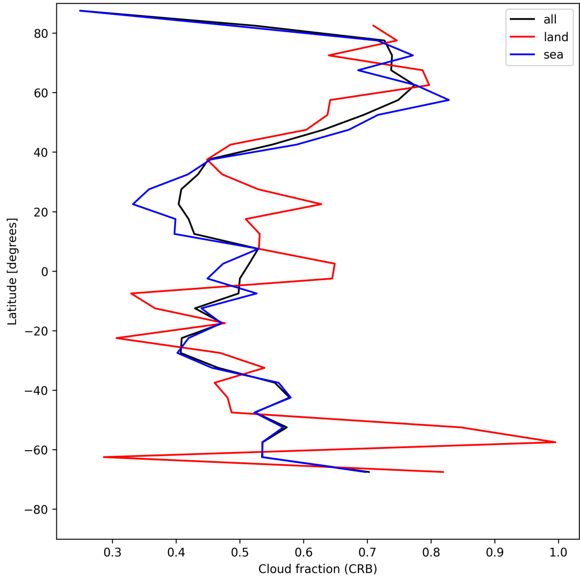
Figure 26: Zonal average of “Cloud fraction (CRB)” for 2025-07-13 to 2025-07-15.
