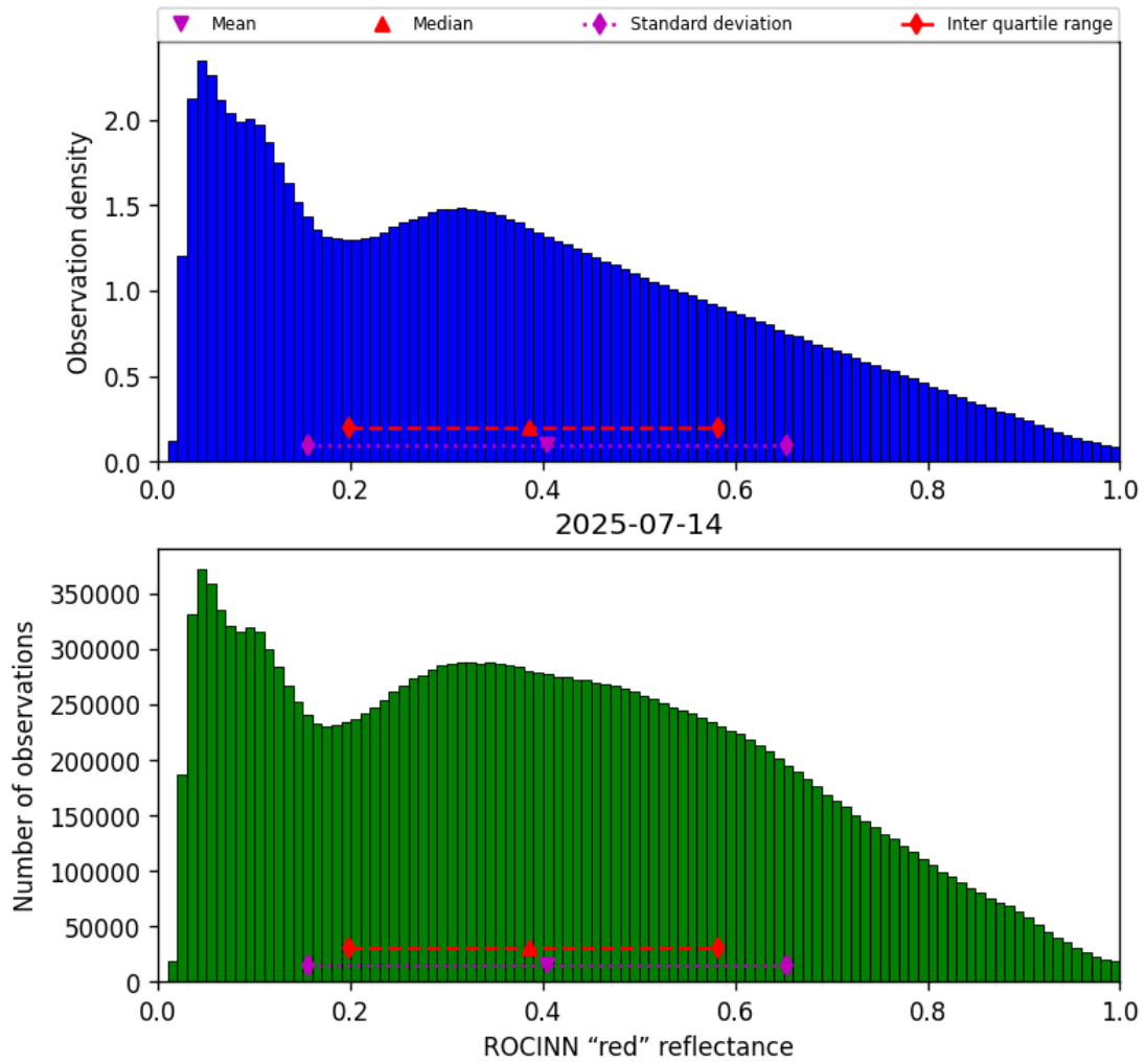
Figure 53: Histogram of “ROCINN “red” reflectance” for 2025-07-13 to 2025-07-15
