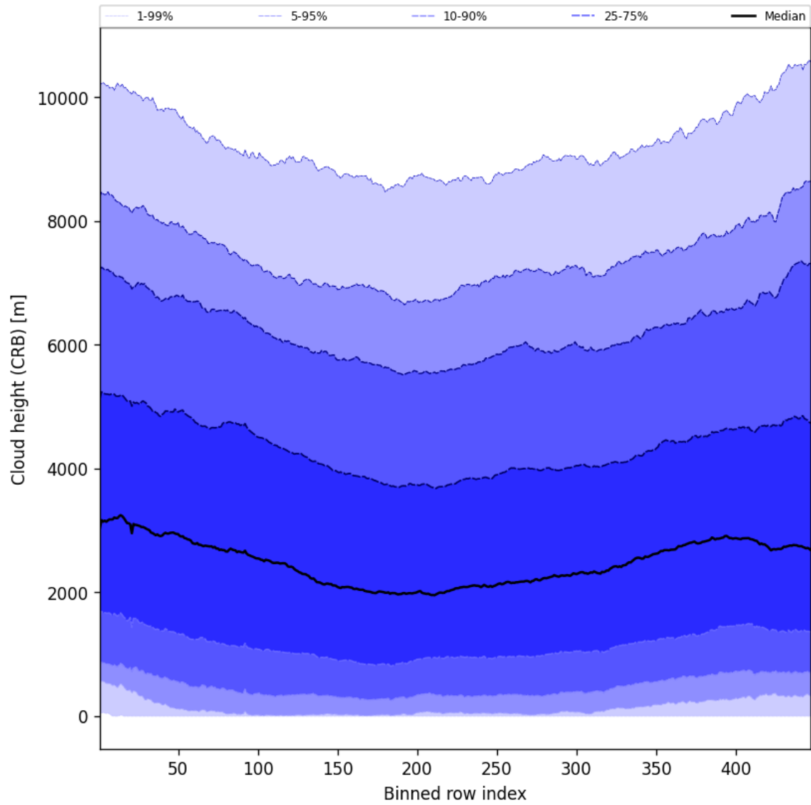
Figure 59: Along track statistics of “Cloud height (CRB)” for 2025-07-13 to 2025-07-15
