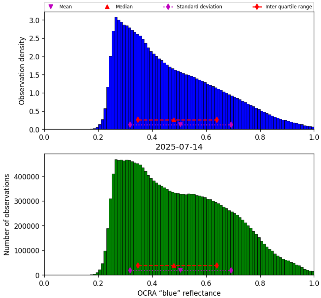
Figure 51: Histogram of “OCRA “blue” reflectance” for 2025-07-13 to 2025-07-15
