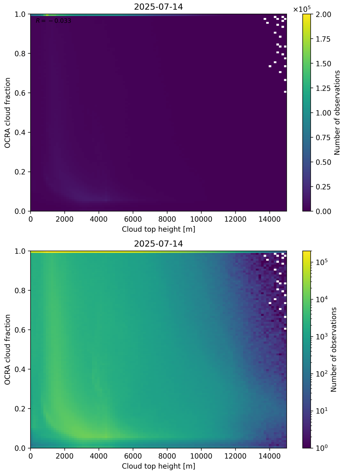
Figure 87: Scatter density plot of “Cloud top height” against “OCRA cloud fraction” for 2025-07-13 to 2025-07-15.
