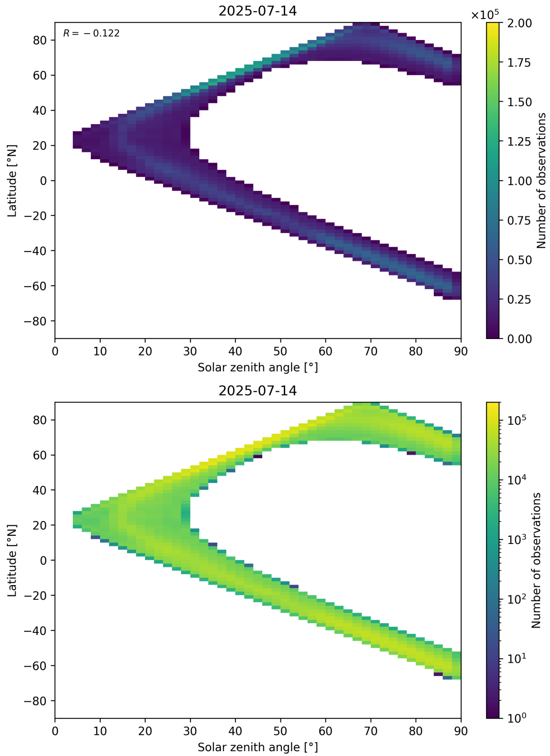
Figure 105: Scatter density plot of “Solar zenith angle” against “Latitude” for 2025-07-13 to 2025-07-15.
