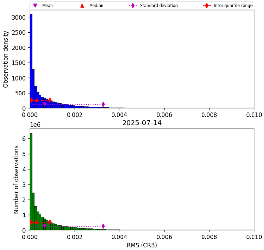
Figure 48: Histogram of “RMS (CRB)” for 2025-07-13 to 2025-07-15
