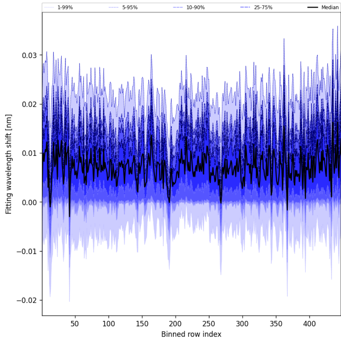
Figure 65: Along track statistics of “Fitting wavelength shift” for 2025-07-13 to 2025-07-15
