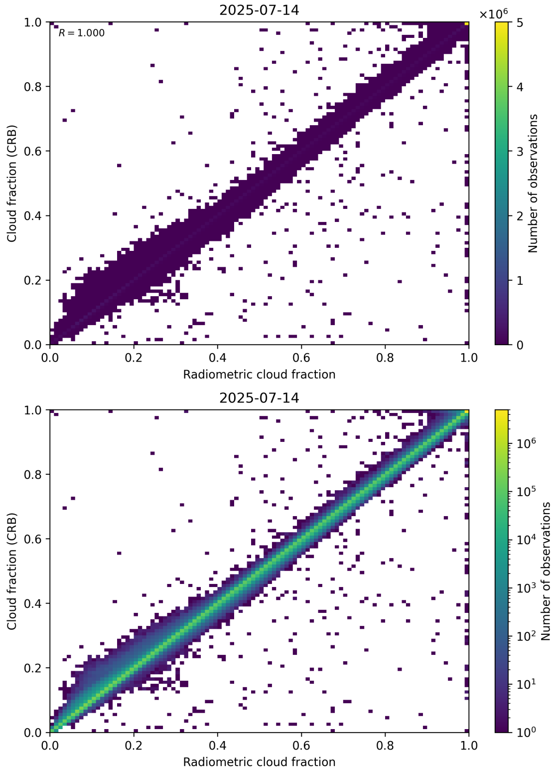
Figure 73: Scatter density plot of “Radiometric cloud fraction” against “Cloud fraction (CRB)” for 2025-07-13 to 2025-07-15.
