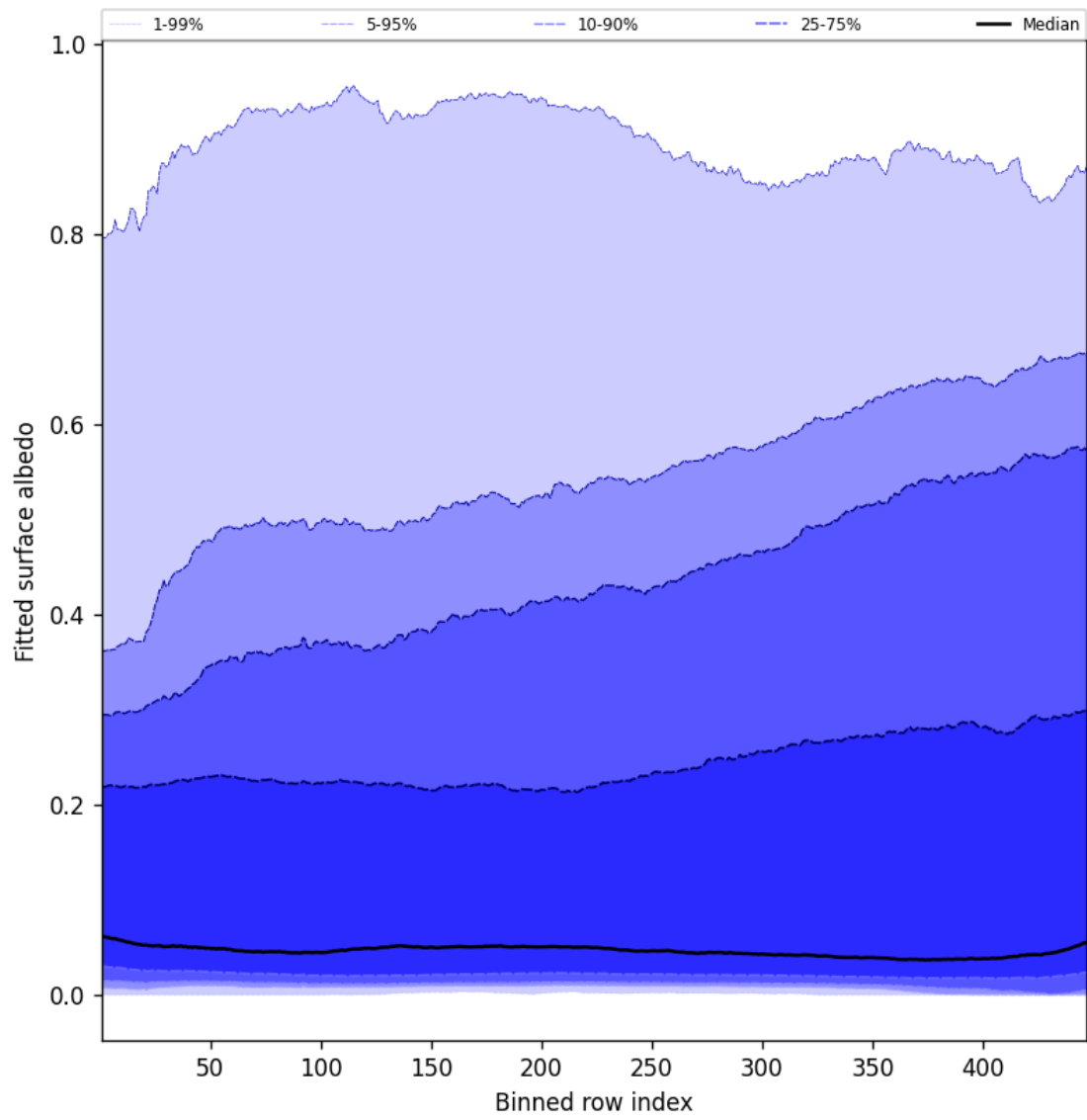
Figure 61: Along track statistics of “Fitted surface albedo” for 2025-07-13 to 2025-07-15
