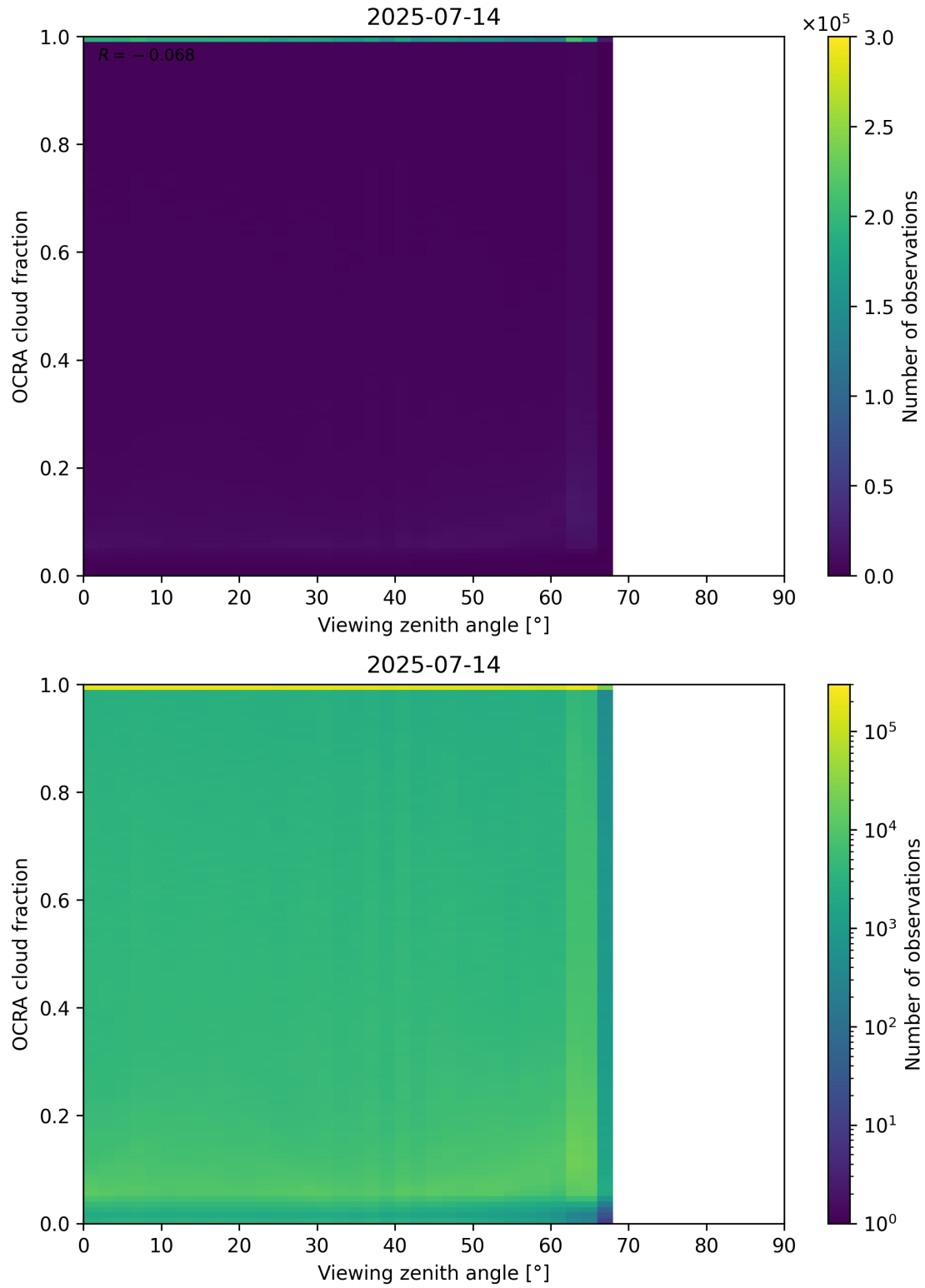
Figure 108: Scatter density plot of “Viewing zenith angle” against “OCRA cloud fraction” for 2025-07-13 to 2025-07-15.
