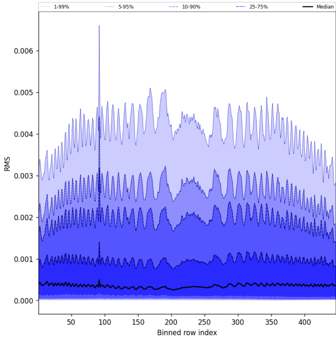
Figure 63: Along track statistics of “RMS” for 2025-07-13 to 2025-07-15
