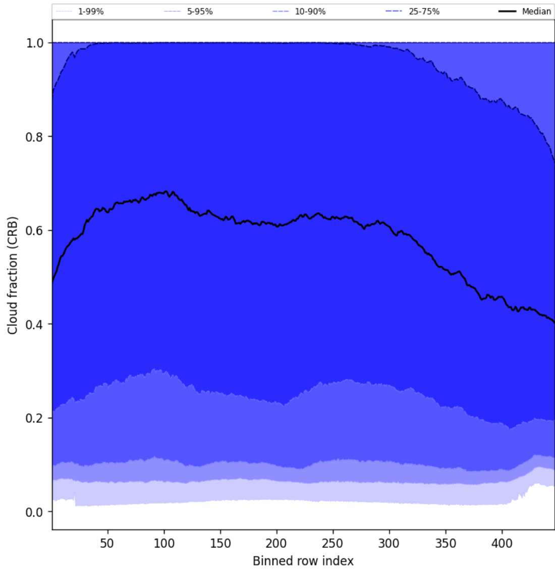
Figure 58: Along track statistics of “Cloud fraction (CRB)” for 2025-07-13 to 2025-07-15
