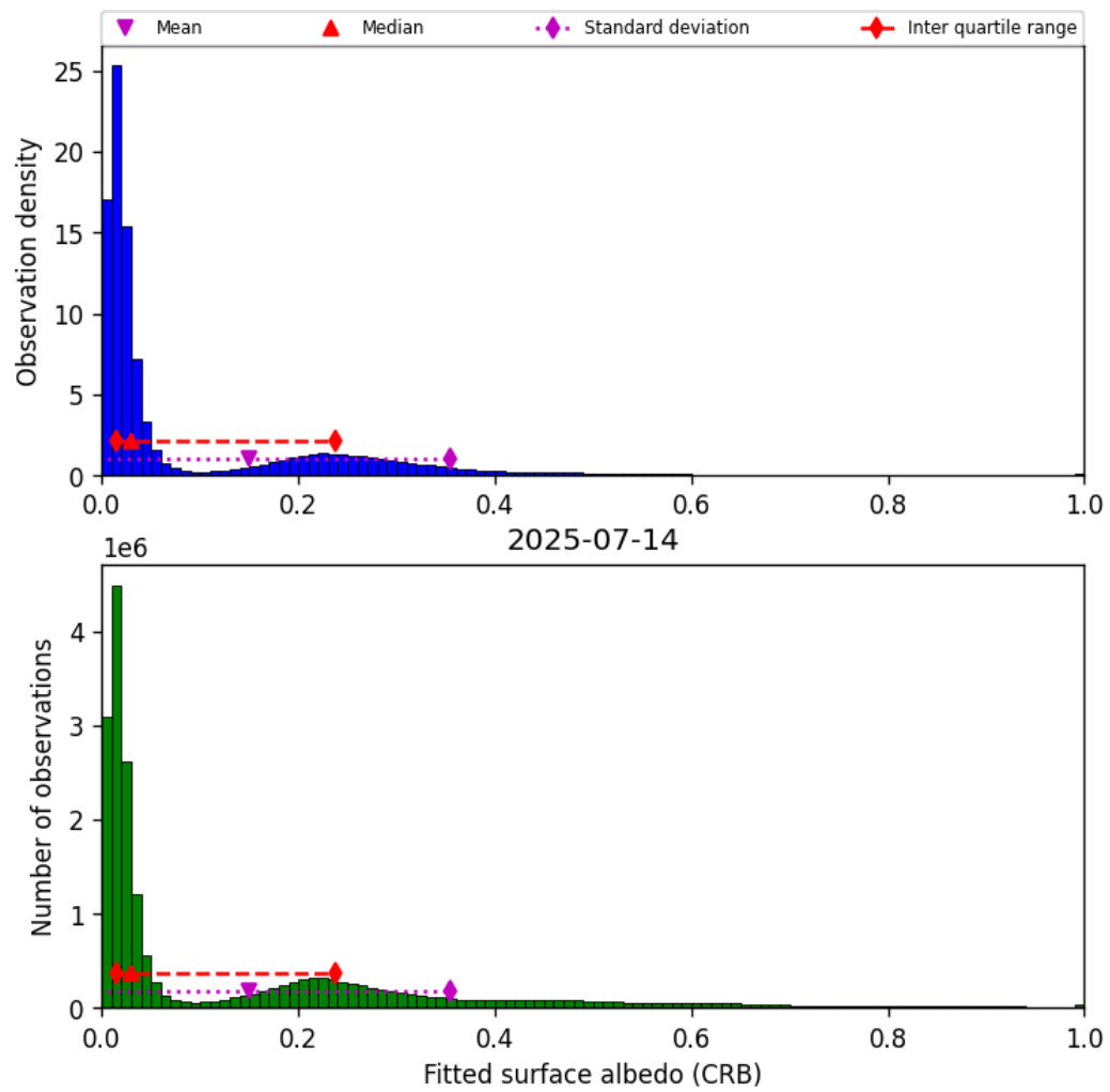
Figure 46: Histogram of “Fitted surface albedo (CRB)” for 2025-07-13 to 2025-07-15
