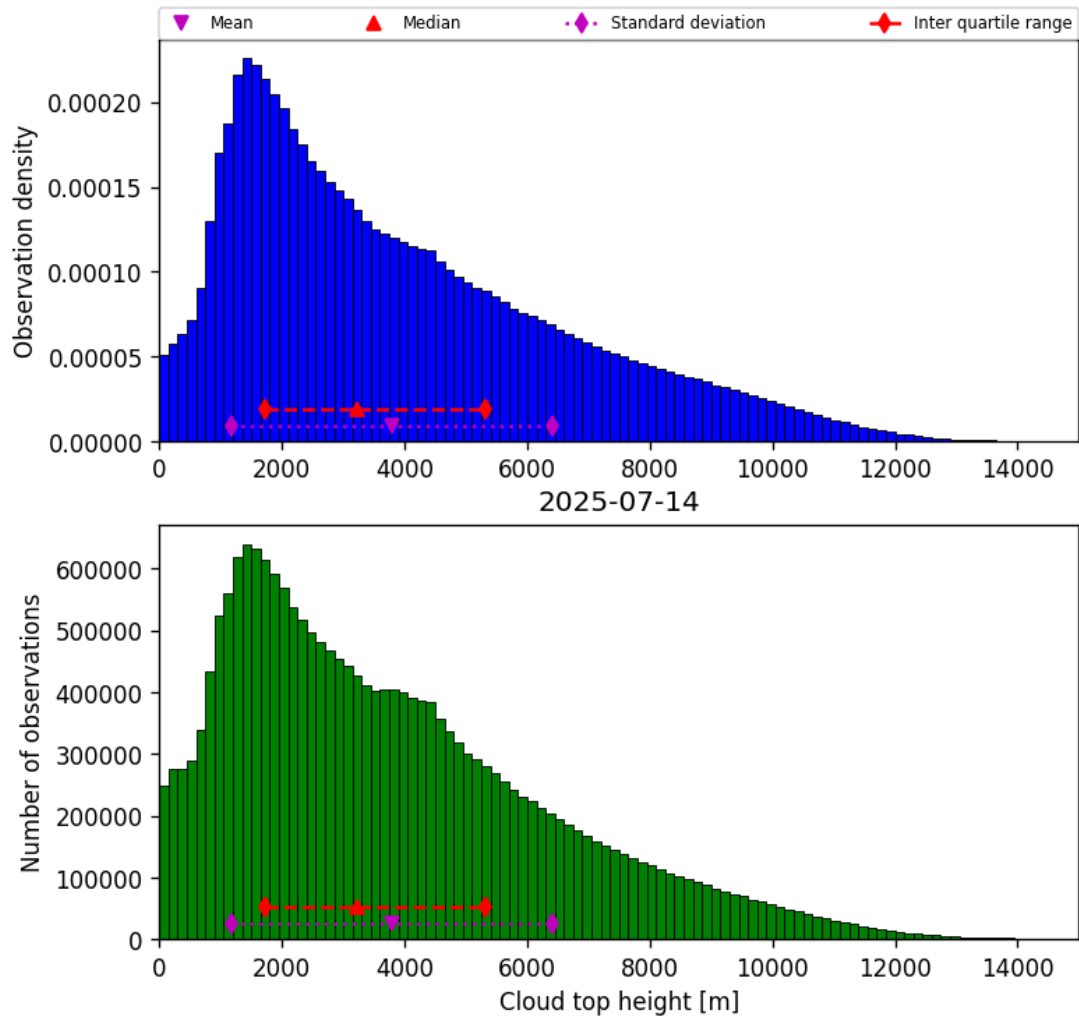
Figure 40: Histogram of “Cloud top height” for 2025-07-13 to 2025-07-15
