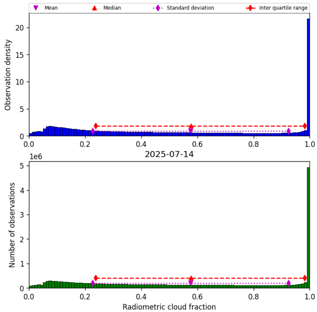
Figure 39: Histogram of “Radiometric cloud fraction” for 2025-07-13 to 2025-07-15
