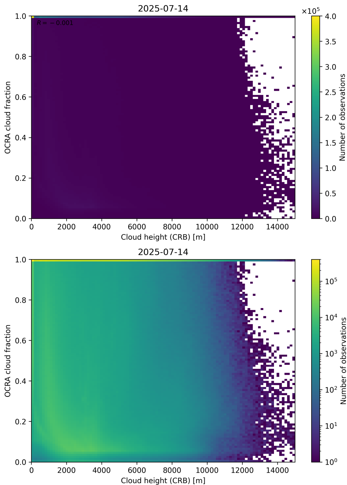
Figure 81: Scatter density plot of “Cloud height (CRB)” against “OCRA cloud fraction” for 2025-07-13 to 2025-07-15.
