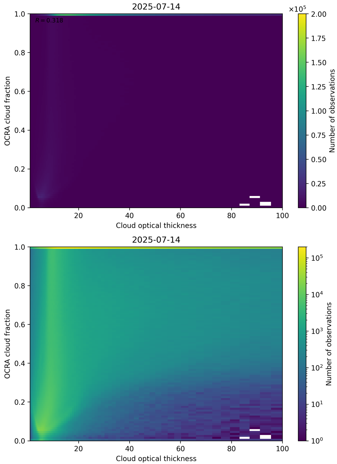
Figure 83: Scatter density plot of “Cloud optical thickness” against “OCRA cloud fraction” for 2025-07-13 to 2025-07-15.
