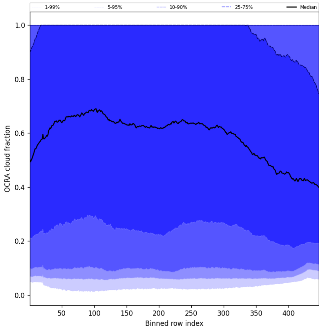
Figure 66: Along track statistics of “OCRA cloud fraction” for 2025-07-13 to 2025-07-15
