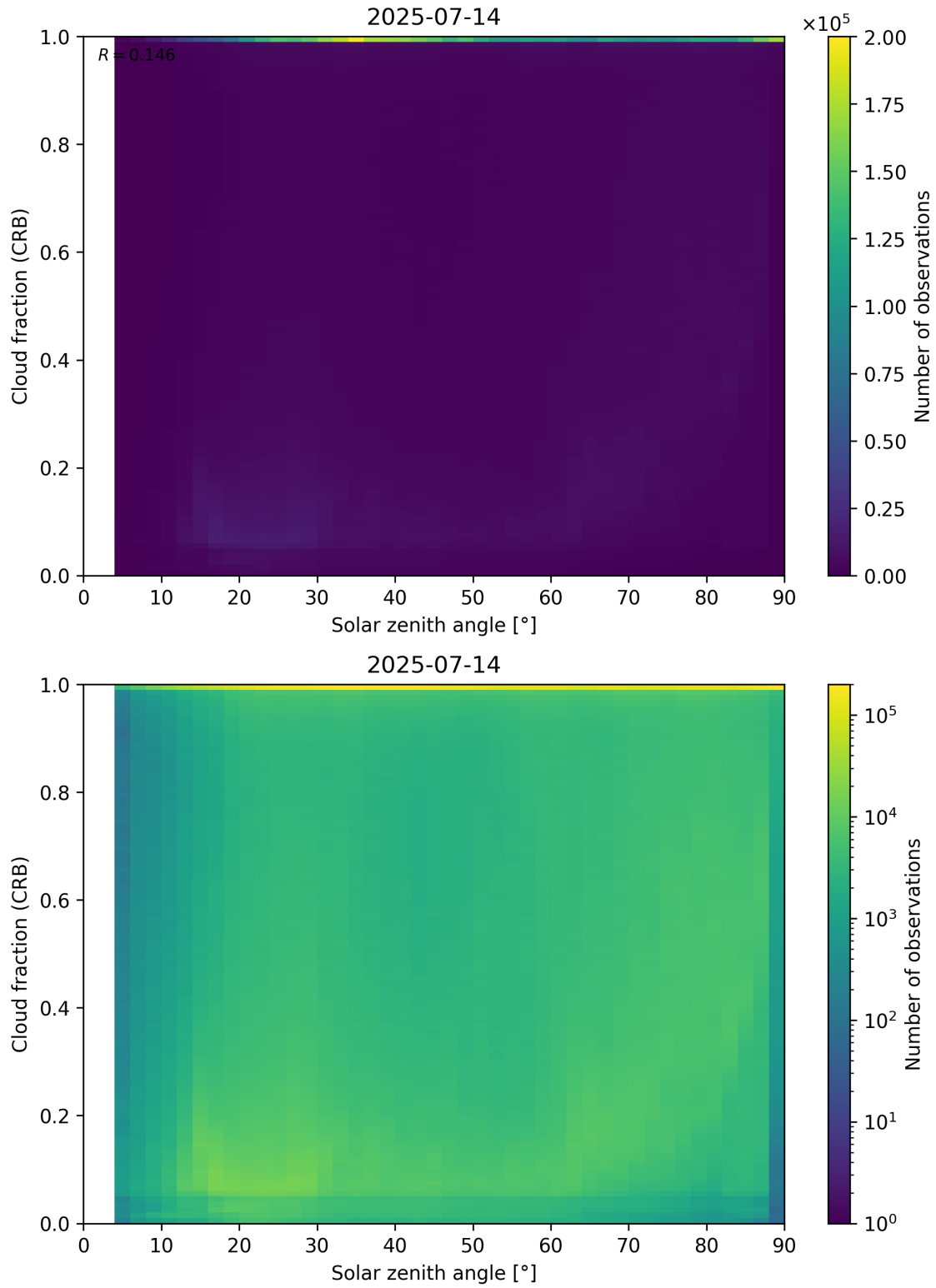
Figure 101: Scatter density plot of “Solar zenith angle” against “Cloud fraction (CRB)” for 2025-07-13 to 2025-07-15.
