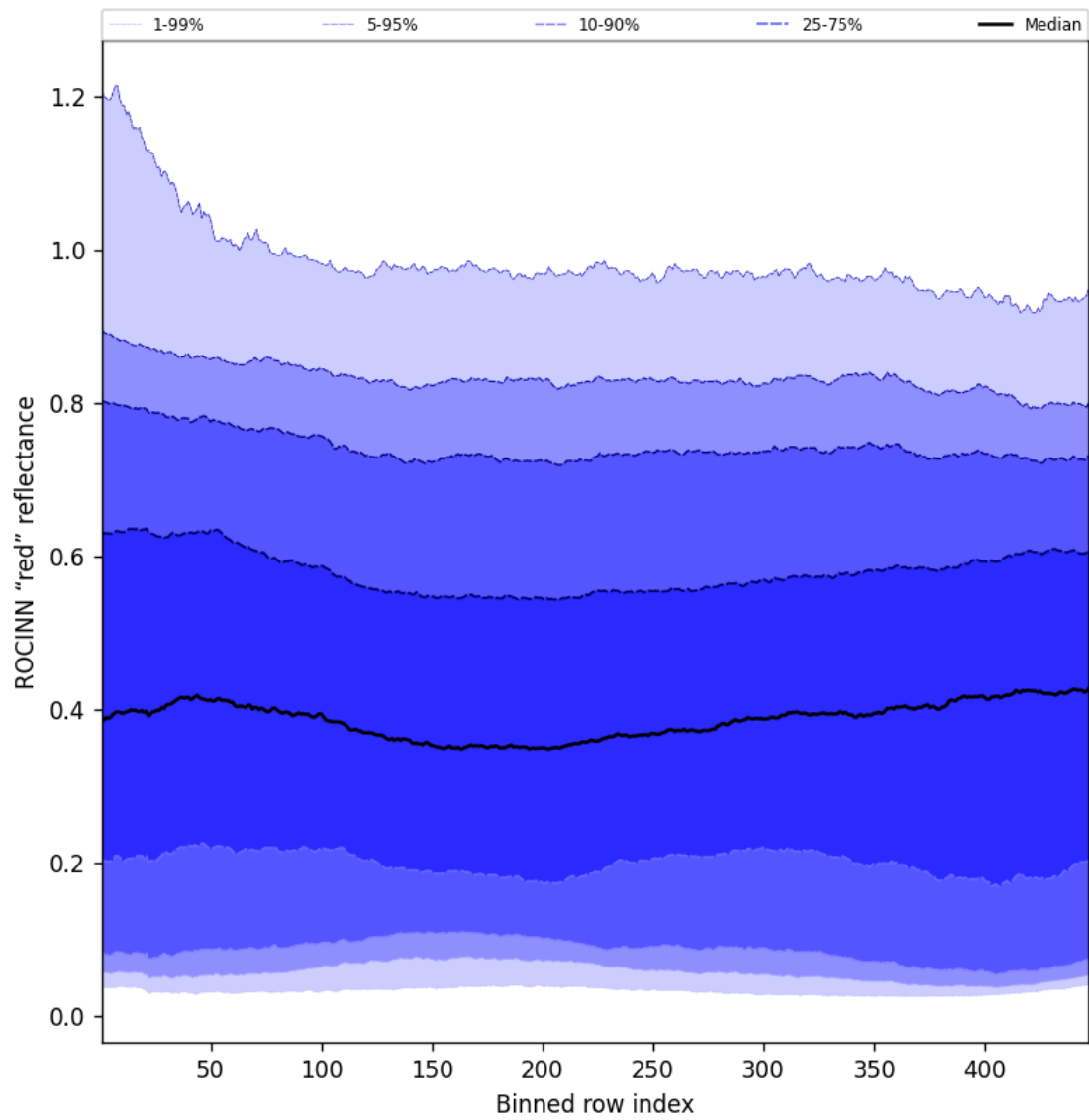
Figure 69: Along track statistics of “ROCINN “red” reflectance” for 2025-07-13 to 2025-07-15
