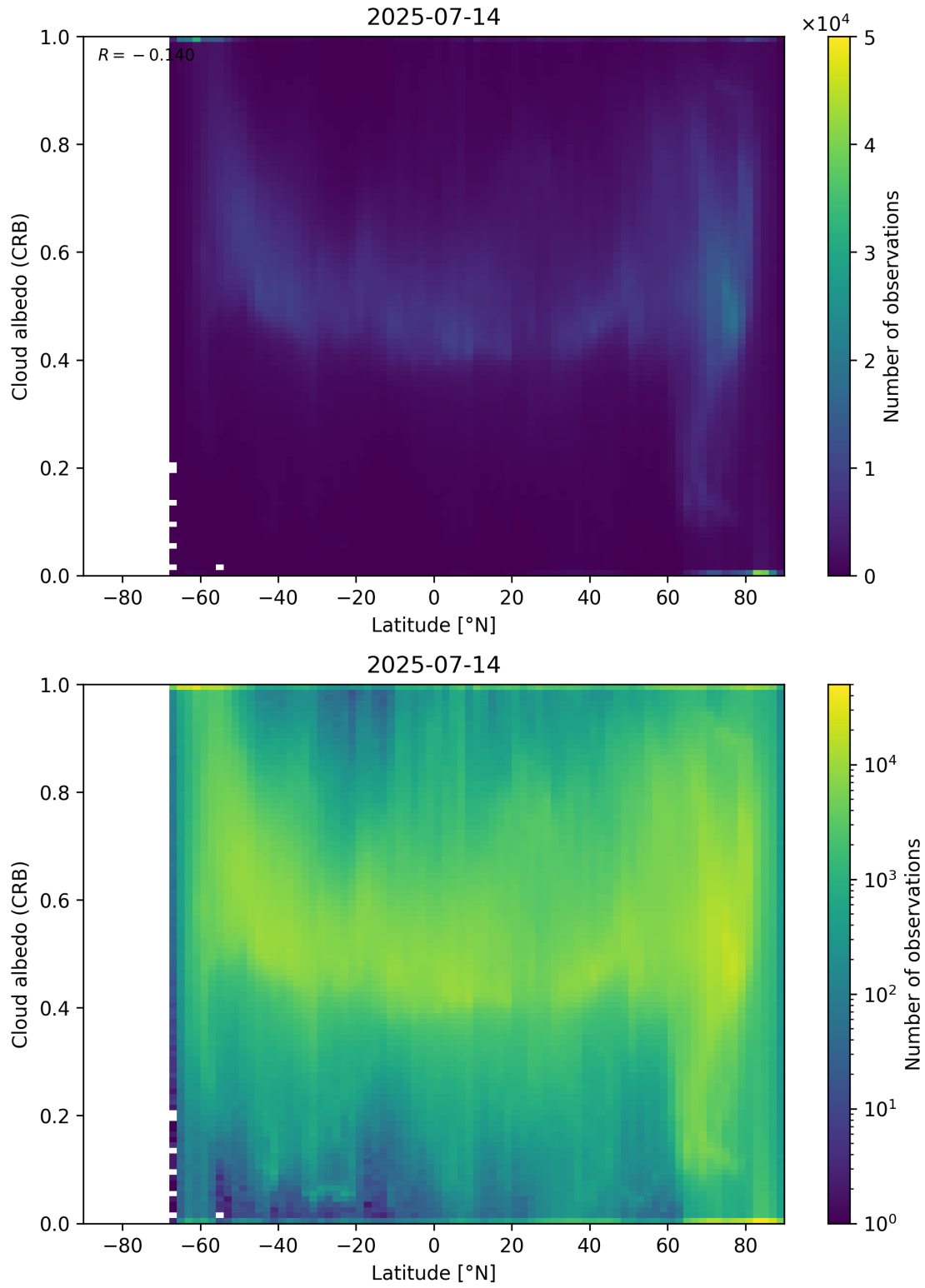
Figure 91: Scatter density plot of “Latitude” against “Cloud albedo (CRB)” for 2025-07-13 to 2025-07-15.
