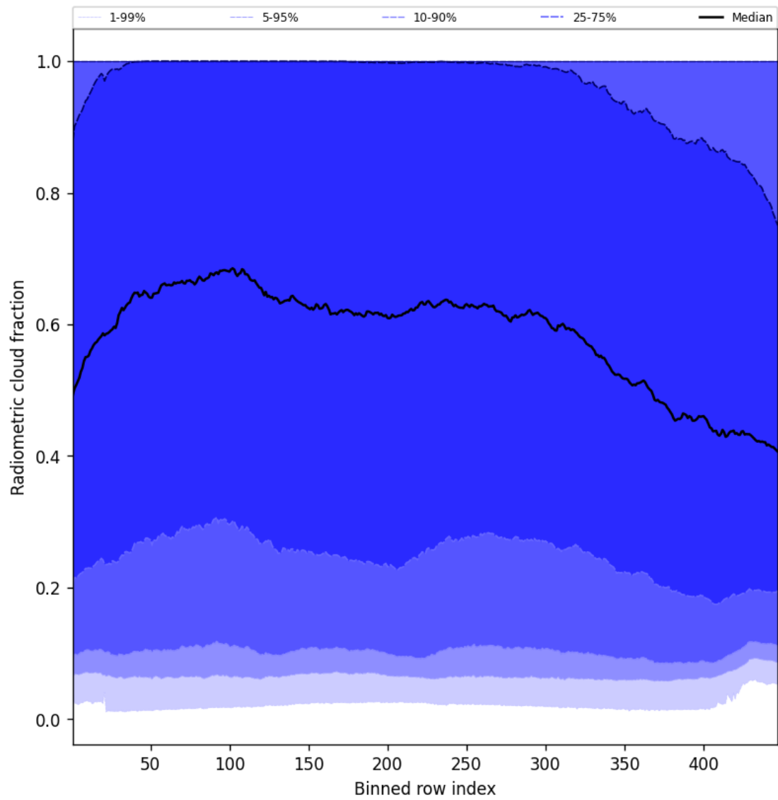
Figure 55: Along track statistics of “Radiometric cloud fraction” for 2025-07-13 to 2025-07-15
