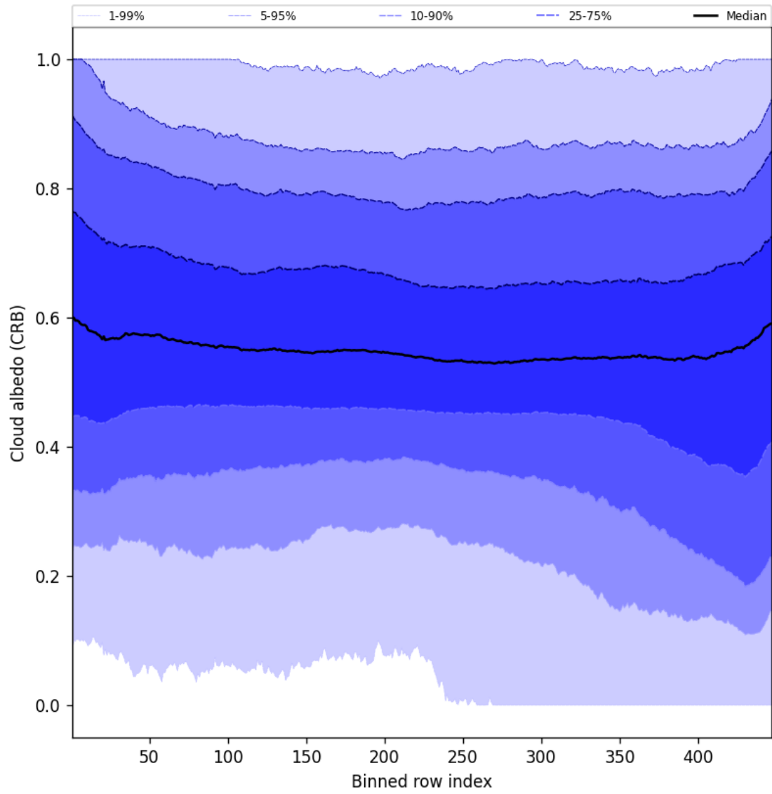
Figure 60: Along track statistics of “Cloud albedo (CRB)” for 2025-07-13 to 2025-07-15
