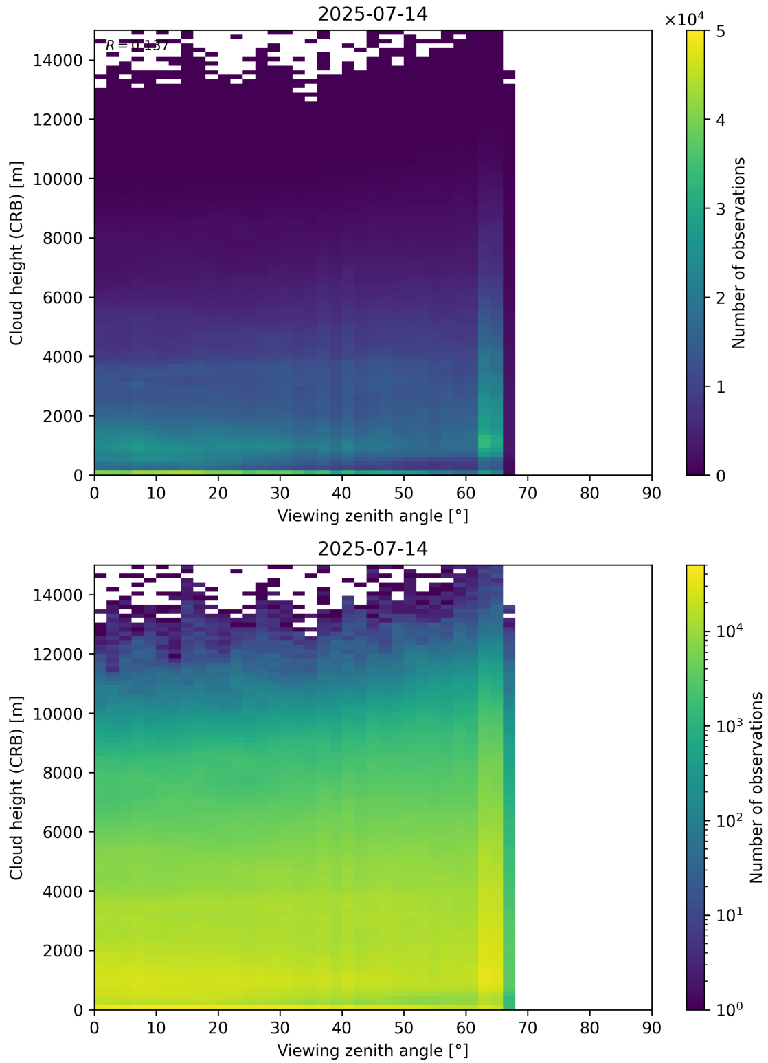
Figure 110: Scatter density plot of “Viewing zenith angle” against “Cloud height (CRB)” for 2025-07-13 to 2025-07-15.
