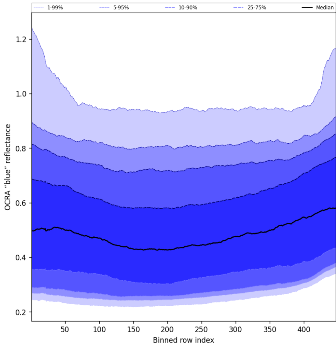
Figure 67: Along track statistics of “OCRA “blue” reflectance” for 2025-07-13 to 2025-07-15
