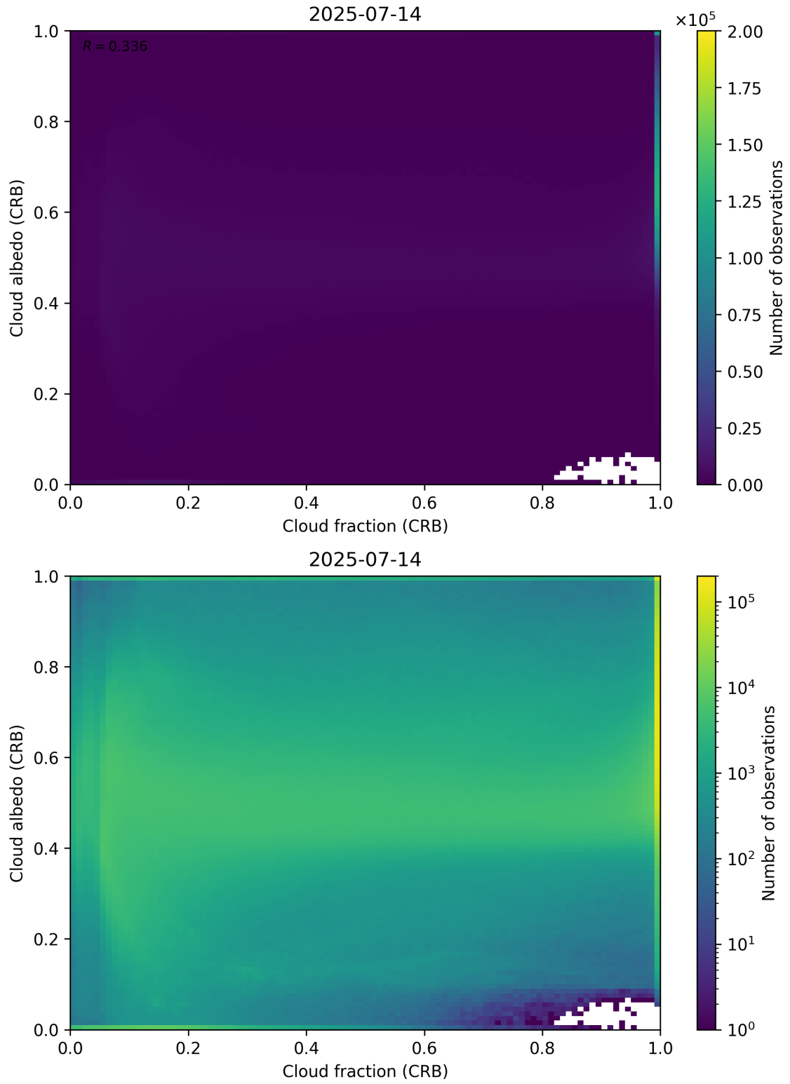
Figure 77: Scatter density plot of “Cloud fraction (CRB)” against “Cloud albedo (CRB)” for 2025-07-13 to 2025-07-15.
