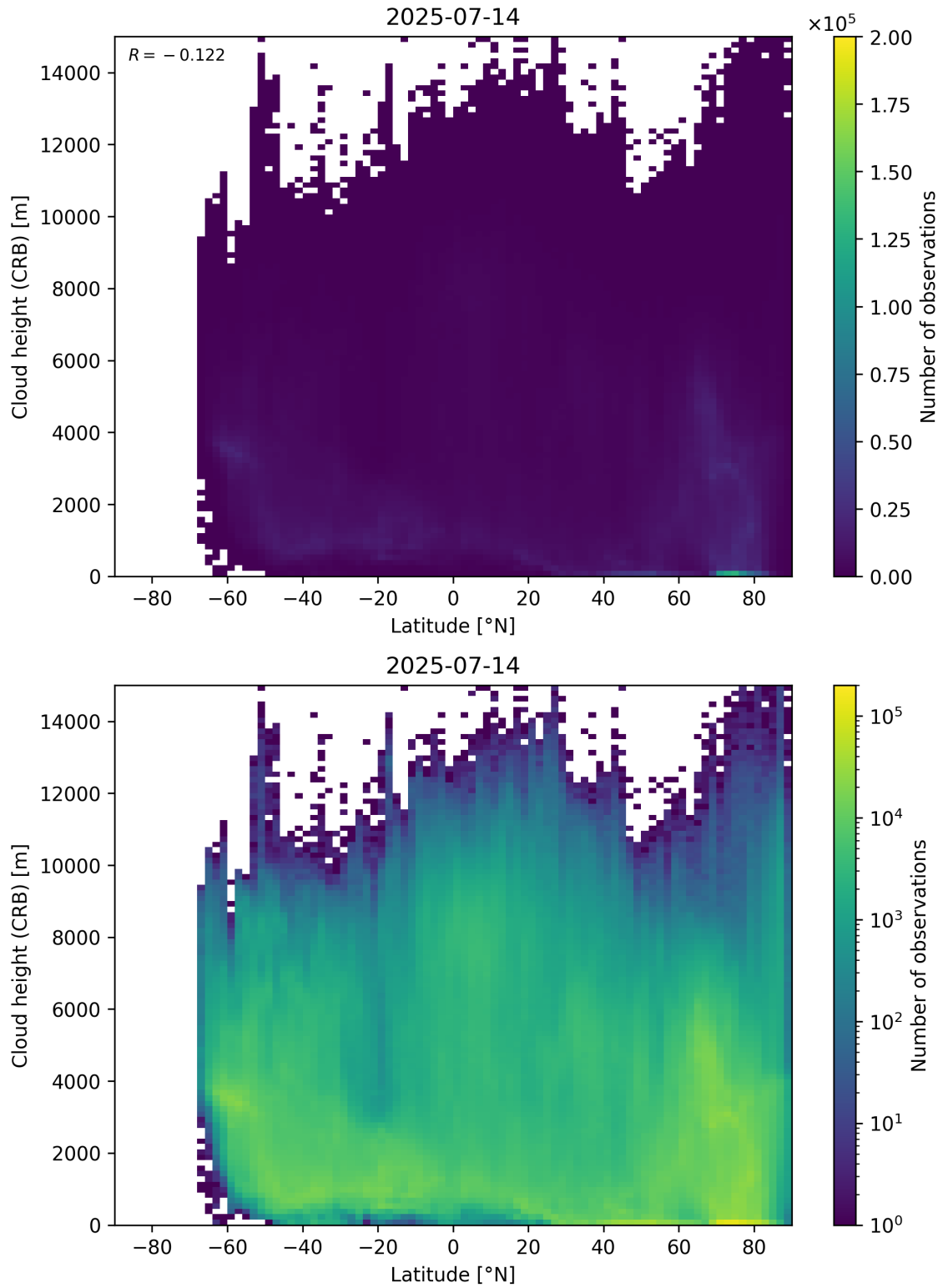
Figure 95: Scatter density plot of “Latitude” against “Cloud height (CRB)” for 2025-07-13 to 2025-07-15.
