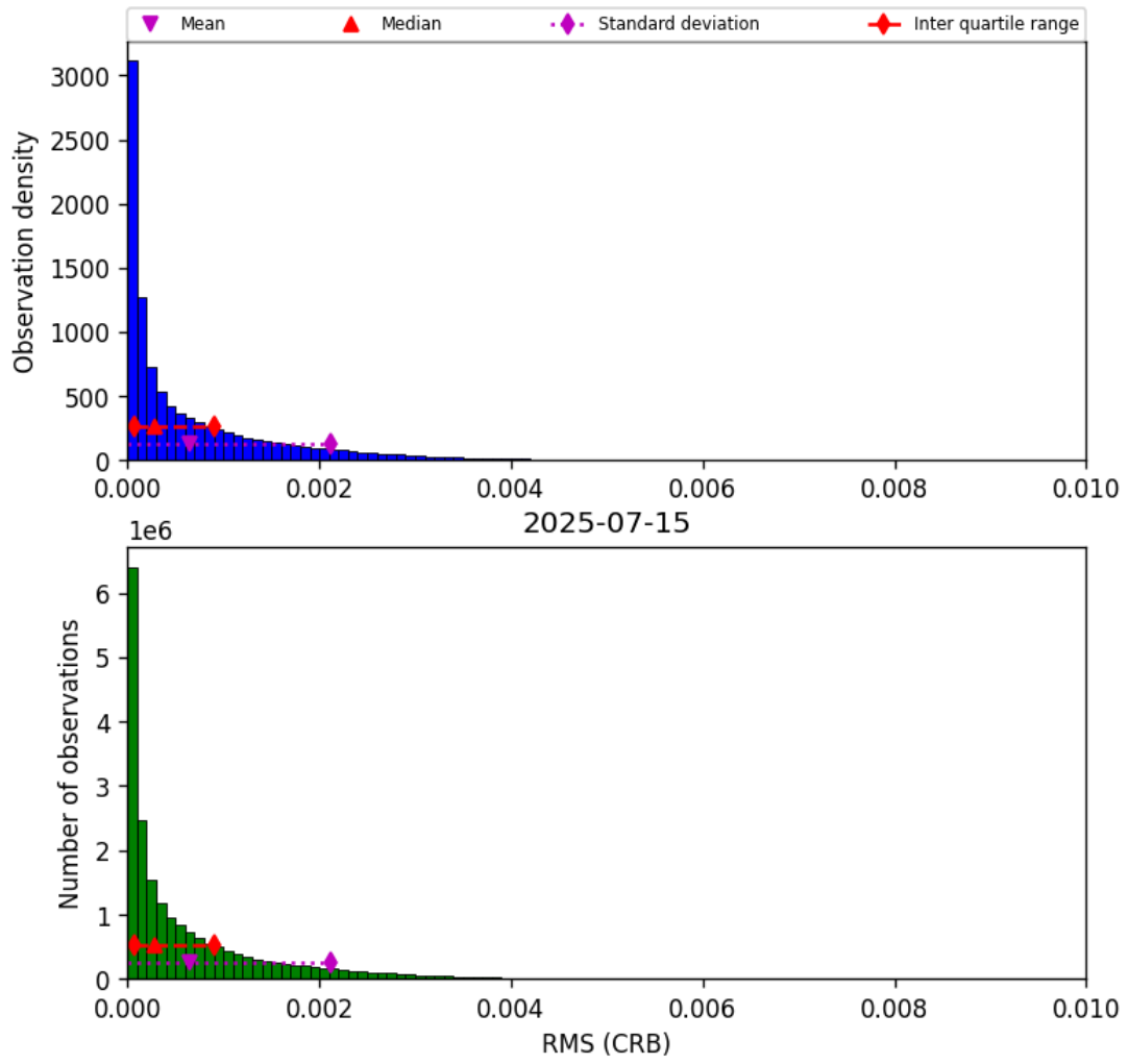
Figure 48: Histogram of “RMS (CRB)” for 2025-07-14 to 2025-07-16
