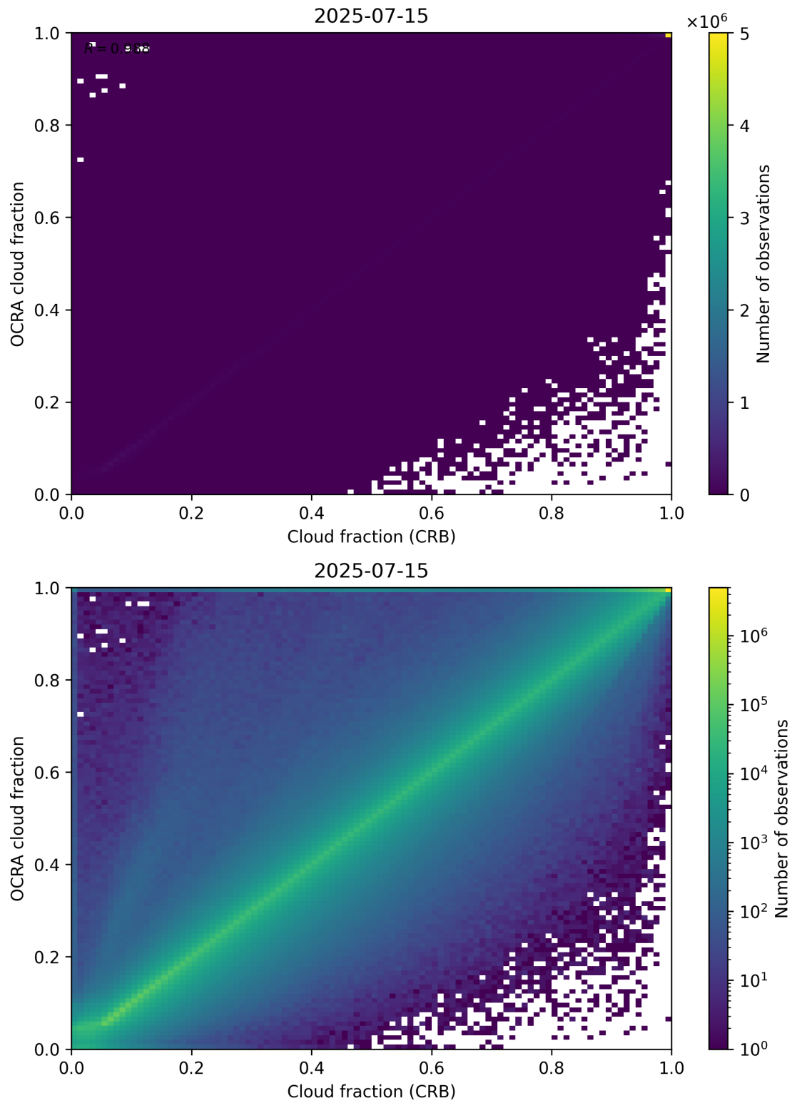
Figure 78: Scatter density plot of “Cloud fraction (CRB)” against “OCRA cloud fraction” for 2025-07-14 to 2025-07-16.
