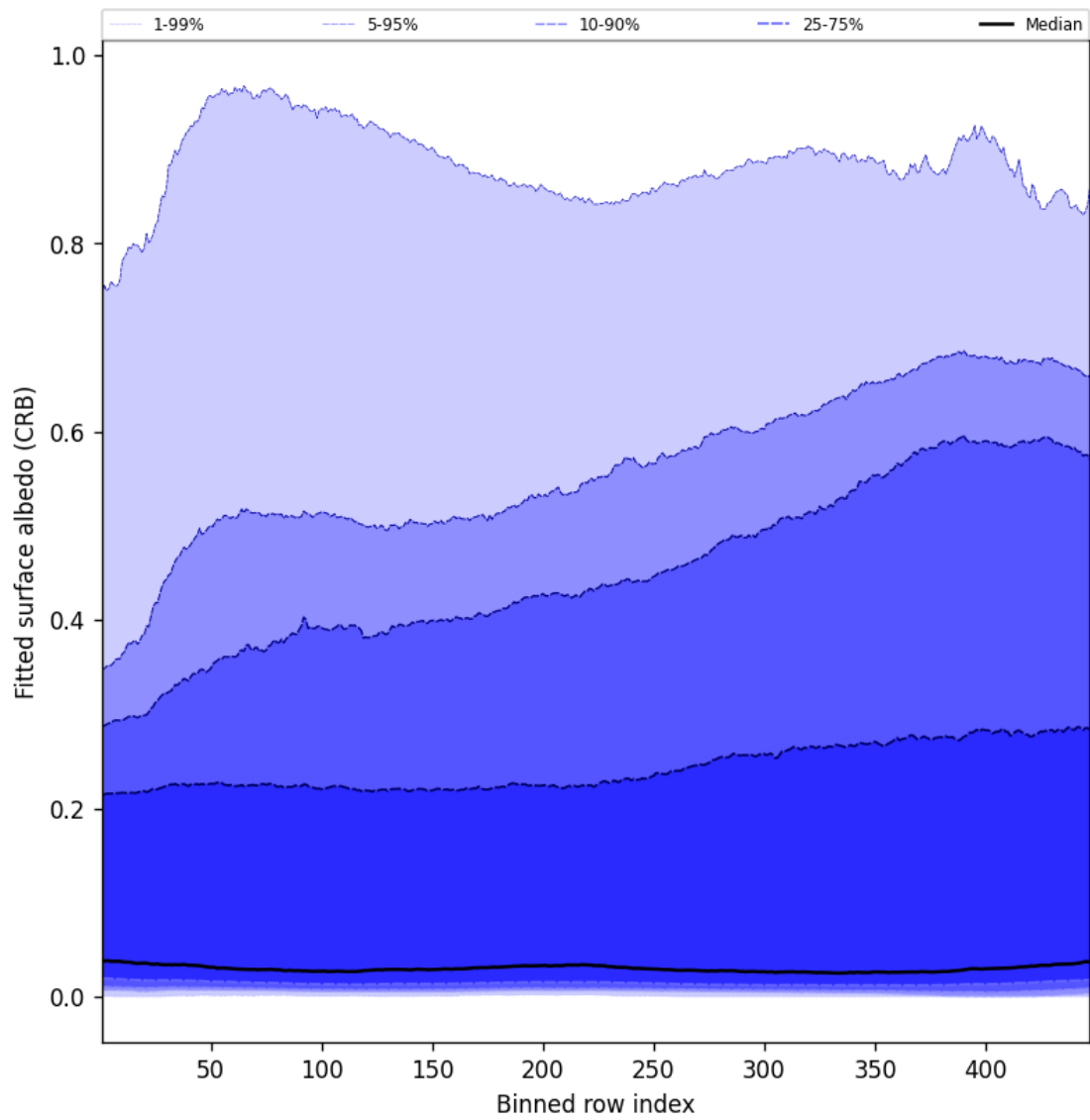
Figure 62: Along track statistics of “Fitted surface albedo (CRB)” for 2025-07-14 to 2025-07-16
