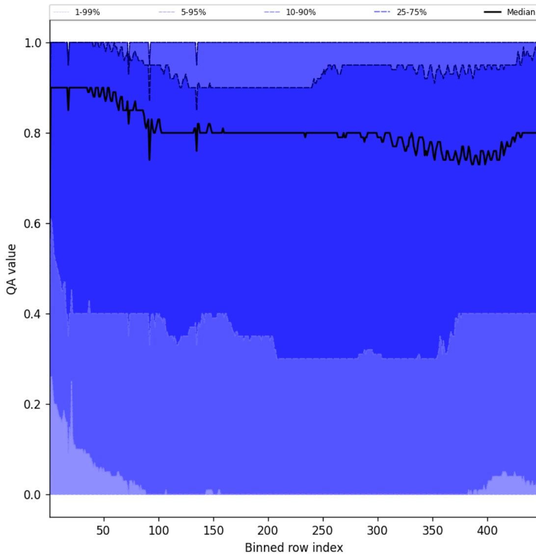
Figure 54: Along track statistics of “QA value” for 2025-07-14 to 2025-07-16
