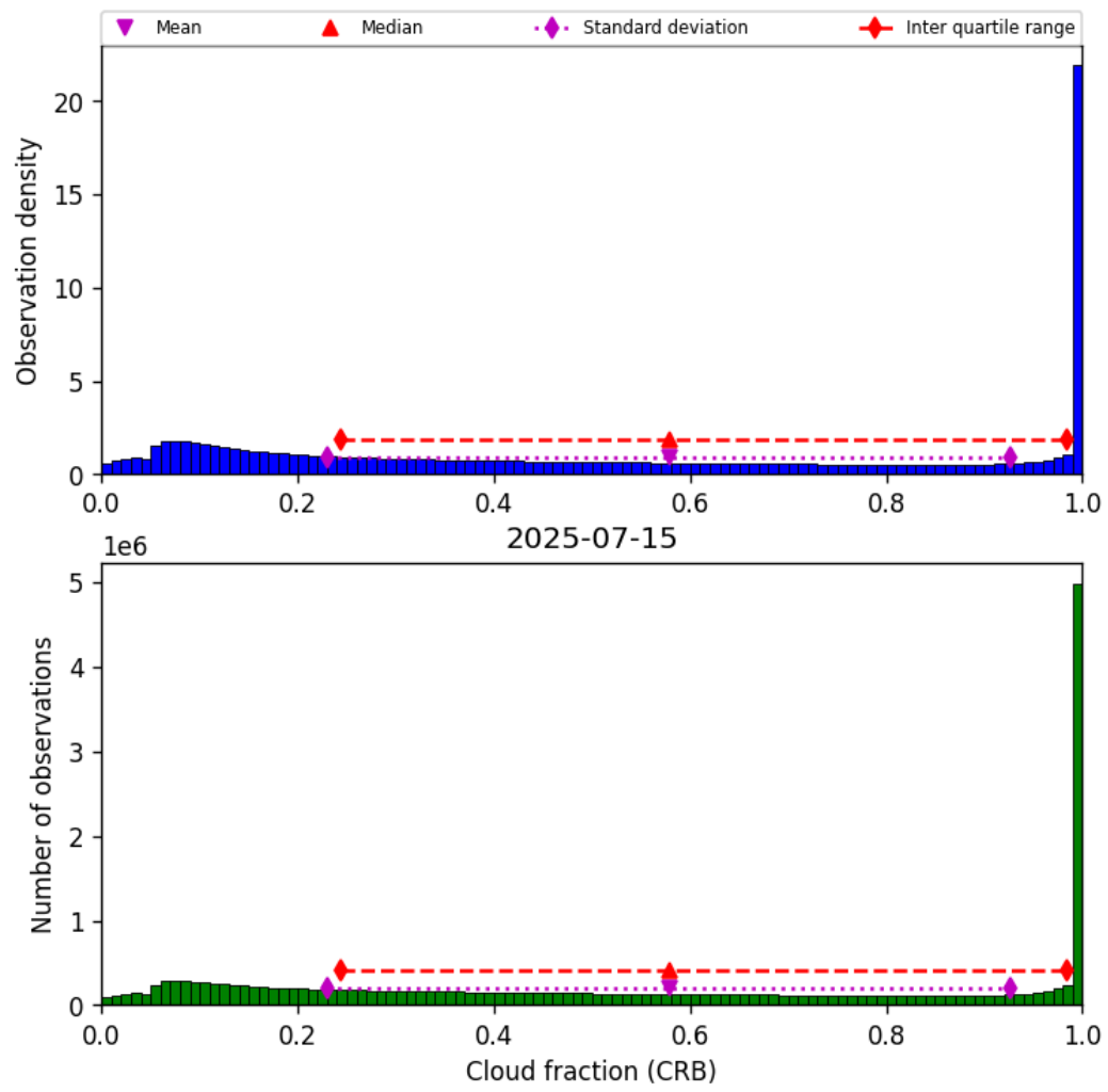
Figure 42: Histogram of “Cloud fraction (CRB)” for 2025-07-14 to 2025-07-16
