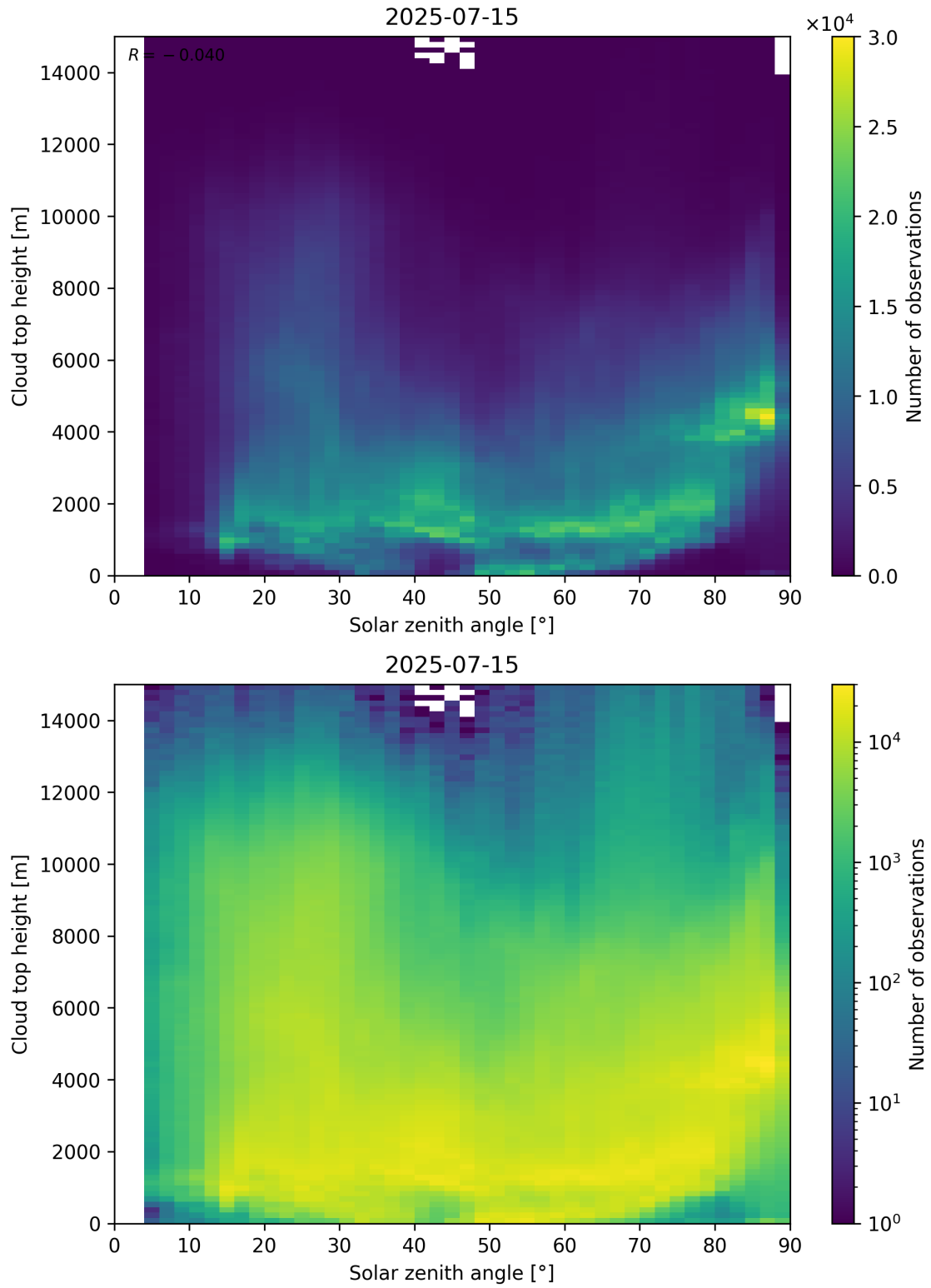
Figure 104: Scatter density plot of “Solar zenith angle” against “Cloud top height” for 2025-07-14 to 2025-07-16.
