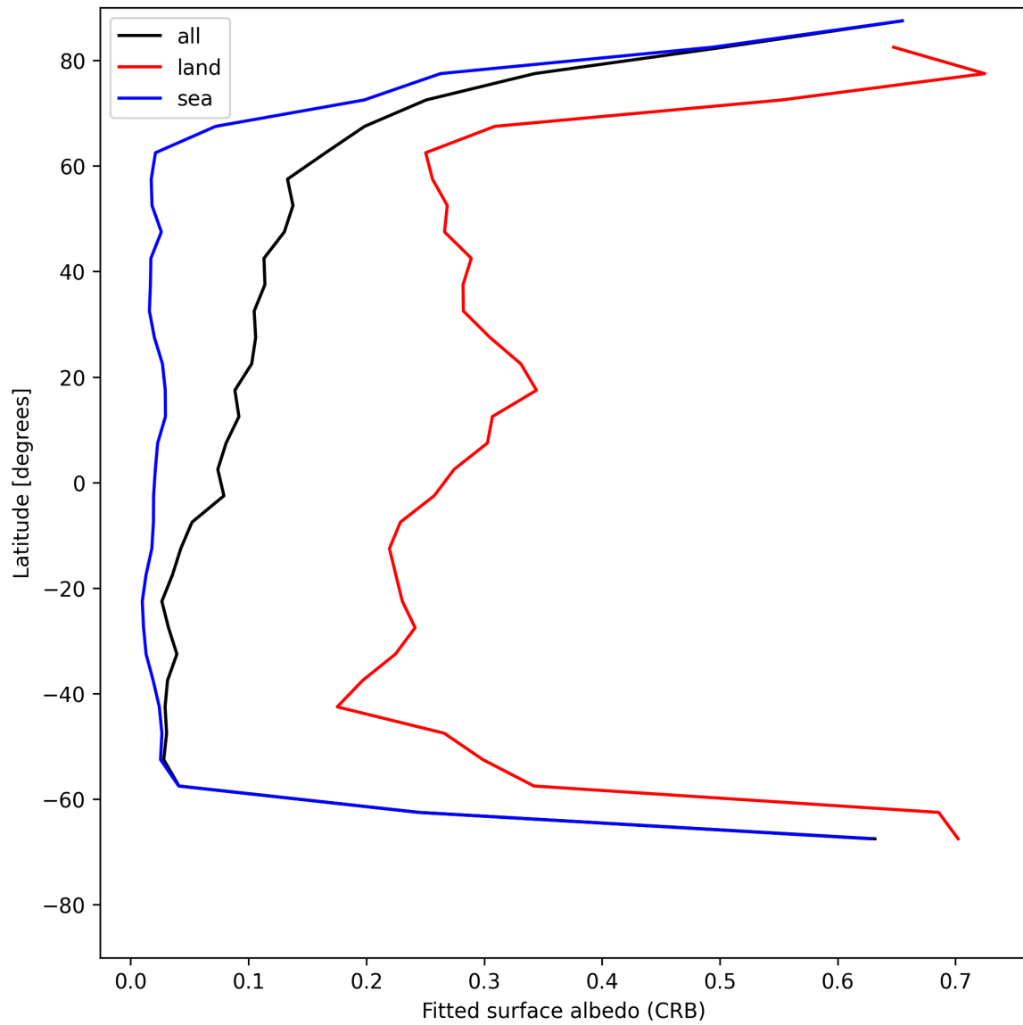
Figure 30: Zonal average of “Fitted surface albedo (CRB)” for 2025-07-14 to 2025-07-16.
