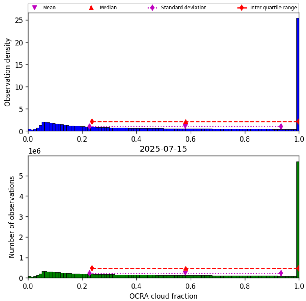
Figure 50: Histogram of “OCRA cloud fraction” for 2025-07-14 to 2025-07-16
