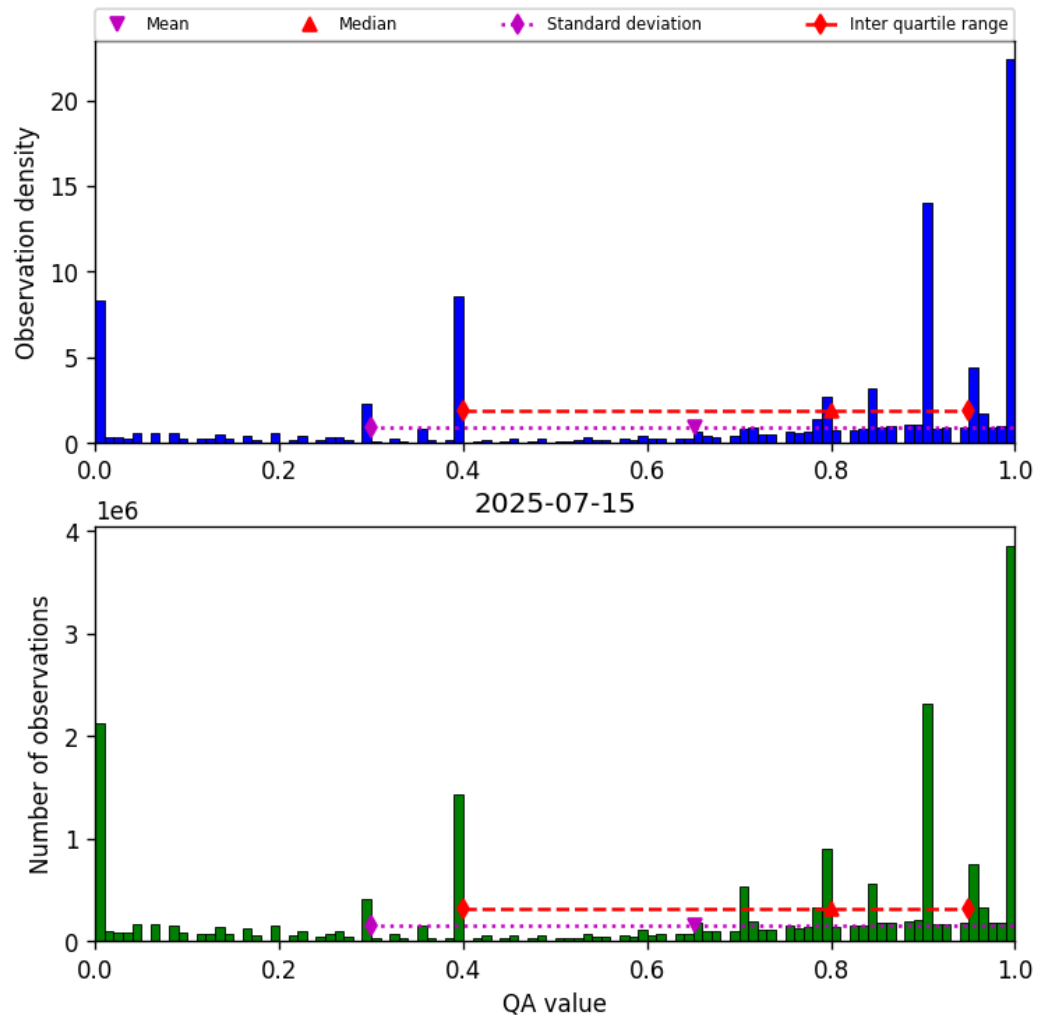
Figure 38: Histogram of “QA value” for 2025-07-14 to 2025-07-16
