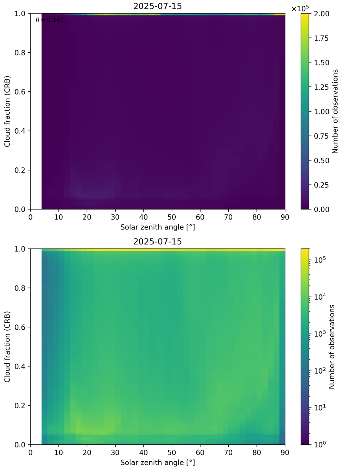
Figure 101: Scatter density plot of “Solar zenith angle” against “Cloud fraction (CRB)” for 2025-07-14 to 2025-07-16.
