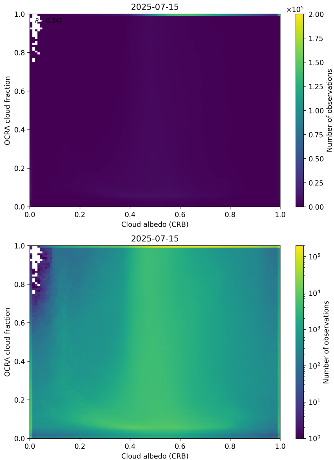
Figure 70: Scatter density plot of “Cloud albedo (CRB)” against “OCRA cloud fraction” for 2025-07-14 to 2025-07-16.
