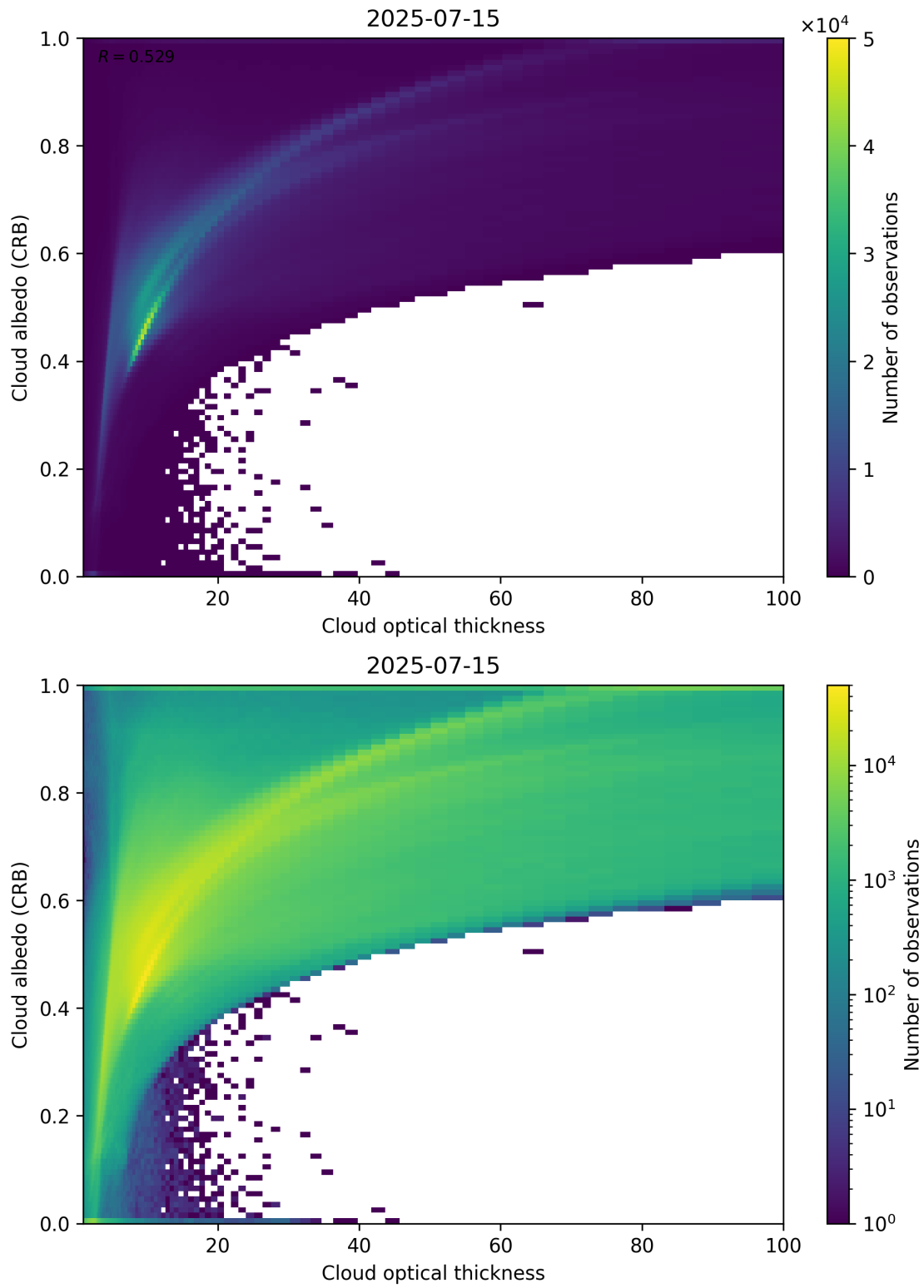
Figure 82: Scatter density plot of “Cloud optical thickness” against “Cloud albedo (CRB)” for 2025-07-14 to 2025-07-16.
