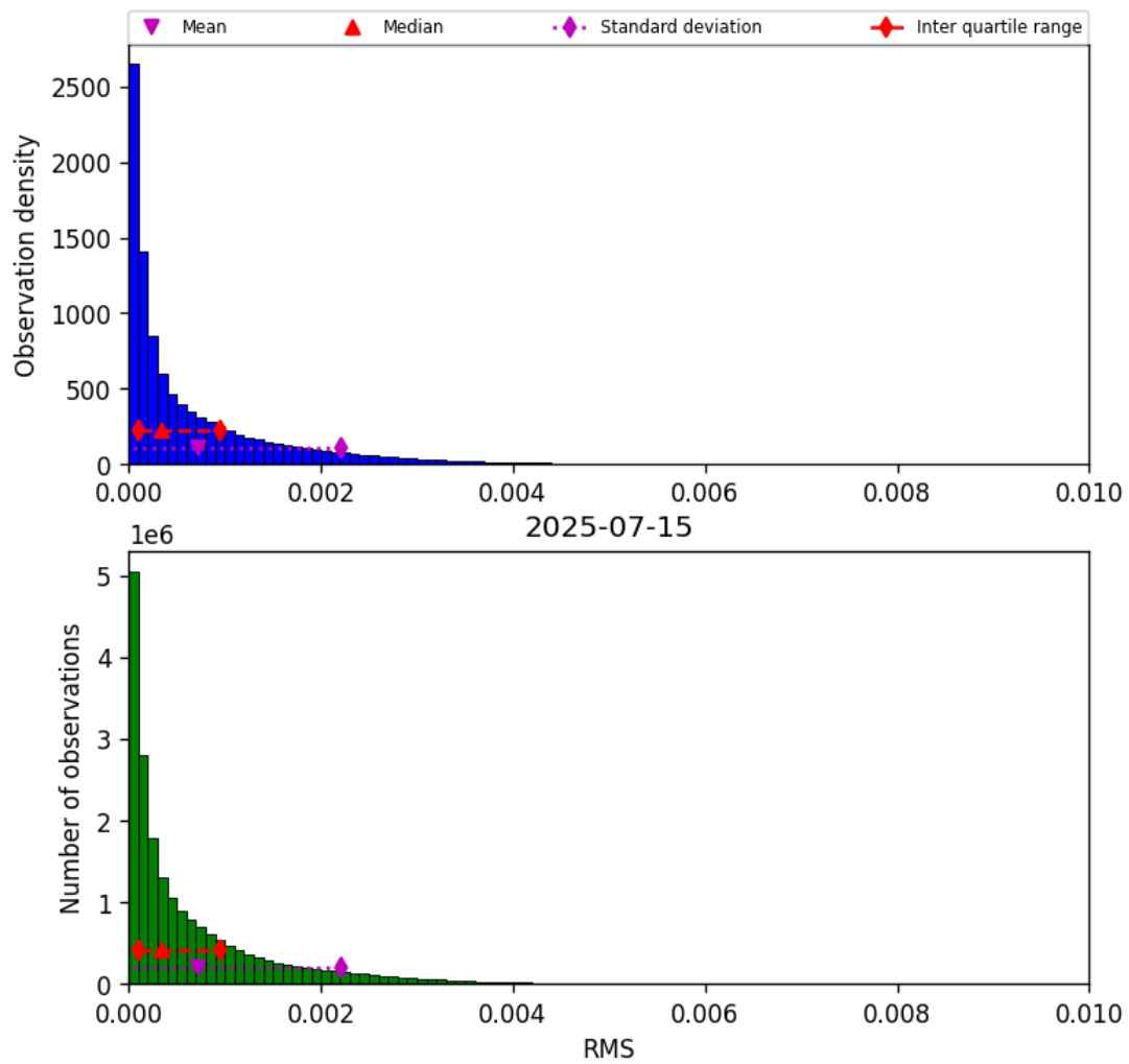
Figure 47: Histogram of “RMS” for 2025-07-14 to 2025-07-16
