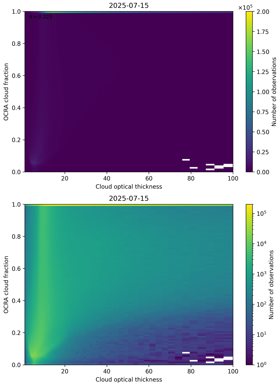
Figure 83: Scatter density plot of “Cloud optical thickness” against “OCRA cloud fraction” for 2025-07-14 to 2025-07-16.
