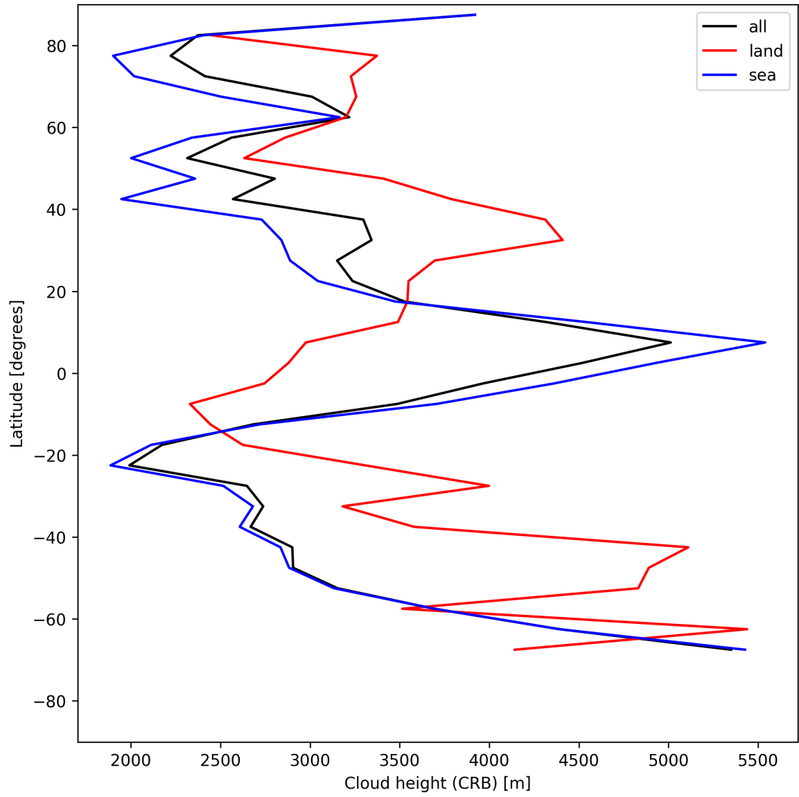
Figure 27: Zonal average of “Cloud height (CRB)” for 2025-07-14 to 2025-07-16.
