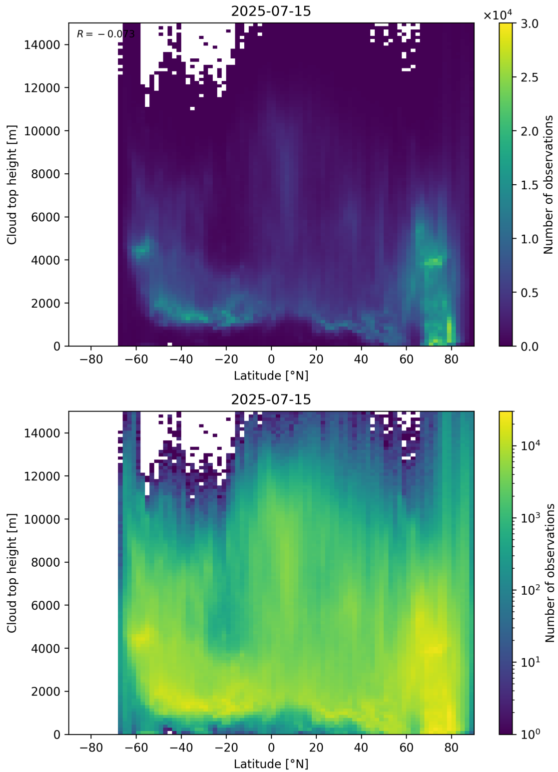
Figure 97: Scatter density plot of “Latitude” against “Cloud top height” for 2025-07-14 to 2025-07-16.
