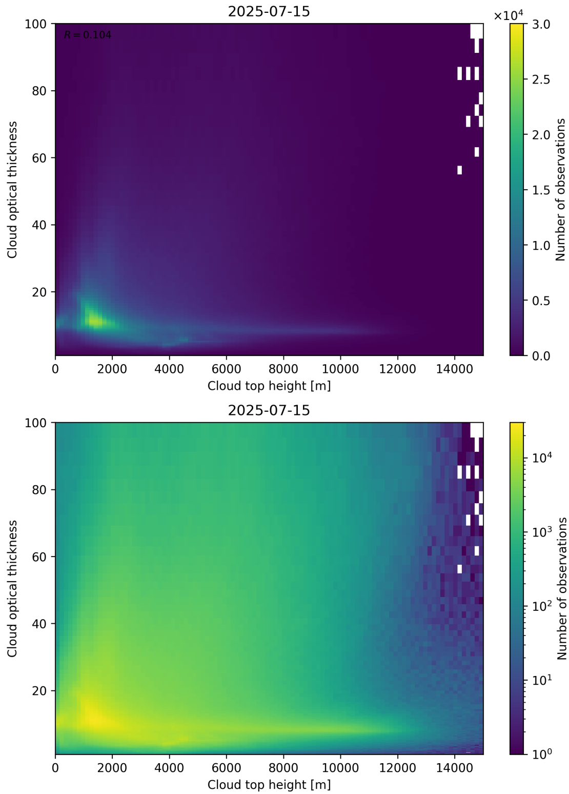
Figure 90: Scatter density plot of “Cloud top height” against “Cloud optical thickness” for 2025-07-14 to 2025-07-16.
