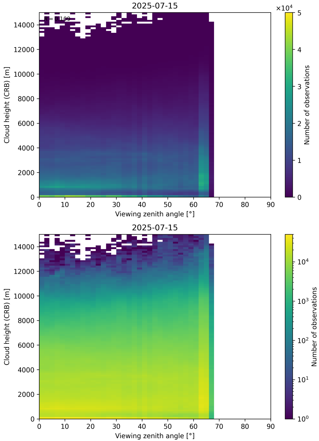
Figure 110: Scatter density plot of “Viewing zenith angle” against “Cloud height (CRB)” for 2025-07-14 to 2025-07-16.
