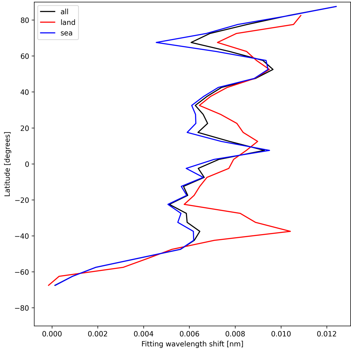
Figure 33: Zonal average of “Fitting wavelength shift” for 2025-07-14 to 2025-07-16.
