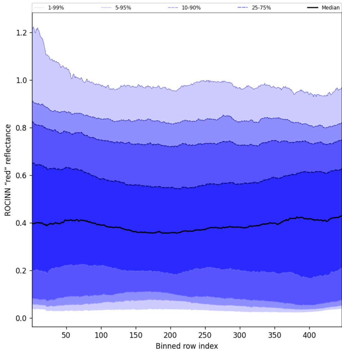
Figure 69: Along track statistics of “ROCINN “red” reflectance” for 2025-07-14 to 2025-07-16
