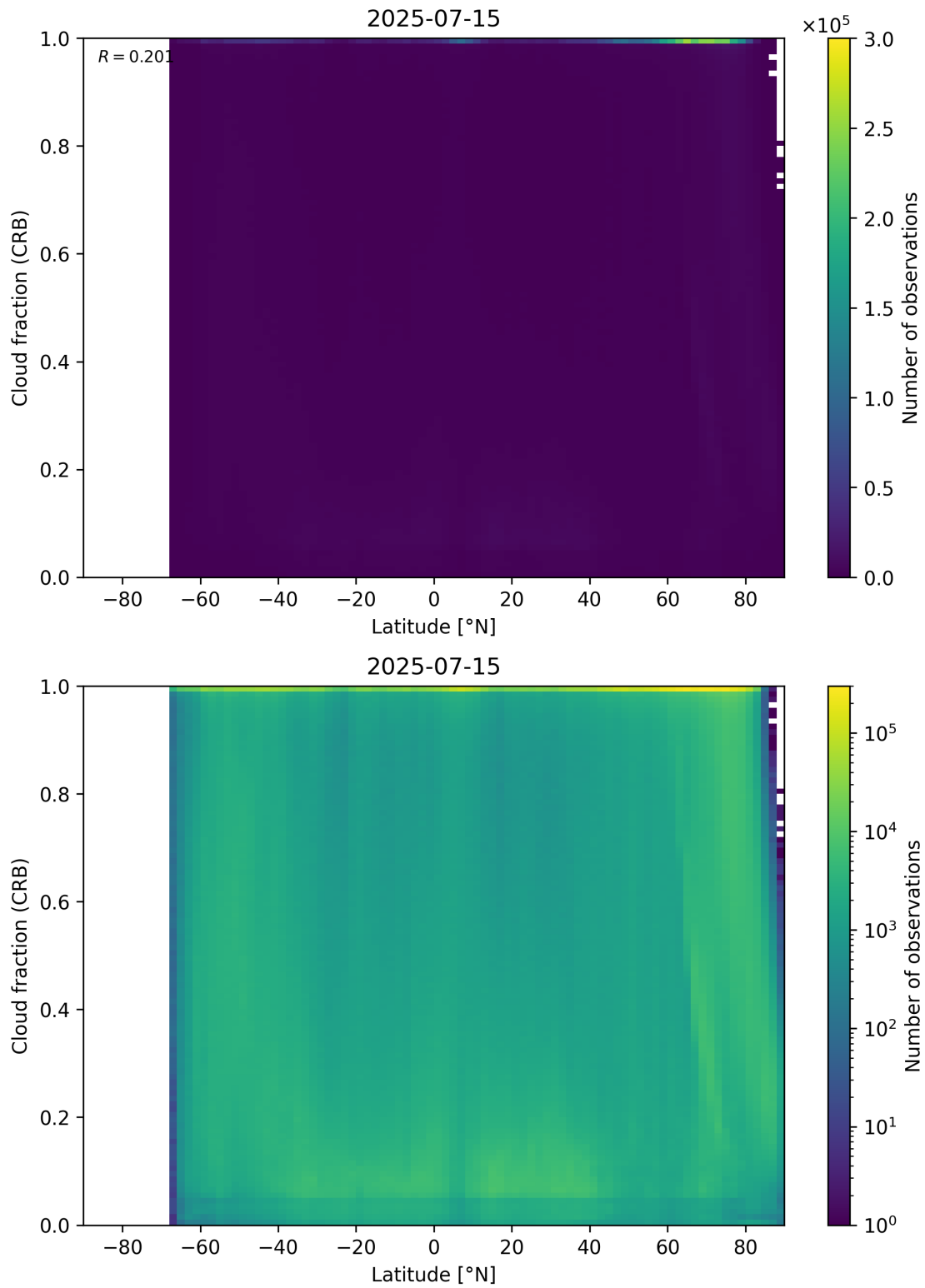
Figure 94: Scatter density plot of “Latitude” against “Cloud fraction (CRB)” for 2025-07-14 to 2025-07-16.
