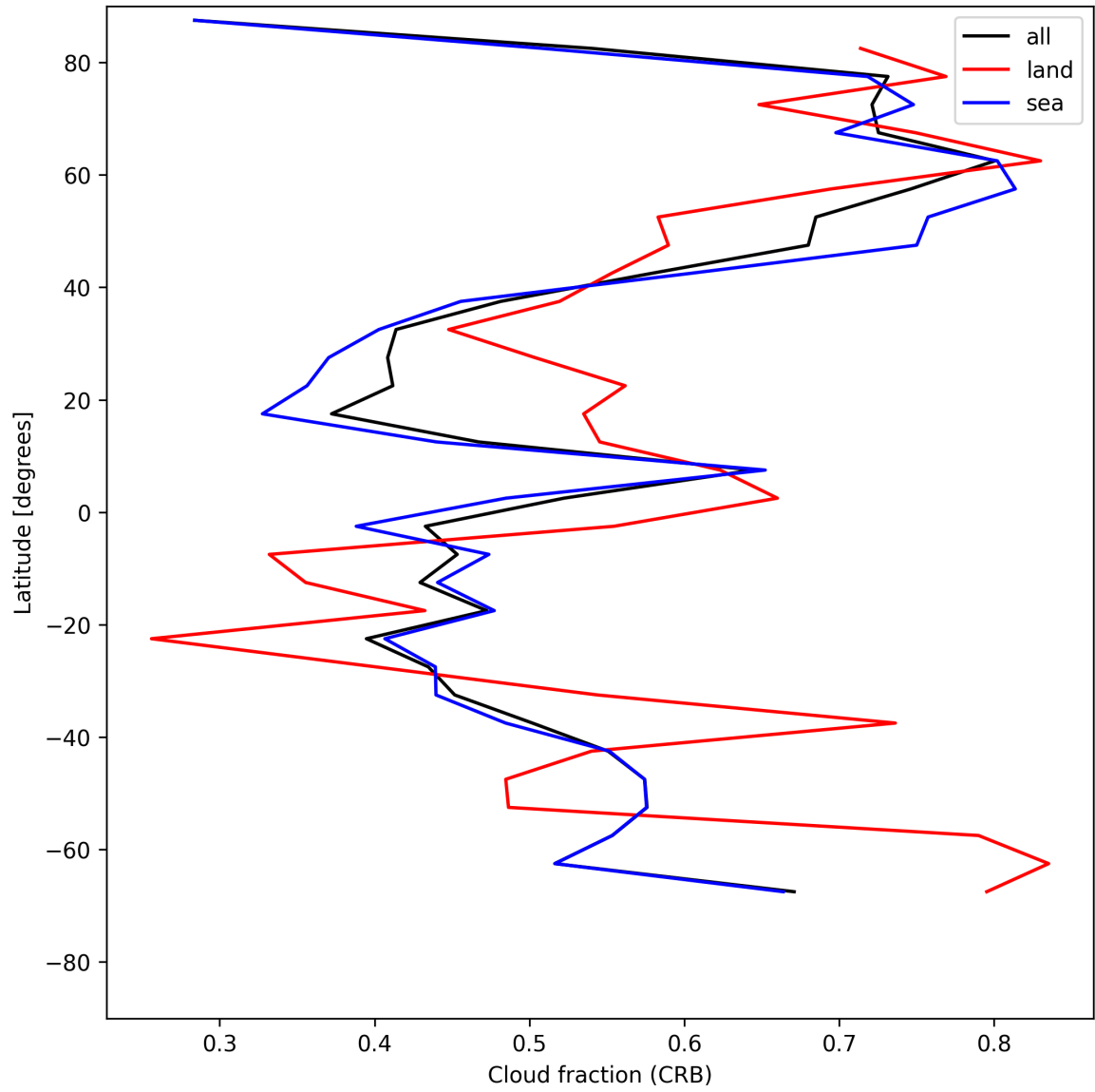
Figure 26: Zonal average of “Cloud fraction (CRB)” for 2025-07-14 to 2025-07-16.
