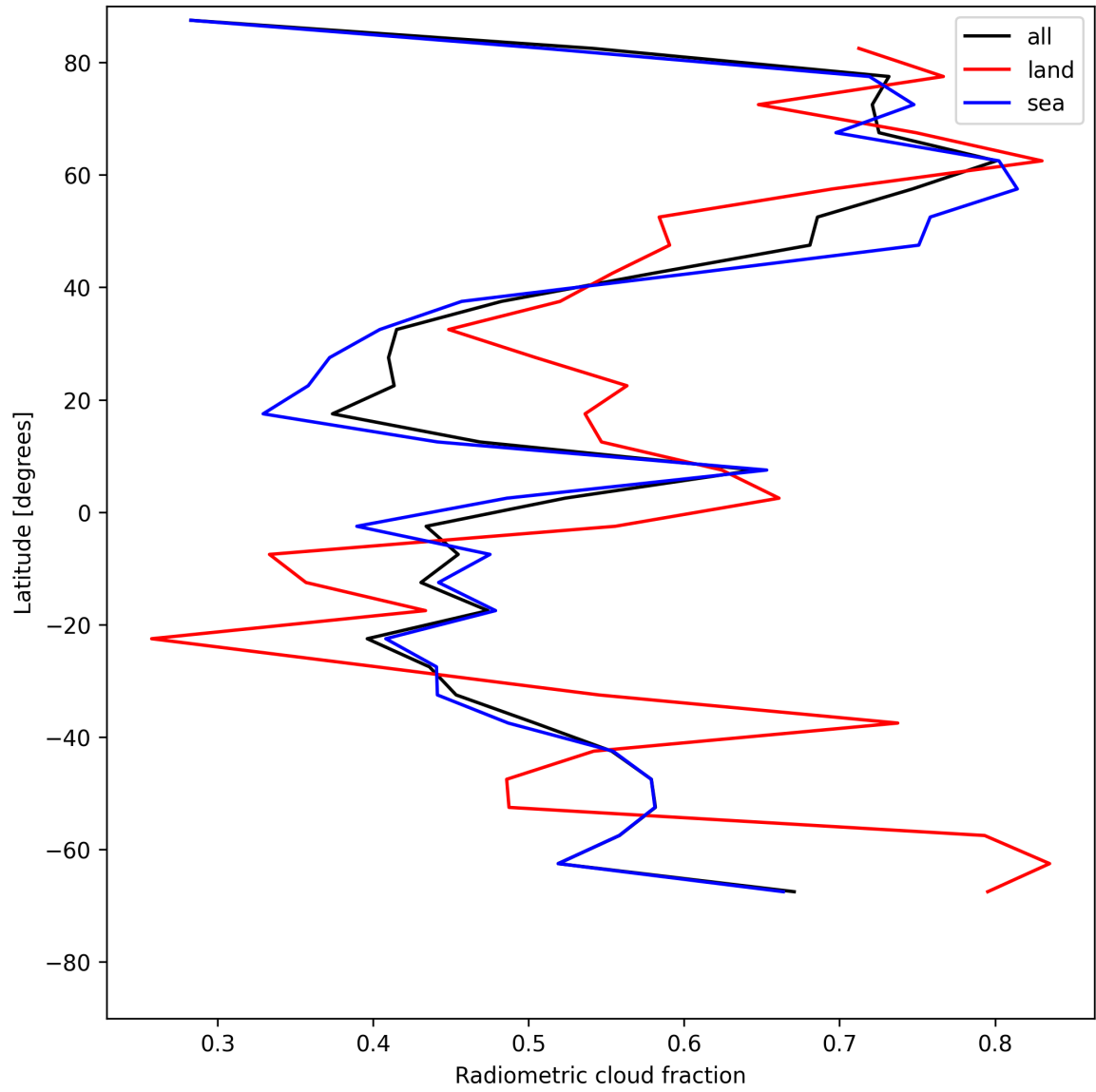
Figure 23: Zonal average of “Radiometric cloud fraction” for 2025-07-14 to 2025-07-16.
