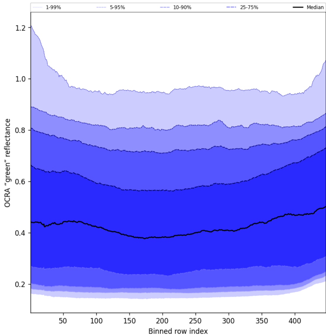
Figure 68: Along track statistics of “OCRA “green” reflectance” for 2025-07-14 to 2025-07-16
