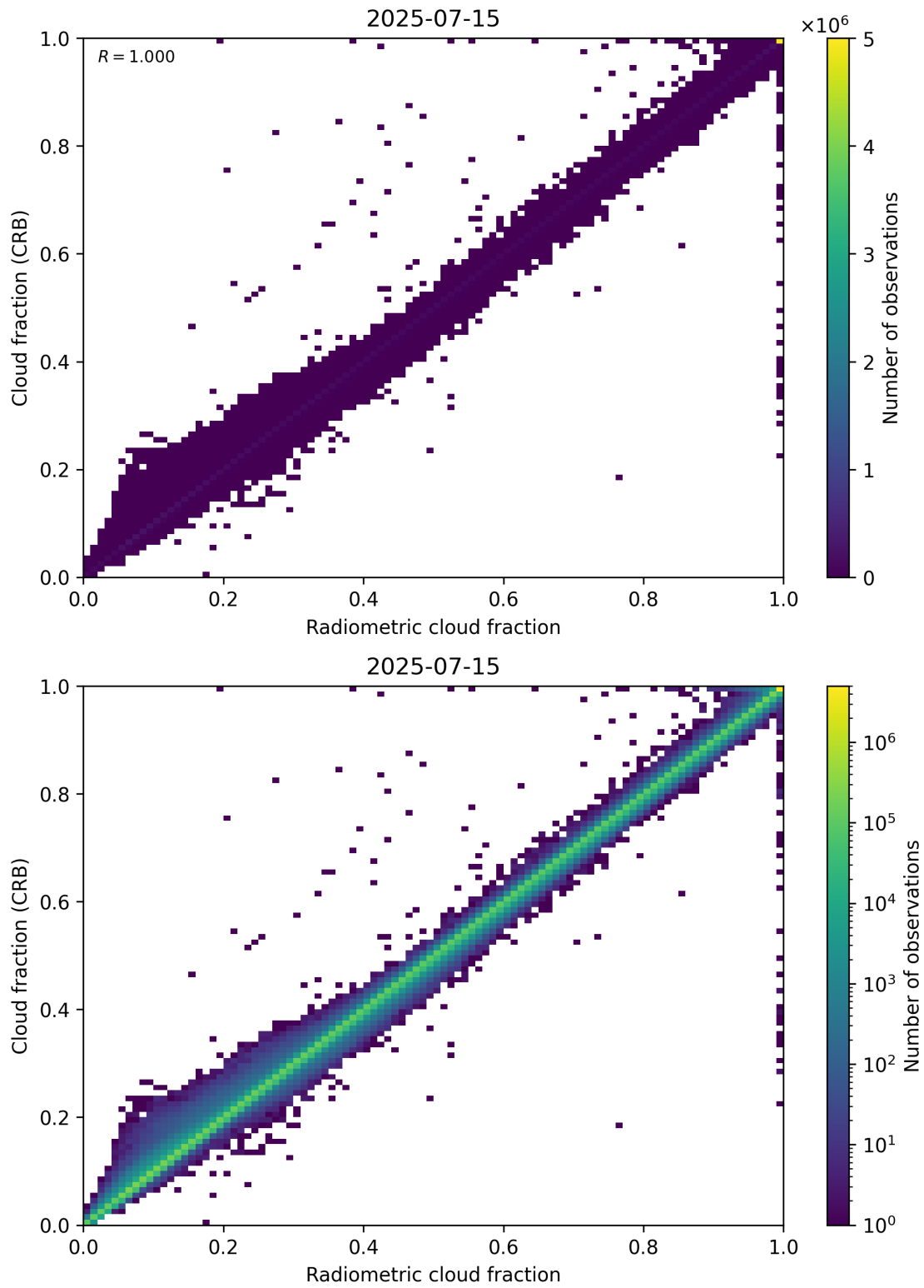
Figure 73: Scatter density plot of “Radiometric cloud fraction” against “Cloud fraction (CRB)” for 2025-07-14 to 2025-07-16.
