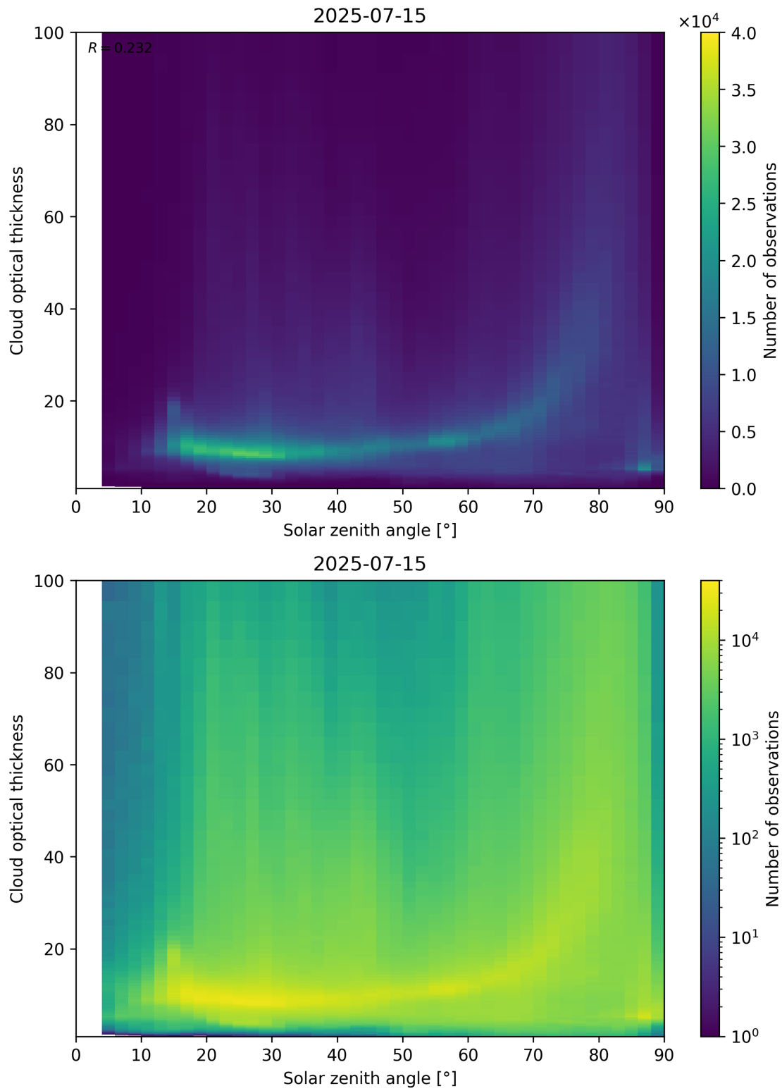
Figure 103: Scatter density plot of “Solar zenith angle” against “Cloud optical thickness” for 2025-07-14 to 2025-07-16.
