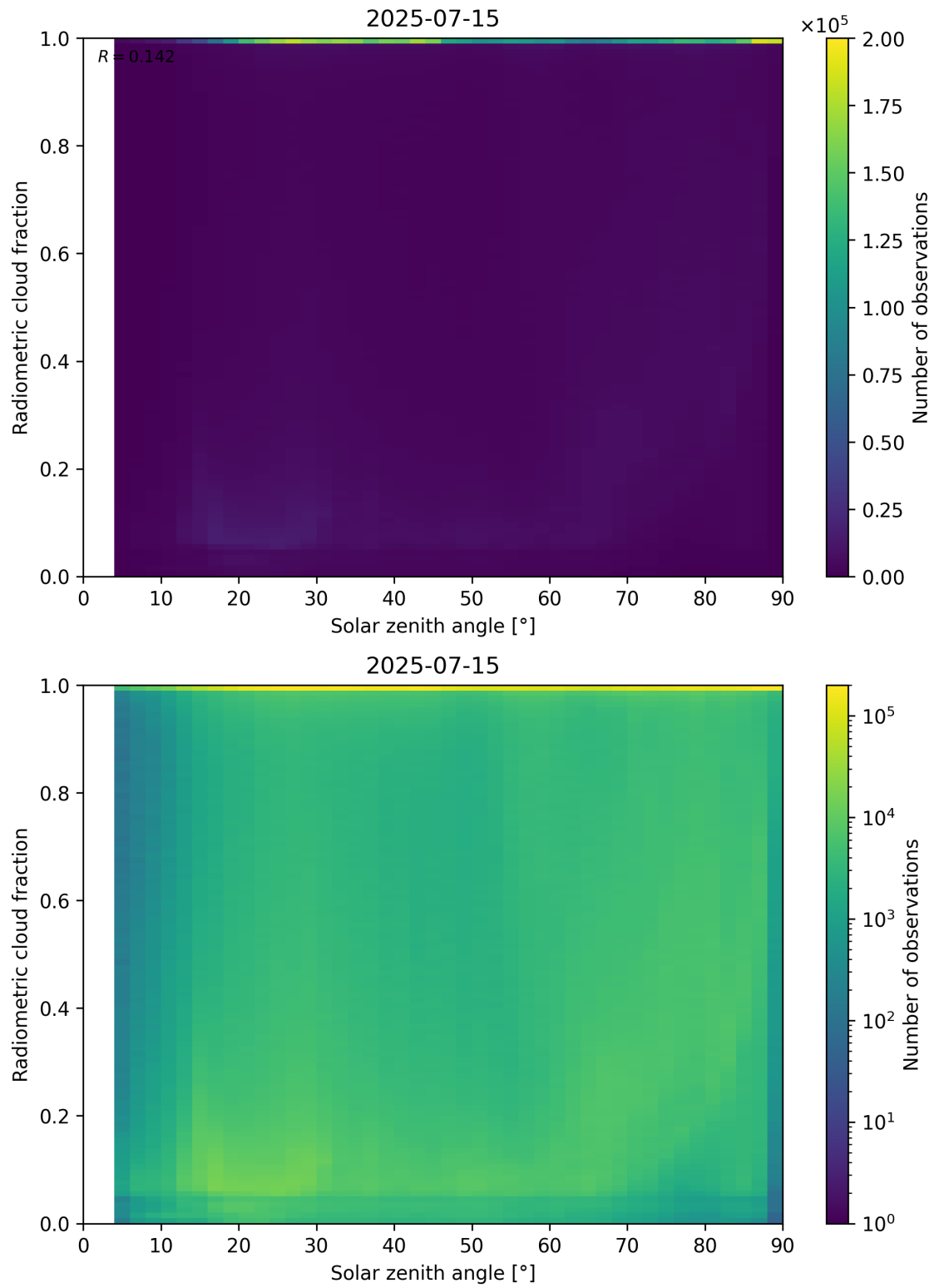
Figure 99: Scatter density plot of “Solar zenith angle” against “Radiometric cloud fraction” for 2025-07-14 to 2025-07-16.
