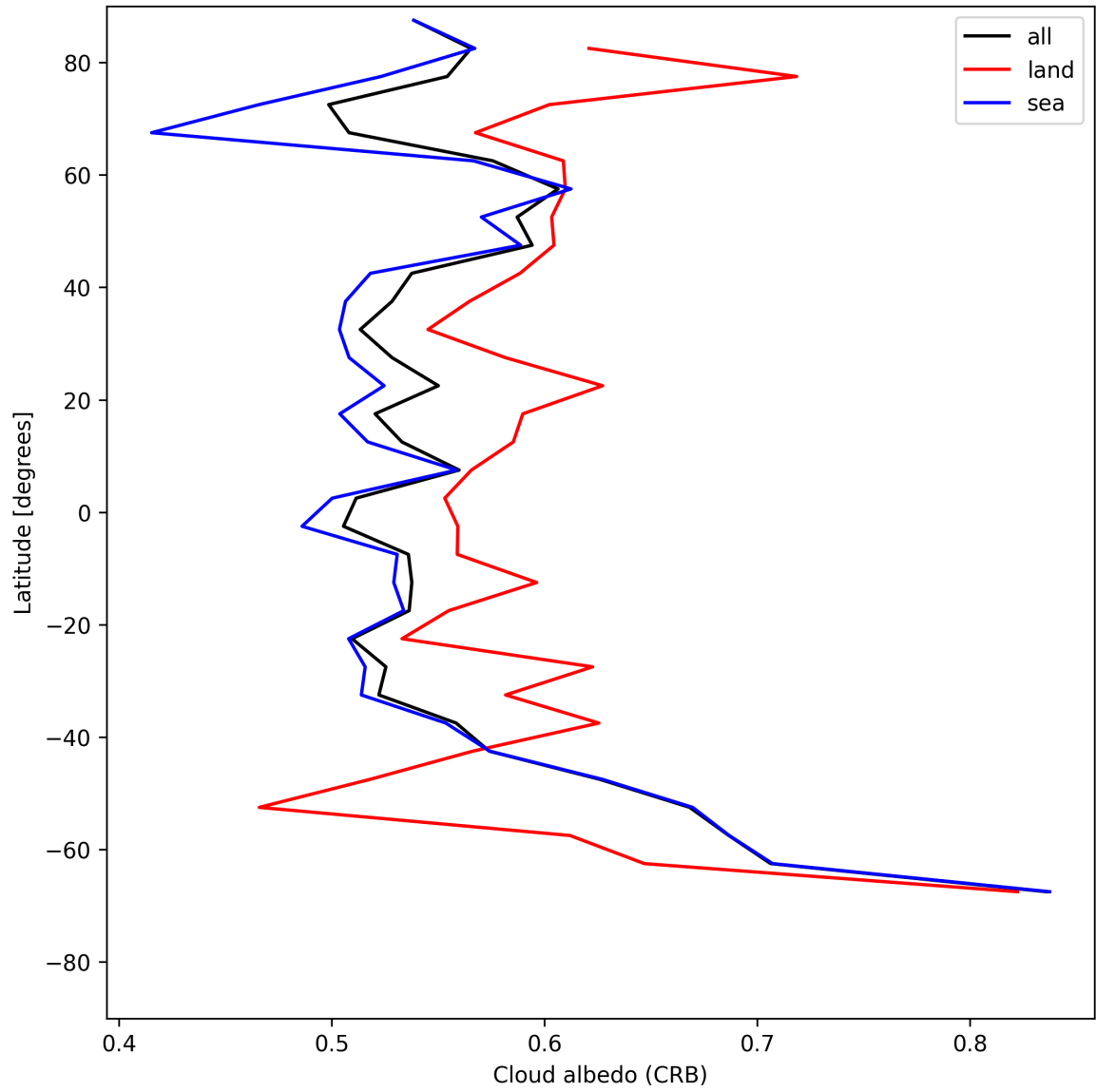
Figure 28: Zonal average of “Cloud albedo (CRB)” for 2025-07-14 to 2025-07-16.
