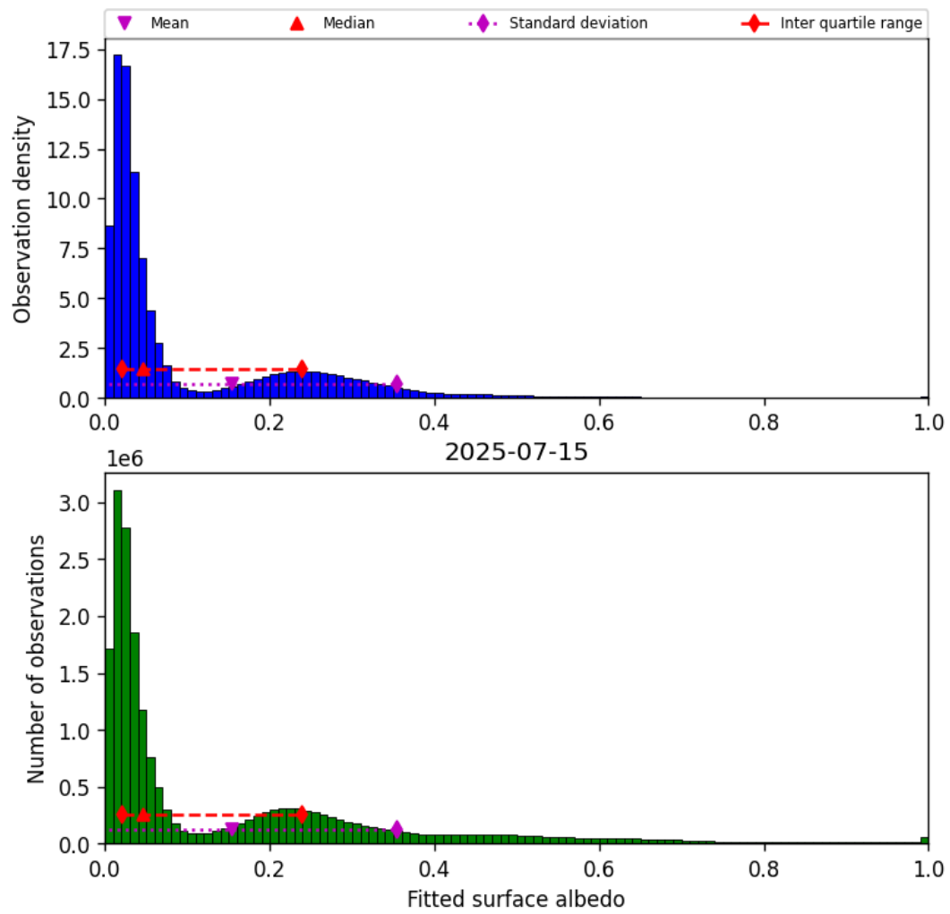
Figure 45: Histogram of “Fitted surface albedo” for 2025-07-14 to 2025-07-16
