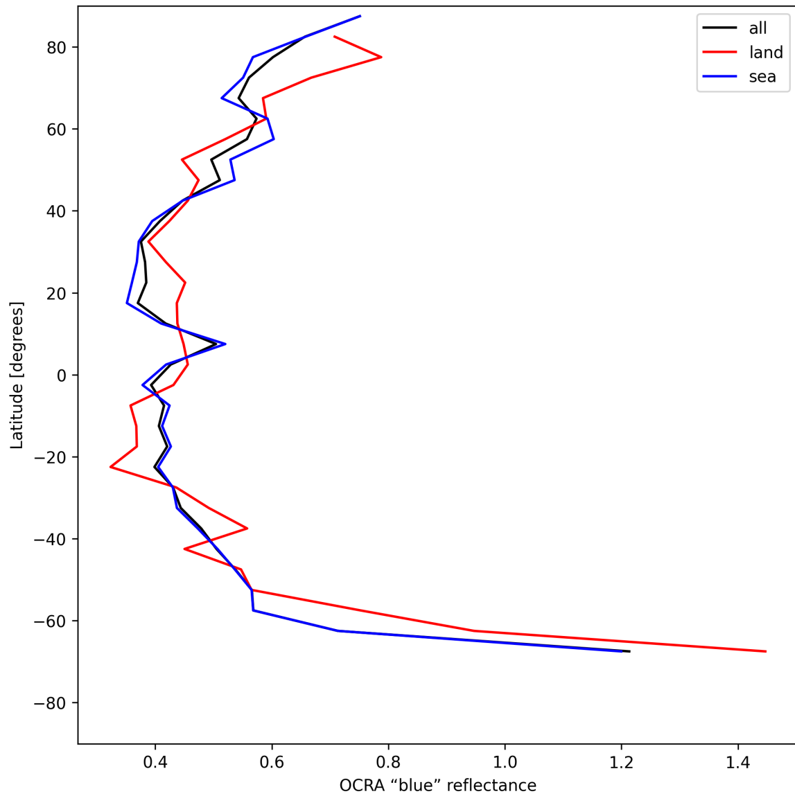
Figure 35: Zonal average of “OCRA “blue” reflectance” for 2025-07-14 to 2025-07-16.
