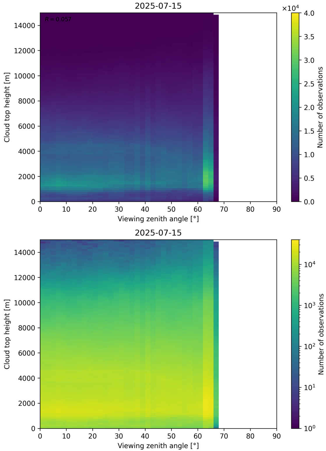
Figure 112: Scatter density plot of “Viewing zenith angle” against “Cloud top height” for 2025-07-14 to 2025-07-16.
