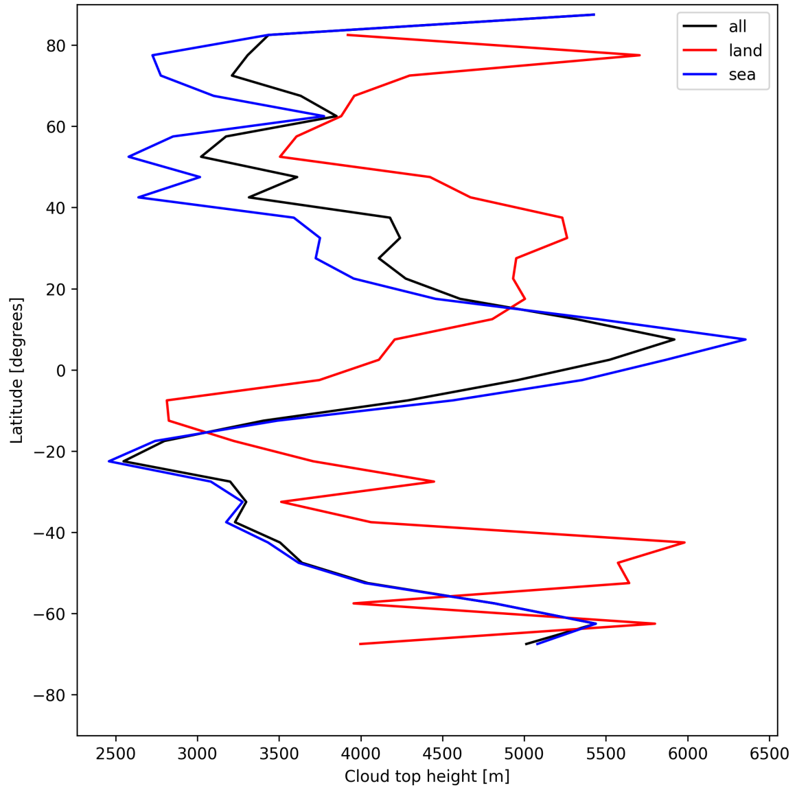
Figure 24: Zonal average of “Cloud top height” for 2025-07-14 to 2025-07-16.
