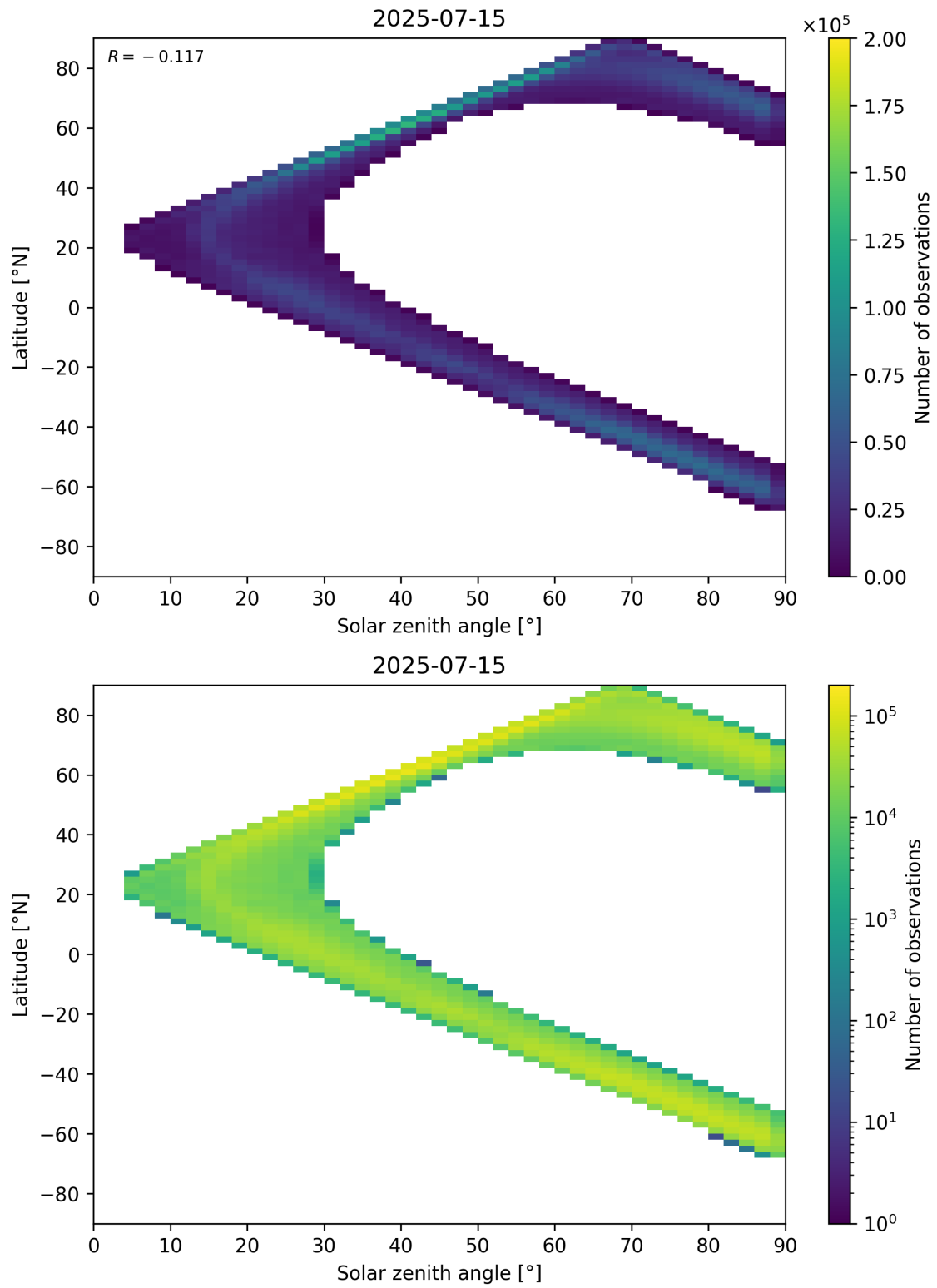
Figure 105: Scatter density plot of “Solar zenith angle” against “Latitude” for 2025-07-14 to 2025-07-16.
