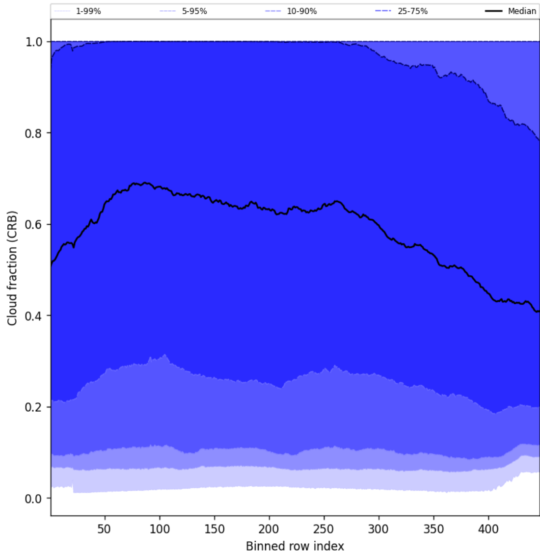
Figure 58: Along track statistics of “Cloud fraction (CRB)” for 2025-07-14 to 2025-07-16
