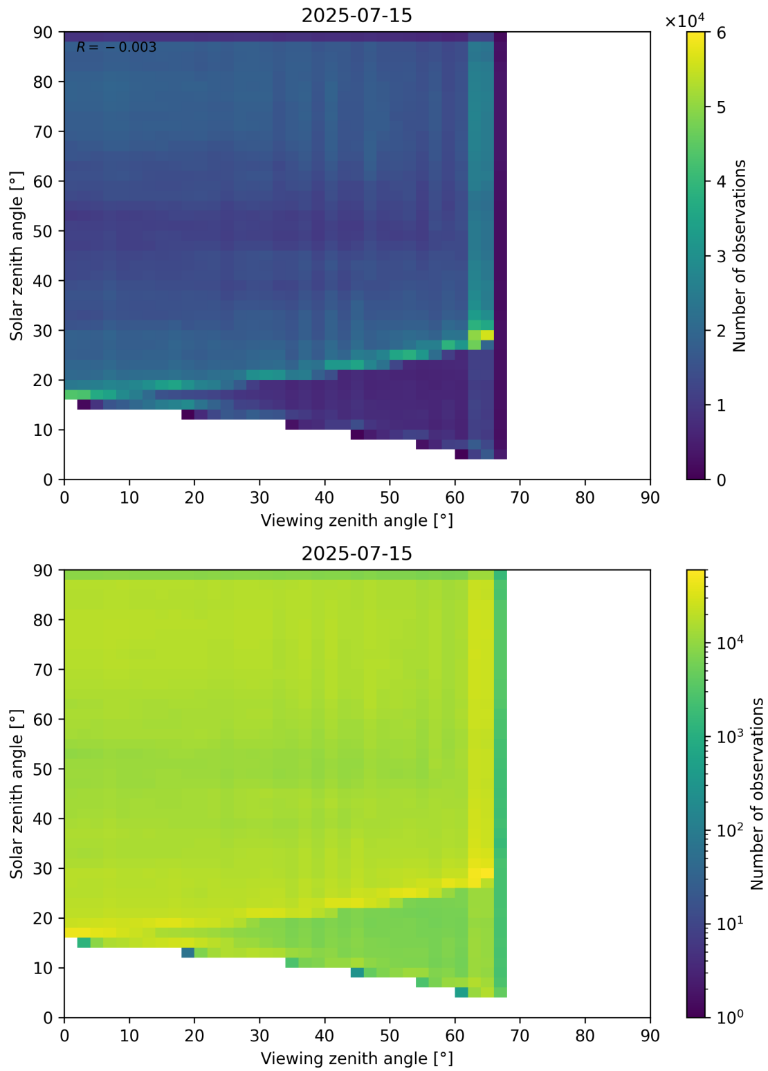
Figure 114: Scatter density plot of “Viewing zenith angle” against “Solar zenith angle” for 2025-07-14 to 2025-07-16.
