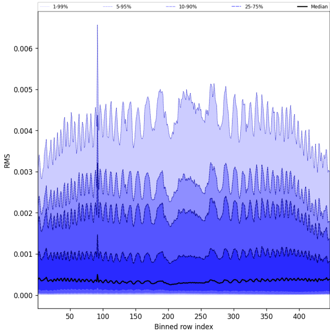
Figure 63: Along track statistics of “RMS” for 2025-07-14 to 2025-07-16
