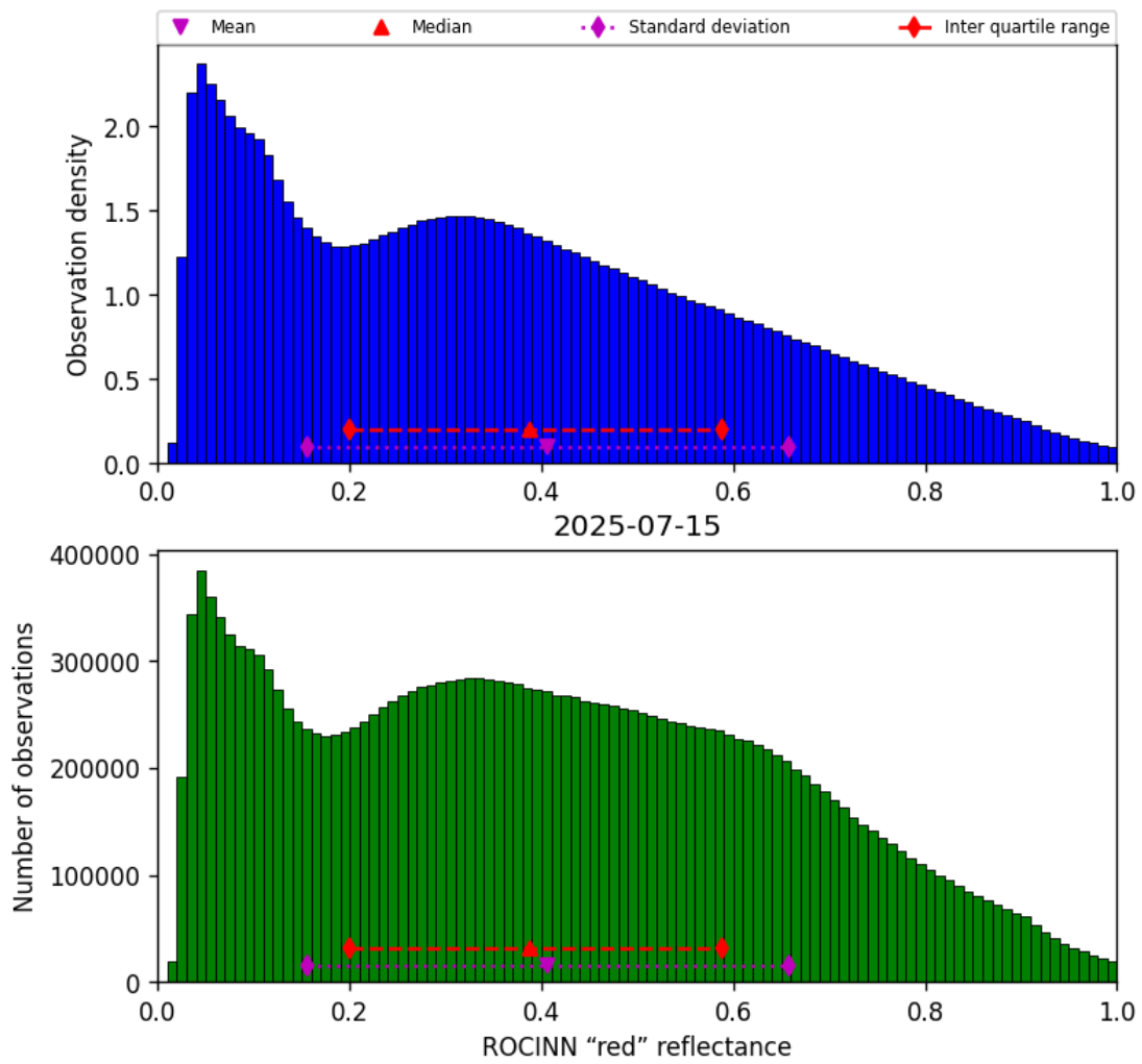
Figure 53: Histogram of “ROCINN “red” reflectance” for 2025-07-14 to 2025-07-16
