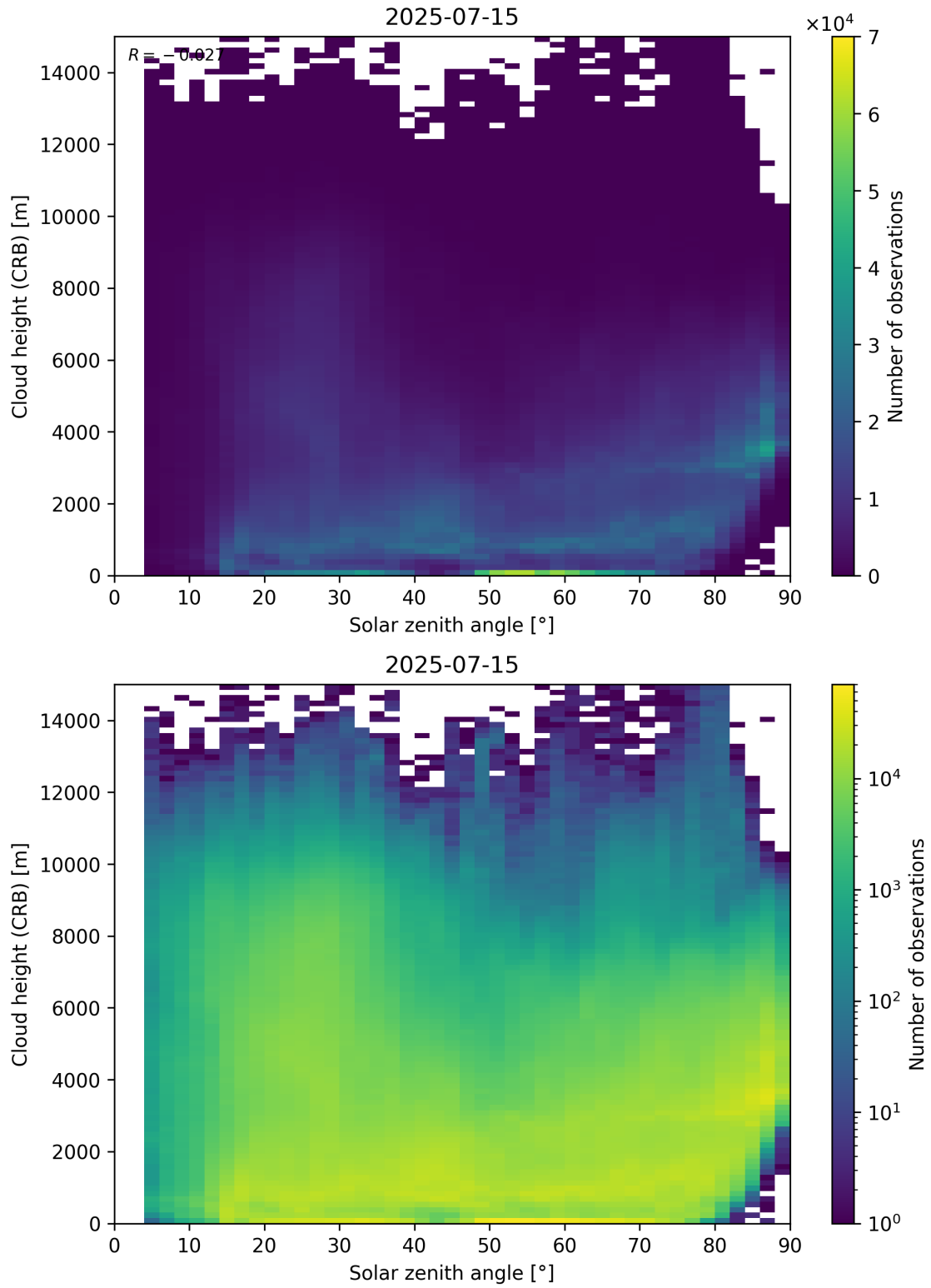
Figure 102: Scatter density plot of “Solar zenith angle” against “Cloud height (CRB)” for 2025-07-14 to 2025-07-16.
