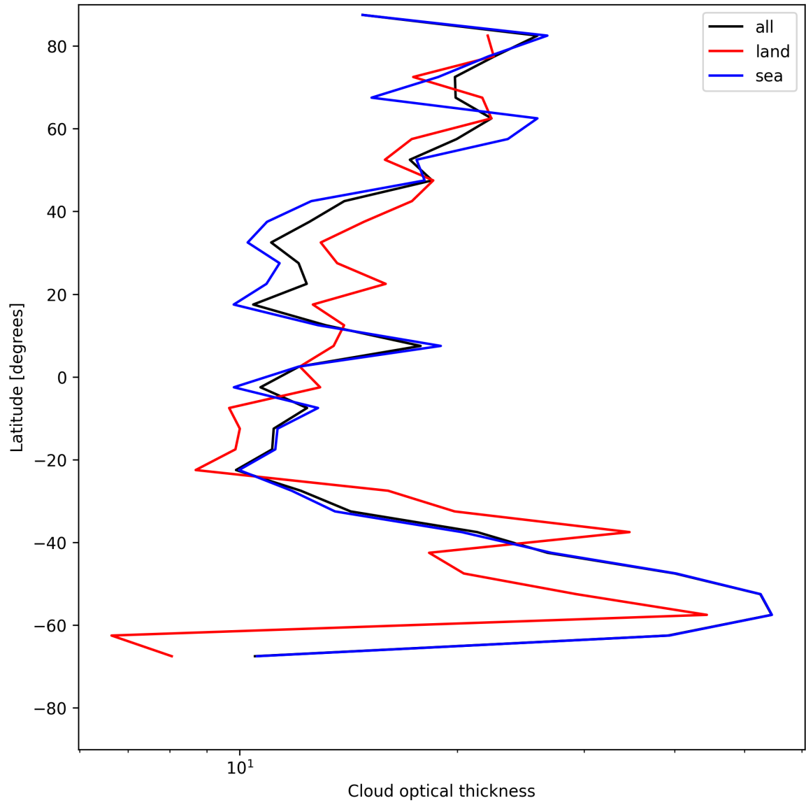
Figure 25: Zonal average of “Cloud optical thickness” for 2025-07-14 to 2025-07-16.
