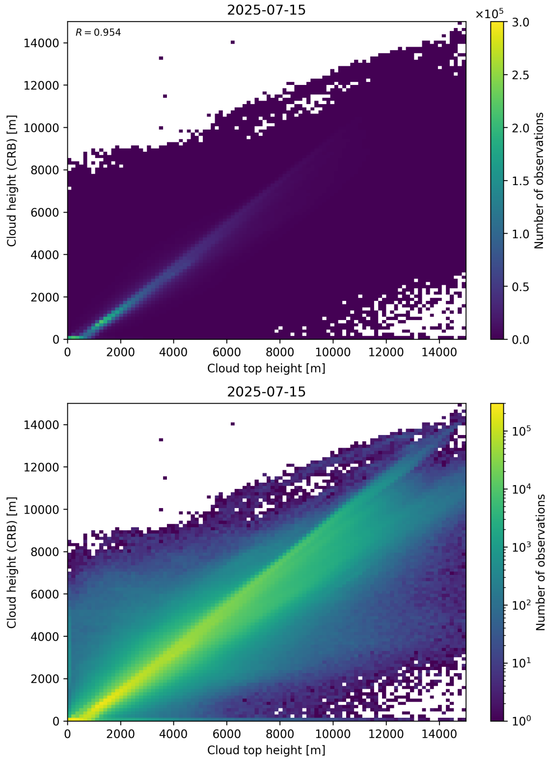
Figure 89: Scatter density plot of “Cloud top height” against “Cloud height (CRB)” for 2025-07-14 to 2025-07-16.
