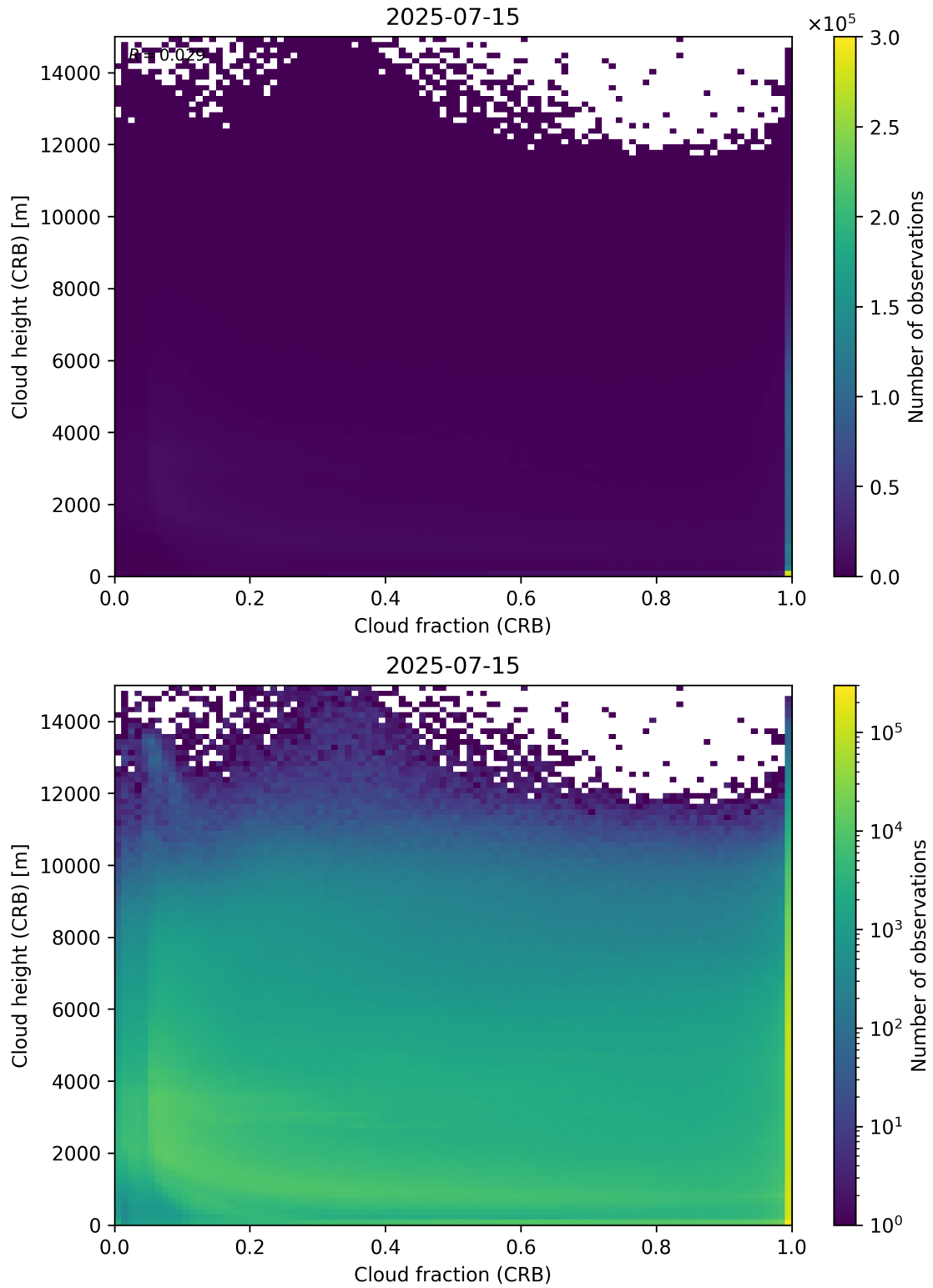
Figure 79: Scatter density plot of “Cloud fraction (CRB)” against “Cloud height (CRB)” for 2025-07-14 to 2025-07-16.
