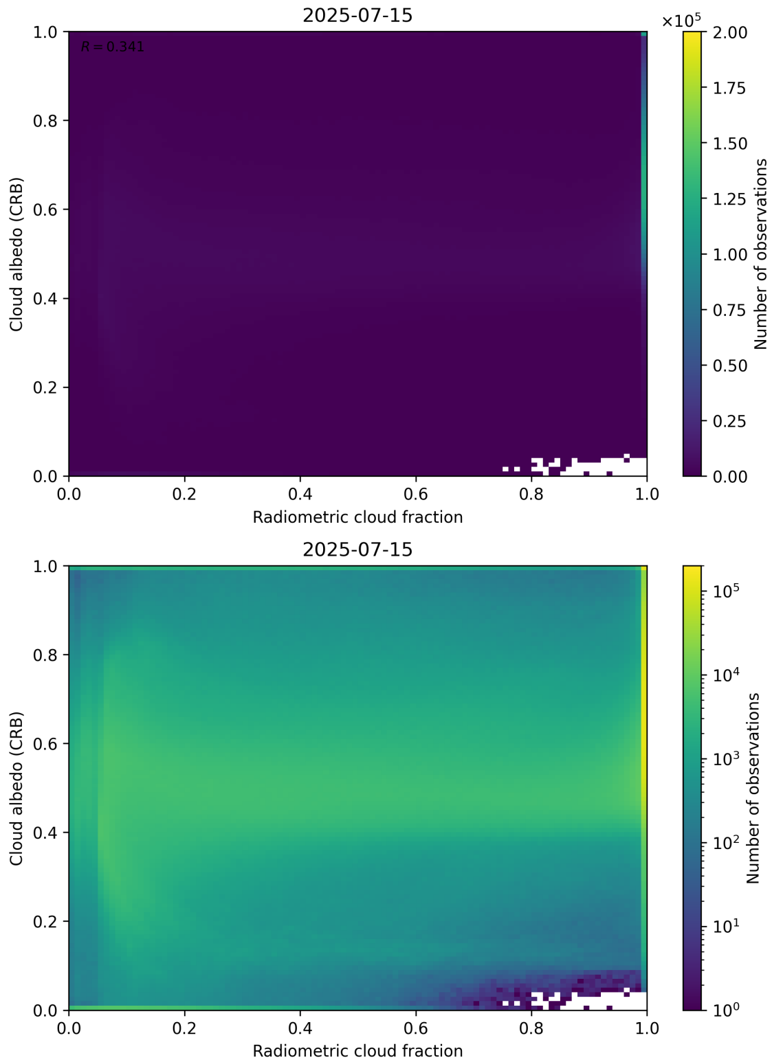
Figure 71: Scatter density plot of “Radiometric cloud fraction” against “Cloud albedo (CRB)” for 2025-07-14 to 2025-07-16.
