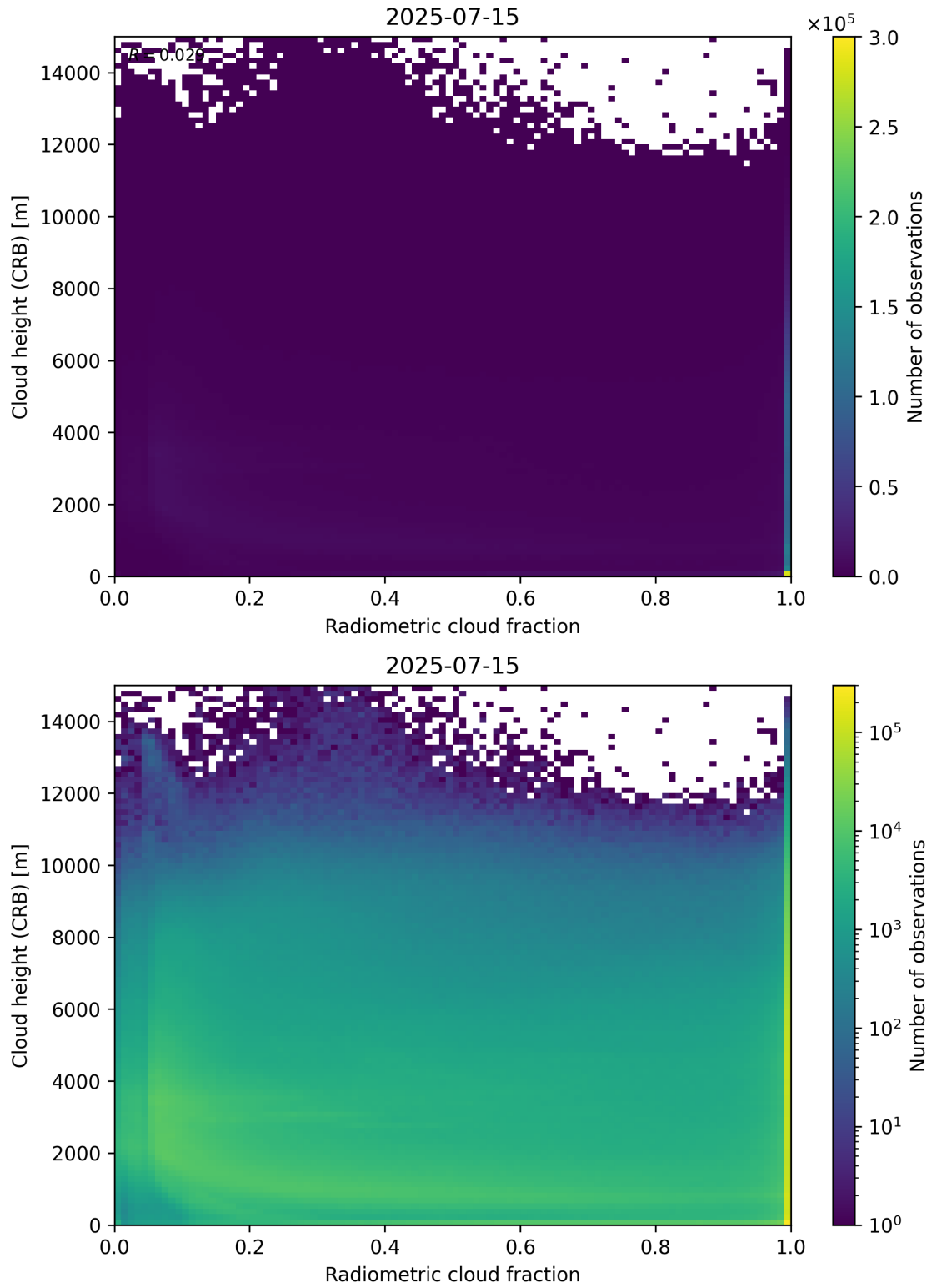
Figure 74: Scatter density plot of “Radiometric cloud fraction” against “Cloud height (CRB)” for 2025-07-14 to 2025-07-16.
