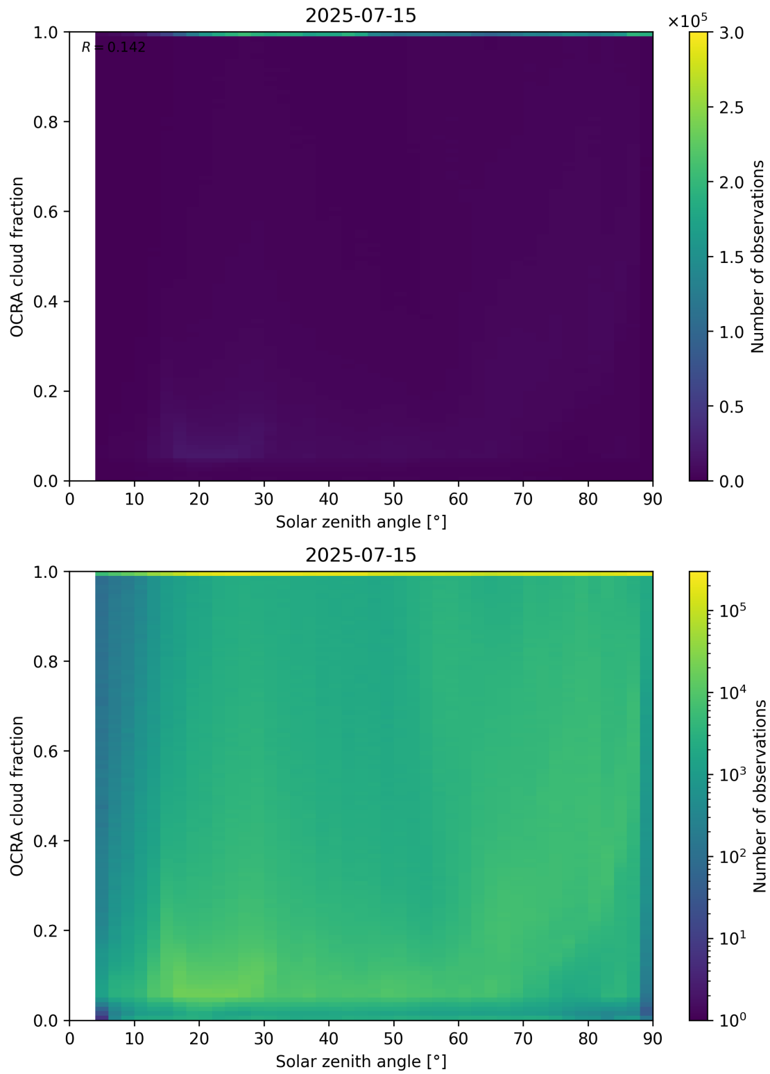
Figure 100: Scatter density plot of “Solar zenith angle” against “OCRA cloud fraction” for 2025-07-14 to 2025-07-16.
