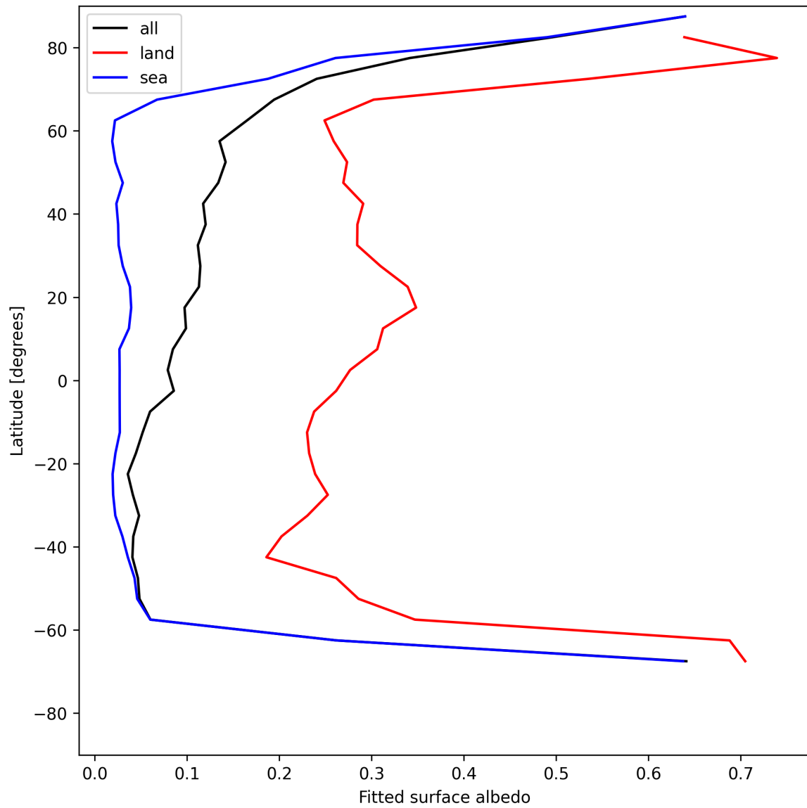
Figure 29: Zonal average of “Fitted surface albedo” for 2025-07-14 to 2025-07-16.
