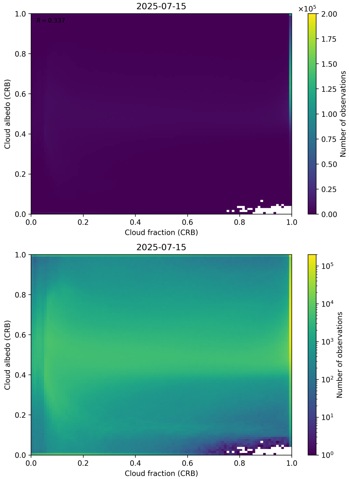
Figure 77: Scatter density plot of “Cloud fraction (CRB)” against “Cloud albedo (CRB)” for 2025-07-14 to 2025-07-16.
