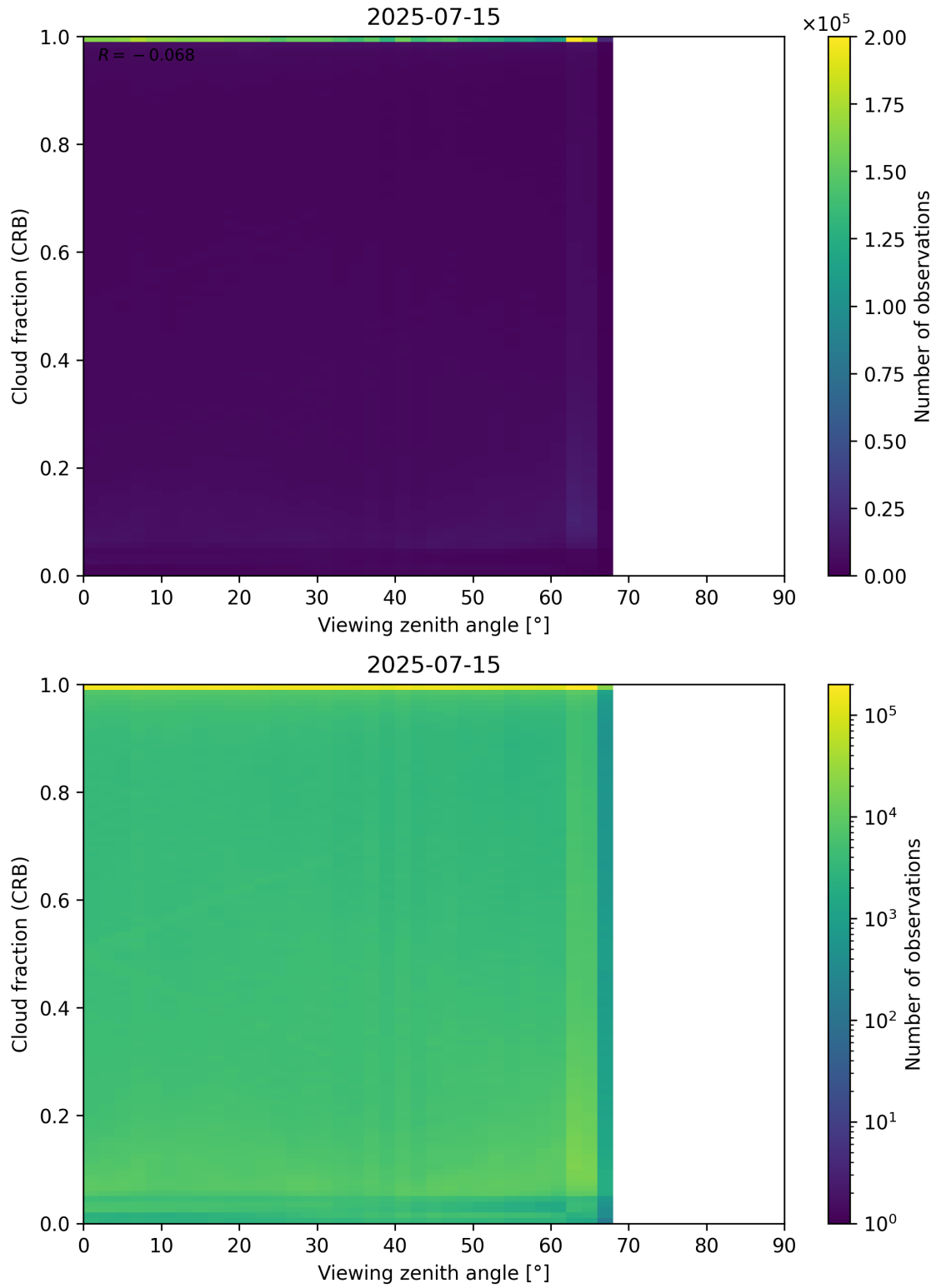
Figure 109: Scatter density plot of “Viewing zenith angle” against “Cloud fraction (CRB)” for 2025-07-14 to 2025-07-16.
