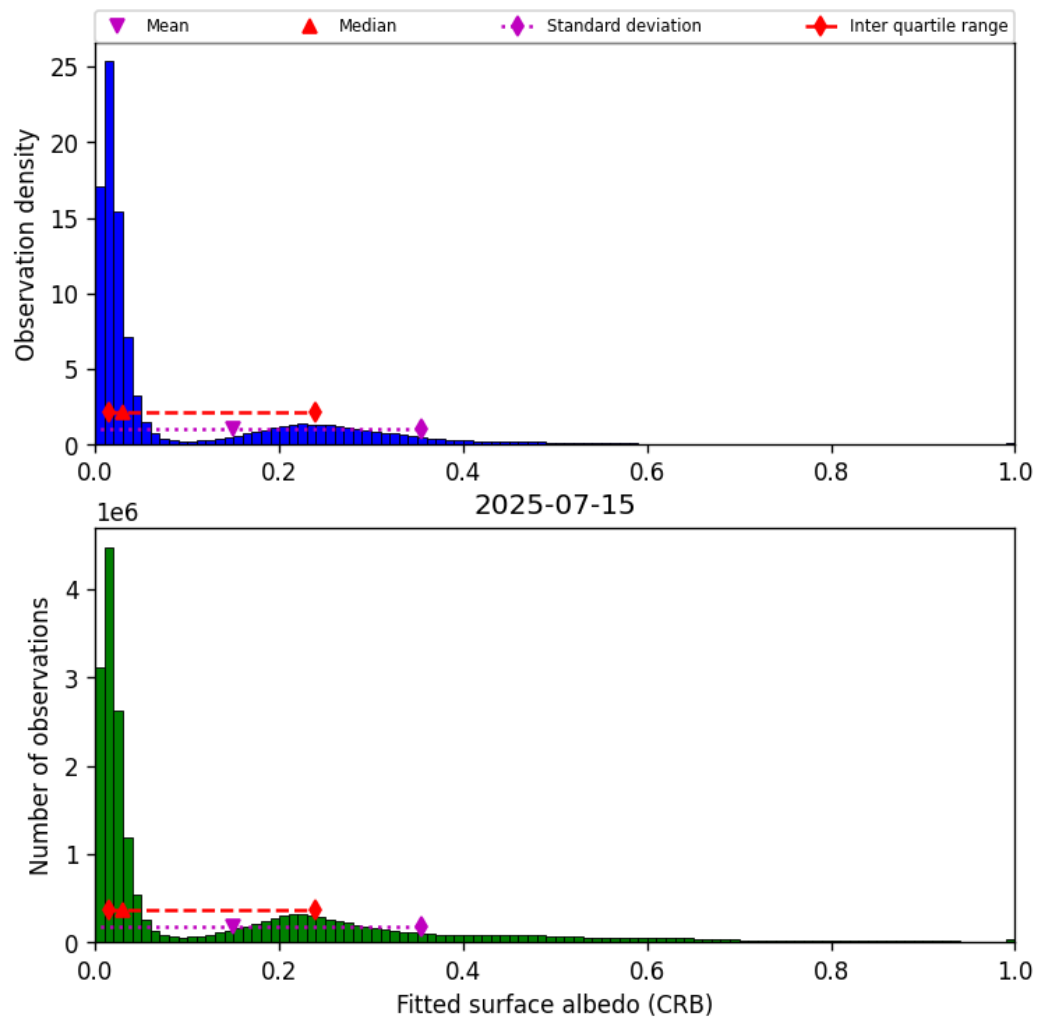
Figure 46: Histogram of “Fitted surface albedo (CRB)” for 2025-07-14 to 2025-07-16
