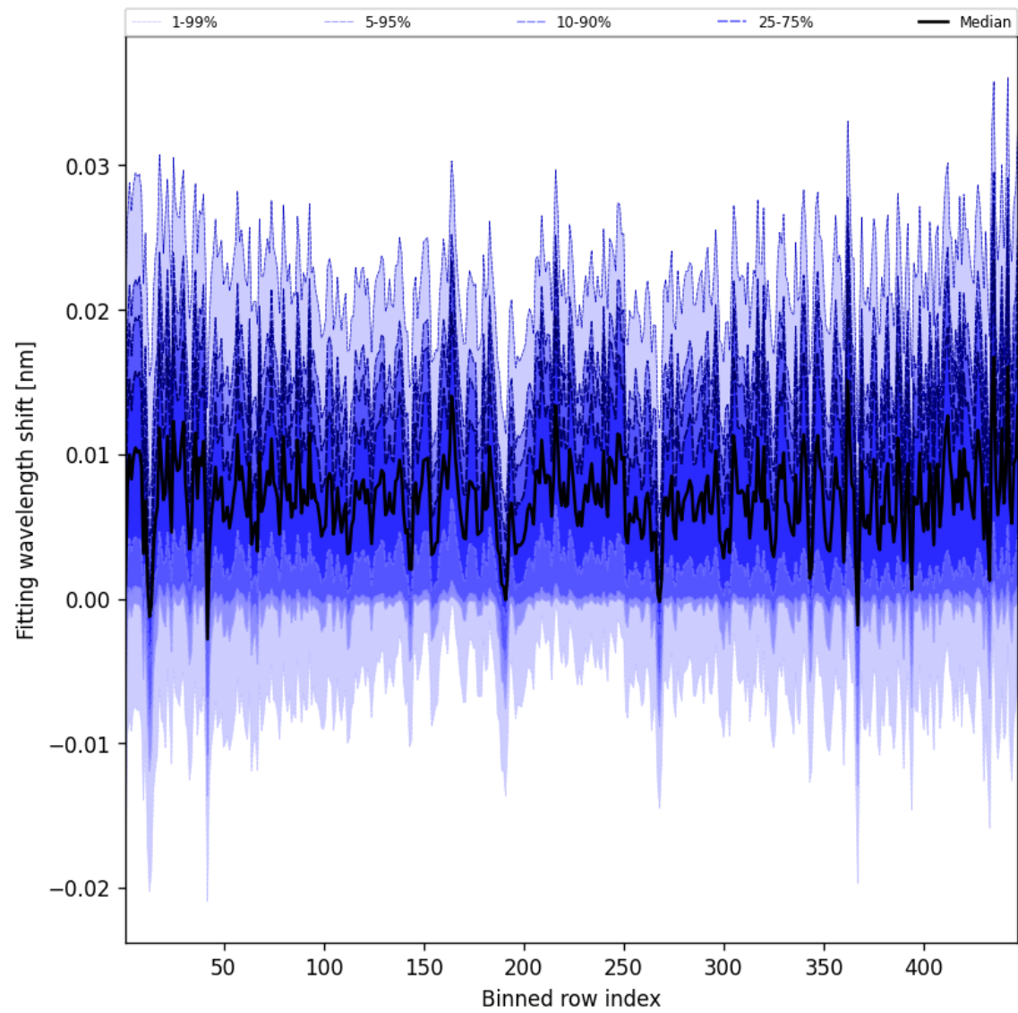
Figure 65: Along track statistics of “Fitting wavelength shift” for 2025-07-14 to 2025-07-16
