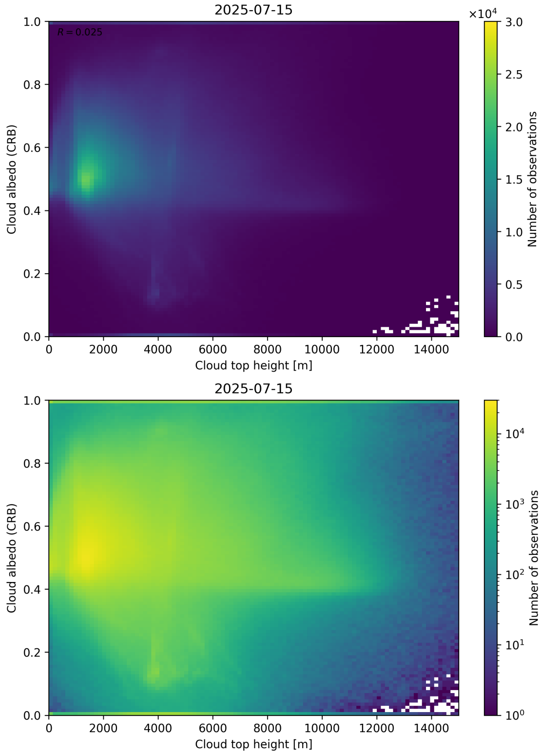
Figure 86: Scatter density plot of “Cloud top height” against “Cloud albedo (CRB)” for 2025-07-14 to 2025-07-16.
