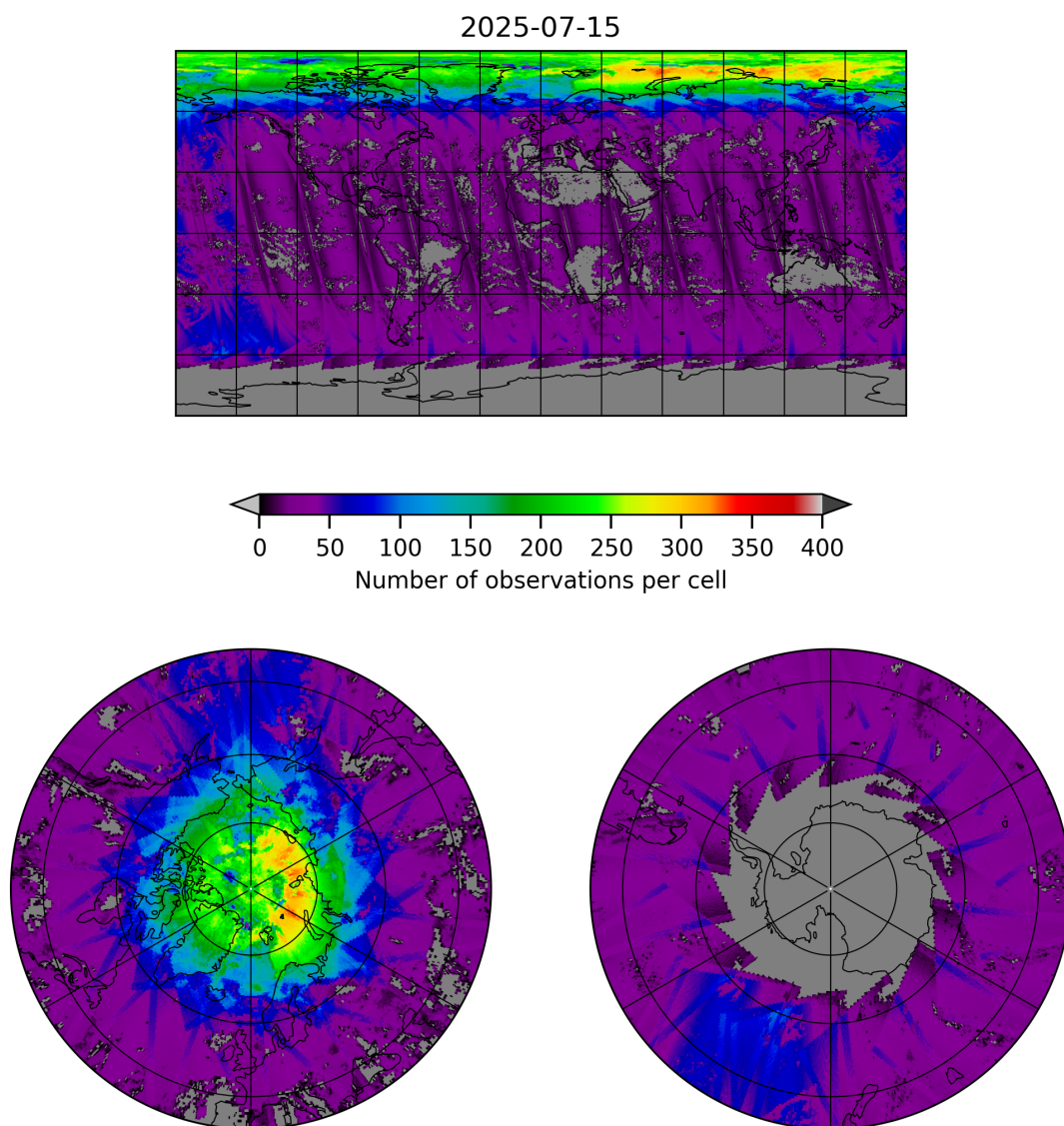
Figure 21: Map of the number of observations for 2025-07-14 to 2025-07-16
