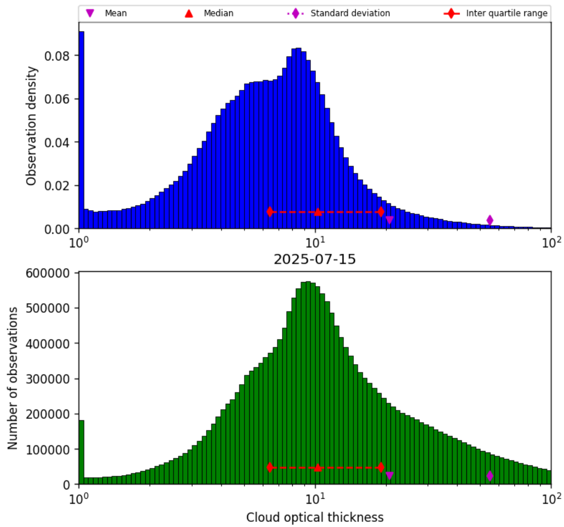
Figure 41: Histogram of “Cloud optical thickness” for 2025-07-14 to 2025-07-16
