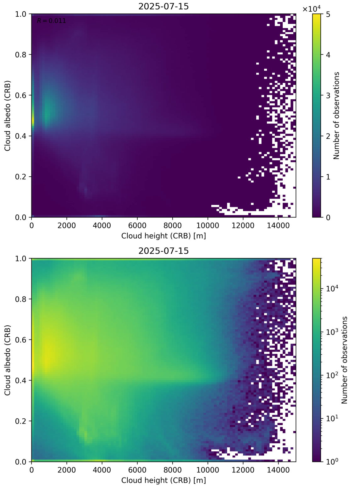
Figure 80: Scatter density plot of “Cloud height (CRB)” against “Cloud albedo (CRB)” for 2025-07-14 to 2025-07-16.
