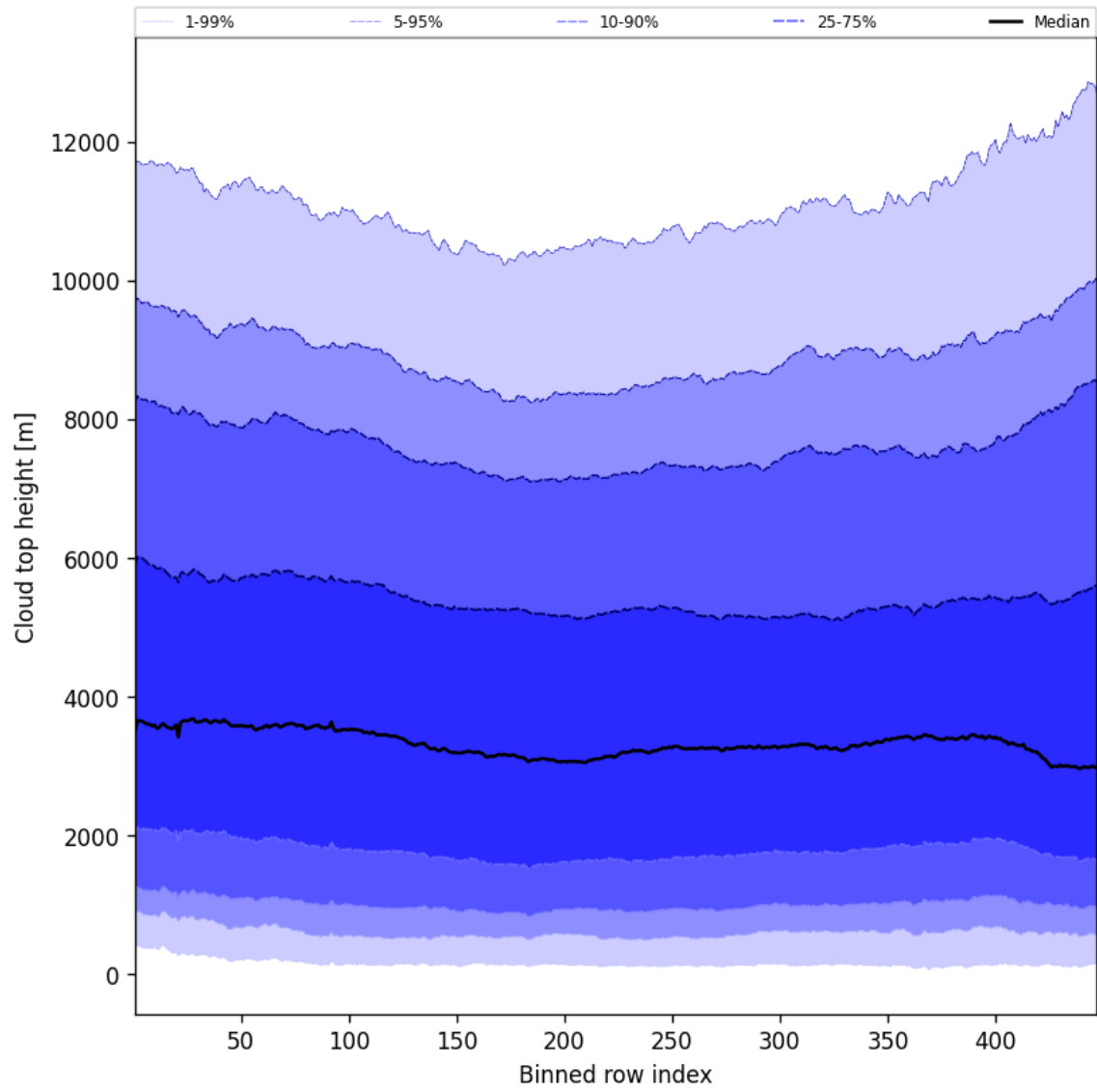
Figure 56: Along track statistics of “Cloud top height” for 2025-07-14 to 2025-07-16
