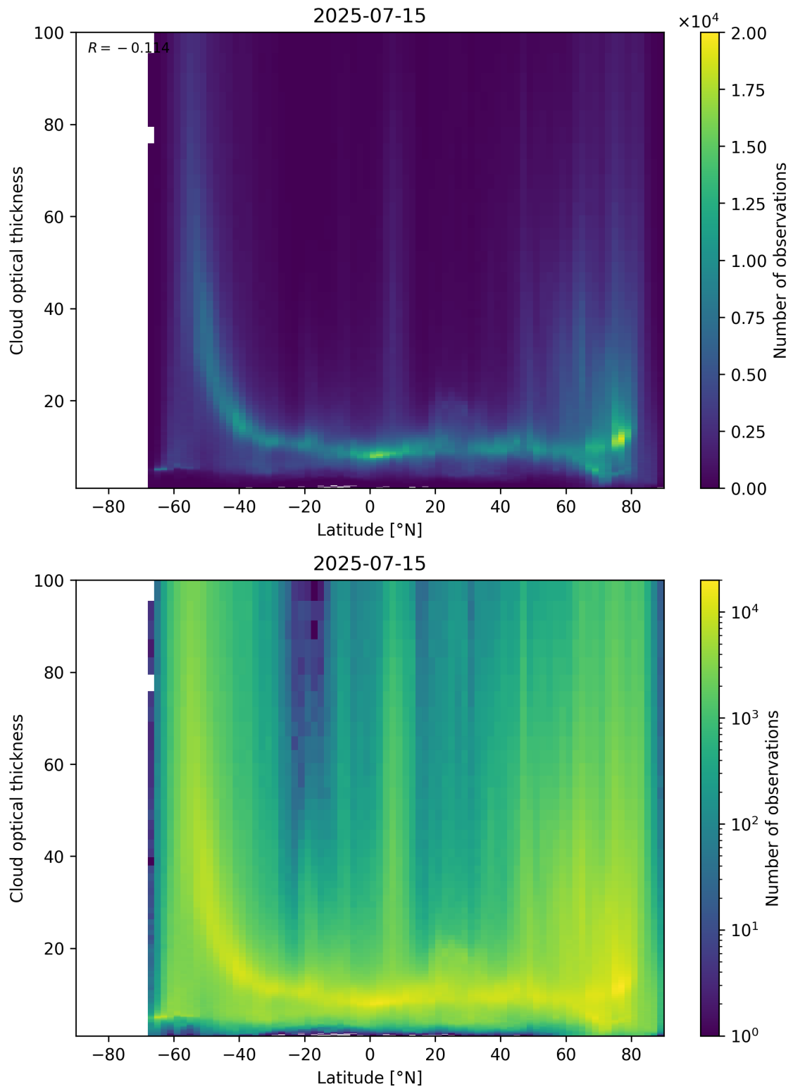
Figure 96: Scatter density plot of “Latitude” against “Cloud optical thickness” for 2025-07-14 to 2025-07-16.
