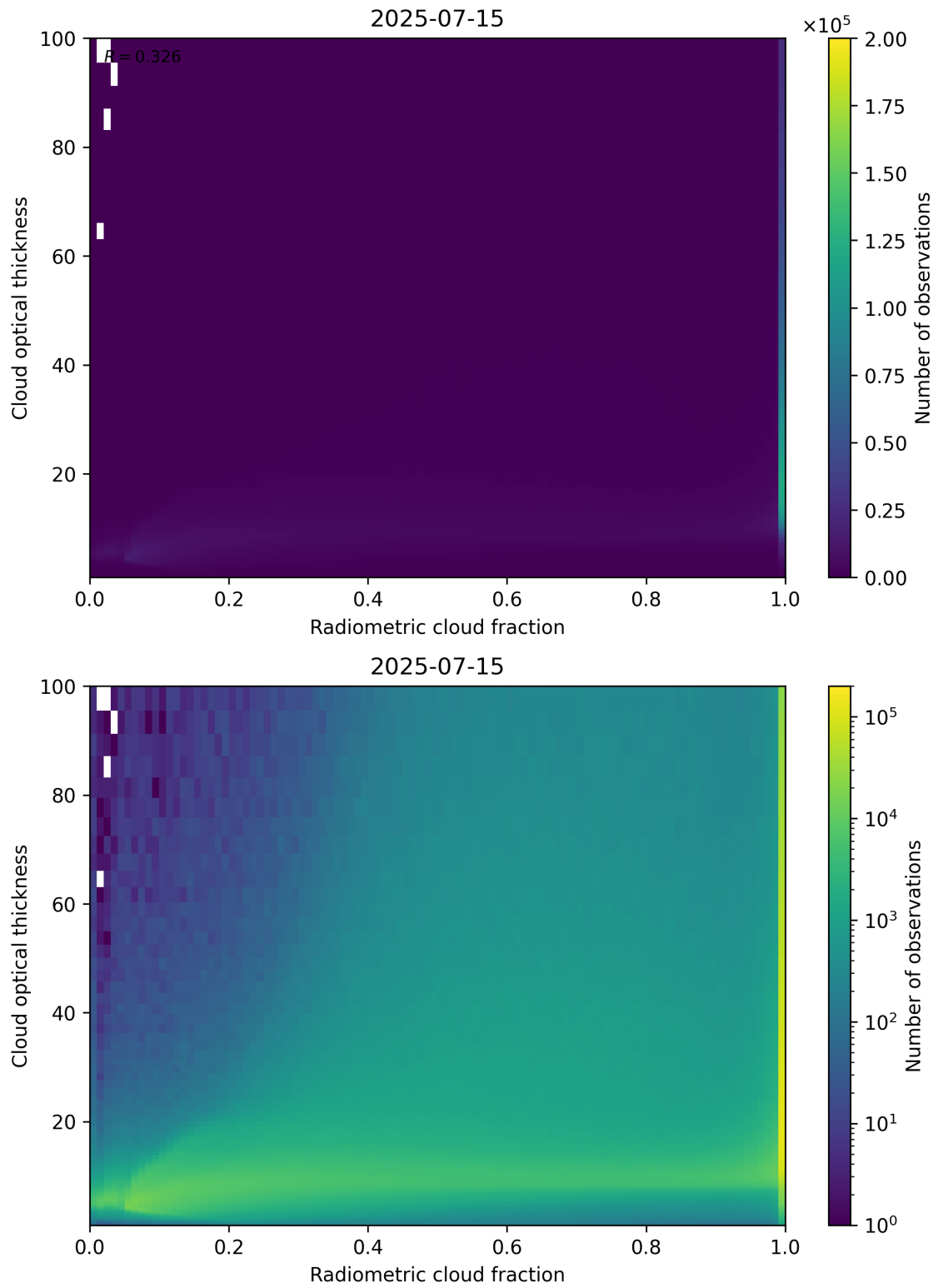
Figure 75: Scatter density plot of “Radiometric cloud fraction” against “Cloud optical thickness” for 2025-07-14 to 2025-07-16.
