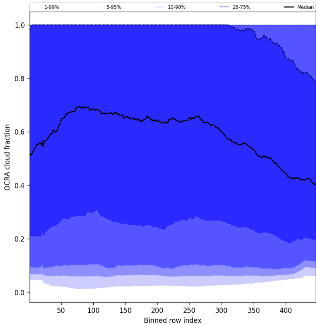
Figure 66: Along track statistics of “OCRA cloud fraction” for 2025-07-14 to 2025-07-16
