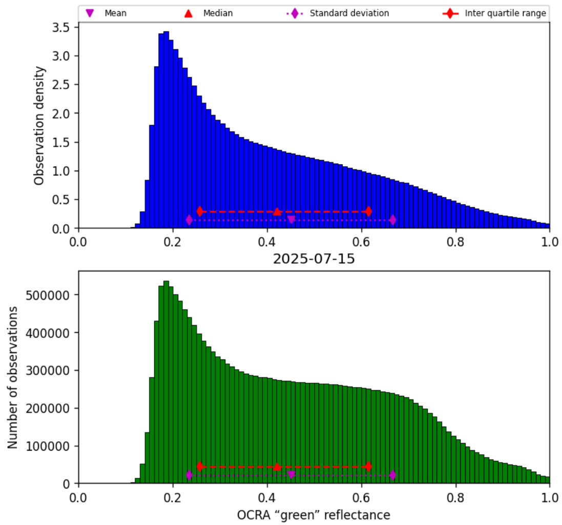
Figure 52: Histogram of “OCRA “green” reflectance” for 2025-07-14 to 2025-07-16
