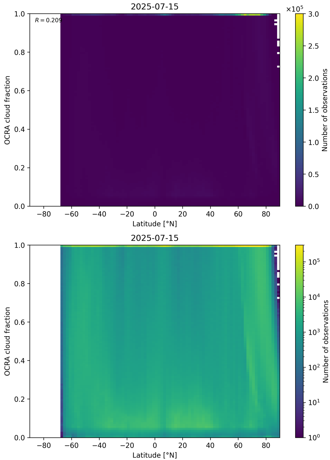
Figure 93: Scatter density plot of “Latitude” against “OCRA cloud fraction” for 2025-07-14 to 2025-07-16.
