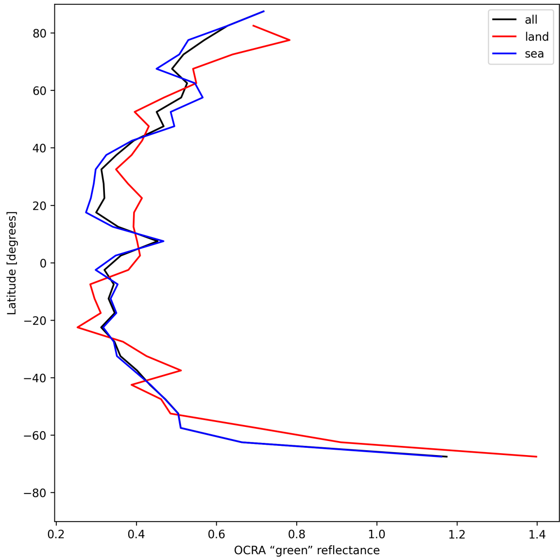
Figure 36: Zonal average of “OCRA “green” reflectance” for 2025-07-14 to 2025-07-16.
