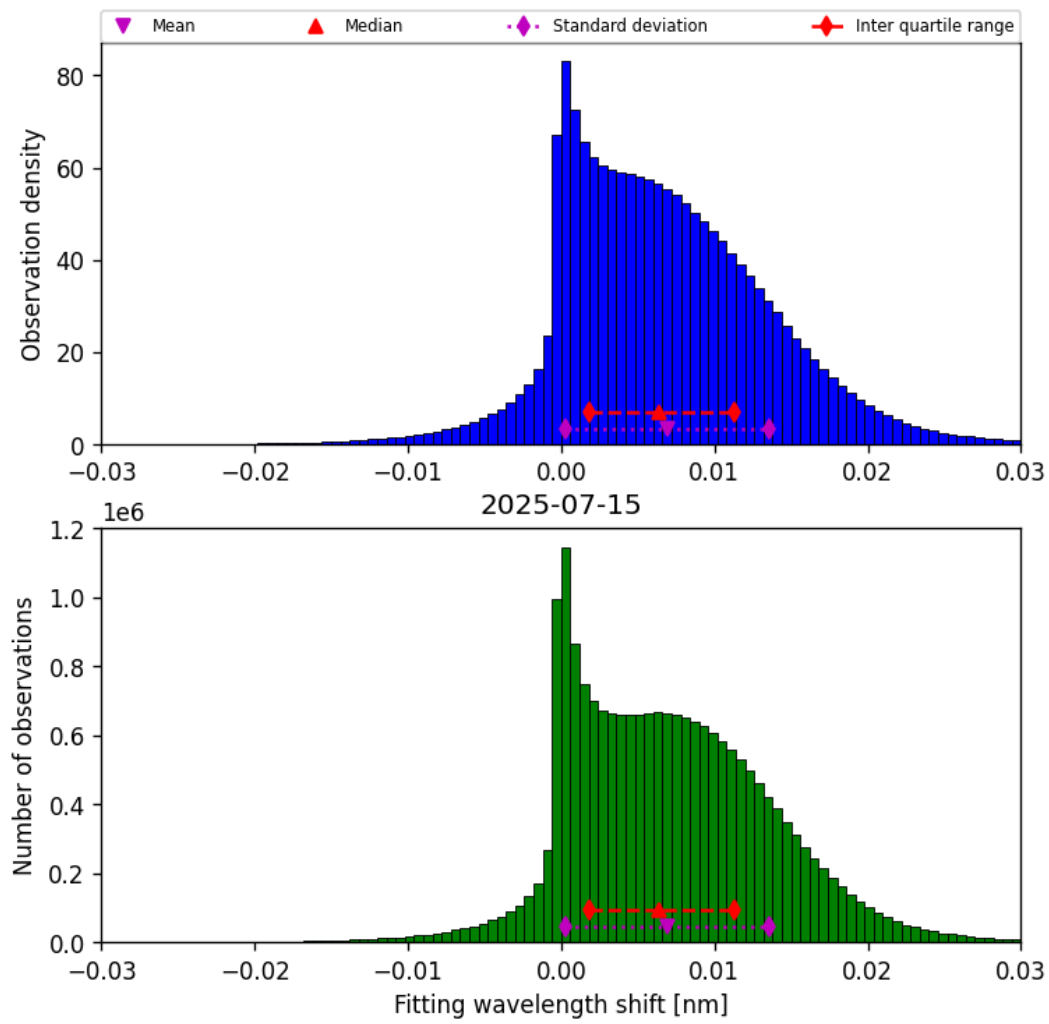
Figure 49: Histogram of “Fitting wavelength shift” for 2025-07-14 to 2025-07-16
