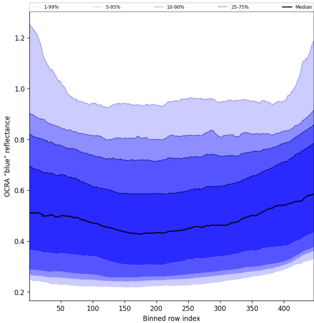
Figure 67: Along track statistics of “OCRA “blue” reflectance” for 2025-07-14 to 2025-07-16
