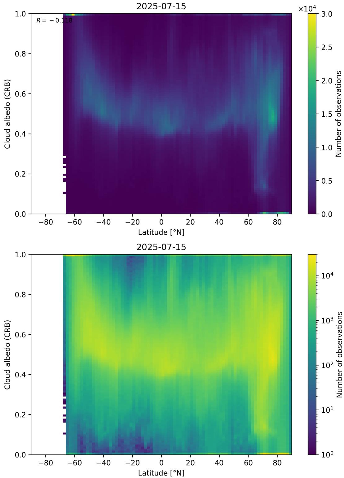
Figure 91: Scatter density plot of “Latitude” against “Cloud albedo (CRB)” for 2025-07-14 to 2025-07-16.
