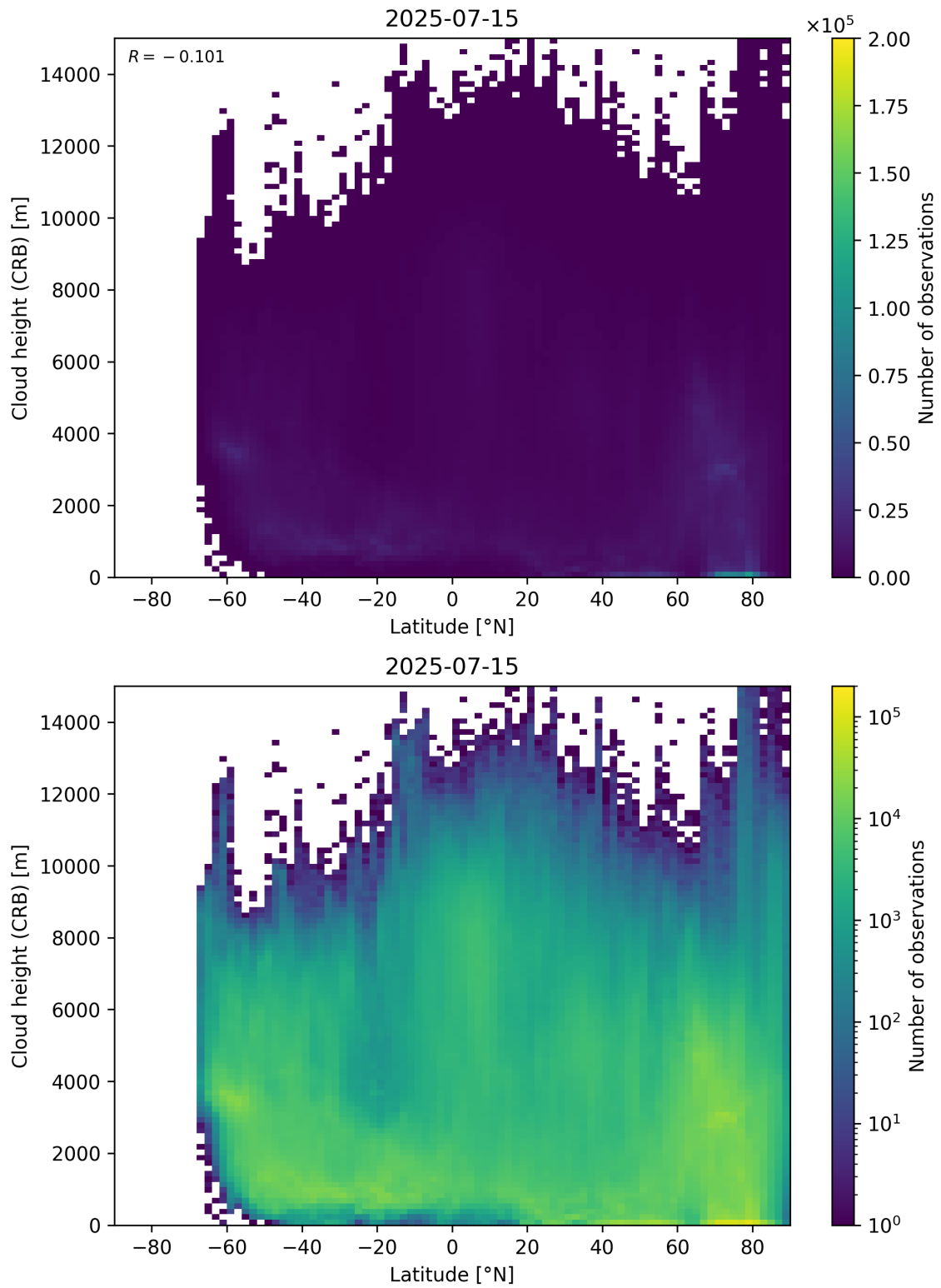
Figure 95: Scatter density plot of “Latitude” against “Cloud height (CRB)” for 2025-07-14 to 2025-07-16.
