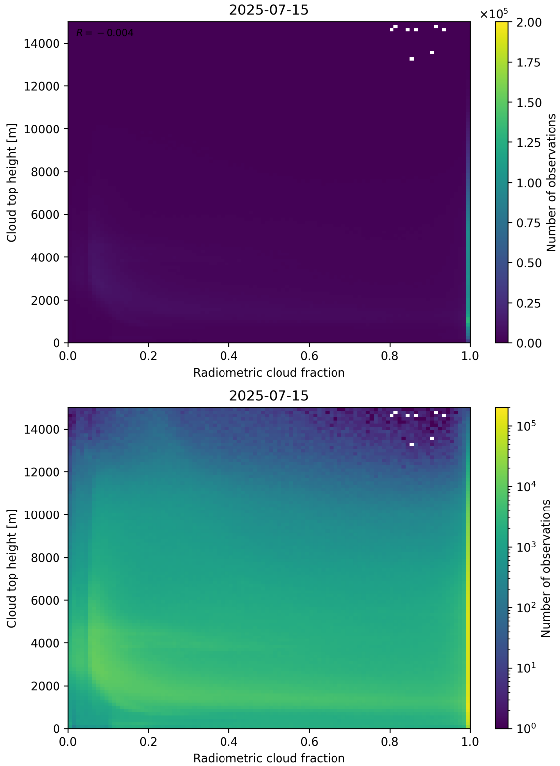
Figure 76: Scatter density plot of “Radiometric cloud fraction” against “Cloud top height” for 2025-07-14 to 2025-07-16.
