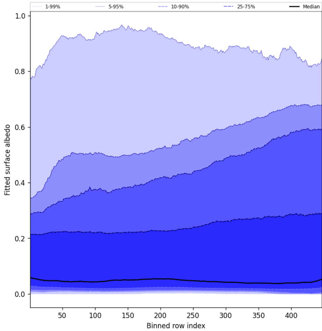
Figure 61: Along track statistics of “Fitted surface albedo” for 2025-07-14 to 2025-07-16
