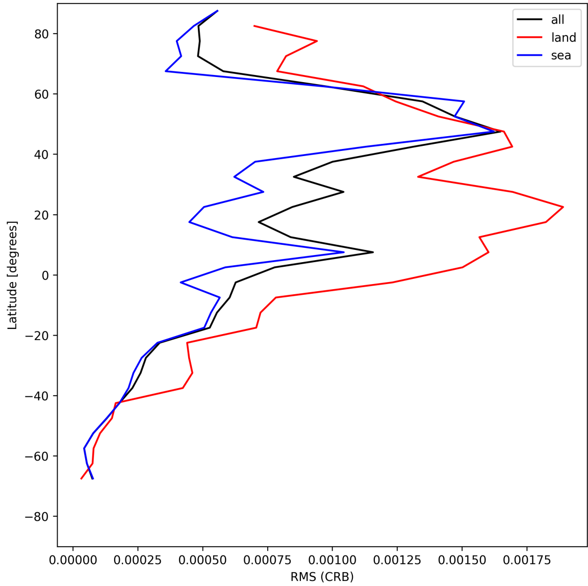
Figure 32: Zonal average of “RMS (CRB)” for 2025-07-14 to 2025-07-16.
