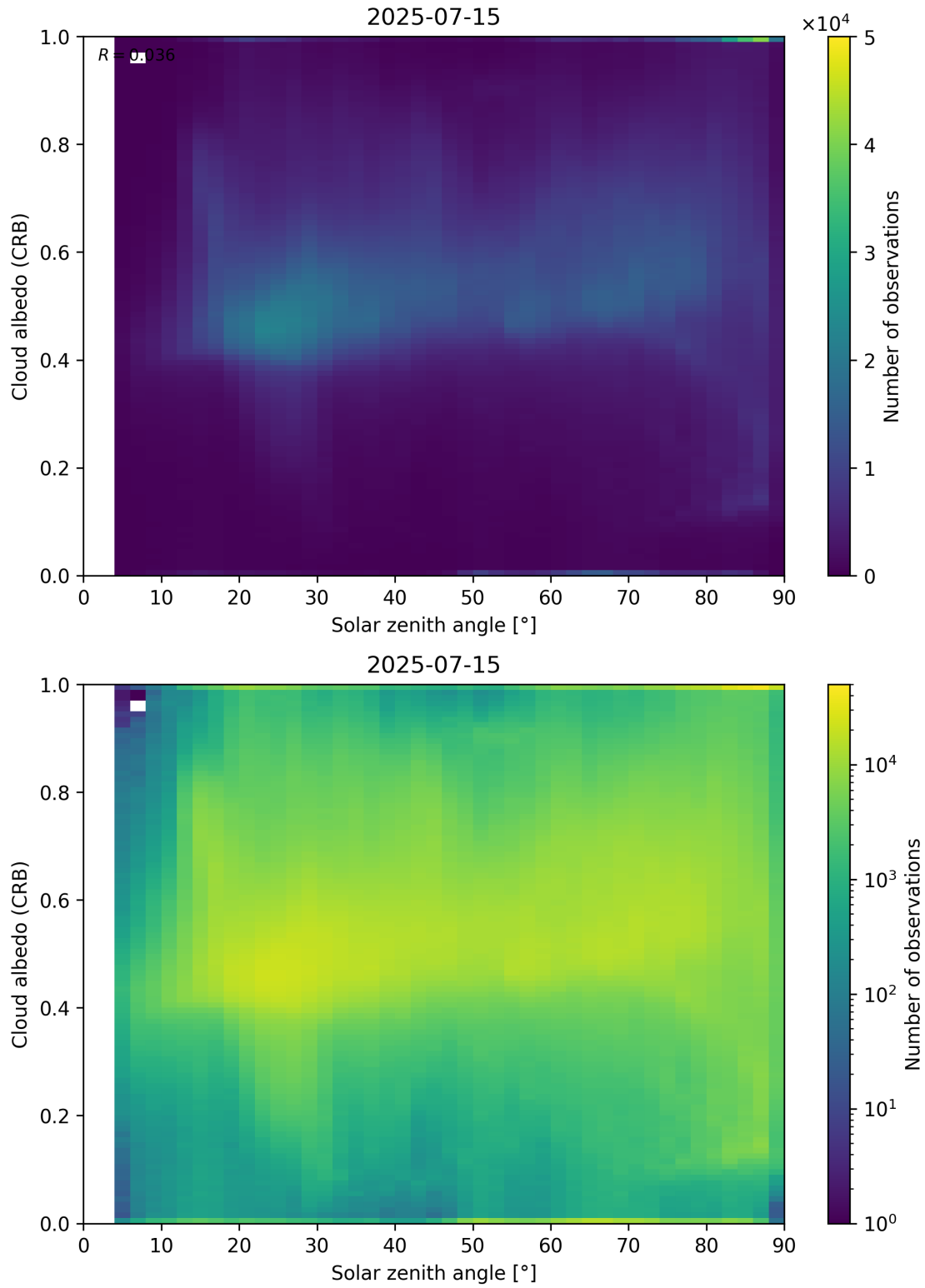
Figure 98: Scatter density plot of “Solar zenith angle” against “Cloud albedo (CRB)” for 2025-07-14 to 2025-07-16.
