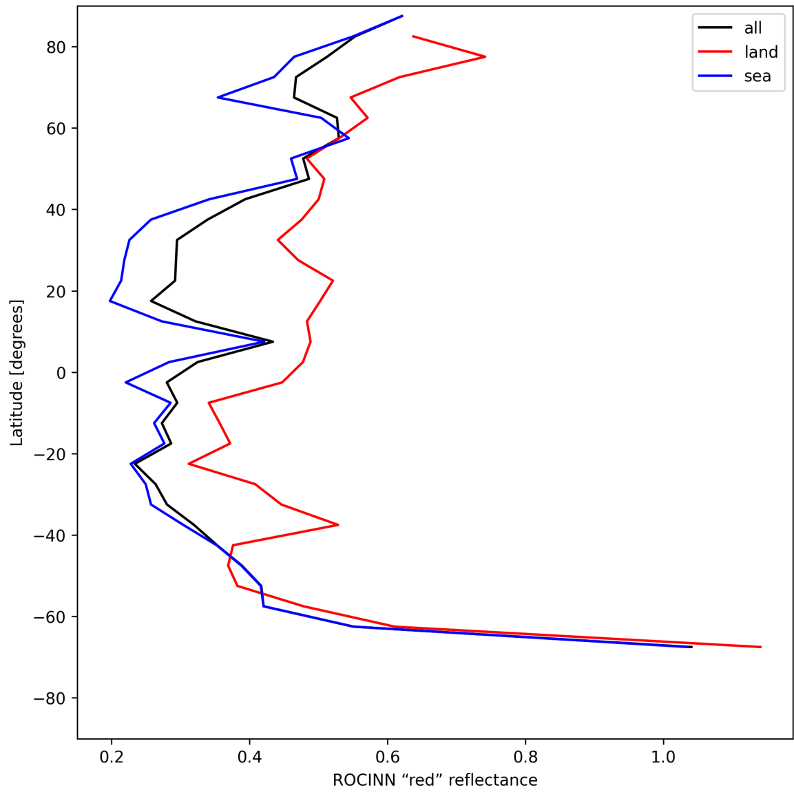
Figure 37: Zonal average of "ROCINN "red" reflectance" for 2025-07-14 to 2025-07-16.
