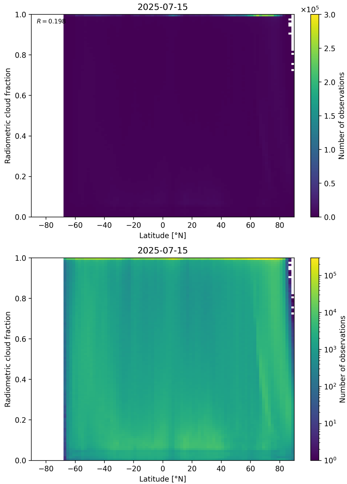
Figure 92: Scatter density plot of “Latitude” against “Radiometric cloud fraction” for 2025-07-14 to 2025-07-16.
