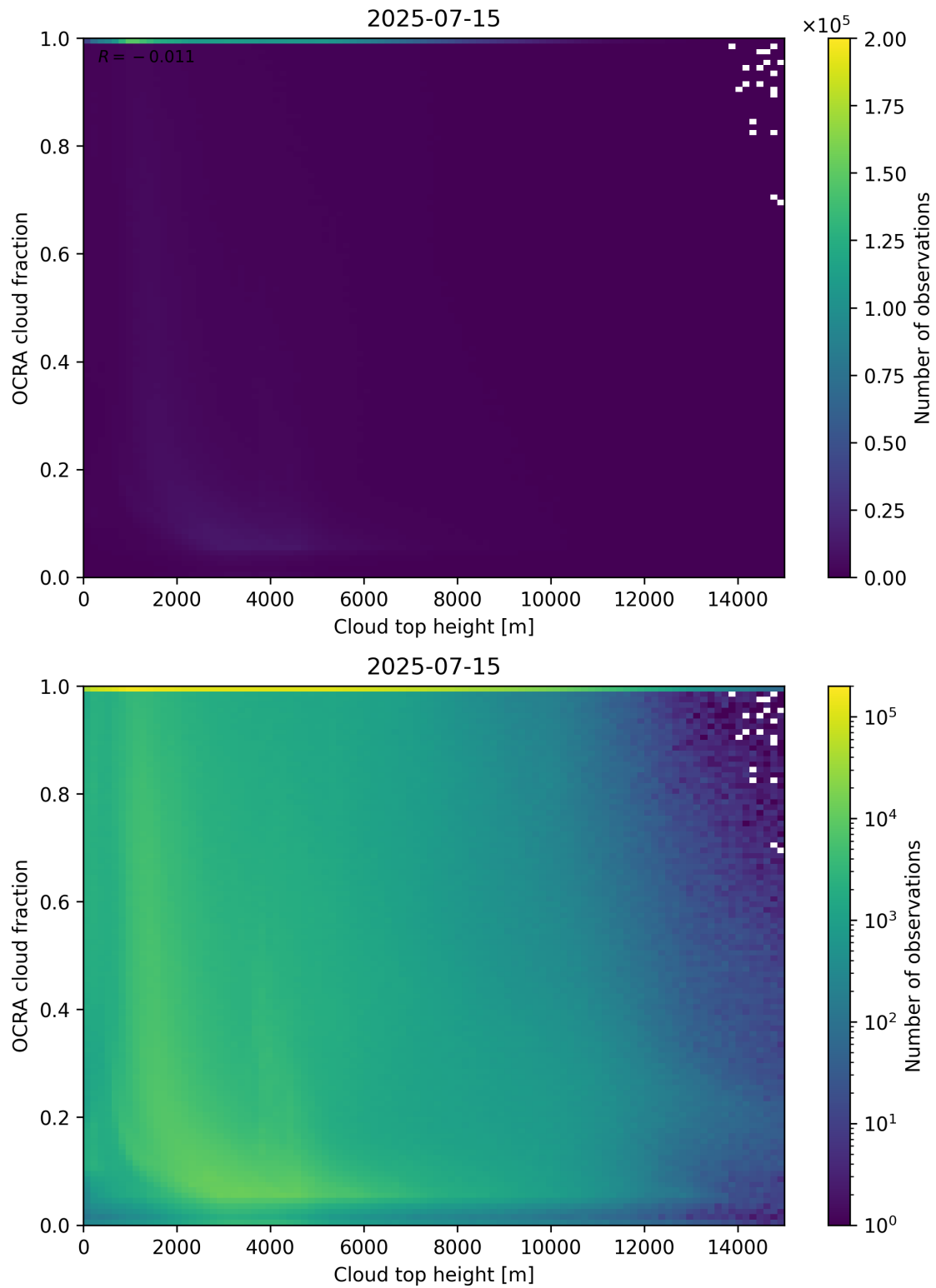
Figure 87: Scatter density plot of “Cloud top height” against “OCRA cloud fraction” for 2025-07-14 to 2025-07-16.
