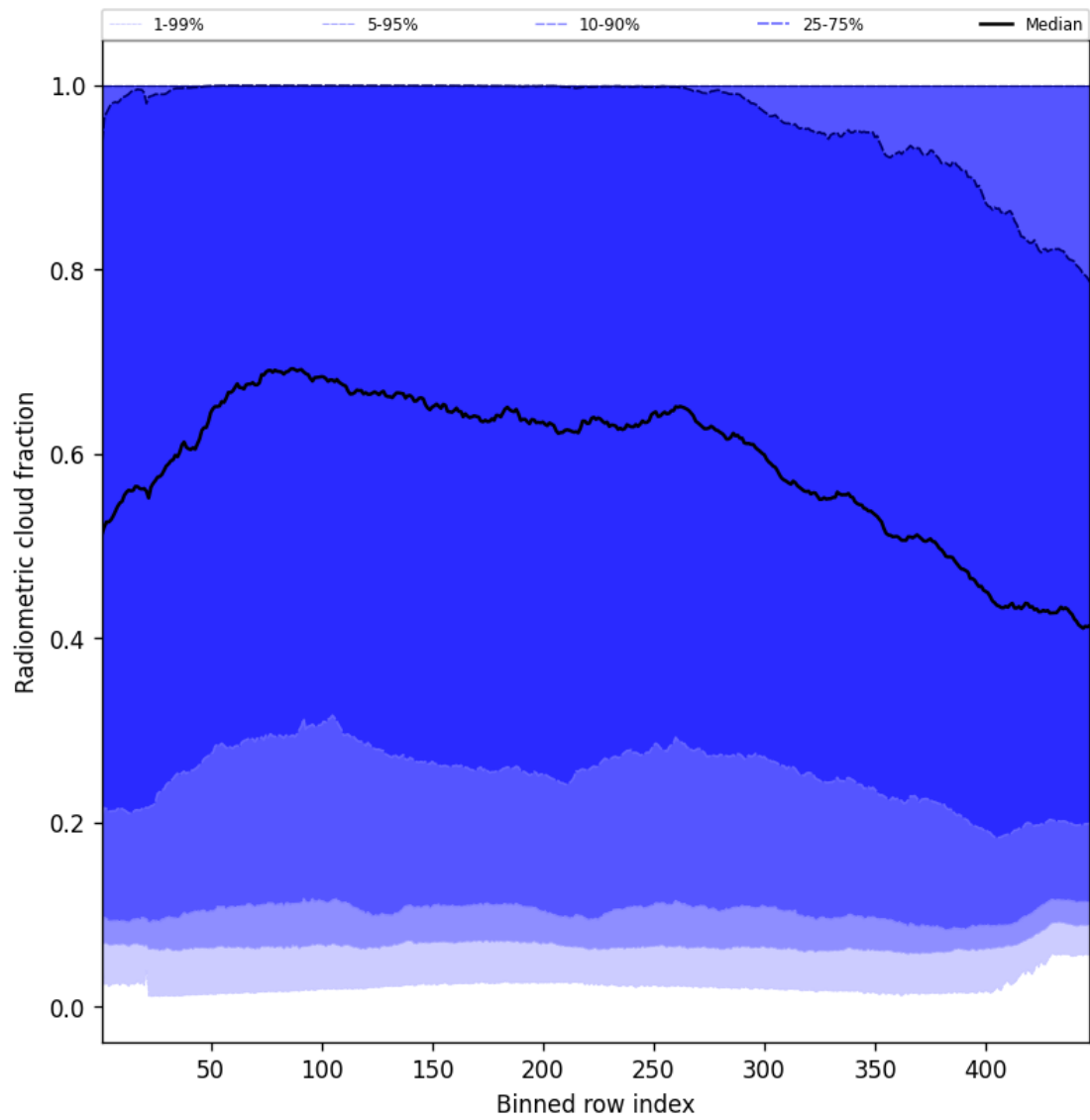
Figure 55: Along track statistics of “Radiometric cloud fraction” for 2025-07-14 to 2025-07-16
