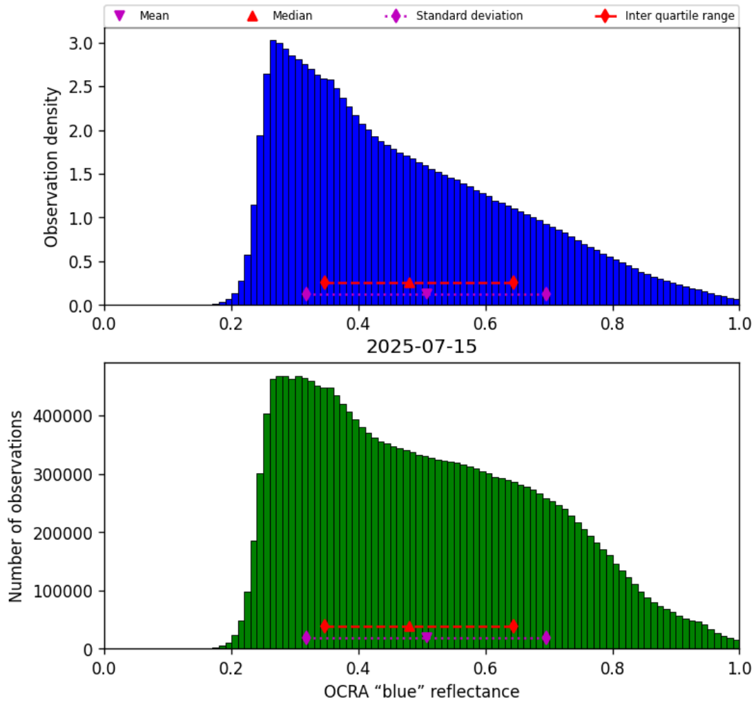
Figure 51: Histogram of “OCRA “blue” reflectance” for 2025-07-14 to 2025-07-16
