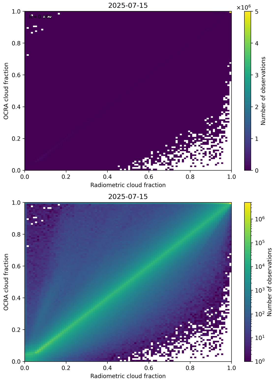
Figure 72: Scatter density plot of “Radiometric cloud fraction” against “OCRA cloud fraction” for 2025-07-14 to 2025-07-16.
