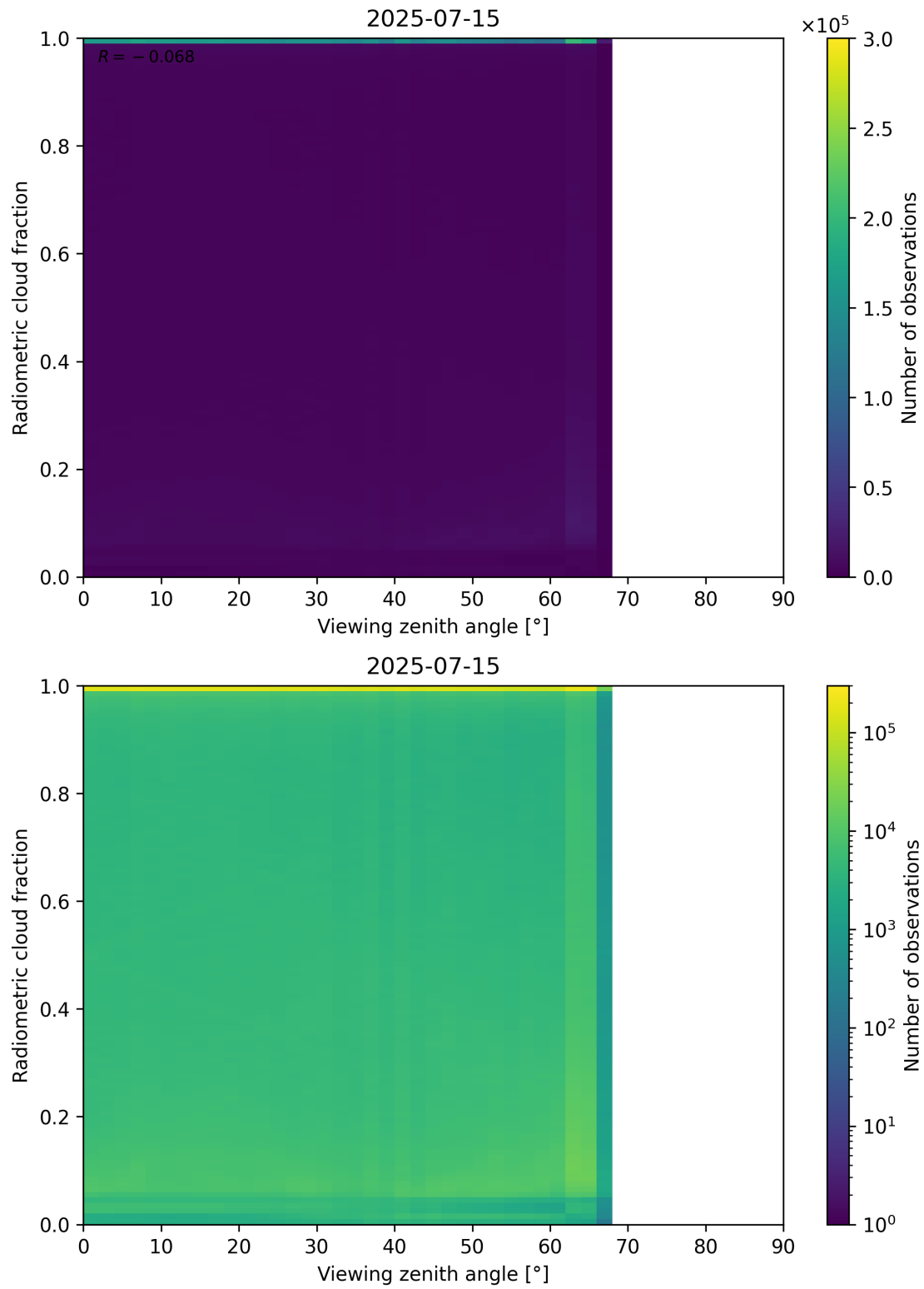
Figure 107: Scatter density plot of “Viewing zenith angle” against “Radiometric cloud fraction” for 2025-07-14 to 2025-07-16.
