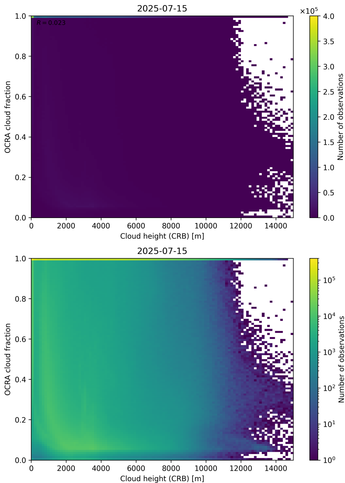
Figure 81: Scatter density plot of “Cloud height (CRB)” against “OCRA cloud fraction” for 2025-07-14 to 2025-07-16.
