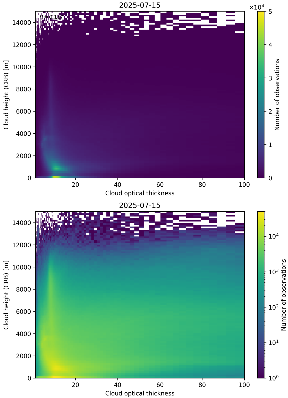
Figure 85: Scatter density plot of “Cloud optical thickness” against “Cloud height (CRB)” for 2025-07-14 to 2025-07-16.
