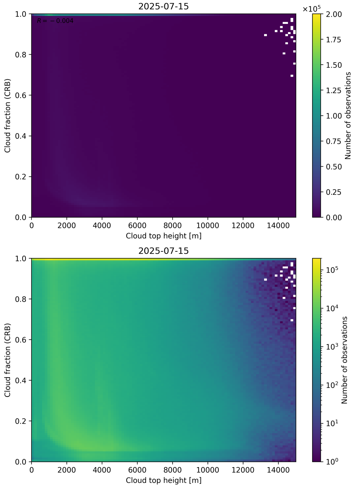
Figure 88: Scatter density plot of “Cloud top height” against “Cloud fraction (CRB)” for 2025-07-14 to 2025-07-16.
