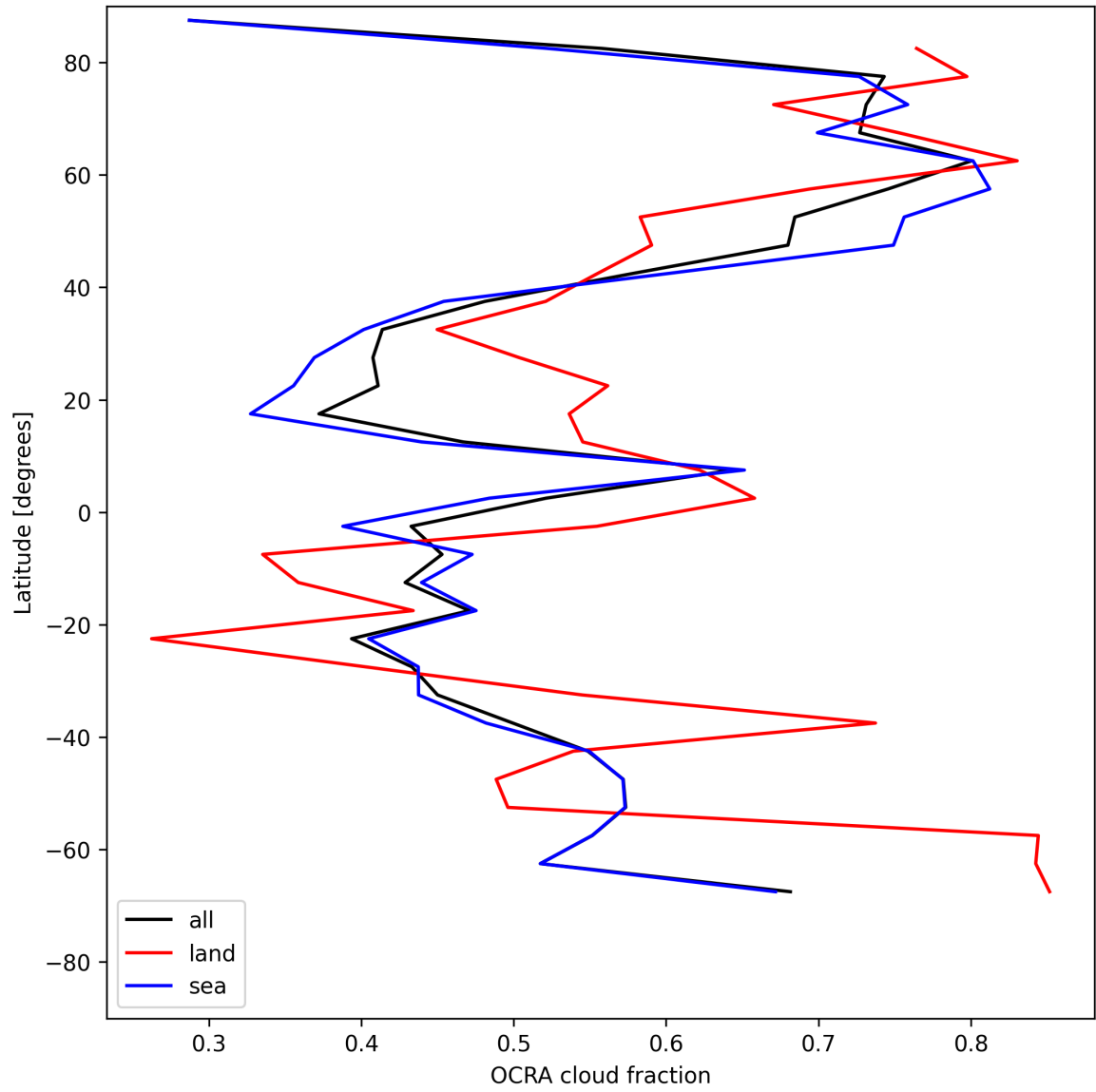
Figure 34: Zonal average of “OCRA cloud fraction” for 2025-07-14 to 2025-07-16.
