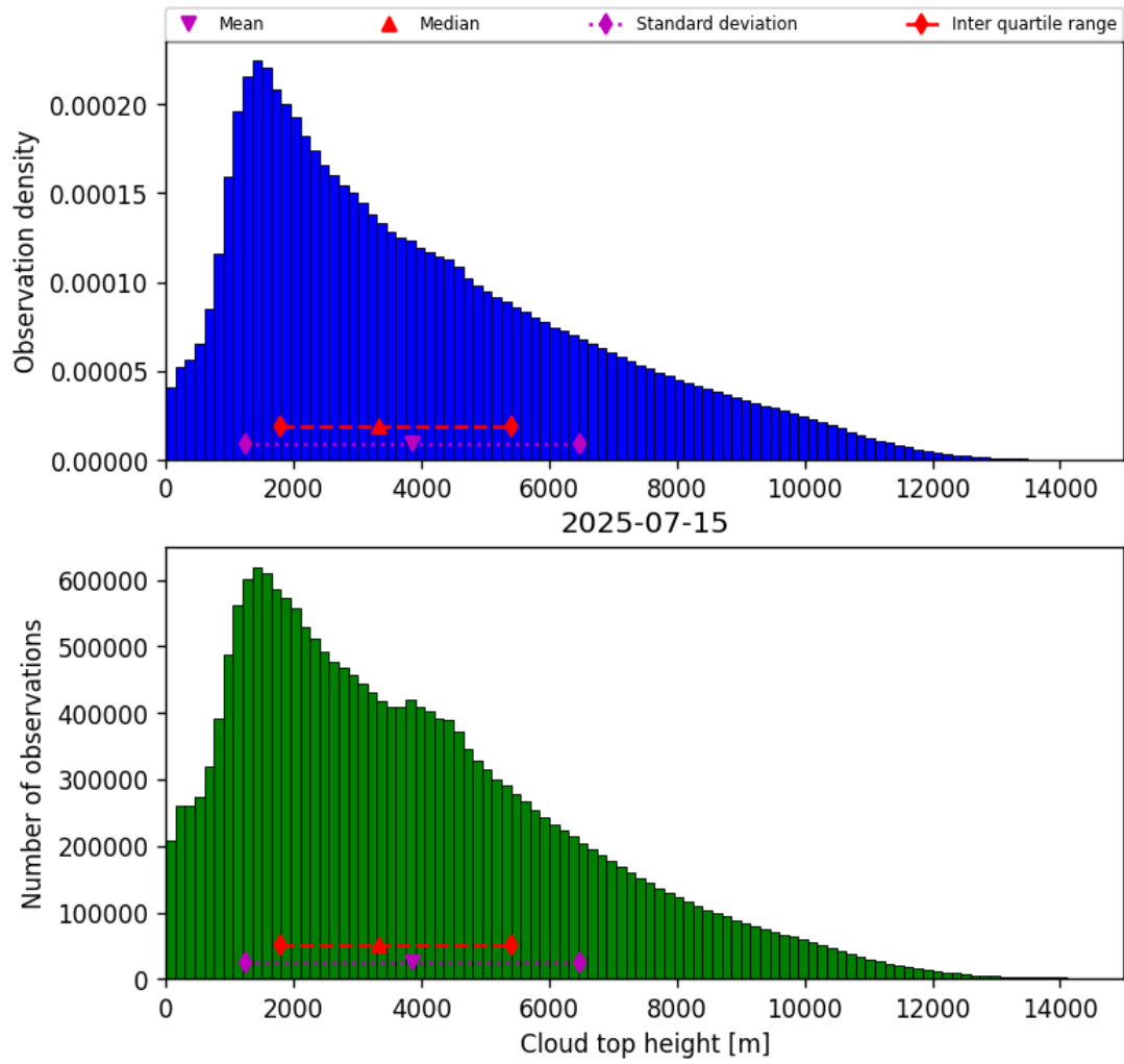
Figure 40: Histogram of “Cloud top height” for 2025-07-14 to 2025-07-16
