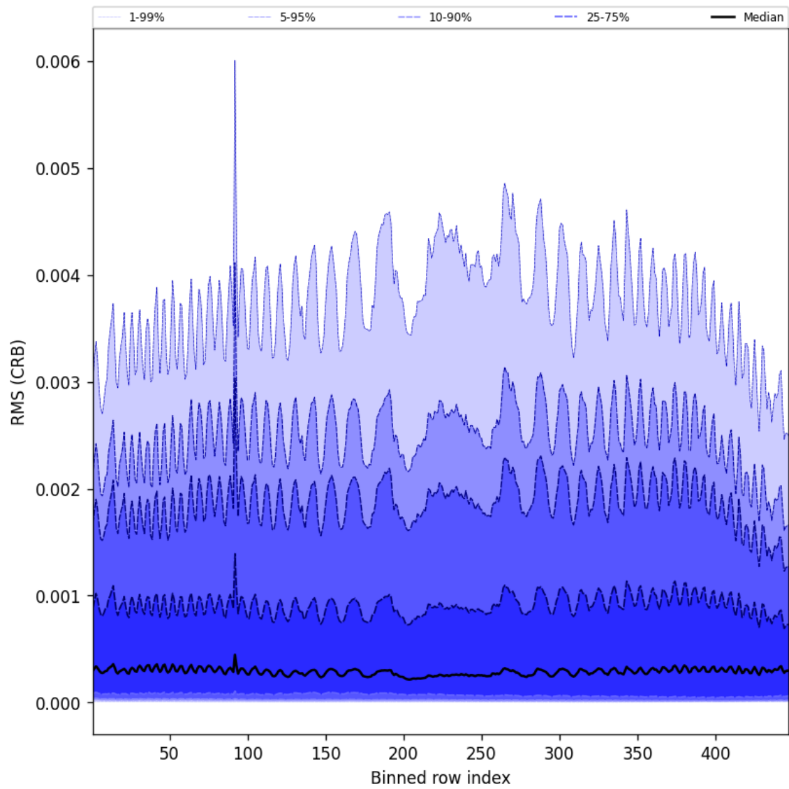
Figure 64: Along track statistics of “RMS (CRB)” for 2025-07-14 to 2025-07-16
