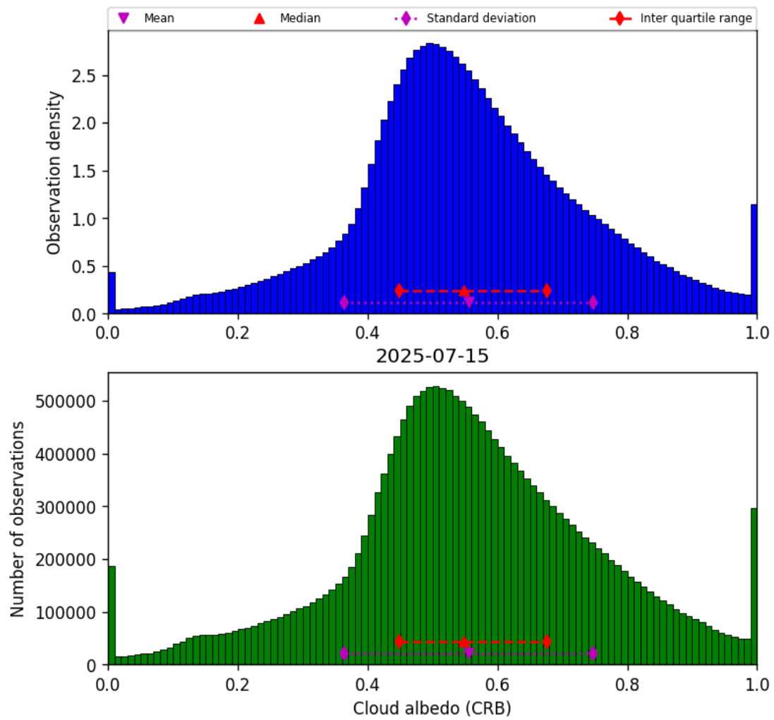
Figure 44: Histogram of “Cloud albedo (CRB)” for 2025-07-14 to 2025-07-16
