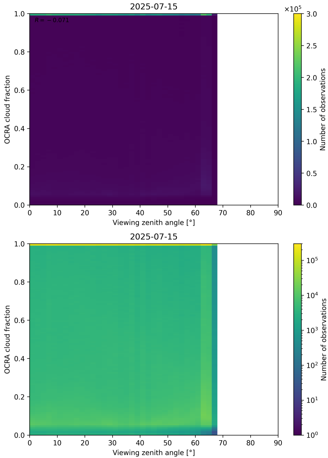
Figure 108: Scatter density plot of “Viewing zenith angle” against “OCRA cloud fraction” for 2025-07-14 to 2025-07-16.
