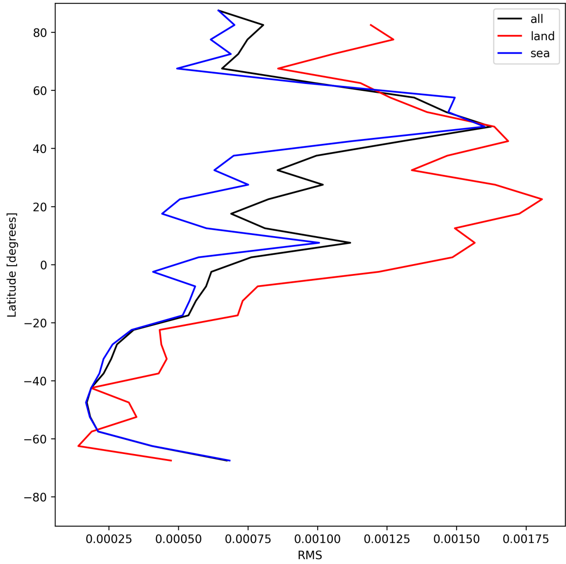
Figure 31: Zonal average of “RMS” for 2025-07-14 to 2025-07-16.
