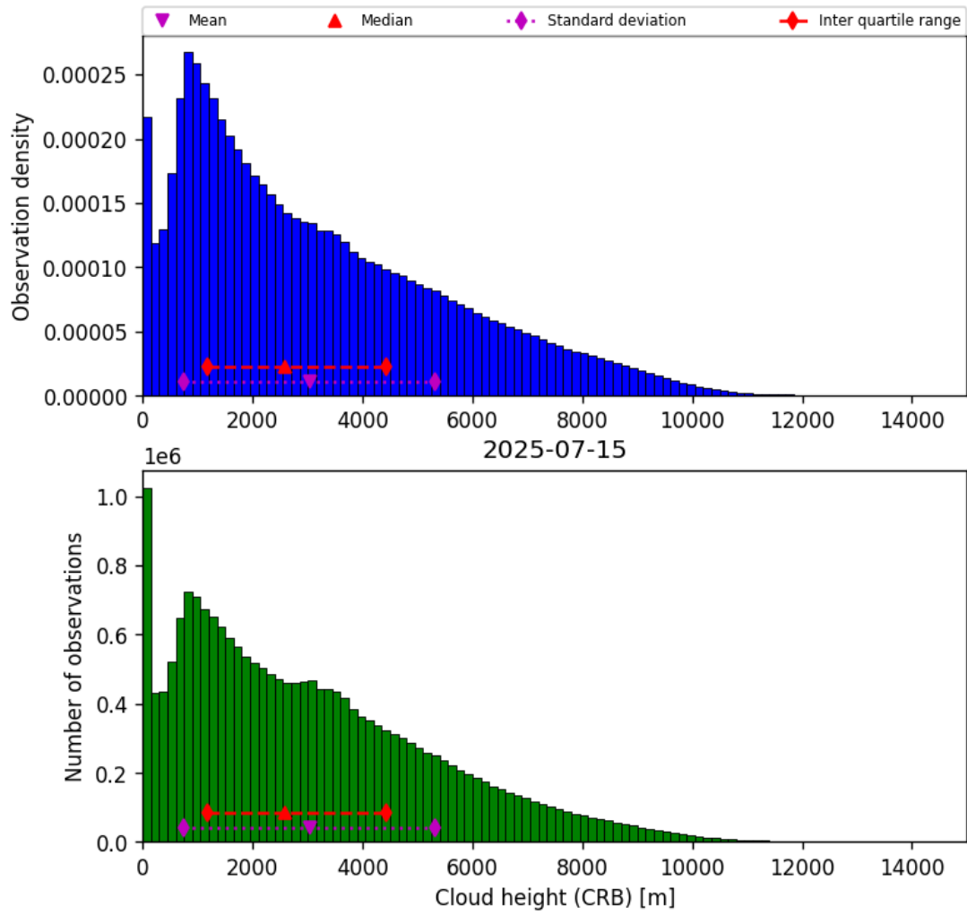
Figure 43: Histogram of “Cloud height (CRB)” for 2025-07-14 to 2025-07-16
