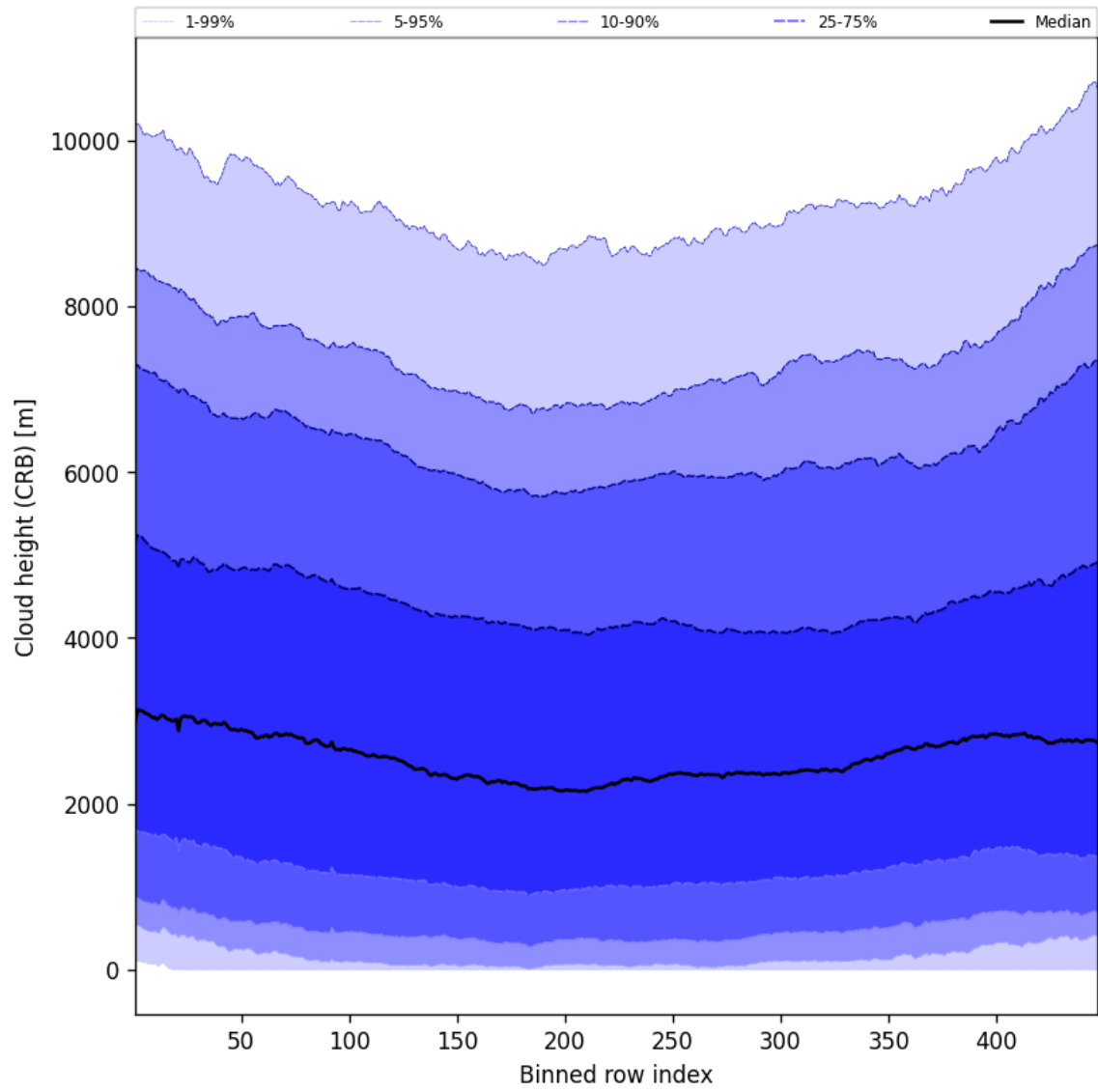
Figure 59: Along track statistics of “Cloud height (CRB)” for 2025-07-14 to 2025-07-16
