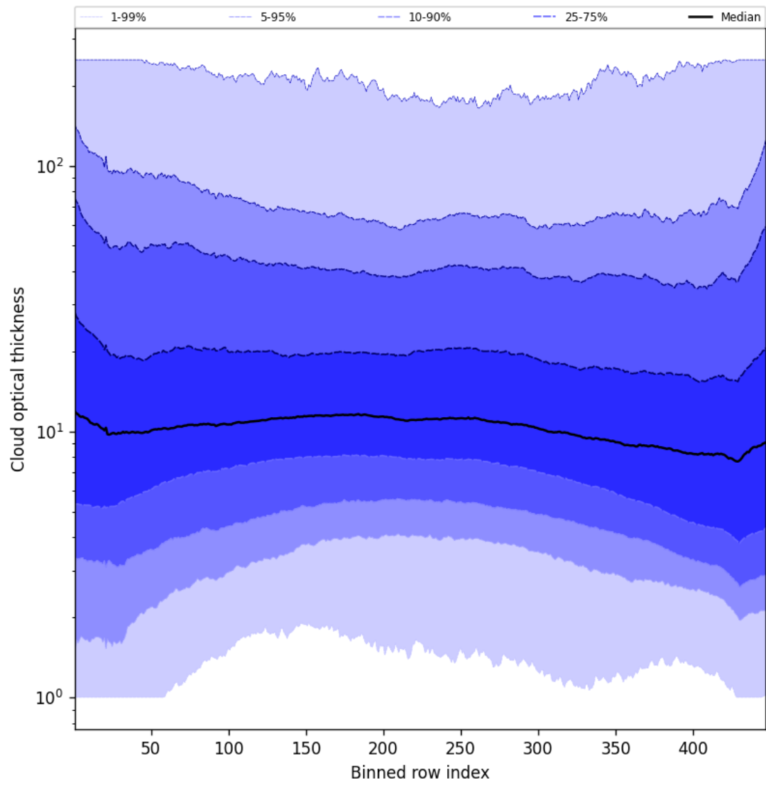
Figure 57: Along track statistics of “Cloud optical thickness” for 2025-07-14 to 2025-07-16
