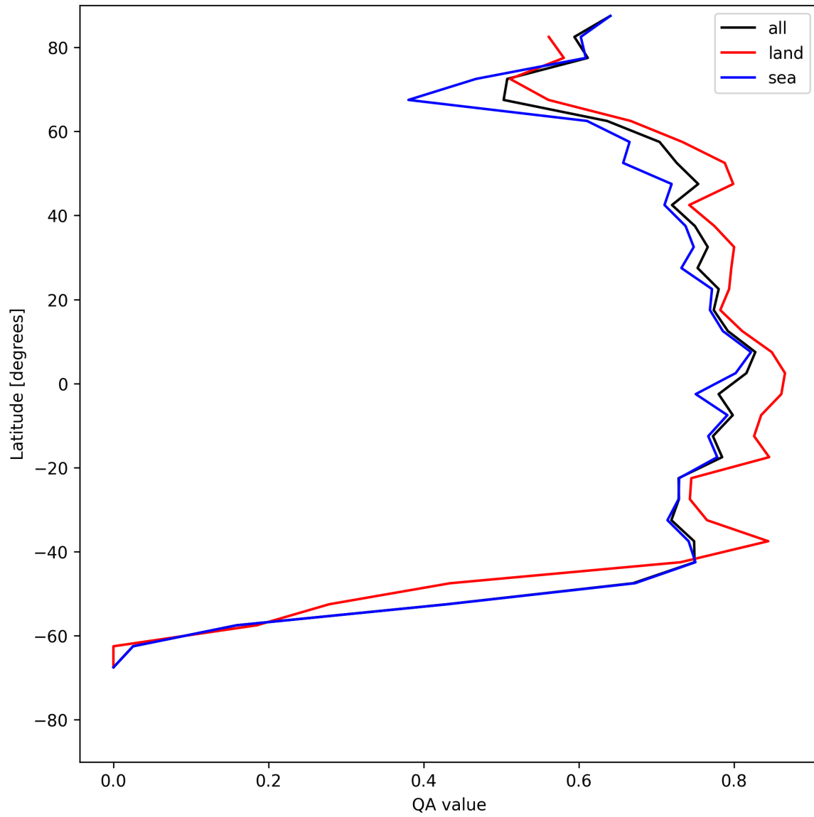
Figure 22: Zonal average of “QA value” for 2025-07-14 to 2025-07-16.
