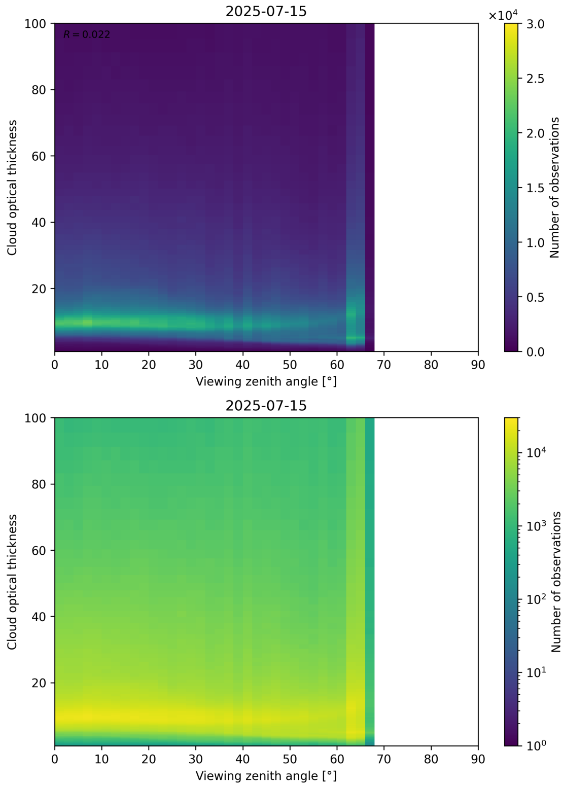
Figure 111: Scatter density plot of “Viewing zenith angle” against “Cloud optical thickness” for 2025-07-14 to 2025-07-16.
