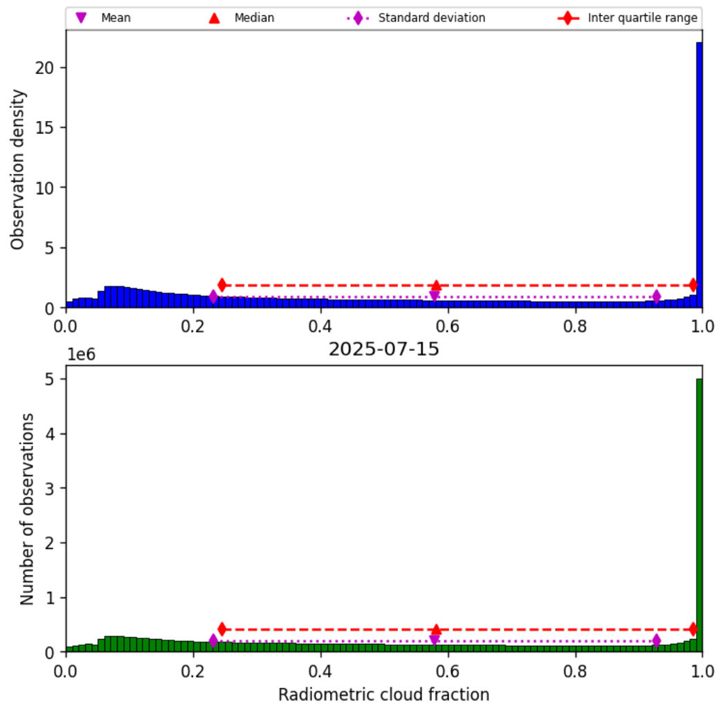
Figure 39: Histogram of “Radiometric cloud fraction” for 2025-07-14 to 2025-07-16
