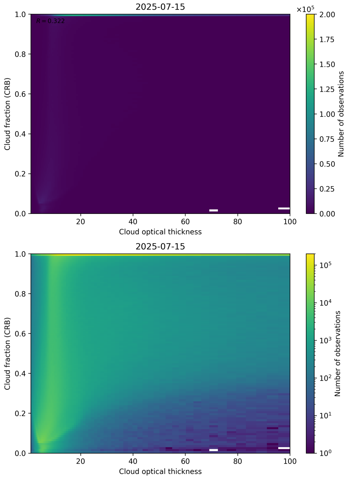
Figure 84: Scatter density plot of “Cloud optical thickness” against “Cloud fraction (CRB)” for 2025-07-14 to 2025-07-16.
