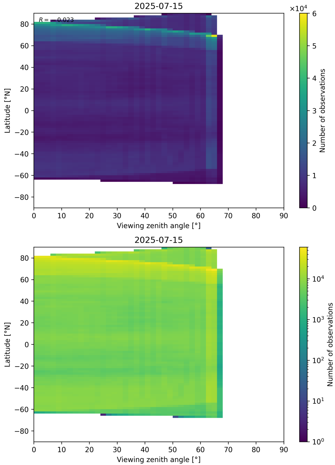
Figure 113: Scatter density plot of “Viewing zenith angle” against “Latitude” for 2025-07-14 to 2025-07-16.
