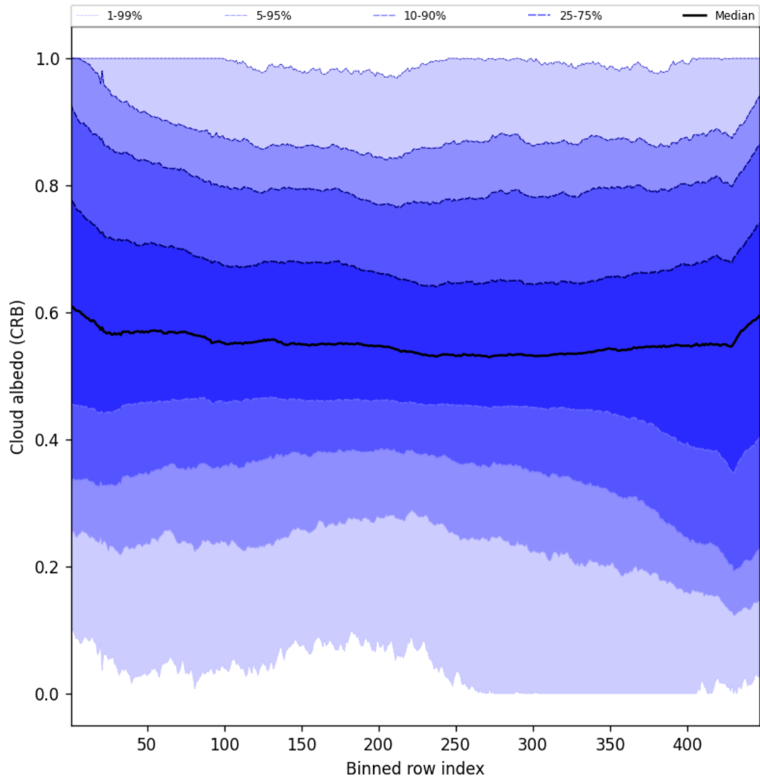
Figure 60: Along track statistics of “Cloud albedo (CRB)” for 2025-07-14 to 2025-07-16
