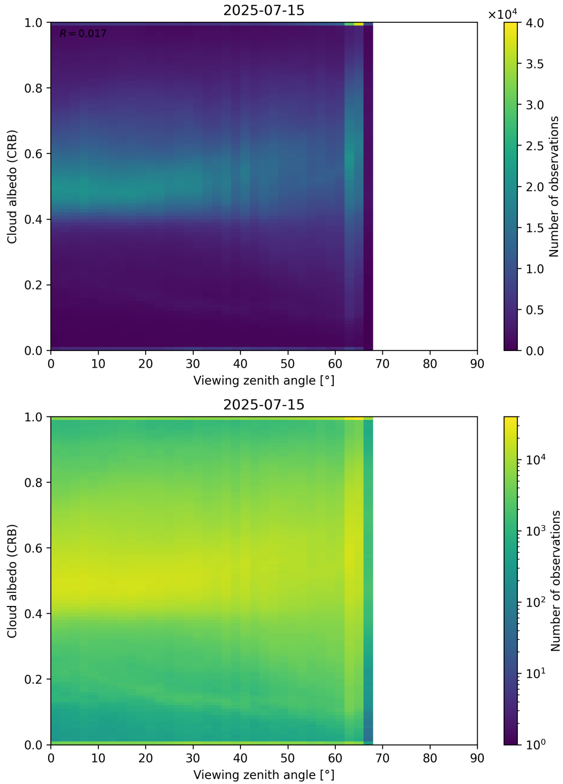
Figure 106: Scatter density plot of “Viewing zenith angle” against “Cloud albedo (CRB)” for 2025-07-14 to 2025-07-16.
