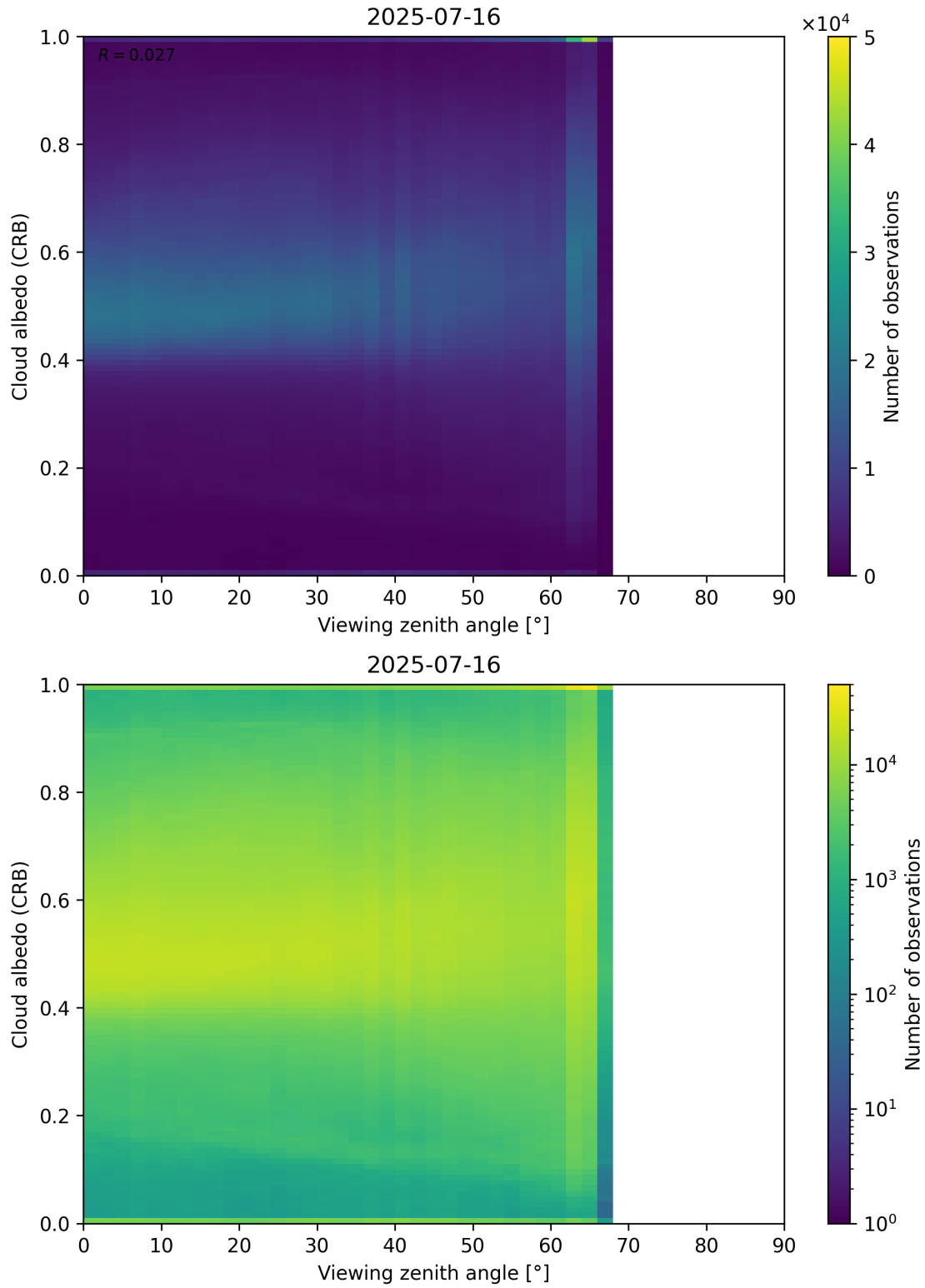
Figure 106: Scatter density plot of “Viewing zenith angle” against “Cloud albedo (CRB)” for 2025-07-15 to 2025-07-17.
