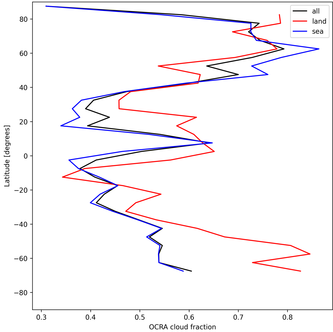
Figure 34: Zonal average of “OCRA cloud fraction” for 2025-07-15 to 2025-07-17.
