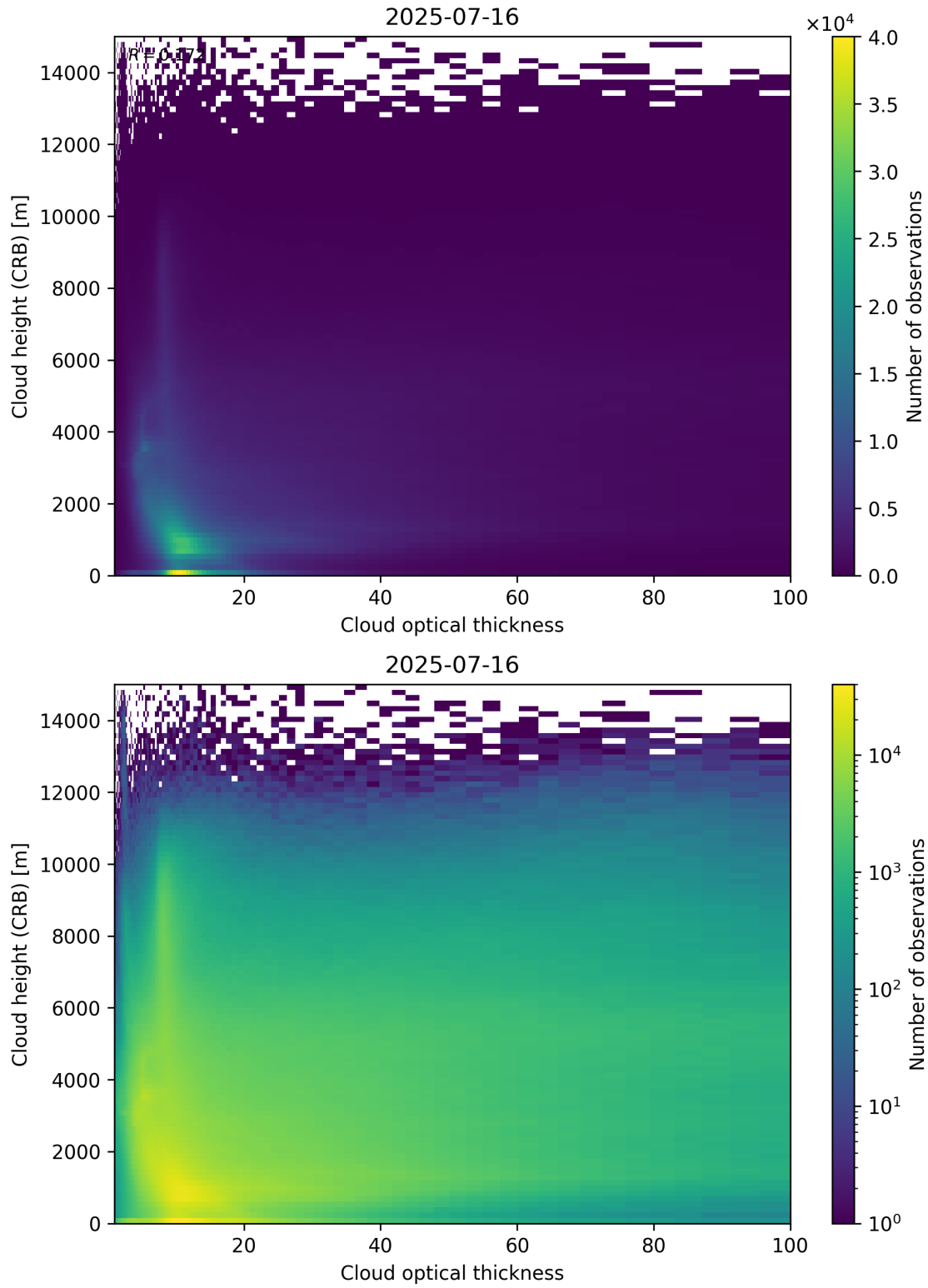
Figure 85: Scatter density plot of “Cloud optical thickness” against “Cloud height (CRB)” for 2025-07-15 to 2025-07-17.
