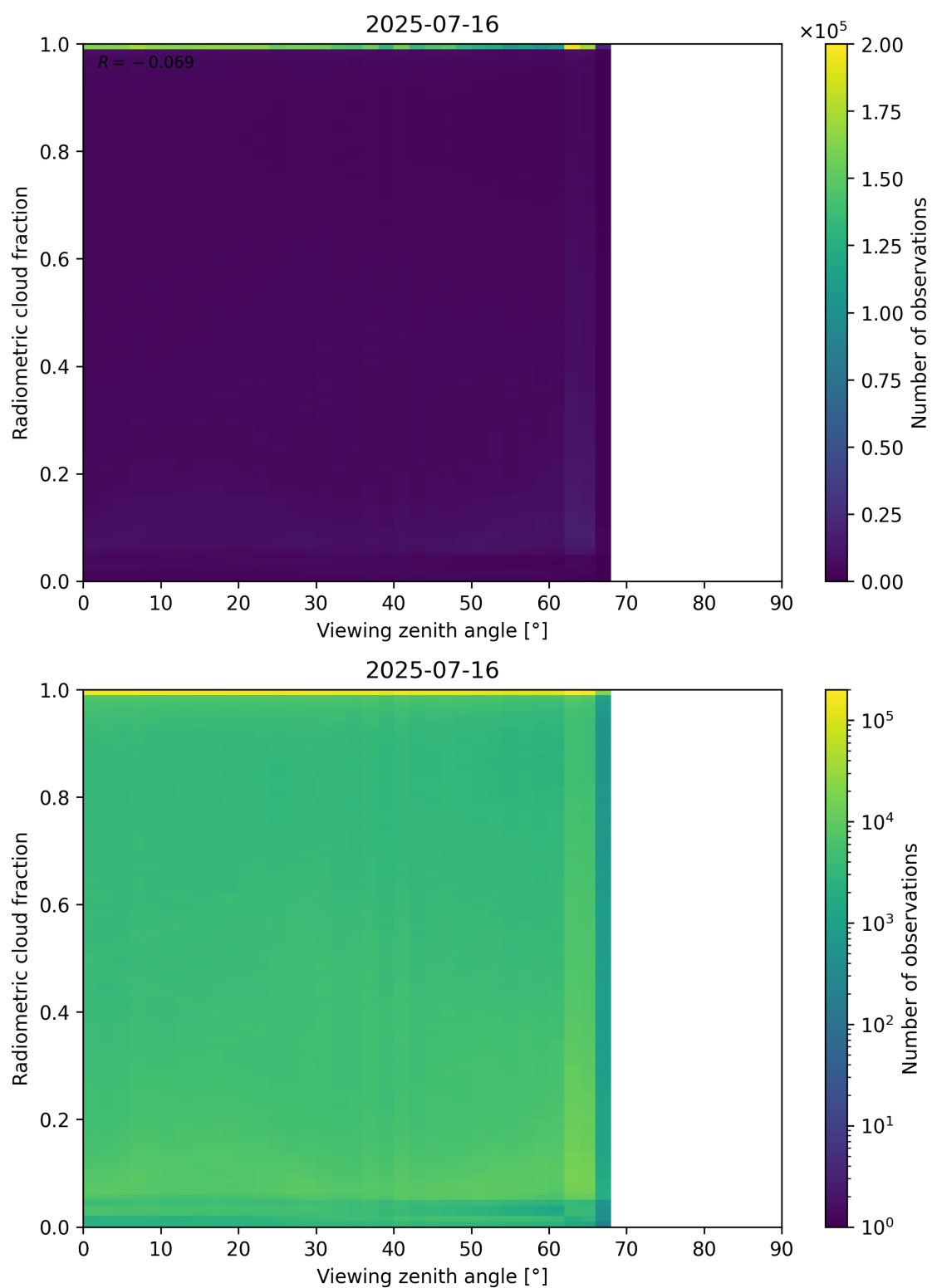
Figure 107: Scatter density plot of “Viewing zenith angle” against “Radiometric cloud fraction” for 2025-07-15 to 2025-07-17.
