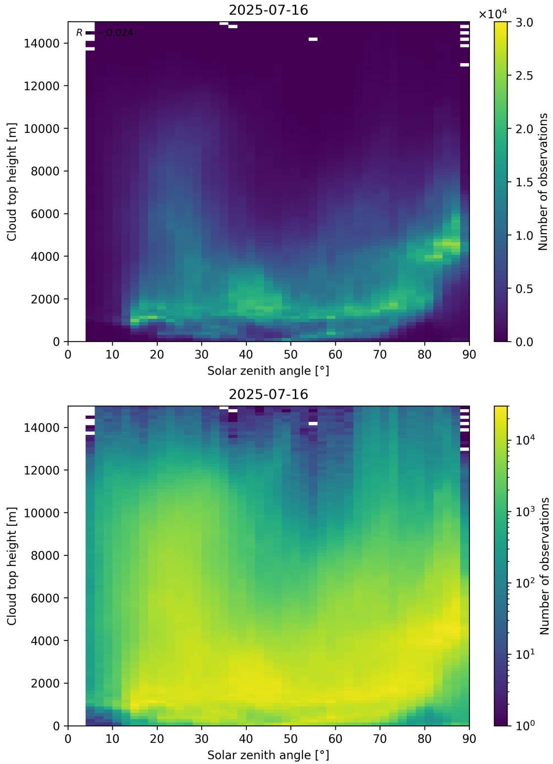
Figure 104: Scatter density plot of “Solar zenith angle” against “Cloud top height” for 2025-07-15 to 2025-07-17.
