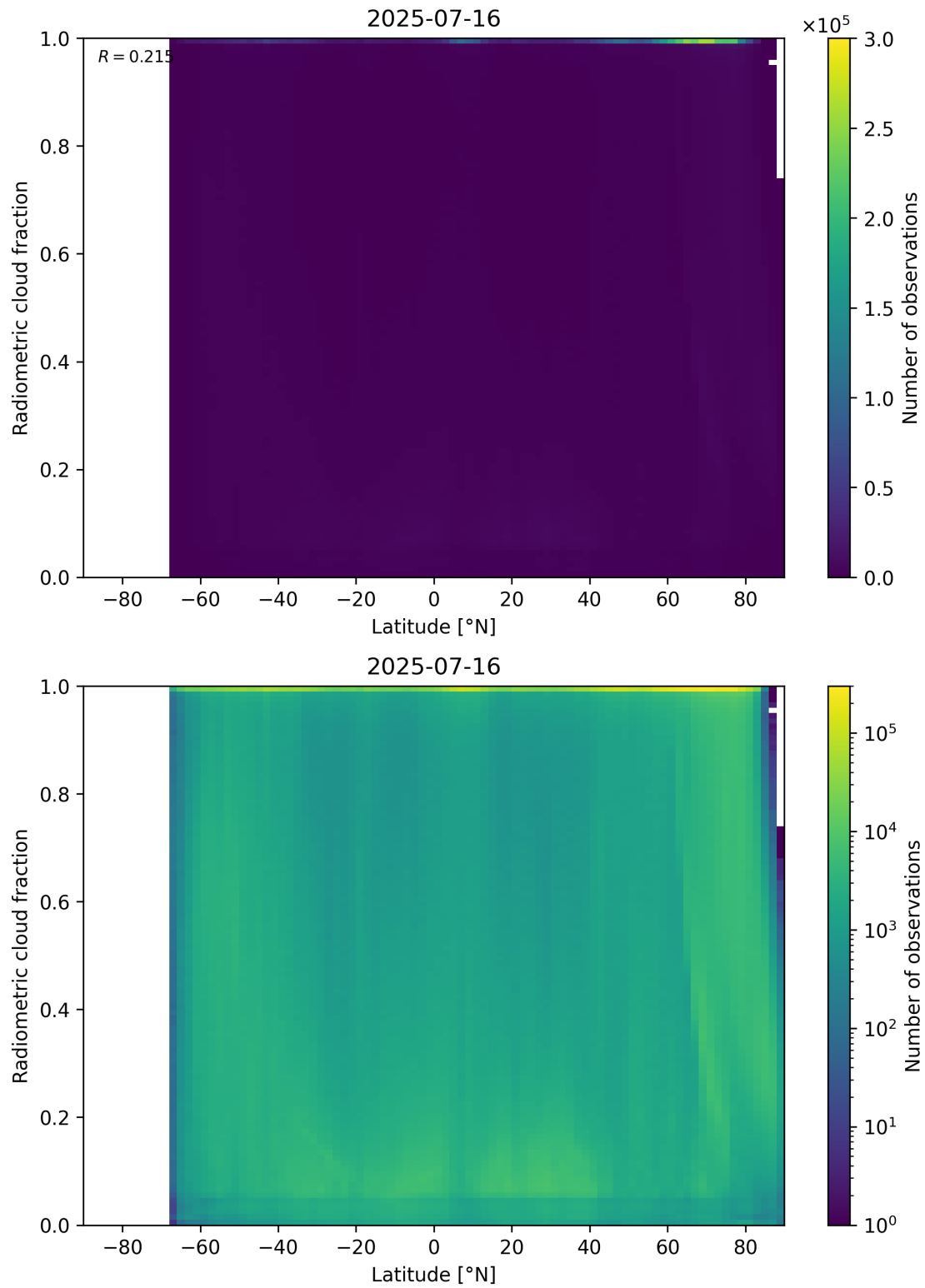
Figure 92: Scatter density plot of “Latitude” against “Radiometric cloud fraction” for 2025-07-15 to 2025-07-17.
