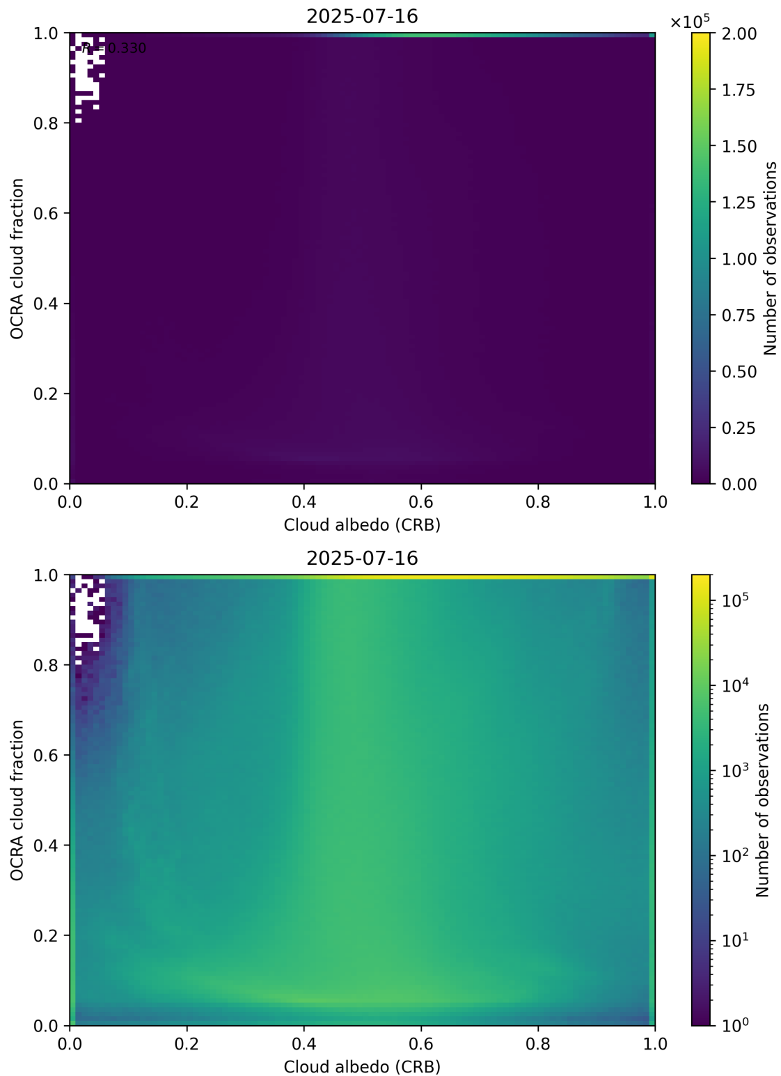
Figure 70: Scatter density plot of “Cloud albedo (CRB)” against “OCRA cloud fraction” for 2025-07-15 to 2025-07-17.
