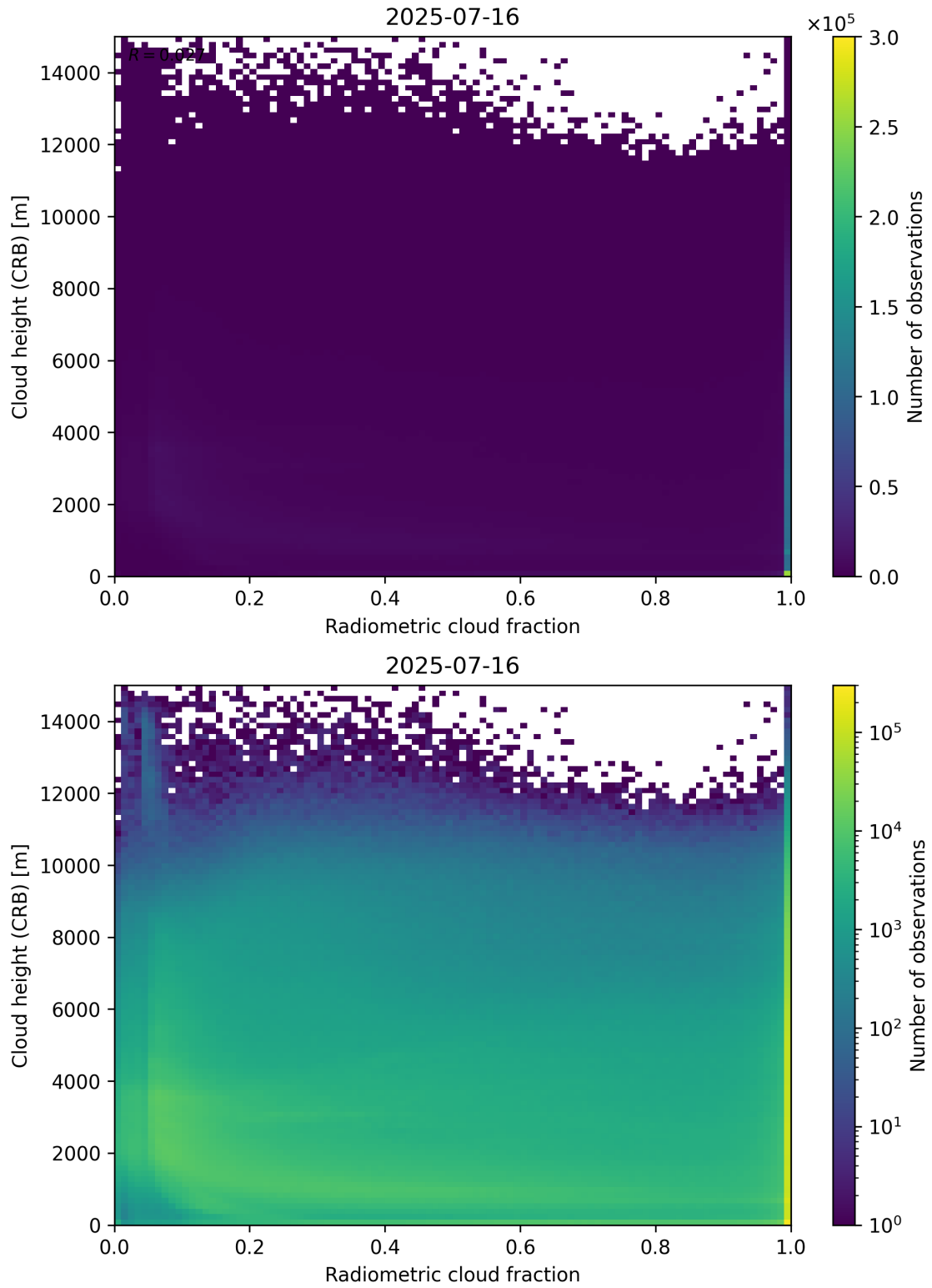
Figure 74: Scatter density plot of “Radiometric cloud fraction” against “Cloud height (CRB)” for 2025-07-15 to 2025-07-17.
