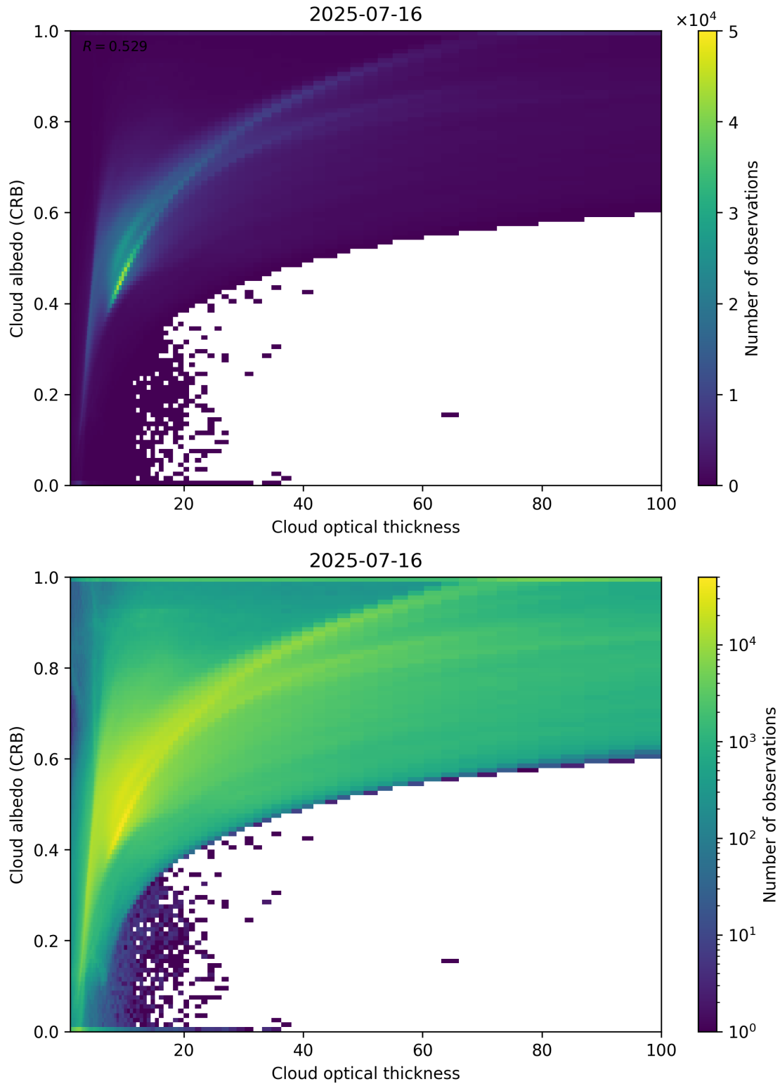
Figure 82: Scatter density plot of “Cloud optical thickness” against “Cloud albedo (CRB)” for 2025-07-15 to 2025-07-17.
