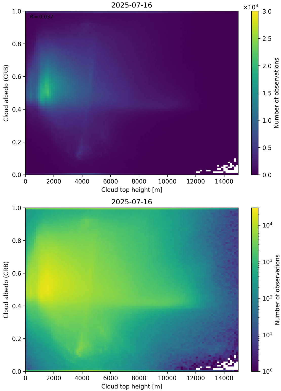
Figure 86: Scatter density plot of “Cloud top height” against “Cloud albedo (CRB)” for 2025-07-15 to 2025-07-17.
