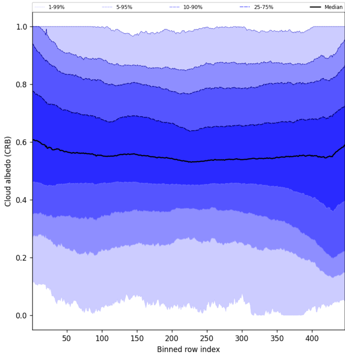
Figure 60: Along track statistics of “Cloud albedo (CRB)” for 2025-07-15 to 2025-07-17
