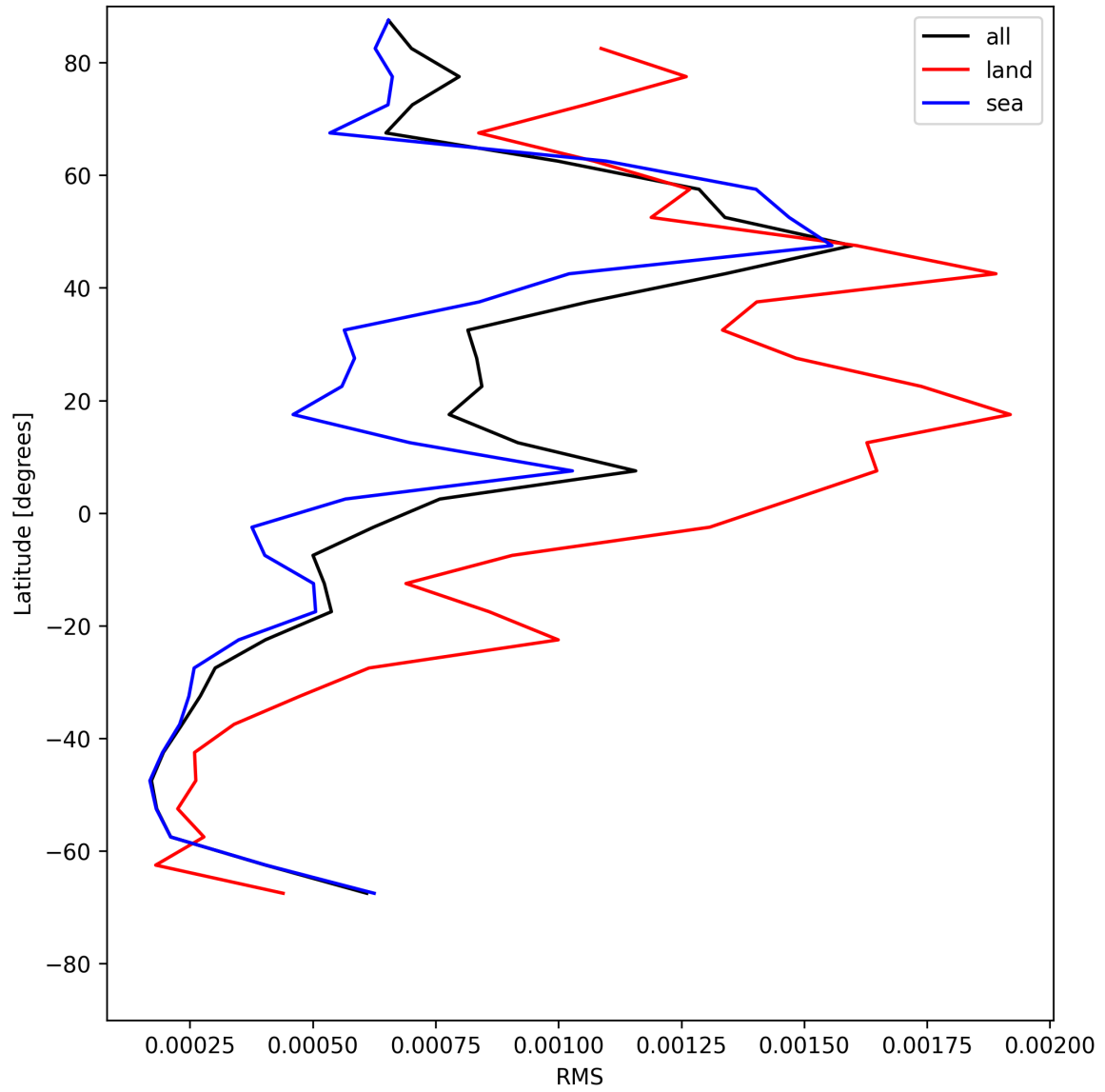
Figure 31: Zonal average of “RMS” for 2025-07-15 to 2025-07-17.
