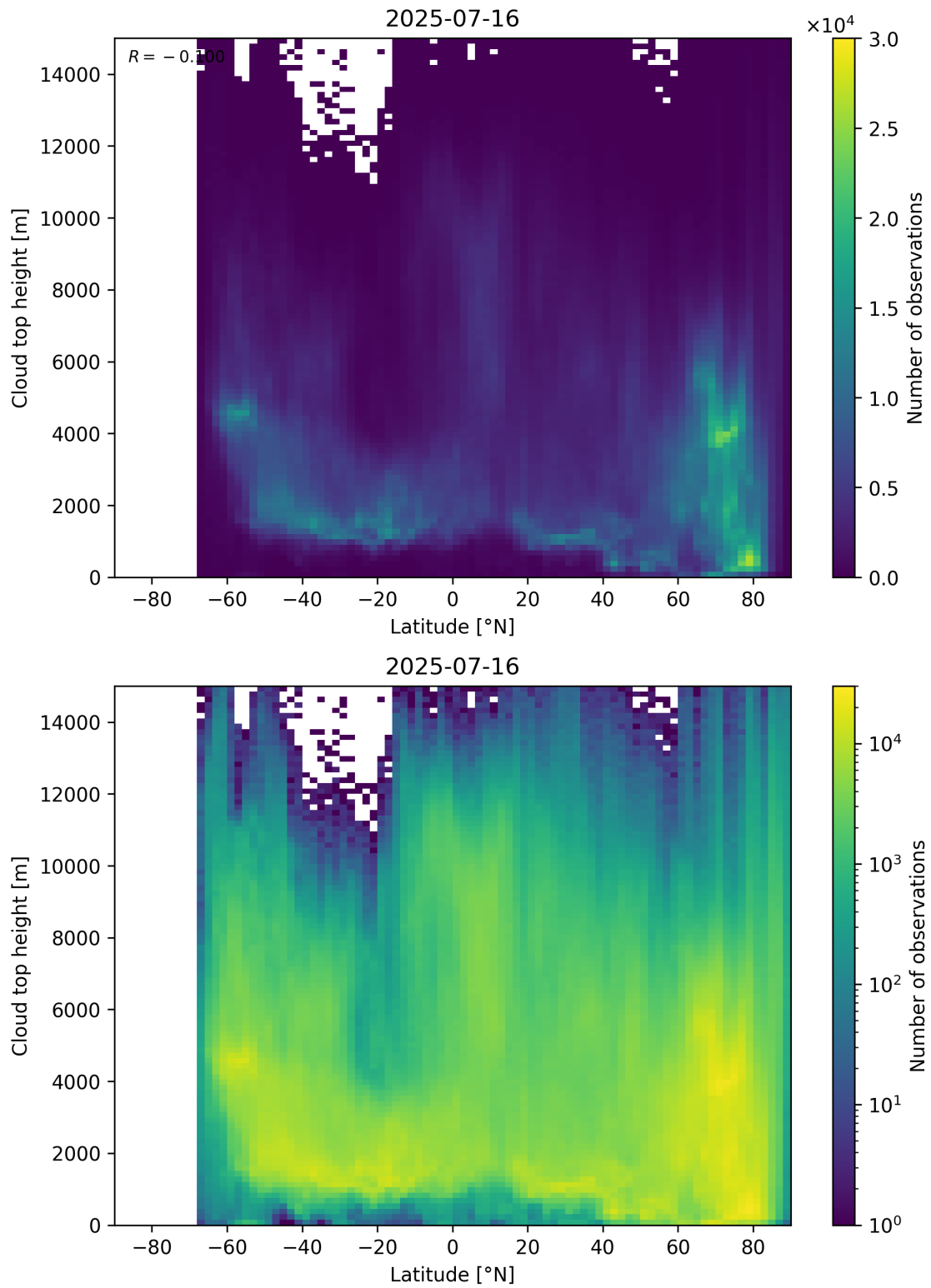
Figure 97: Scatter density plot of “Latitude” against “Cloud top height” for 2025-07-15 to 2025-07-17.
