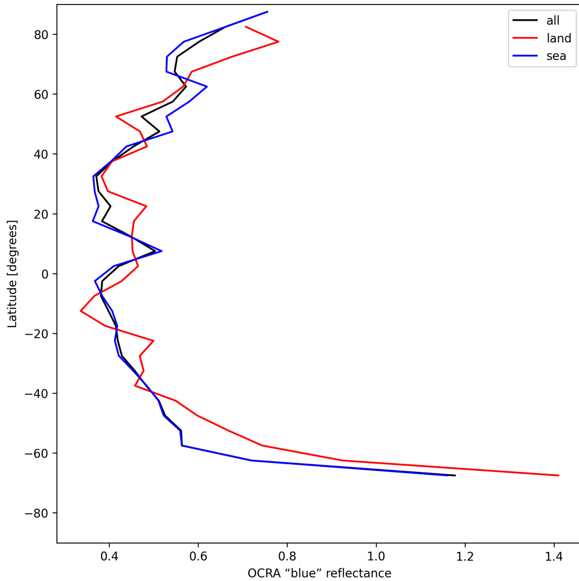
Figure 35: Zonal average of “OCRA “blue” reflectance” for 2025-07-15 to 2025-07-17.
