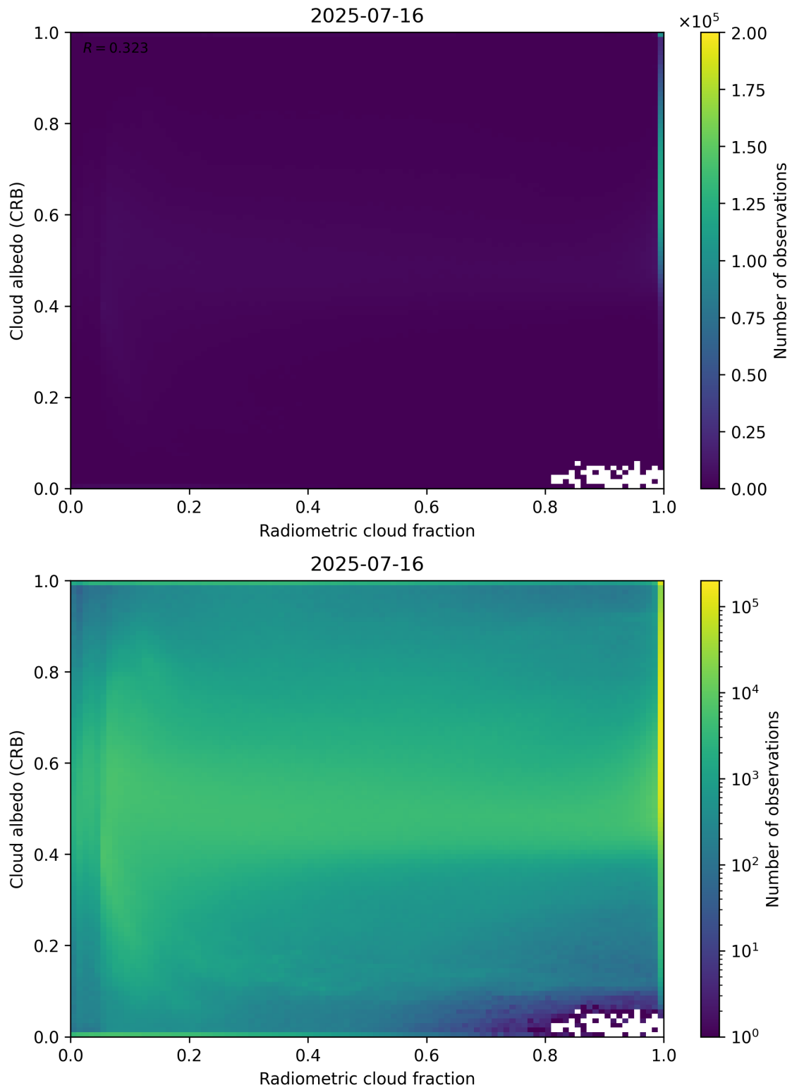
Figure 71: Scatter density plot of “Radiometric cloud fraction” against “Cloud albedo (CRB)” for 2025-07-15 to 2025-07-17.
