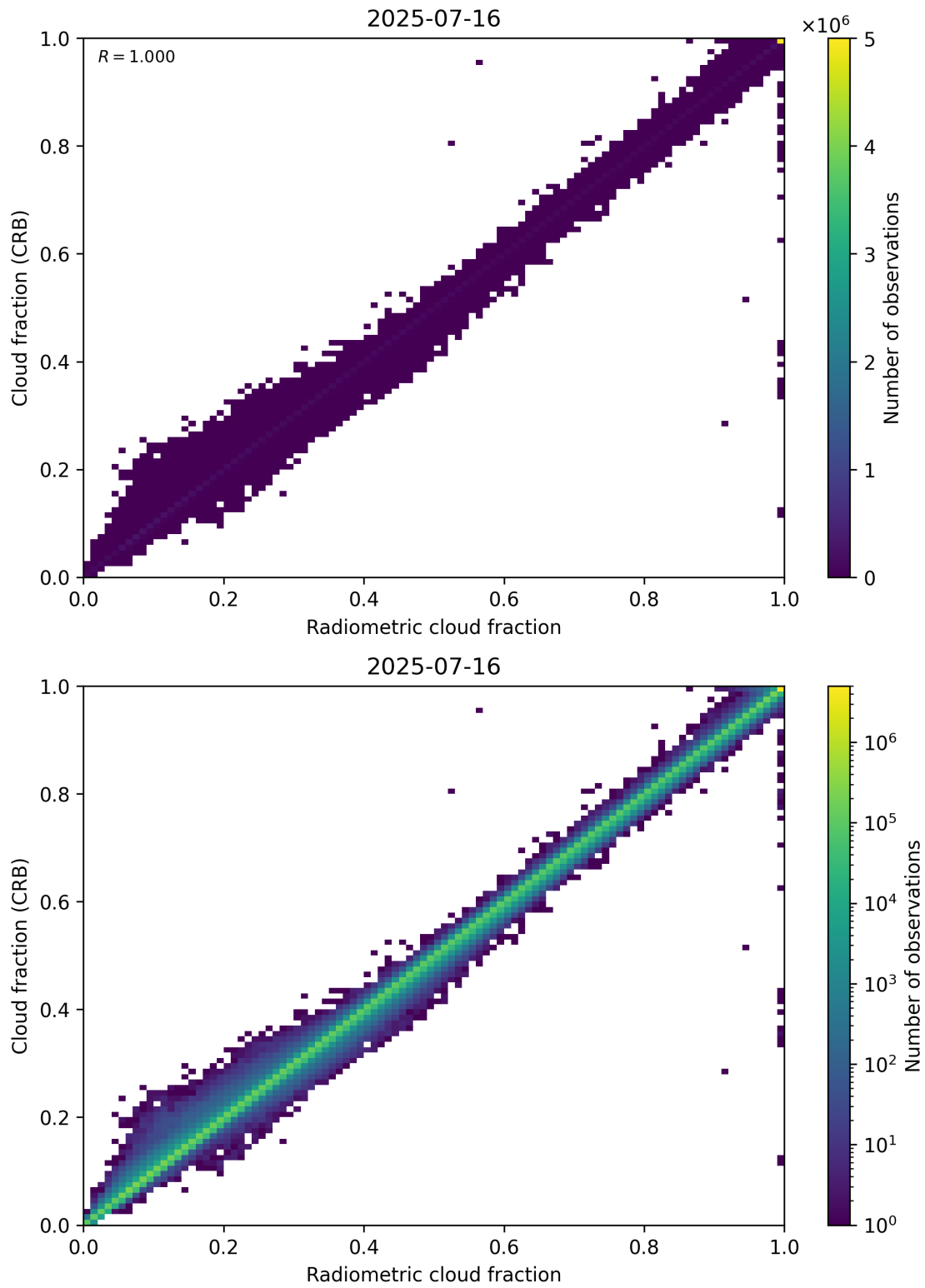
Figure 73: Scatter density plot of “Radiometric cloud fraction” against “Cloud fraction (CRB)” for 2025-07-15 to 2025-07-17.
