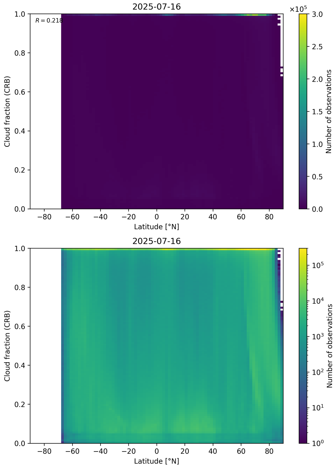
Figure 94: Scatter density plot of “Latitude” against “Cloud fraction (CRB)” for 2025-07-15 to 2025-07-17.
