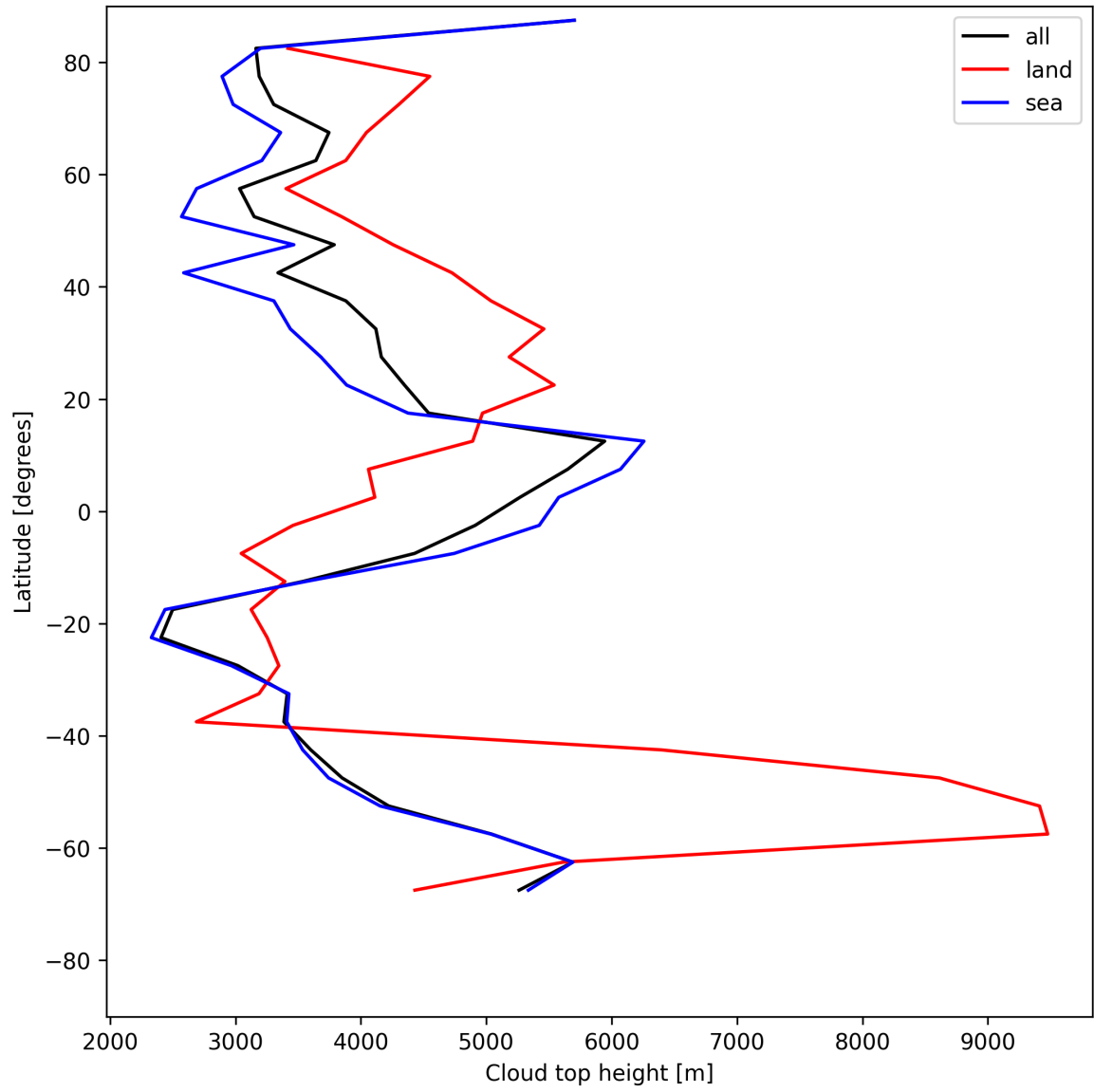
Figure 24: Zonal average of “Cloud top height” for 2025-07-15 to 2025-07-17.
