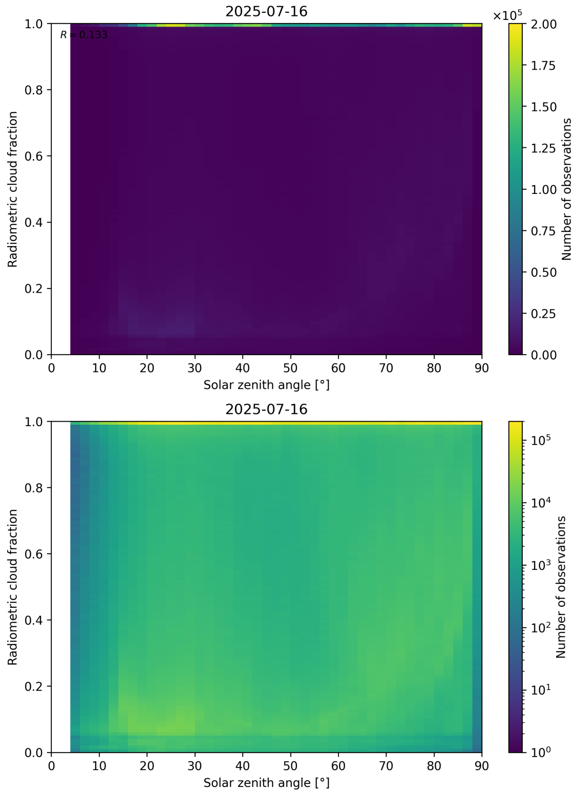
Figure 99: Scatter density plot of “Solar zenith angle” against “Radiometric cloud fraction” for 2025-07-15 to 2025-07-17.
