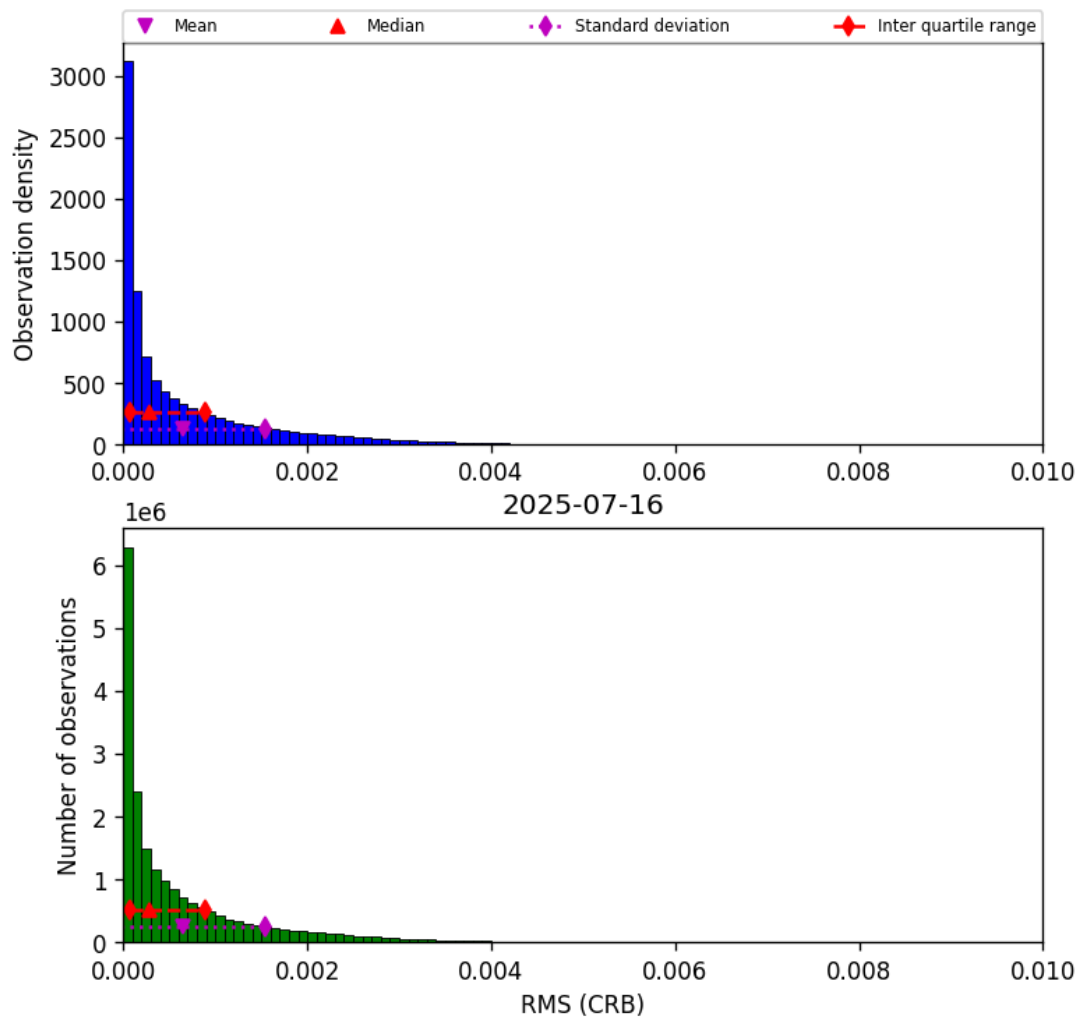
Figure 48: Histogram of “RMS (CRB)” for 2025-07-15 to 2025-07-17
