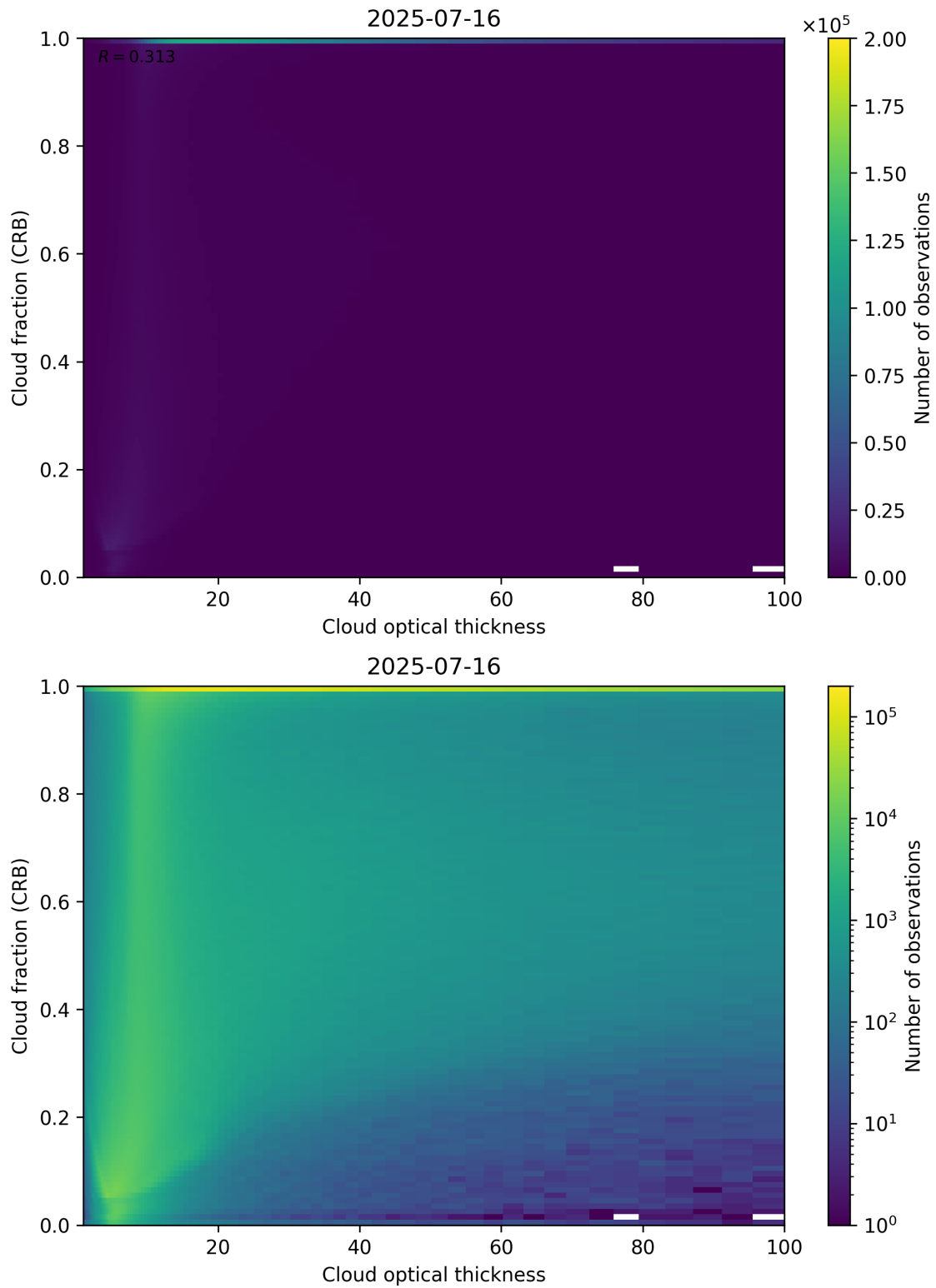
Figure 84: Scatter density plot of “Cloud optical thickness” against “Cloud fraction (CRB)” for 2025-07-15 to 2025-07-17.
