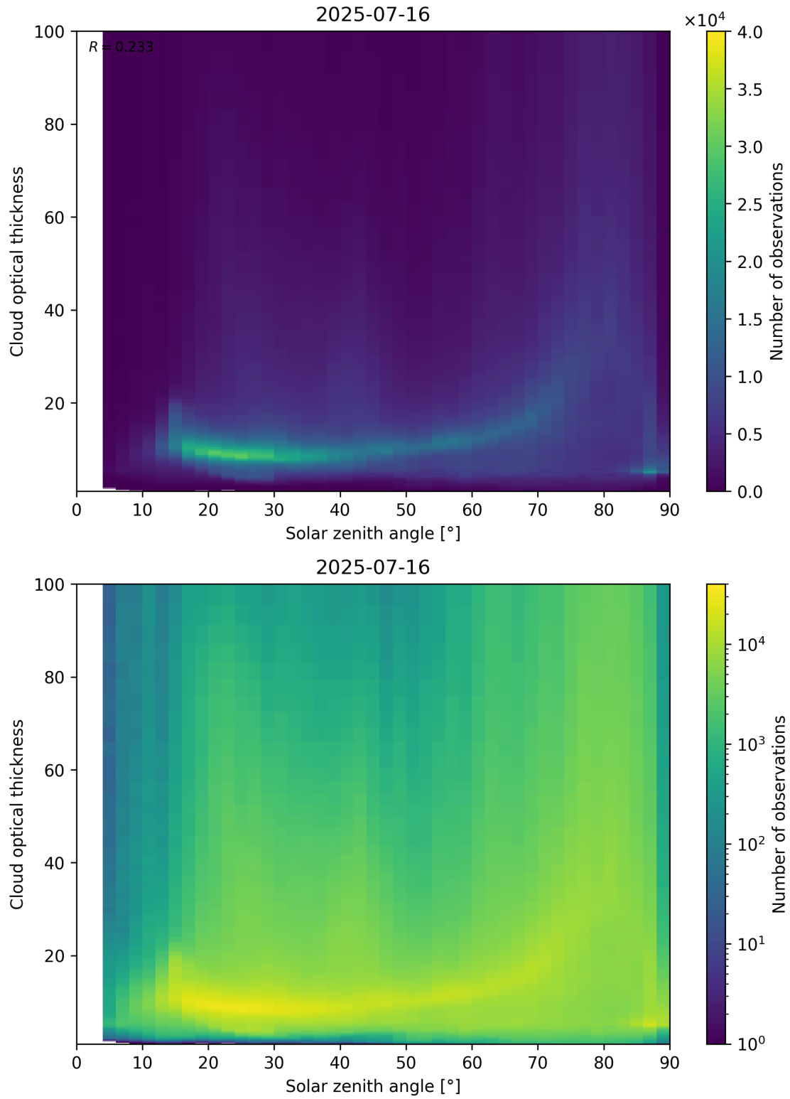
Figure 103: Scatter density plot of “Solar zenith angle” against “Cloud optical thickness” for 2025-07-15 to 2025-07-17.
