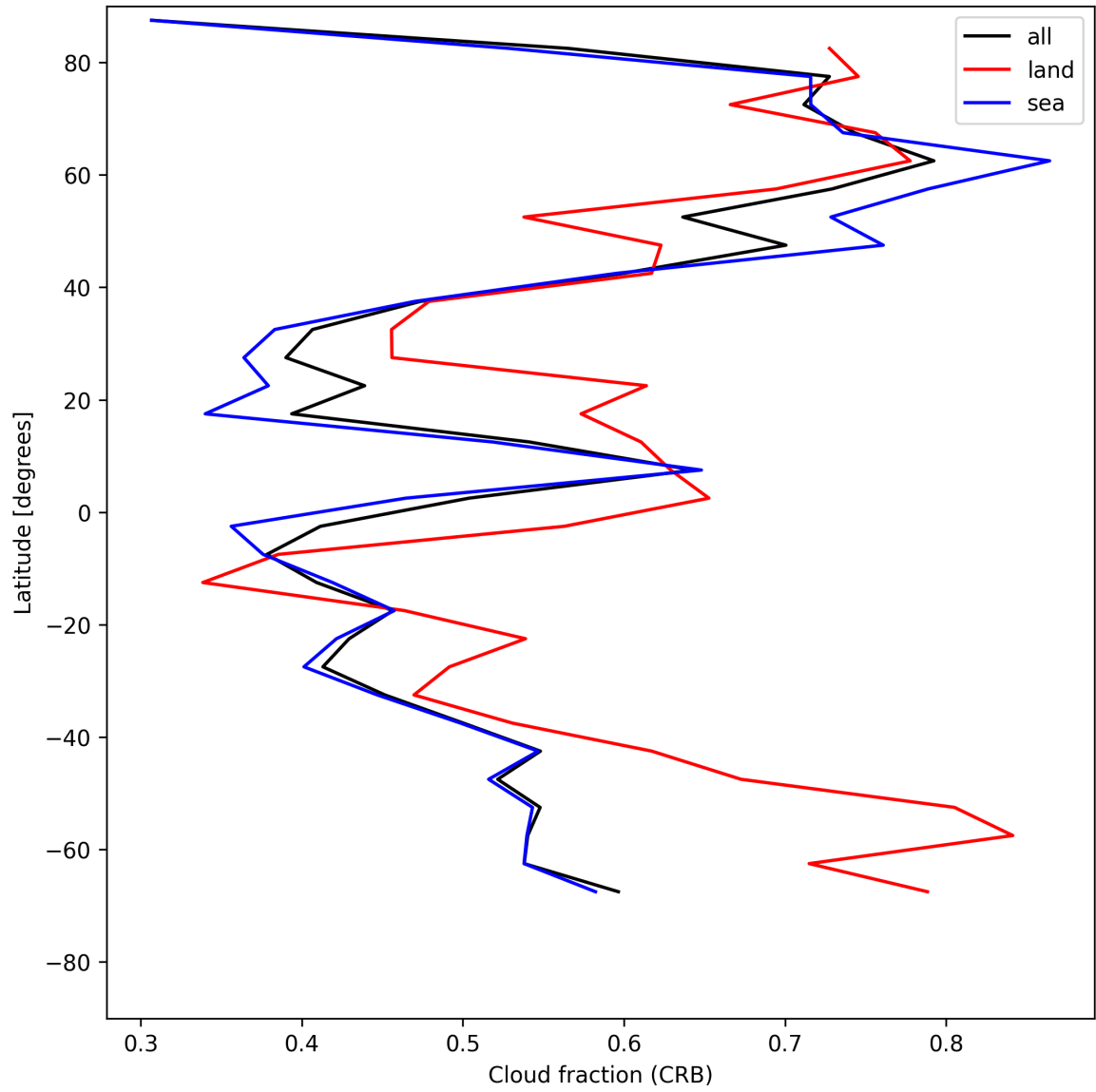
Figure 26: Zonal average of “Cloud fraction (CRB)” for 2025-07-15 to 2025-07-17.
