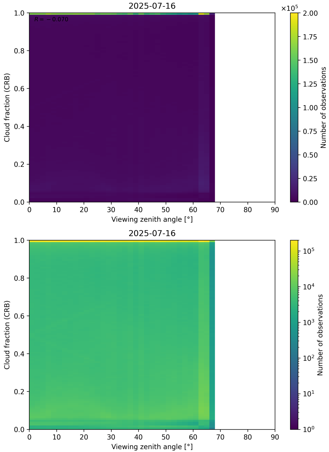
Figure 109: Scatter density plot of “Viewing zenith angle” against “Cloud fraction (CRB)” for 2025-07-15 to 2025-07-17.
