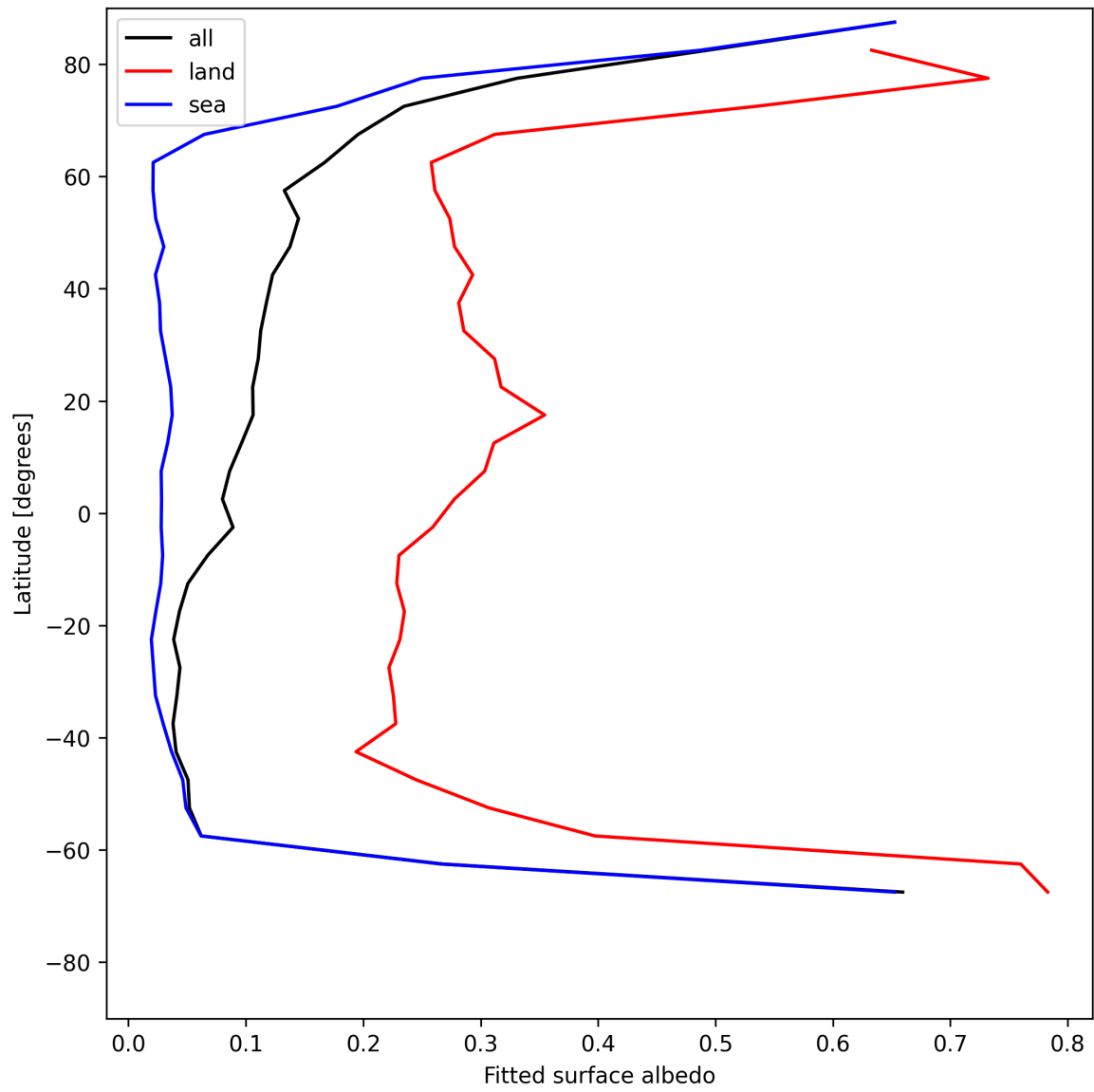
Figure 29: Zonal average of “Fitted surface albedo” for 2025-07-15 to 2025-07-17.
