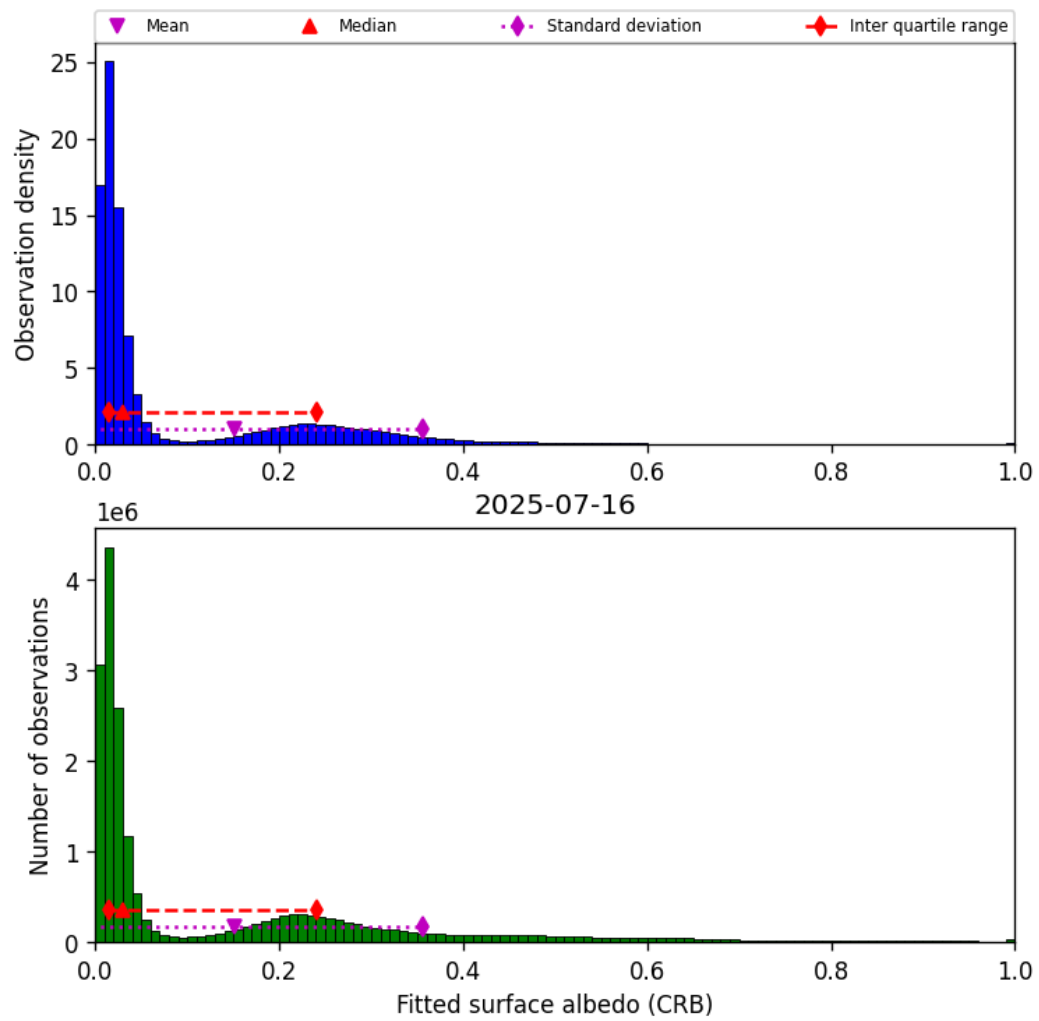
Figure 46: Histogram of “Fitted surface albedo (CRB)” for 2025-07-15 to 2025-07-17
