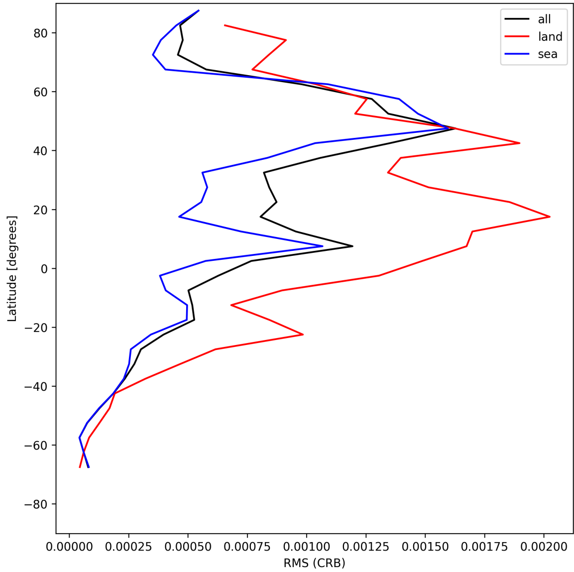
Figure 32: Zonal average of “RMS (CRB)” for 2025-07-15 to 2025-07-17.
