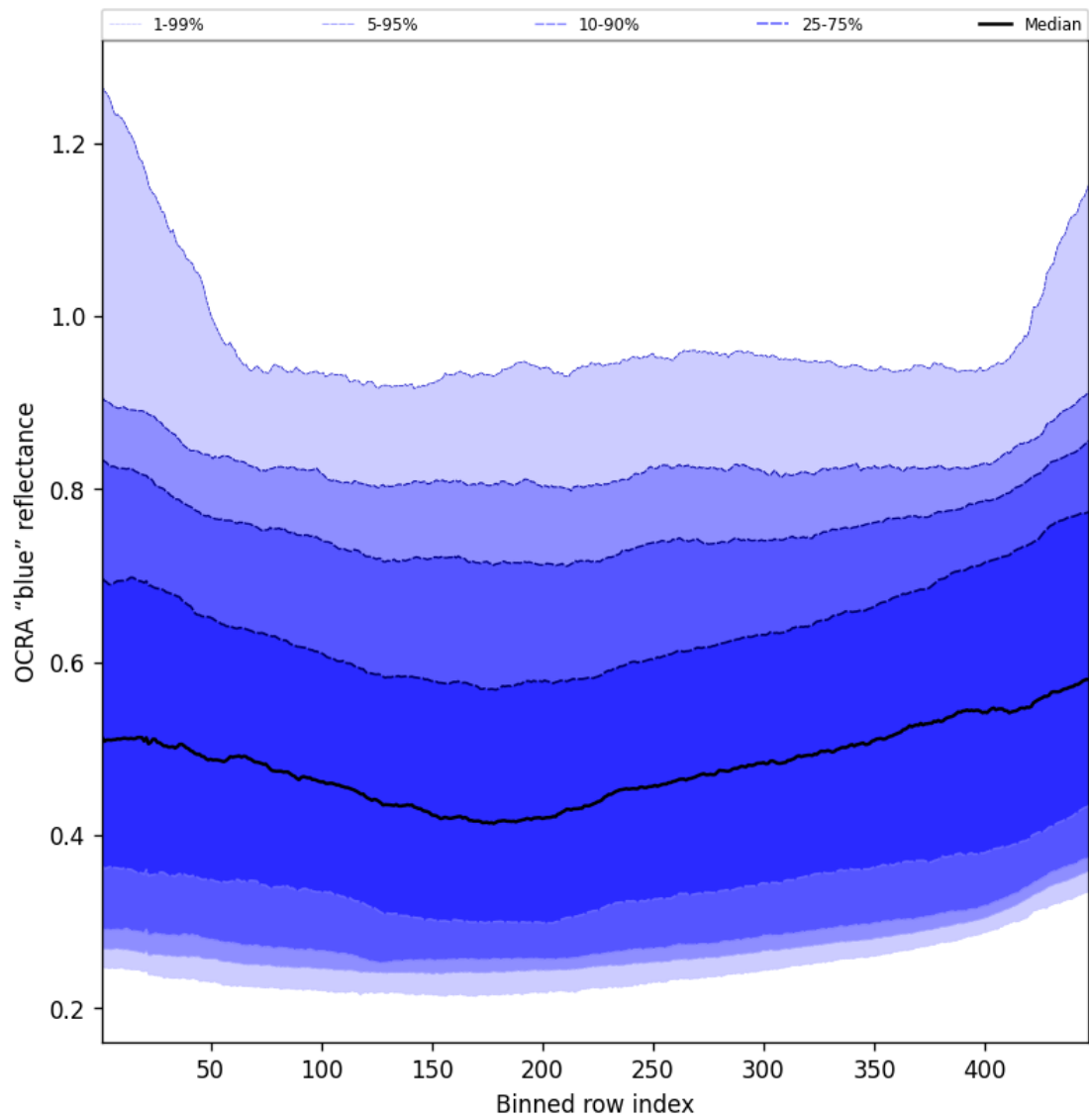
Figure 67: Along track statistics of “OCRA “blue” reflectance” for 2025-07-15 to 2025-07-17
