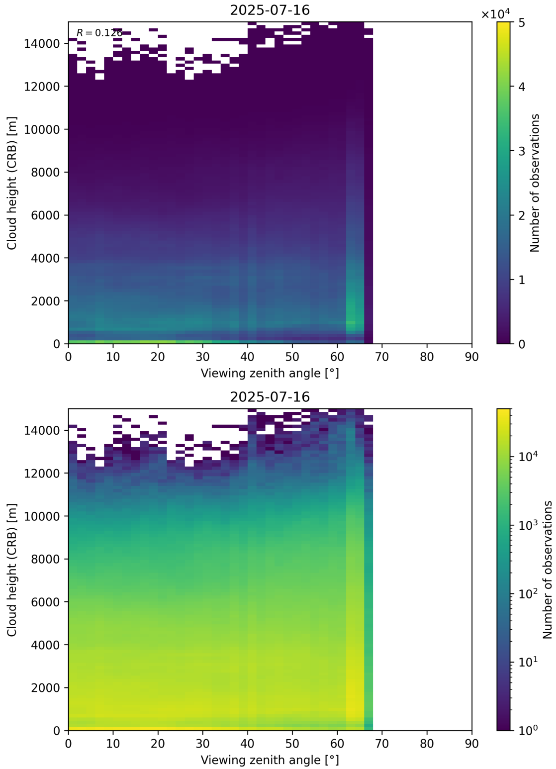
Figure 110: Scatter density plot of “Viewing zenith angle” against “Cloud height (CRB)” for 2025-07-15 to 2025-07-17.
