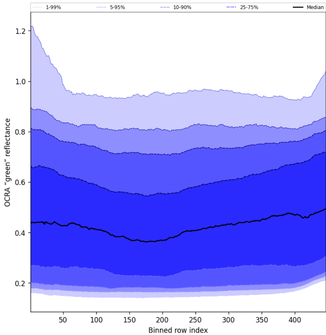
Figure 68: Along track statistics of “OCRA “green” reflectance” for 2025-07-15 to 2025-07-17
