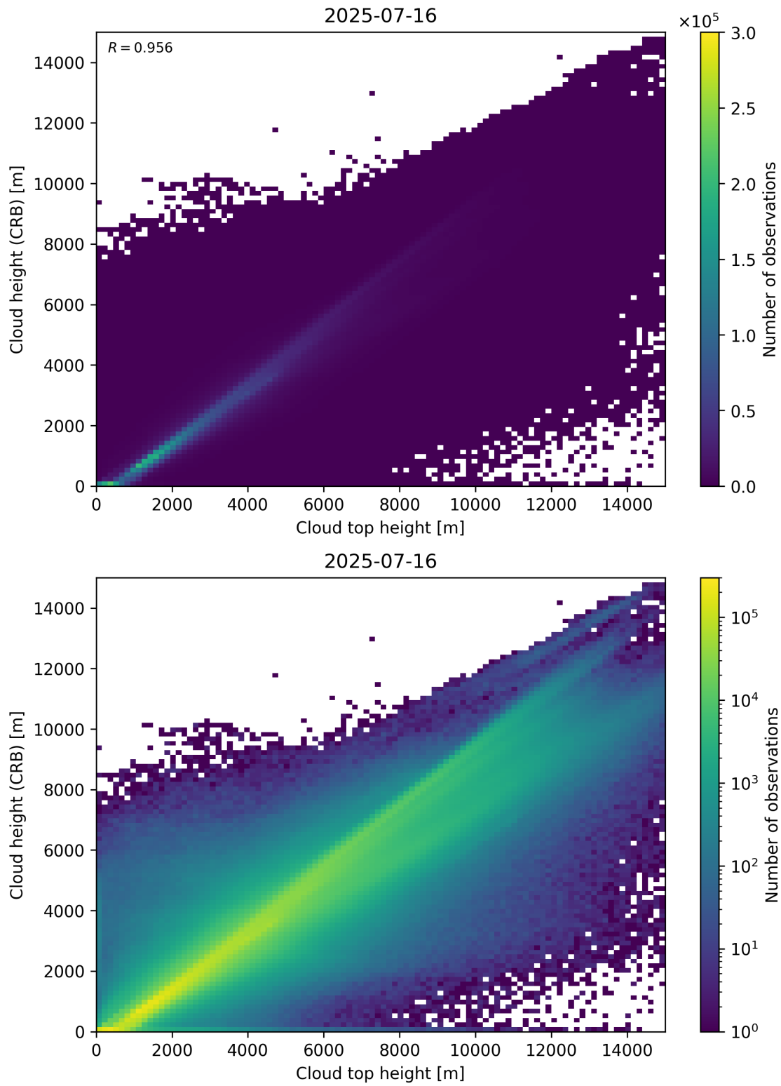
Figure 89: Scatter density plot of “Cloud top height” against “Cloud height (CRB)” for 2025-07-15 to 2025-07-17.
