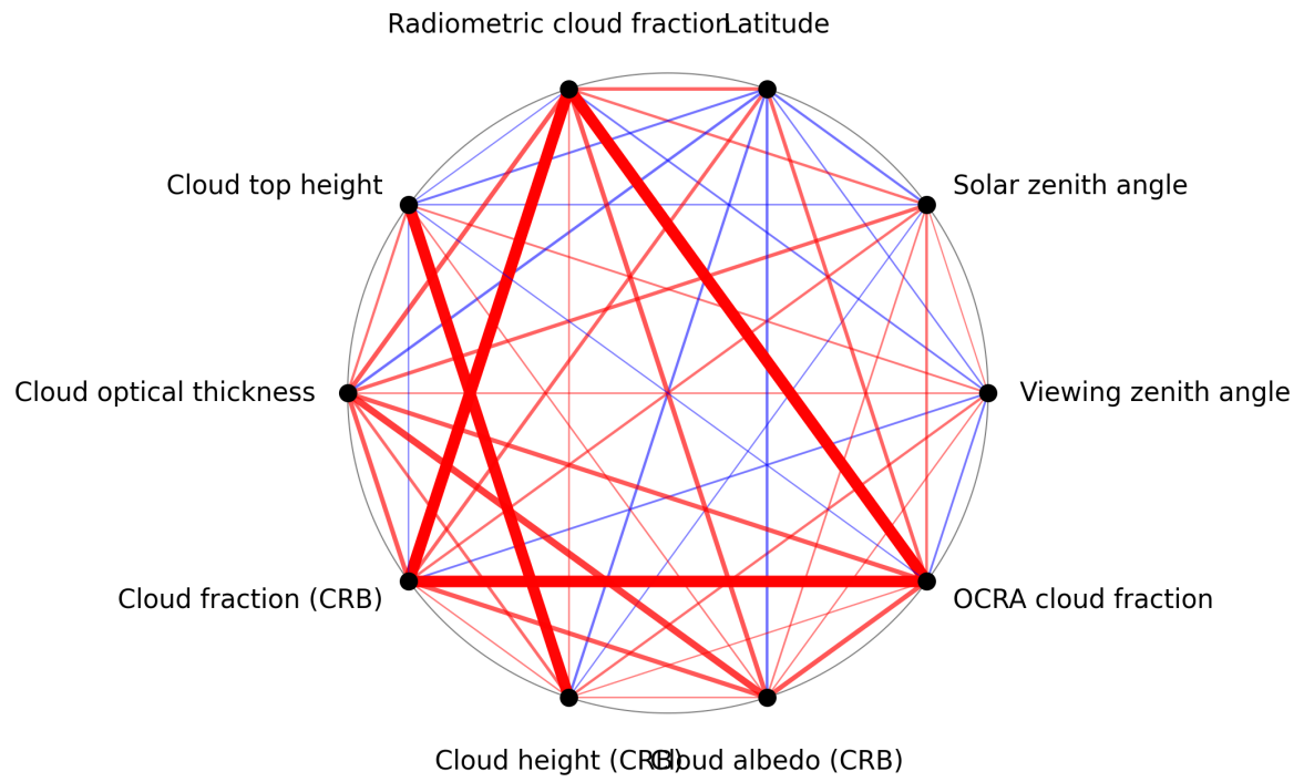
Figure 1: Map of correlation graph for 2025-07-15 to 2025-07-17.
