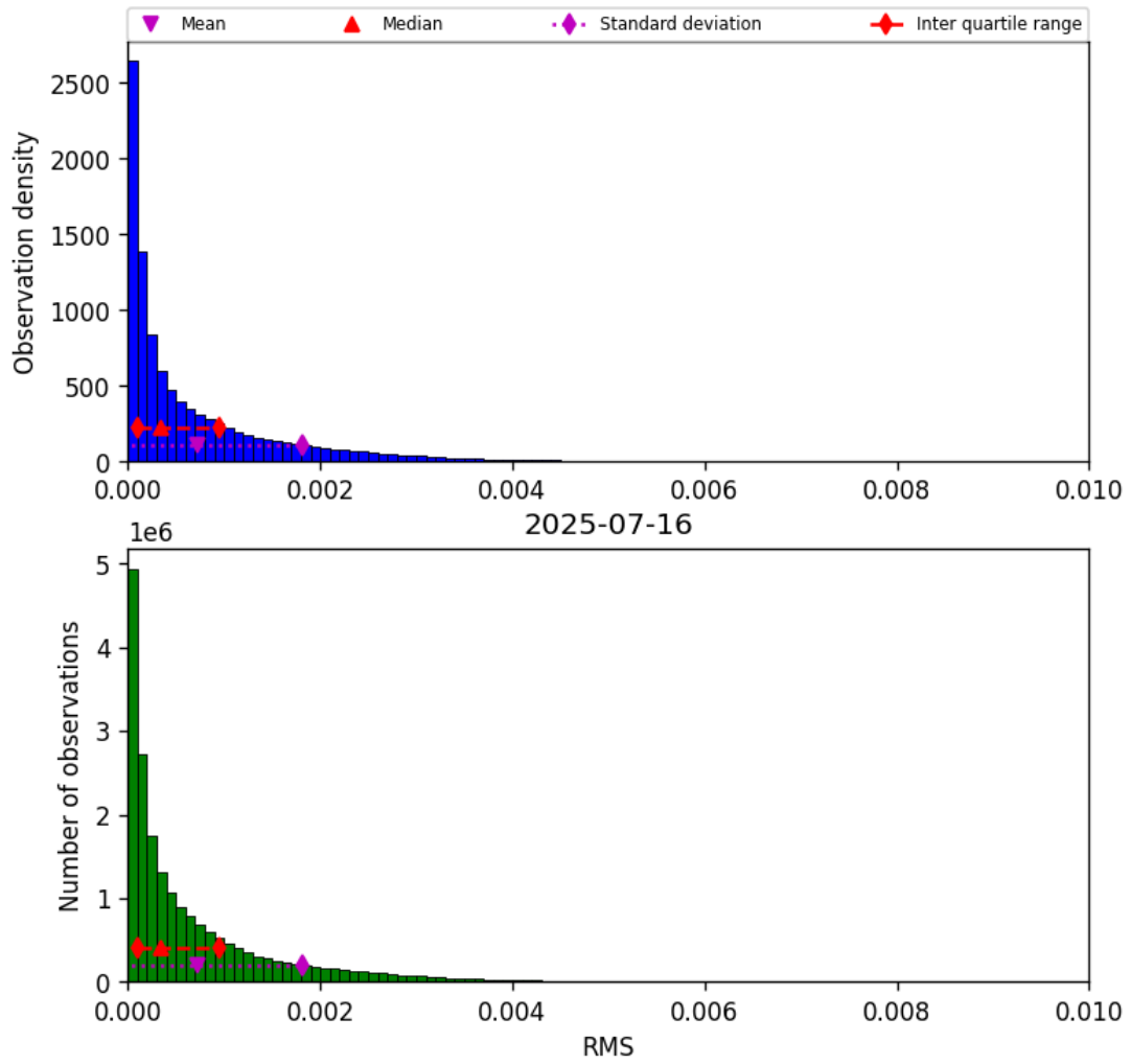
Figure 47: Histogram of “RMS” for 2025-07-15 to 2025-07-17
