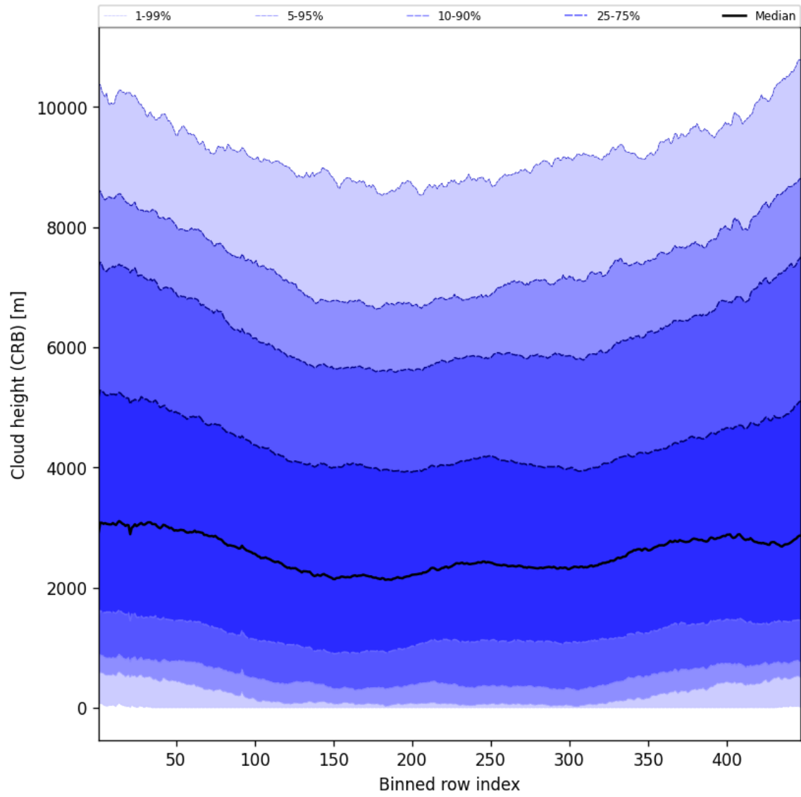
Figure 59: Along track statistics of “Cloud height (CRB)” for 2025-07-15 to 2025-07-17
