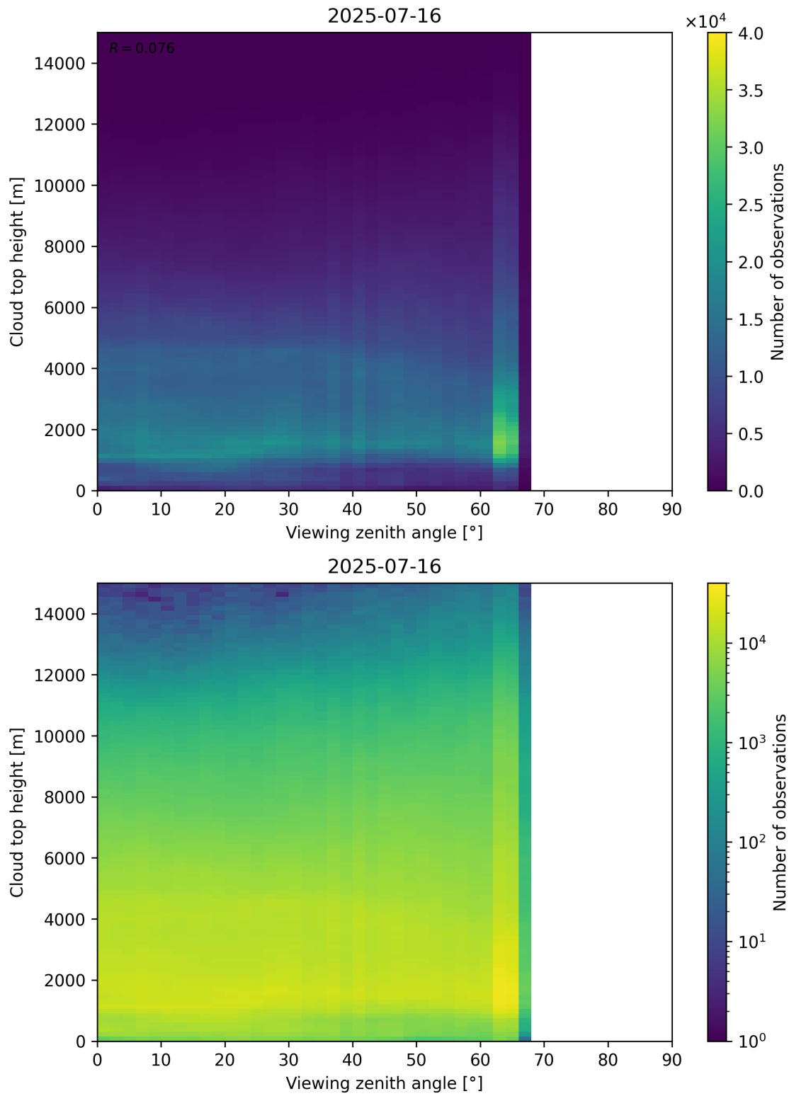
Figure 112: Scatter density plot of “Viewing zenith angle” against “Cloud top height” for 2025-07-15 to 2025-07-17.
