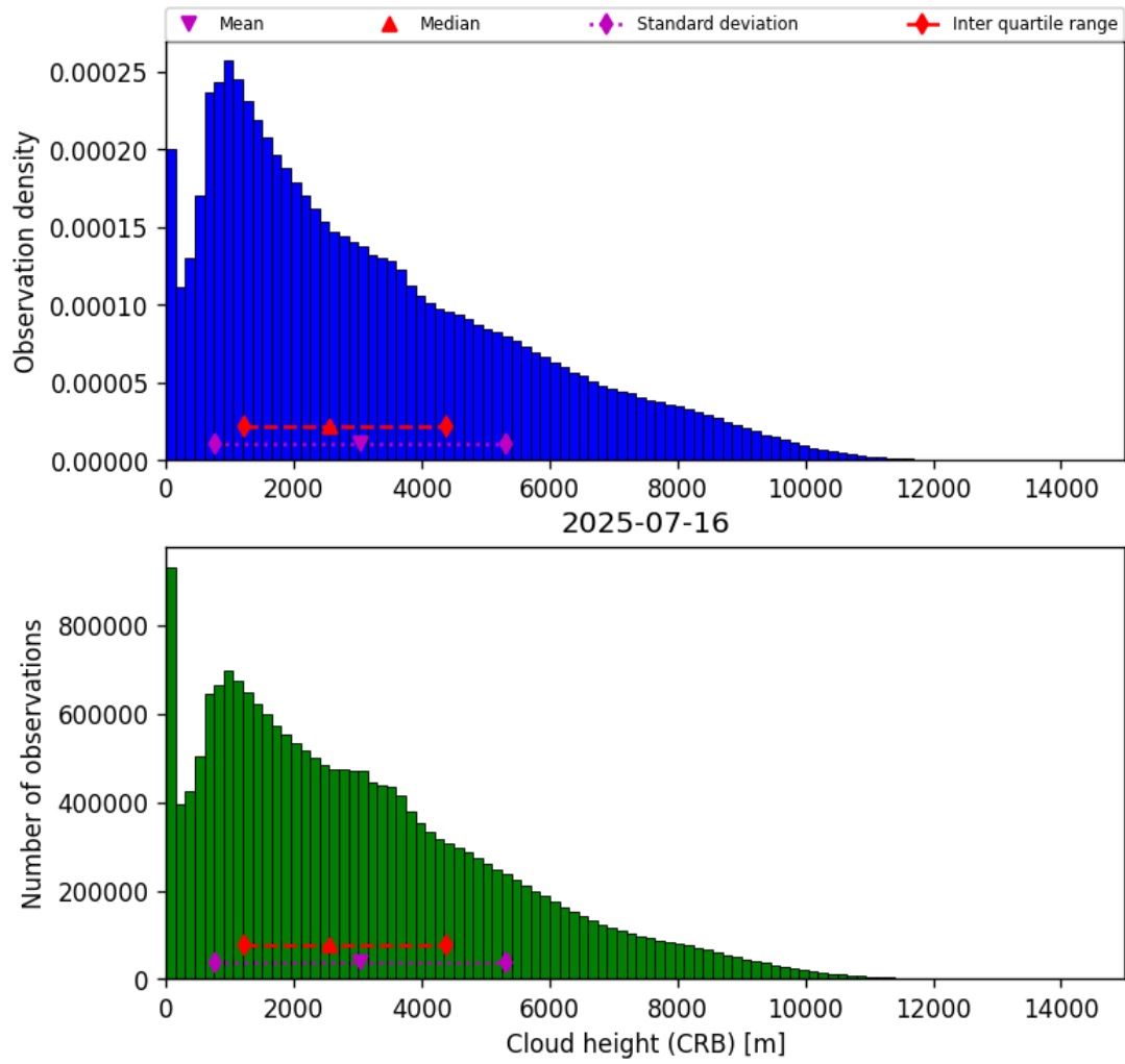
Figure 43: Histogram of “Cloud height (CRB)” for 2025-07-15 to 2025-07-17
