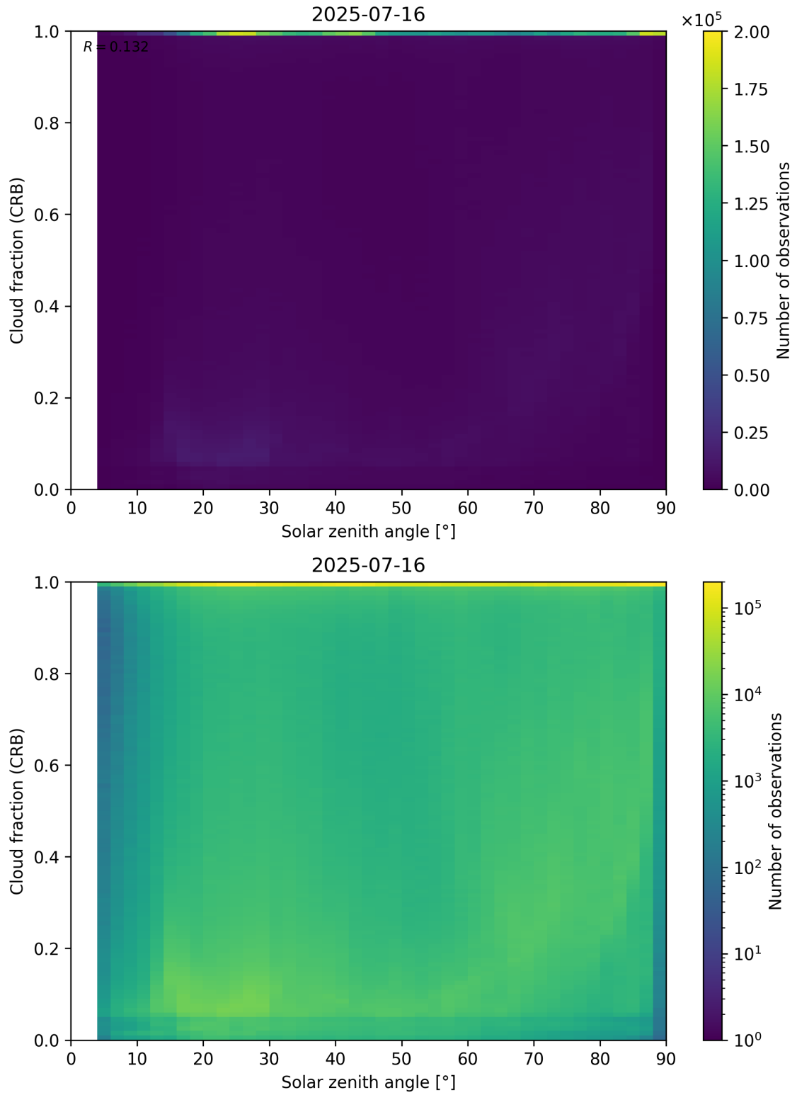
Figure 101: Scatter density plot of “Solar zenith angle” against “Cloud fraction (CRB)” for 2025-07-15 to 2025-07-17.
