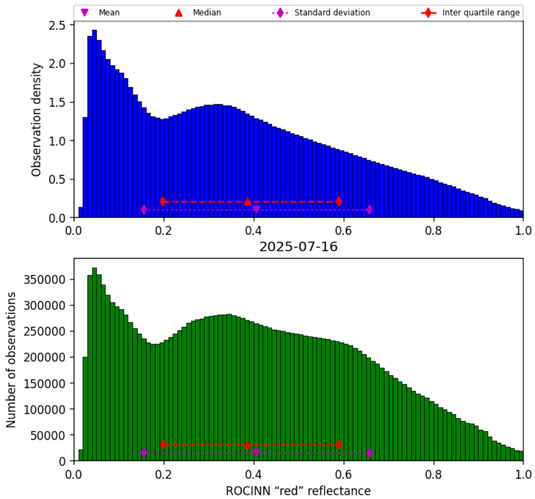
Figure 53: Histogram of “ROCINN “red” reflectance” for 2025-07-15 to 2025-07-17
