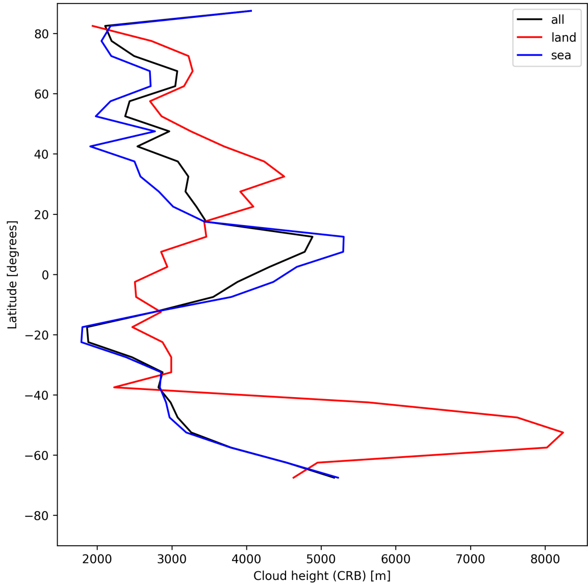
Figure 27: Zonal average of “Cloud height (CRB)” for 2025-07-15 to 2025-07-17.
