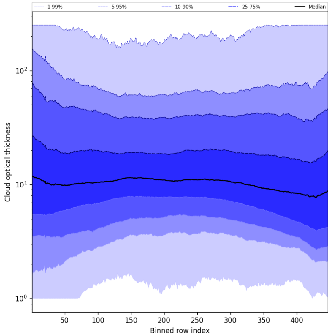
Figure 57: Along track statistics of “Cloud optical thickness” for 2025-07-15 to 2025-07-17
