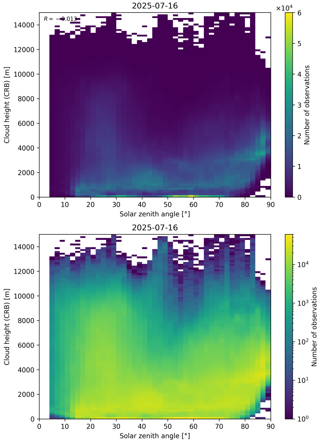
Figure 102: Scatter density plot of “Solar zenith angle” against “Cloud height (CRB)” for 2025-07-15 to 2025-07-17.
