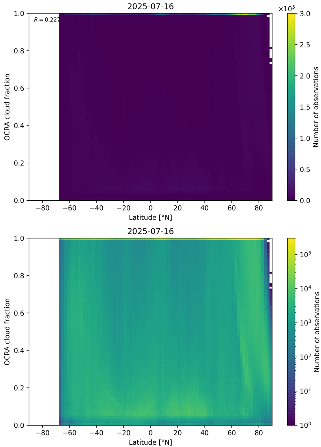
Figure 93: Scatter density plot of “Latitude” against “OCRA cloud fraction” for 2025-07-15 to 2025-07-17.
