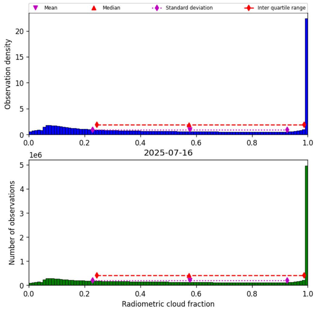
Figure 39: Histogram of “Radiometric cloud fraction” for 2025-07-15 to 2025-07-17
