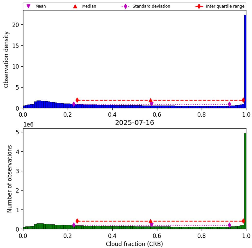
Figure 42: Histogram of “Cloud fraction (CRB)” for 2025-07-15 to 2025-07-17
