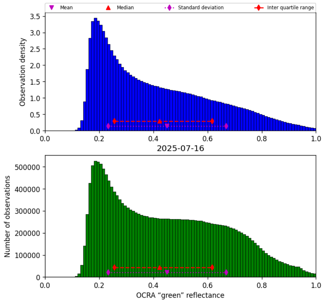
Figure 52: Histogram of “OCRA “green” reflectance” for 2025-07-15 to 2025-07-17
