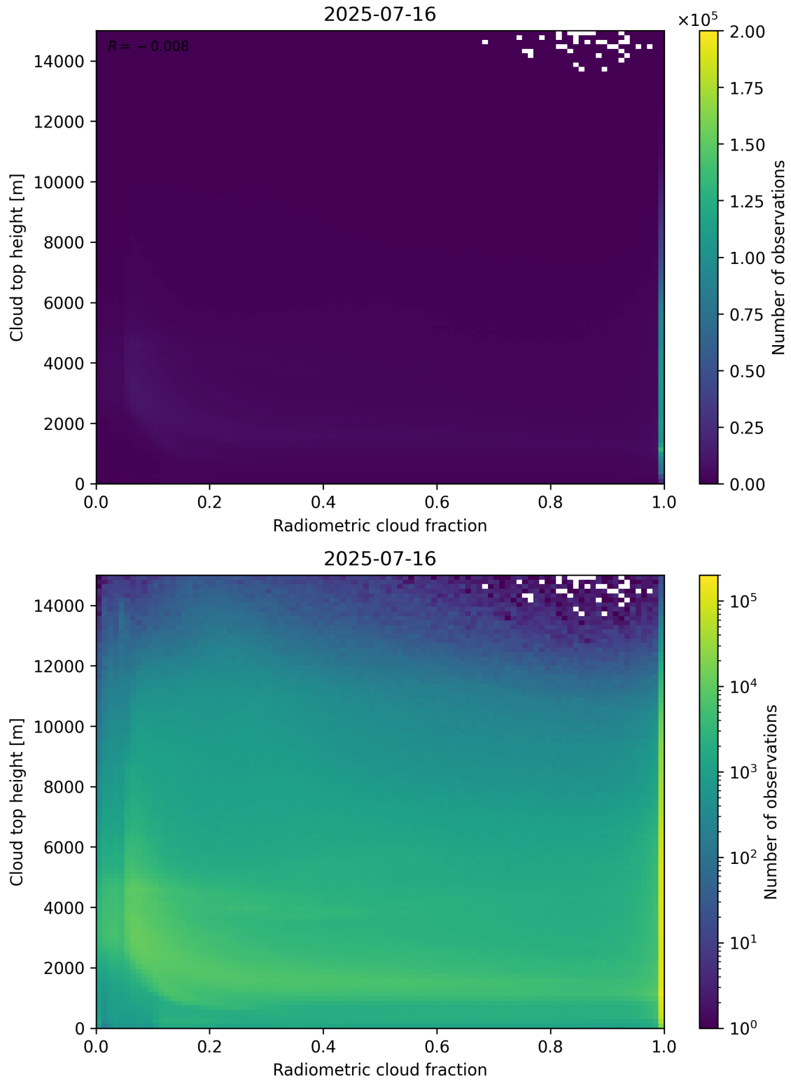
Figure 76: Scatter density plot of “Radiometric cloud fraction” against “Cloud top height” for 2025-07-15 to 2025-07-17.
