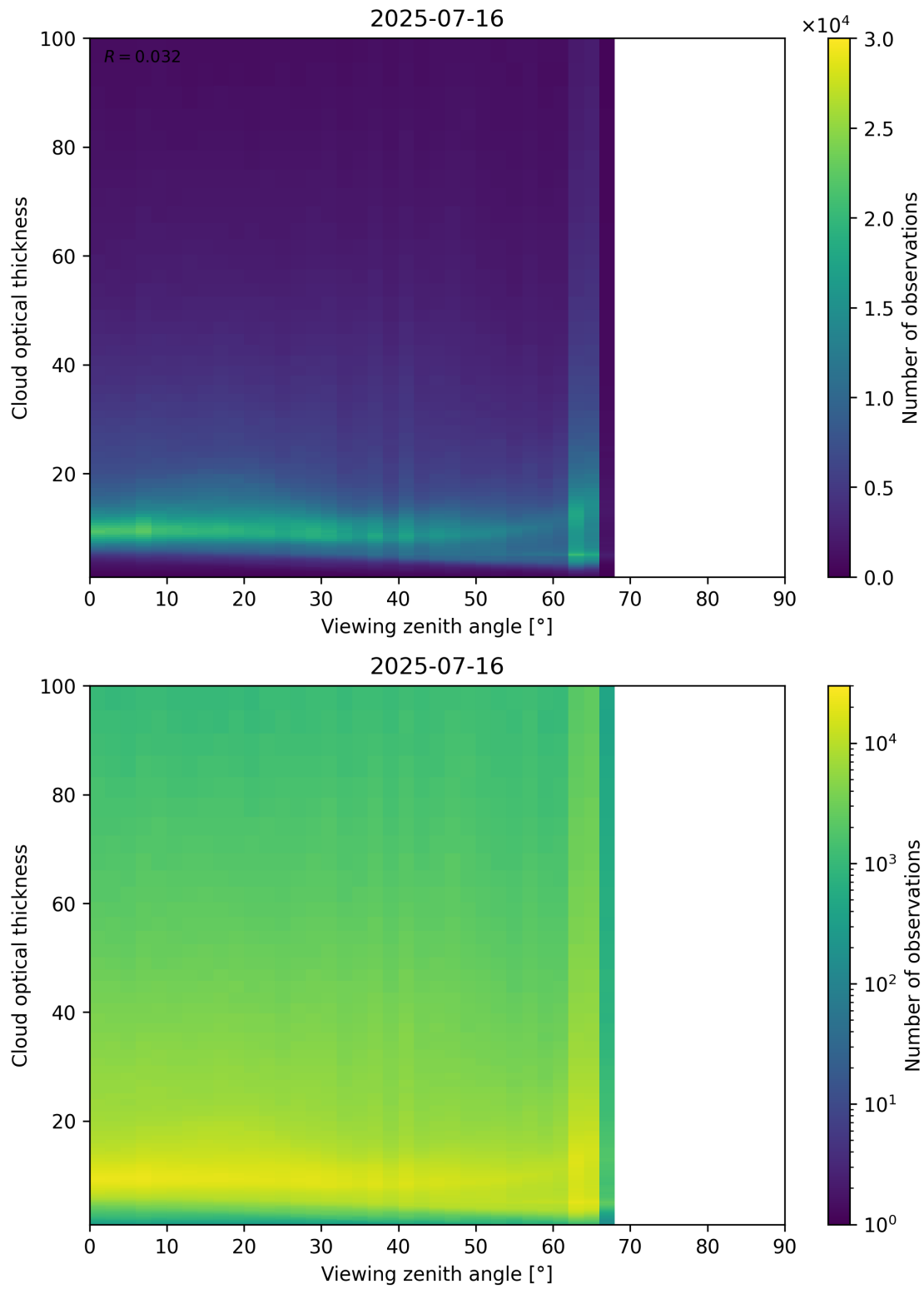
Figure 111: Scatter density plot of “Viewing zenith angle” against “Cloud optical thickness” for 2025-07-15 to 2025-07-17.
