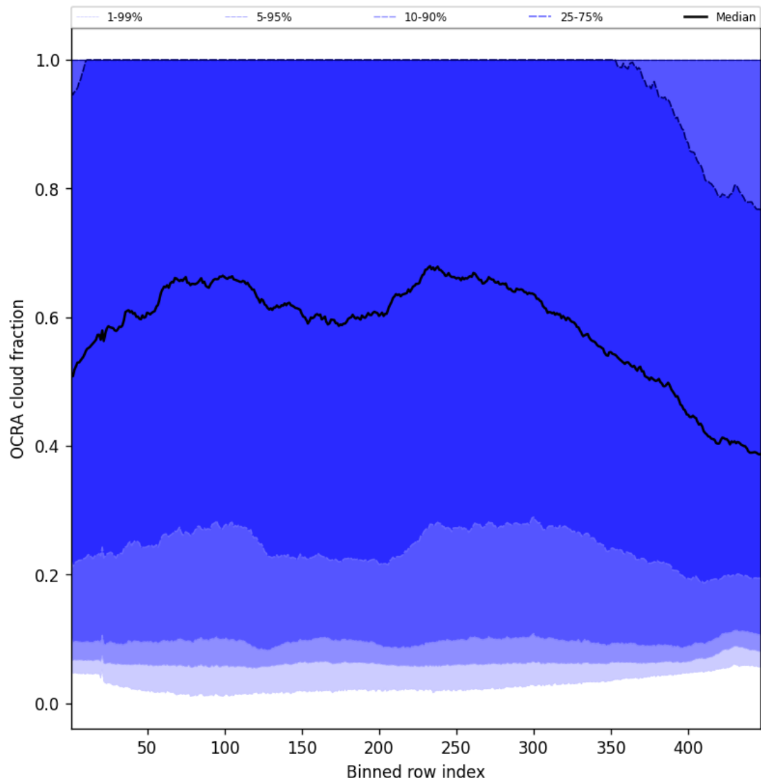
Figure 66: Along track statistics of “OCRA cloud fraction” for 2025-07-15 to 2025-07-17
