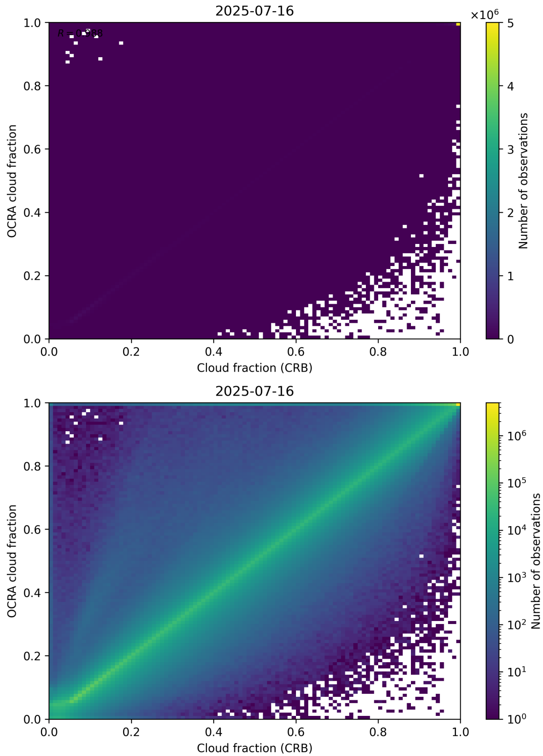
Figure 78: Scatter density plot of “Cloud fraction (CRB)” against “OCRA cloud fraction” for 2025-07-15 to 2025-07-17.
