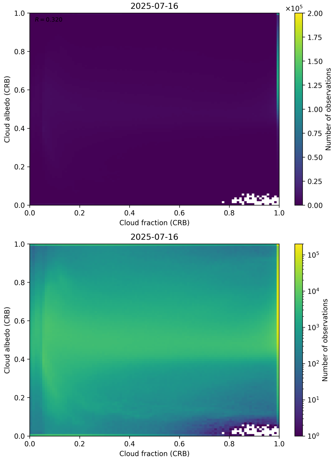
Figure 77: Scatter density plot of “Cloud fraction (CRB)” against “Cloud albedo (CRB)” for 2025-07-15 to 2025-07-17.
