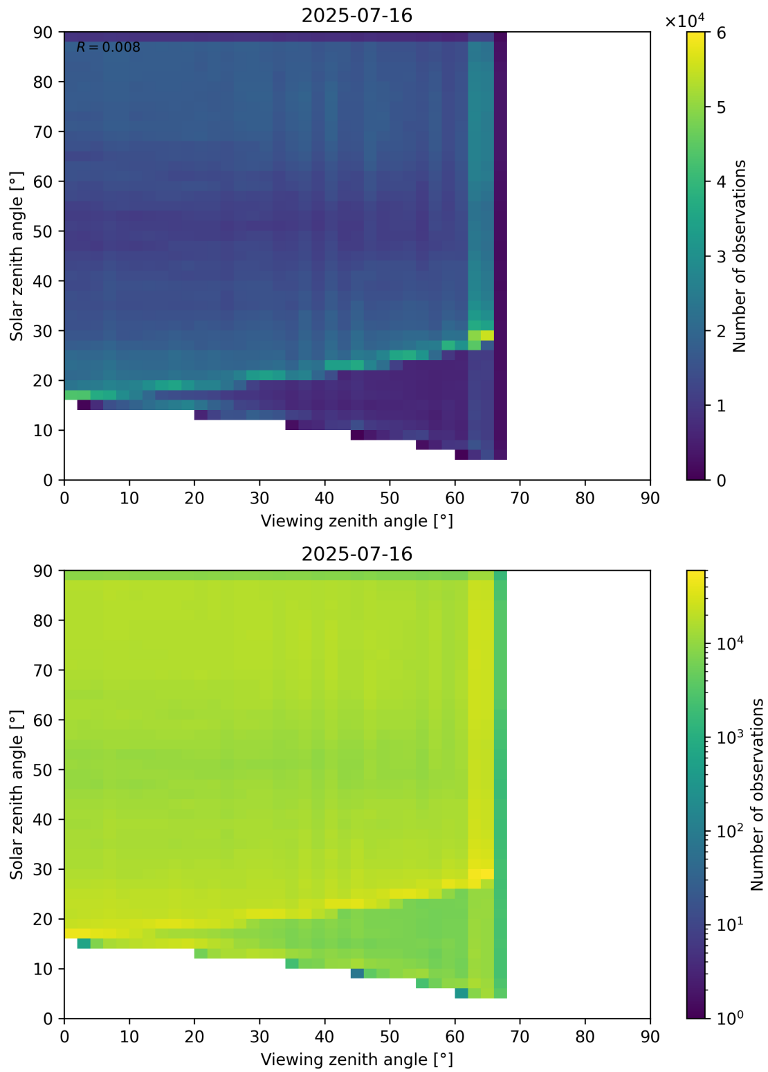
Figure 114: Scatter density plot of “Viewing zenith angle” against “Solar zenith angle” for 2025-07-15 to 2025-07-17.
