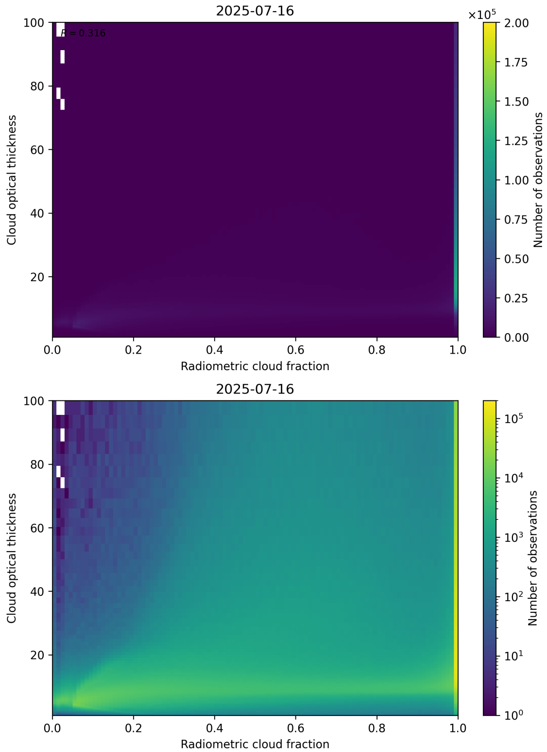
Figure 75: Scatter density plot of “Radiometric cloud fraction” against “Cloud optical thickness” for 2025-07-15 to 2025-07-17.
