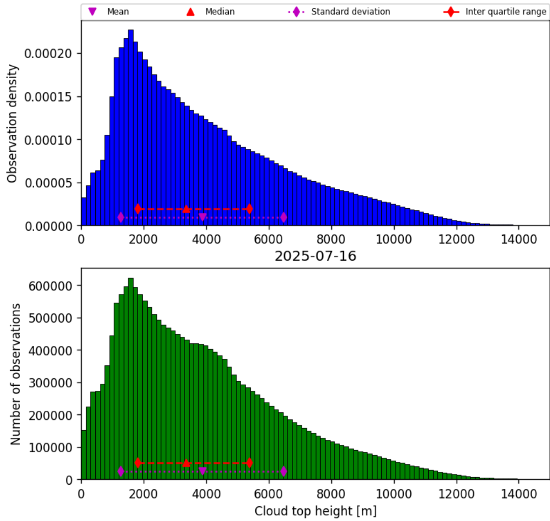
Figure 40: Histogram of “Cloud top height” for 2025-07-15 to 2025-07-17
