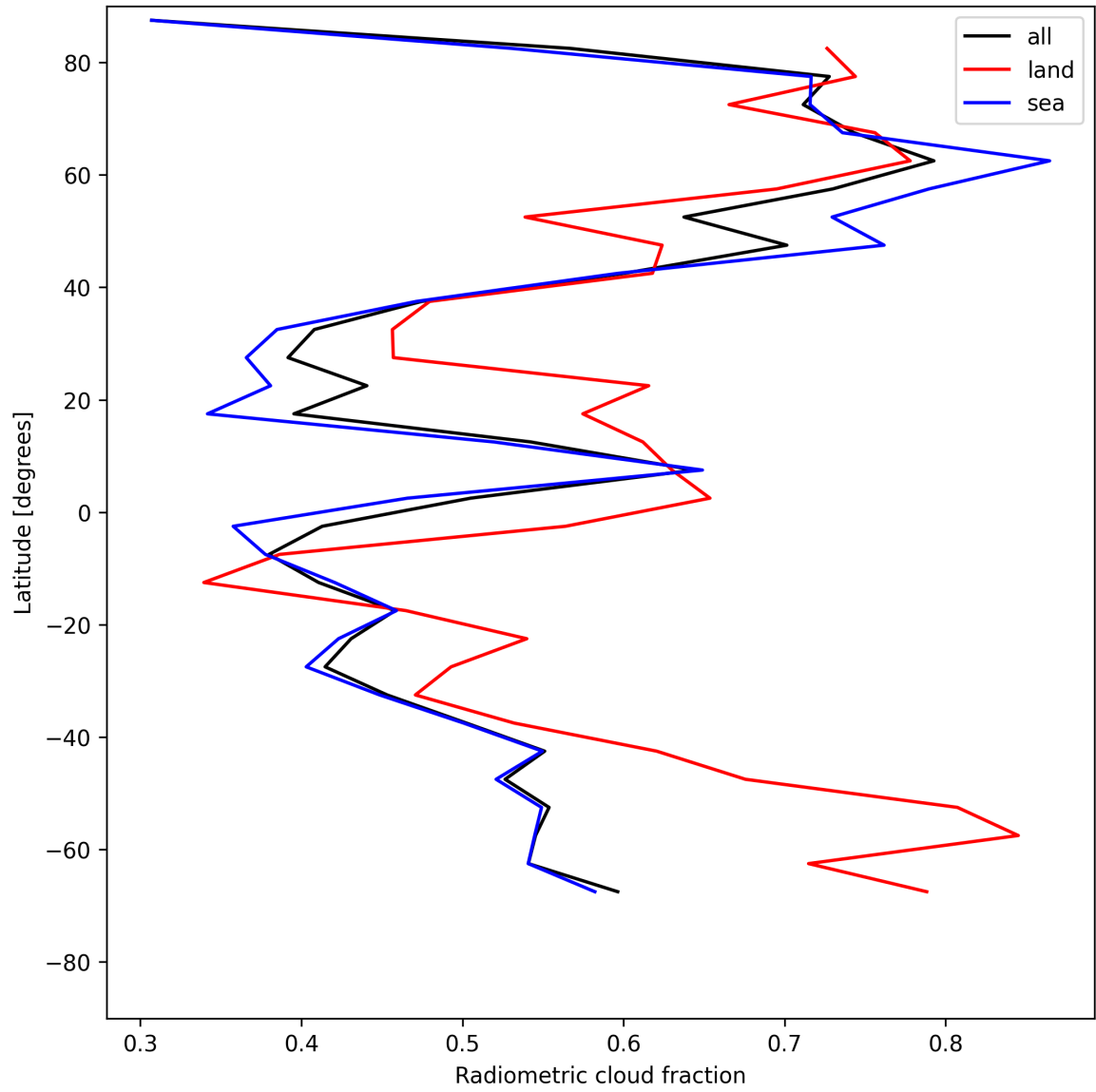
Figure 23: Zonal average of “Radiometric cloud fraction” for 2025-07-15 to 2025-07-17.
