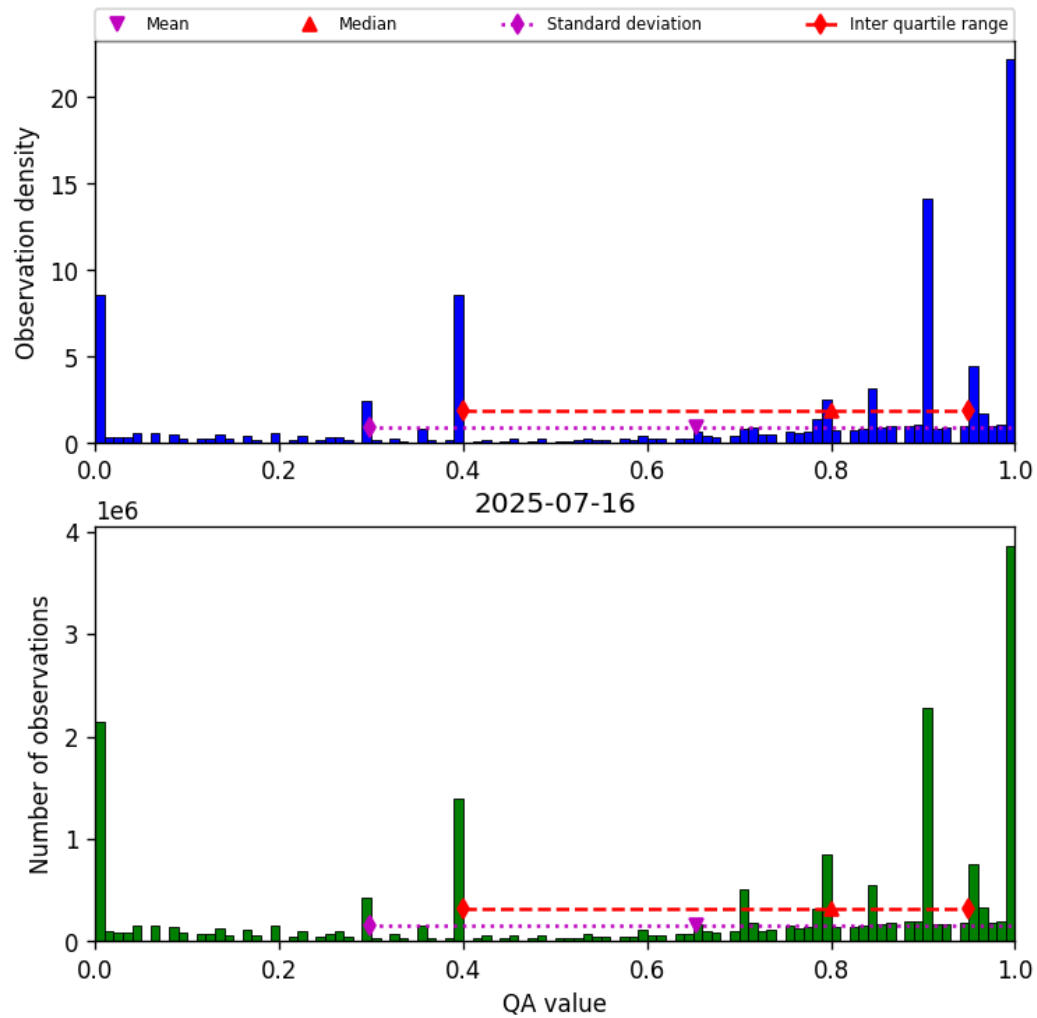
Figure 38: Histogram of “QA value” for 2025-07-15 to 2025-07-17
