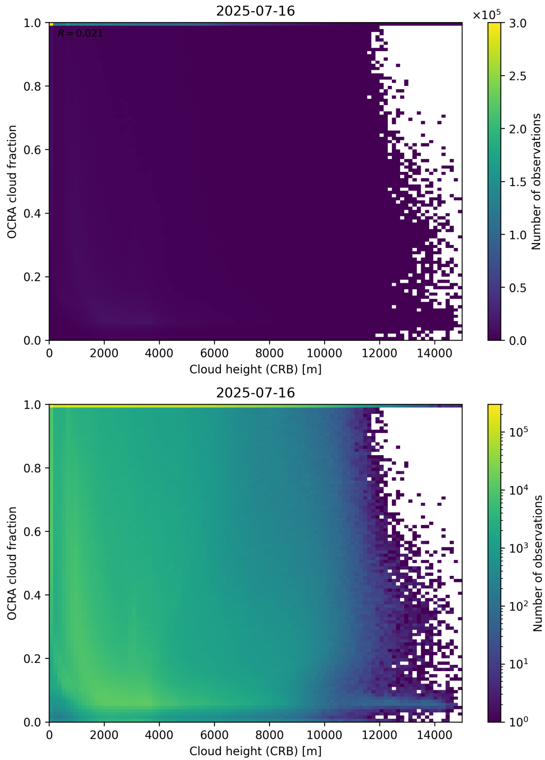
Figure 81: Scatter density plot of “Cloud height (CRB)” against “OCRA cloud fraction” for 2025-07-15 to 2025-07-17.
