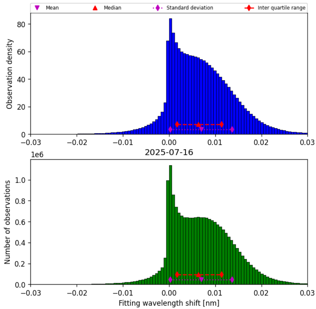
Figure 49: Histogram of “Fitting wavelength shift” for 2025-07-15 to 2025-07-17
