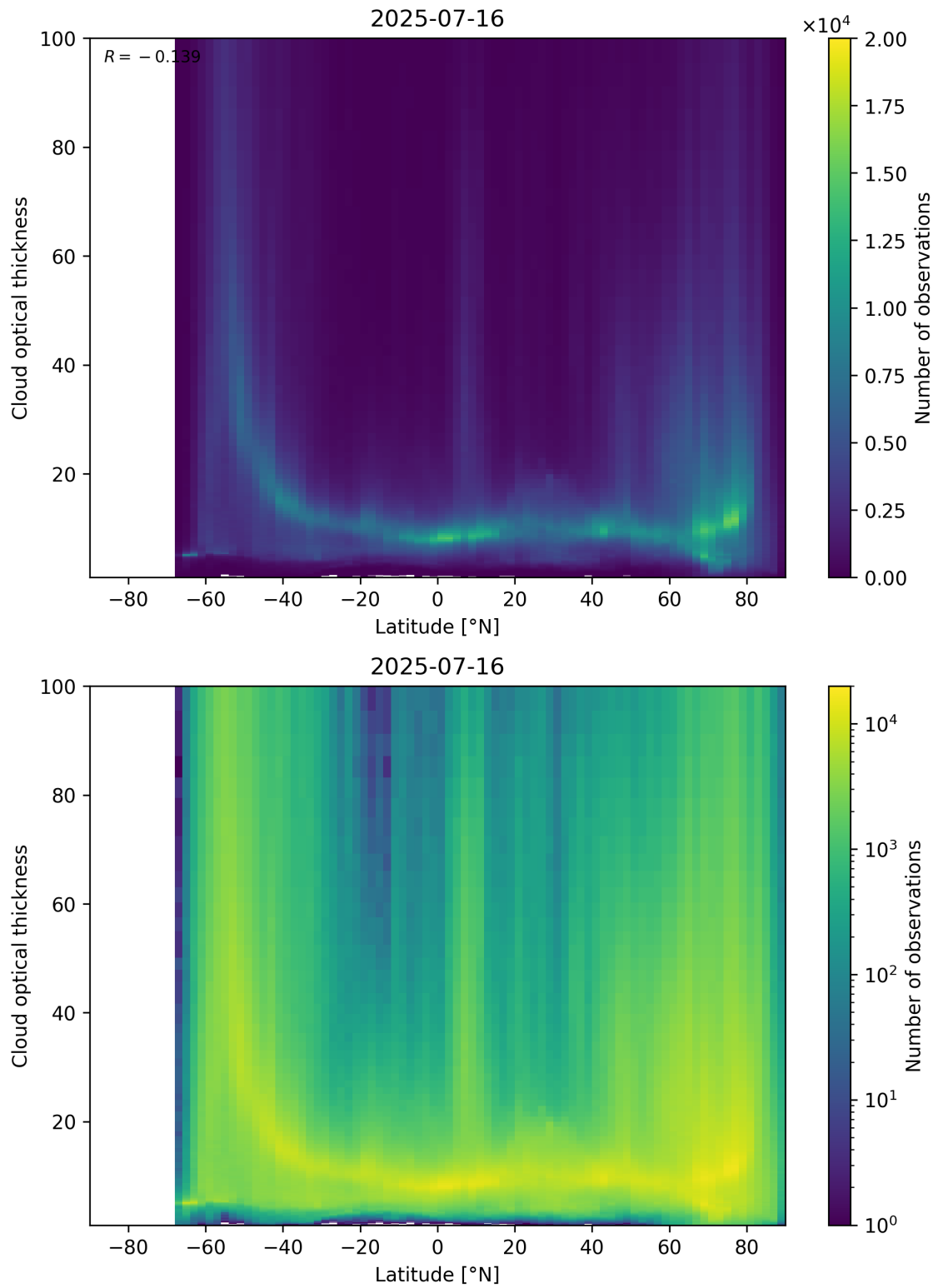
Figure 96: Scatter density plot of “Latitude” against “Cloud optical thickness” for 2025-07-15 to 2025-07-17.
