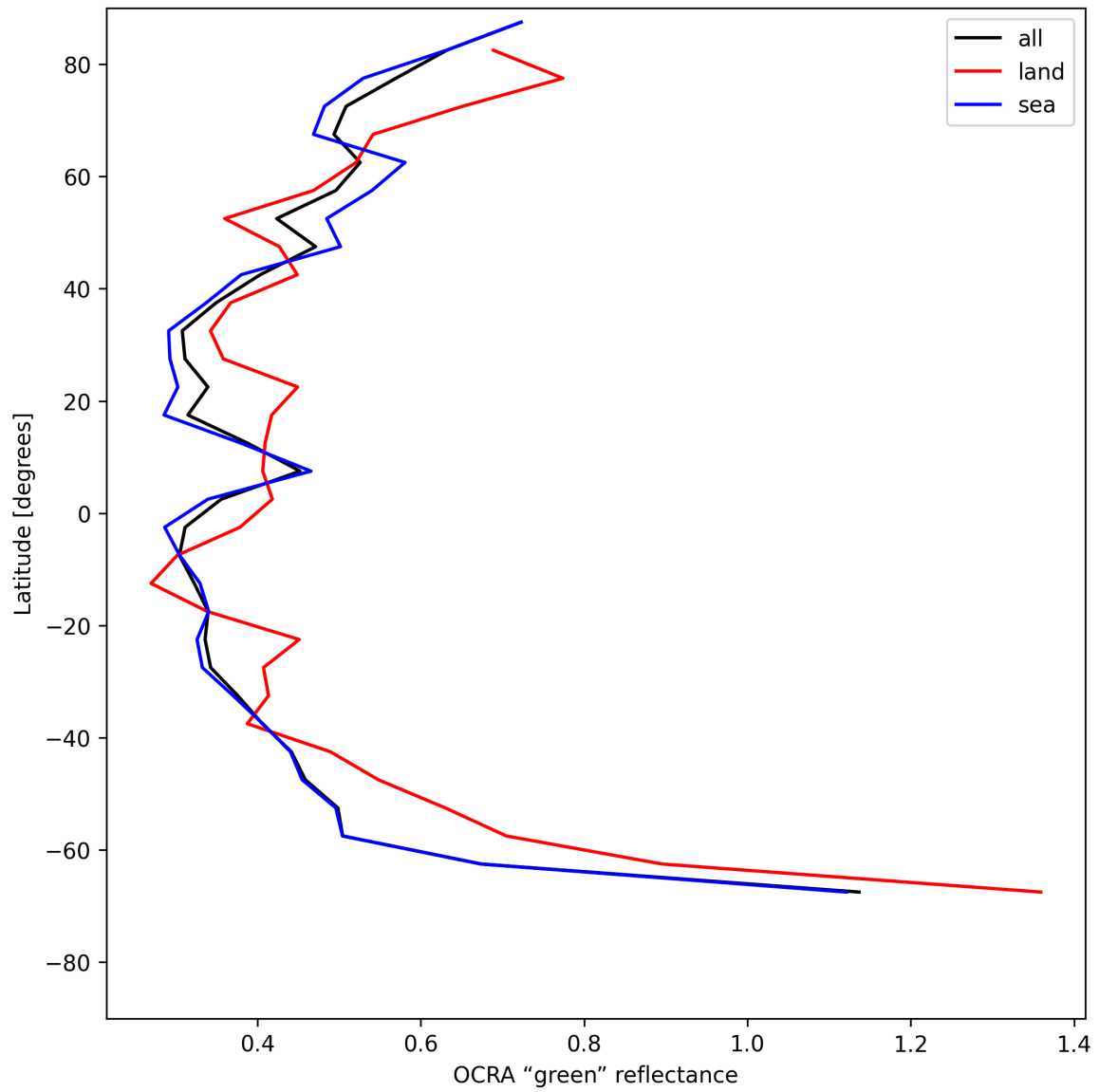
Figure 36: Zonal average of “OCRA “green” reflectance” for 2025-07-15 to 2025-07-17.
