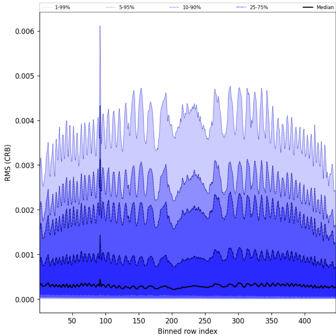
Figure 64: Along track statistics of “RMS (CRB)” for 2025-07-15 to 2025-07-17
