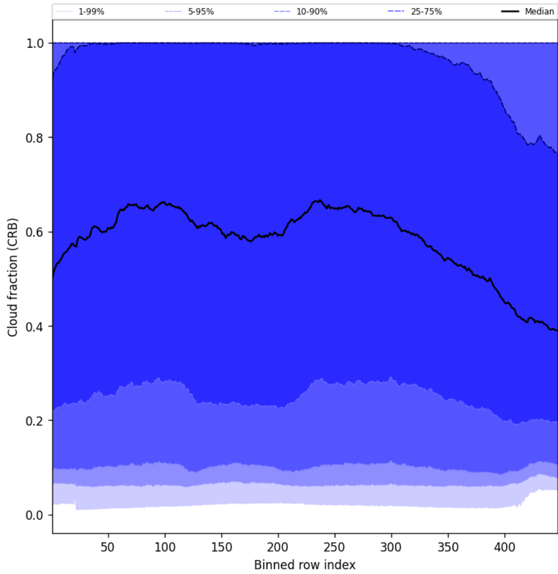
Figure 58: Along track statistics of “Cloud fraction (CRB)” for 2025-07-15 to 2025-07-17
