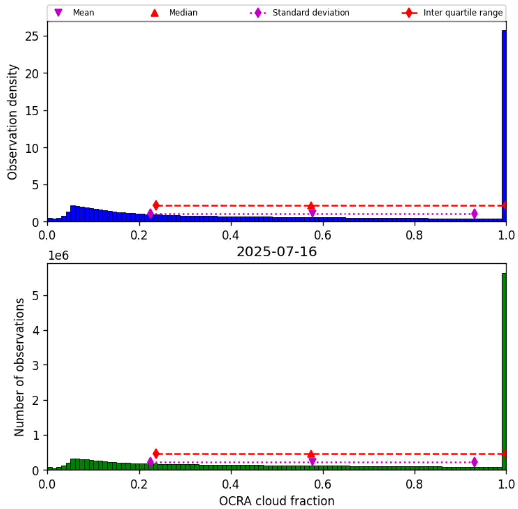
Figure 50: Histogram of “OCRA cloud fraction” for 2025-07-15 to 2025-07-17
