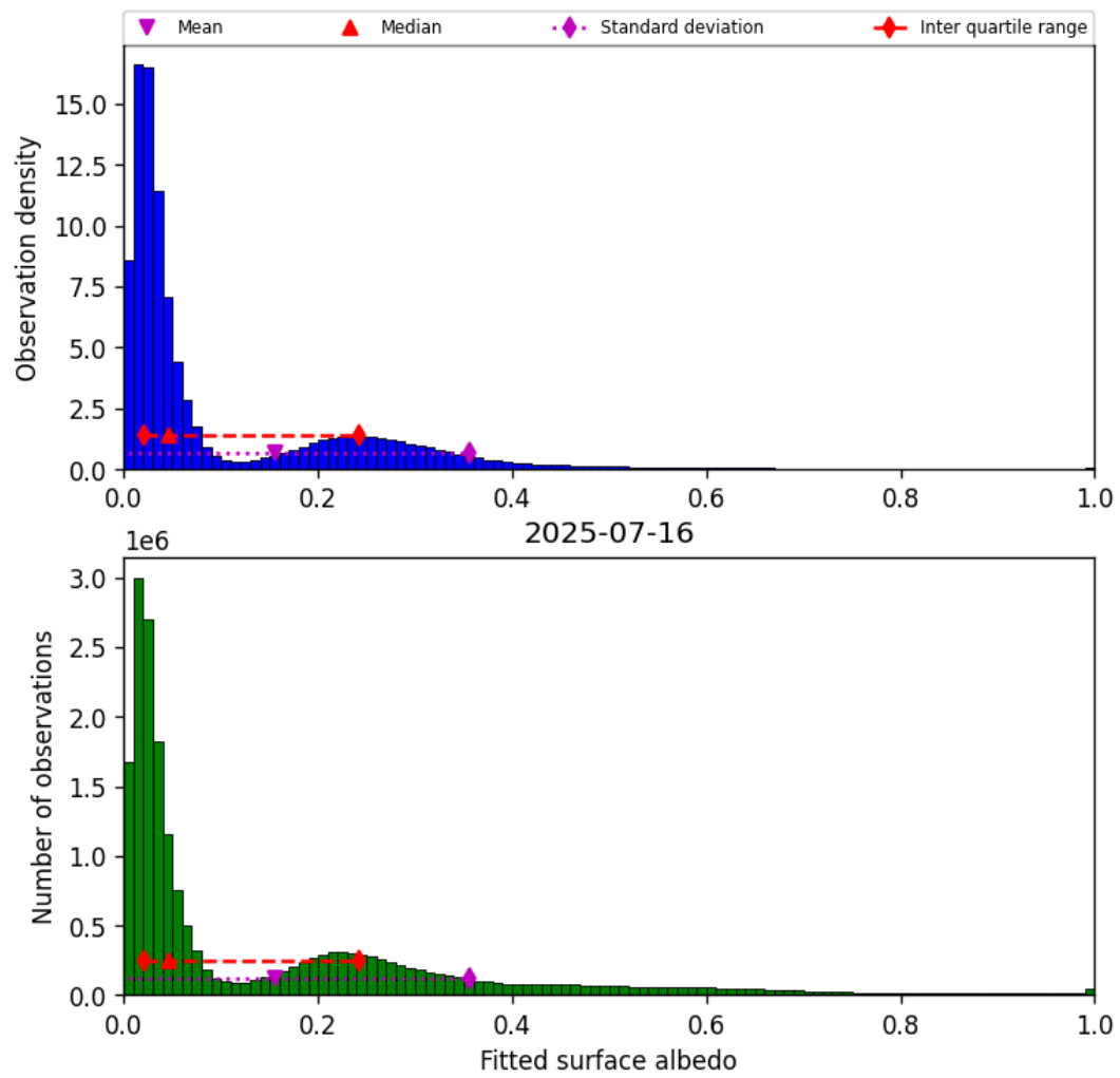
Figure 45: Histogram of “Fitted surface albedo” for 2025-07-15 to 2025-07-17
