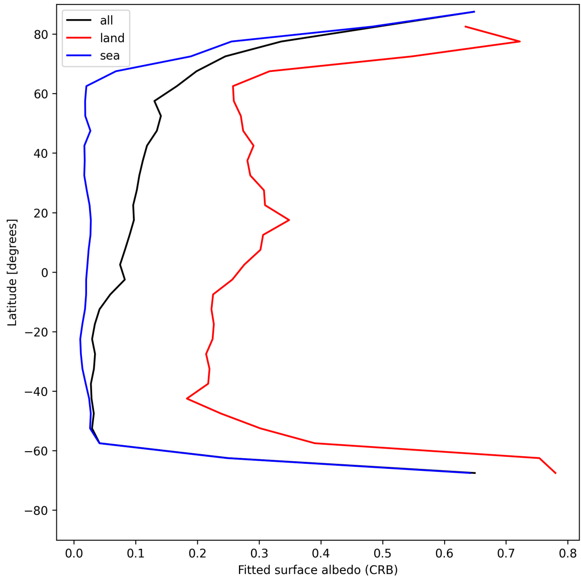
Figure 30: Zonal average of “Fitted surface albedo (CRB)” for 2025-07-15 to 2025-07-17.
