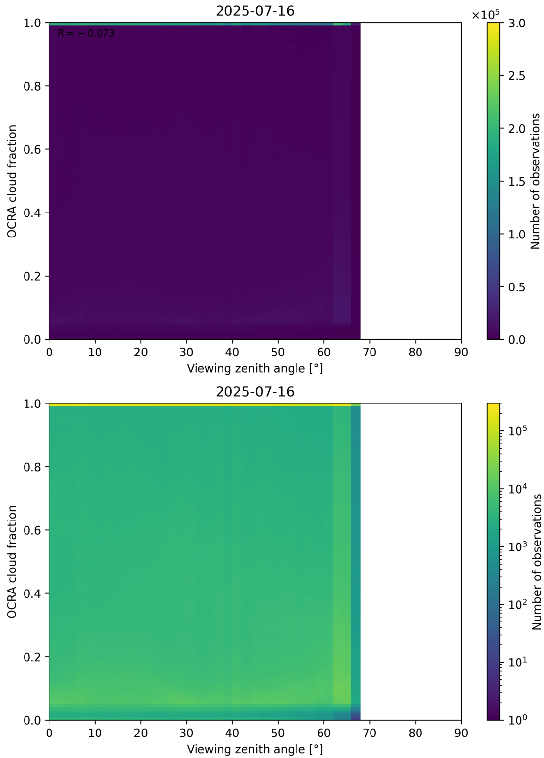
Figure 108: Scatter density plot of “Viewing zenith angle” against “OCRA cloud fraction” for 2025-07-15 to 2025-07-17.
