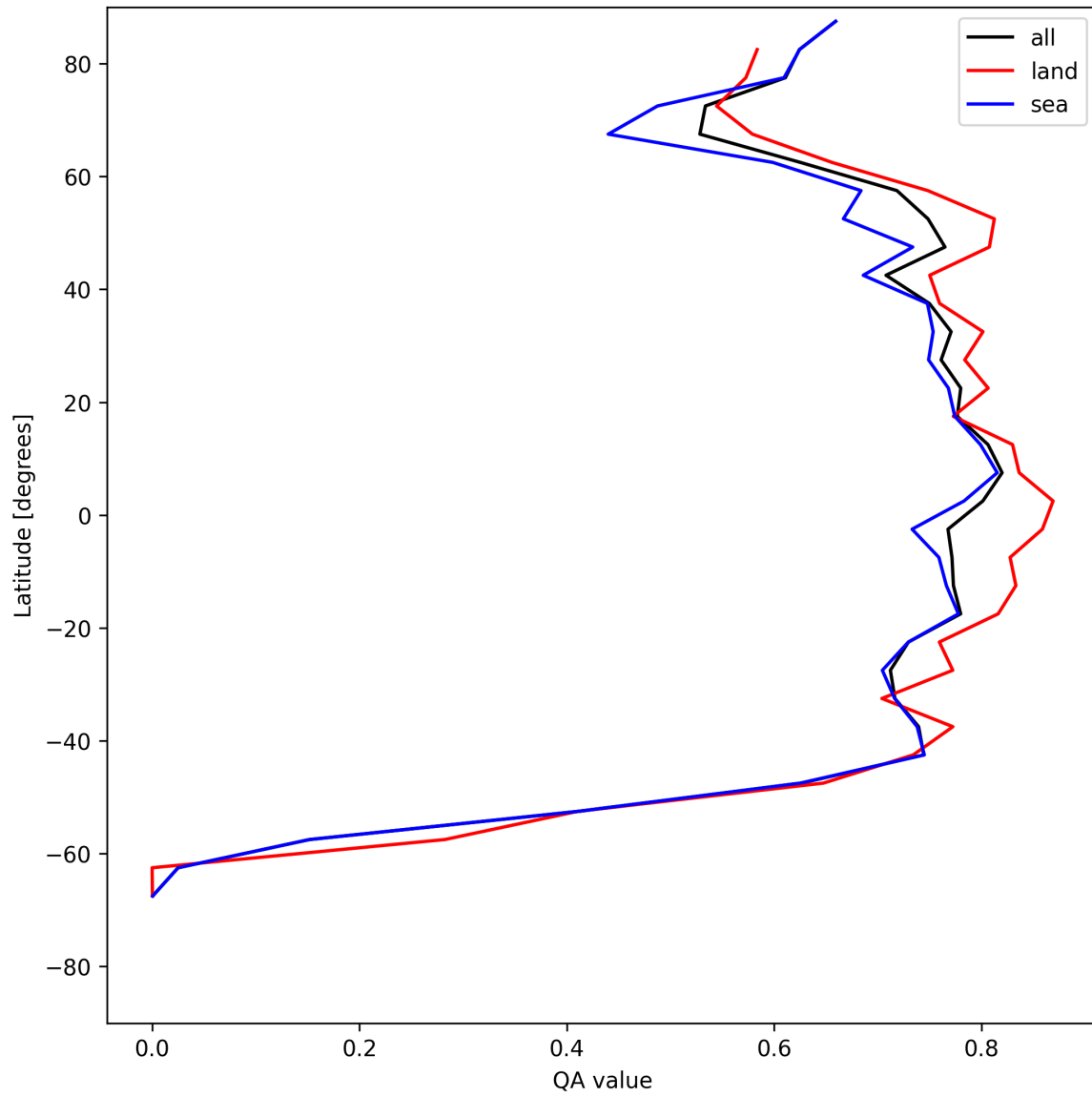
Figure 22: Zonal average of “QA value” for 2025-07-15 to 2025-07-17.
