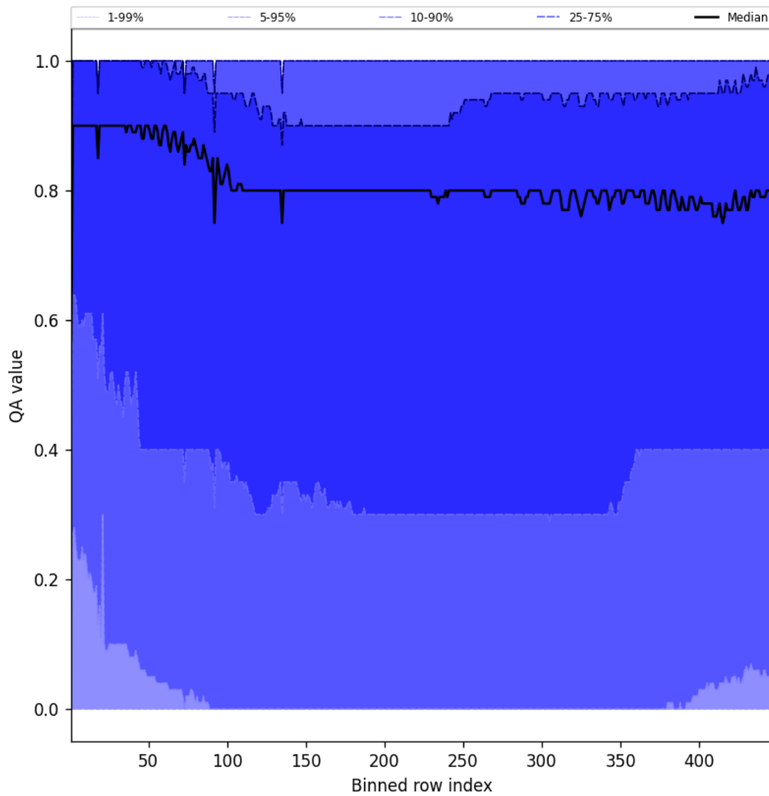
Figure 54: Along track statistics of “QA value” for 2025-07-15 to 2025-07-17
