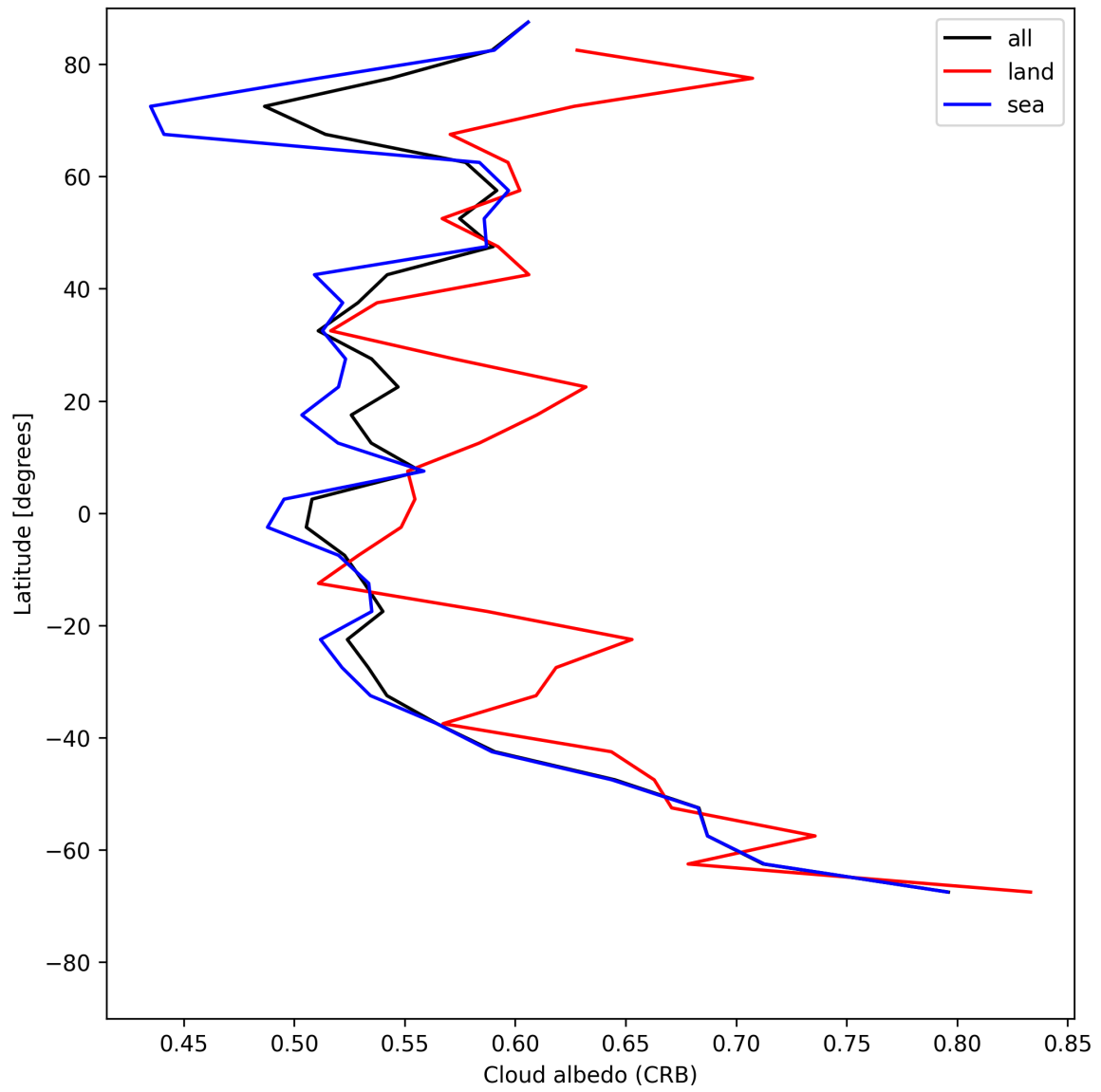
Figure 28: Zonal average of “Cloud albedo (CRB)” for 2025-07-15 to 2025-07-17.
