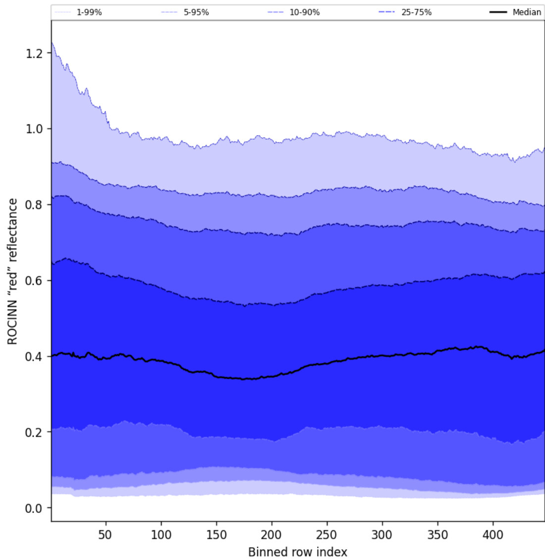
Figure 69: Along track statistics of "ROCINN "red" reflectance" for 2025-07-15 to 2025-07-17
