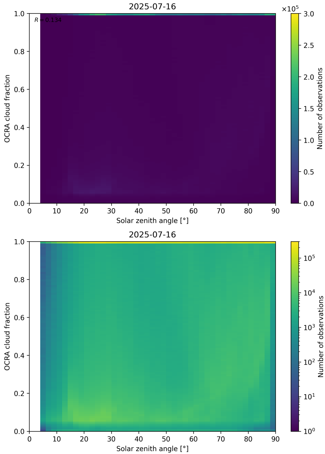
Figure 100: Scatter density plot of “Solar zenith angle” against “OCRA cloud fraction” for 2025-07-15 to 2025-07-17.
