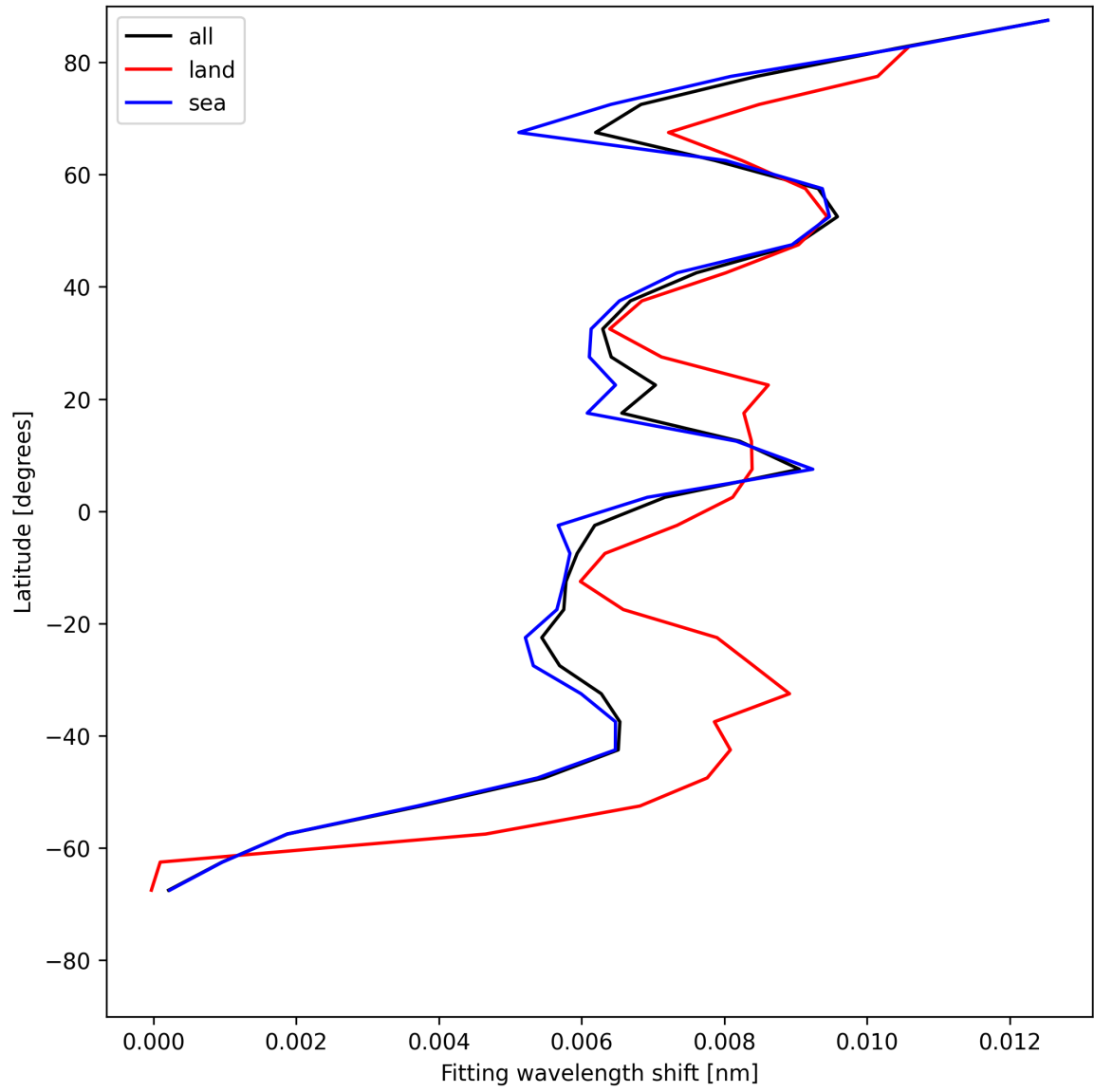
Figure 33: Zonal average of “Fitting wavelength shift” for 2025-07-15 to 2025-07-17.
