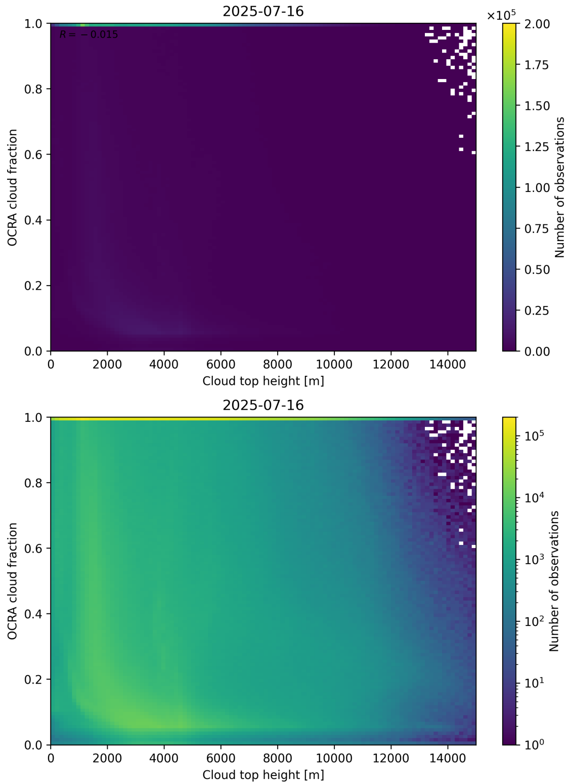
Figure 87: Scatter density plot of “Cloud top height” against “OCRA cloud fraction” for 2025-07-15 to 2025-07-17.
