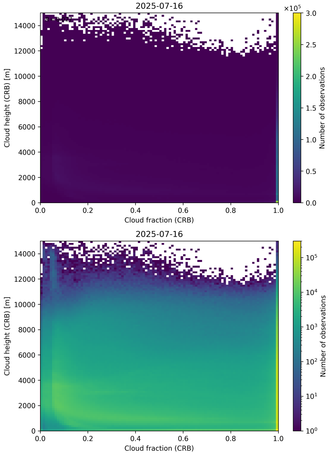
Figure 79: Scatter density plot of “Cloud fraction (CRB)” against “Cloud height (CRB)” for 2025-07-15 to 2025-07-17.
