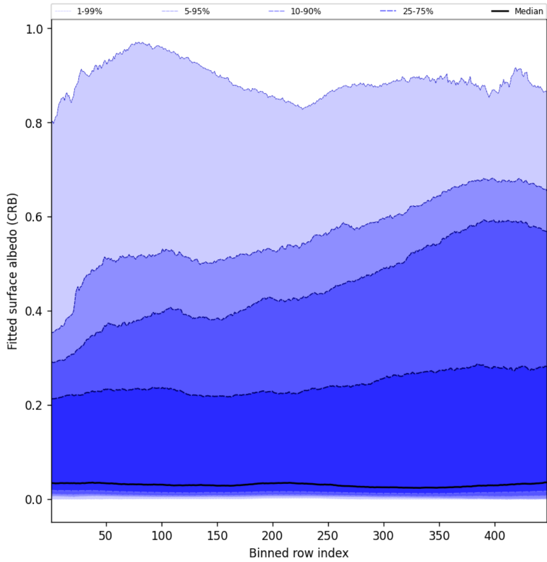
Figure 62: Along track statistics of “Fitted surface albedo (CRB)” for 2025-07-15 to 2025-07-17
