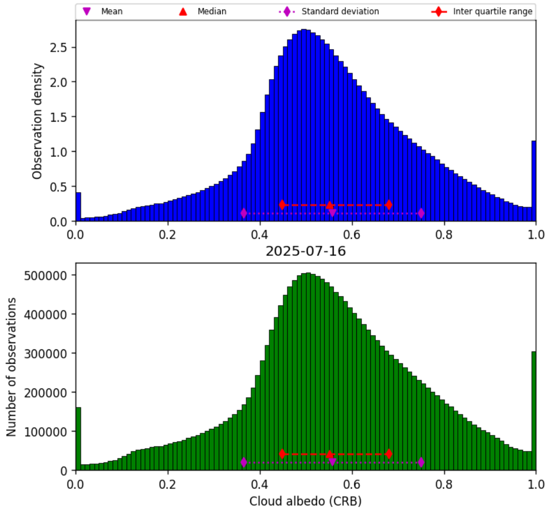
Figure 44: Histogram of “Cloud albedo (CRB)” for 2025-07-15 to 2025-07-17
