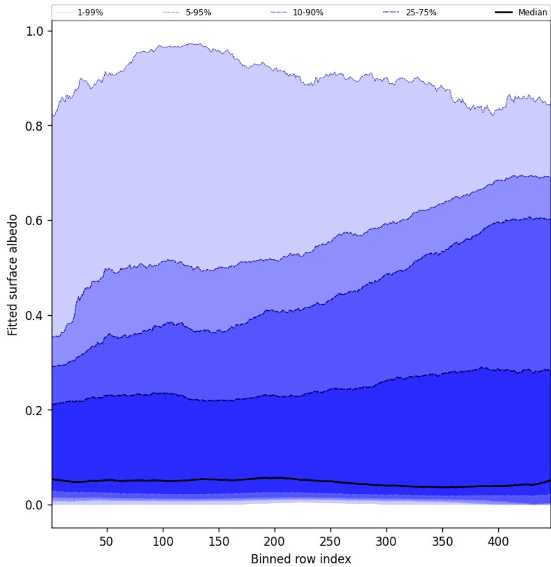
Figure 61: Along track statistics of “Fitted surface albedo” for 2025-07-15 to 2025-07-17
