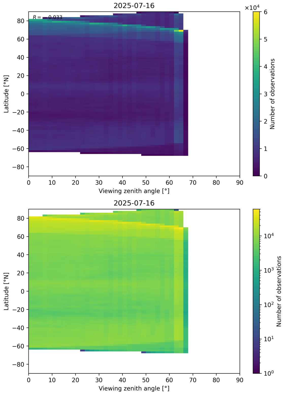
Figure 113: Scatter density plot of “Viewing zenith angle” against “Latitude” for 2025-07-15 to 2025-07-17.
