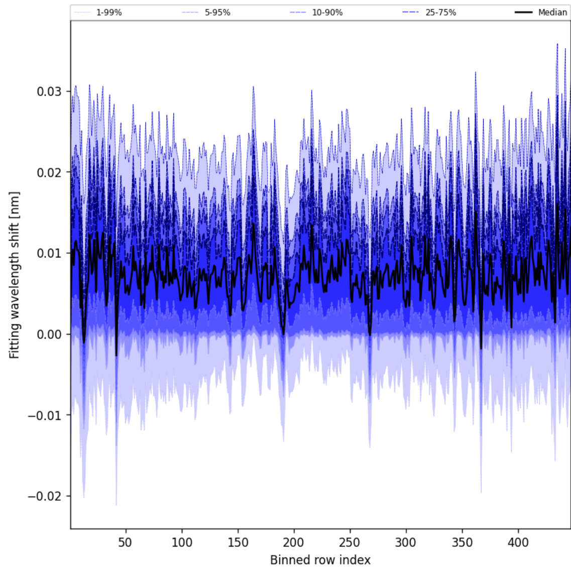
Figure 65: Along track statistics of “Fitting wavelength shift” for 2025-07-15 to 2025-07-17
