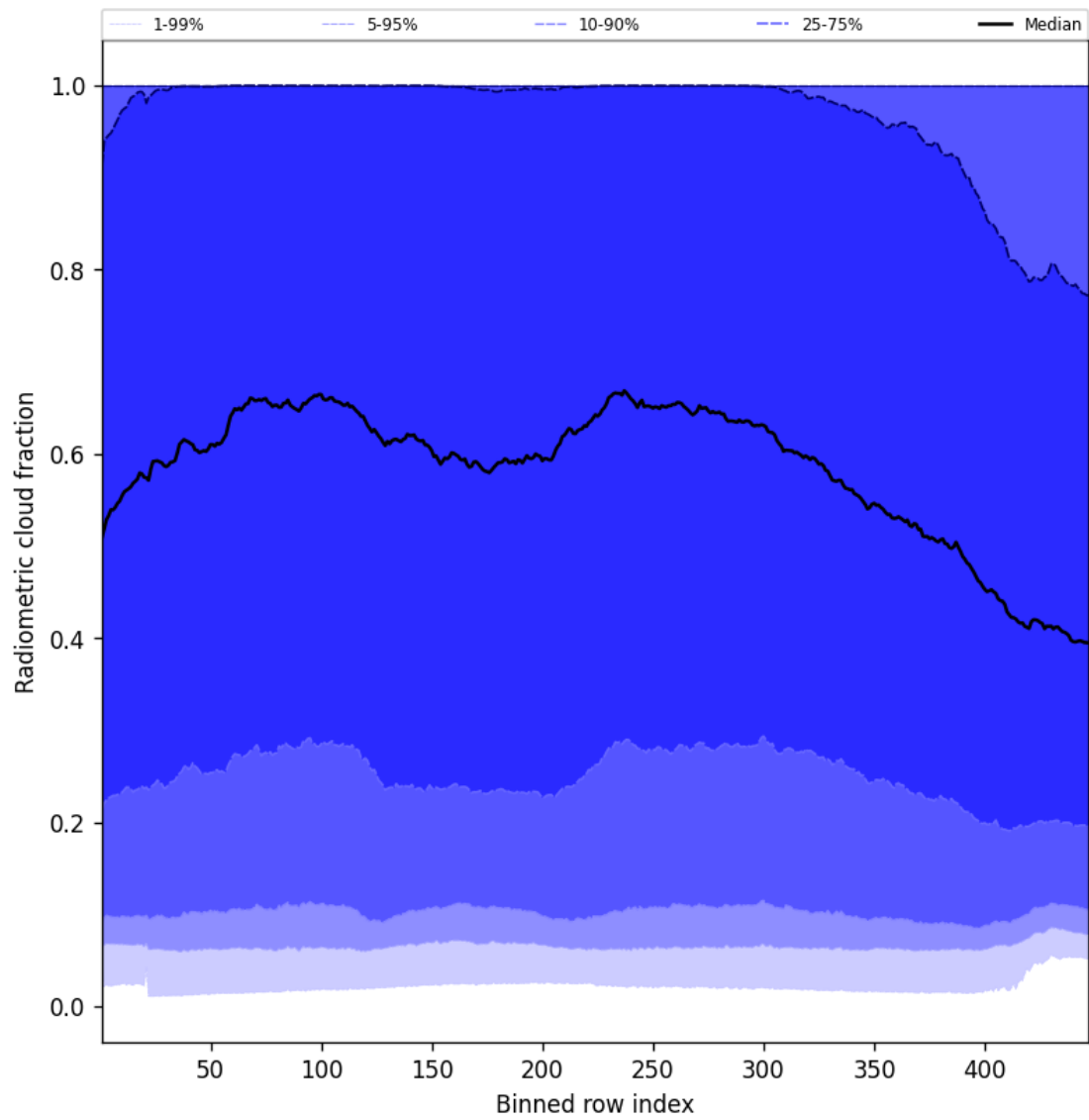
Figure 55: Along track statistics of “Radiometric cloud fraction” for 2025-07-15 to 2025-07-17
