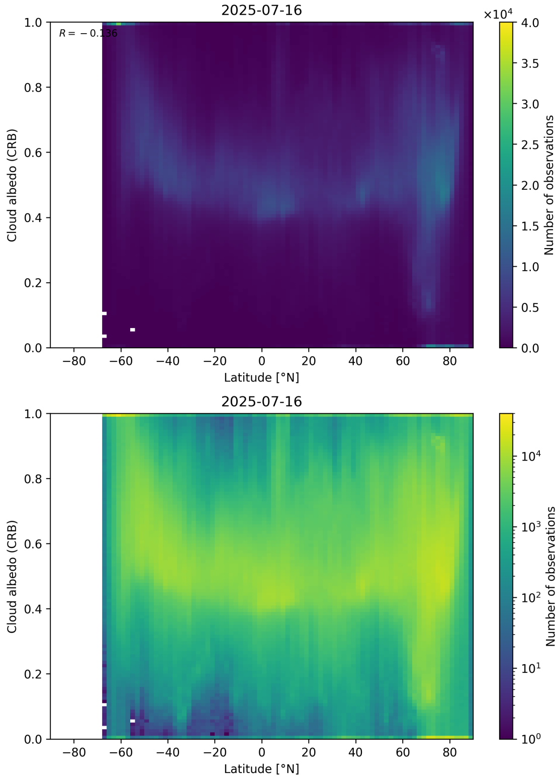
Figure 91: Scatter density plot of “Latitude” against “Cloud albedo (CRB)” for 2025-07-15 to 2025-07-17.
