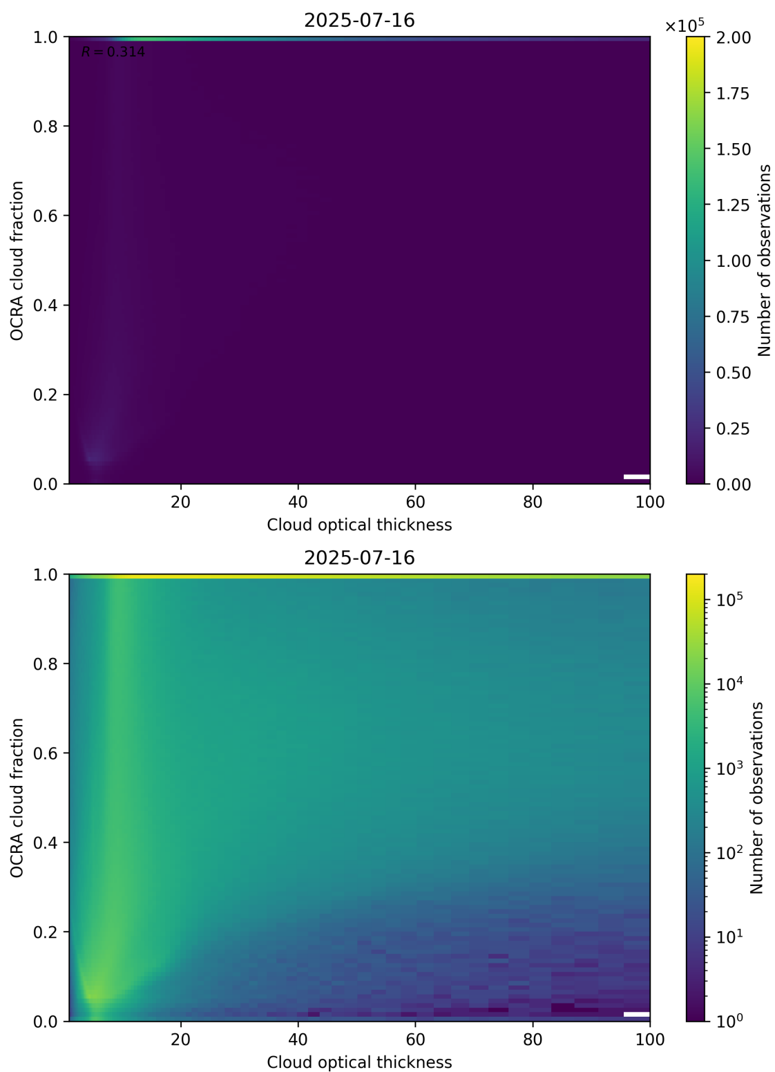
Figure 83: Scatter density plot of “Cloud optical thickness” against “OCRA cloud fraction” for 2025-07-15 to 2025-07-17.
