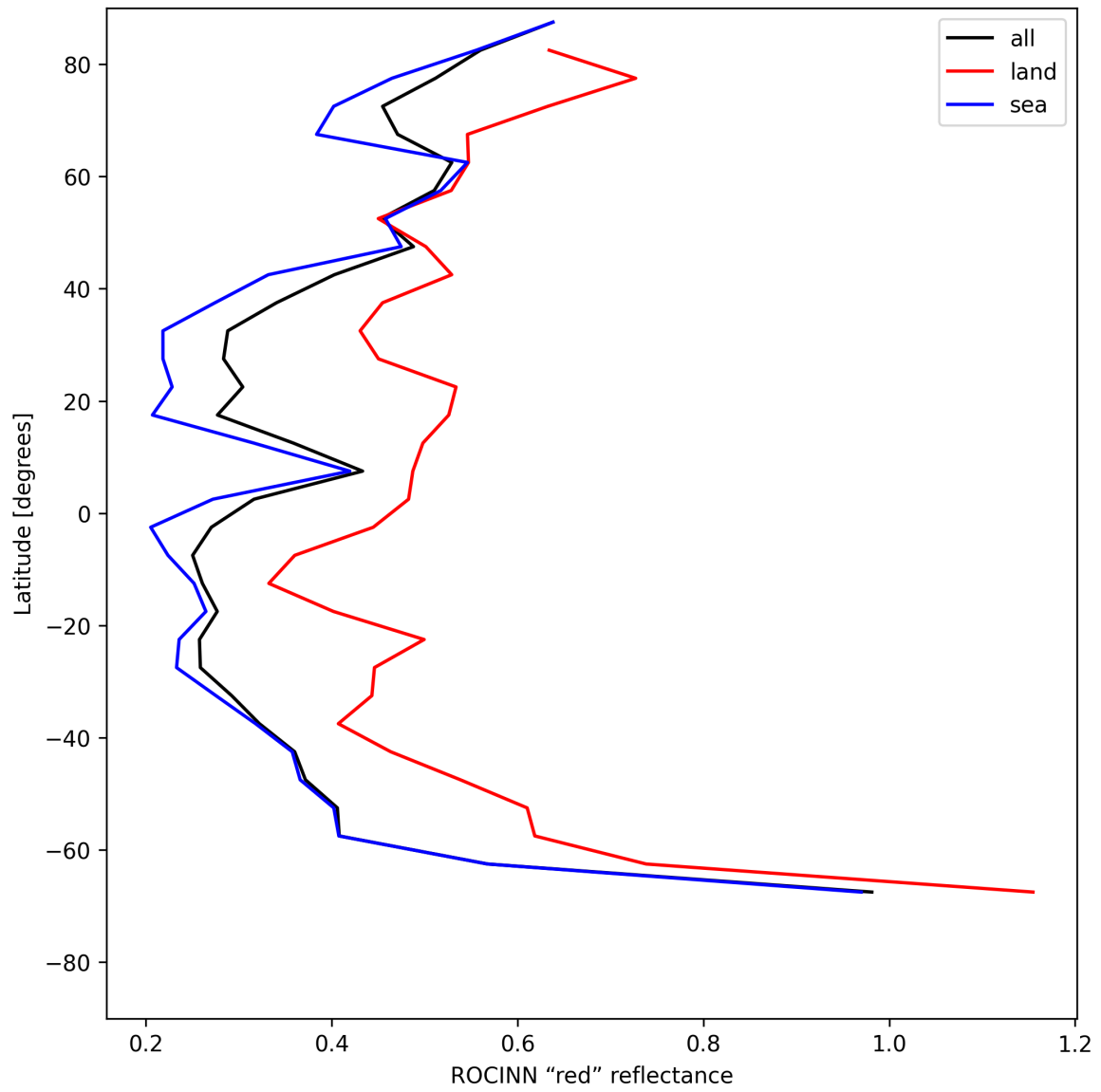
Figure 37: Zonal average of “ROCINN “red” reflectance” for 2025-07-15 to 2025-07-17.
