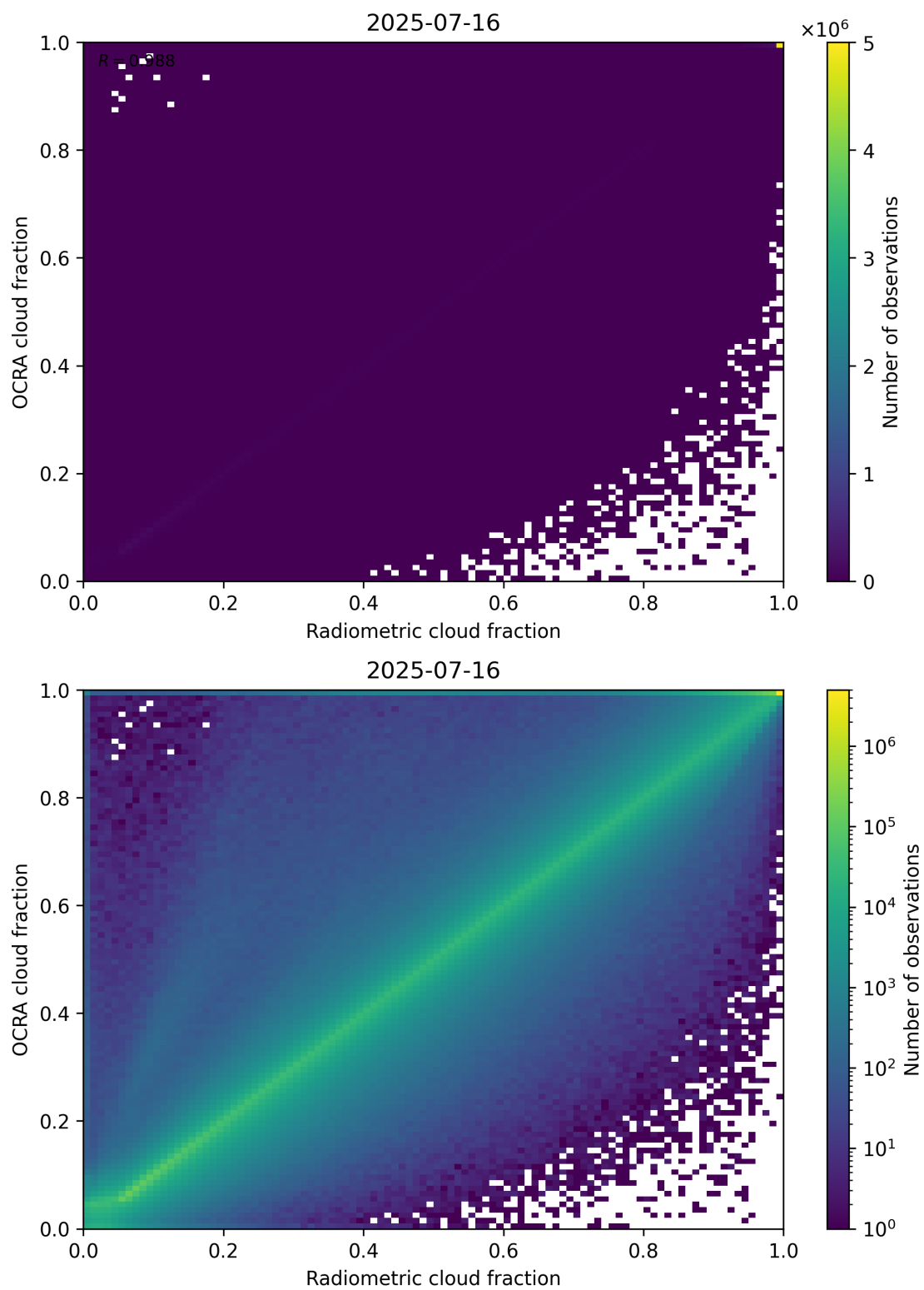
Figure 72: Scatter density plot of “Radiometric cloud fraction” against “OCRA cloud fraction” for 2025-07-15 to 2025-07-17.
