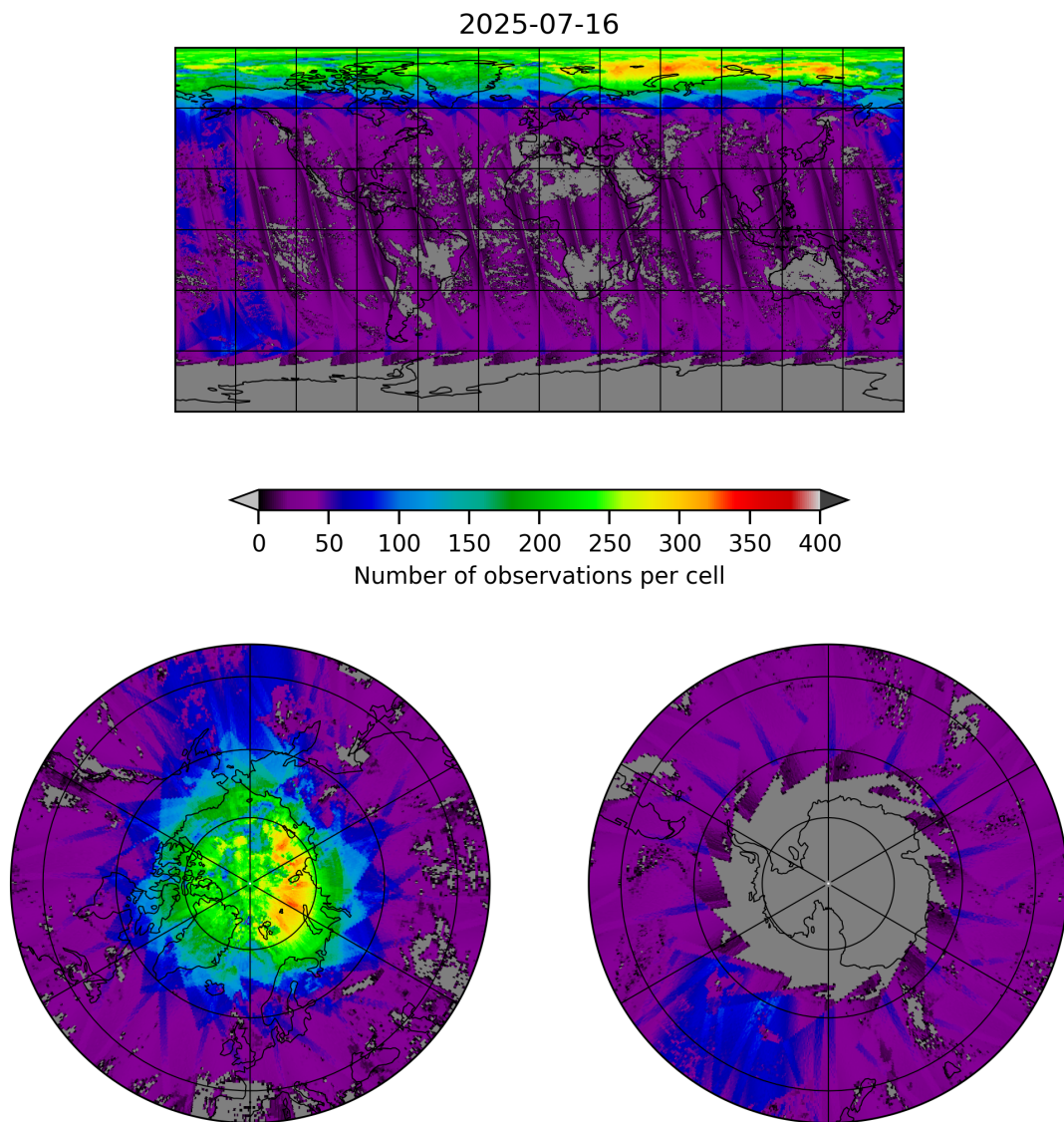
Figure 21: Map of the number of observations for 2025-07-15 to 2025-07-17
