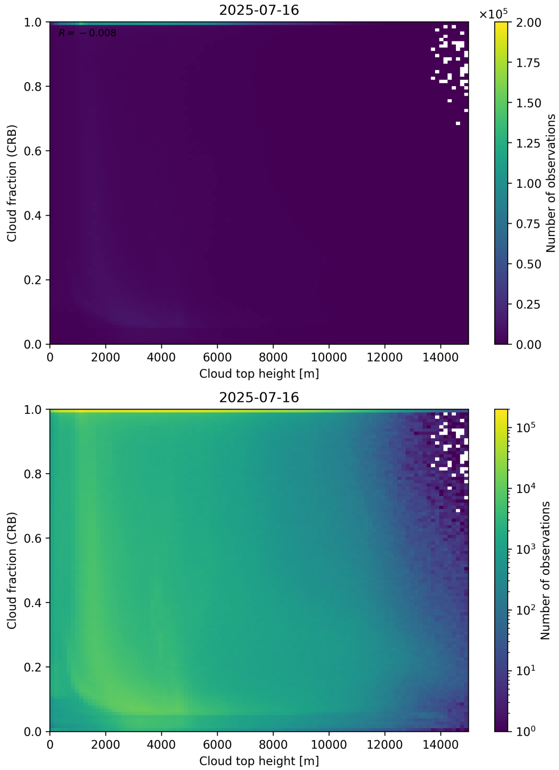
Figure 88: Scatter density plot of “Cloud top height” against “Cloud fraction (CRB)” for 2025-07-15 to 2025-07-17.
