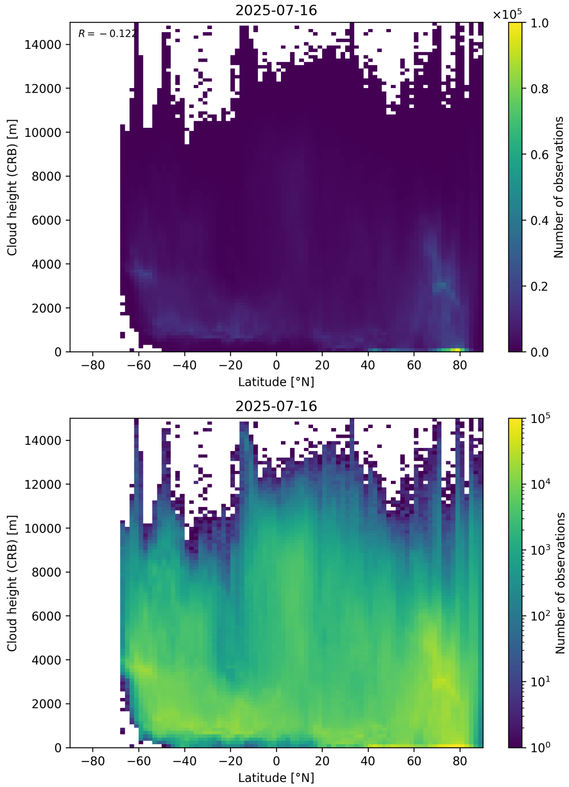
Figure 95: Scatter density plot of “Latitude” against “Cloud height (CRB)” for 2025-07-15 to 2025-07-17.
