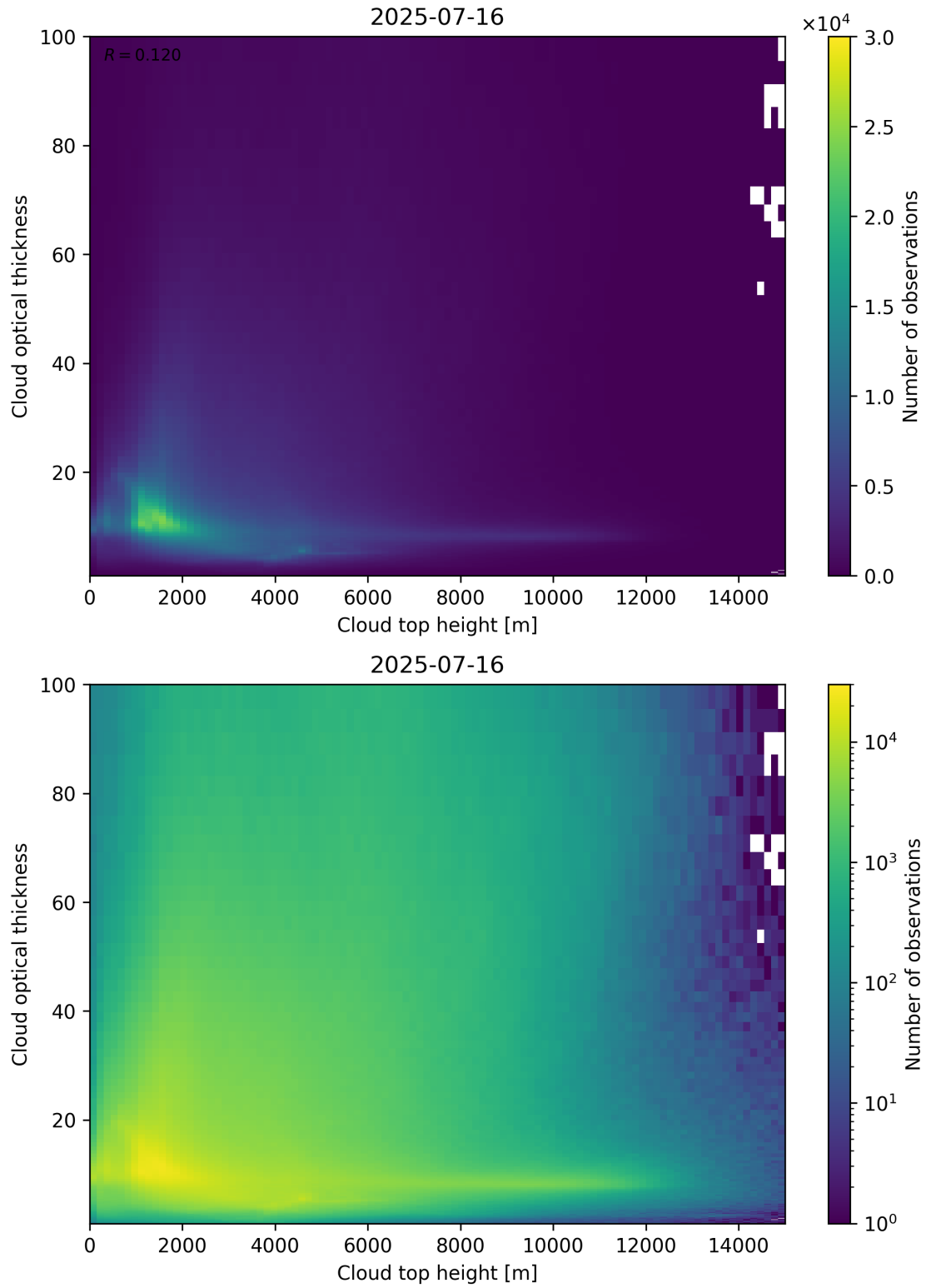
Figure 90: Scatter density plot of “Cloud top height” against “Cloud optical thickness” for 2025-07-15 to 2025-07-17.
