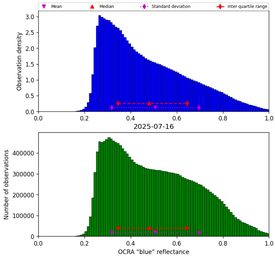
Figure 51: Histogram of “OCRA “blue” reflectance” for 2025-07-15 to 2025-07-17
