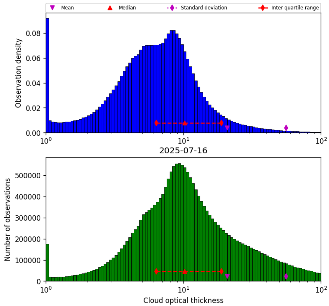
Figure 41: Histogram of “Cloud optical thickness” for 2025-07-15 to 2025-07-17
