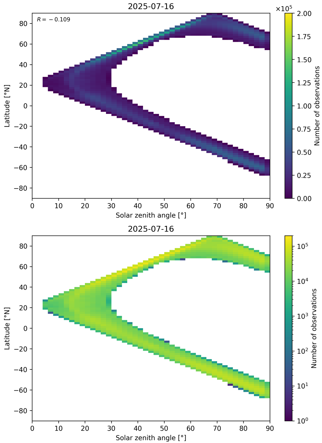
Figure 105: Scatter density plot of “Solar zenith angle” against “Latitude” for 2025-07-15 to 2025-07-17.
