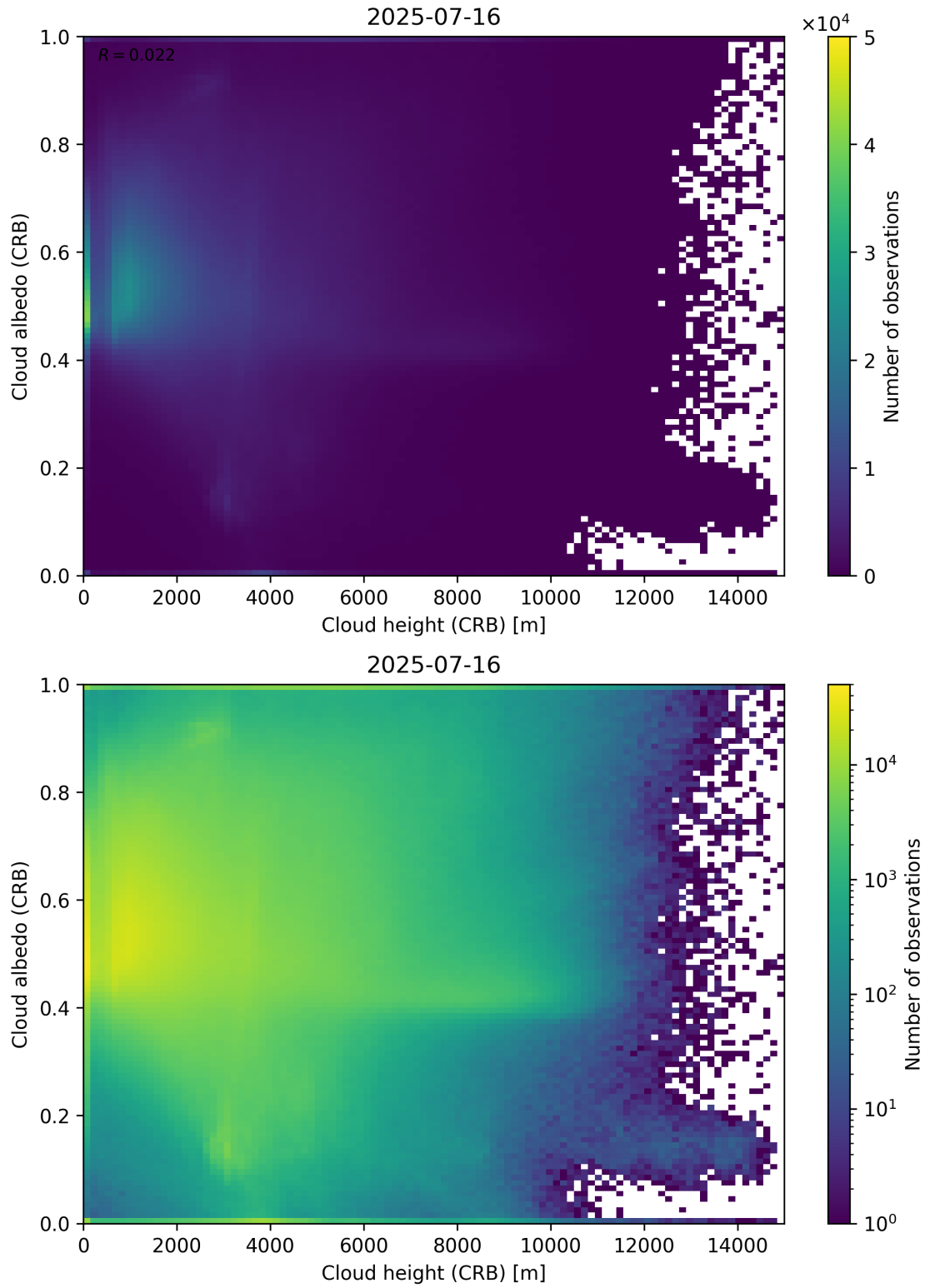
Figure 80: Scatter density plot of “Cloud height (CRB)” against “Cloud albedo (CRB)” for 2025-07-15 to 2025-07-17.
