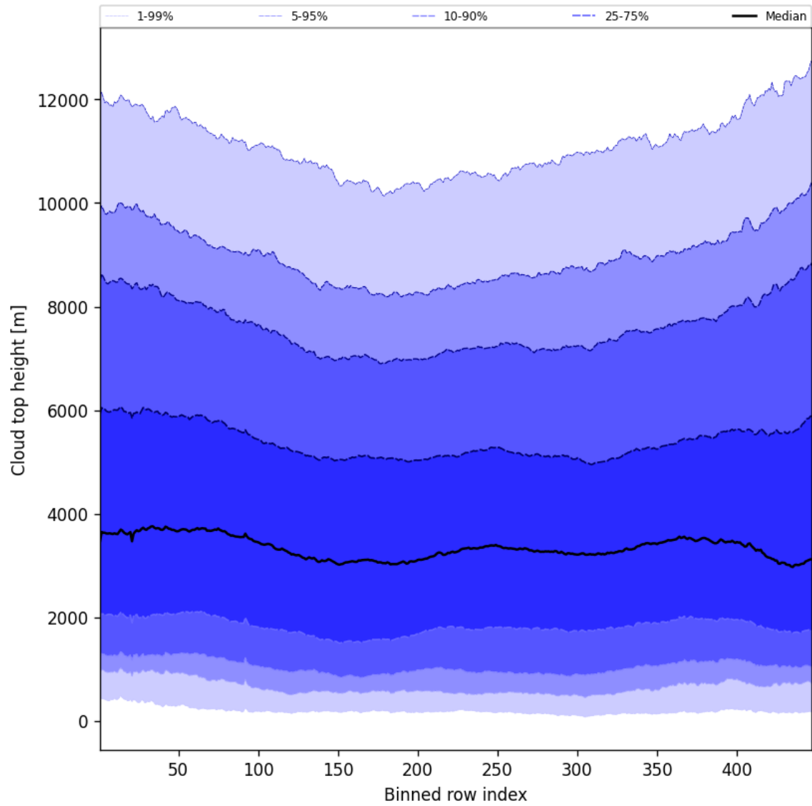
Figure 56: Along track statistics of “Cloud top height” for 2025-07-15 to 2025-07-17
