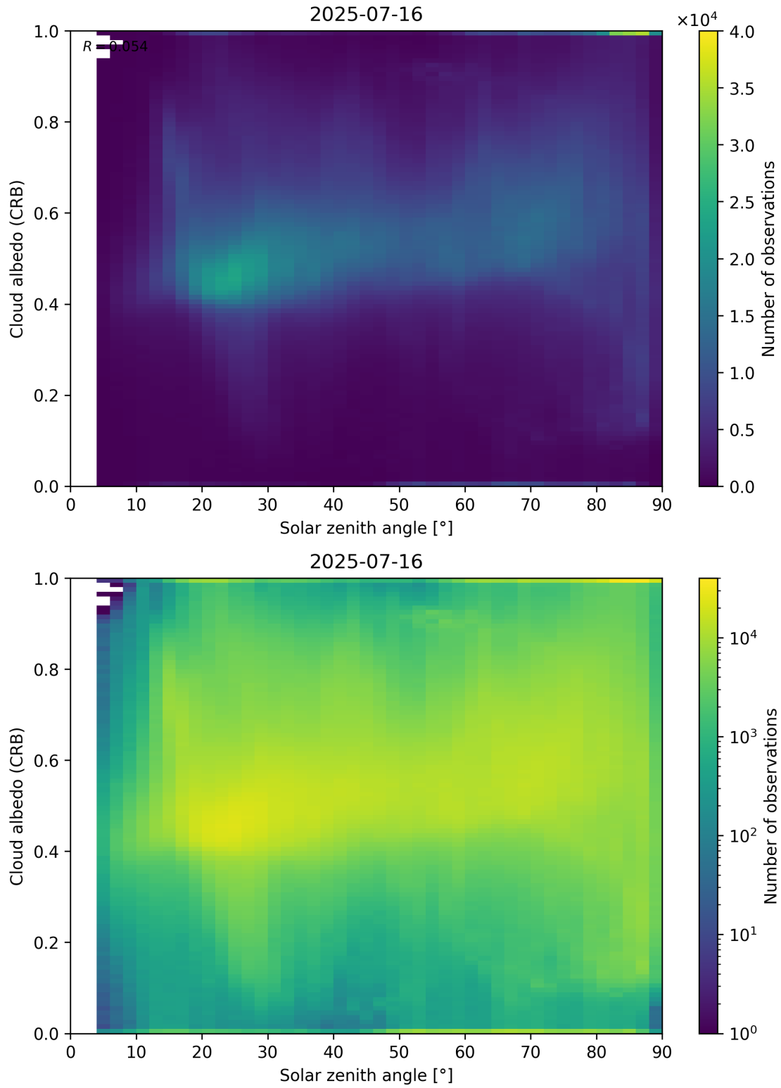
Figure 98: Scatter density plot of “Solar zenith angle” against “Cloud albedo (CRB)” for 2025-07-15 to 2025-07-17.
