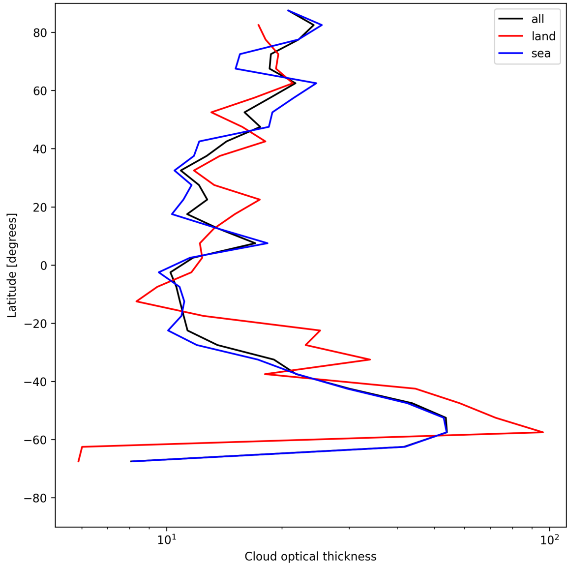
Figure 25: Zonal average of “Cloud optical thickness” for 2025-07-15 to 2025-07-17.
