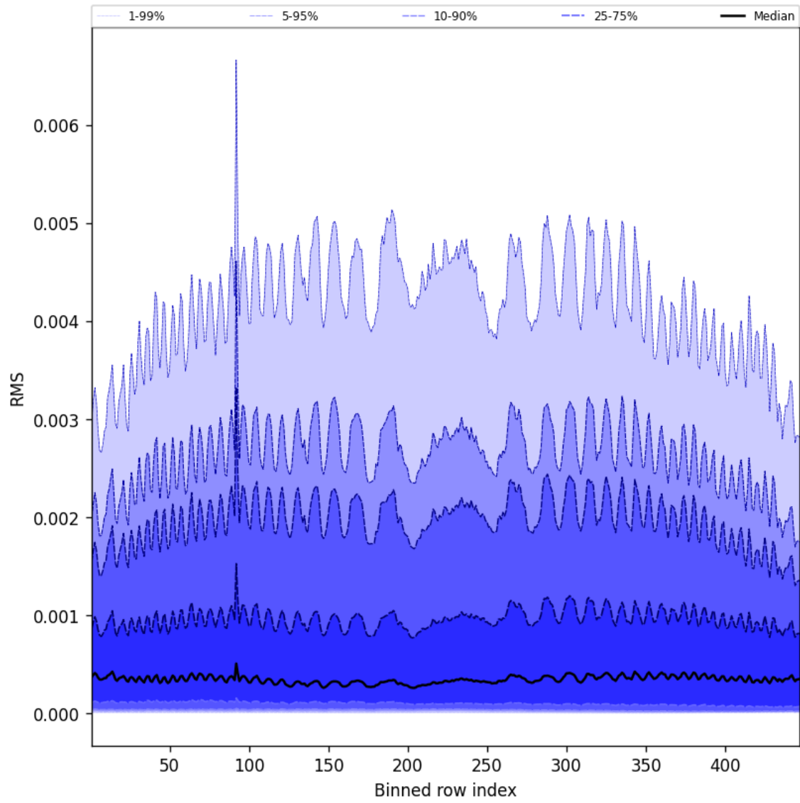
Figure 63: Along track statistics of “RMS” for 2025-07-15 to 2025-07-17
