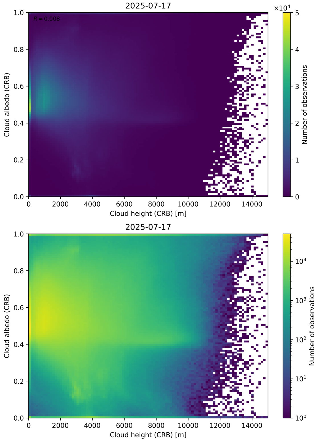
Figure 80: Scatter density plot of “Cloud height (CRB)” against “Cloud albedo (CRB)” for 2025-07-16 to 2025-07-18.
