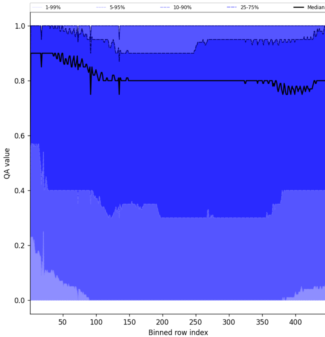
Figure 54: Along track statistics of “QA value” for 2025-07-16 to 2025-07-18
