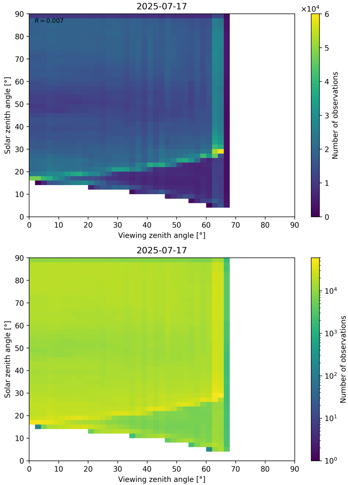
Figure 114: Scatter density plot of “Viewing zenith angle” against “Solar zenith angle” for 2025-07-16 to 2025-07-18.
