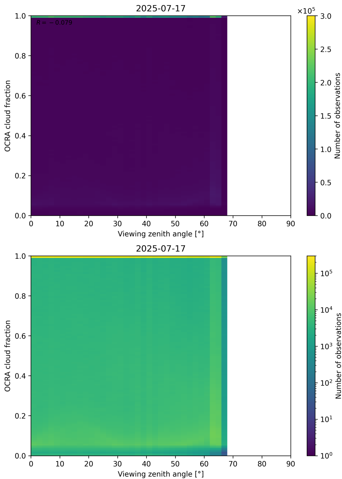
Figure 108: Scatter density plot of “Viewing zenith angle” against “OCRA cloud fraction” for 2025-07-16 to 2025-07-18.
