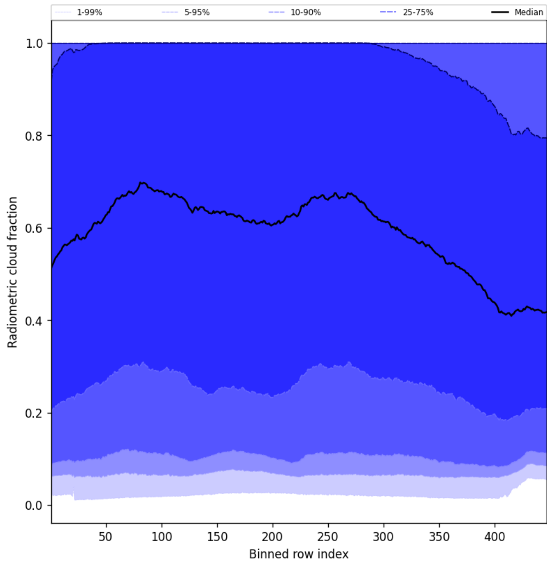
Figure 55: Along track statistics of “Radiometric cloud fraction” for 2025-07-16 to 2025-07-18
