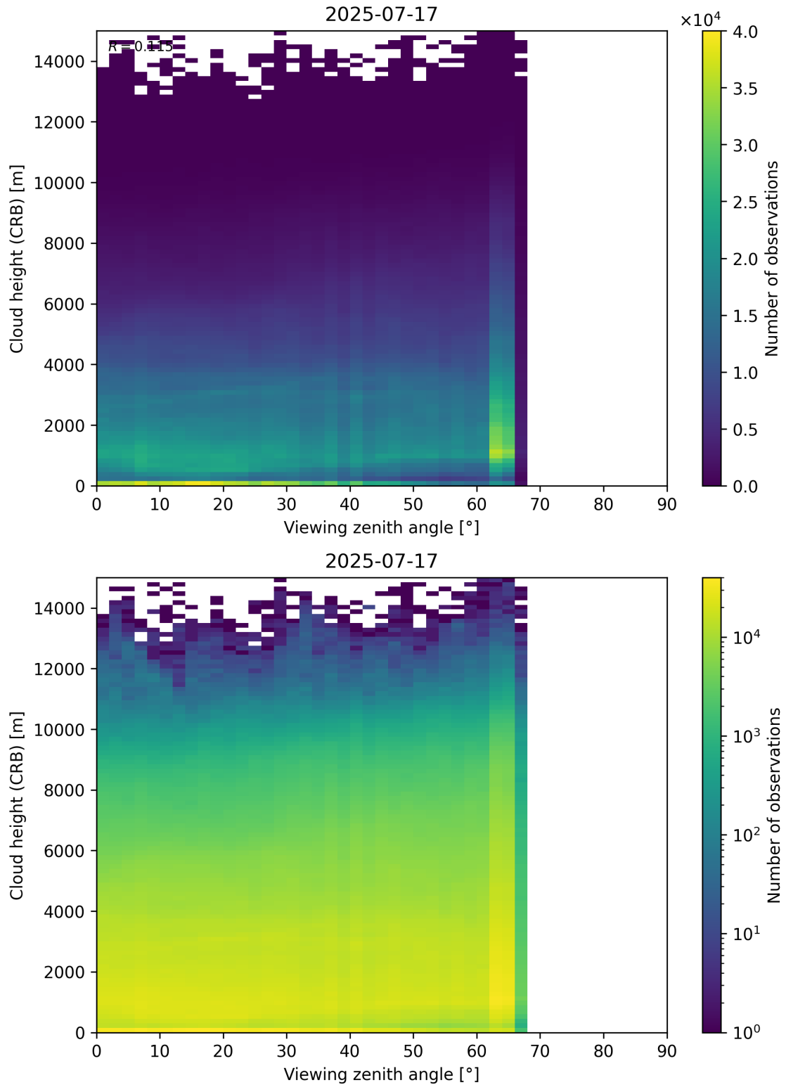
Figure 110: Scatter density plot of “Viewing zenith angle” against “Cloud height (CRB)” for 2025-07-16 to 2025-07-18.
