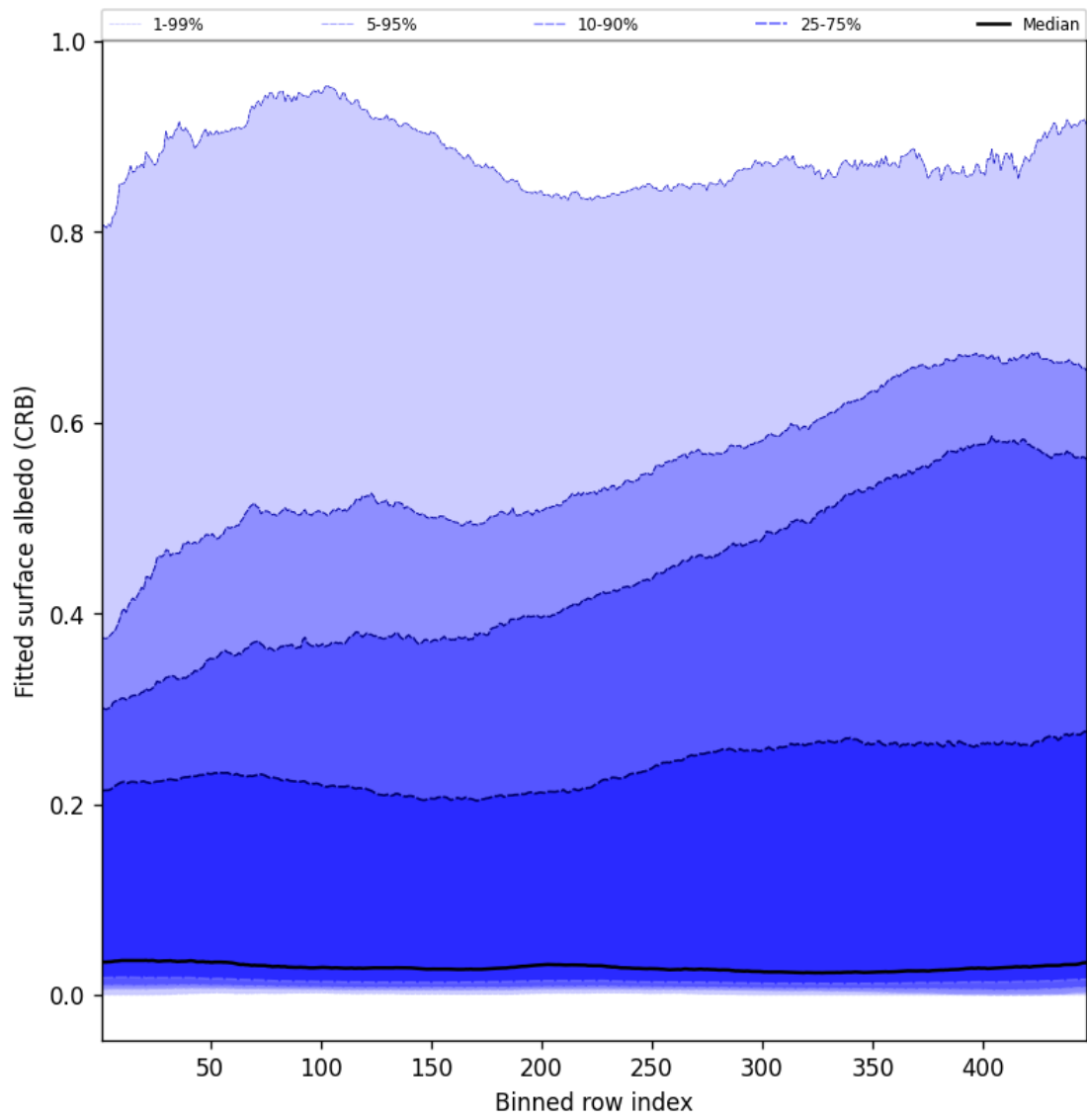
Figure 62: Along track statistics of “Fitted surface albedo (CRB)” for 2025-07-16 to 2025-07-18
