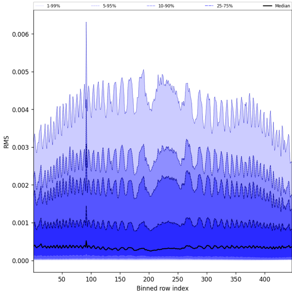
Figure 63: Along track statistics of “RMS” for 2025-07-16 to 2025-07-18
