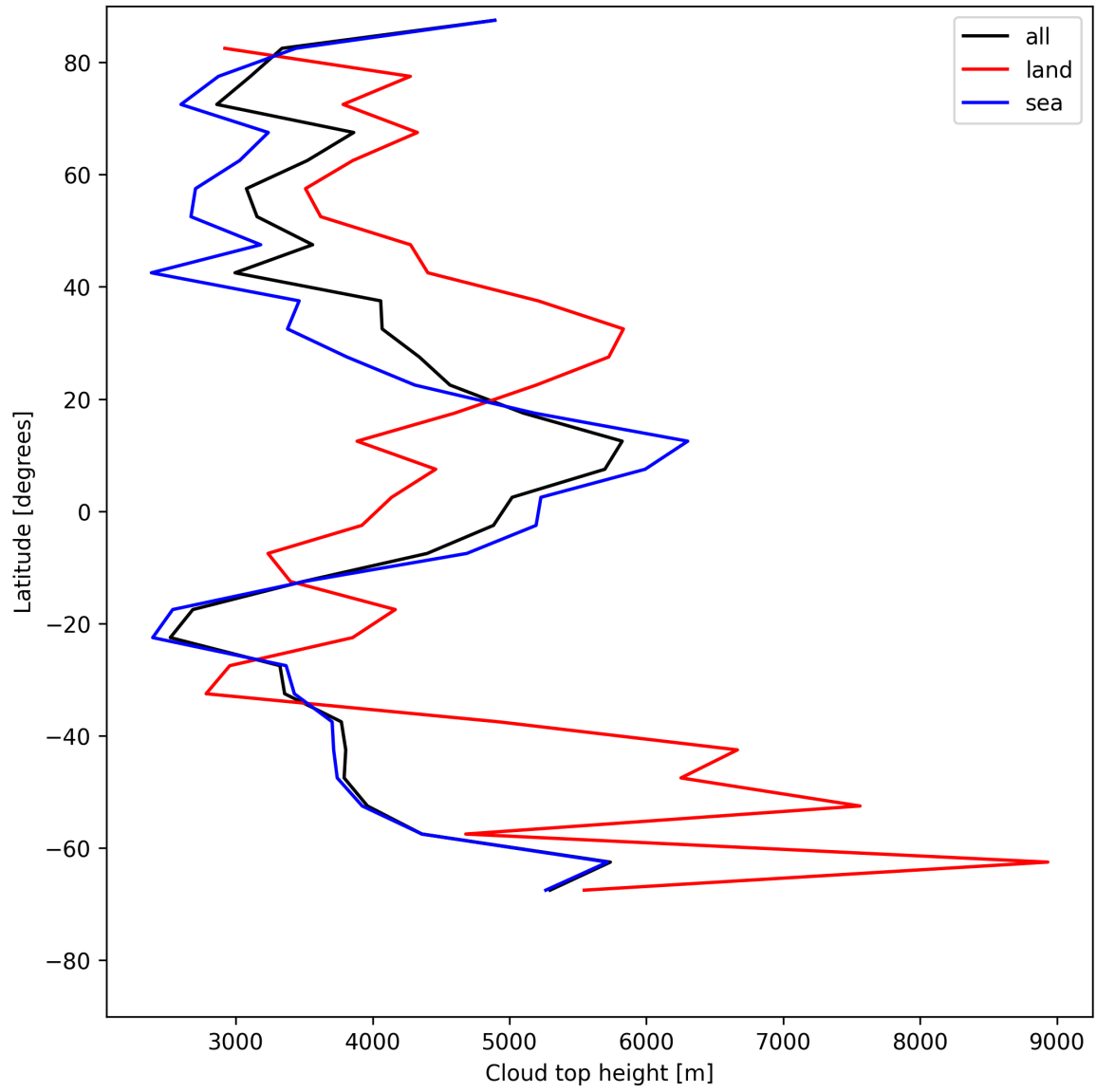
Figure 24: Zonal average of “Cloud top height” for 2025-07-16 to 2025-07-18.
