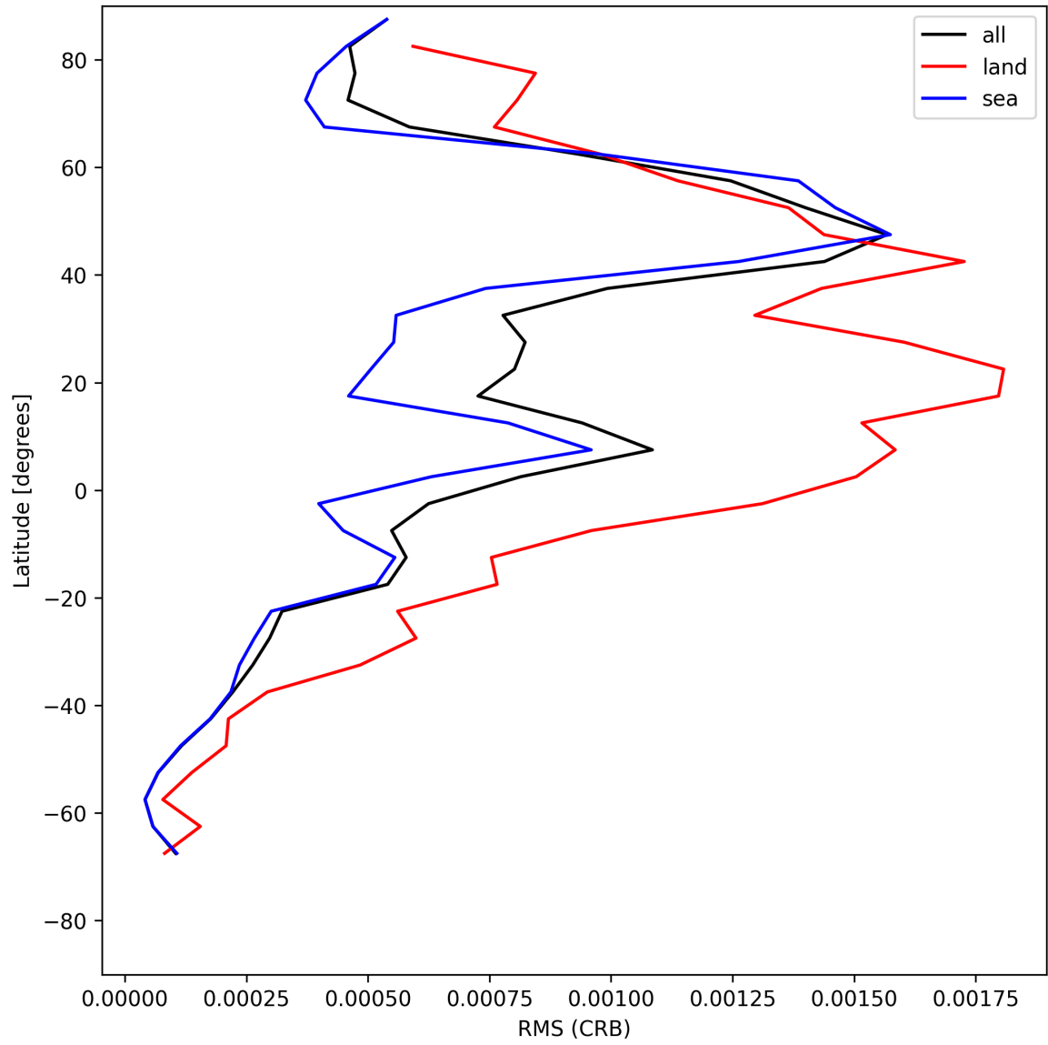
Figure 32: Zonal average of “RMS (CRB)” for 2025-07-16 to 2025-07-18.
