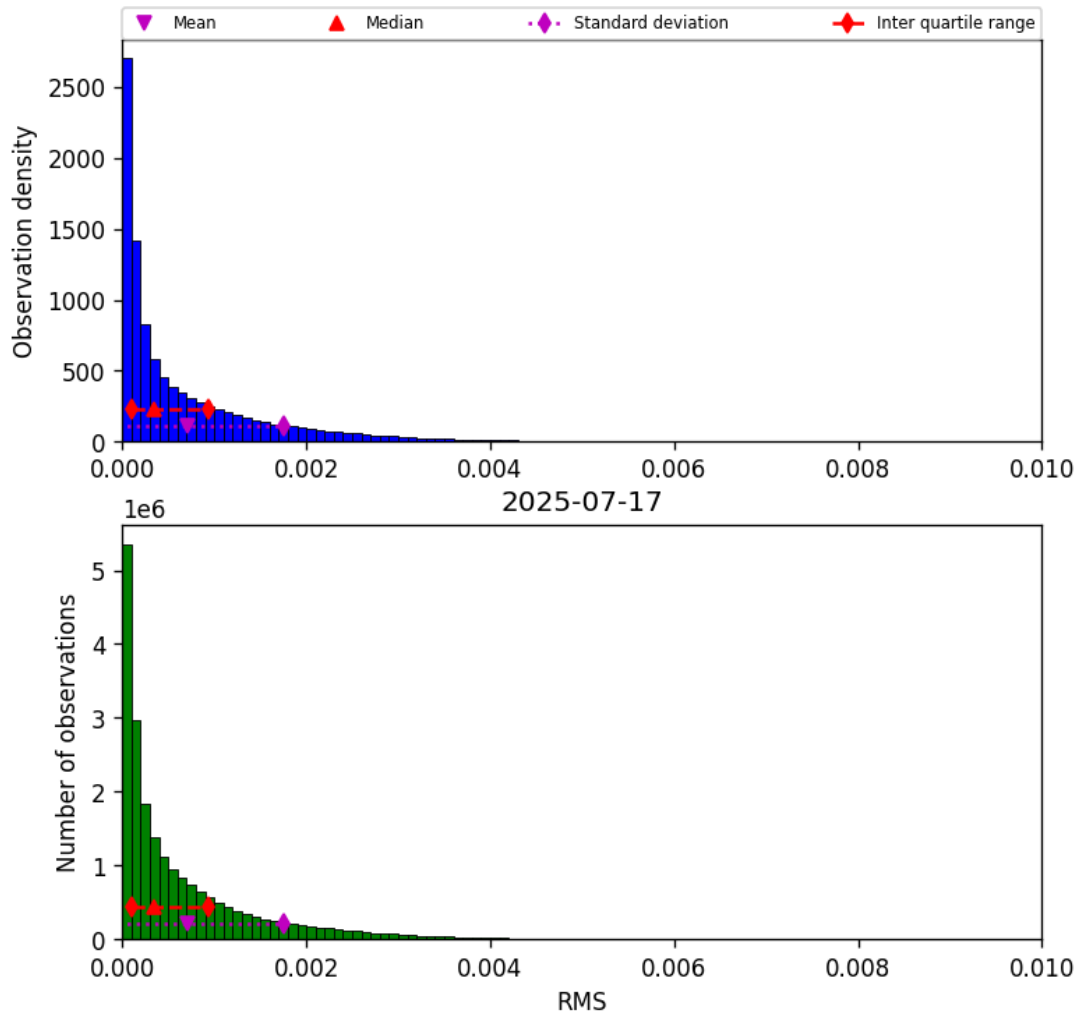
Figure 47: Histogram of “RMS” for 2025-07-16 to 2025-07-18
