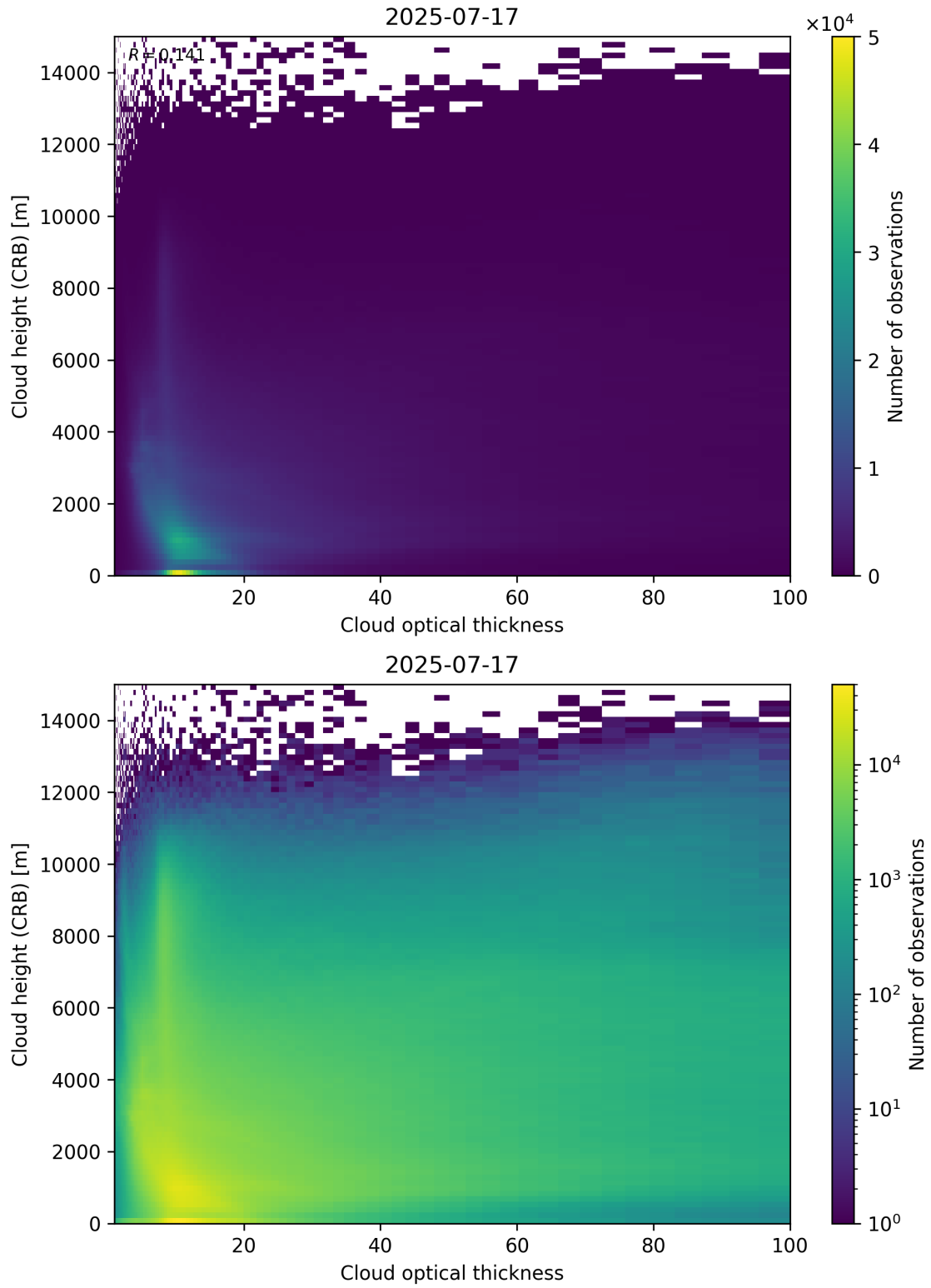
Figure 85: Scatter density plot of “Cloud optical thickness” against “Cloud height (CRB)” for 2025-07-16 to 2025-07-18.
