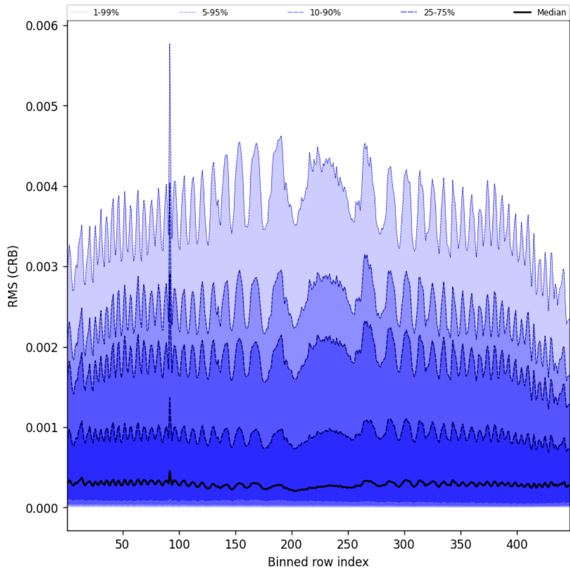
Figure 64: Along track statistics of “RMS (CRB)” for 2025-07-16 to 2025-07-18
