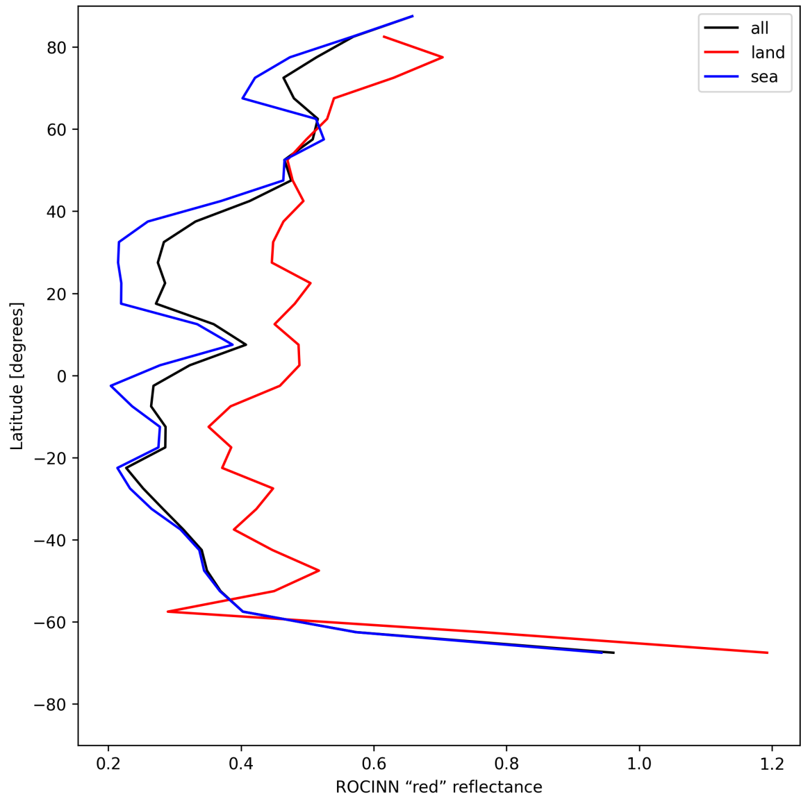
Figure 37: Zonal average of “ROCINN “red” reflectance” for 2025-07-16 to 2025-07-18.
