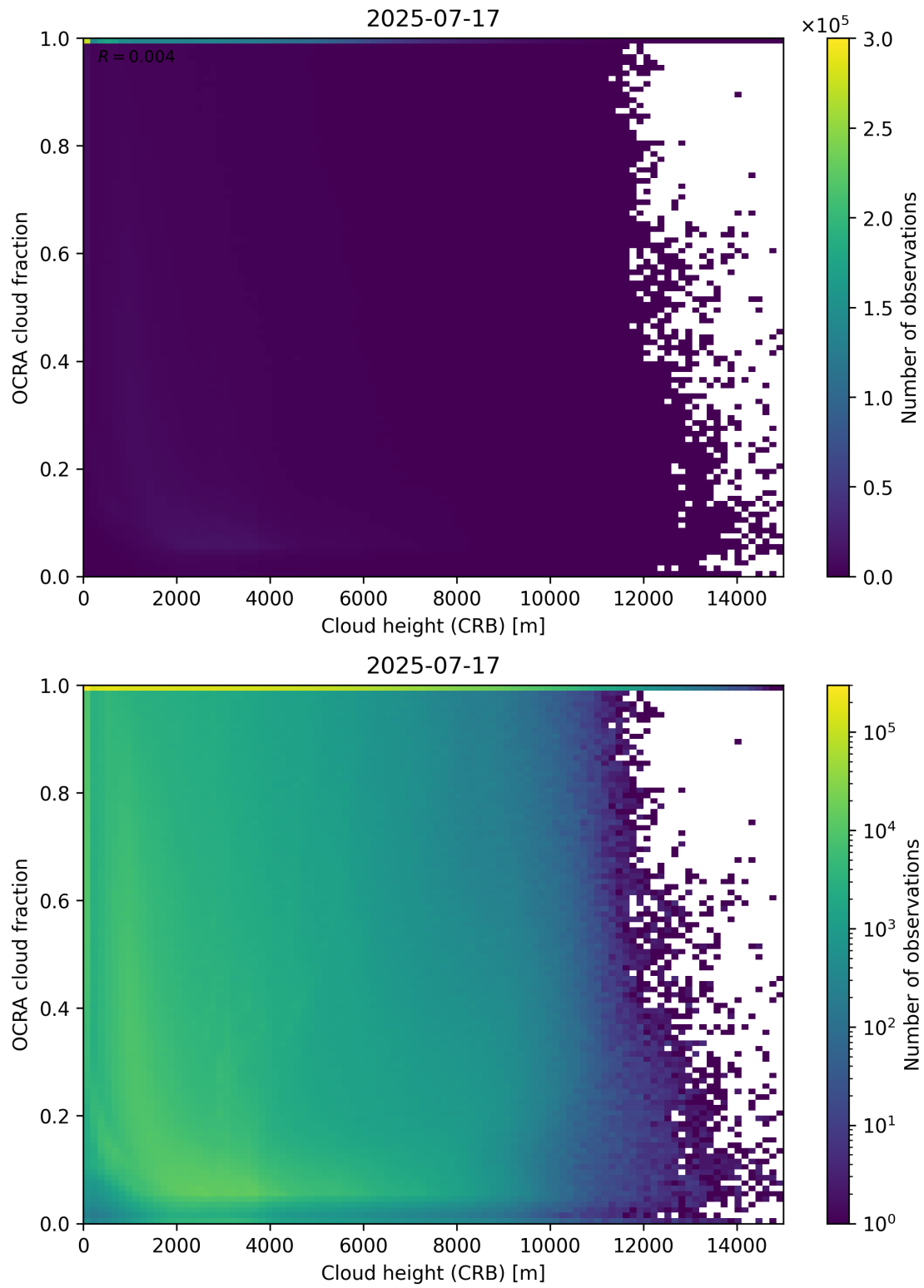
Figure 81: Scatter density plot of “Cloud height (CRB)” against “OCRA cloud fraction” for 2025-07-16 to 2025-07-18.
