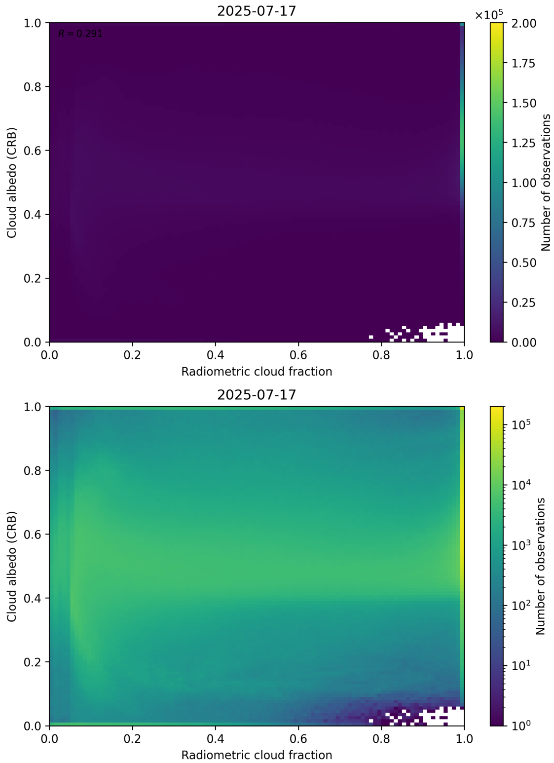
Figure 71: Scatter density plot of “Radiometric cloud fraction” against “Cloud albedo (CRB)” for 2025-07-16 to 2025-07-18.
