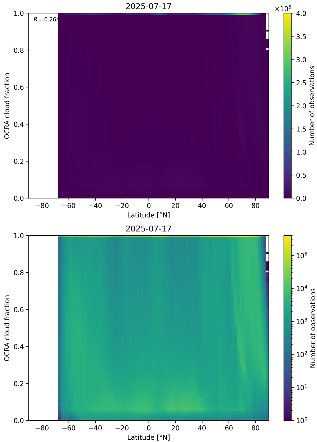
Figure 93: Scatter density plot of “Latitude” against “OCRA cloud fraction” for 2025-07-16 to 2025-07-18.
