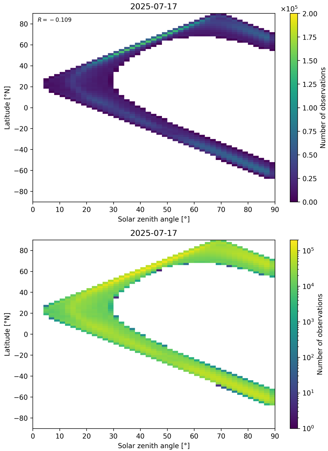
Figure 105: Scatter density plot of “Solar zenith angle” against “Latitude” for 2025-07-16 to 2025-07-18.
