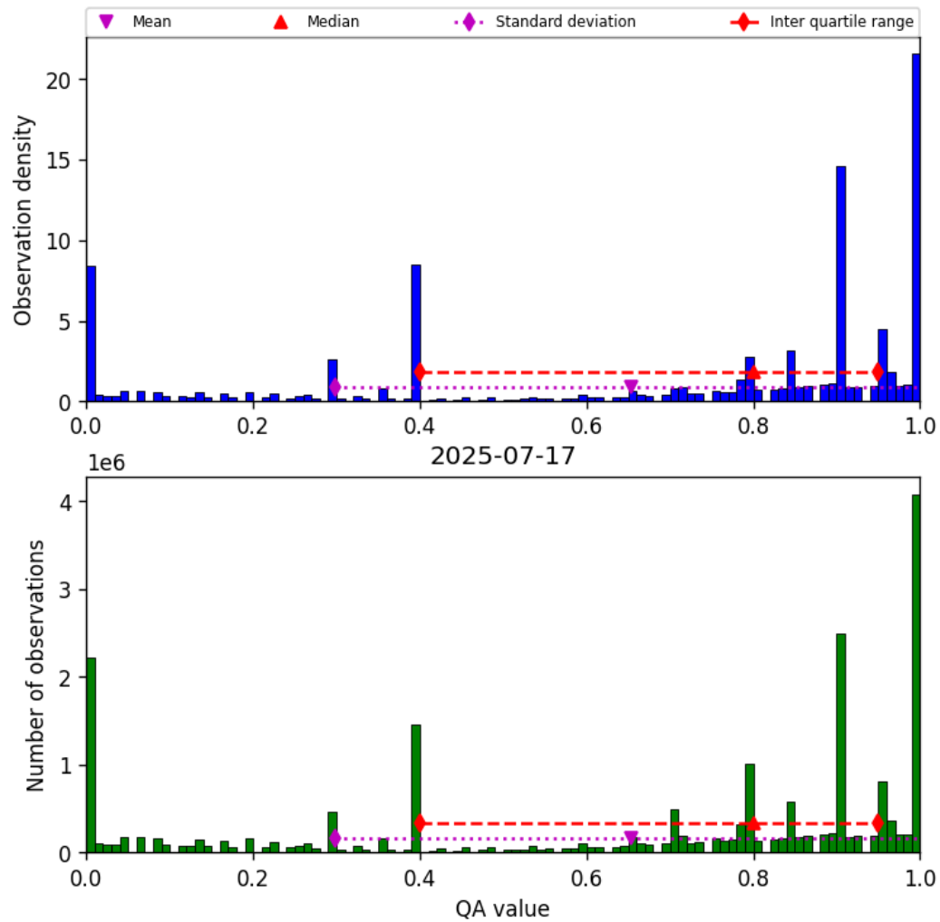
Figure 38: Histogram of “QA value” for 2025-07-16 to 2025-07-18
