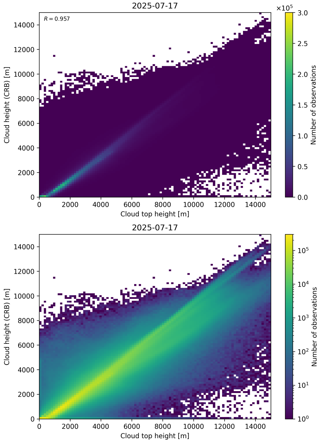
Figure 89: Scatter density plot of “Cloud top height” against “Cloud height (CRB)” for 2025-07-16 to 2025-07-18.
