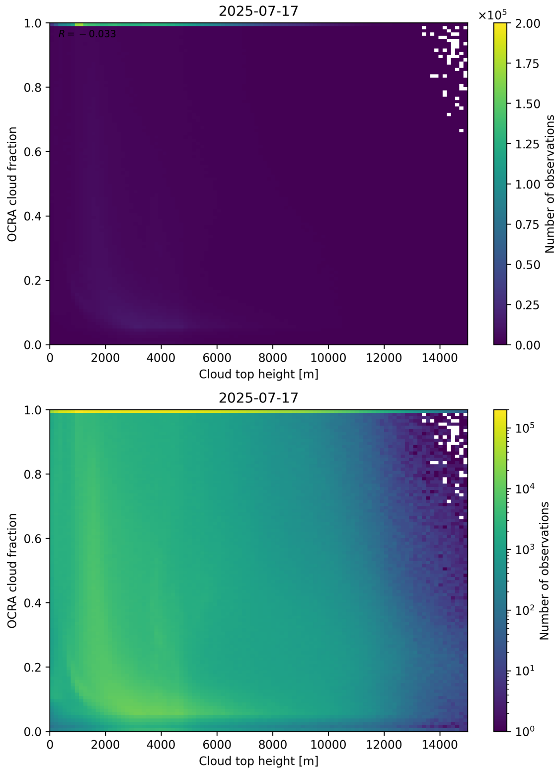
Figure 87: Scatter density plot of “Cloud top height” against “OCRA cloud fraction” for 2025-07-16 to 2025-07-18.
