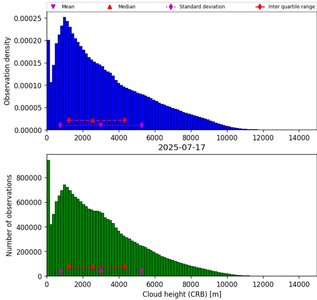
Figure 43: Histogram of “Cloud height (CRB)” for 2025-07-16 to 2025-07-18
