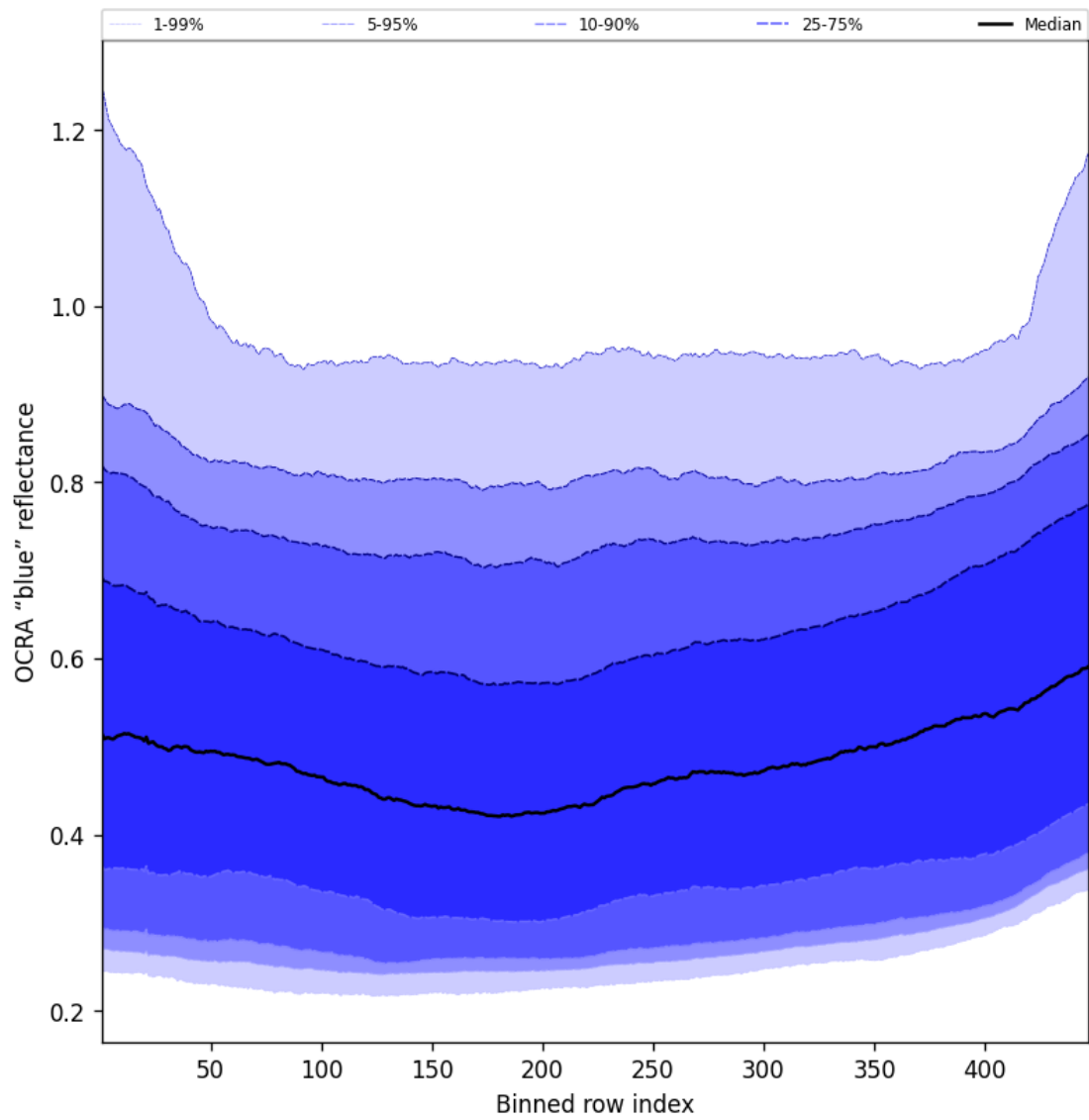
Figure 67: Along track statistics of “OCRA “blue” reflectance” for 2025-07-16 to 2025-07-18
