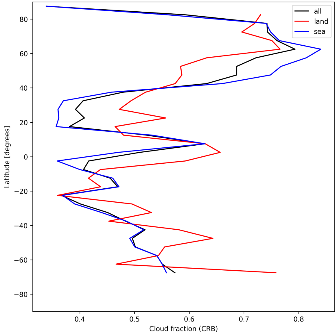
Figure 26: Zonal average of “Cloud fraction (CRB)” for 2025-07-16 to 2025-07-18.
