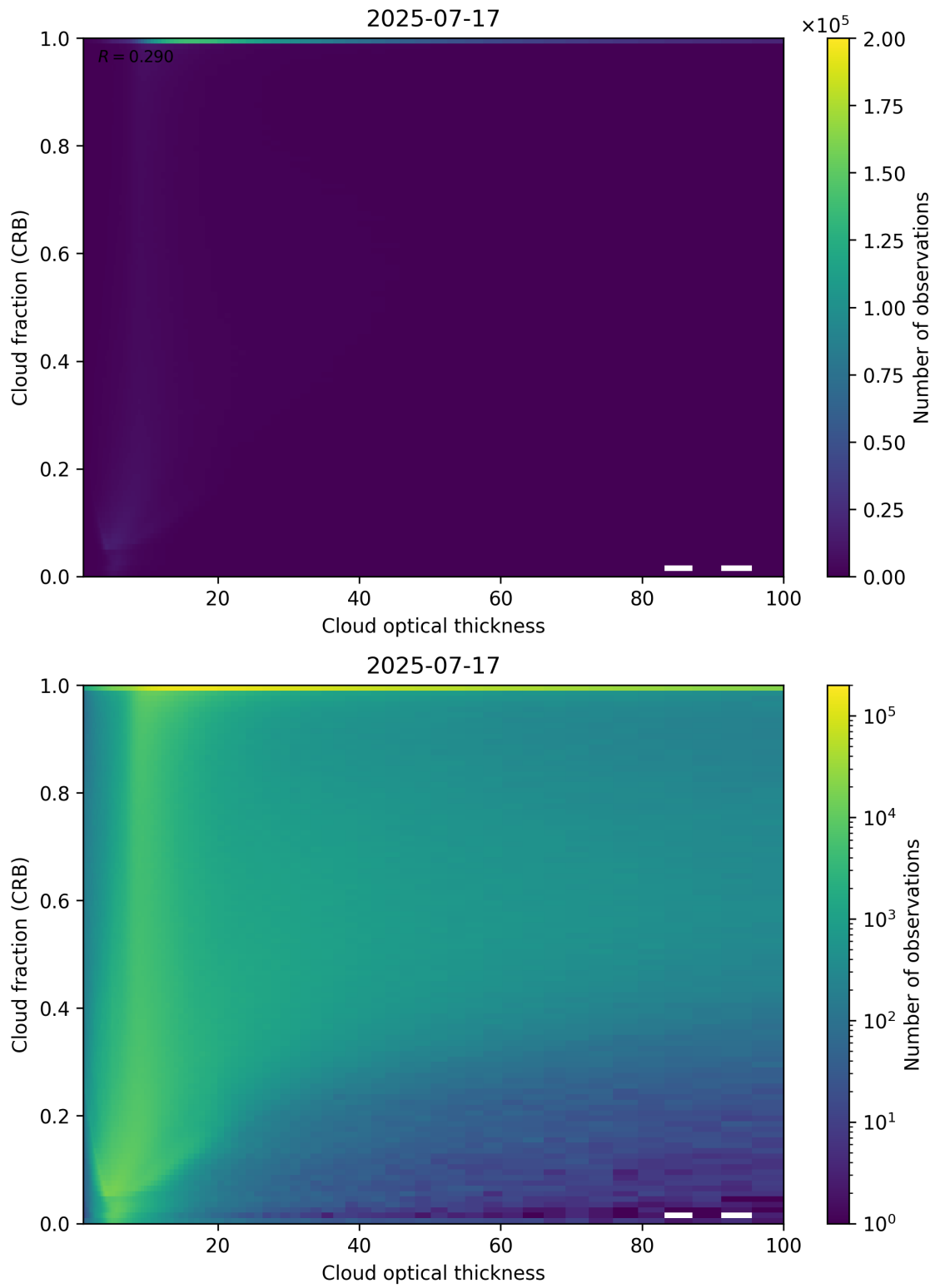
Figure 84: Scatter density plot of “Cloud optical thickness” against “Cloud fraction (CRB)” for 2025-07-16 to 2025-07-18.
