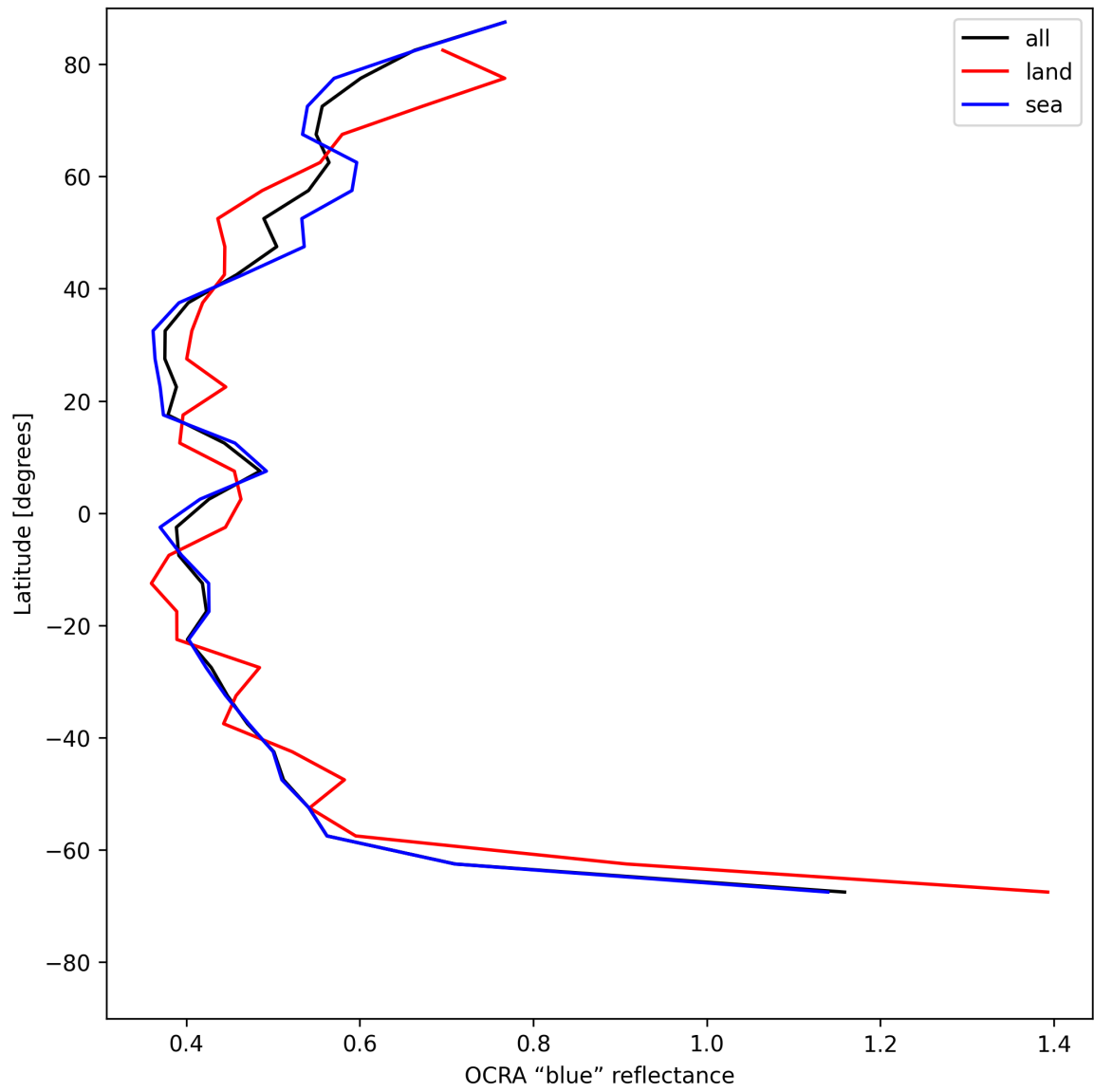
Figure 35: Zonal average of "OCRA "blue" reflectance" for 2025-07-16 to 2025-07-18.
