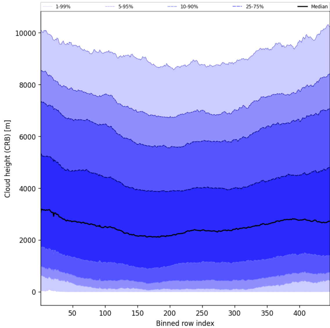
Figure 59: Along track statistics of “Cloud height (CRB)” for 2025-07-16 to 2025-07-18
