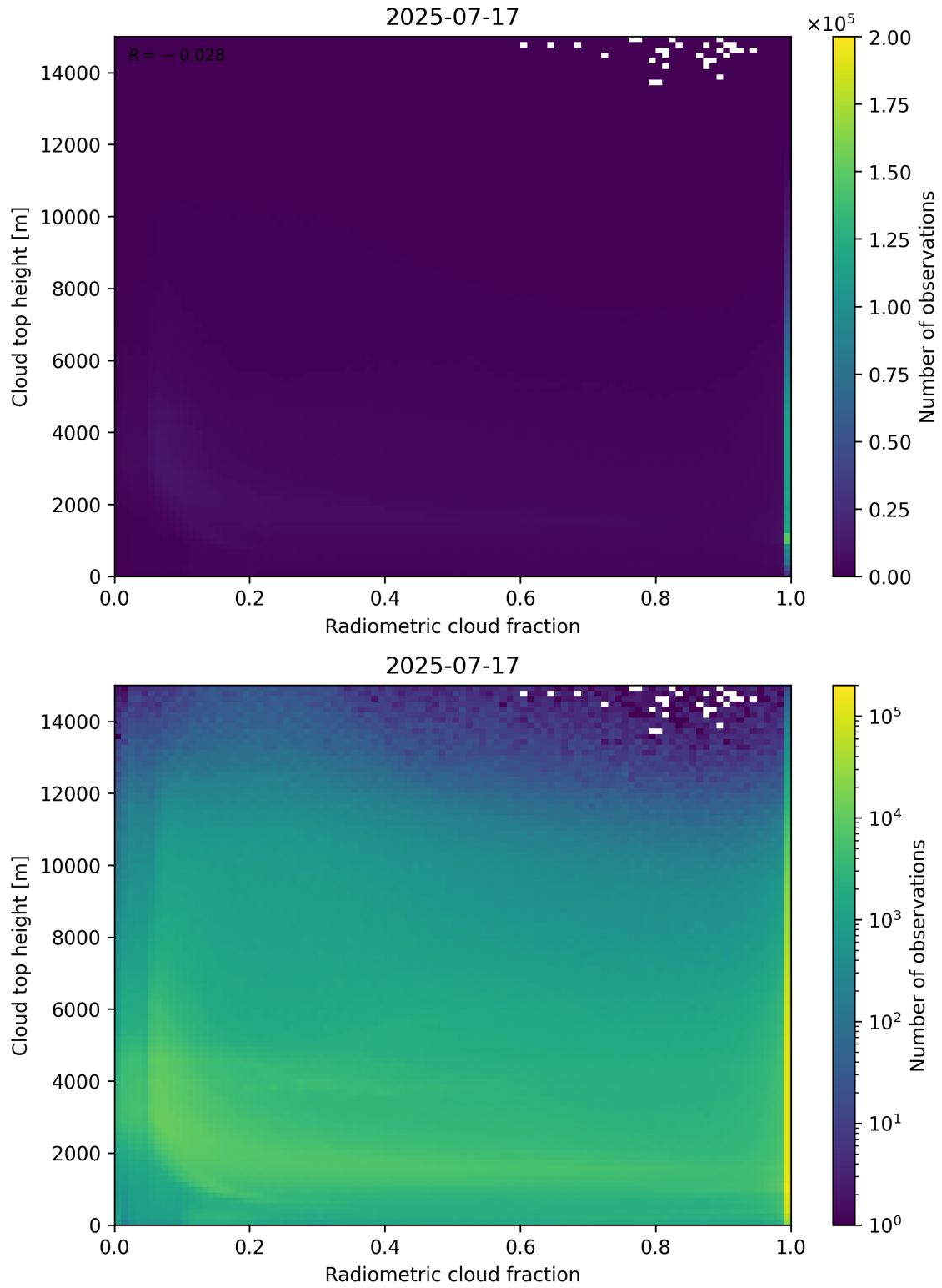
Figure 76: Scatter density plot of “Radiometric cloud fraction” against “Cloud top height” for 2025-07-16 to 2025-07-18.
