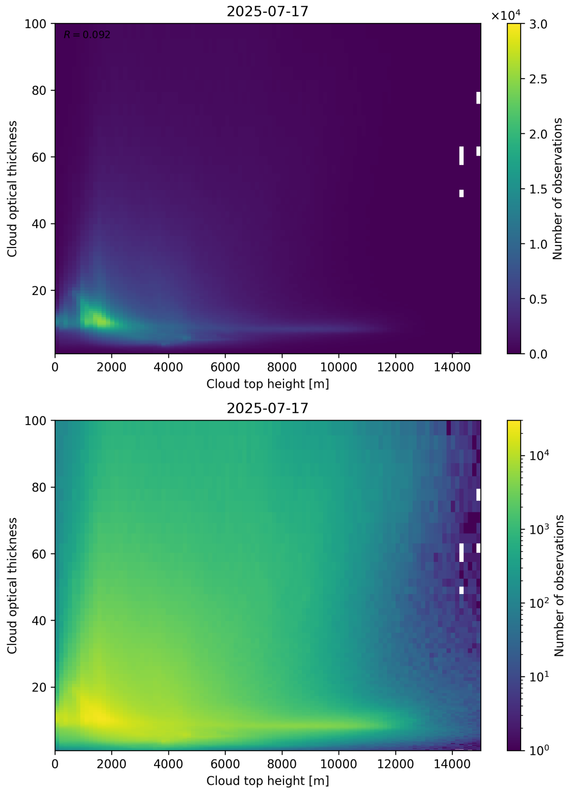
Figure 90: Scatter density plot of “Cloud top height” against “Cloud optical thickness” for 2025-07-16 to 2025-07-18.
