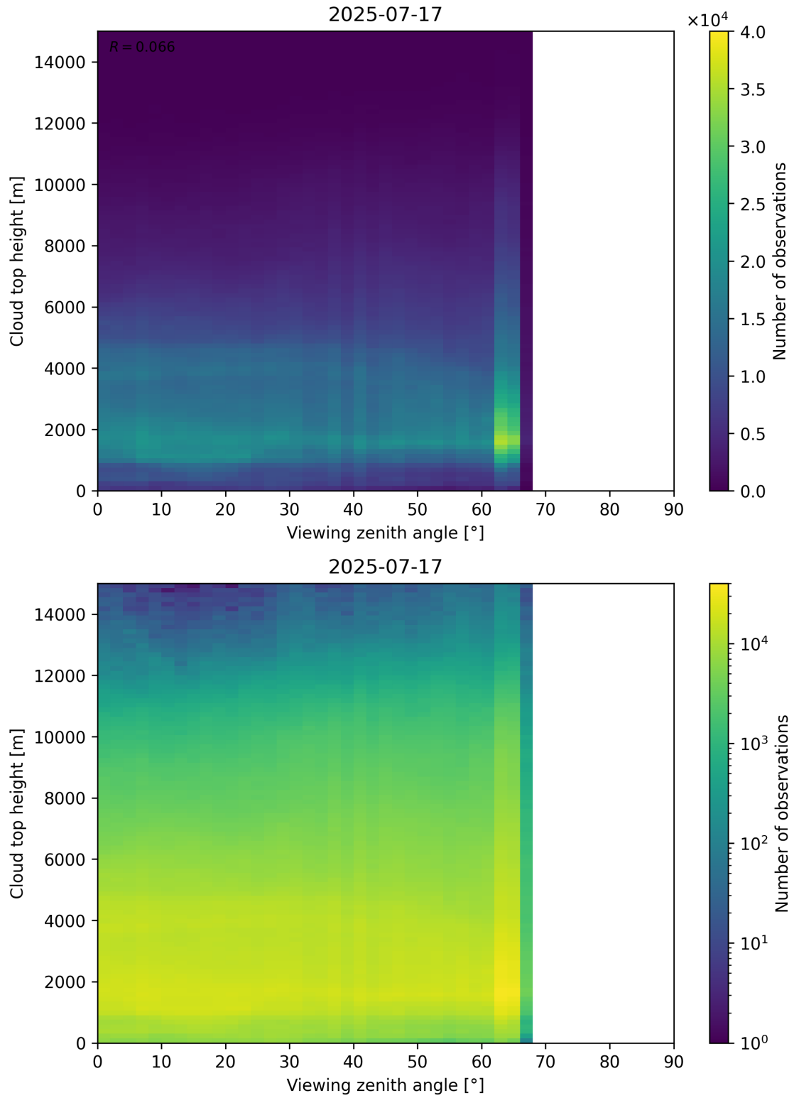
Figure 112: Scatter density plot of “Viewing zenith angle” against “Cloud top height” for 2025-07-16 to 2025-07-18.
