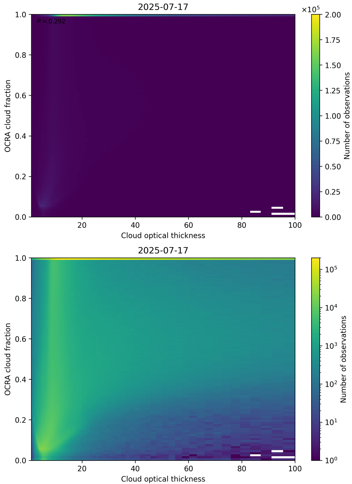
Figure 83: Scatter density plot of “Cloud optical thickness” against “OCRA cloud fraction” for 2025-07-16 to 2025-07-18.
