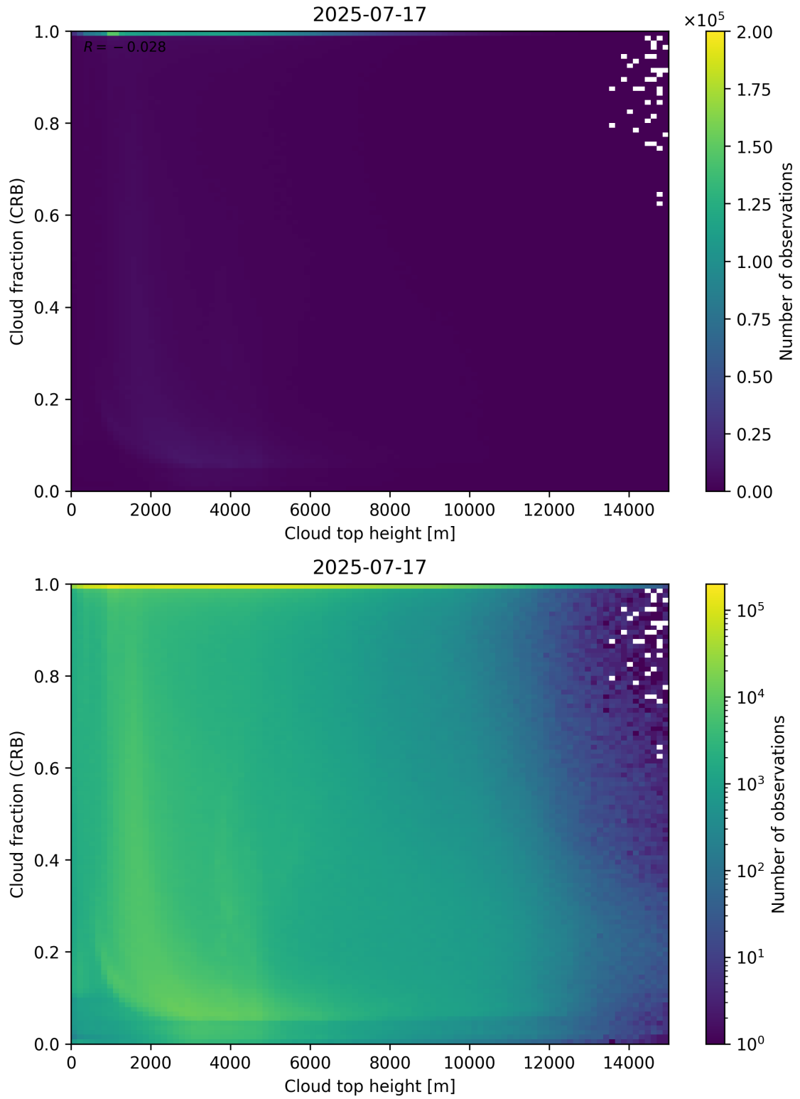
Figure 88: Scatter density plot of “Cloud top height” against “Cloud fraction (CRB)” for 2025-07-16 to 2025-07-18.
