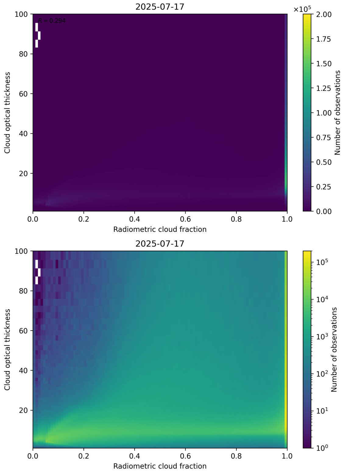
Figure 75: Scatter density plot of “Radiometric cloud fraction” against “Cloud optical thickness” for 2025-07-16 to 2025-07-18.
