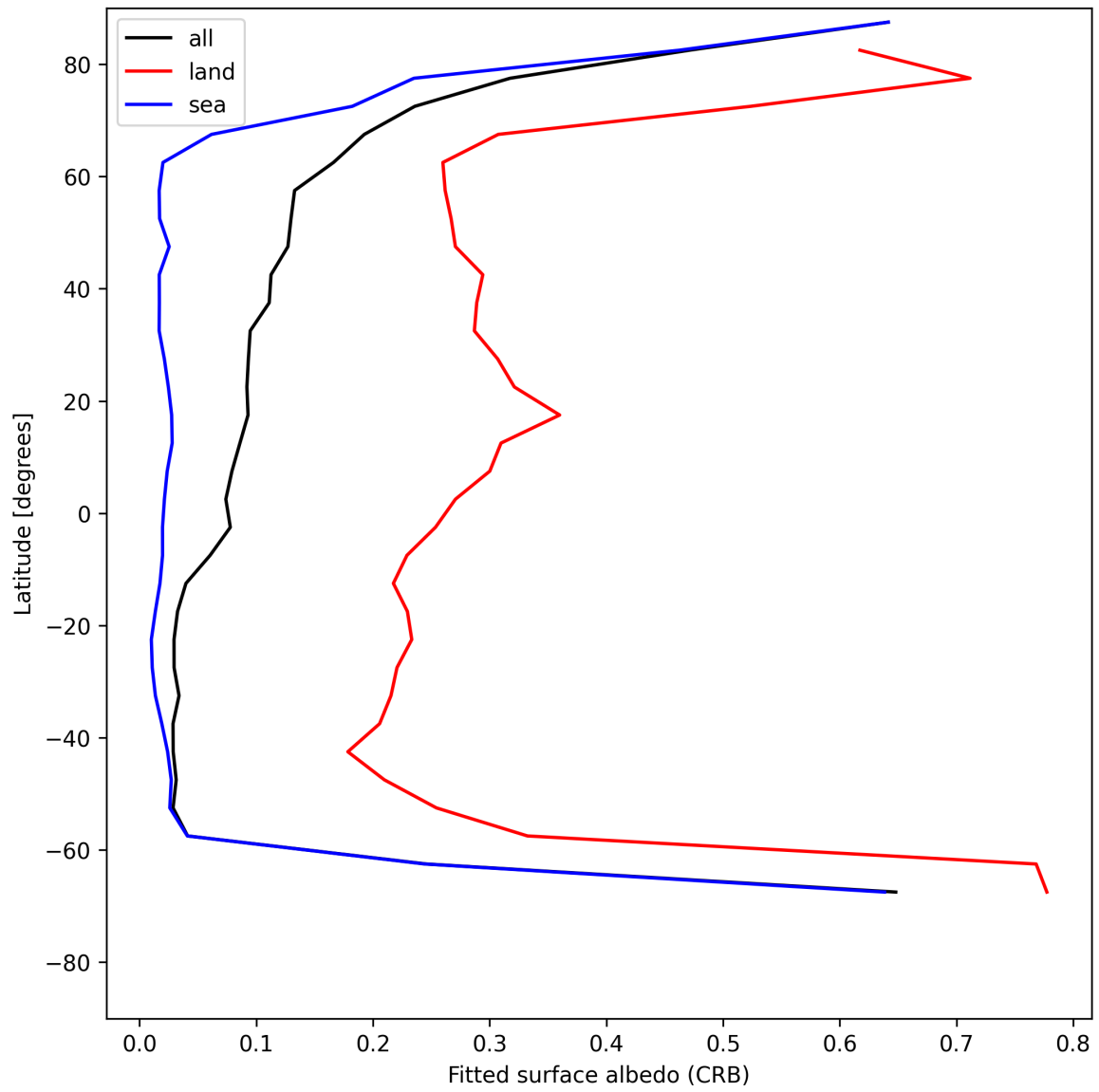
Figure 30: Zonal average of “Fitted surface albedo (CRB)” for 2025-07-16 to 2025-07-18.
