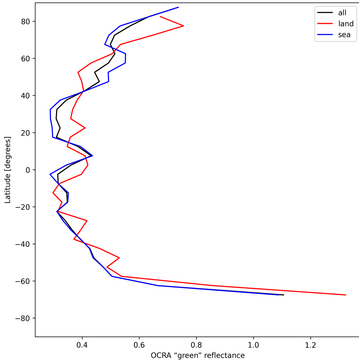
Figure 36: Zonal average of “OCRA “green” reflectance” for 2025-07-16 to 2025-07-18.
