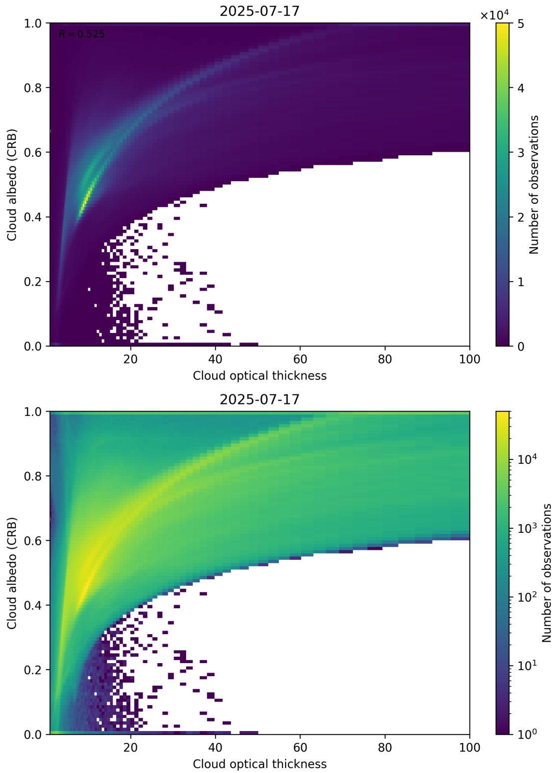
Figure 82: Scatter density plot of “Cloud optical thickness” against “Cloud albedo (CRB)” for 2025-07-16 to 2025-07-18.
