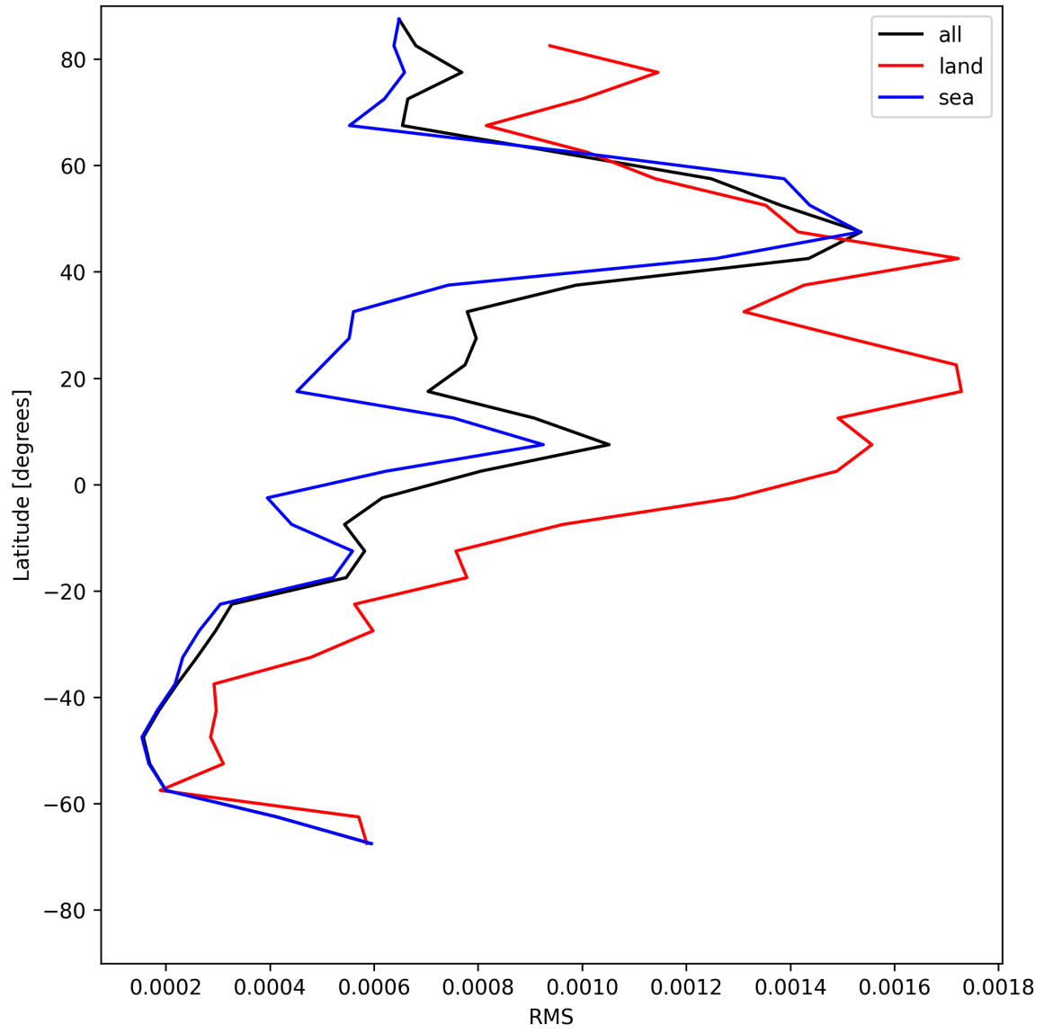
Figure 31: Zonal average of “RMS” for 2025-07-16 to 2025-07-18.
