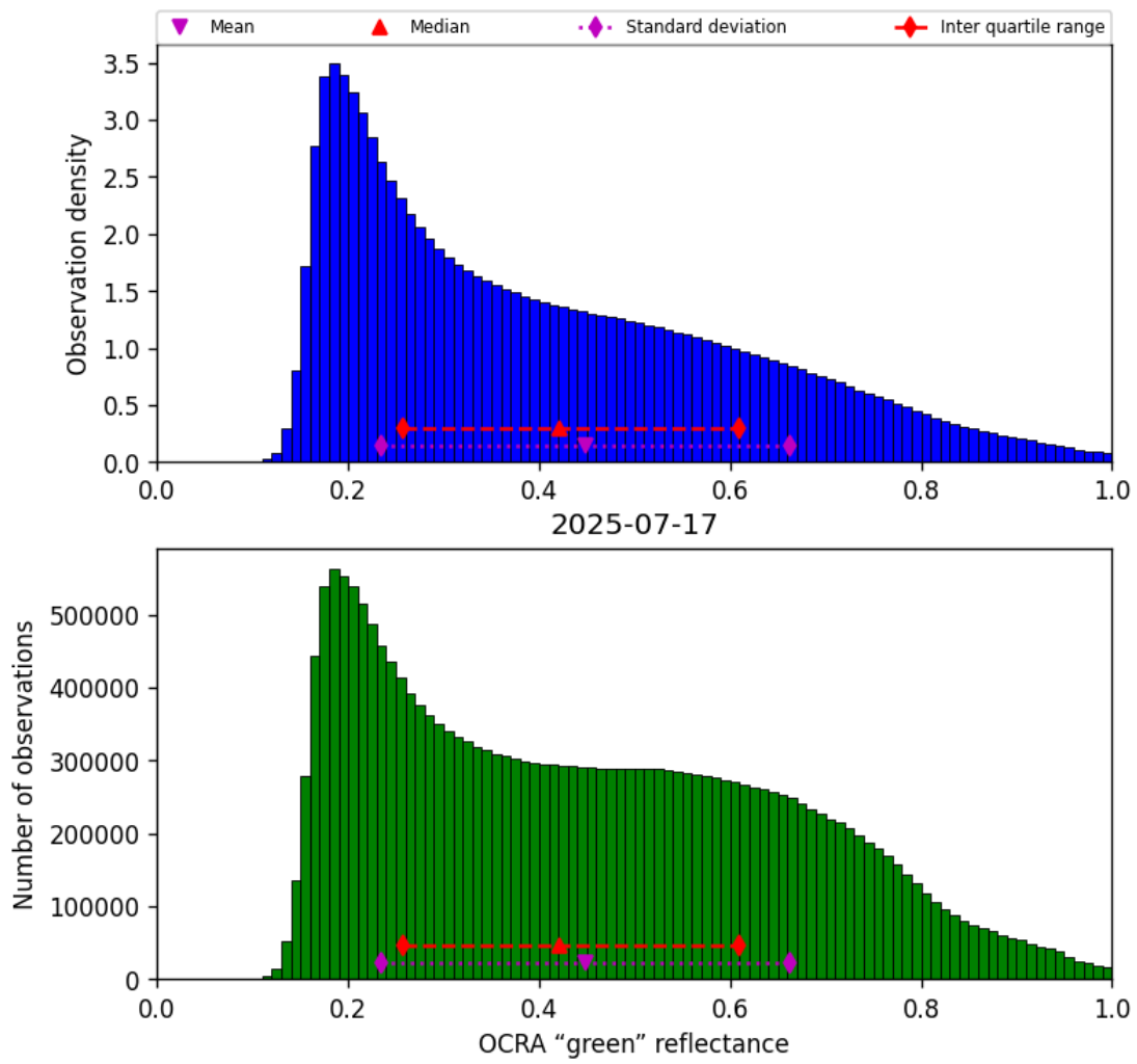
Figure 52: Histogram of “OCRA “green” reflectance” for 2025-07-16 to 2025-07-18
