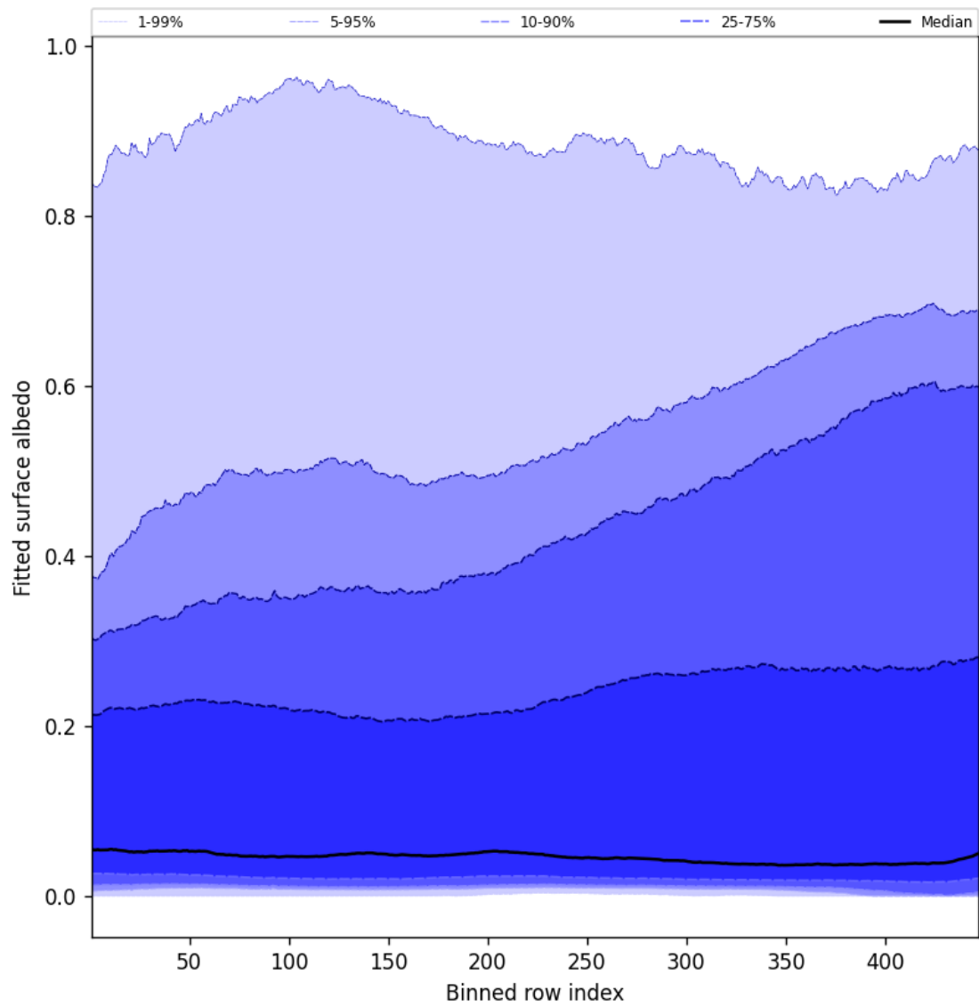
Figure 61: Along track statistics of “Fitted surface albedo” for 2025-07-16 to 2025-07-18
