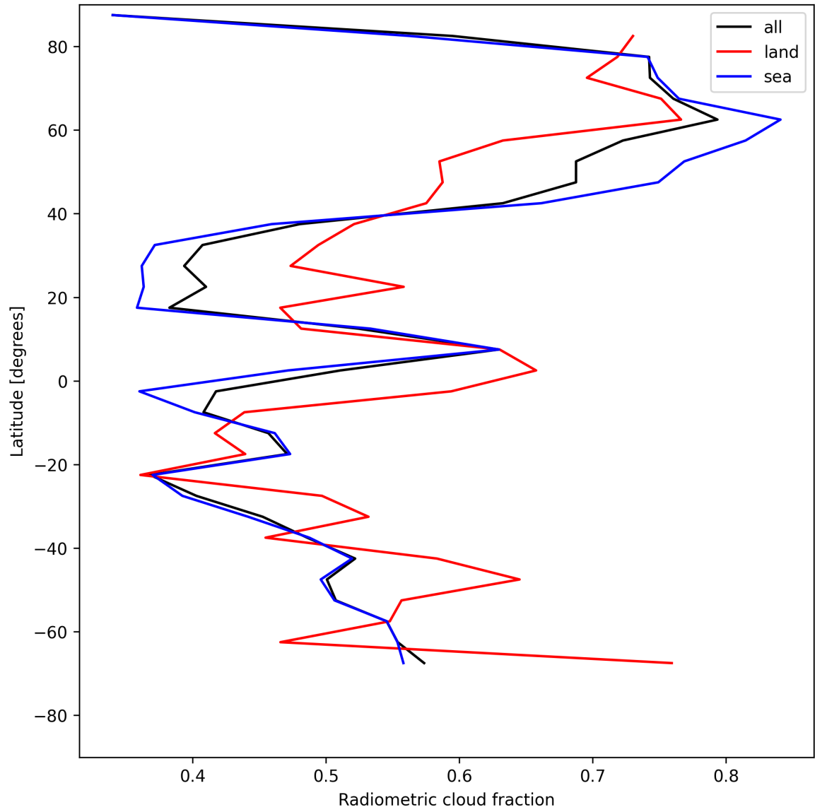
Figure 23: Zonal average of “Radiometric cloud fraction” for 2025-07-16 to 2025-07-18.
