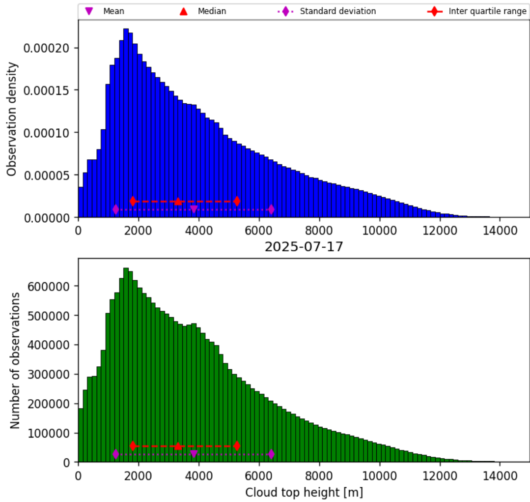
Figure 40: Histogram of “Cloud top height” for 2025-07-16 to 2025-07-18
