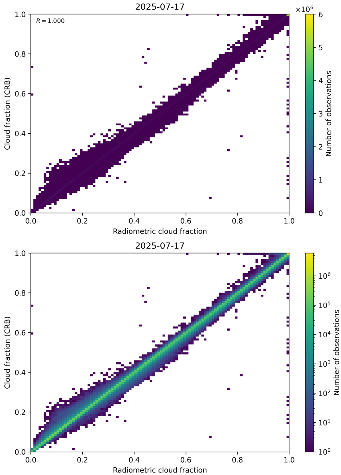
Figure 73: Scatter density plot of “Radiometric cloud fraction” against “Cloud fraction (CRB)” for 2025-07-16 to 2025-07-18.
