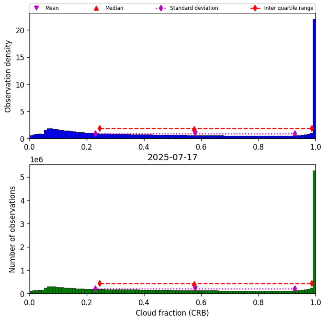
Figure 42: Histogram of “Cloud fraction (CRB)” for 2025-07-16 to 2025-07-18
