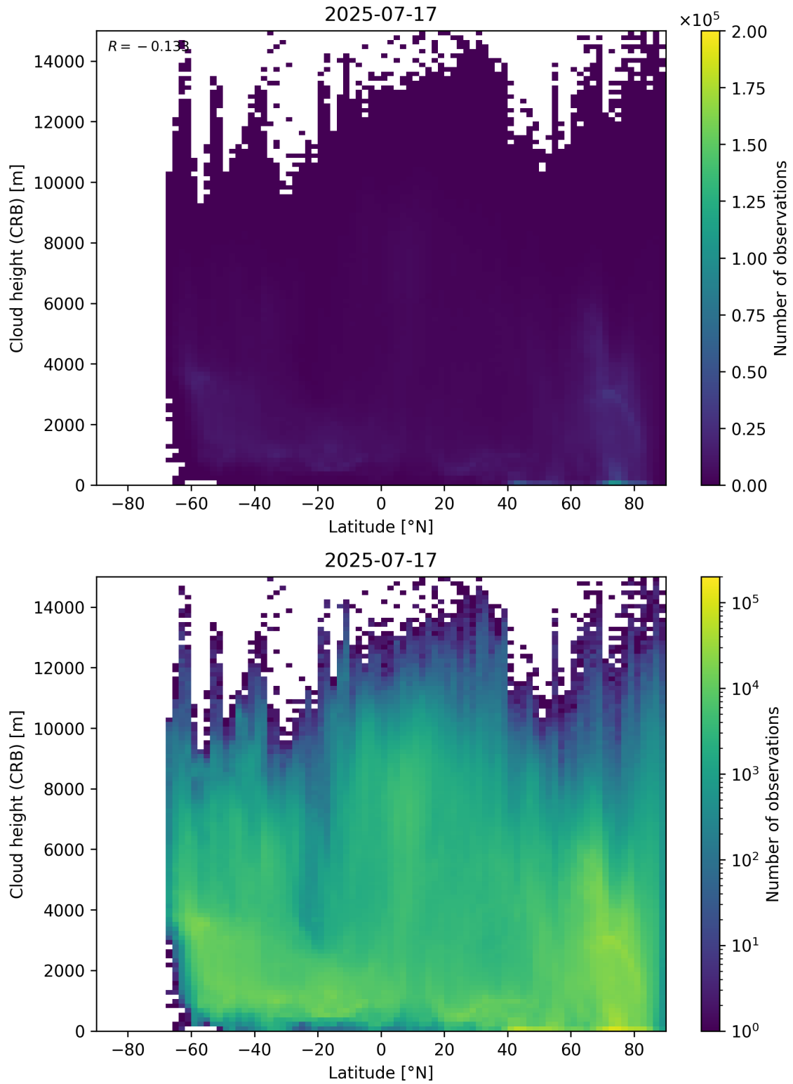
Figure 95: Scatter density plot of “Latitude” against “Cloud height (CRB)” for 2025-07-16 to 2025-07-18.
