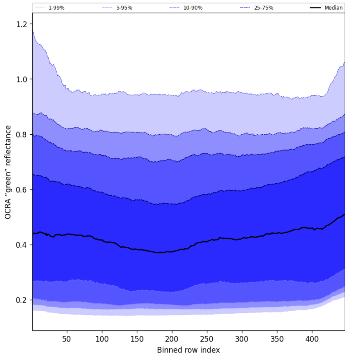
Figure 68: Along track statistics of “OCRA “green” reflectance” for 2025-07-16 to 2025-07-18
