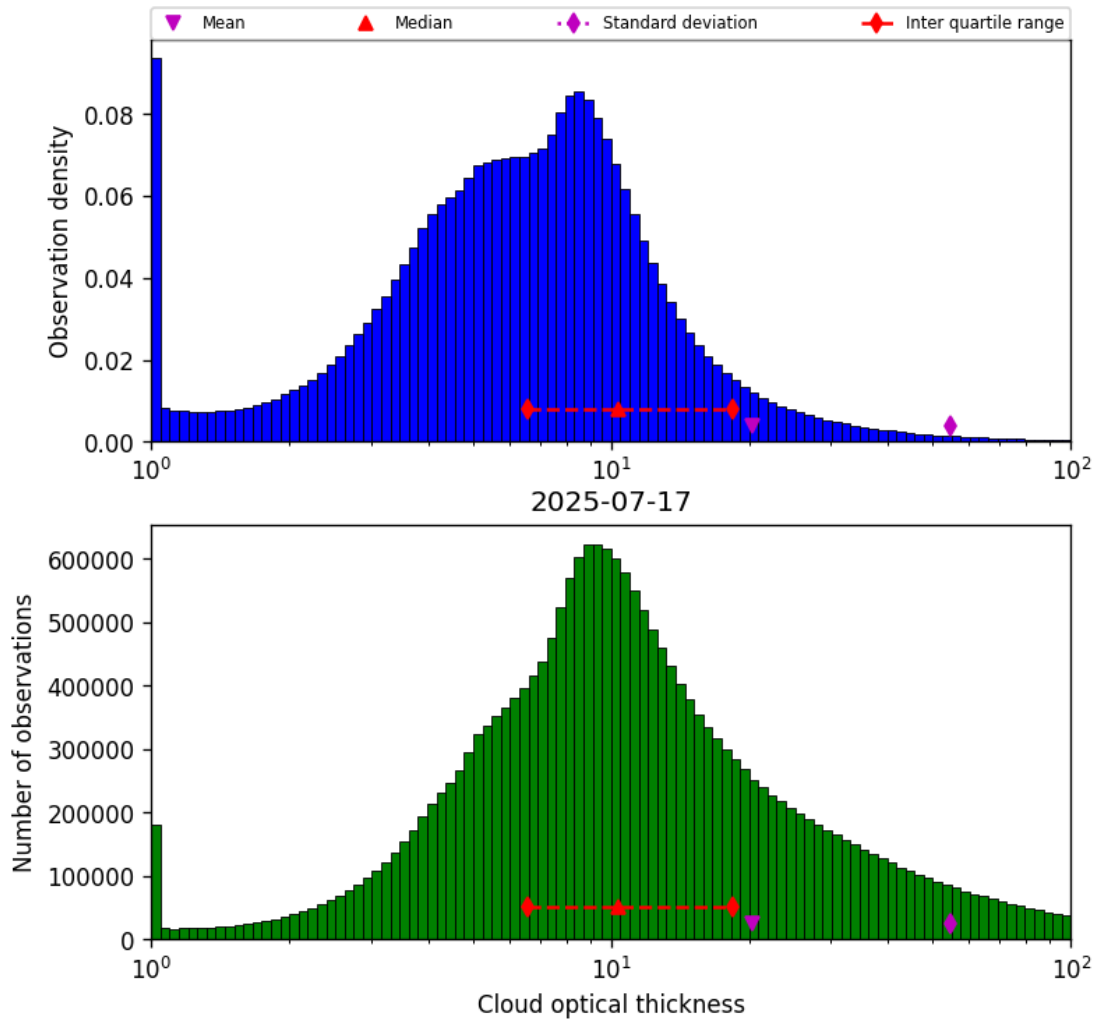
Figure 41: Histogram of “Cloud optical thickness” for 2025-07-16 to 2025-07-18
