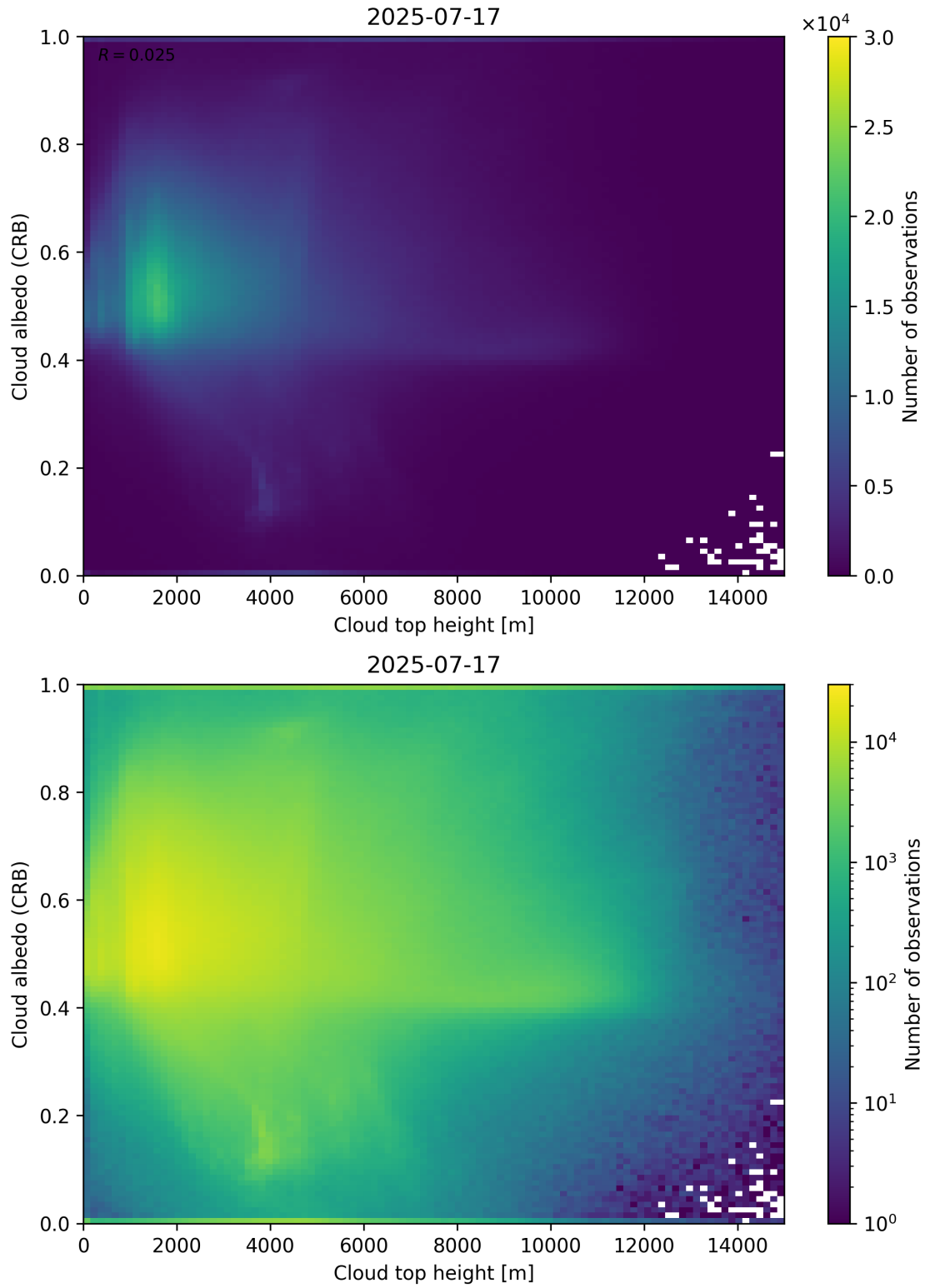
Figure 86: Scatter density plot of “Cloud top height” against “Cloud albedo (CRB)” for 2025-07-16 to 2025-07-18.
