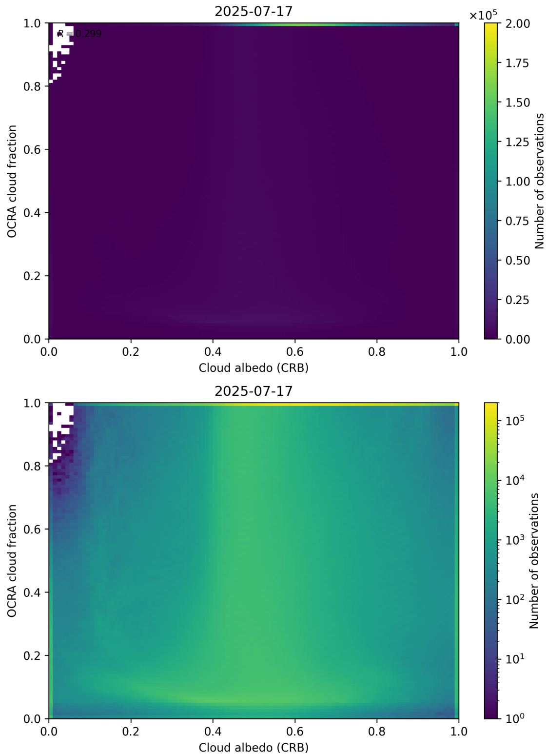
Figure 70: Scatter density plot of “Cloud albedo (CRB)” against “OCRA cloud fraction” for 2025-07-16 to 2025-07-18.
