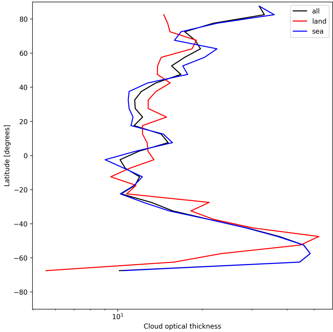
Figure 25: Zonal average of “Cloud optical thickness” for 2025-07-16 to 2025-07-18.
