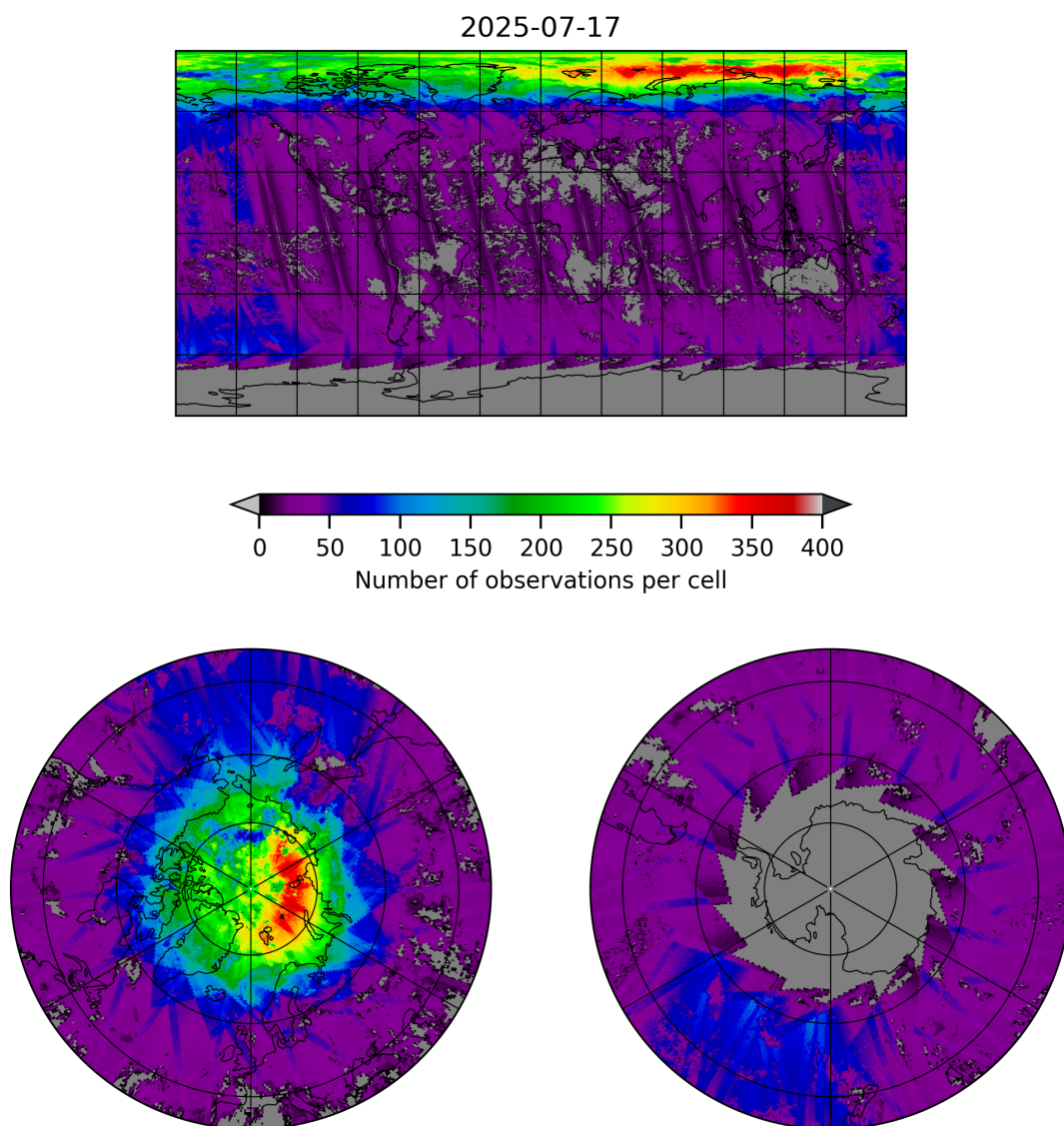
Figure 21: Map of the number of observations for 2025-07-16 to 2025-07-18
