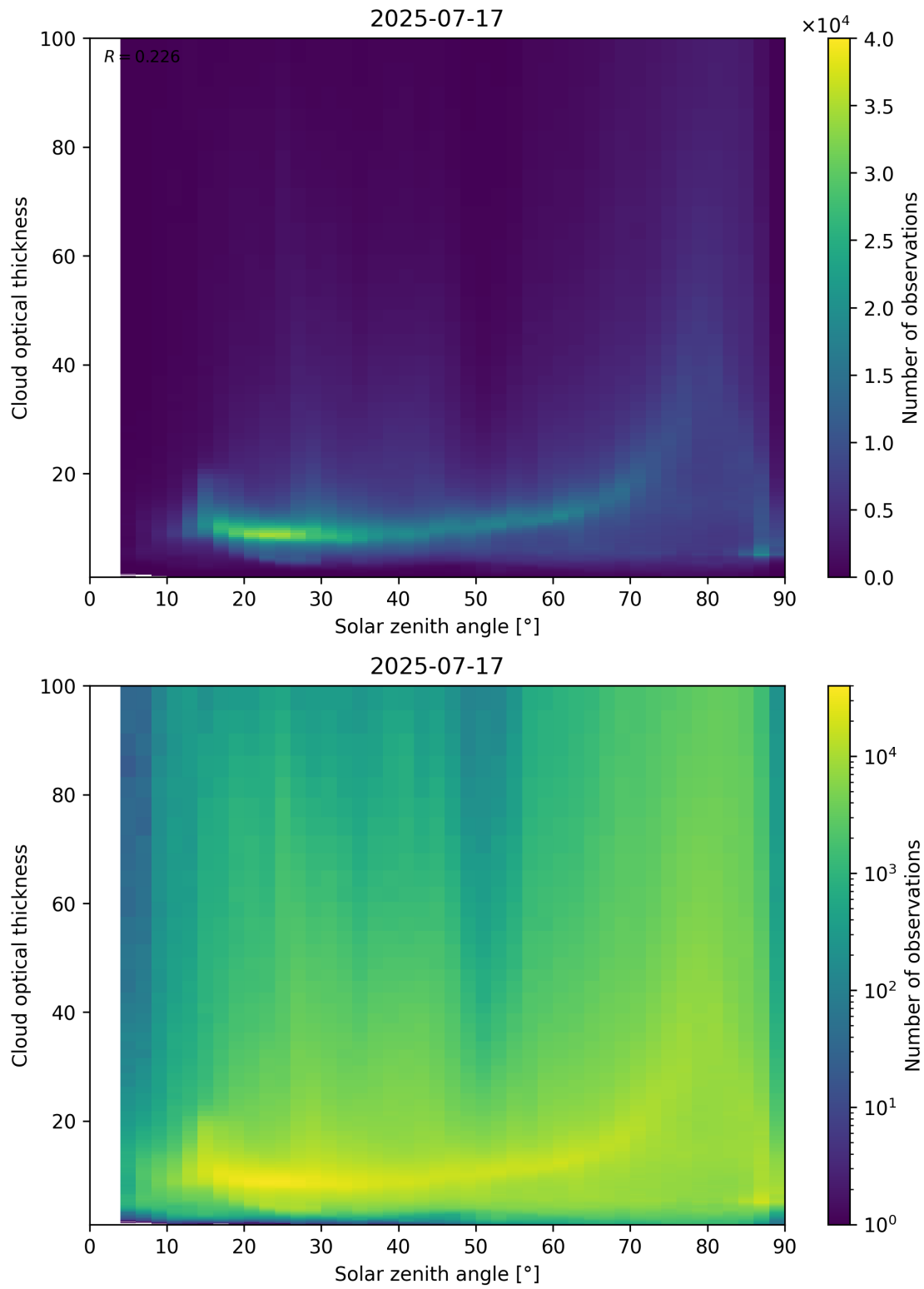
Figure 103: Scatter density plot of “Solar zenith angle” against “Cloud optical thickness” for 2025-07-16 to 2025-07-18.
