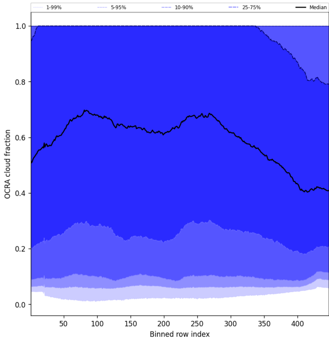
Figure 66: Along track statistics of “OCRA cloud fraction” for 2025-07-16 to 2025-07-18
