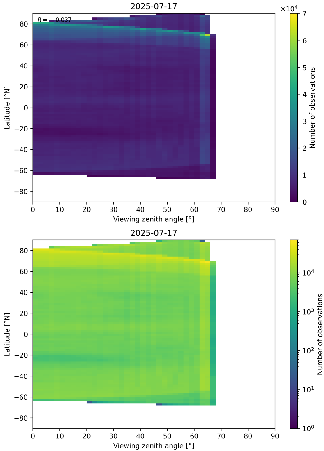
Figure 113: Scatter density plot of “Viewing zenith angle” against “Latitude” for 2025-07-16 to 2025-07-18.
