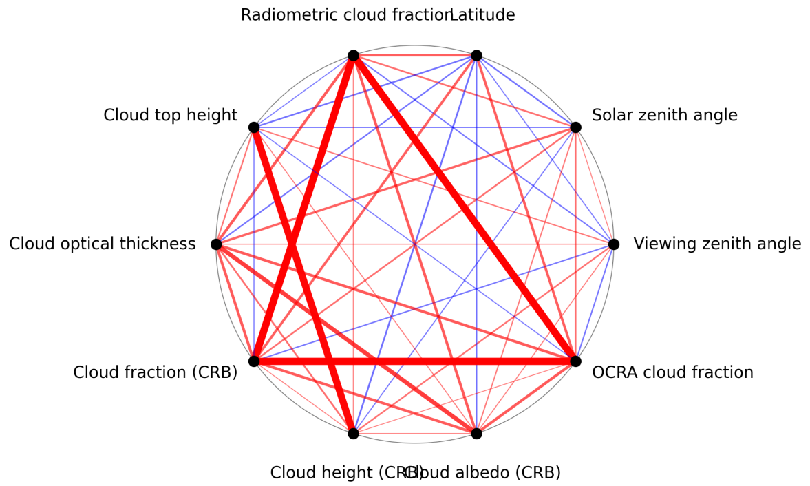
Figure 1: Map of correlation graph for 2025-07-16 to 2025-07-18.
