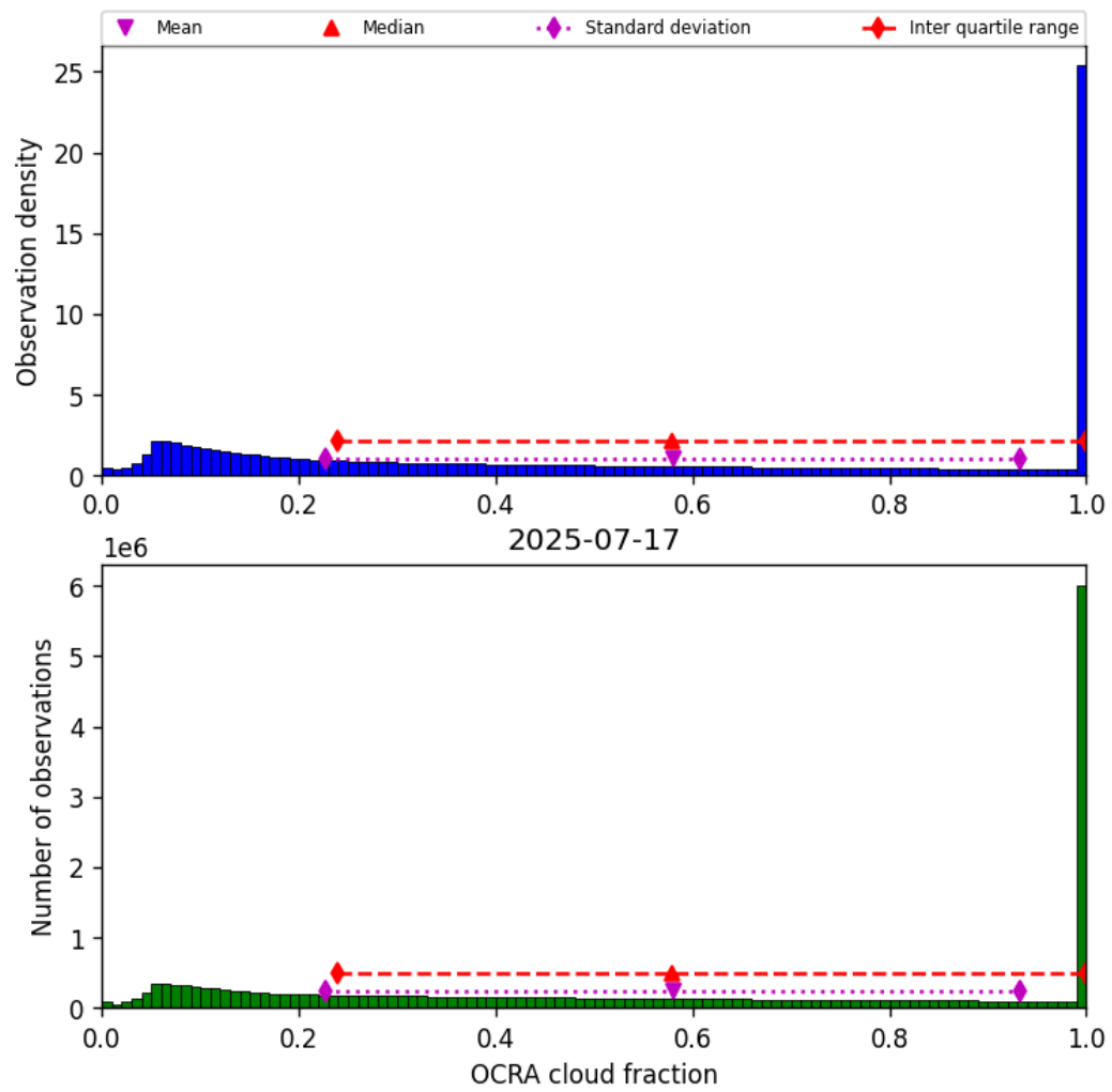
Figure 50: Histogram of “OCRA cloud fraction” for 2025-07-16 to 2025-07-18
