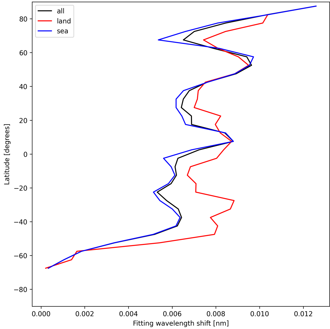
Figure 33: Zonal average of “Fitting wavelength shift” for 2025-07-16 to 2025-07-18.
