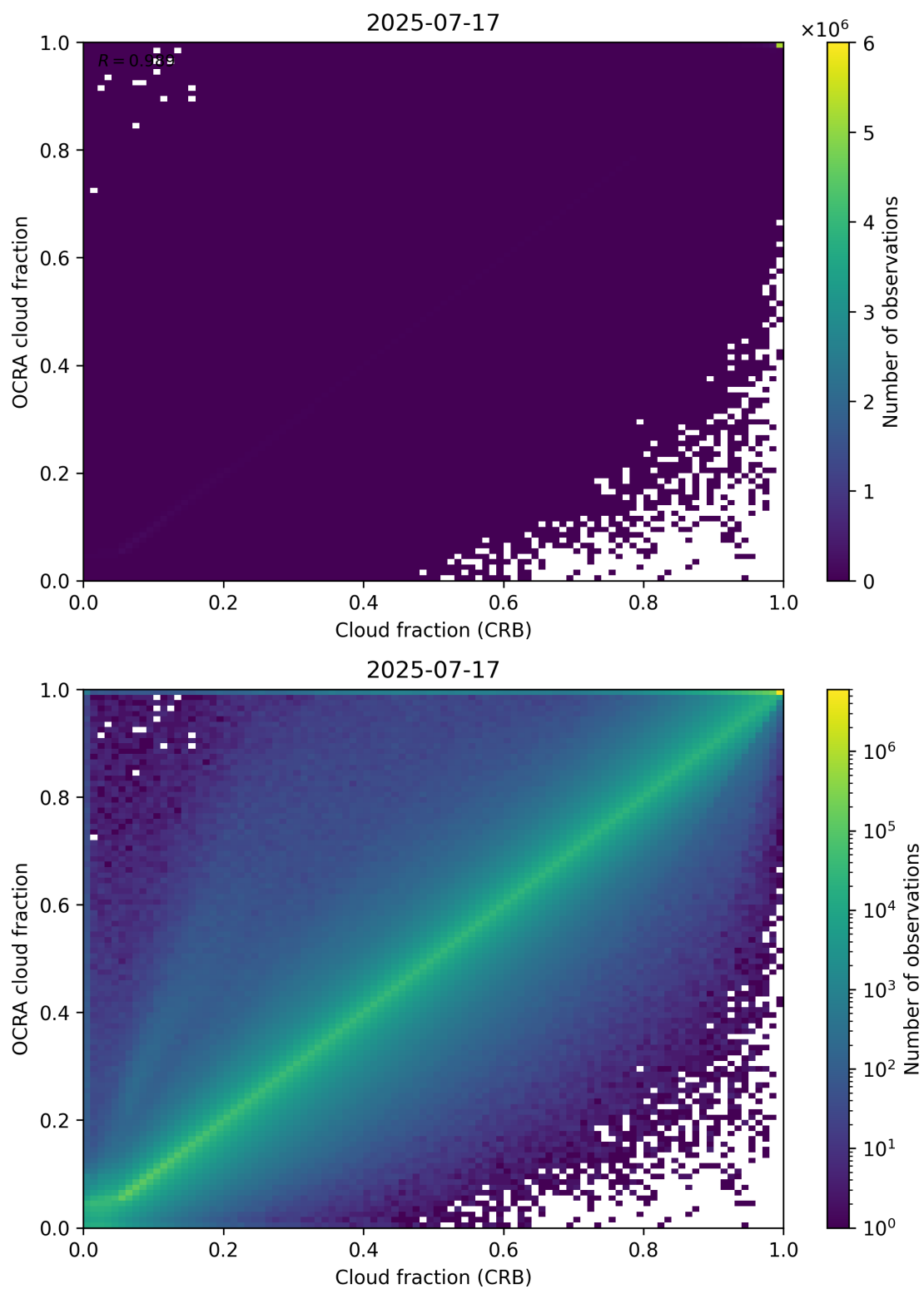
Figure 78: Scatter density plot of “Cloud fraction (CRB)” against “OCRA cloud fraction” for 2025-07-16 to 2025-07-18.
