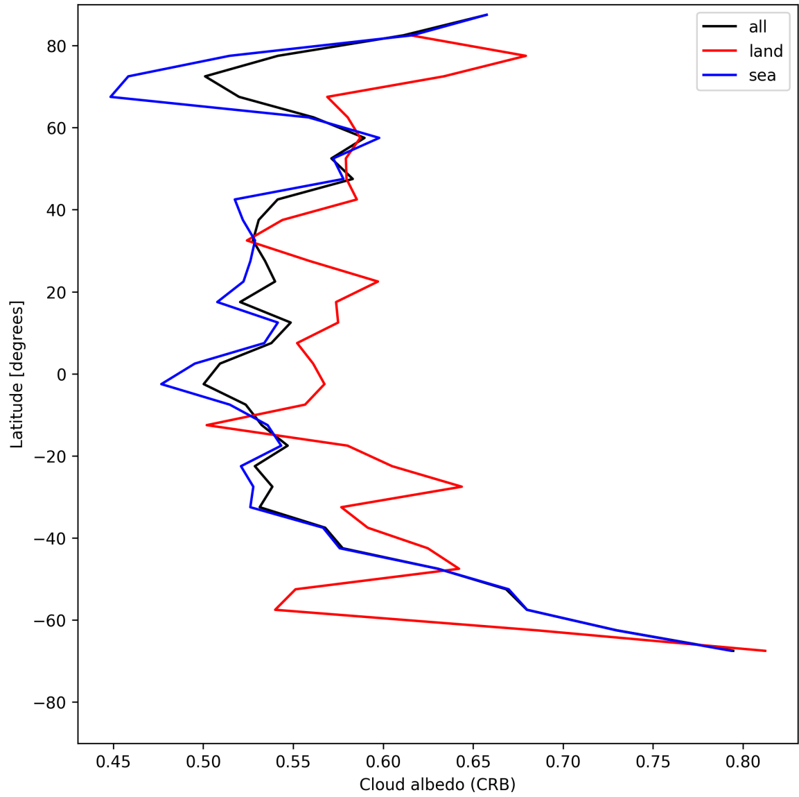
Figure 28: Zonal average of “Cloud albedo (CRB)” for 2025-07-16 to 2025-07-18.
