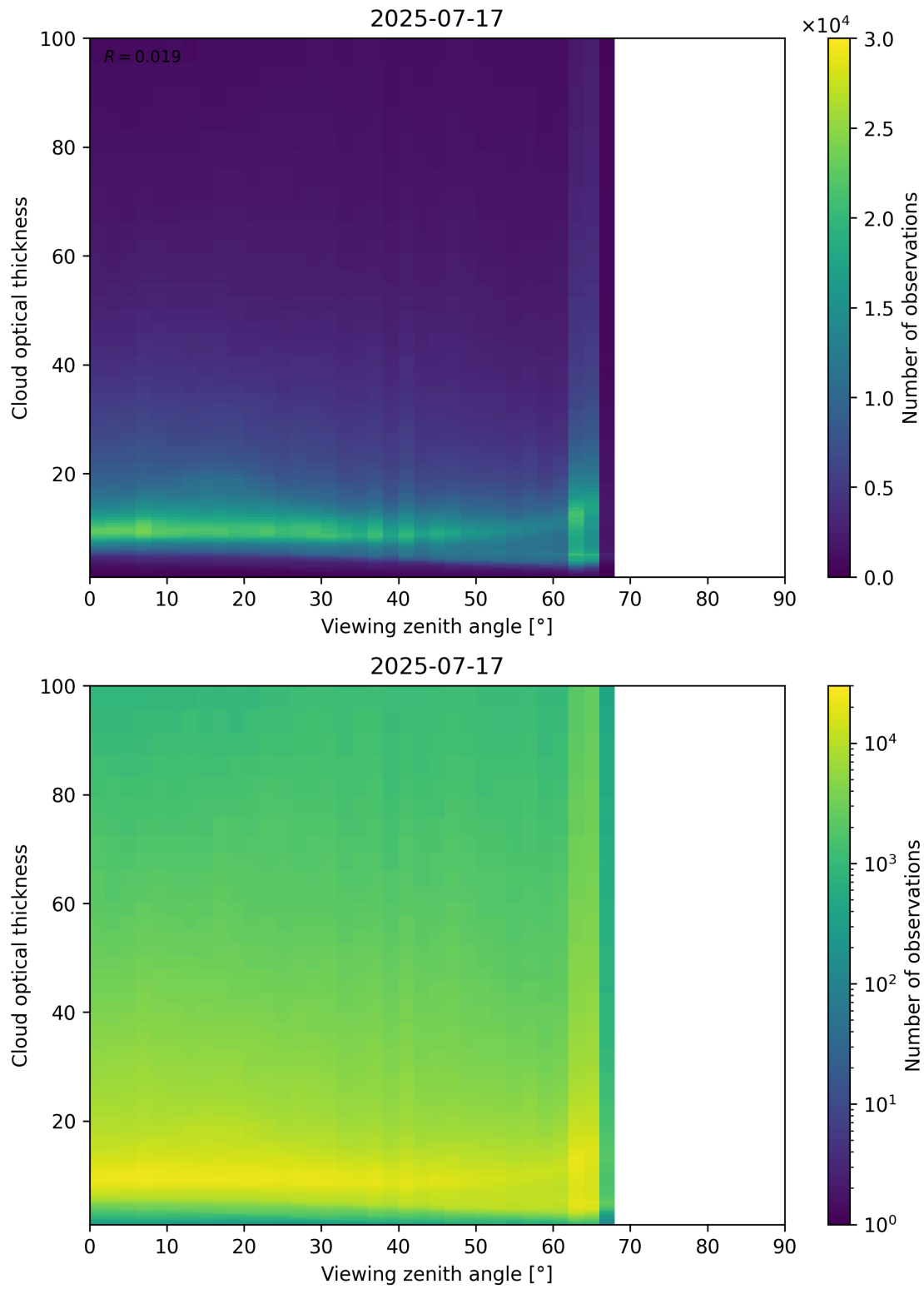
Figure 111: Scatter density plot of “Viewing zenith angle” against “Cloud optical thickness” for 2025-07-16 to 2025-07-18.
