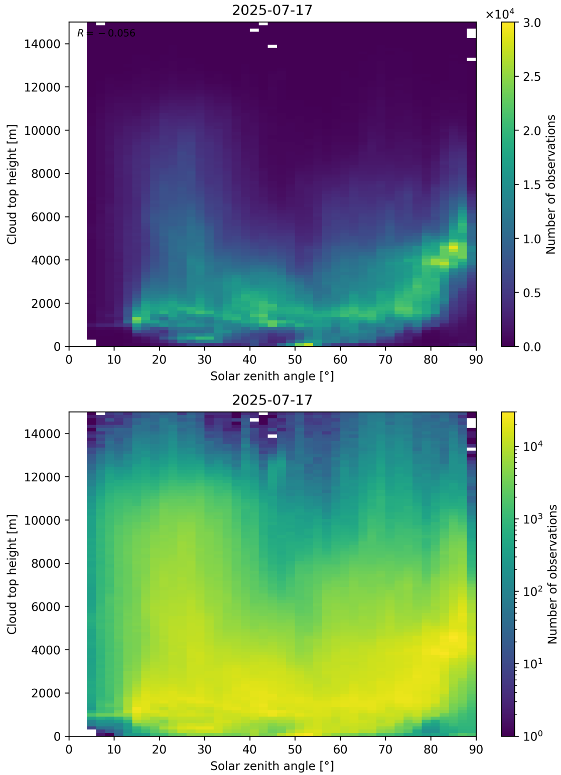
Figure 104: Scatter density plot of “Solar zenith angle” against “Cloud top height” for 2025-07-16 to 2025-07-18.
