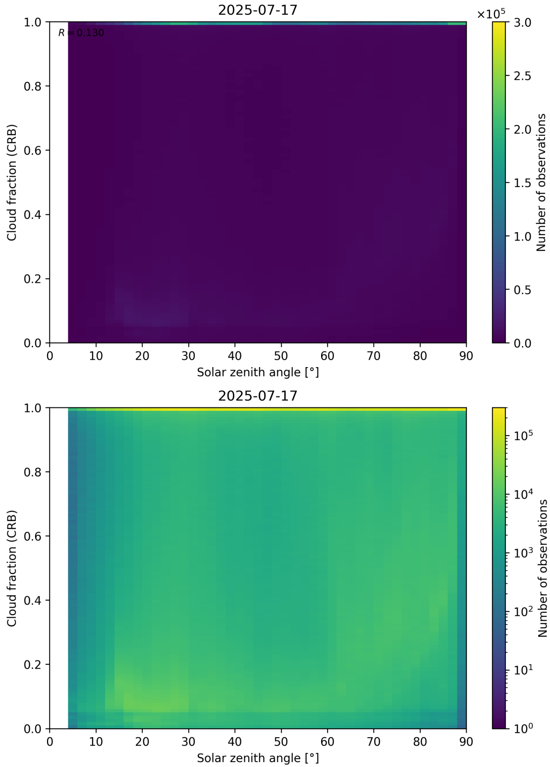
Figure 101: Scatter density plot of “Solar zenith angle” against “Cloud fraction (CRB)” for 2025-07-16 to 2025-07-18.
