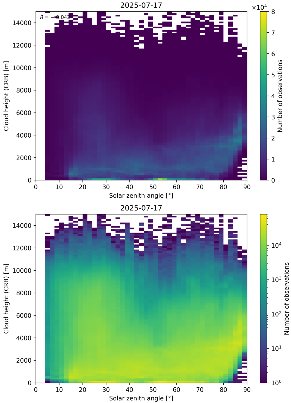
Figure 102: Scatter density plot of “Solar zenith angle” against “Cloud height (CRB)” for 2025-07-16 to 2025-07-18.
