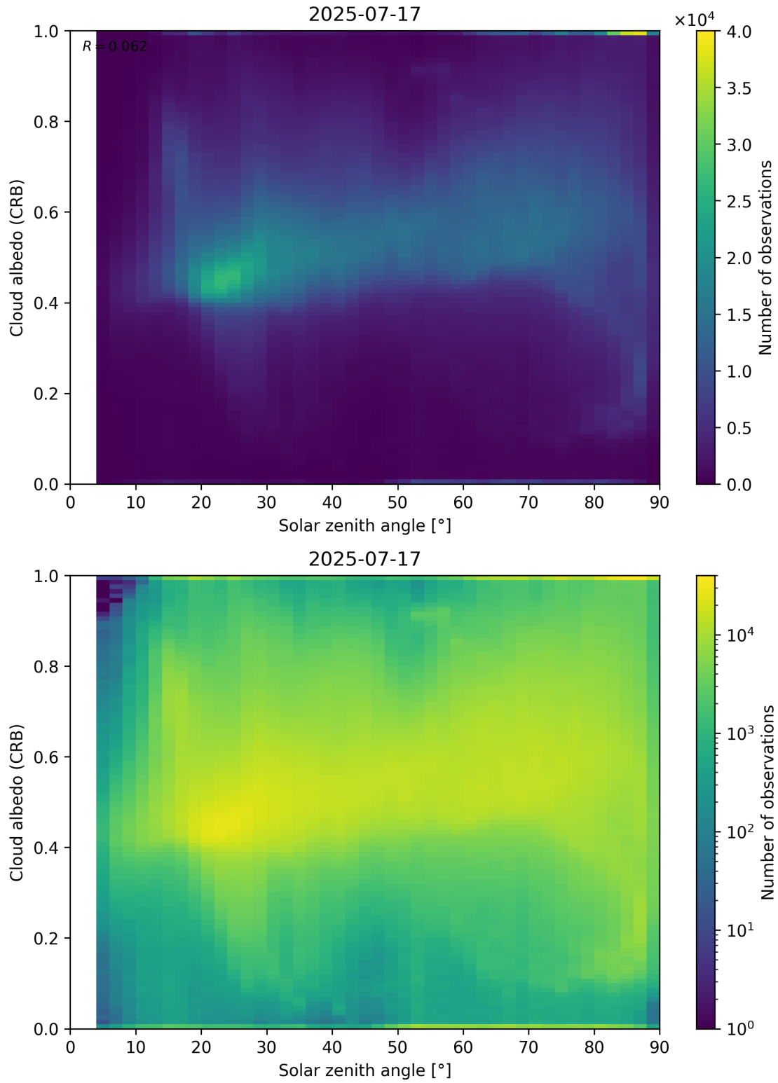
Figure 98: Scatter density plot of “Solar zenith angle” against “Cloud albedo (CRB)” for 2025-07-16 to 2025-07-18.
