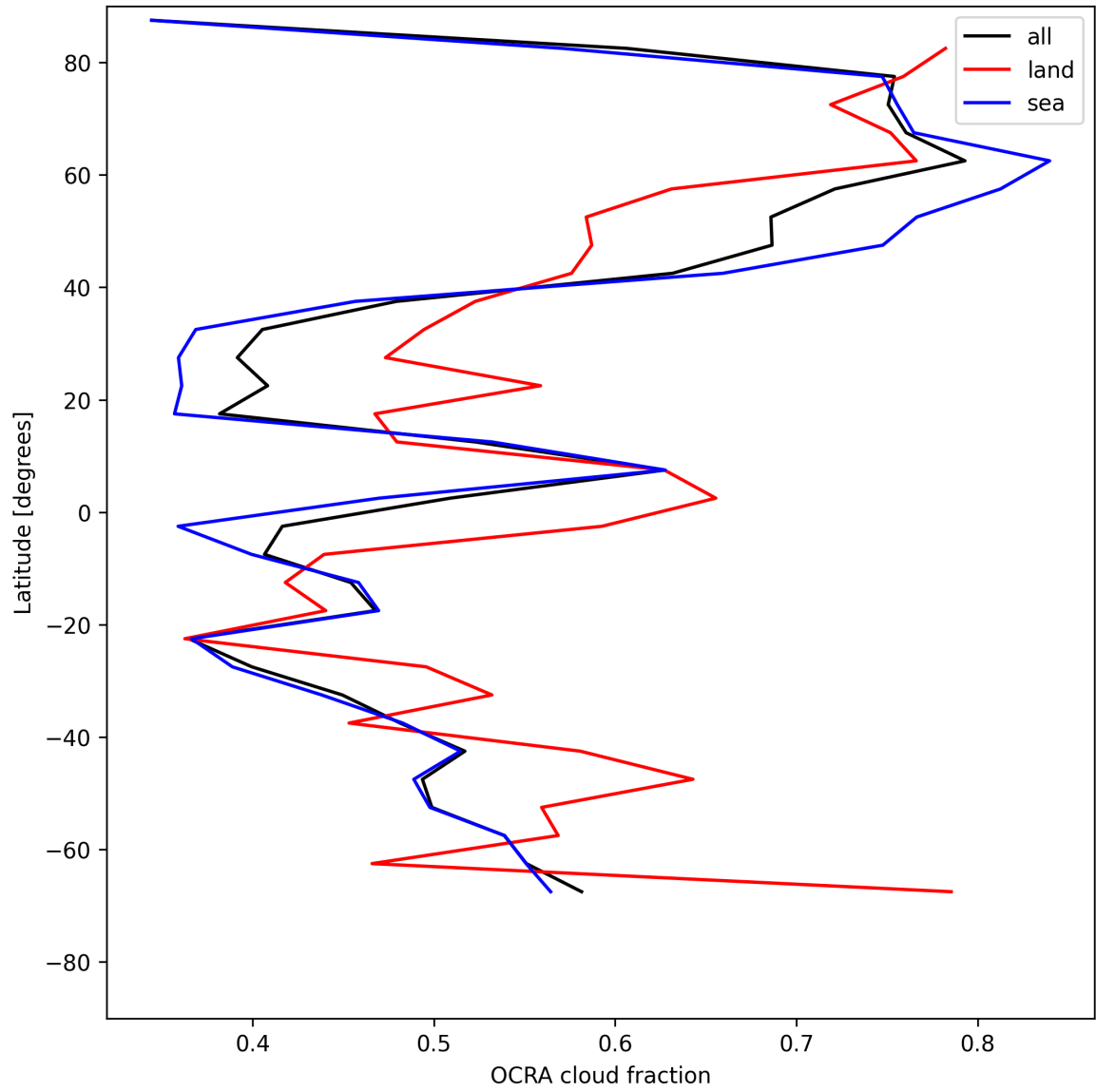
Figure 34: Zonal average of “OCRA cloud fraction” for 2025-07-16 to 2025-07-18.
