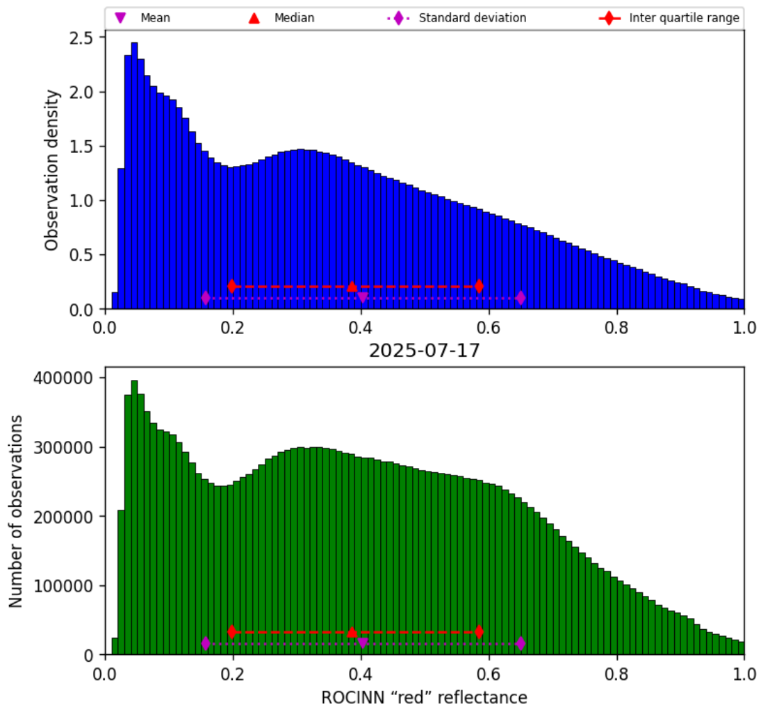
Figure 53: Histogram of “ROCINN “red” reflectance” for 2025-07-16 to 2025-07-18
