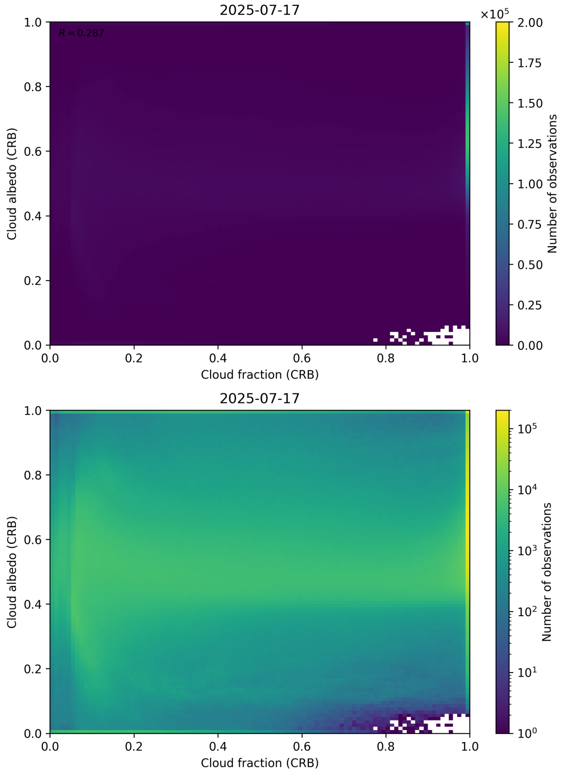
Figure 77: Scatter density plot of “Cloud fraction (CRB)” against “Cloud albedo (CRB)” for 2025-07-16 to 2025-07-18.
