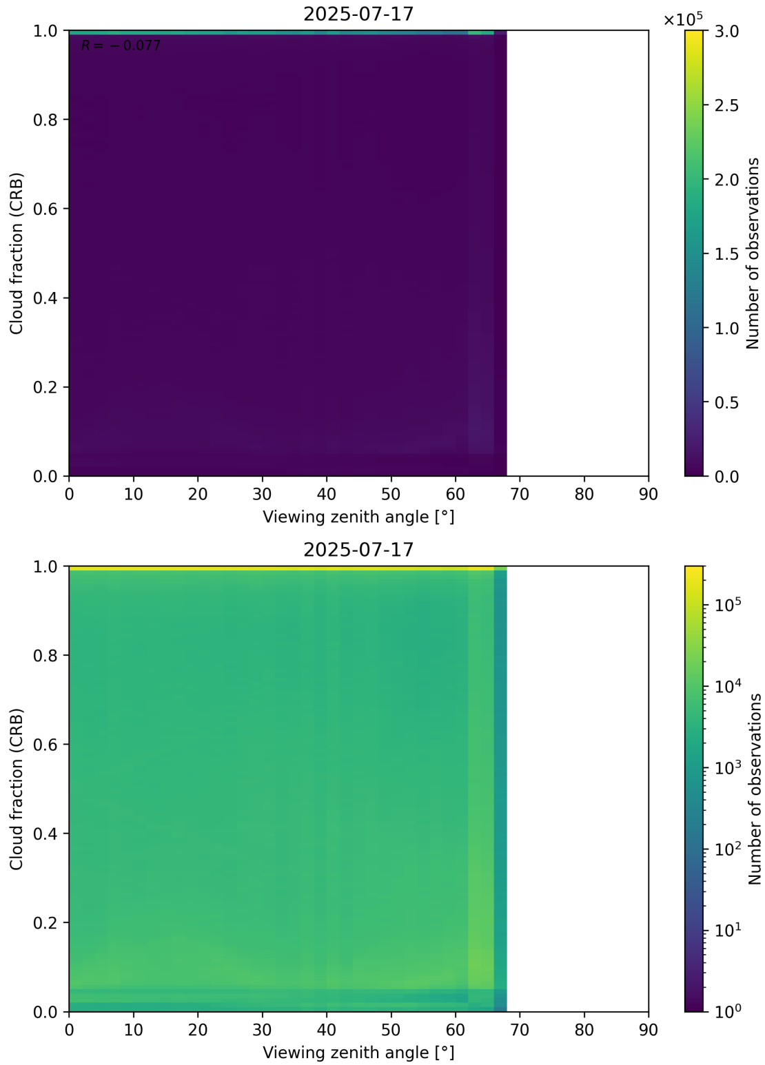
Figure 109: Scatter density plot of “Viewing zenith angle” against “Cloud fraction (CRB)” for 2025-07-16 to 2025-07-18.
