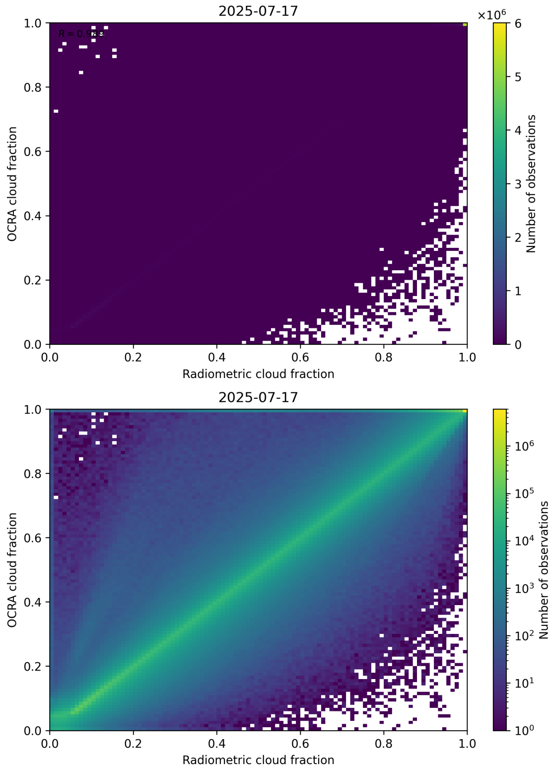
Figure 72: Scatter density plot of “Radiometric cloud fraction” against “OCRA cloud fraction” for 2025-07-16 to 2025-07-18.
