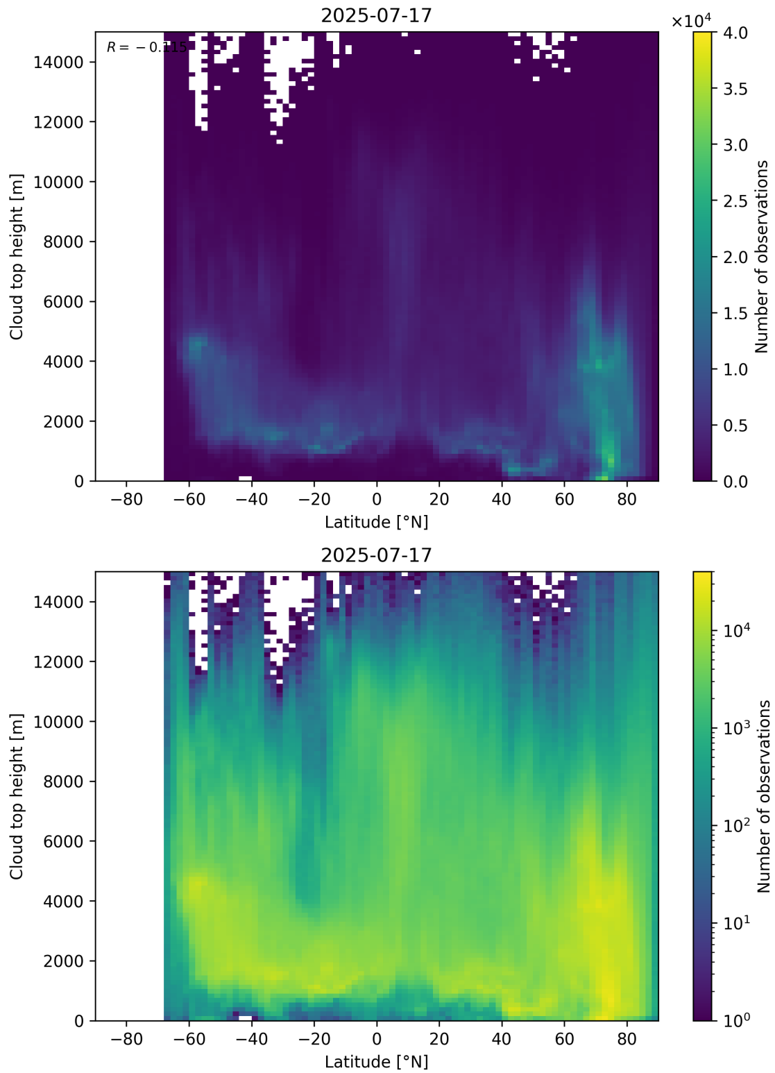
Figure 97: Scatter density plot of “Latitude” against “Cloud top height” for 2025-07-16 to 2025-07-18.
