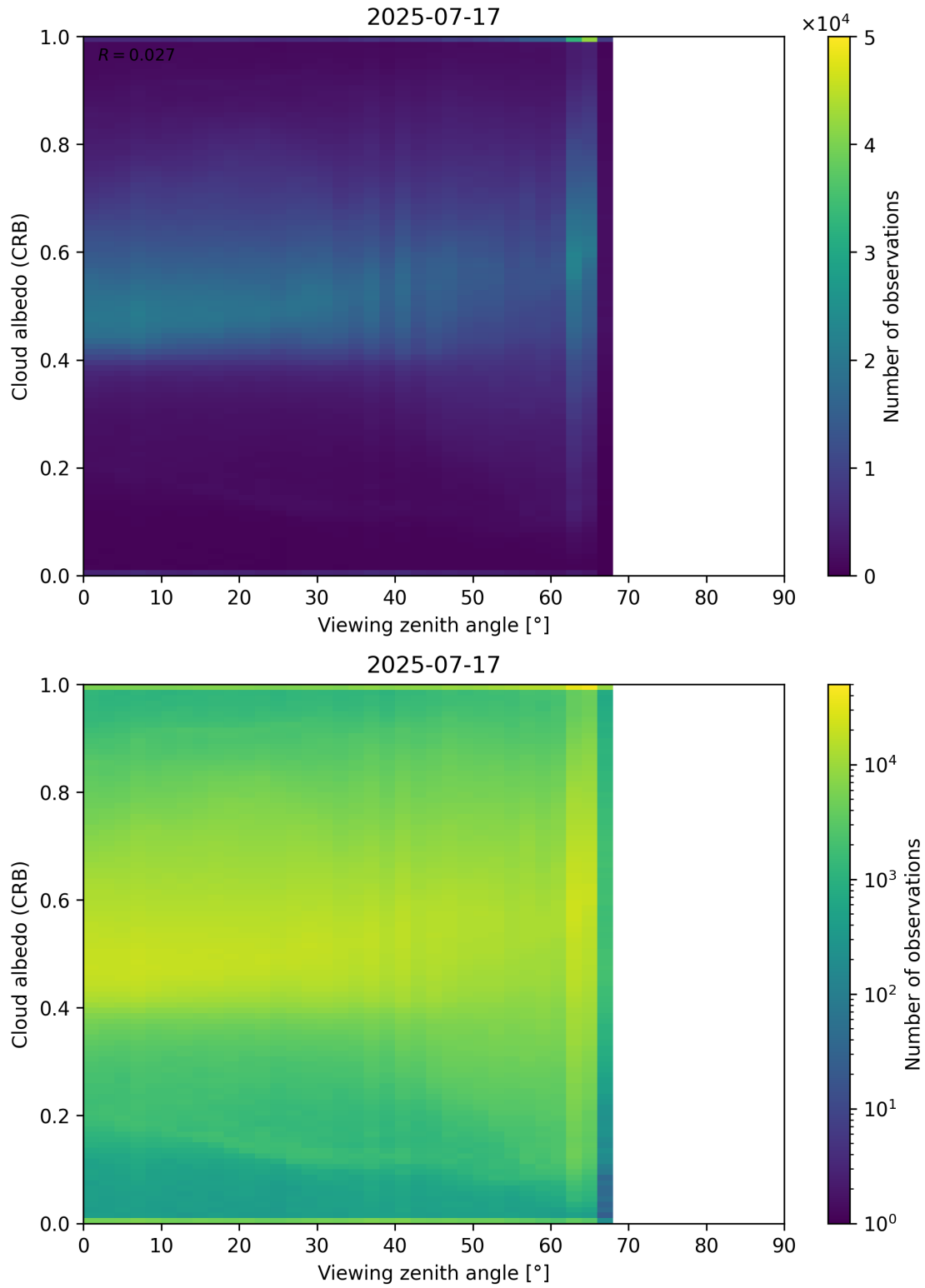
Figure 106: Scatter density plot of “Viewing zenith angle” against “Cloud albedo (CRB)” for 2025-07-16 to 2025-07-18.
