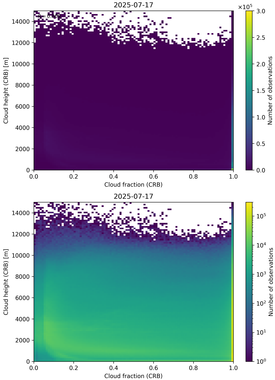
Figure 79: Scatter density plot of “Cloud fraction (CRB)” against “Cloud height (CRB)” for 2025-07-16 to 2025-07-18.
