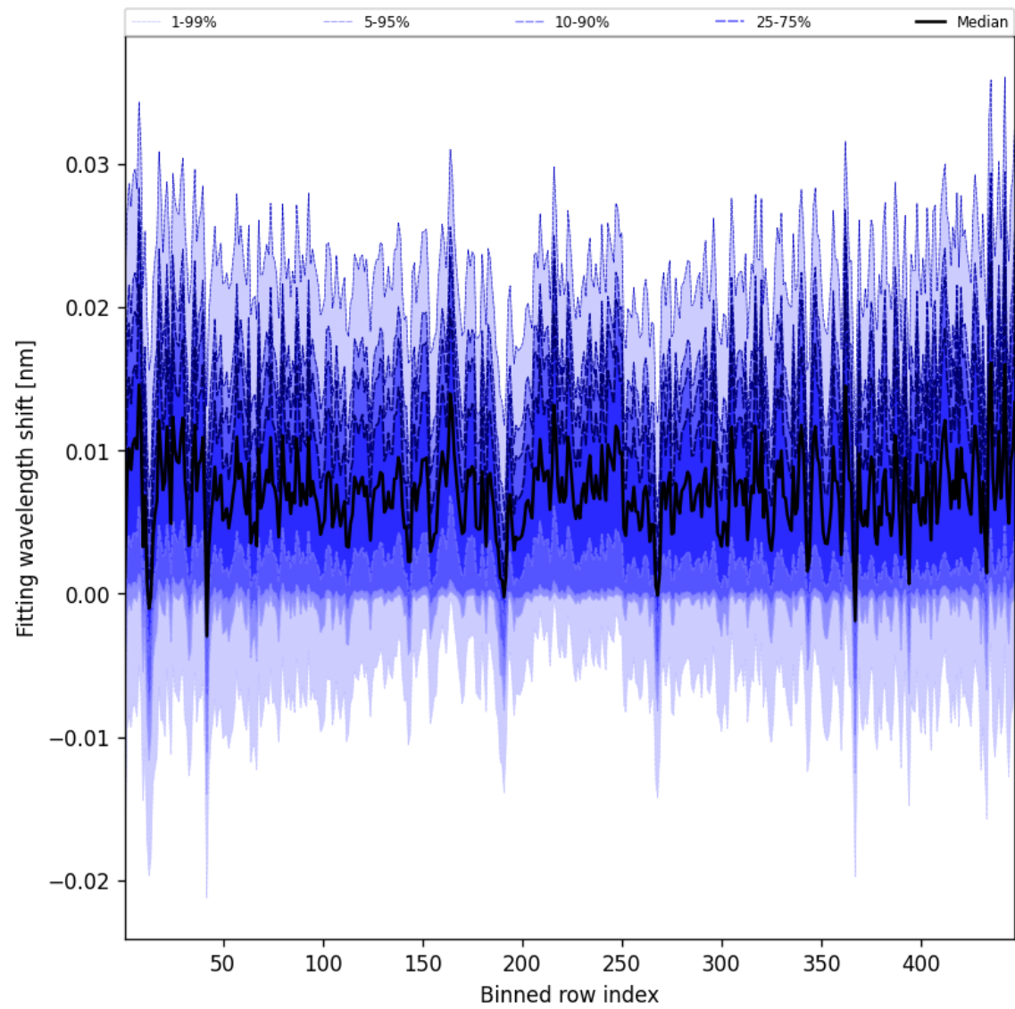
Figure 65: Along track statistics of “Fitting wavelength shift” for 2025-07-16 to 2025-07-18
