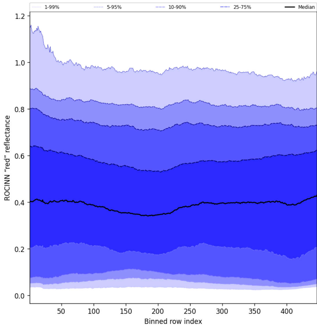
Figure 69: Along track statistics of "ROCINN "red" reflectance" for 2025-07-16 to 2025-07-18
