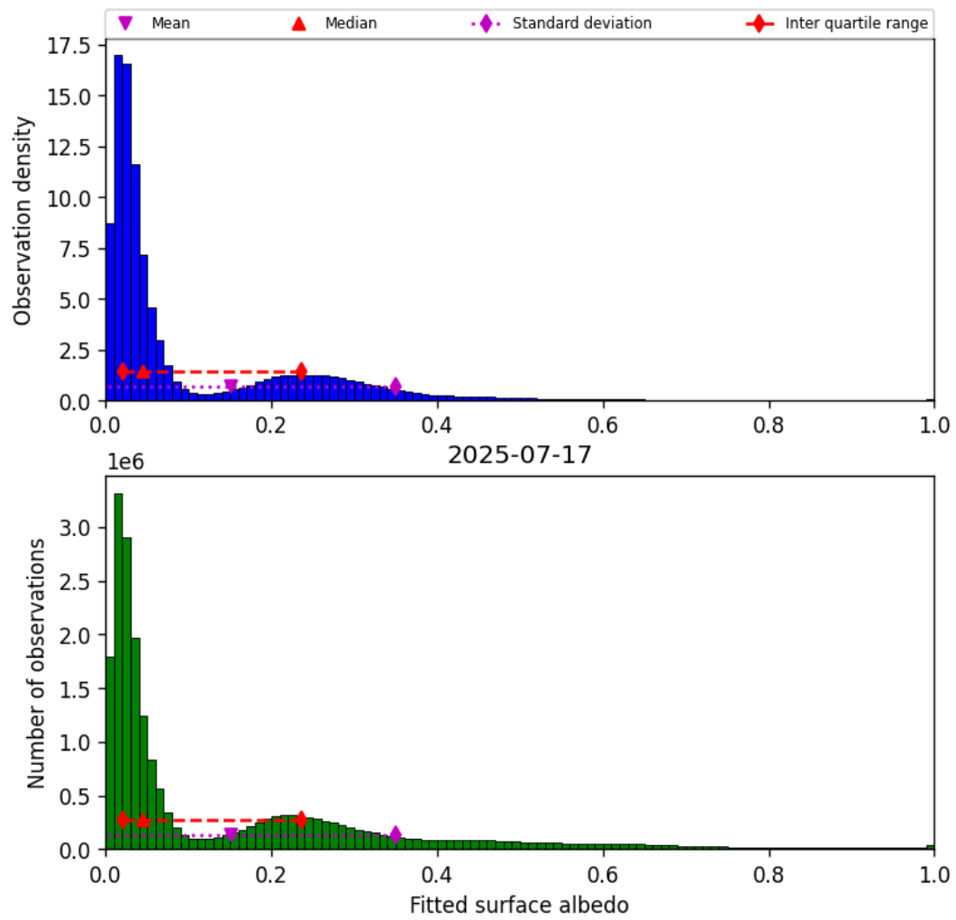
Figure 45: Histogram of “Fitted surface albedo” for 2025-07-16 to 2025-07-18
