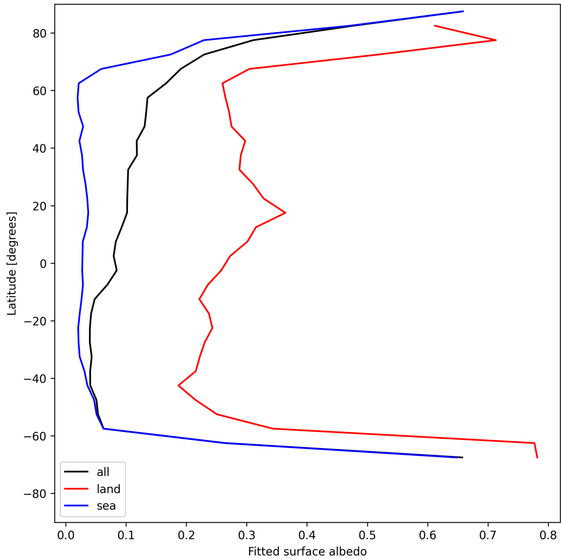
Figure 29: Zonal average of “Fitted surface albedo” for 2025-07-16 to 2025-07-18.
