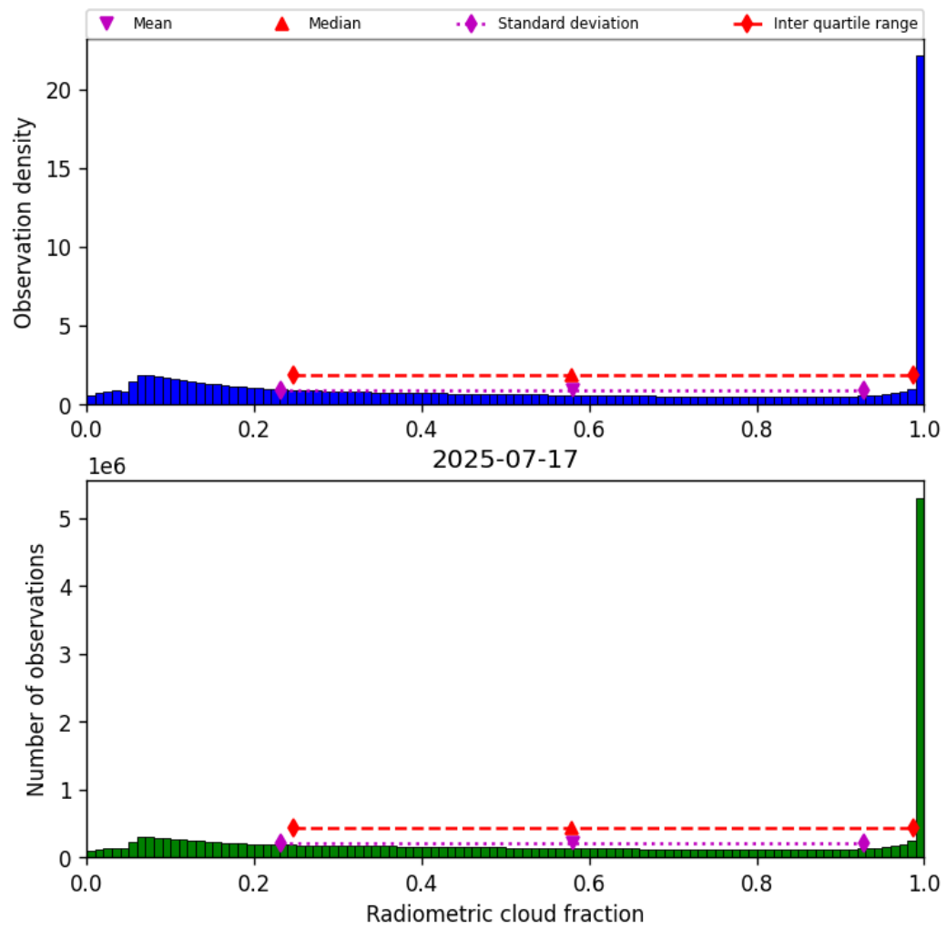
Figure 39: Histogram of “Radiometric cloud fraction” for 2025-07-16 to 2025-07-18
