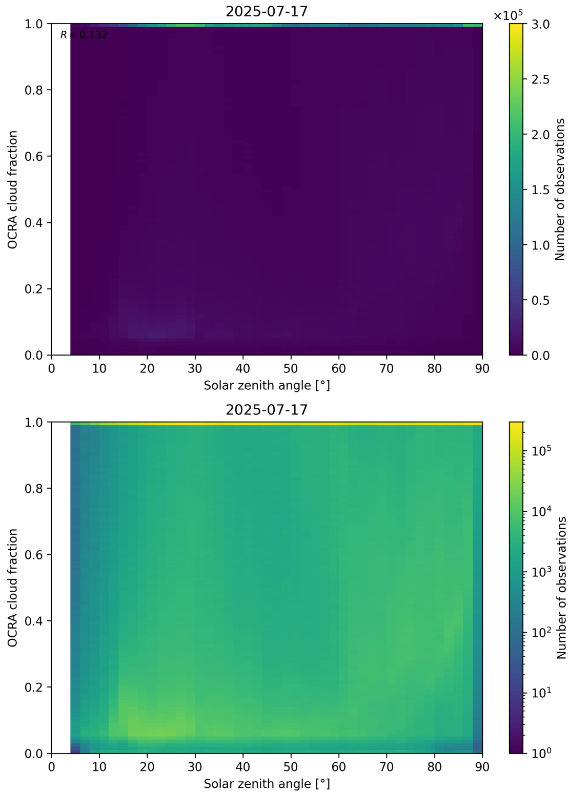
Figure 100: Scatter density plot of “Solar zenith angle” against “OCRA cloud fraction” for 2025-07-16 to 2025-07-18.
