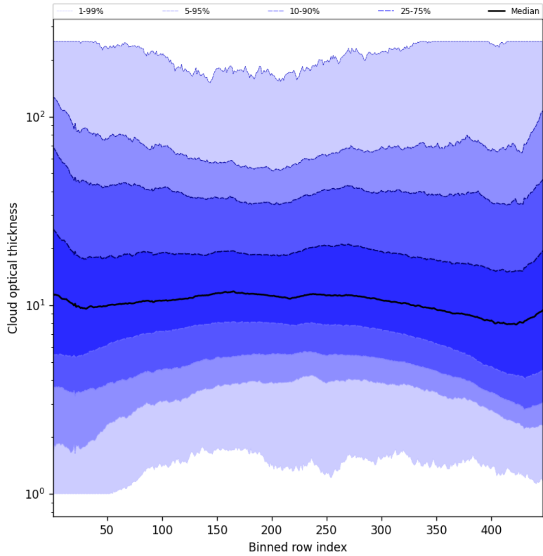
Figure 57: Along track statistics of “Cloud optical thickness” for 2025-07-16 to 2025-07-18
