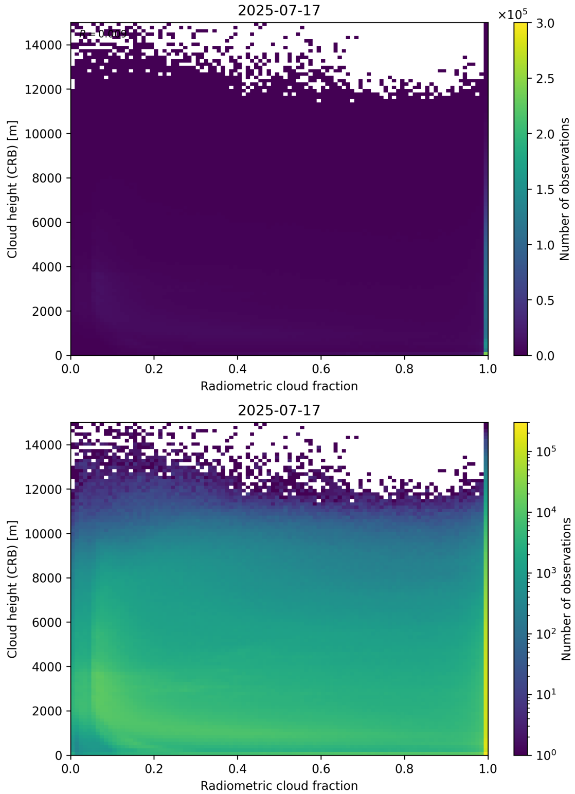
Figure 74: Scatter density plot of “Radiometric cloud fraction” against “Cloud height (CRB)” for 2025-07-16 to 2025-07-18.
