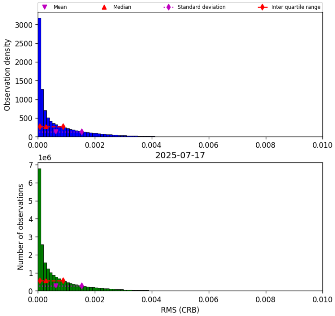
Figure 48: Histogram of “RMS (CRB)” for 2025-07-16 to 2025-07-18
