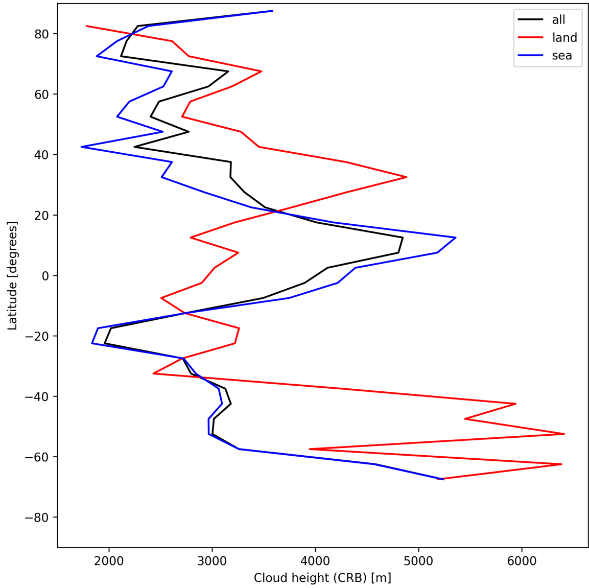
Figure 27: Zonal average of “Cloud height (CRB)” for 2025-07-16 to 2025-07-18.
