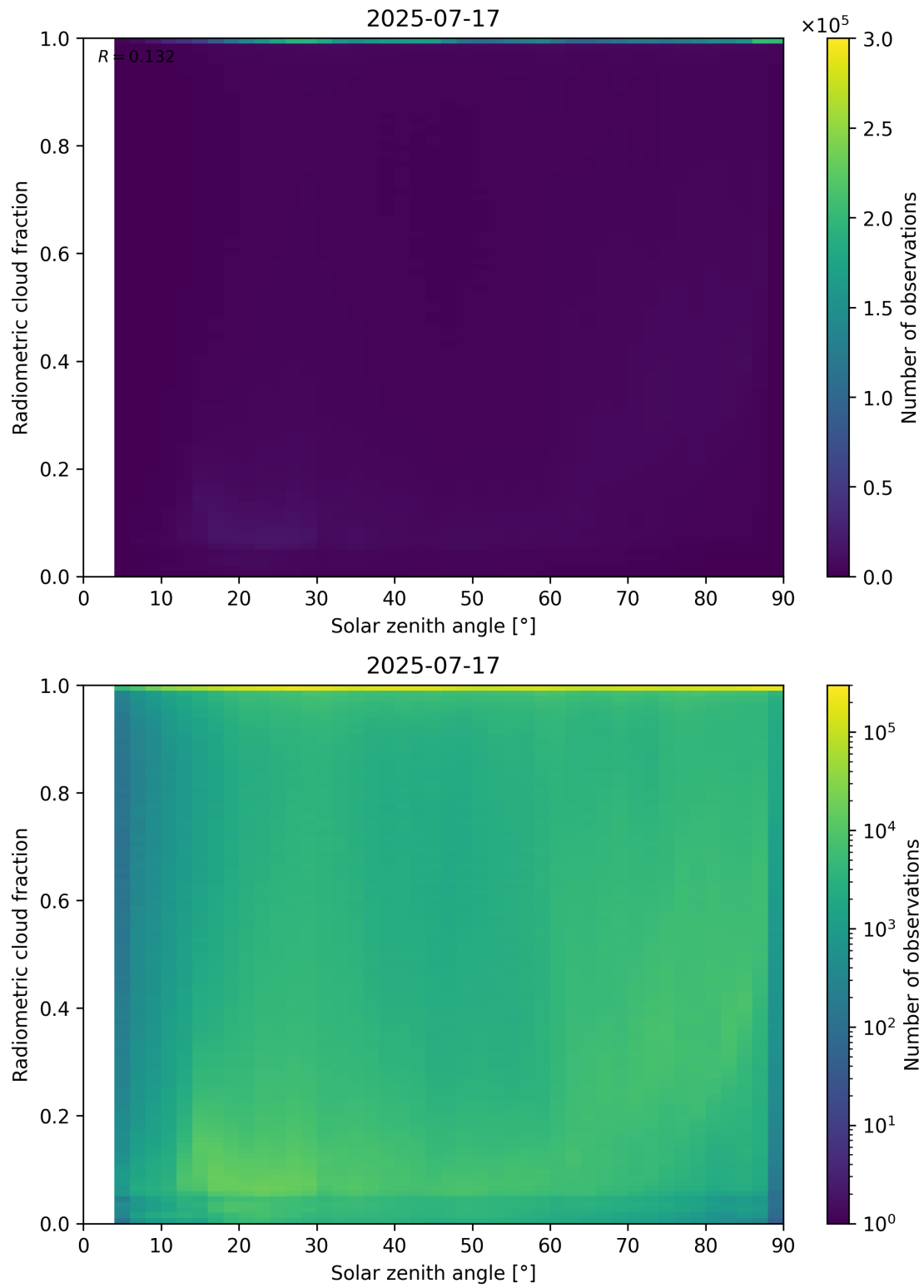
Figure 99: Scatter density plot of “Solar zenith angle” against “Radiometric cloud fraction” for 2025-07-16 to 2025-07-18.
