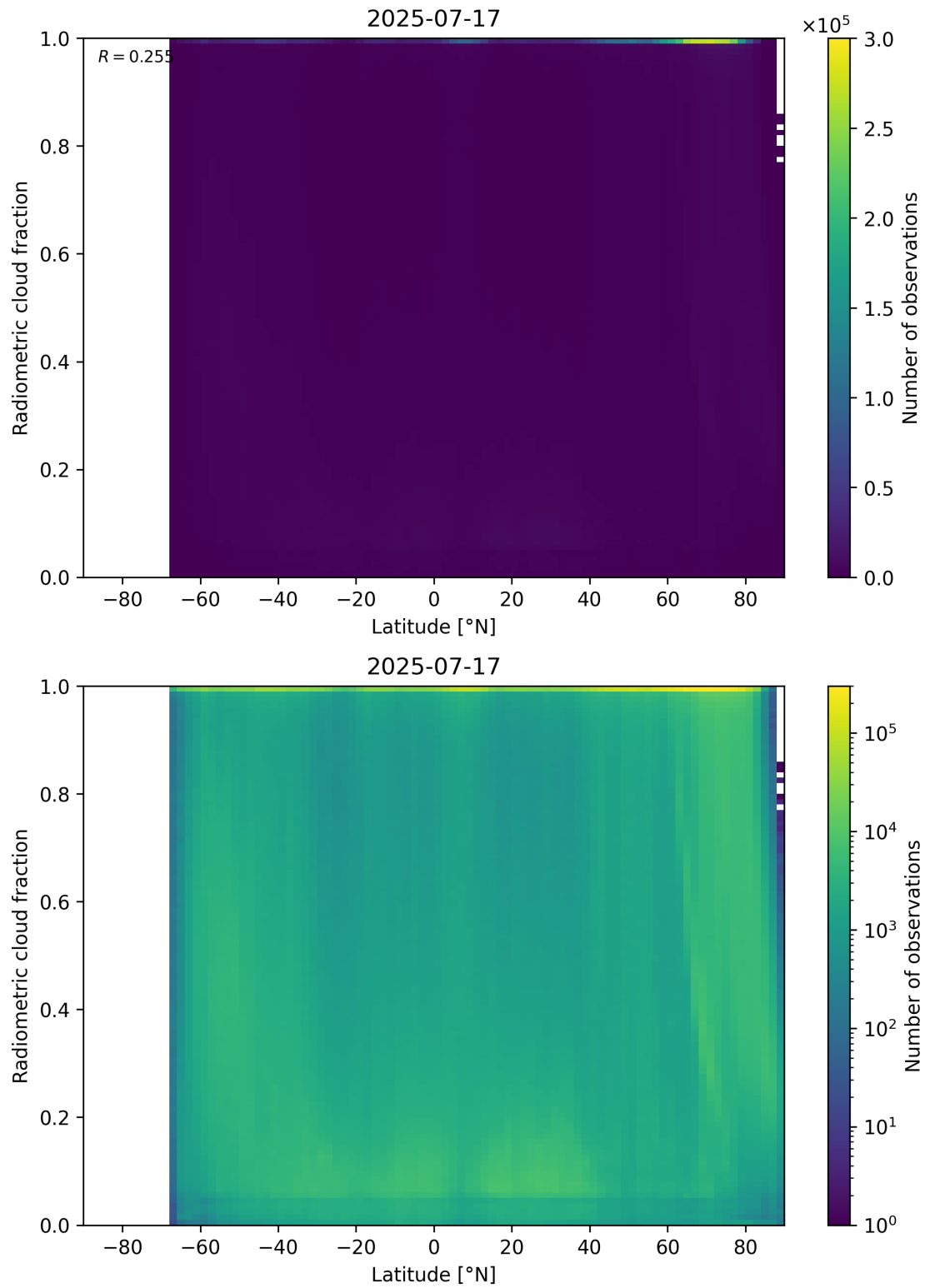
Figure 92: Scatter density plot of “Latitude” against “Radiometric cloud fraction” for 2025-07-16 to 2025-07-18.
