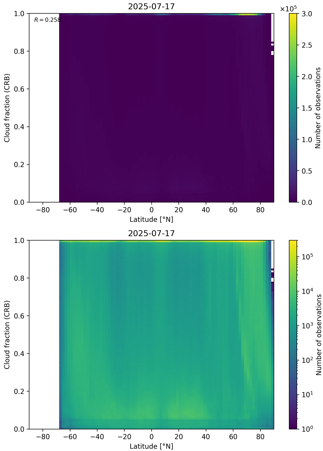
Figure 94: Scatter density plot of “Latitude” against “Cloud fraction (CRB)” for 2025-07-16 to 2025-07-18.
