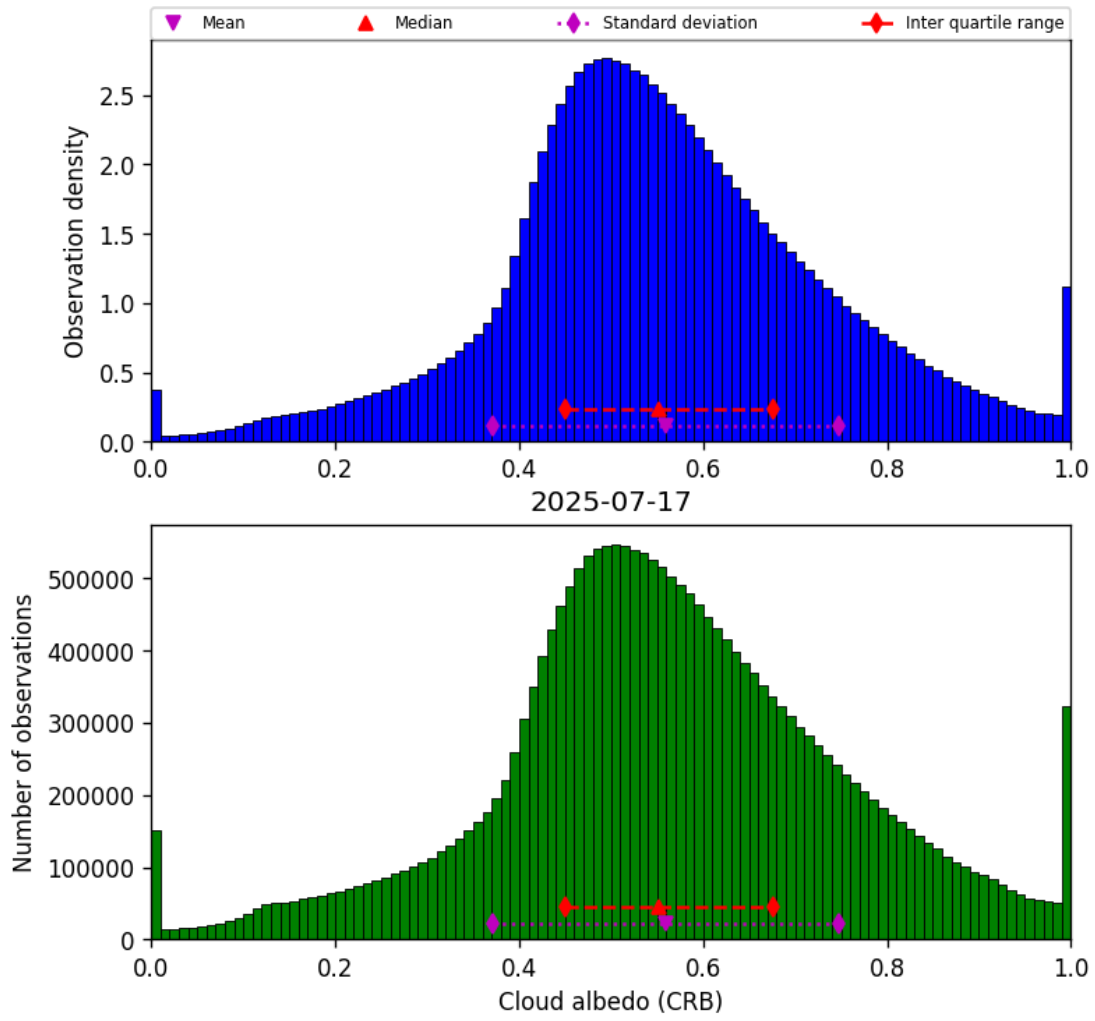
Figure 44: Histogram of “Cloud albedo (CRB)” for 2025-07-16 to 2025-07-18
