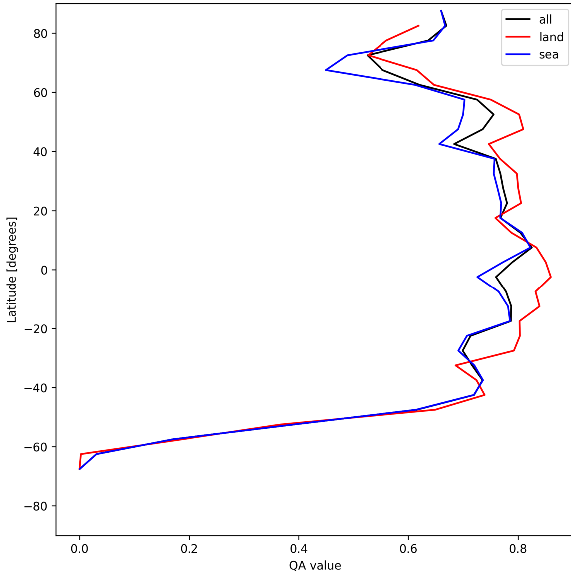
Figure 22: Zonal average of “QA value” for 2025-07-16 to 2025-07-18.
