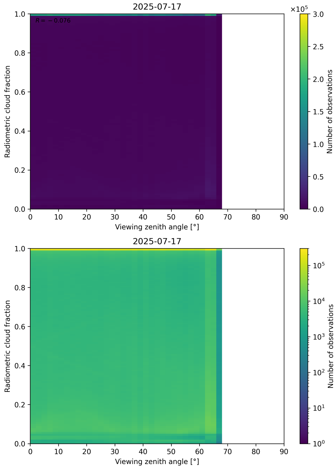
Figure 107: Scatter density plot of “Viewing zenith angle” against “Radiometric cloud fraction” for 2025-07-16 to 2025-07-18.
