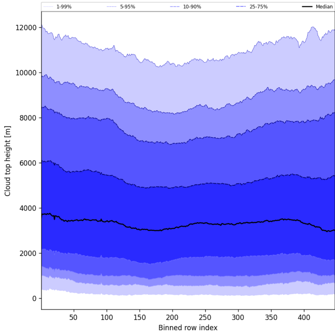
Figure 56: Along track statistics of “Cloud top height” for 2025-07-16 to 2025-07-18
