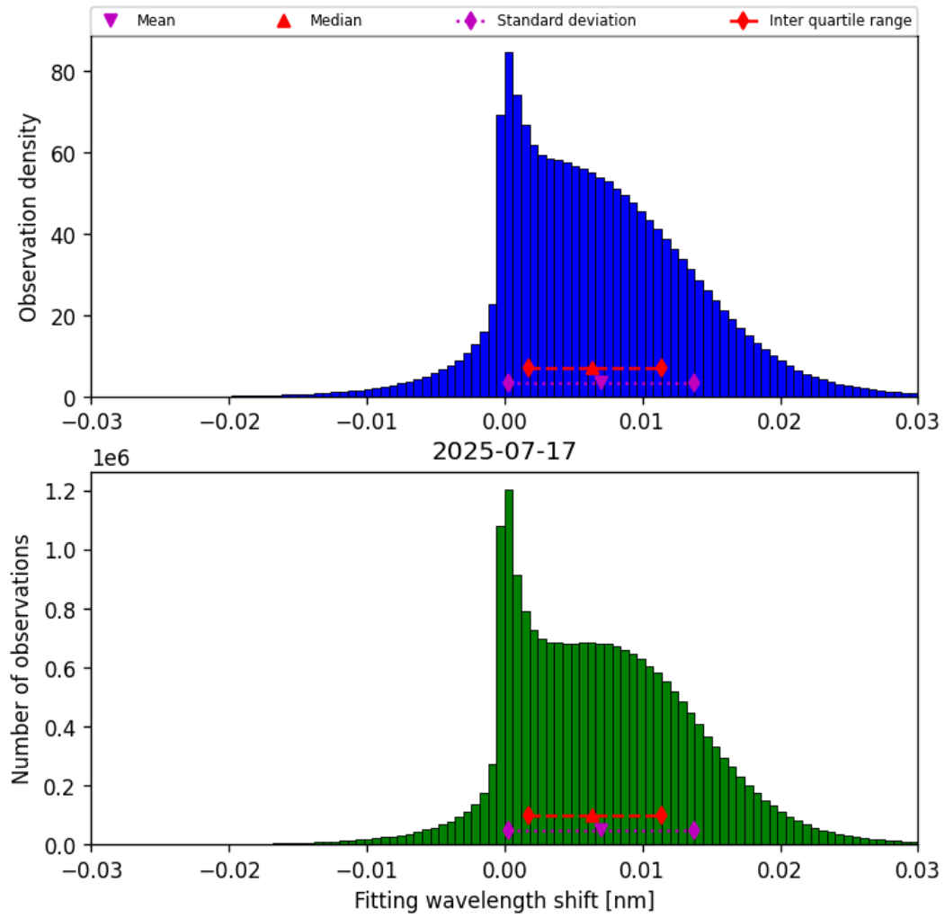
Figure 49: Histogram of “Fitting wavelength shift” for 2025-07-16 to 2025-07-18
