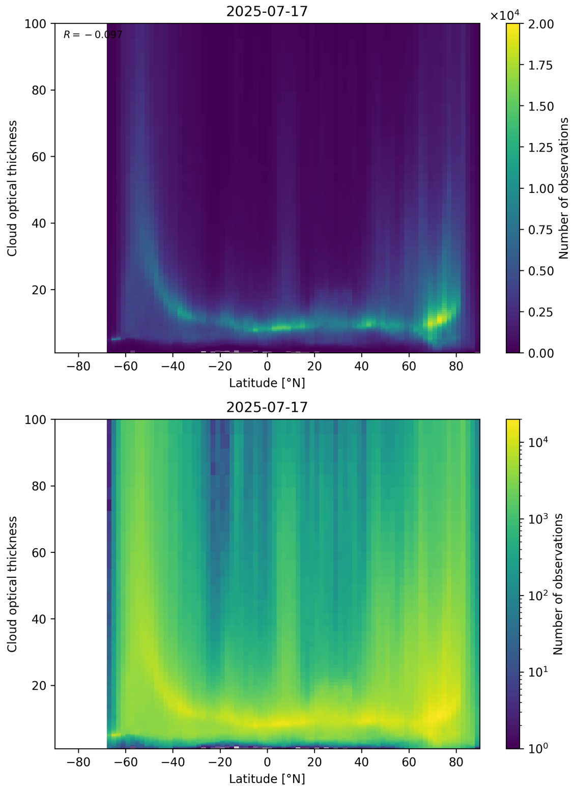
Figure 96: Scatter density plot of “Latitude” against “Cloud optical thickness” for 2025-07-16 to 2025-07-18.
