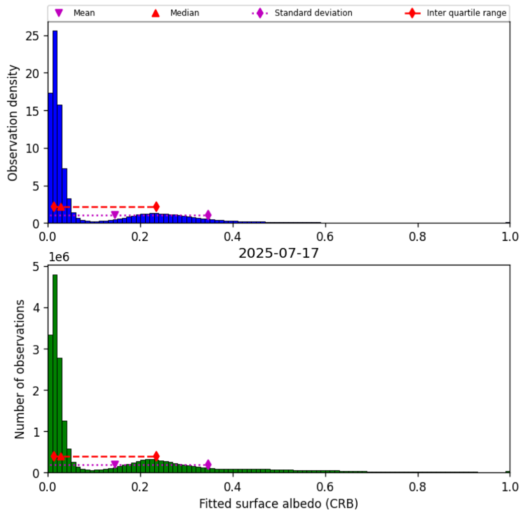
Figure 46: Histogram of “Fitted surface albedo (CRB)” for 2025-07-16 to 2025-07-18
