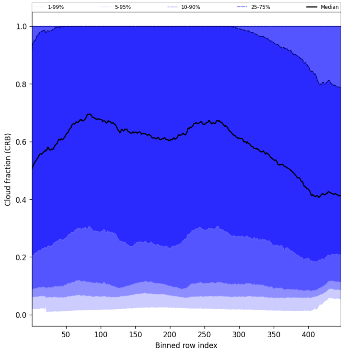
Figure 58: Along track statistics of “Cloud fraction (CRB)” for 2025-07-16 to 2025-07-18
