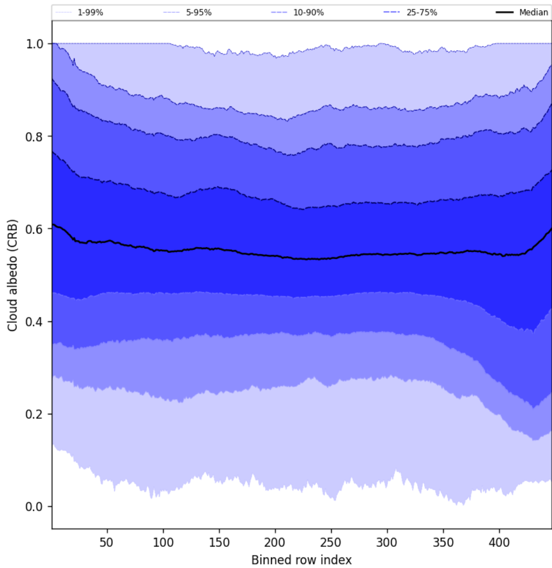
Figure 60: Along track statistics of “Cloud albedo (CRB)” for 2025-07-16 to 2025-07-18
