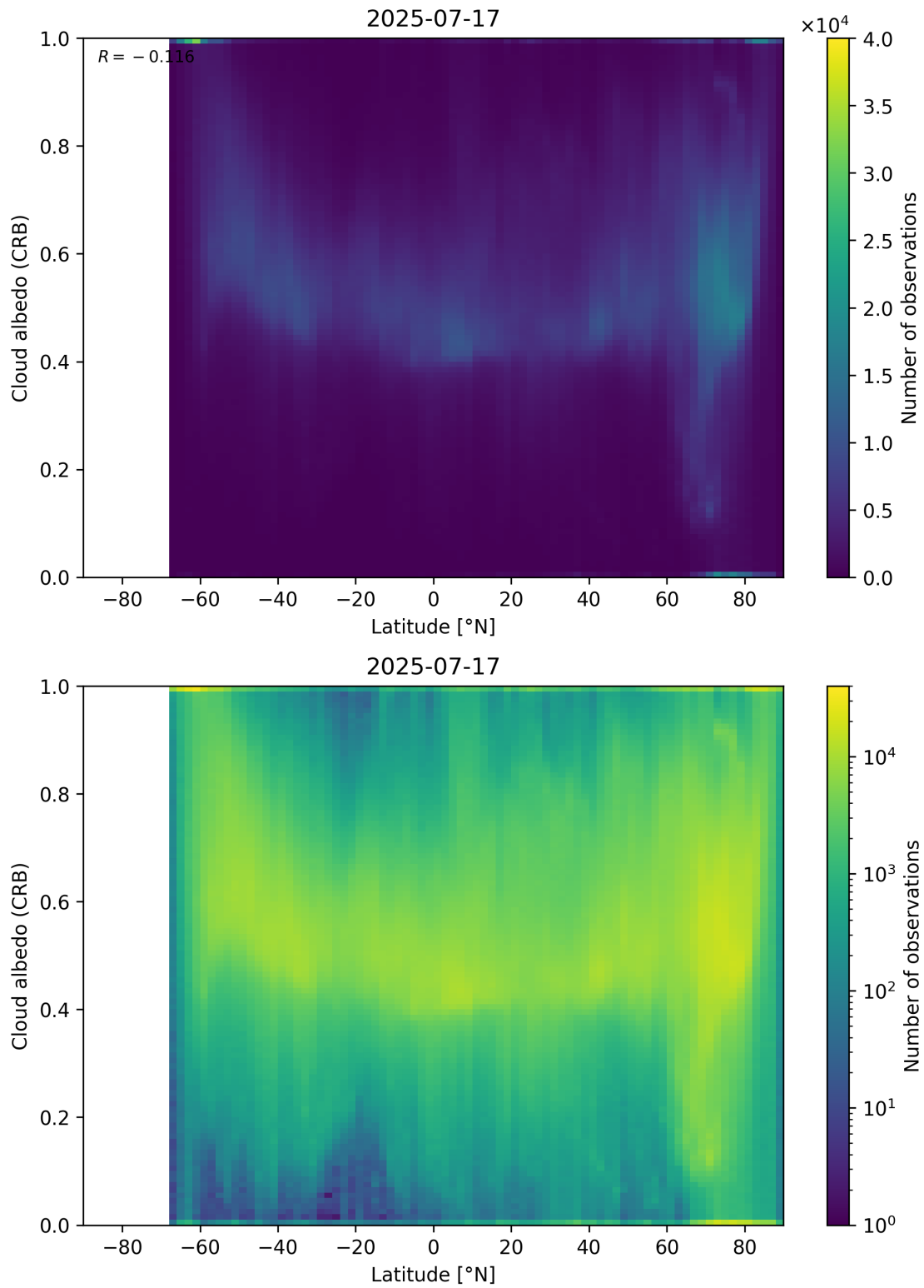
Figure 91: Scatter density plot of “Latitude” against “Cloud albedo (CRB)” for 2025-07-16 to 2025-07-18.
