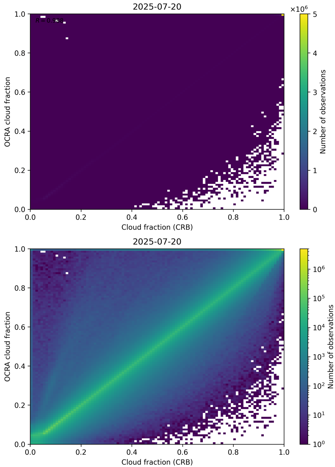
Figure 78: Scatter density plot of “Cloud fraction (CRB)” against “OCRA cloud fraction” for 2025-07-19 to 2025-07-21.
