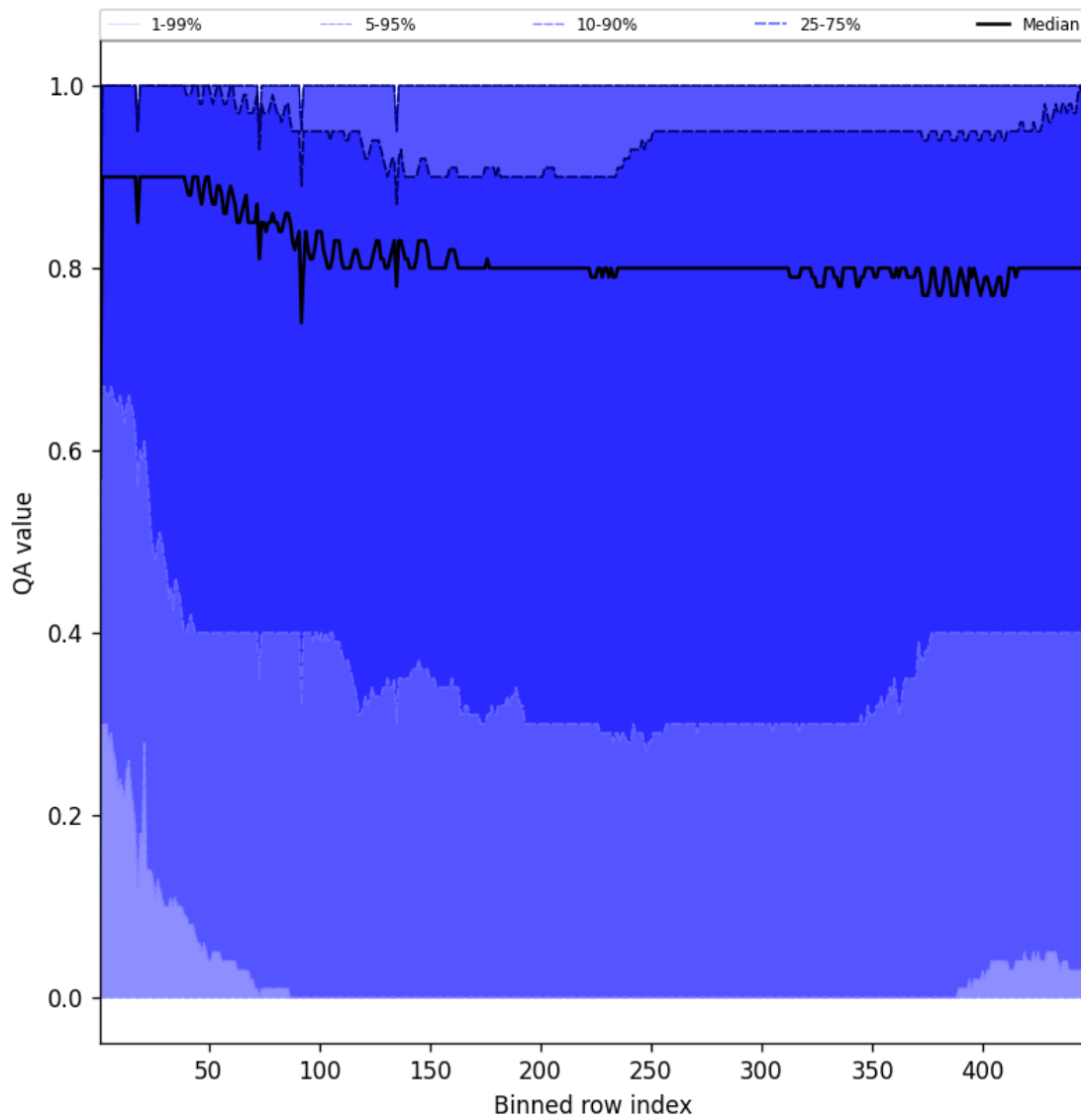
Figure 54: Along track statistics of “QA value” for 2025-07-19 to 2025-07-21
