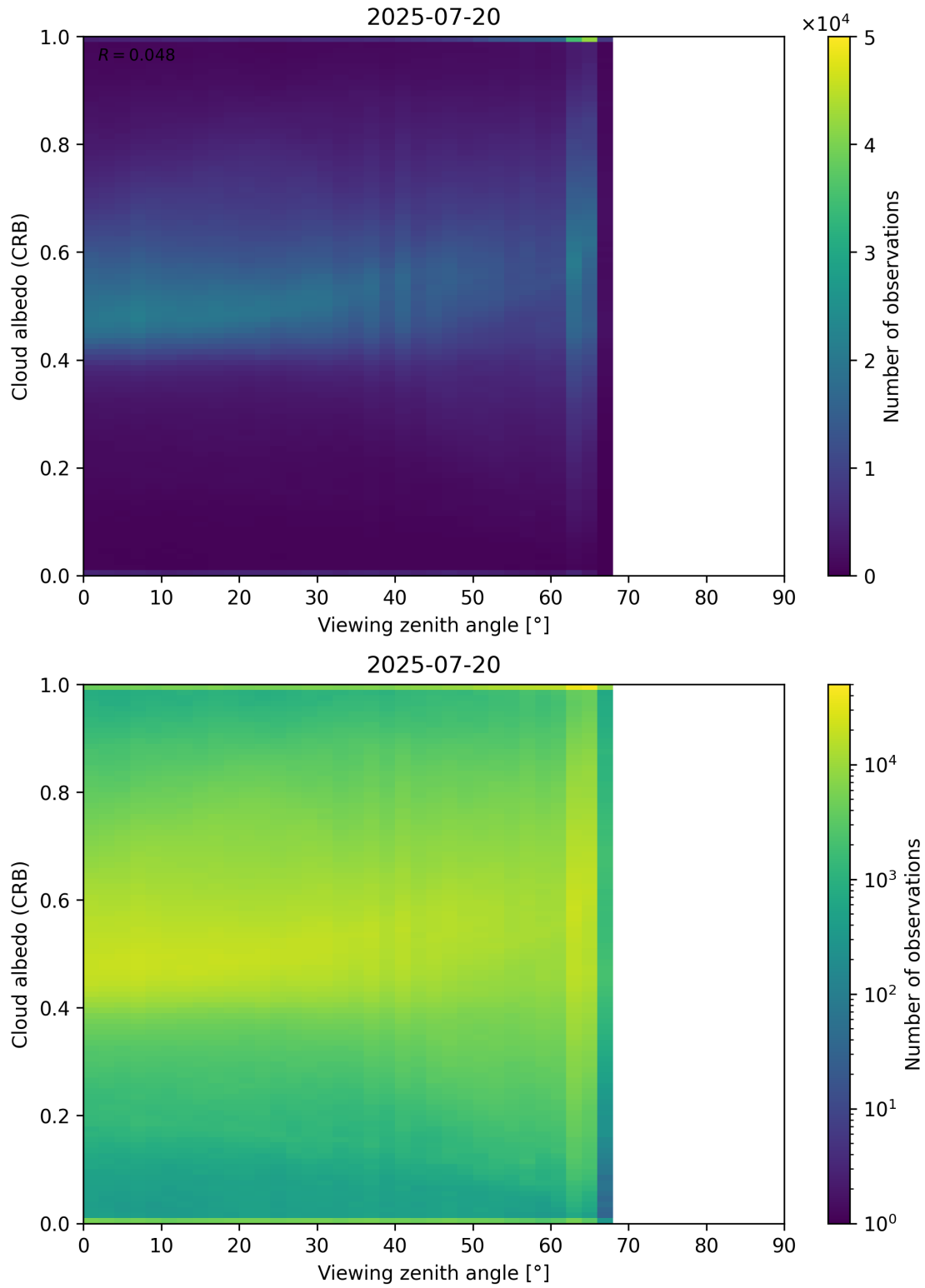
Figure 106: Scatter density plot of “Viewing zenith angle” against “Cloud albedo (CRB)” for 2025-07-19 to 2025-07-21.
