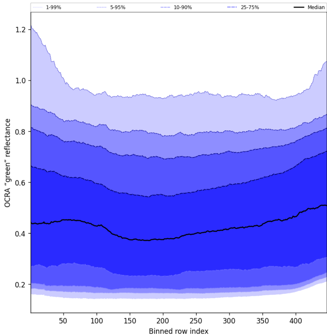
Figure 68: Along track statistics of “OCRA “green” reflectance” for 2025-07-19 to 2025-07-21
