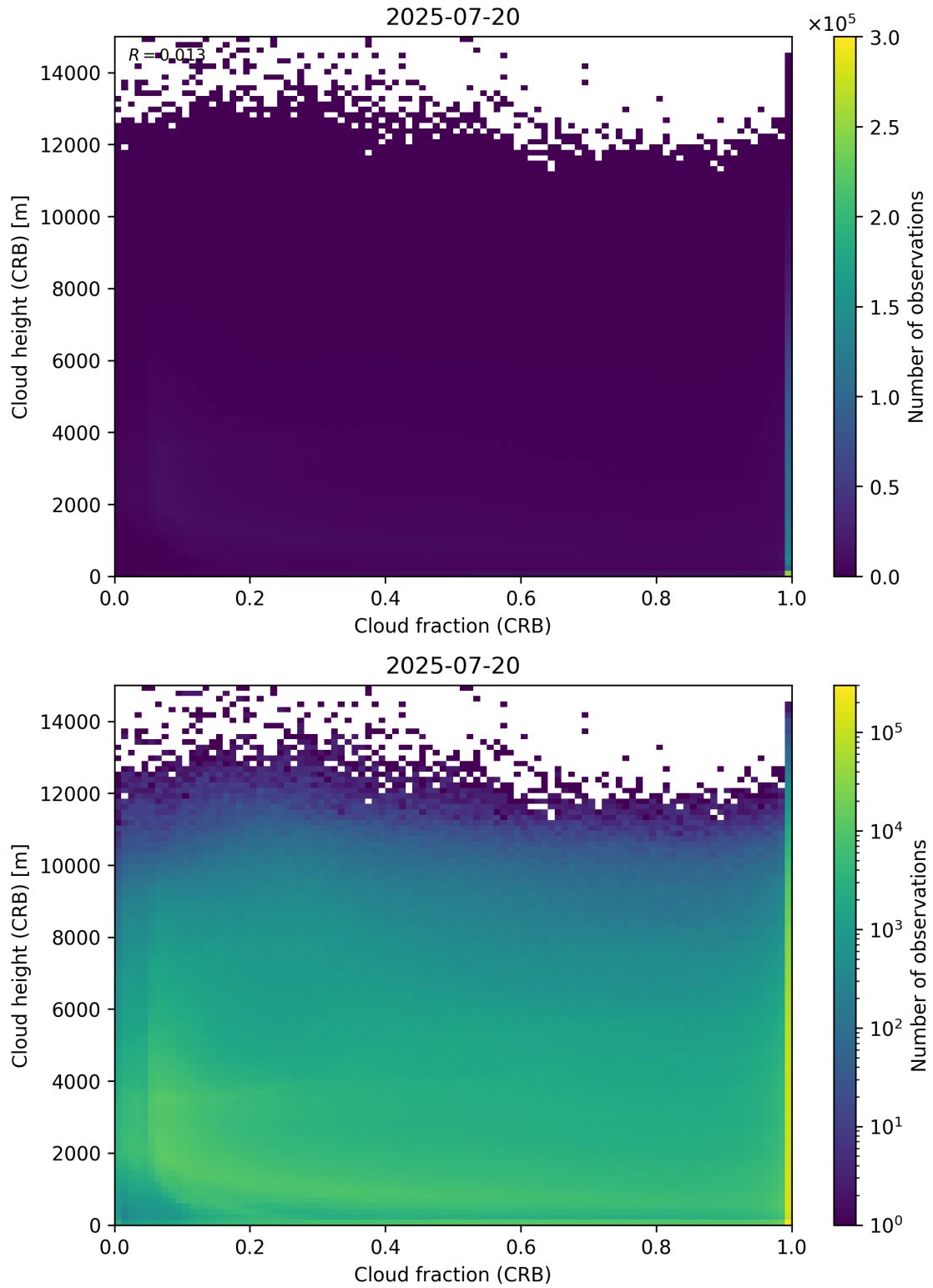
Figure 79: Scatter density plot of “Cloud fraction (CRB)” against “Cloud height (CRB)” for 2025-07-19 to 2025-07-21.
