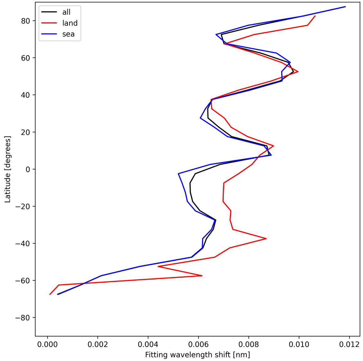
Figure 33: Zonal average of “Fitting wavelength shift” for 2025-07-19 to 2025-07-21.
