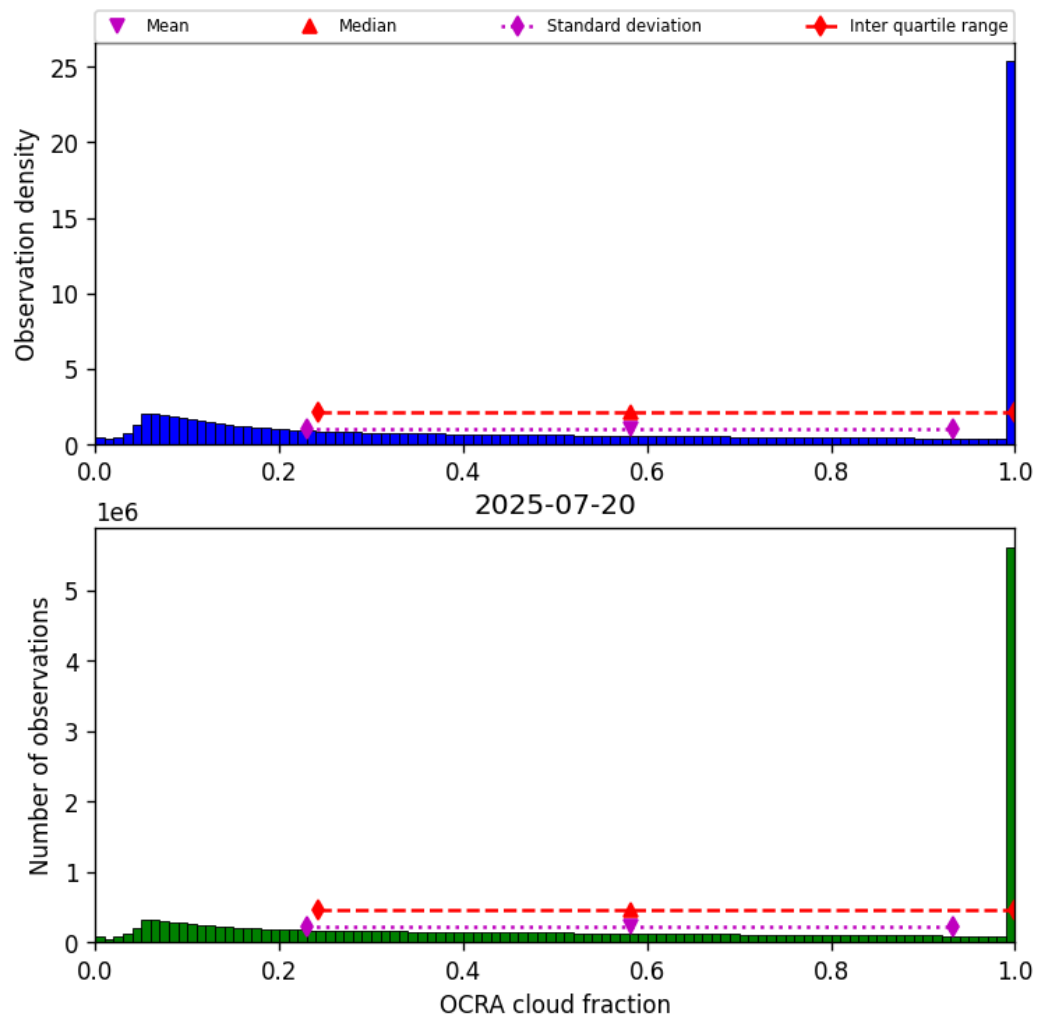
Figure 50: Histogram of “OCRA cloud fraction” for 2025-07-19 to 2025-07-21
