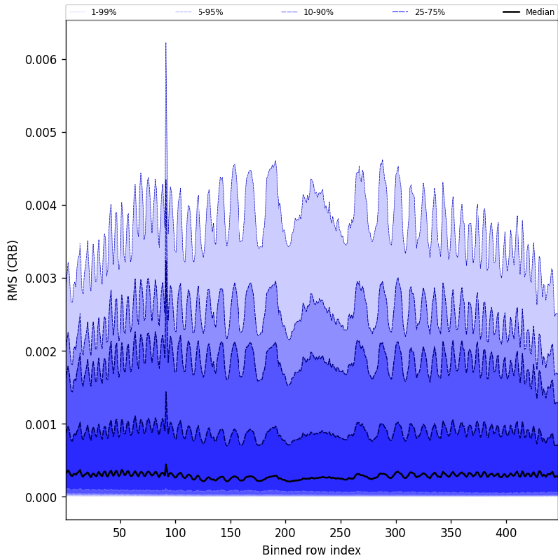
Figure 64: Along track statistics of “RMS (CRB)” for 2025-07-19 to 2025-07-21
