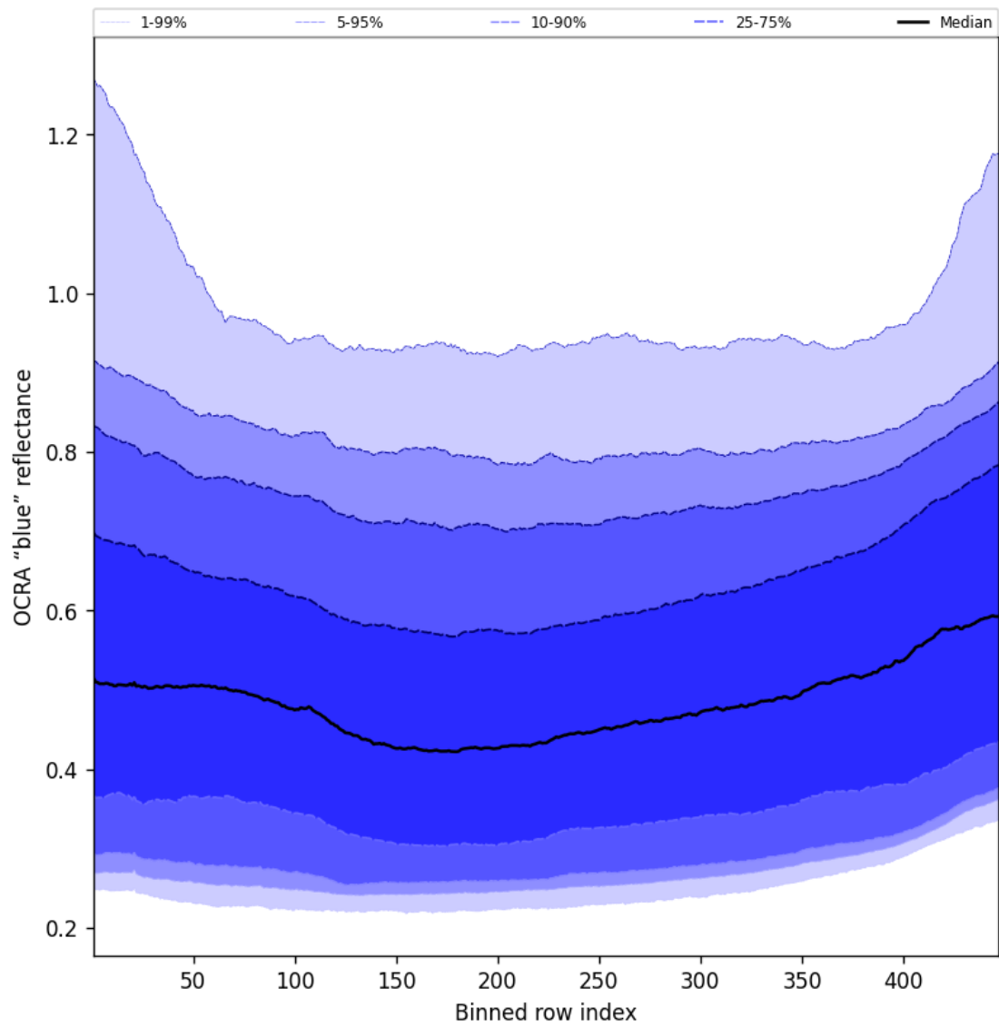
Figure 67: Along track statistics of “OCRA “blue” reflectance” for 2025-07-19 to 2025-07-21
