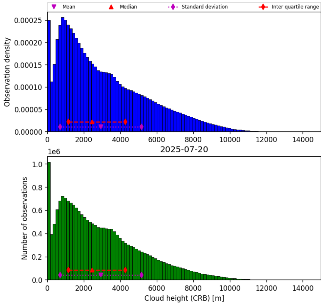
Figure 43: Histogram of “Cloud height (CRB)” for 2025-07-19 to 2025-07-21
