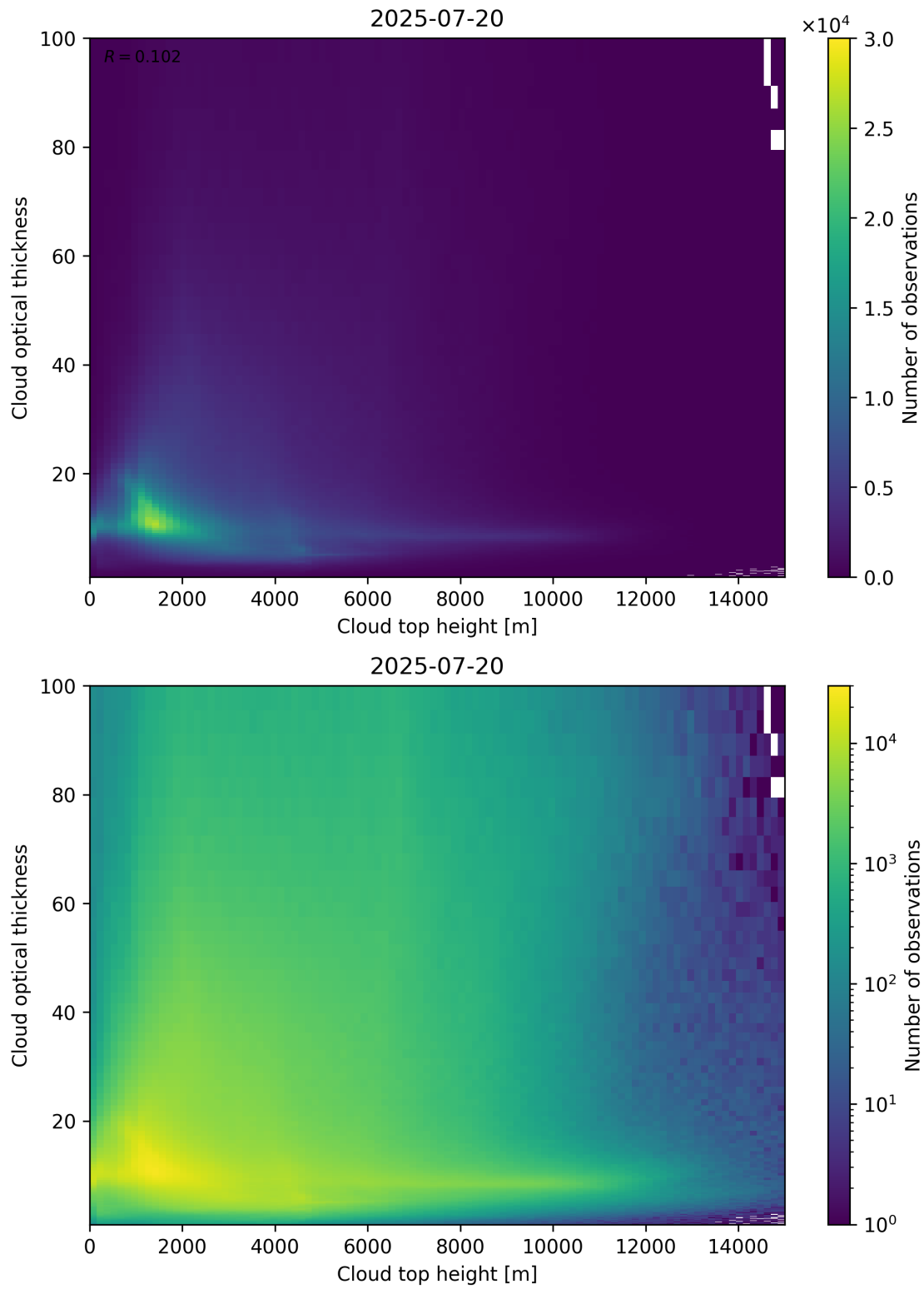
Figure 90: Scatter density plot of “Cloud top height” against “Cloud optical thickness” for 2025-07-19 to 2025-07-21.
