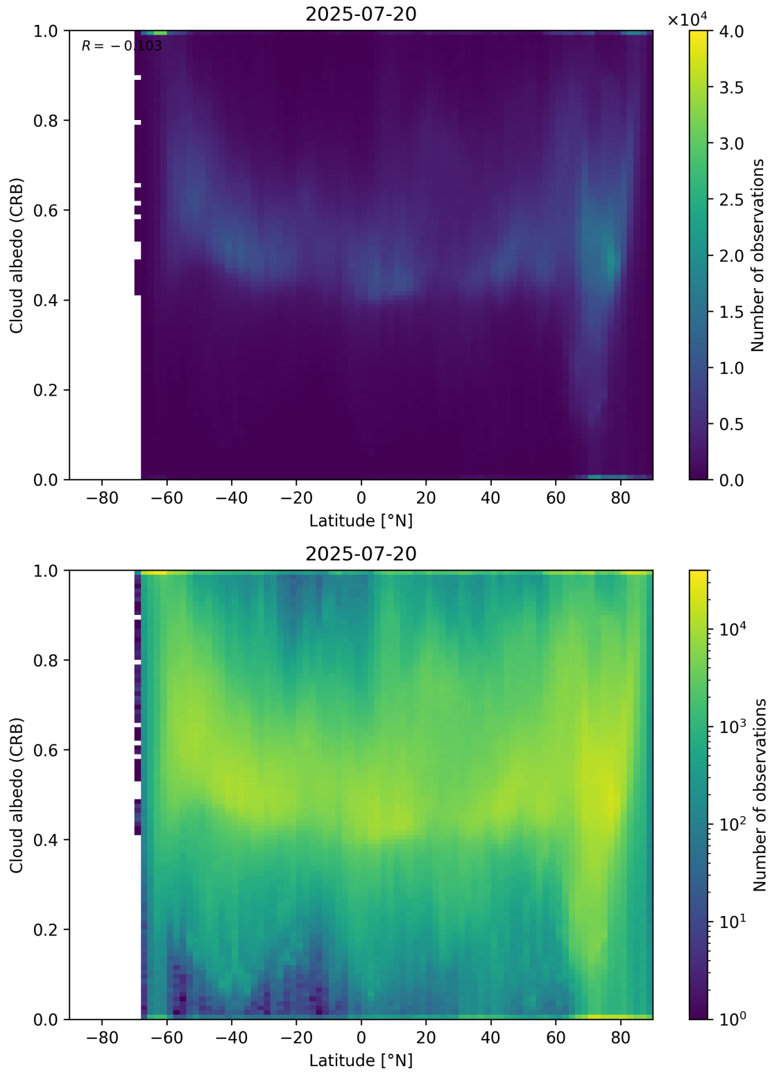
Figure 91: Scatter density plot of “Latitude” against “Cloud albedo (CRB)” for 2025-07-19 to 2025-07-21.
