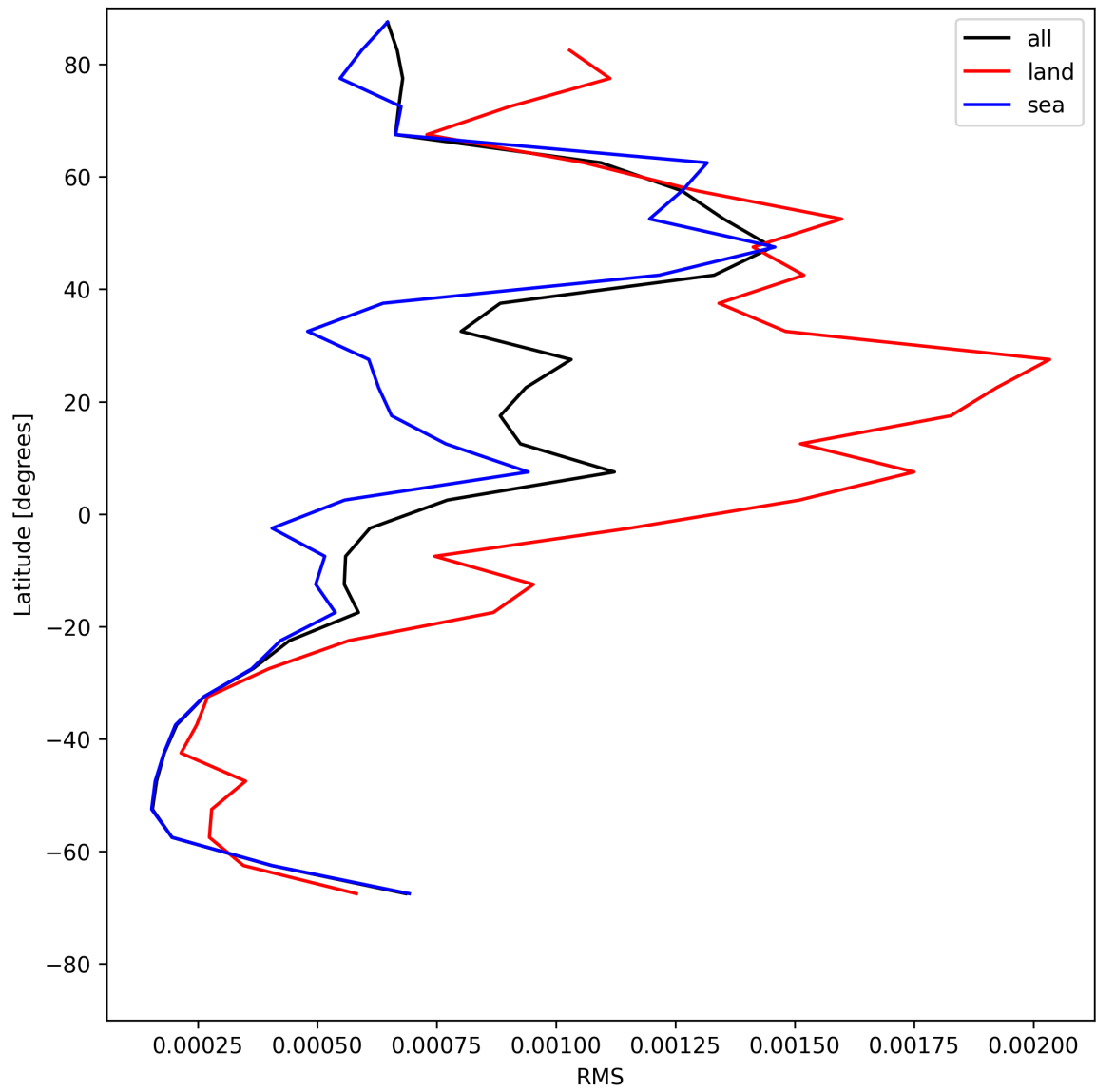
Figure 31: Zonal average of “RMS” for 2025-07-19 to 2025-07-21.
