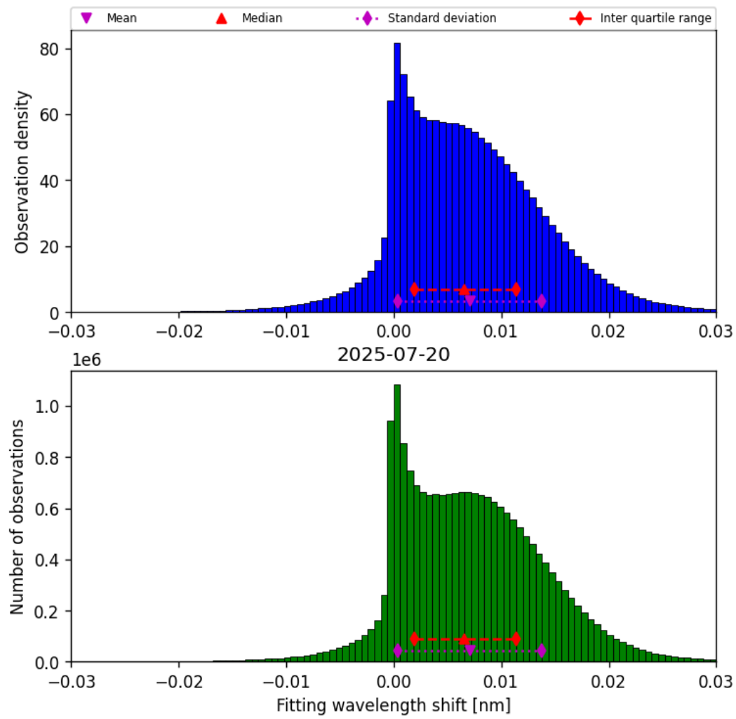
Figure 49: Histogram of “Fitting wavelength shift” for 2025-07-19 to 2025-07-21
