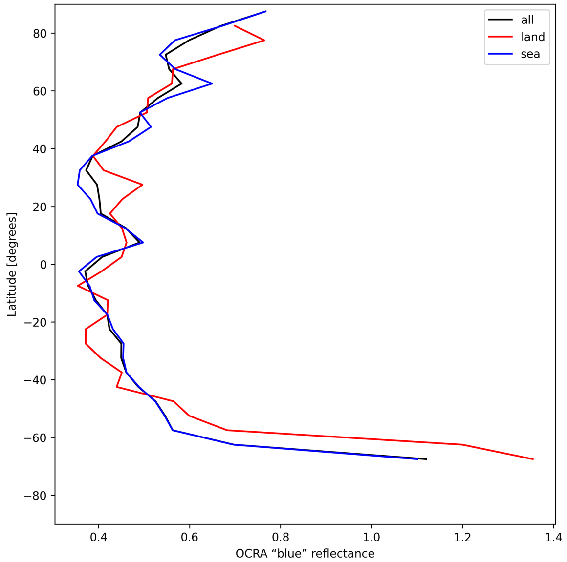
Figure 35: Zonal average of “OCRA “blue” reflectance” for 2025-07-19 to 2025-07-21.
