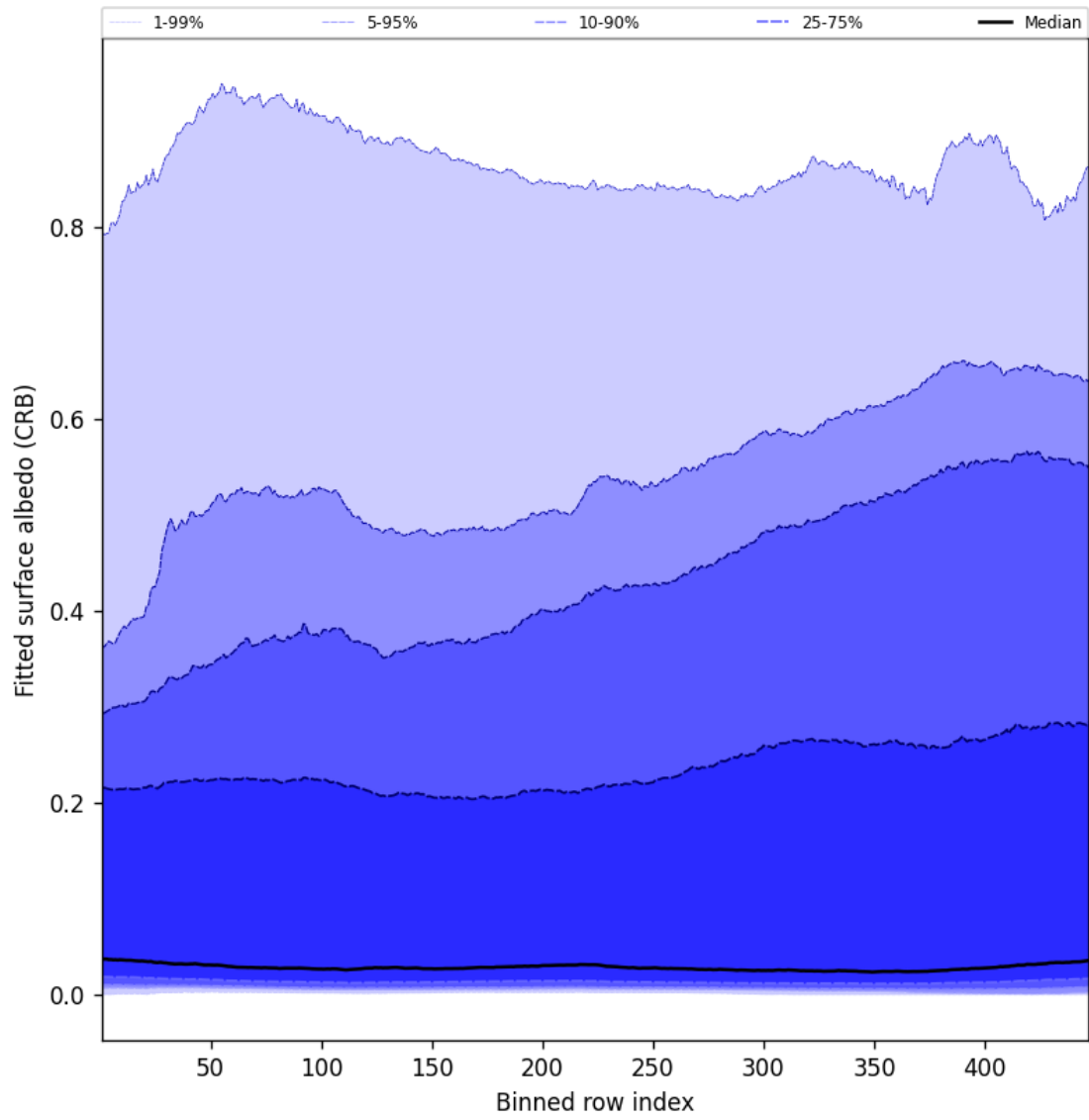
Figure 62: Along track statistics of “Fitted surface albedo (CRB)” for 2025-07-19 to 2025-07-21
