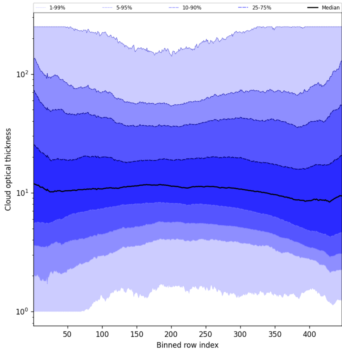
Figure 57: Along track statistics of “Cloud optical thickness” for 2025-07-19 to 2025-07-21
