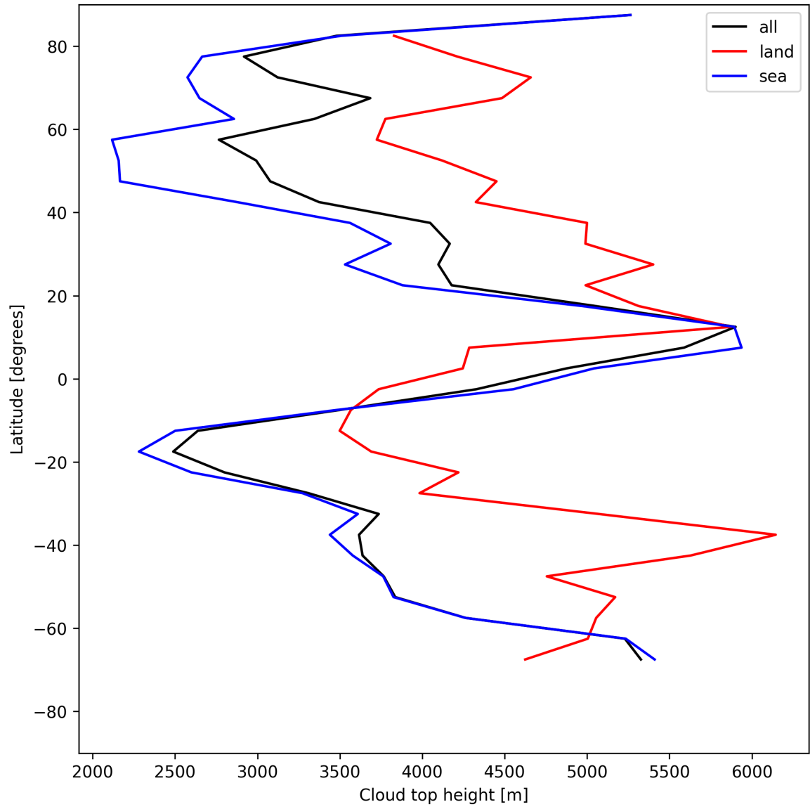
Figure 24: Zonal average of “Cloud top height” for 2025-07-19 to 2025-07-21.
