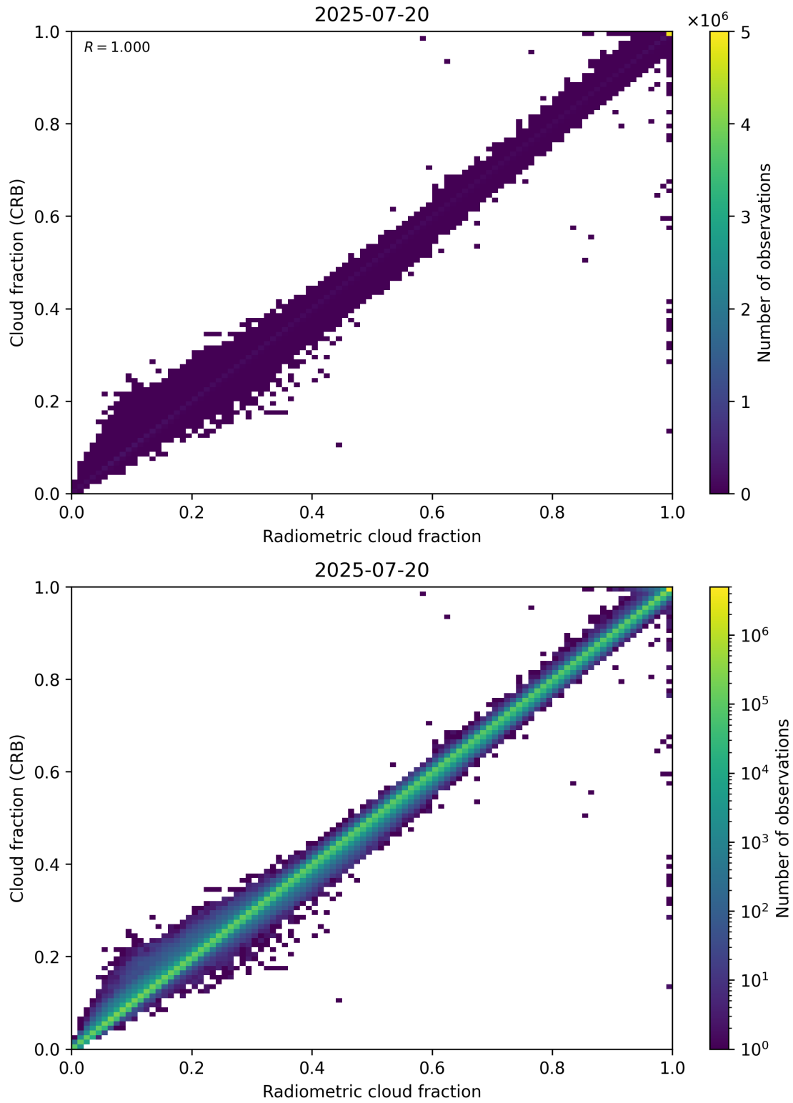
Figure 73: Scatter density plot of “Radiometric cloud fraction” against “Cloud fraction (CRB)” for 2025-07-19 to 2025-07-21.
