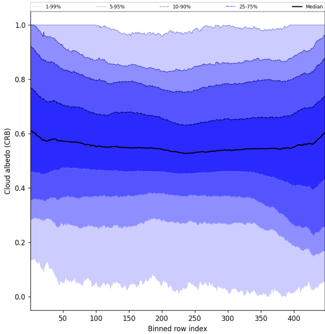
Figure 60: Along track statistics of “Cloud albedo (CRB)” for 2025-07-19 to 2025-07-21
