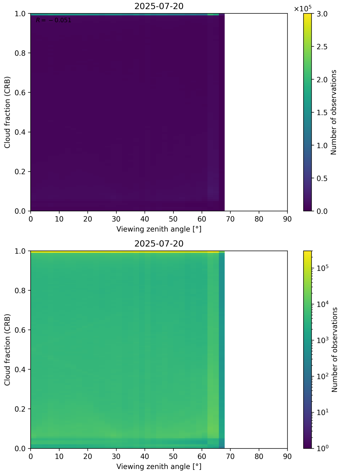
Figure 109: Scatter density plot of “Viewing zenith angle” against “Cloud fraction (CRB)” for 2025-07-19 to 2025-07-21.
