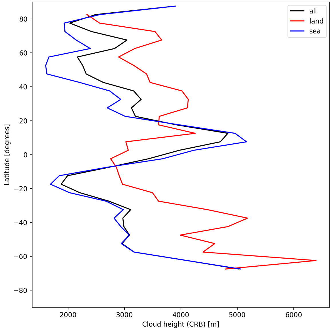
Figure 27: Zonal average of “Cloud height (CRB)” for 2025-07-19 to 2025-07-21.
