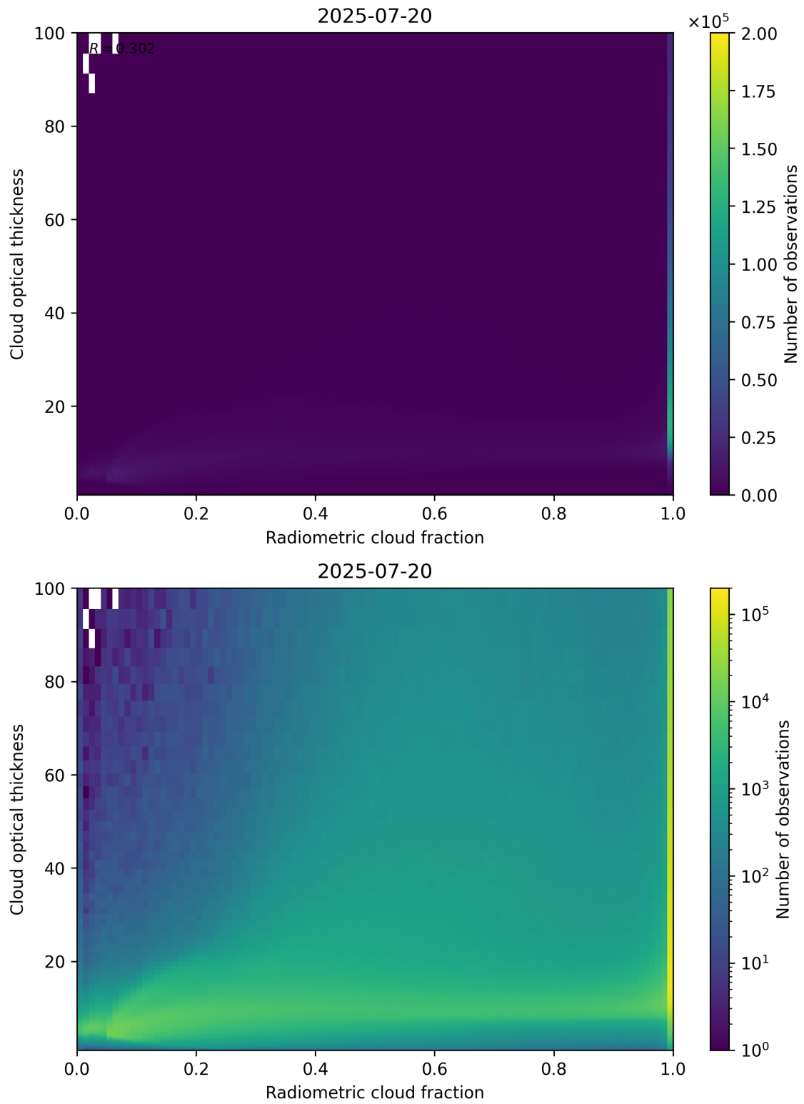
Figure 75: Scatter density plot of “Radiometric cloud fraction” against “Cloud optical thickness” for 2025-07-19 to 2025-07-21.
