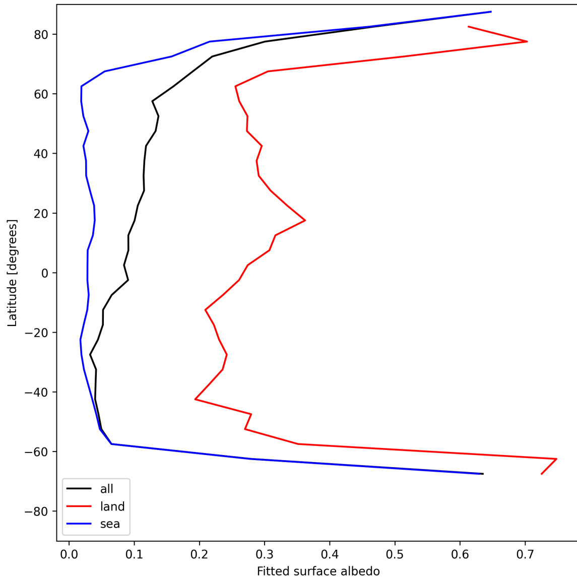
Figure 29: Zonal average of “Fitted surface albedo” for 2025-07-19 to 2025-07-21.
