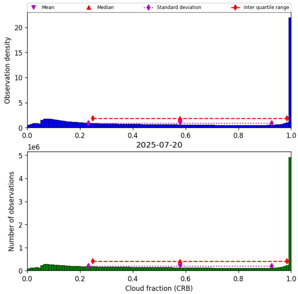
Figure 42: Histogram of “Cloud fraction (CRB)” for 2025-07-19 to 2025-07-21
