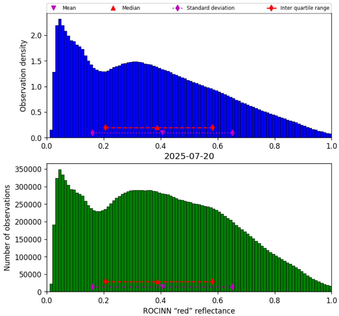
Figure 53: Histogram of “ROCINN “red” reflectance” for 2025-07-19 to 2025-07-21
