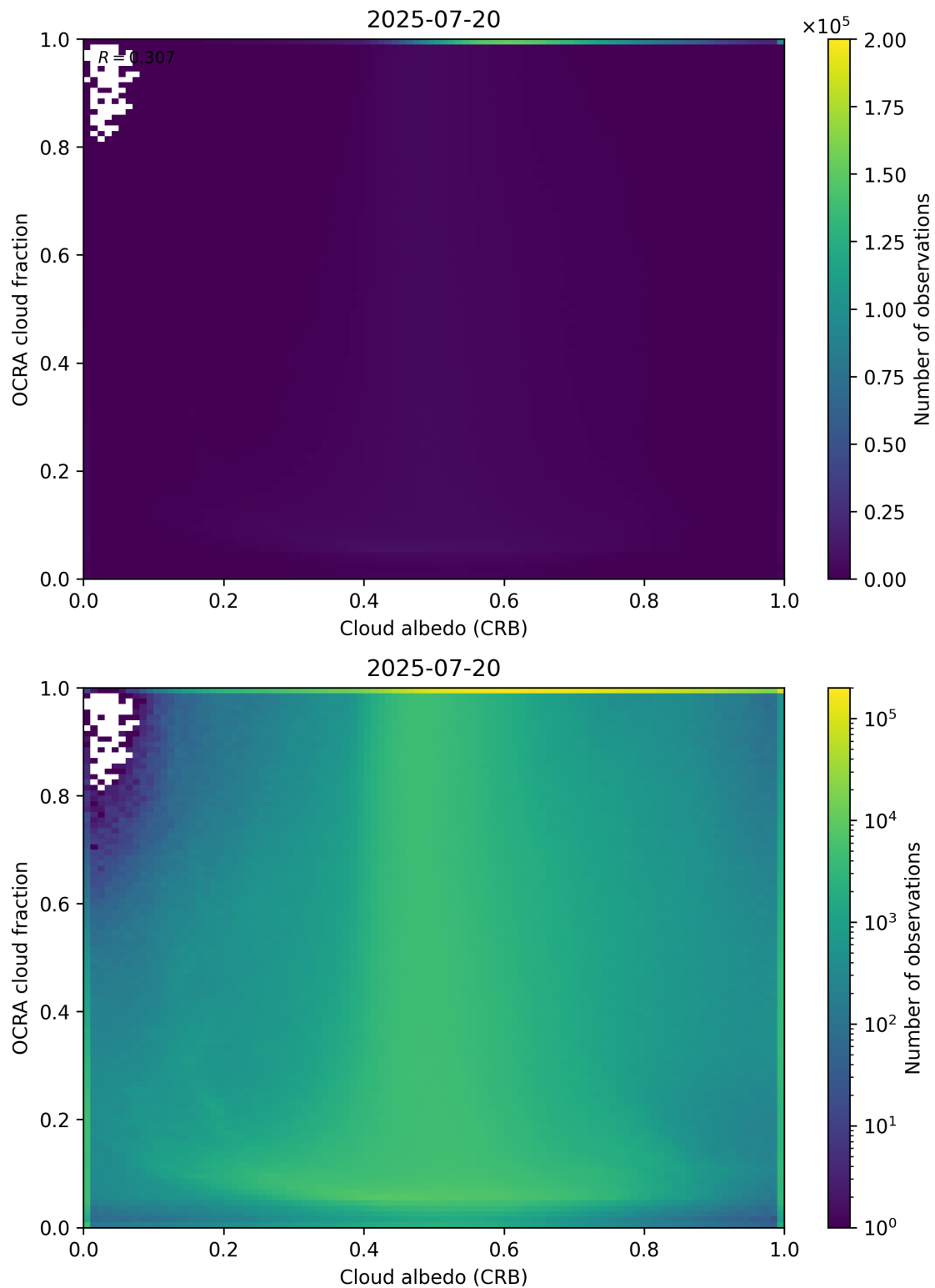
Figure 70: Scatter density plot of “Cloud albedo (CRB)” against “OCRA cloud fraction” for 2025-07-19 to 2025-07-21.
