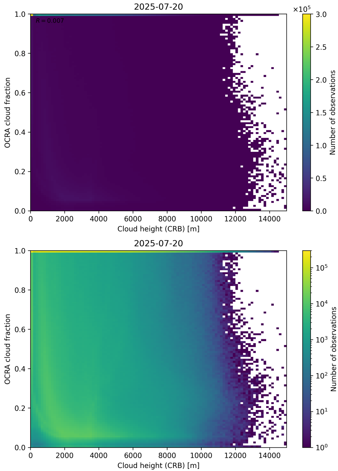
Figure 81: Scatter density plot of “Cloud height (CRB)” against “OCRA cloud fraction” for 2025-07-19 to 2025-07-21.
