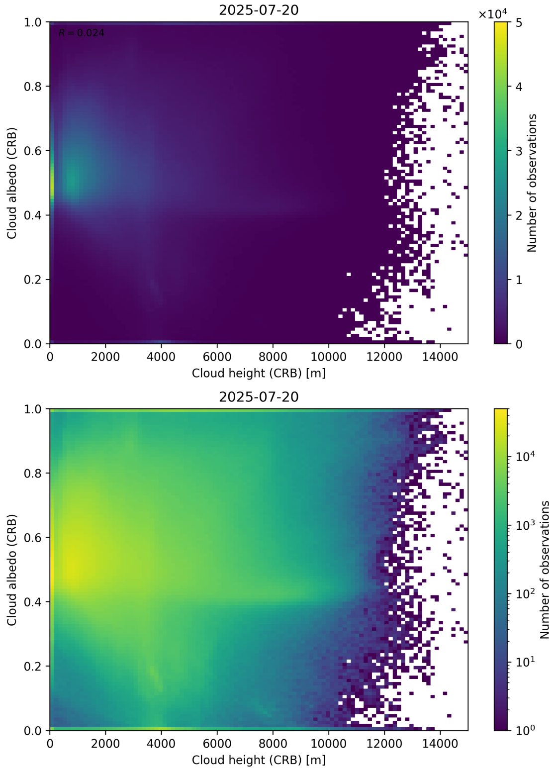
Figure 80: Scatter density plot of “Cloud height (CRB)” against “Cloud albedo (CRB)” for 2025-07-19 to 2025-07-21.
