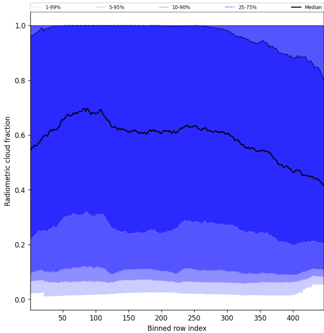
Figure 55: Along track statistics of “Radiometric cloud fraction” for 2025-07-19 to 2025-07-21
