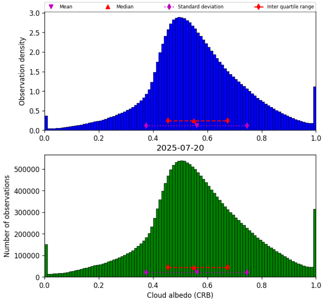
Figure 44: Histogram of “Cloud albedo (CRB)” for 2025-07-19 to 2025-07-21
