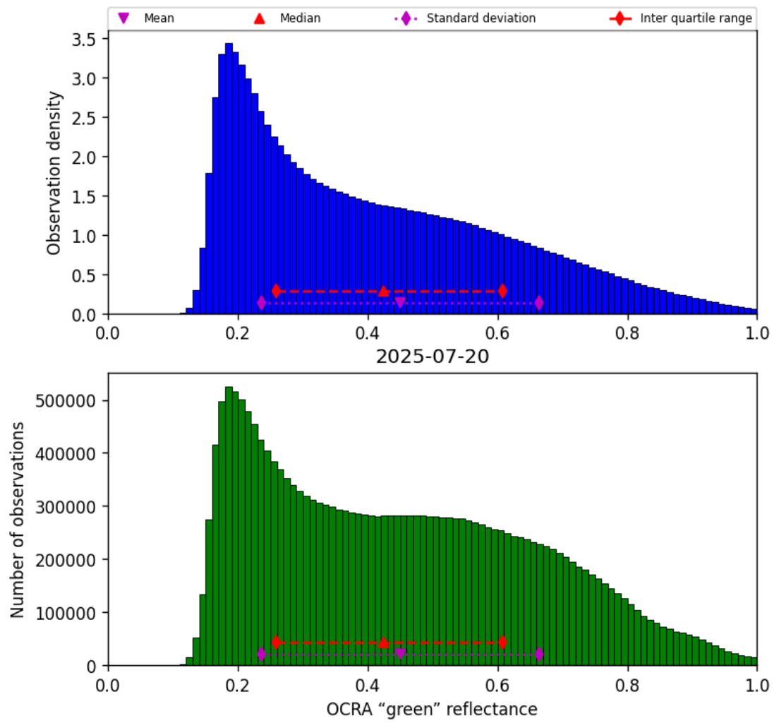
Figure 52: Histogram of “OCRA “green” reflectance” for 2025-07-19 to 2025-07-21
