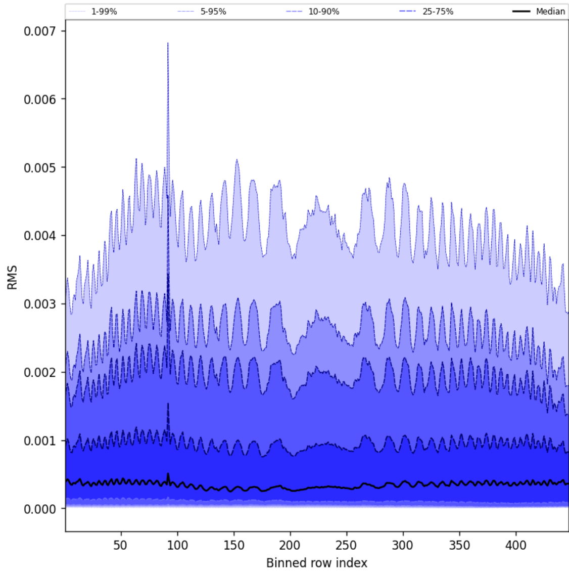
Figure 63: Along track statistics of “RMS” for 2025-07-19 to 2025-07-21
