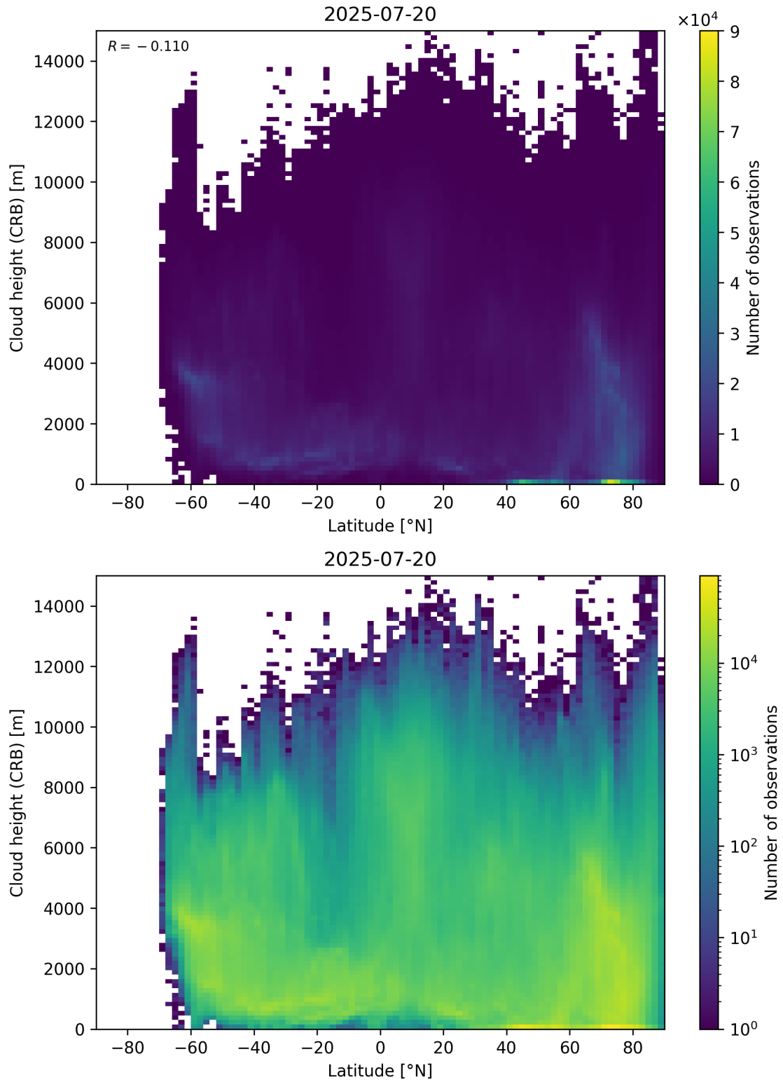
Figure 95: Scatter density plot of “Latitude” against “Cloud height (CRB)” for 2025-07-19 to 2025-07-21.
