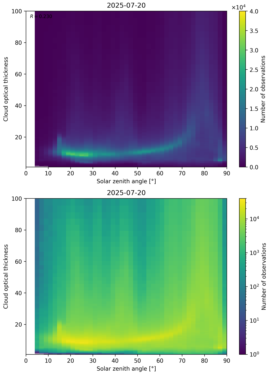
Figure 103: Scatter density plot of “Solar zenith angle” against “Cloud optical thickness” for 2025-07-19 to 2025-07-21.
