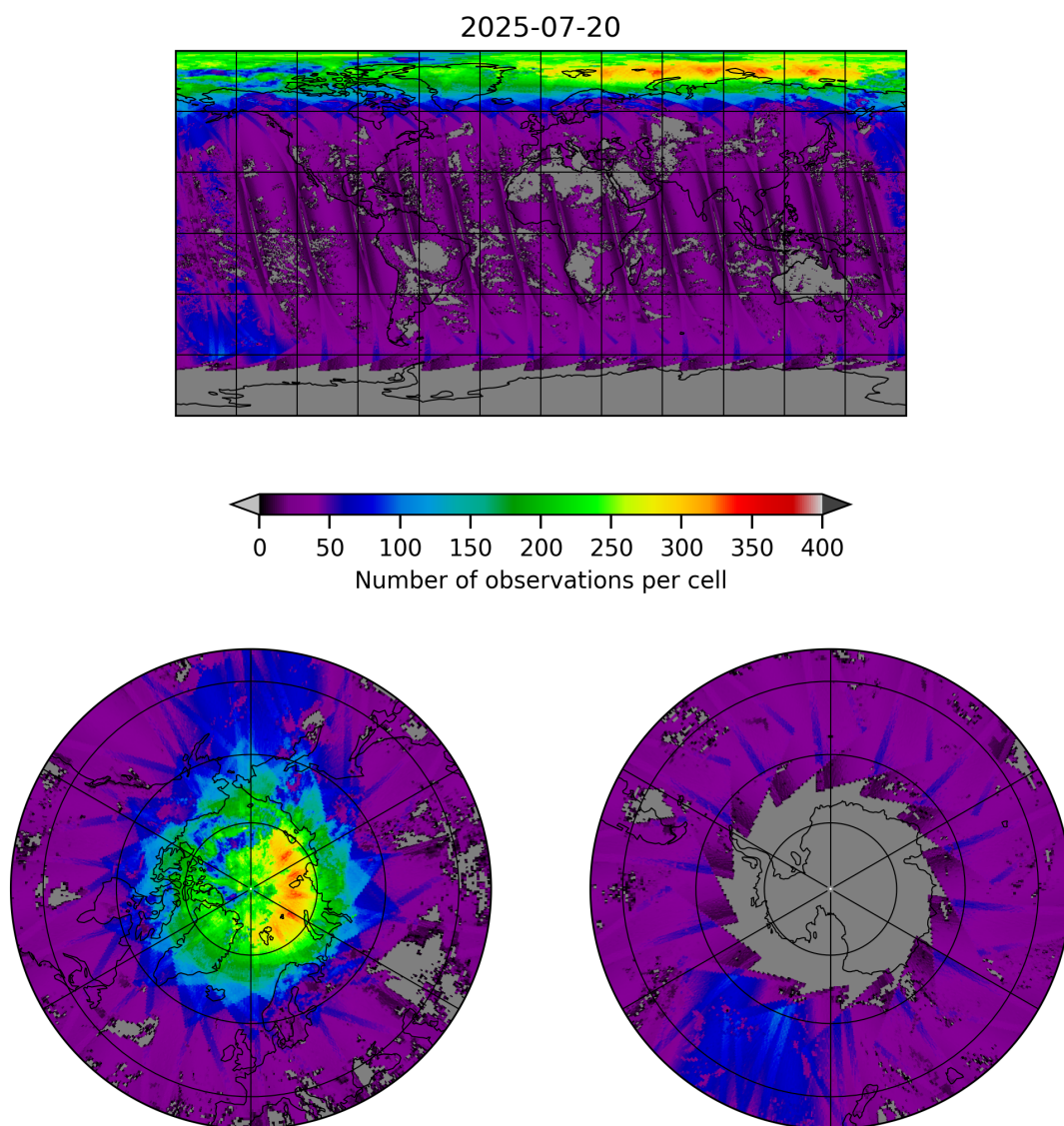
Figure 21: Map of the number of observations for 2025-07-19 to 2025-07-21
