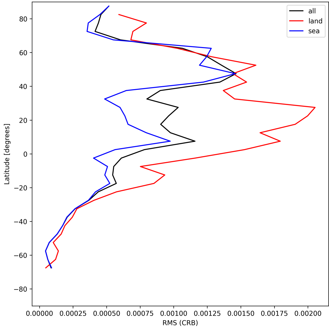
Figure 32: Zonal average of “RMS (CRB)” for 2025-07-19 to 2025-07-21.
