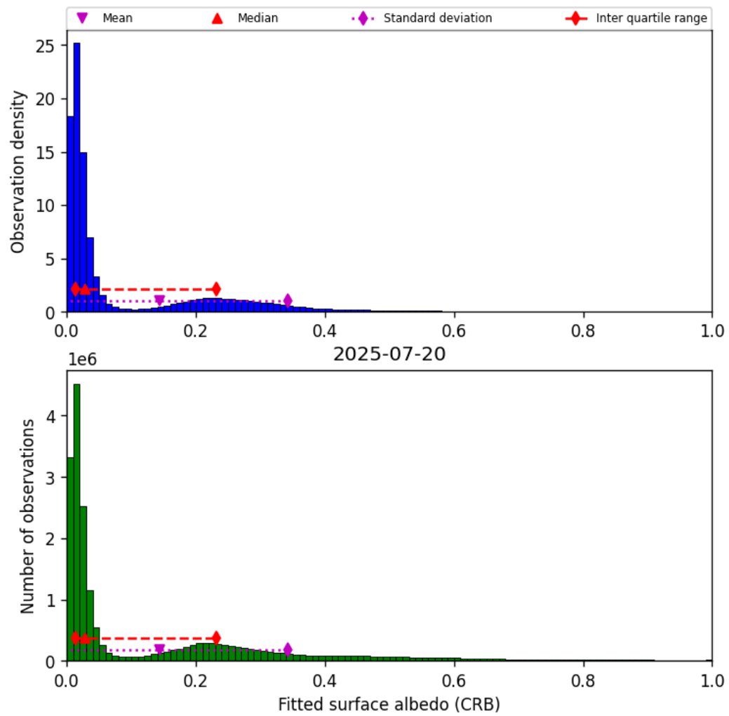
Figure 46: Histogram of “Fitted surface albedo (CRB)” for 2025-07-19 to 2025-07-21
