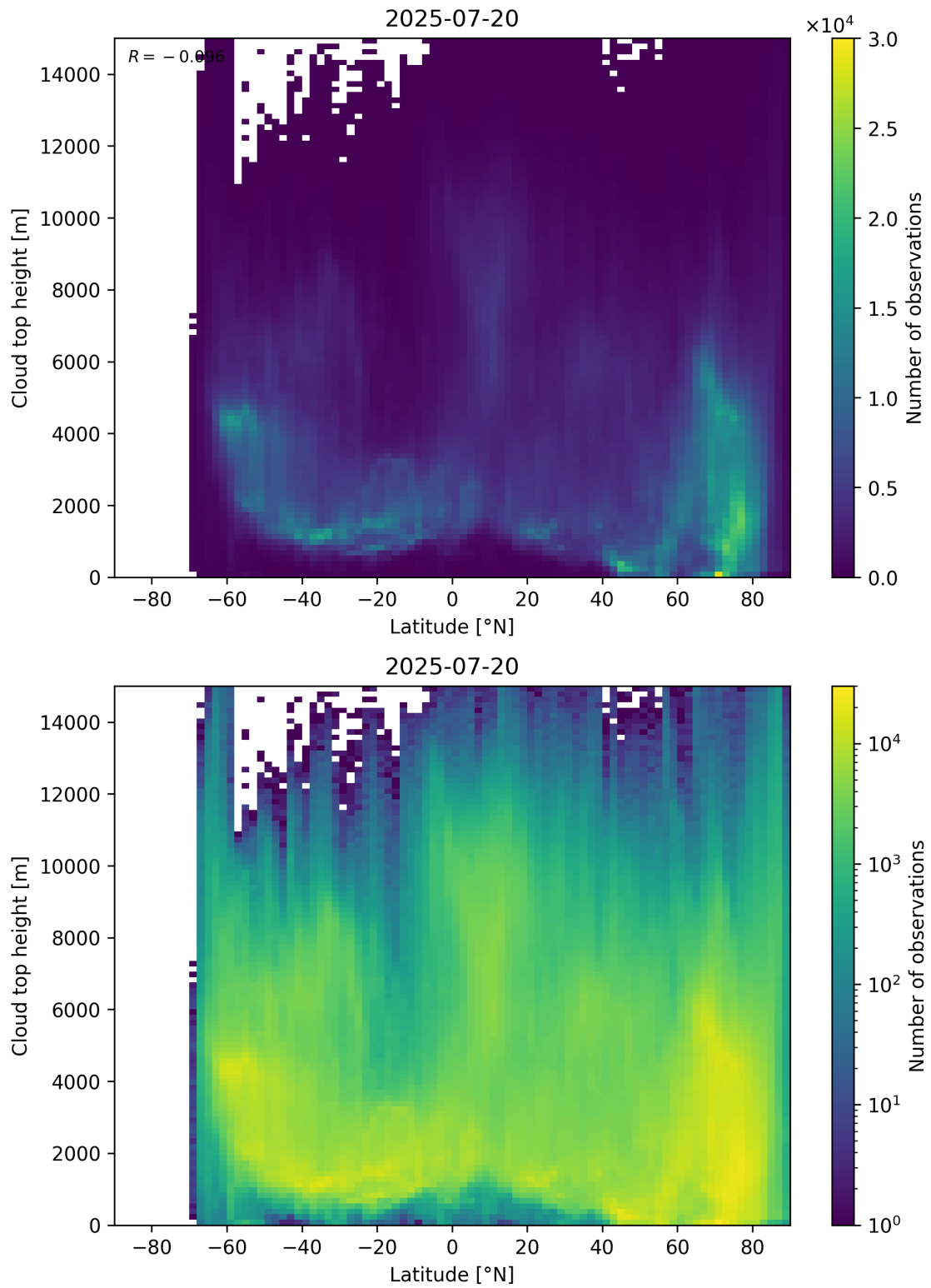
Figure 97: Scatter density plot of “Latitude” against “Cloud top height” for 2025-07-19 to 2025-07-21.
