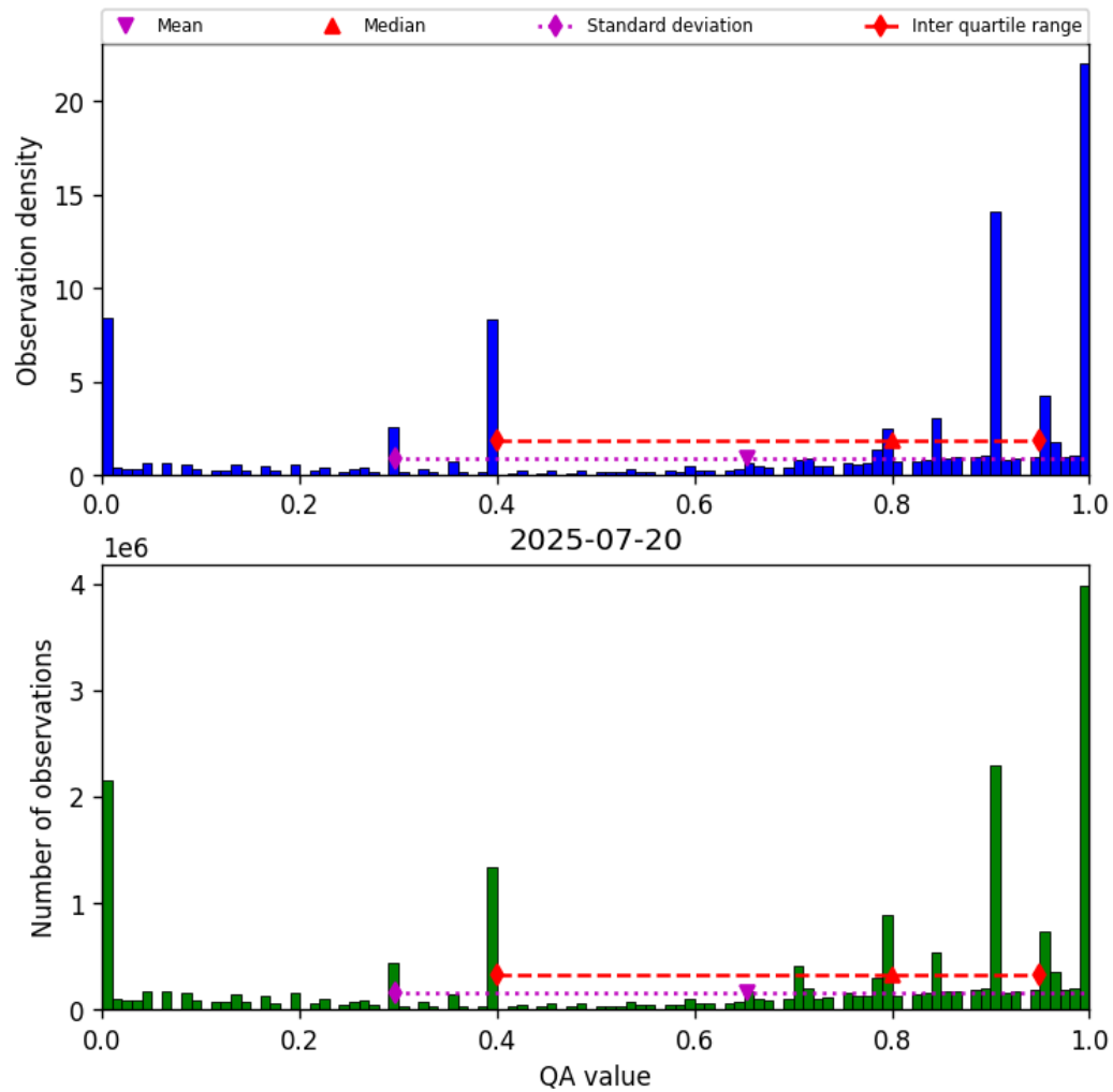
Figure 38: Histogram of “QA value” for 2025-07-19 to 2025-07-21
