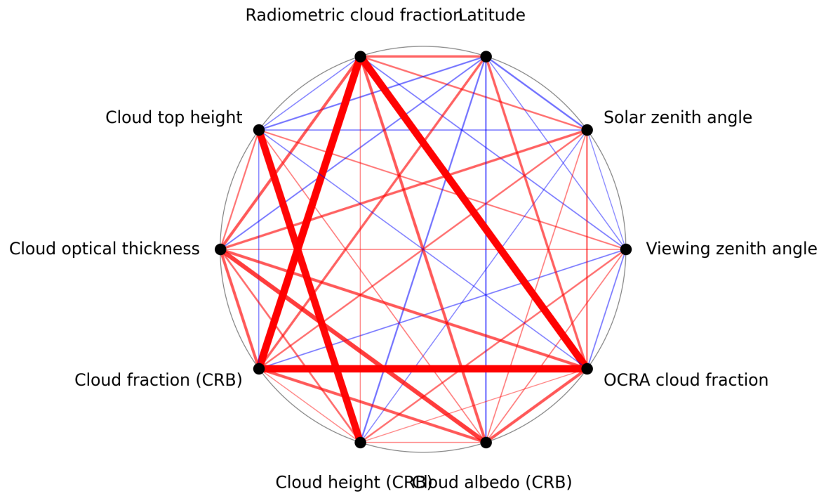
Figure 1: Map of correlation graph for 2025-07-19 to 2025-07-21.
