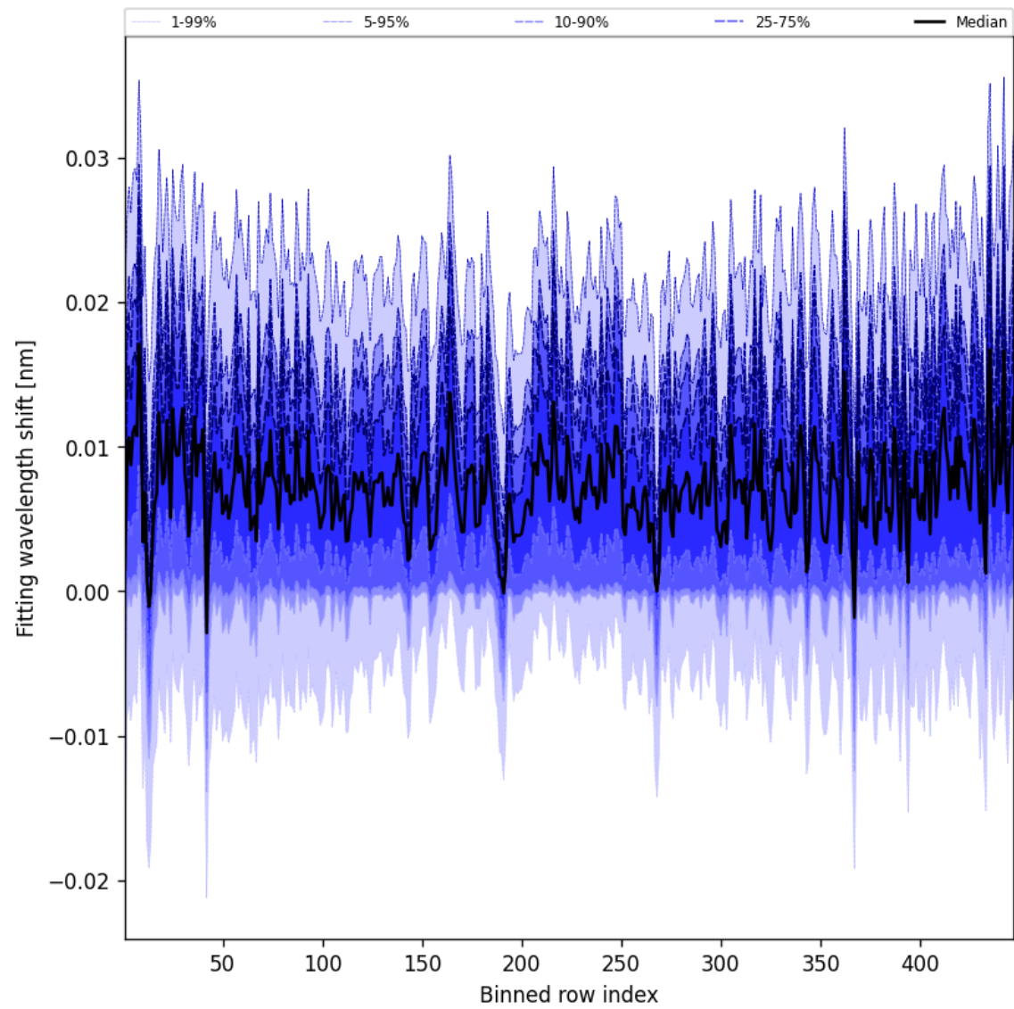
Figure 65: Along track statistics of “Fitting wavelength shift” for 2025-07-19 to 2025-07-21
