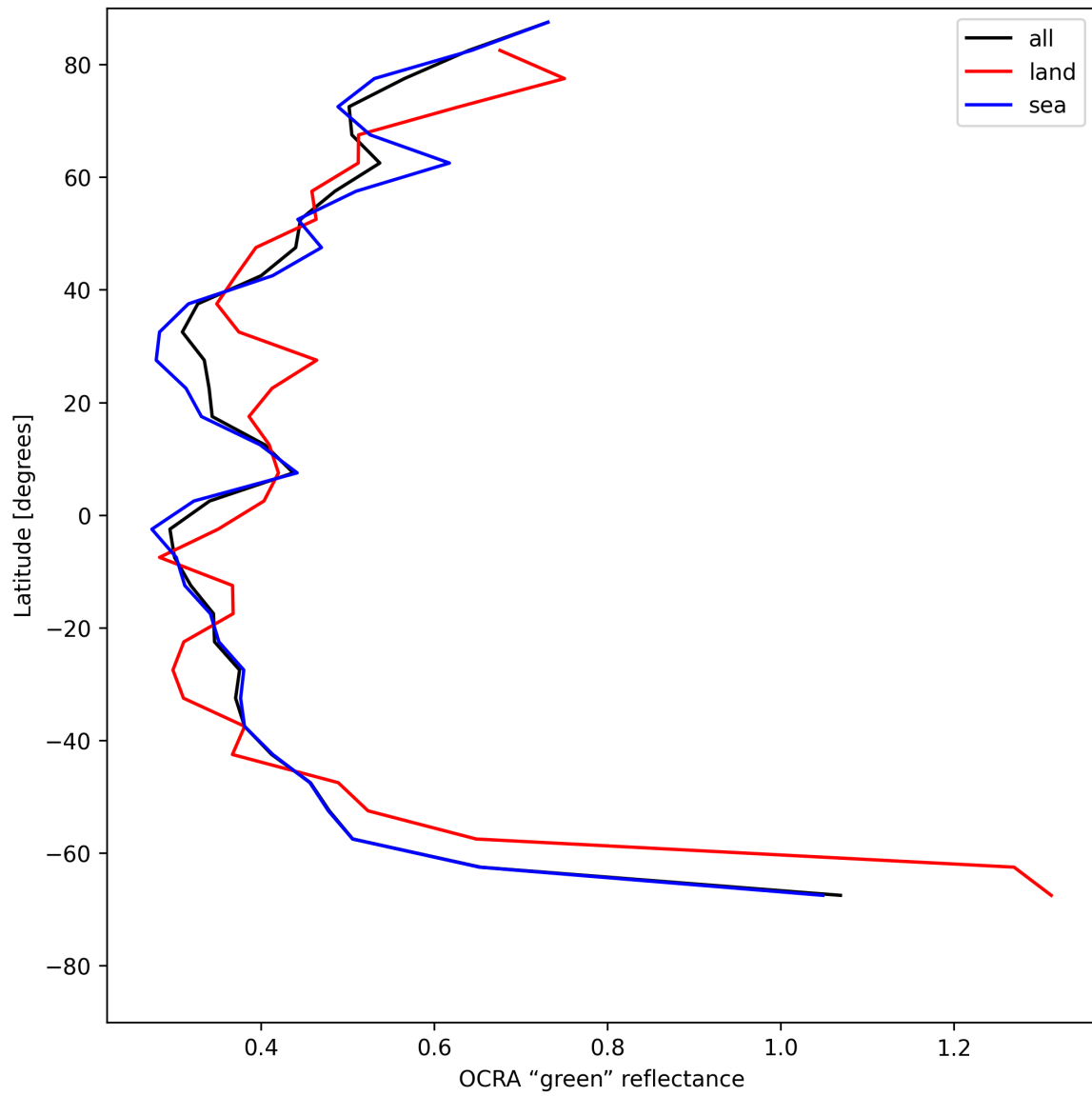
Figure 36: Zonal average of “OCRA “green” reflectance” for 2025-07-19 to 2025-07-21.
