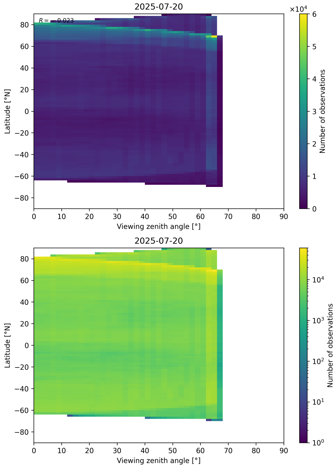
Figure 113: Scatter density plot of “Viewing zenith angle” against “Latitude” for 2025-07-19 to 2025-07-21.
