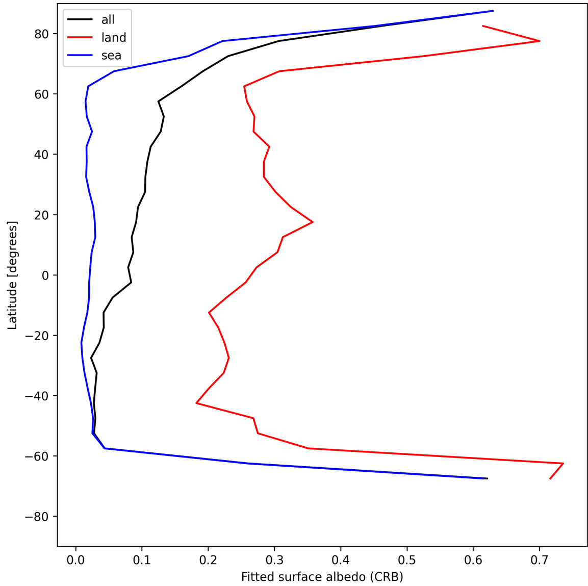
Figure 30: Zonal average of “Fitted surface albedo (CRB)” for 2025-07-19 to 2025-07-21.
