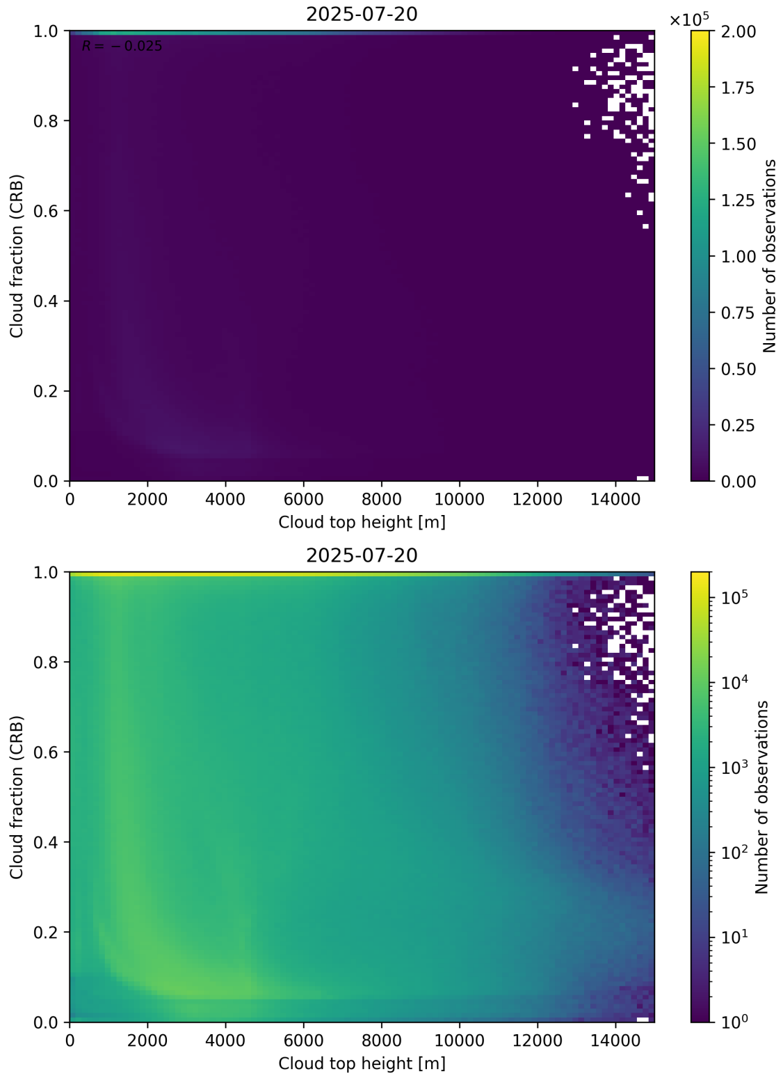
Figure 88: Scatter density plot of “Cloud top height” against “Cloud fraction (CRB)” for 2025-07-19 to 2025-07-21.
