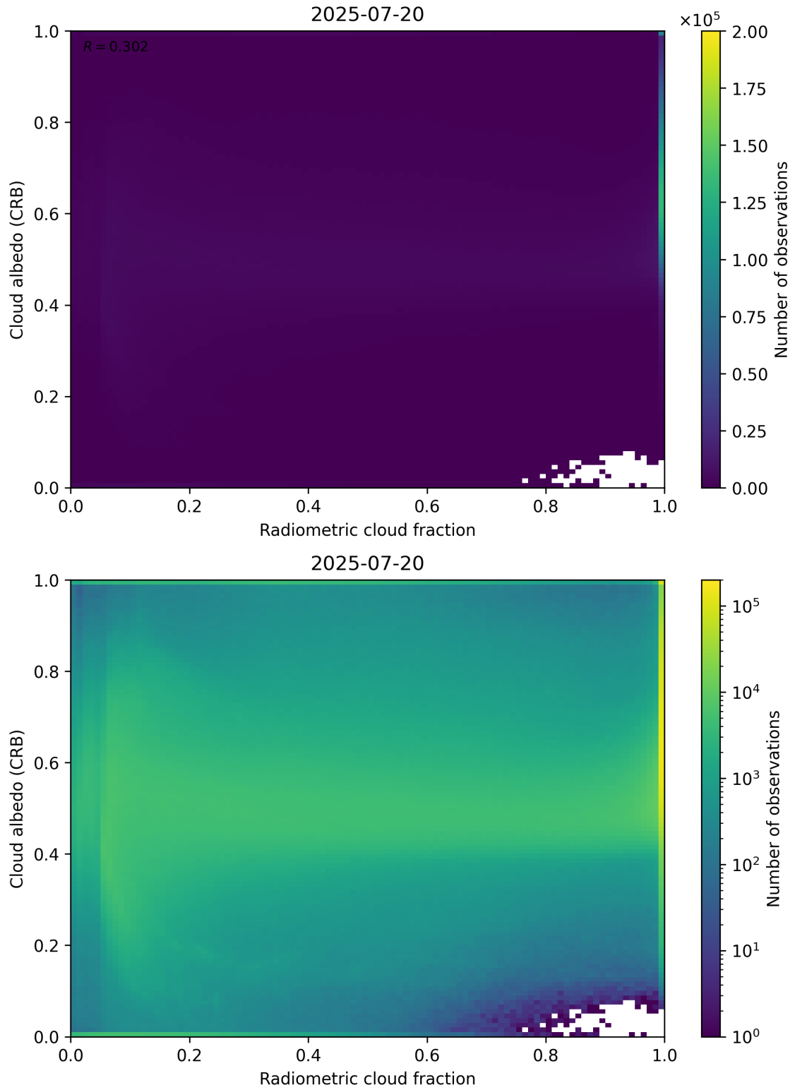
Figure 71: Scatter density plot of “Radiometric cloud fraction” against “Cloud albedo (CRB)” for 2025-07-19 to 2025-07-21.
