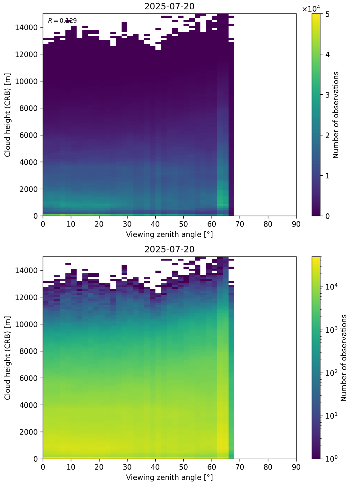
Figure 110: Scatter density plot of “Viewing zenith angle” against “Cloud height (CRB)” for 2025-07-19 to 2025-07-21.
