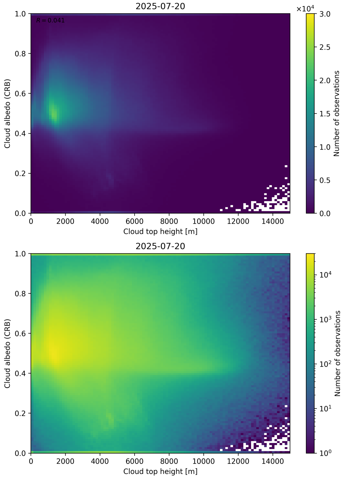
Figure 86: Scatter density plot of “Cloud top height” against “Cloud albedo (CRB)” for 2025-07-19 to 2025-07-21.
