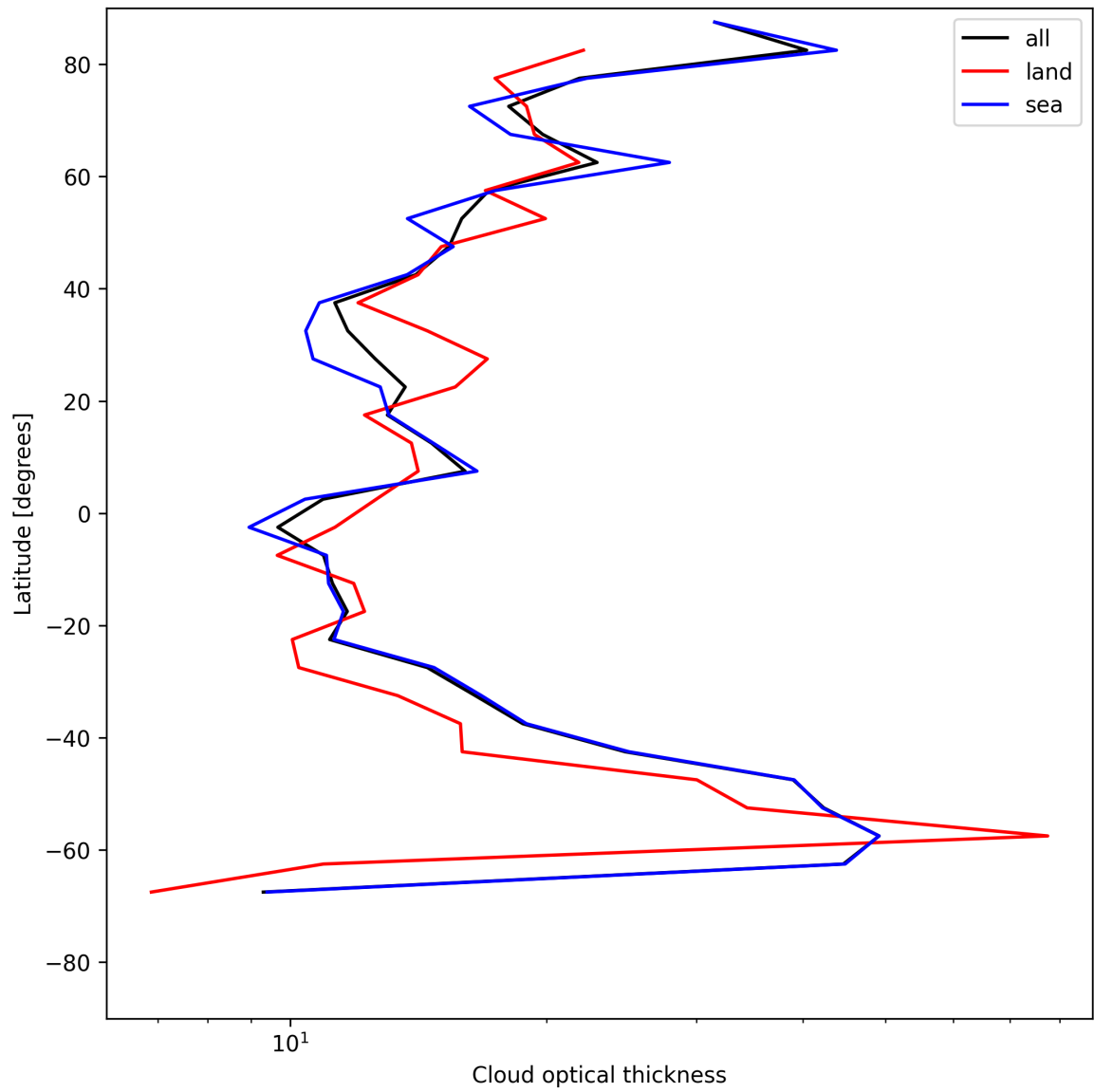
Figure 25: Zonal average of “Cloud optical thickness” for 2025-07-19 to 2025-07-21.
