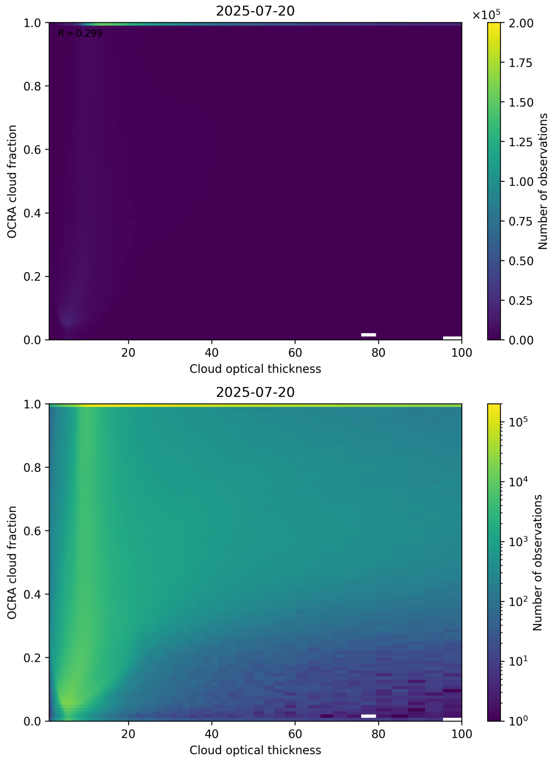
Figure 83: Scatter density plot of “Cloud optical thickness” against “OCRA cloud fraction” for 2025-07-19 to 2025-07-21.
