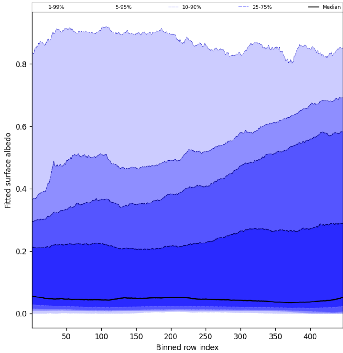
Figure 61: Along track statistics of “Fitted surface albedo” for 2025-07-19 to 2025-07-21
