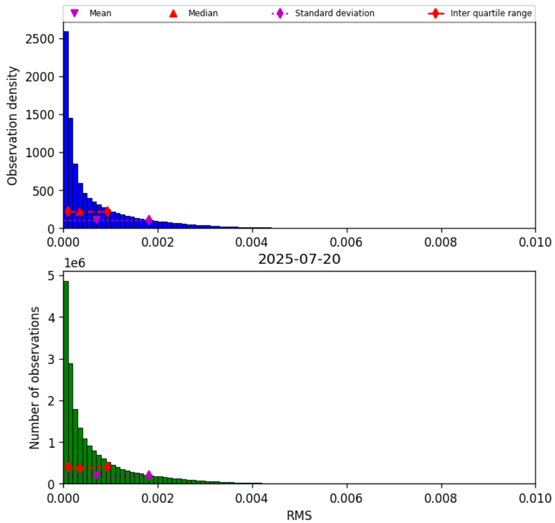
Figure 47: Histogram of “RMS” for 2025-07-19 to 2025-07-21
