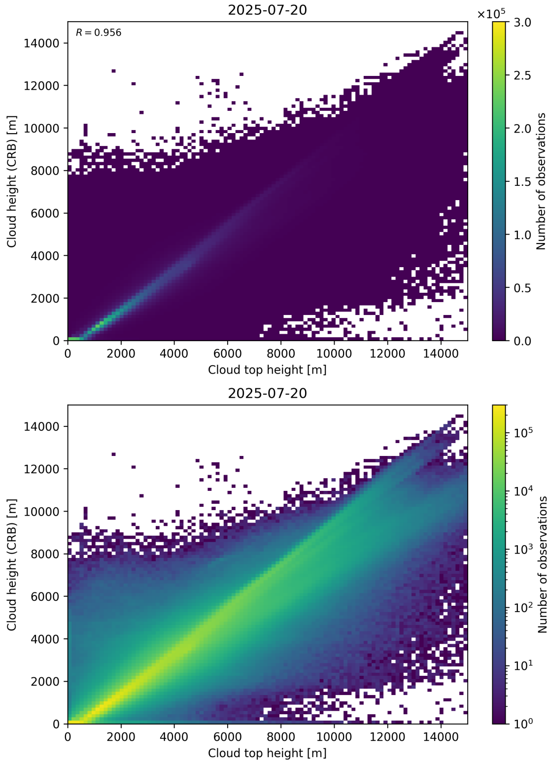
Figure 89: Scatter density plot of “Cloud top height” against “Cloud height (CRB)” for 2025-07-19 to 2025-07-21.
