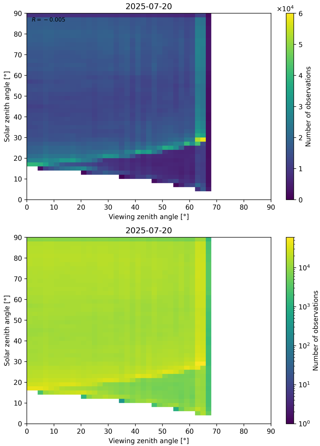
Figure 114: Scatter density plot of “Viewing zenith angle” against “Solar zenith angle” for 2025-07-19 to 2025-07-21.
