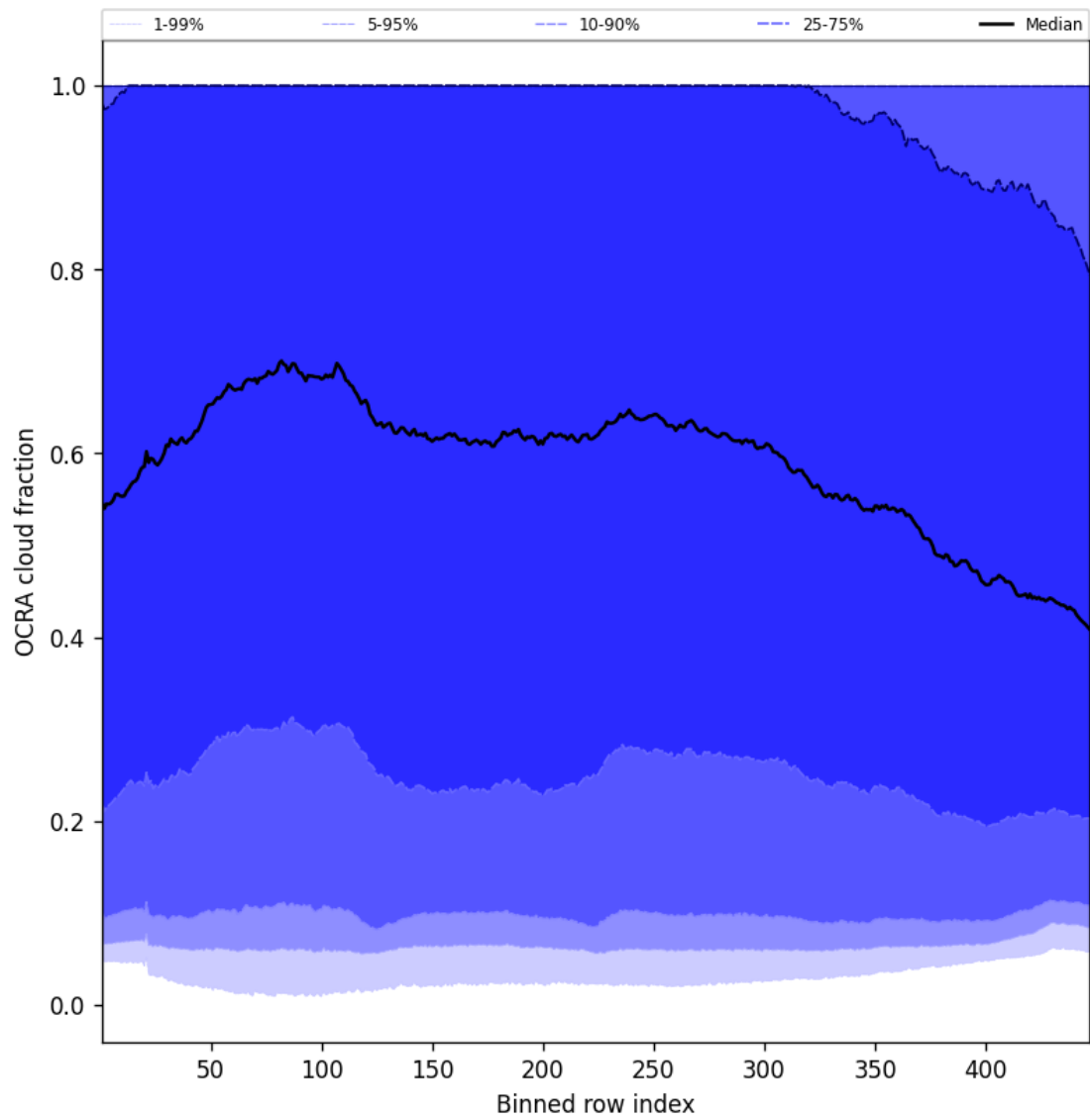
Figure 66: Along track statistics of “OCRA cloud fraction” for 2025-07-19 to 2025-07-21
