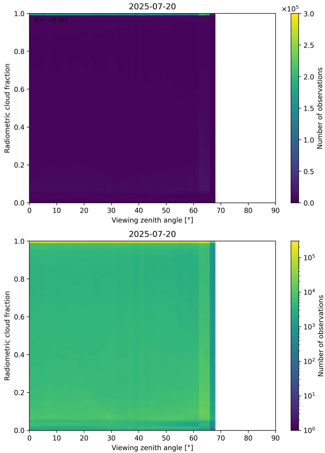
Figure 107: Scatter density plot of “Viewing zenith angle” against “Radiometric cloud fraction” for 2025-07-19 to 2025-07-21.
