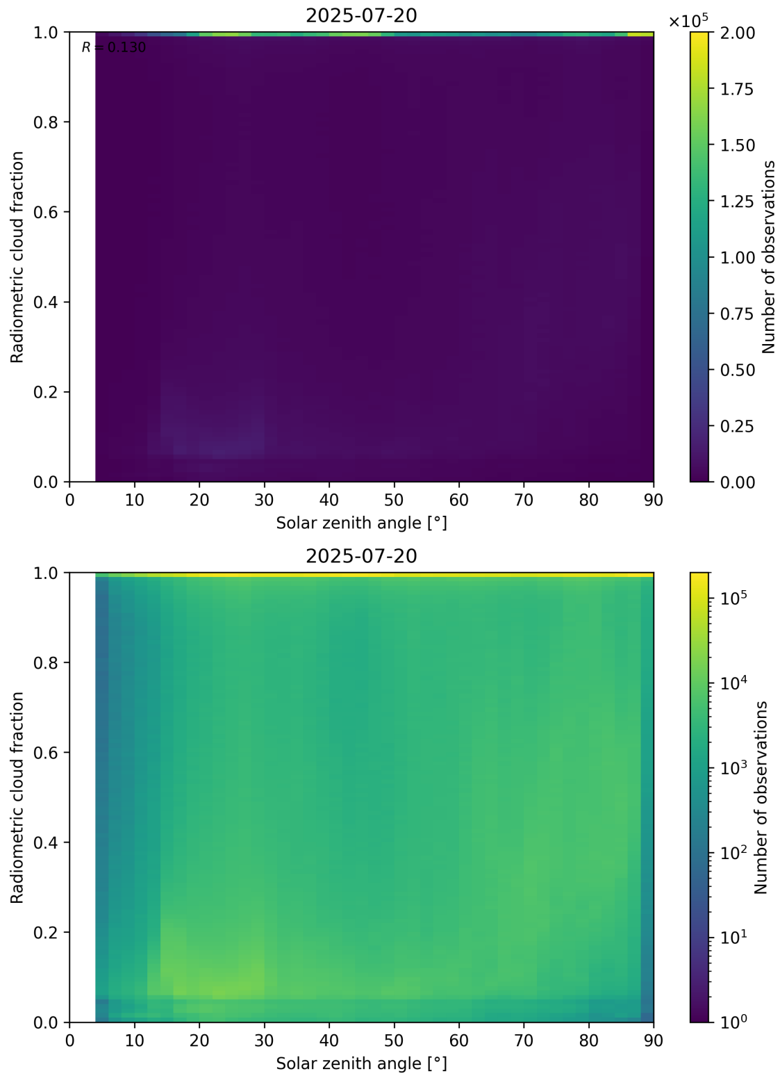
Figure 99: Scatter density plot of “Solar zenith angle” against “Radiometric cloud fraction” for 2025-07-19 to 2025-07-21.
