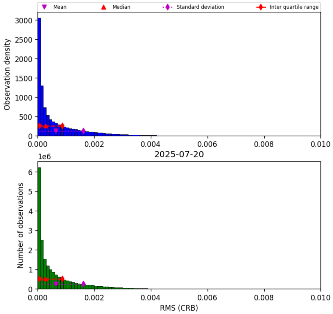
Figure 48: Histogram of “RMS (CRB)” for 2025-07-19 to 2025-07-21
