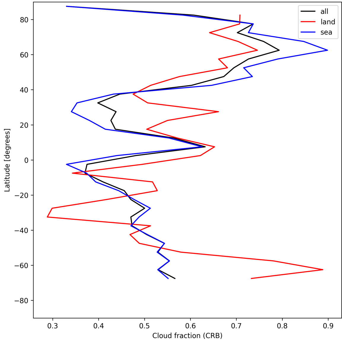
Figure 26: Zonal average of “Cloud fraction (CRB)” for 2025-07-19 to 2025-07-21.
