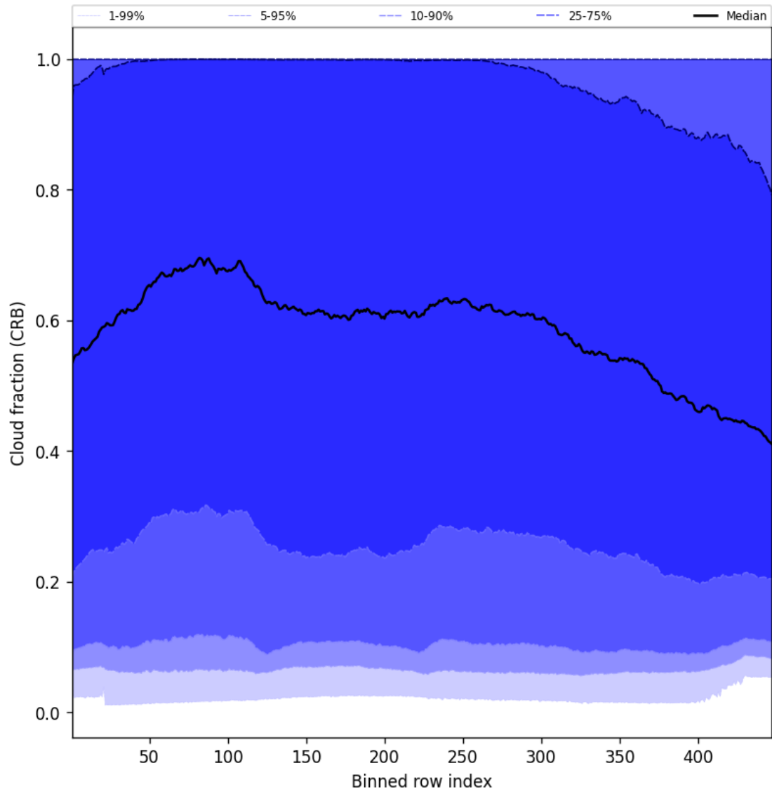
Figure 58: Along track statistics of “Cloud fraction (CRB)” for 2025-07-19 to 2025-07-21
