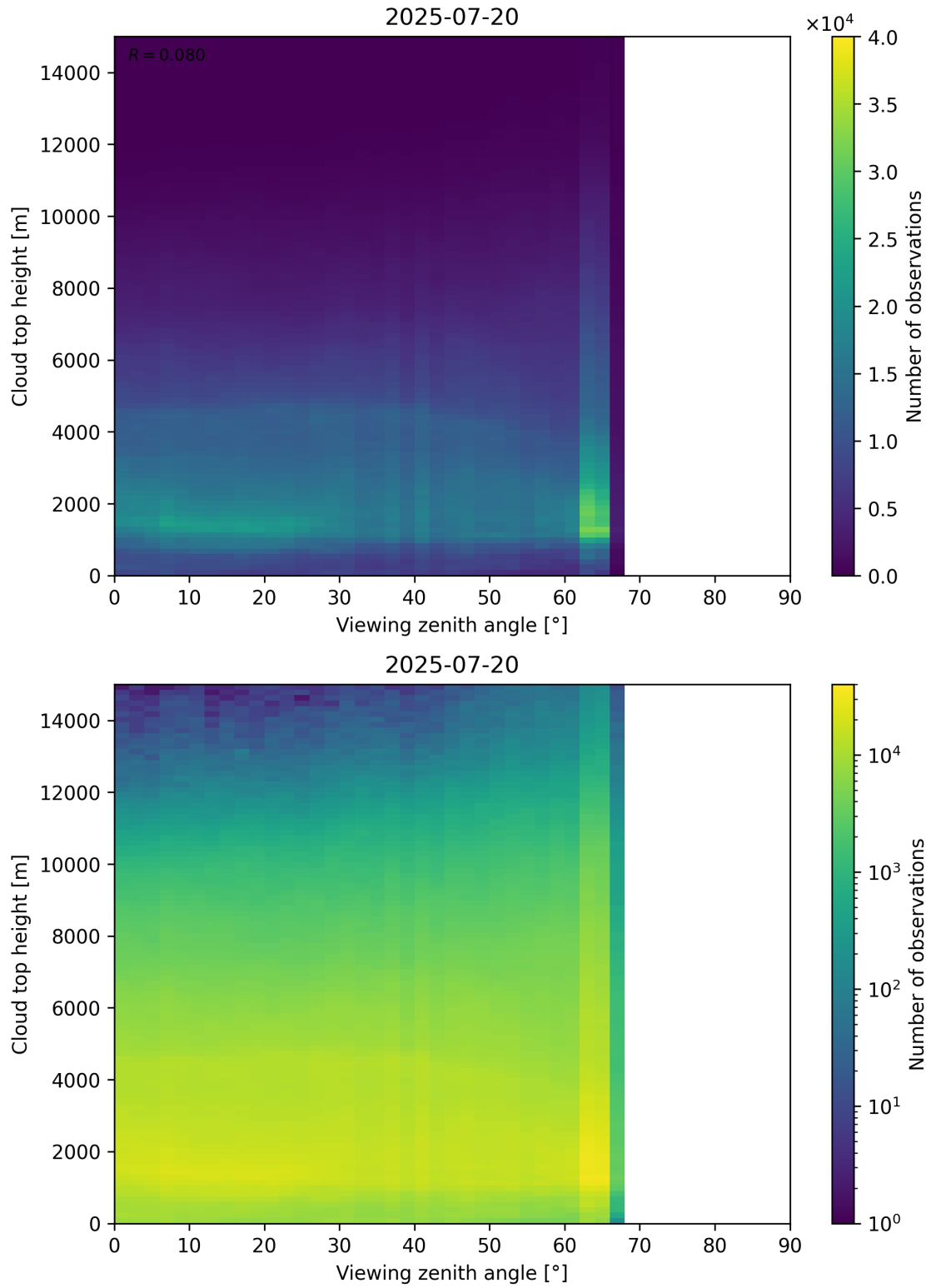
Figure 112: Scatter density plot of “Viewing zenith angle” against “Cloud top height” for 2025-07-19 to 2025-07-21.
