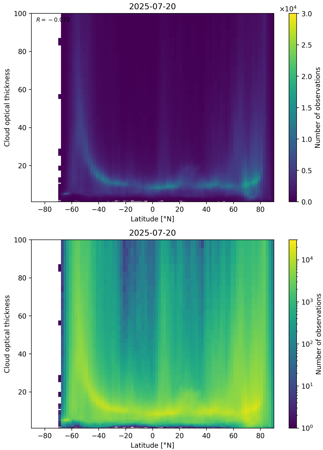
Figure 96: Scatter density plot of “Latitude” against “Cloud optical thickness” for 2025-07-19 to 2025-07-21.
