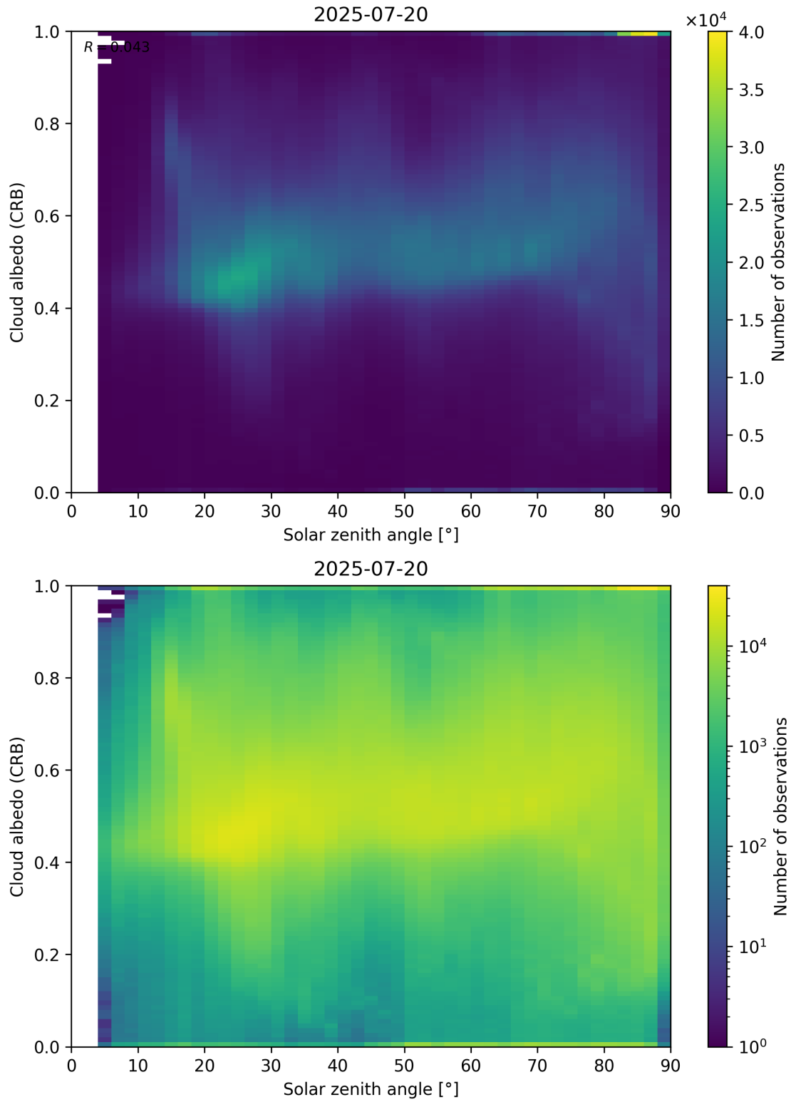
Figure 98: Scatter density plot of “Solar zenith angle” against “Cloud albedo (CRB)” for 2025-07-19 to 2025-07-21.
