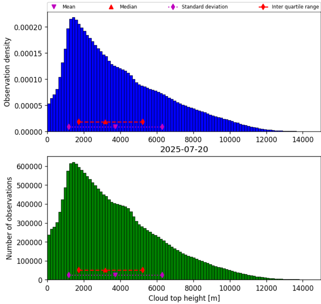
Figure 40: Histogram of “Cloud top height” for 2025-07-19 to 2025-07-21
