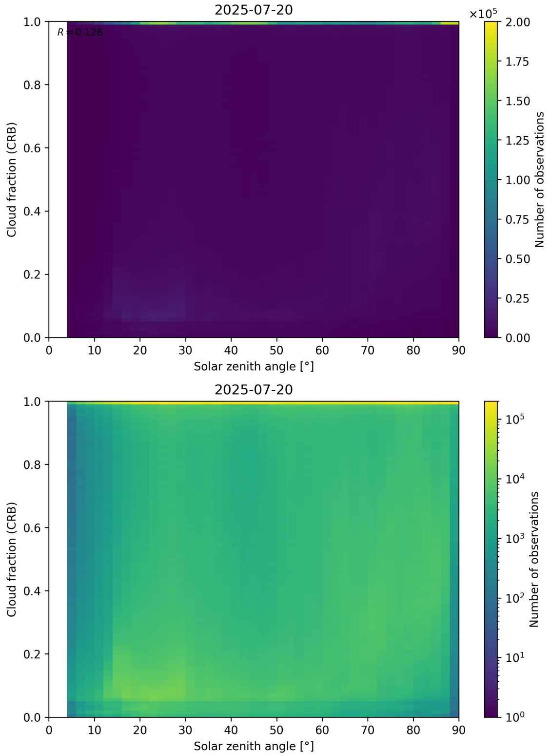
Figure 101: Scatter density plot of “Solar zenith angle” against “Cloud fraction (CRB)” for 2025-07-19 to 2025-07-21.
