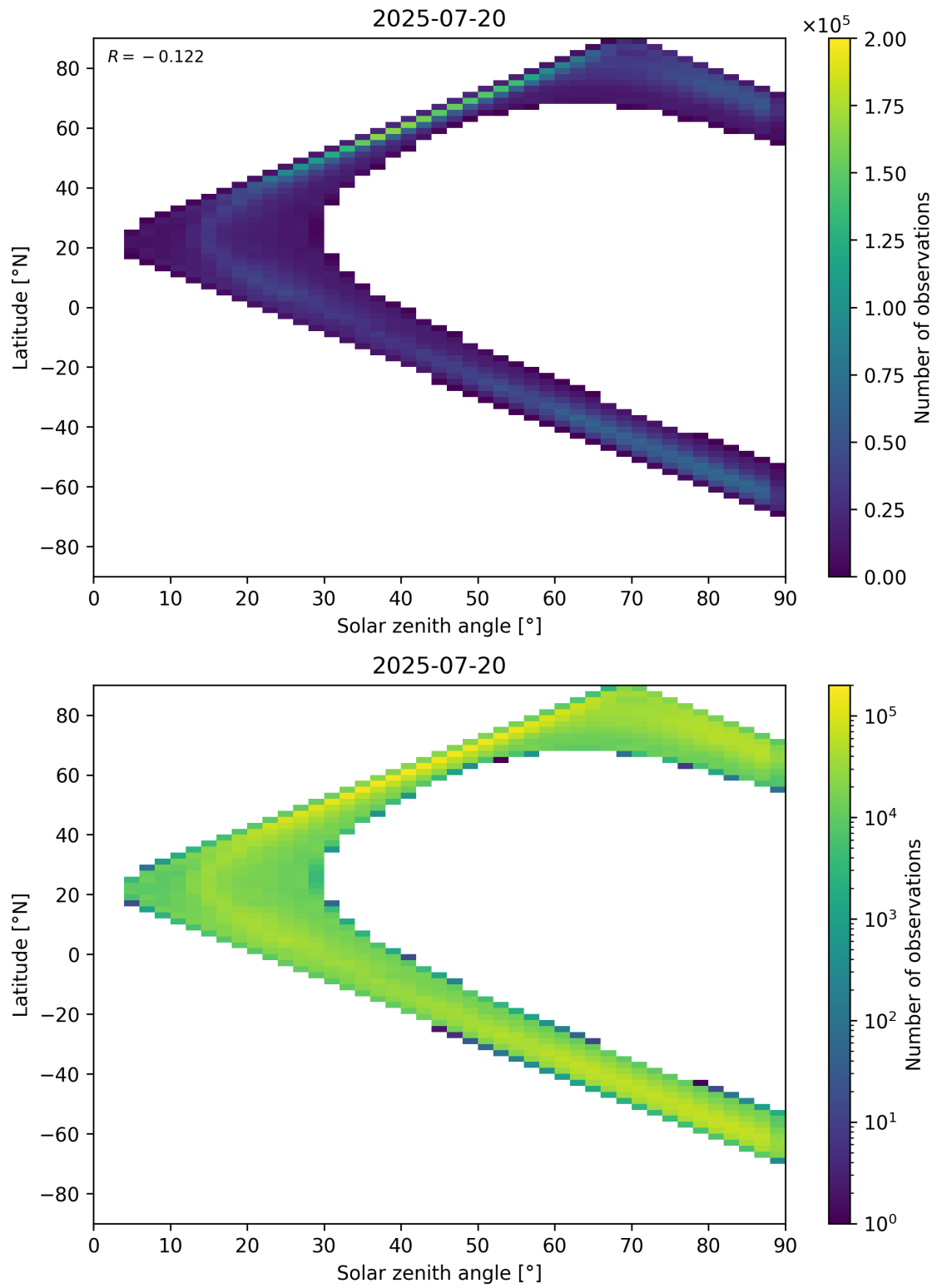
Figure 105: Scatter density plot of “Solar zenith angle” against “Latitude” for 2025-07-19 to 2025-07-21.
