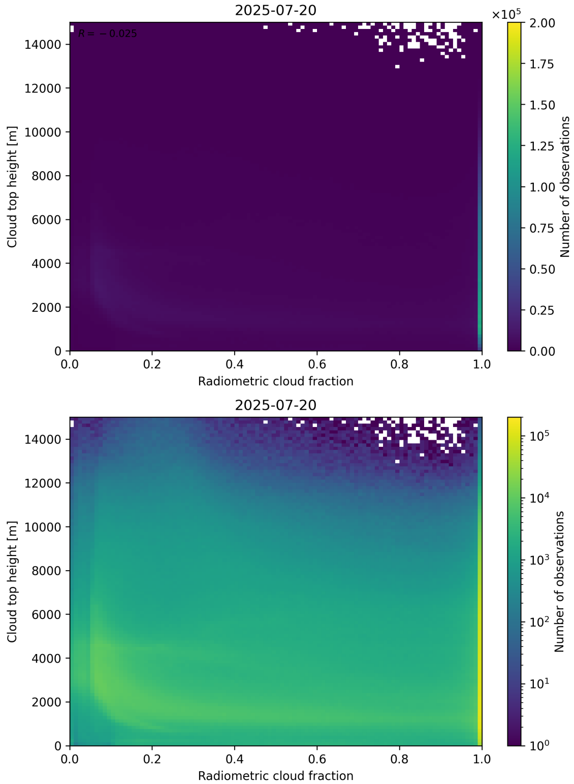
Figure 76: Scatter density plot of “Radiometric cloud fraction” against “Cloud top height” for 2025-07-19 to 2025-07-21.
