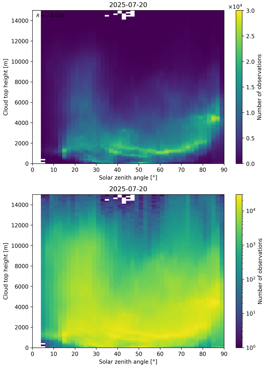
Figure 104: Scatter density plot of “Solar zenith angle” against “Cloud top height” for 2025-07-19 to 2025-07-21.
