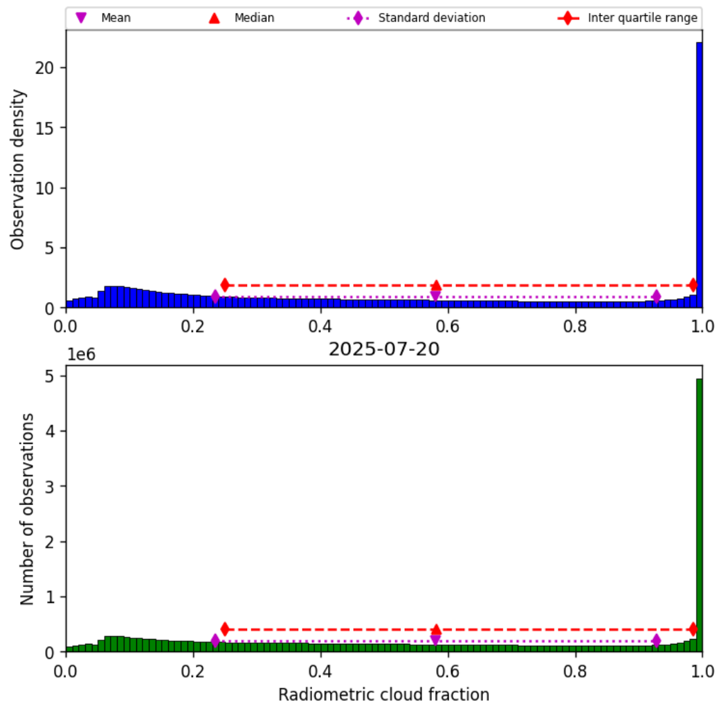
Figure 39: Histogram of “Radiometric cloud fraction” for 2025-07-19 to 2025-07-21
