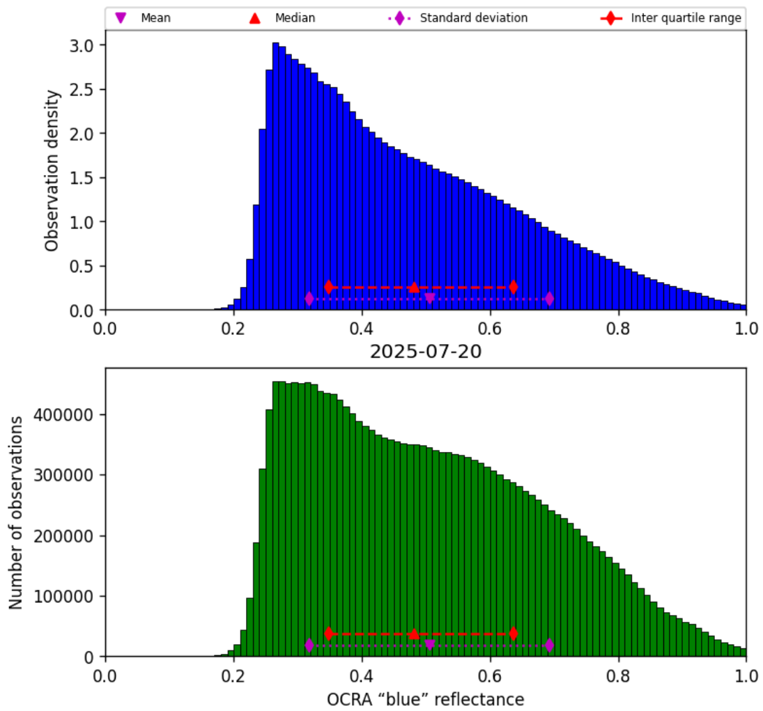
Figure 51: Histogram of “OCRA “blue” reflectance” for 2025-07-19 to 2025-07-21
