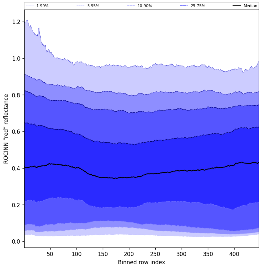
Figure 69: Along track statistics of “ROCINN “red” reflectance” for 2025-07-19 to 2025-07-21
