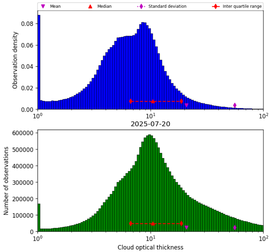
Figure 41: Histogram of “Cloud optical thickness” for 2025-07-19 to 2025-07-21
