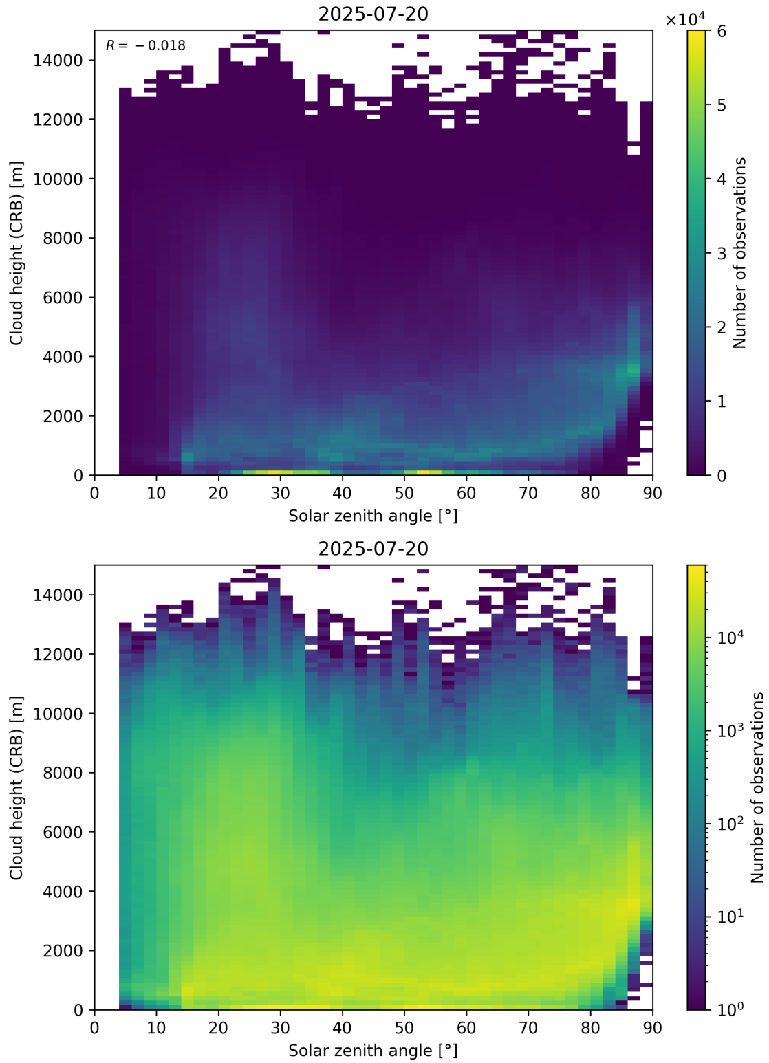
Figure 102: Scatter density plot of “Solar zenith angle” against “Cloud height (CRB)” for 2025-07-19 to 2025-07-21.
