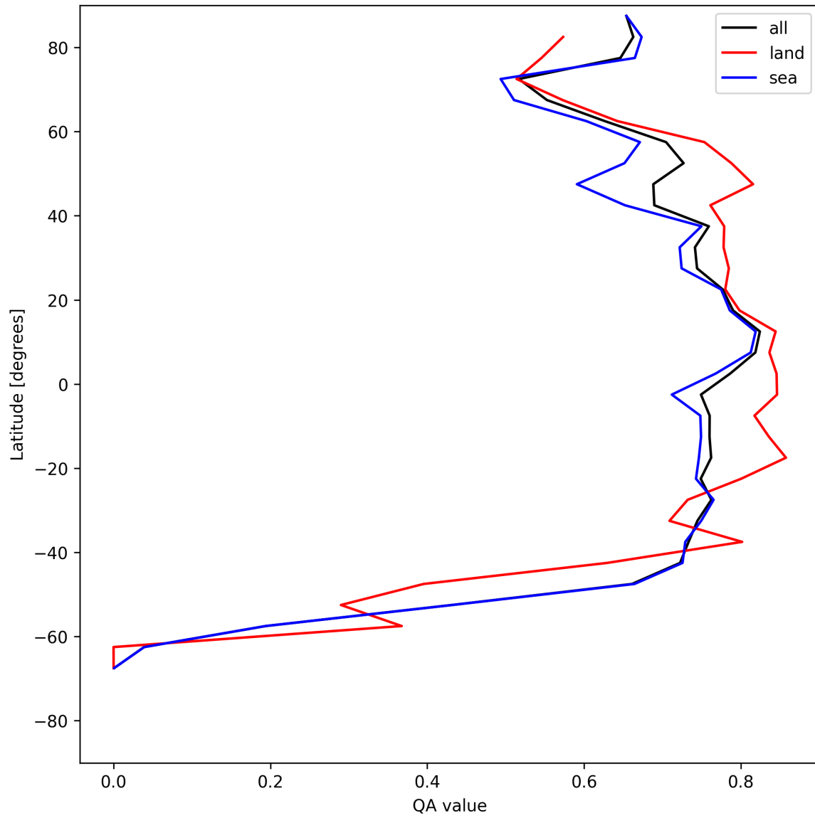
Figure 22: Zonal average of “QA value” for 2025-07-19 to 2025-07-21.
