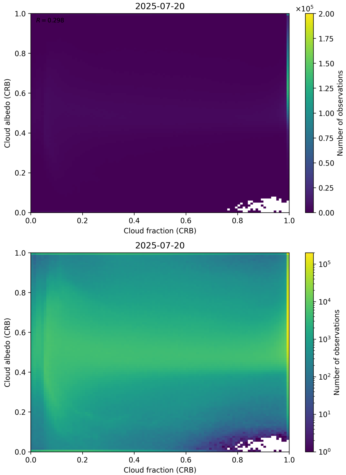
Figure 77: Scatter density plot of “Cloud fraction (CRB)” against “Cloud albedo (CRB)” for 2025-07-19 to 2025-07-21.
