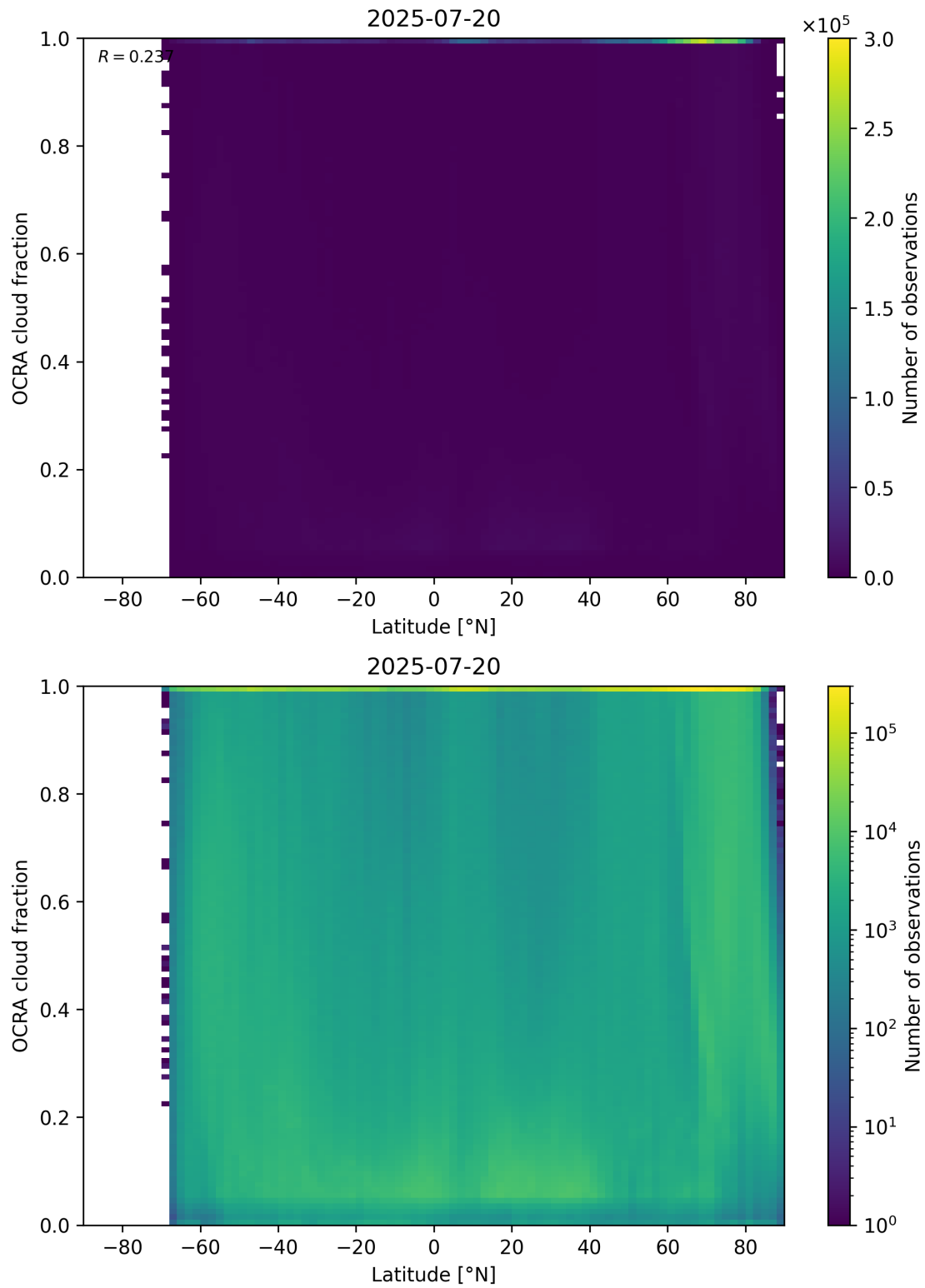
Figure 93: Scatter density plot of “Latitude” against “OCRA cloud fraction” for 2025-07-19 to 2025-07-21.
