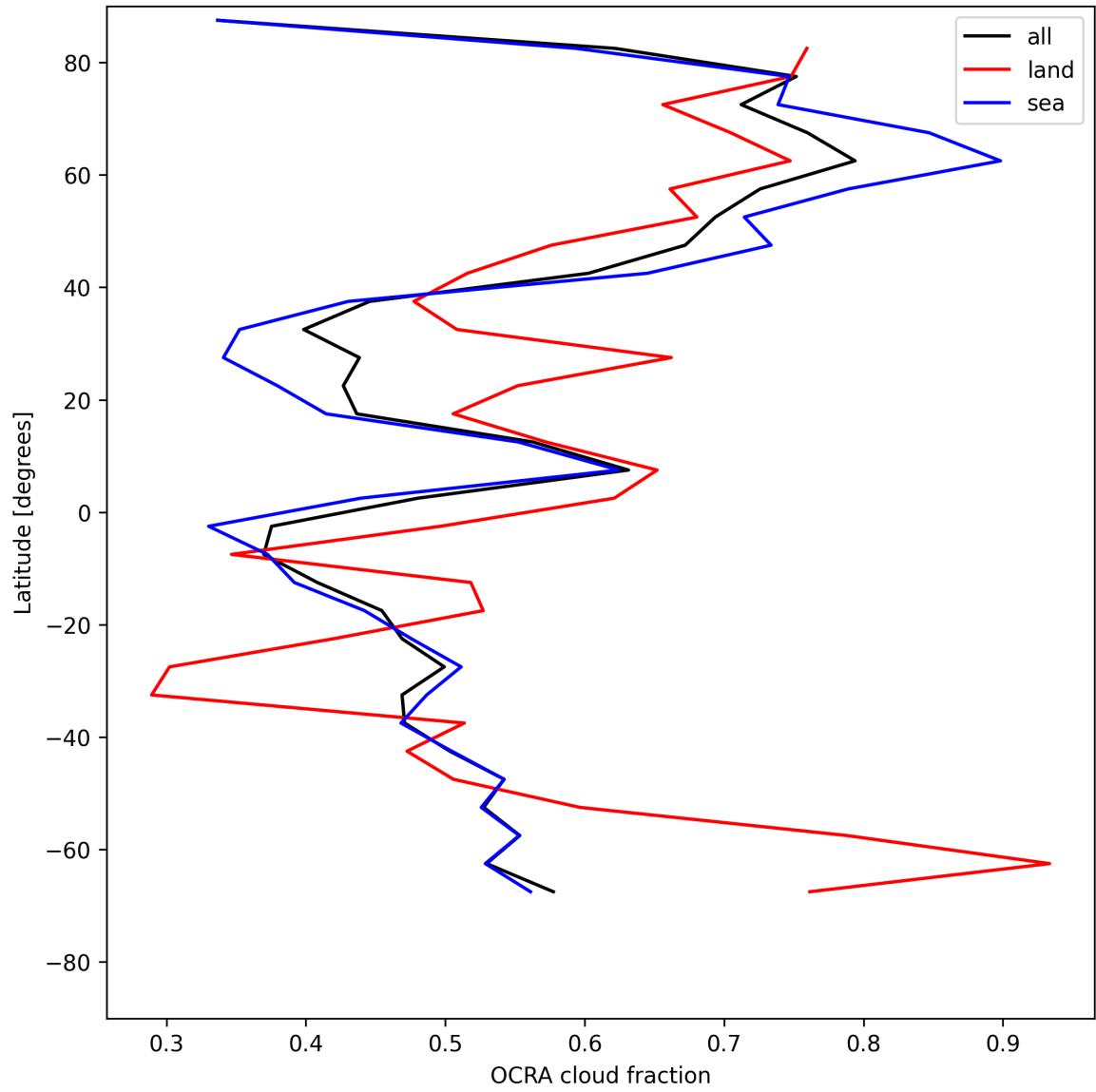
Figure 34: Zonal average of “OCRA cloud fraction” for 2025-07-19 to 2025-07-21.
