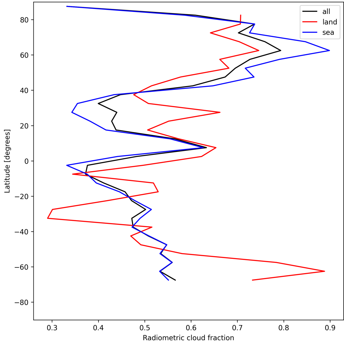
Figure 23: Zonal average of “Radiometric cloud fraction” for 2025-07-19 to 2025-07-21.
