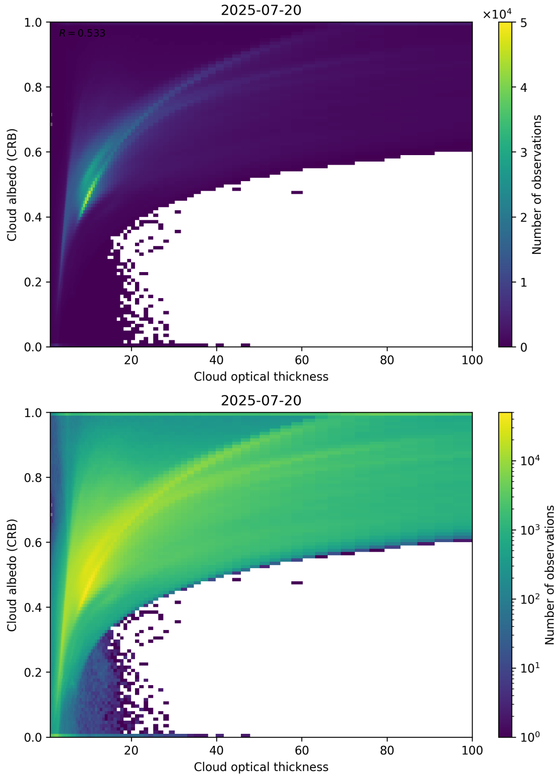
Figure 82: Scatter density plot of “Cloud optical thickness” against “Cloud albedo (CRB)” for 2025-07-19 to 2025-07-21.
