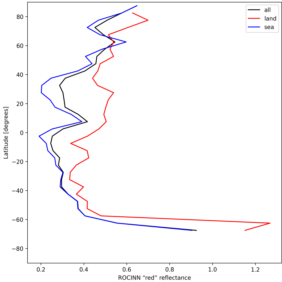
Figure 37: Zonal average of “ROCINN “red” reflectance” for 2025-07-19 to 2025-07-21.
