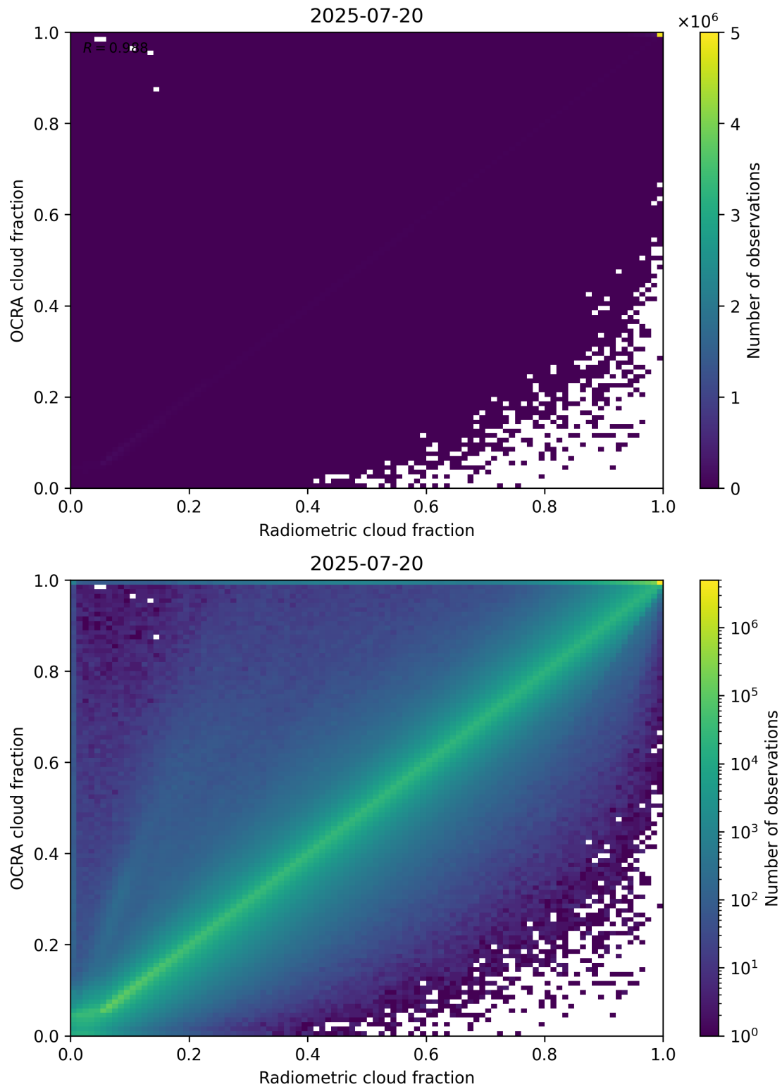
Figure 72: Scatter density plot of “Radiometric cloud fraction” against “OCRA cloud fraction” for 2025-07-19 to 2025-07-21.
