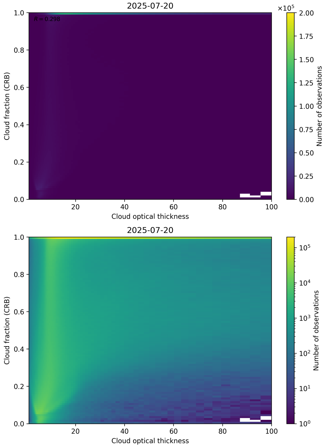
Figure 84: Scatter density plot of “Cloud optical thickness” against “Cloud fraction (CRB)” for 2025-07-19 to 2025-07-21.
