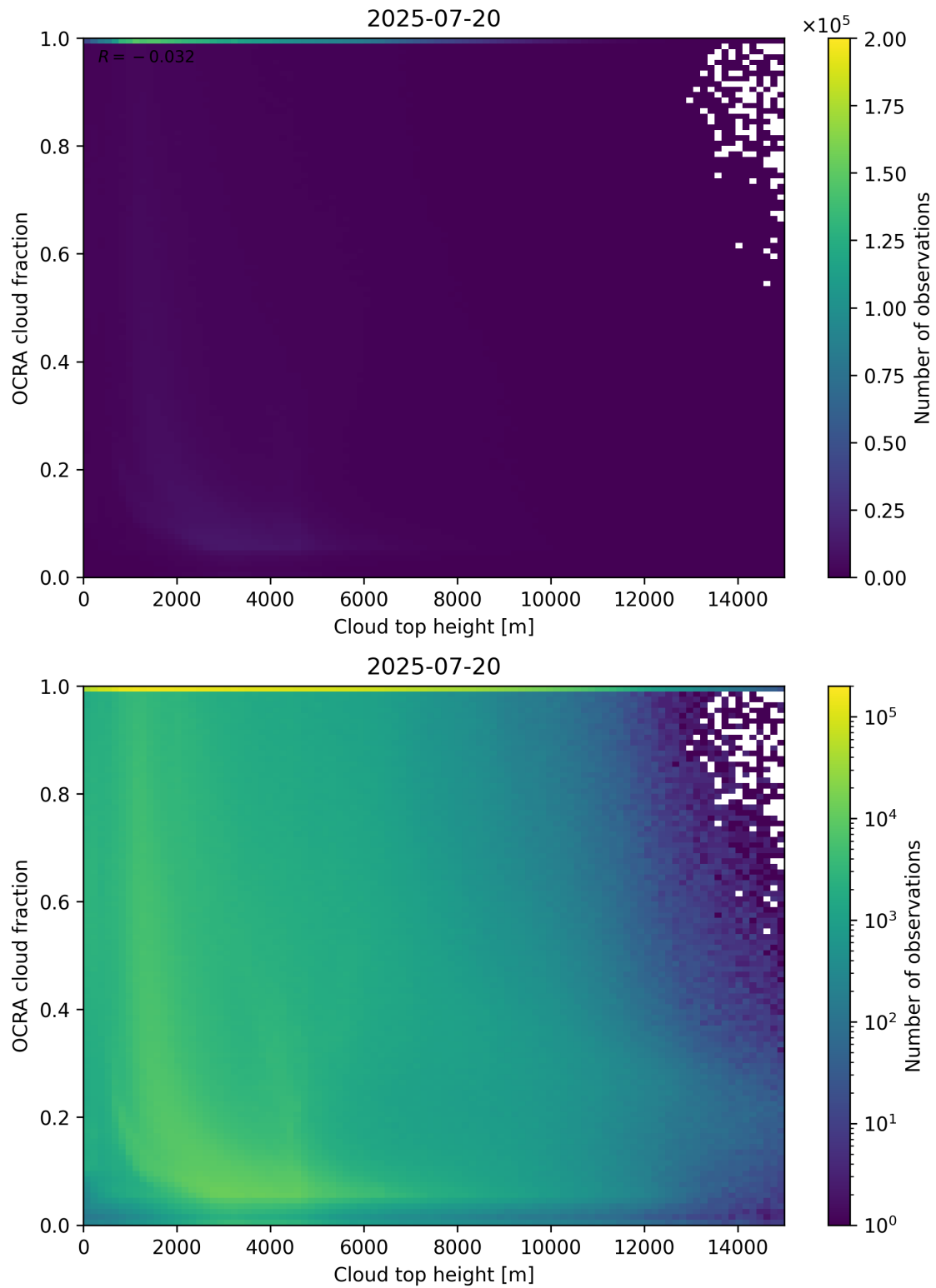
Figure 87: Scatter density plot of “Cloud top height” against “OCRA cloud fraction” for 2025-07-19 to 2025-07-21.
