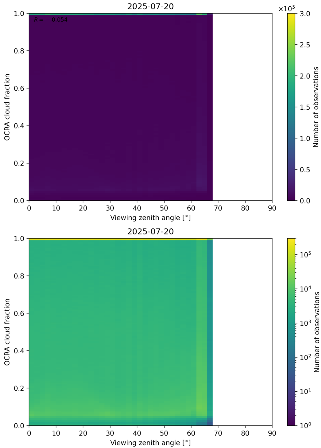
Figure 108: Scatter density plot of “Viewing zenith angle” against “OCRA cloud fraction” for 2025-07-19 to 2025-07-21.
