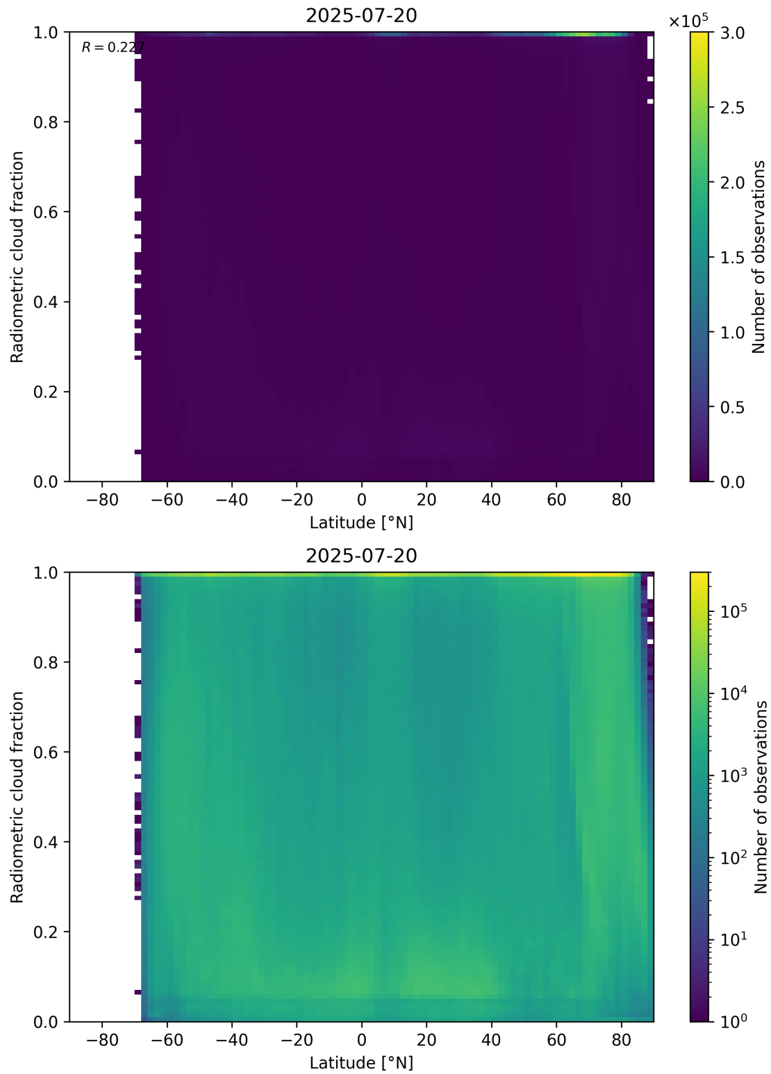
Figure 92: Scatter density plot of “Latitude” against “Radiometric cloud fraction” for 2025-07-19 to 2025-07-21.
