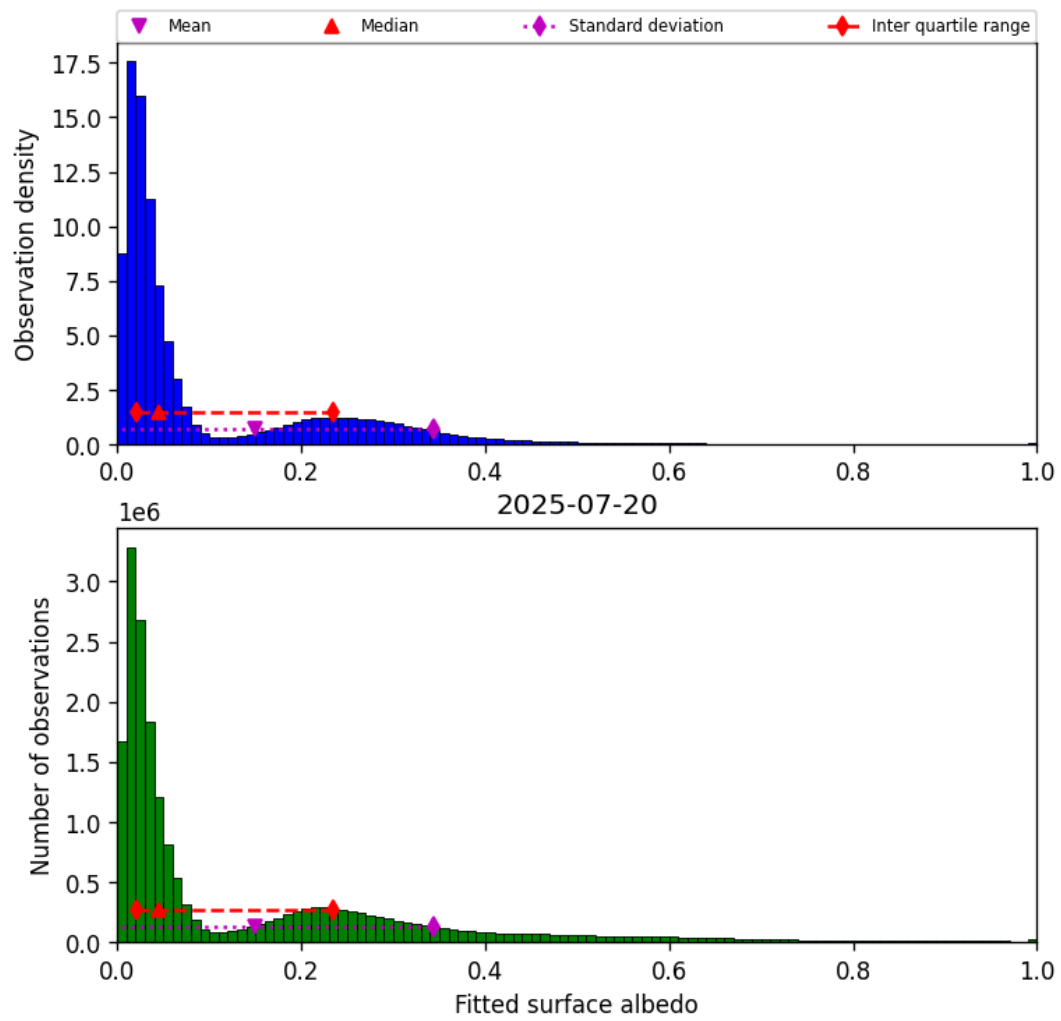
Figure 45: Histogram of “Fitted surface albedo” for 2025-07-19 to 2025-07-21
