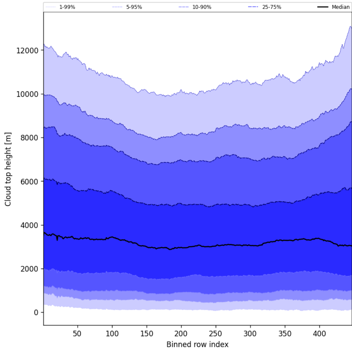
Figure 56: Along track statistics of “Cloud top height” for 2025-07-19 to 2025-07-21
