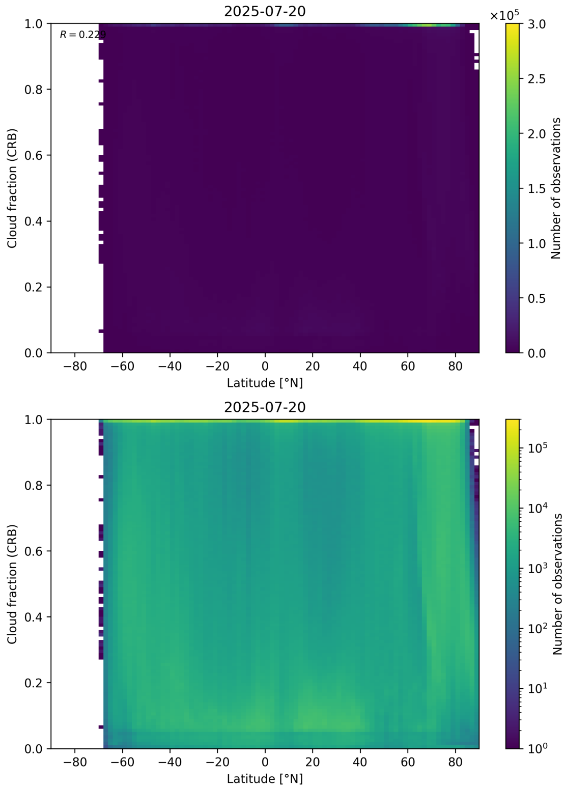
Figure 94: Scatter density plot of “Latitude” against “Cloud fraction (CRB)” for 2025-07-19 to 2025-07-21.
