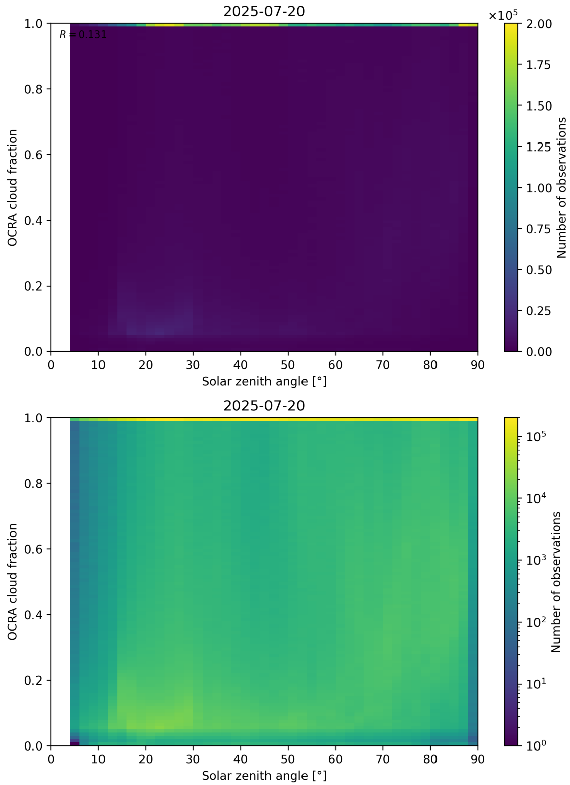
Figure 100: Scatter density plot of “Solar zenith angle” against “OCRA cloud fraction” for 2025-07-19 to 2025-07-21.
