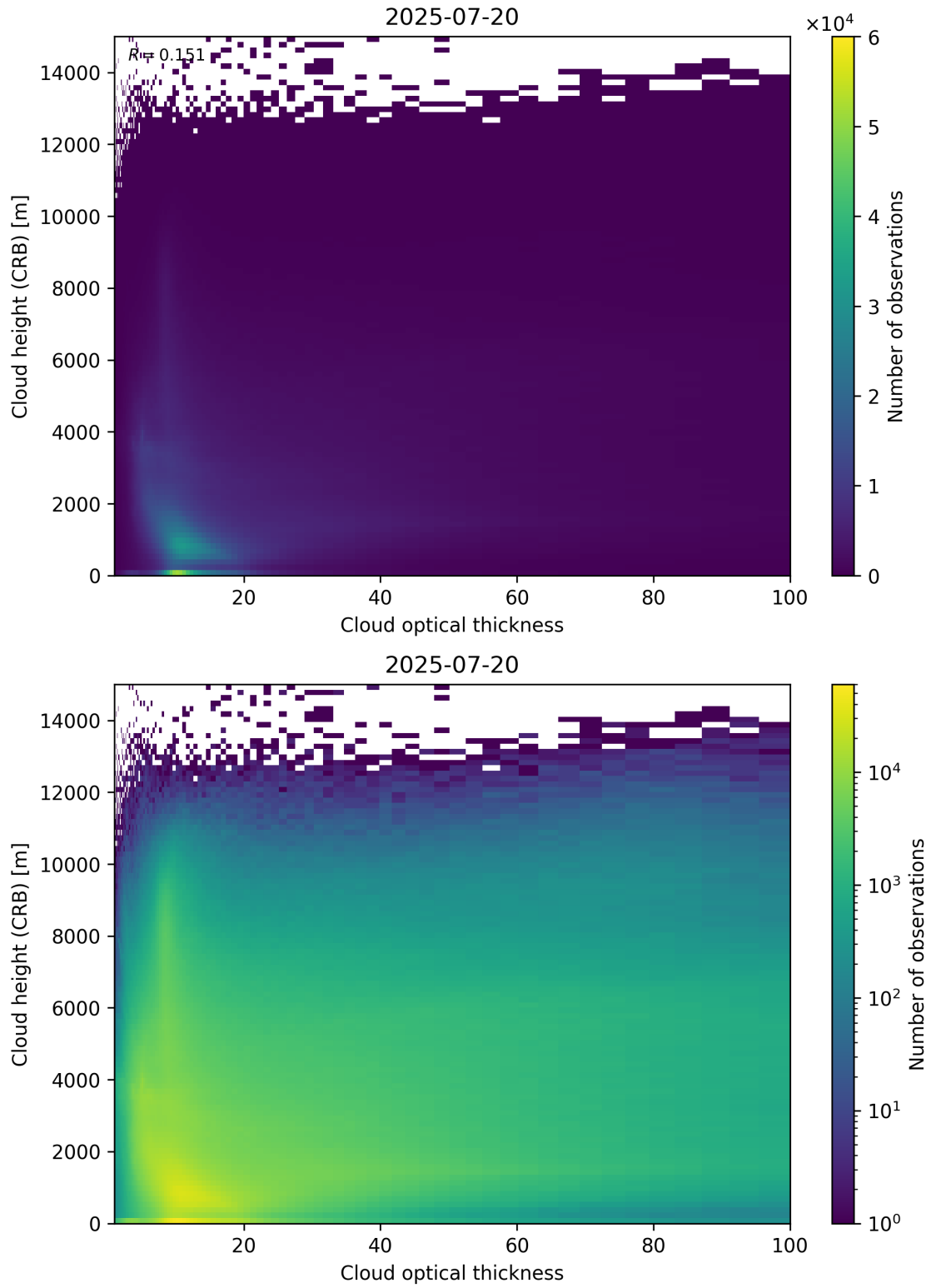
Figure 85: Scatter density plot of “Cloud optical thickness” against “Cloud height (CRB)” for 2025-07-19 to 2025-07-21.
