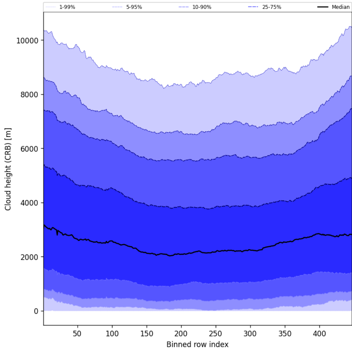
Figure 59: Along track statistics of “Cloud height (CRB)” for 2025-07-19 to 2025-07-21
