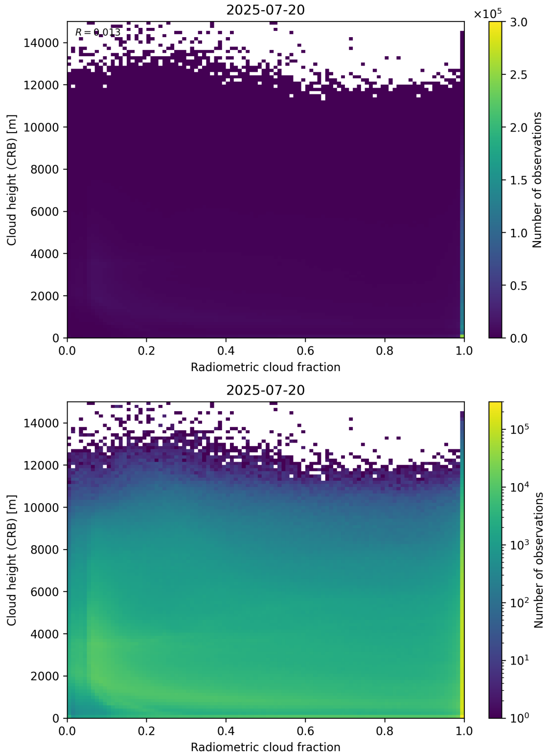
Figure 74: Scatter density plot of “Radiometric cloud fraction” against “Cloud height (CRB)” for 2025-07-19 to 2025-07-21.
