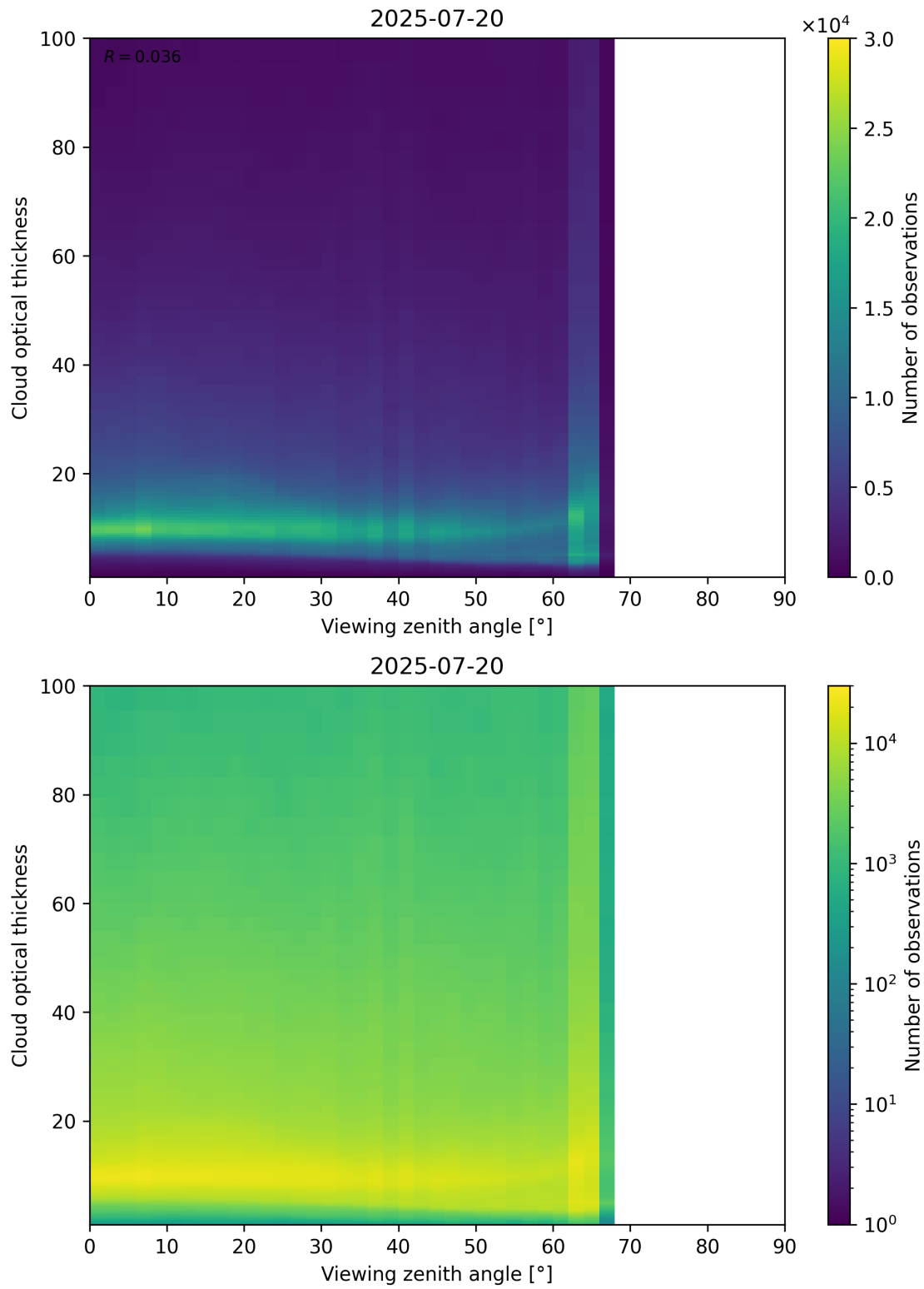
Figure 111: Scatter density plot of “Viewing zenith angle” against “Cloud optical thickness” for 2025-07-19 to 2025-07-21.
