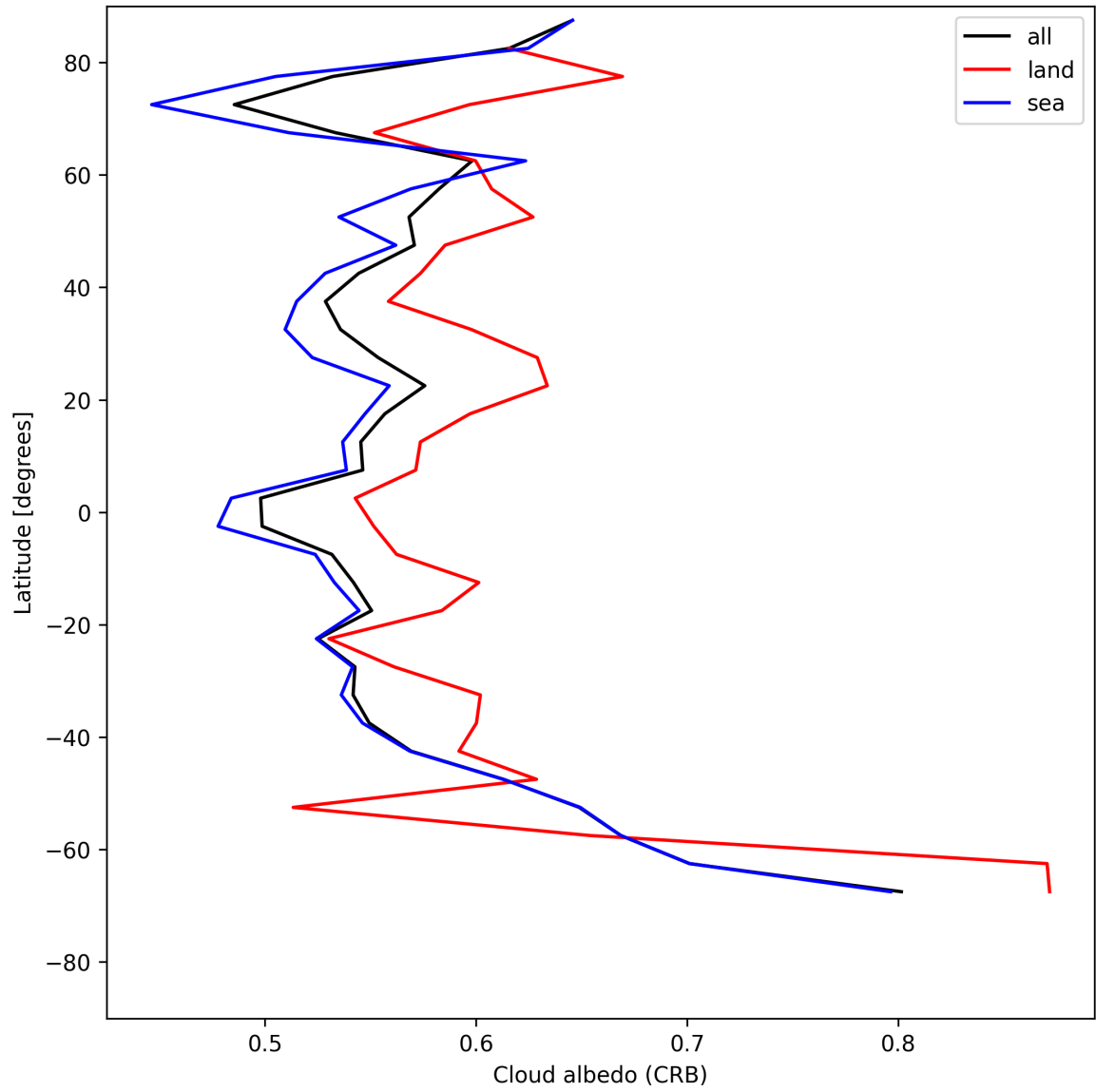
Figure 28: Zonal average of “Cloud albedo (CRB)” for 2025-07-19 to 2025-07-21.
