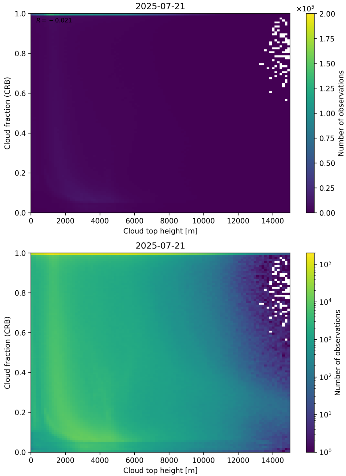
Figure 88: Scatter density plot of “Cloud top height” against “Cloud fraction (CRB)” for 2025-07-20 to 2025-07-22.
