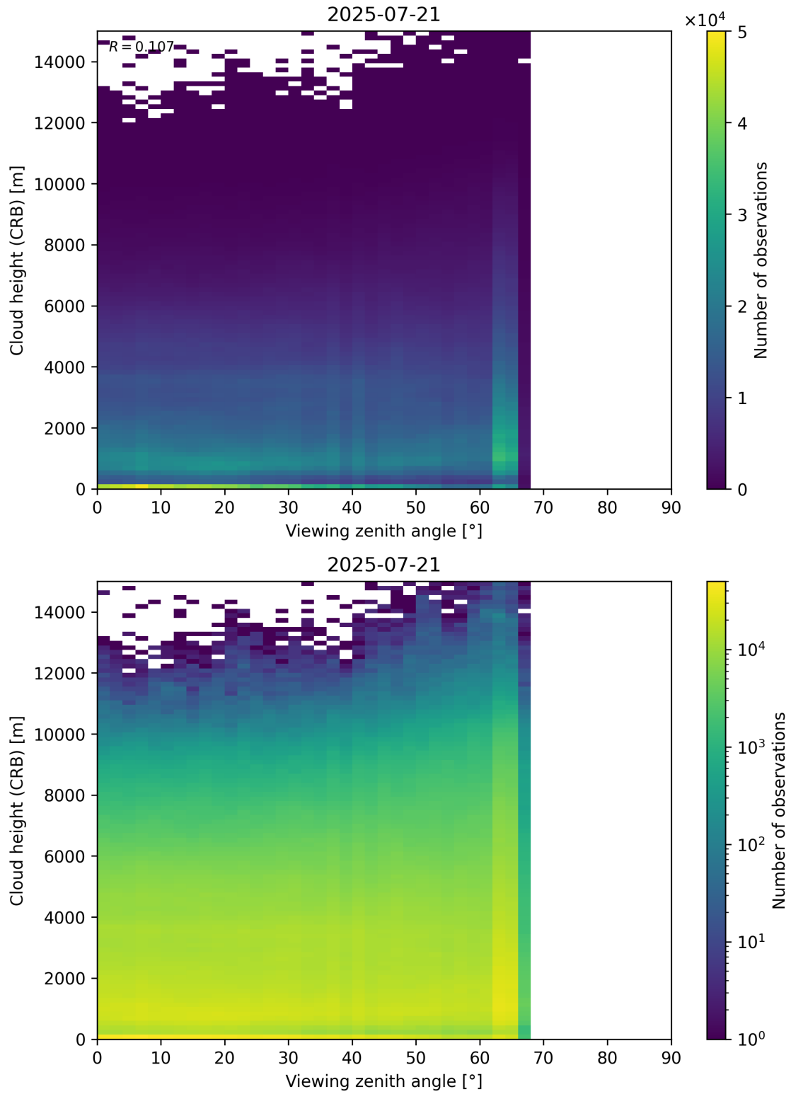
Figure 110: Scatter density plot of “Viewing zenith angle” against “Cloud height (CRB)” for 2025-07-20 to 2025-07-22.
