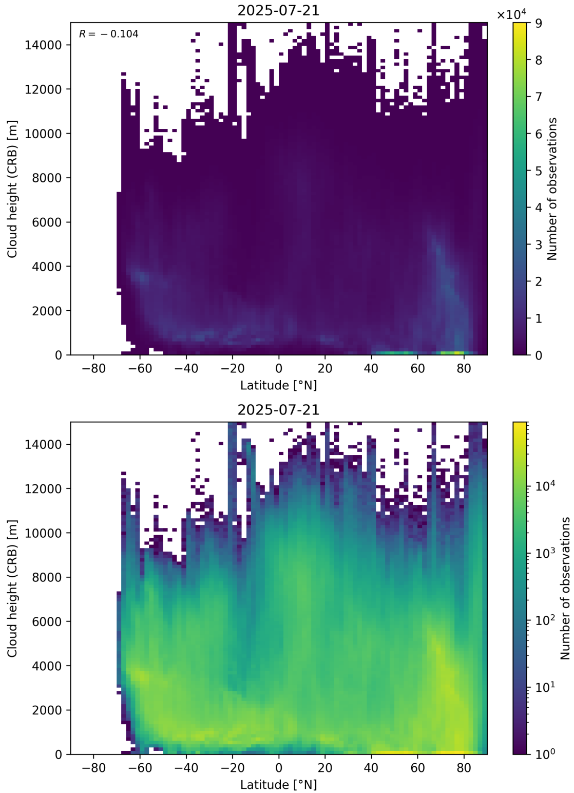
Figure 95: Scatter density plot of “Latitude” against “Cloud height (CRB)” for 2025-07-20 to 2025-07-22.
