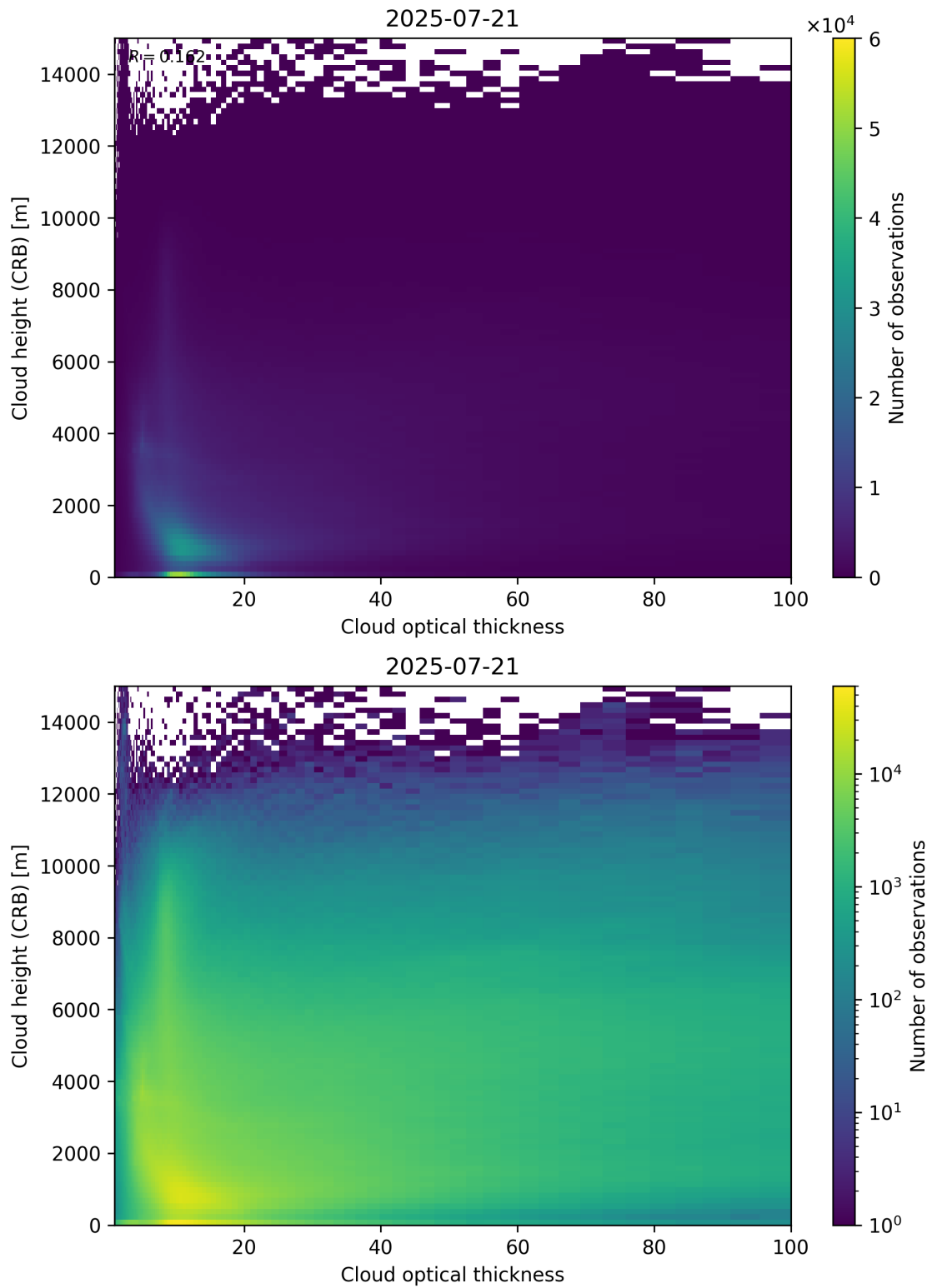
Figure 85: Scatter density plot of “Cloud optical thickness” against “Cloud height (CRB)” for 2025-07-20 to 2025-07-22.
