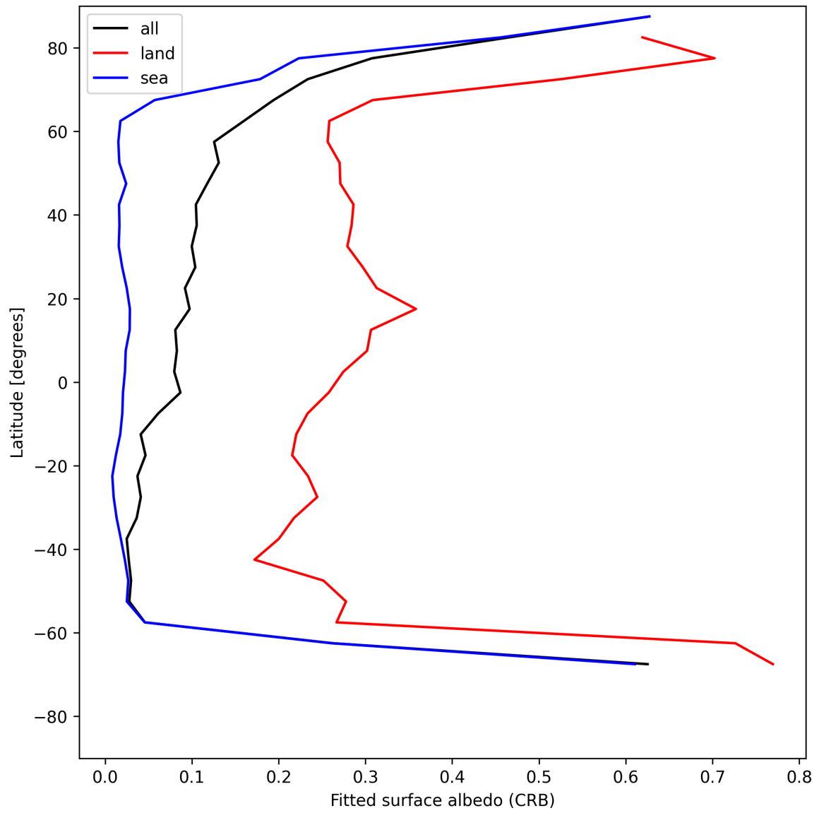
Figure 30: Zonal average of “Fitted surface albedo (CRB)” for 2025-07-20 to 2025-07-22.
