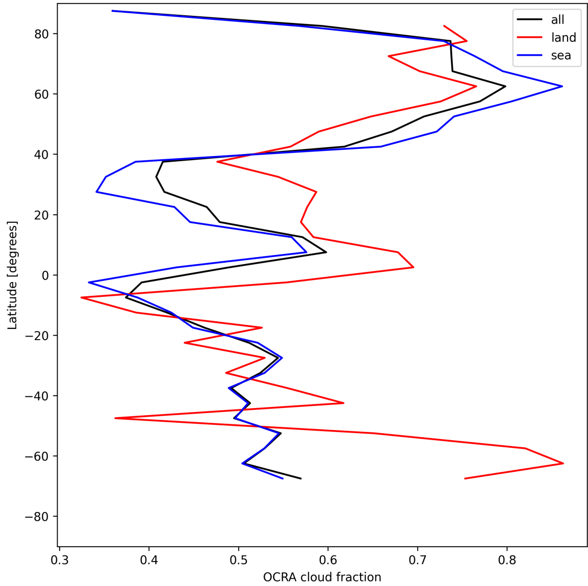
Figure 34: Zonal average of “OCRA cloud fraction” for 2025-07-20 to 2025-07-22.
