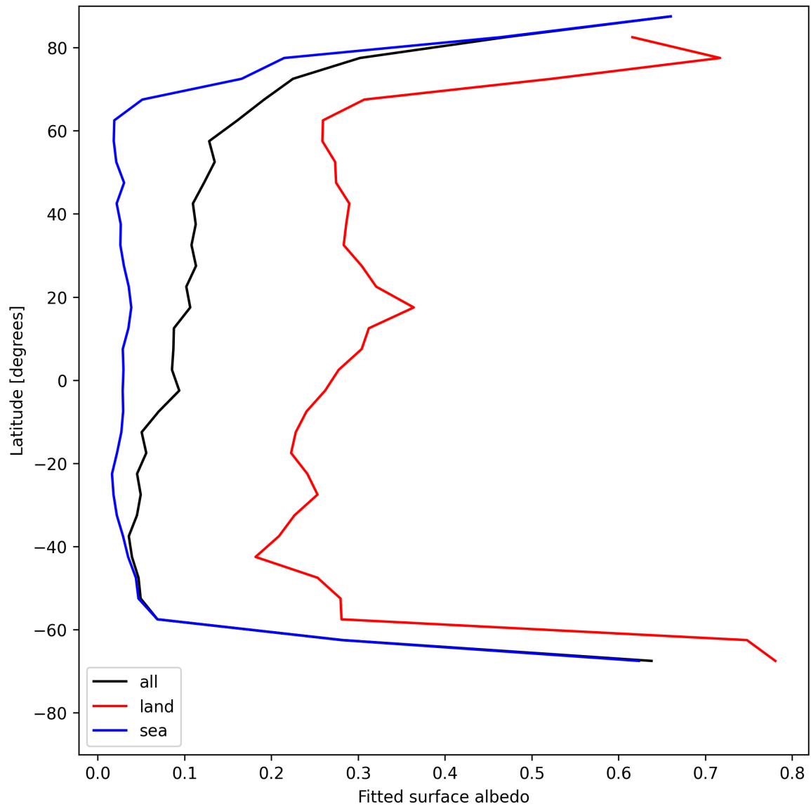
Figure 29: Zonal average of “Fitted surface albedo” for 2025-07-20 to 2025-07-22.
