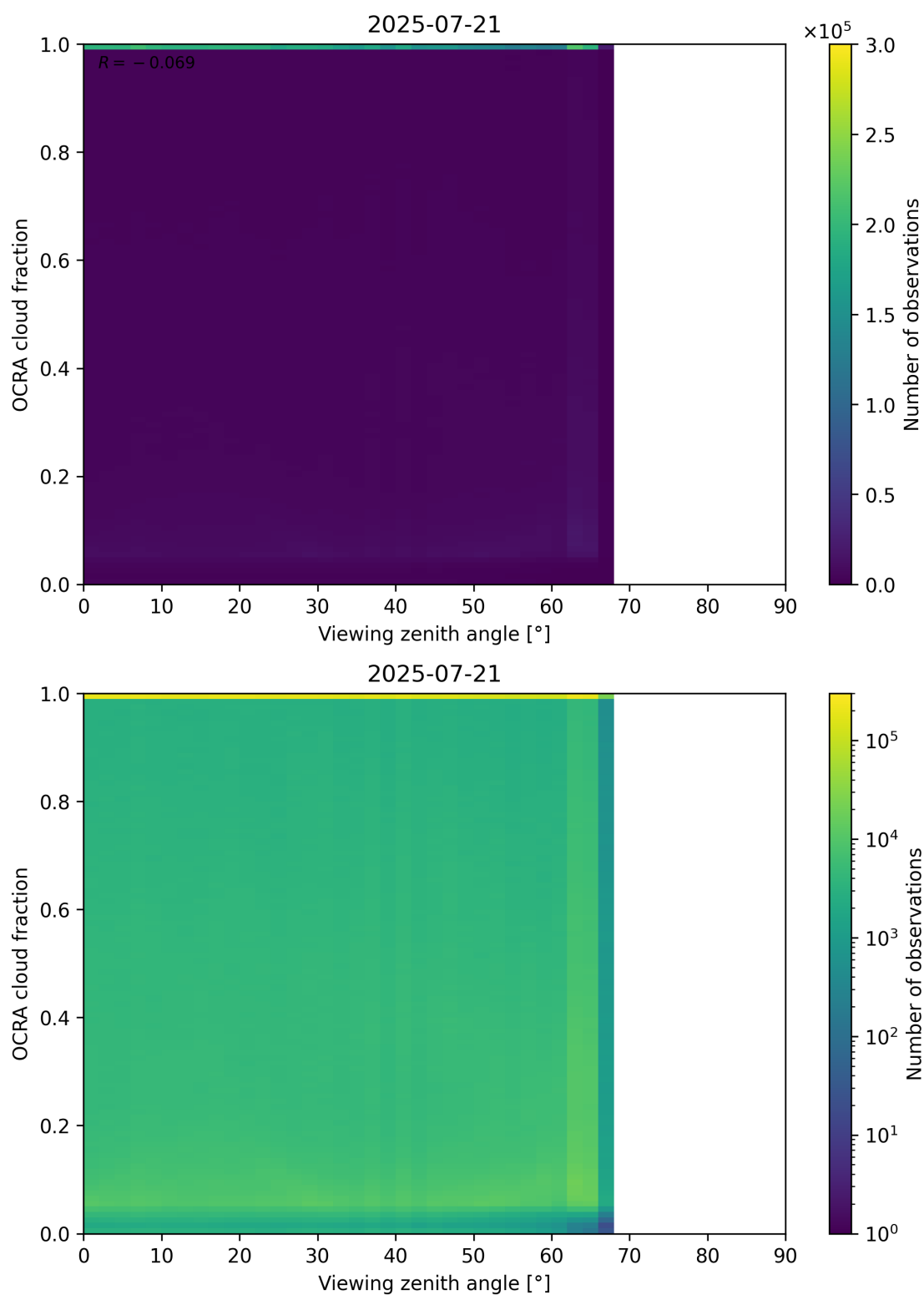
Figure 108: Scatter density plot of “Viewing zenith angle” against “OCRA cloud fraction” for 2025-07-20 to 2025-07-22.
