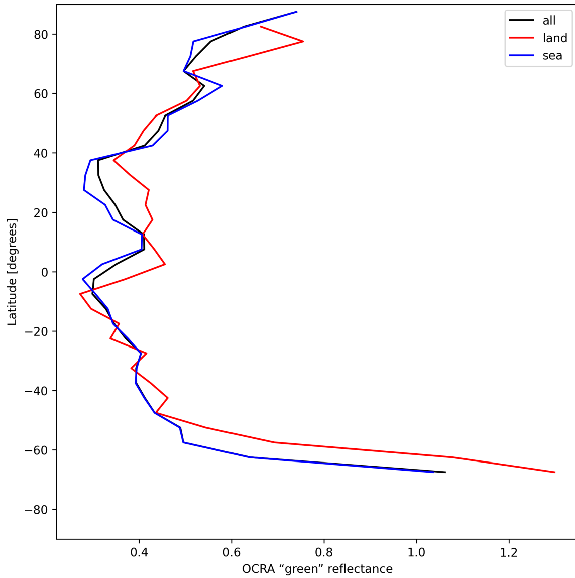
Figure 36: Zonal average of “OCRA “green” reflectance” for 2025-07-20 to 2025-07-22.
