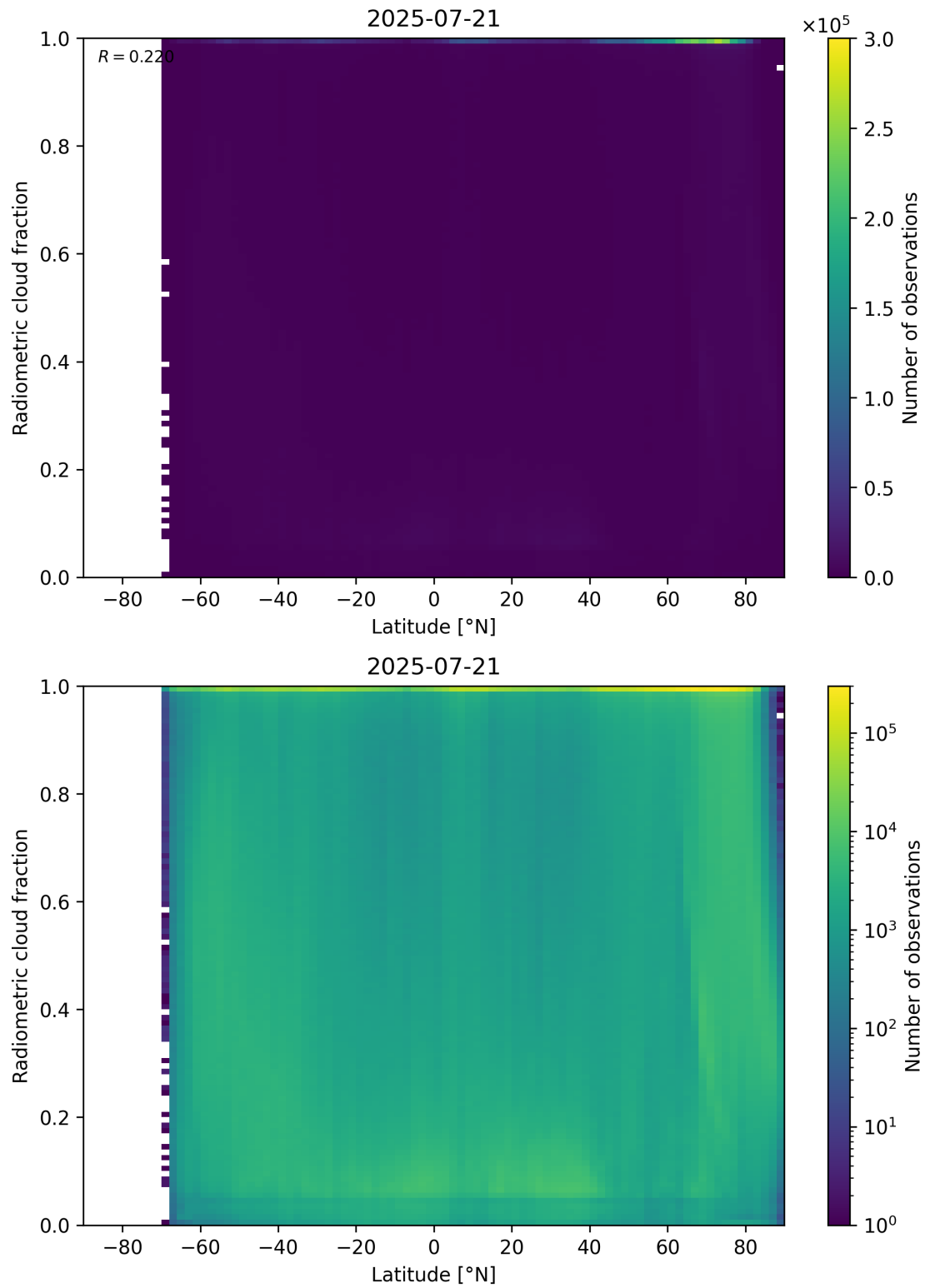
Figure 92: Scatter density plot of “Latitude” against “Radiometric cloud fraction” for 2025-07-20 to 2025-07-22.
