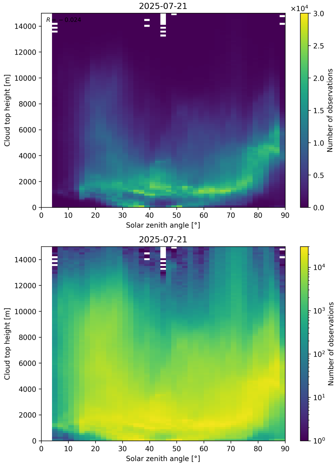
Figure 104: Scatter density plot of “Solar zenith angle” against “Cloud top height” for 2025-07-20 to 2025-07-22.
