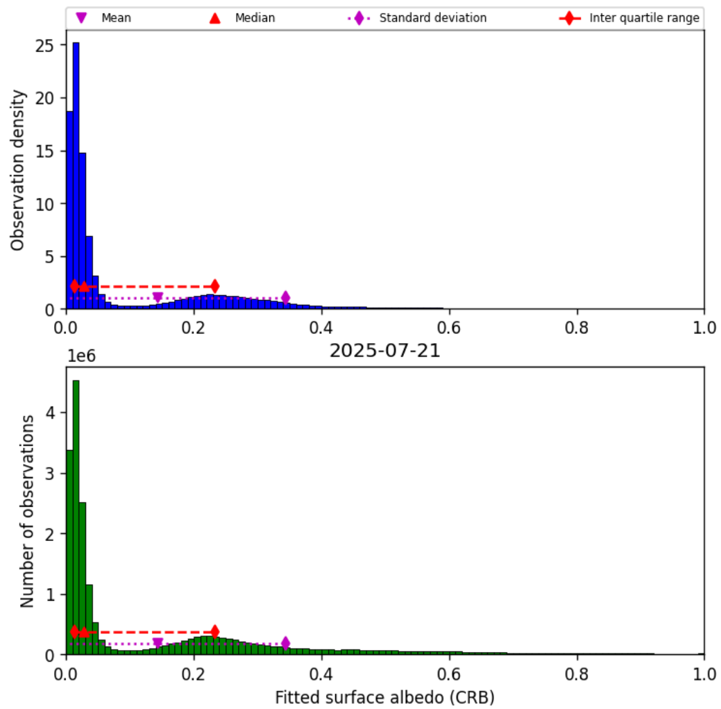
Figure 46: Histogram of “Fitted surface albedo (CRB)” for 2025-07-20 to 2025-07-22
