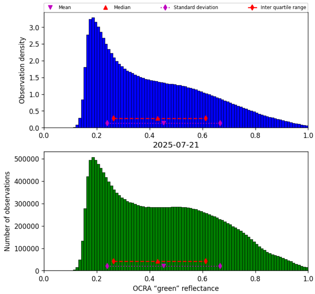
Figure 52: Histogram of “OCRA “green” reflectance” for 2025-07-20 to 2025-07-22
