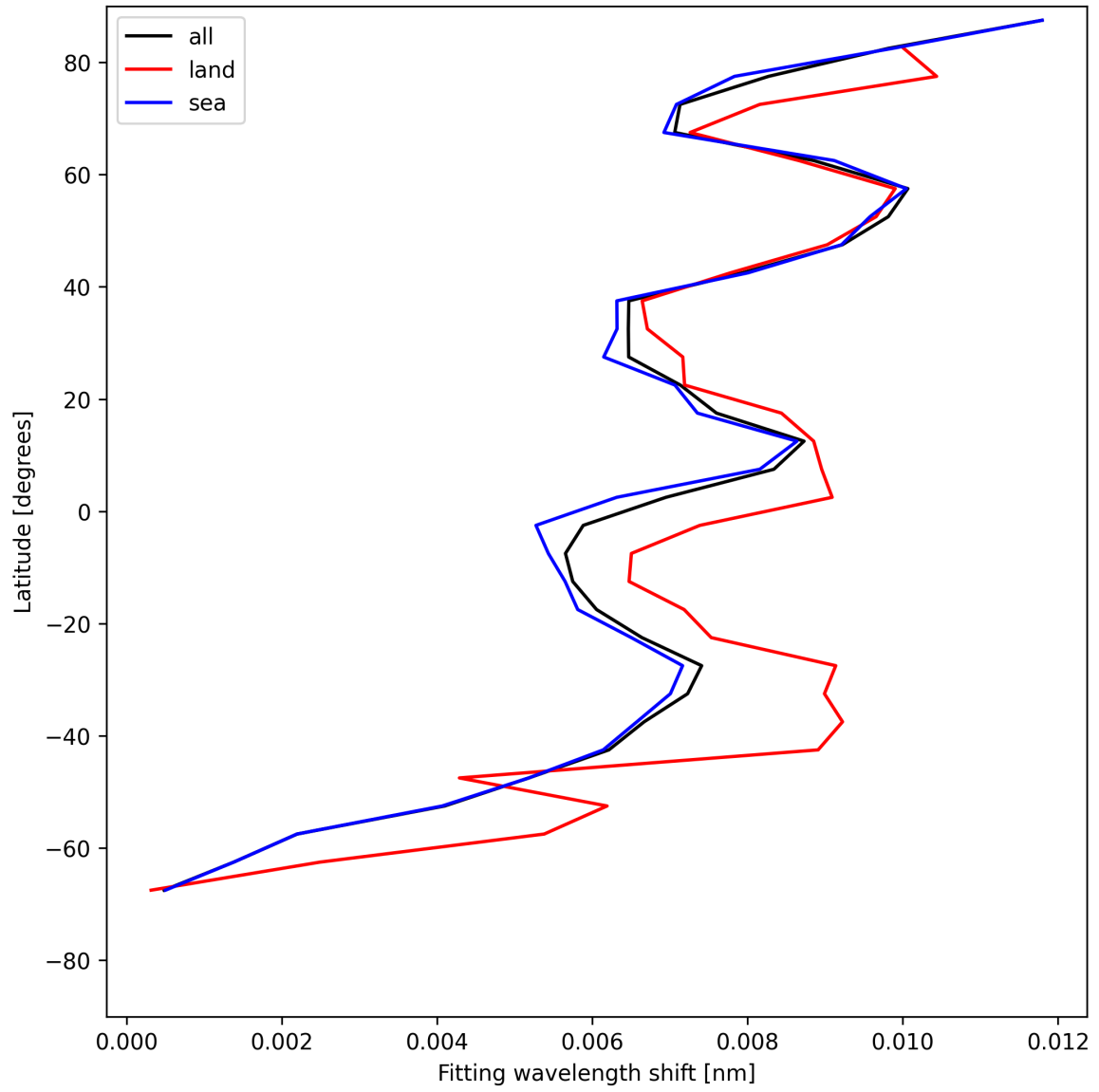
Figure 33: Zonal average of “Fitting wavelength shift” for 2025-07-20 to 2025-07-22.
