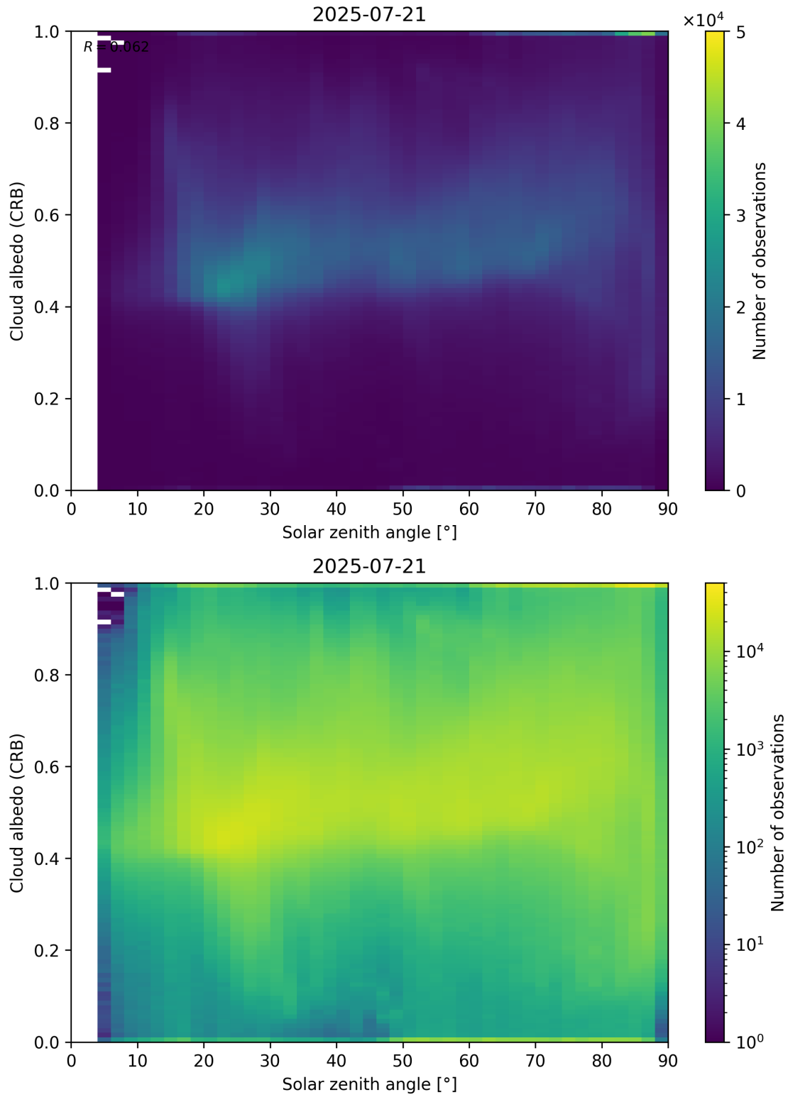
Figure 98: Scatter density plot of “Solar zenith angle” against “Cloud albedo (CRB)” for 2025-07-20 to 2025-07-22.
