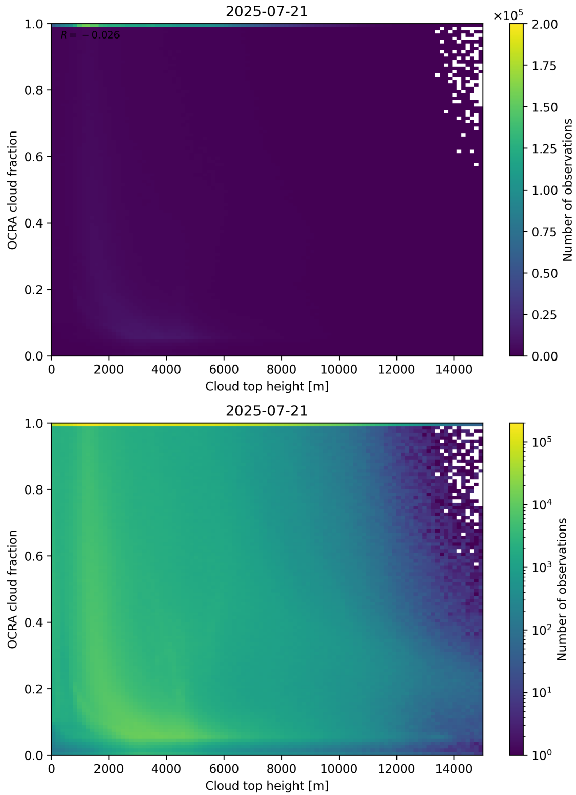
Figure 87: Scatter density plot of “Cloud top height” against “OCRA cloud fraction” for 2025-07-20 to 2025-07-22.
