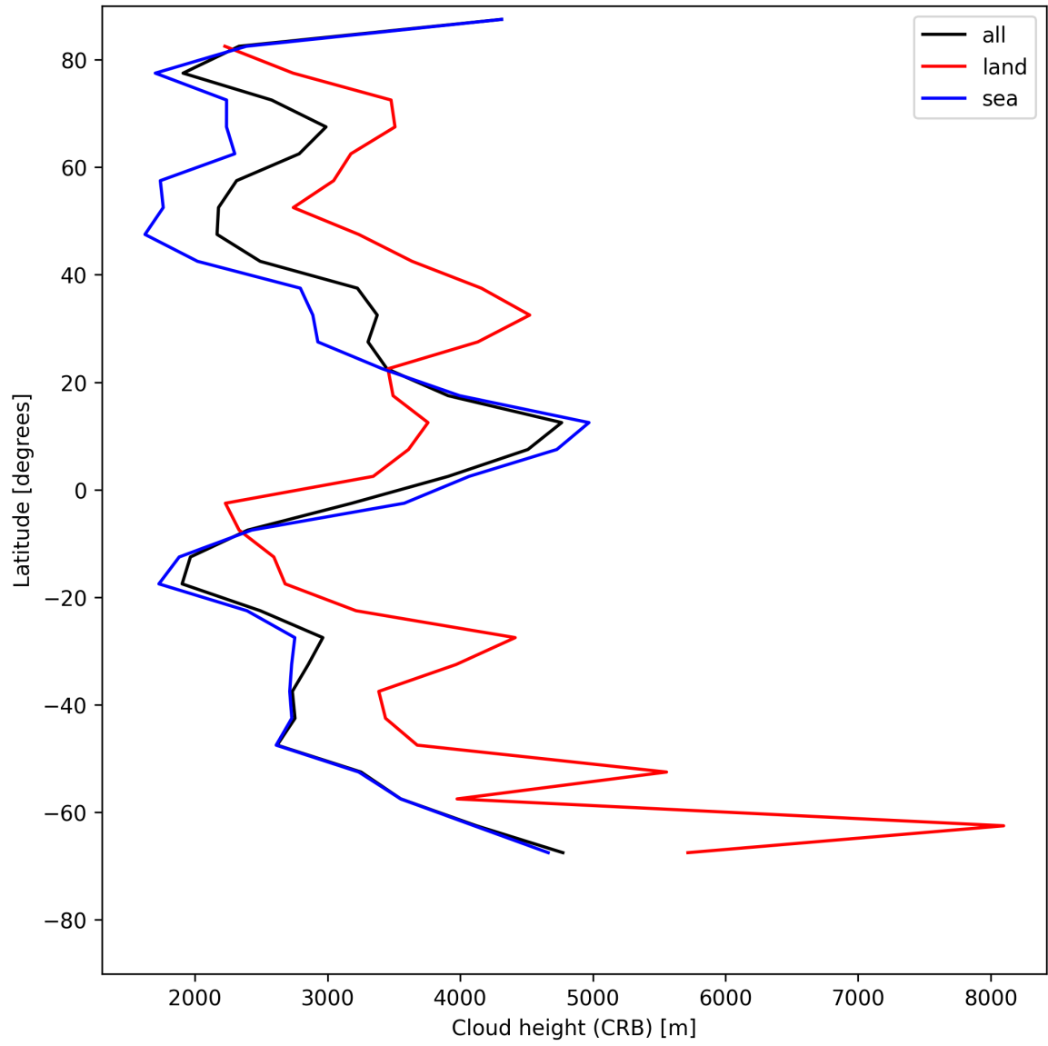
Figure 27: Zonal average of “Cloud height (CRB)” for 2025-07-20 to 2025-07-22.
