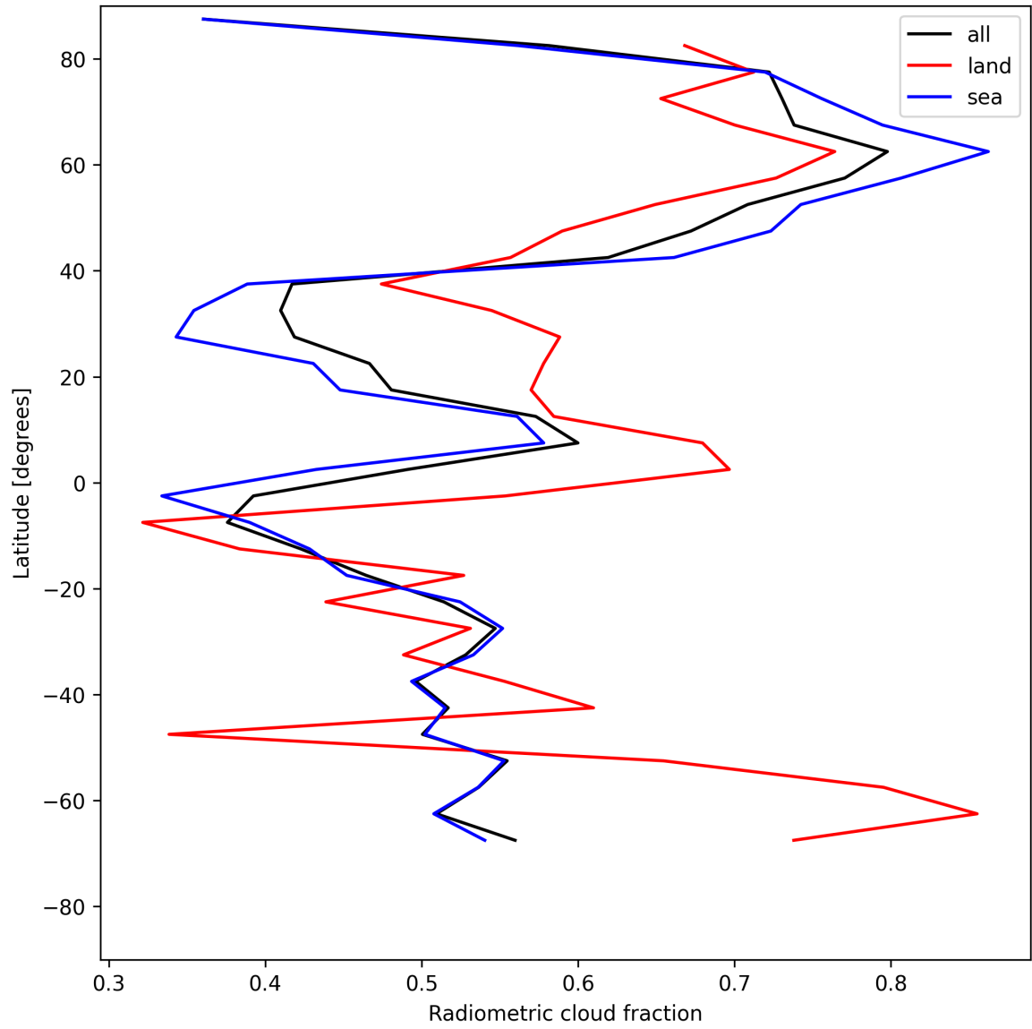
Figure 23: Zonal average of “Radiometric cloud fraction” for 2025-07-20 to 2025-07-22.
