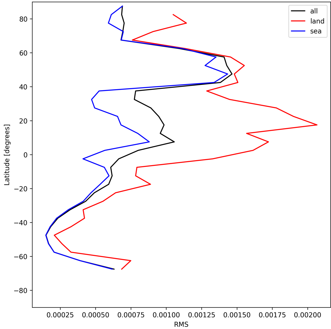
Figure 31: Zonal average of “RMS” for 2025-07-20 to 2025-07-22.
