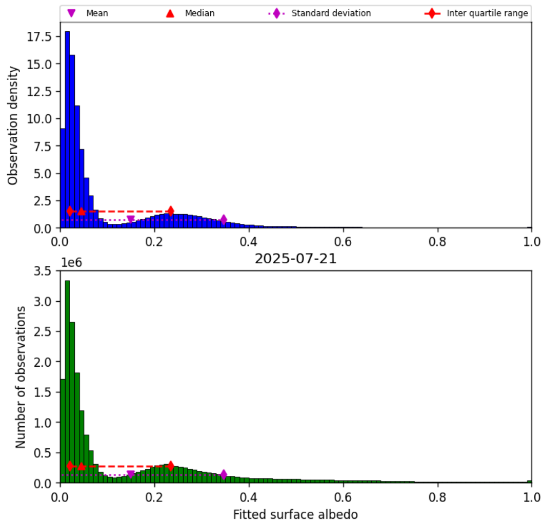
Figure 45: Histogram of “Fitted surface albedo” for 2025-07-20 to 2025-07-22
