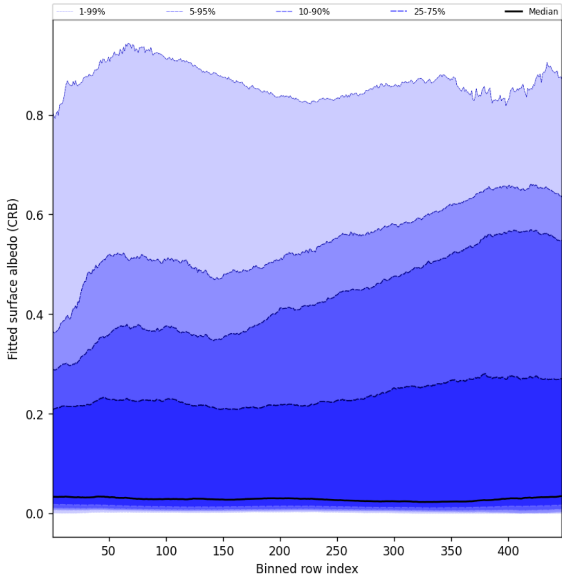
Figure 62: Along track statistics of “Fitted surface albedo (CRB)” for 2025-07-20 to 2025-07-22
