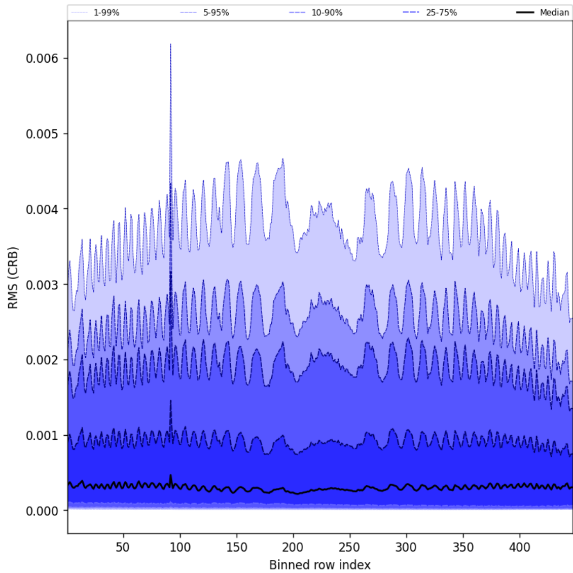
Figure 64: Along track statistics of “RMS (CRB)” for 2025-07-20 to 2025-07-22
