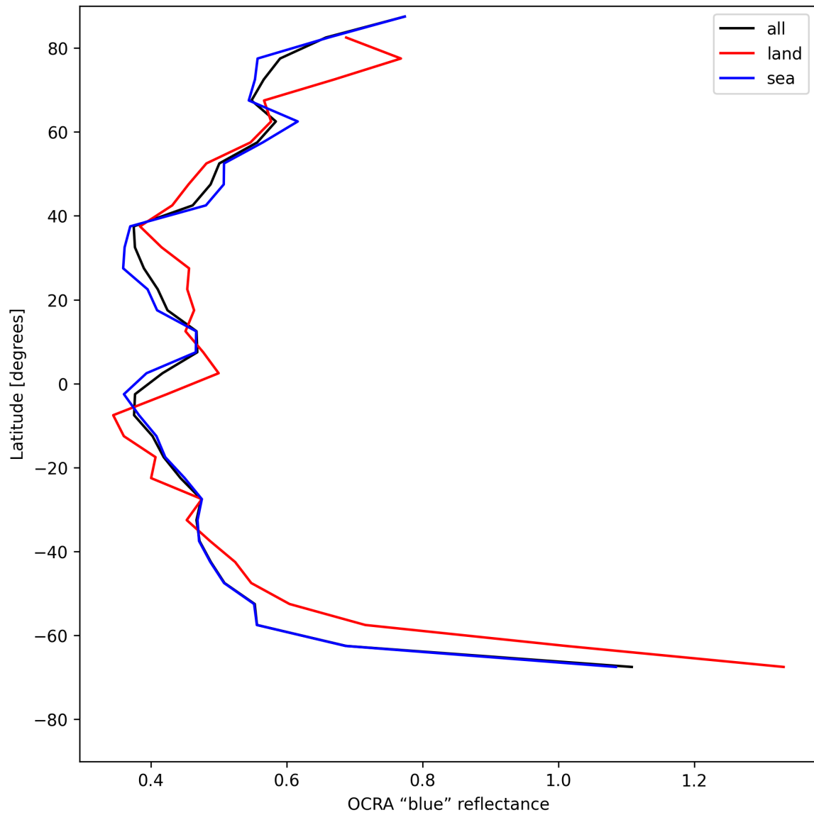
Figure 35: Zonal average of “OCRA “blue” reflectance” for 2025-07-20 to 2025-07-22.
