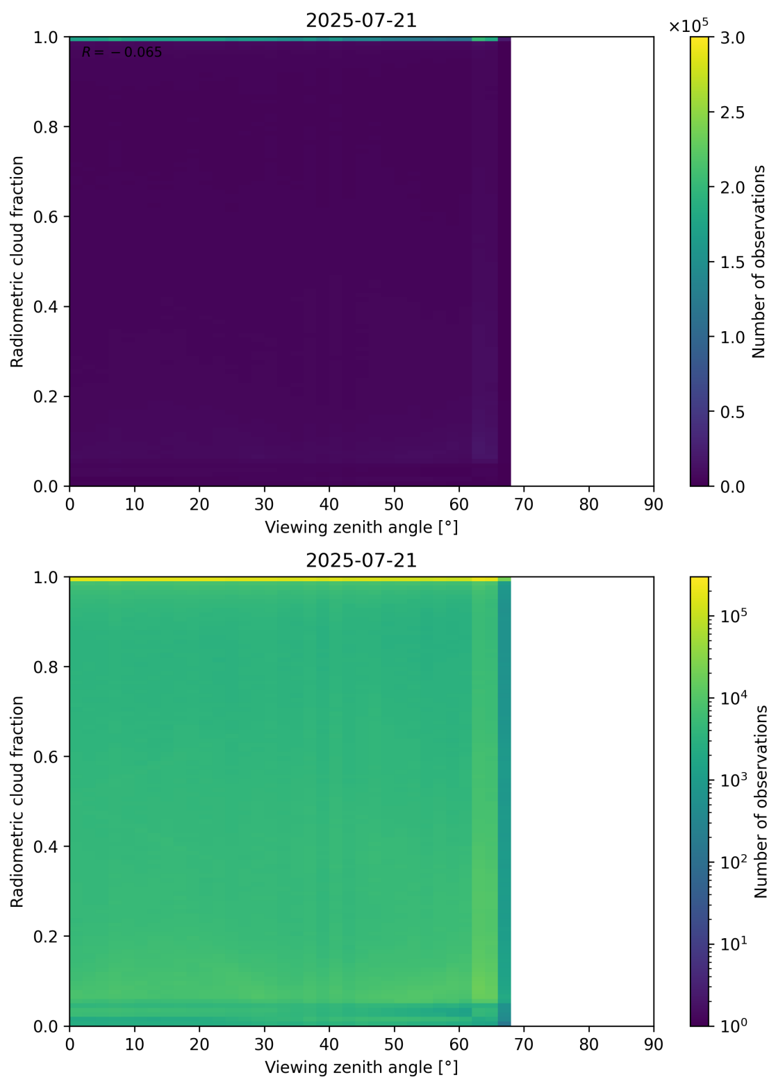
Figure 107: Scatter density plot of “Viewing zenith angle” against “Radiometric cloud fraction” for 2025-07-20 to 2025-07-22.
