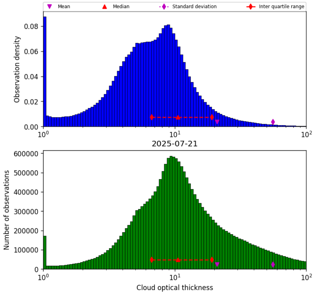
Figure 41: Histogram of “Cloud optical thickness” for 2025-07-20 to 2025-07-22
