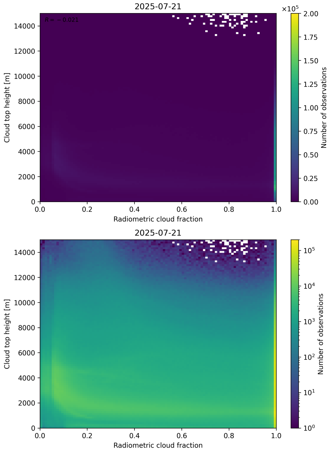
Figure 76: Scatter density plot of “Radiometric cloud fraction” against “Cloud top height” for 2025-07-20 to 2025-07-22.
