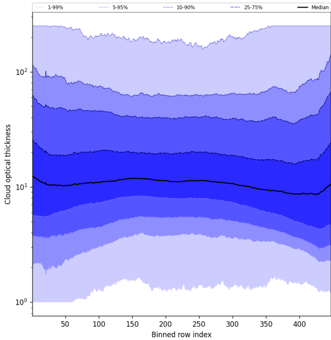
Figure 57: Along track statistics of “Cloud optical thickness” for 2025-07-20 to 2025-07-22
