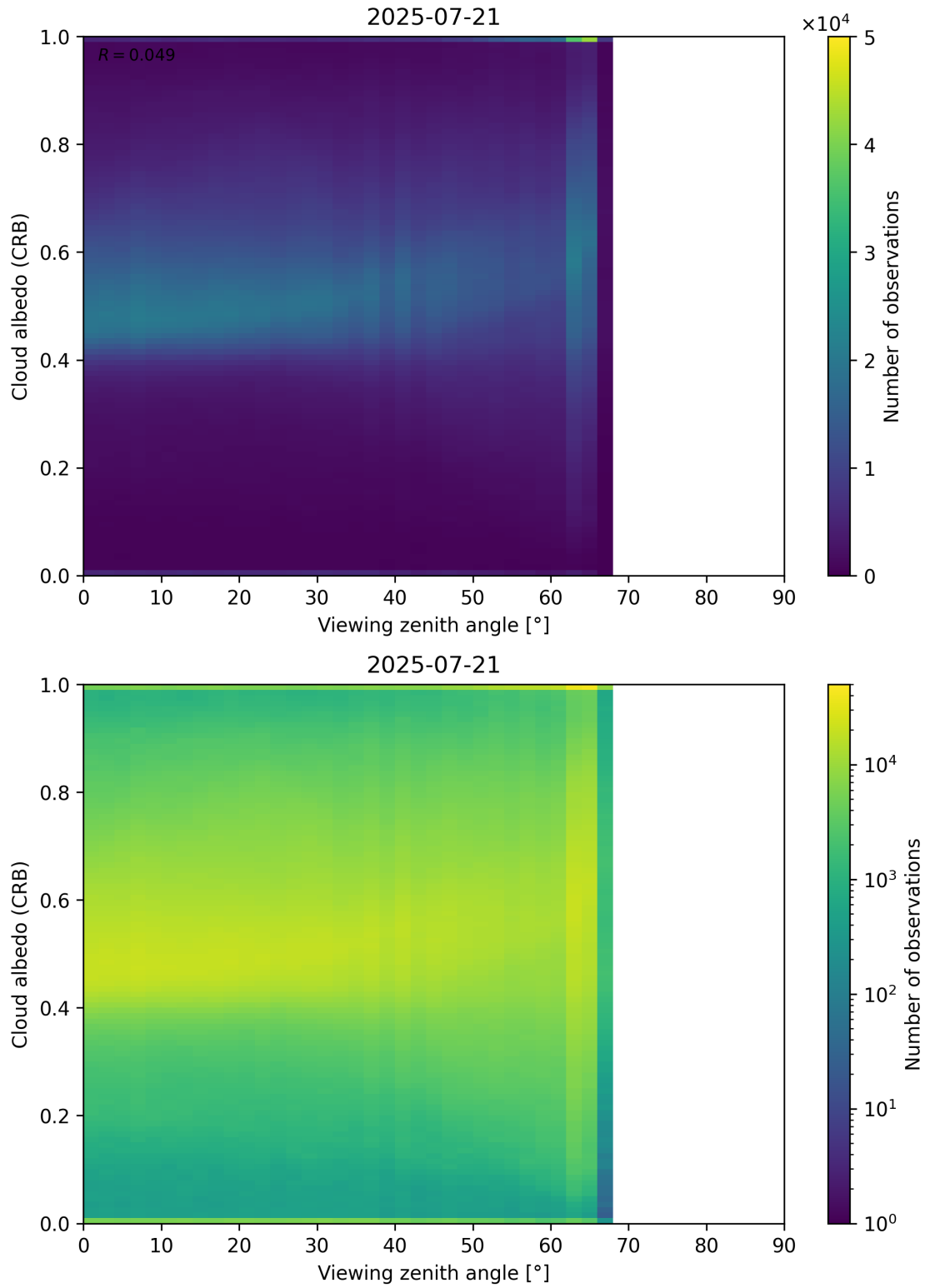
Figure 106: Scatter density plot of “Viewing zenith angle” against “Cloud albedo (CRB)” for 2025-07-20 to 2025-07-22.
