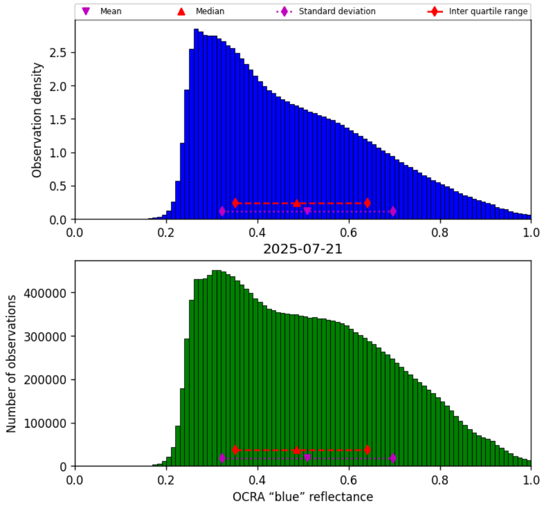
Figure 51: Histogram of “OCRA “blue” reflectance” for 2025-07-20 to 2025-07-22
