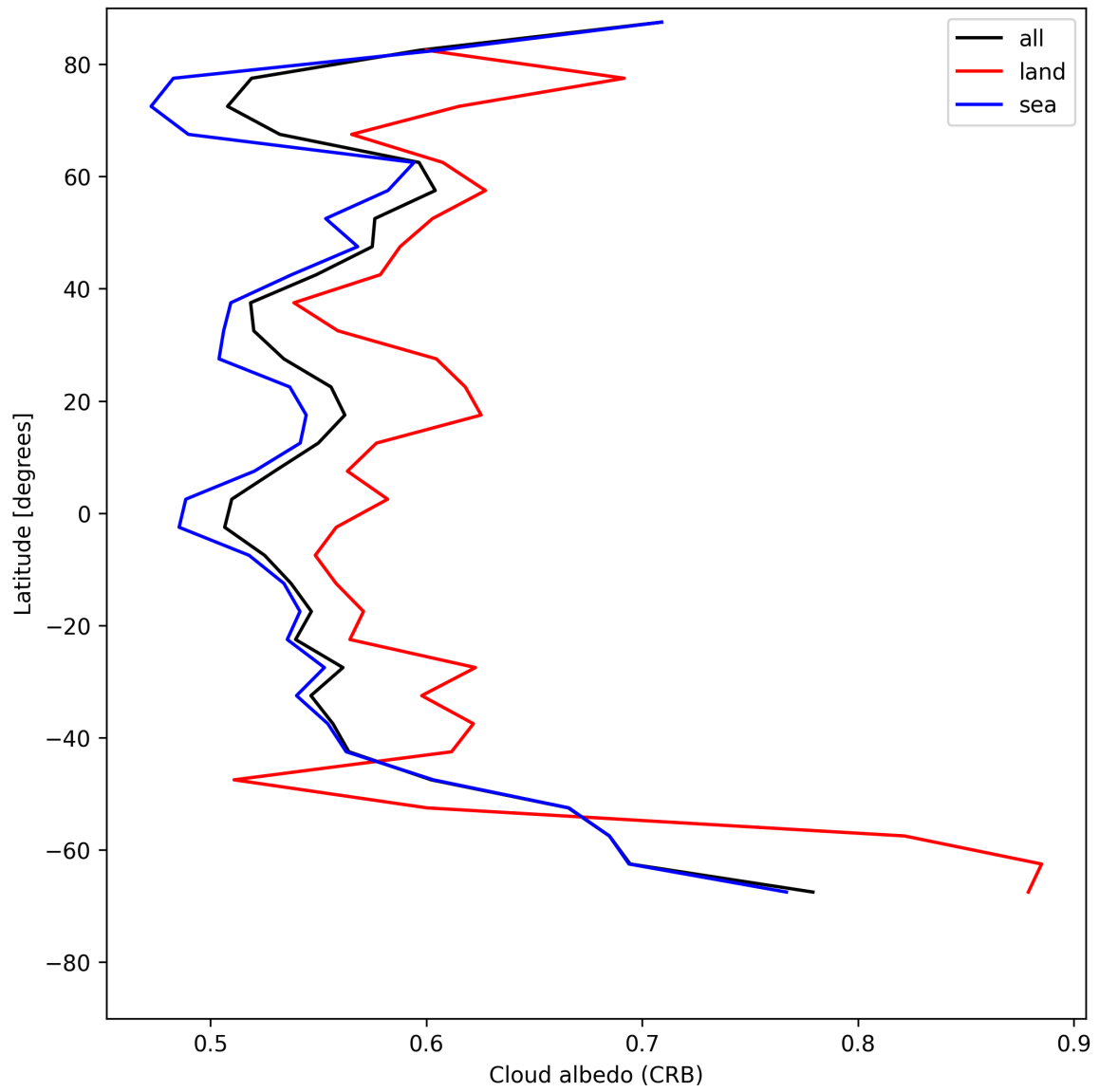
Figure 28: Zonal average of “Cloud albedo (CRB)” for 2025-07-20 to 2025-07-22.
