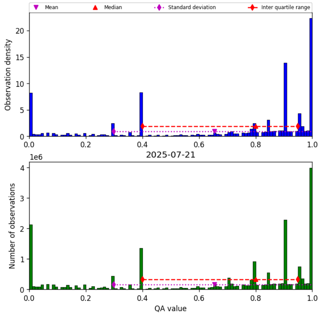
Figure 38: Histogram of “QA value” for 2025-07-20 to 2025-07-22
