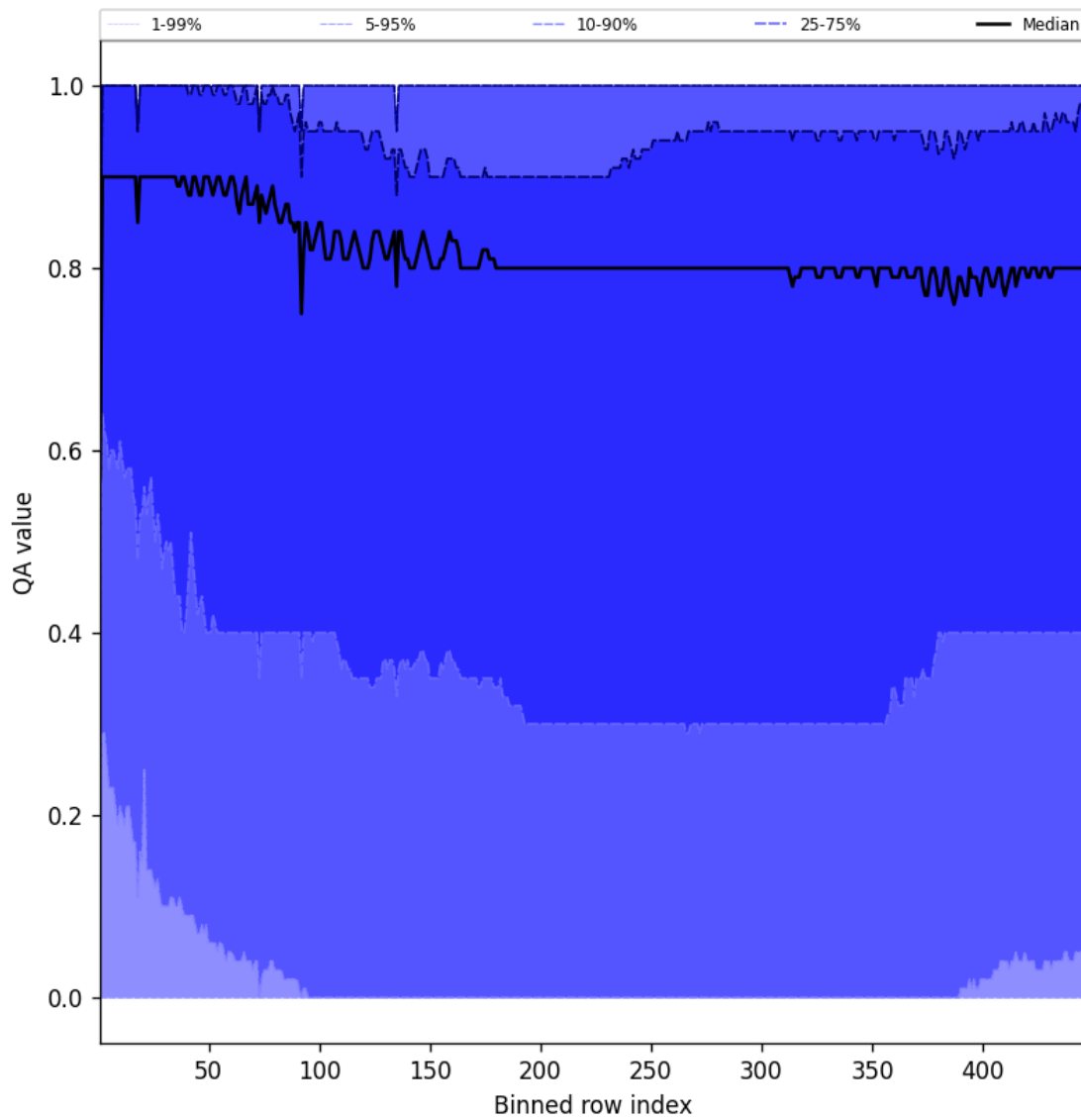
Figure 54: Along track statistics of “QA value” for 2025-07-20 to 2025-07-22
