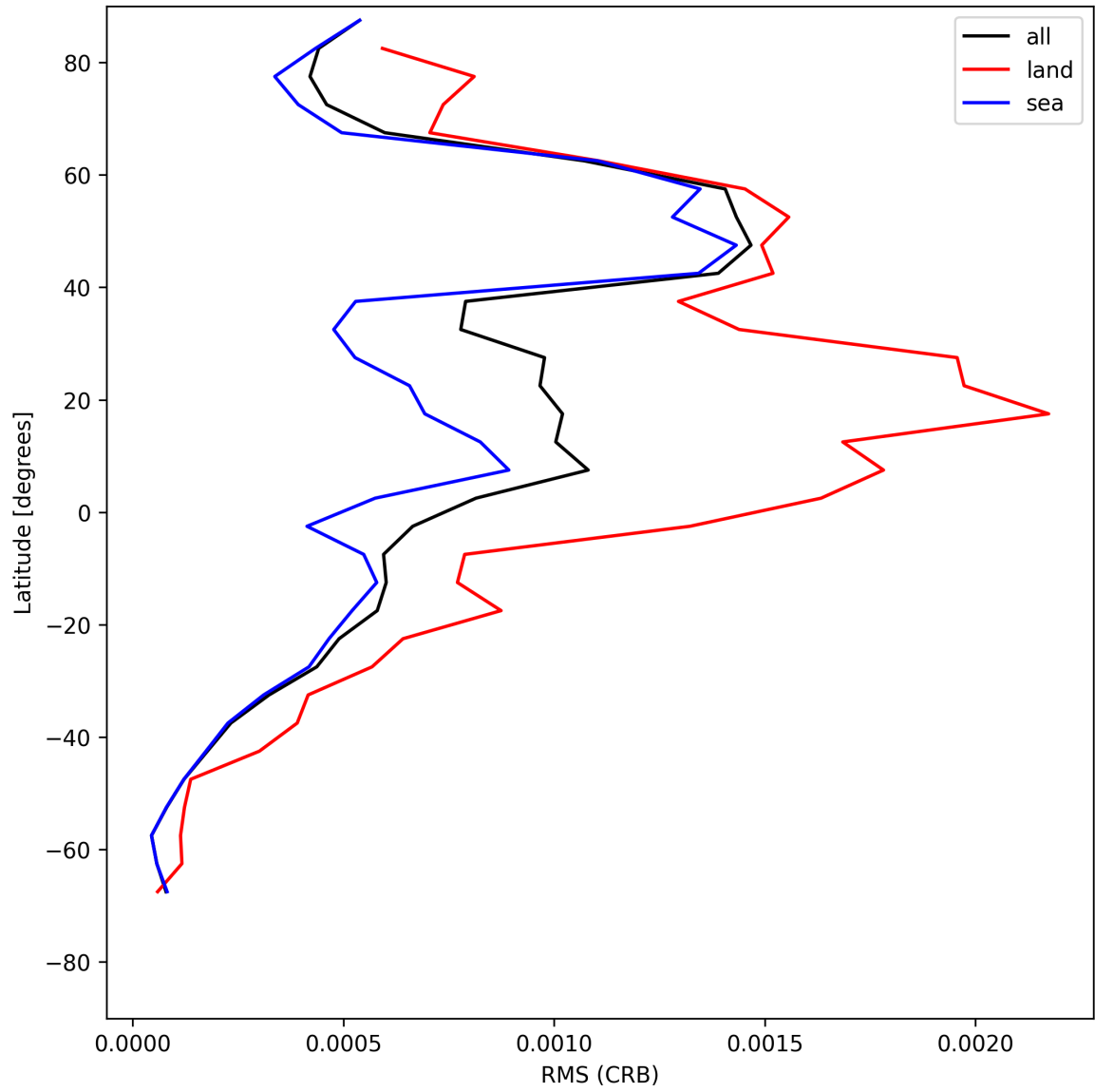
Figure 32: Zonal average of “RMS (CRB)” for 2025-07-20 to 2025-07-22.
