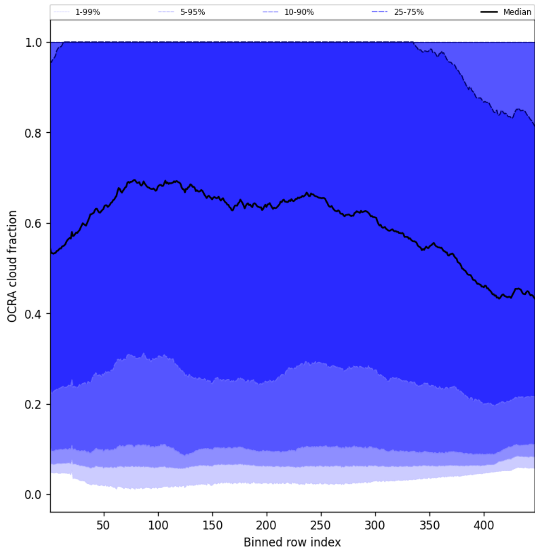
Figure 66: Along track statistics of “OCRA cloud fraction” for 2025-07-20 to 2025-07-22
