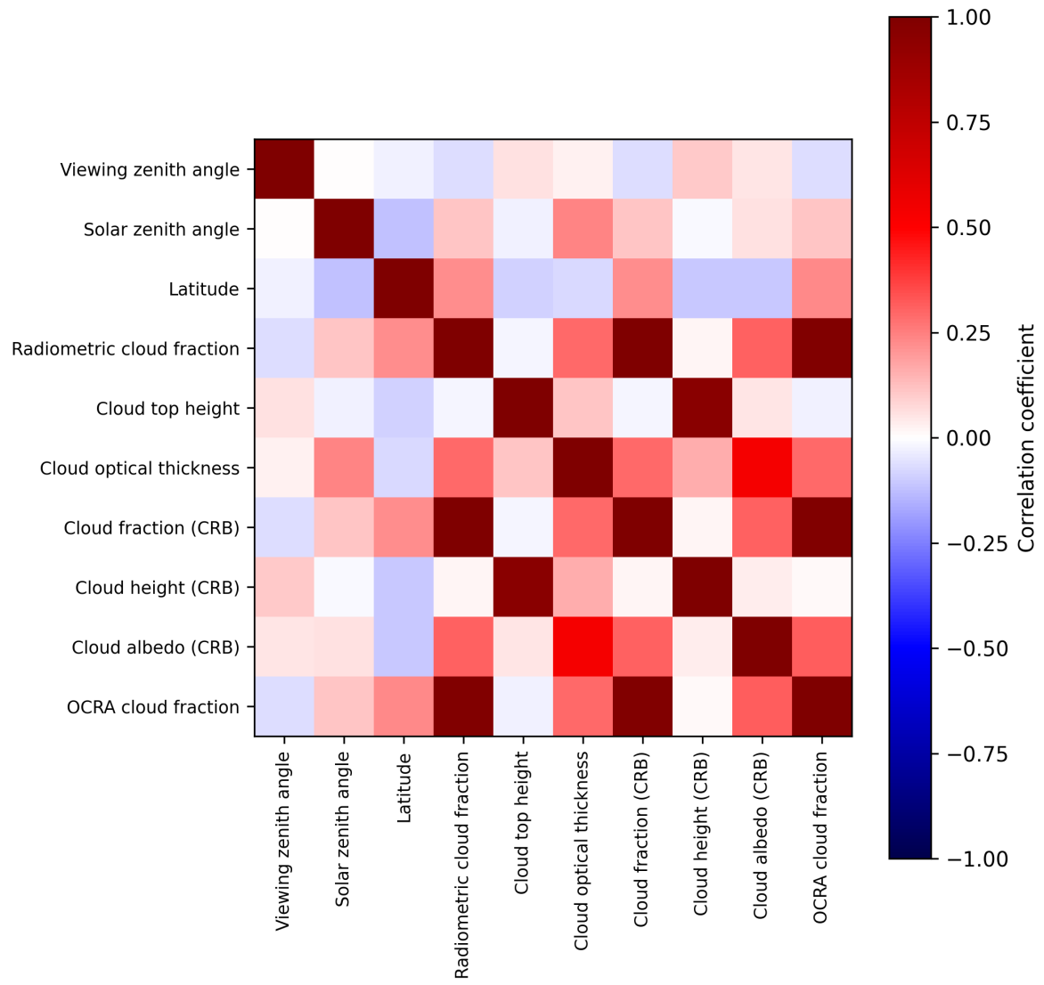
Figure 2: Map of correlation matrix for 2025-07-20 to 2025-07-22.
