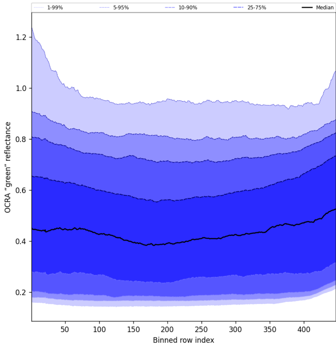
Figure 68: Along track statistics of “OCRA “green” reflectance” for 2025-07-20 to 2025-07-22
