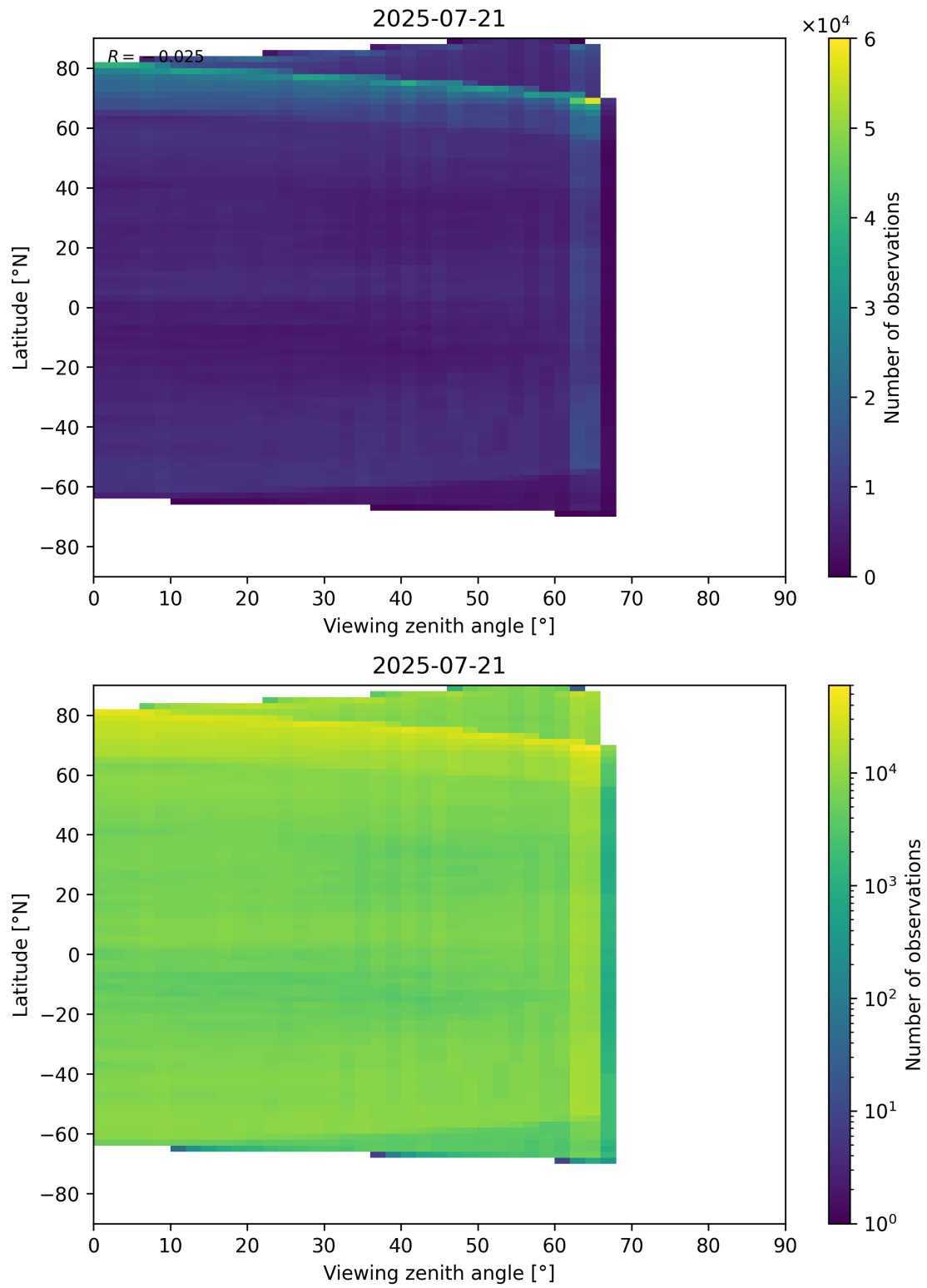
Figure 113: Scatter density plot of “Viewing zenith angle” against “Latitude” for 2025-07-20 to 2025-07-22.
