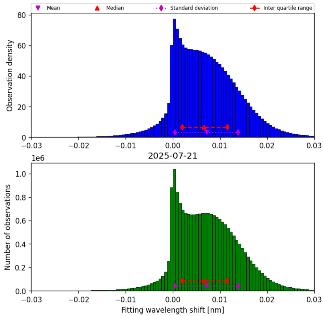
Figure 49: Histogram of “Fitting wavelength shift” for 2025-07-20 to 2025-07-22
