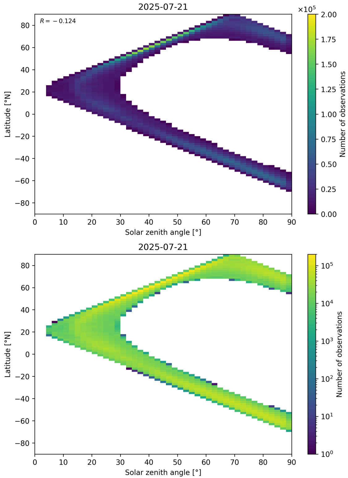
Figure 105: Scatter density plot of “Solar zenith angle” against “Latitude” for 2025-07-20 to 2025-07-22.
