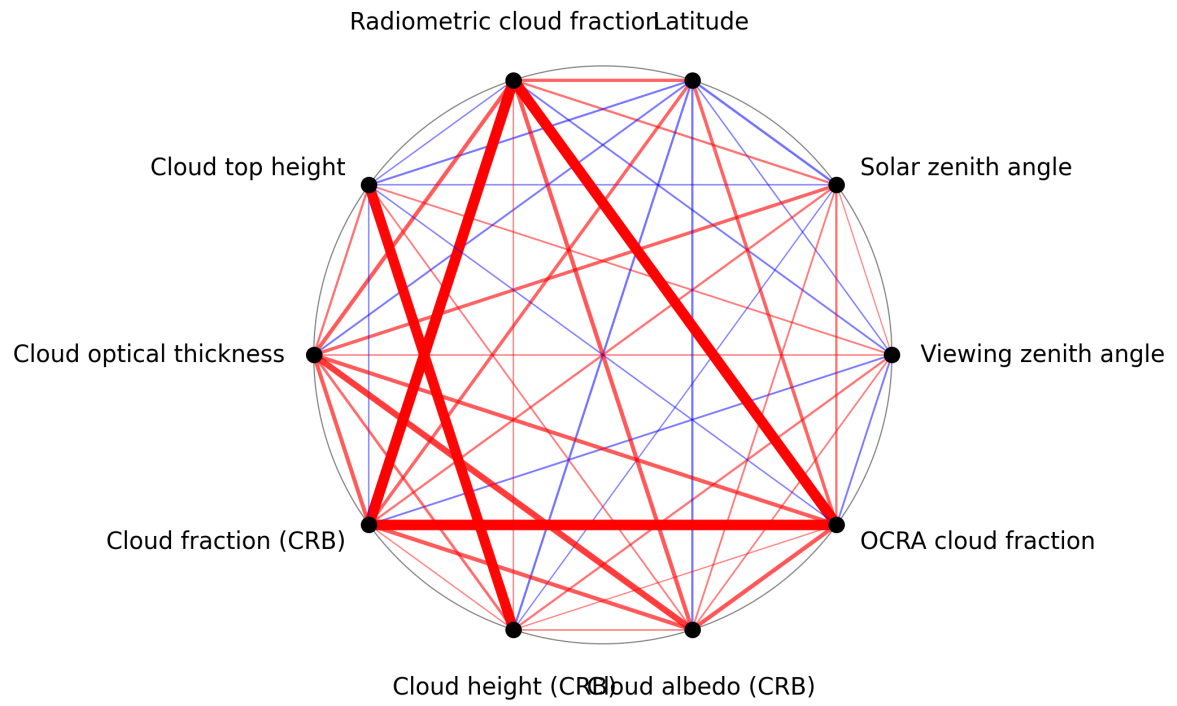
Figure 1: Map of correlation graph for 2025-07-20 to 2025-07-22.
