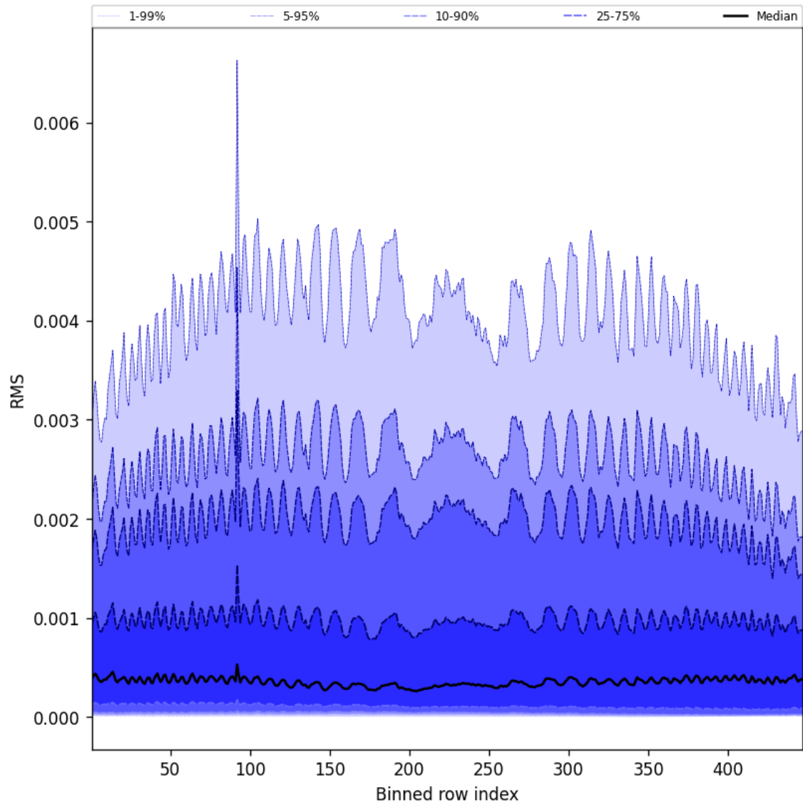
Figure 63: Along track statistics of “RMS” for 2025-07-20 to 2025-07-22
