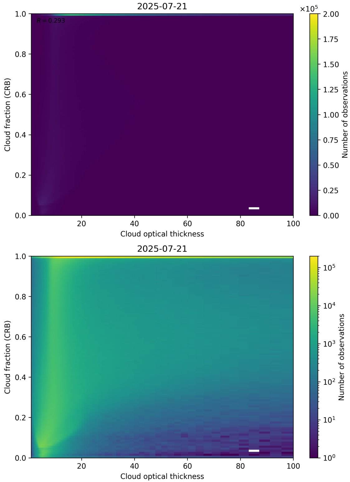
Figure 84: Scatter density plot of “Cloud optical thickness” against “Cloud fraction (CRB)” for 2025-07-20 to 2025-07-22.
