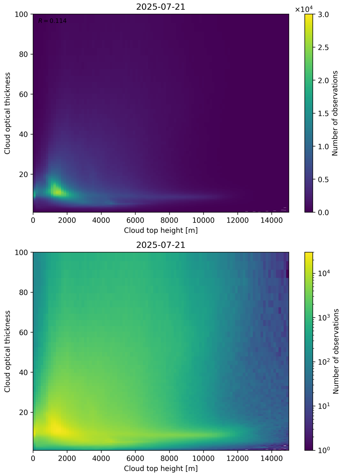
Figure 90: Scatter density plot of “Cloud top height” against “Cloud optical thickness” for 2025-07-20 to 2025-07-22.
