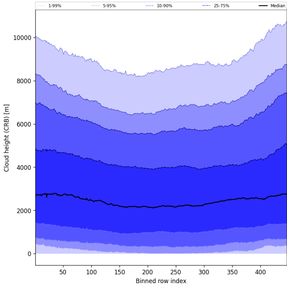
Figure 59: Along track statistics of “Cloud height (CRB)” for 2025-07-20 to 2025-07-22
