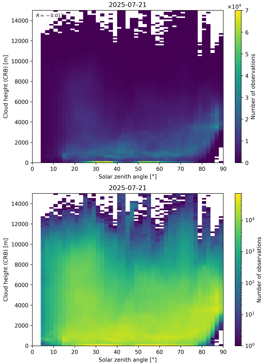
Figure 102: Scatter density plot of “Solar zenith angle” against “Cloud height (CRB)” for 2025-07-20 to 2025-07-22.
