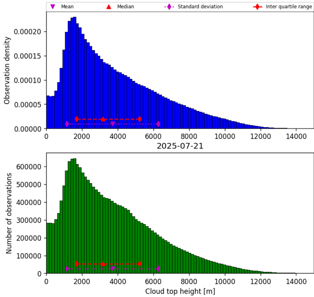
Figure 40: Histogram of “Cloud top height” for 2025-07-20 to 2025-07-22
