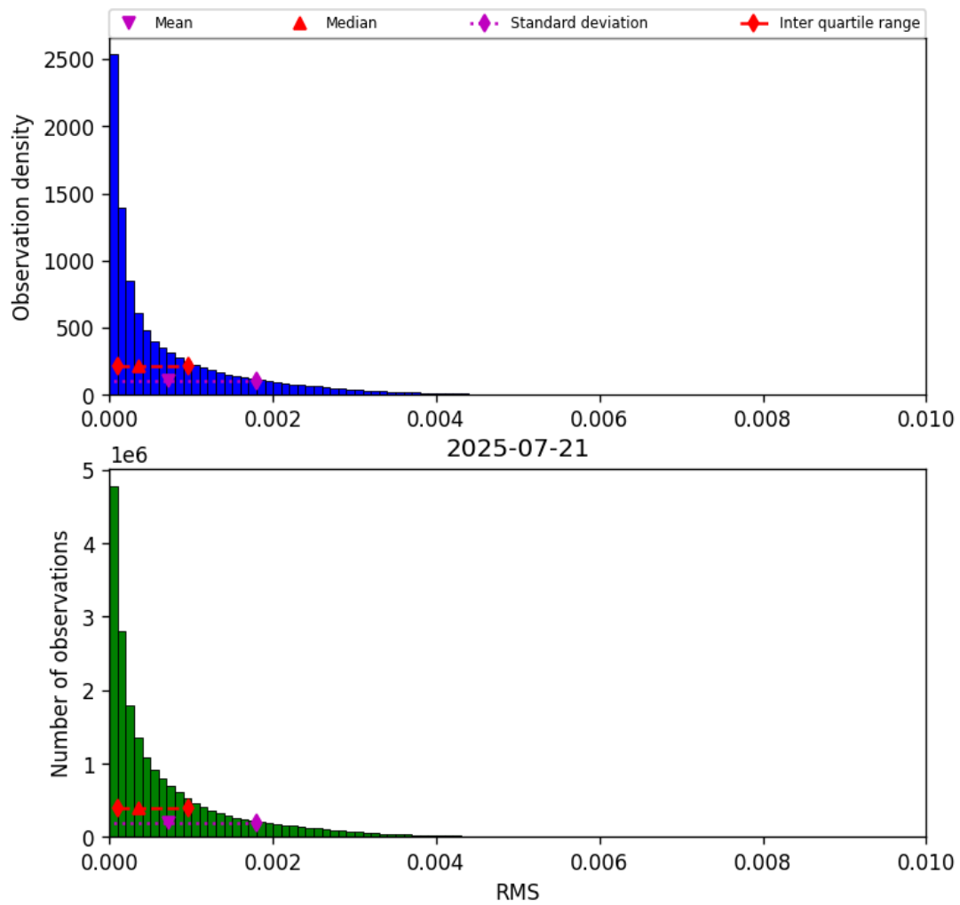
Figure 47: Histogram of “RMS” for 2025-07-20 to 2025-07-22
