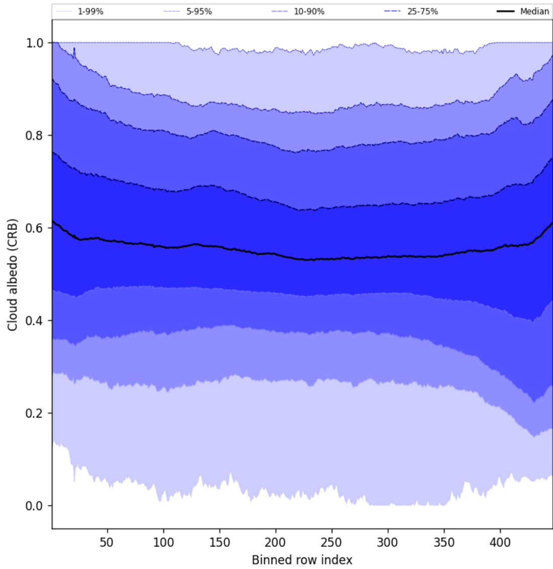
Figure 60: Along track statistics of “Cloud albedo (CRB)” for 2025-07-20 to 2025-07-22
