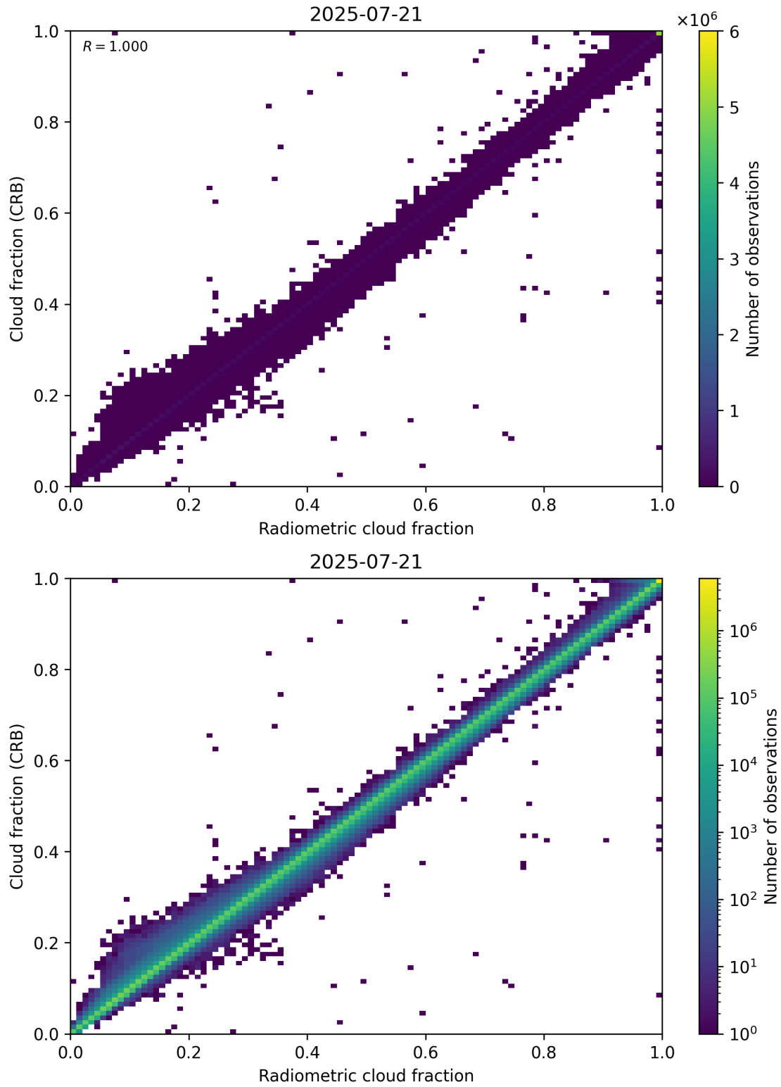
Figure 73: Scatter density plot of “Radiometric cloud fraction” against “Cloud fraction (CRB)” for 2025-07-20 to 2025-07-22.
