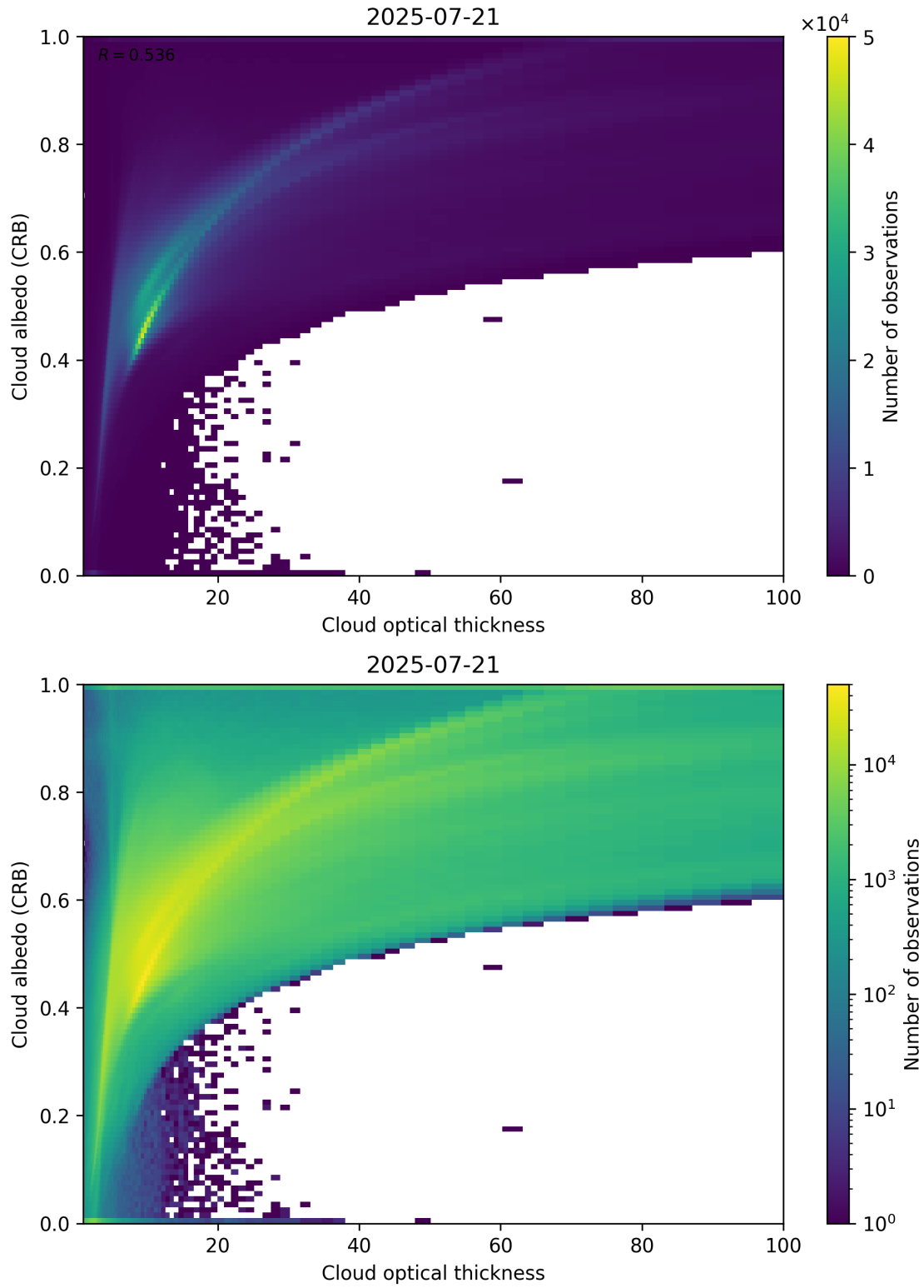
Figure 82: Scatter density plot of “Cloud optical thickness” against “Cloud albedo (CRB)” for 2025-07-20 to 2025-07-22.
