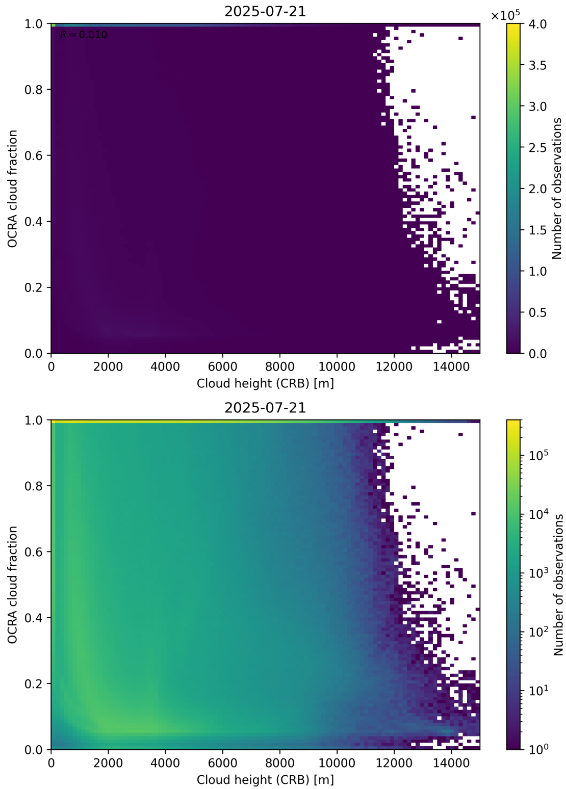
Figure 81: Scatter density plot of “Cloud height (CRB)” against “OCRA cloud fraction” for 2025-07-20 to 2025-07-22.
