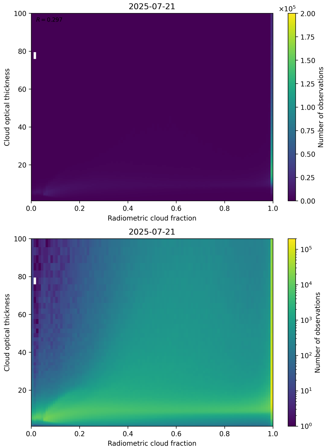
Figure 75: Scatter density plot of “Radiometric cloud fraction” against “Cloud optical thickness” for 2025-07-20 to 2025-07-22.
