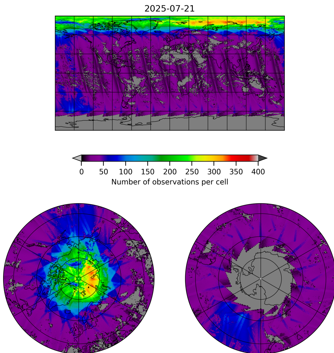
Figure 21: Map of the number of observations for 2025-07-20 to 2025-07-22
