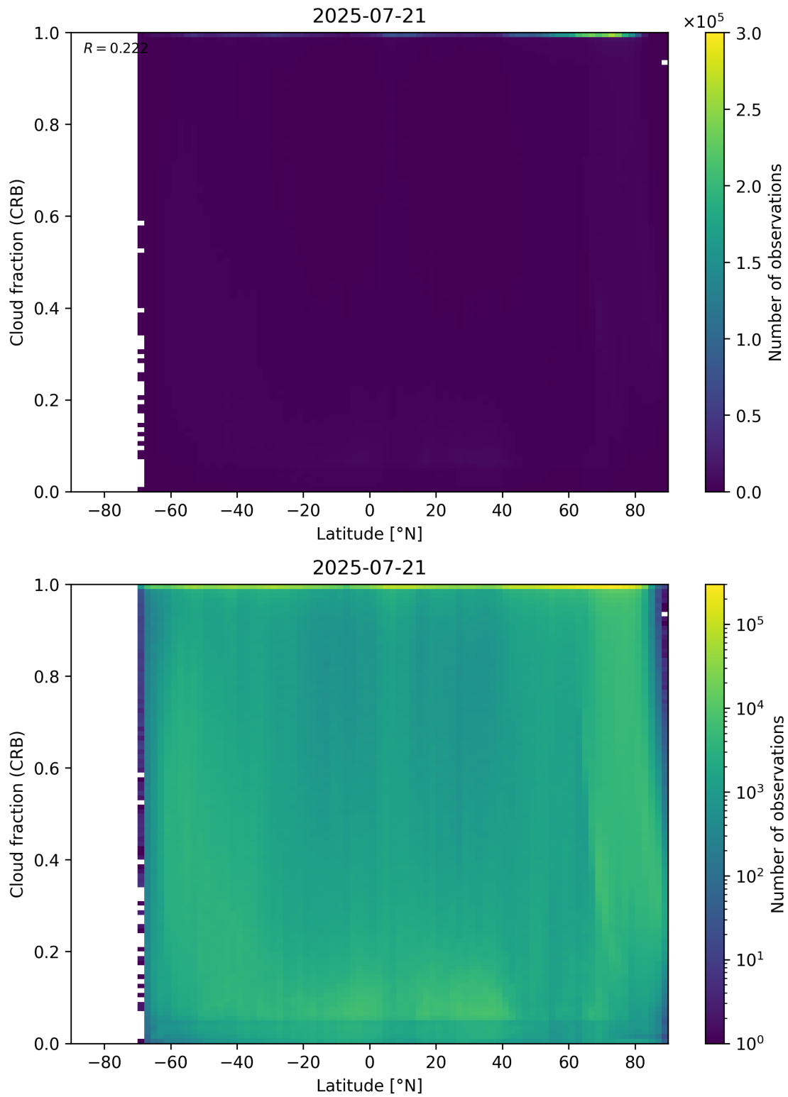
Figure 94: Scatter density plot of “Latitude” against “Cloud fraction (CRB)” for 2025-07-20 to 2025-07-22.
