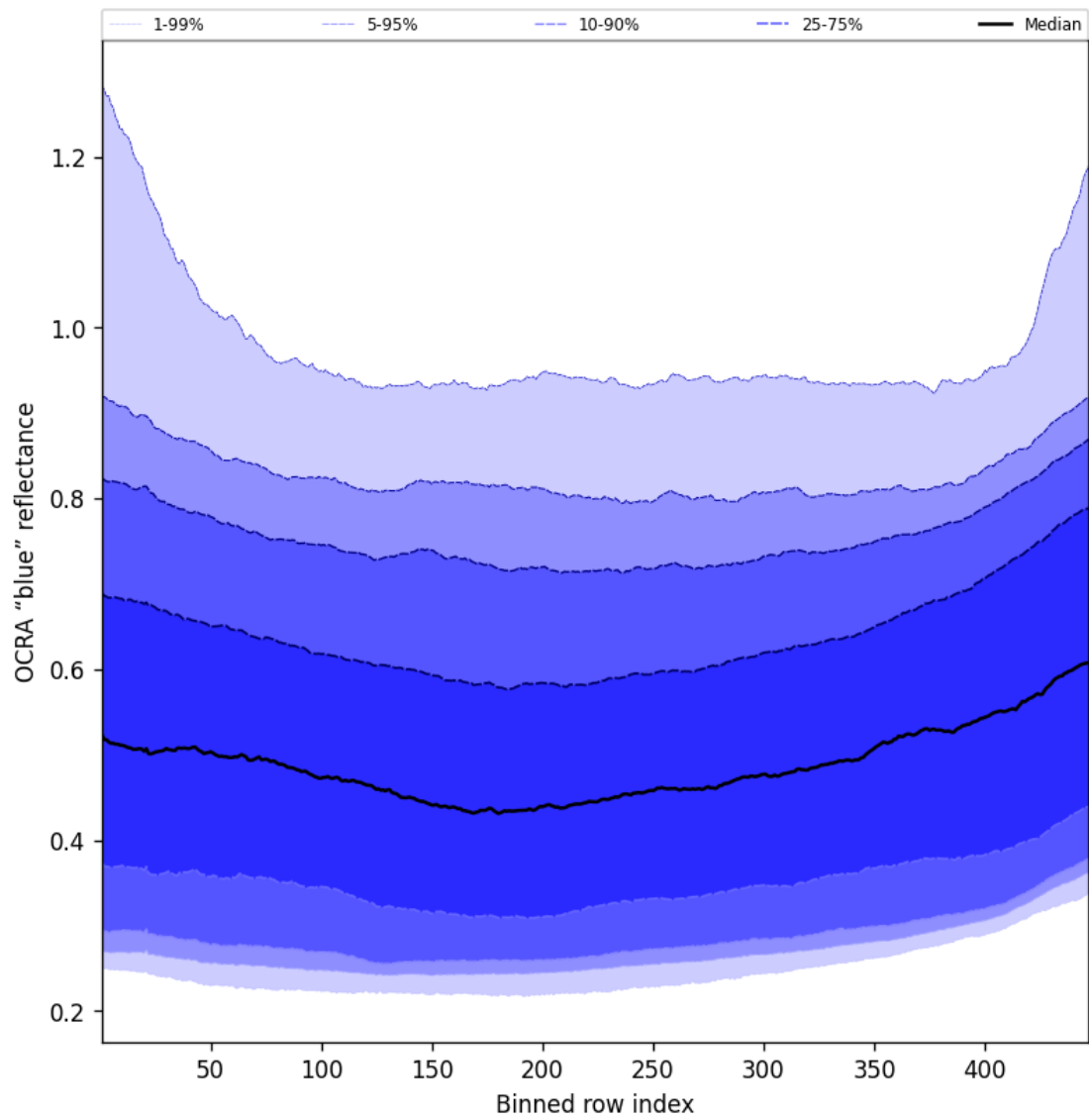
Figure 67: Along track statistics of “OCRA “blue” reflectance” for 2025-07-20 to 2025-07-22
