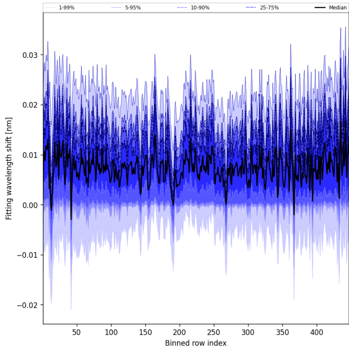
Figure 65: Along track statistics of “Fitting wavelength shift” for 2025-07-20 to 2025-07-22
