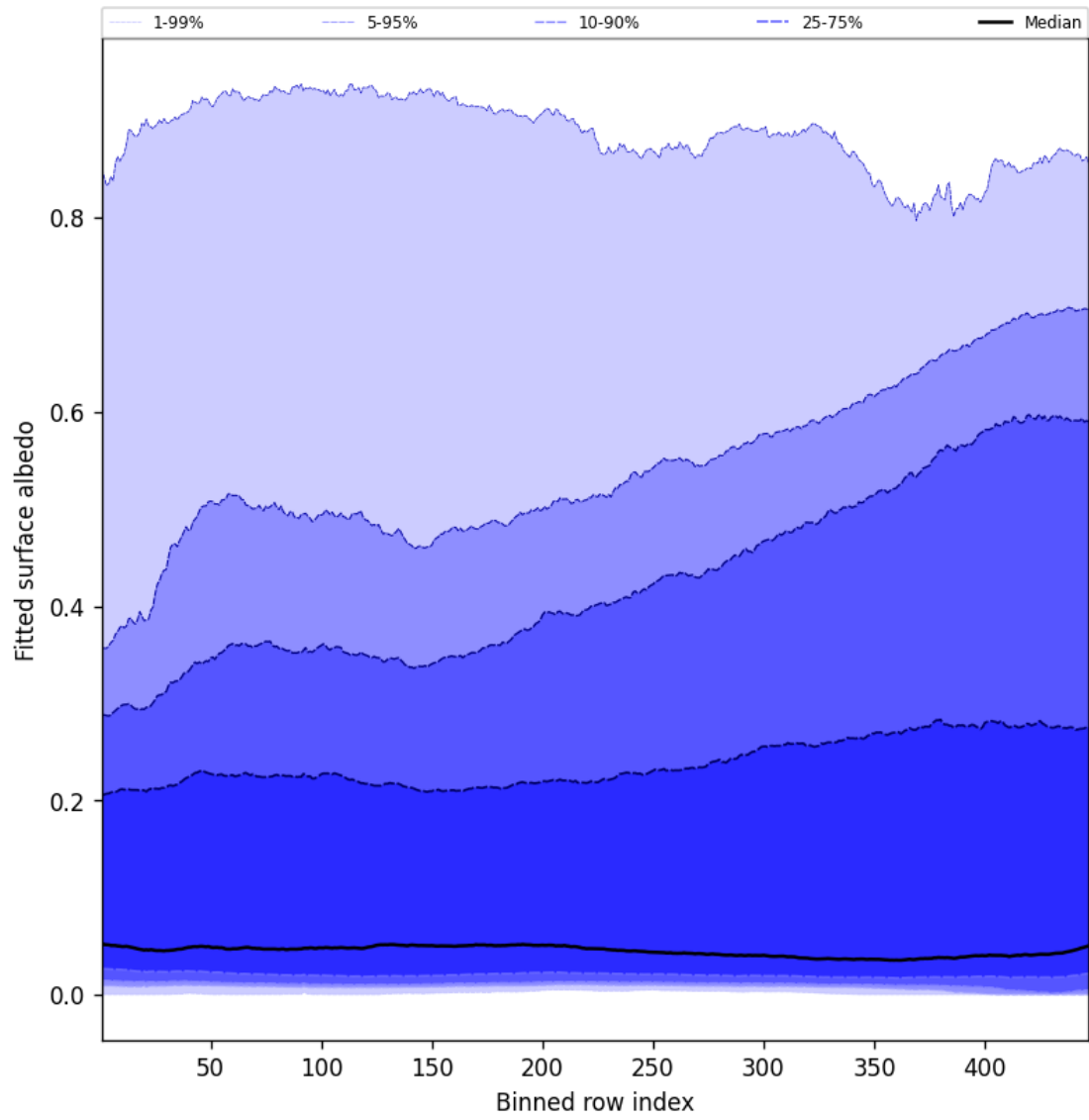
Figure 61: Along track statistics of “Fitted surface albedo” for 2025-07-20 to 2025-07-22
