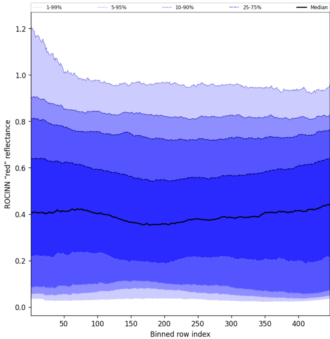
Figure 69: Along track statistics of "ROCINN "red" reflectance" for 2025-07-20 to 2025-07-22
