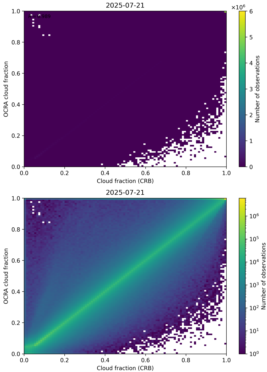
Figure 78: Scatter density plot of “Cloud fraction (CRB)” against “OCRA cloud fraction” for 2025-07-20 to 2025-07-22.
