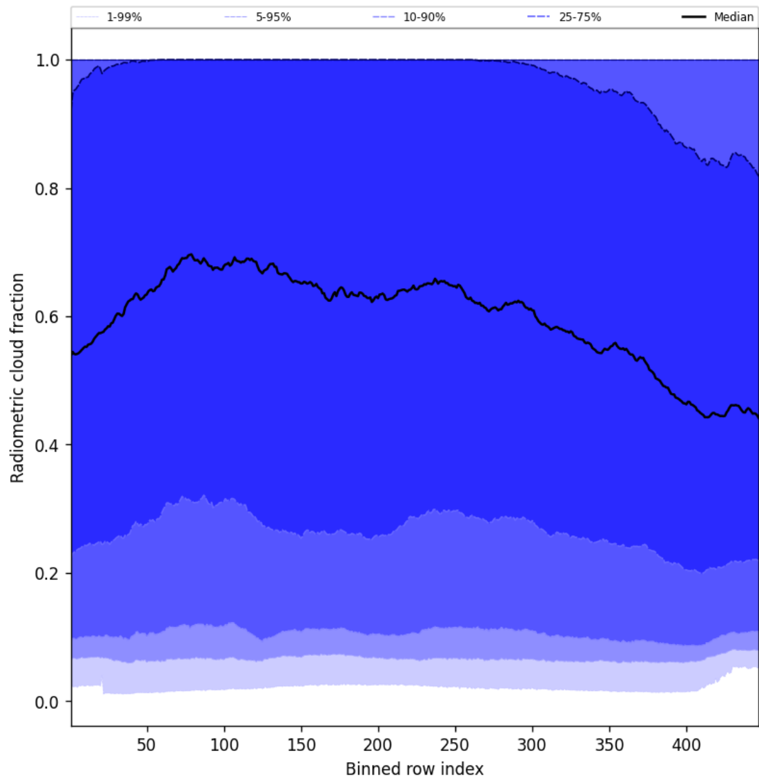
Figure 55: Along track statistics of “Radiometric cloud fraction” for 2025-07-20 to 2025-07-22
