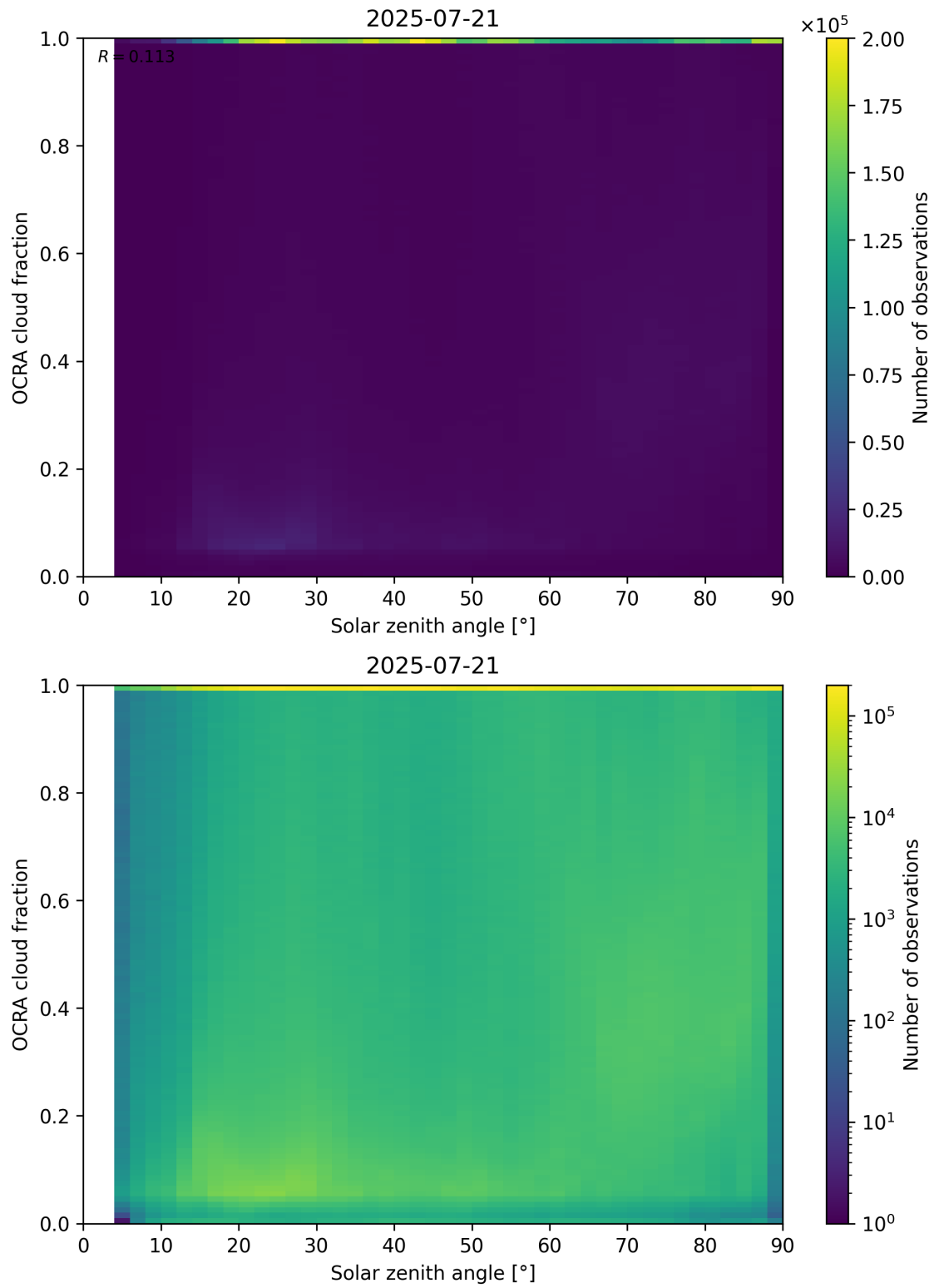
Figure 100: Scatter density plot of “Solar zenith angle” against “OCRA cloud fraction” for 2025-07-20 to 2025-07-22.
