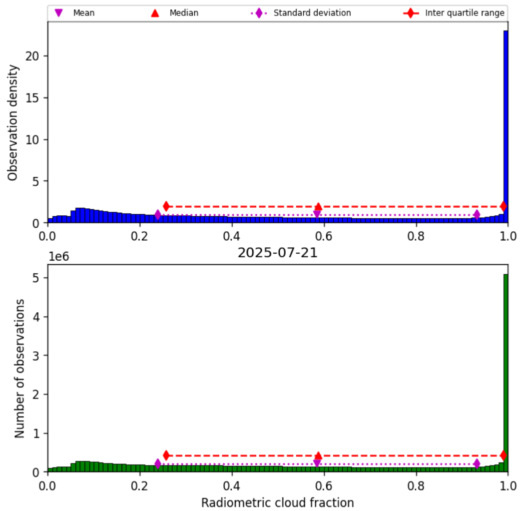
Figure 39: Histogram of “Radiometric cloud fraction” for 2025-07-20 to 2025-07-22
