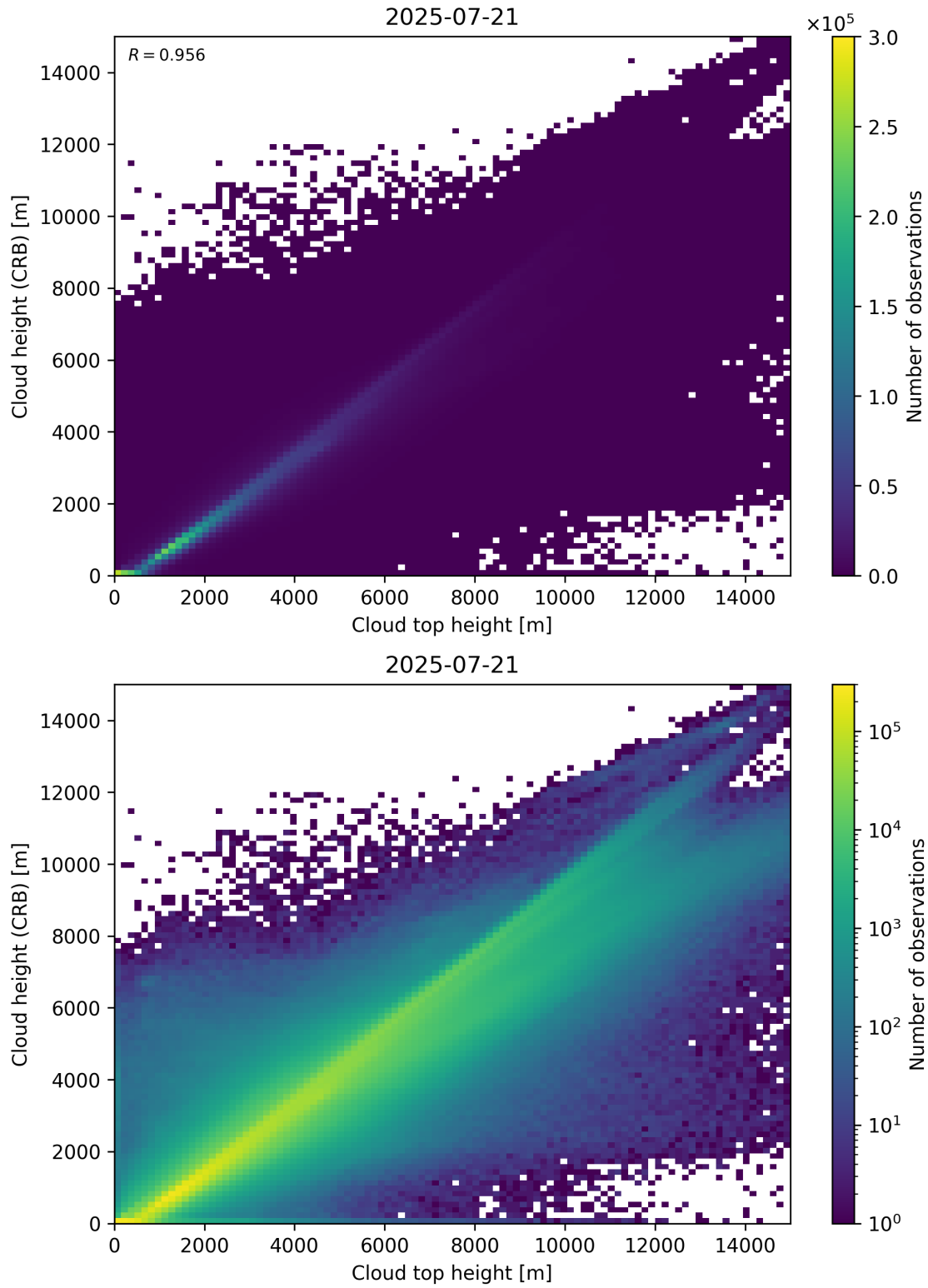
Figure 89: Scatter density plot of “Cloud top height” against “Cloud height (CRB)” for 2025-07-20 to 2025-07-22.
