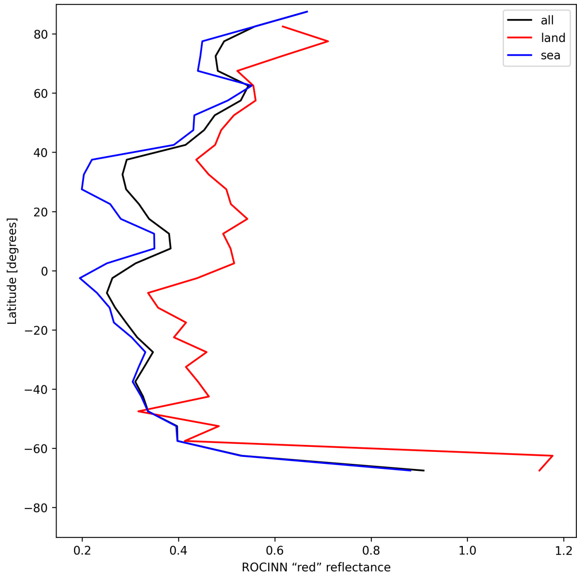
Figure 37: Zonal average of “ROCINN “red” reflectance” for 2025-07-20 to 2025-07-22.
