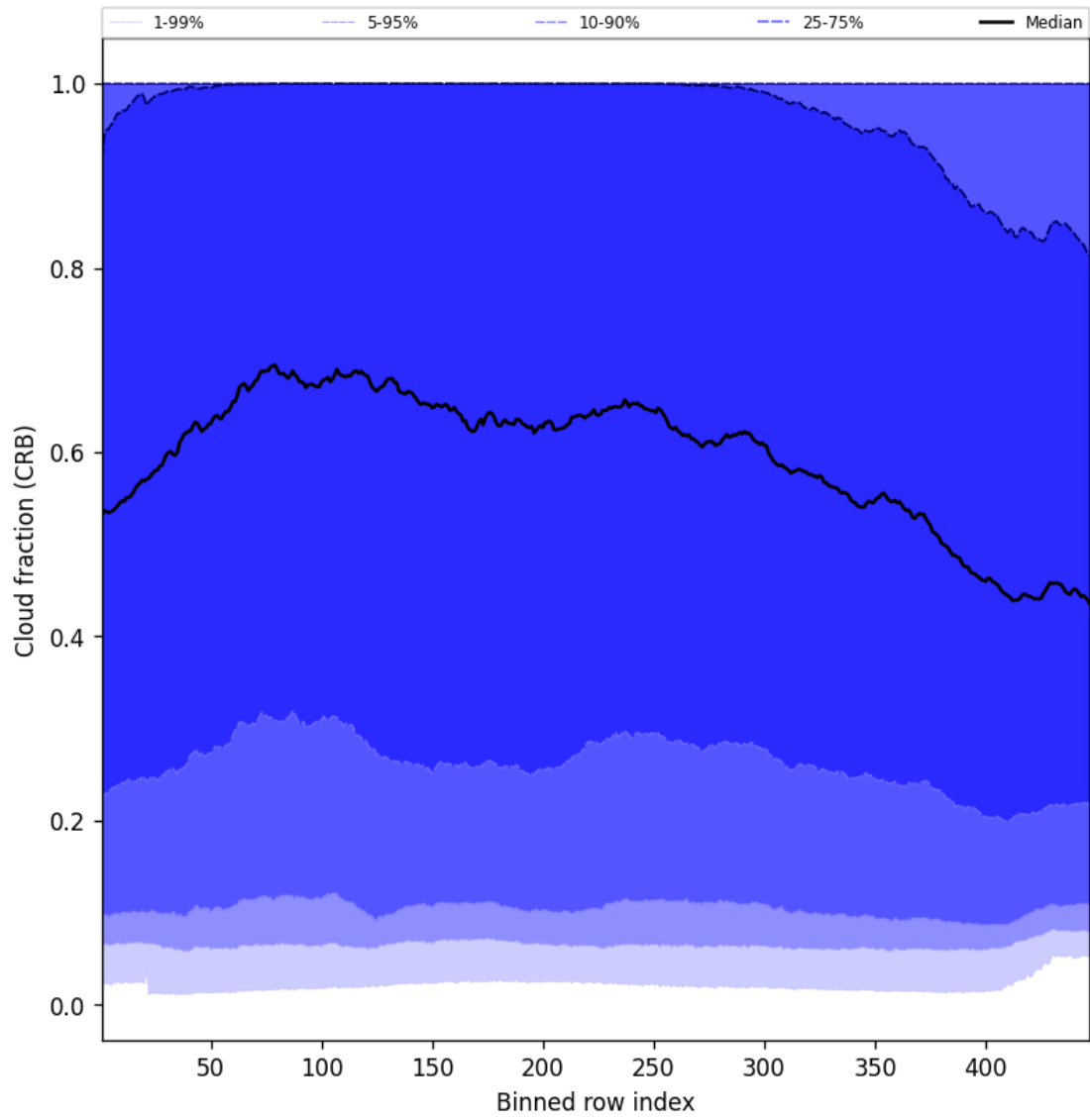
Figure 58: Along track statistics of “Cloud fraction (CRB)” for 2025-07-20 to 2025-07-22
