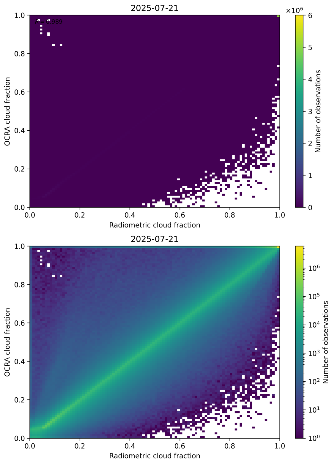
Figure 72: Scatter density plot of “Radiometric cloud fraction” against “OCRA cloud fraction” for 2025-07-20 to 2025-07-22.
