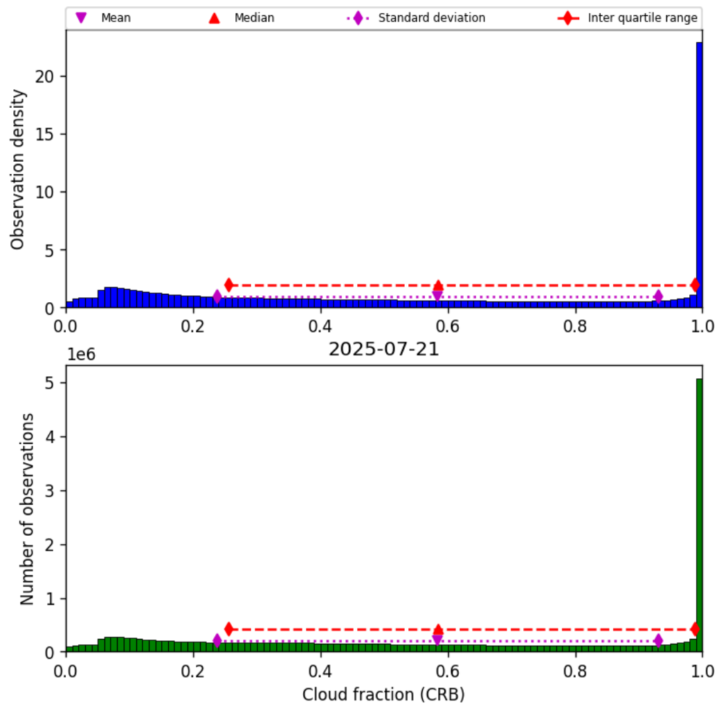
Figure 42: Histogram of “Cloud fraction (CRB)” for 2025-07-20 to 2025-07-22
