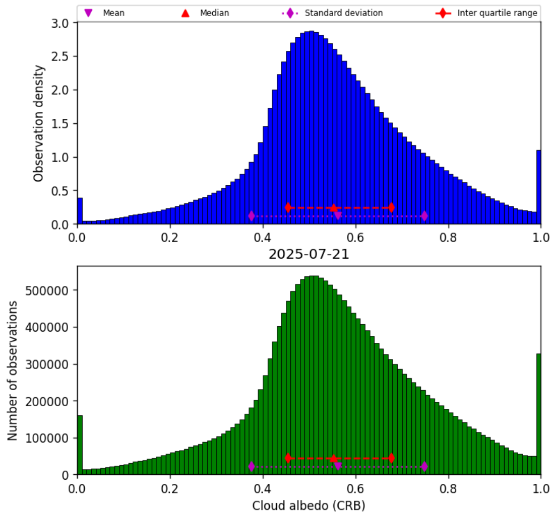
Figure 44: Histogram of “Cloud albedo (CRB)” for 2025-07-20 to 2025-07-22
