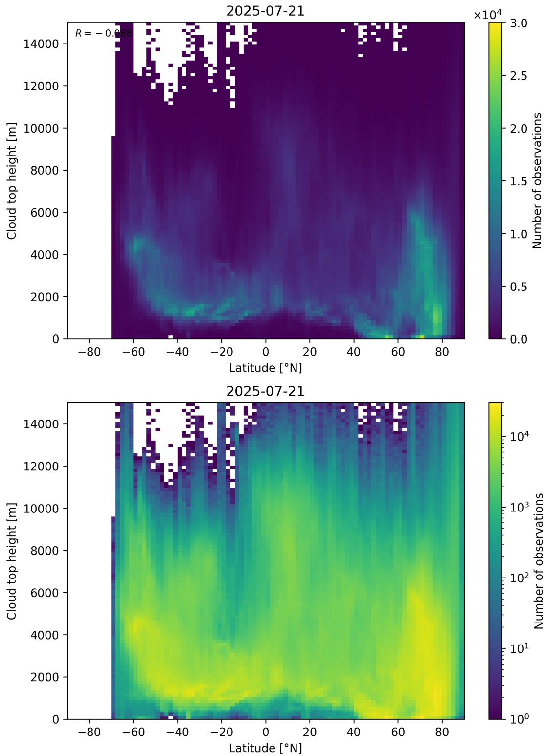
Figure 97: Scatter density plot of “Latitude” against “Cloud top height” for 2025-07-20 to 2025-07-22.
