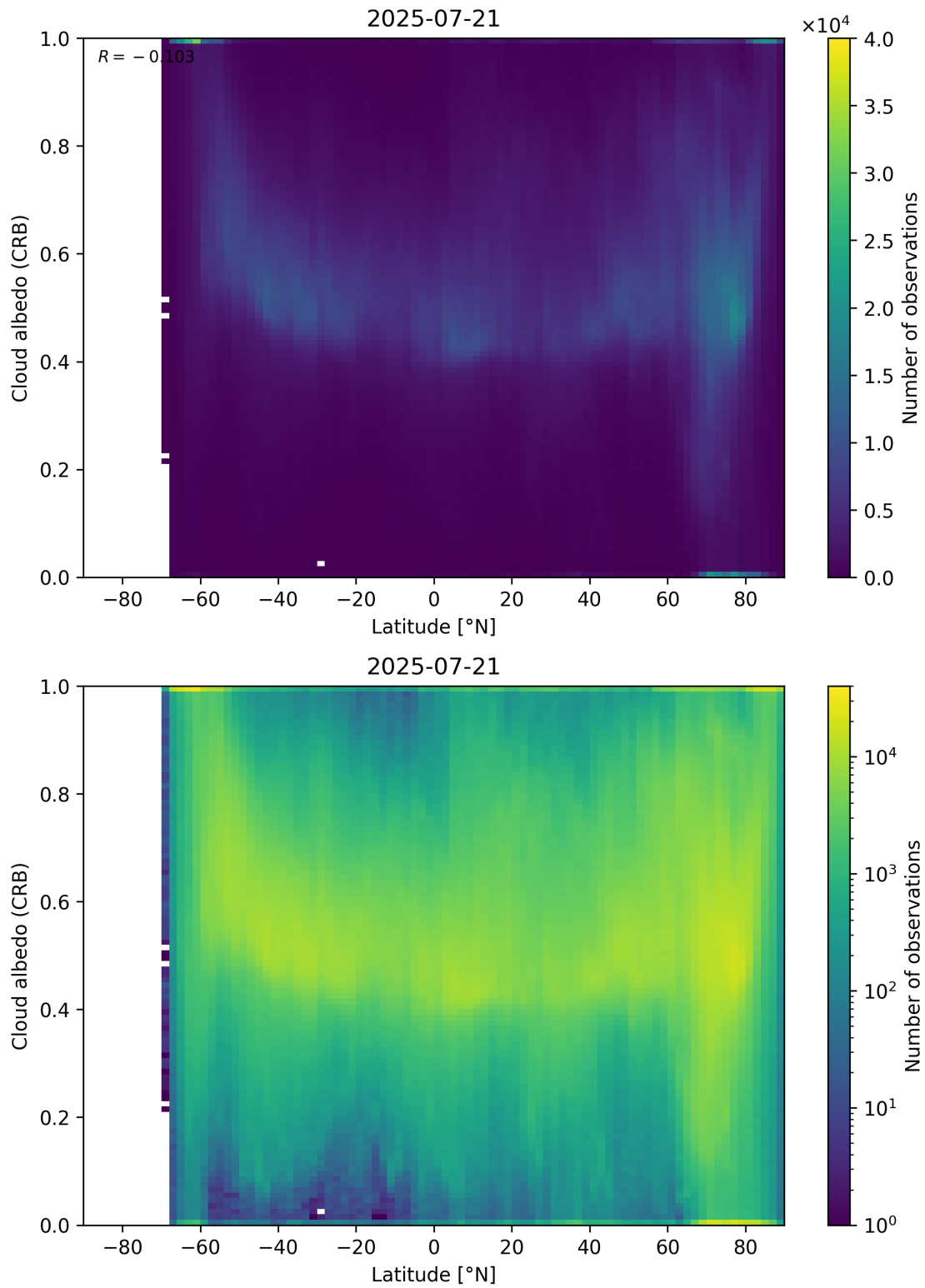
Figure 91: Scatter density plot of “Latitude” against “Cloud albedo (CRB)” for 2025-07-20 to 2025-07-22.
