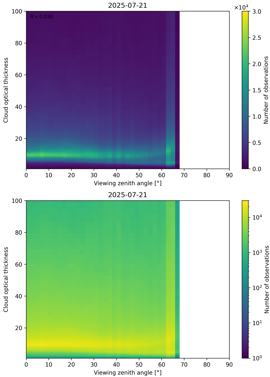
Figure 111: Scatter density plot of “Viewing zenith angle” against “Cloud optical thickness” for 2025-07-20 to 2025-07-22.
