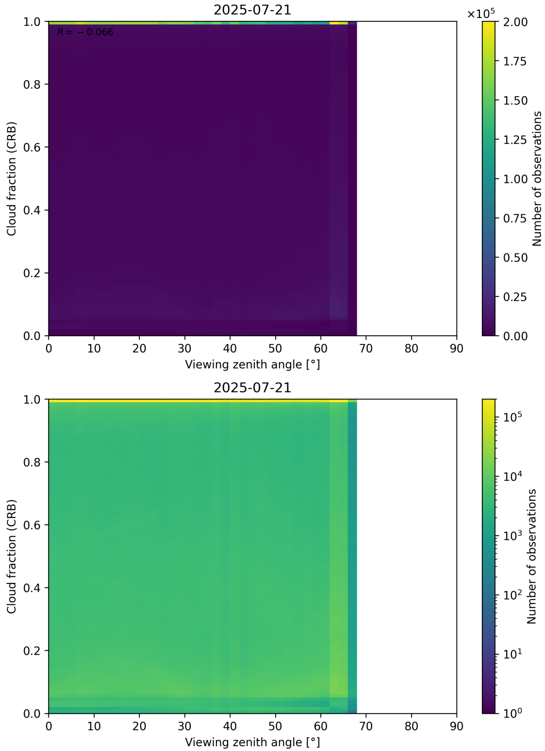
Figure 109: Scatter density plot of “Viewing zenith angle” against “Cloud fraction (CRB)” for 2025-07-20 to 2025-07-22.
