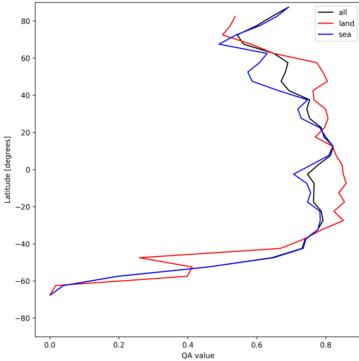
Figure 22: Zonal average of “QA value” for 2025-07-20 to 2025-07-22.
