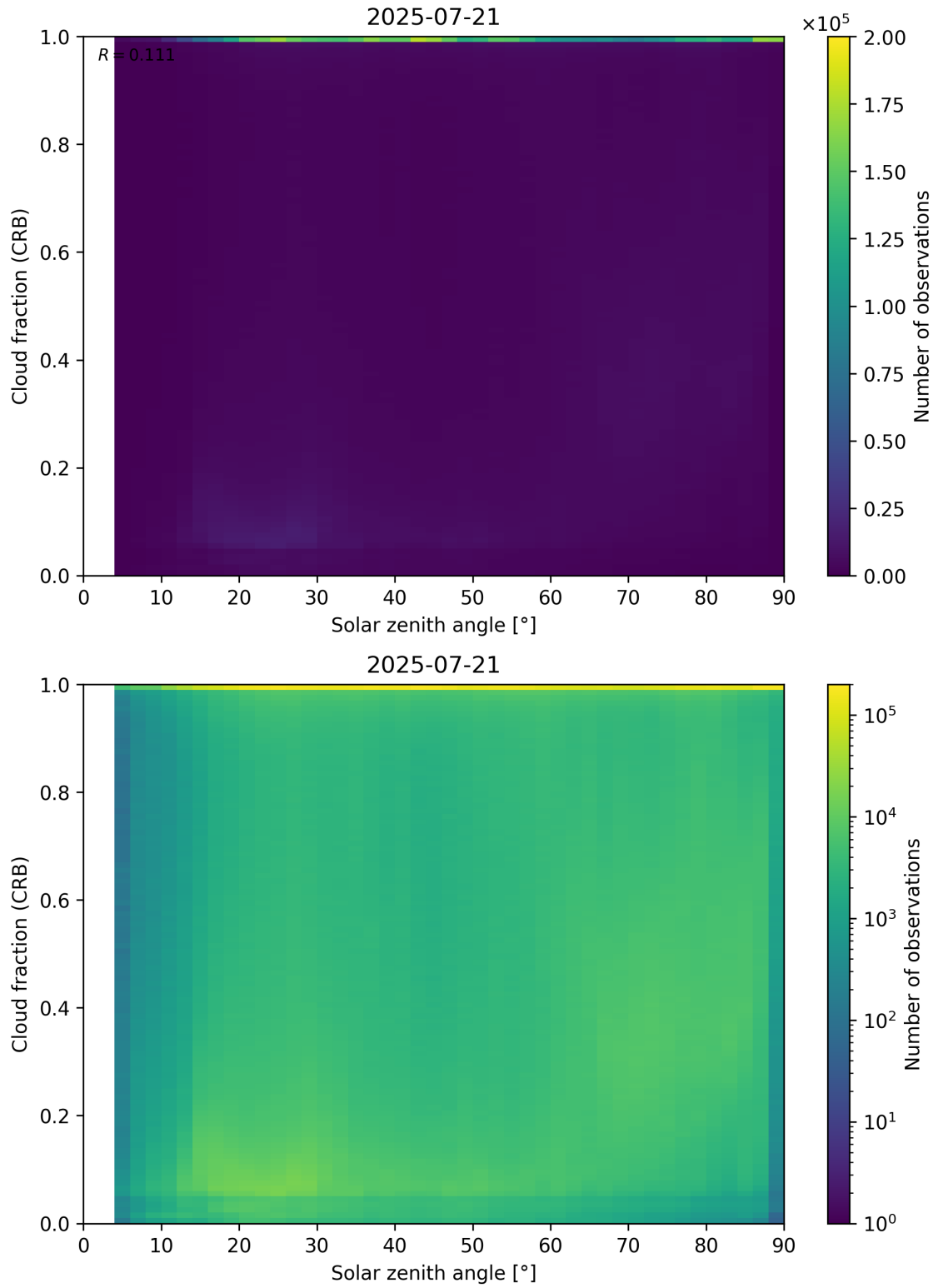
Figure 101: Scatter density plot of “Solar zenith angle” against “Cloud fraction (CRB)” for 2025-07-20 to 2025-07-22.
