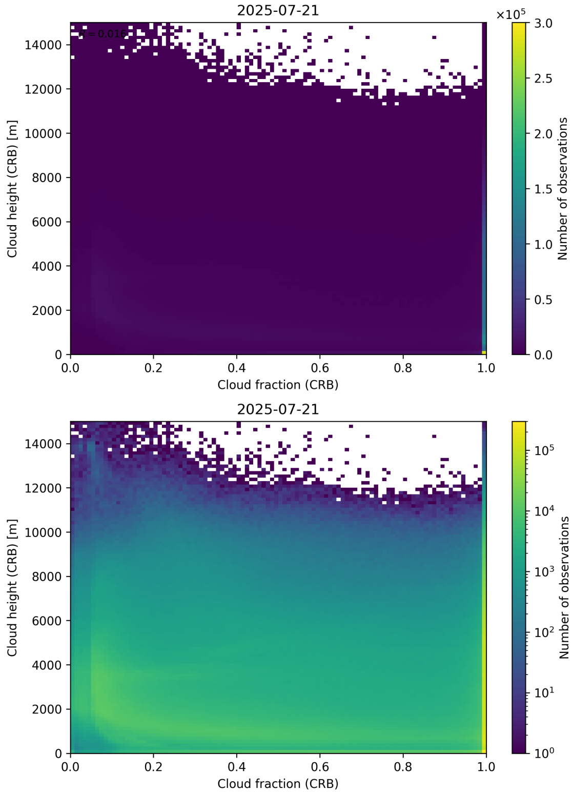
Figure 79: Scatter density plot of “Cloud fraction (CRB)” against “Cloud height (CRB)” for 2025-07-20 to 2025-07-22.
