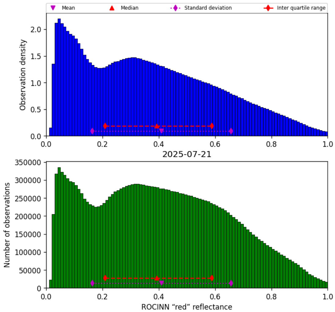
Figure 53: Histogram of “ROCINN “red” reflectance” for 2025-07-20 to 2025-07-22
