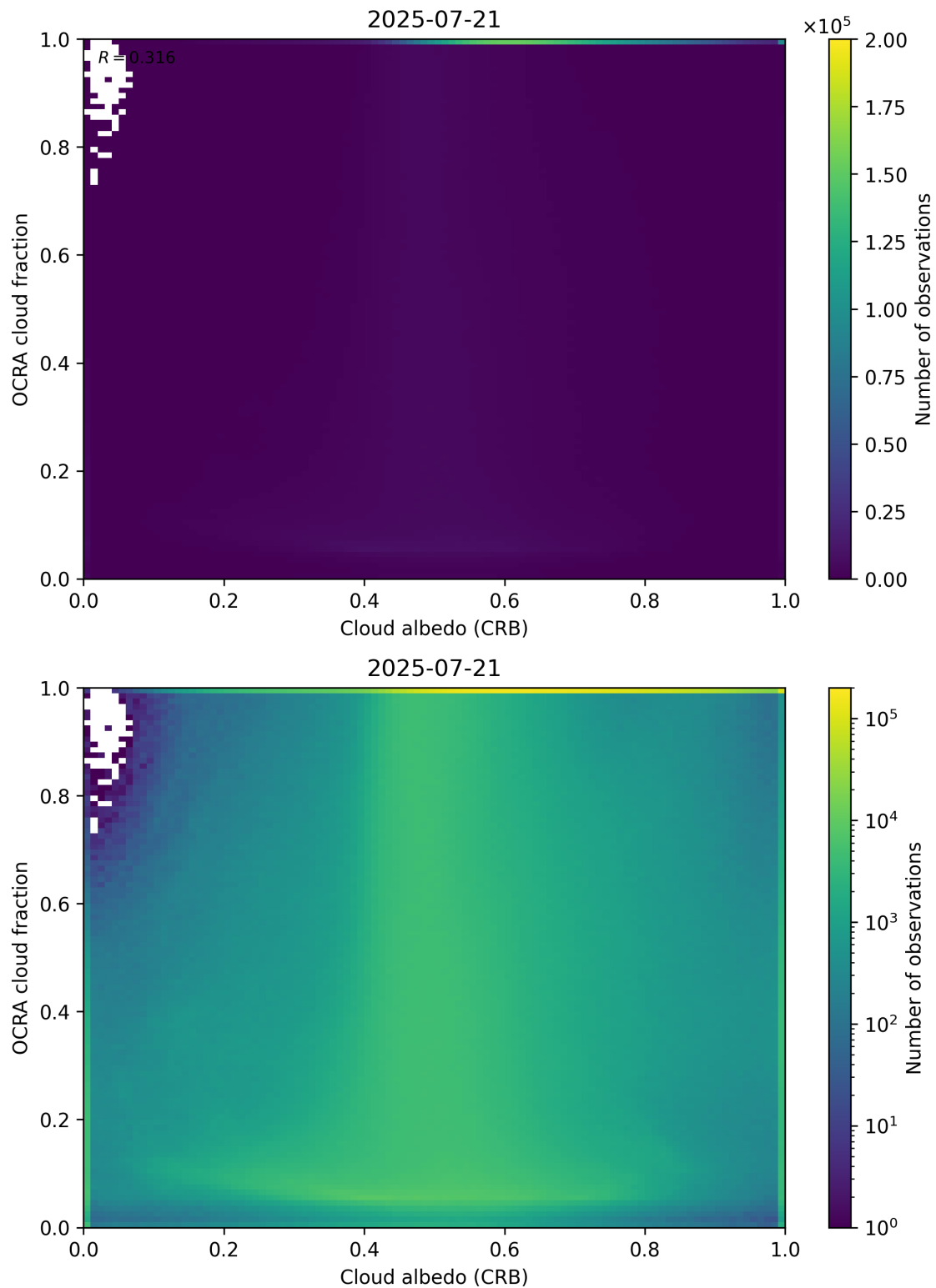
Figure 70: Scatter density plot of “Cloud albedo (CRB)” against “OCRA cloud fraction” for 2025-07-20 to 2025-07-22.
