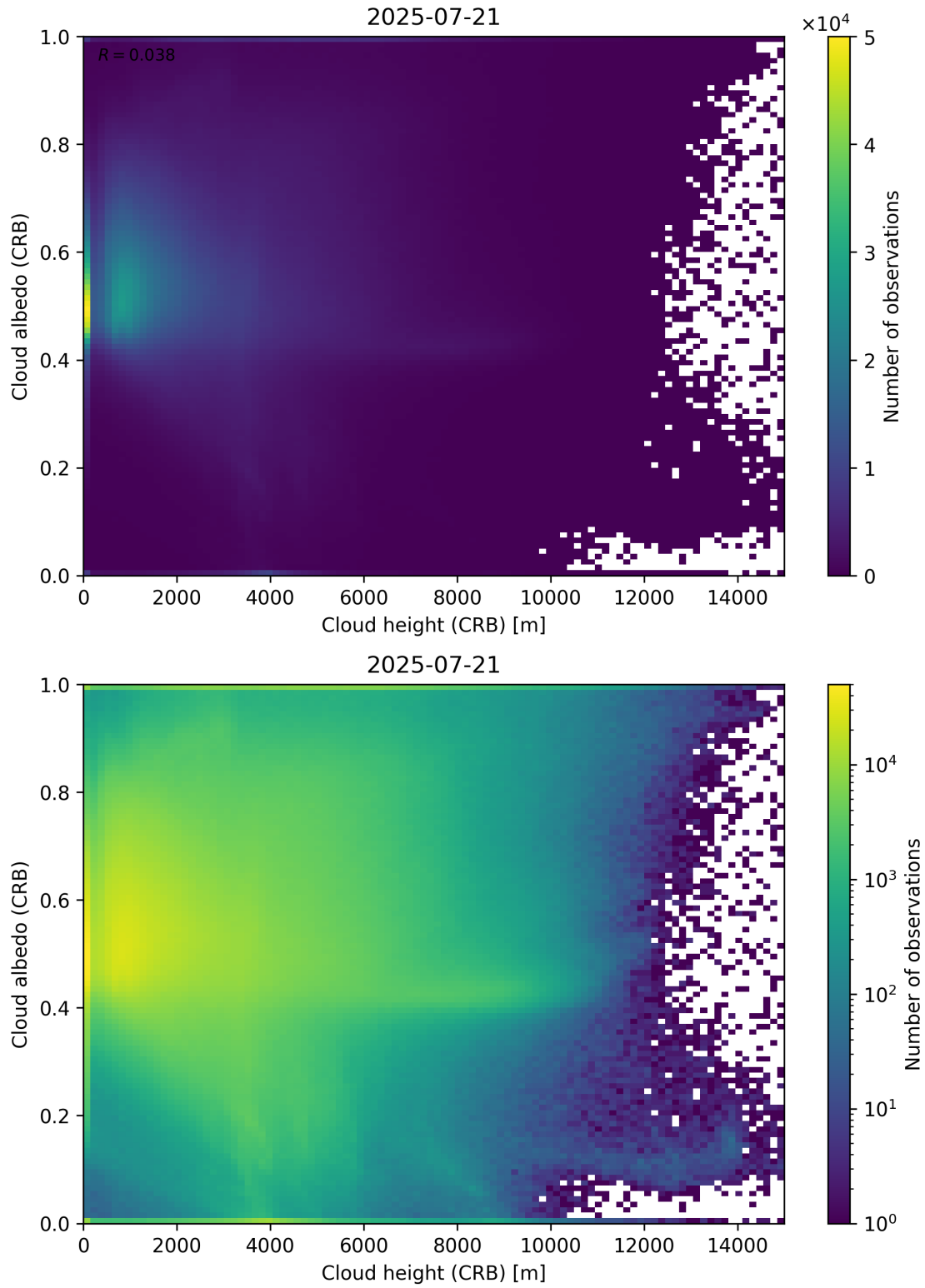
Figure 80: Scatter density plot of “Cloud height (CRB)” against “Cloud albedo (CRB)” for 2025-07-20 to 2025-07-22.
