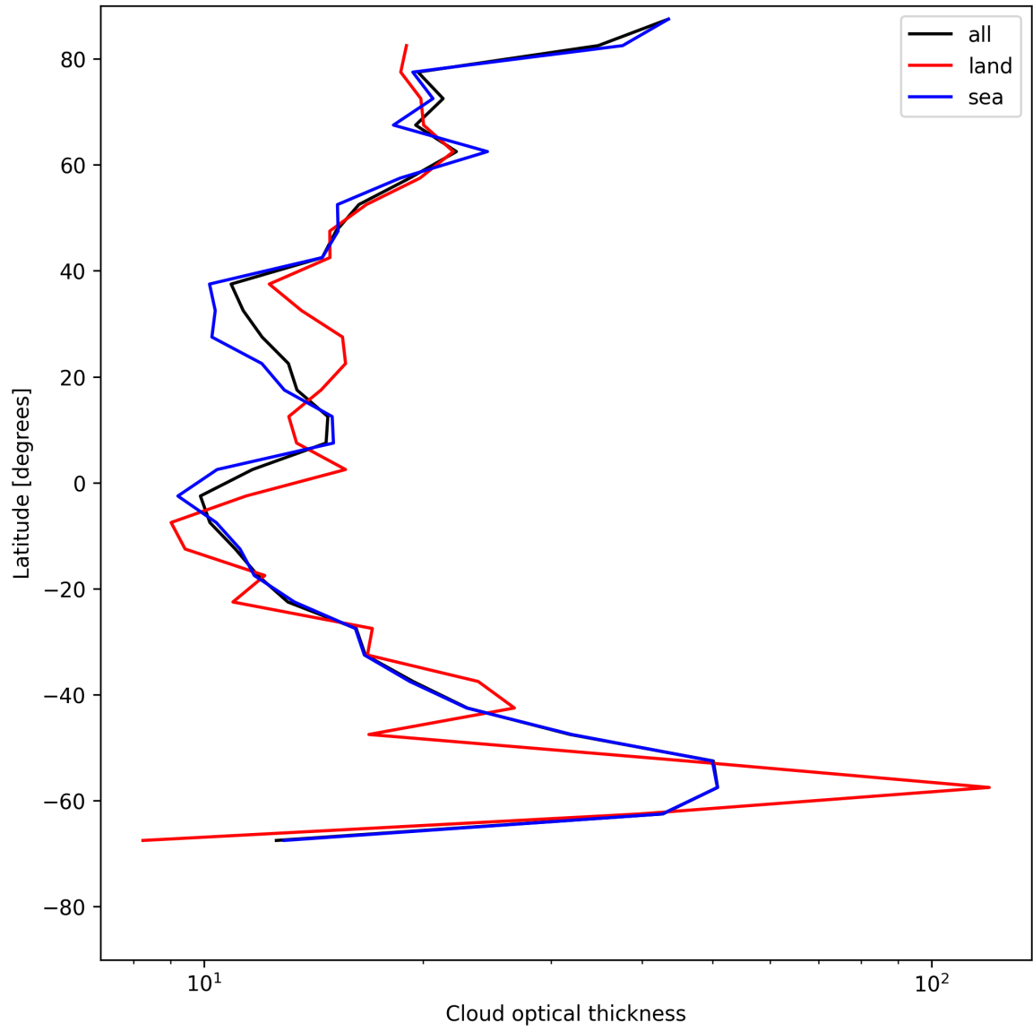
Figure 25: Zonal average of “Cloud optical thickness” for 2025-07-20 to 2025-07-22.
