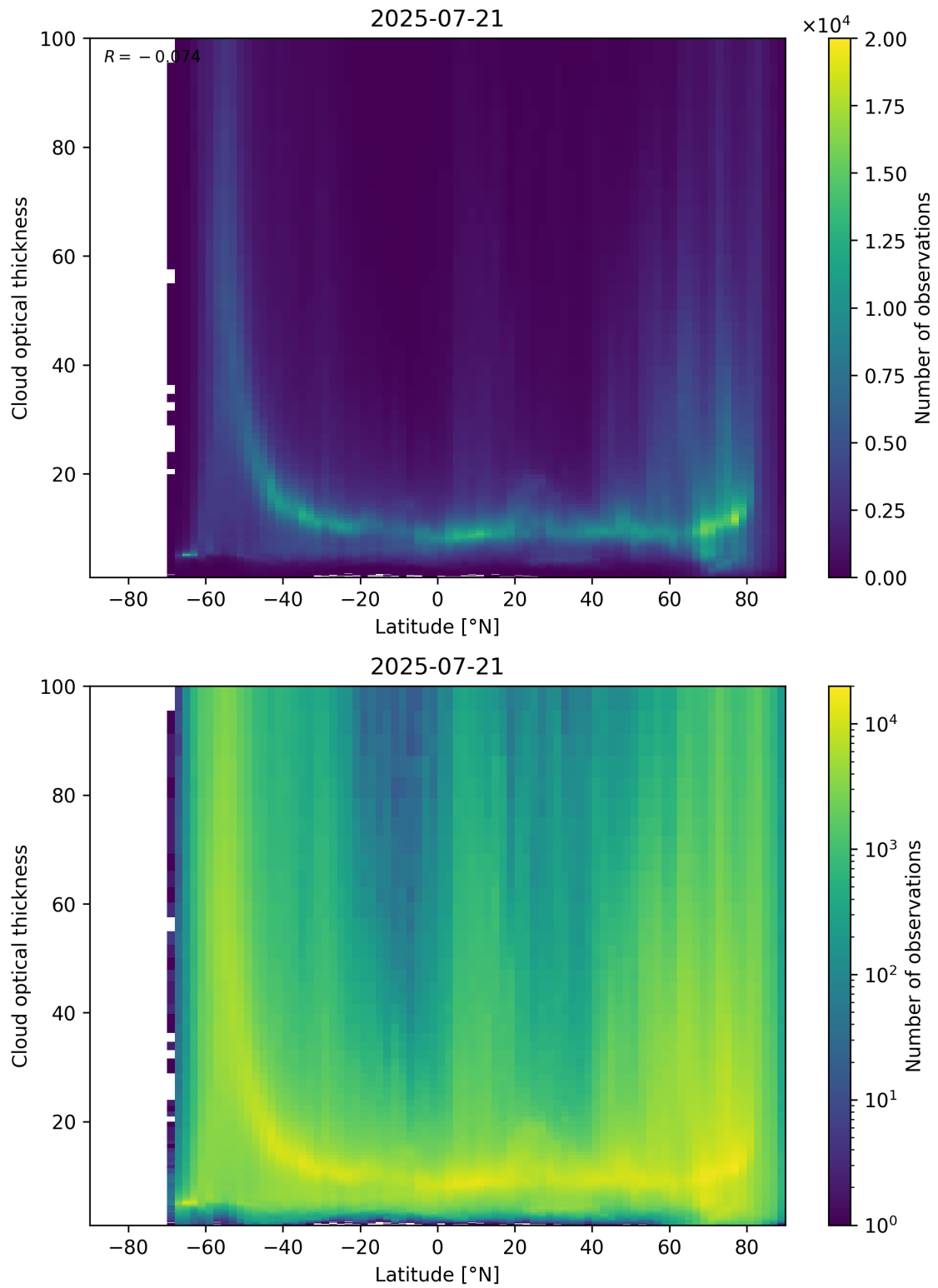
Figure 96: Scatter density plot of “Latitude” against “Cloud optical thickness” for 2025-07-20 to 2025-07-22.
