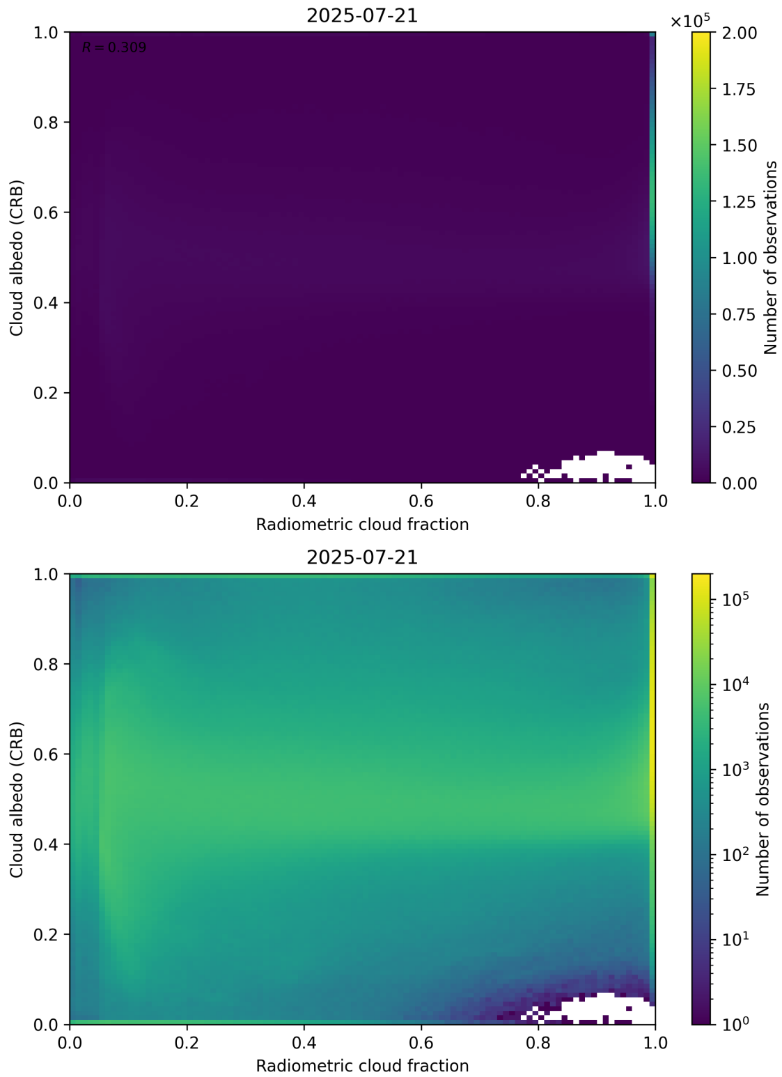
Figure 71: Scatter density plot of “Radiometric cloud fraction” against “Cloud albedo (CRB)” for 2025-07-20 to 2025-07-22.
