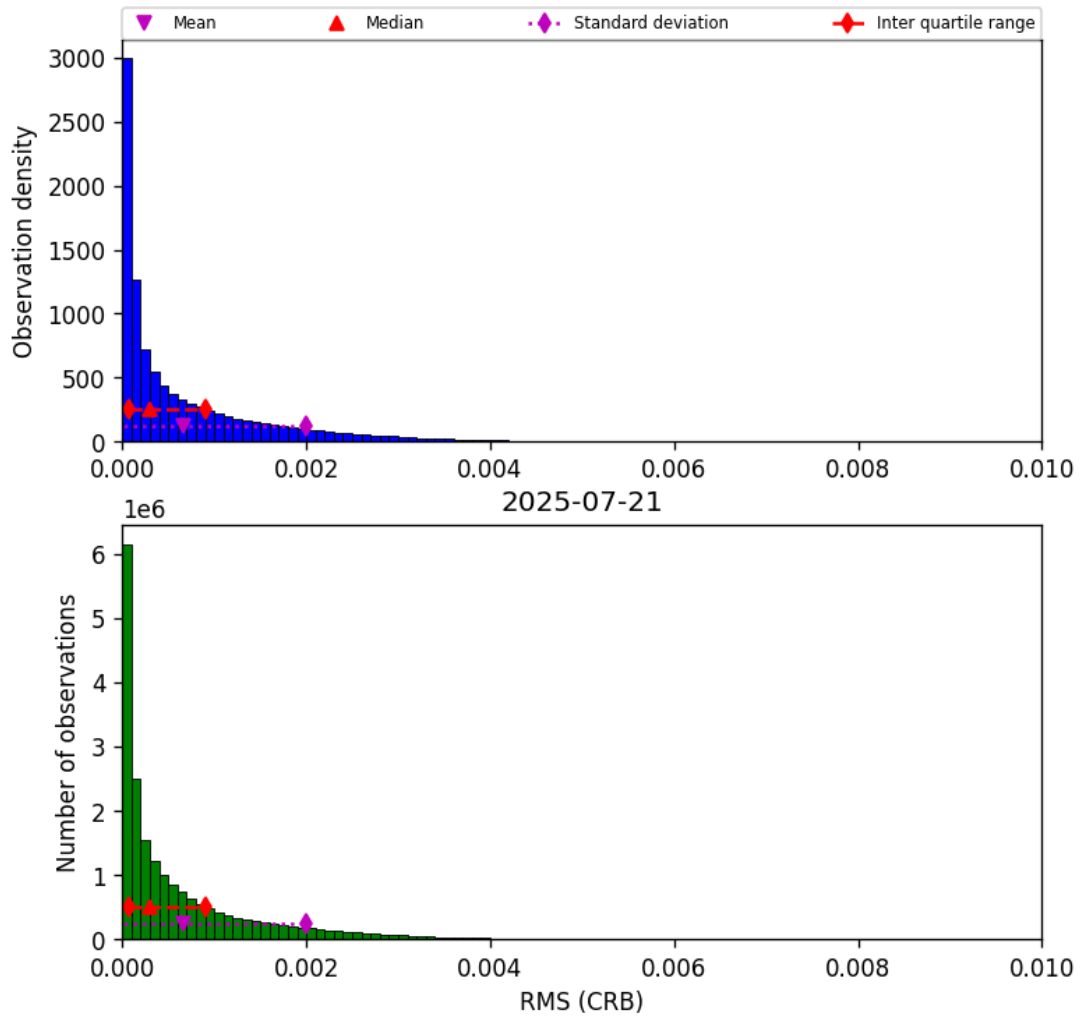
Figure 48: Histogram of “RMS (CRB)” for 2025-07-20 to 2025-07-22
