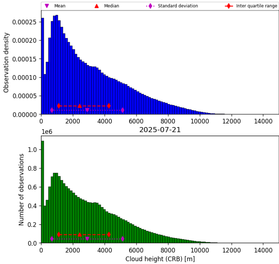
Figure 43: Histogram of “Cloud height (CRB)” for 2025-07-20 to 2025-07-22
