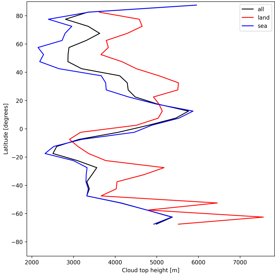
Figure 24: Zonal average of “Cloud top height” for 2025-07-20 to 2025-07-22.
