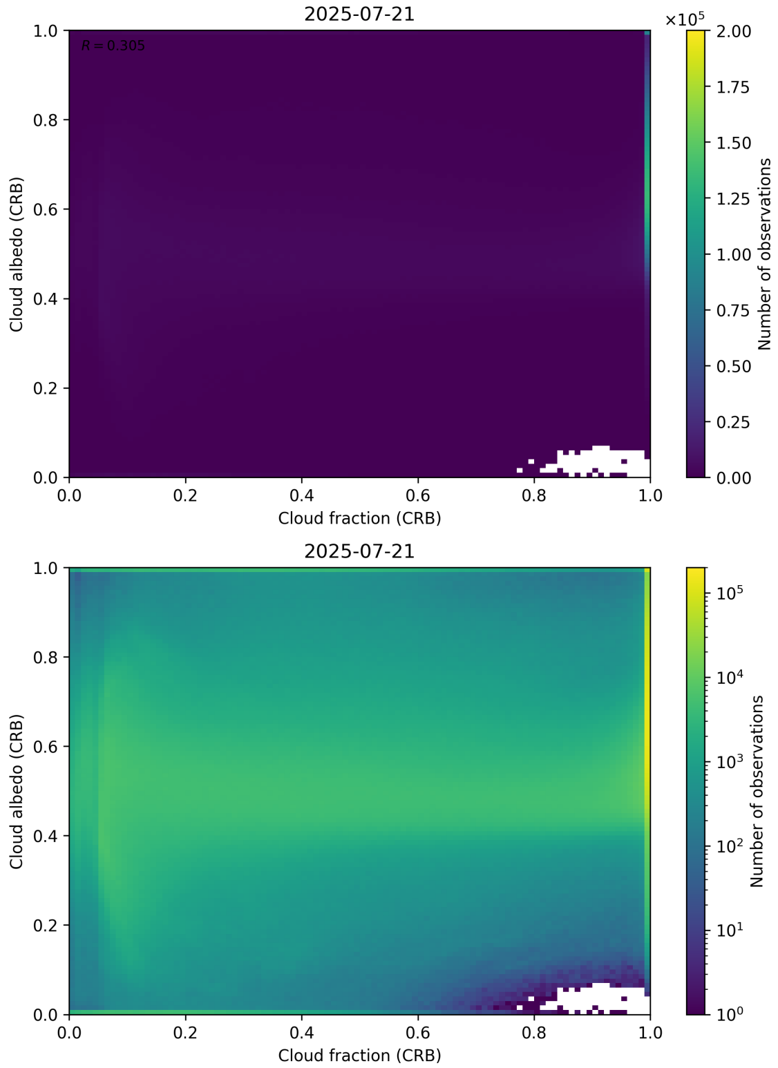
Figure 77: Scatter density plot of “Cloud fraction (CRB)” against “Cloud albedo (CRB)” for 2025-07-20 to 2025-07-22.
