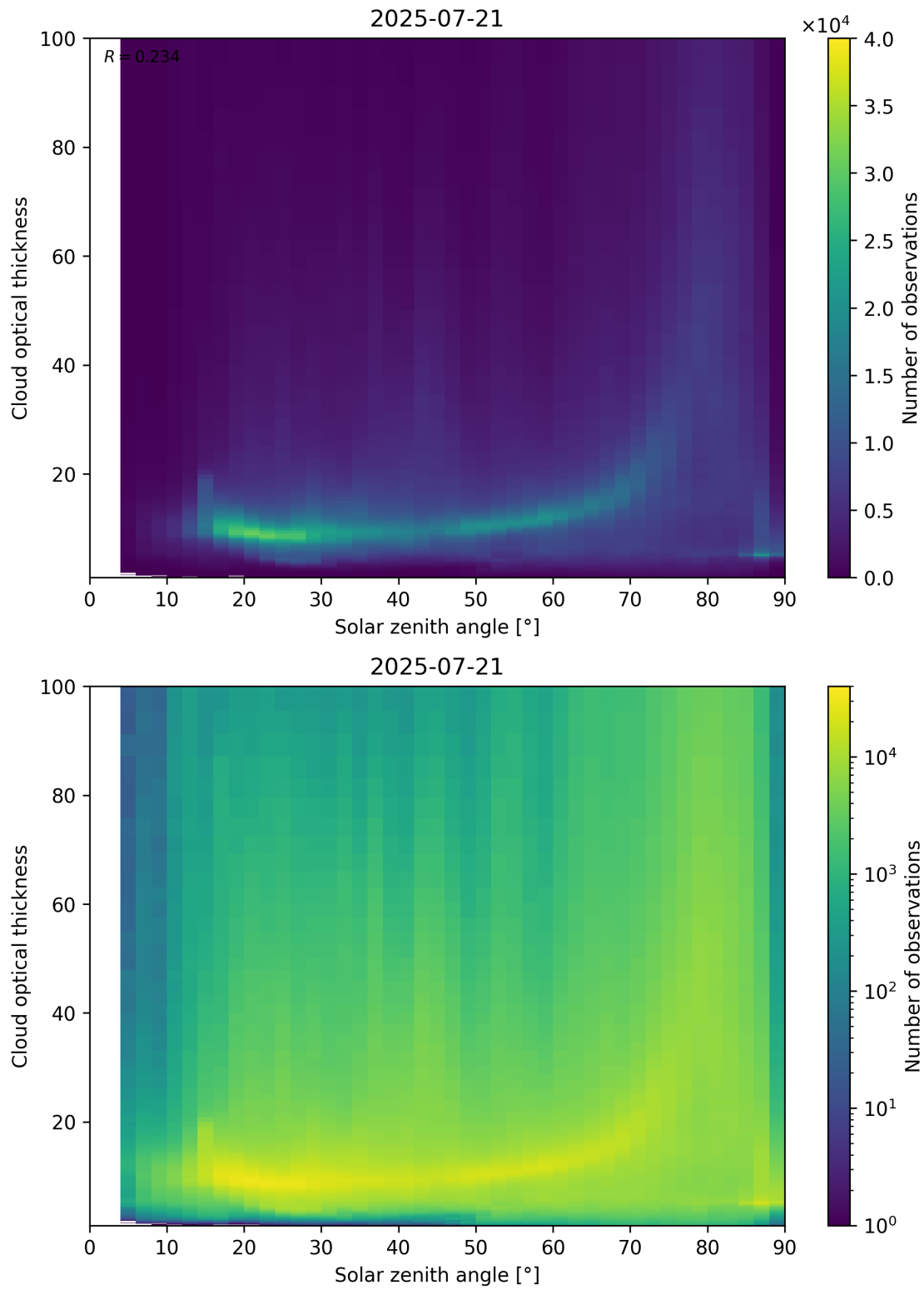
Figure 103: Scatter density plot of “Solar zenith angle” against “Cloud optical thickness” for 2025-07-20 to 2025-07-22.
