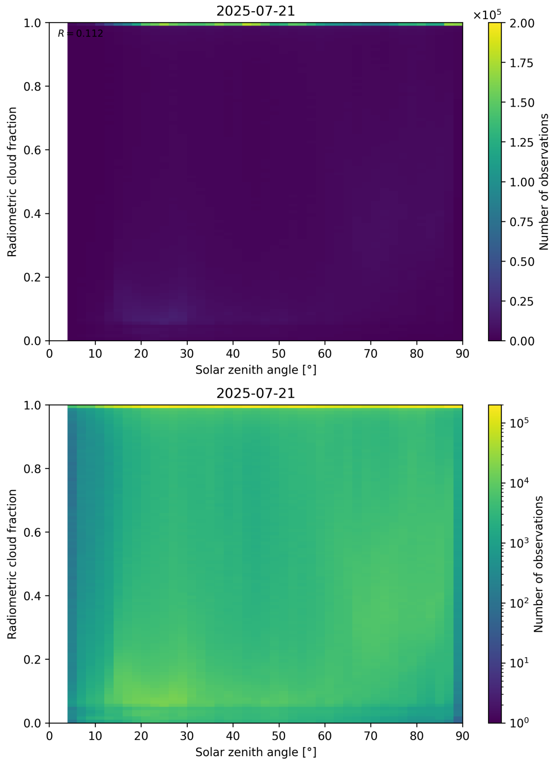
Figure 99: Scatter density plot of “Solar zenith angle” against “Radiometric cloud fraction” for 2025-07-20 to 2025-07-22.
