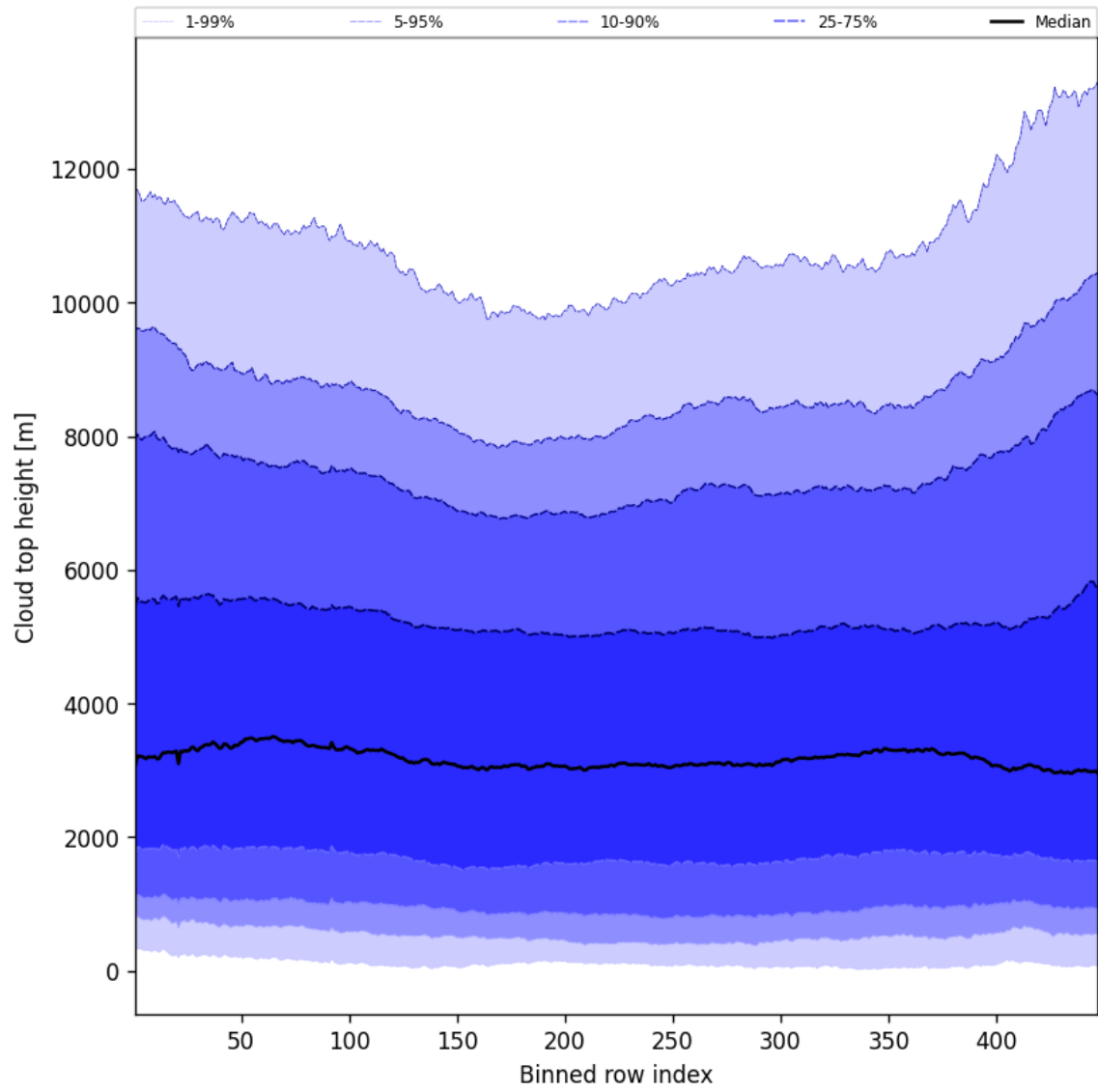
Figure 56: Along track statistics of “Cloud top height” for 2025-07-20 to 2025-07-22
