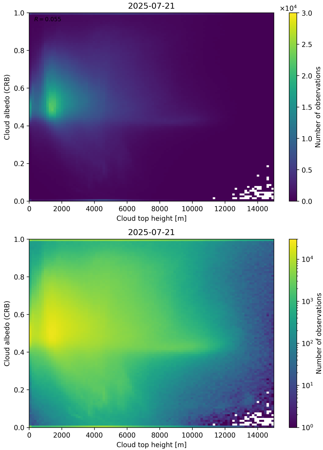
Figure 86: Scatter density plot of “Cloud top height” against “Cloud albedo (CRB)” for 2025-07-20 to 2025-07-22.
