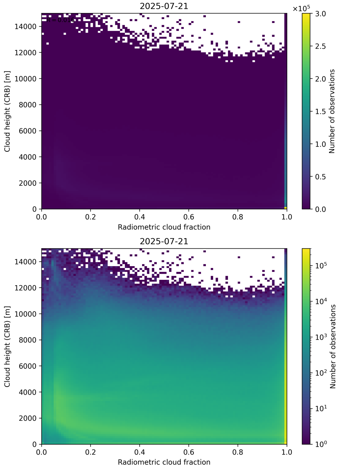
Figure 74: Scatter density plot of “Radiometric cloud fraction” against “Cloud height (CRB)” for 2025-07-20 to 2025-07-22.
