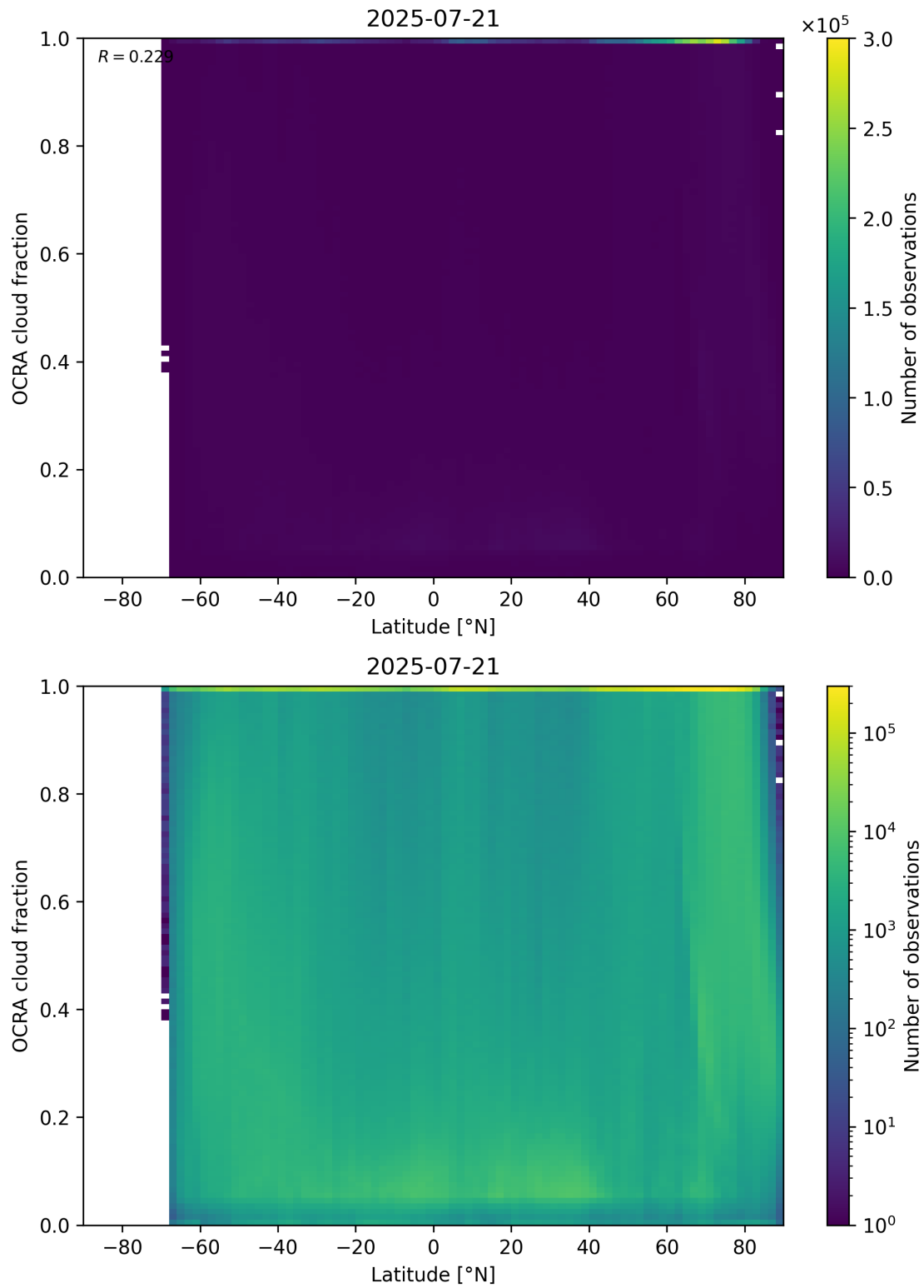
Figure 93: Scatter density plot of “Latitude” against “OCRA cloud fraction” for 2025-07-20 to 2025-07-22.
