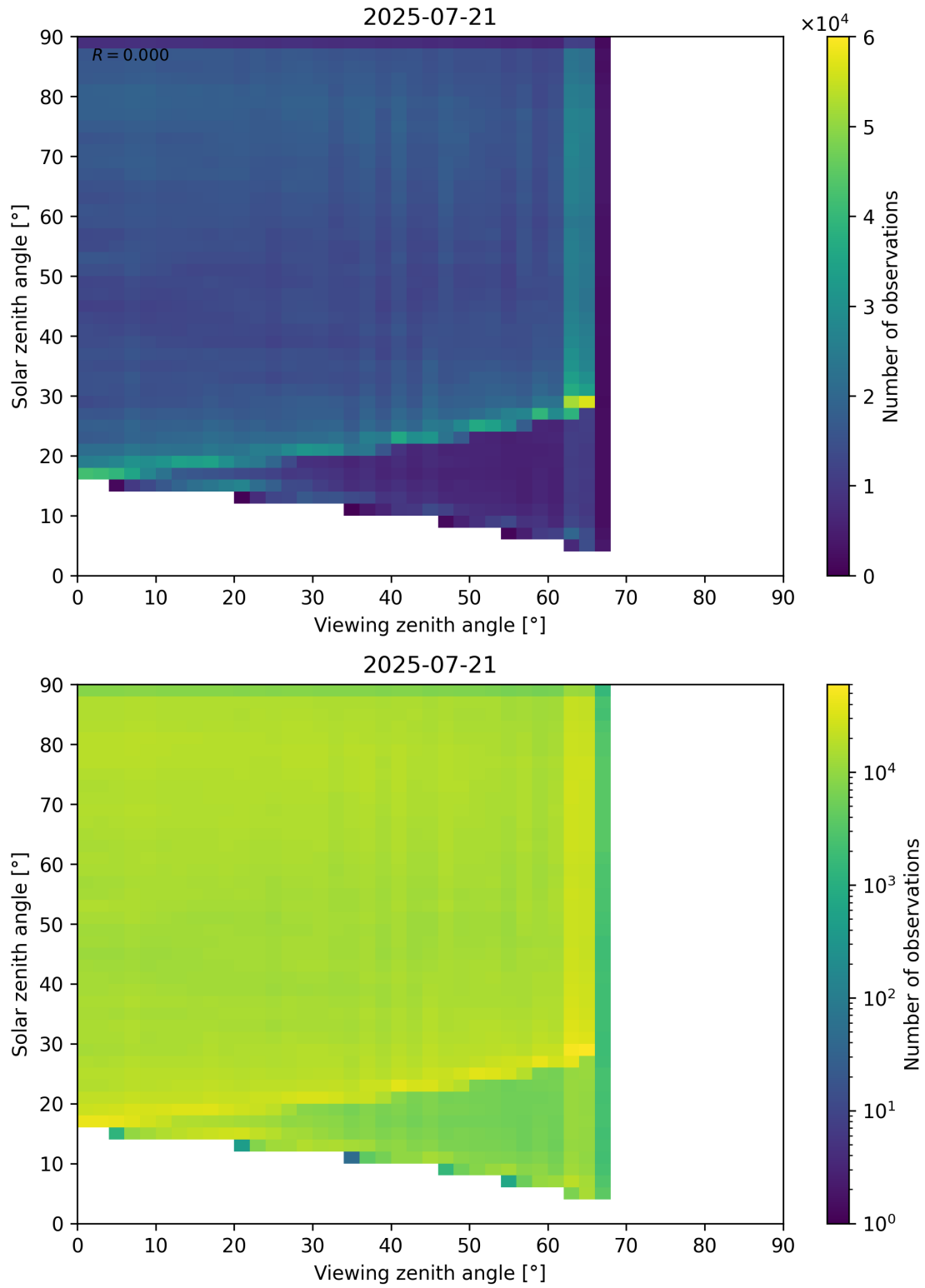
Figure 114: Scatter density plot of “Viewing zenith angle” against “Solar zenith angle” for 2025-07-20 to 2025-07-22.
