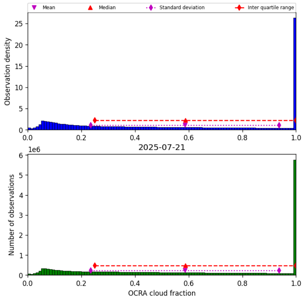
Figure 50: Histogram of “OCRA cloud fraction” for 2025-07-20 to 2025-07-22
