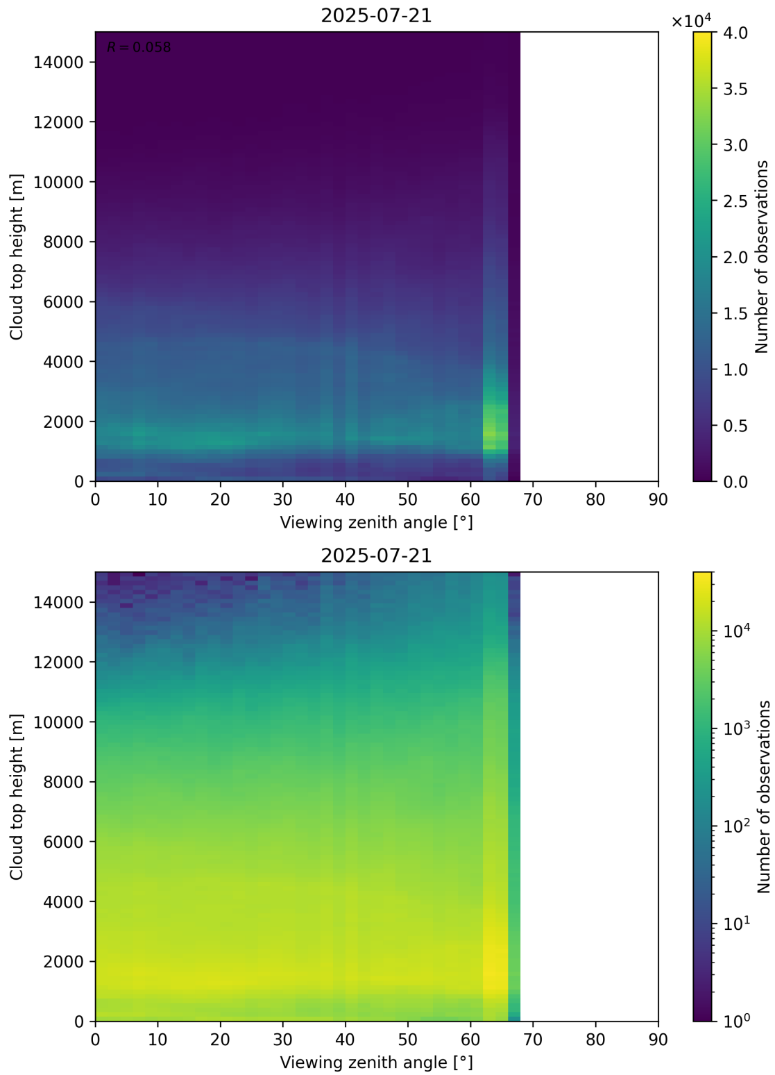
Figure 112: Scatter density plot of “Viewing zenith angle” against “Cloud top height” for 2025-07-20 to 2025-07-22.
