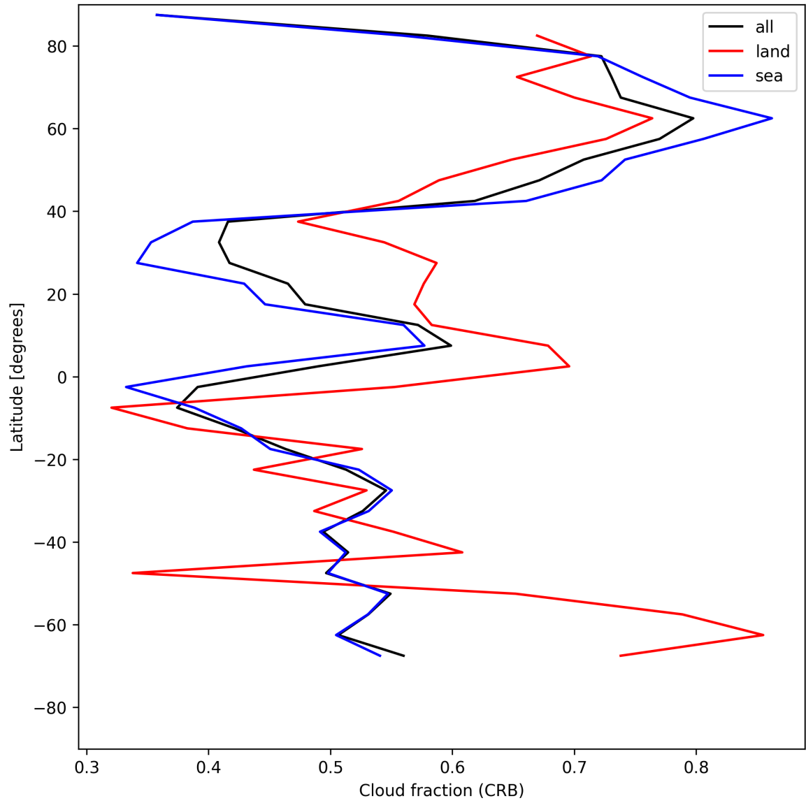
Figure 26: Zonal average of “Cloud fraction (CRB)” for 2025-07-20 to 2025-07-22.
