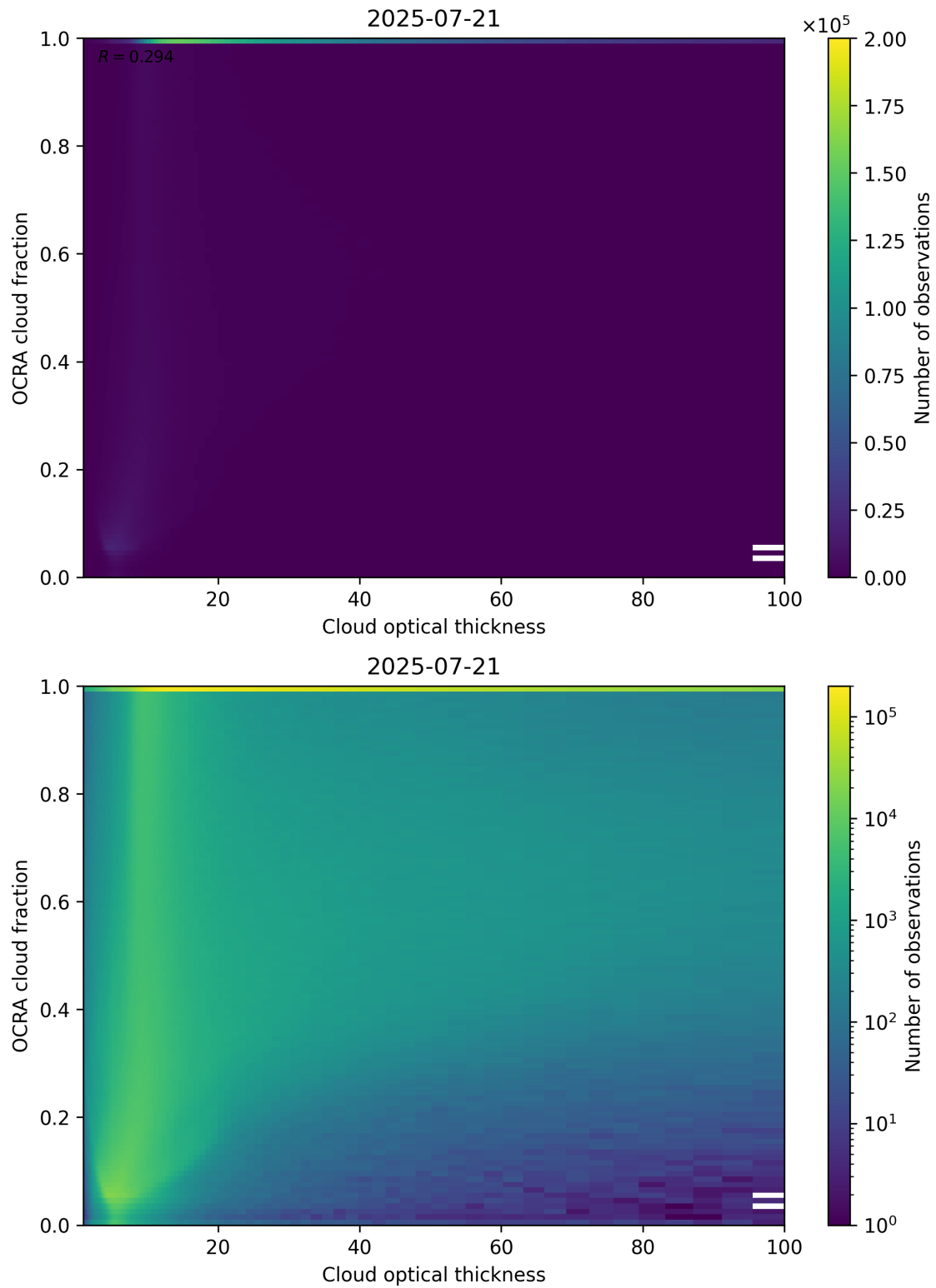
Figure 83: Scatter density plot of “Cloud optical thickness” against “OCRA cloud fraction” for 2025-07-20 to 2025-07-22.
