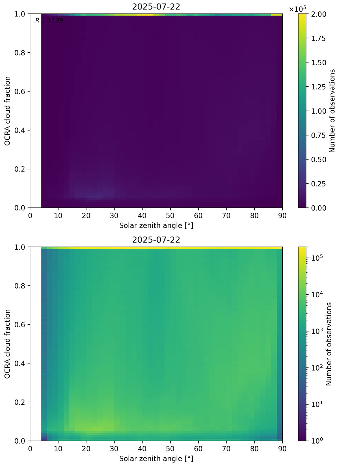
Figure 100: Scatter density plot of “Solar zenith angle” against “OCRA cloud fraction” for 2025-07-21 to 2025-07-23.
