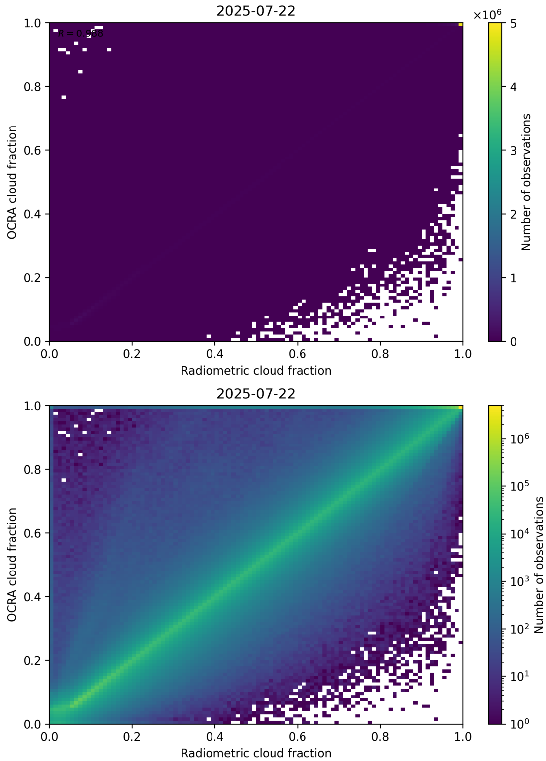
Figure 72: Scatter density plot of “Radiometric cloud fraction” against “OCRA cloud fraction” for 2025-07-21 to 2025-07-23.
