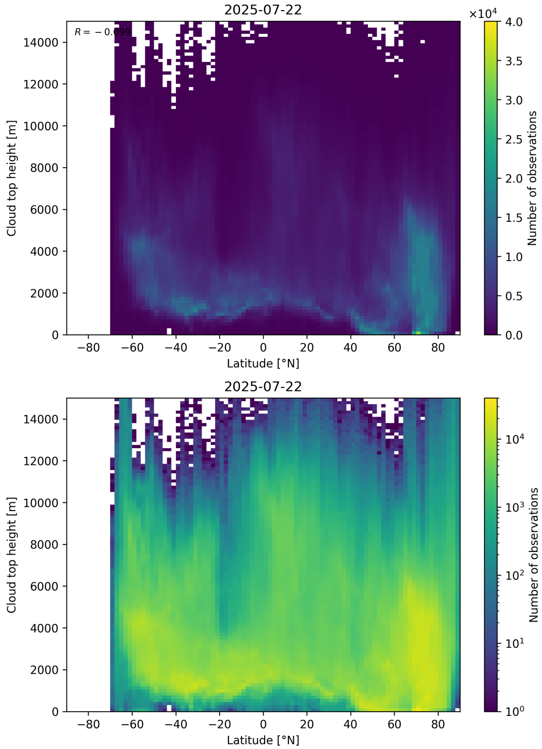
Figure 97: Scatter density plot of “Latitude” against “Cloud top height” for 2025-07-21 to 2025-07-23.
