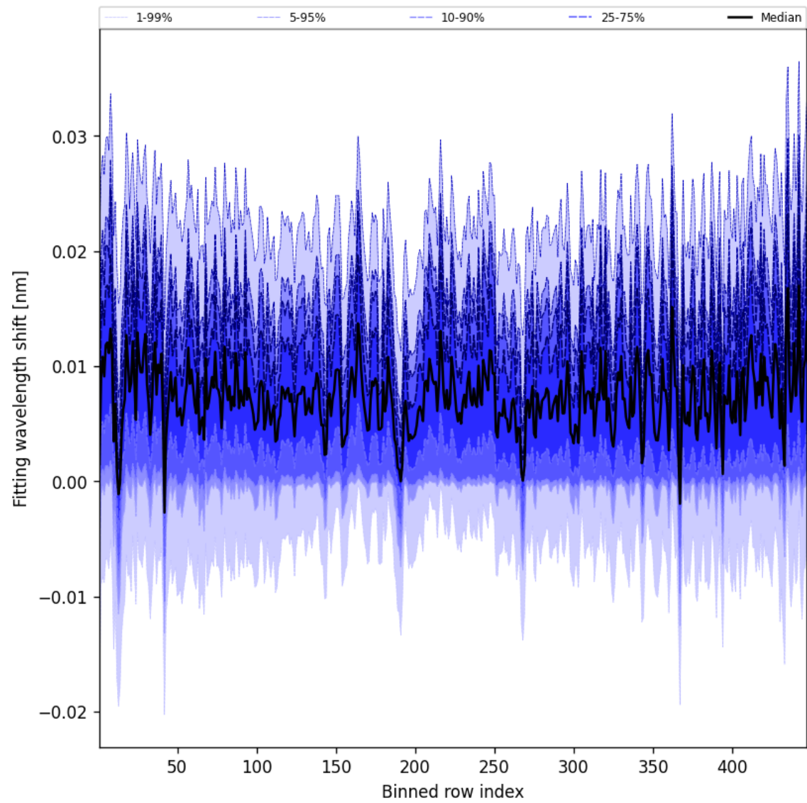
Figure 65: Along track statistics of “Fitting wavelength shift” for 2025-07-21 to 2025-07-23
