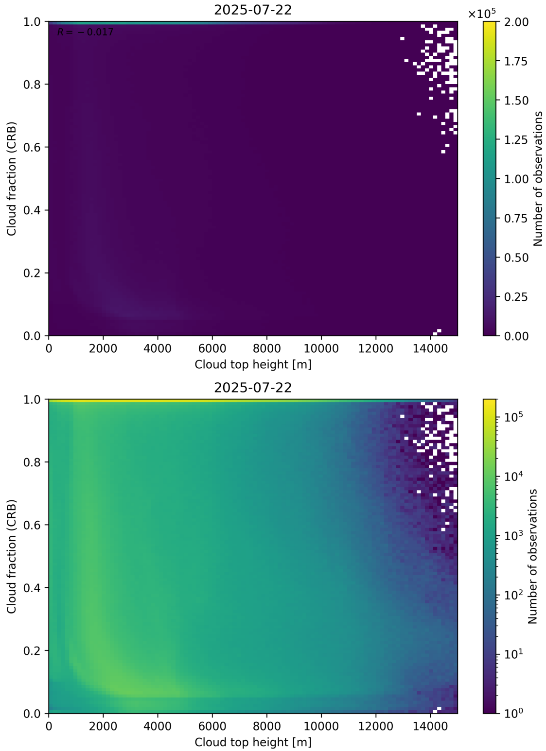
Figure 88: Scatter density plot of “Cloud top height” against “Cloud fraction (CRB)” for 2025-07-21 to 2025-07-23.
