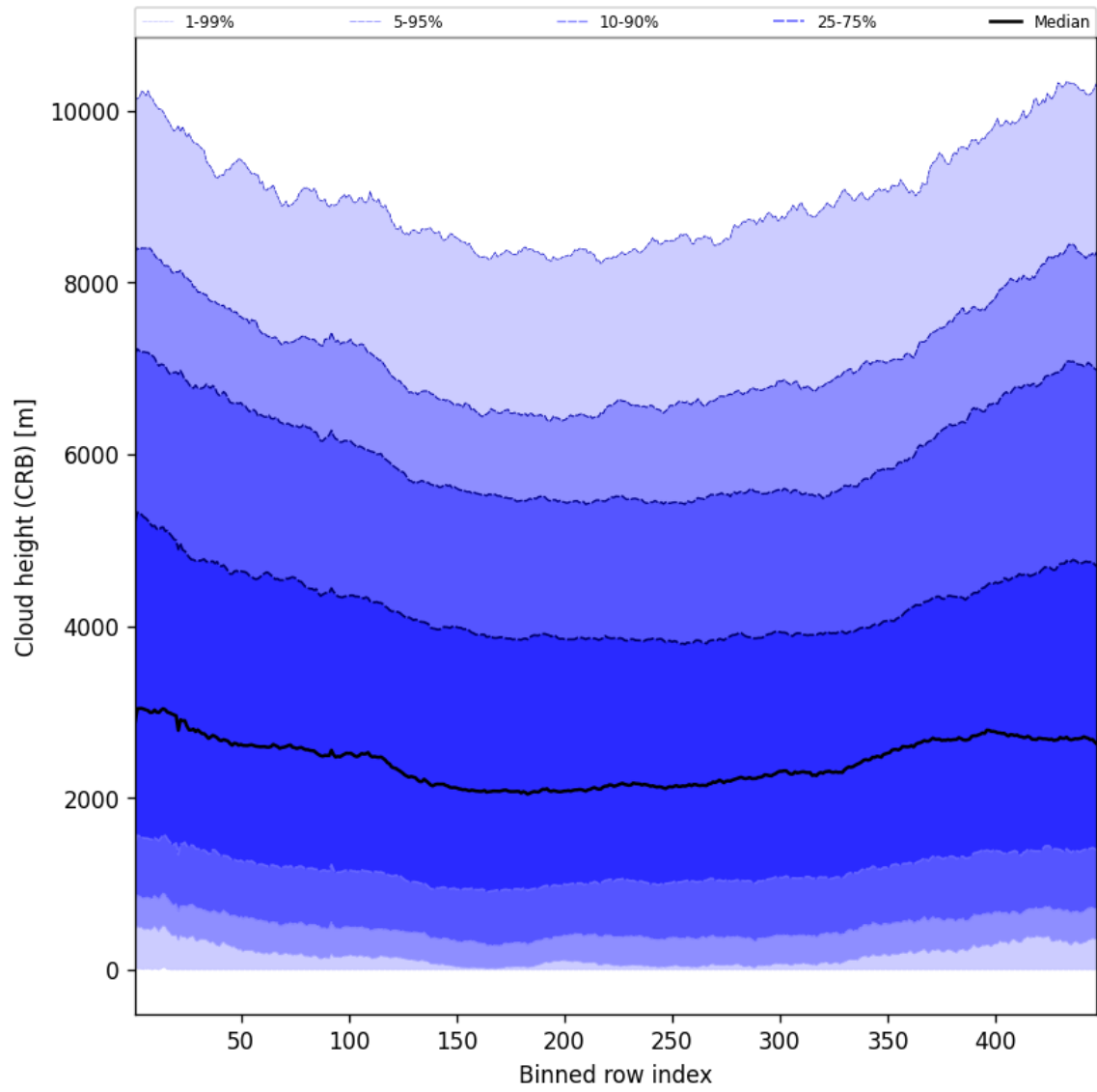
Figure 59: Along track statistics of “Cloud height (CRB)” for 2025-07-21 to 2025-07-23
