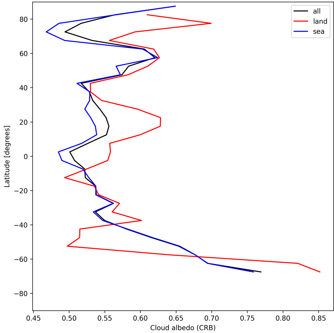
Figure 28: Zonal average of “Cloud albedo (CRB)” for 2025-07-21 to 2025-07-23.
