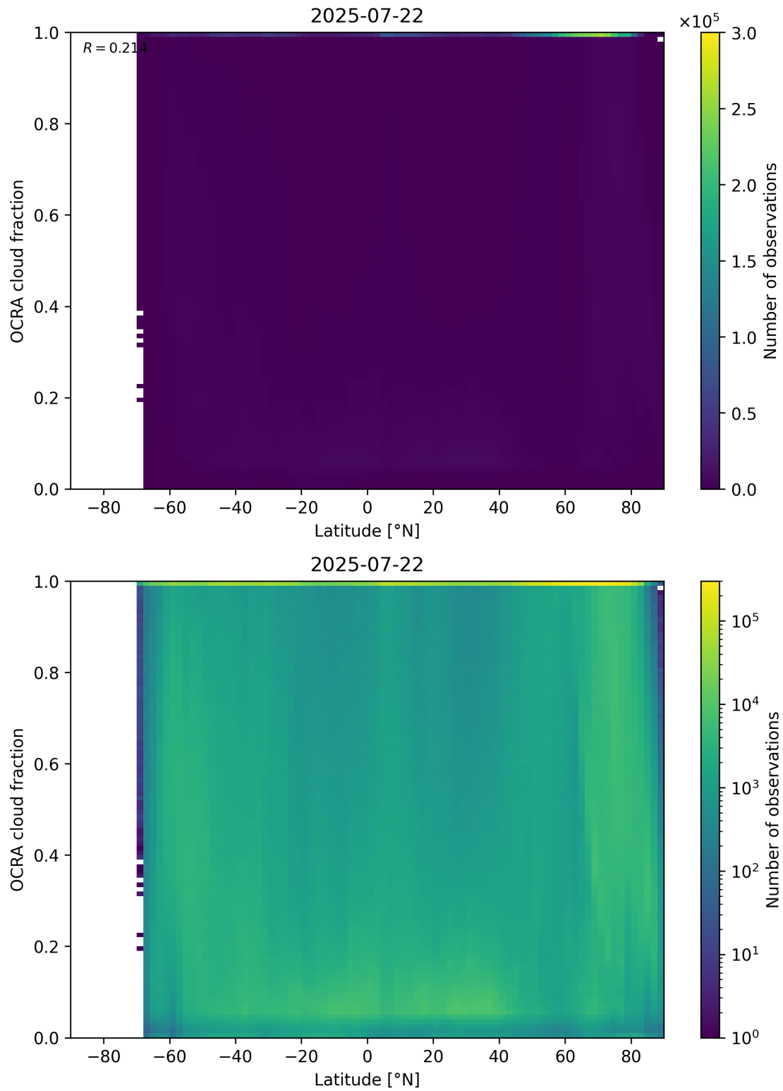
Figure 93: Scatter density plot of “Latitude” against “OCRA cloud fraction” for 2025-07-21 to 2025-07-23.
