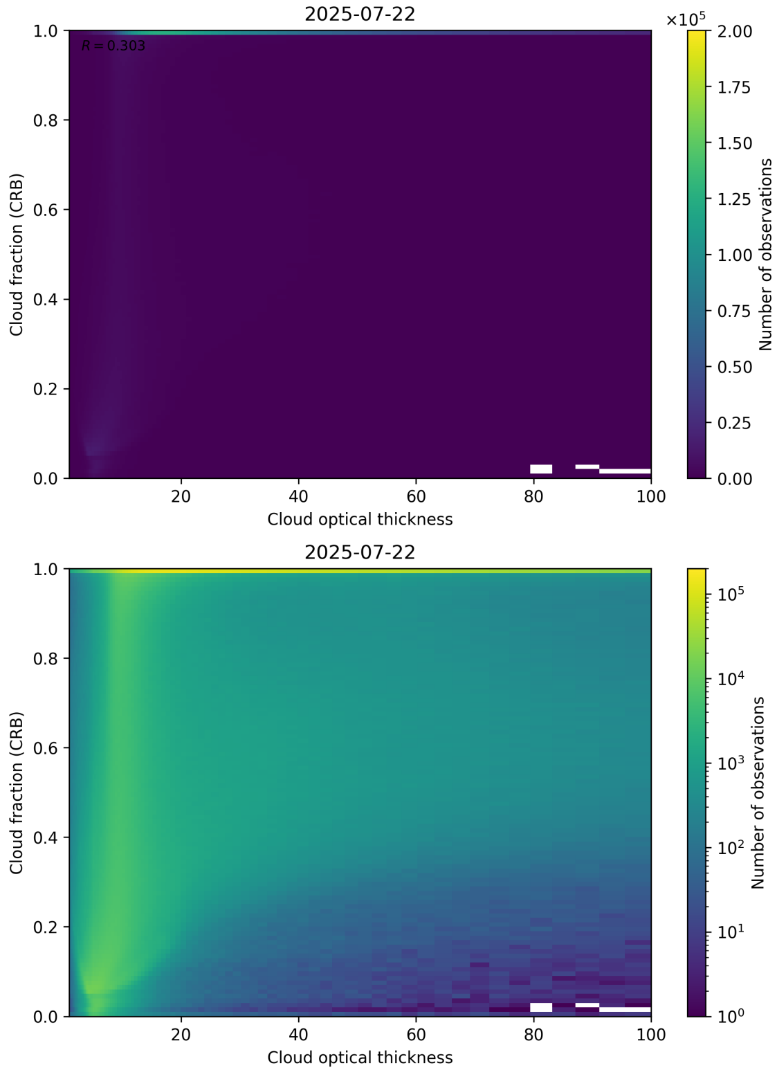
Figure 84: Scatter density plot of “Cloud optical thickness” against “Cloud fraction (CRB)” for 2025-07-21 to 2025-07-23.
