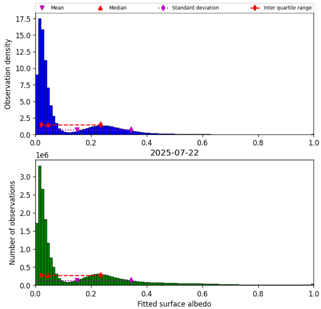
Figure 45: Histogram of “Fitted surface albedo” for 2025-07-21 to 2025-07-23
