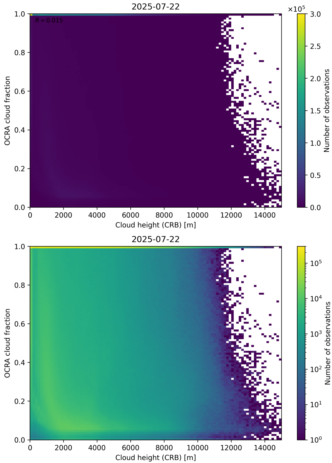
Figure 81: Scatter density plot of “Cloud height (CRB)” against “OCRA cloud fraction” for 2025-07-21 to 2025-07-23.
