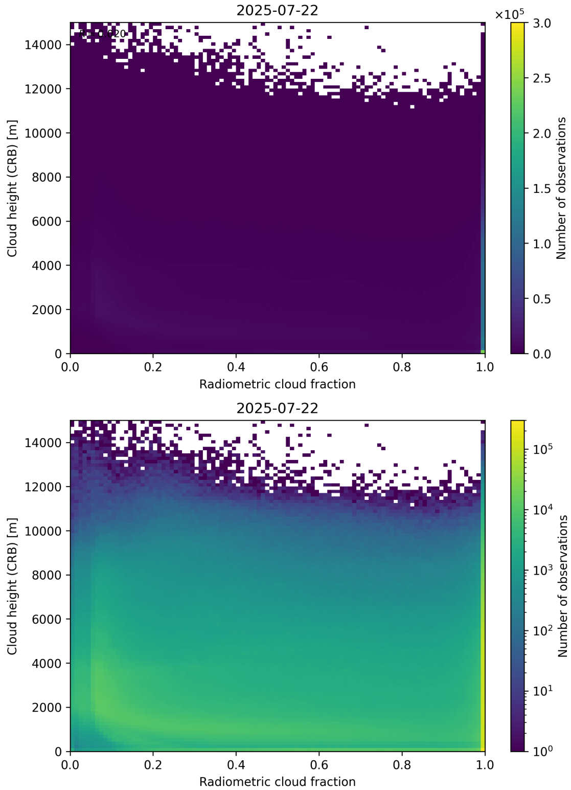
Figure 74: Scatter density plot of “Radiometric cloud fraction” against “Cloud height (CRB)” for 2025-07-21 to 2025-07-23.
