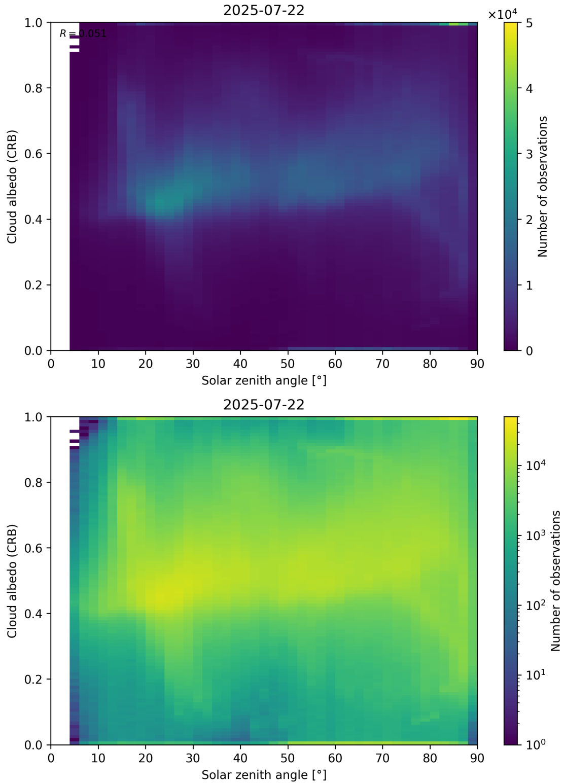
Figure 98: Scatter density plot of “Solar zenith angle” against “Cloud albedo (CRB)” for 2025-07-21 to 2025-07-23.
