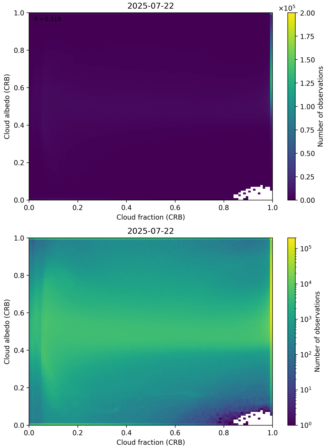
Figure 77: Scatter density plot of “Cloud fraction (CRB)” against “Cloud albedo (CRB)” for 2025-07-21 to 2025-07-23.
