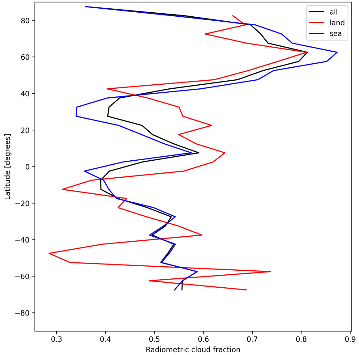
Figure 23: Zonal average of “Radiometric cloud fraction” for 2025-07-21 to 2025-07-23.
