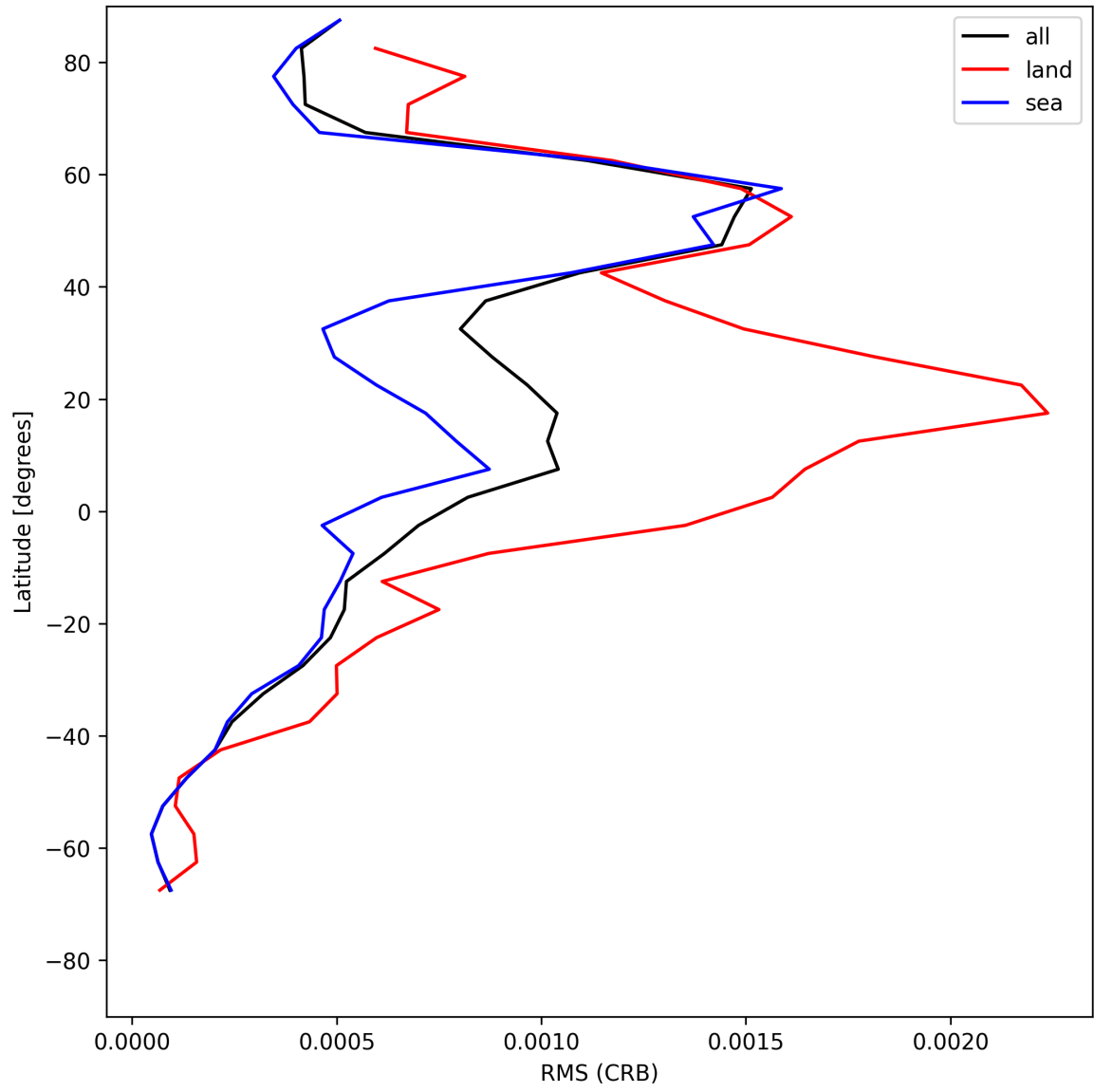
Figure 32: Zonal average of “RMS (CRB)” for 2025-07-21 to 2025-07-23.
