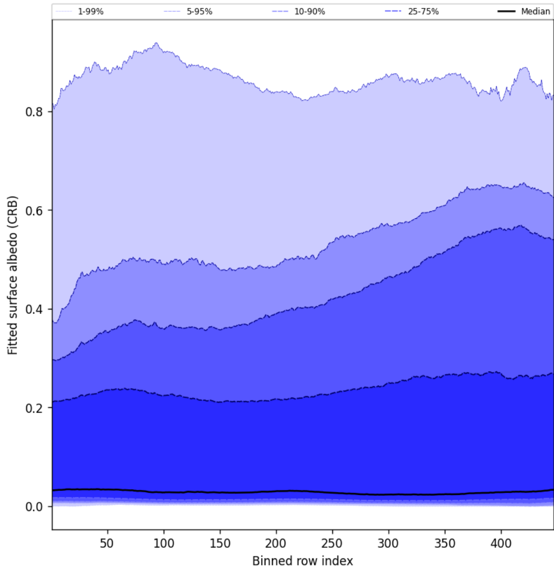
Figure 62: Along track statistics of “Fitted surface albedo (CRB)” for 2025-07-21 to 2025-07-23
