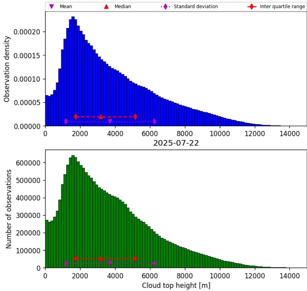
Figure 40: Histogram of “Cloud top height” for 2025-07-21 to 2025-07-23
