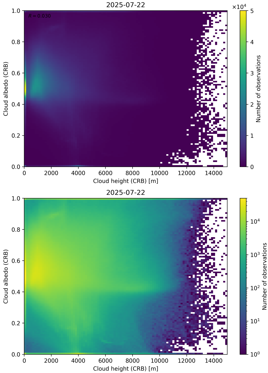
Figure 80: Scatter density plot of “Cloud height (CRB)” against “Cloud albedo (CRB)” for 2025-07-21 to 2025-07-23.
