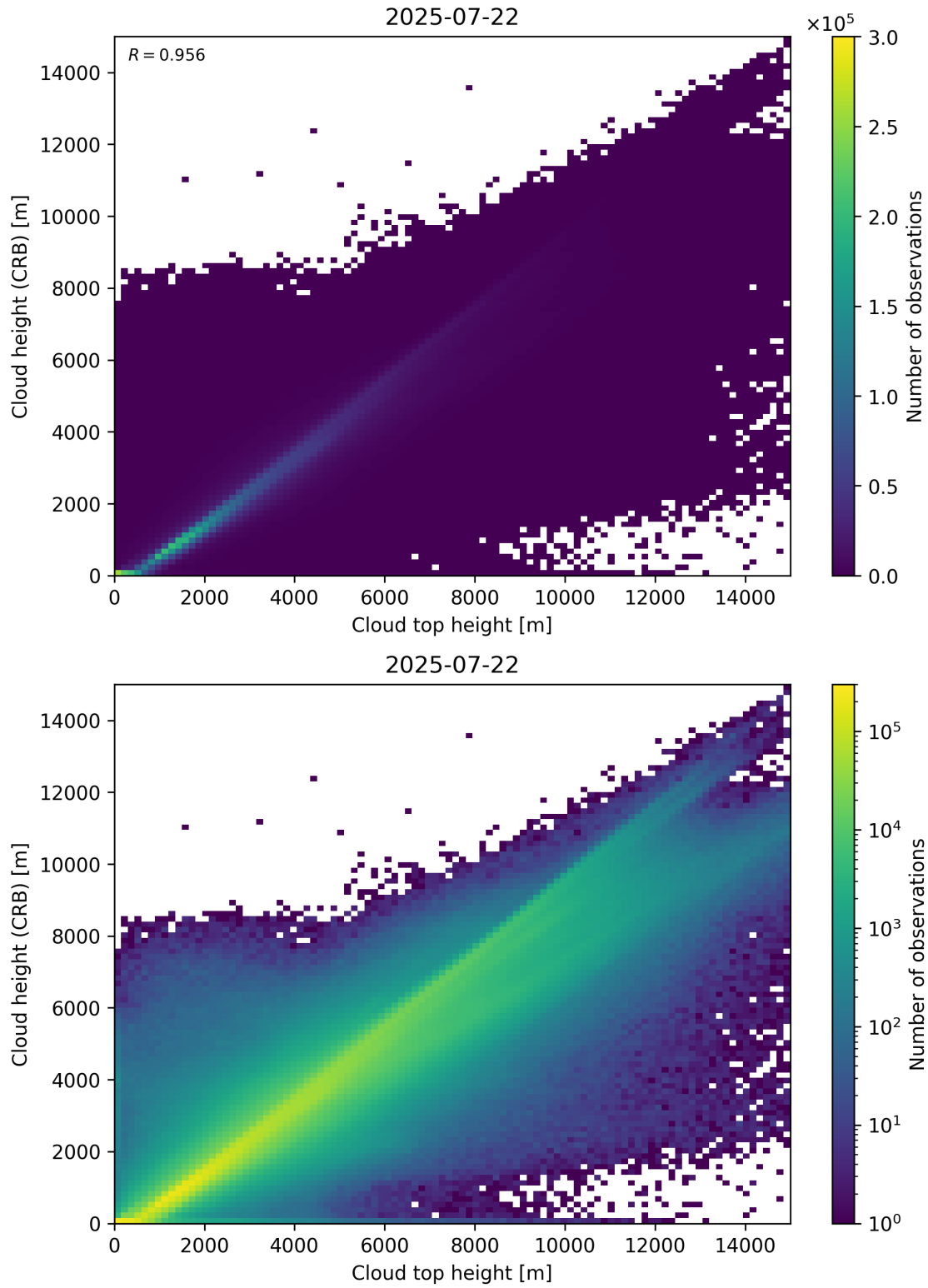
Figure 89: Scatter density plot of “Cloud top height” against “Cloud height (CRB)” for 2025-07-21 to 2025-07-23.
