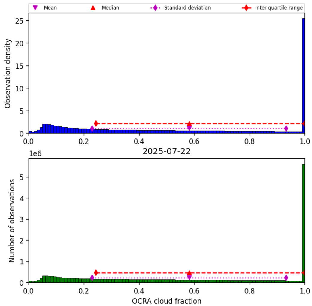
Figure 50: Histogram of “OCRA cloud fraction” for 2025-07-21 to 2025-07-23
