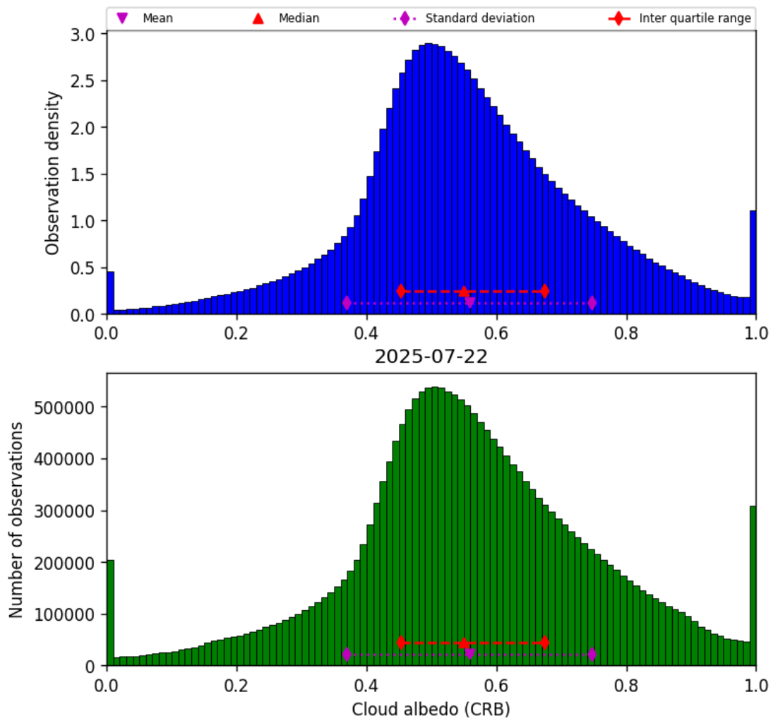
Figure 44: Histogram of “Cloud albedo (CRB)” for 2025-07-21 to 2025-07-23
