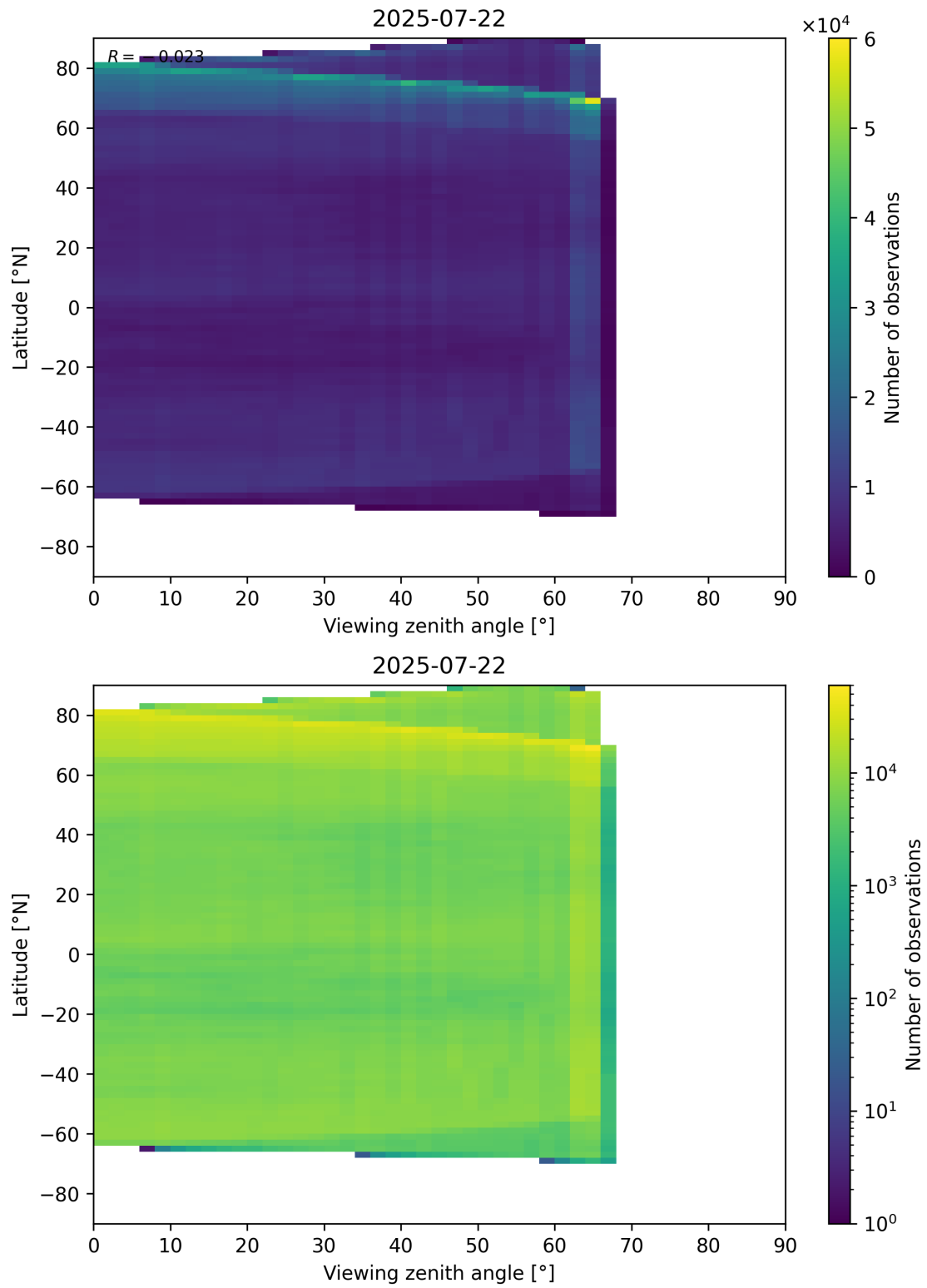
Figure 113: Scatter density plot of “Viewing zenith angle” against “Latitude” for 2025-07-21 to 2025-07-23.
