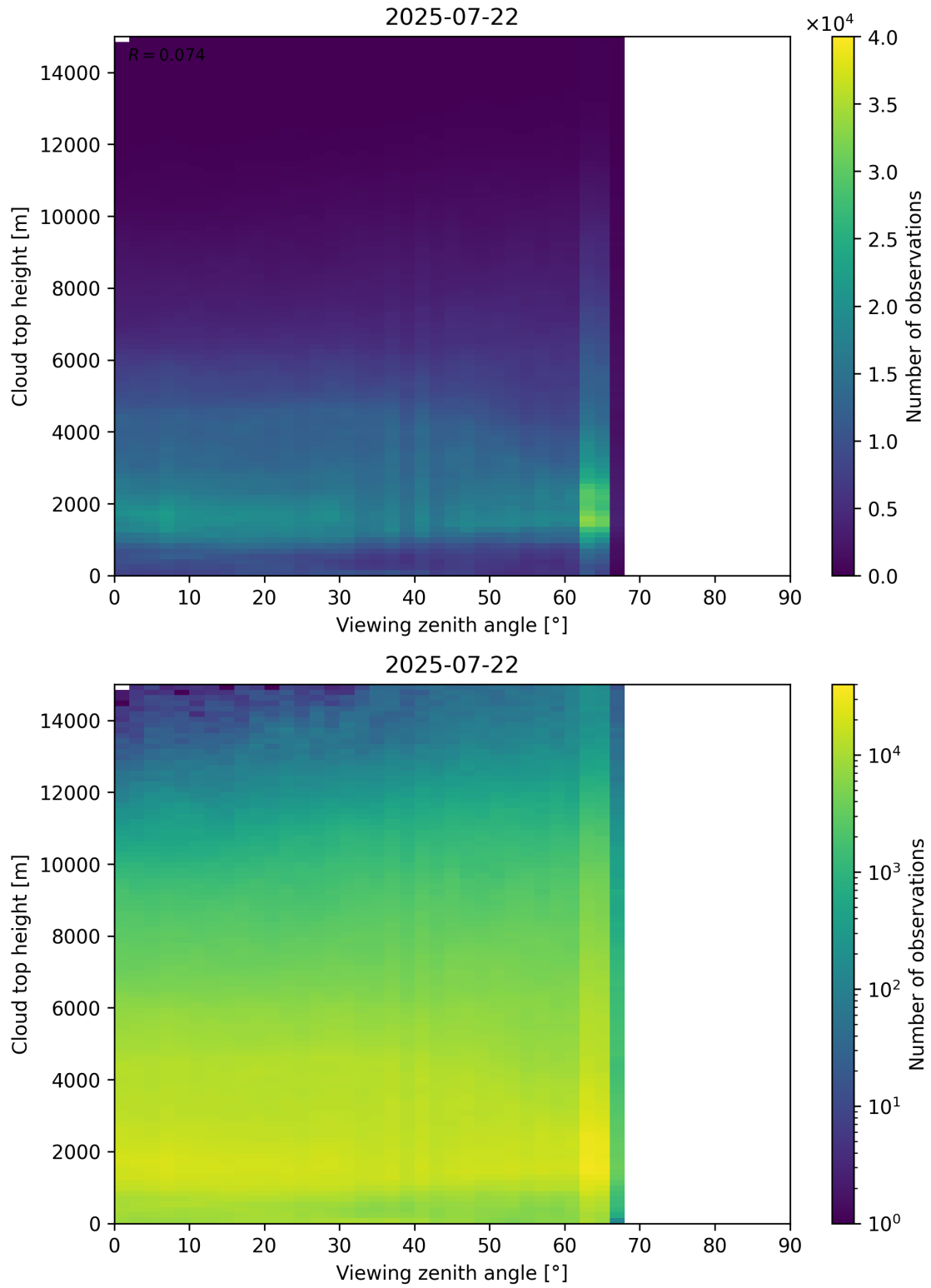
Figure 112: Scatter density plot of “Viewing zenith angle” against “Cloud top height” for 2025-07-21 to 2025-07-23.
