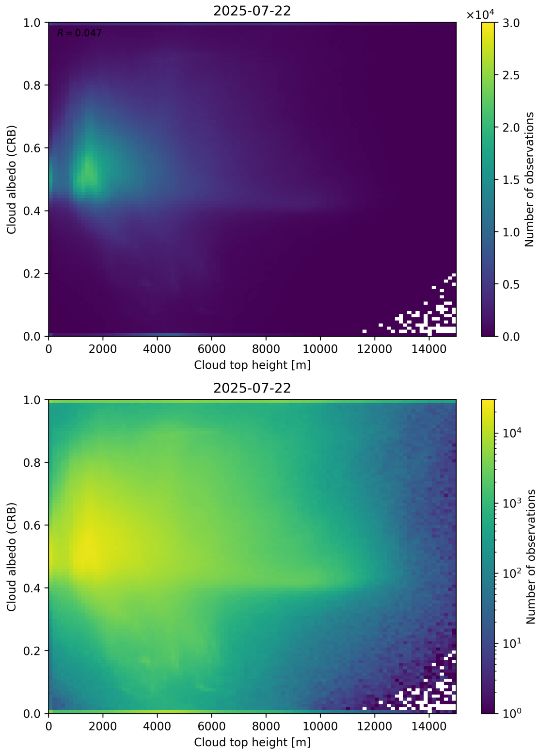
Figure 86: Scatter density plot of “Cloud top height” against “Cloud albedo (CRB)” for 2025-07-21 to 2025-07-23.
