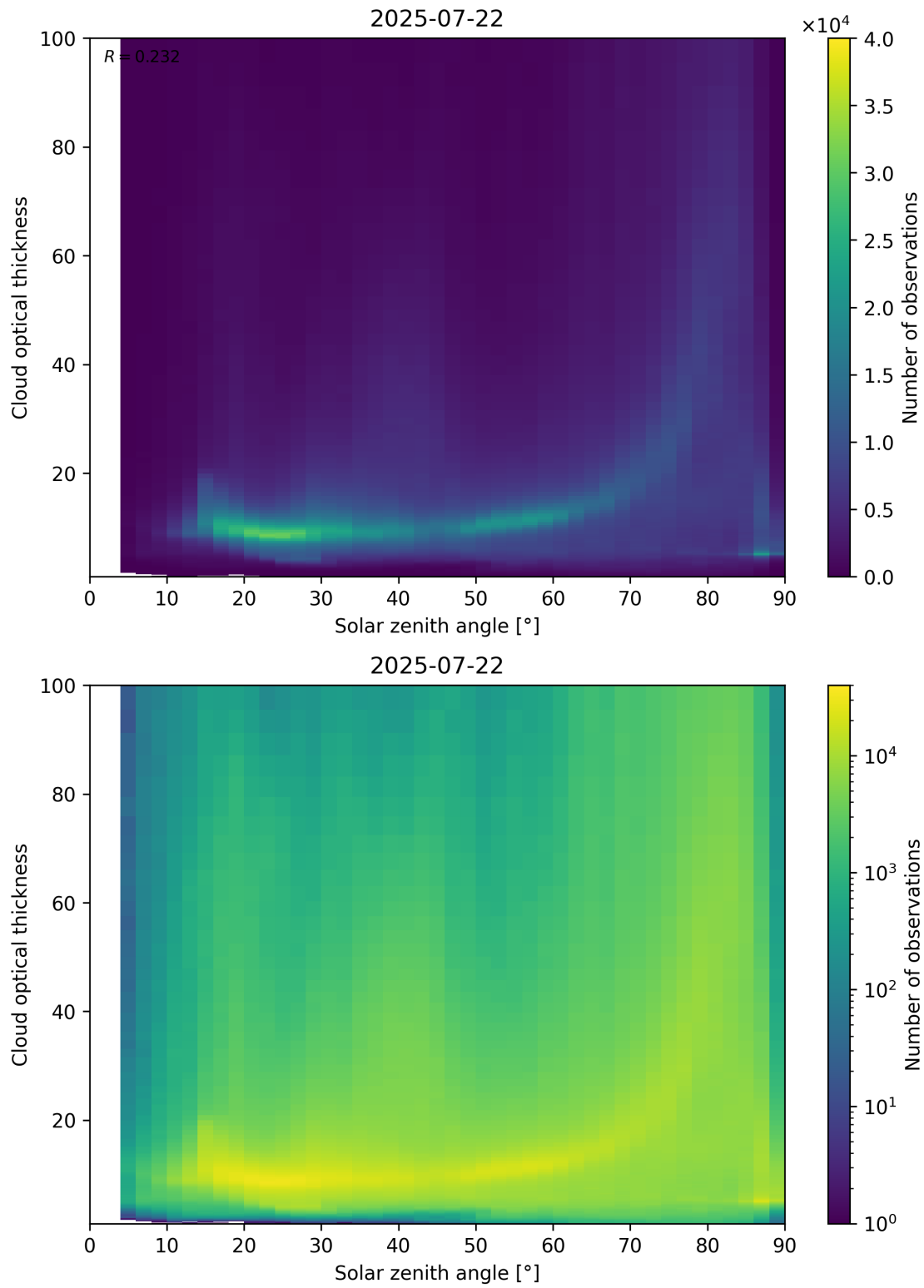
Figure 103: Scatter density plot of “Solar zenith angle” against “Cloud optical thickness” for 2025-07-21 to 2025-07-23.
