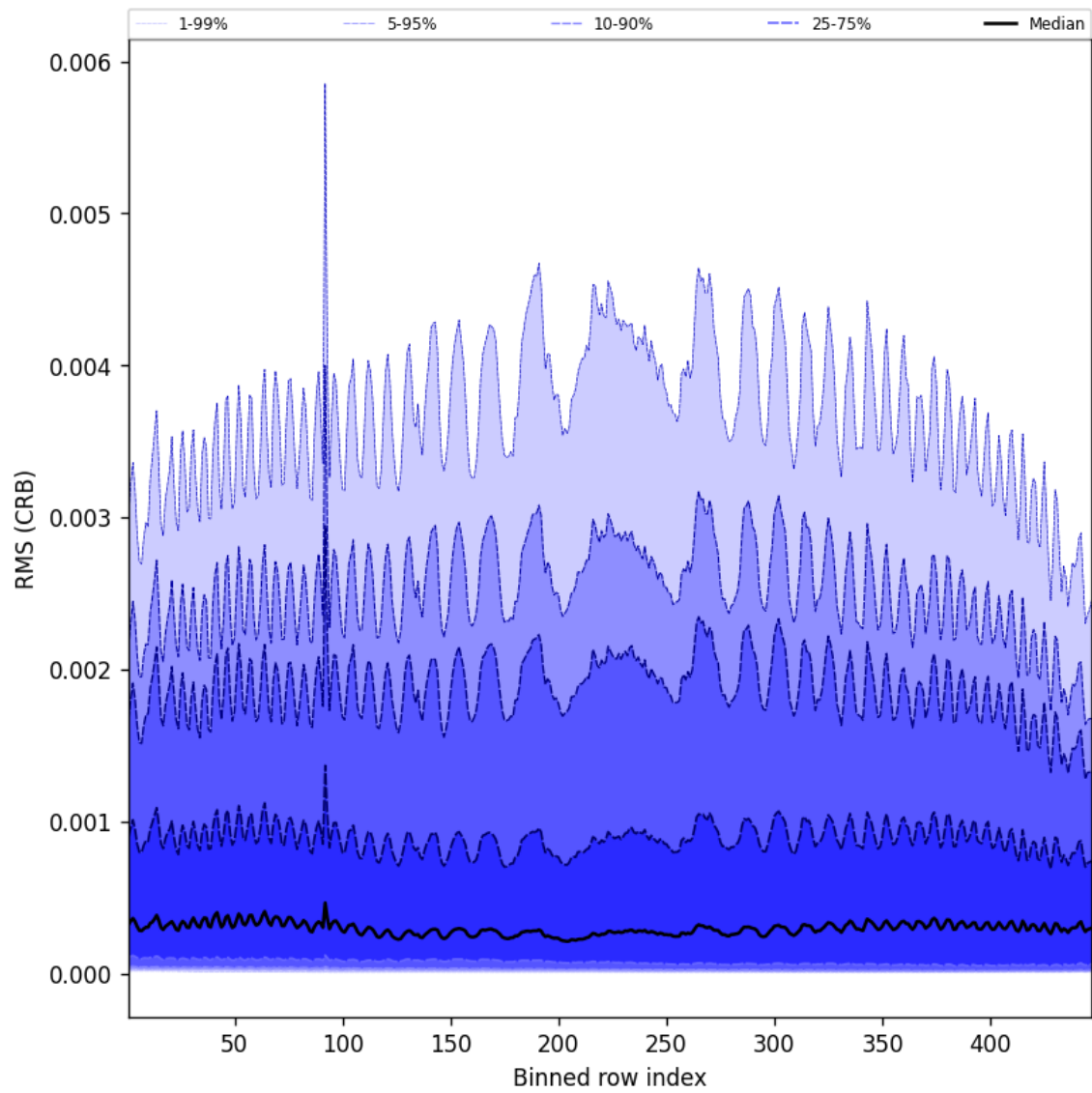
Figure 64: Along track statistics of “RMS (CRB)” for 2025-07-21 to 2025-07-23
