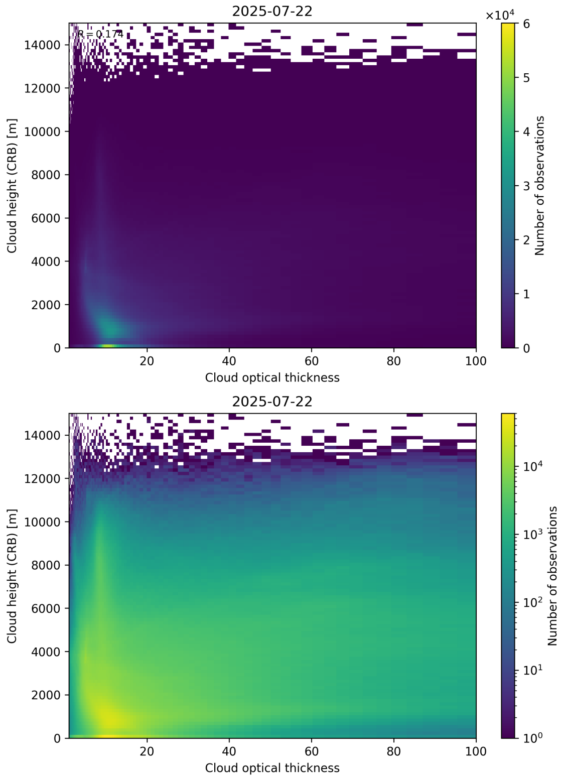
Figure 85: Scatter density plot of “Cloud optical thickness” against “Cloud height (CRB)” for 2025-07-21 to 2025-07-23.
