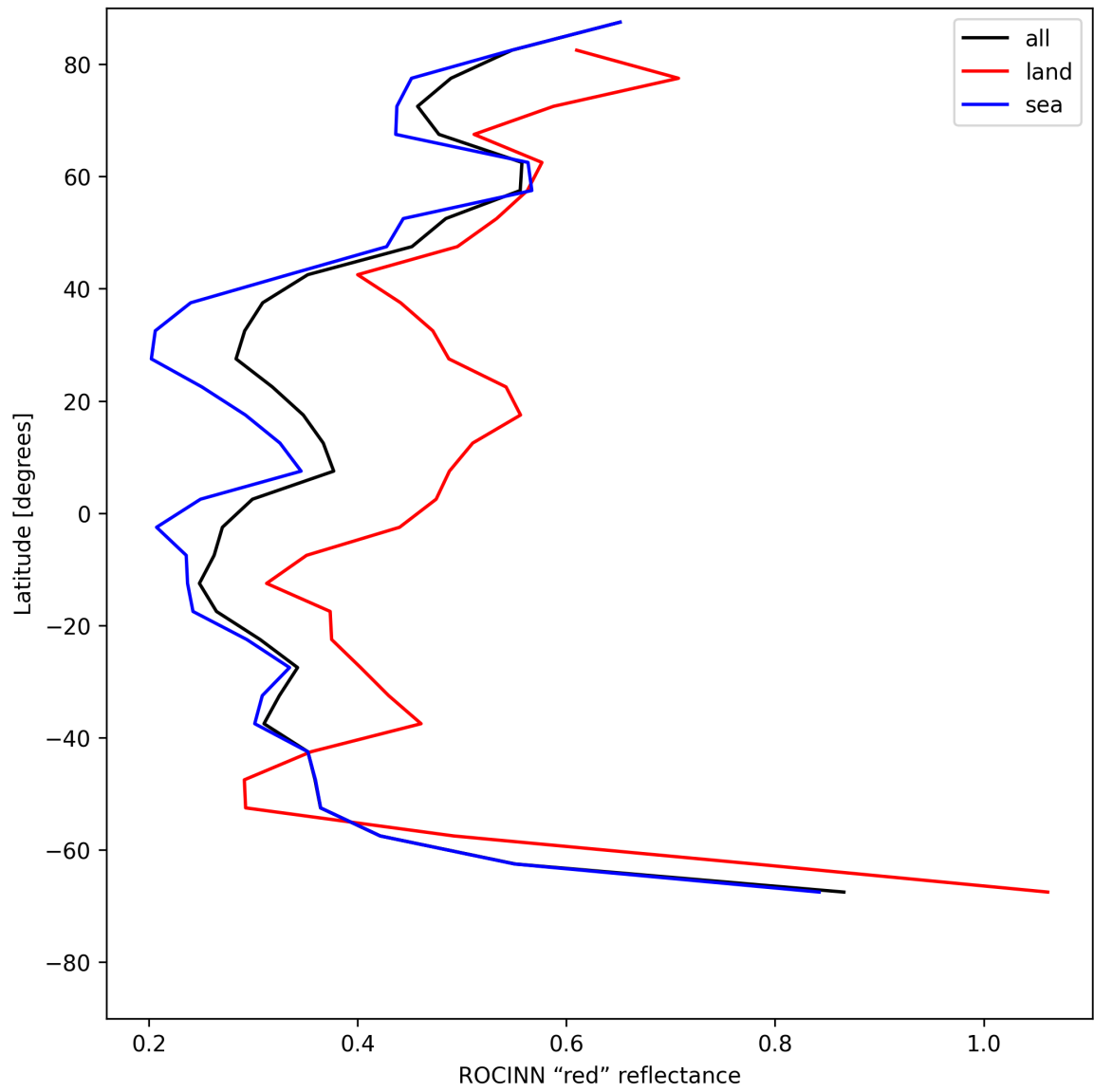
Figure 37: Zonal average of “ROCINN “red” reflectance” for 2025-07-21 to 2025-07-23.
