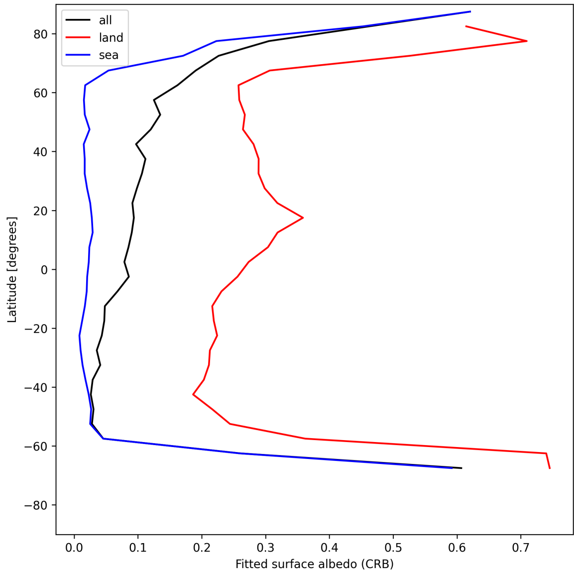
Figure 30: Zonal average of “Fitted surface albedo (CRB)” for 2025-07-21 to 2025-07-23.
