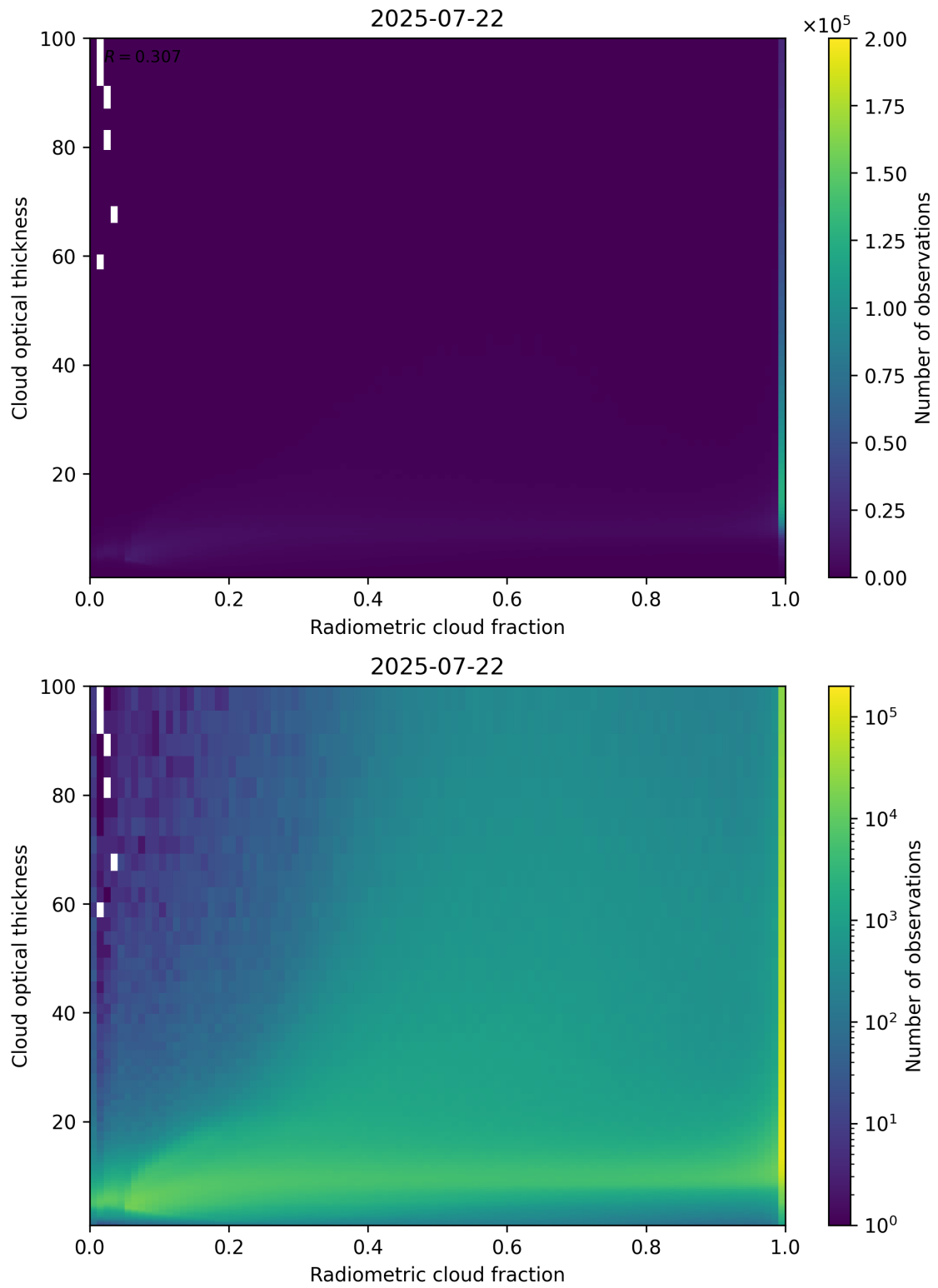
Figure 75: Scatter density plot of “Radiometric cloud fraction” against “Cloud optical thickness” for 2025-07-21 to 2025-07-23.
