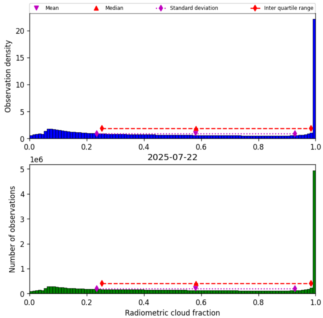
Figure 39: Histogram of “Radiometric cloud fraction” for 2025-07-21 to 2025-07-23
