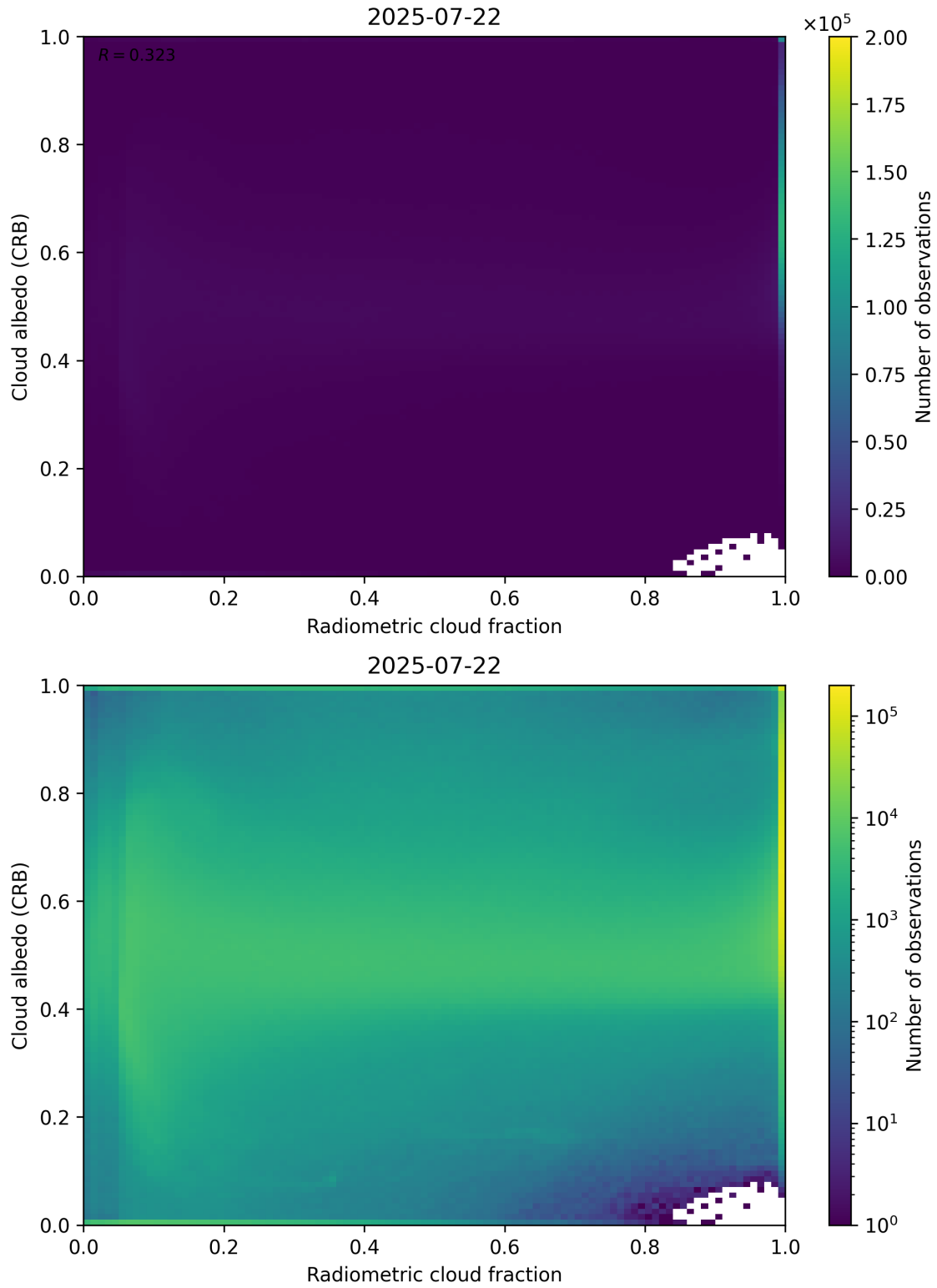
Figure 71: Scatter density plot of “Radiometric cloud fraction” against “Cloud albedo (CRB)” for 2025-07-21 to 2025-07-23.
