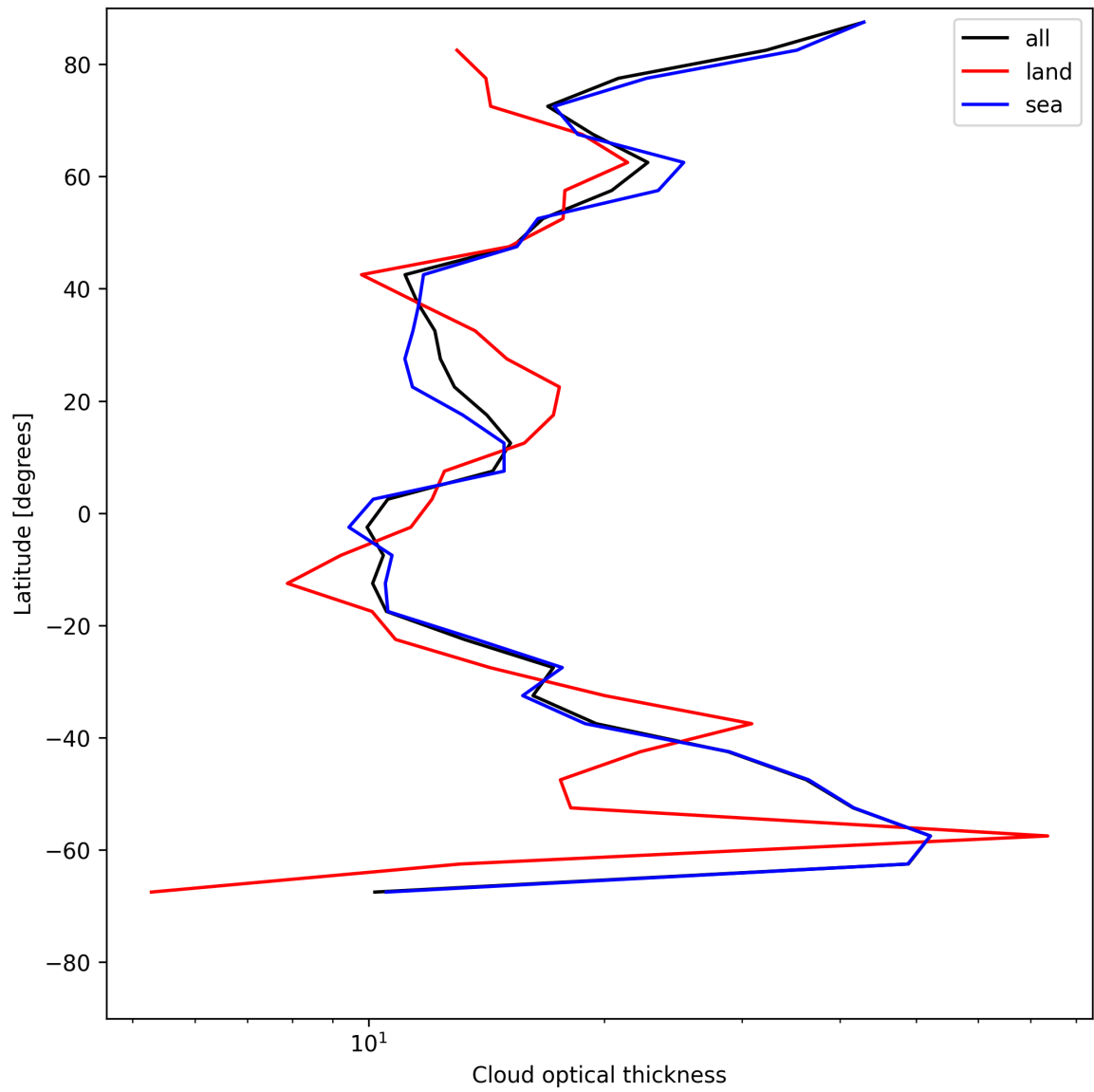
Figure 25: Zonal average of “Cloud optical thickness” for 2025-07-21 to 2025-07-23.
