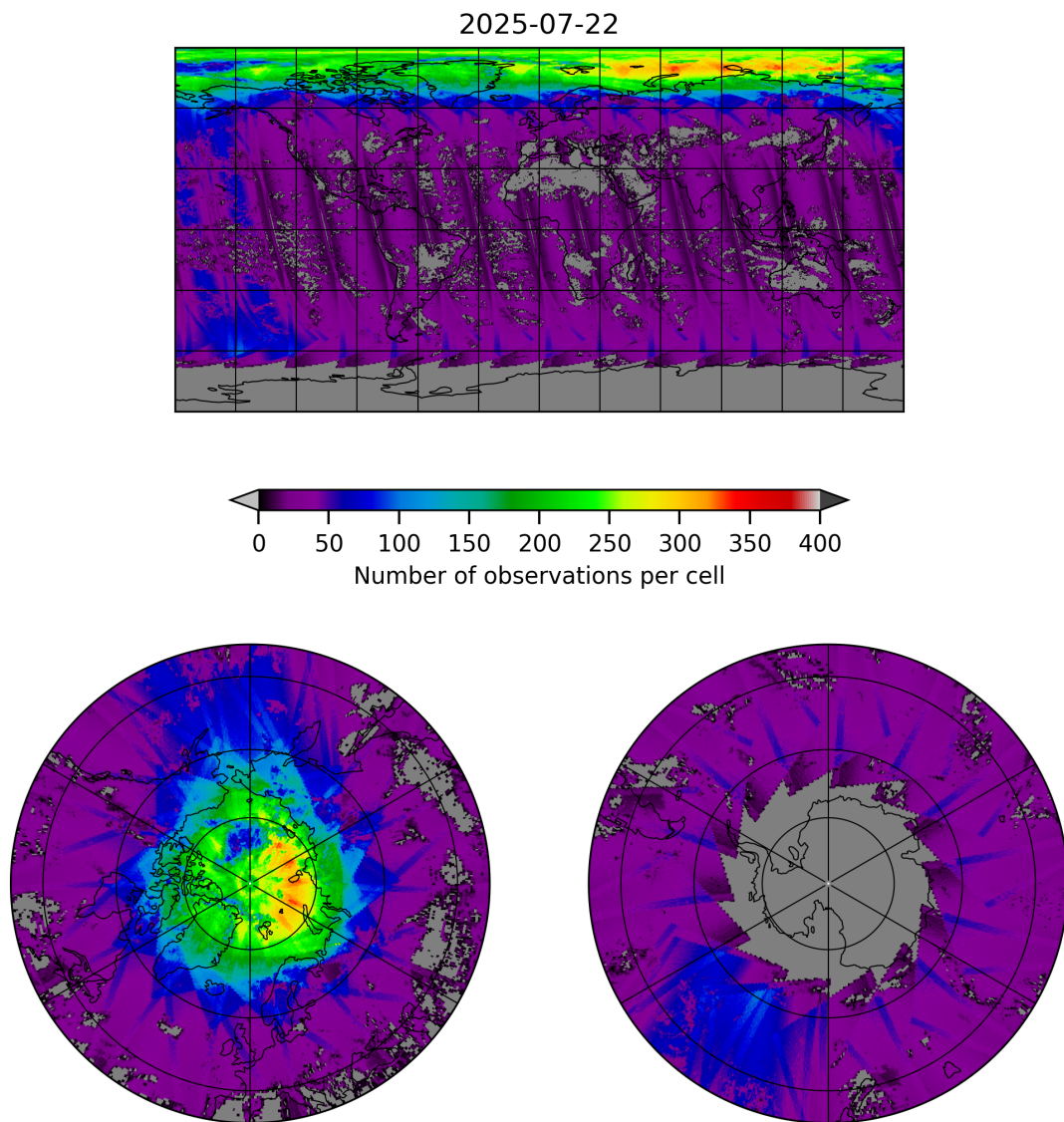
Figure 21: Map of the number of observations for 2025-07-21 to 2025-07-23
