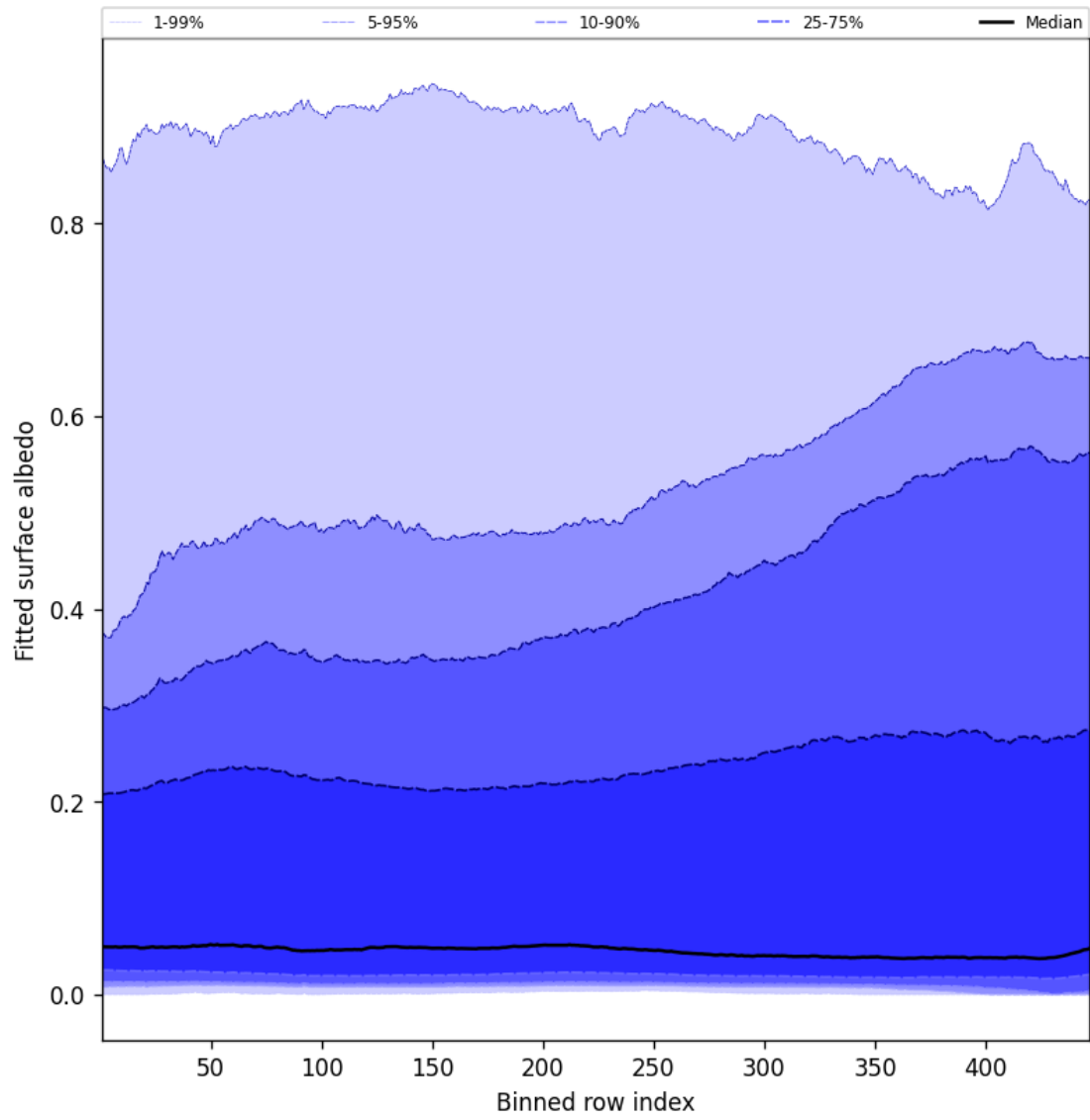
Figure 61: Along track statistics of “Fitted surface albedo” for 2025-07-21 to 2025-07-23
