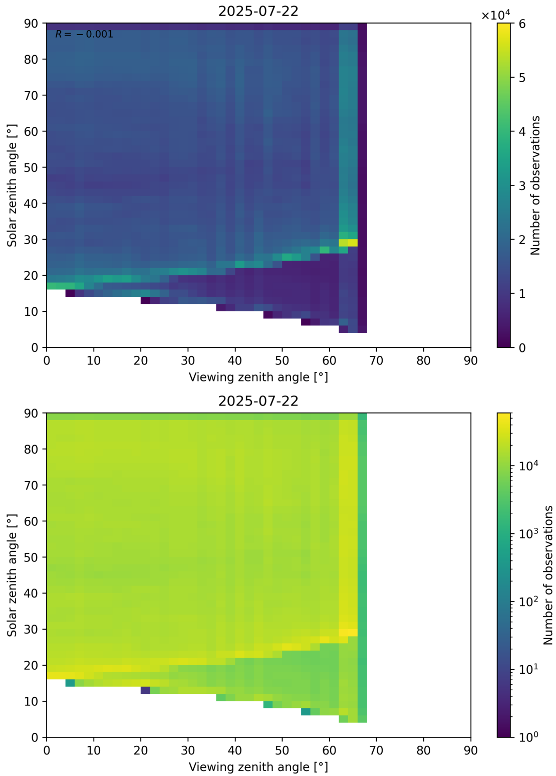
Figure 114: Scatter density plot of “Viewing zenith angle” against “Solar zenith angle” for 2025-07-21 to 2025-07-23.
