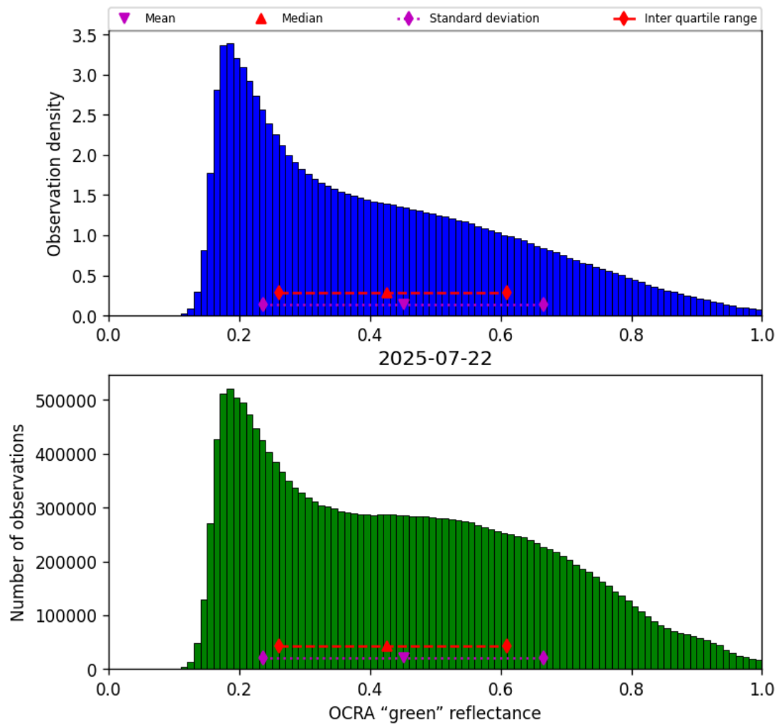
Figure 52: Histogram of “OCRA “green” reflectance” for 2025-07-21 to 2025-07-23
