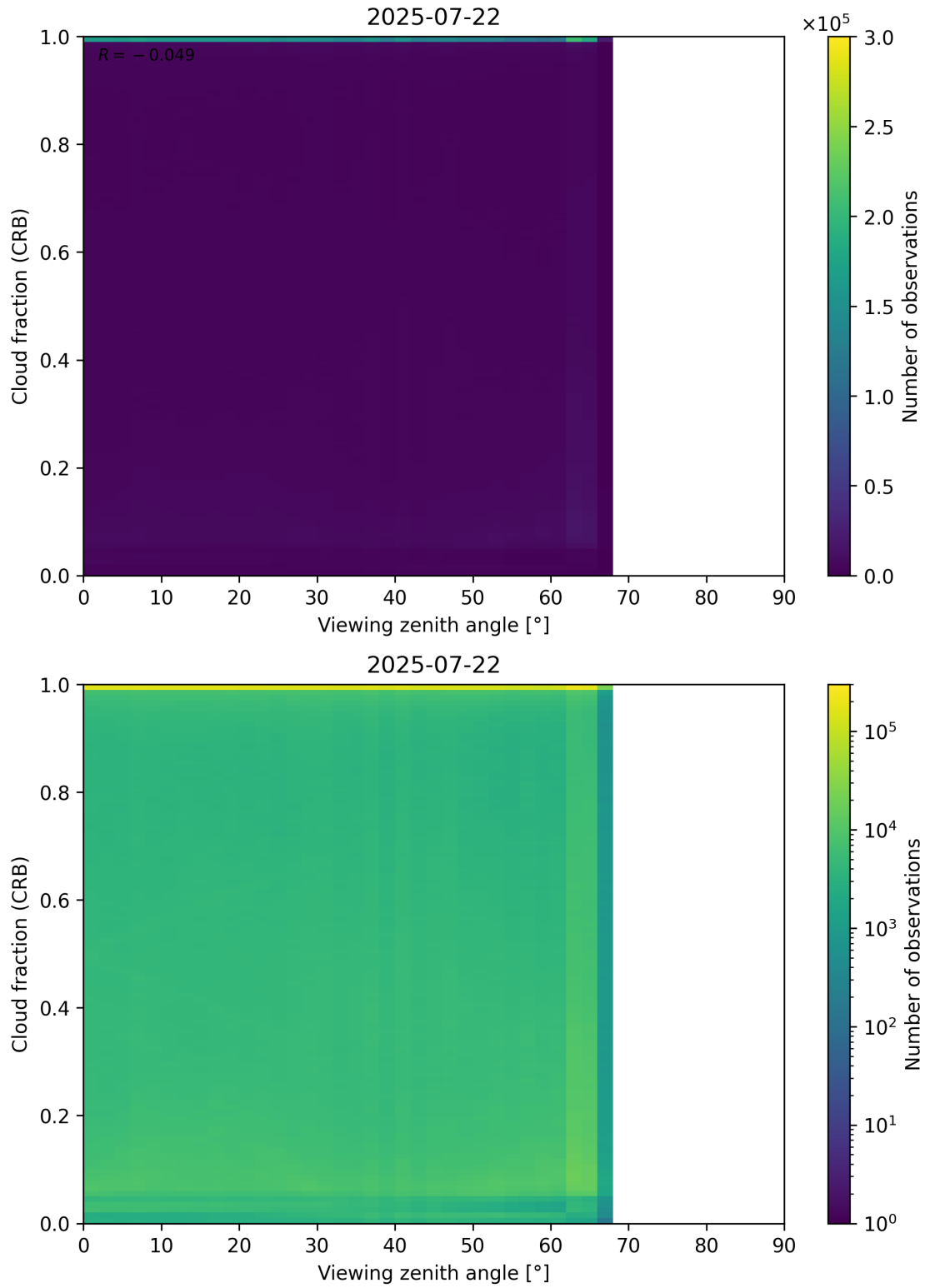
Figure 109: Scatter density plot of “Viewing zenith angle” against “Cloud fraction (CRB)” for 2025-07-21 to 2025-07-23.
