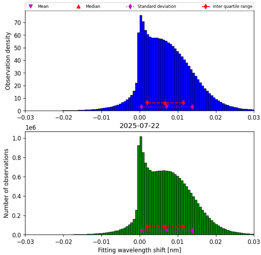
Figure 49: Histogram of “Fitting wavelength shift” for 2025-07-21 to 2025-07-23
