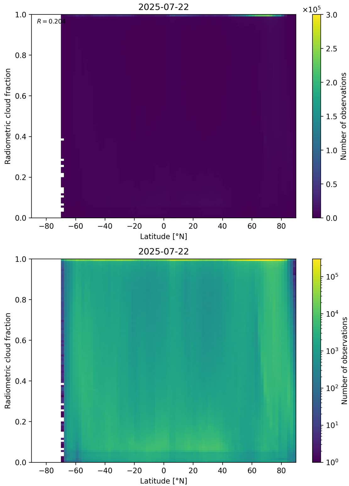
Figure 92: Scatter density plot of “Latitude” against “Radiometric cloud fraction” for 2025-07-21 to 2025-07-23.
