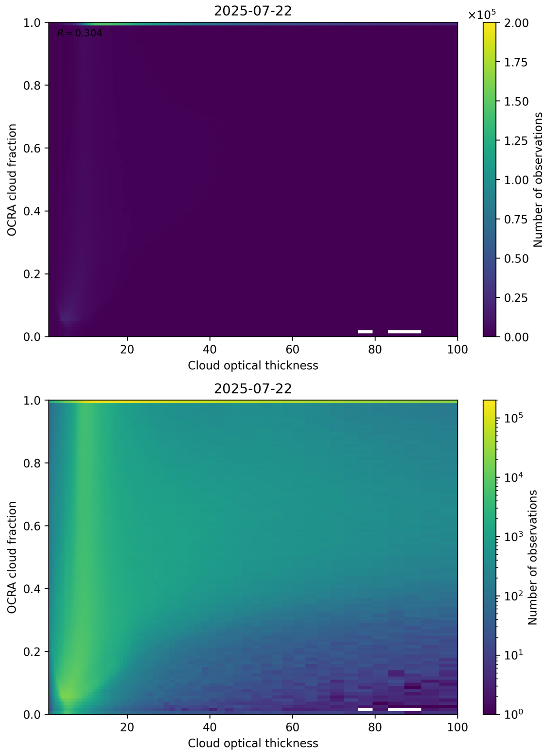
Figure 83: Scatter density plot of “Cloud optical thickness” against “OCRA cloud fraction” for 2025-07-21 to 2025-07-23.
