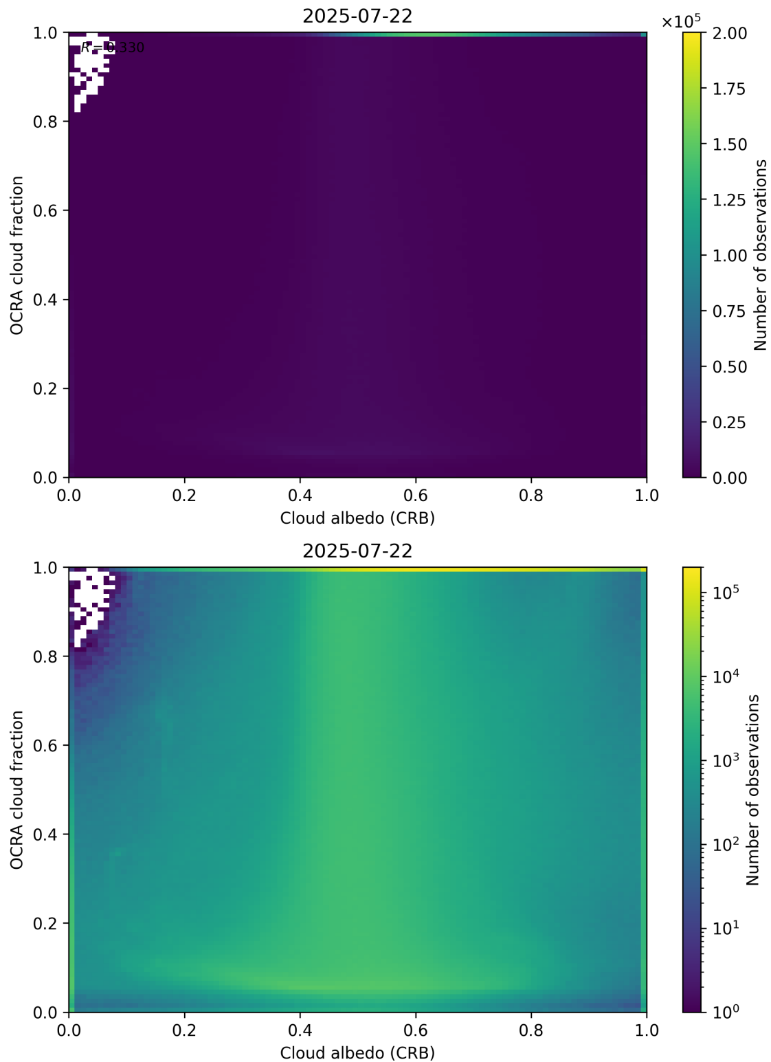
Figure 70: Scatter density plot of “Cloud albedo (CRB)” against “OCRA cloud fraction” for 2025-07-21 to 2025-07-23.
