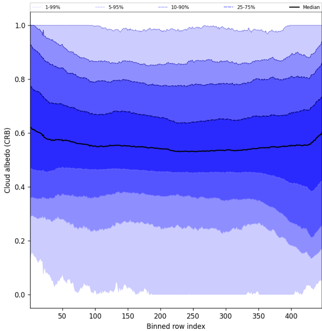
Figure 60: Along track statistics of “Cloud albedo (CRB)” for 2025-07-21 to 2025-07-23
