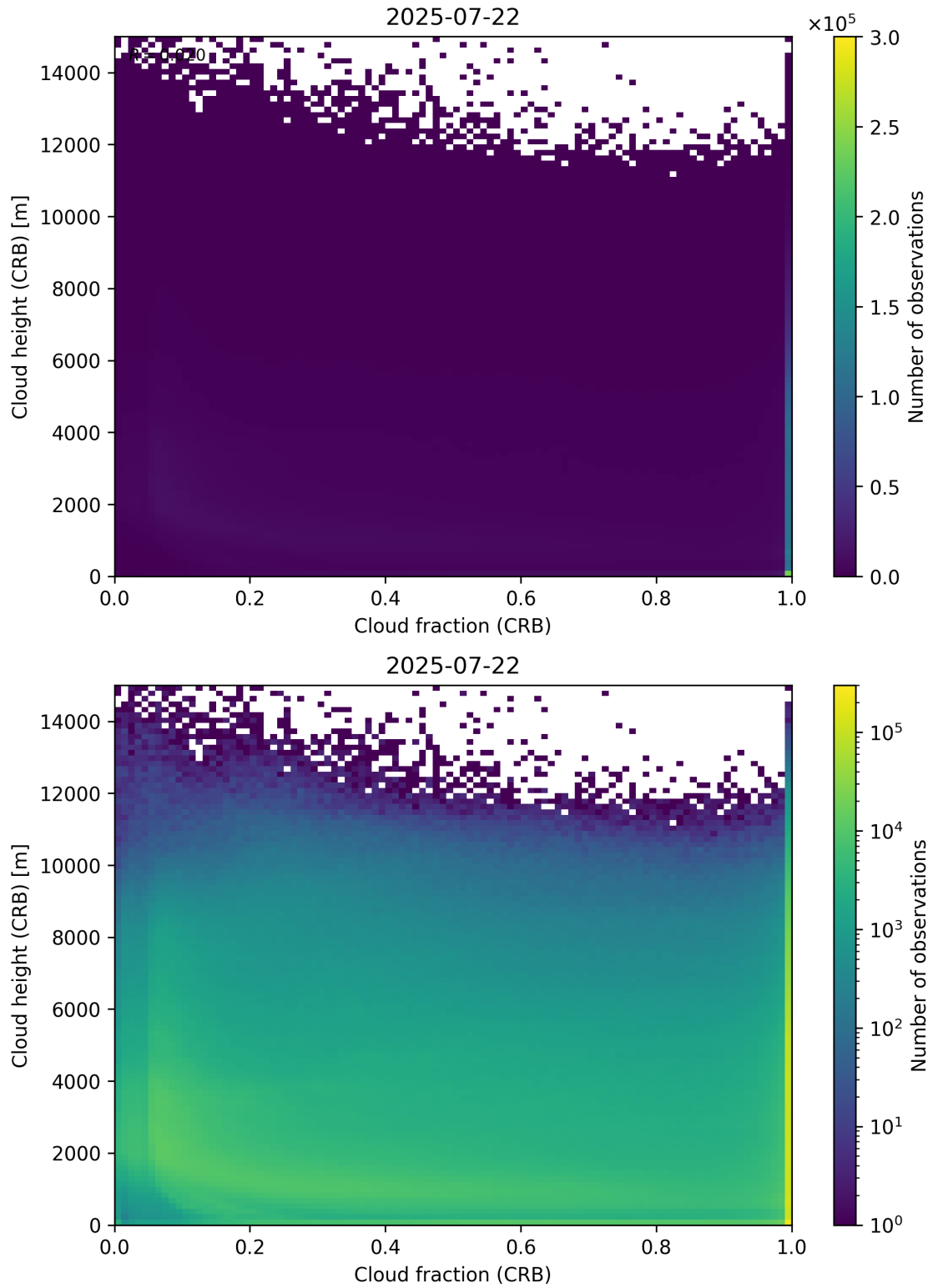
Figure 79: Scatter density plot of “Cloud fraction (CRB)” against “Cloud height (CRB)” for 2025-07-21 to 2025-07-23.
