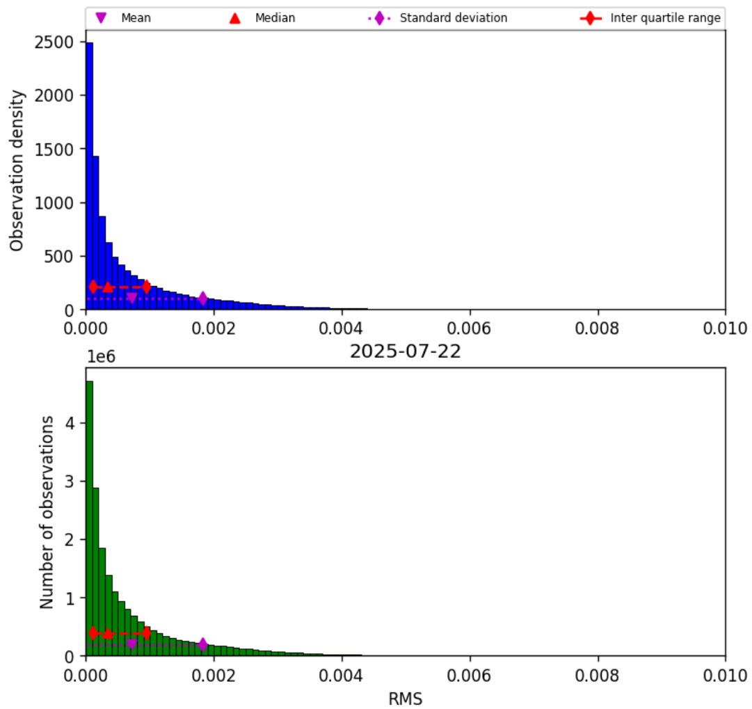
Figure 47: Histogram of “RMS” for 2025-07-21 to 2025-07-23
