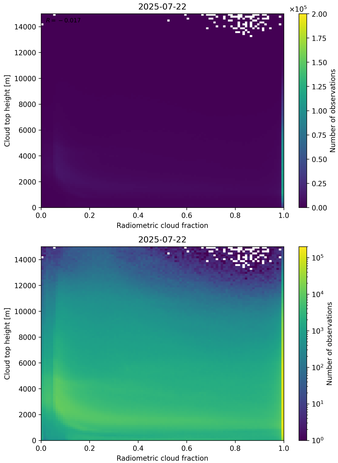
Figure 76: Scatter density plot of “Radiometric cloud fraction” against “Cloud top height” for 2025-07-21 to 2025-07-23.
