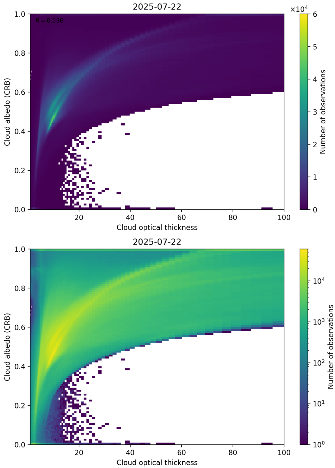
Figure 82: Scatter density plot of “Cloud optical thickness” against “Cloud albedo (CRB)” for 2025-07-21 to 2025-07-23.
