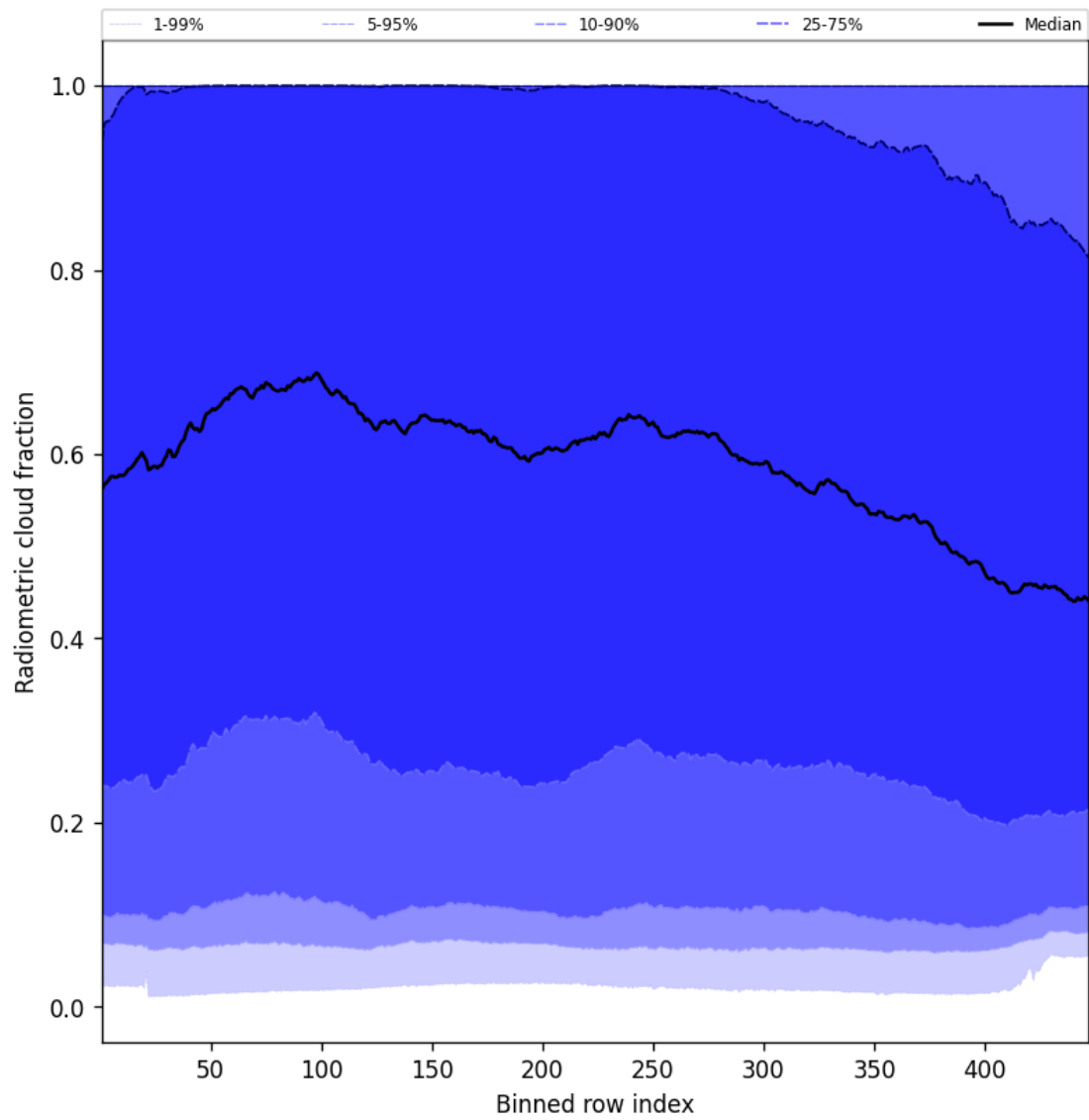
Figure 55: Along track statistics of “Radiometric cloud fraction” for 2025-07-21 to 2025-07-23
