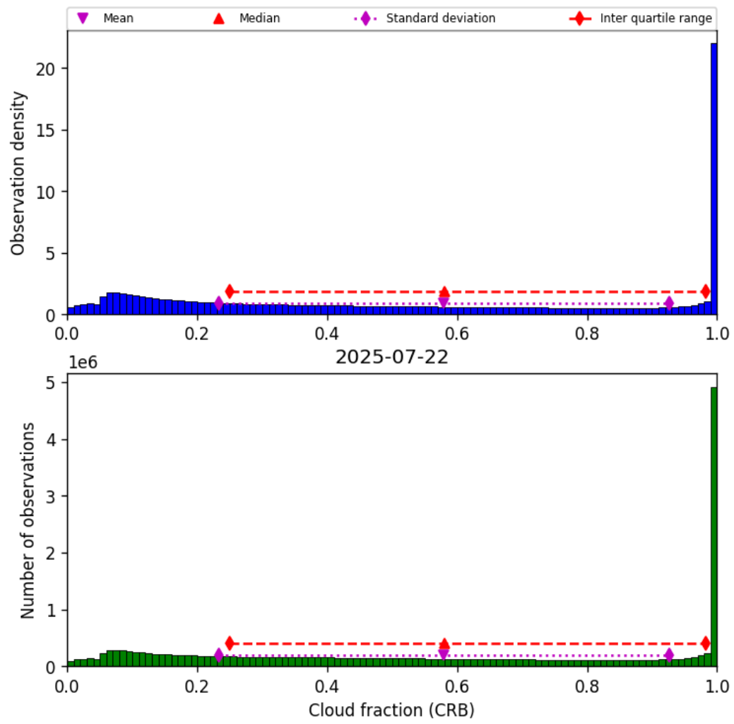
Figure 42: Histogram of “Cloud fraction (CRB)” for 2025-07-21 to 2025-07-23
