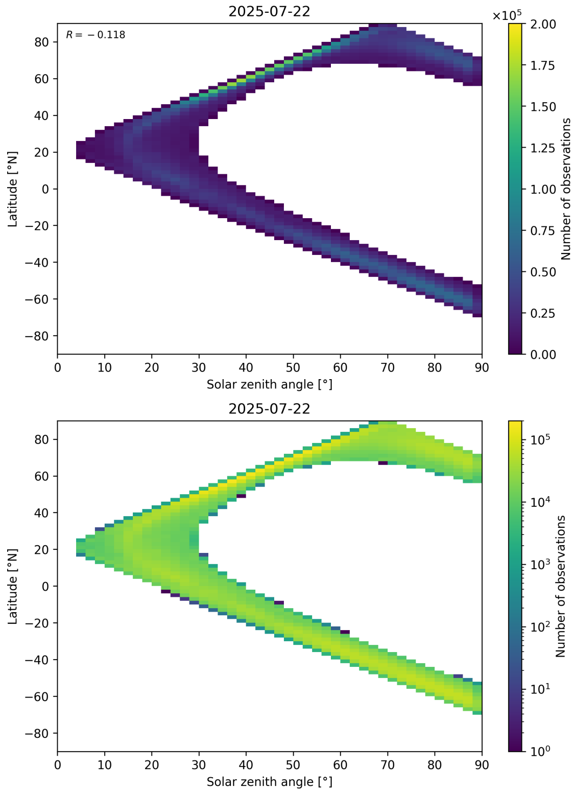
Figure 105: Scatter density plot of “Solar zenith angle” against “Latitude” for 2025-07-21 to 2025-07-23.
