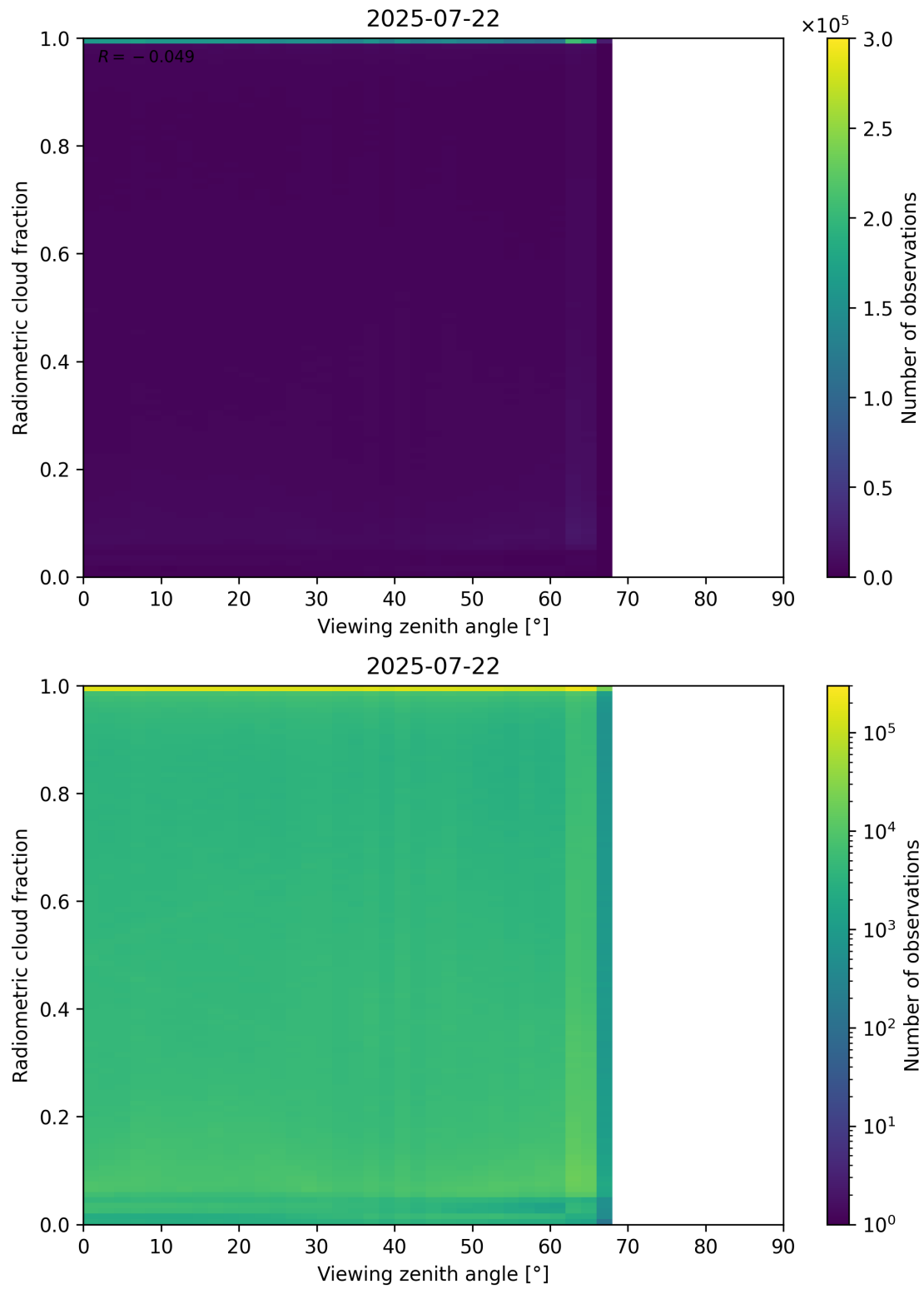
Figure 107: Scatter density plot of “Viewing zenith angle” against “Radiometric cloud fraction” for 2025-07-21 to 2025-07-23.
