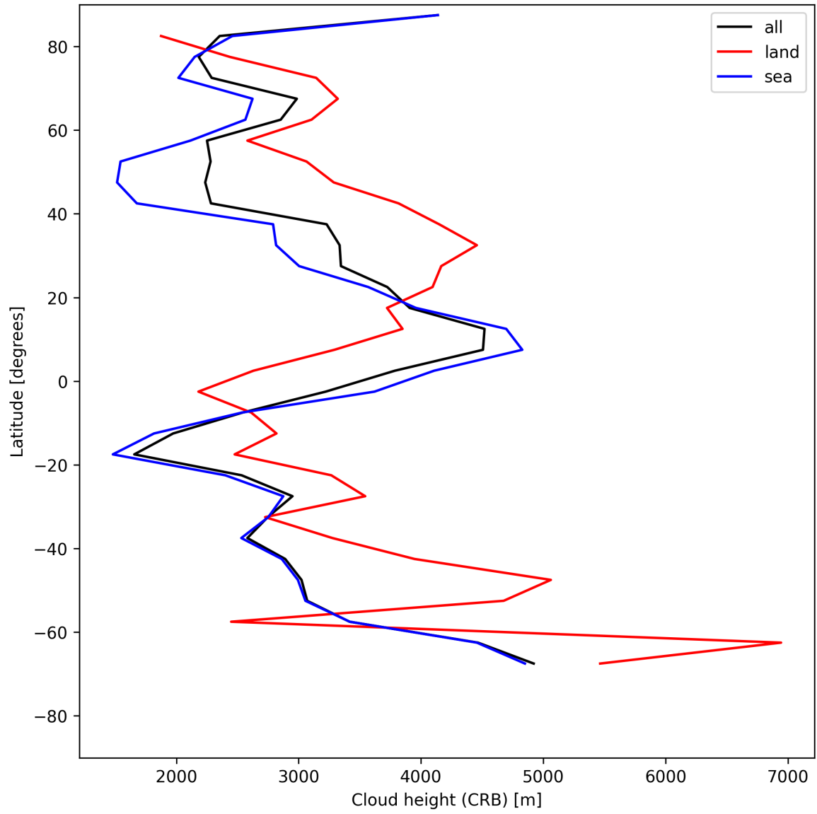
Figure 27: Zonal average of “Cloud height (CRB)” for 2025-07-21 to 2025-07-23.
