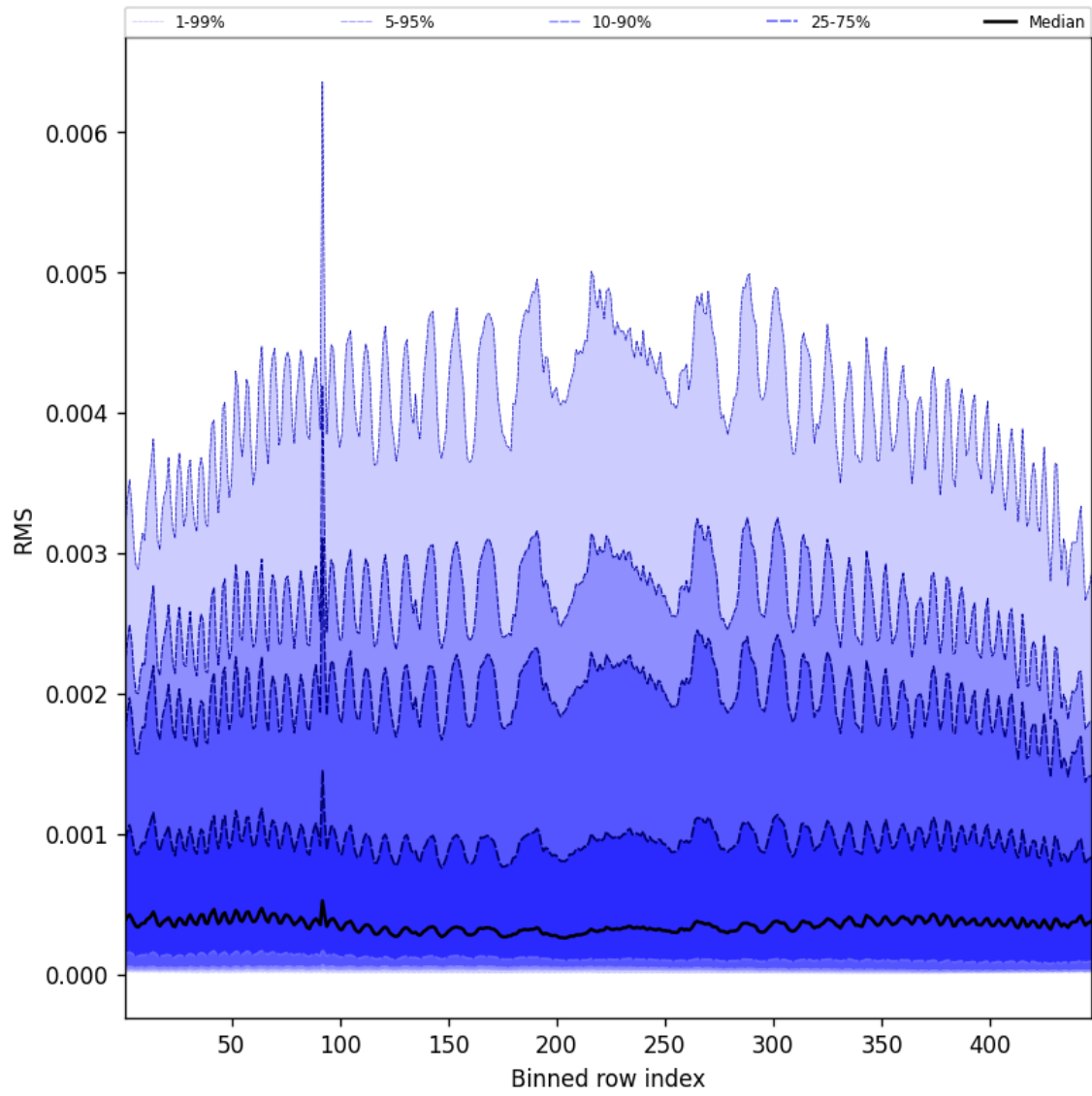
Figure 63: Along track statistics of “RMS” for 2025-07-21 to 2025-07-23
