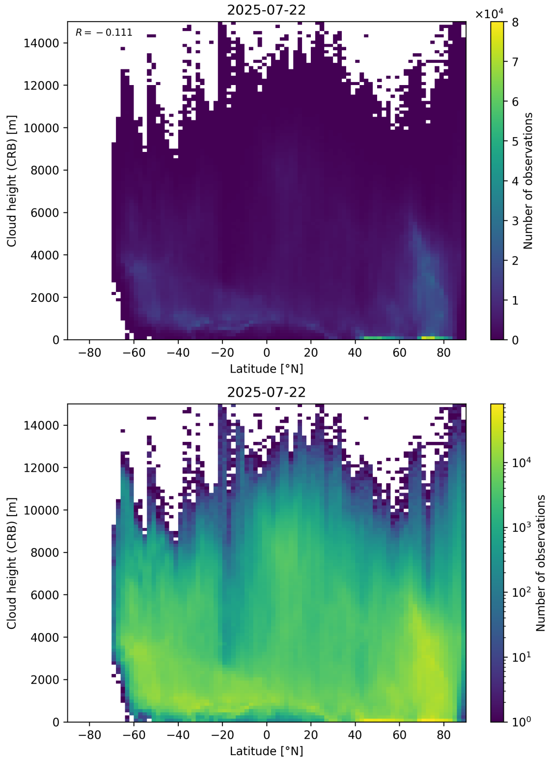
Figure 95: Scatter density plot of “Latitude” against “Cloud height (CRB)” for 2025-07-21 to 2025-07-23.
