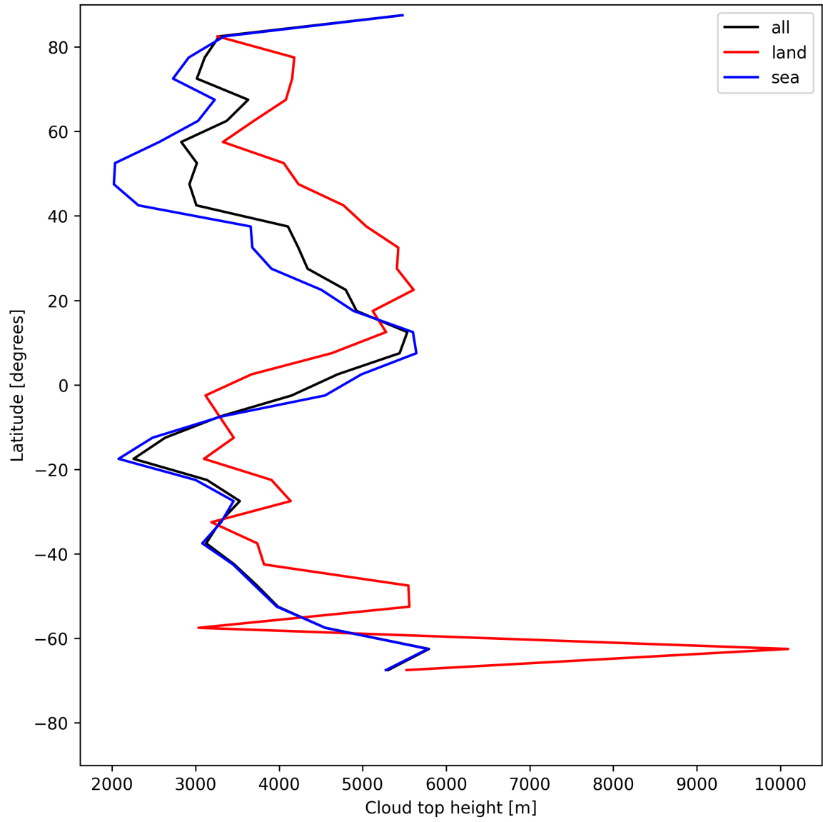
Figure 24: Zonal average of “Cloud top height” for 2025-07-21 to 2025-07-23.
