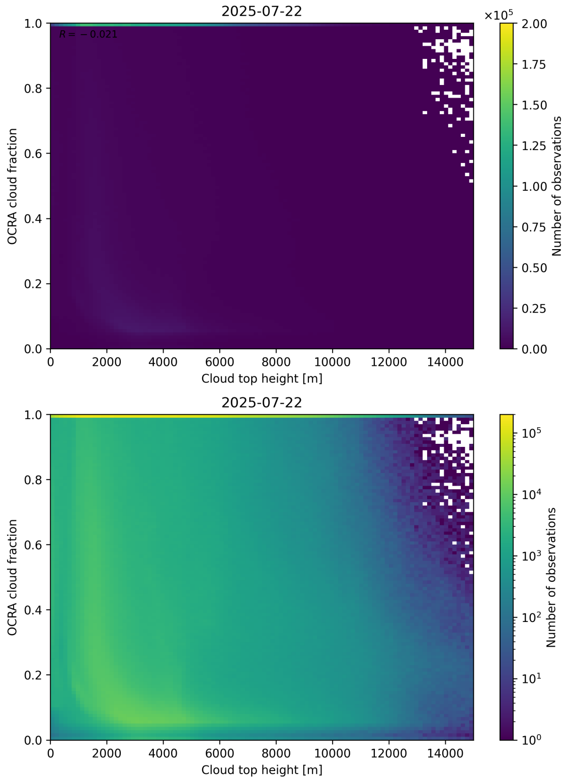
Figure 87: Scatter density plot of “Cloud top height” against “OCRA cloud fraction” for 2025-07-21 to 2025-07-23.
