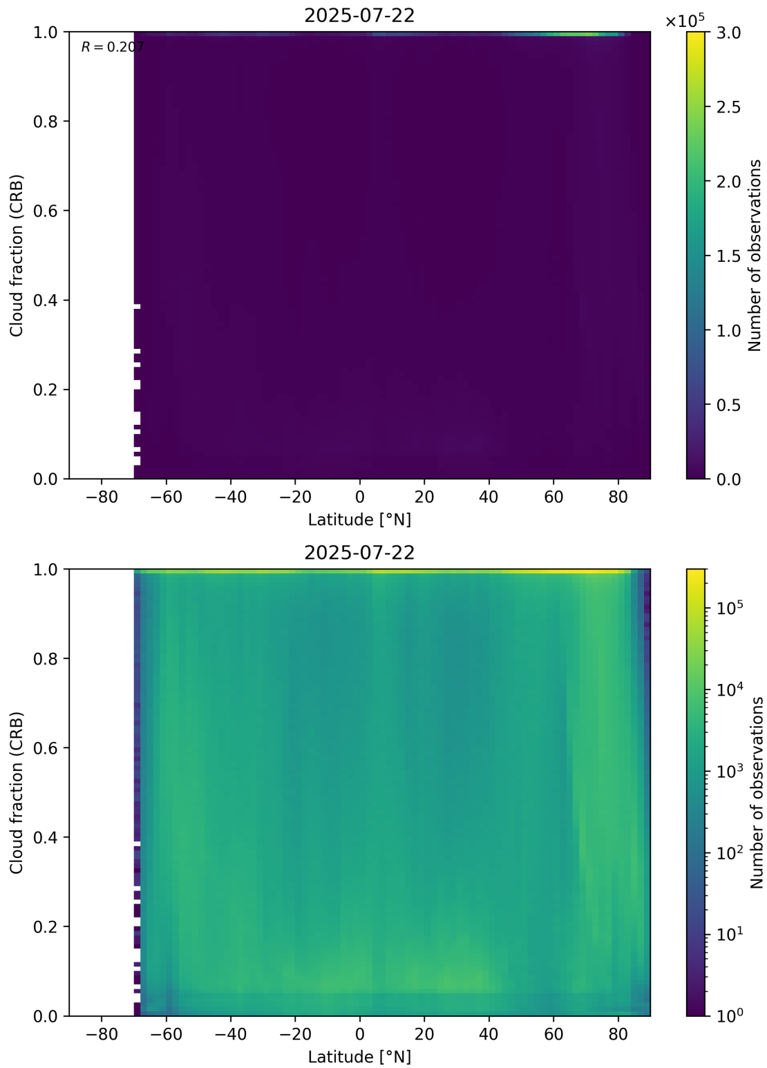
Figure 94: Scatter density plot of “Latitude” against “Cloud fraction (CRB)” for 2025-07-21 to 2025-07-23.
