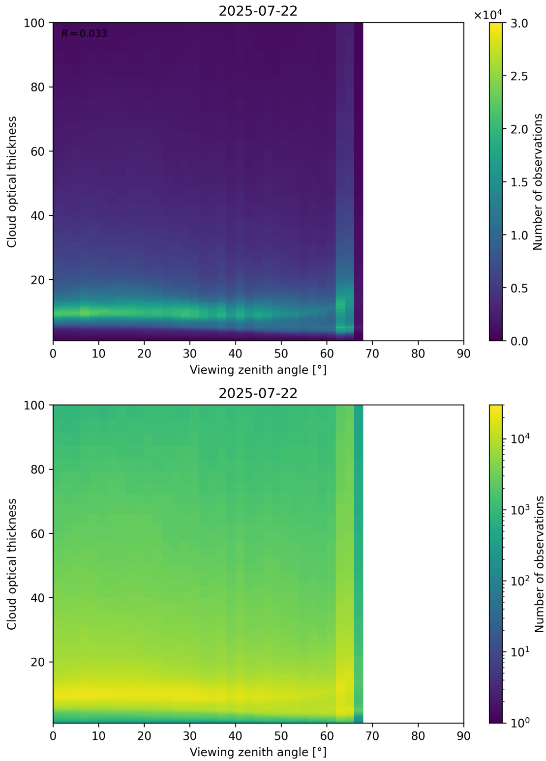
Figure 111: Scatter density plot of “Viewing zenith angle” against “Cloud optical thickness” for 2025-07-21 to 2025-07-23.
