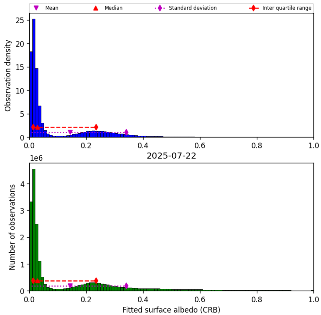
Figure 46: Histogram of “Fitted surface albedo (CRB)” for 2025-07-21 to 2025-07-23
