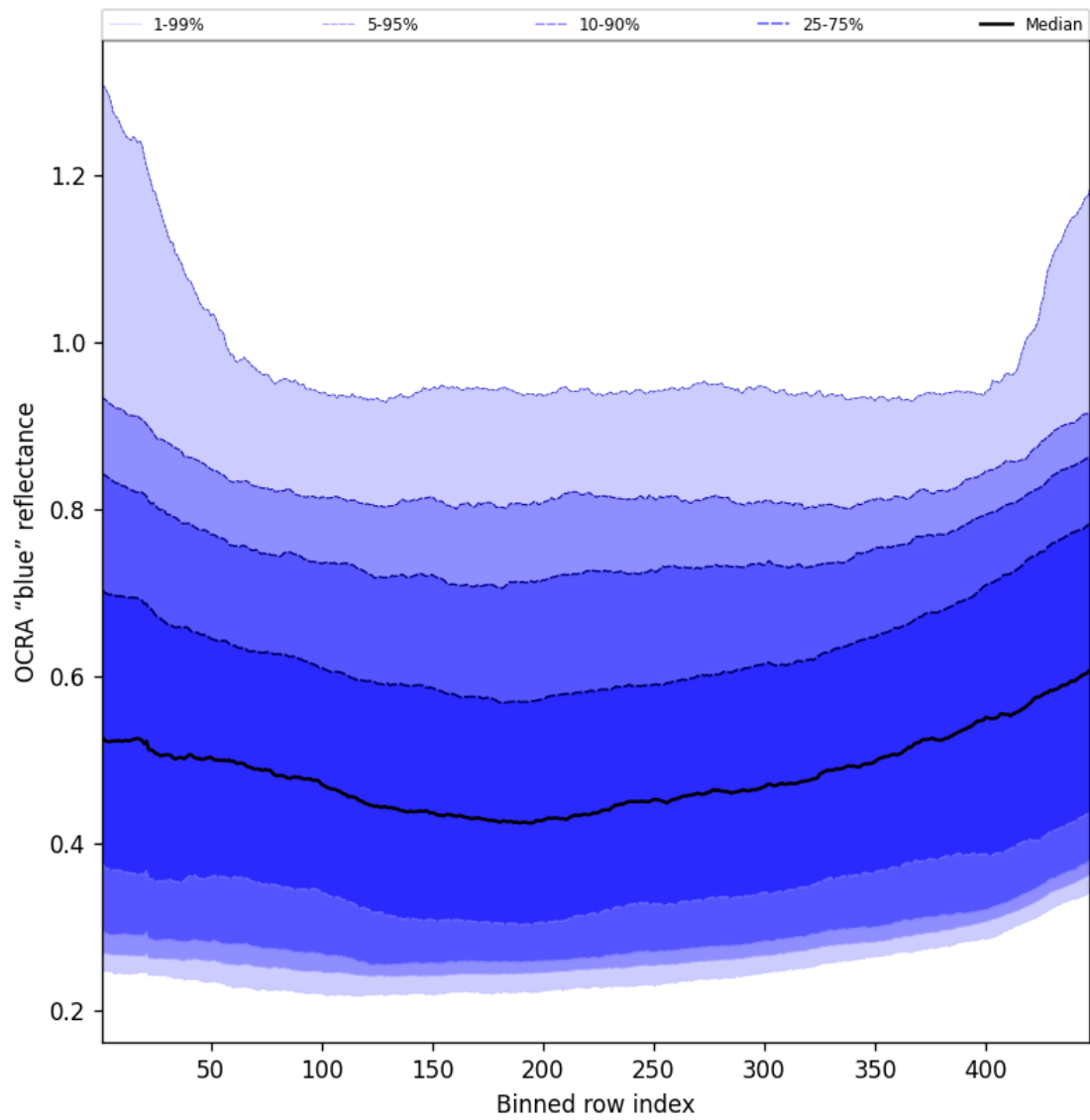
Figure 67: Along track statistics of “OCRA “blue” reflectance” for 2025-07-21 to 2025-07-23
