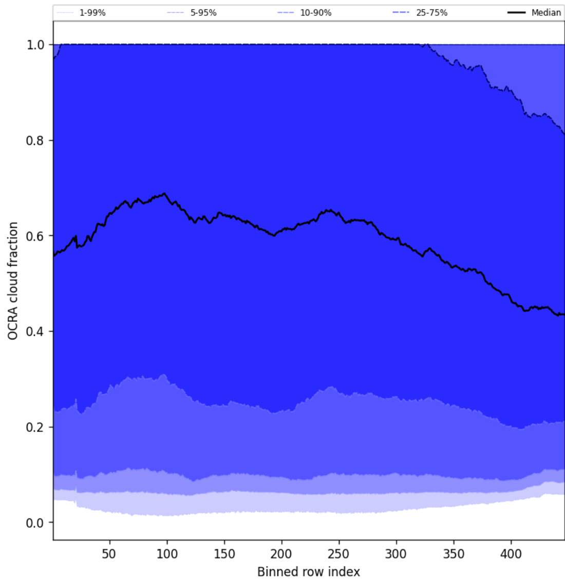
Figure 66: Along track statistics of “OCRA cloud fraction” for 2025-07-21 to 2025-07-23
