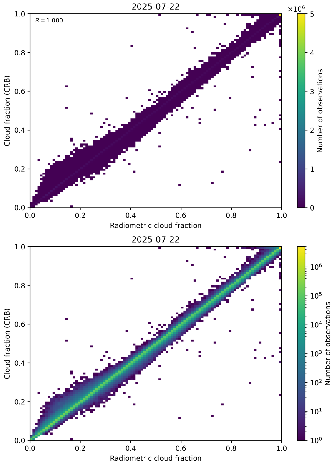
Figure 73: Scatter density plot of “Radiometric cloud fraction” against “Cloud fraction (CRB)” for 2025-07-21 to 2025-07-23.
