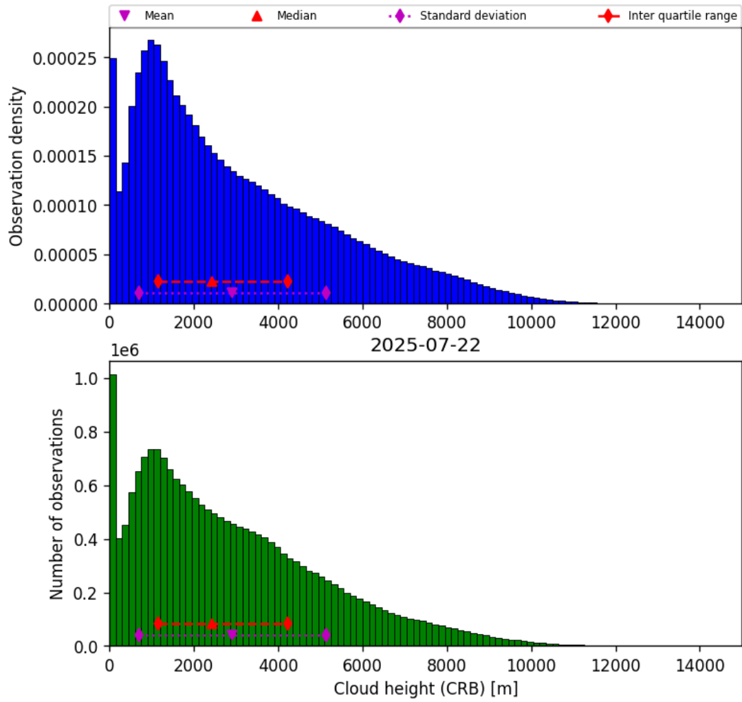
Figure 43: Histogram of “Cloud height (CRB)” for 2025-07-21 to 2025-07-23
