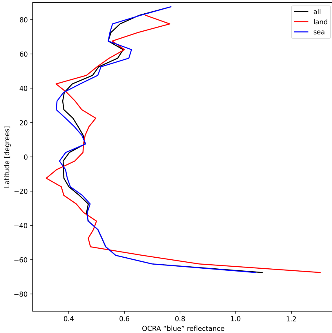
Figure 35: Zonal average of "OCRA "blue" reflectance" for 2025-07-21 to 2025-07-23.
