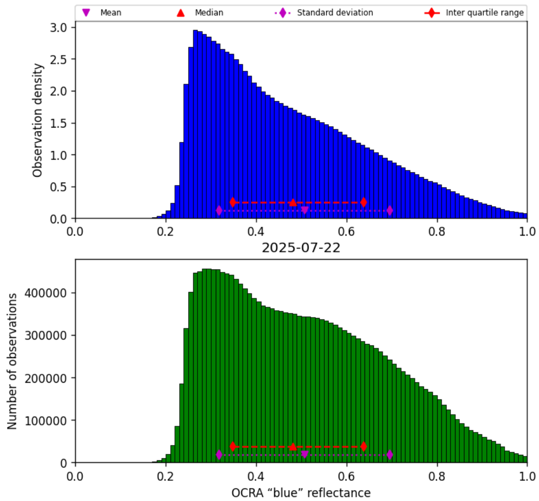
Figure 51: Histogram of “OCRA “blue” reflectance” for 2025-07-21 to 2025-07-23
