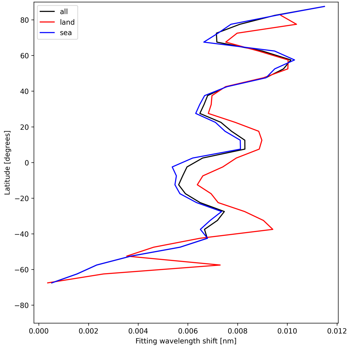
Figure 33: Zonal average of “Fitting wavelength shift” for 2025-07-21 to 2025-07-23.
