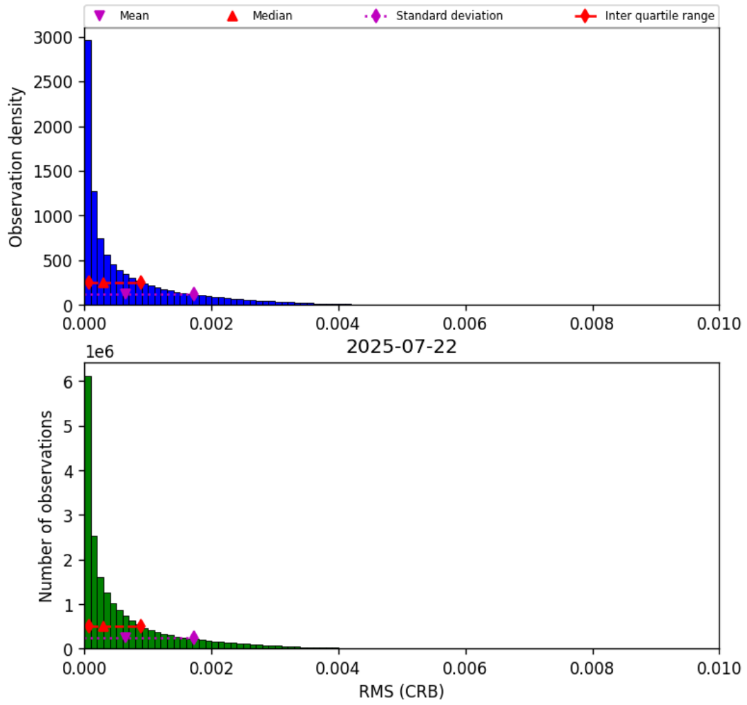
Figure 48: Histogram of “RMS (CRB)” for 2025-07-21 to 2025-07-23
