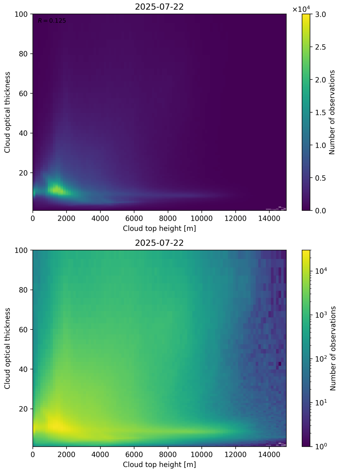
Figure 90: Scatter density plot of “Cloud top height” against “Cloud optical thickness” for 2025-07-21 to 2025-07-23.
