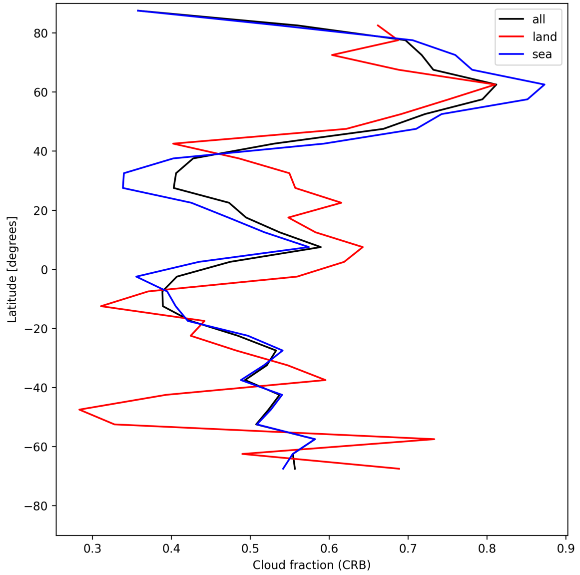
Figure 26: Zonal average of “Cloud fraction (CRB)” for 2025-07-21 to 2025-07-23.
