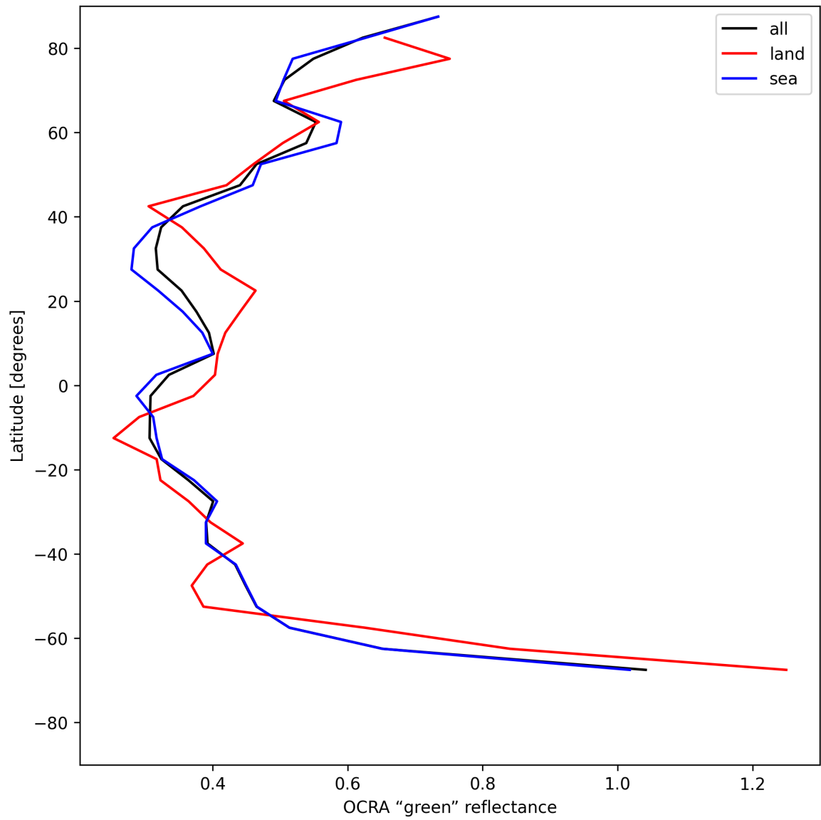
Figure 36: Zonal average of “OCRA “green” reflectance” for 2025-07-21 to 2025-07-23.
