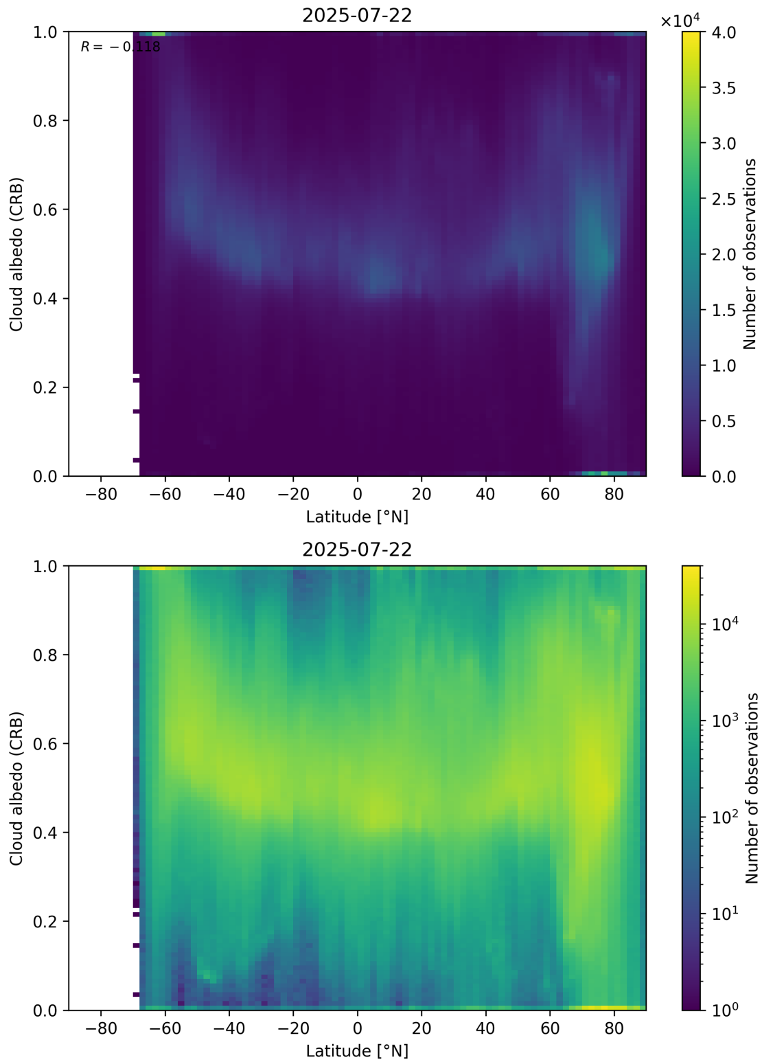
Figure 91: Scatter density plot of “Latitude” against “Cloud albedo (CRB)” for 2025-07-21 to 2025-07-23.
