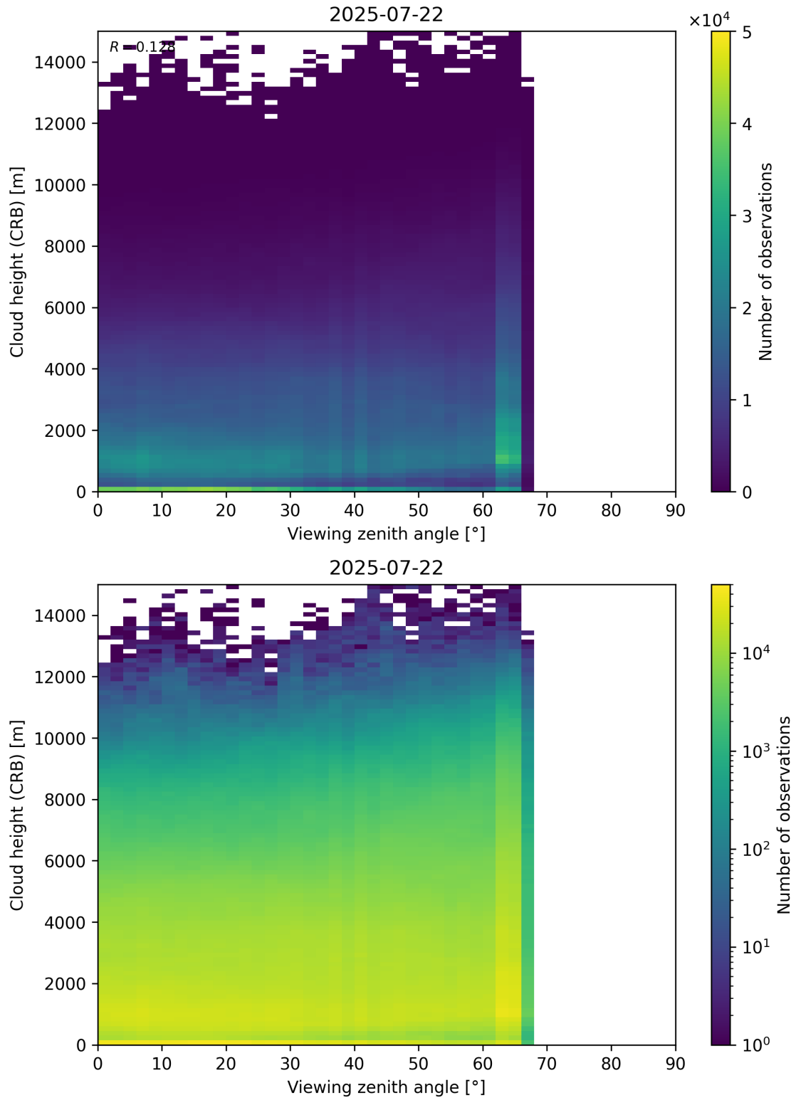
Figure 110: Scatter density plot of “Viewing zenith angle” against “Cloud height (CRB)” for 2025-07-21 to 2025-07-23.
