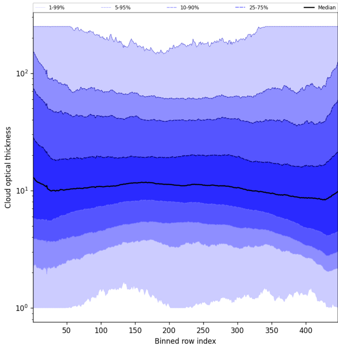
Figure 57: Along track statistics of “Cloud optical thickness” for 2025-07-21 to 2025-07-23
