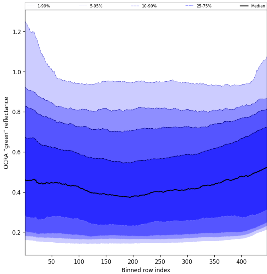
Figure 68: Along track statistics of “OCRA “green” reflectance” for 2025-07-21 to 2025-07-23
