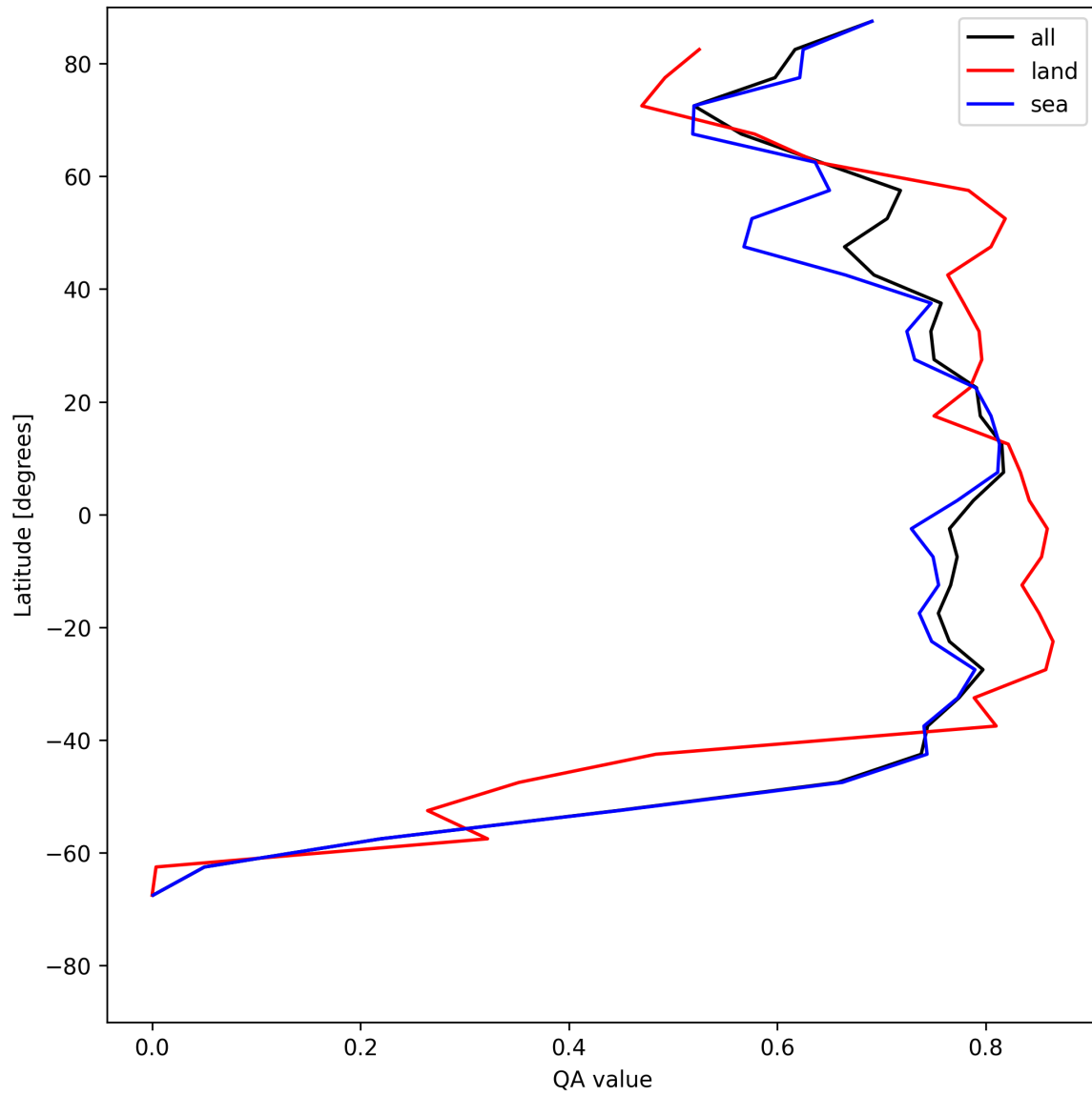
Figure 22: Zonal average of “QA value” for 2025-07-21 to 2025-07-23.
