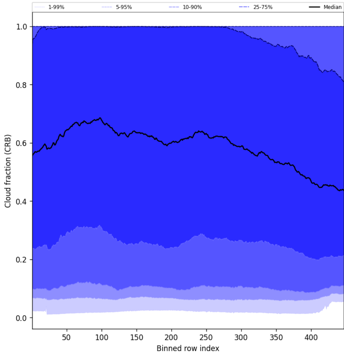
Figure 58: Along track statistics of “Cloud fraction (CRB)” for 2025-07-21 to 2025-07-23
