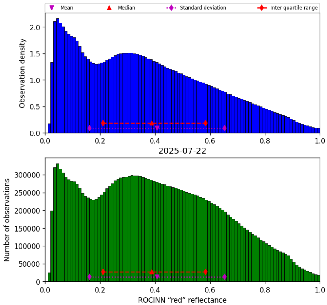
Figure 53: Histogram of “ROCINN “red” reflectance” for 2025-07-21 to 2025-07-23
