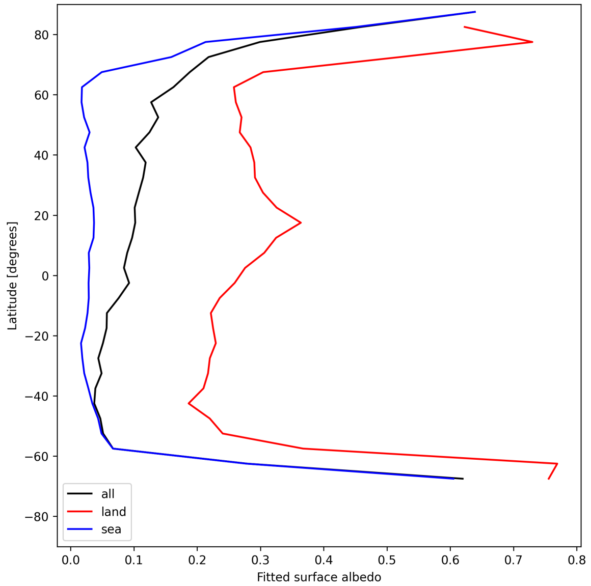
Figure 29: Zonal average of “Fitted surface albedo” for 2025-07-21 to 2025-07-23.
