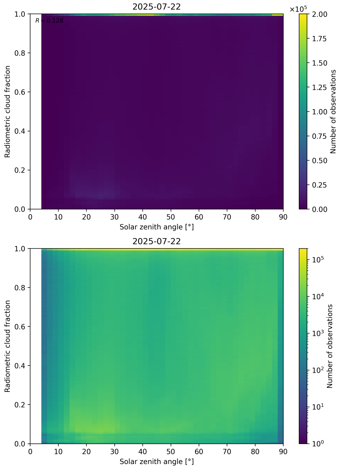
Figure 99: Scatter density plot of “Solar zenith angle” against “Radiometric cloud fraction” for 2025-07-21 to 2025-07-23.
