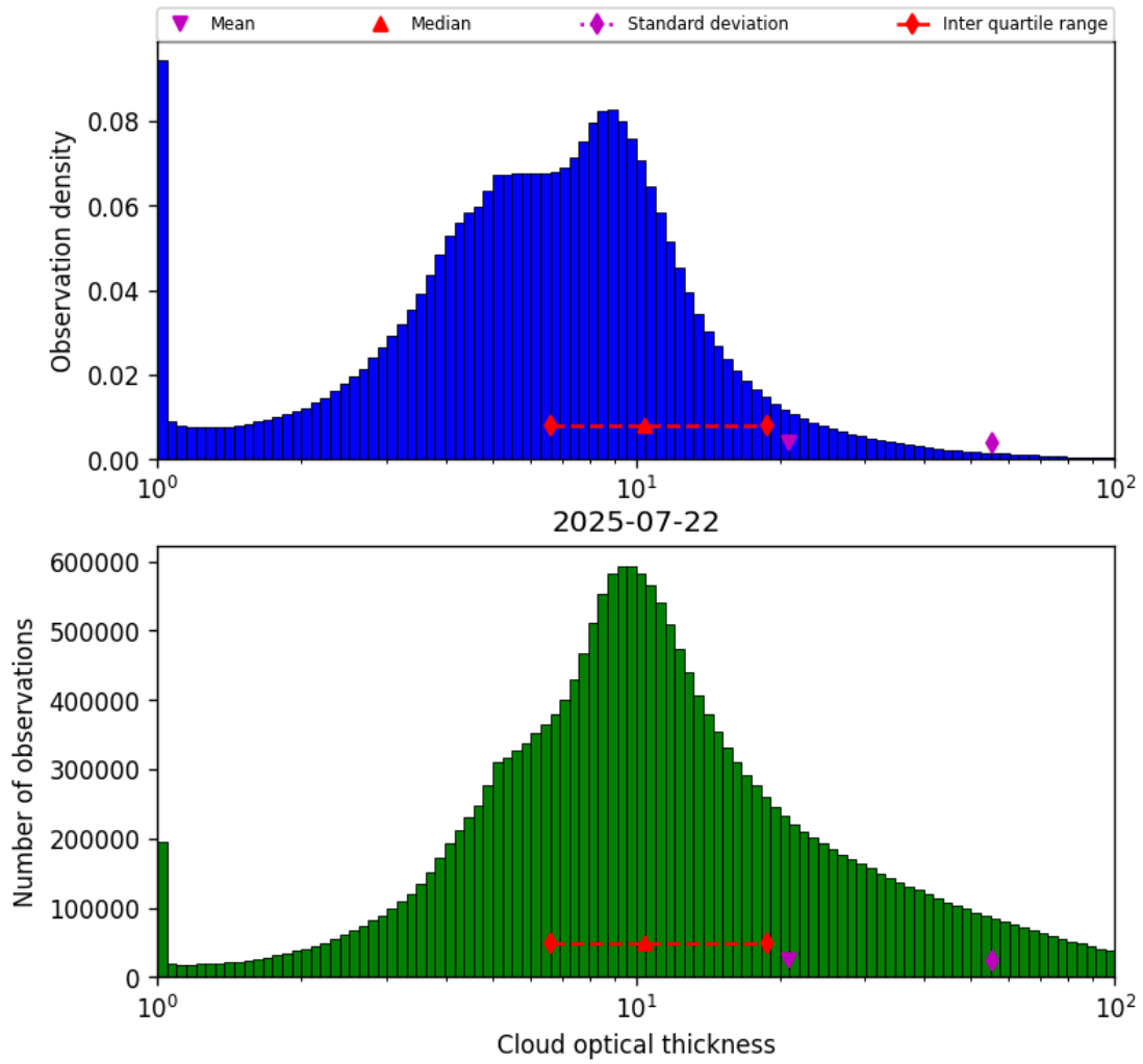
Figure 41: Histogram of “Cloud optical thickness” for 2025-07-21 to 2025-07-23
