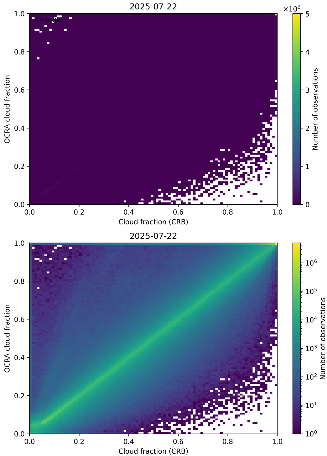
Figure 78: Scatter density plot of “Cloud fraction (CRB)” against “OCRA cloud fraction” for 2025-07-21 to 2025-07-23.
