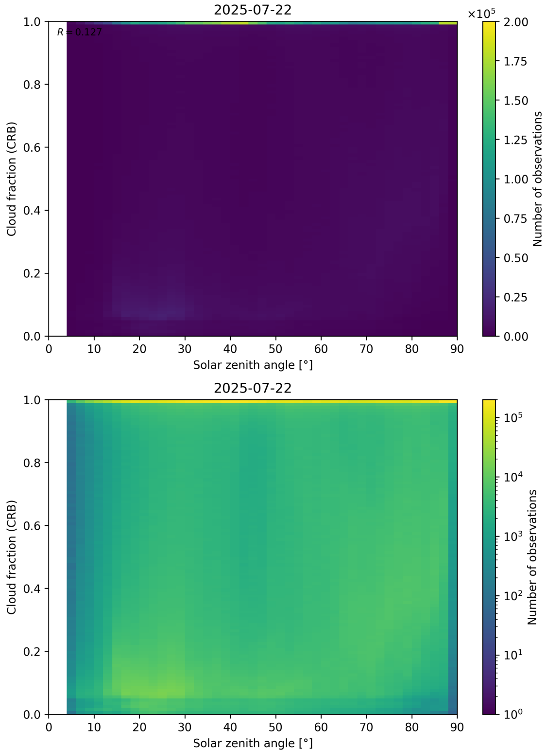
Figure 101: Scatter density plot of “Solar zenith angle” against “Cloud fraction (CRB)” for 2025-07-21 to 2025-07-23.
