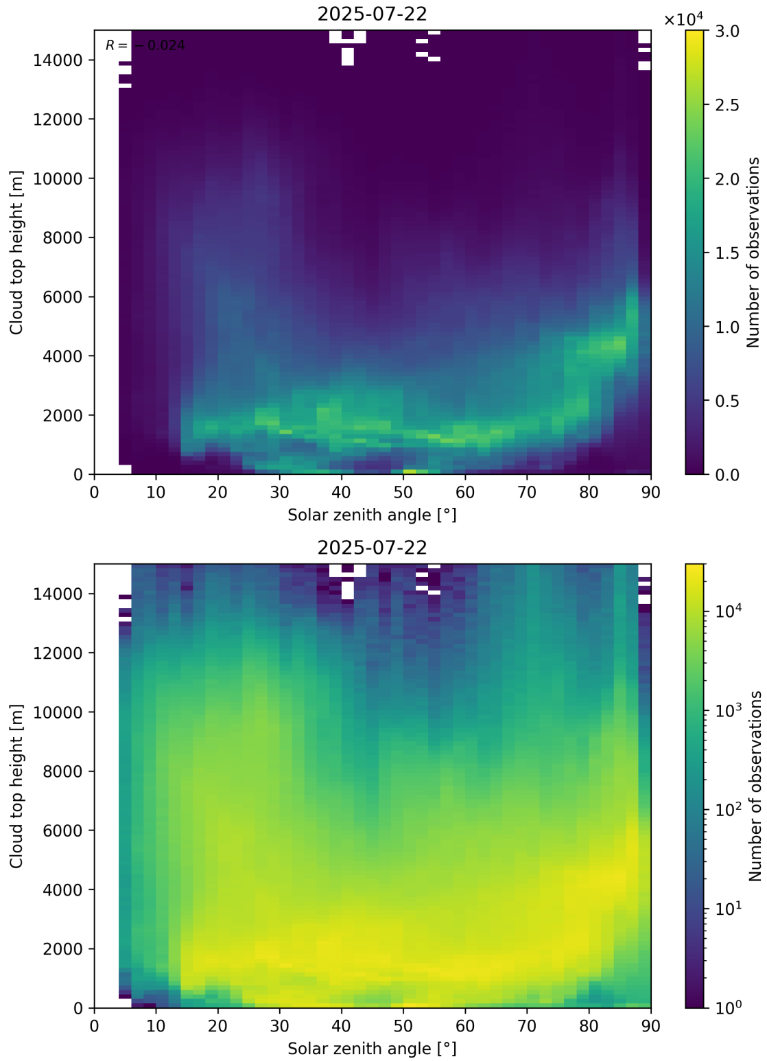
Figure 104: Scatter density plot of “Solar zenith angle” against “Cloud top height” for 2025-07-21 to 2025-07-23.
