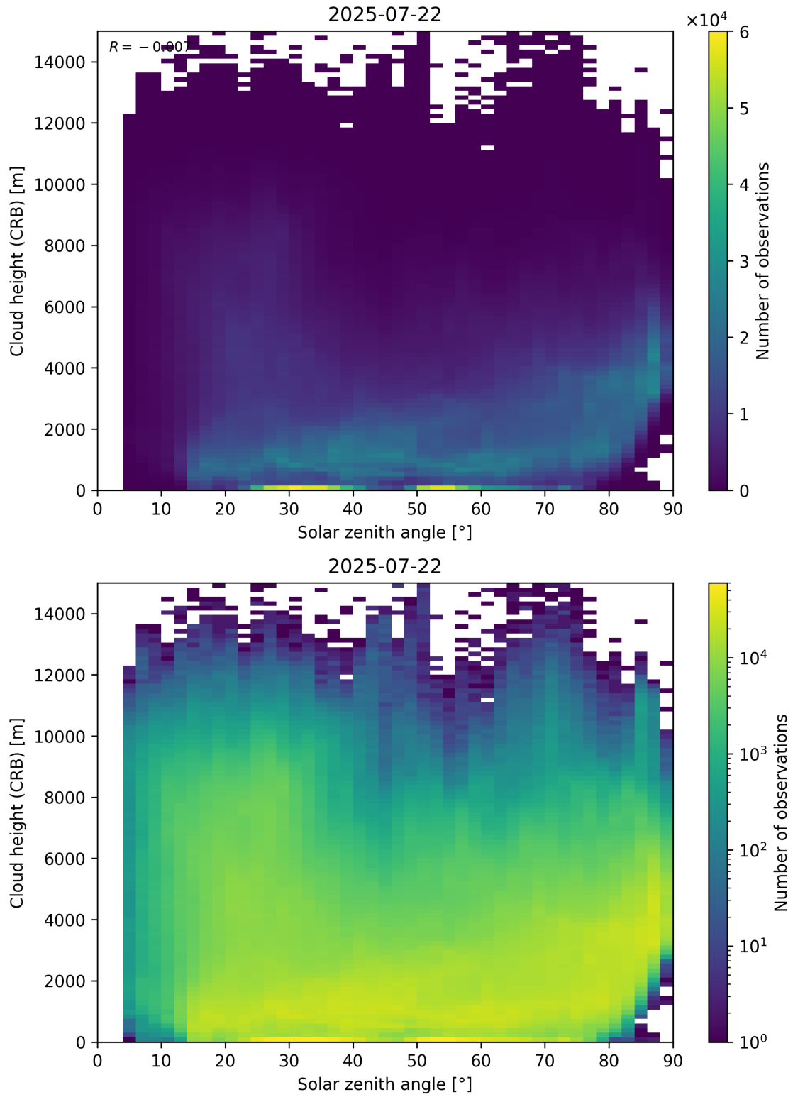
Figure 102: Scatter density plot of “Solar zenith angle” against “Cloud height (CRB)” for 2025-07-21 to 2025-07-23.
