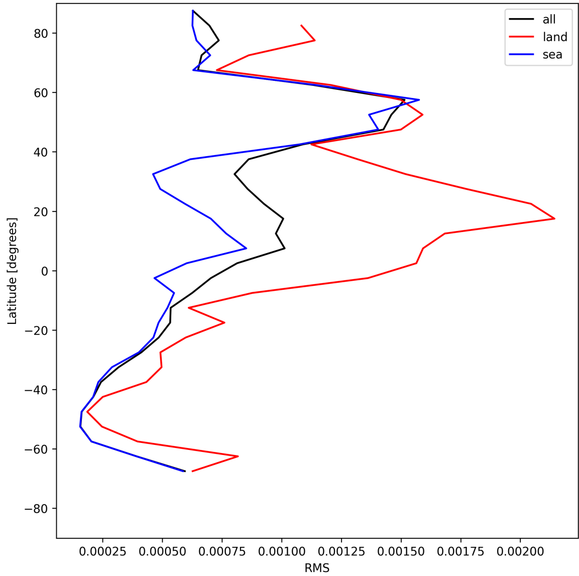
Figure 31: Zonal average of “RMS” for 2025-07-21 to 2025-07-23.
