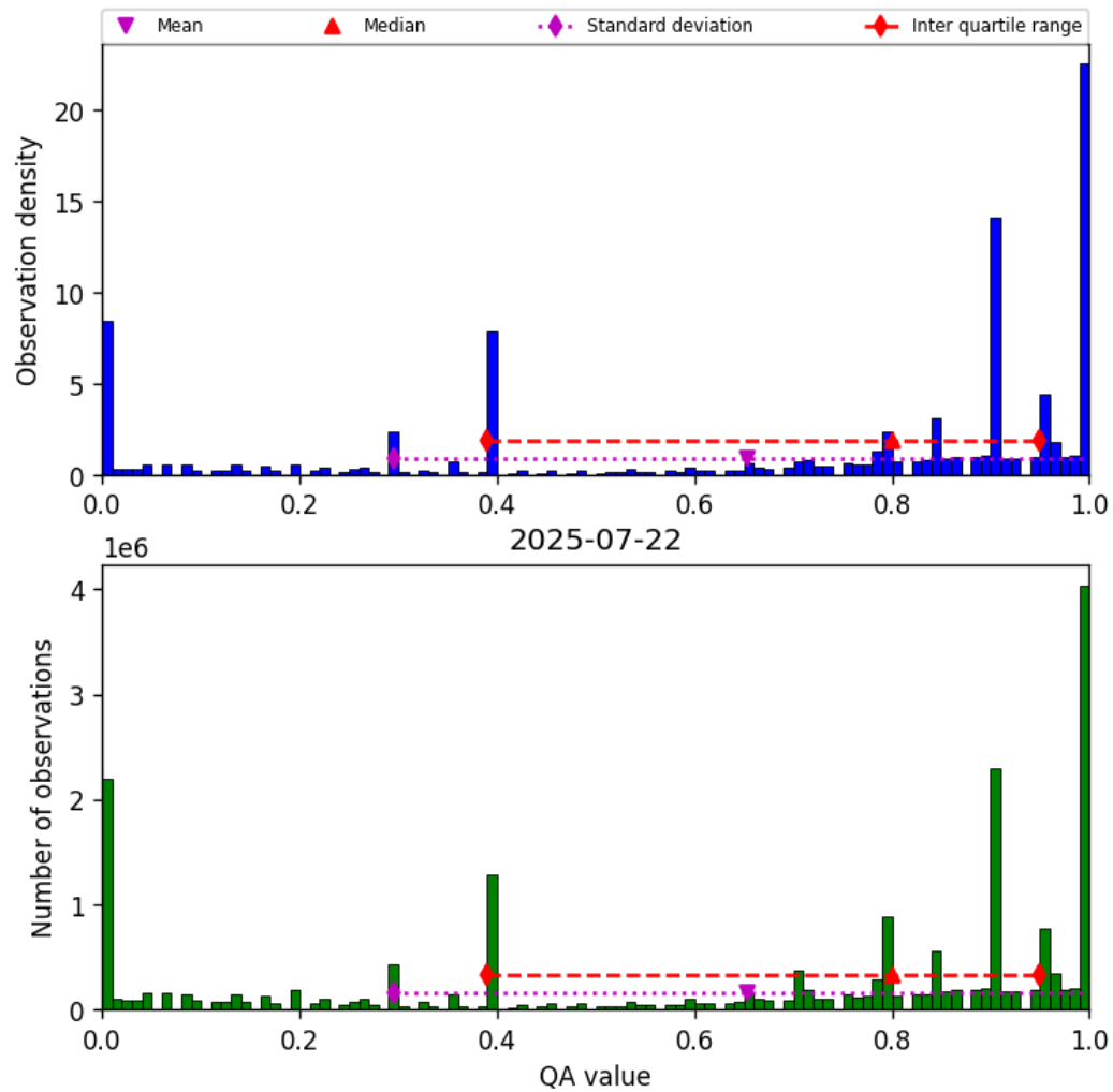
Figure 38: Histogram of “QA value” for 2025-07-21 to 2025-07-23
