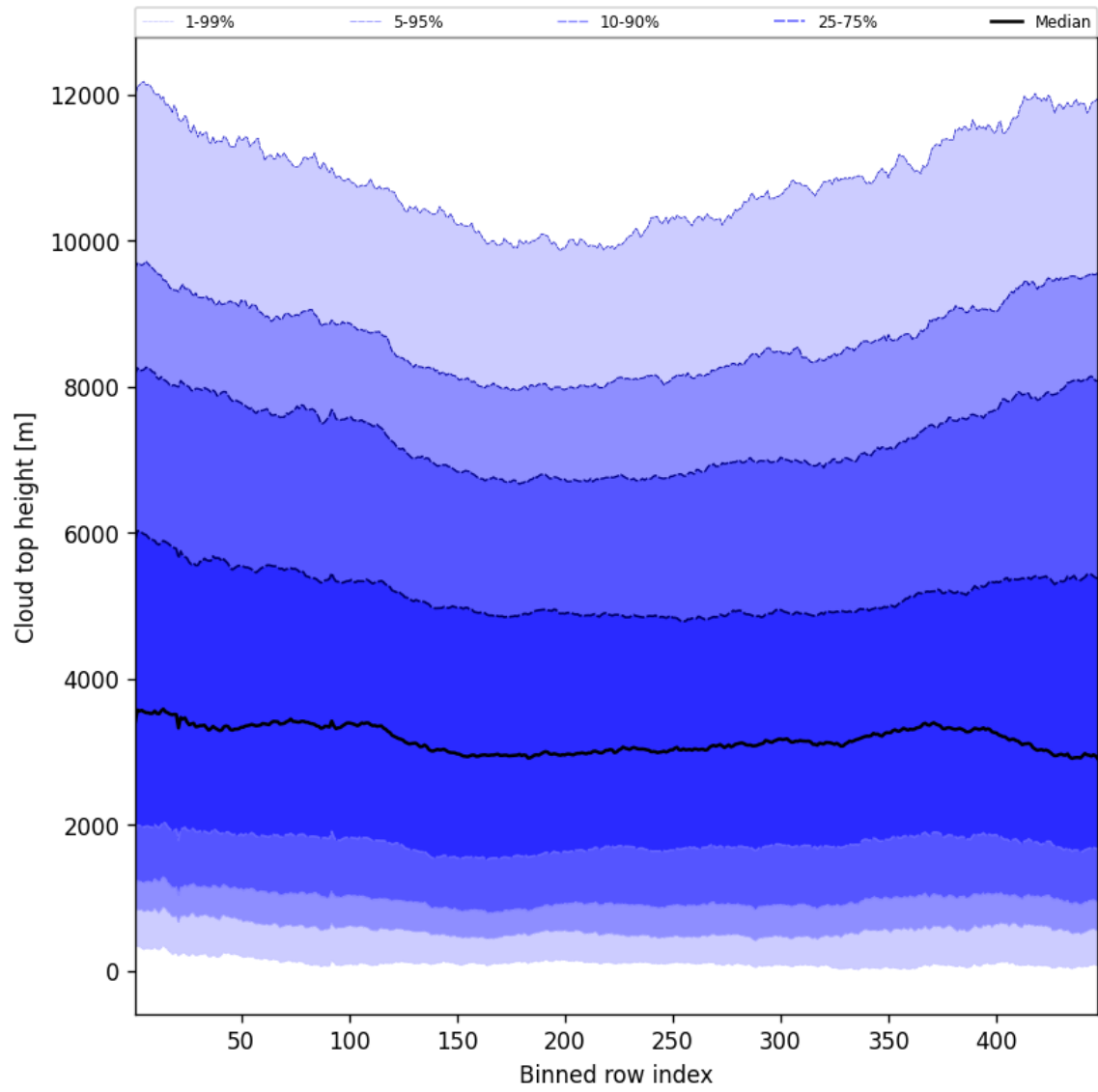
Figure 56: Along track statistics of “Cloud top height” for 2025-07-21 to 2025-07-23
