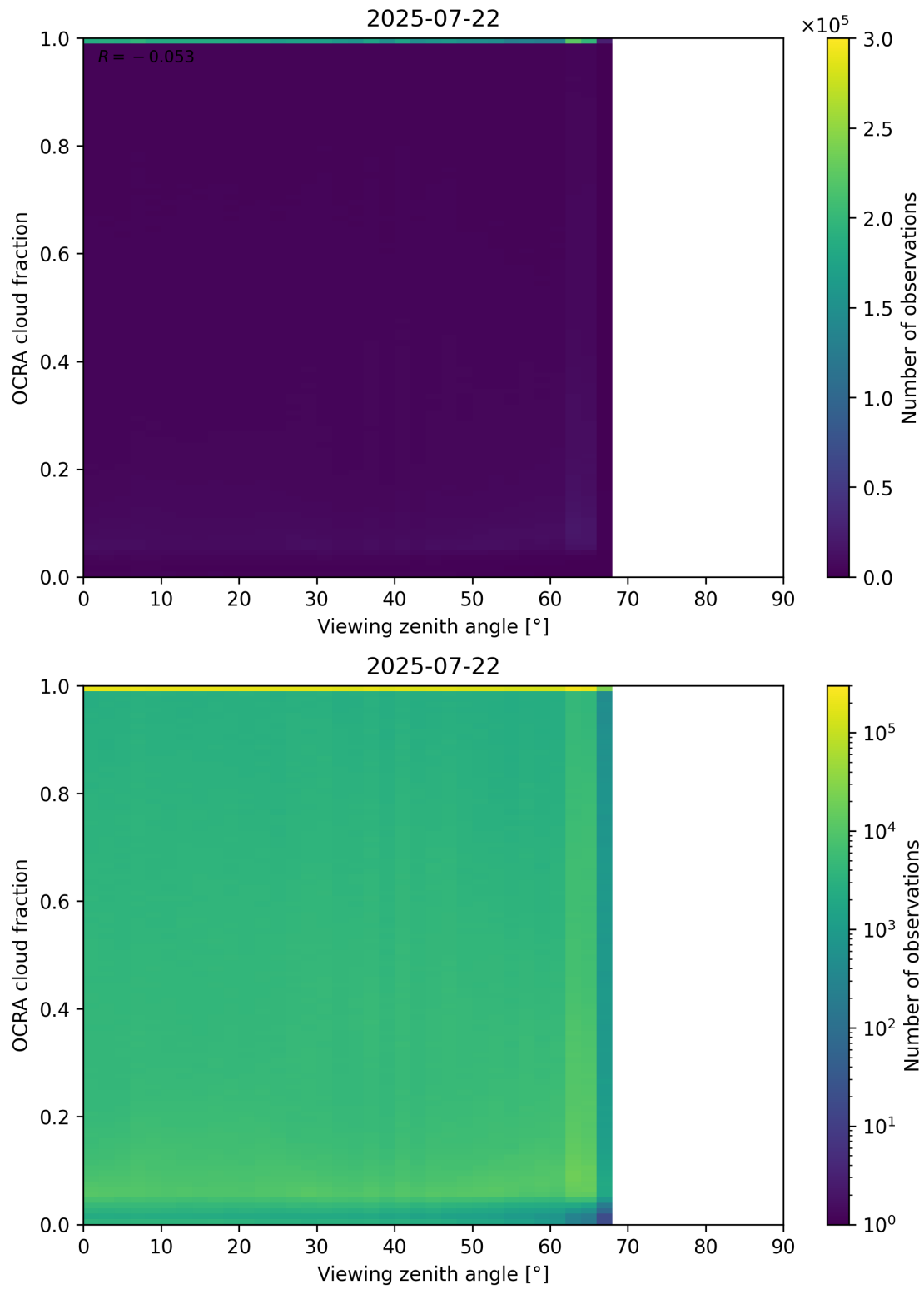
Figure 108: Scatter density plot of “Viewing zenith angle” against “OCRA cloud fraction” for 2025-07-21 to 2025-07-23.
