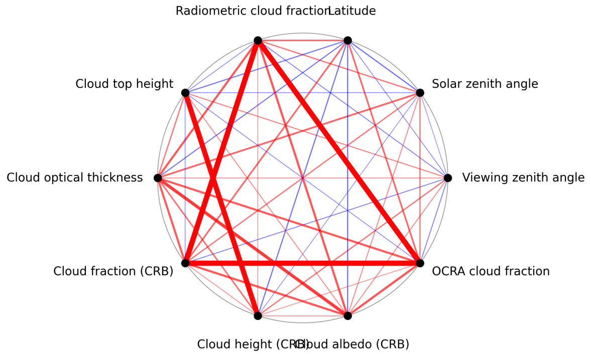
Figure 1: Map of correlation graph for 2025-07-21 to 2025-07-23.
