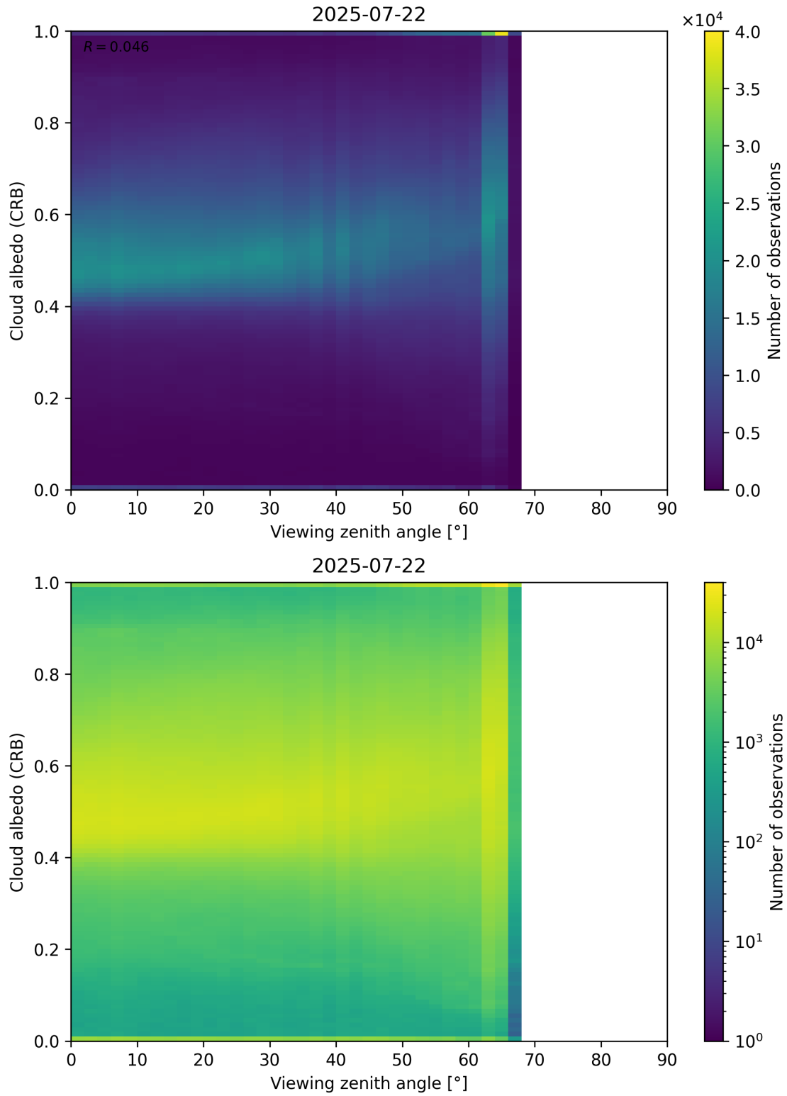
Figure 106: Scatter density plot of “Viewing zenith angle” against “Cloud albedo (CRB)” for 2025-07-21 to 2025-07-23.
