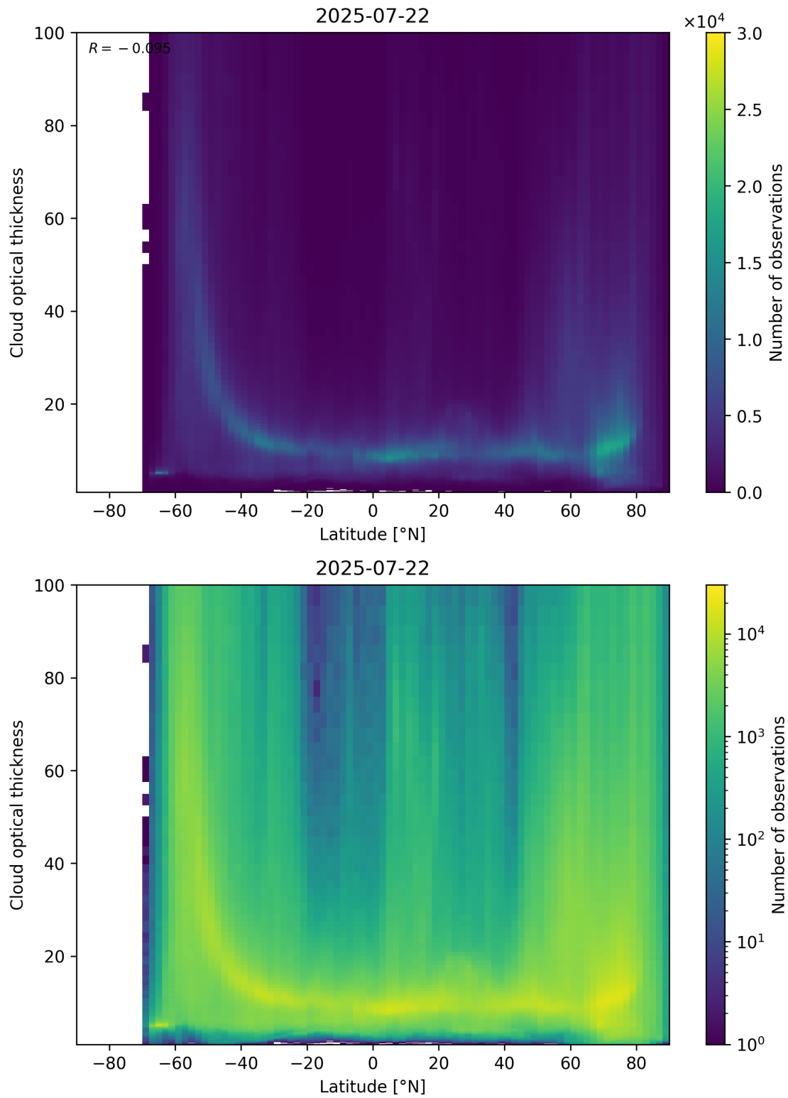
Figure 96: Scatter density plot of “Latitude” against “Cloud optical thickness” for 2025-07-21 to 2025-07-23.
