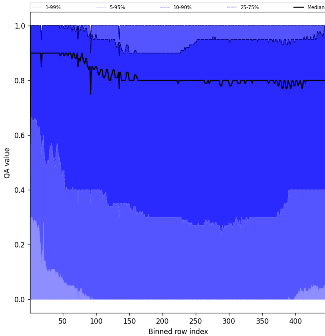
Figure 54: Along track statistics of “QA value” for 2025-07-21 to 2025-07-23
