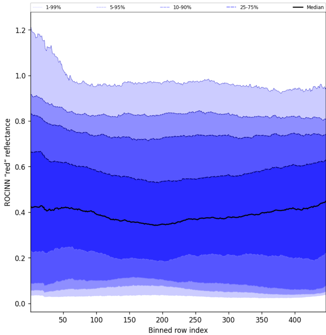
Figure 69: Along track statistics of "ROCINN "red" reflectance" for 2025-07-21 to 2025-07-23
