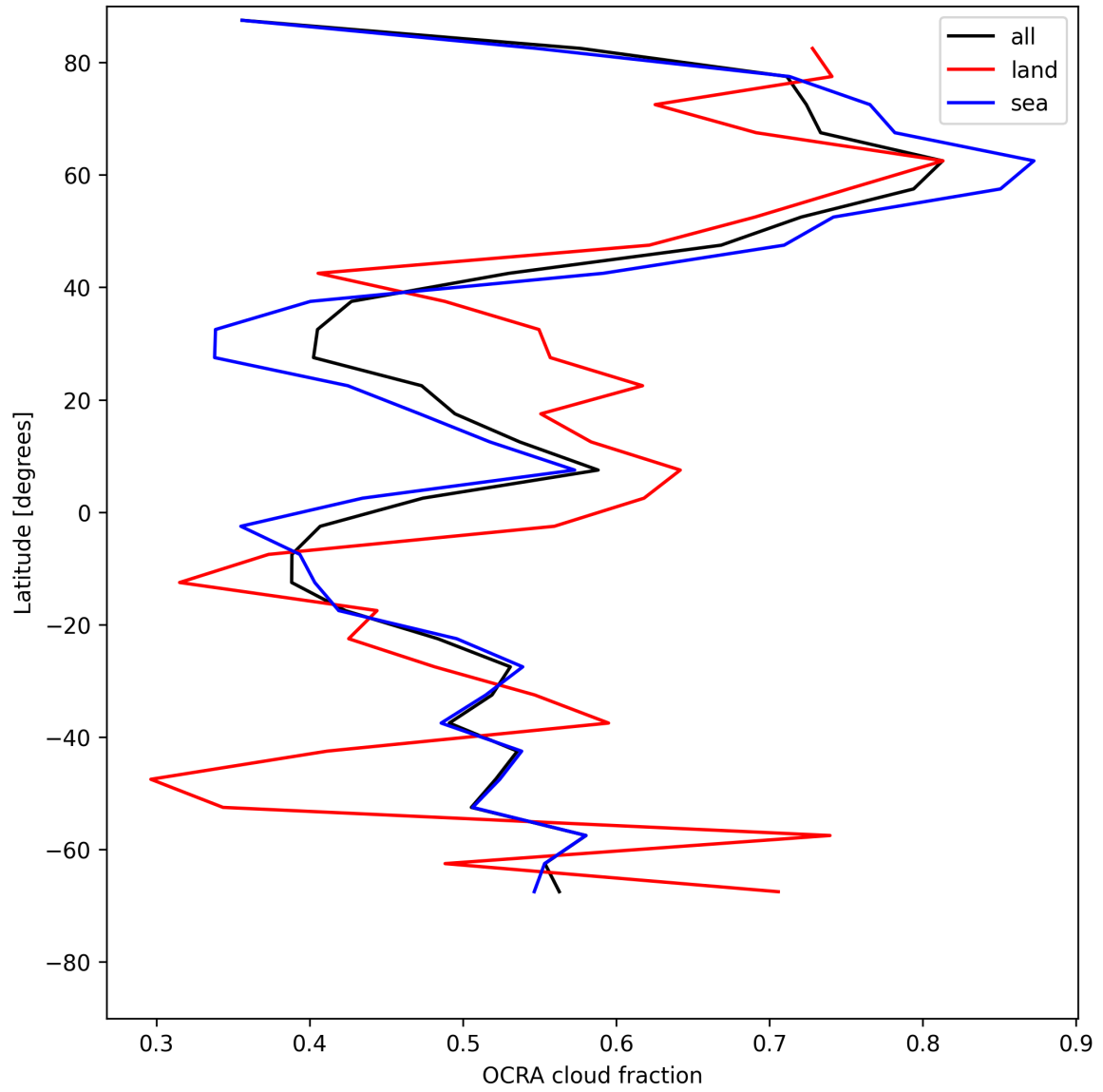
Figure 34: Zonal average of “OCRA cloud fraction” for 2025-07-21 to 2025-07-23.
