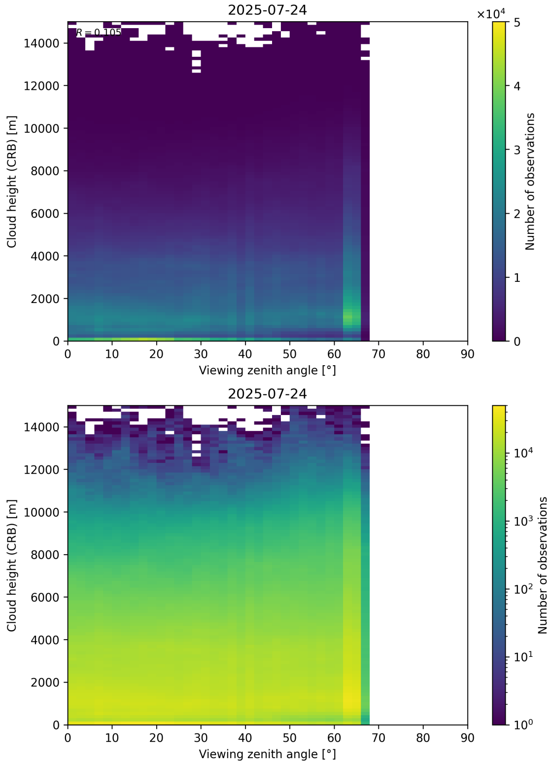
Figure 110: Scatter density plot of “Viewing zenith angle” against “Cloud height (CRB)” for 2025-07-24 to 2025-07-25.
