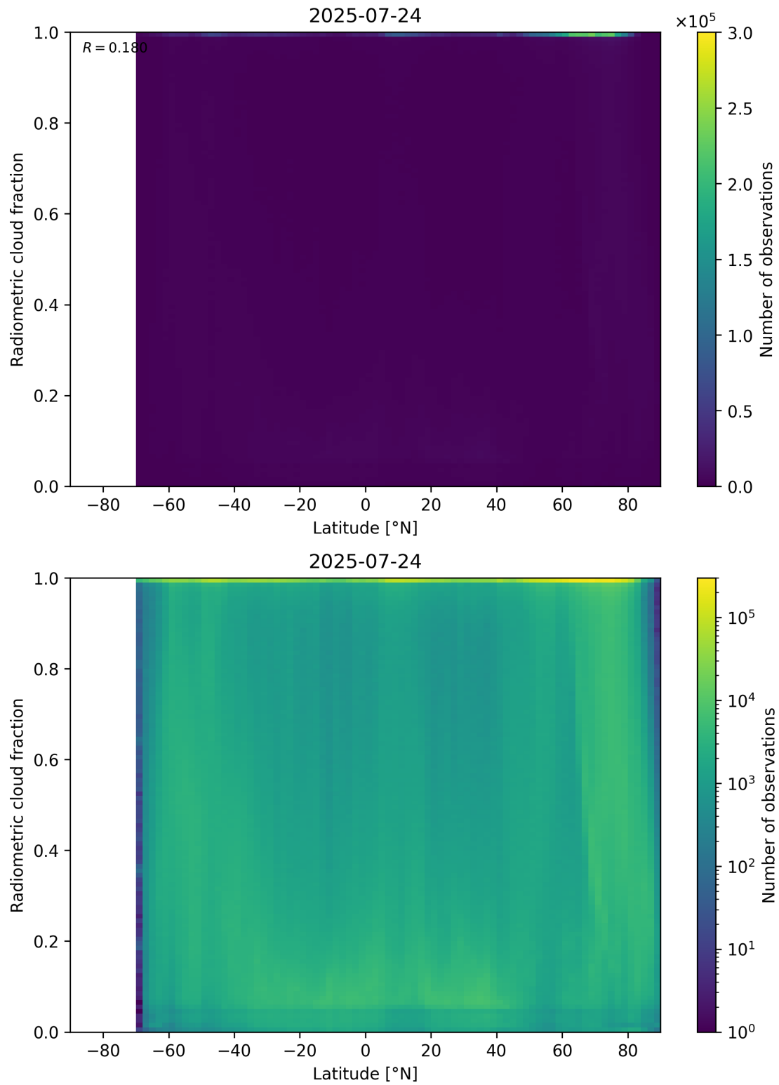
Figure 92: Scatter density plot of “Latitude” against “Radiometric cloud fraction” for 2025-07-24 to 2025-07-25.
