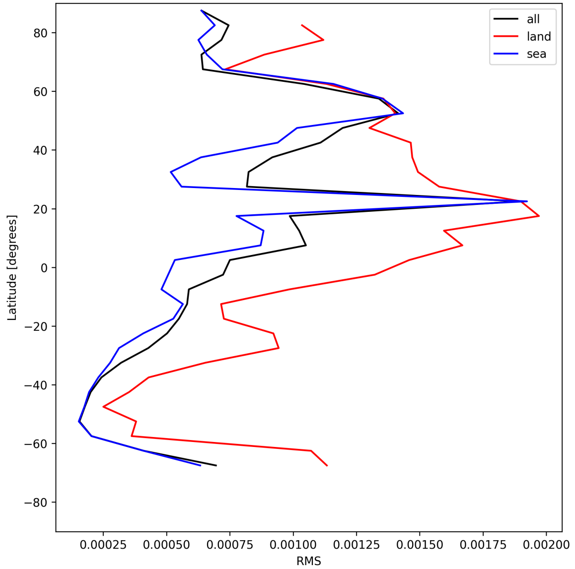
Figure 31: Zonal average of “RMS” for 2025-07-24 to 2025-07-25.
