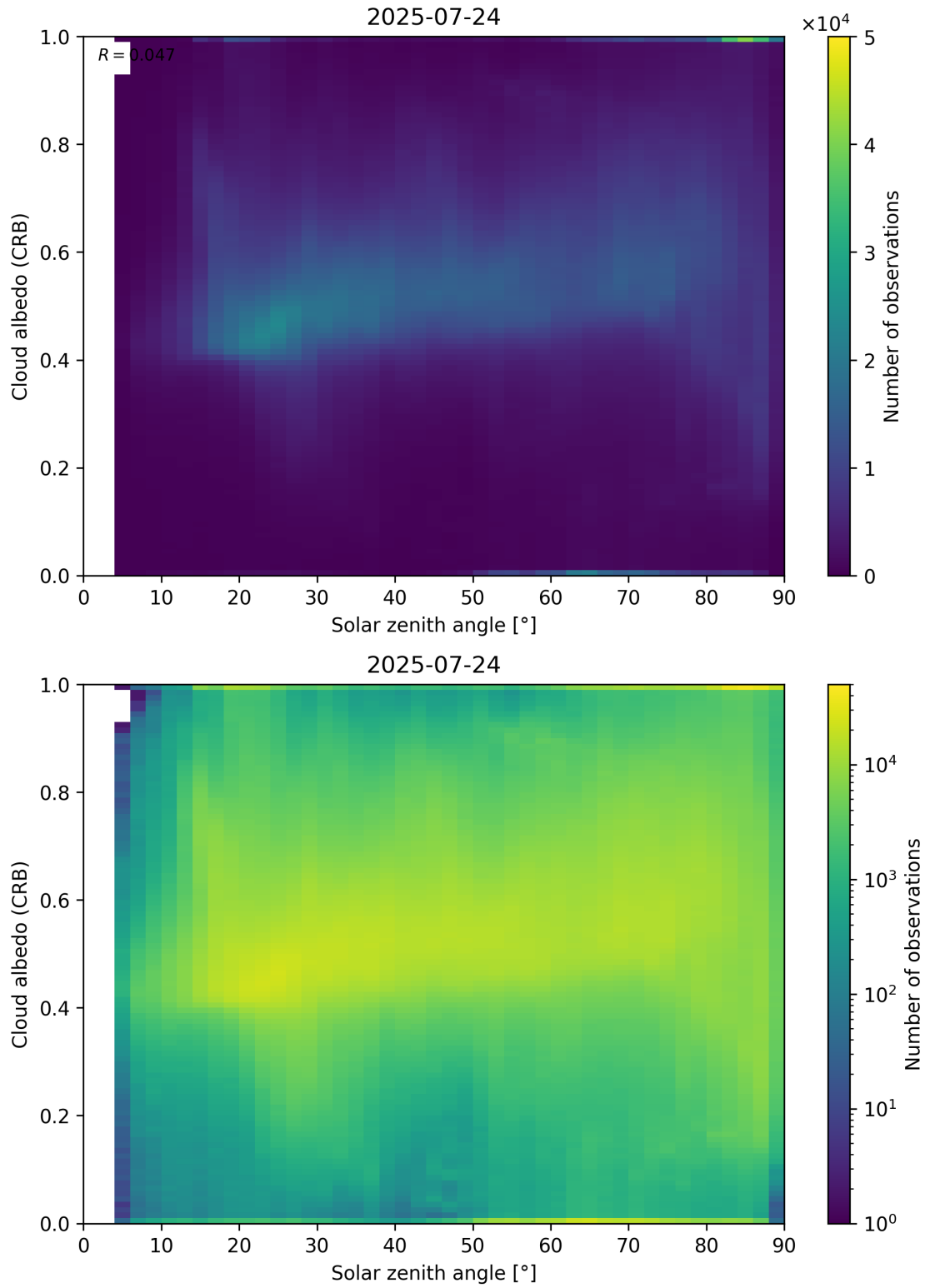
Figure 98: Scatter density plot of “Solar zenith angle” against “Cloud albedo (CRB)” for 2025-07-24 to 2025-07-25.
