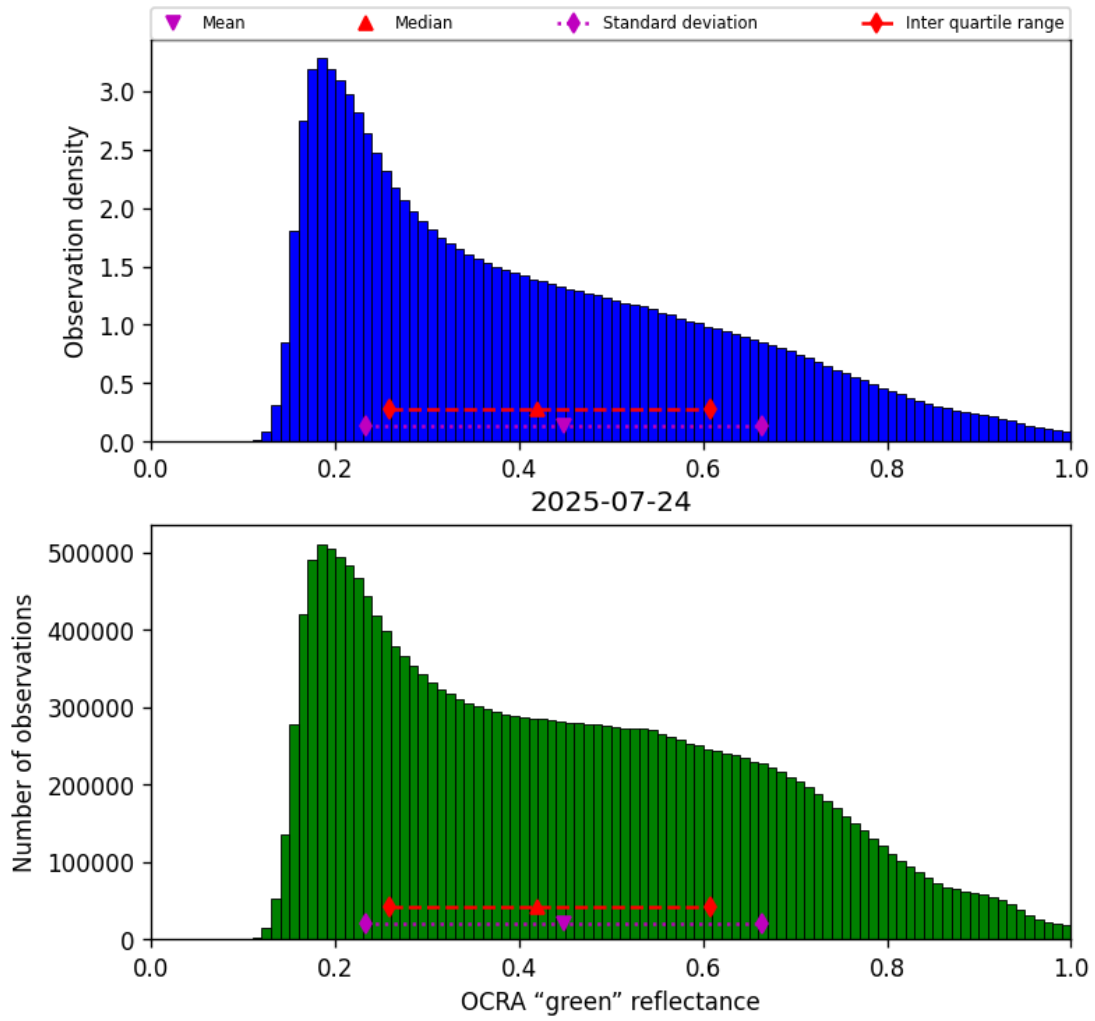
Figure 52: Histogram of “OCRA “green” reflectance” for 2025-07-24 to 2025-07-25
