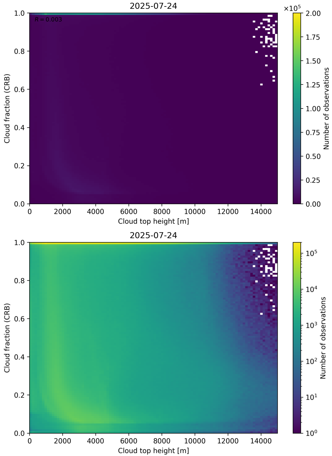
Figure 88: Scatter density plot of “Cloud top height” against “Cloud fraction (CRB)” for 2025-07-24 to 2025-07-25.
