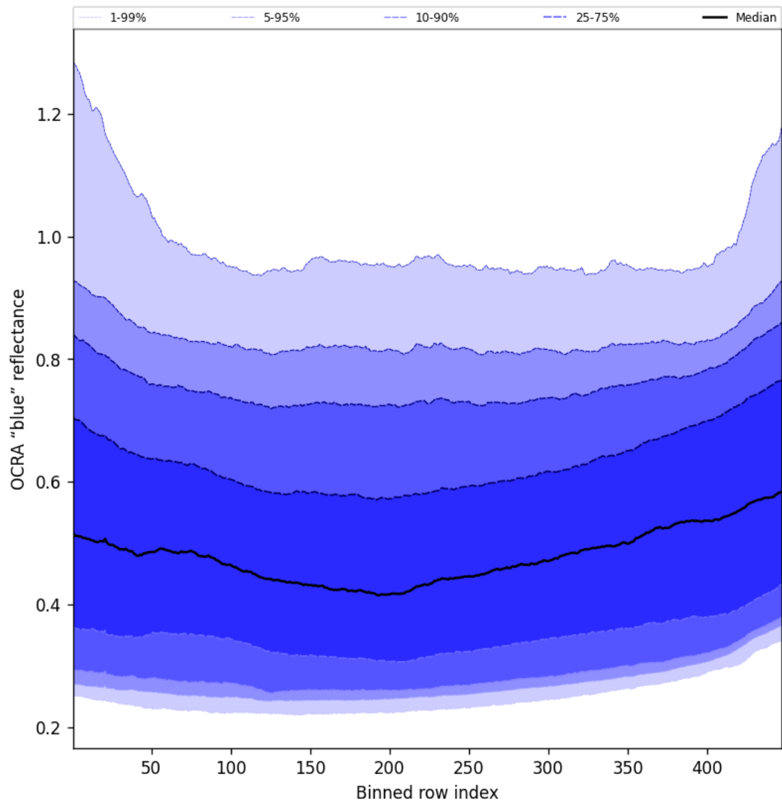
Figure 67: Along track statistics of “OCRA “blue” reflectance” for 2025-07-24 to 2025-07-25
