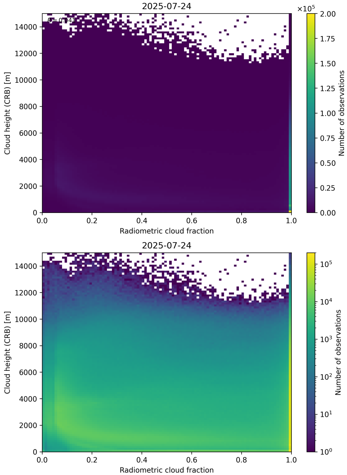
Figure 74: Scatter density plot of “Radiometric cloud fraction” against “Cloud height (CRB)” for 2025-07-24 to 2025-07-25.
