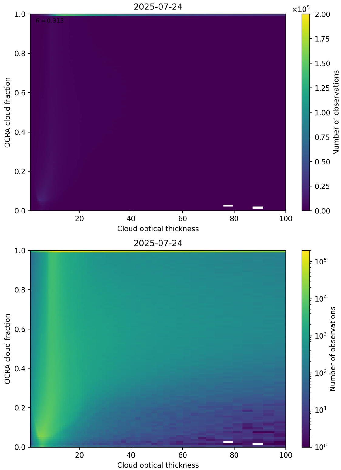
Figure 83: Scatter density plot of “Cloud optical thickness” against “OCRA cloud fraction” for 2025-07-24 to 2025-07-25.
