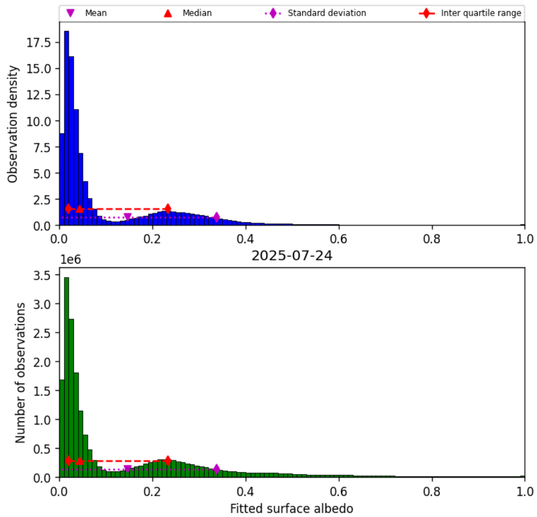
Figure 45: Histogram of “Fitted surface albedo” for 2025-07-24 to 2025-07-25
