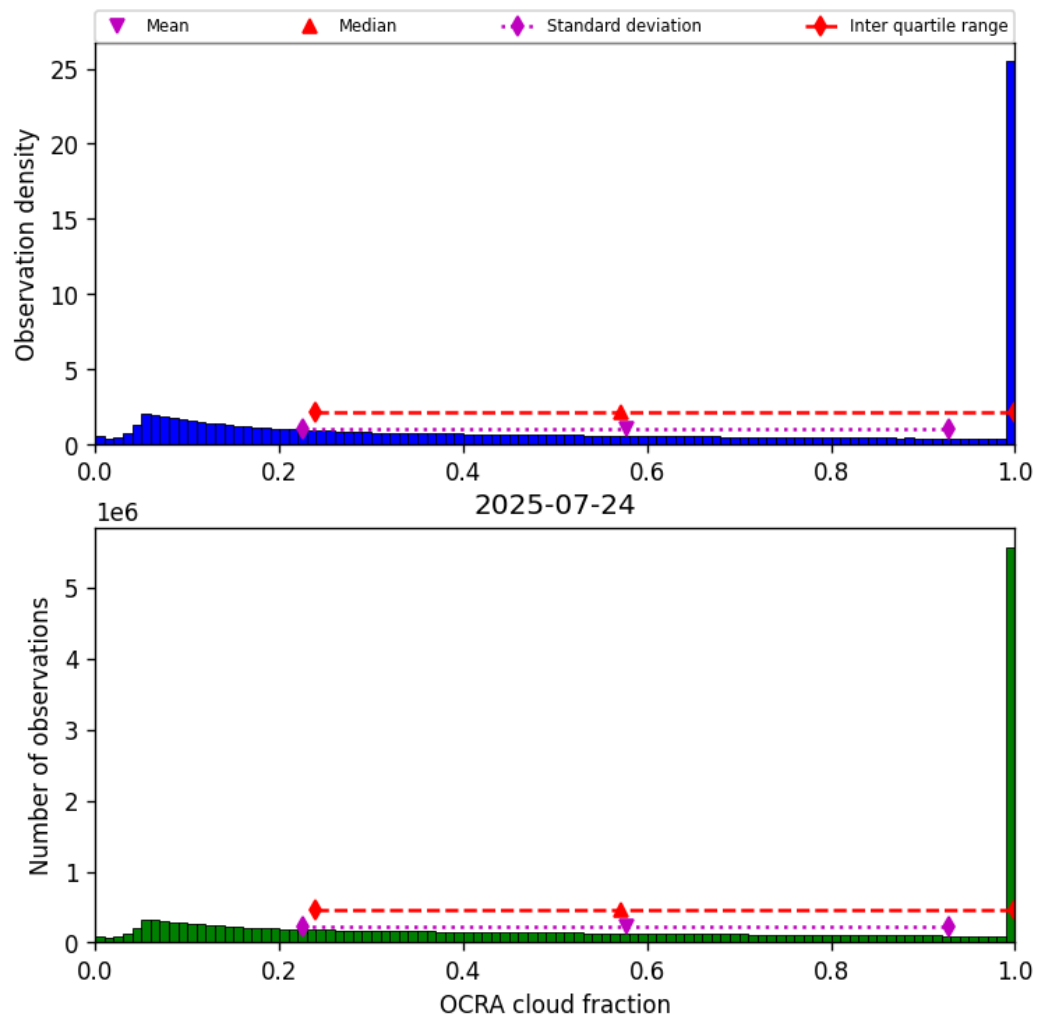
Figure 50: Histogram of “OCRA cloud fraction” for 2025-07-24 to 2025-07-25
