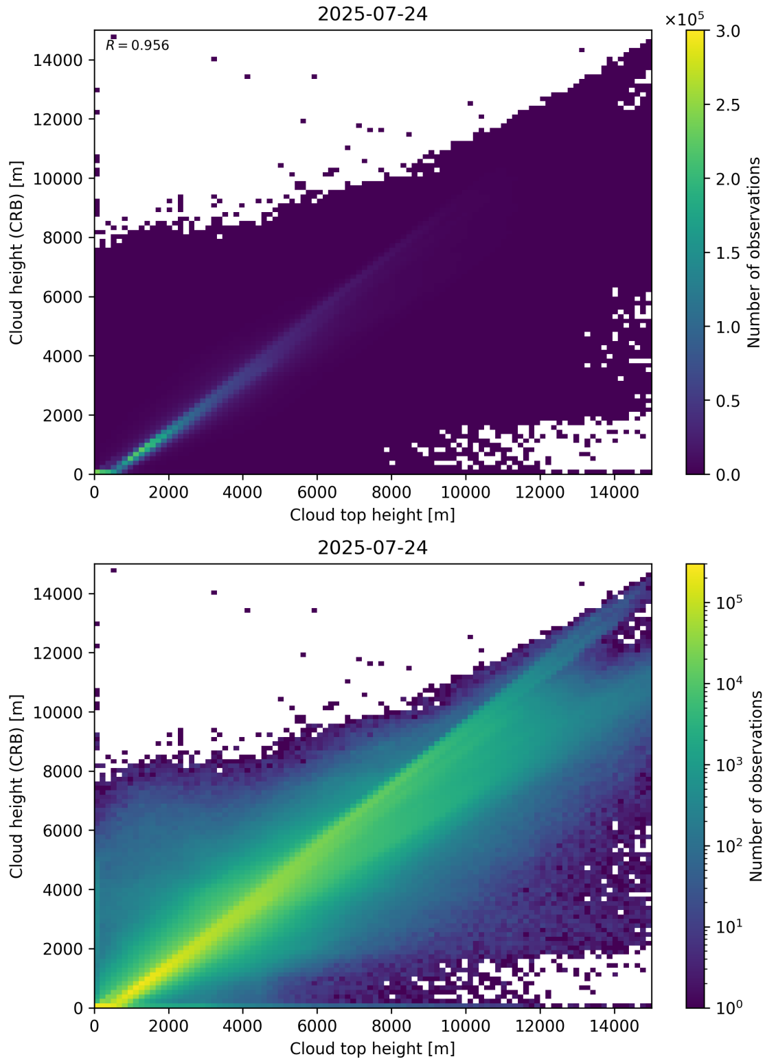
Figure 89: Scatter density plot of “Cloud top height” against “Cloud height (CRB)” for 2025-07-24 to 2025-07-25.
