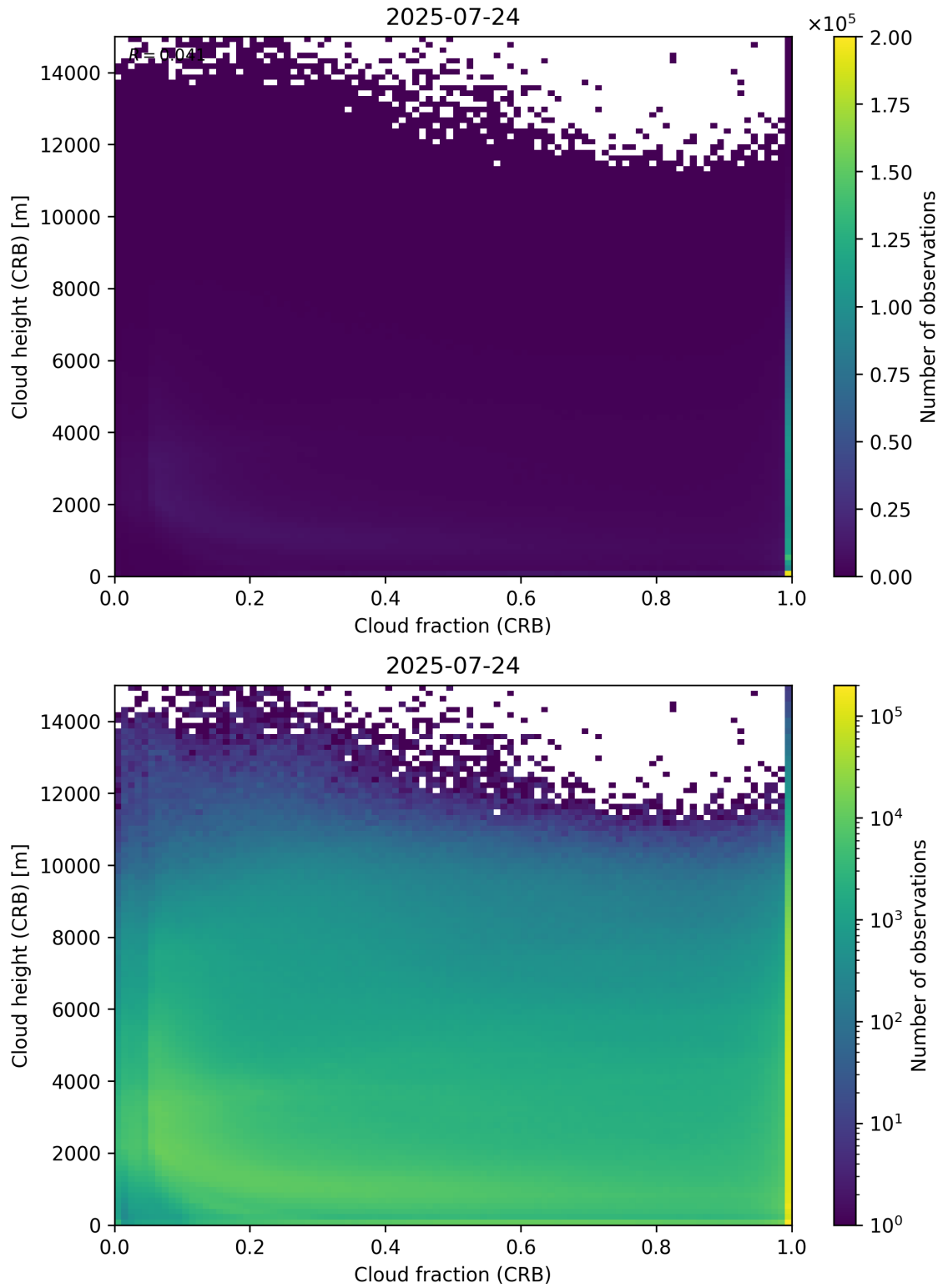
Figure 79: Scatter density plot of “Cloud fraction (CRB)” against “Cloud height (CRB)” for 2025-07-24 to 2025-07-25.
