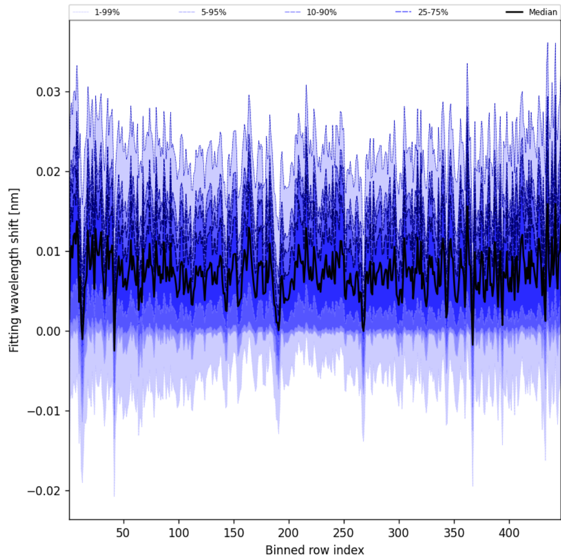
Figure 65: Along track statistics of “Fitting wavelength shift” for 2025-07-24 to 2025-07-25
