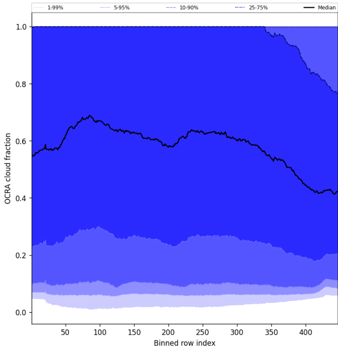
Figure 66: Along track statistics of “OCRA cloud fraction” for 2025-07-24 to 2025-07-25
