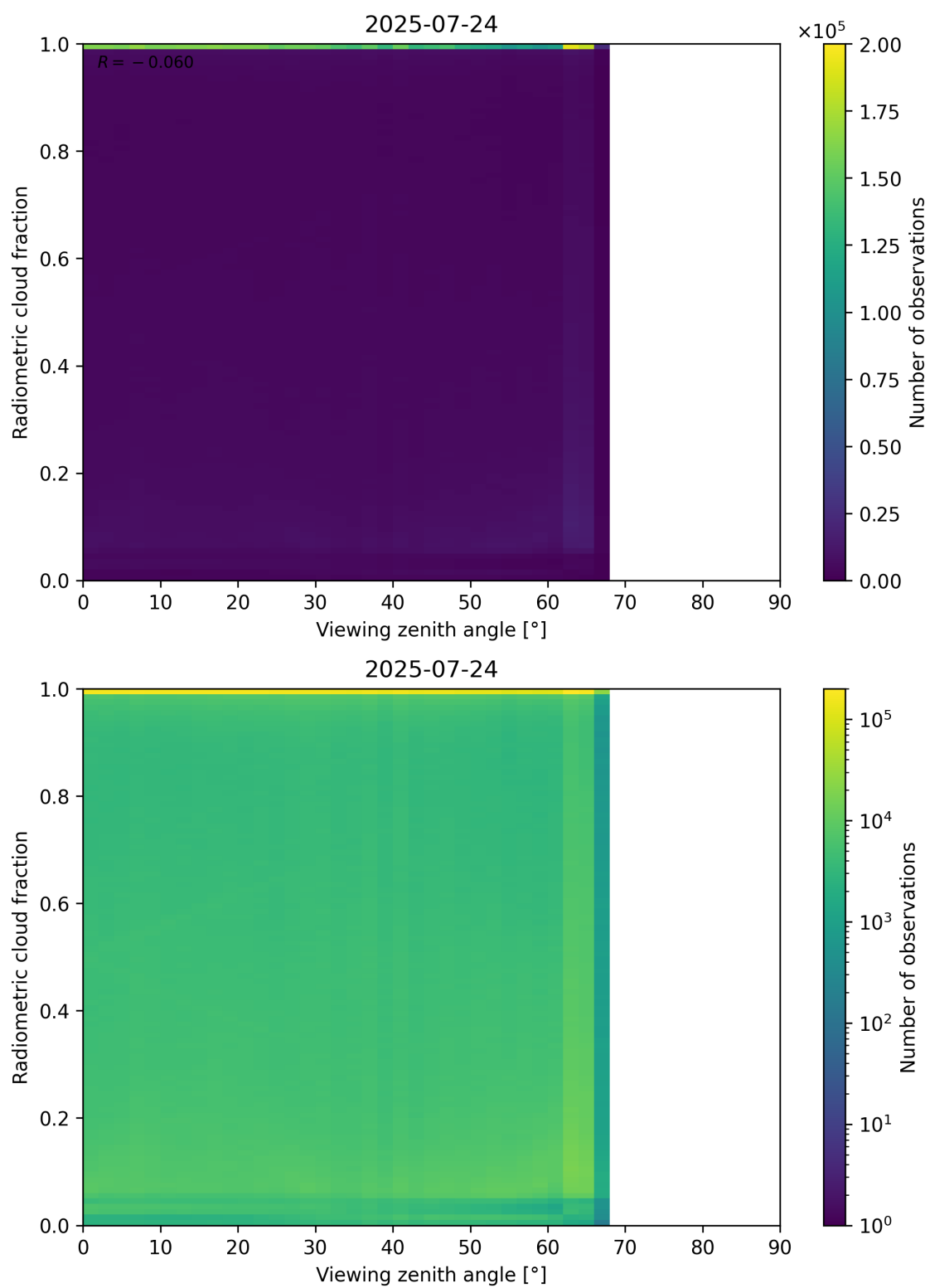
Figure 107: Scatter density plot of “Viewing zenith angle” against “Radiometric cloud fraction” for 2025-07-24 to 2025-07-25.
