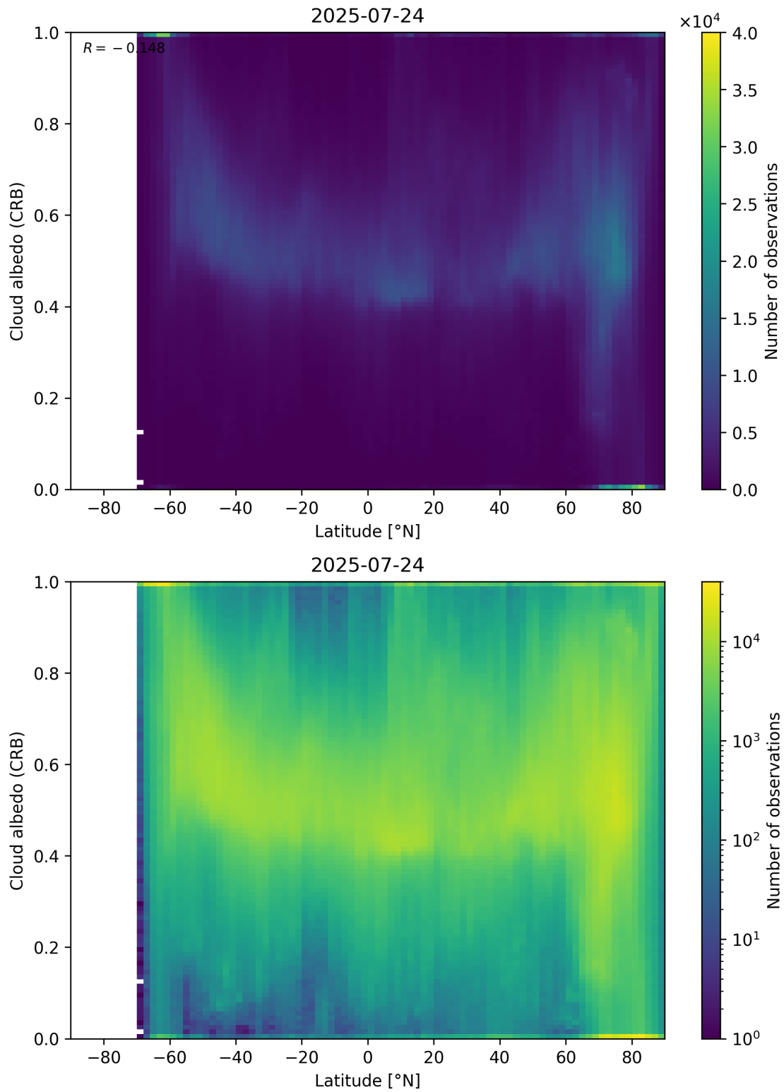
Figure 91: Scatter density plot of “Latitude” against “Cloud albedo (CRB)” for 2025-07-24 to 2025-07-25.
