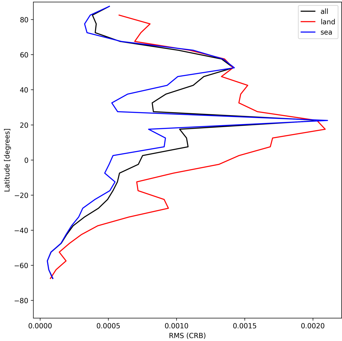
Figure 32: Zonal average of “RMS (CRB)” for 2025-07-24 to 2025-07-25.
