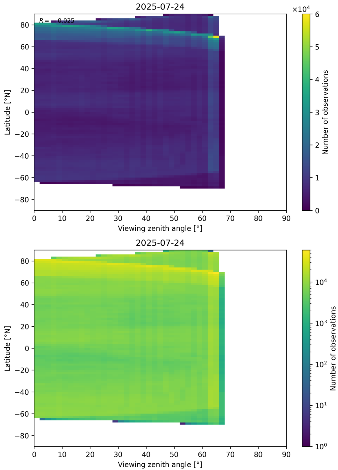
Figure 113: Scatter density plot of “Viewing zenith angle” against “Latitude” for 2025-07-24 to 2025-07-25.
