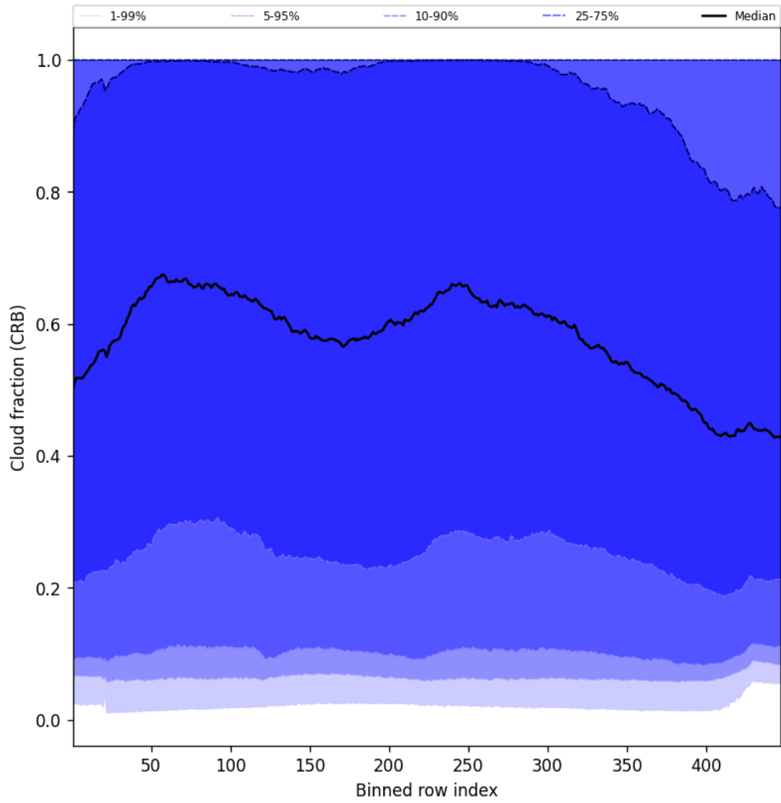
Figure 58: Along track statistics of “Cloud fraction (CRB)” for 2025-07-25 to 2025-07-27
