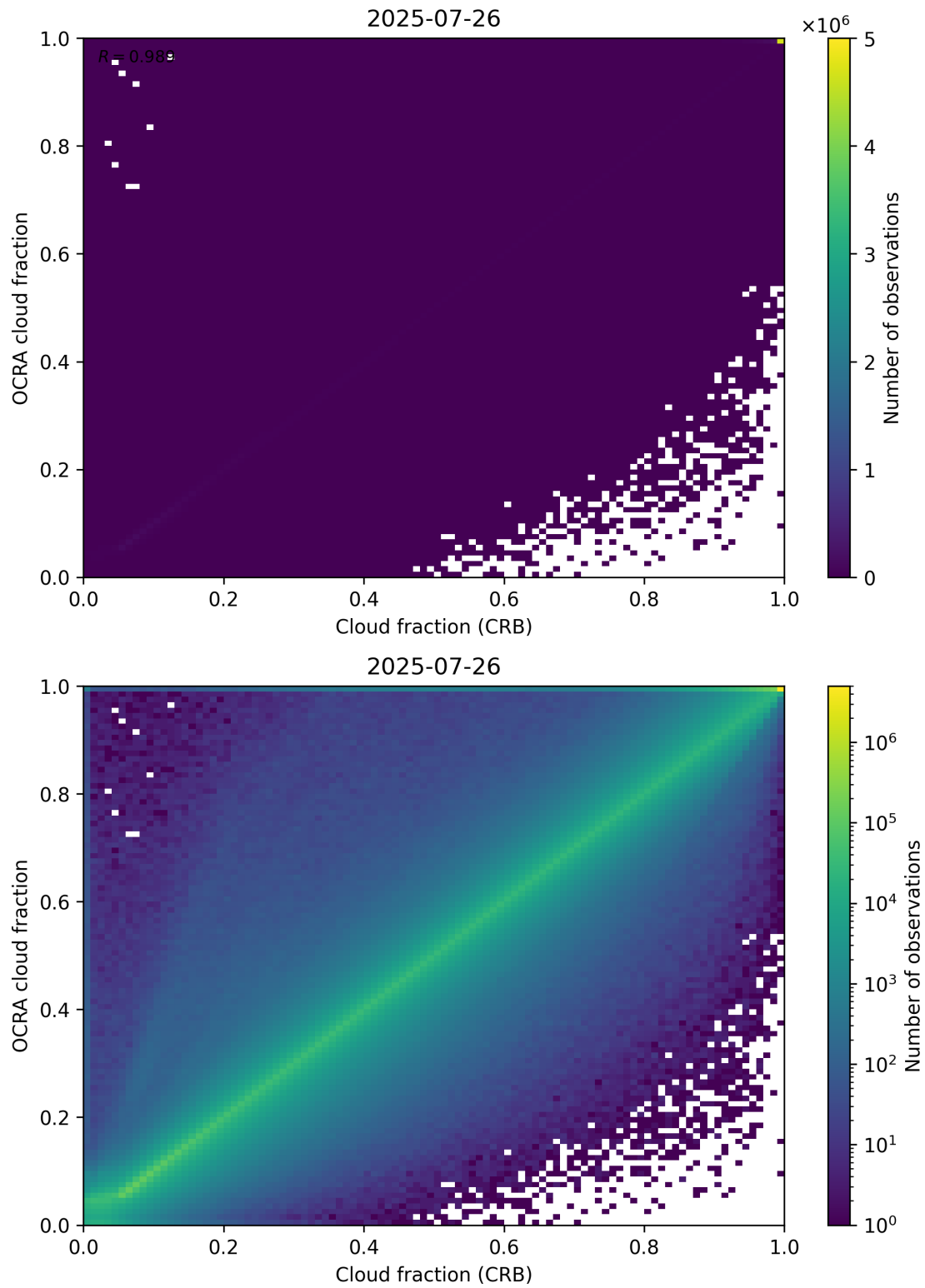
Figure 78: Scatter density plot of “Cloud fraction (CRB)” against “OCRA cloud fraction” for 2025-07-25 to 2025-07-27.
