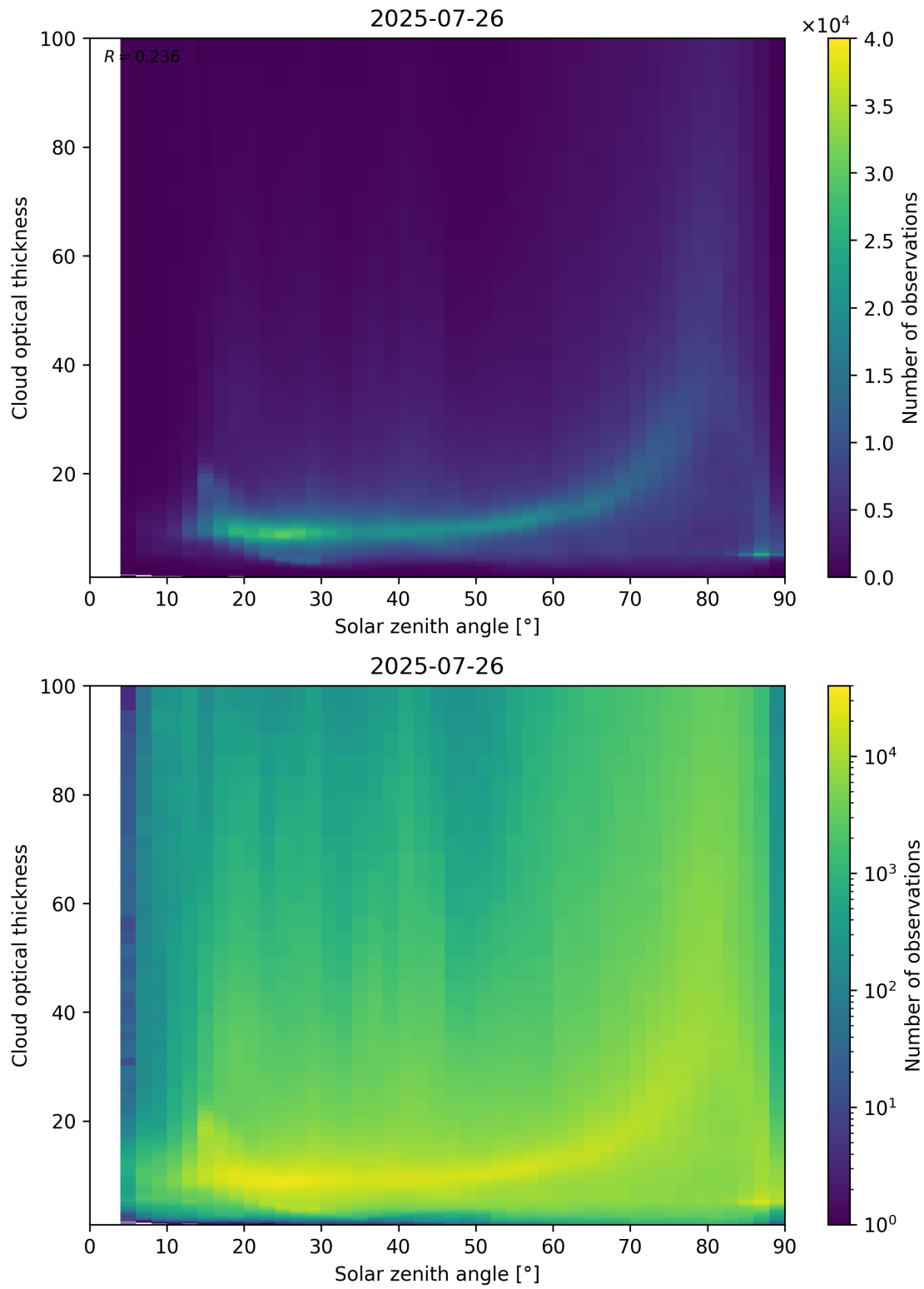
Figure 103: Scatter density plot of “Solar zenith angle” against “Cloud optical thickness” for 2025-07-25 to 2025-07-27.
