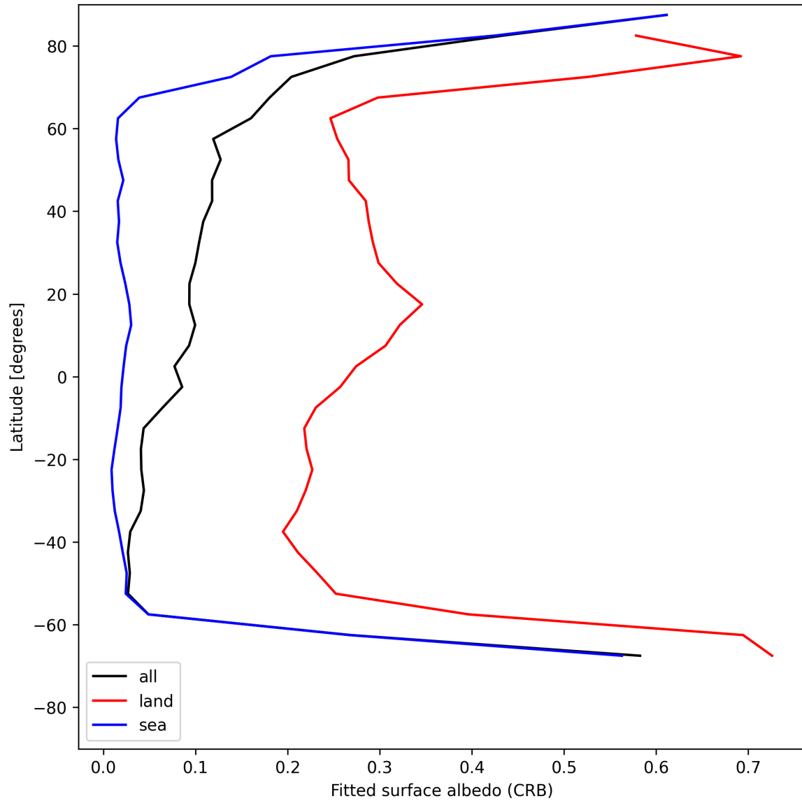
Figure 30: Zonal average of “Fitted surface albedo (CRB)” for 2025-07-25 to 2025-07-27.
