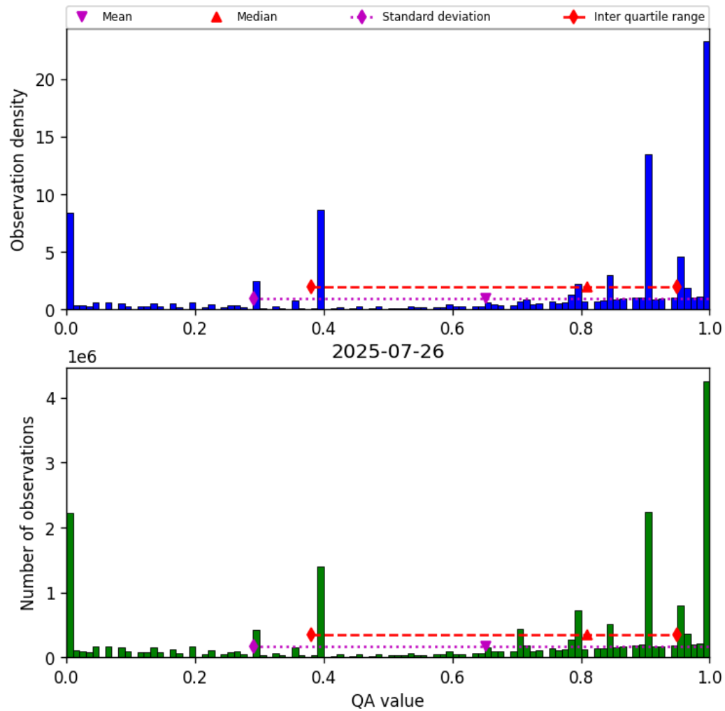
Figure 38: Histogram of “QA value” for 2025-07-25 to 2025-07-27
