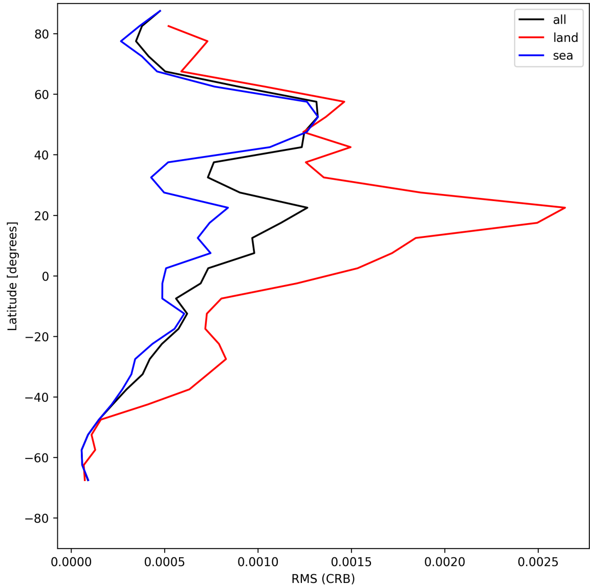
Figure 32: Zonal average of “RMS (CRB)” for 2025-07-25 to 2025-07-27.
