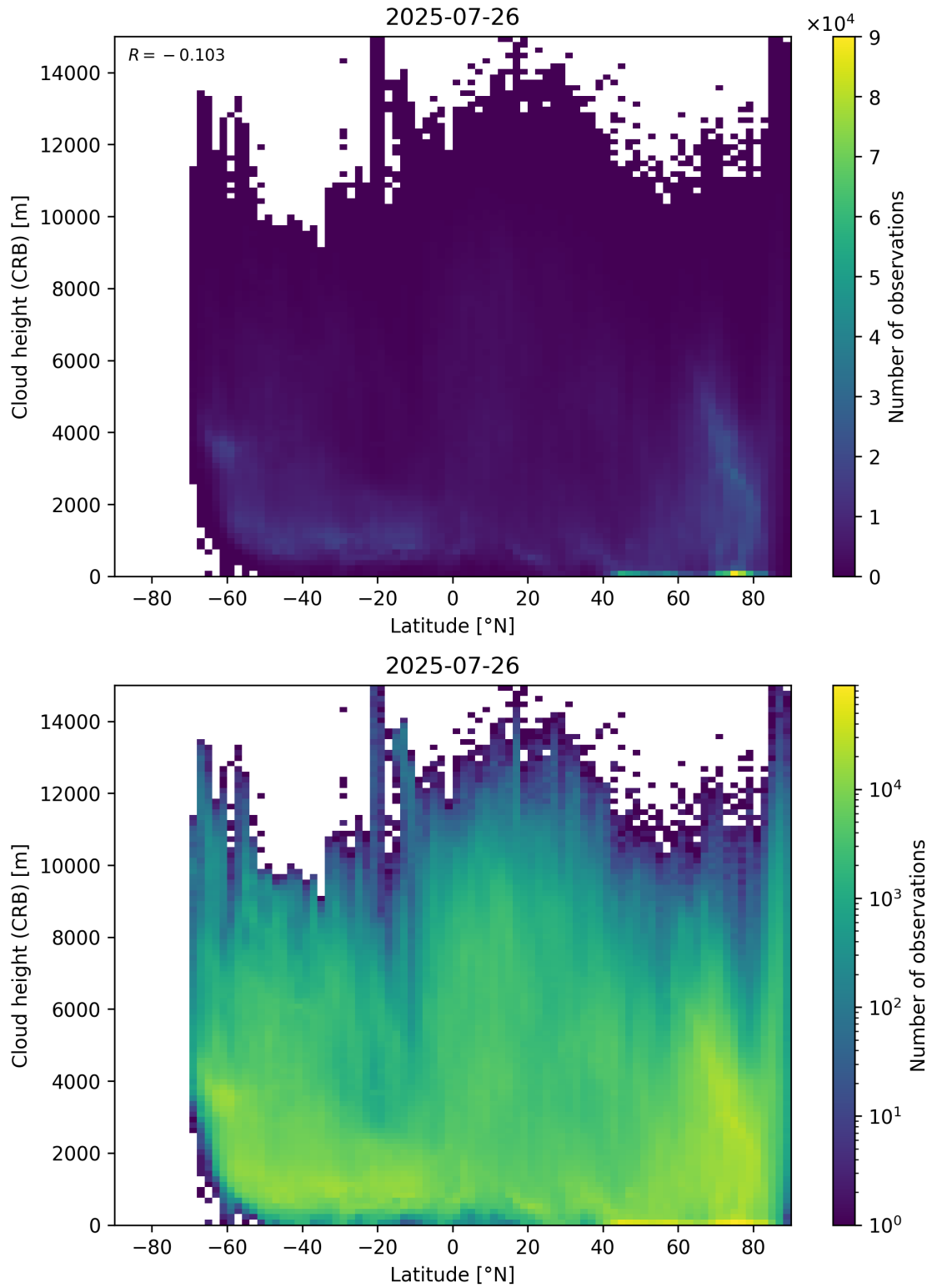
Figure 95: Scatter density plot of “Latitude” against “Cloud height (CRB)” for 2025-07-25 to 2025-07-27.
