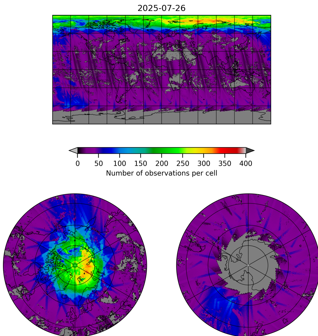
Figure 21: Map of the number of observations for 2025-07-25 to 2025-07-27
