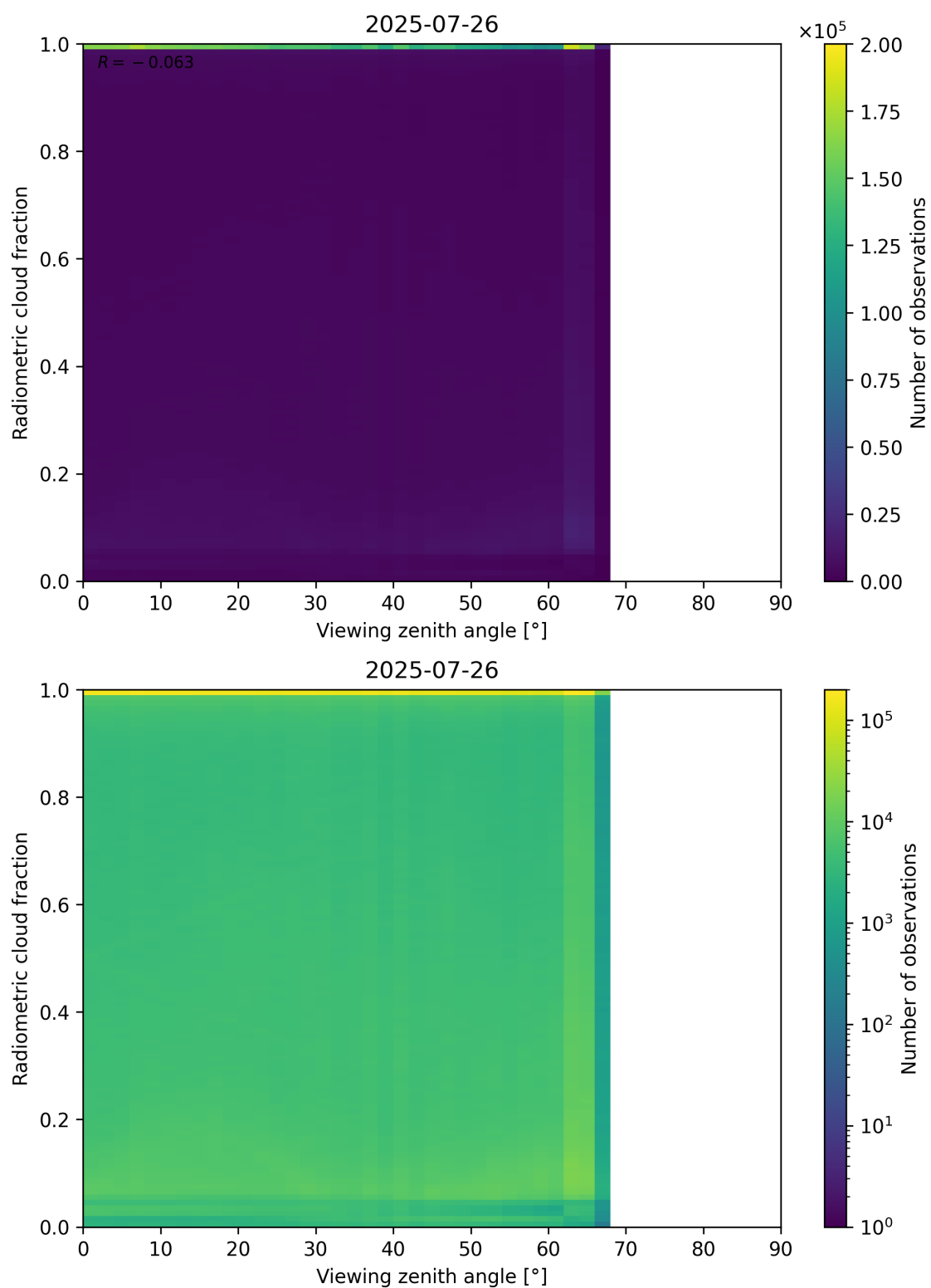
Figure 107: Scatter density plot of “Viewing zenith angle” against “Radiometric cloud fraction” for 2025-07-25 to 2025-07-27.
