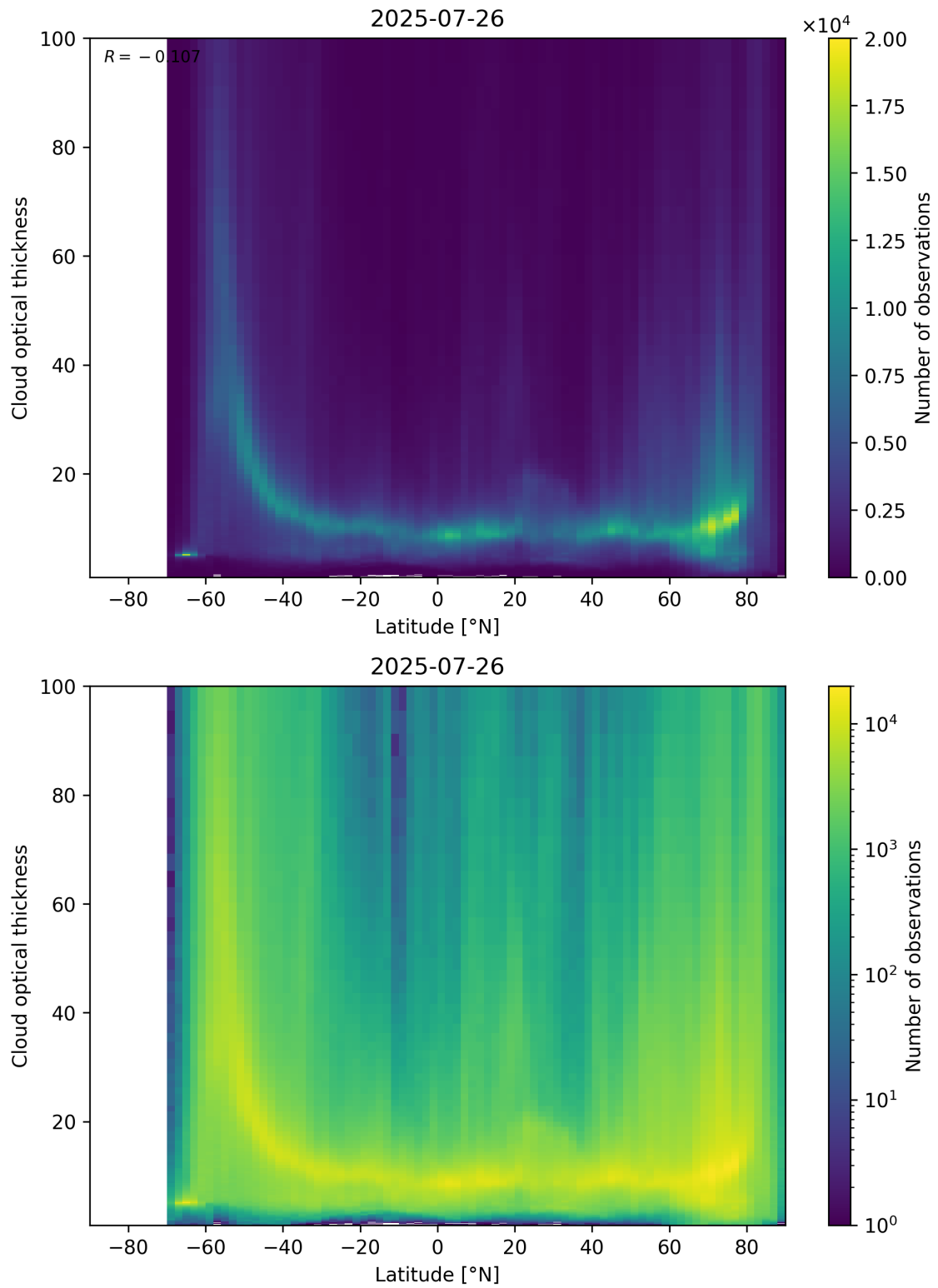
Figure 96: Scatter density plot of “Latitude” against “Cloud optical thickness” for 2025-07-25 to 2025-07-27.
