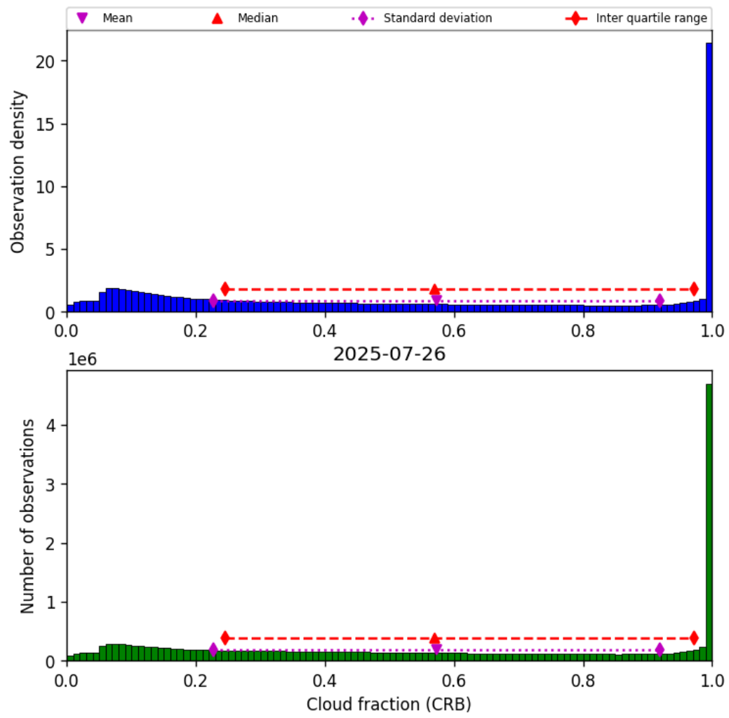
Figure 42: Histogram of “Cloud fraction (CRB)” for 2025-07-25 to 2025-07-27
