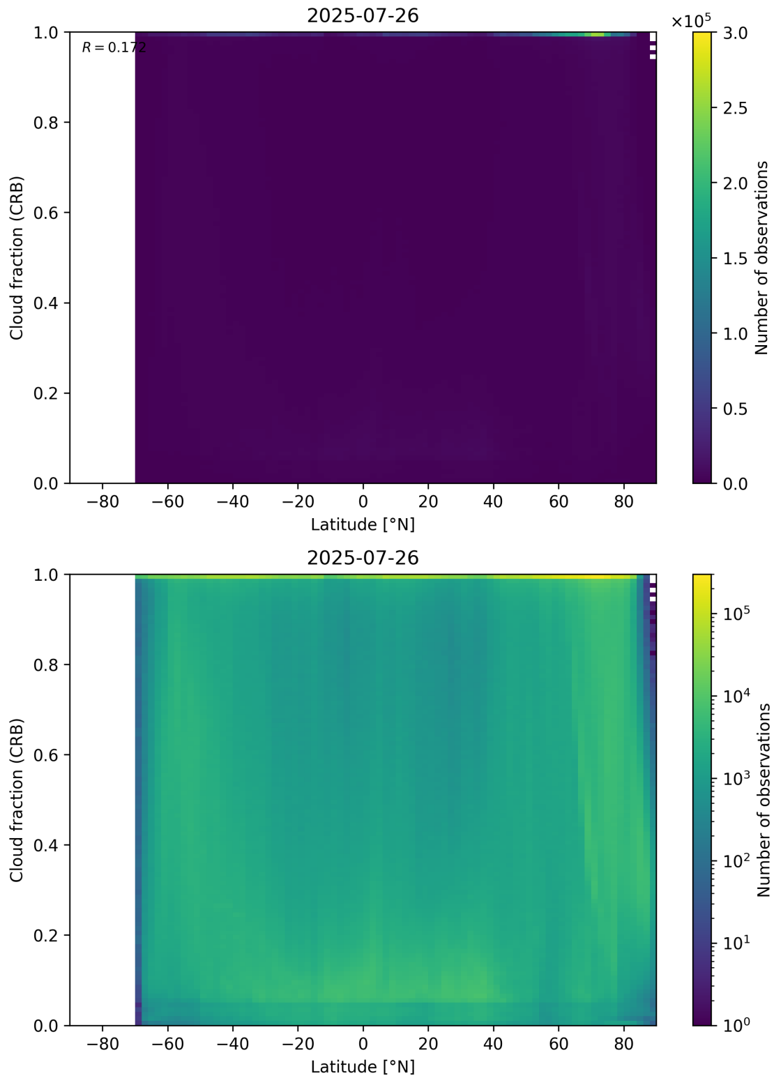
Figure 94: Scatter density plot of “Latitude” against “Cloud fraction (CRB)” for 2025-07-25 to 2025-07-27.
