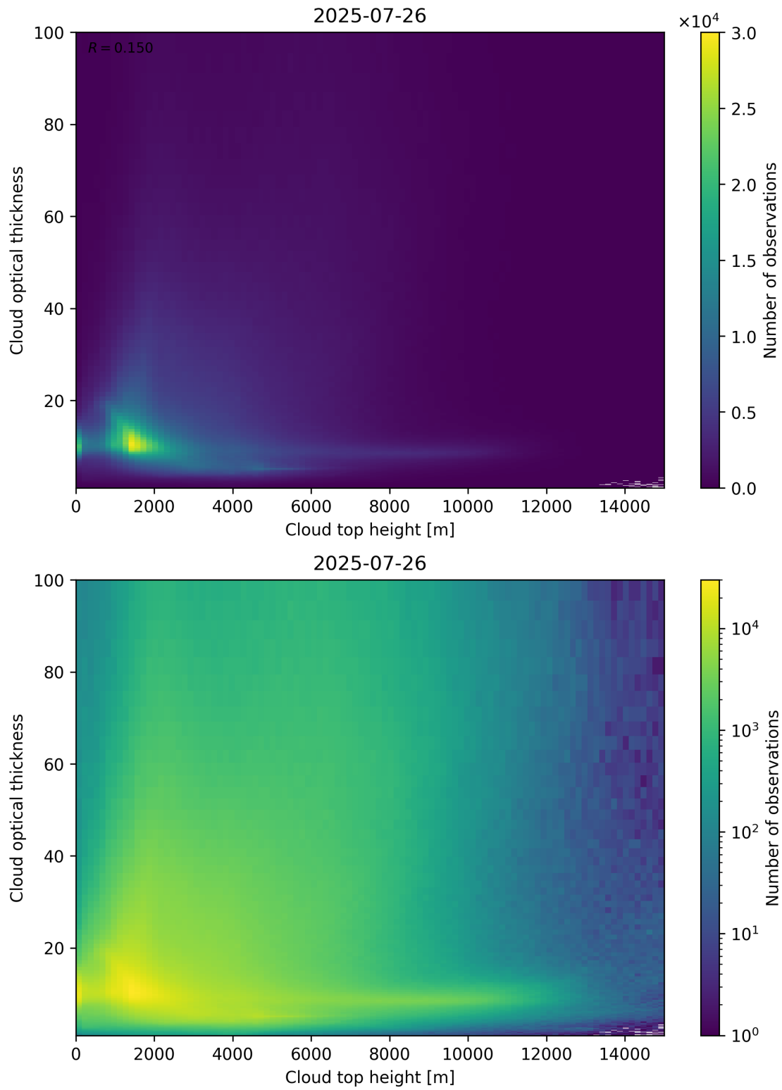
Figure 90: Scatter density plot of “Cloud top height” against “Cloud optical thickness” for 2025-07-25 to 2025-07-27.
