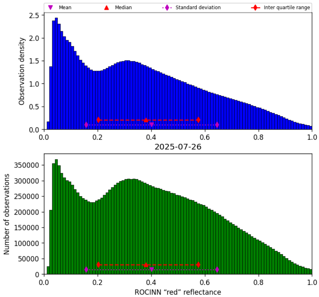
Figure 53: Histogram of “ROCINN “red” reflectance” for 2025-07-25 to 2025-07-27
