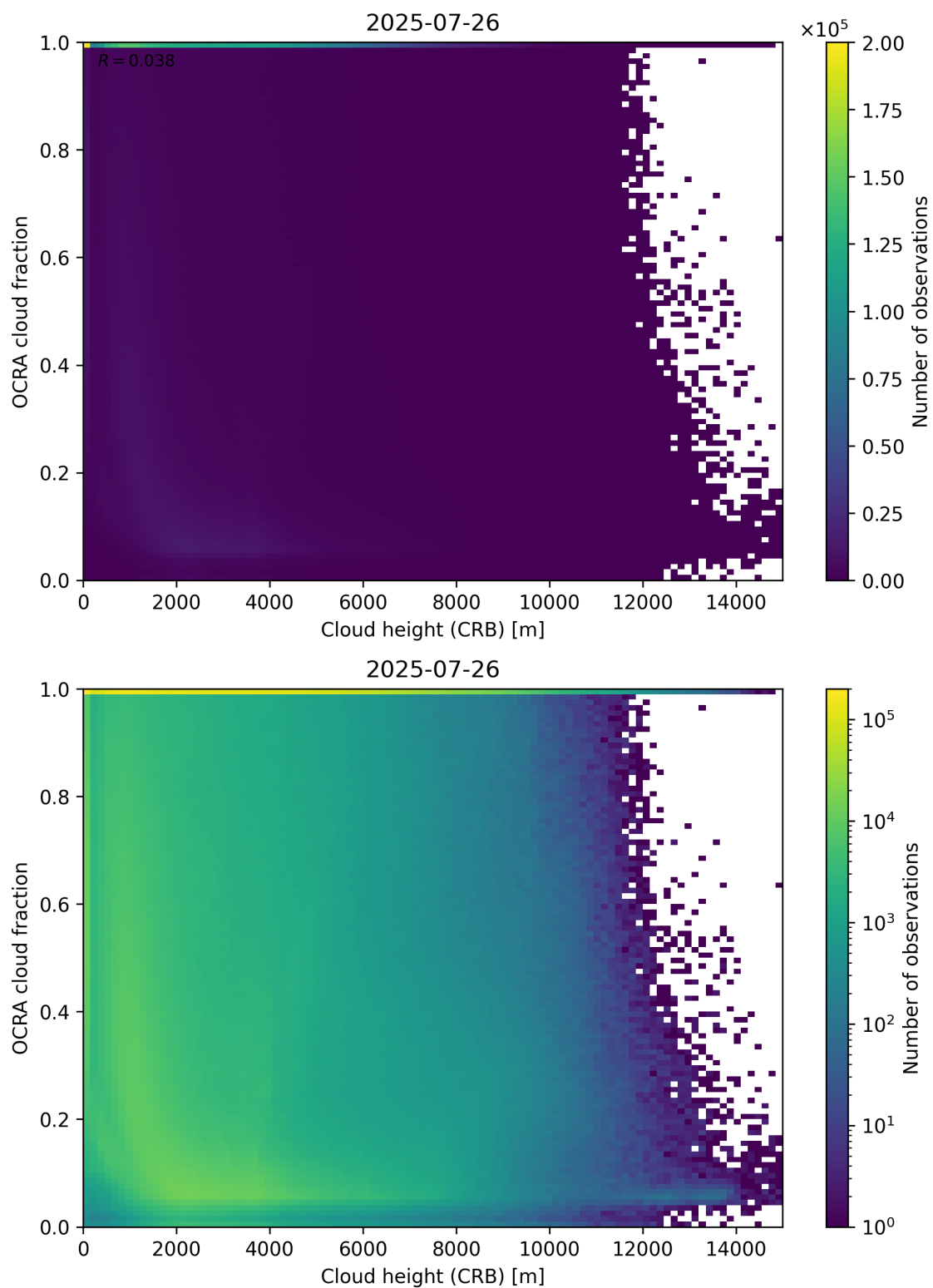
Figure 81: Scatter density plot of “Cloud height (CRB)” against “OCRA cloud fraction” for 2025-07-25 to 2025-07-27.
