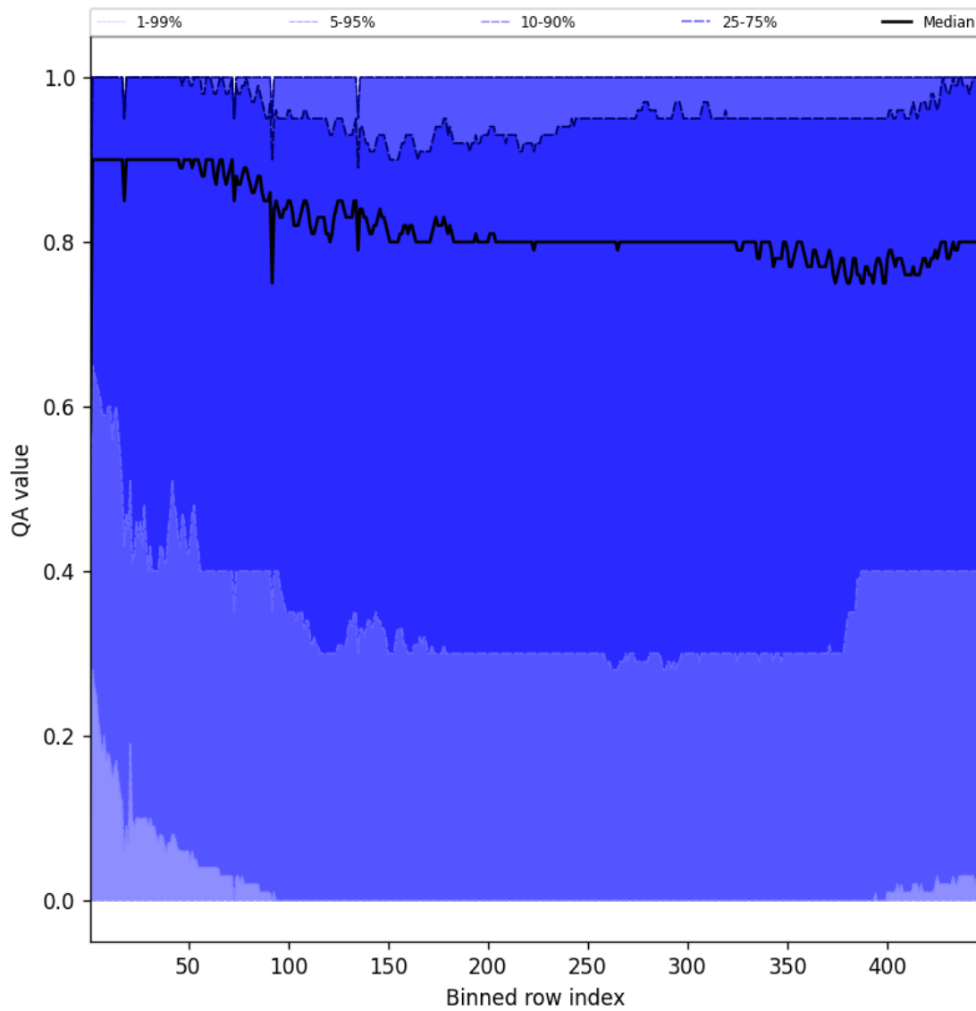
Figure 54: Along track statistics of “QA value” for 2025-07-25 to 2025-07-27
