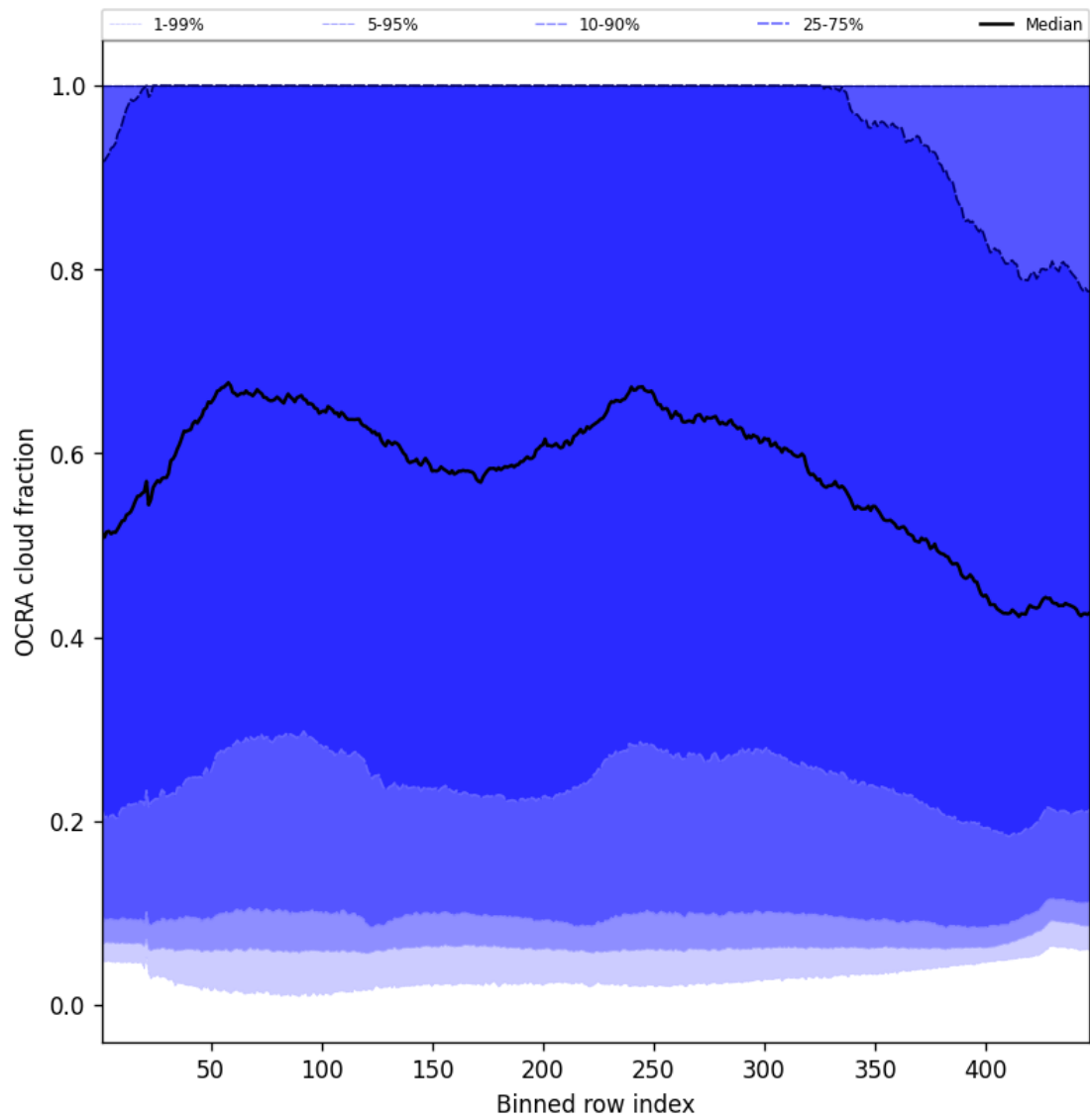
Figure 66: Along track statistics of “OCRA cloud fraction” for 2025-07-25 to 2025-07-27
