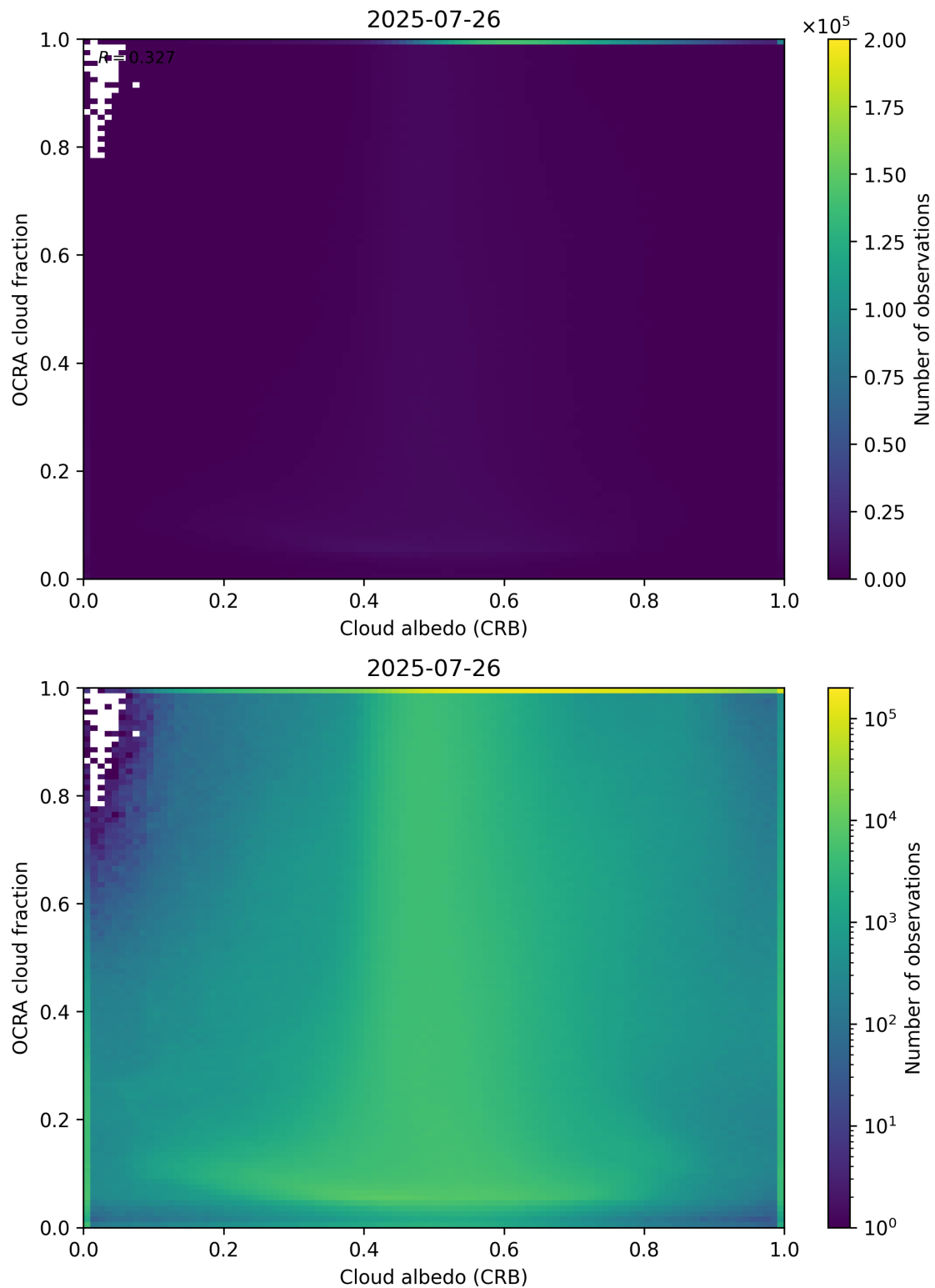
Figure 70: Scatter density plot of “Cloud albedo (CRB)” against “OCRA cloud fraction” for 2025-07-25 to 2025-07-27.
