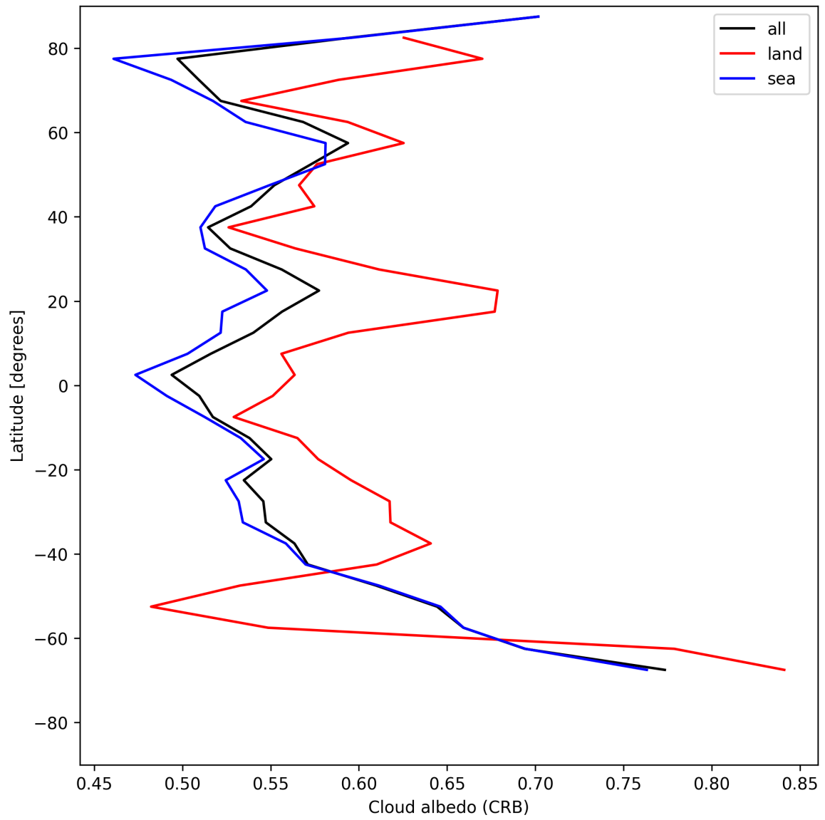
Figure 28: Zonal average of “Cloud albedo (CRB)” for 2025-07-25 to 2025-07-27.
