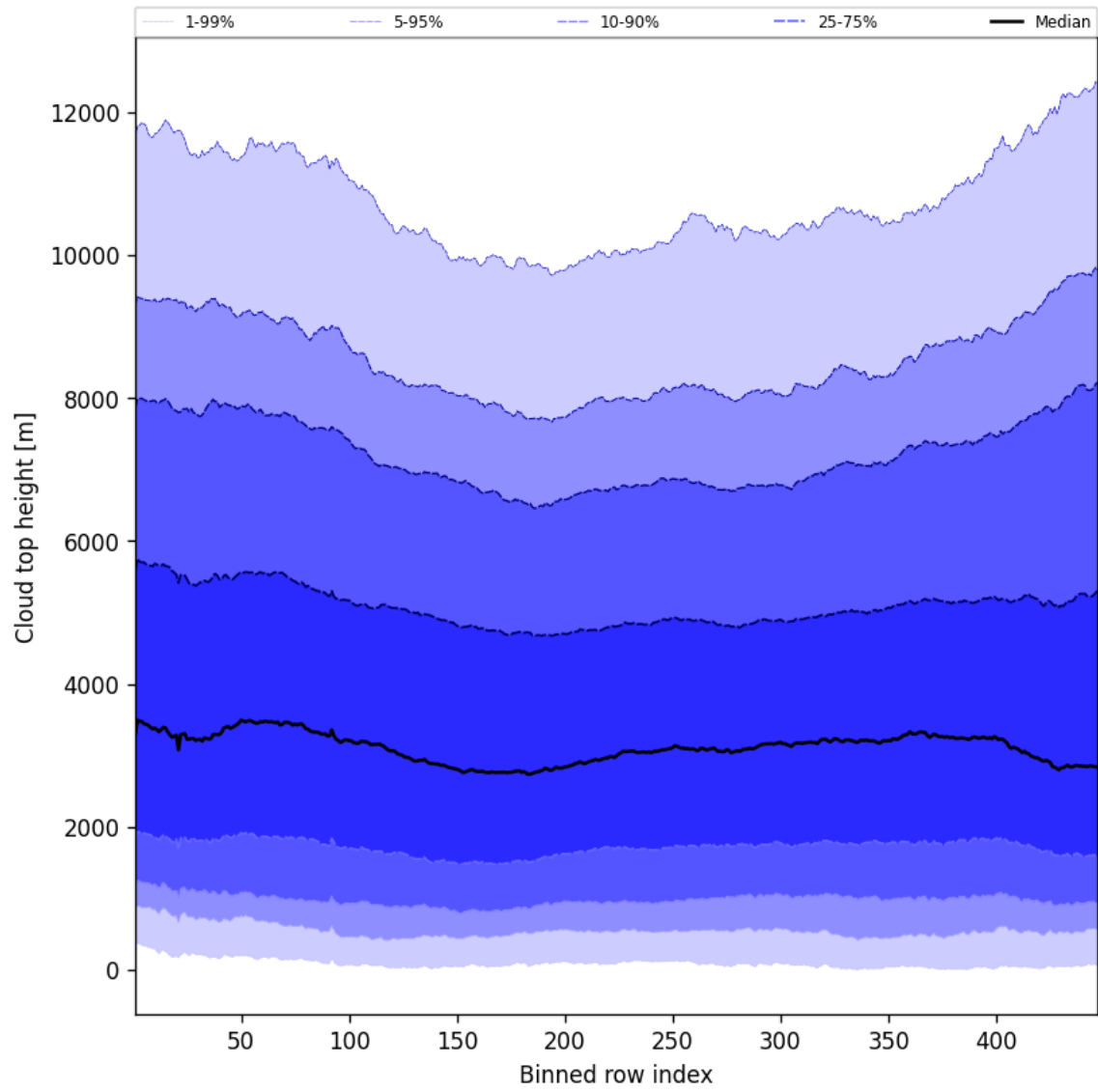
Figure 56: Along track statistics of “Cloud top height” for 2025-07-25 to 2025-07-27
