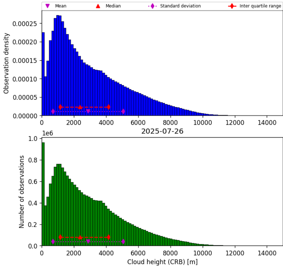
Figure 43: Histogram of “Cloud height (CRB)” for 2025-07-25 to 2025-07-27
