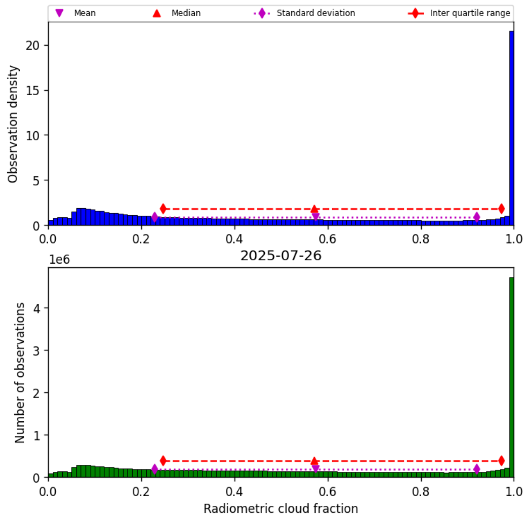
Figure 39: Histogram of “Radiometric cloud fraction” for 2025-07-25 to 2025-07-27
