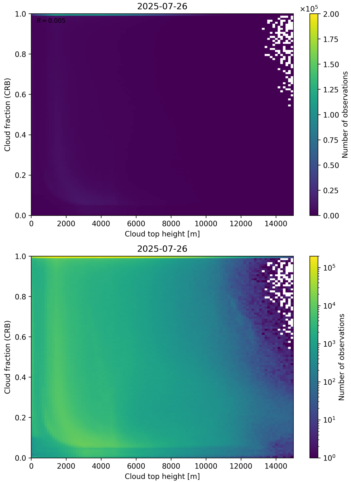
Figure 88: Scatter density plot of “Cloud top height” against “Cloud fraction (CRB)” for 2025-07-25 to 2025-07-27.
