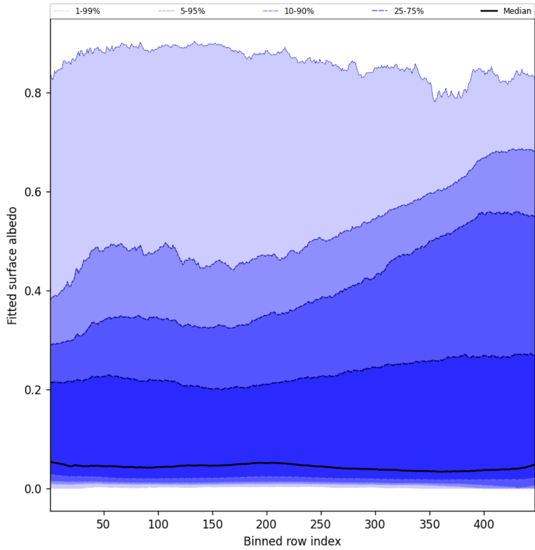
Figure 61: Along track statistics of “Fitted surface albedo” for 2025-07-25 to 2025-07-27
