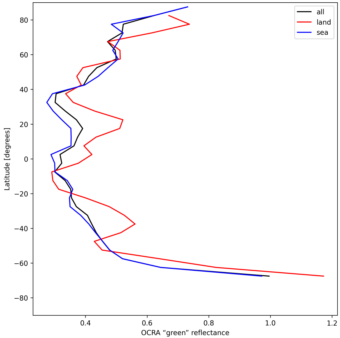
Figure 36: Zonal average of “OCRA “green” reflectance” for 2025-07-25 to 2025-07-27.
