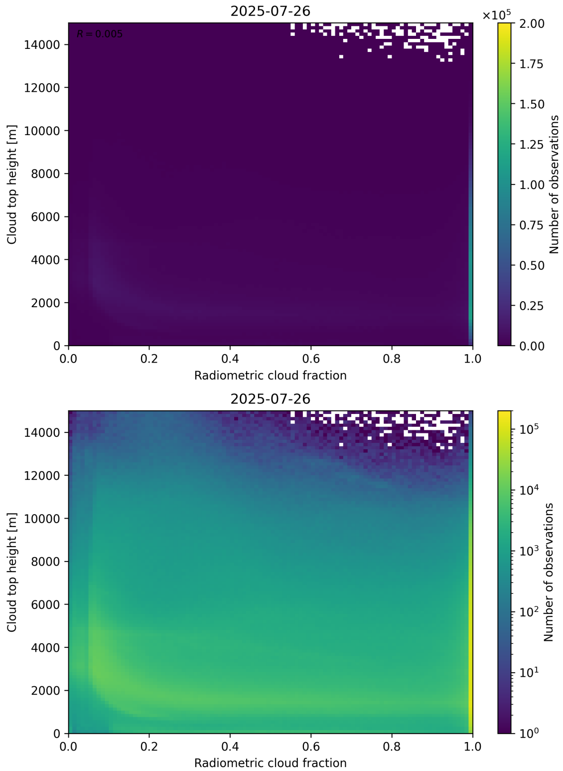
Figure 76: Scatter density plot of “Radiometric cloud fraction” against “Cloud top height” for 2025-07-25 to 2025-07-27.
