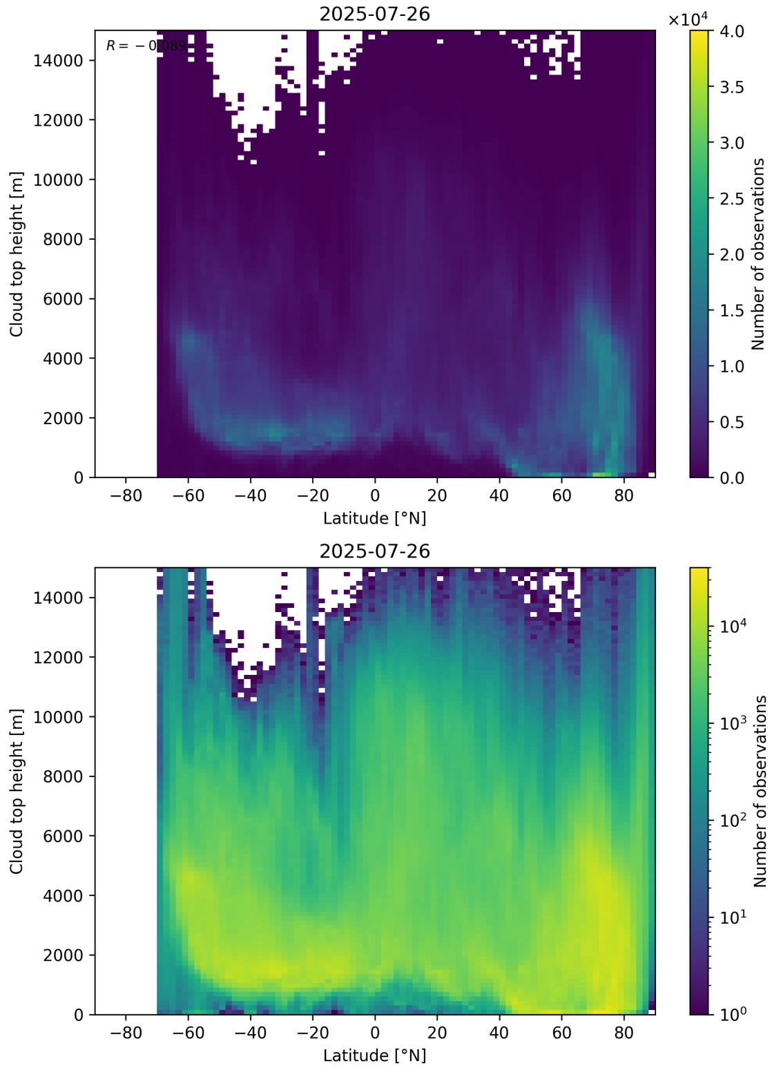
Figure 97: Scatter density plot of “Latitude” against “Cloud top height” for 2025-07-25 to 2025-07-27.
