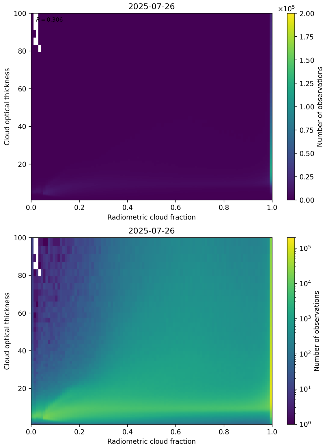
Figure 75: Scatter density plot of “Radiometric cloud fraction” against “Cloud optical thickness” for 2025-07-25 to 2025-07-27.
