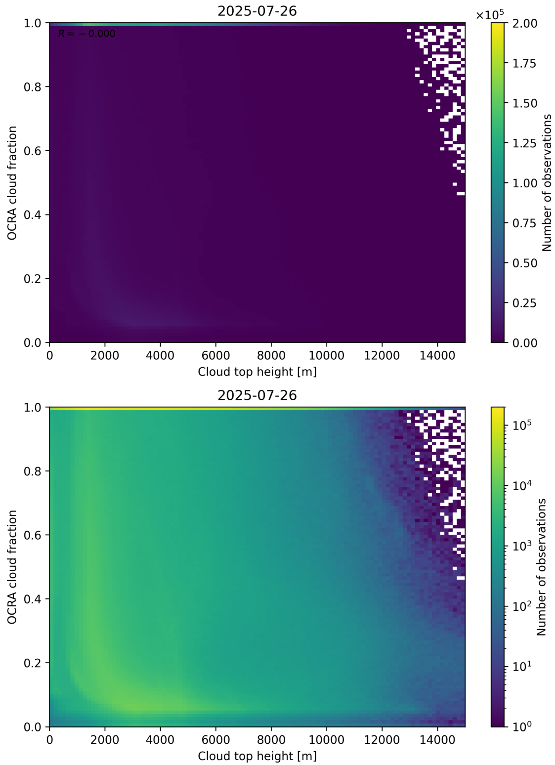
Figure 87: Scatter density plot of “Cloud top height” against “OCRA cloud fraction” for 2025-07-25 to 2025-07-27.
