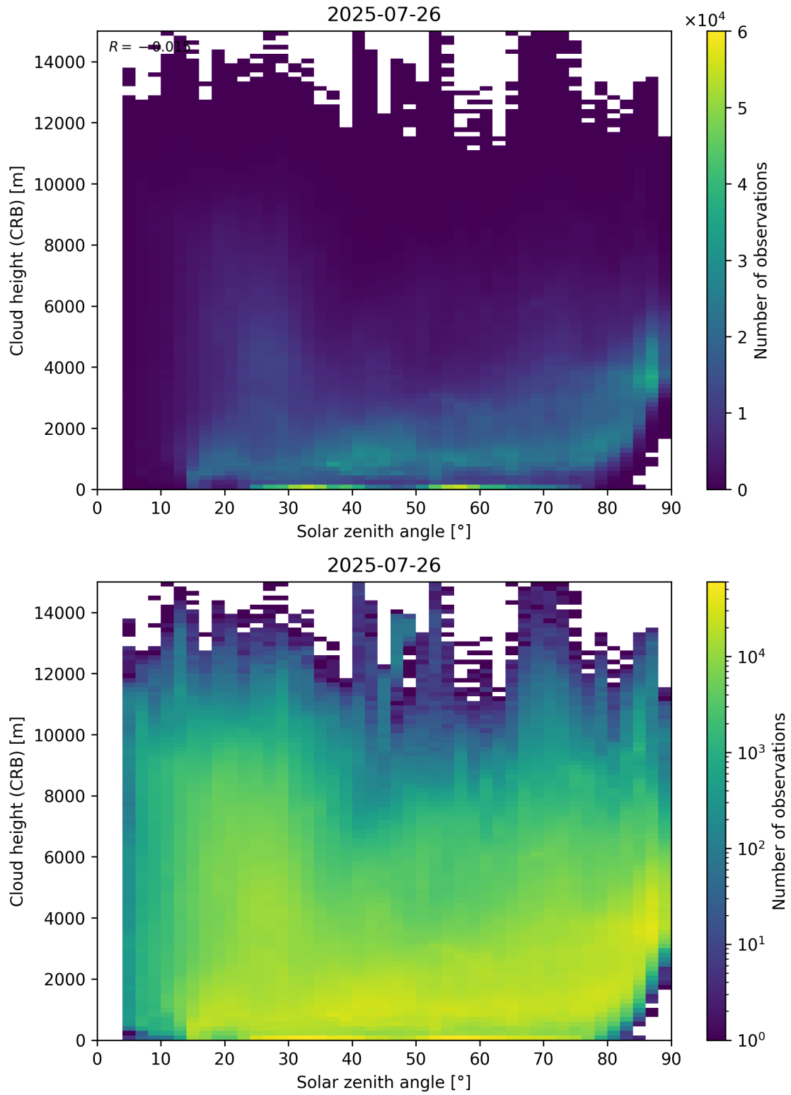
Figure 102: Scatter density plot of “Solar zenith angle” against “Cloud height (CRB)” for 2025-07-25 to 2025-07-27.
