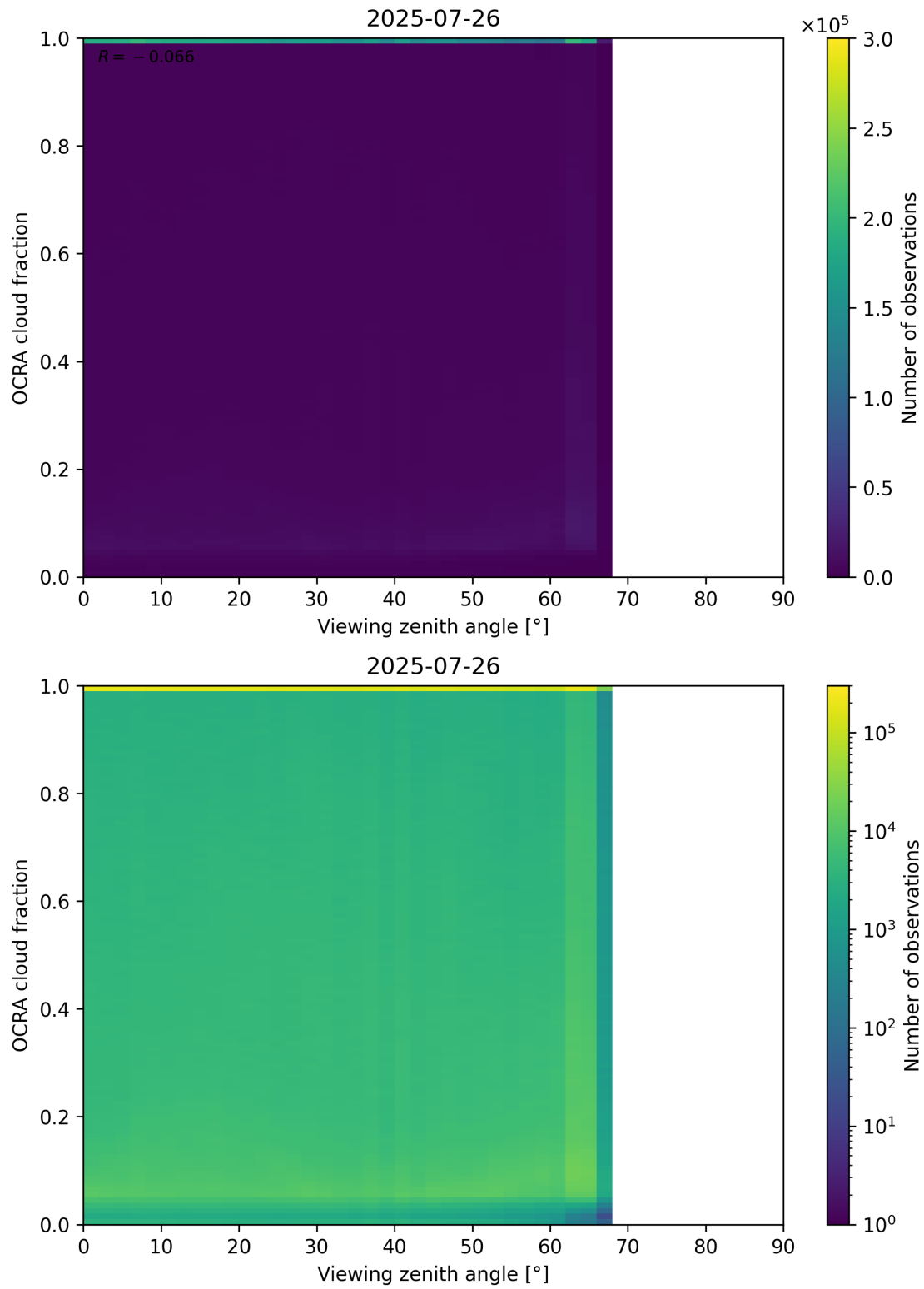
Figure 108: Scatter density plot of “Viewing zenith angle” against “OCRA cloud fraction” for 2025-07-25 to 2025-07-27.
