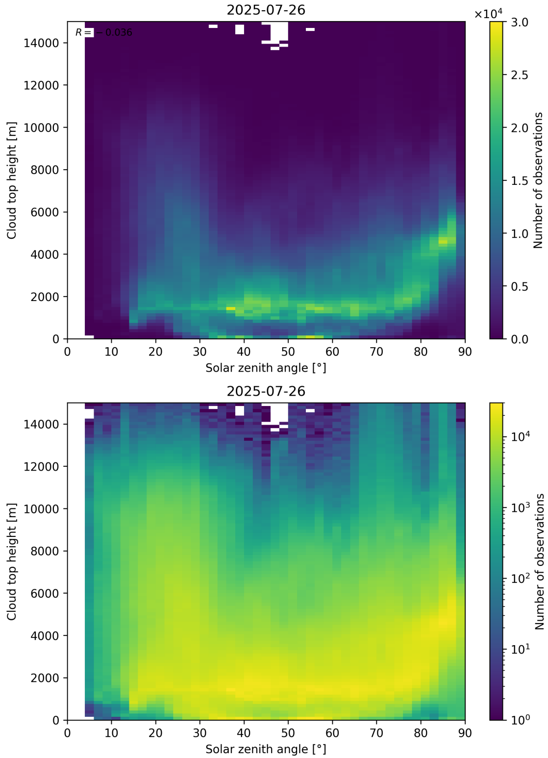
Figure 104: Scatter density plot of “Solar zenith angle” against “Cloud top height” for 2025-07-25 to 2025-07-27.
