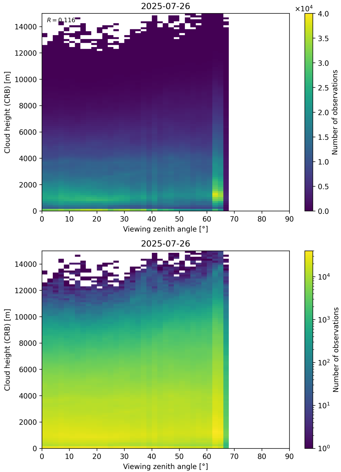
Figure 110: Scatter density plot of “Viewing zenith angle” against “Cloud height (CRB)” for 2025-07-25 to 2025-07-27.
