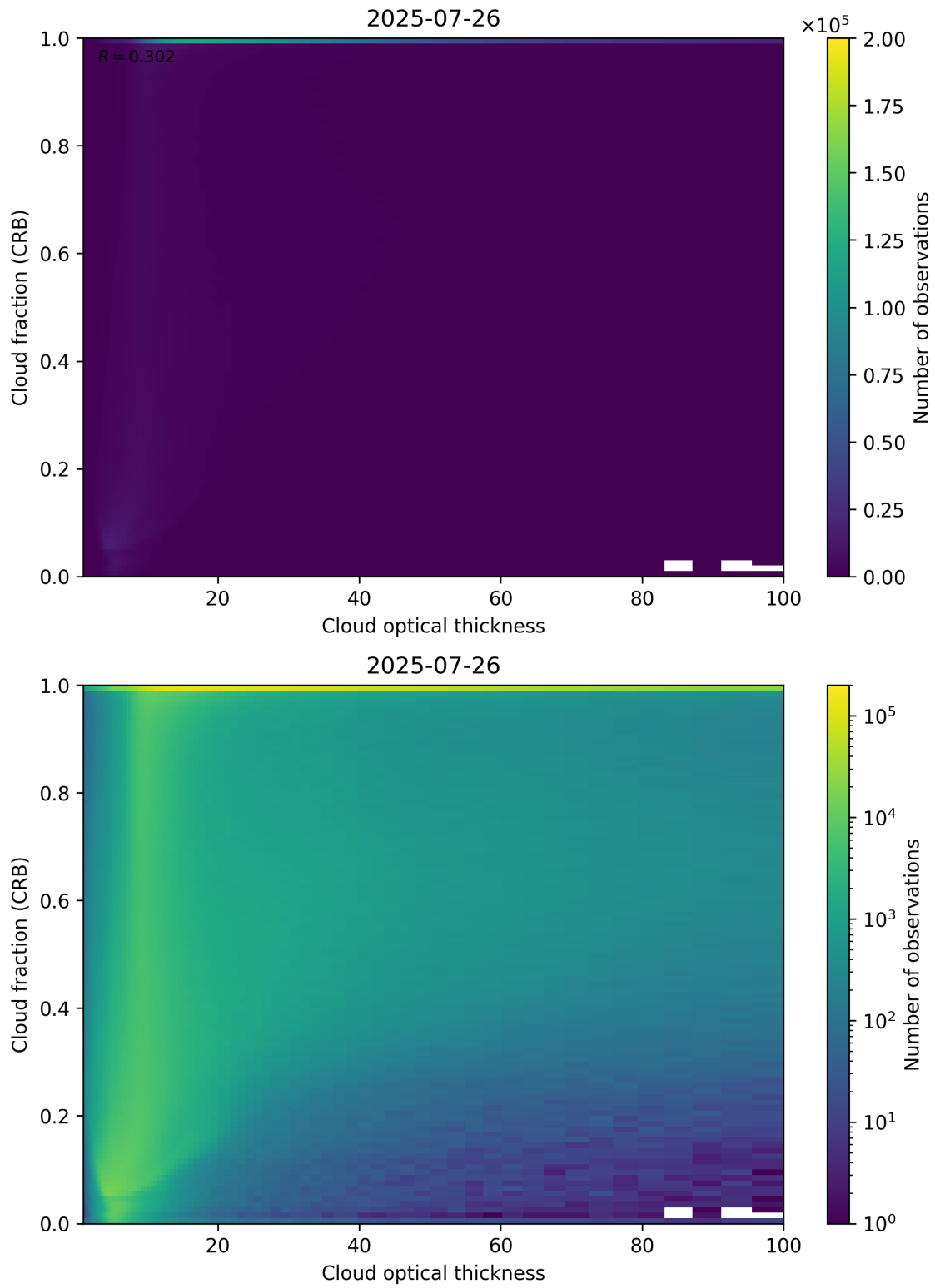
Figure 84: Scatter density plot of “Cloud optical thickness” against “Cloud fraction (CRB)” for 2025-07-25 to 2025-07-27.
