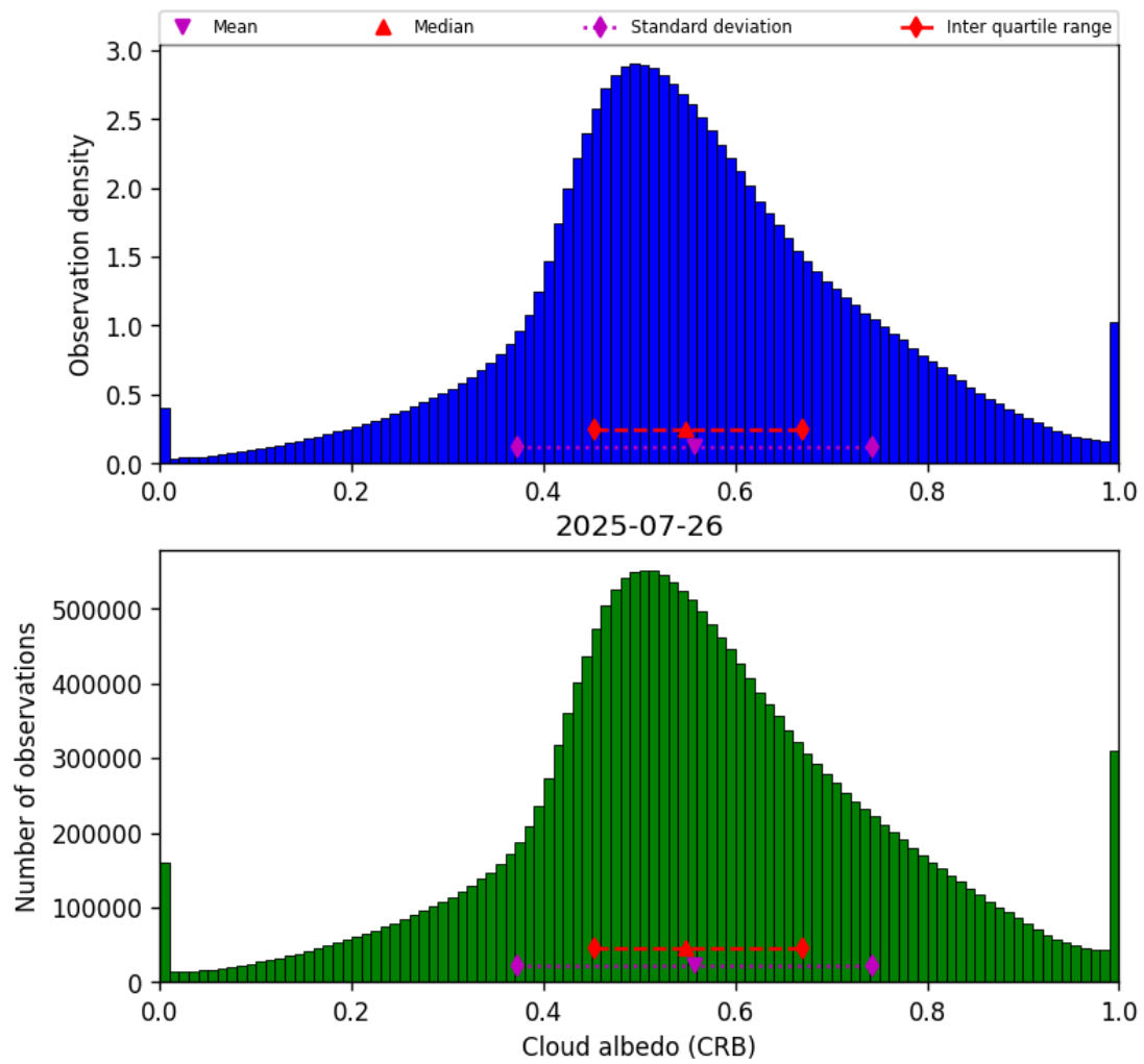
Figure 44: Histogram of “Cloud albedo (CRB)” for 2025-07-25 to 2025-07-27
