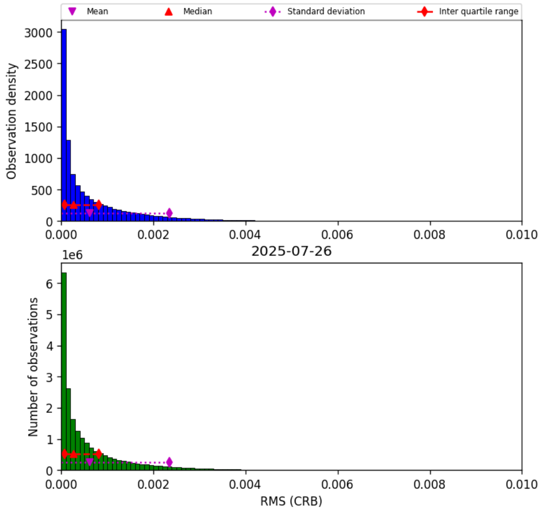
Figure 48: Histogram of “RMS (CRB)” for 2025-07-25 to 2025-07-27
