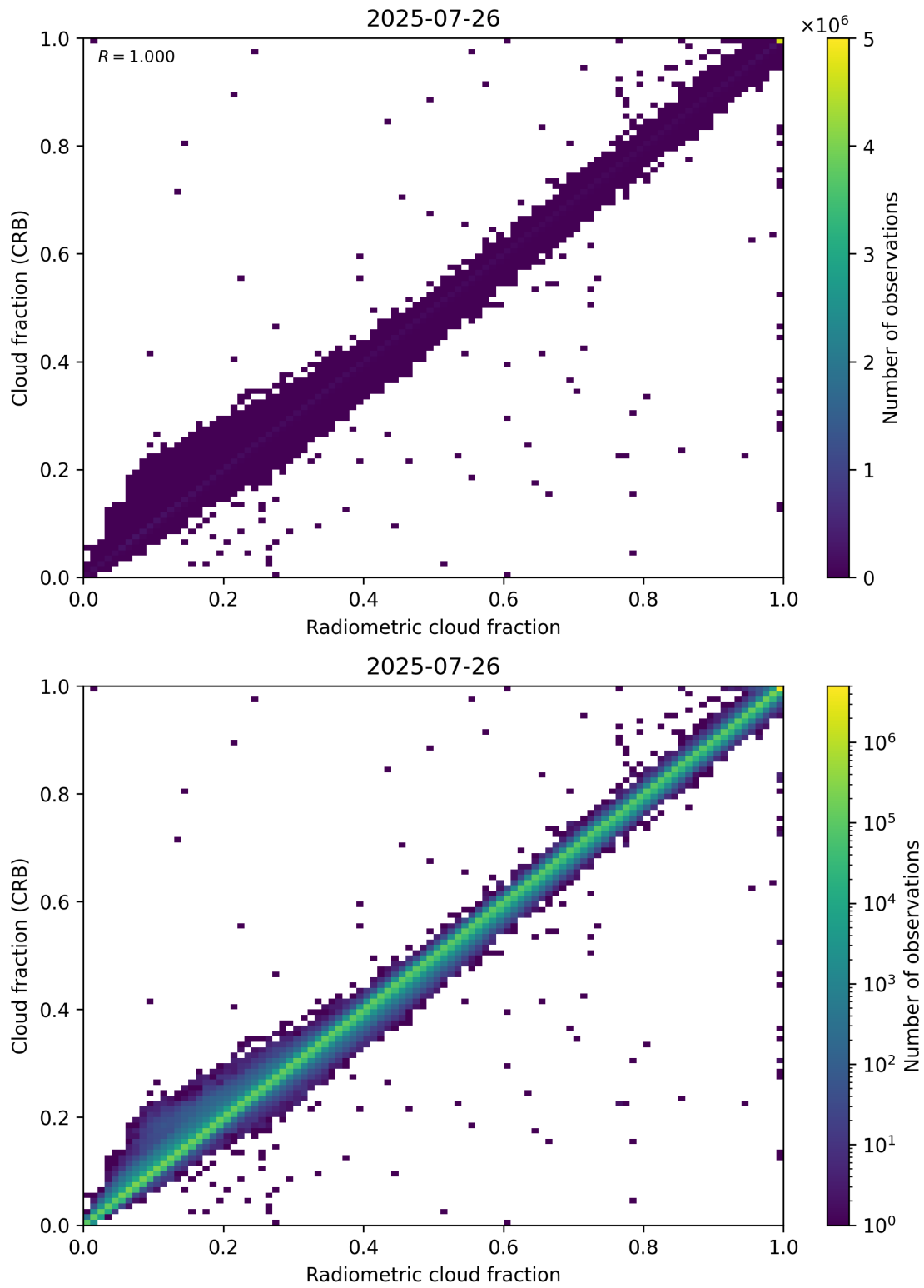
Figure 73: Scatter density plot of “Radiometric cloud fraction” against “Cloud fraction (CRB)” for 2025-07-25 to 2025-07-27.
