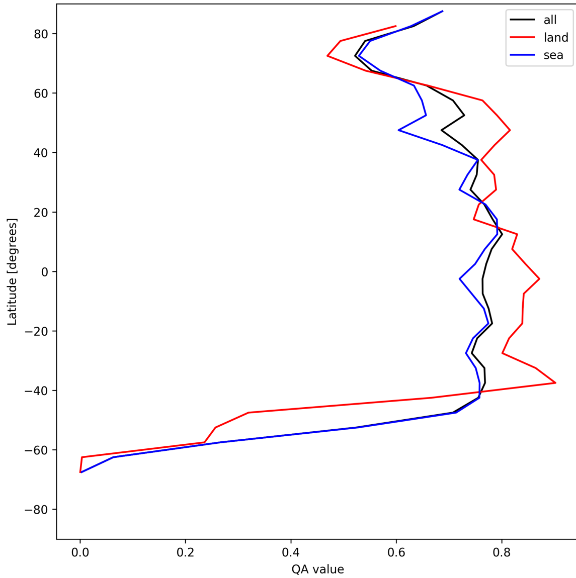
Figure 22: Zonal average of “QA value” for 2025-07-25 to 2025-07-27.
