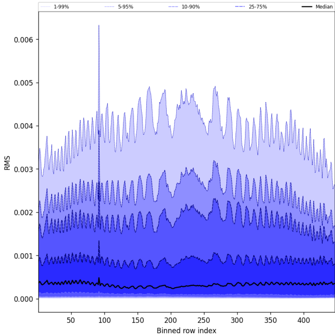
Figure 63: Along track statistics of “RMS” for 2025-07-25 to 2025-07-27
