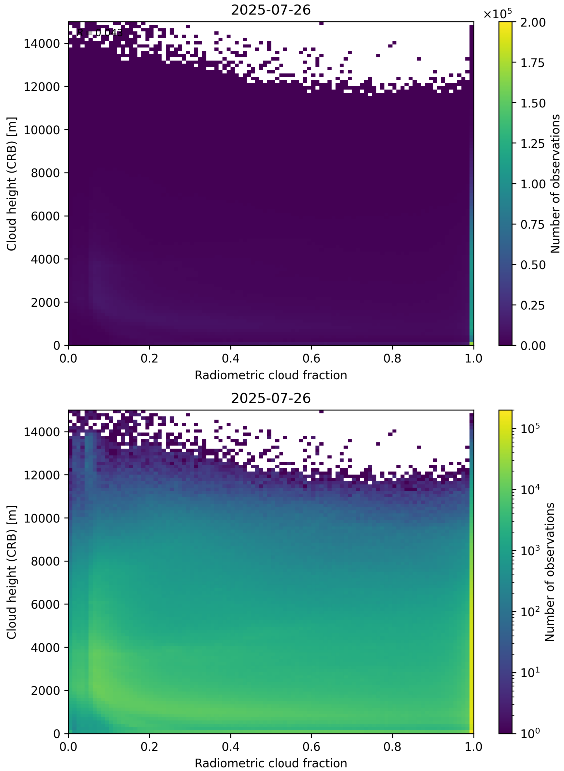
Figure 74: Scatter density plot of “Radiometric cloud fraction” against “Cloud height (CRB)” for 2025-07-25 to 2025-07-27.
