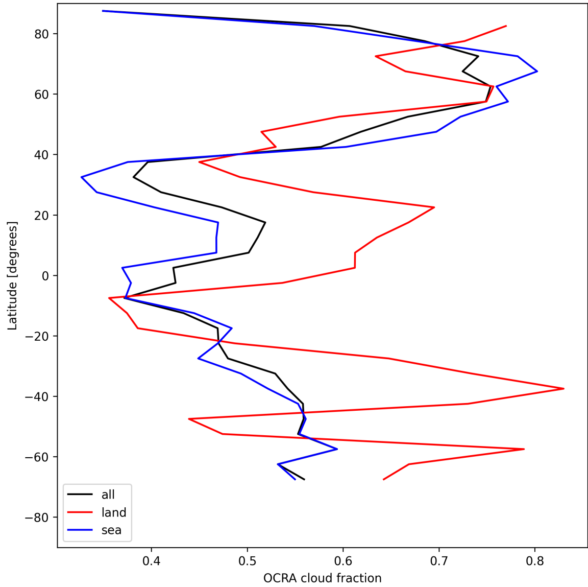
Figure 34: Zonal average of “OCRA cloud fraction” for 2025-07-25 to 2025-07-27.
