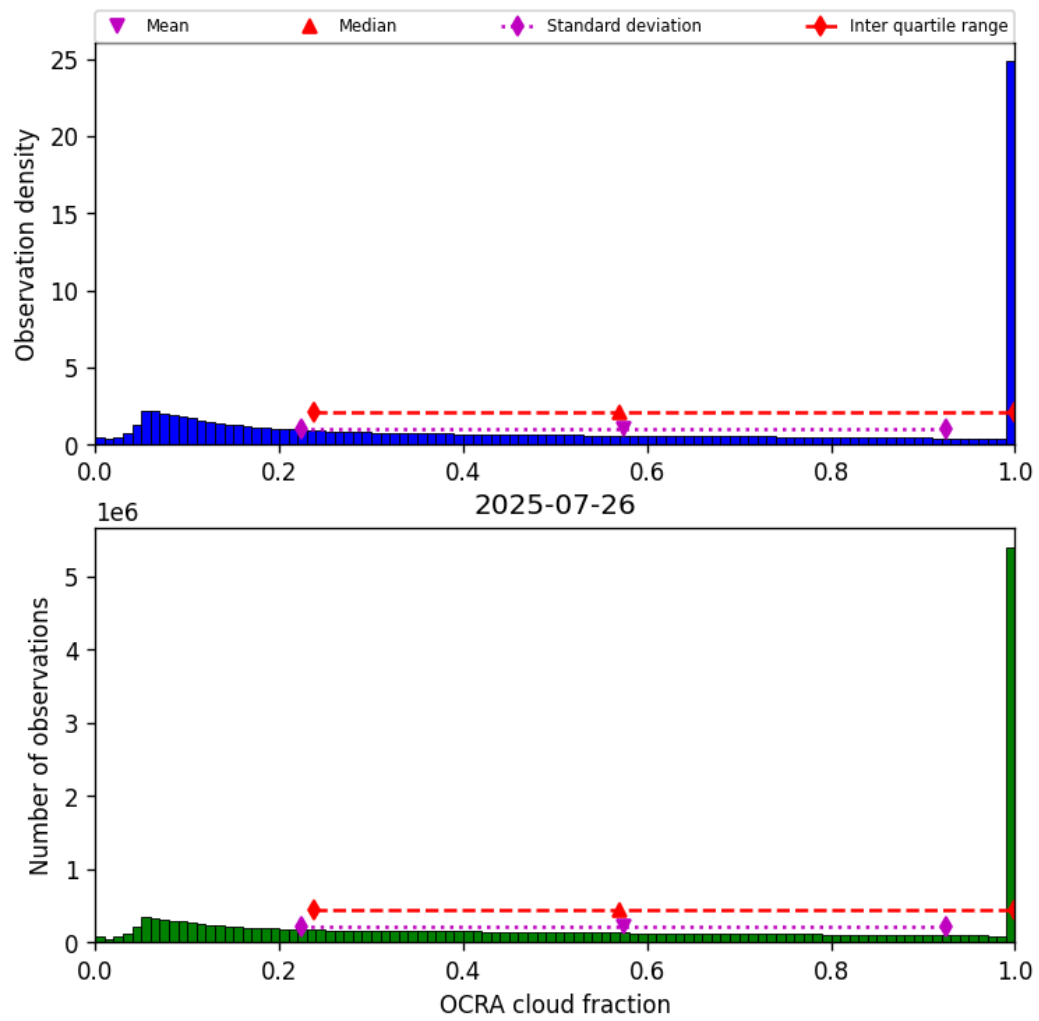
Figure 50: Histogram of “OCRA cloud fraction” for 2025-07-25 to 2025-07-27
