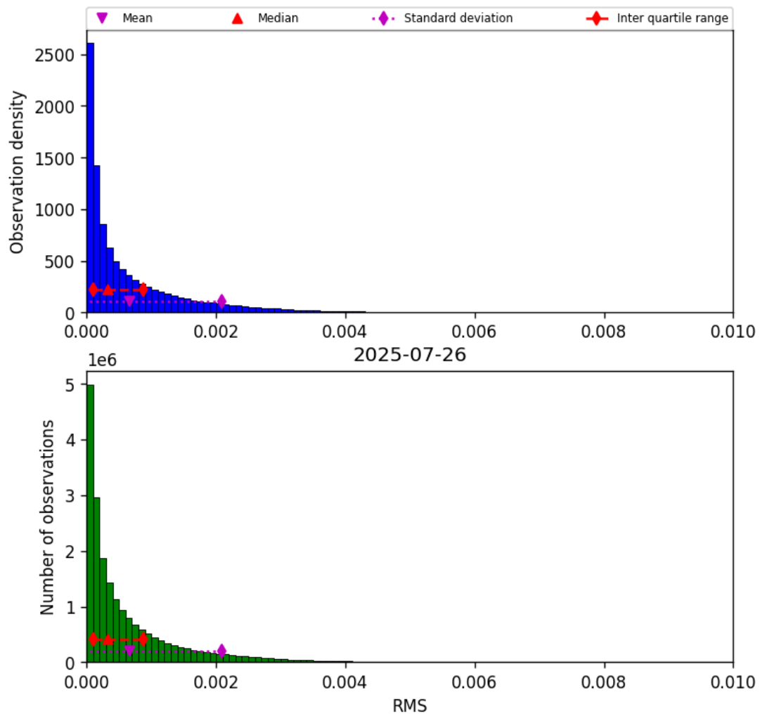
Figure 47: Histogram of “RMS” for 2025-07-25 to 2025-07-27
