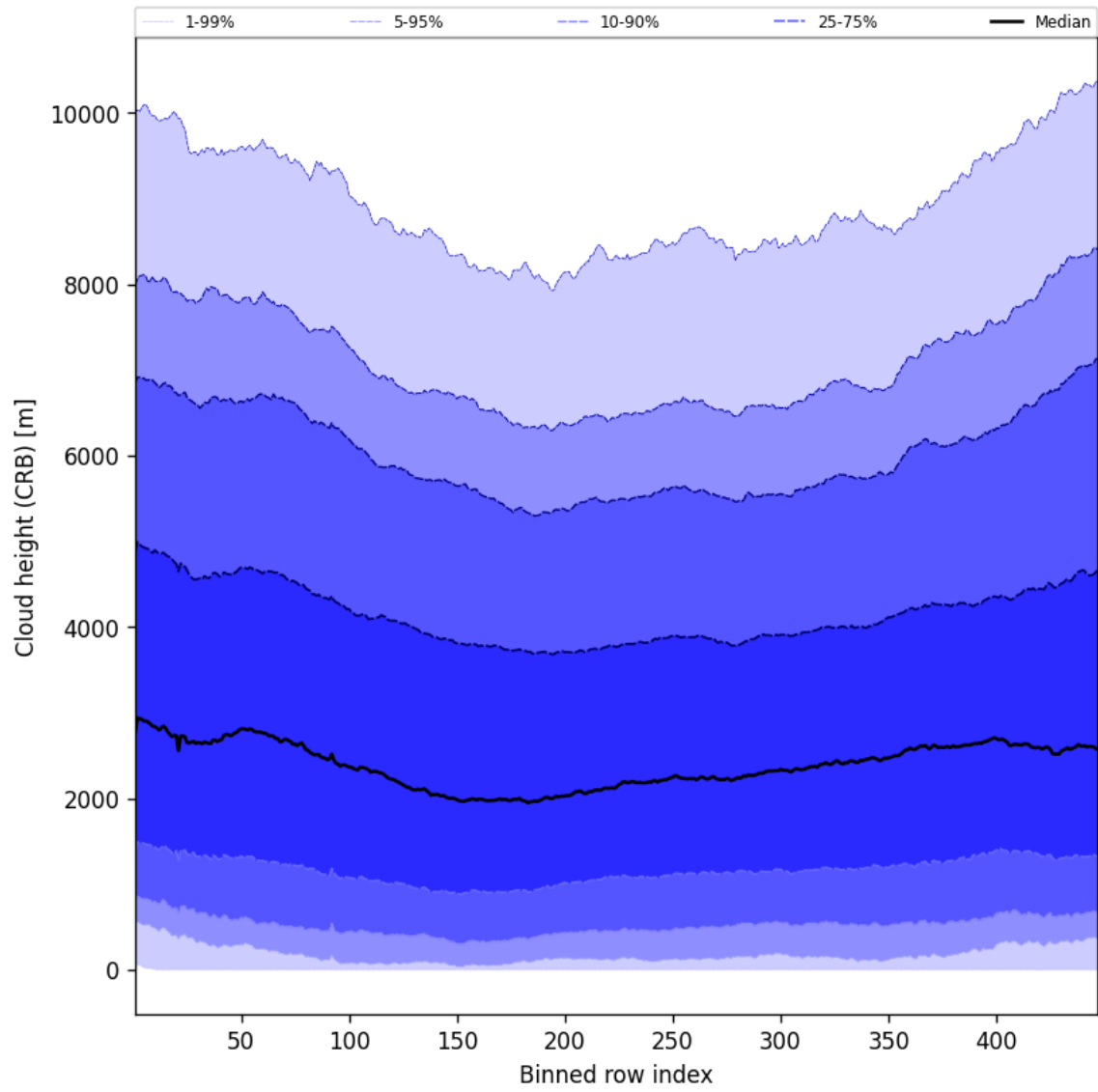
Figure 59: Along track statistics of “Cloud height (CRB)” for 2025-07-25 to 2025-07-27
