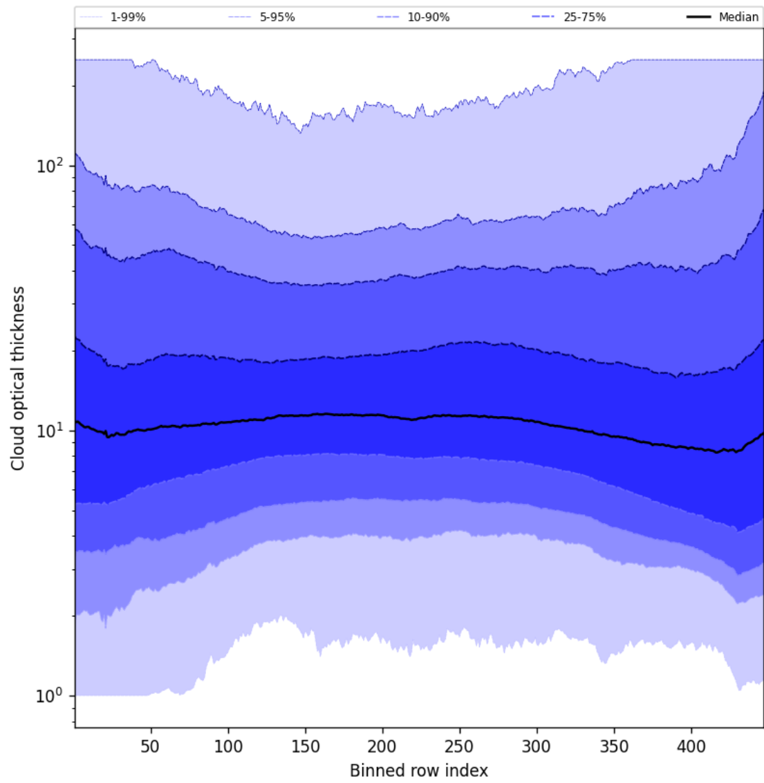
Figure 57: Along track statistics of “Cloud optical thickness” for 2025-07-25 to 2025-07-27
