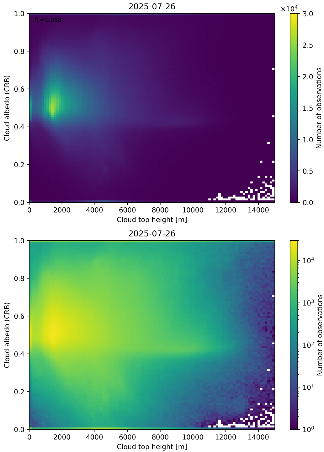
Figure 86: Scatter density plot of “Cloud top height” against “Cloud albedo (CRB)” for 2025-07-25 to 2025-07-27.
