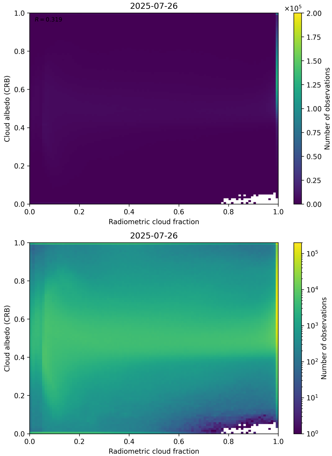
Figure 71: Scatter density plot of “Radiometric cloud fraction” against “Cloud albedo (CRB)” for 2025-07-25 to 2025-07-27.
