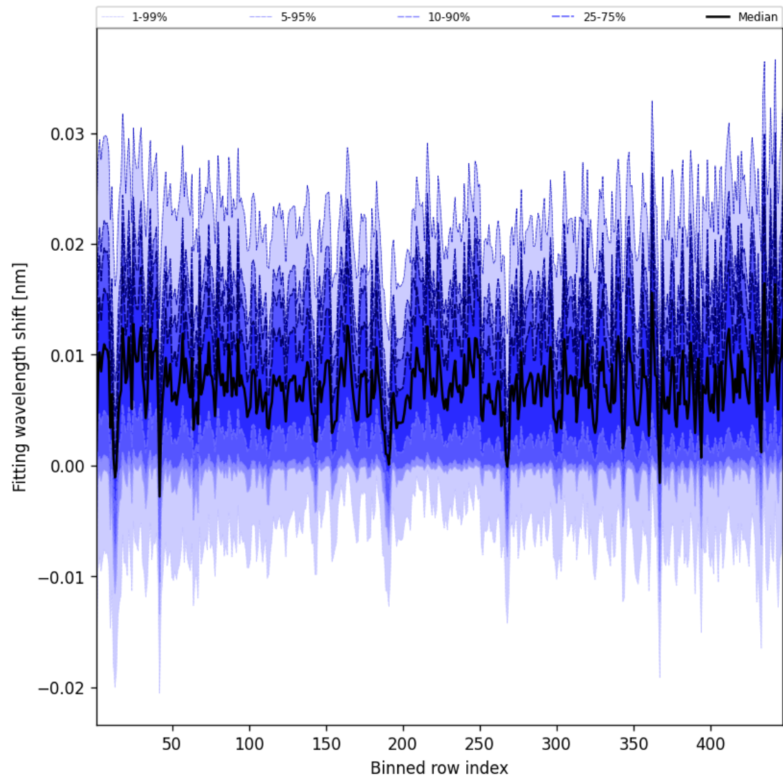
Figure 65: Along track statistics of “Fitting wavelength shift” for 2025-07-25 to 2025-07-27
