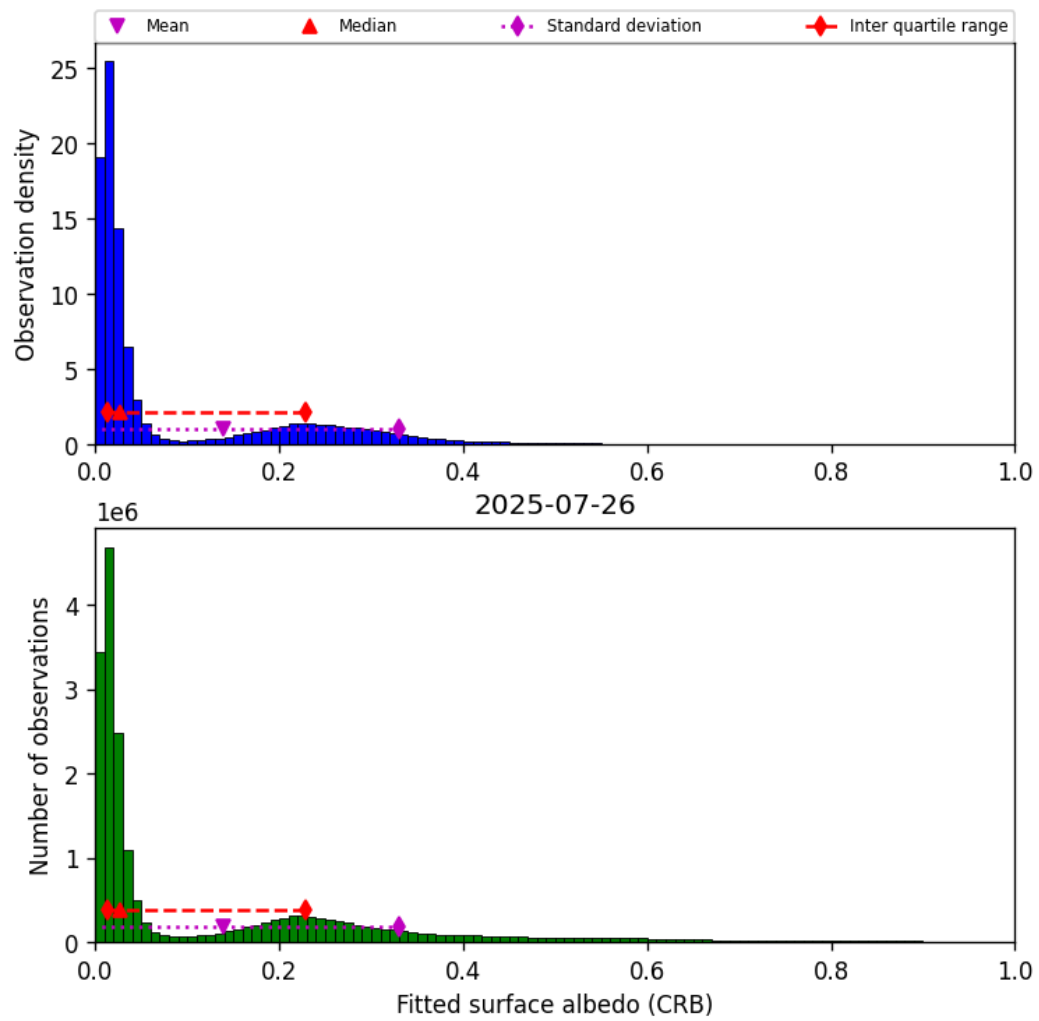
Figure 46: Histogram of “Fitted surface albedo (CRB)” for 2025-07-25 to 2025-07-27
