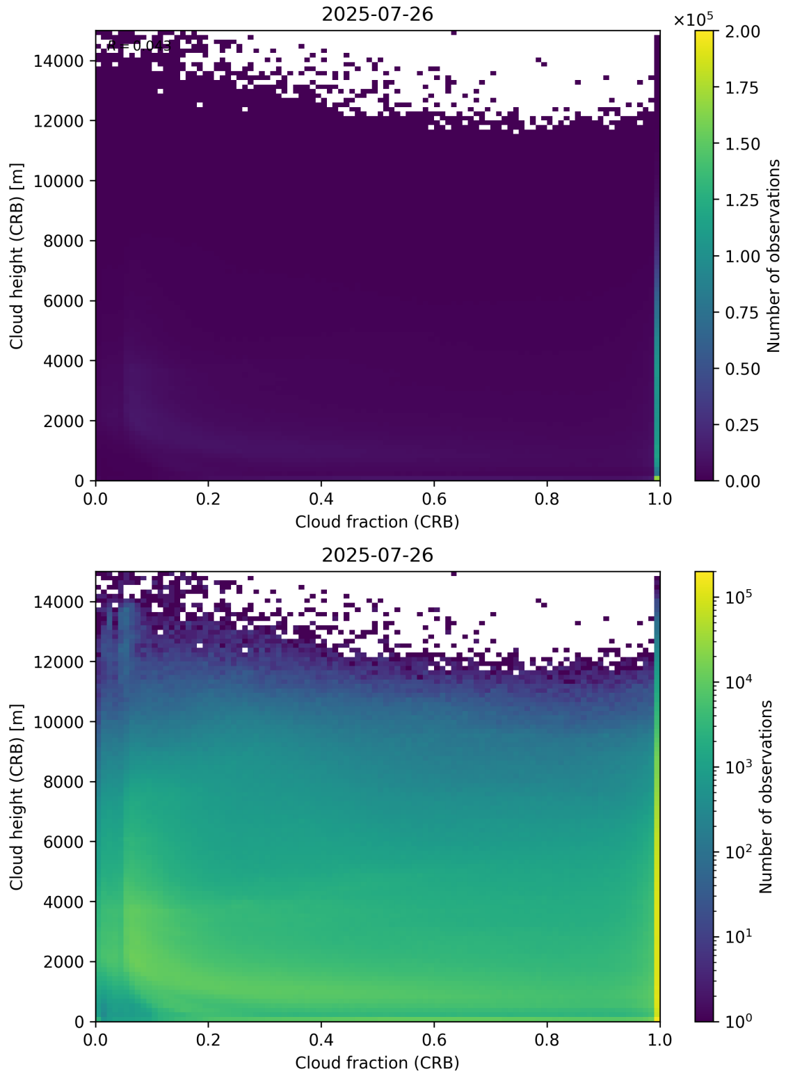
Figure 79: Scatter density plot of “Cloud fraction (CRB)” against “Cloud height (CRB)” for 2025-07-25 to 2025-07-27.
