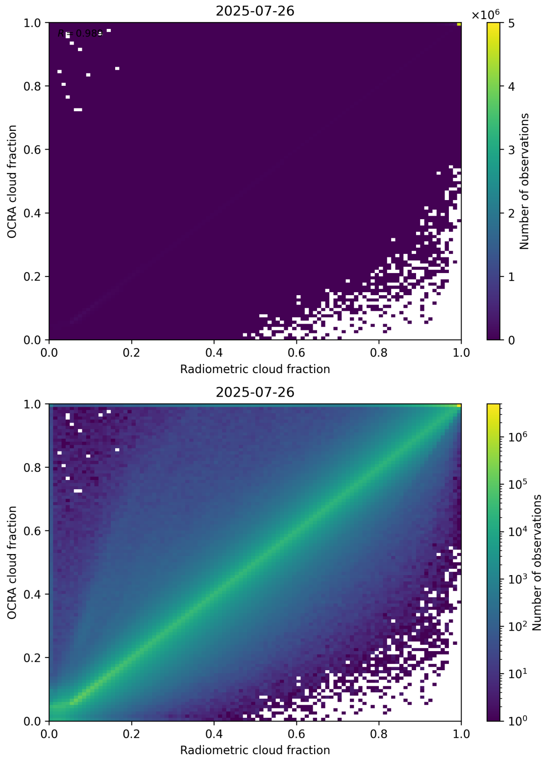
Figure 72: Scatter density plot of “Radiometric cloud fraction” against “OCRA cloud fraction” for 2025-07-25 to 2025-07-27.
