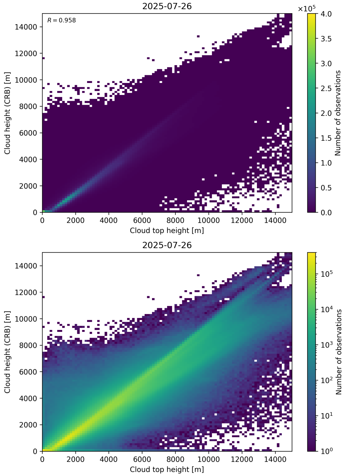
Figure 89: Scatter density plot of “Cloud top height” against “Cloud height (CRB)” for 2025-07-25 to 2025-07-27.
