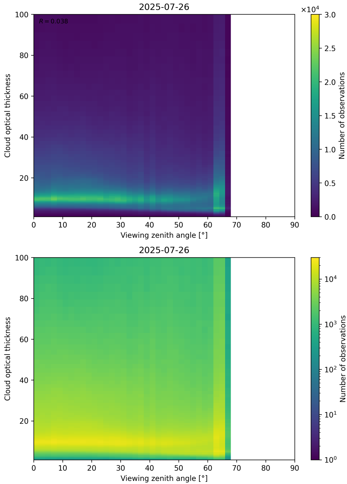
Figure 111: Scatter density plot of “Viewing zenith angle” against “Cloud optical thickness” for 2025-07-25 to 2025-07-27.
