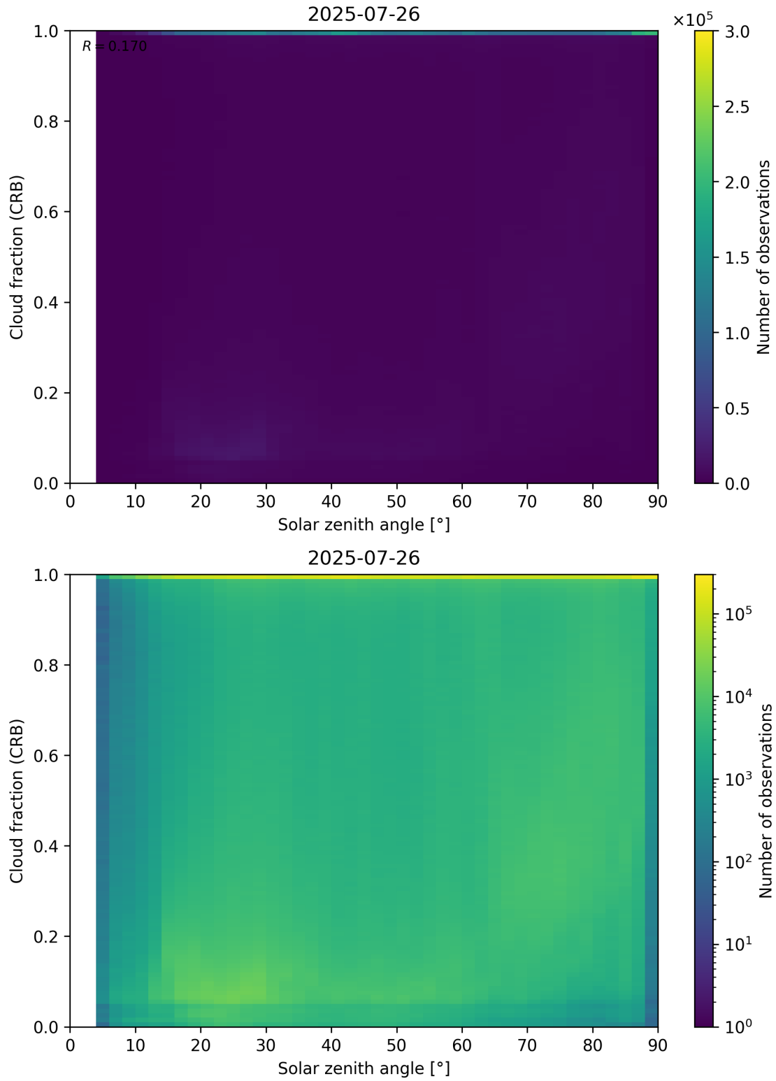
Figure 101: Scatter density plot of “Solar zenith angle” against “Cloud fraction (CRB)” for 2025-07-25 to 2025-07-27.
