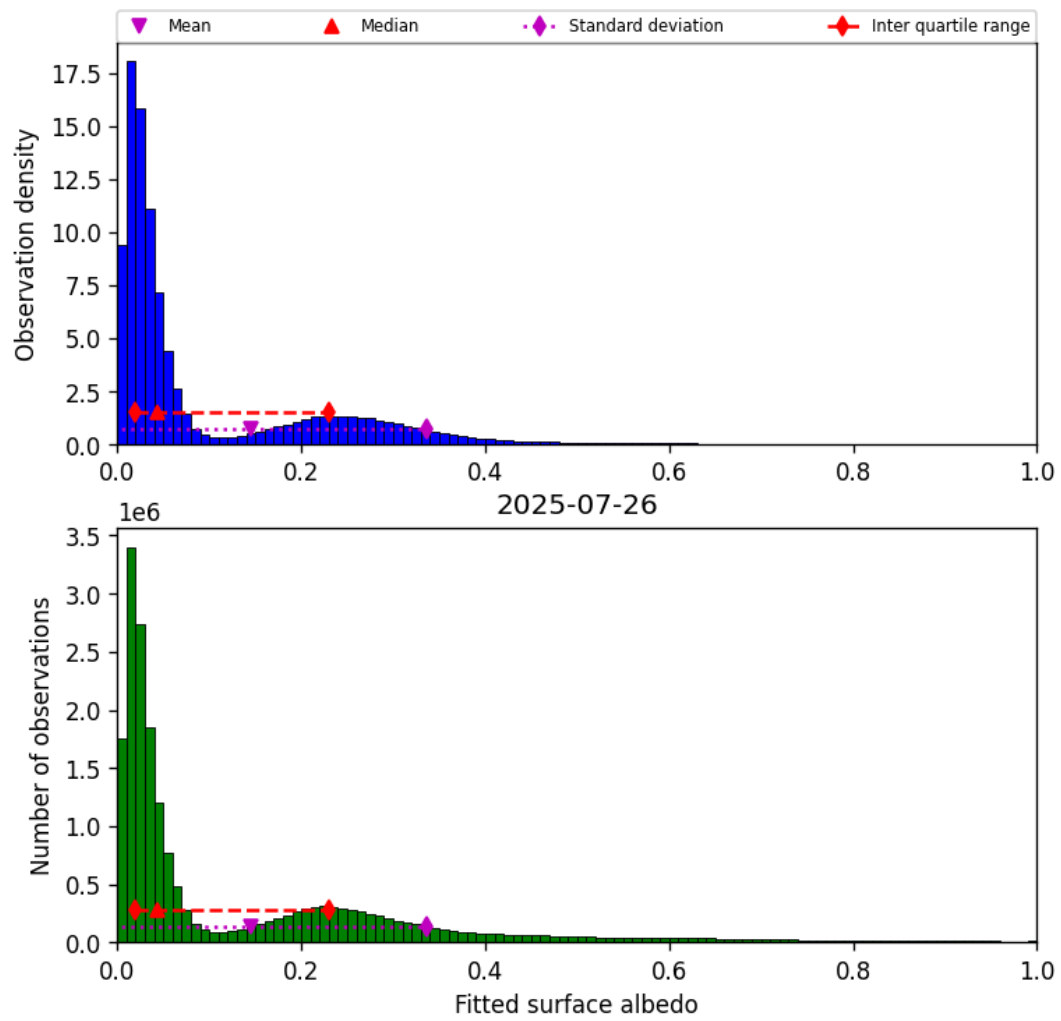
Figure 45: Histogram of “Fitted surface albedo” for 2025-07-25 to 2025-07-27
