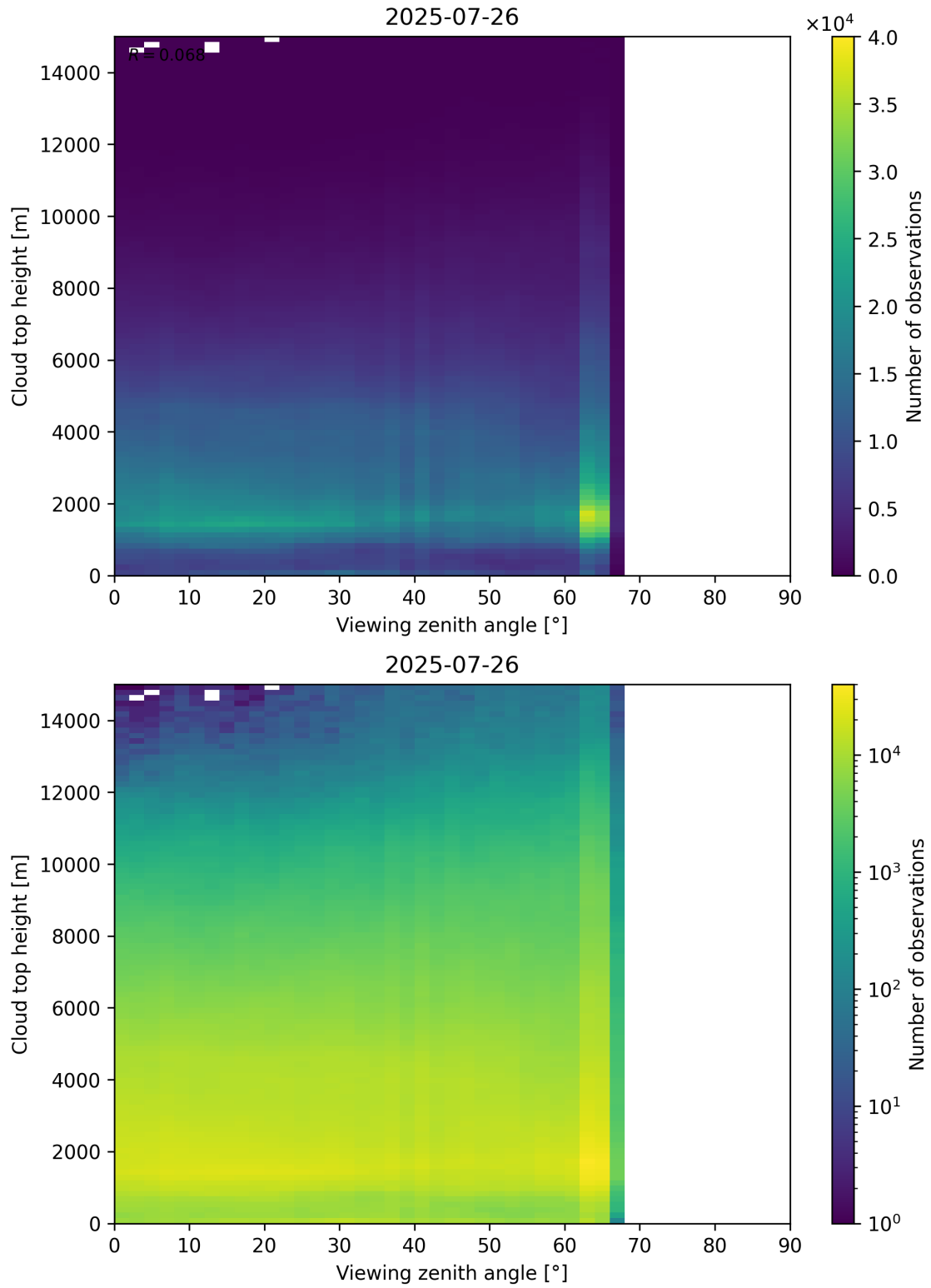
Figure 112: Scatter density plot of “Viewing zenith angle” against “Cloud top height” for 2025-07-25 to 2025-07-27.
