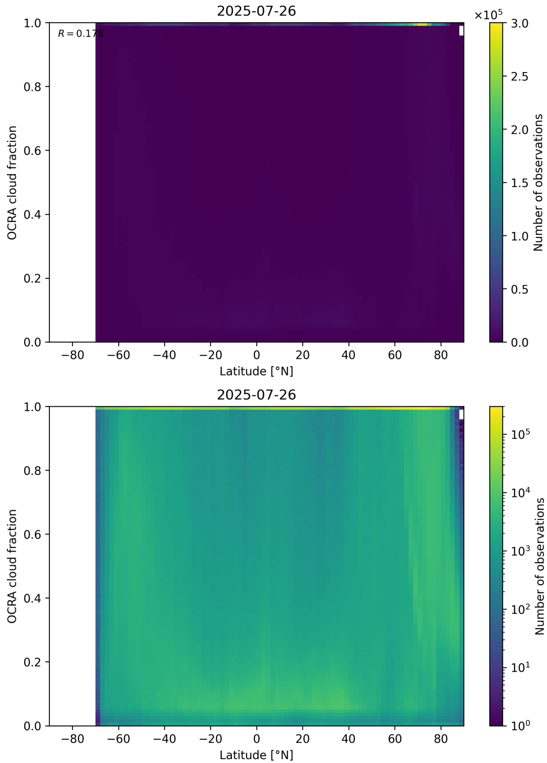
Figure 93: Scatter density plot of “Latitude” against “OCRA cloud fraction” for 2025-07-25 to 2025-07-27.
