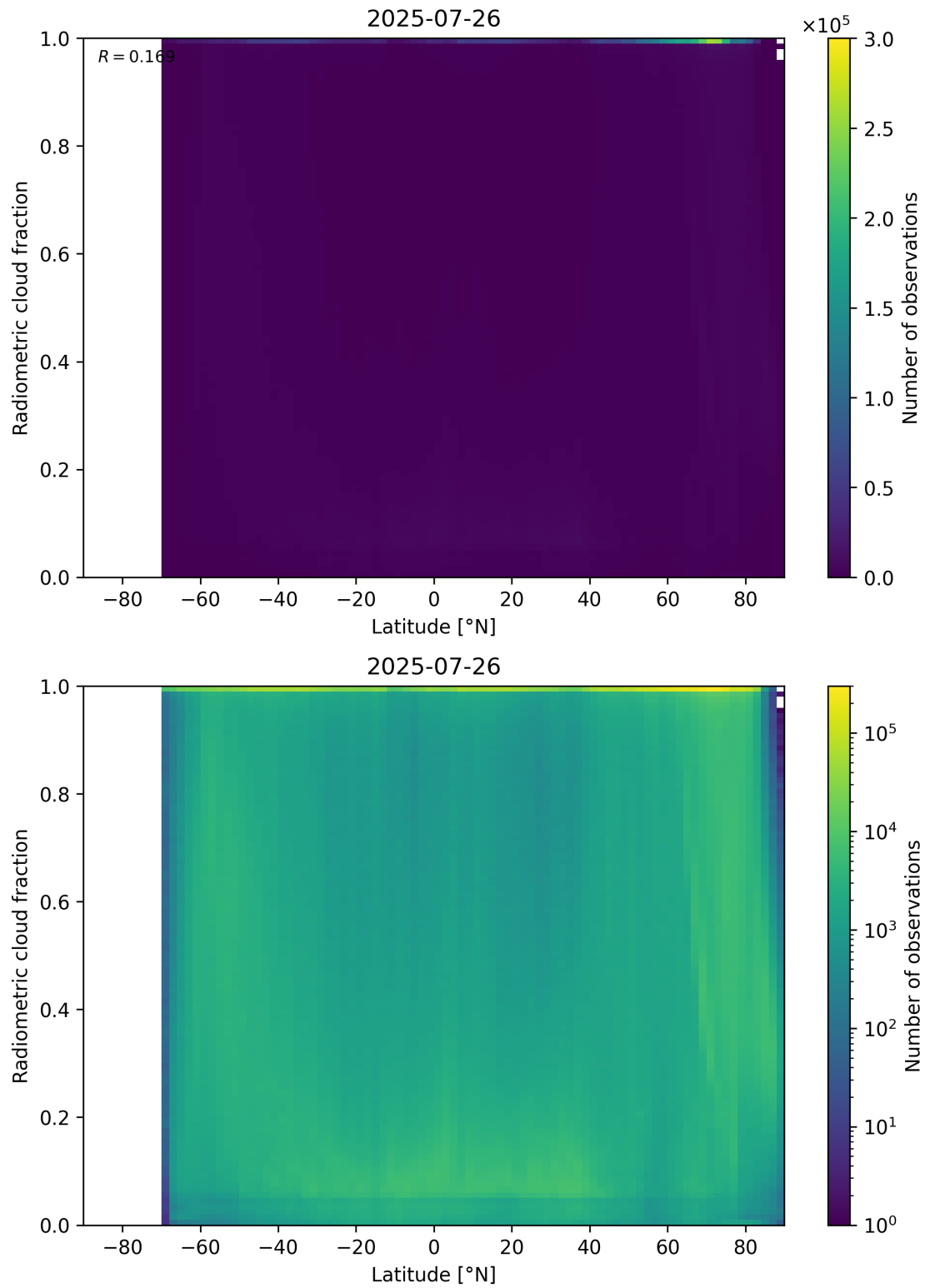
Figure 92: Scatter density plot of “Latitude” against “Radiometric cloud fraction” for 2025-07-25 to 2025-07-27.
