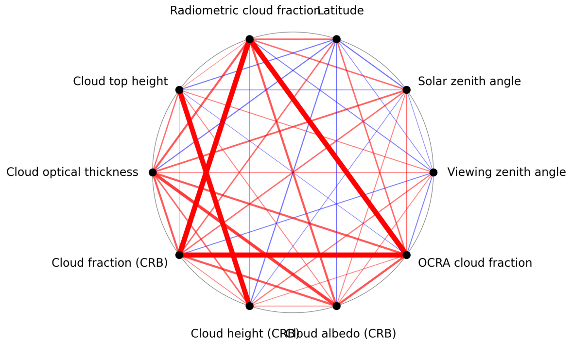
Figure 1: Map of correlation graph for 2025-07-25 to 2025-07-27.
