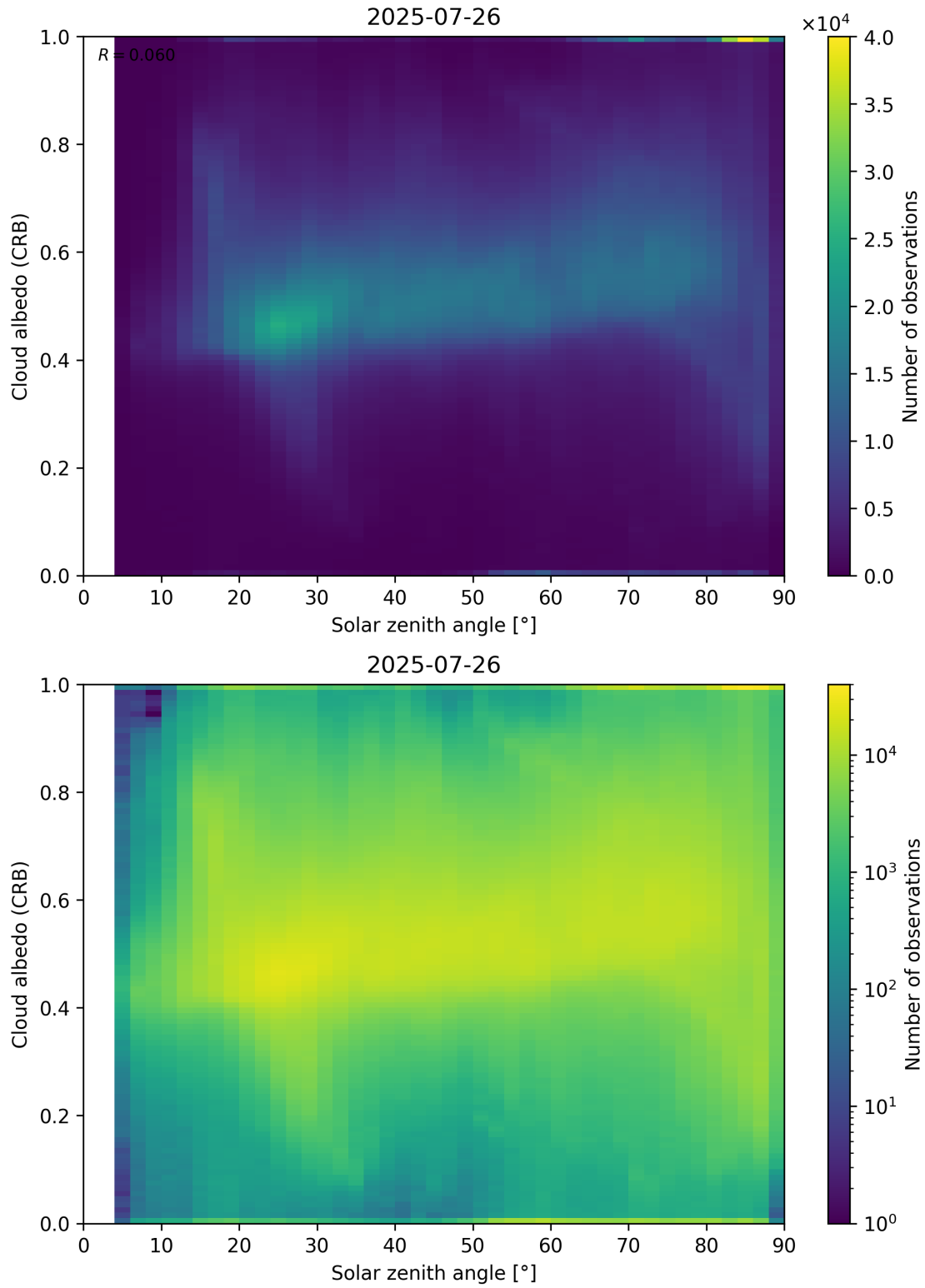
Figure 98: Scatter density plot of “Solar zenith angle” against “Cloud albedo (CRB)” for 2025-07-25 to 2025-07-27.
