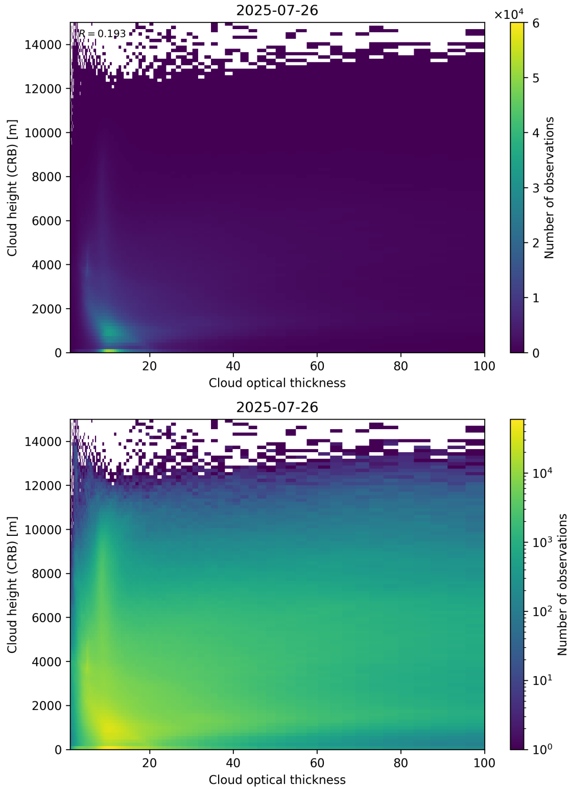
Figure 85: Scatter density plot of “Cloud optical thickness” against “Cloud height (CRB)” for 2025-07-25 to 2025-07-27.
