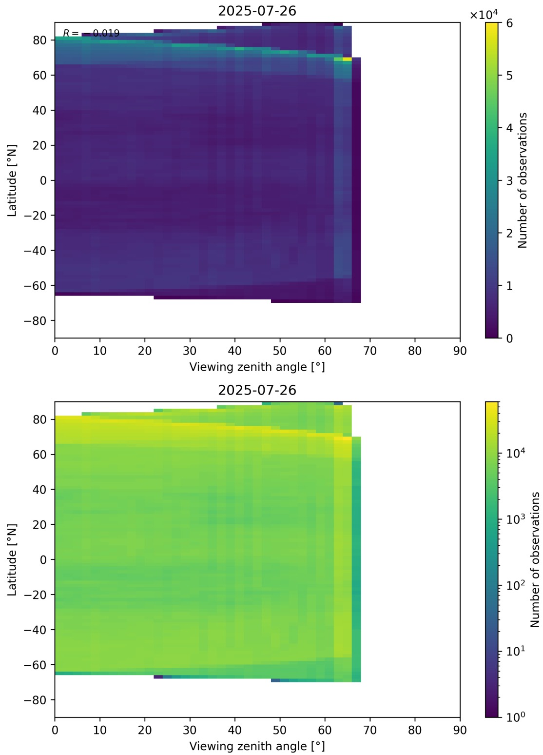
Figure 113: Scatter density plot of “Viewing zenith angle” against “Latitude” for 2025-07-25 to 2025-07-27.
