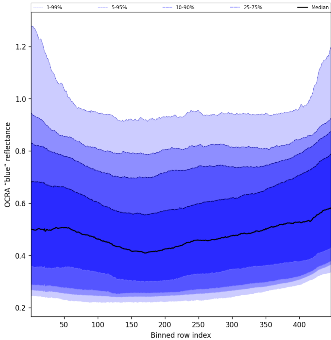
Figure 67: Along track statistics of “OCRA “blue” reflectance” for 2025-07-25 to 2025-07-27
