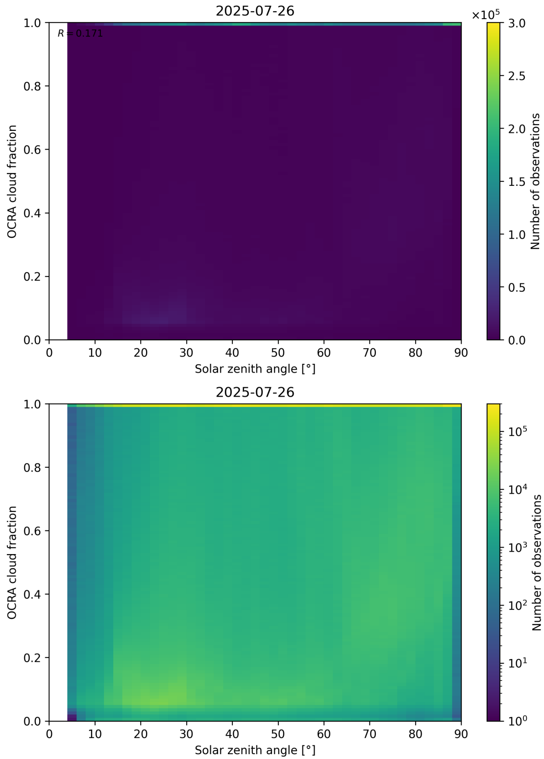
Figure 100: Scatter density plot of “Solar zenith angle” against “OCRA cloud fraction” for 2025-07-25 to 2025-07-27.
