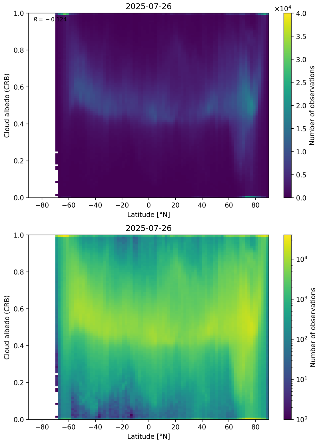
Figure 91: Scatter density plot of “Latitude” against “Cloud albedo (CRB)” for 2025-07-25 to 2025-07-27.
