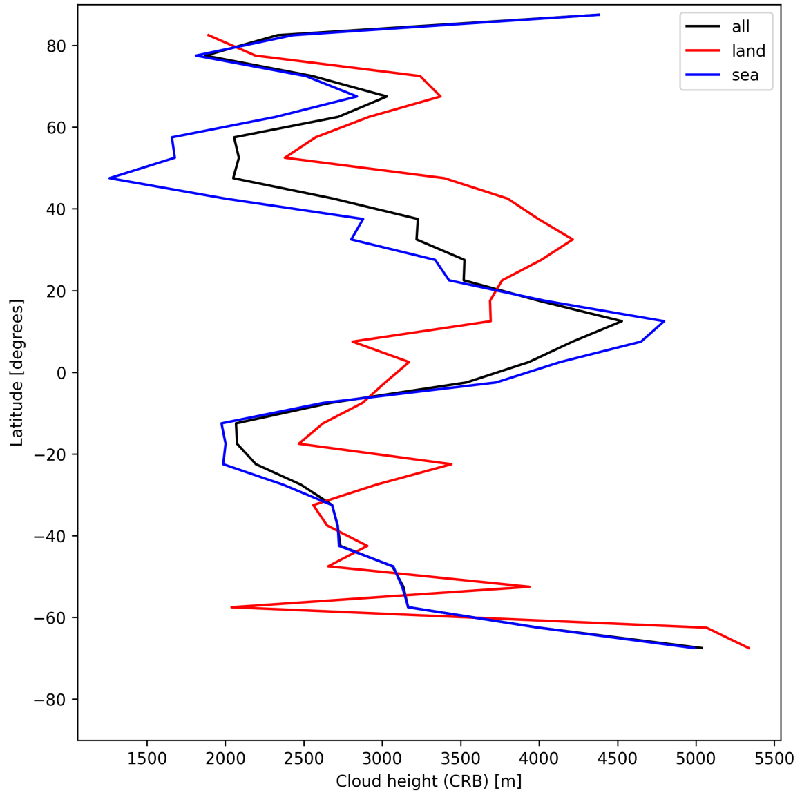
Figure 27: Zonal average of “Cloud height (CRB)” for 2025-07-25 to 2025-07-27.
