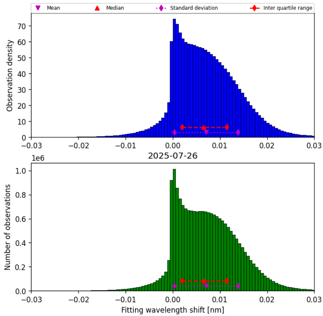
Figure 49: Histogram of “Fitting wavelength shift” for 2025-07-25 to 2025-07-27
