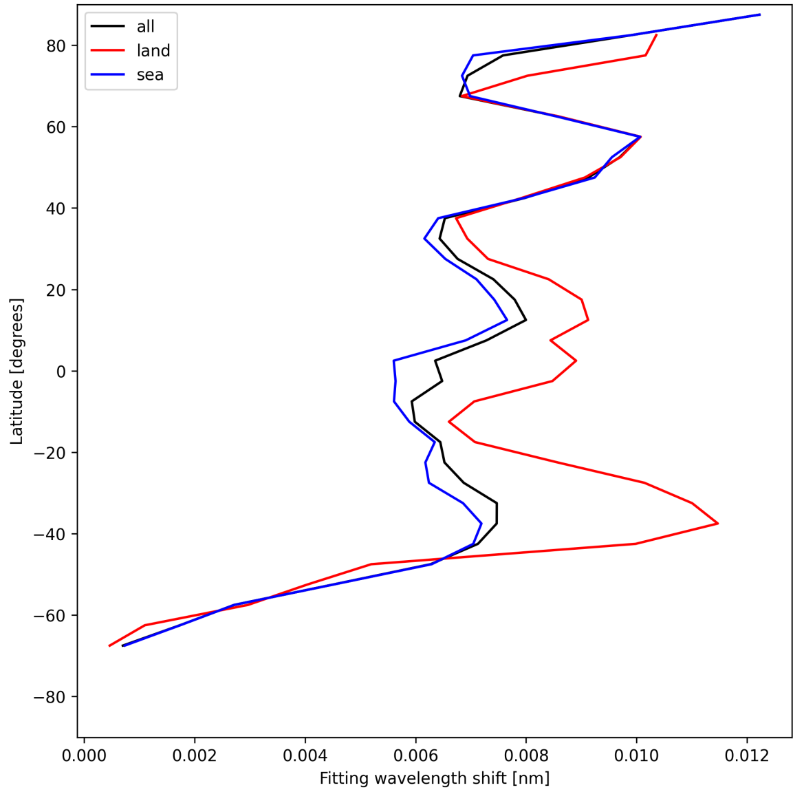
Figure 33: Zonal average of “Fitting wavelength shift” for 2025-07-25 to 2025-07-27.
