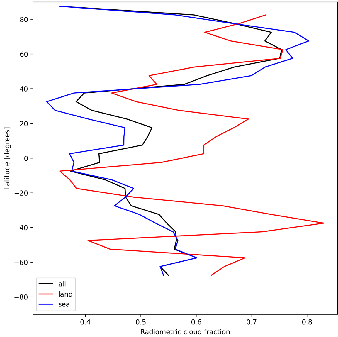
Figure 23: Zonal average of “Radiometric cloud fraction” for 2025-07-25 to 2025-07-27.
