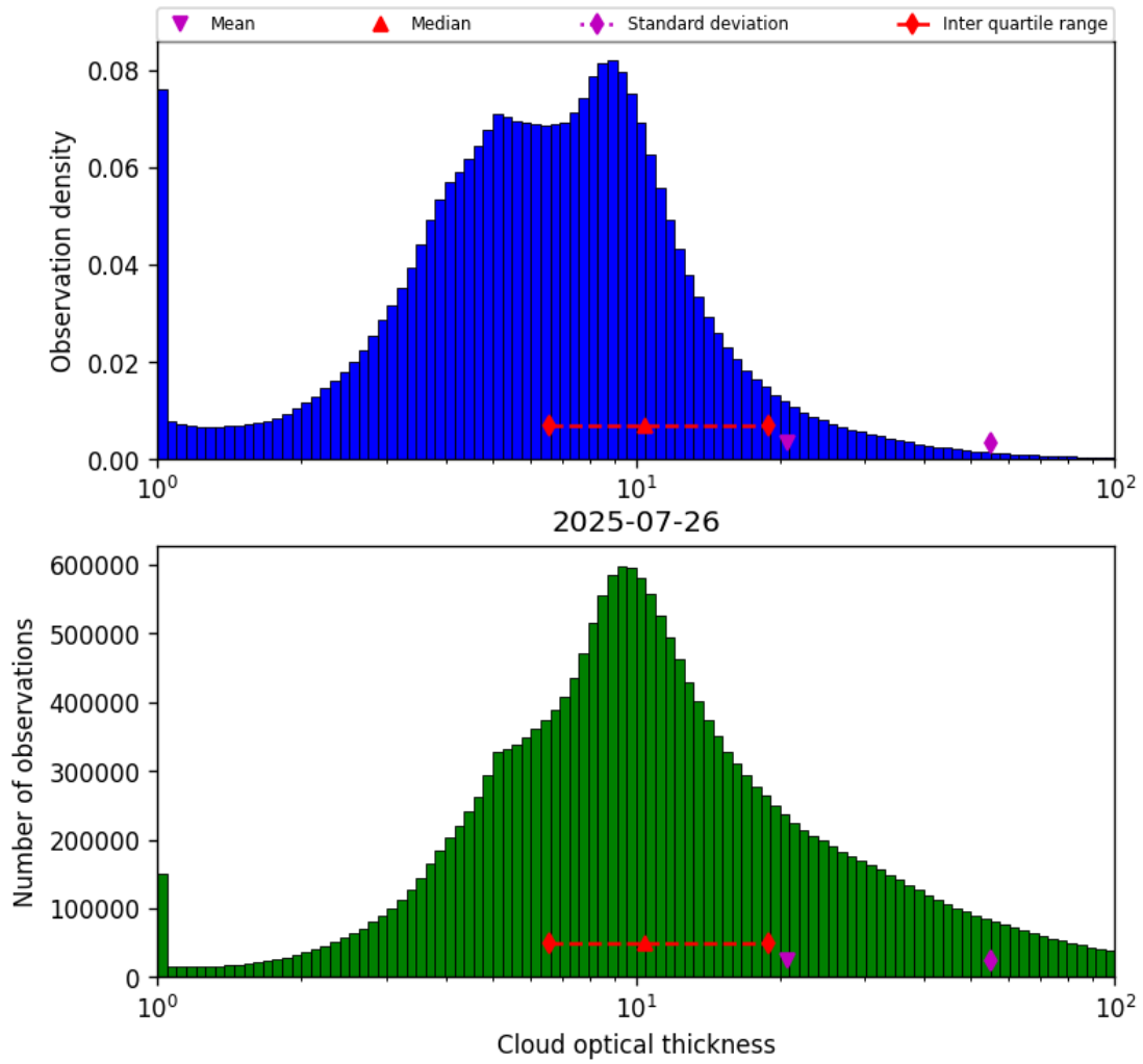
Figure 41: Histogram of “Cloud optical thickness” for 2025-07-25 to 2025-07-27
