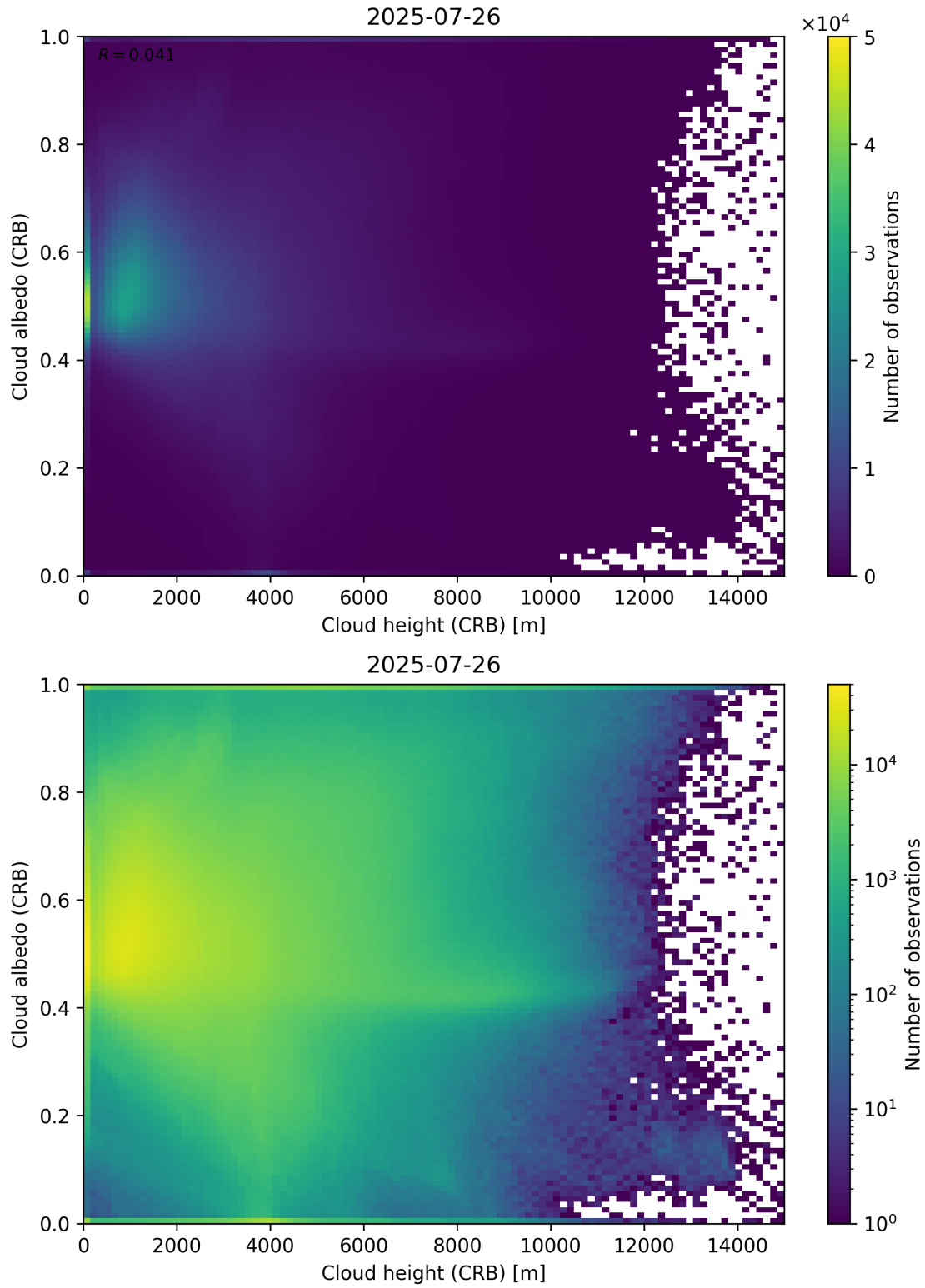
Figure 80: Scatter density plot of “Cloud height (CRB)” against “Cloud albedo (CRB)” for 2025-07-25 to 2025-07-27.
