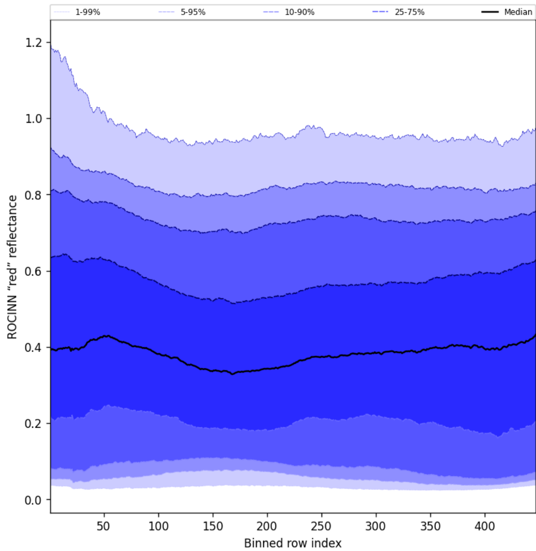
Figure 69: Along track statistics of "ROCINN "red" reflectance" for 2025-07-25 to 2025-07-27
