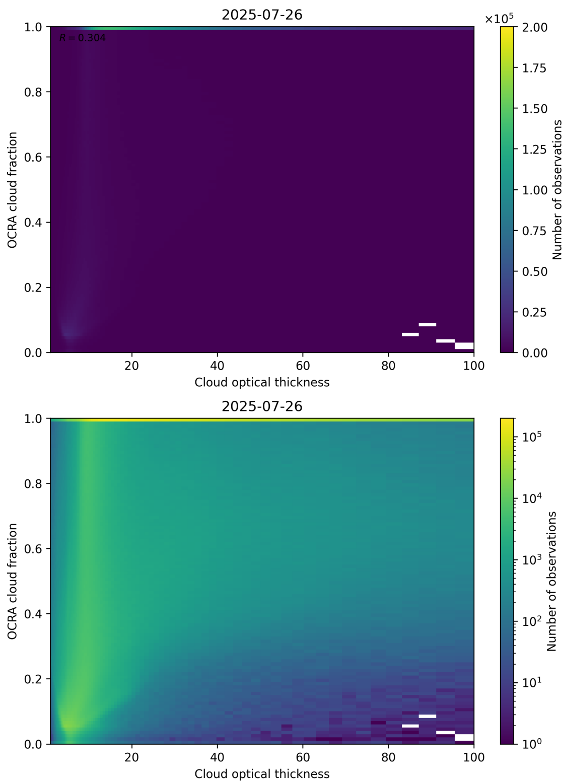
Figure 83: Scatter density plot of “Cloud optical thickness” against “OCRA cloud fraction” for 2025-07-25 to 2025-07-27.
