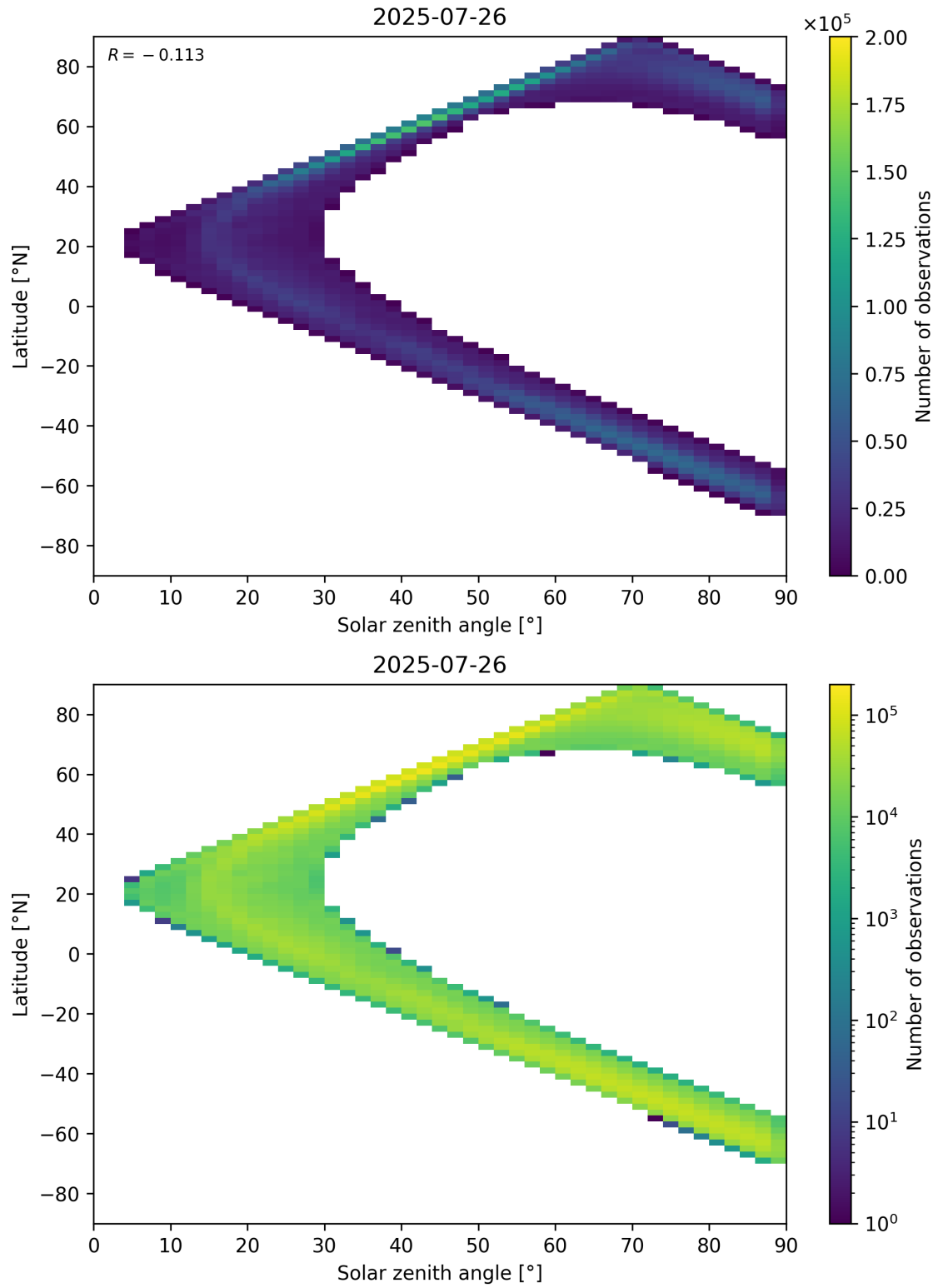
Figure 105: Scatter density plot of “Solar zenith angle” against “Latitude” for 2025-07-25 to 2025-07-27.
