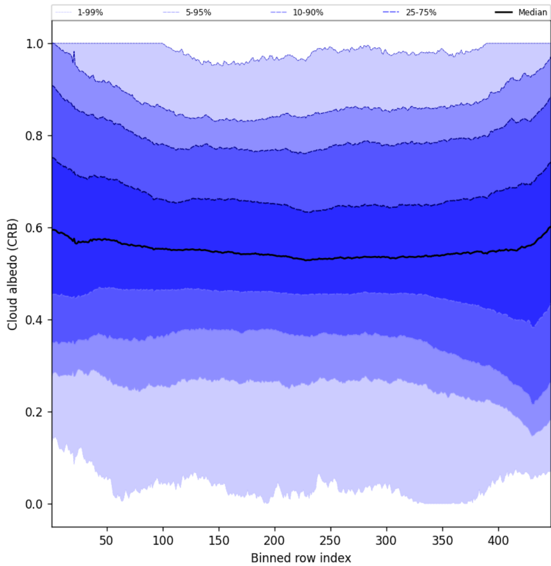
Figure 60: Along track statistics of “Cloud albedo (CRB)” for 2025-07-25 to 2025-07-27
