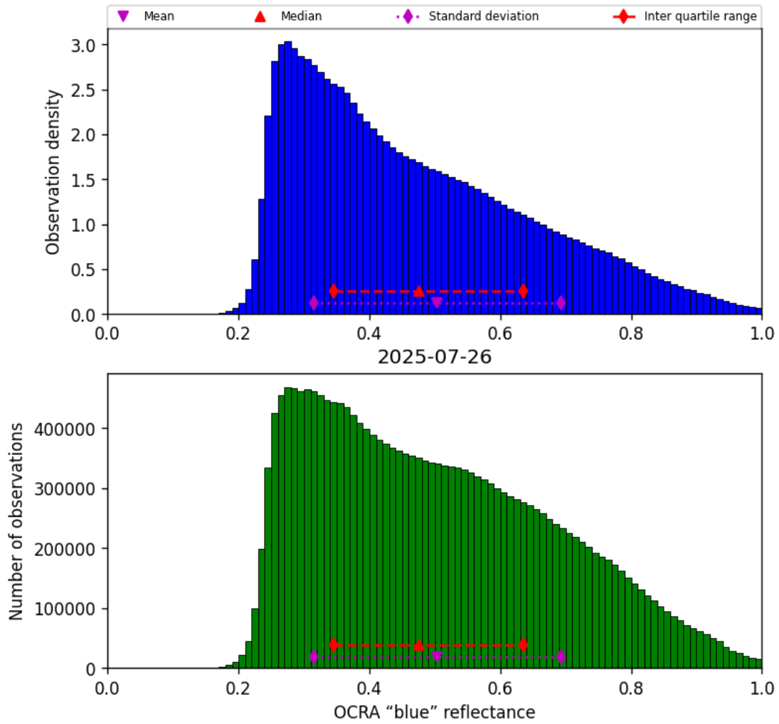
Figure 51: Histogram of “OCRA “blue” reflectance” for 2025-07-25 to 2025-07-27
