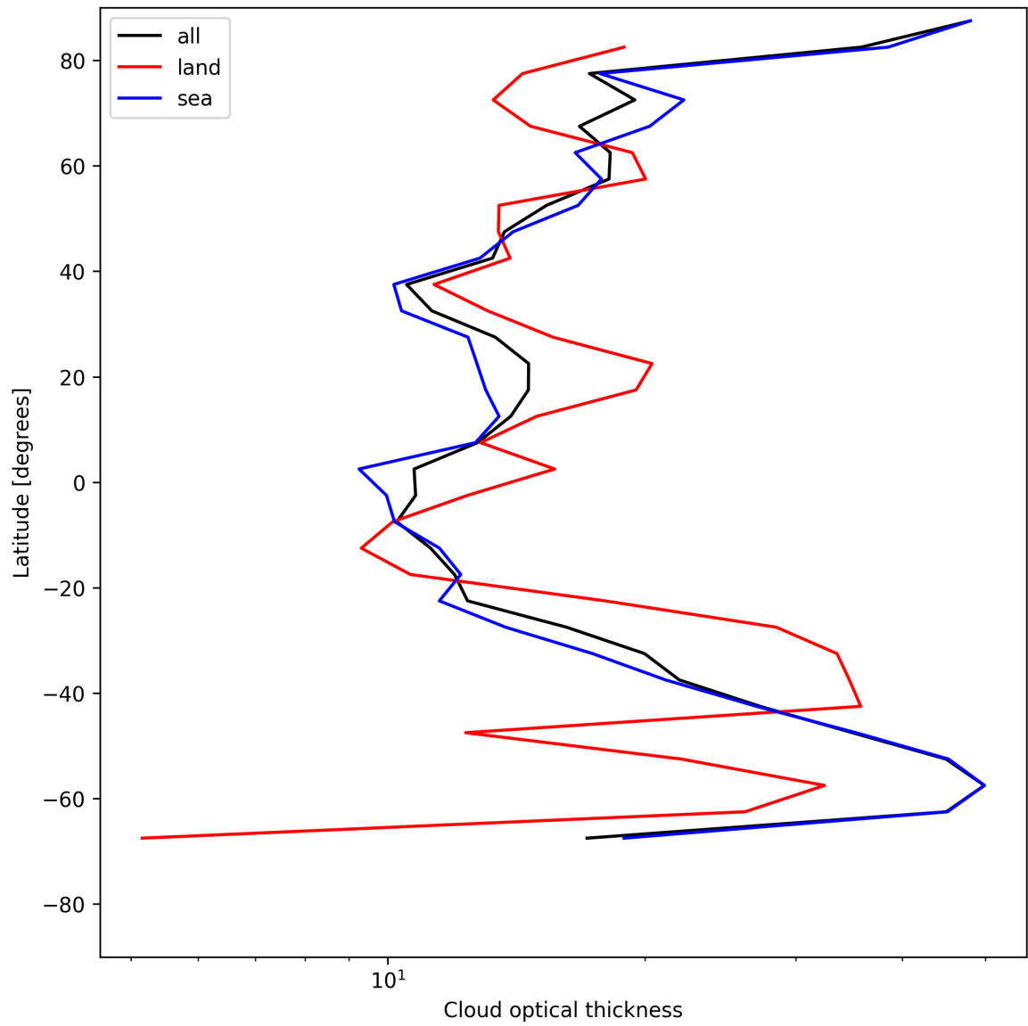
Figure 25: Zonal average of “Cloud optical thickness” for 2025-07-25 to 2025-07-27.
