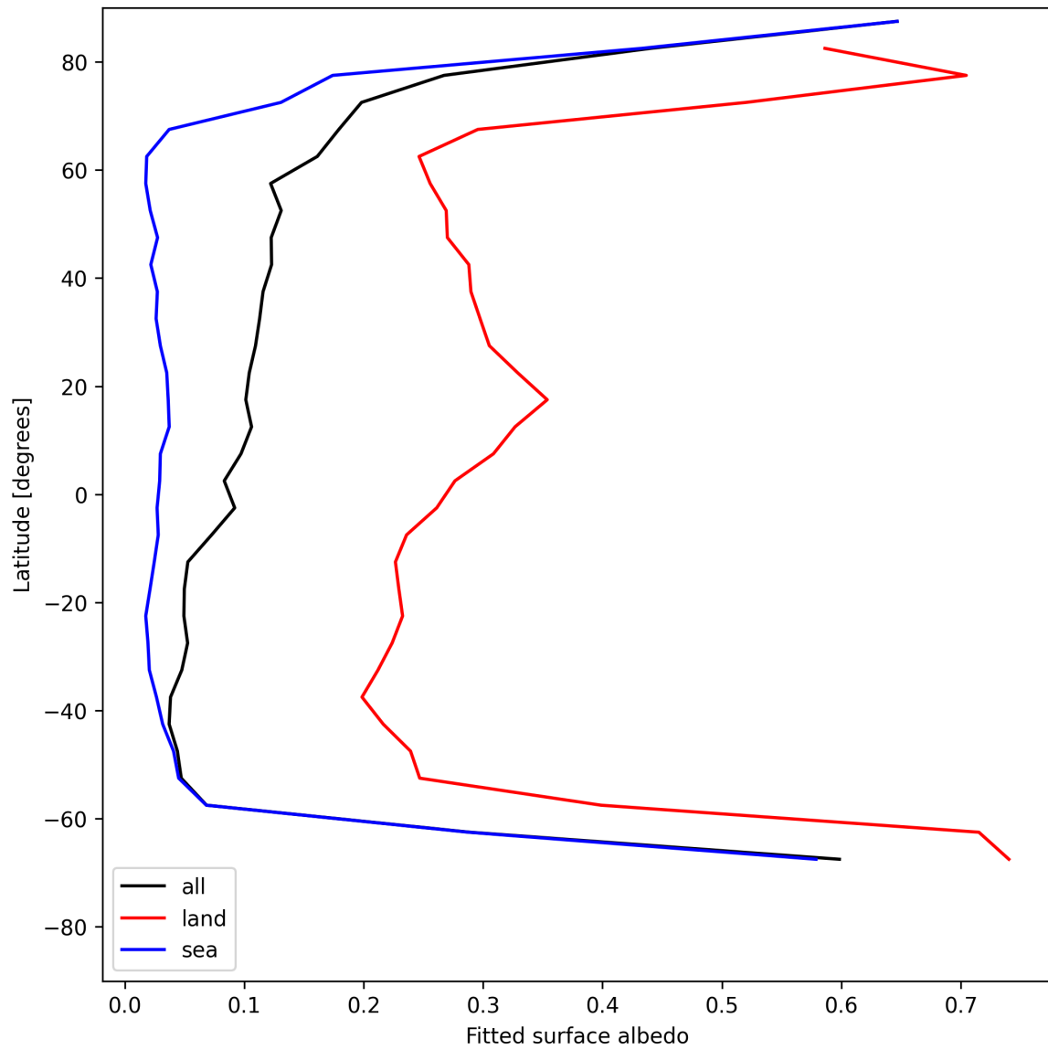
Figure 29: Zonal average of “Fitted surface albedo” for 2025-07-25 to 2025-07-27.
