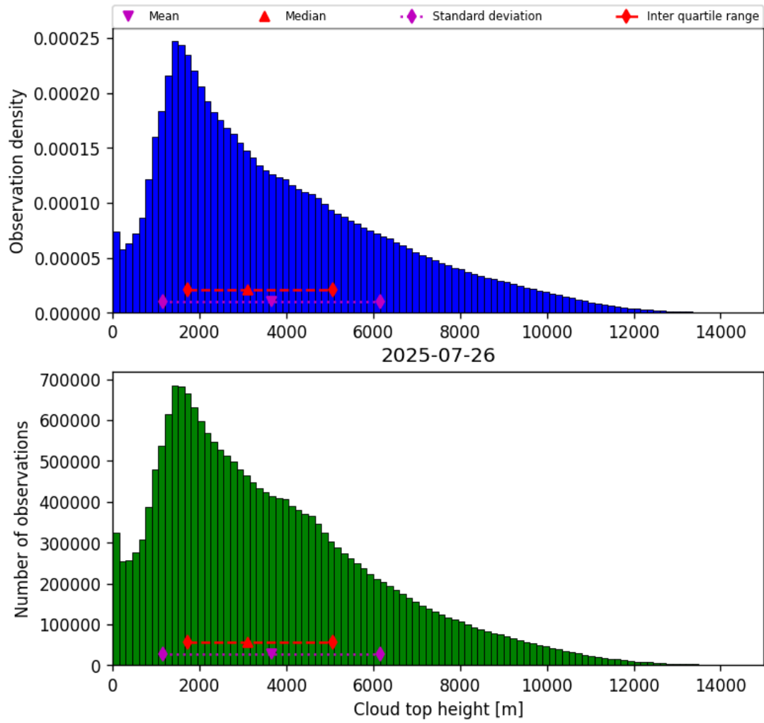
Figure 40: Histogram of “Cloud top height” for 2025-07-25 to 2025-07-27
