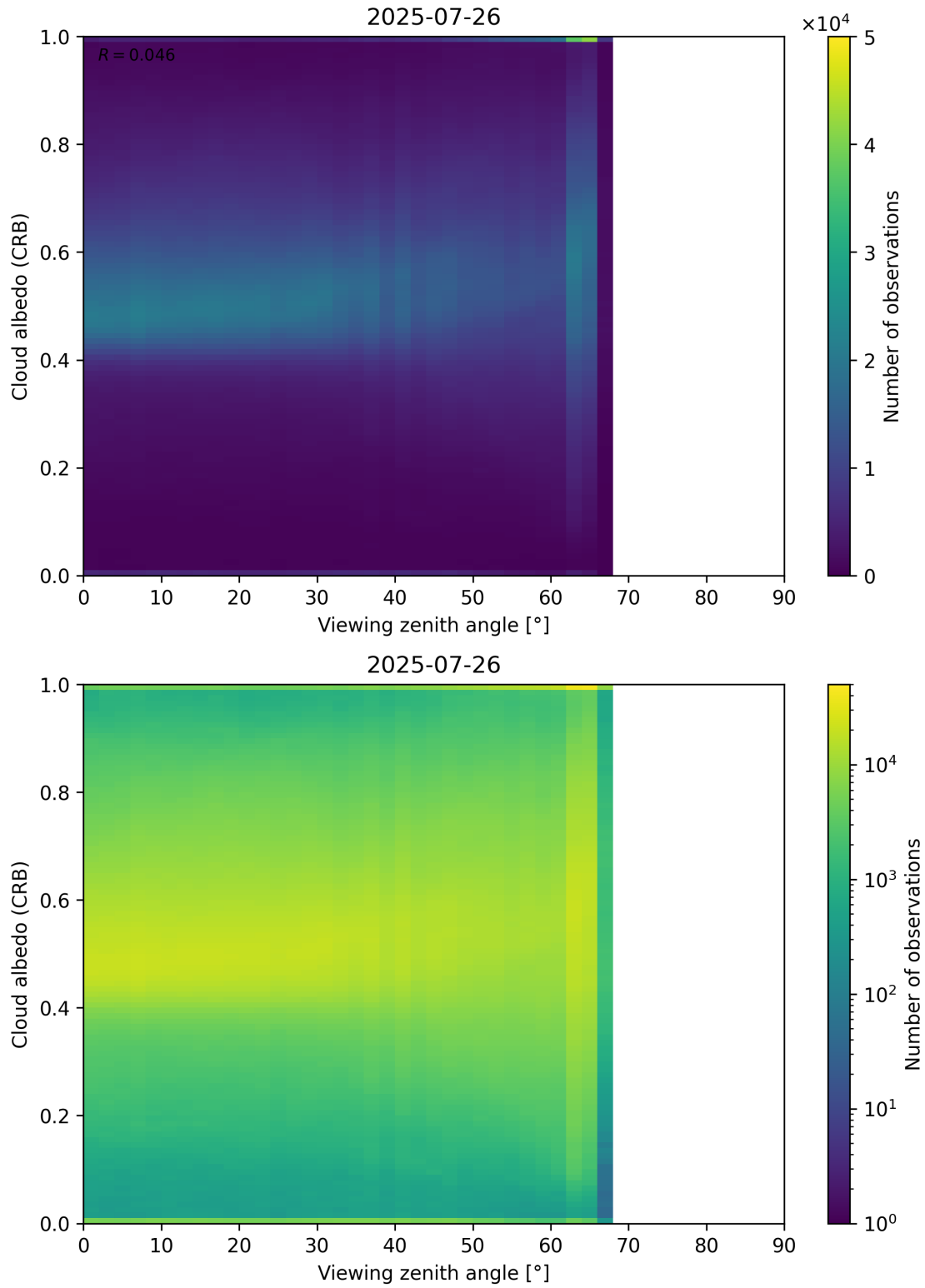
Figure 106: Scatter density plot of “Viewing zenith angle” against “Cloud albedo (CRB)” for 2025-07-25 to 2025-07-27.
