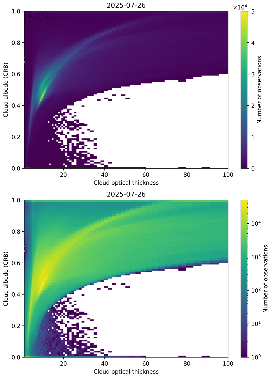
Figure 82: Scatter density plot of “Cloud optical thickness” against “Cloud albedo (CRB)” for 2025-07-25 to 2025-07-27.
