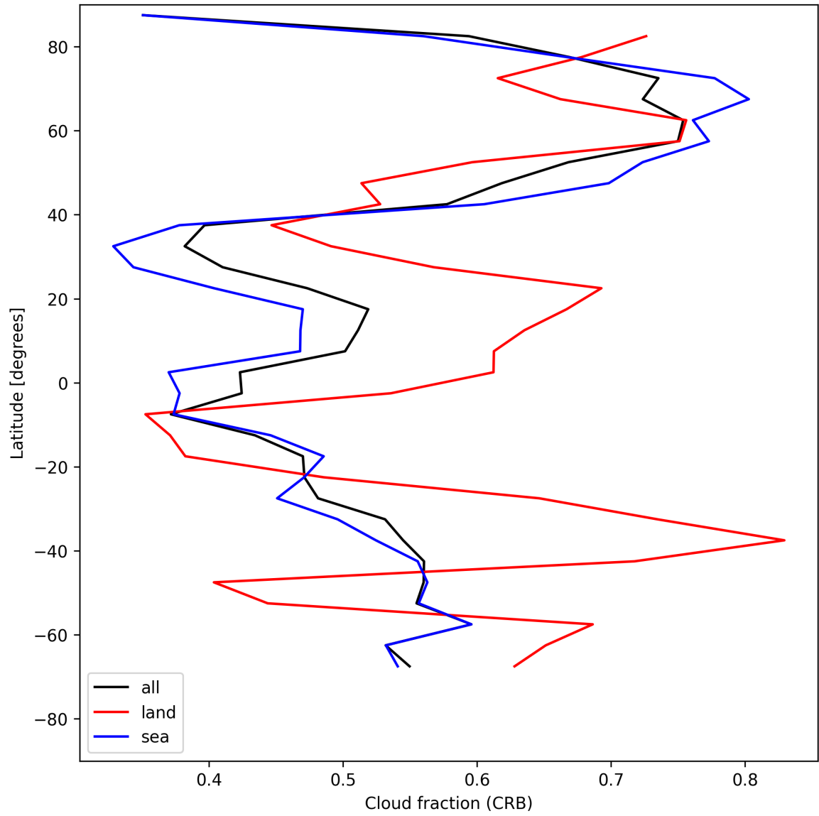
Figure 26: Zonal average of “Cloud fraction (CRB)” for 2025-07-25 to 2025-07-27.
