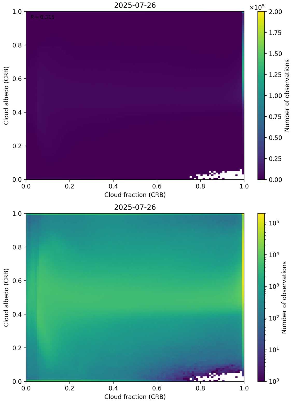
Figure 77: Scatter density plot of “Cloud fraction (CRB)” against “Cloud albedo (CRB)” for 2025-07-25 to 2025-07-27.
