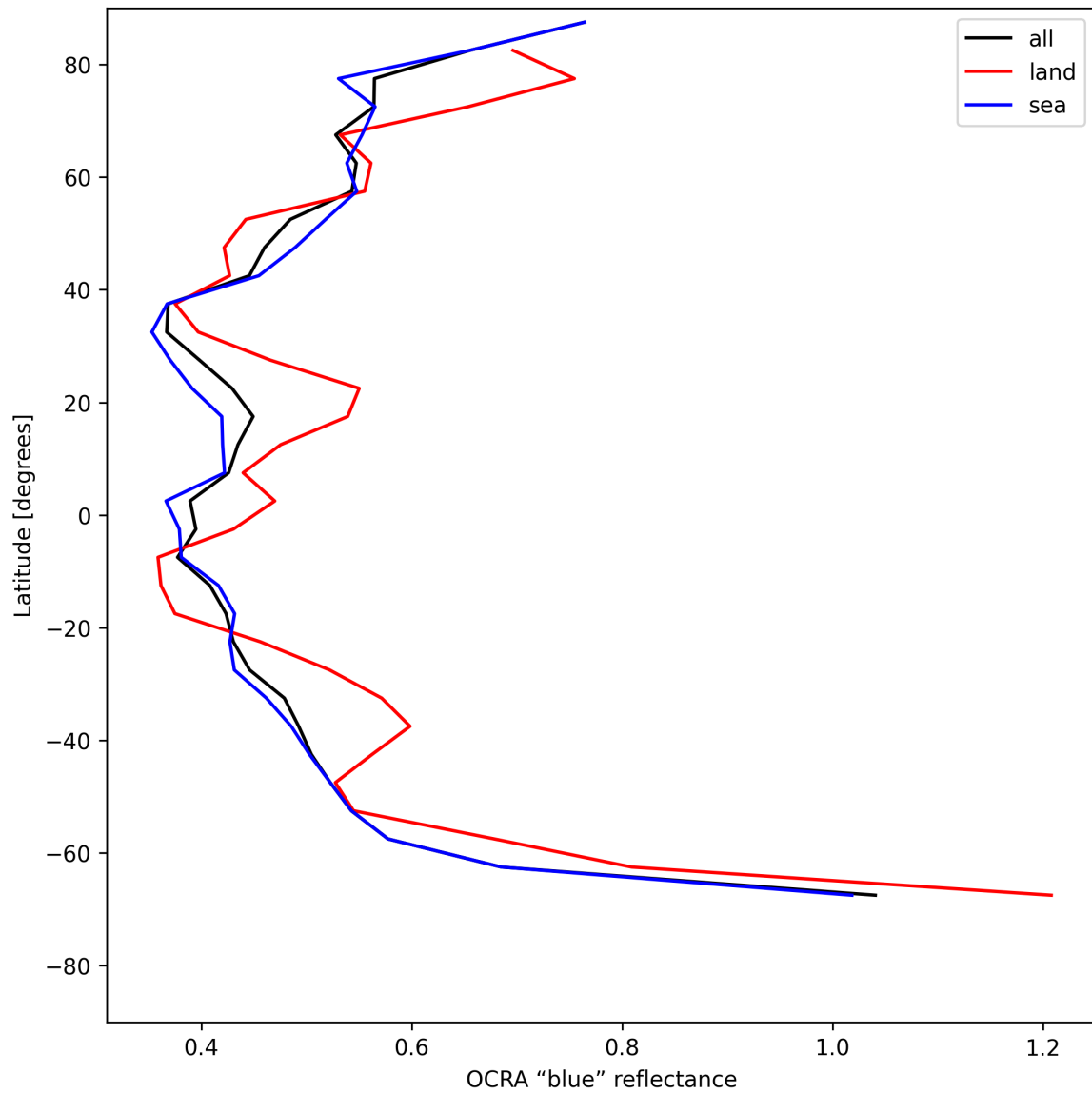
Figure 35: Zonal average of “OCRA “blue” reflectance” for 2025-07-25 to 2025-07-27.
