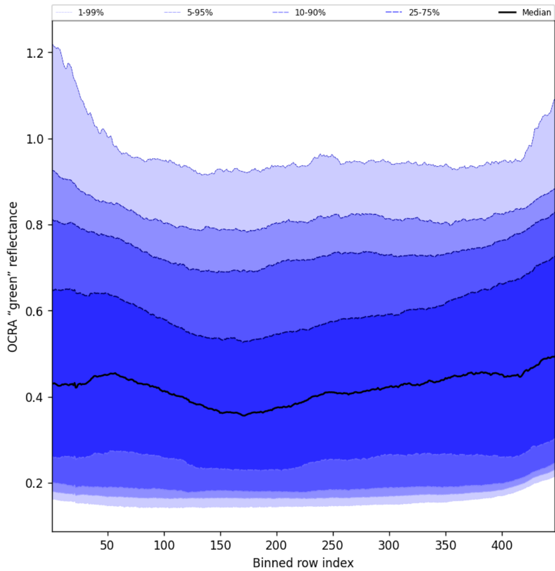
Figure 68: Along track statistics of “OCRA “green” reflectance” for 2025-07-25 to 2025-07-27
