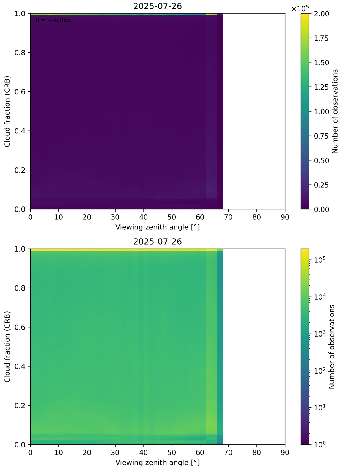
Figure 109: Scatter density plot of “Viewing zenith angle” against “Cloud fraction (CRB)” for 2025-07-25 to 2025-07-27.
