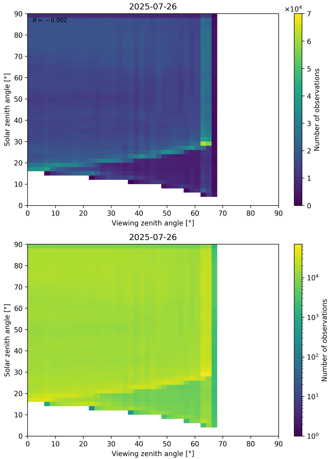
Figure 114: Scatter density plot of “Viewing zenith angle” against “Solar zenith angle” for 2025-07-25 to 2025-07-27.
