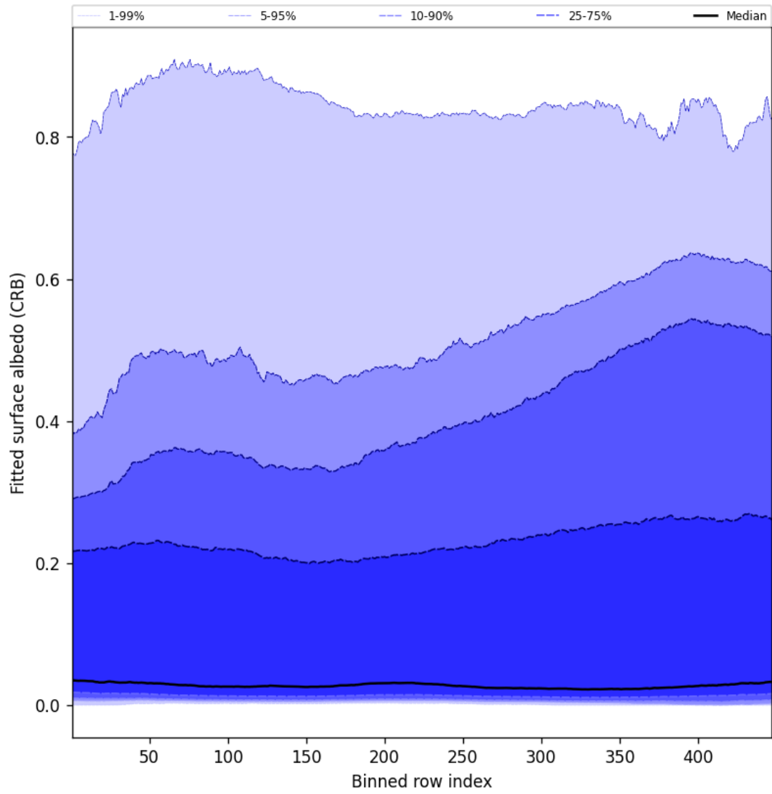
Figure 62: Along track statistics of “Fitted surface albedo (CRB)” for 2025-07-25 to 2025-07-27
