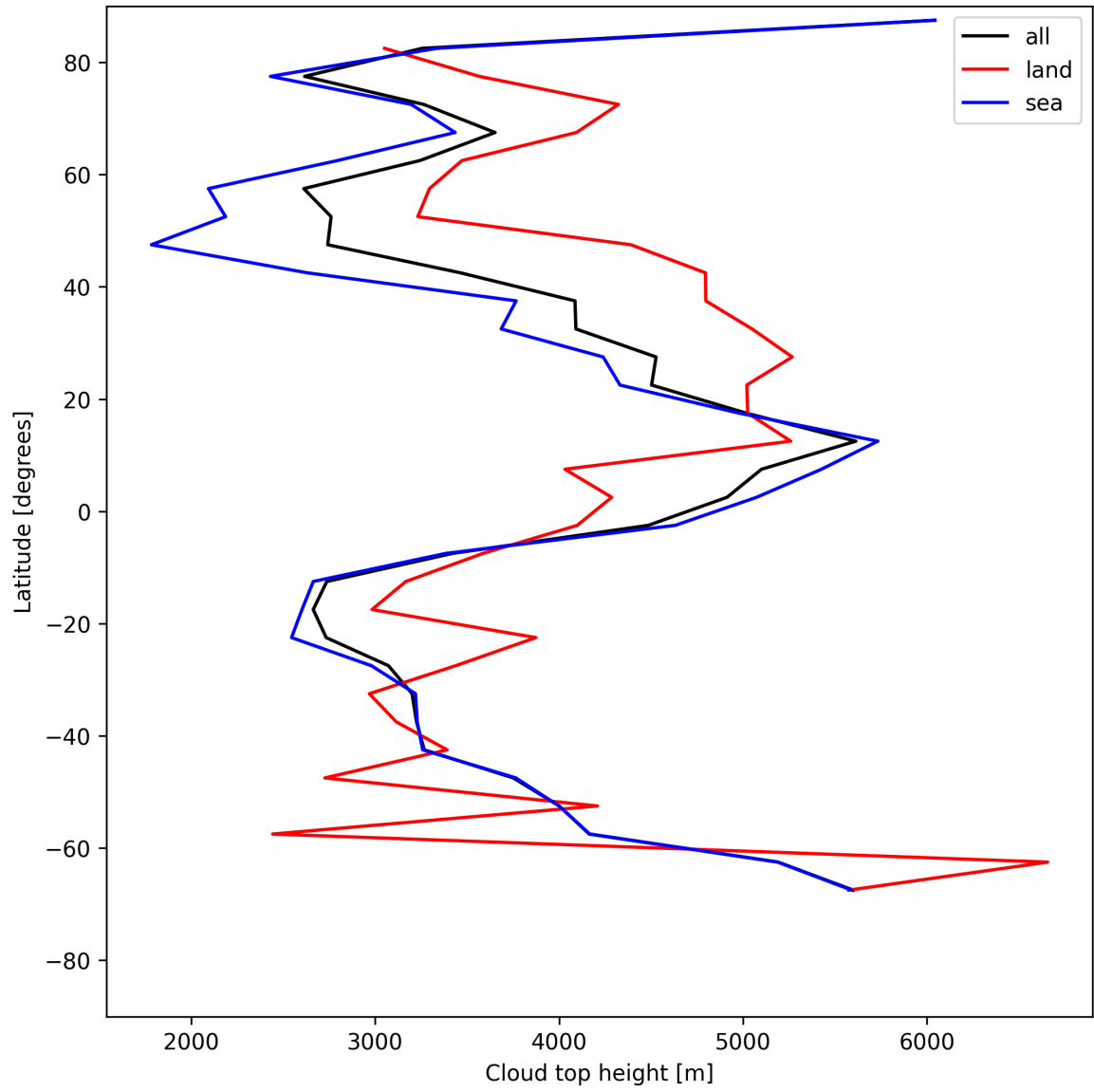
Figure 24: Zonal average of “Cloud top height” for 2025-07-25 to 2025-07-27.
