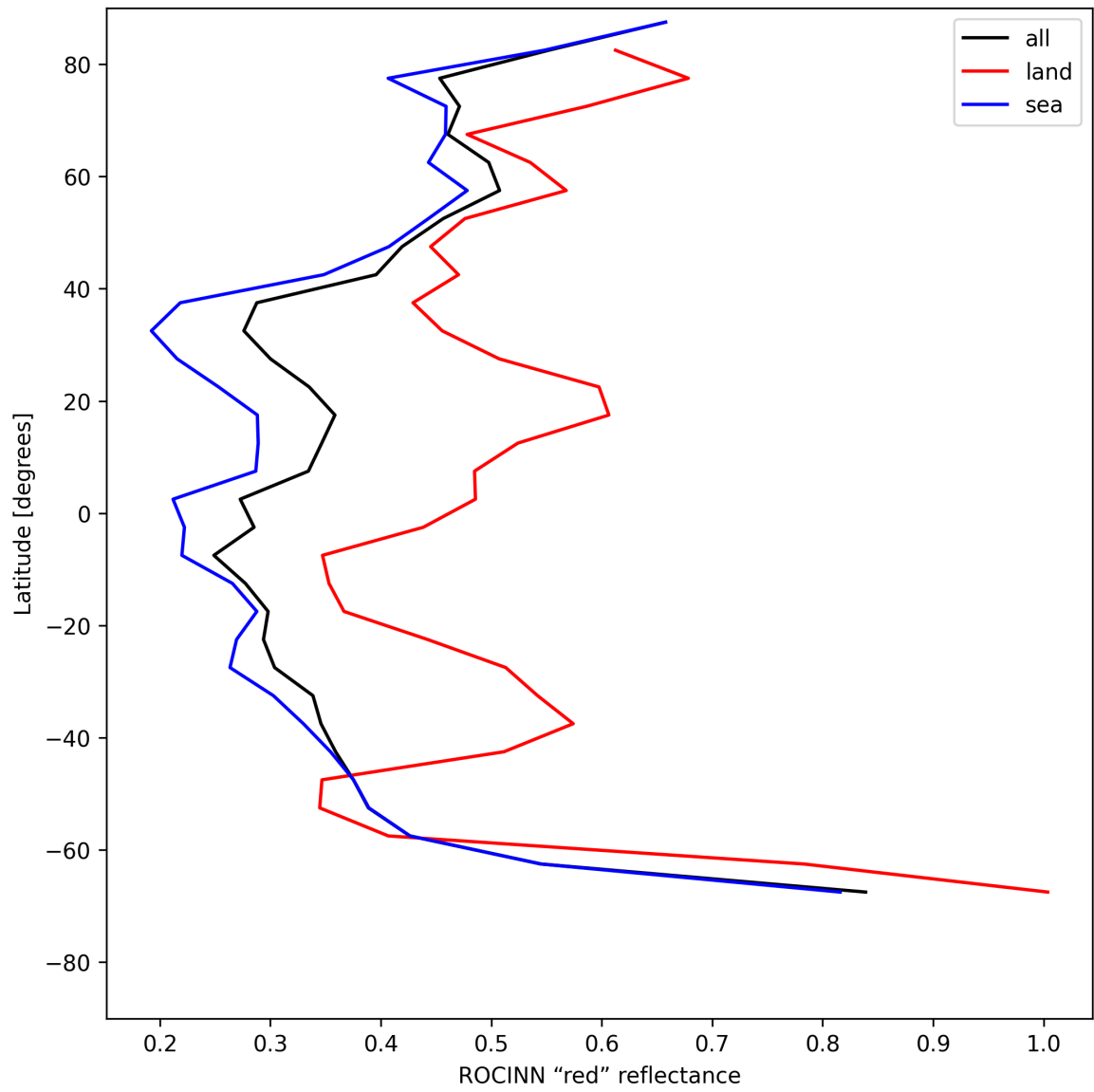
Figure 37: Zonal average of “ROCINN “red” reflectance” for 2025-07-25 to 2025-07-27.
