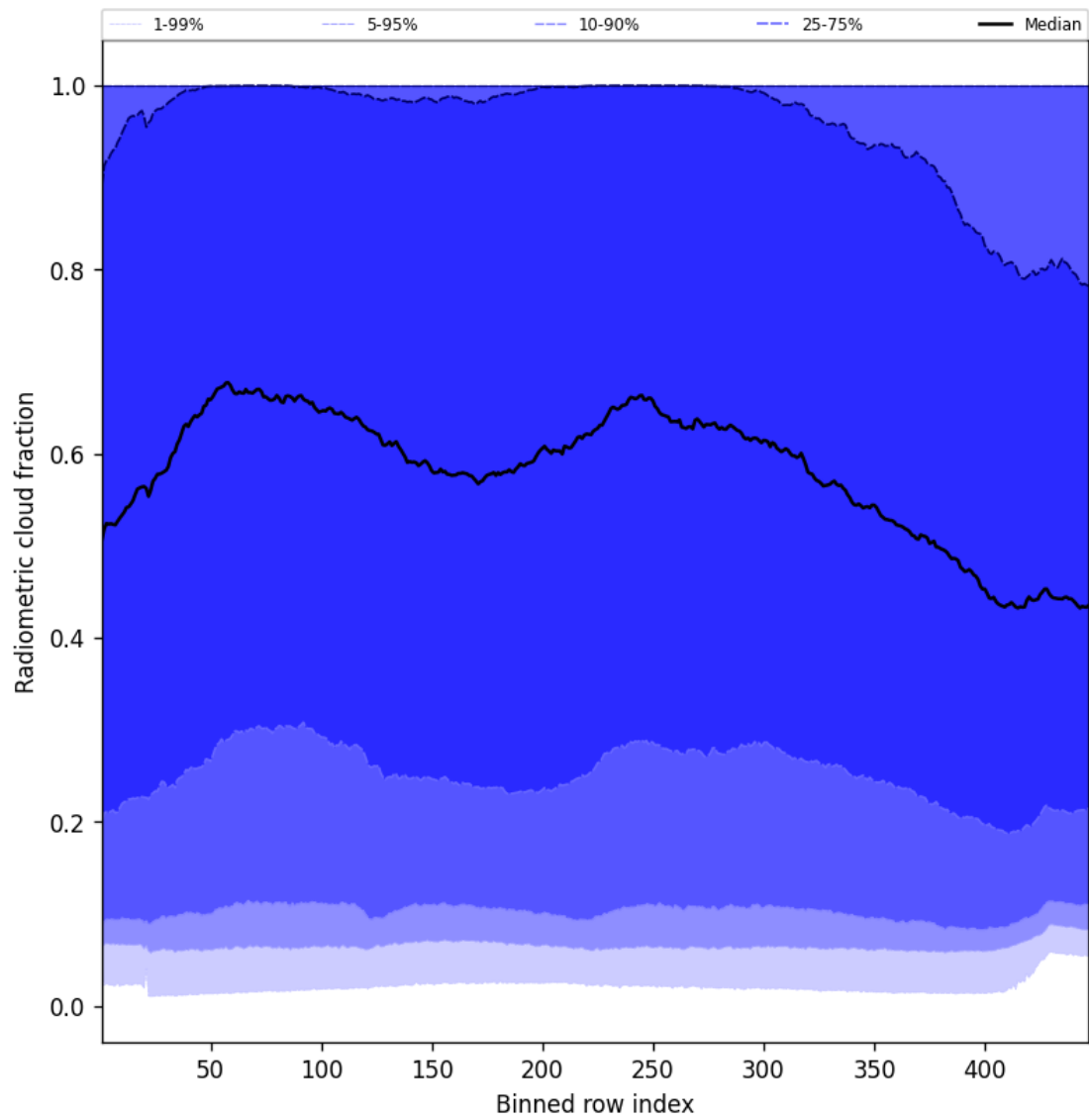
Figure 55: Along track statistics of “Radiometric cloud fraction” for 2025-07-25 to 2025-07-27
