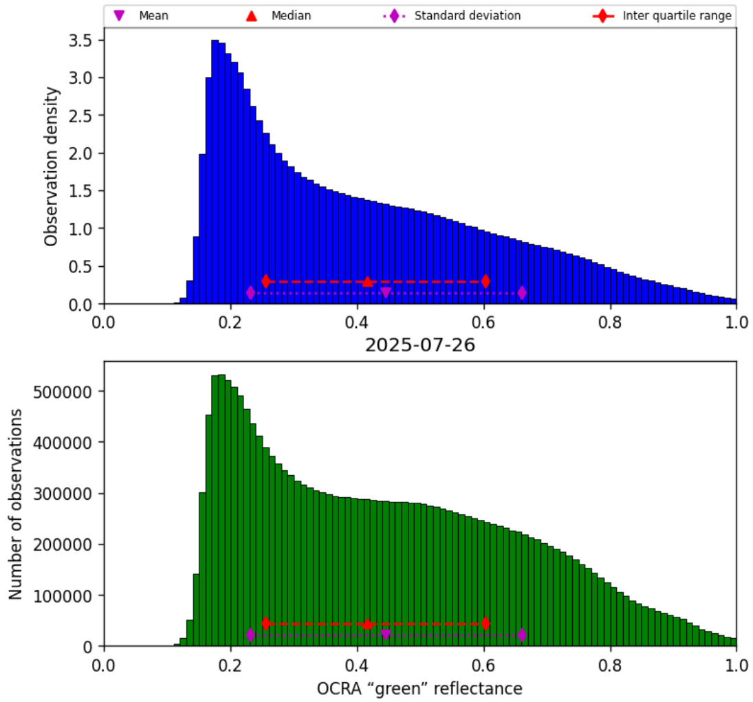
Figure 52: Histogram of “OCRA “green” reflectance” for 2025-07-25 to 2025-07-27
