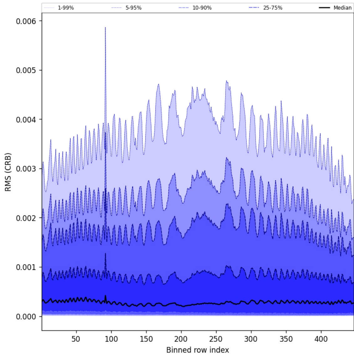
Figure 64: Along track statistics of “RMS (CRB)” for 2025-07-25 to 2025-07-27
