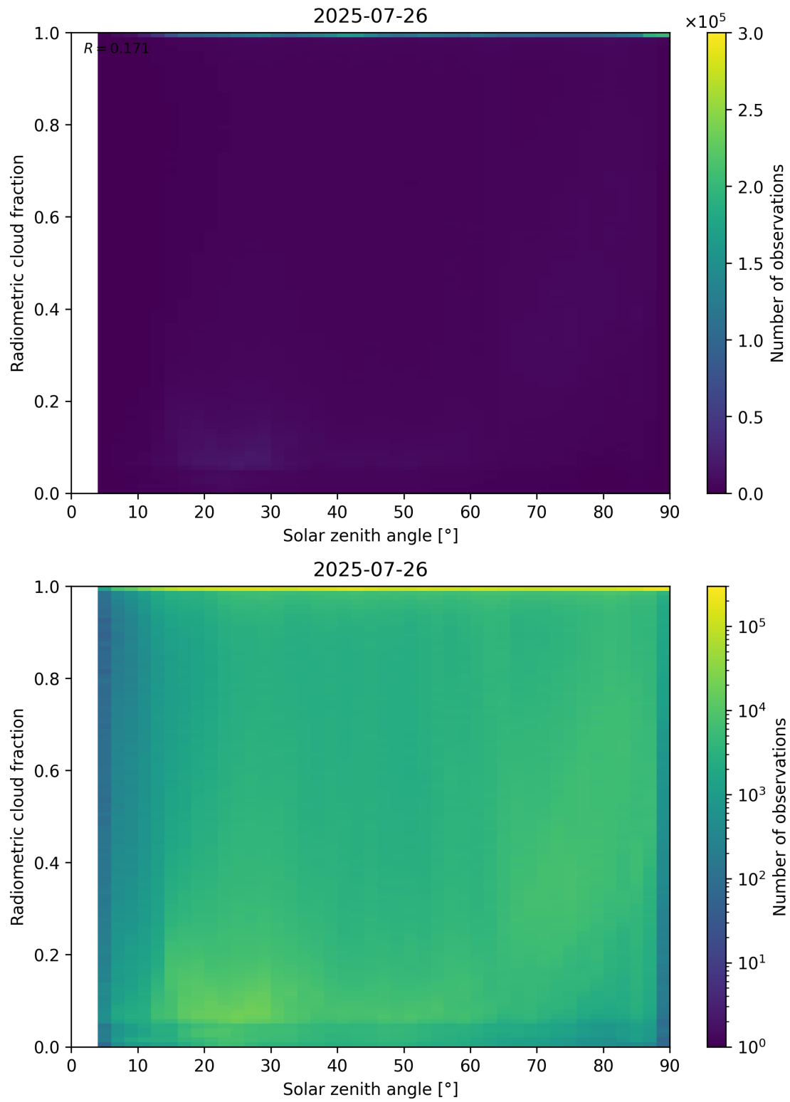
Figure 99: Scatter density plot of “Solar zenith angle” against “Radiometric cloud fraction” for 2025-07-25 to 2025-07-27.
