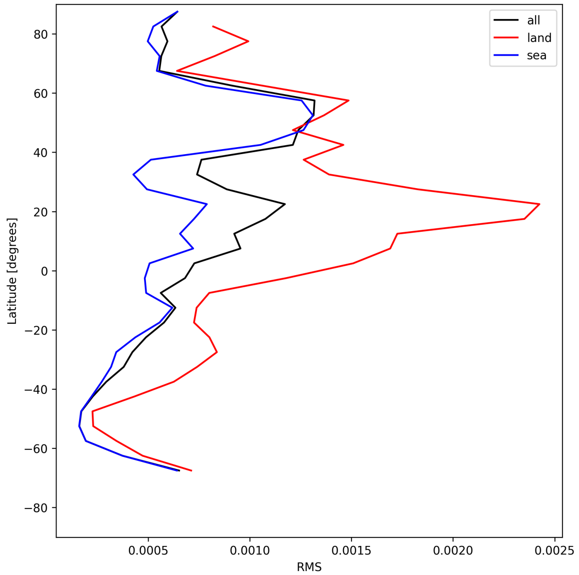
Figure 31: Zonal average of “RMS” for 2025-07-25 to 2025-07-27.
