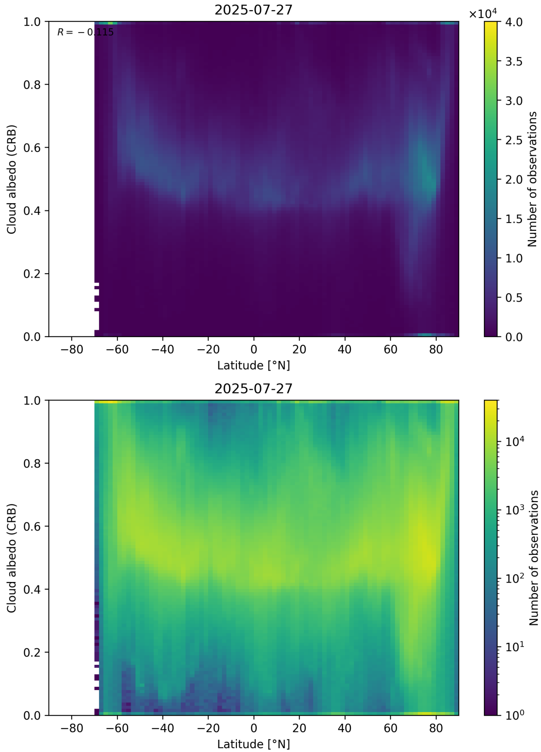
Figure 91: Scatter density plot of “Latitude” against “Cloud albedo (CRB)” for 2025-07-26 to 2025-07-28.
