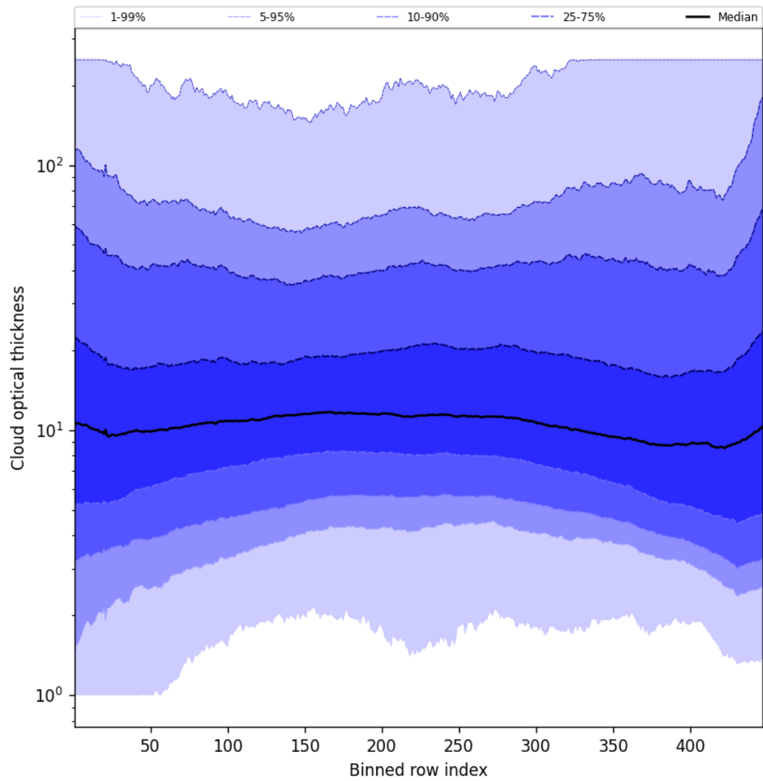
Figure 57: Along track statistics of “Cloud optical thickness” for 2025-07-26 to 2025-07-28
