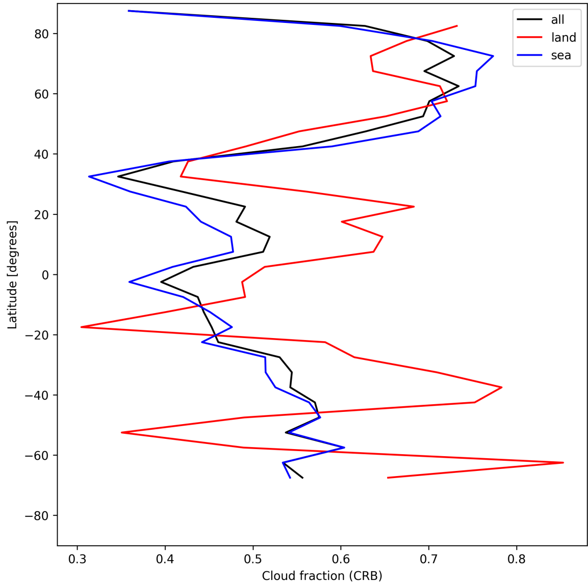
Figure 26: Zonal average of “Cloud fraction (CRB)” for 2025-07-26 to 2025-07-28.
