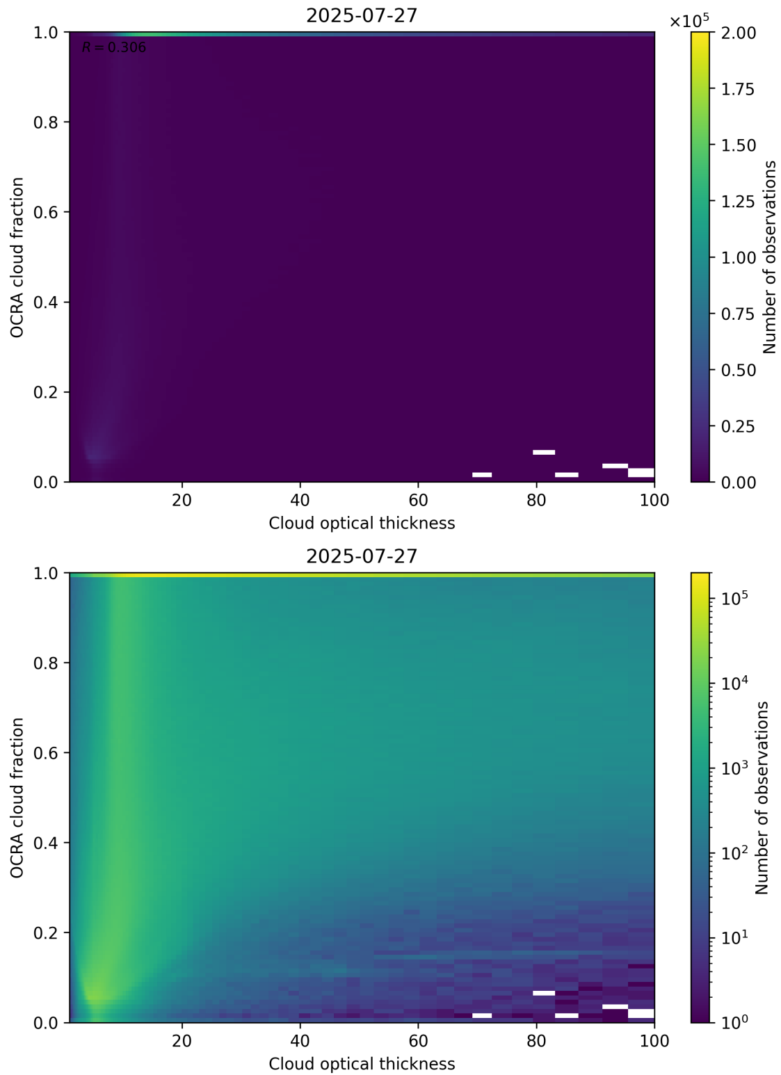
Figure 83: Scatter density plot of “Cloud optical thickness” against “OCRA cloud fraction” for 2025-07-26 to 2025-07-28.
