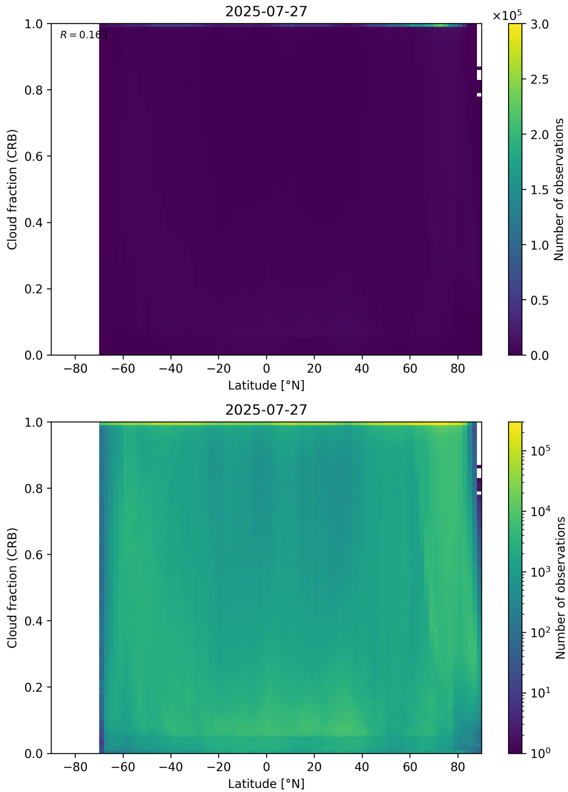
Figure 94: Scatter density plot of “Latitude” against “Cloud fraction (CRB)” for 2025-07-26 to 2025-07-28.
