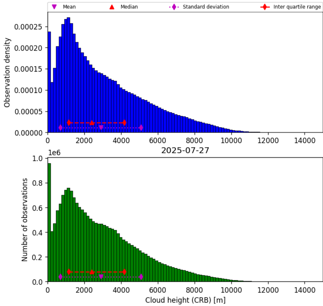
Figure 43: Histogram of “Cloud height (CRB)” for 2025-07-26 to 2025-07-28
