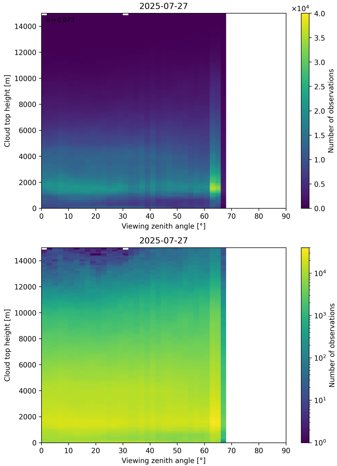
Figure 112: Scatter density plot of “Viewing zenith angle” against “Cloud top height” for 2025-07-26 to 2025-07-28.
