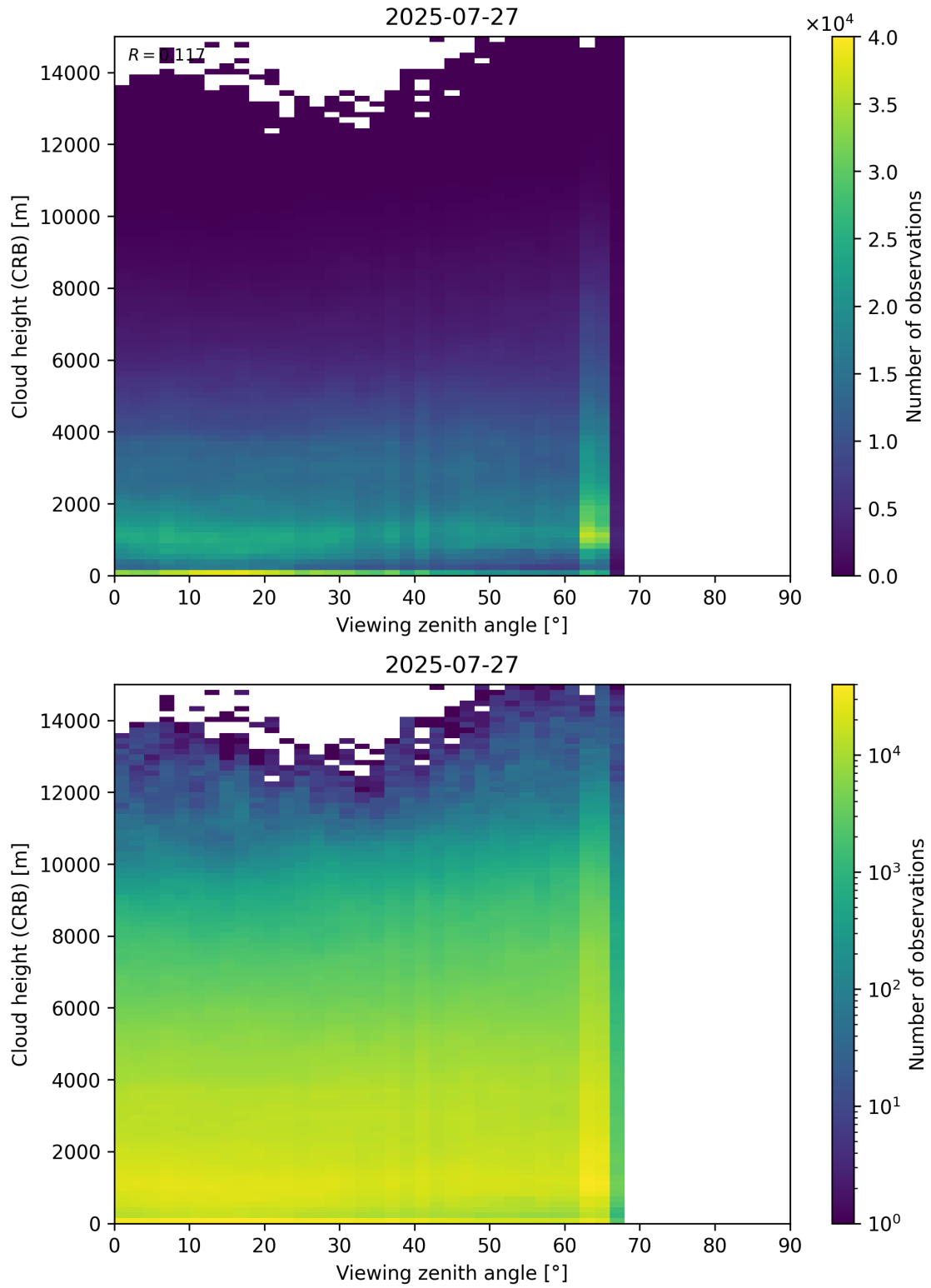
Figure 110: Scatter density plot of “Viewing zenith angle” against “Cloud height (CRB)” for 2025-07-26 to 2025-07-28.
