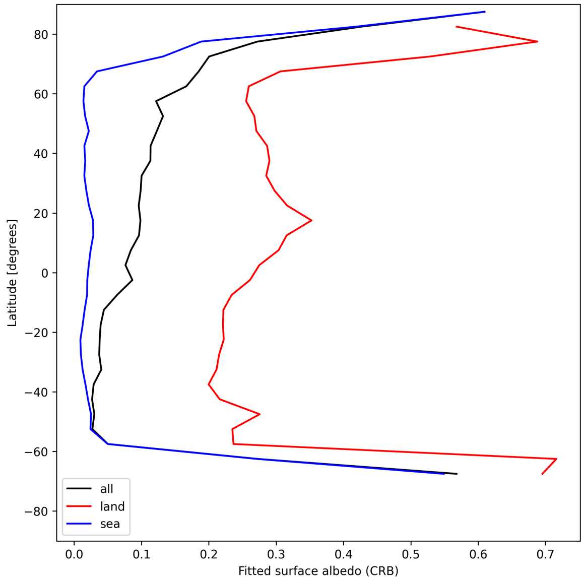
Figure 30: Zonal average of “Fitted surface albedo (CRB)” for 2025-07-26 to 2025-07-28.
