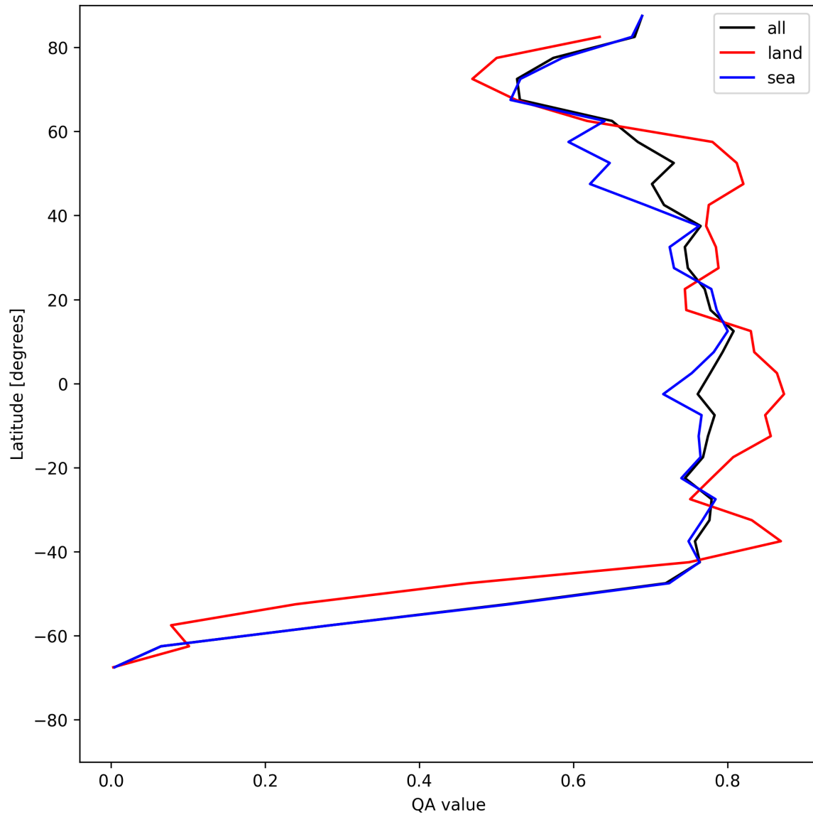
Figure 22: Zonal average of “QA value” for 2025-07-26 to 2025-07-28.
