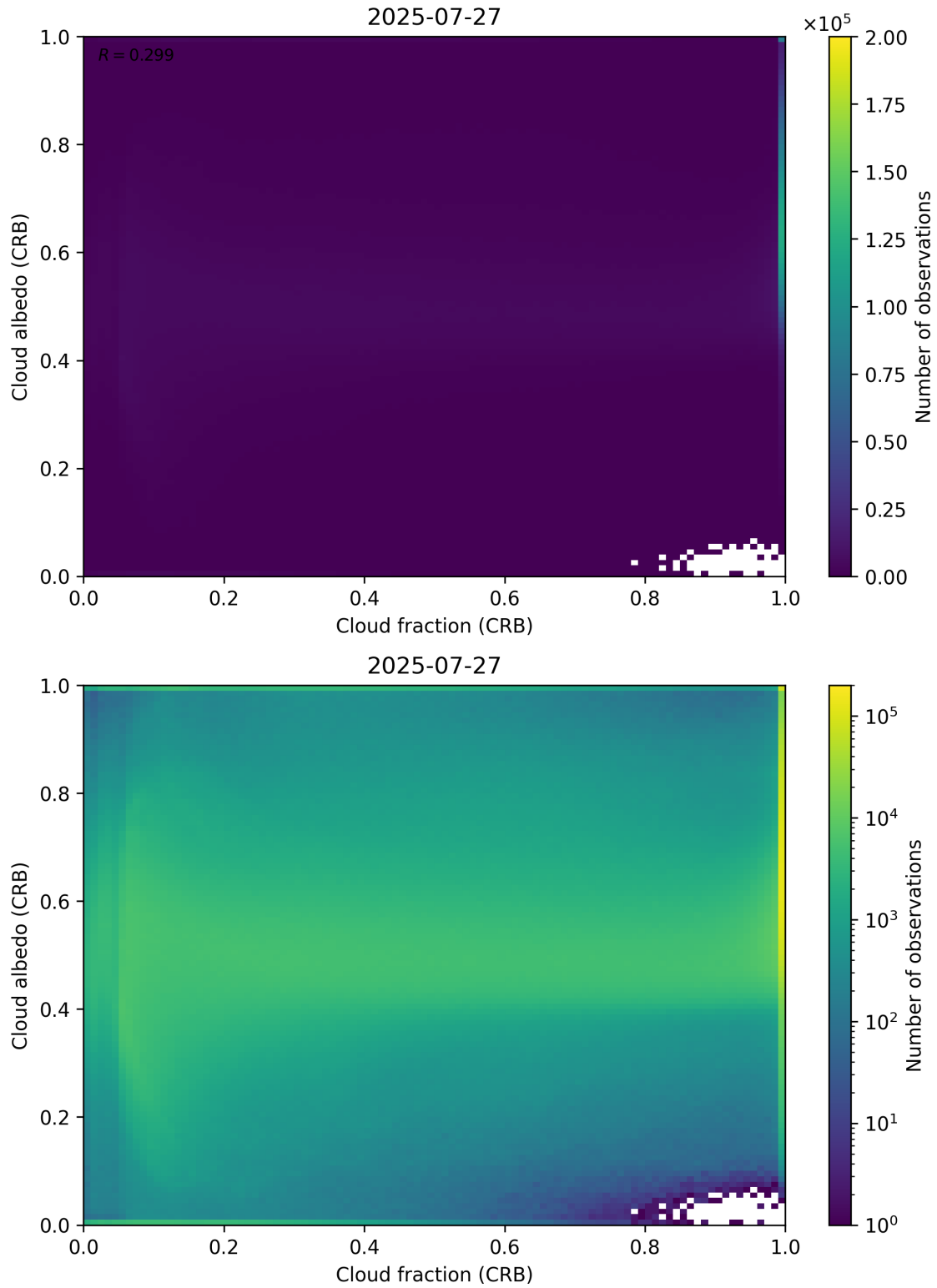
Figure 77: Scatter density plot of “Cloud fraction (CRB)” against “Cloud albedo (CRB)” for 2025-07-26 to 2025-07-28.
