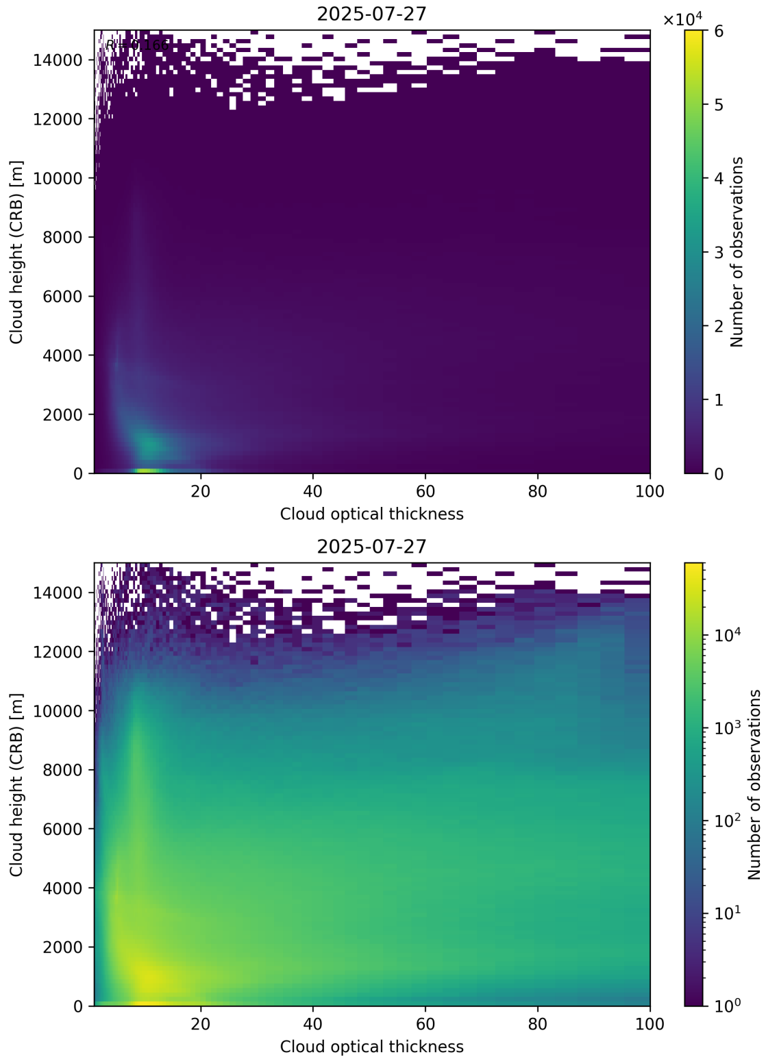
Figure 85: Scatter density plot of “Cloud optical thickness” against “Cloud height (CRB)” for 2025-07-26 to 2025-07-28.
