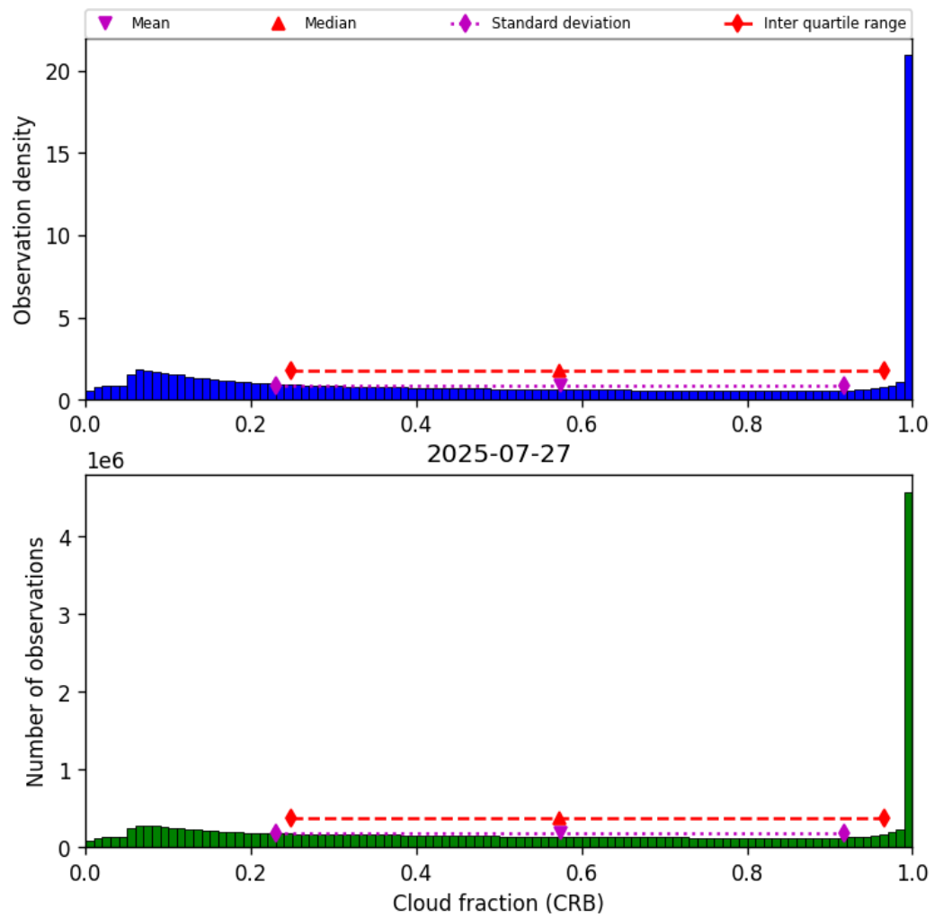
Figure 42: Histogram of “Cloud fraction (CRB)” for 2025-07-26 to 2025-07-28
