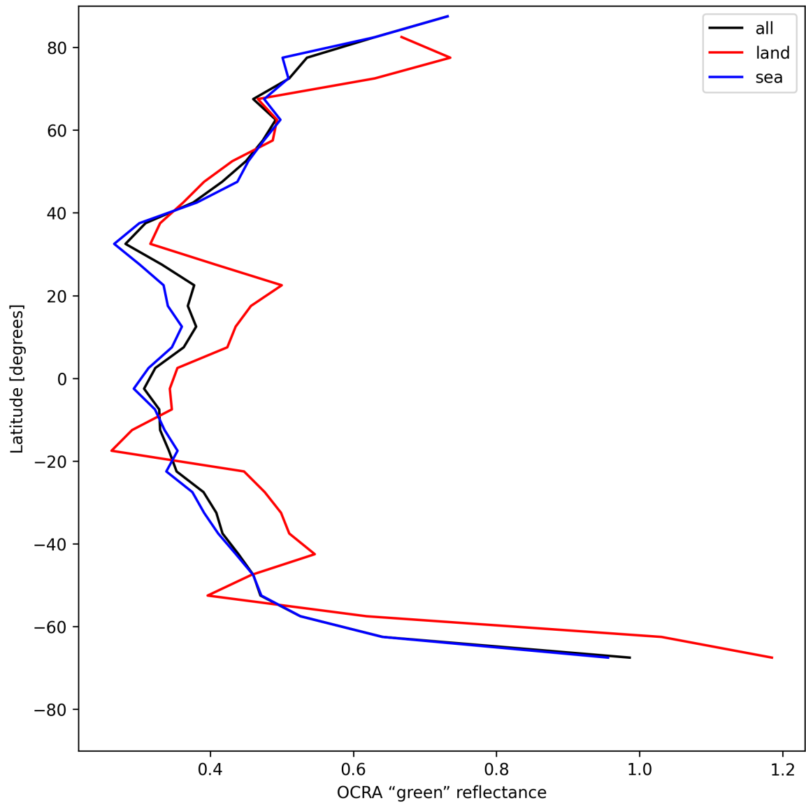
Figure 36: Zonal average of “OCRA “green” reflectance” for 2025-07-26 to 2025-07-28.
