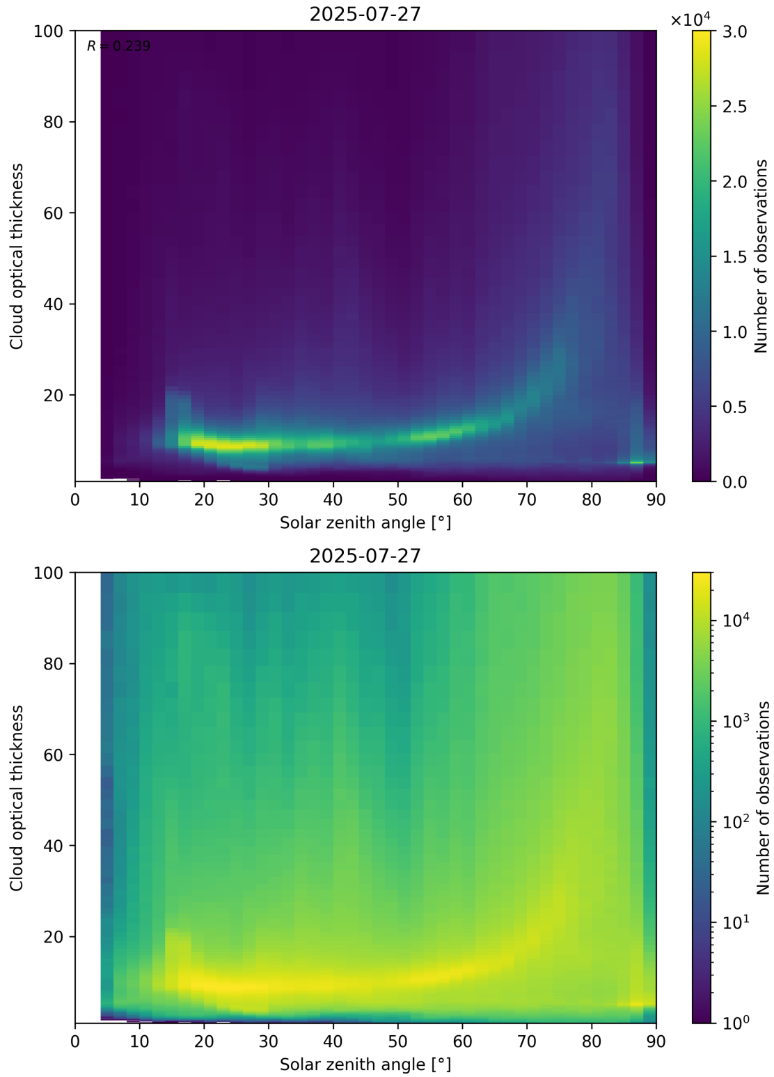
Figure 103: Scatter density plot of “Solar zenith angle” against “Cloud optical thickness” for 2025-07-26 to 2025-07-28.
