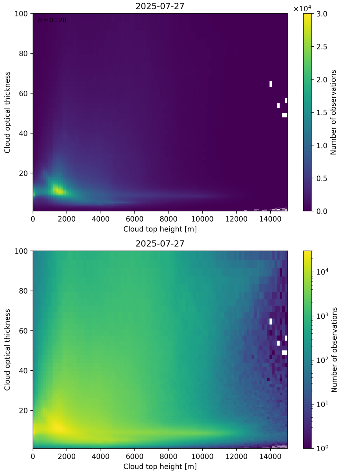
Figure 90: Scatter density plot of “Cloud top height” against “Cloud optical thickness” for 2025-07-26 to 2025-07-28.
