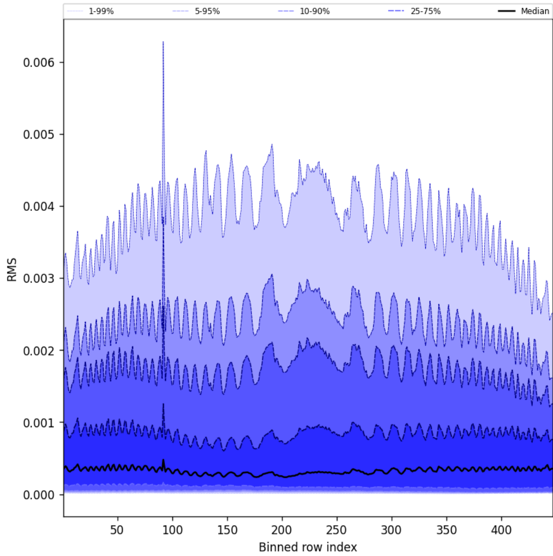
Figure 63: Along track statistics of “RMS” for 2025-07-26 to 2025-07-28
