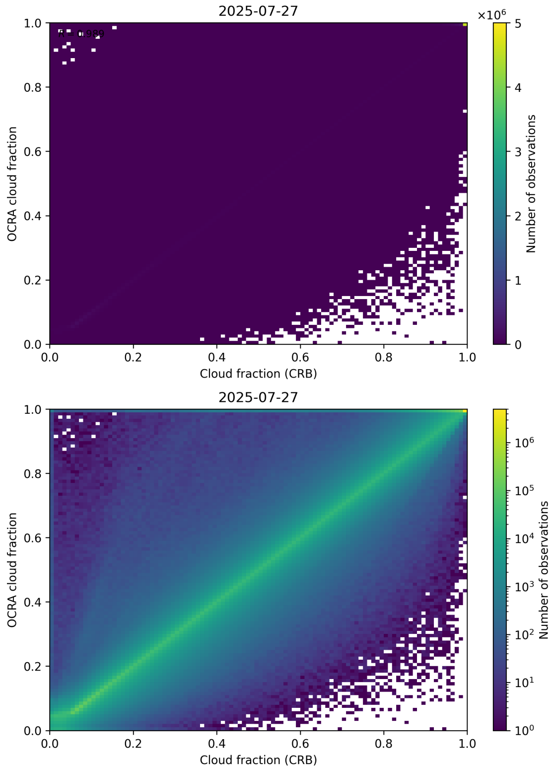
Figure 78: Scatter density plot of “Cloud fraction (CRB)” against “OCRA cloud fraction” for 2025-07-26 to 2025-07-28.
