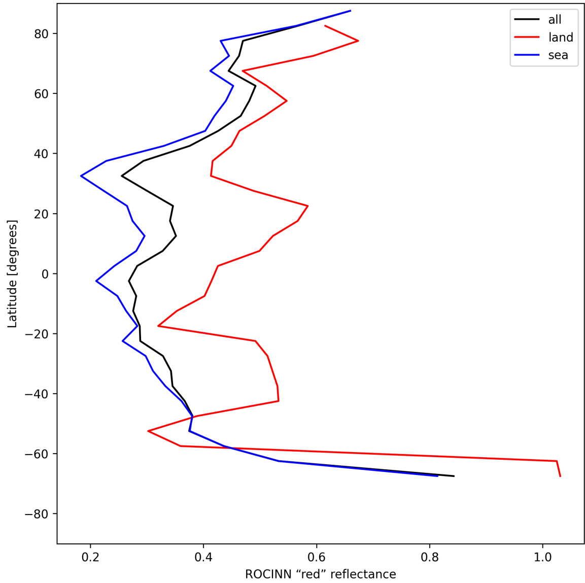
Figure 37: Zonal average of “ROCINN “red” reflectance” for 2025-07-26 to 2025-07-28.
