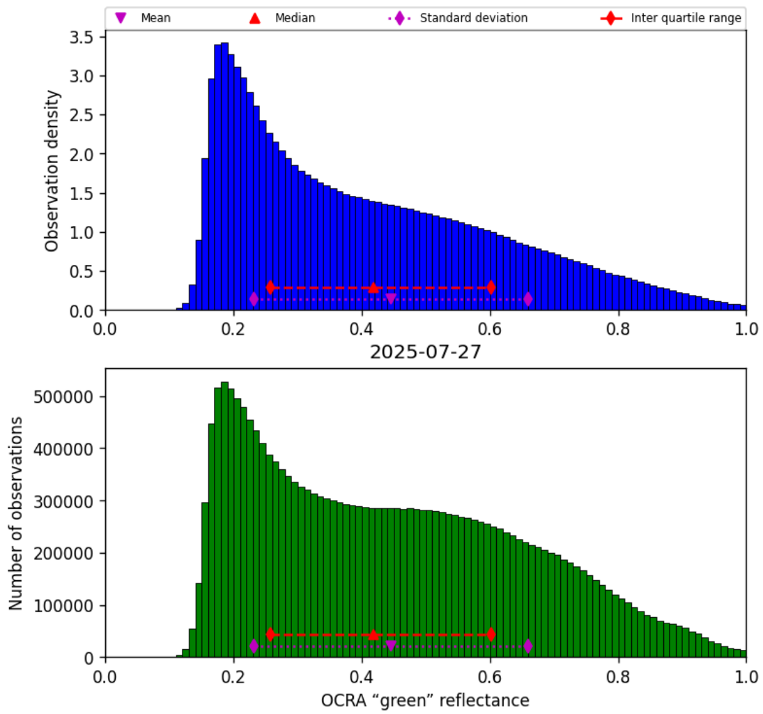
Figure 52: Histogram of “OCRA “green” reflectance” for 2025-07-26 to 2025-07-28
