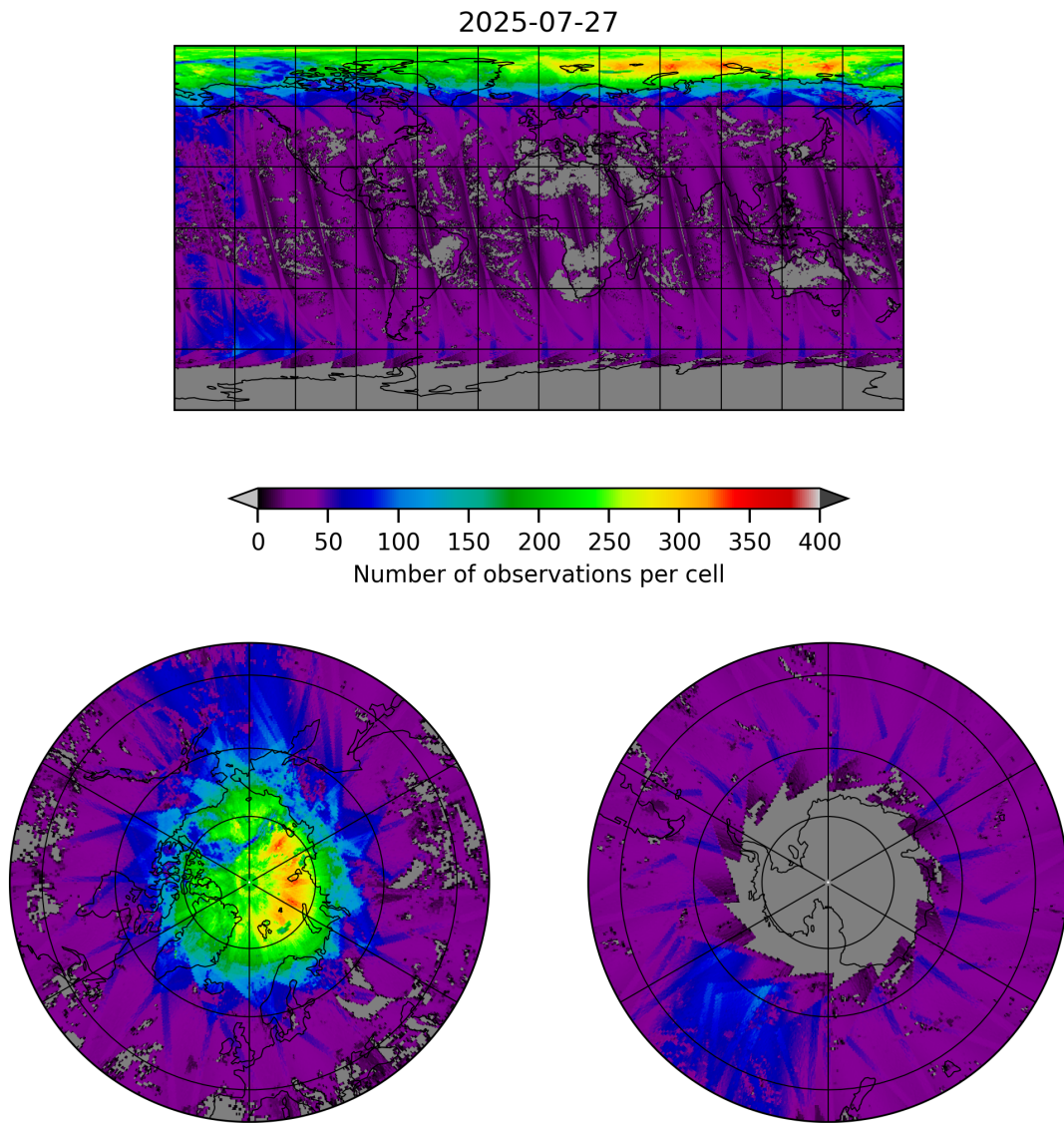
Figure 21: Map of the number of observations for 2025-07-26 to 2025-07-28
