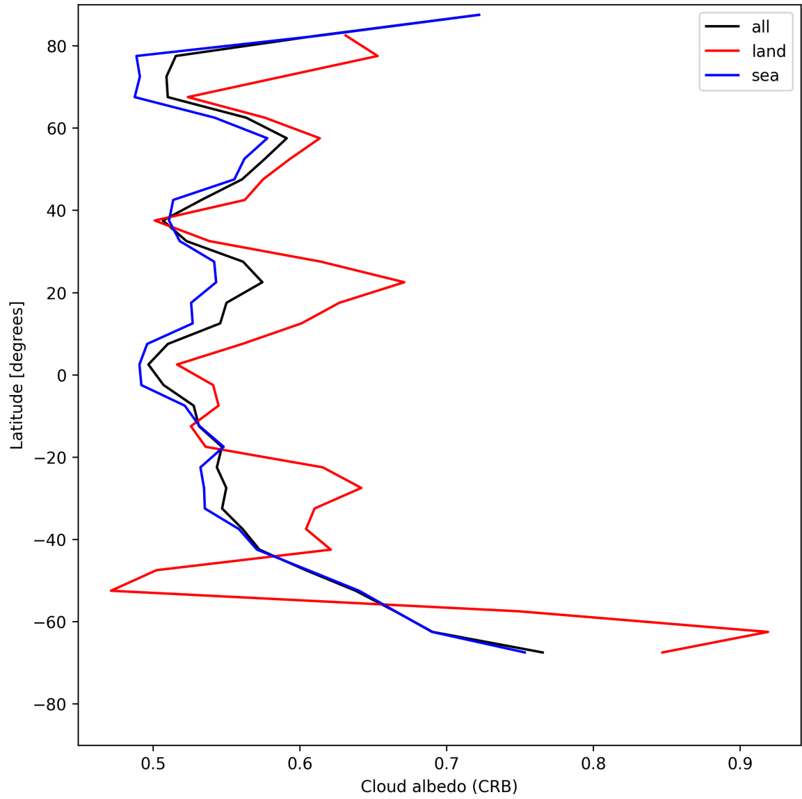
Figure 28: Zonal average of “Cloud albedo (CRB)” for 2025-07-26 to 2025-07-28.
