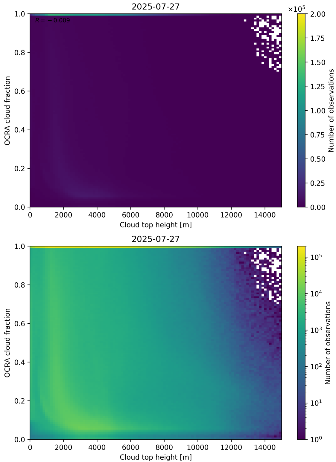
Figure 87: Scatter density plot of “Cloud top height” against “OCRA cloud fraction” for 2025-07-26 to 2025-07-28.
