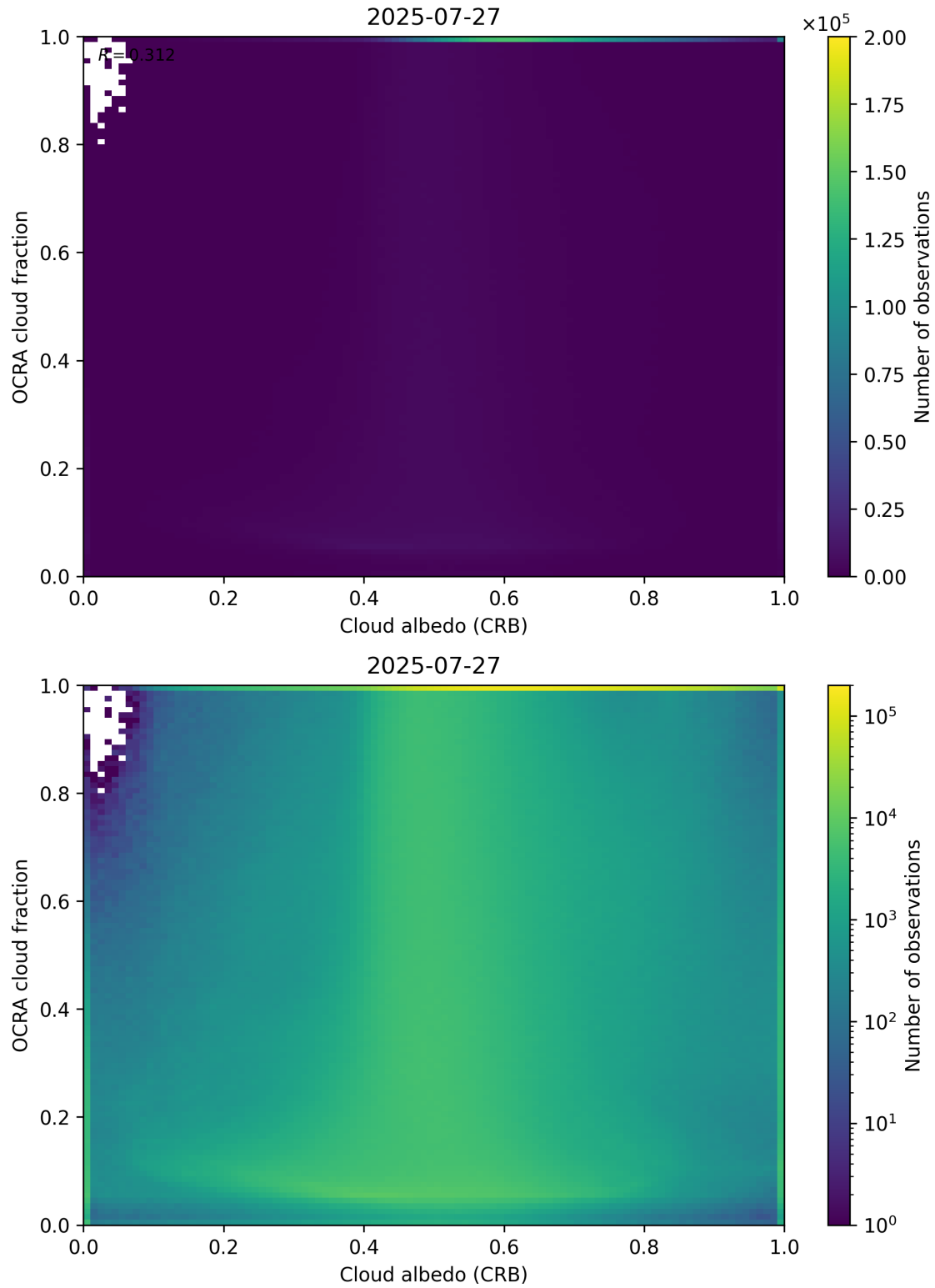
Figure 70: Scatter density plot of “Cloud albedo (CRB)” against “OCRA cloud fraction” for 2025-07-26 to 2025-07-28.
