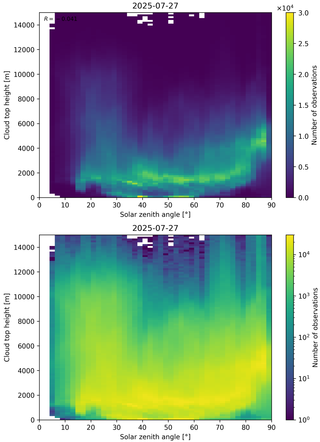
Figure 104: Scatter density plot of “Solar zenith angle” against “Cloud top height” for 2025-07-26 to 2025-07-28.
