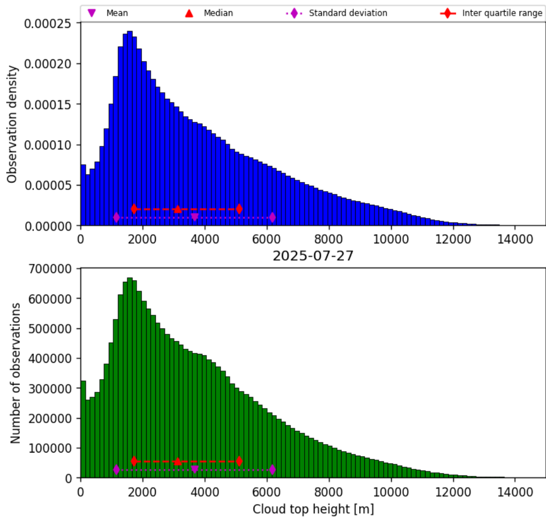
Figure 40: Histogram of “Cloud top height” for 2025-07-26 to 2025-07-28
