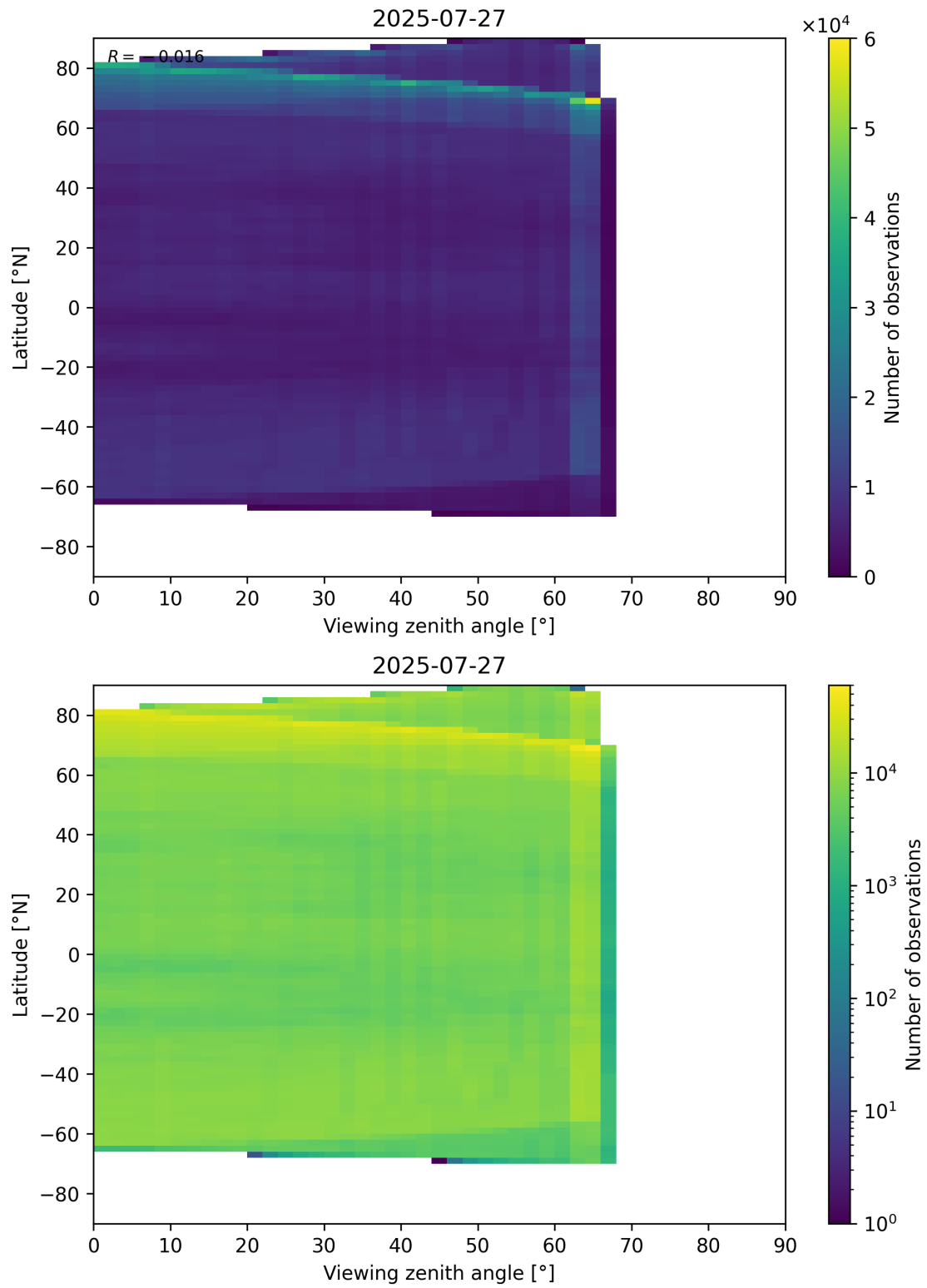
Figure 113: Scatter density plot of “Viewing zenith angle” against “Latitude” for 2025-07-26 to 2025-07-28.
