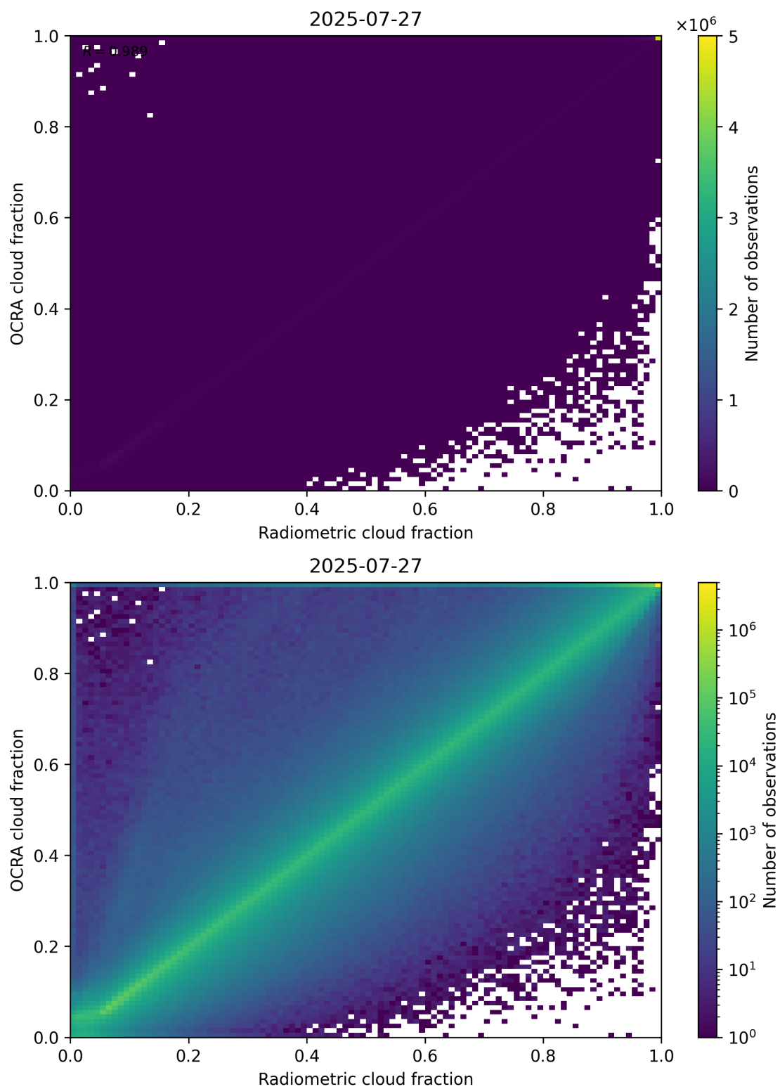
Figure 72: Scatter density plot of “Radiometric cloud fraction” against “OCRA cloud fraction” for 2025-07-26 to 2025-07-28.
