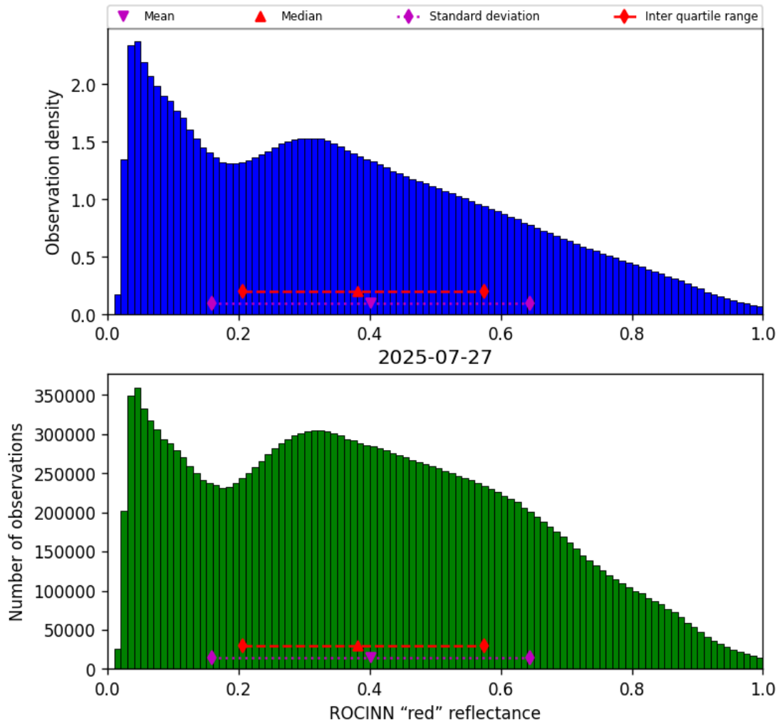
Figure 53: Histogram of “ROCINN “red” reflectance” for 2025-07-26 to 2025-07-28
