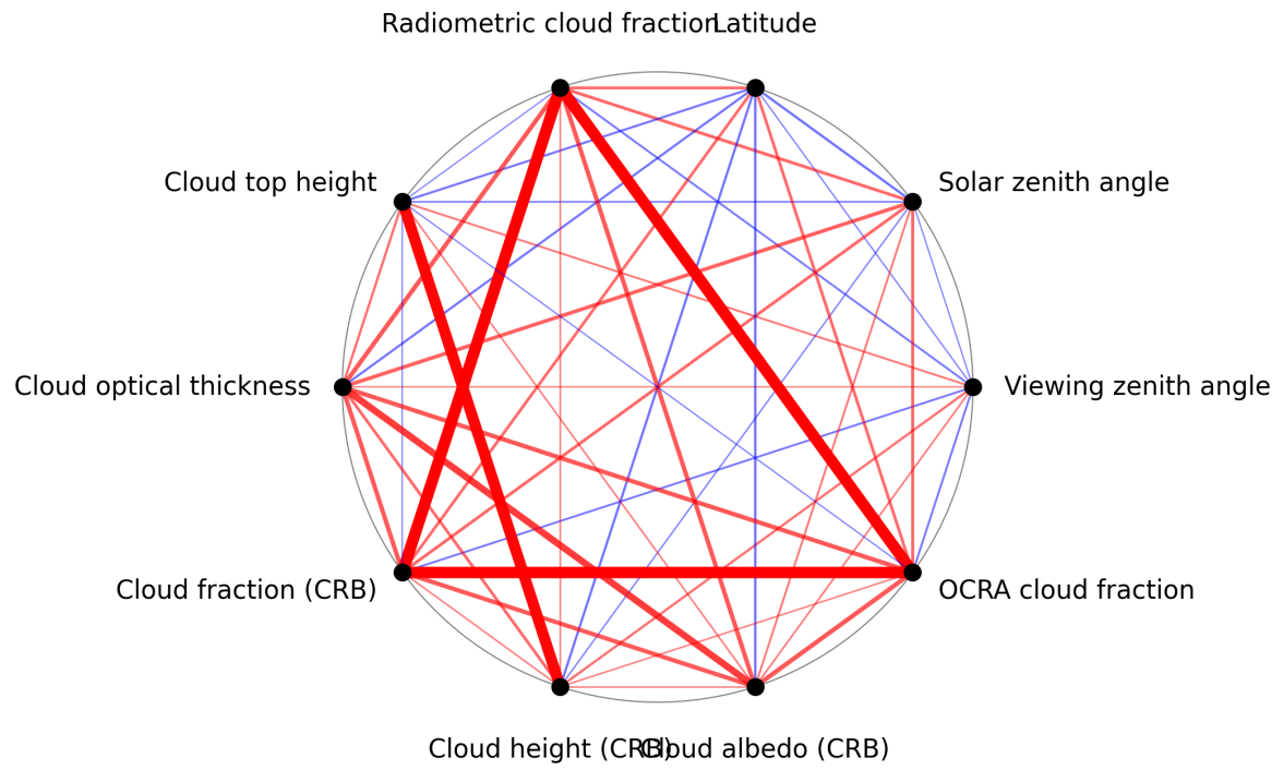
Figure 1: Map of correlation graph for 2025-07-26 to 2025-07-28.
