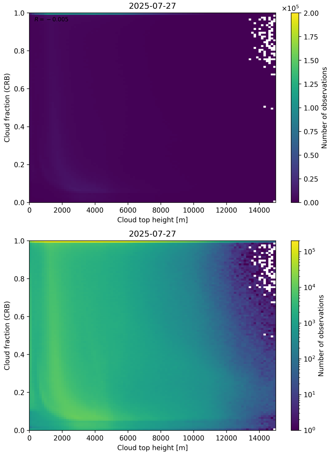
Figure 88: Scatter density plot of “Cloud top height” against “Cloud fraction (CRB)” for 2025-07-26 to 2025-07-28.
