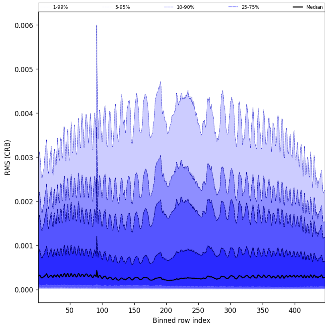
Figure 64: Along track statistics of “RMS (CRB)” for 2025-07-26 to 2025-07-28
