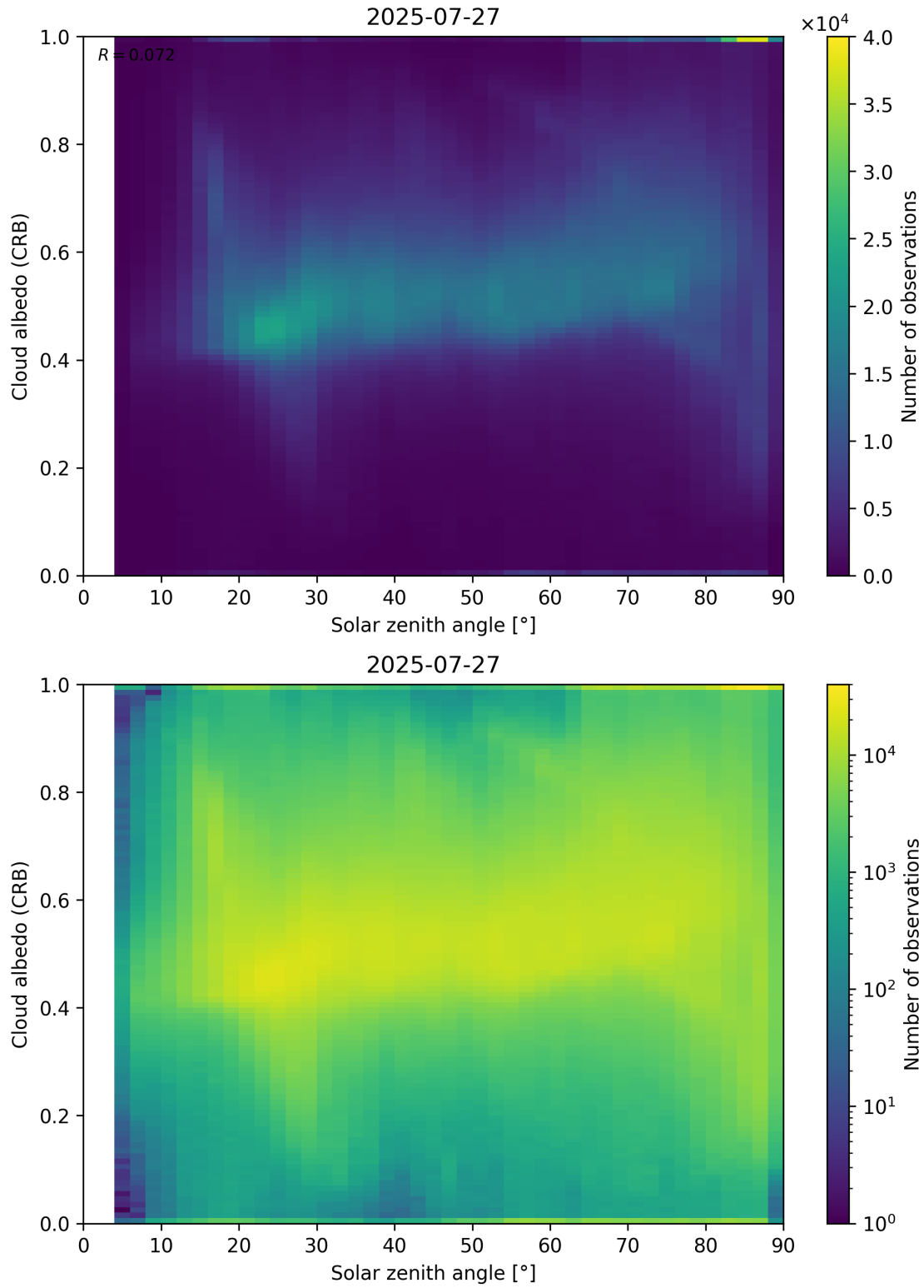
Figure 98: Scatter density plot of “Solar zenith angle” against “Cloud albedo (CRB)” for 2025-07-26 to 2025-07-28.
