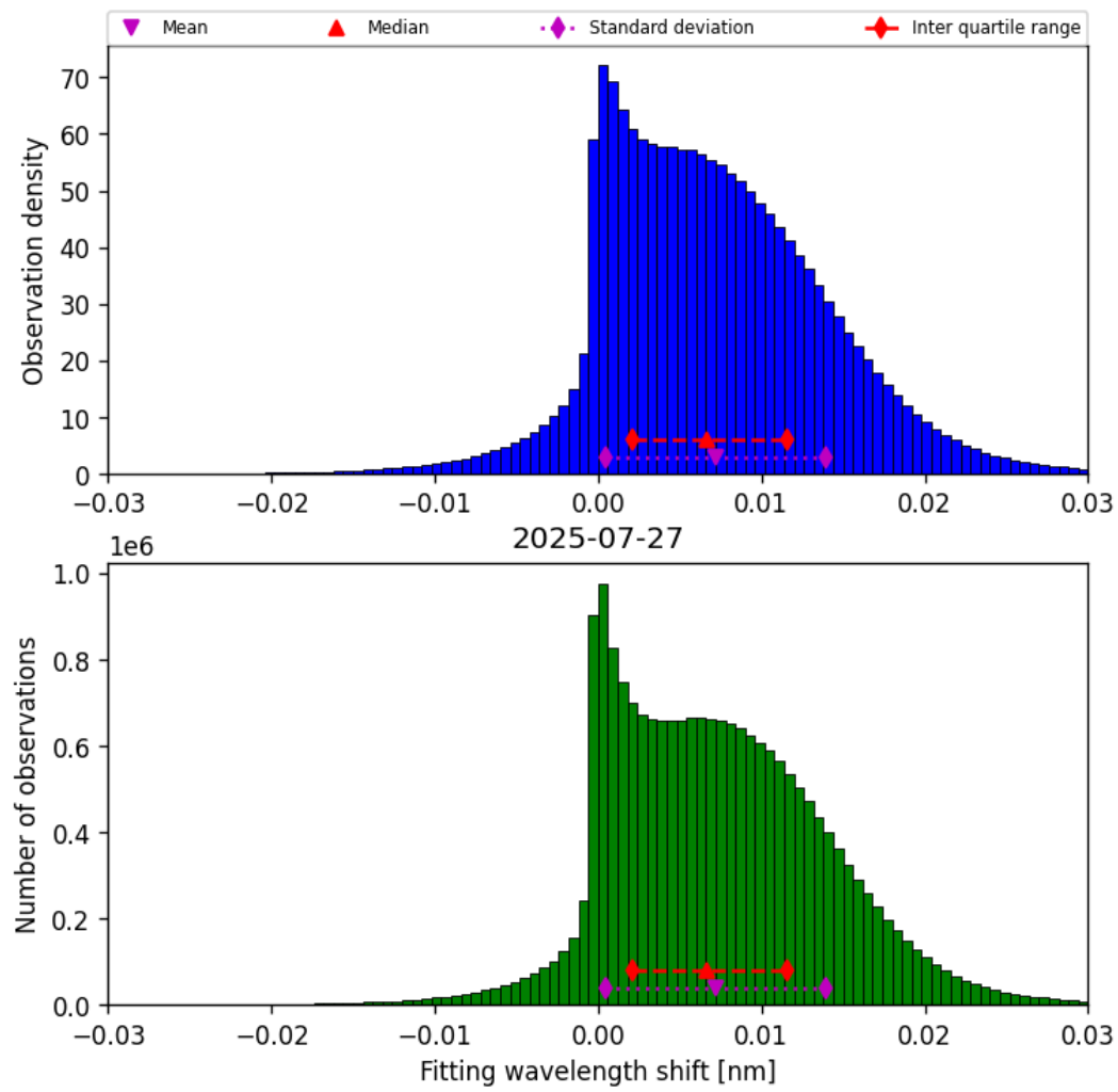
Figure 49: Histogram of “Fitting wavelength shift” for 2025-07-26 to 2025-07-28
