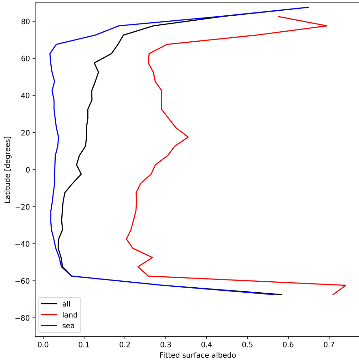
Figure 29: Zonal average of “Fitted surface albedo” for 2025-07-26 to 2025-07-28.
