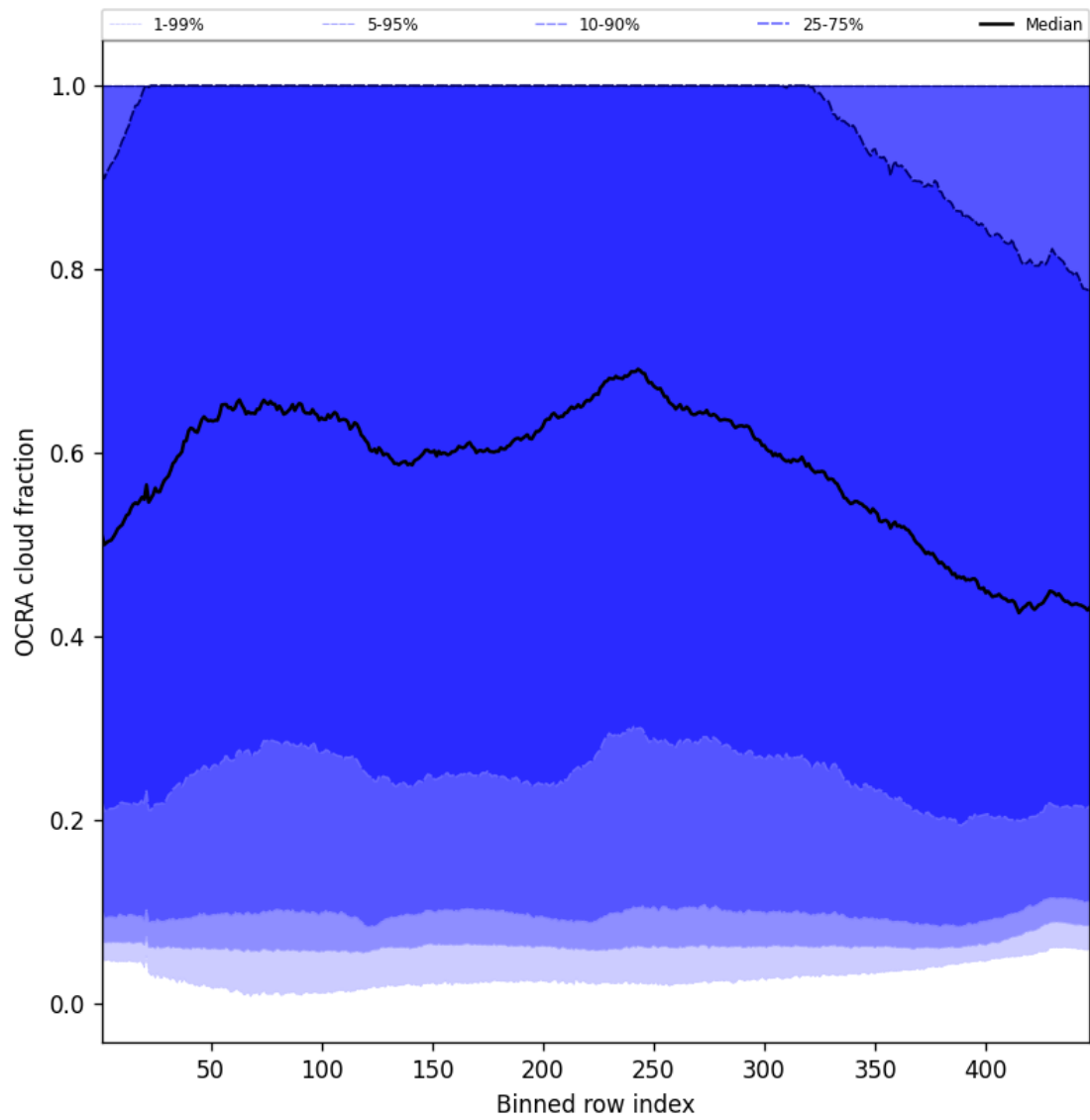
Figure 66: Along track statistics of “OCRA cloud fraction” for 2025-07-26 to 2025-07-28
