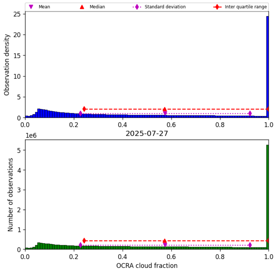
Figure 50: Histogram of “OCRA cloud fraction” for 2025-07-26 to 2025-07-28
