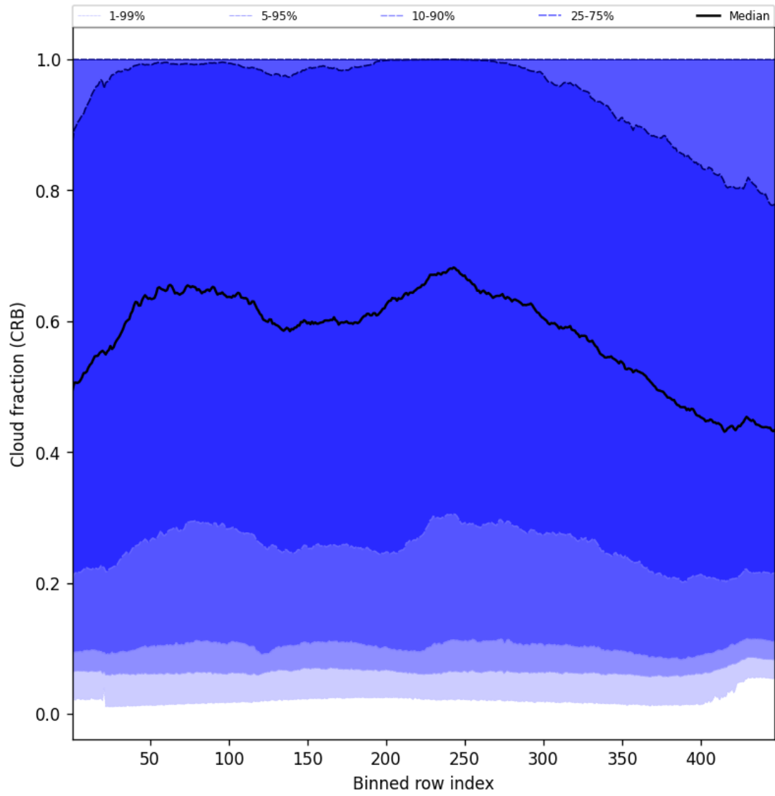
Figure 58: Along track statistics of “Cloud fraction (CRB)” for 2025-07-26 to 2025-07-28
