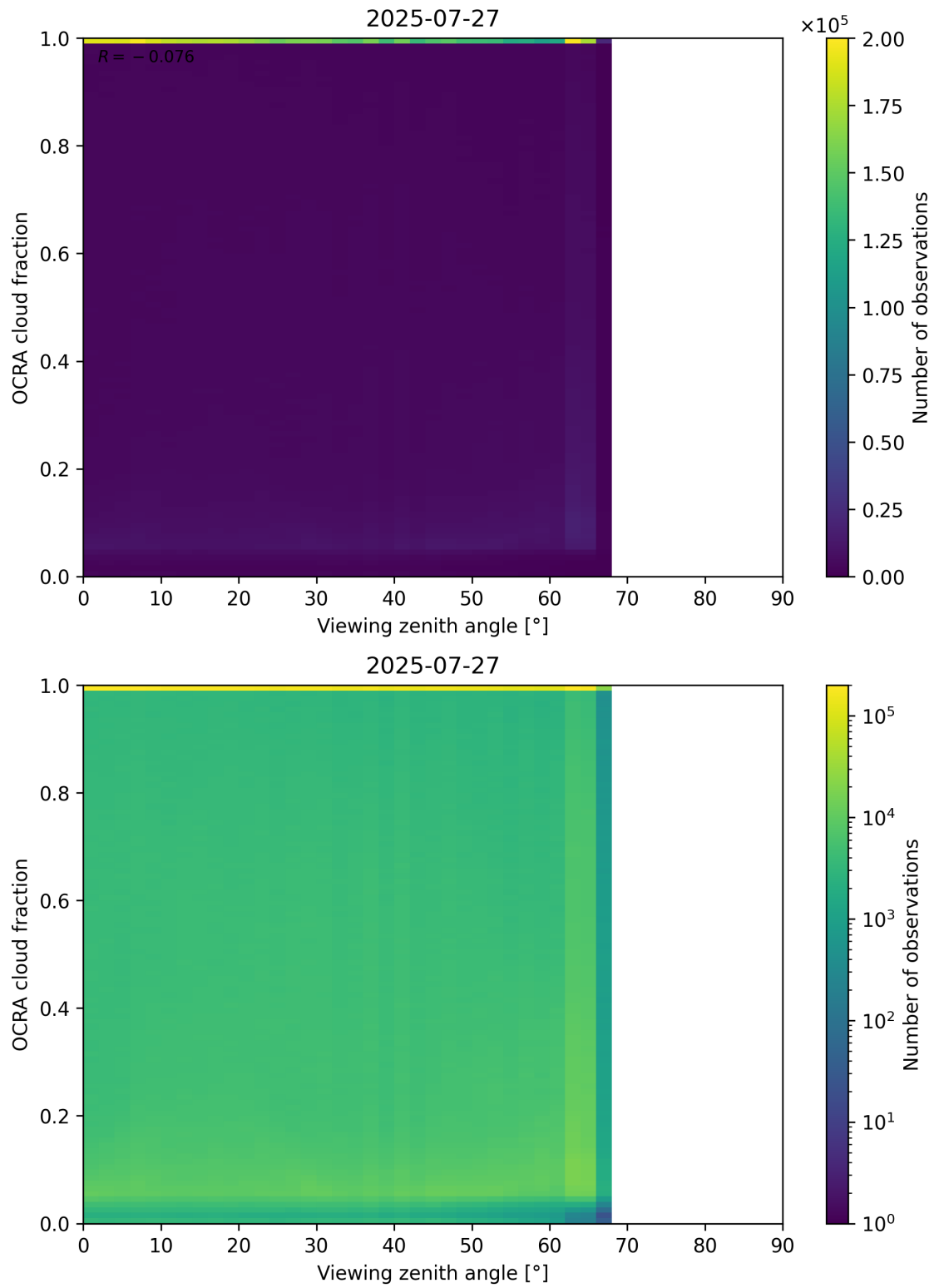
Figure 108: Scatter density plot of “Viewing zenith angle” against “OCRA cloud fraction” for 2025-07-26 to 2025-07-28.
