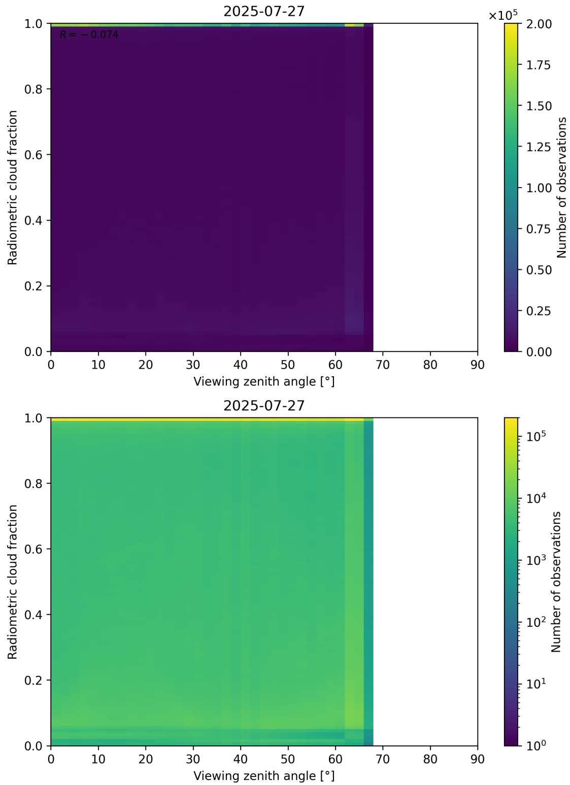
Figure 107: Scatter density plot of “Viewing zenith angle” against “Radiometric cloud fraction” for 2025-07-26 to 2025-07-28.
