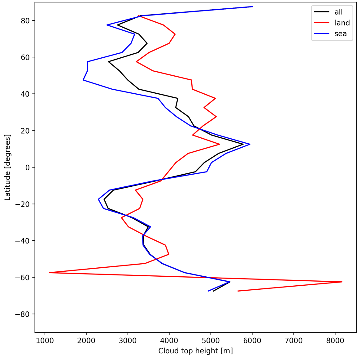
Figure 24: Zonal average of “Cloud top height” for 2025-07-26 to 2025-07-28.
