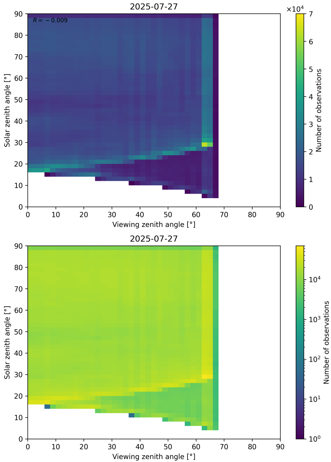
Figure 114: Scatter density plot of “Viewing zenith angle” against “Solar zenith angle” for 2025-07-26 to 2025-07-28.
