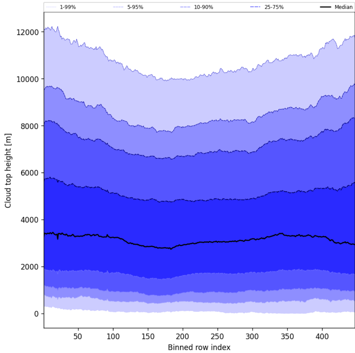
Figure 56: Along track statistics of “Cloud top height” for 2025-07-26 to 2025-07-28
