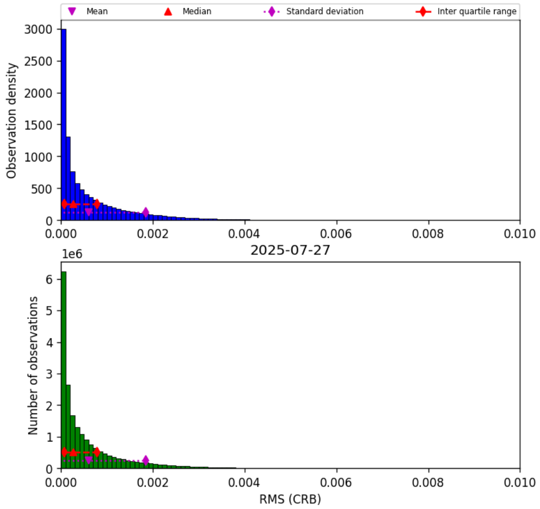
Figure 48: Histogram of “RMS (CRB)” for 2025-07-26 to 2025-07-28
