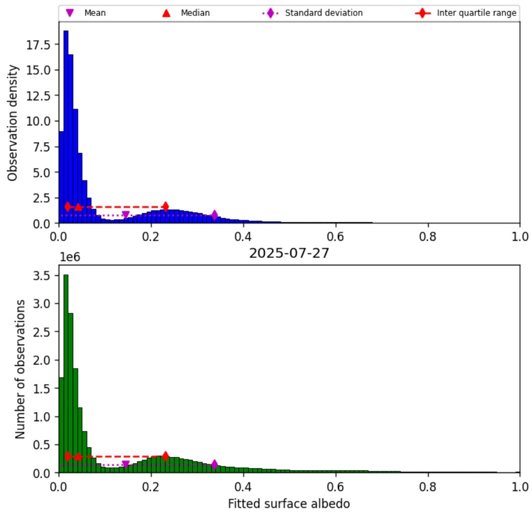
Figure 45: Histogram of “Fitted surface albedo” for 2025-07-26 to 2025-07-28
