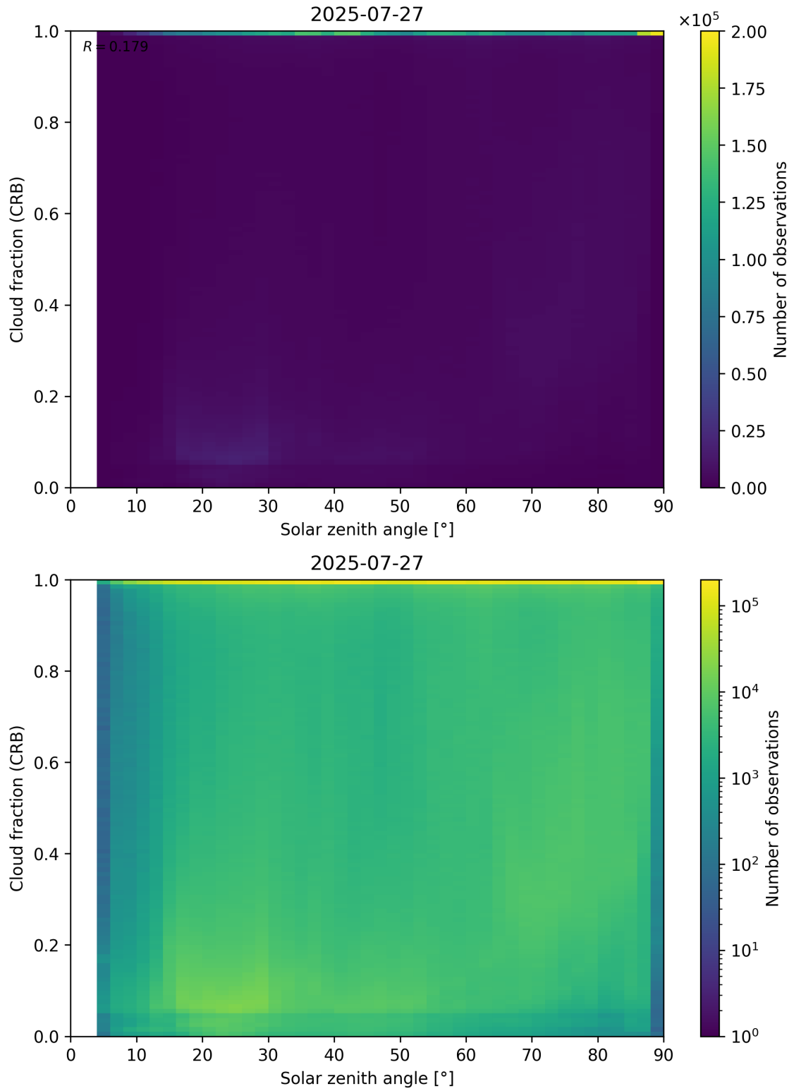
Figure 101: Scatter density plot of “Solar zenith angle” against “Cloud fraction (CRB)” for 2025-07-26 to 2025-07-28.
