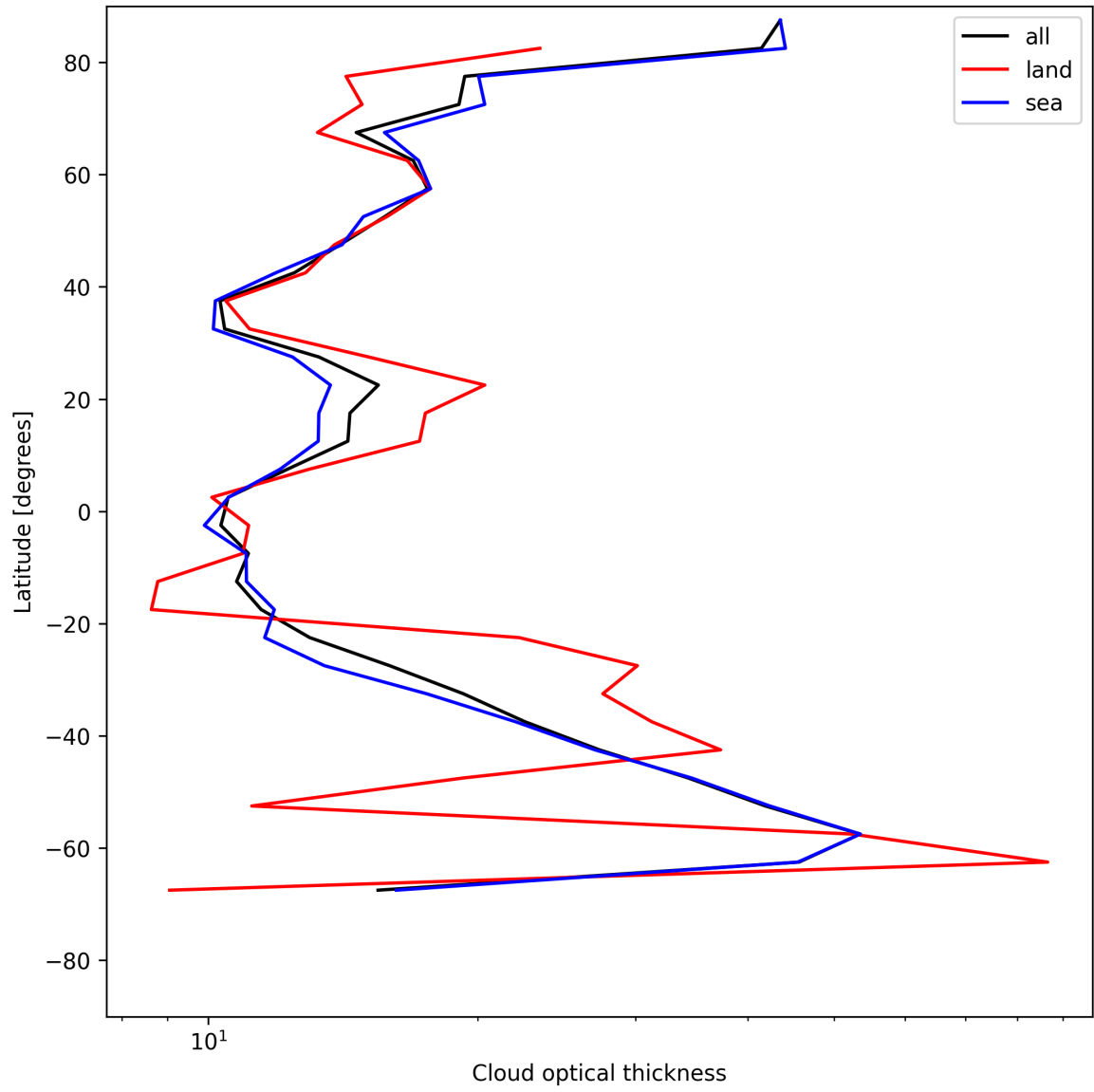
Figure 25: Zonal average of “Cloud optical thickness” for 2025-07-26 to 2025-07-28.
