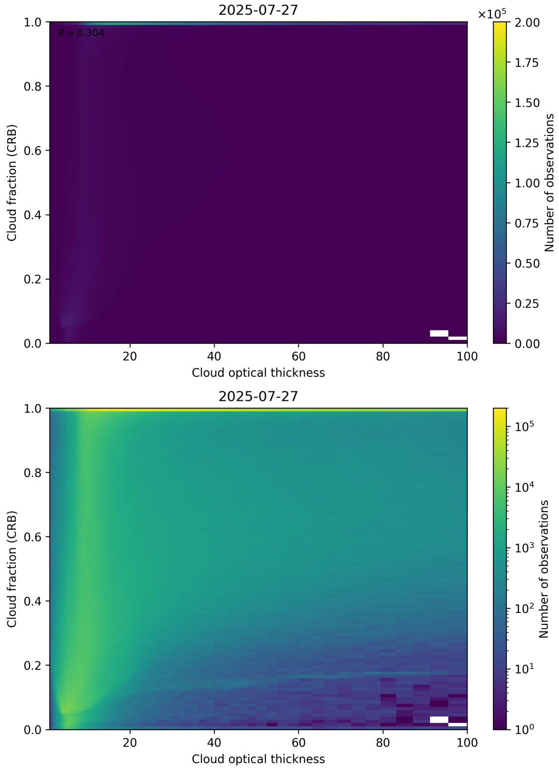
Figure 84: Scatter density plot of “Cloud optical thickness” against “Cloud fraction (CRB)” for 2025-07-26 to 2025-07-28.
