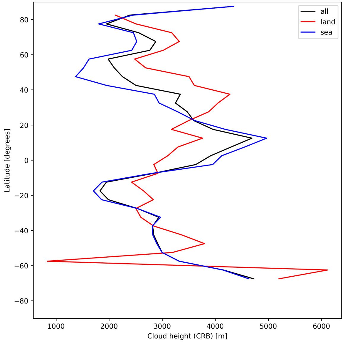
Figure 27: Zonal average of “Cloud height (CRB)” for 2025-07-26 to 2025-07-28.
