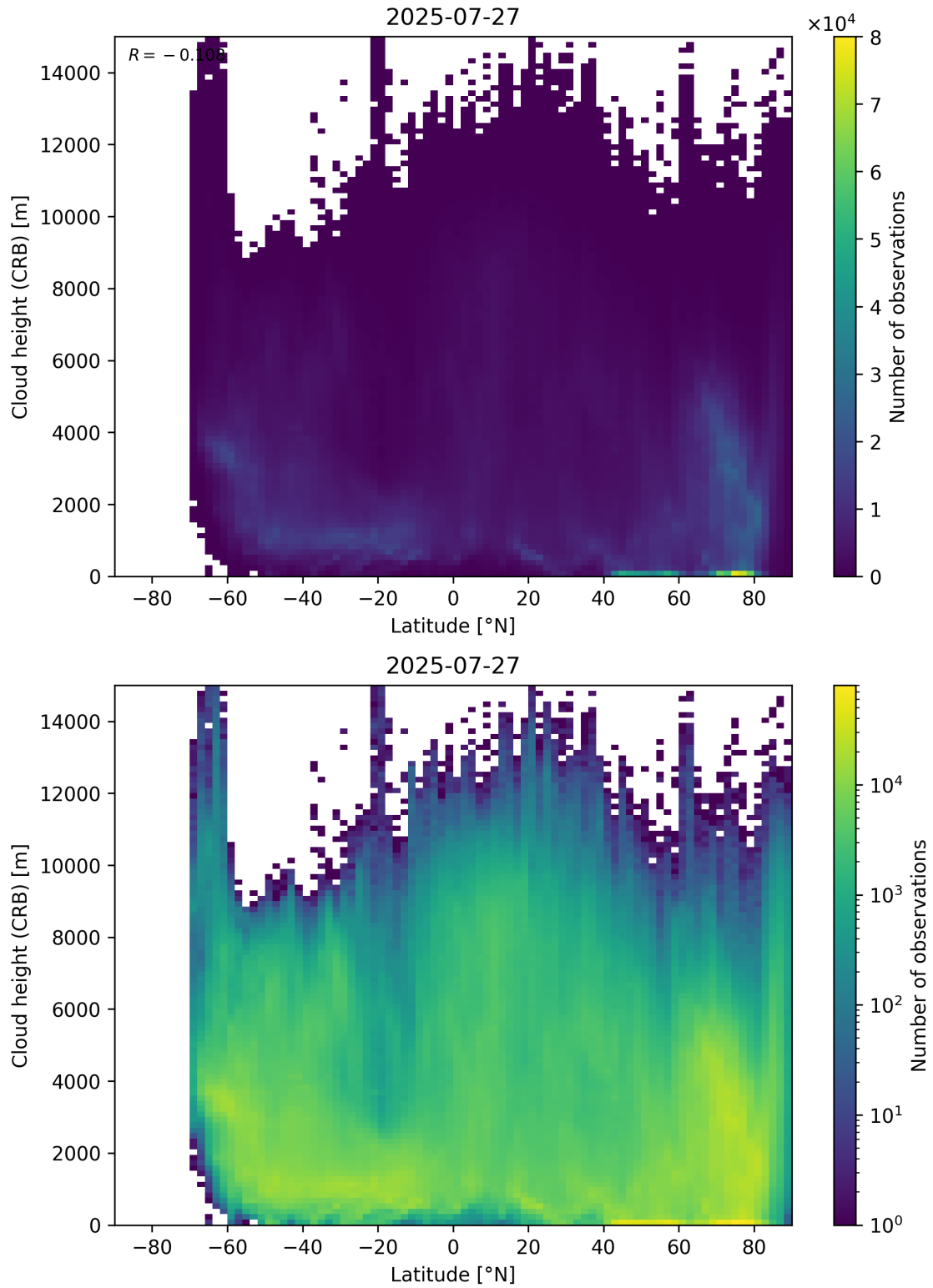
Figure 95: Scatter density plot of “Latitude” against “Cloud height (CRB)” for 2025-07-26 to 2025-07-28.
