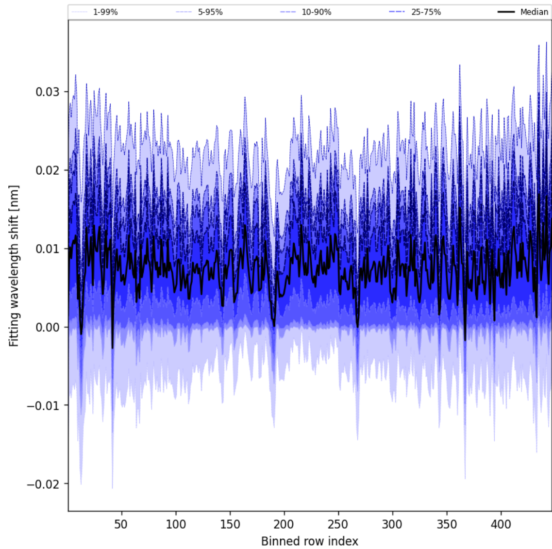
Figure 65: Along track statistics of “Fitting wavelength shift” for 2025-07-26 to 2025-07-28
