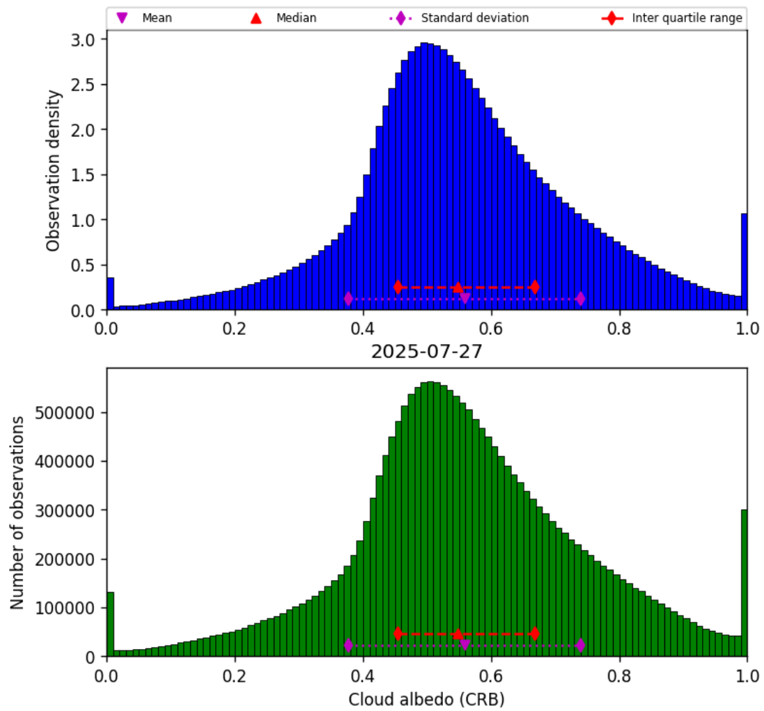
Figure 44: Histogram of “Cloud albedo (CRB)” for 2025-07-26 to 2025-07-28
