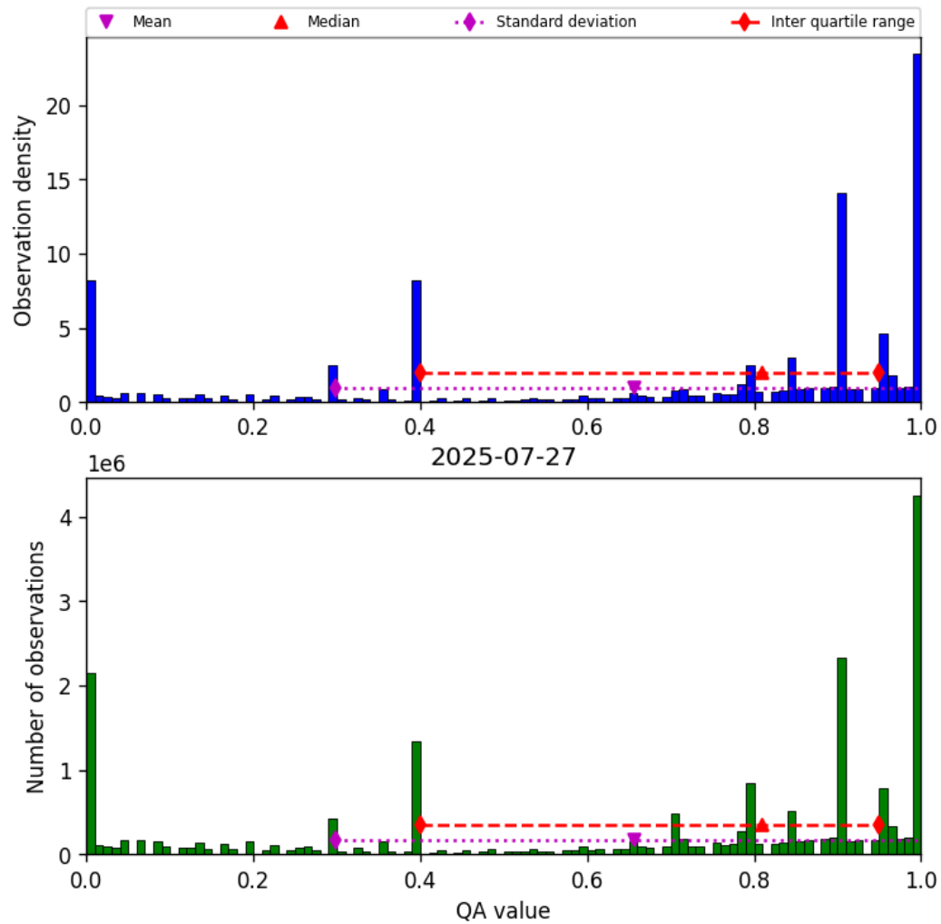
Figure 38: Histogram of “QA value” for 2025-07-26 to 2025-07-28
