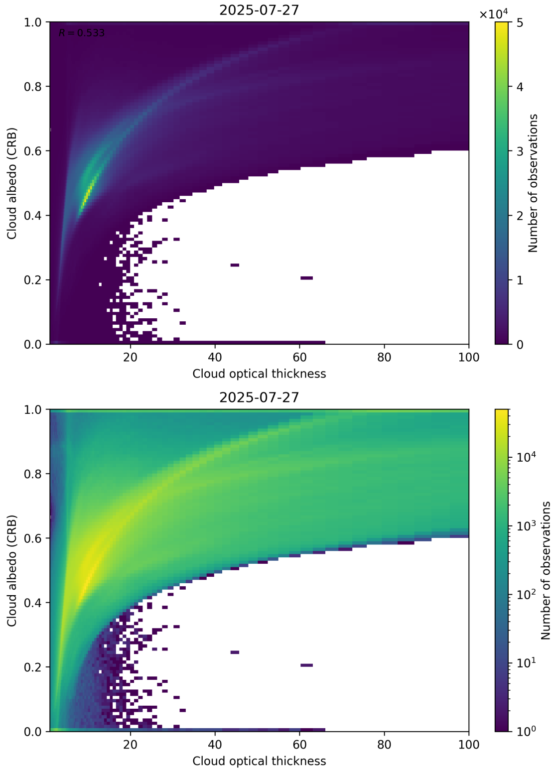
Figure 82: Scatter density plot of “Cloud optical thickness” against “Cloud albedo (CRB)” for 2025-07-26 to 2025-07-28.
