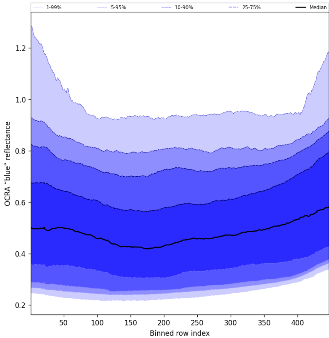
Figure 67: Along track statistics of “OCRA “blue” reflectance” for 2025-07-26 to 2025-07-28
