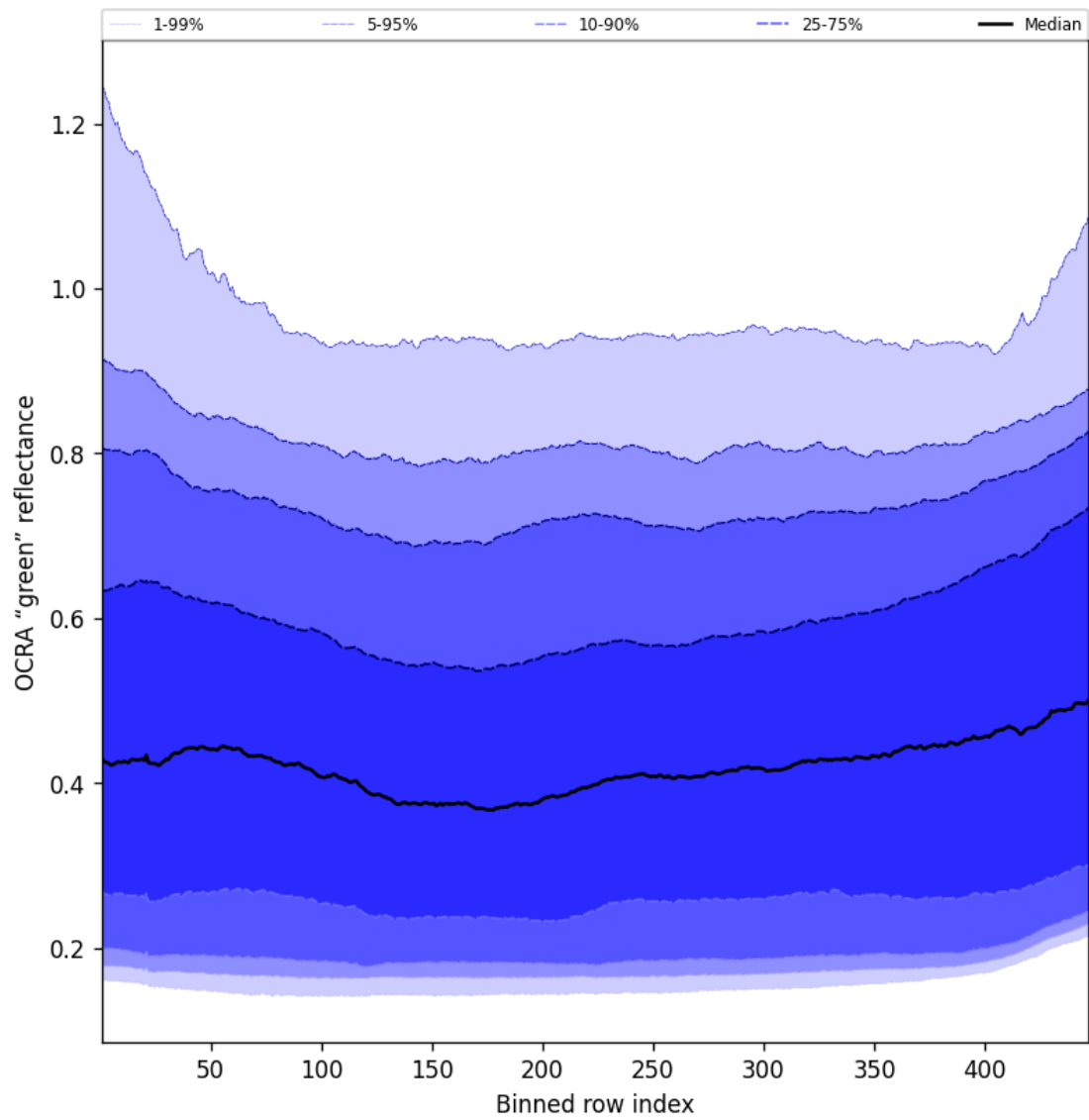
Figure 68: Along track statistics of “OCRA “green” reflectance” for 2025-07-26 to 2025-07-28
