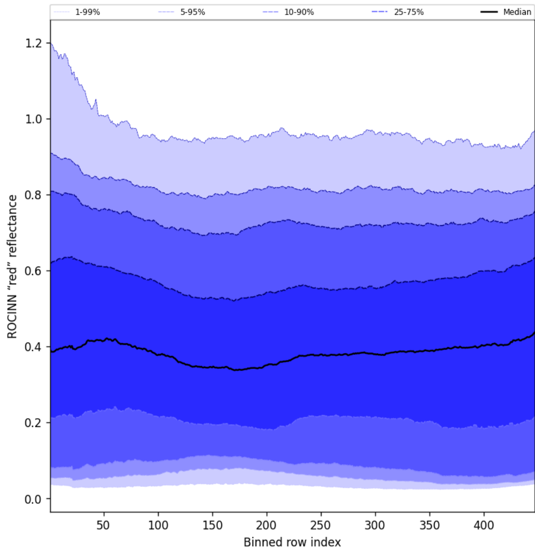
Figure 69: Along track statistics of “ROCINN “red” reflectance” for 2025-07-26 to 2025-07-28
