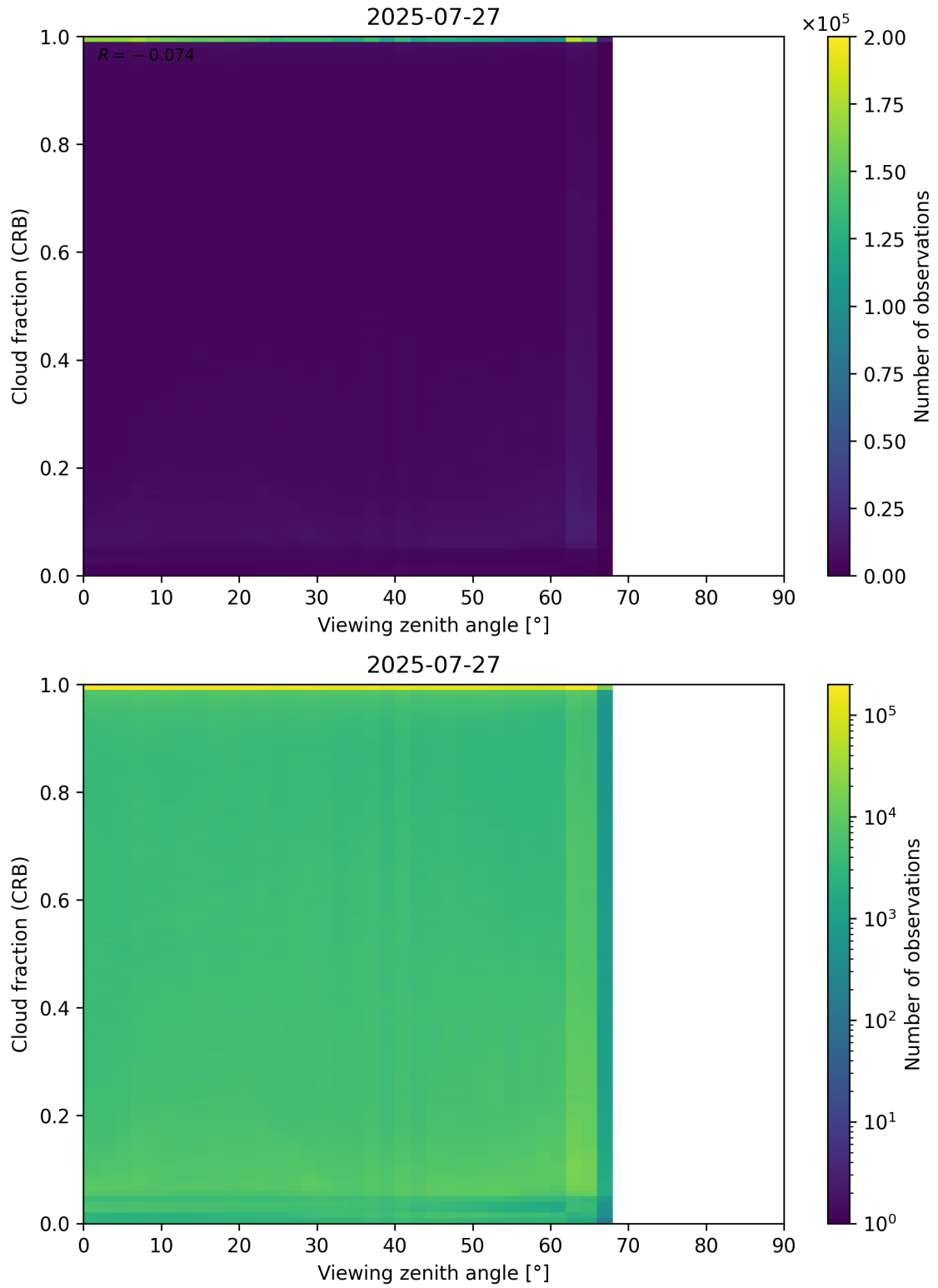
Figure 109: Scatter density plot of “Viewing zenith angle” against “Cloud fraction (CRB)” for 2025-07-26 to 2025-07-28.
