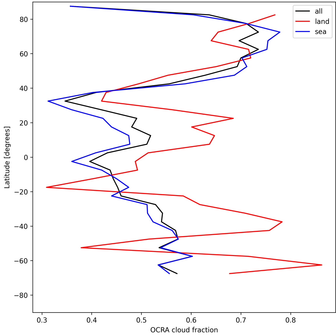
Figure 34: Zonal average of “OCRA cloud fraction” for 2025-07-26 to 2025-07-28.
