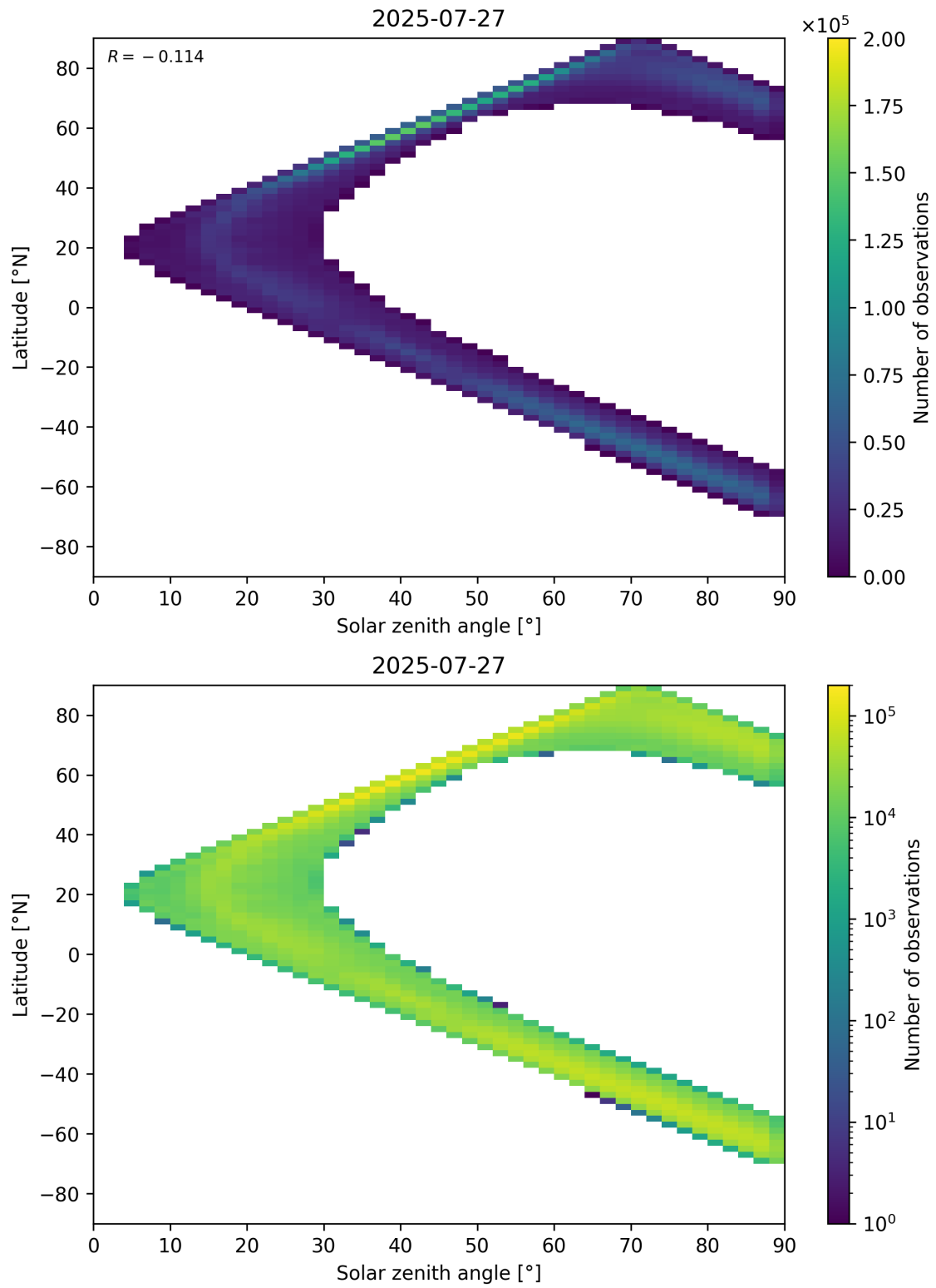
Figure 105: Scatter density plot of “Solar zenith angle” against “Latitude” for 2025-07-26 to 2025-07-28.
