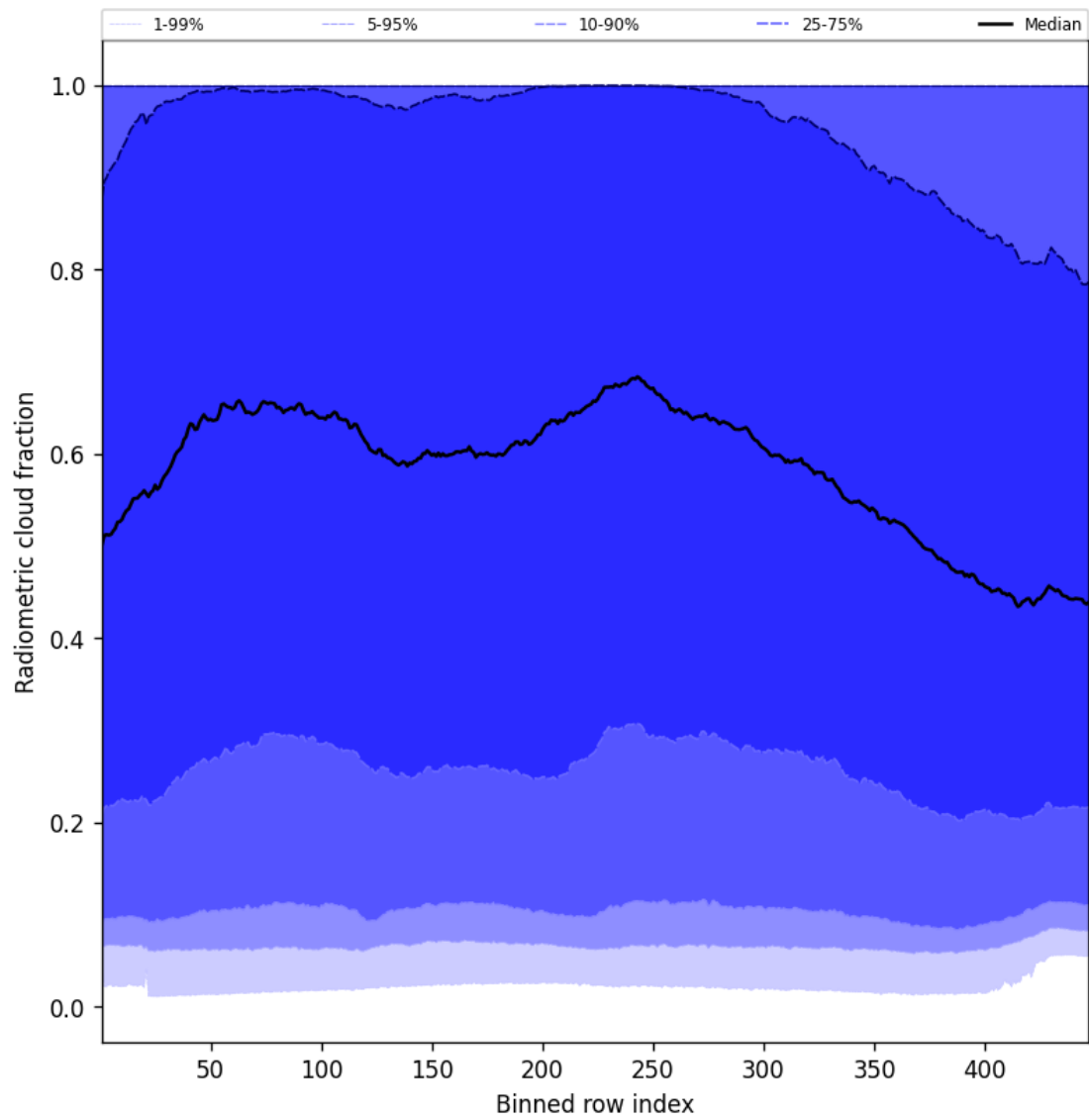
Figure 55: Along track statistics of “Radiometric cloud fraction” for 2025-07-26 to 2025-07-28
