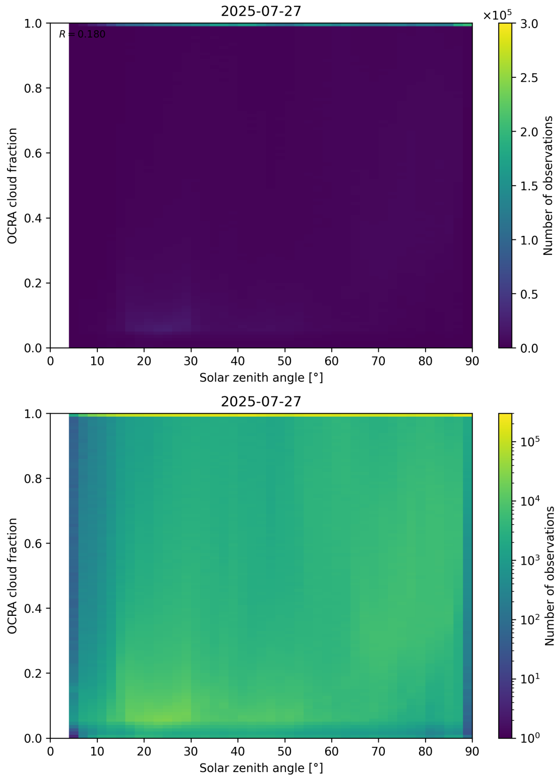
Figure 100: Scatter density plot of “Solar zenith angle” against “OCRA cloud fraction” for 2025-07-26 to 2025-07-28.
