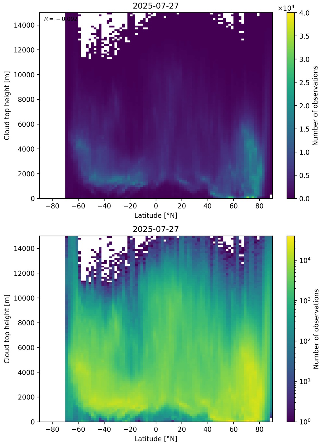
Figure 97: Scatter density plot of “Latitude” against “Cloud top height” for 2025-07-26 to 2025-07-28.
