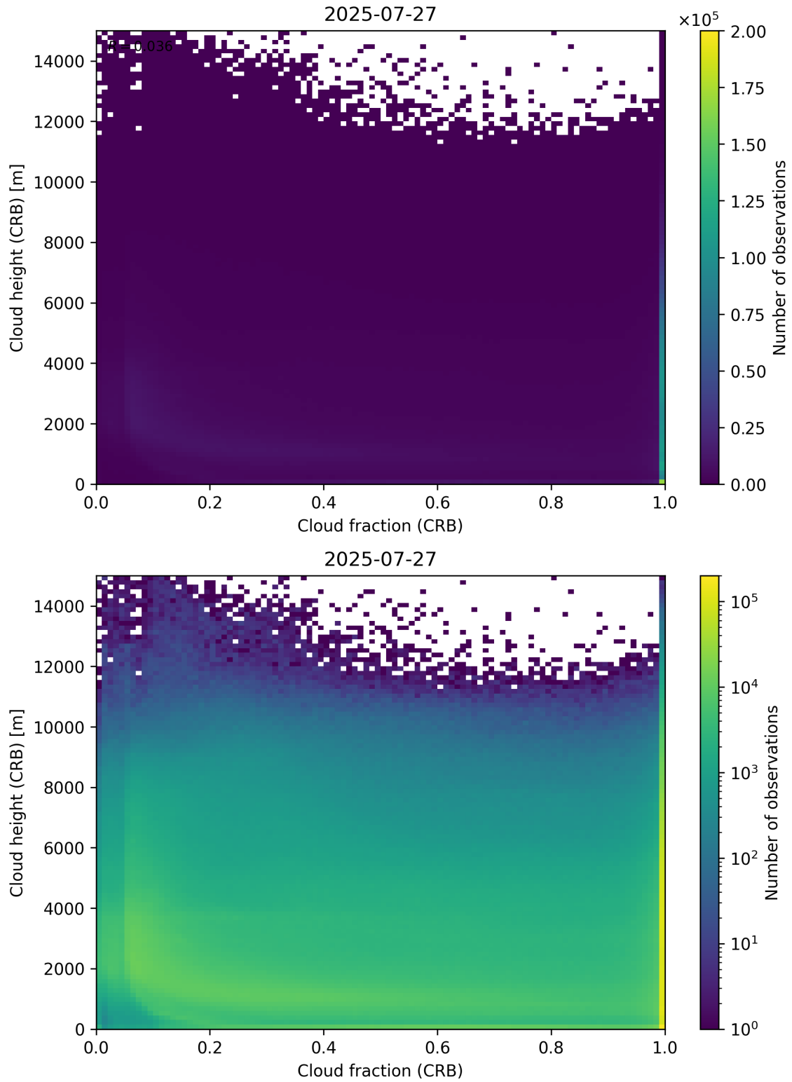
Figure 79: Scatter density plot of “Cloud fraction (CRB)” against “Cloud height (CRB)” for 2025-07-26 to 2025-07-28.
