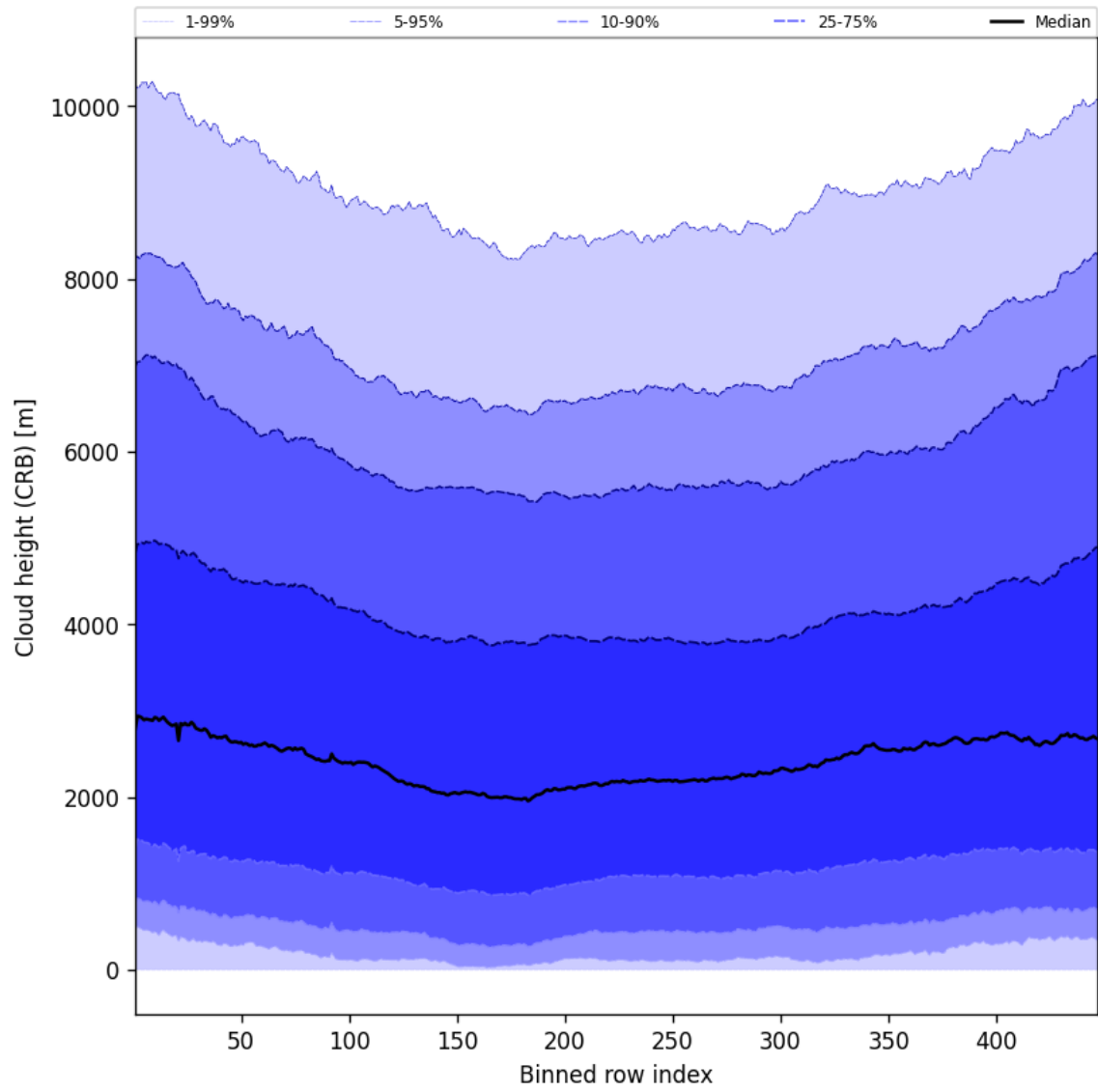
Figure 59: Along track statistics of “Cloud height (CRB)” for 2025-07-26 to 2025-07-28
