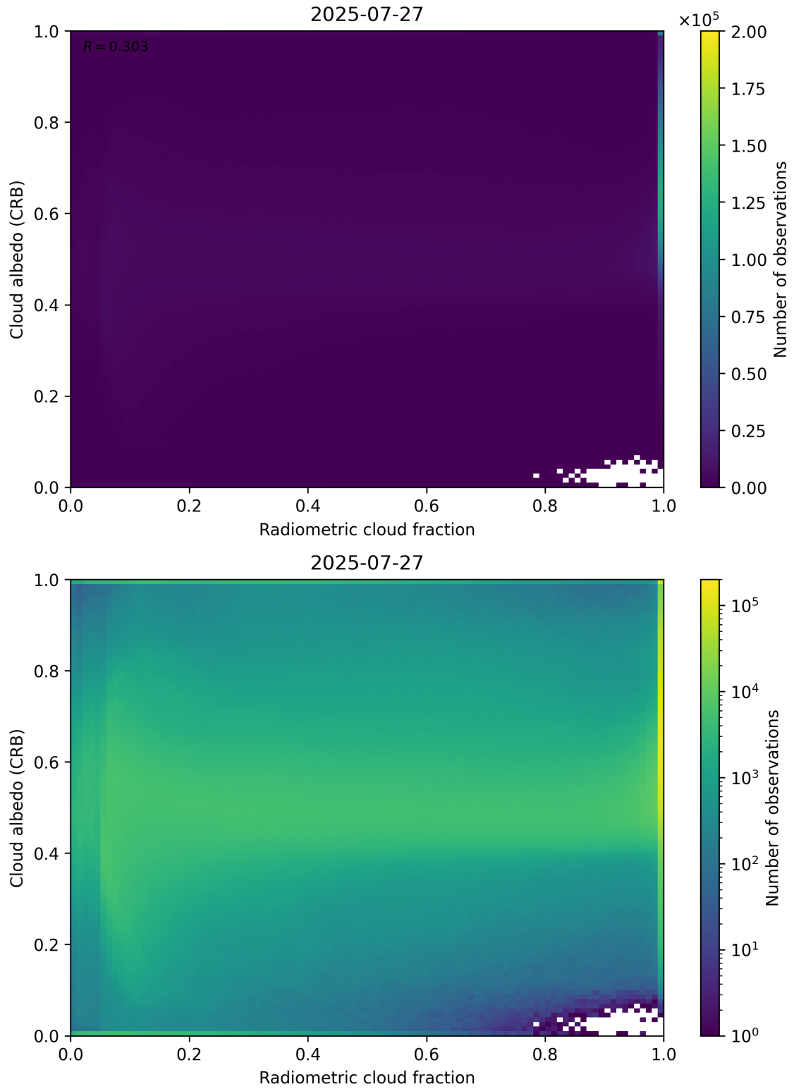
Figure 71: Scatter density plot of “Radiometric cloud fraction” against “Cloud albedo (CRB)” for 2025-07-26 to 2025-07-28.
