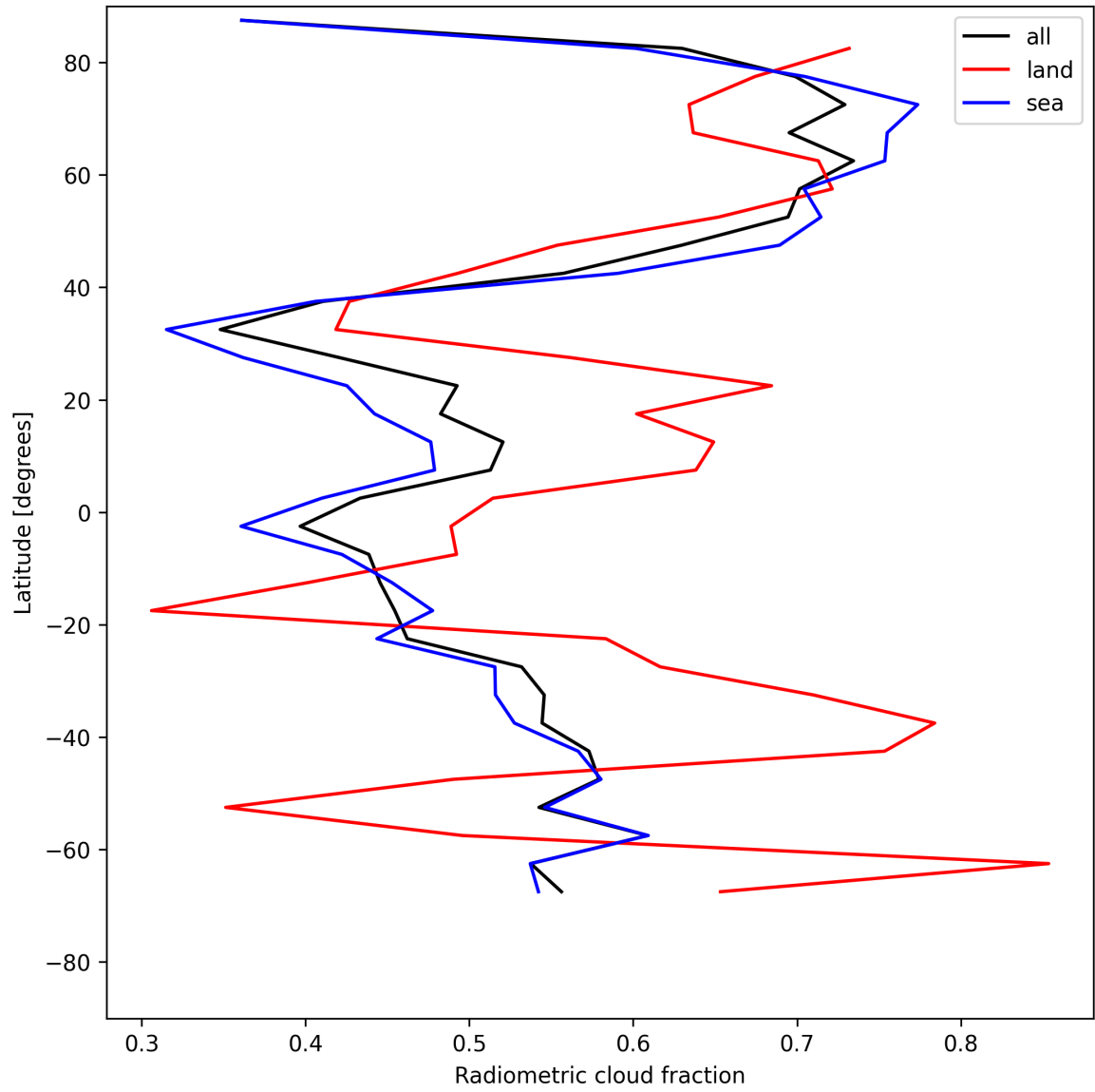
Figure 23: Zonal average of “Radiometric cloud fraction” for 2025-07-26 to 2025-07-28.
