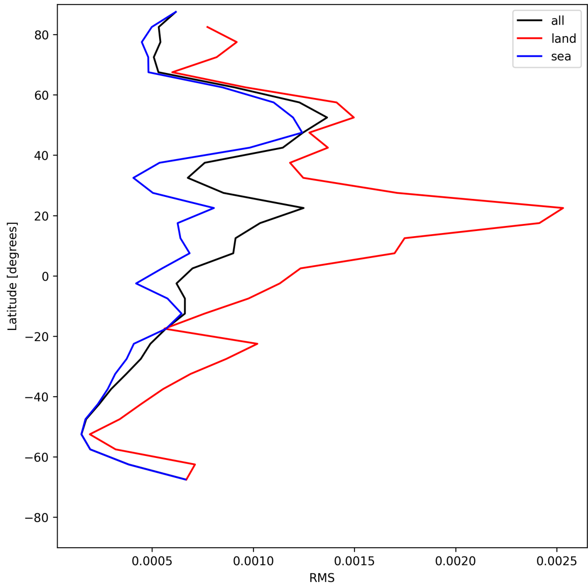
Figure 31: Zonal average of “RMS” for 2025-07-26 to 2025-07-28.
