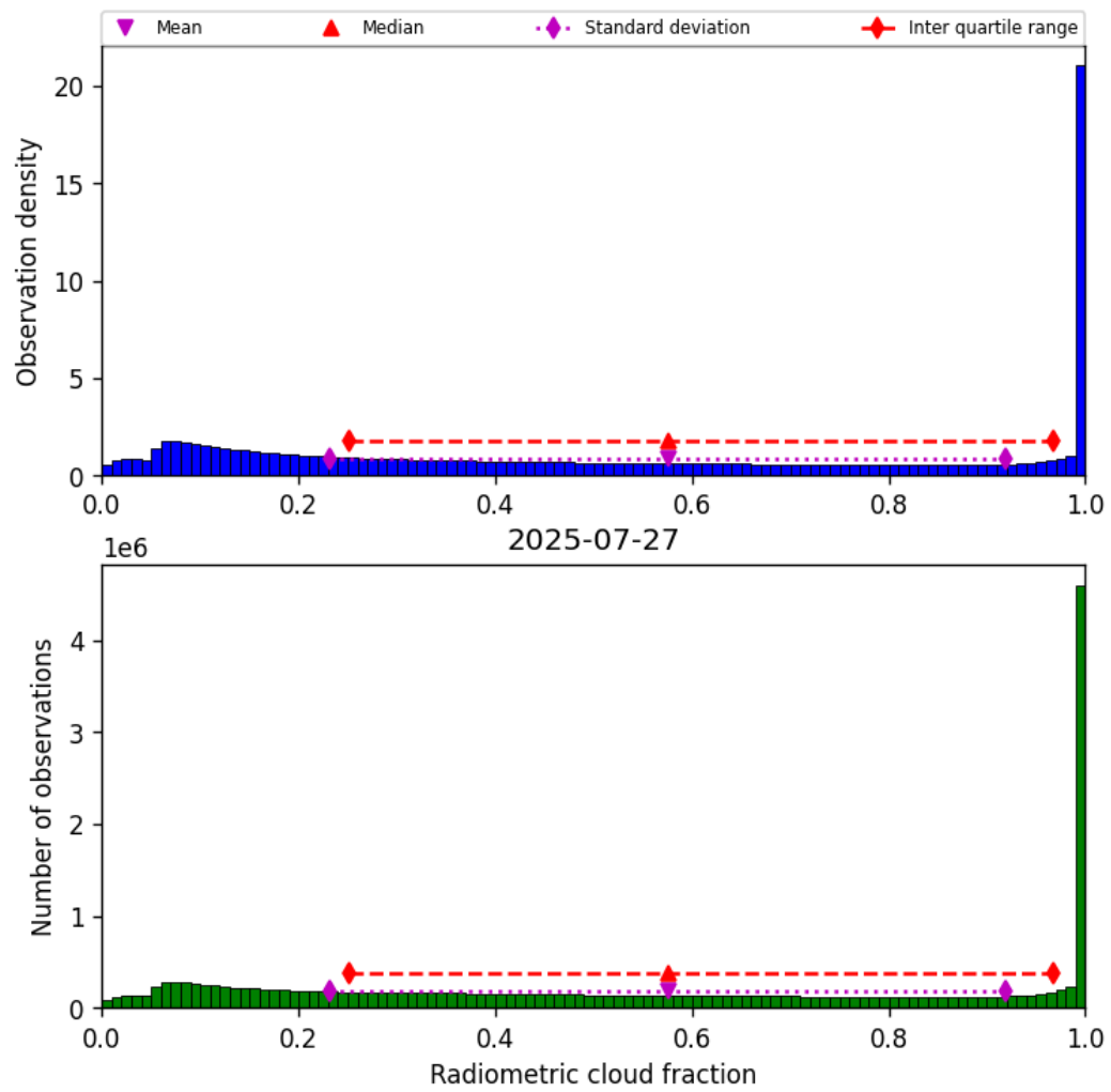
Figure 39: Histogram of “Radiometric cloud fraction” for 2025-07-26 to 2025-07-28
