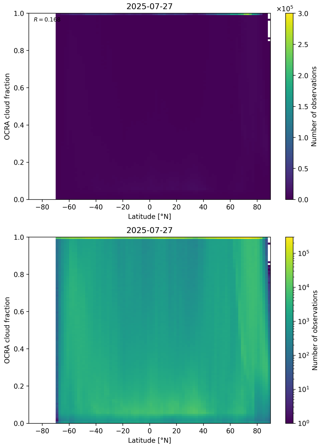
Figure 93: Scatter density plot of “Latitude” against “OCRA cloud fraction” for 2025-07-26 to 2025-07-28.
