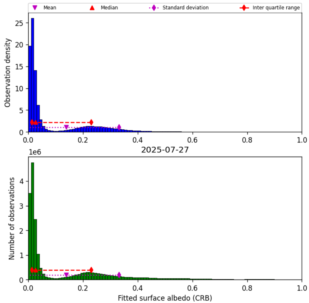
Figure 46: Histogram of “Fitted surface albedo (CRB)” for 2025-07-26 to 2025-07-28
