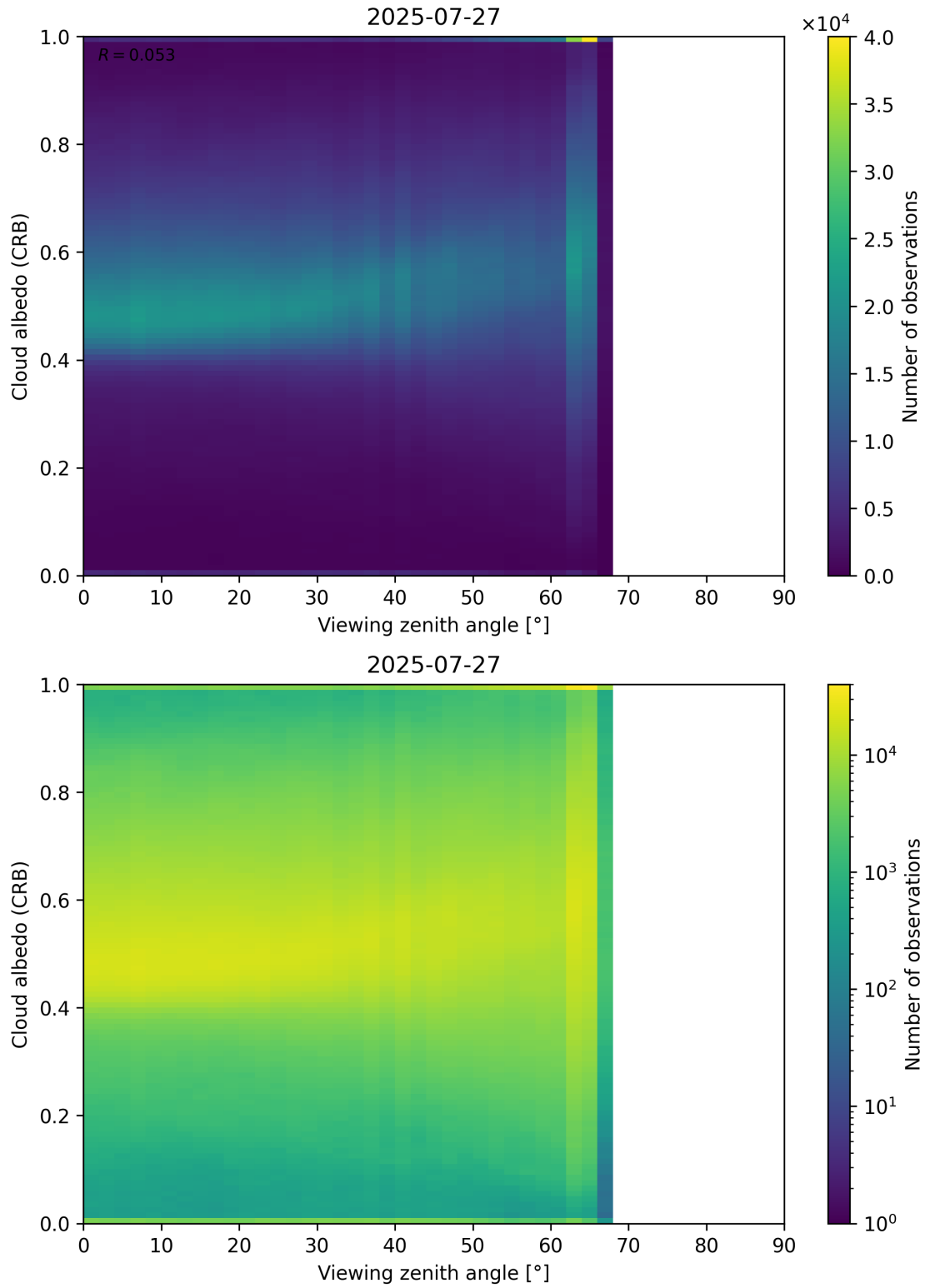
Figure 106: Scatter density plot of “Viewing zenith angle” against “Cloud albedo (CRB)” for 2025-07-26 to 2025-07-28.
