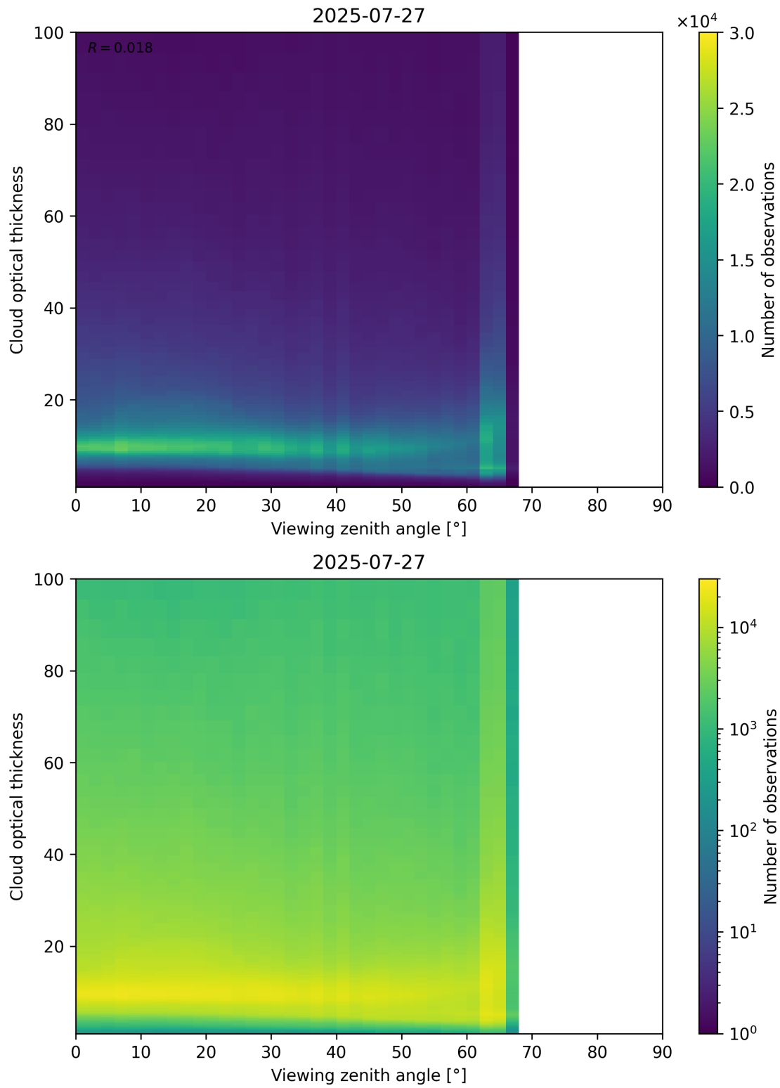
Figure 111: Scatter density plot of “Viewing zenith angle” against “Cloud optical thickness” for 2025-07-26 to 2025-07-28.
