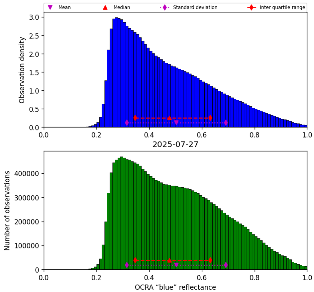
Figure 51: Histogram of “OCRA “blue” reflectance” for 2025-07-26 to 2025-07-28
