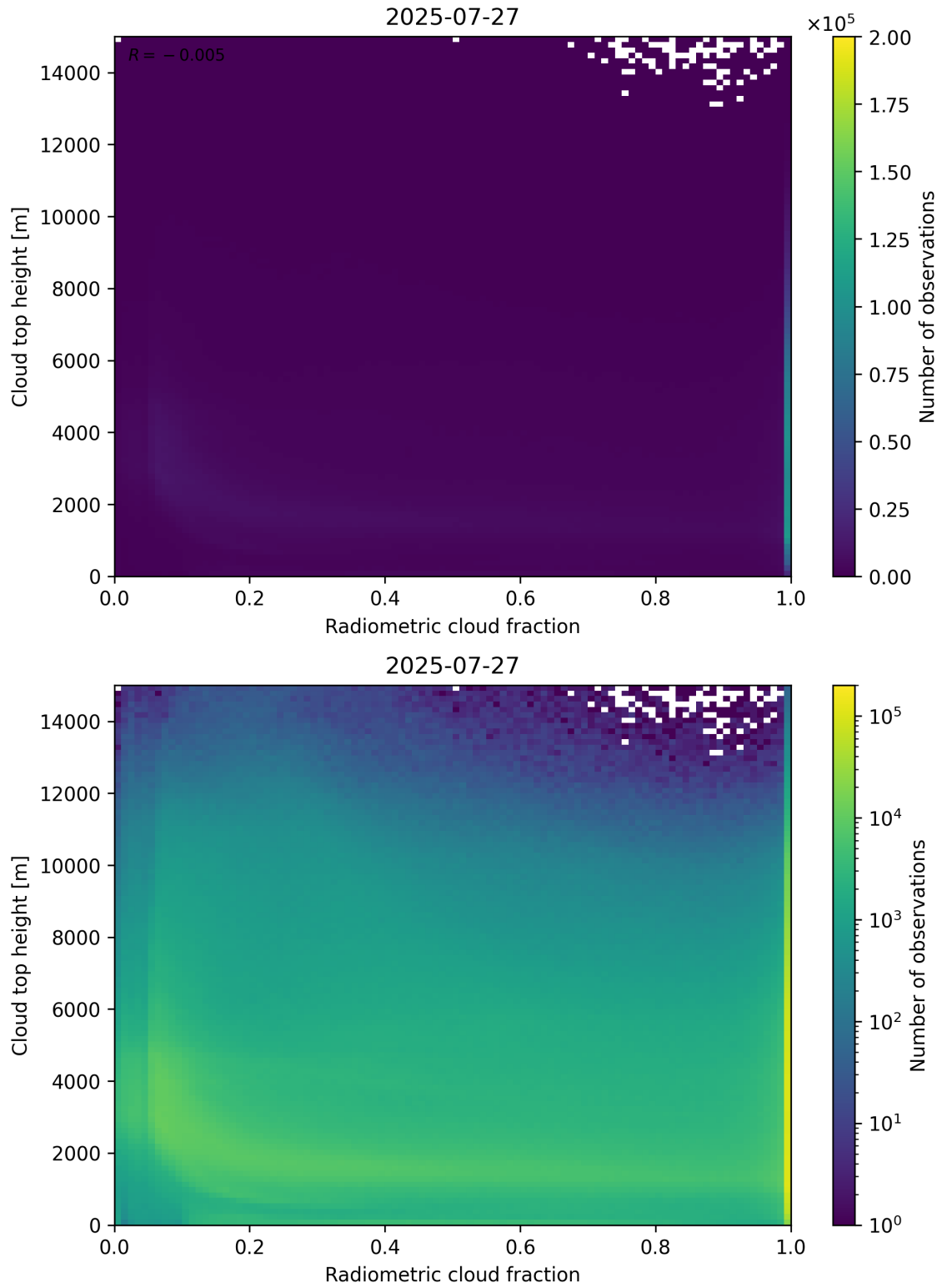
Figure 76: Scatter density plot of “Radiometric cloud fraction” against “Cloud top height” for 2025-07-26 to 2025-07-28.
