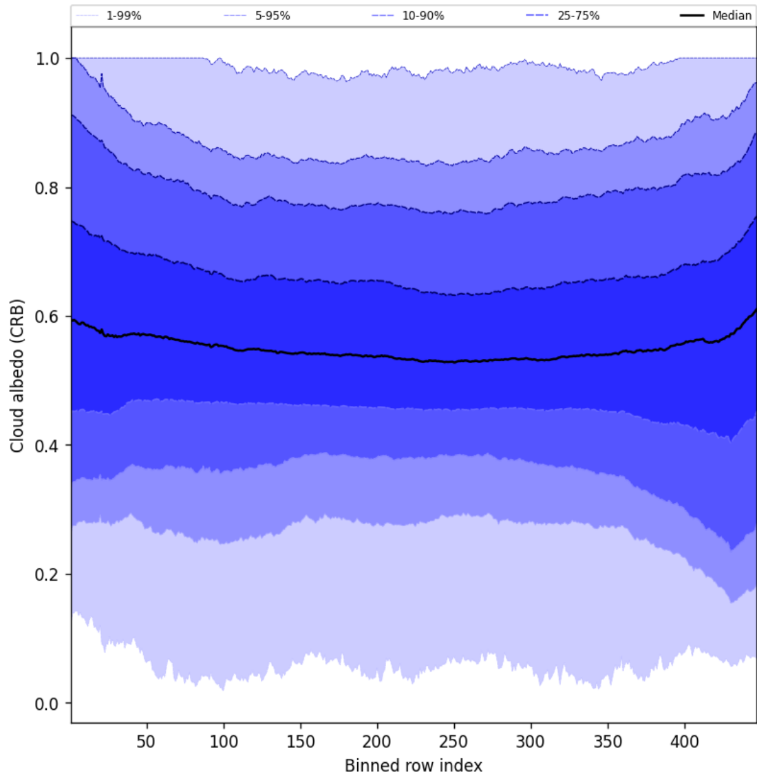
Figure 60: Along track statistics of “Cloud albedo (CRB)” for 2025-07-26 to 2025-07-28
