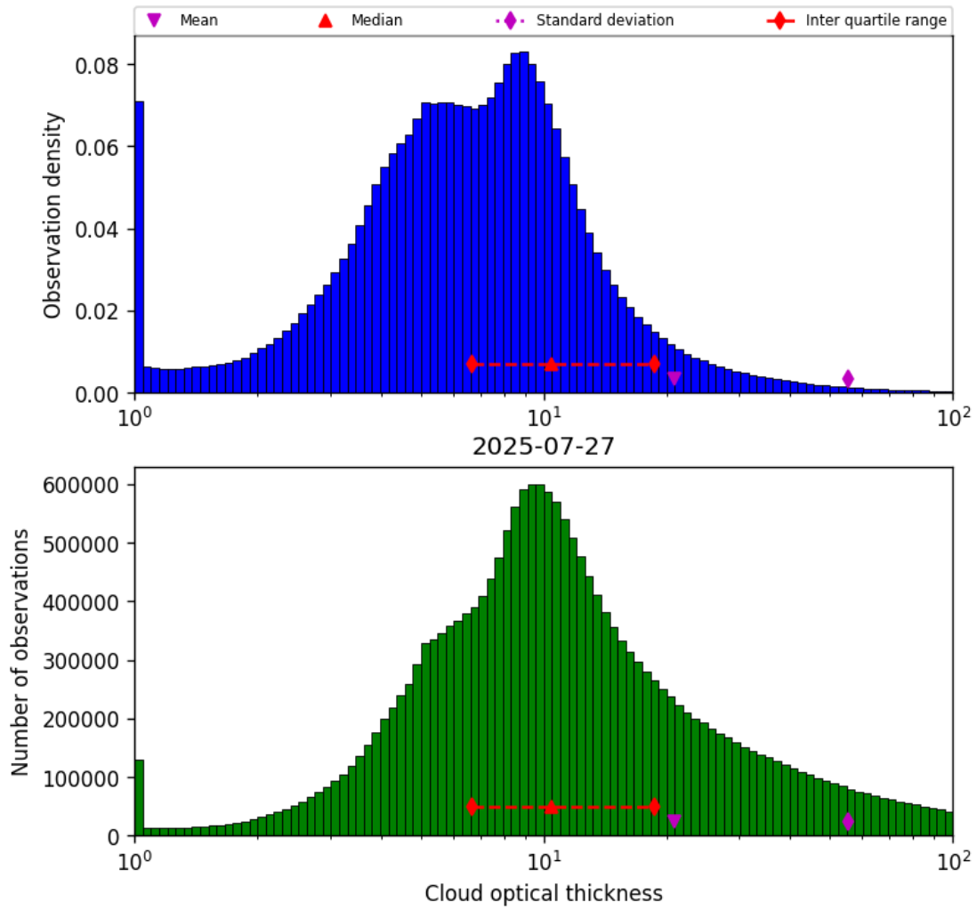
Figure 41: Histogram of “Cloud optical thickness” for 2025-07-26 to 2025-07-28
