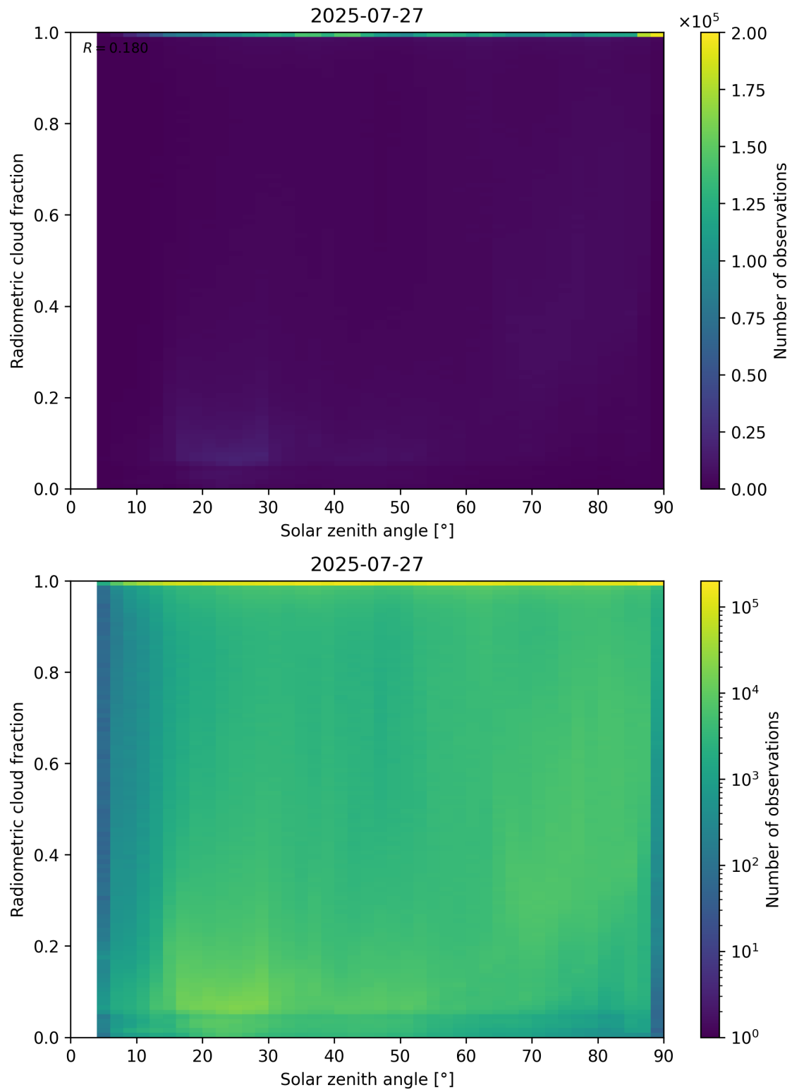
Figure 99: Scatter density plot of “Solar zenith angle” against “Radiometric cloud fraction” for 2025-07-26 to 2025-07-28.
