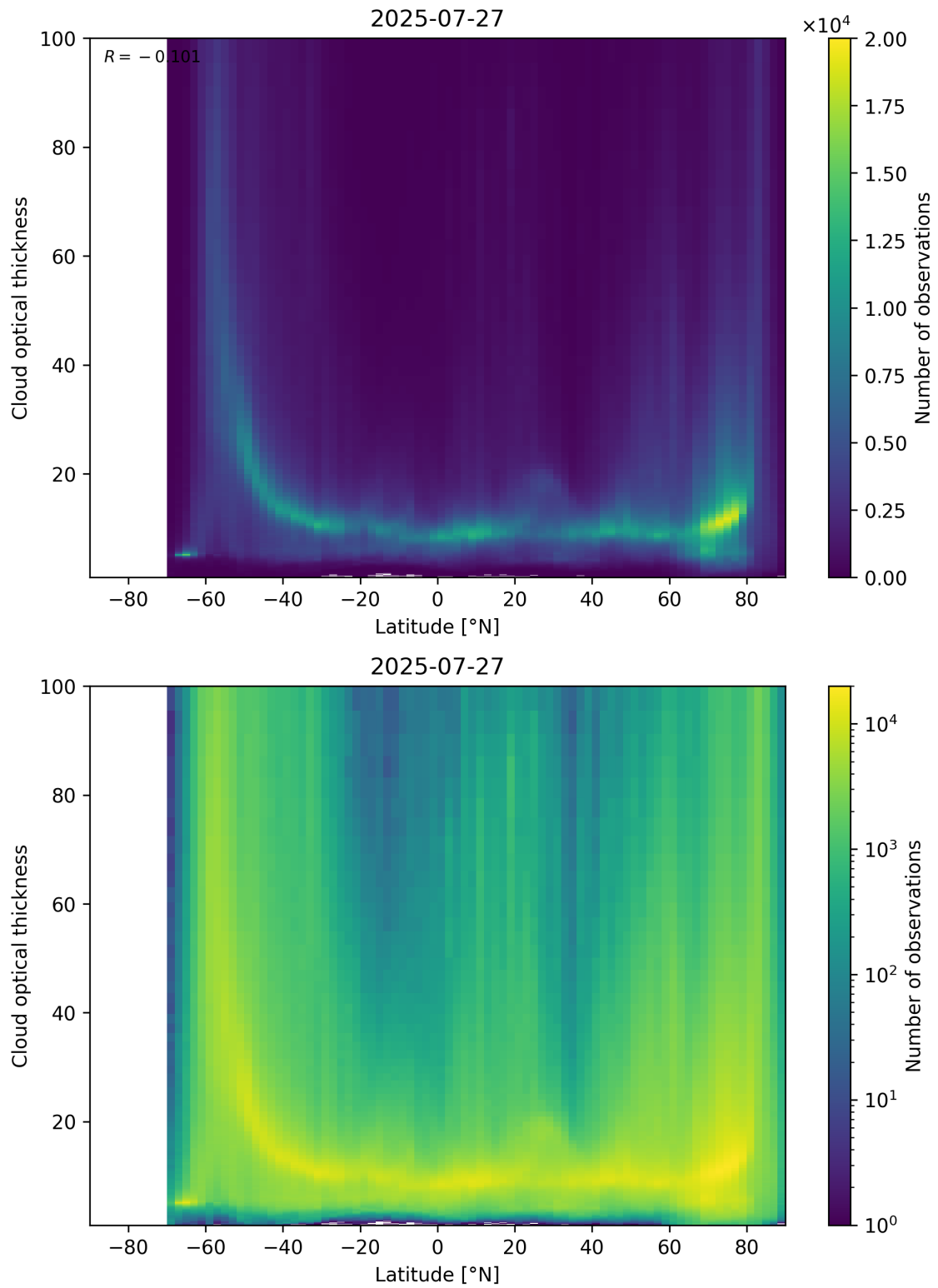
Figure 96: Scatter density plot of “Latitude” against “Cloud optical thickness” for 2025-07-26 to 2025-07-28.
