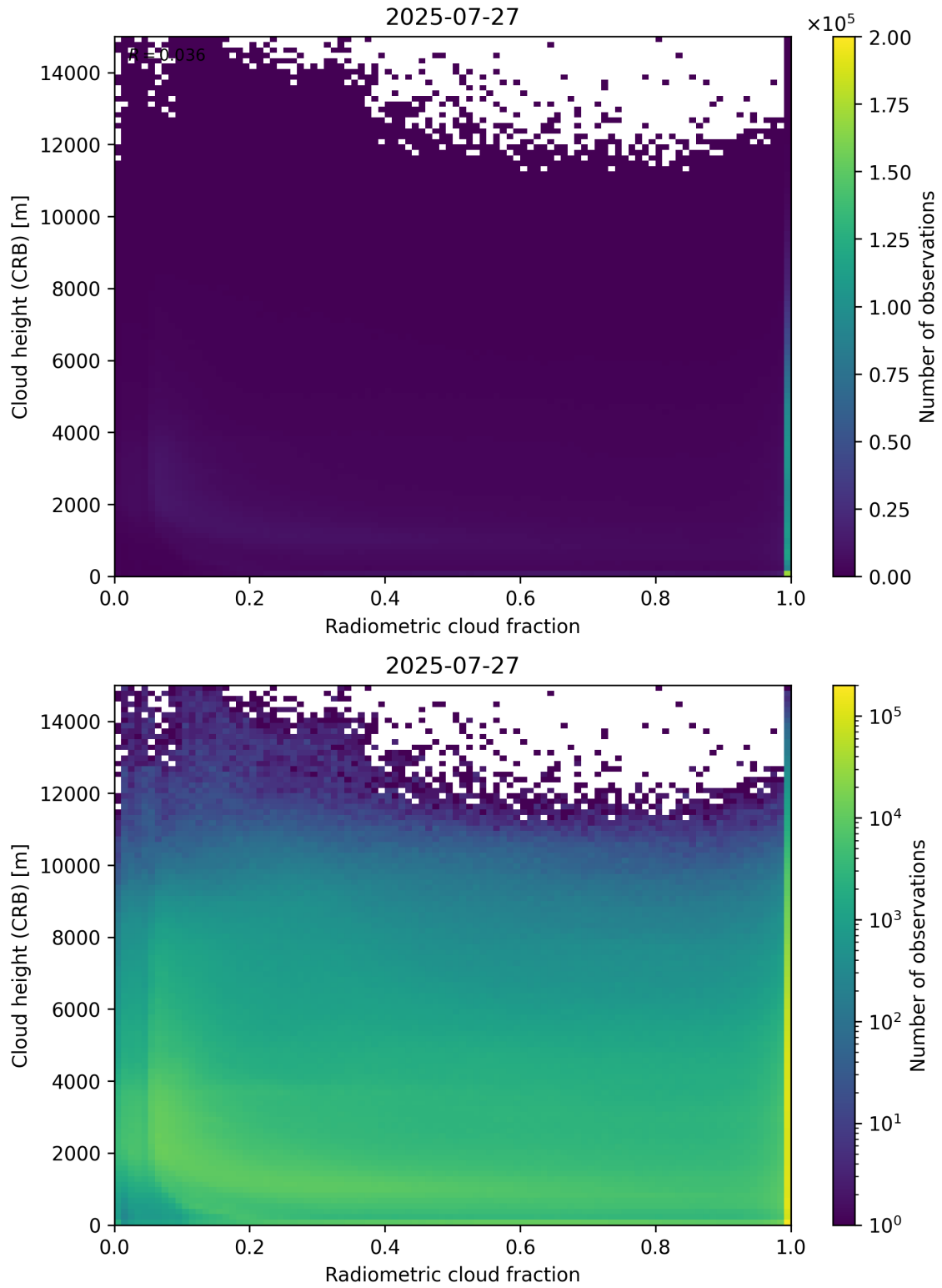
Figure 74: Scatter density plot of “Radiometric cloud fraction” against “Cloud height (CRB)” for 2025-07-26 to 2025-07-28.
