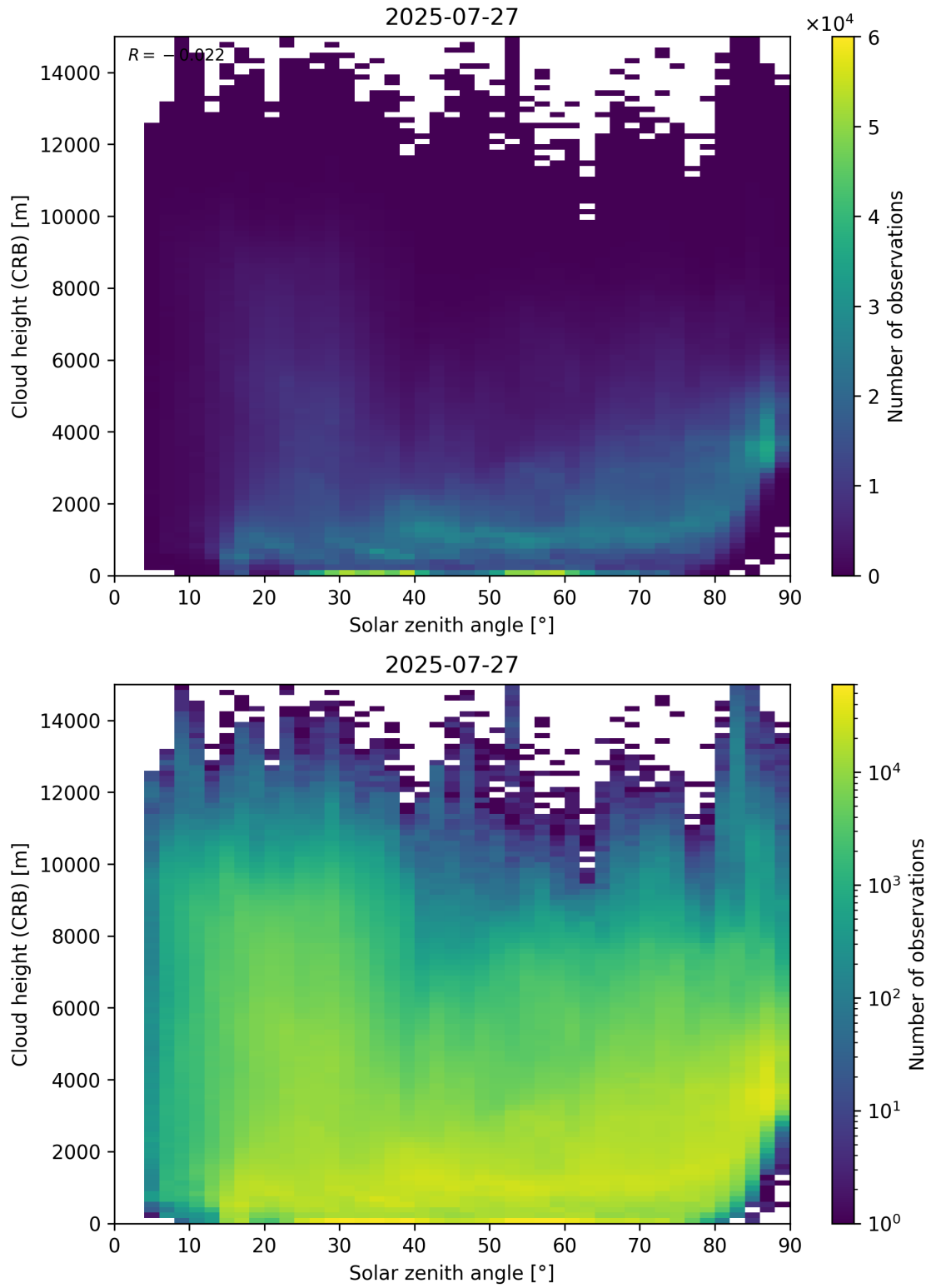
Figure 102: Scatter density plot of “Solar zenith angle” against “Cloud height (CRB)” for 2025-07-26 to 2025-07-28.
