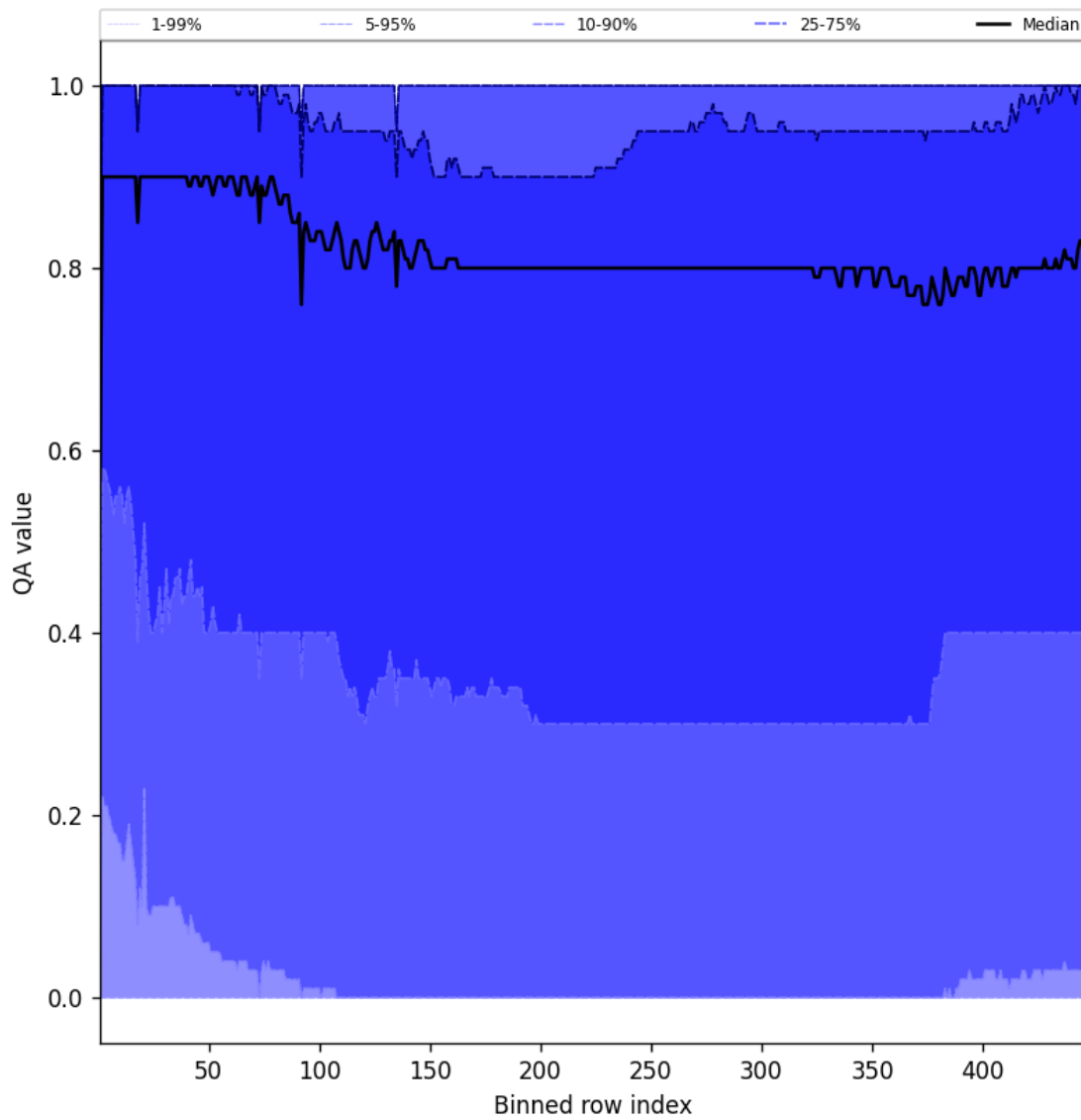
Figure 54: Along track statistics of “QA value” for 2025-07-26 to 2025-07-28
