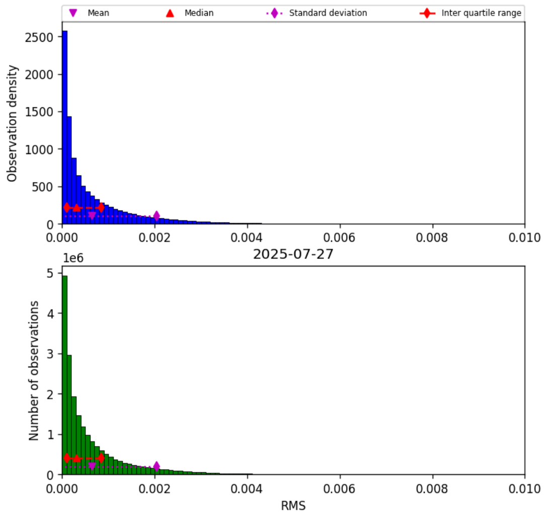
Figure 47: Histogram of “RMS” for 2025-07-26 to 2025-07-28
