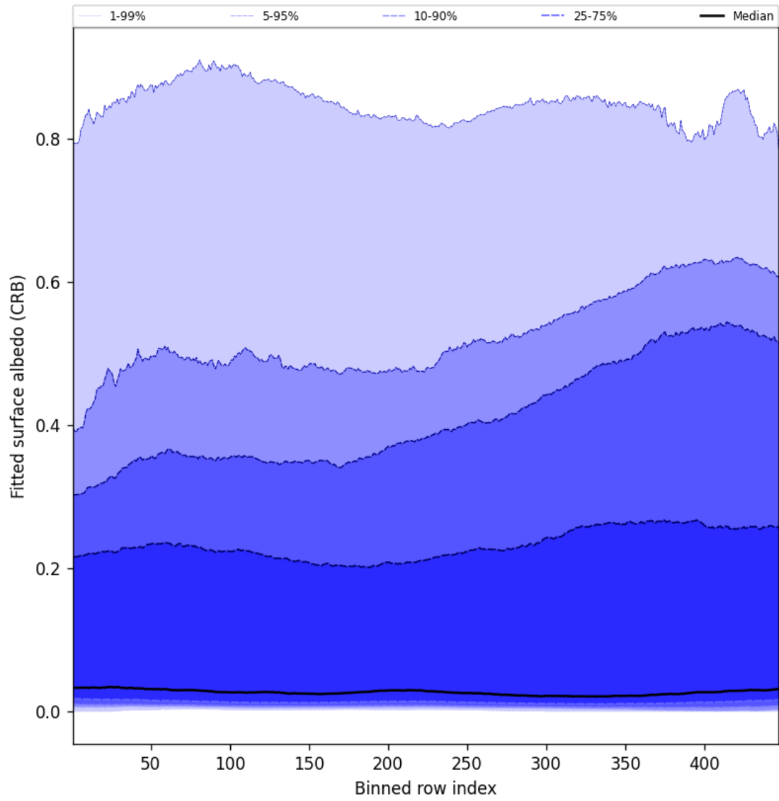
Figure 62: Along track statistics of “Fitted surface albedo (CRB)” for 2025-07-26 to 2025-07-28
