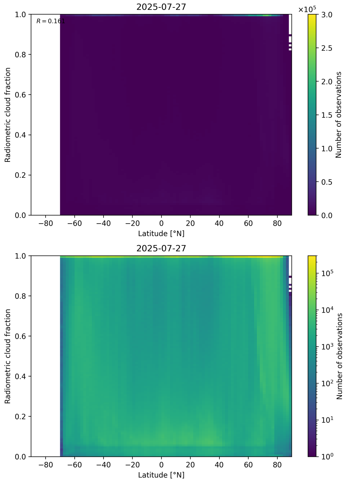
Figure 92: Scatter density plot of “Latitude” against “Radiometric cloud fraction” for 2025-07-26 to 2025-07-28.
