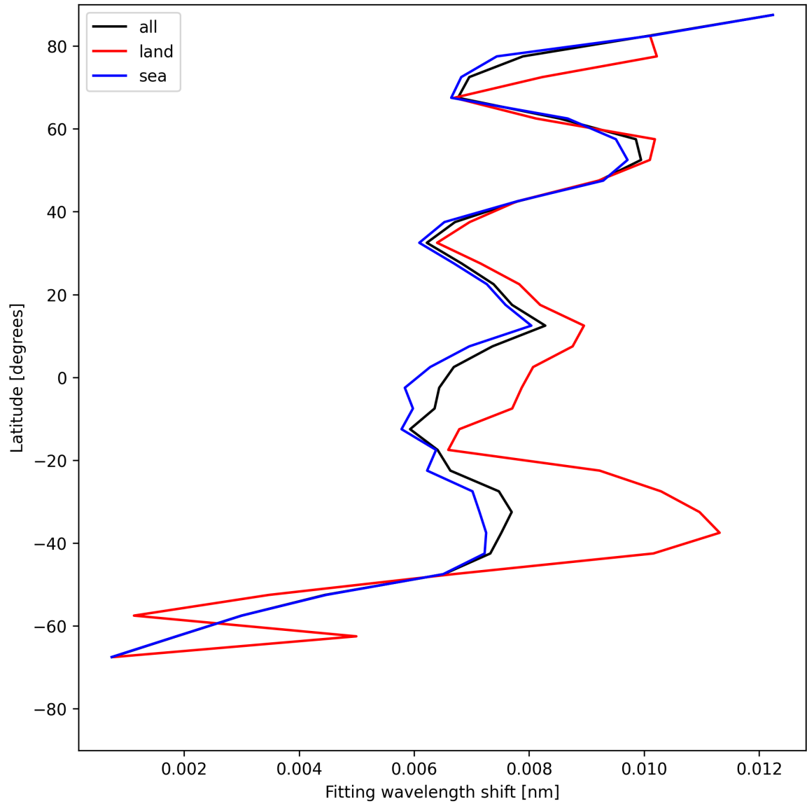
Figure 33: Zonal average of “Fitting wavelength shift” for 2025-07-26 to 2025-07-28.
