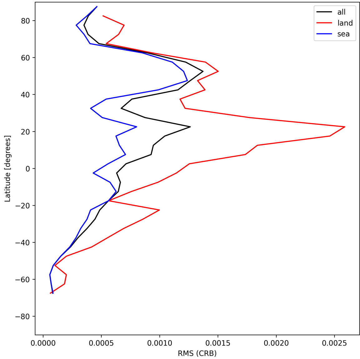
Figure 32: Zonal average of “RMS (CRB)” for 2025-07-26 to 2025-07-28.
