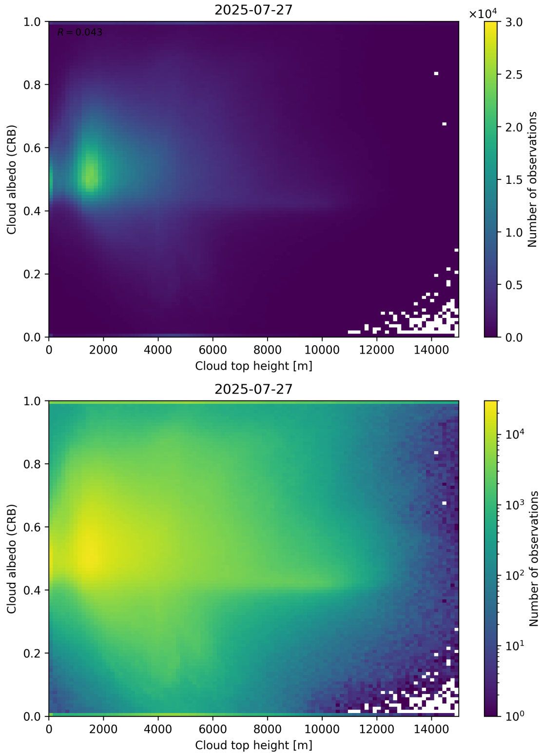
Figure 86: Scatter density plot of “Cloud top height” against “Cloud albedo (CRB)” for 2025-07-26 to 2025-07-28.
