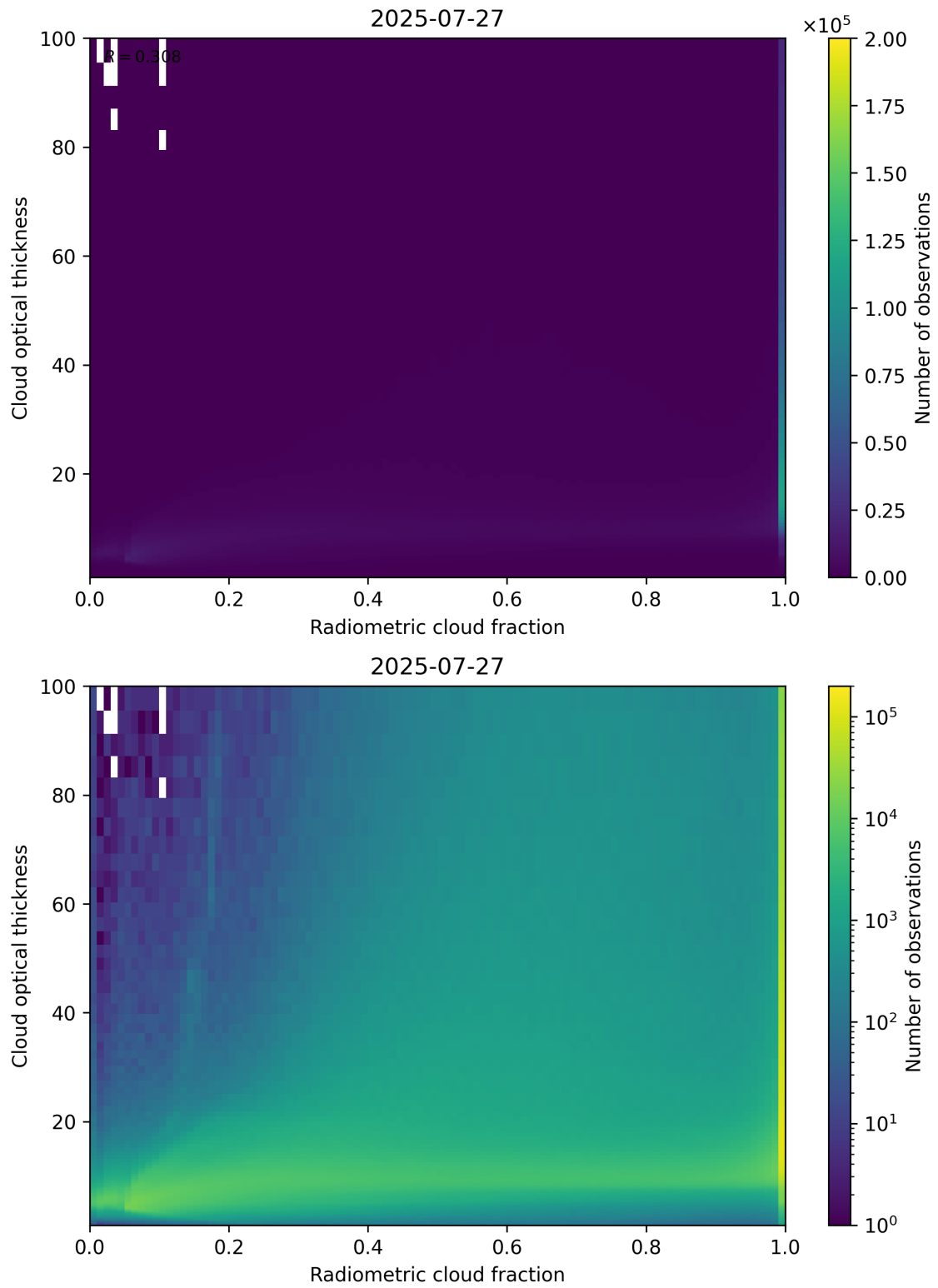
Figure 75: Scatter density plot of “Radiometric cloud fraction” against “Cloud optical thickness” for 2025-07-26 to 2025-07-28.
