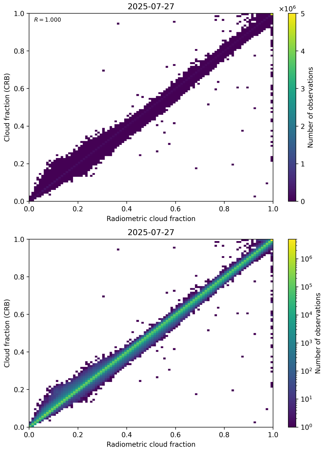
Figure 73: Scatter density plot of “Radiometric cloud fraction” against “Cloud fraction (CRB)” for 2025-07-26 to 2025-07-28.
