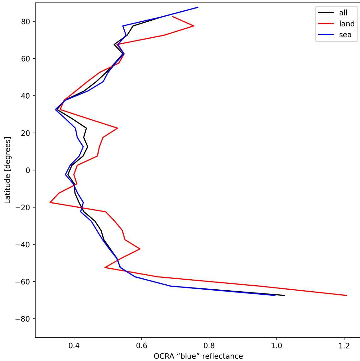
Figure 35: Zonal average of “OCRA “blue” reflectance” for 2025-07-26 to 2025-07-28.
