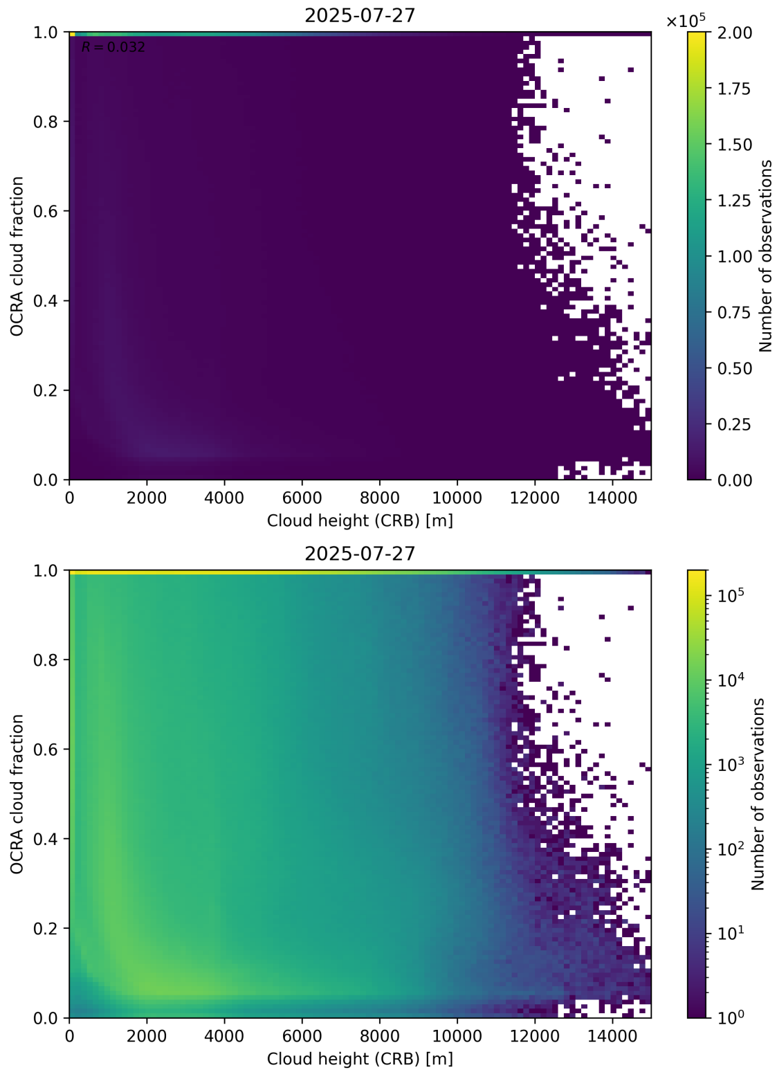
Figure 81: Scatter density plot of “Cloud height (CRB)” against “OCRA cloud fraction” for 2025-07-26 to 2025-07-28.
