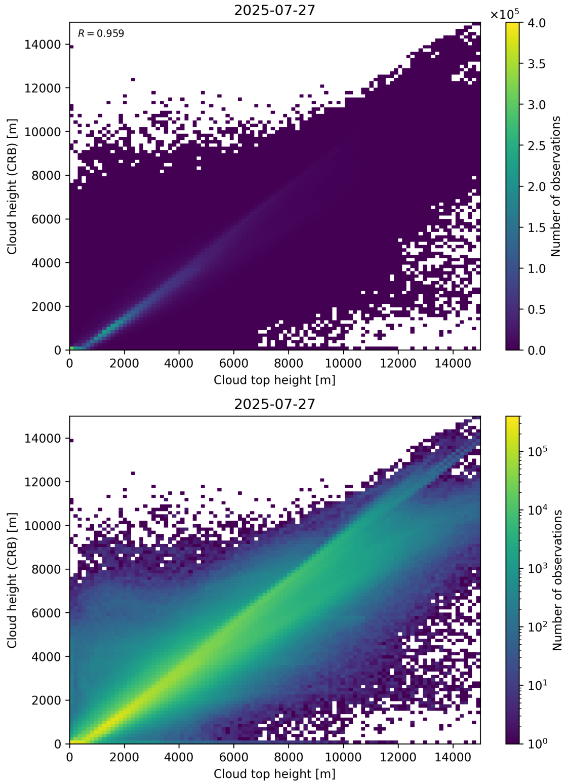
Figure 89: Scatter density plot of “Cloud top height” against “Cloud height (CRB)” for 2025-07-26 to 2025-07-28.
