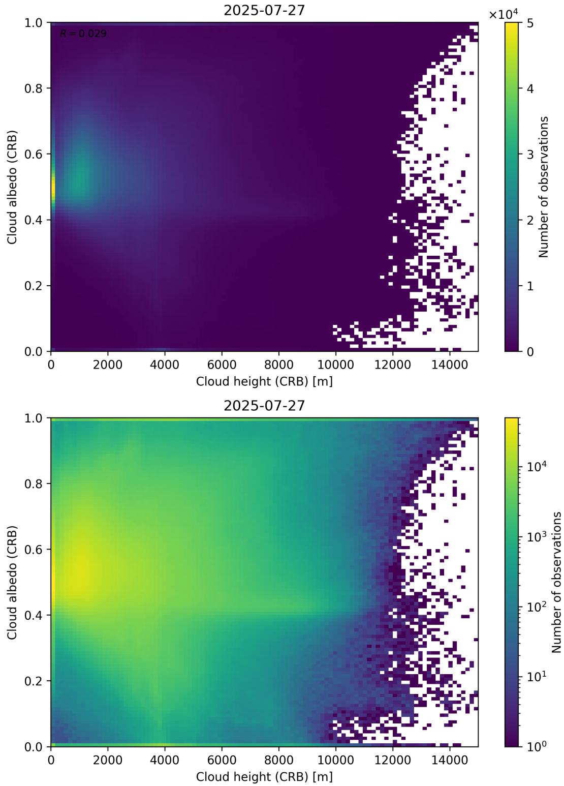
Figure 80: Scatter density plot of “Cloud height (CRB)” against “Cloud albedo (CRB)” for 2025-07-26 to 2025-07-28.
