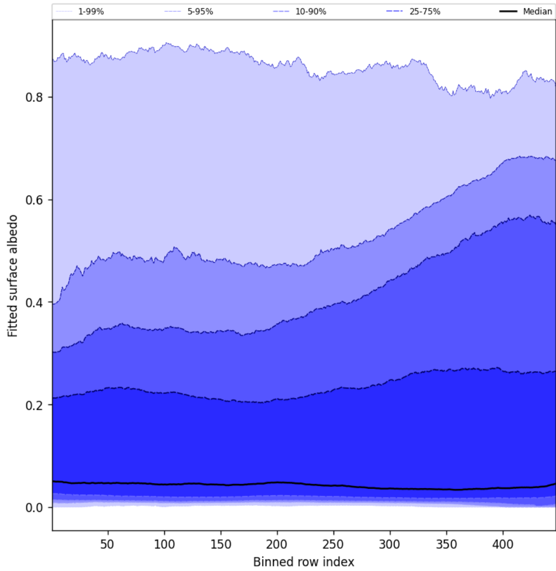
Figure 61: Along track statistics of “Fitted surface albedo” for 2025-07-26 to 2025-07-28
