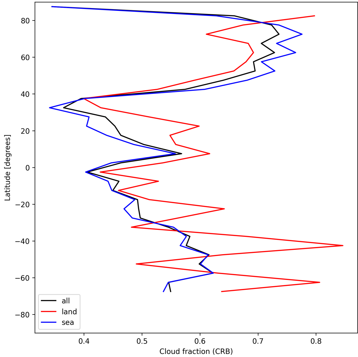
Figure 26: Zonal average of “Cloud fraction (CRB)” for 2025-07-27 to 2025-07-29.
