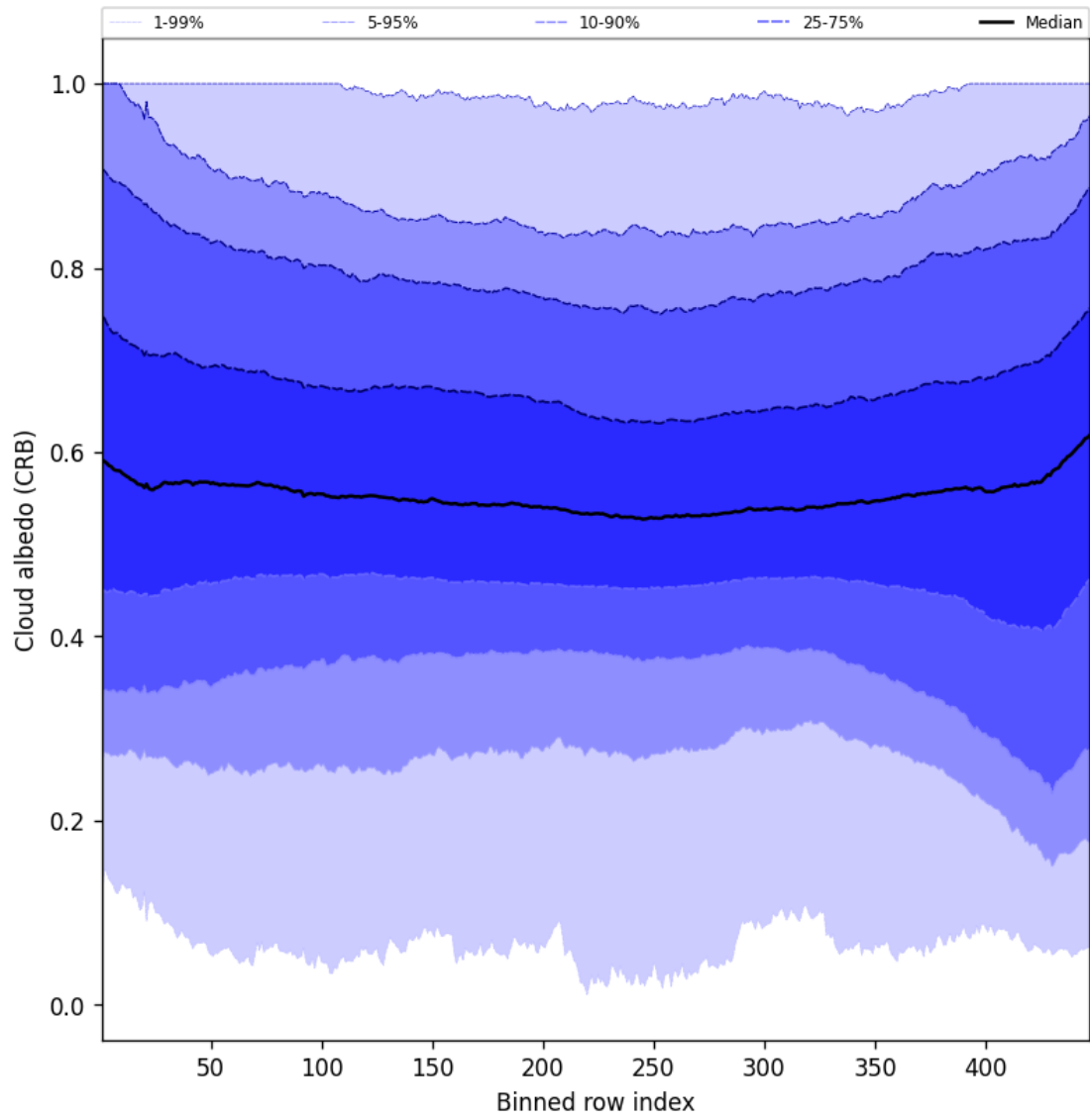
Figure 60: Along track statistics of “Cloud albedo (CRB)” for 2025-07-27 to 2025-07-29
