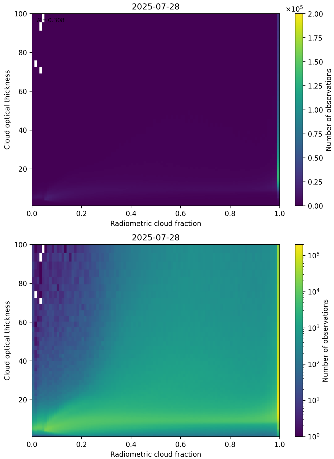
Figure 75: Scatter density plot of “Radiometric cloud fraction” against “Cloud optical thickness” for 2025-07-27 to 2025-07-29.
