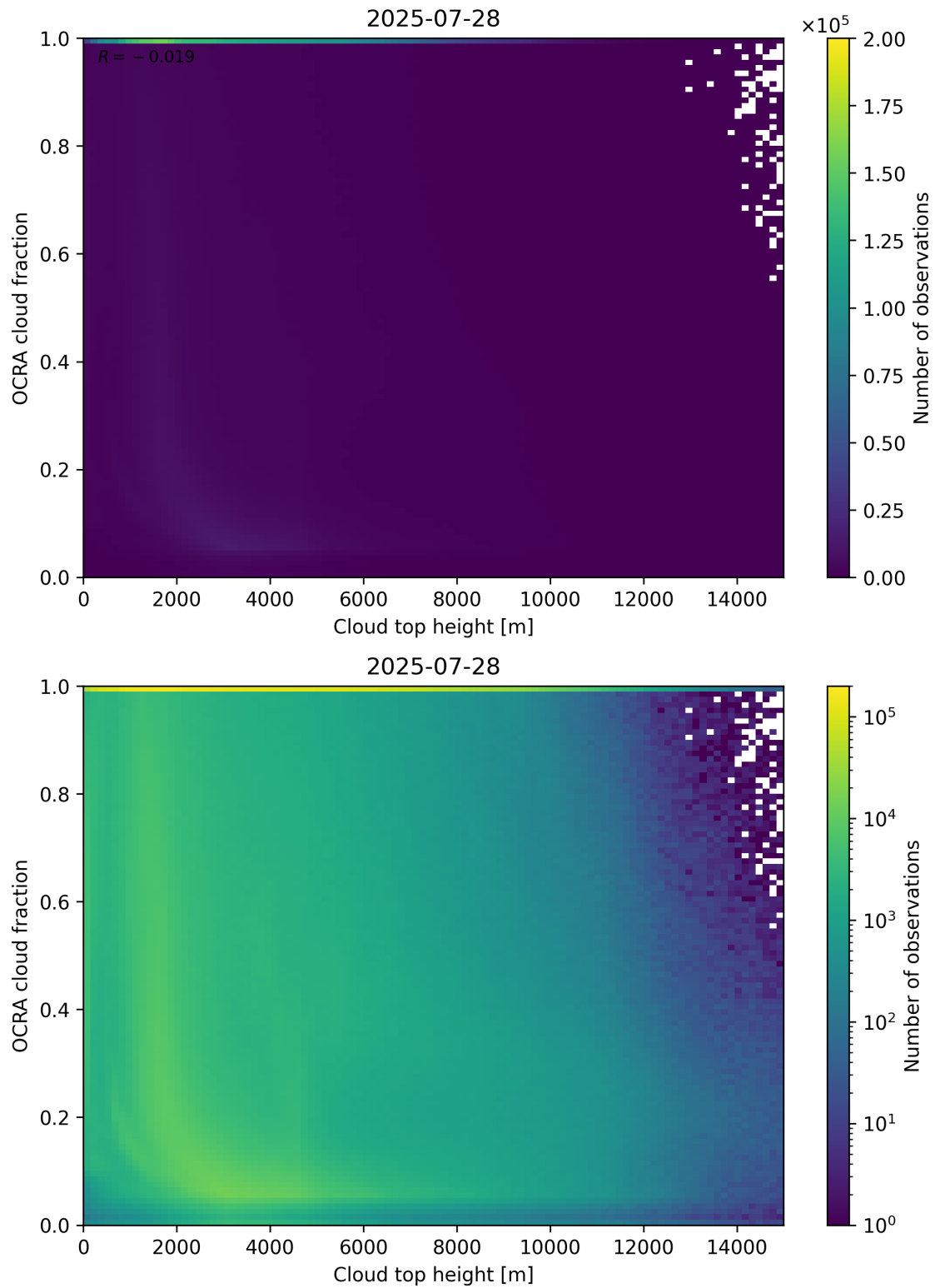
Figure 87: Scatter density plot of “Cloud top height” against “OCRA cloud fraction” for 2025-07-27 to 2025-07-29.
