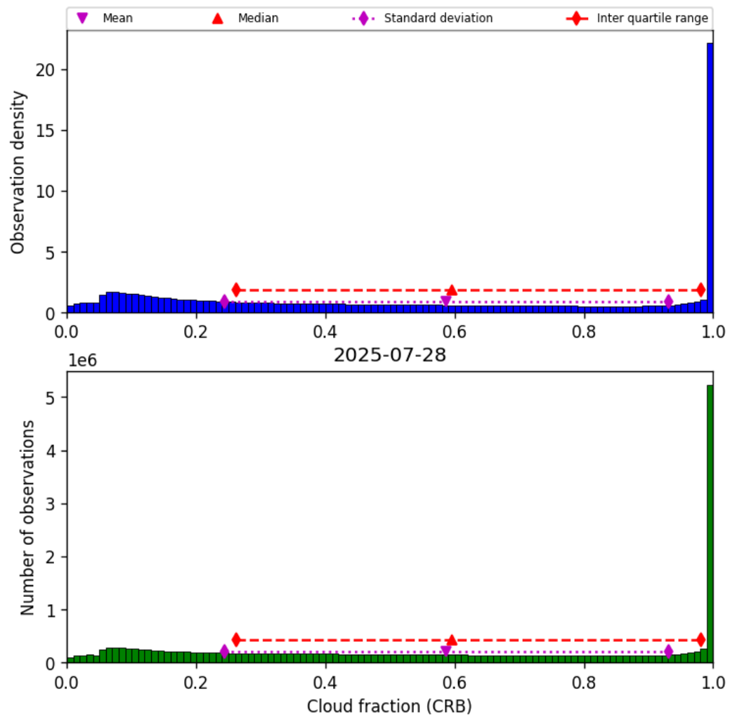
Figure 42: Histogram of “Cloud fraction (CRB)” for 2025-07-27 to 2025-07-29
