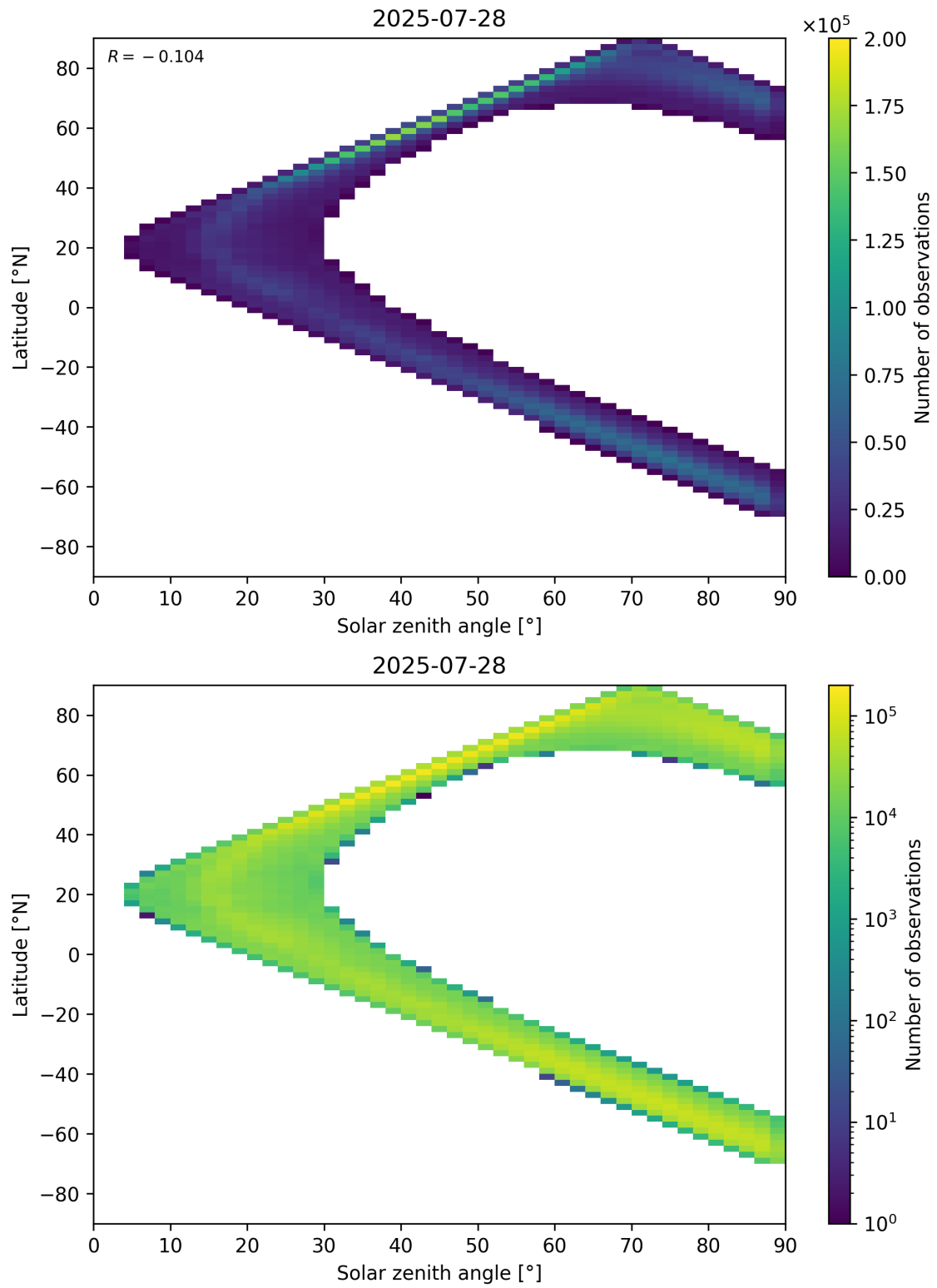
Figure 105: Scatter density plot of “Solar zenith angle” against “Latitude” for 2025-07-27 to 2025-07-29.
