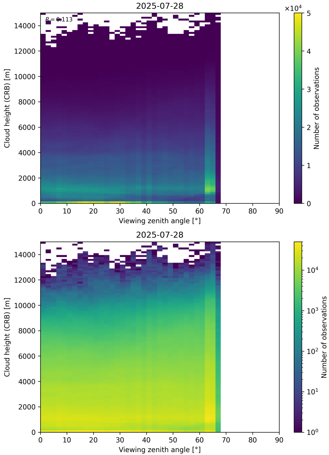
Figure 110: Scatter density plot of “Viewing zenith angle” against “Cloud height (CRB)” for 2025-07-27 to 2025-07-29.
