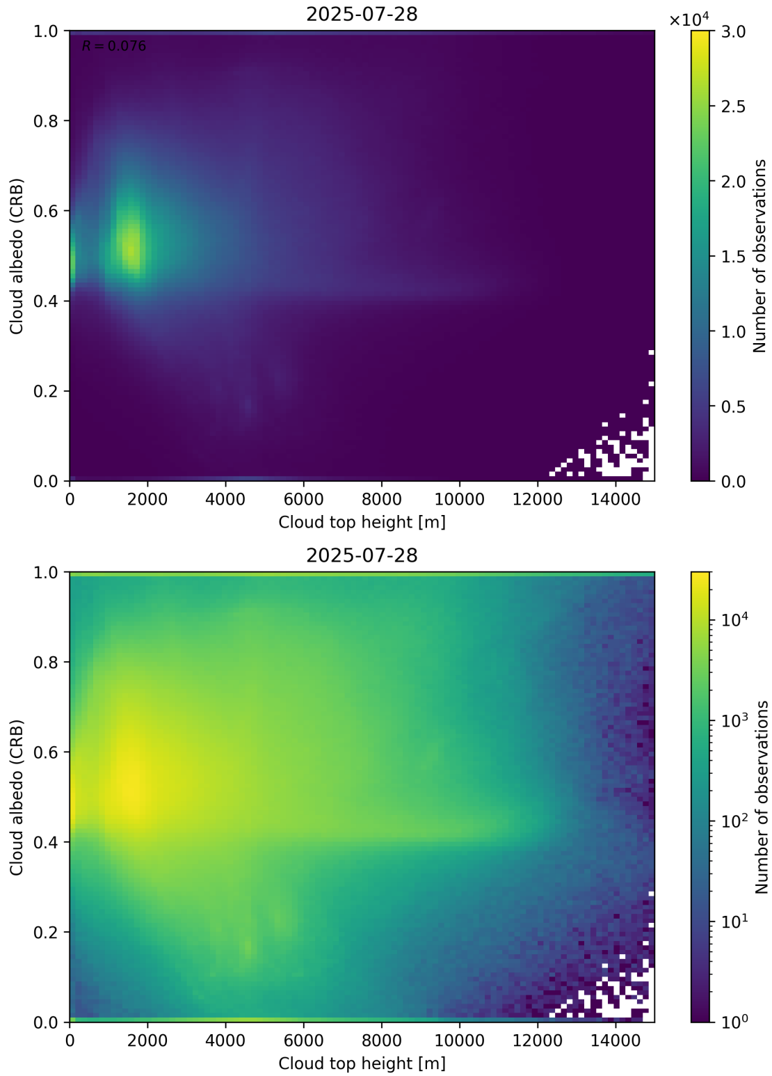
Figure 86: Scatter density plot of “Cloud top height” against “Cloud albedo (CRB)” for 2025-07-27 to 2025-07-29.
