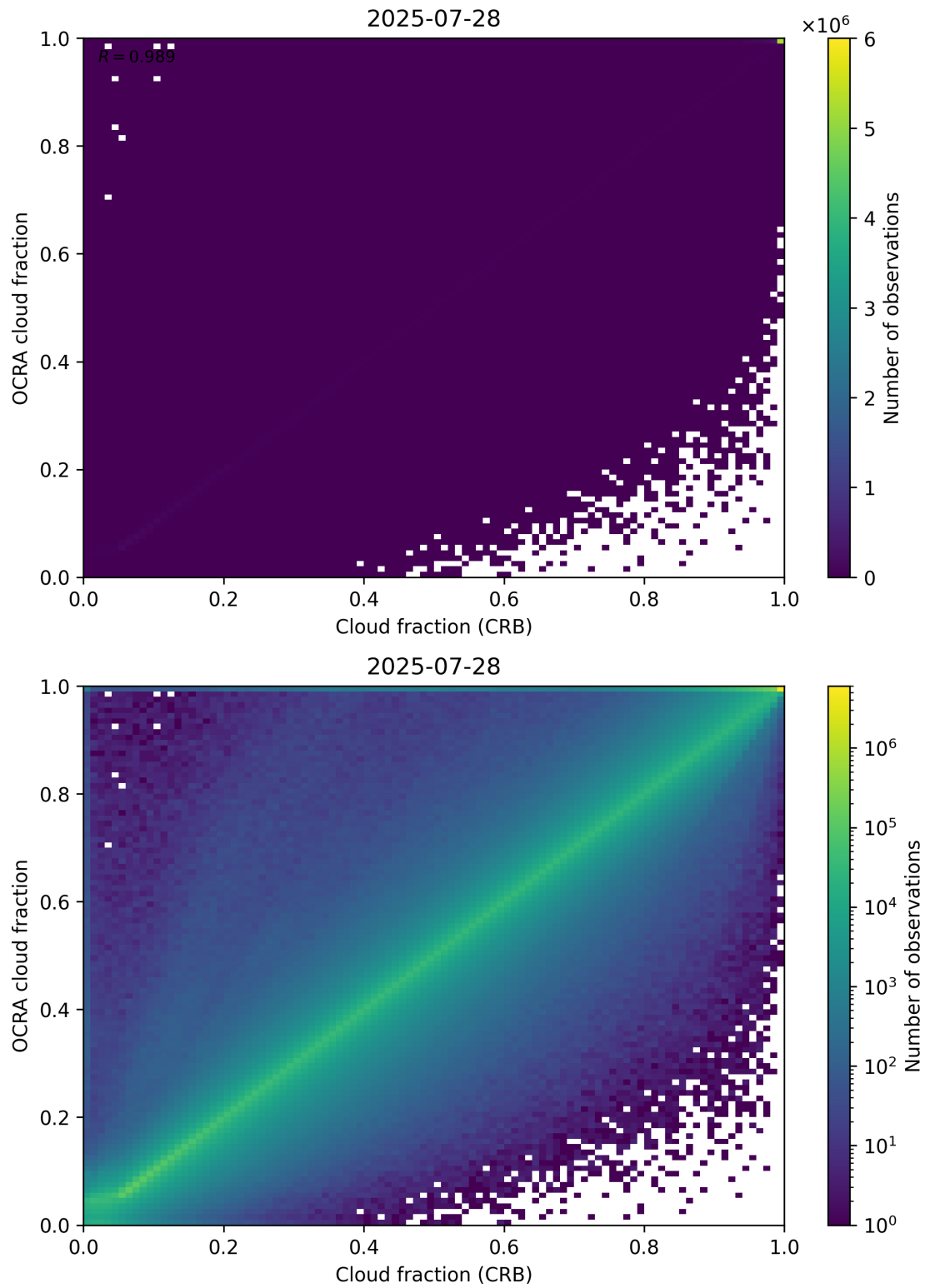
Figure 78: Scatter density plot of “Cloud fraction (CRB)” against “OCRA cloud fraction” for 2025-07-27 to 2025-07-29.
