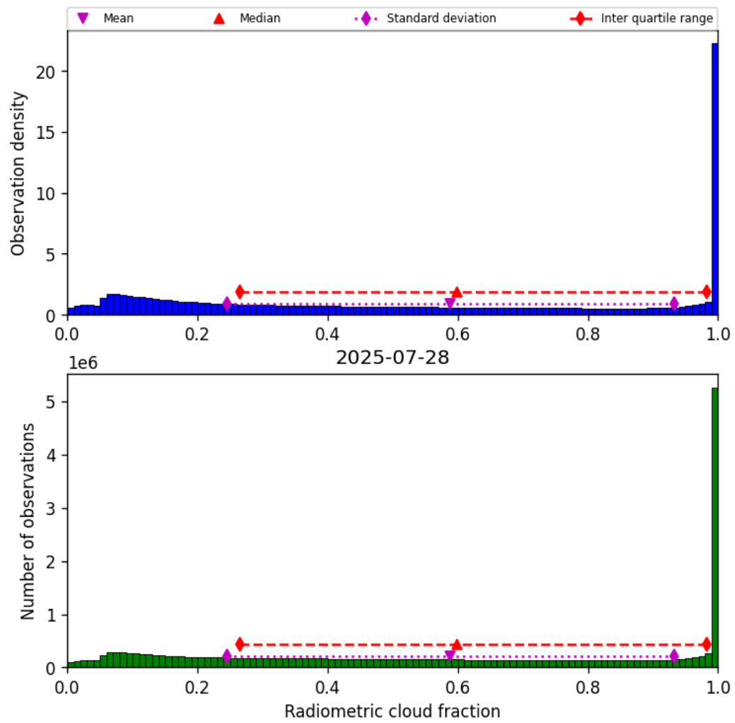
Figure 39: Histogram of “Radiometric cloud fraction” for 2025-07-27 to 2025-07-29
