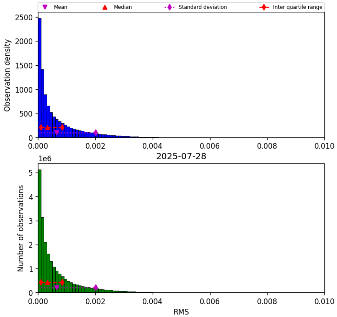
Figure 47: Histogram of “RMS” for 2025-07-27 to 2025-07-29
