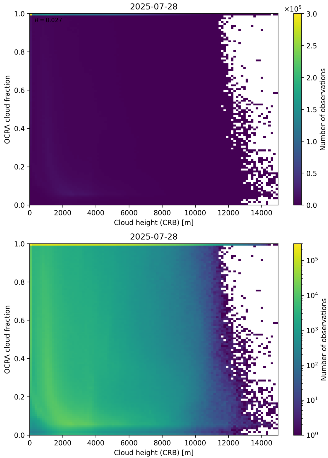
Figure 81: Scatter density plot of “Cloud height (CRB)” against “OCRA cloud fraction” for 2025-07-27 to 2025-07-29.
