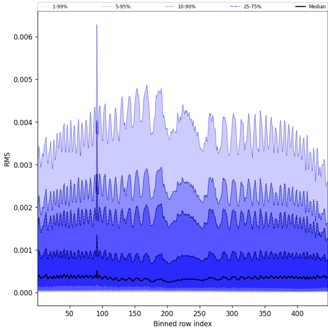
Figure 63: Along track statistics of “RMS” for 2025-07-27 to 2025-07-29
