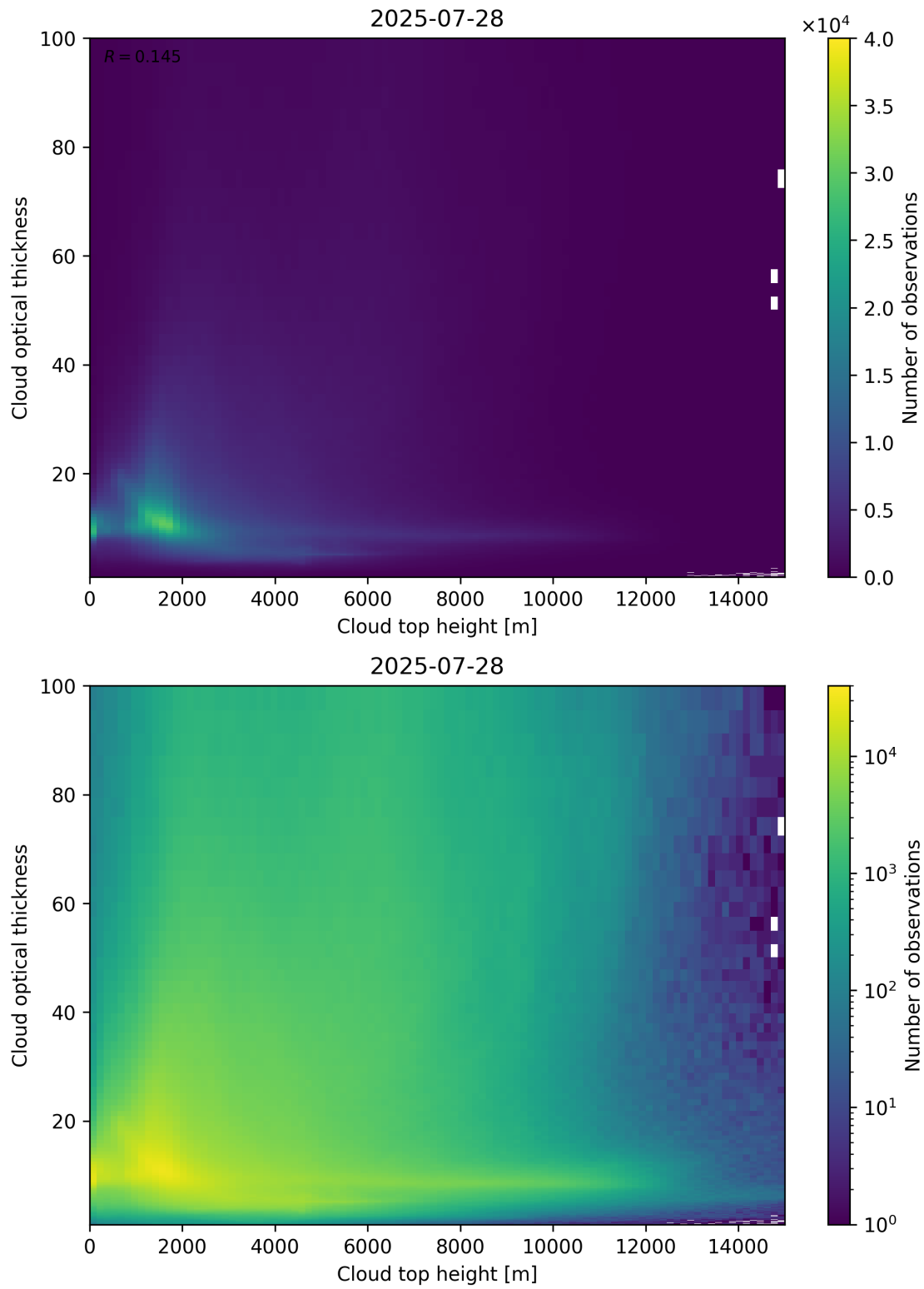
Figure 90: Scatter density plot of “Cloud top height” against “Cloud optical thickness” for 2025-07-27 to 2025-07-29.
