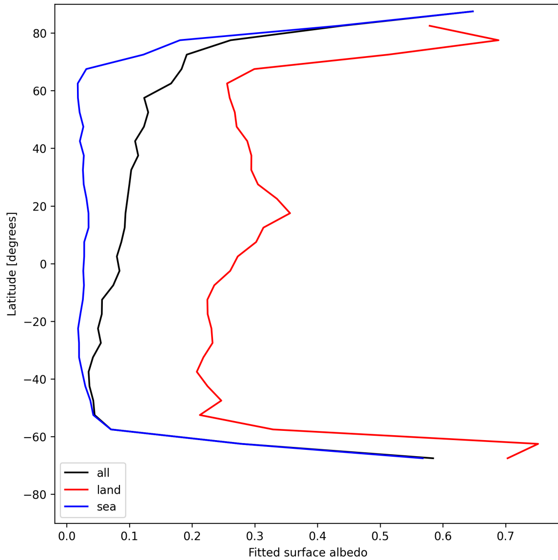
Figure 29: Zonal average of “Fitted surface albedo” for 2025-07-27 to 2025-07-29.
