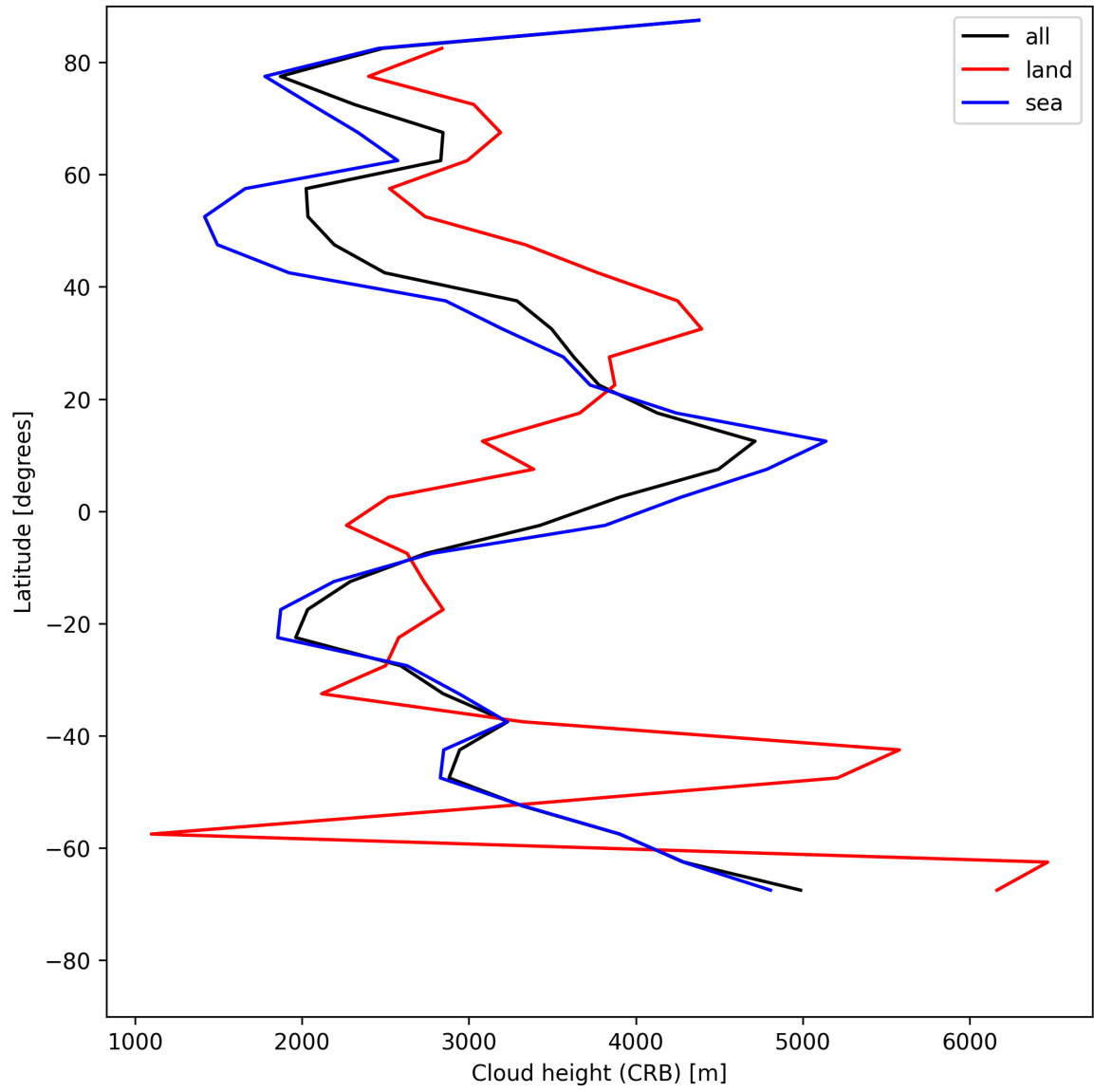
Figure 27: Zonal average of “Cloud height (CRB)” for 2025-07-27 to 2025-07-29.
