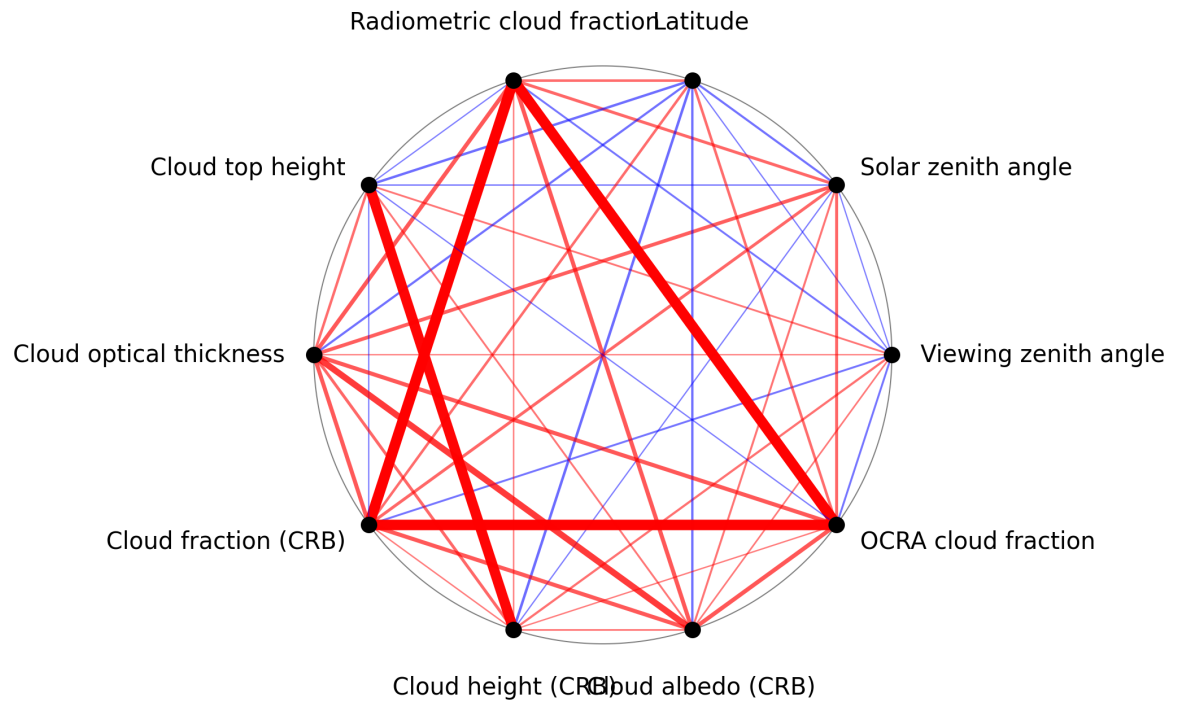
Figure 1: Map of correlation graph for 2025-07-27 to 2025-07-29.
