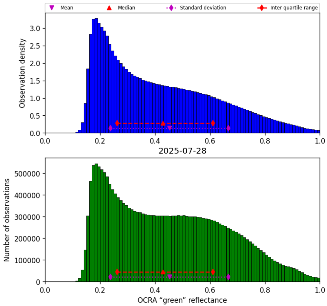
Figure 52: Histogram of “OCRA “green” reflectance” for 2025-07-27 to 2025-07-29
