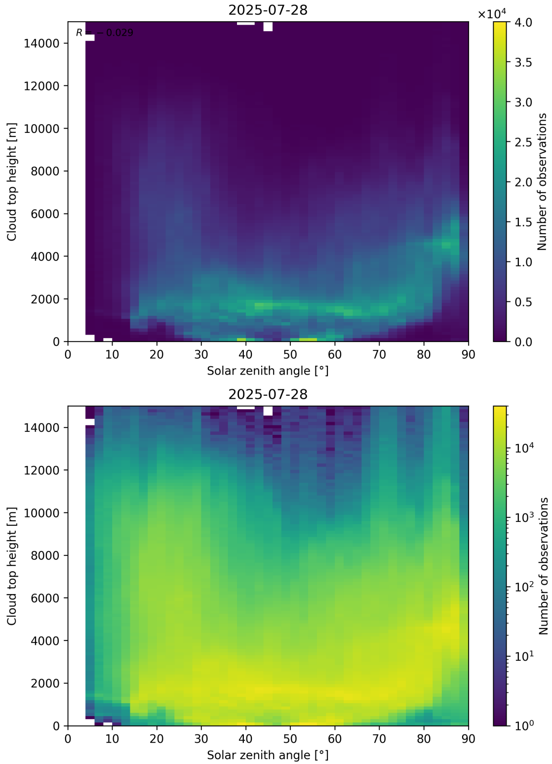
Figure 104: Scatter density plot of “Solar zenith angle” against “Cloud top height” for 2025-07-27 to 2025-07-29.
