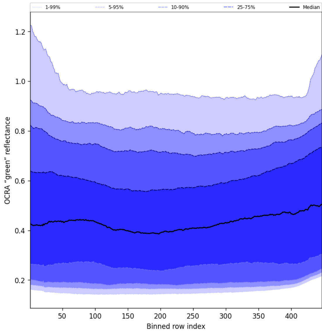
Figure 68: Along track statistics of “OCRA “green” reflectance” for 2025-07-27 to 2025-07-29
