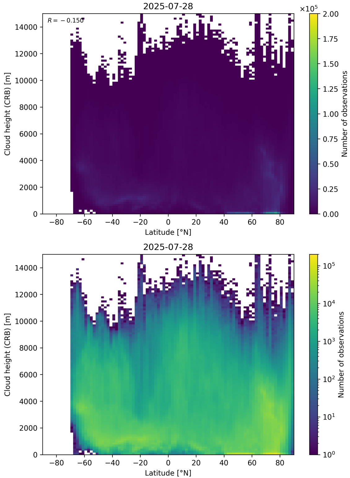
Figure 95: Scatter density plot of “Latitude” against “Cloud height (CRB)” for 2025-07-27 to 2025-07-29.
