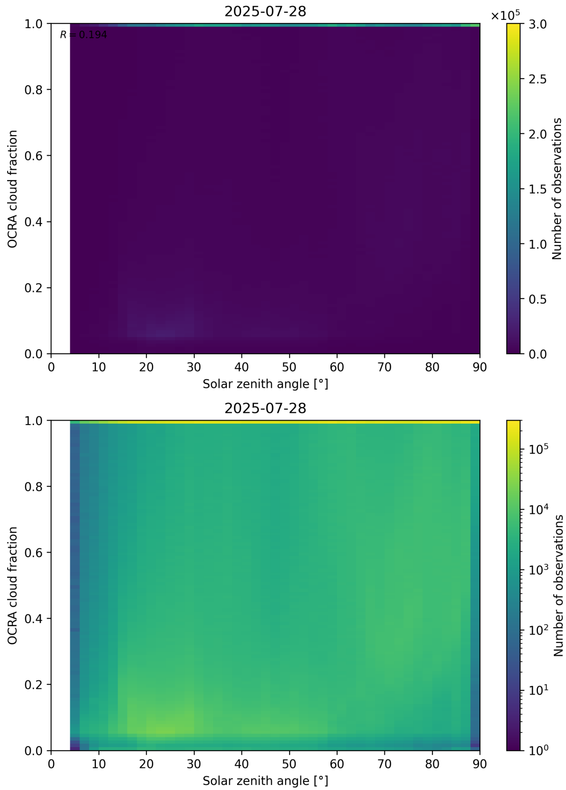
Figure 100: Scatter density plot of “Solar zenith angle” against “OCRA cloud fraction” for 2025-07-27 to 2025-07-29.
