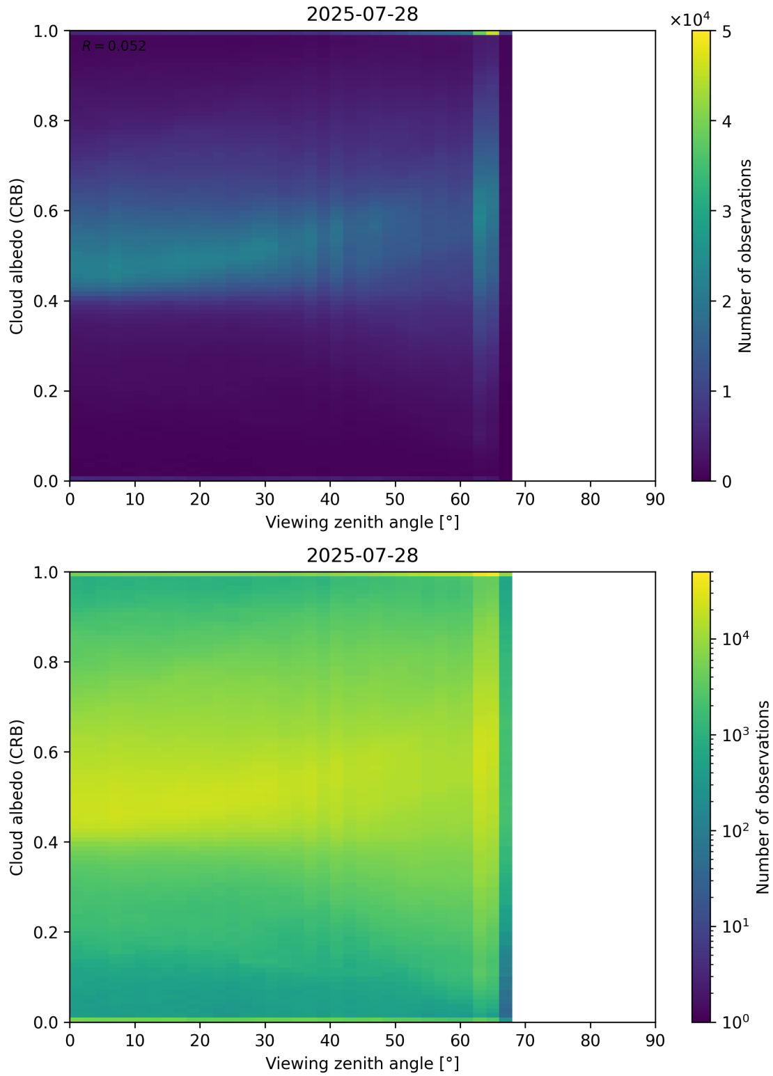
Figure 106: Scatter density plot of “Viewing zenith angle” against “Cloud albedo (CRB)” for 2025-07-27 to 2025-07-29.
