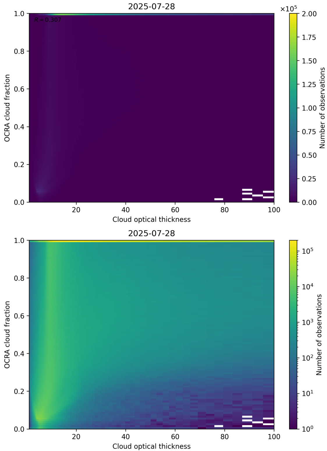
Figure 83: Scatter density plot of “Cloud optical thickness” against “OCRA cloud fraction” for 2025-07-27 to 2025-07-29.
