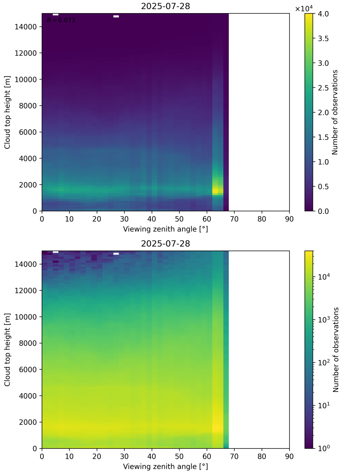
Figure 112: Scatter density plot of “Viewing zenith angle” against “Cloud top height” for 2025-07-27 to 2025-07-29.
