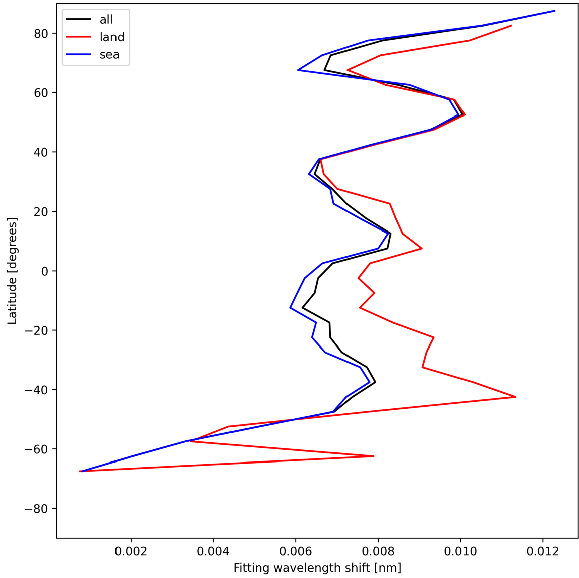
Figure 33: Zonal average of “Fitting wavelength shift” for 2025-07-27 to 2025-07-29.
