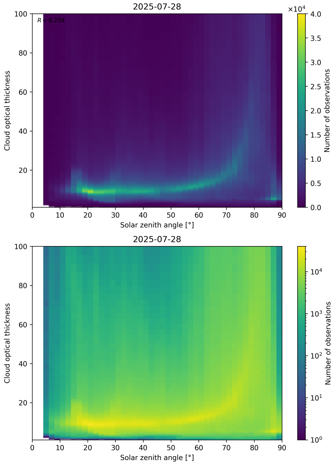
Figure 103: Scatter density plot of “Solar zenith angle” against “Cloud optical thickness” for 2025-07-27 to 2025-07-29.
