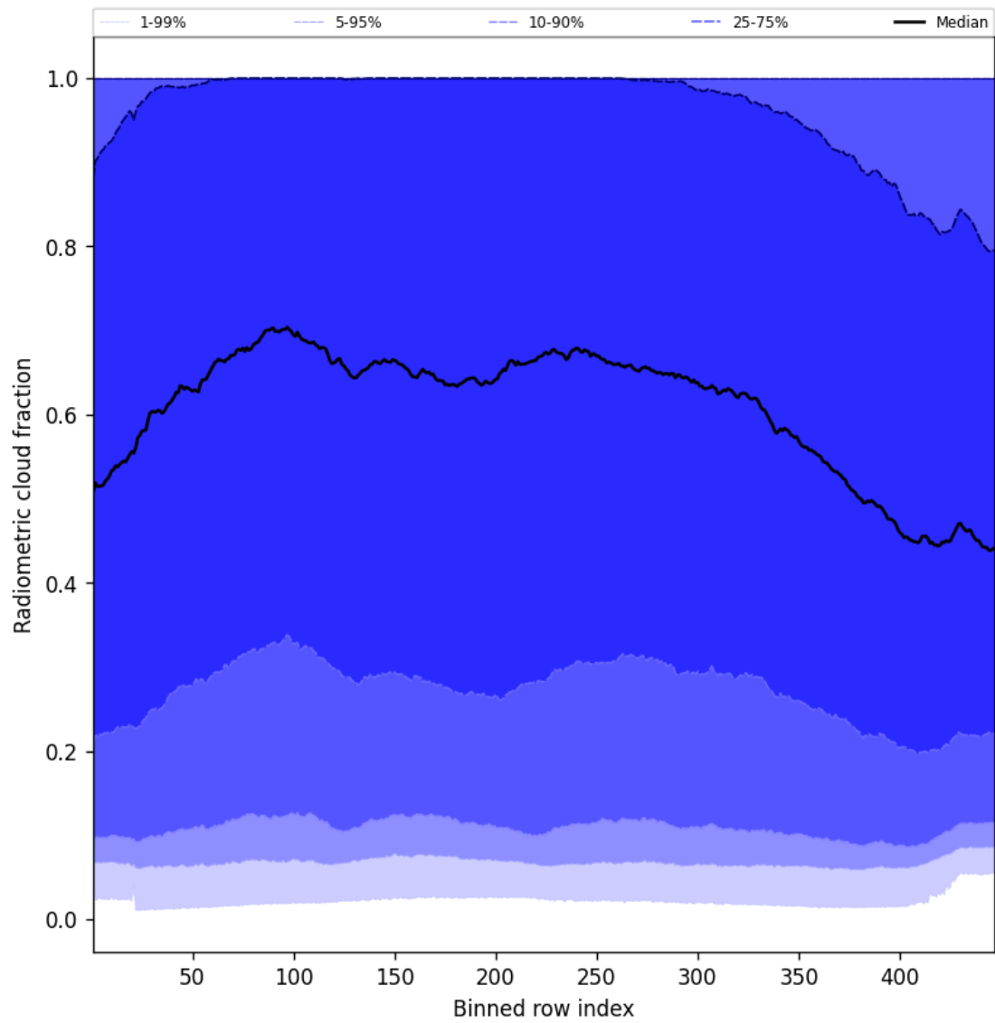
Figure 55: Along track statistics of “Radiometric cloud fraction” for 2025-07-27 to 2025-07-29
