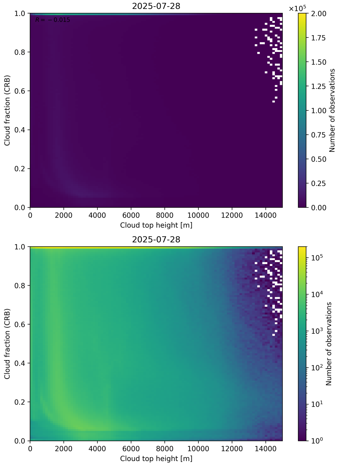
Figure 88: Scatter density plot of “Cloud top height” against “Cloud fraction (CRB)” for 2025-07-27 to 2025-07-29.
