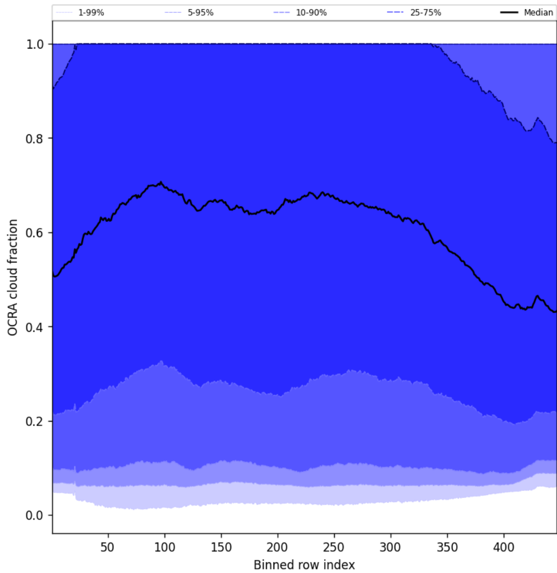
Figure 66: Along track statistics of “OCRA cloud fraction” for 2025-07-27 to 2025-07-29
