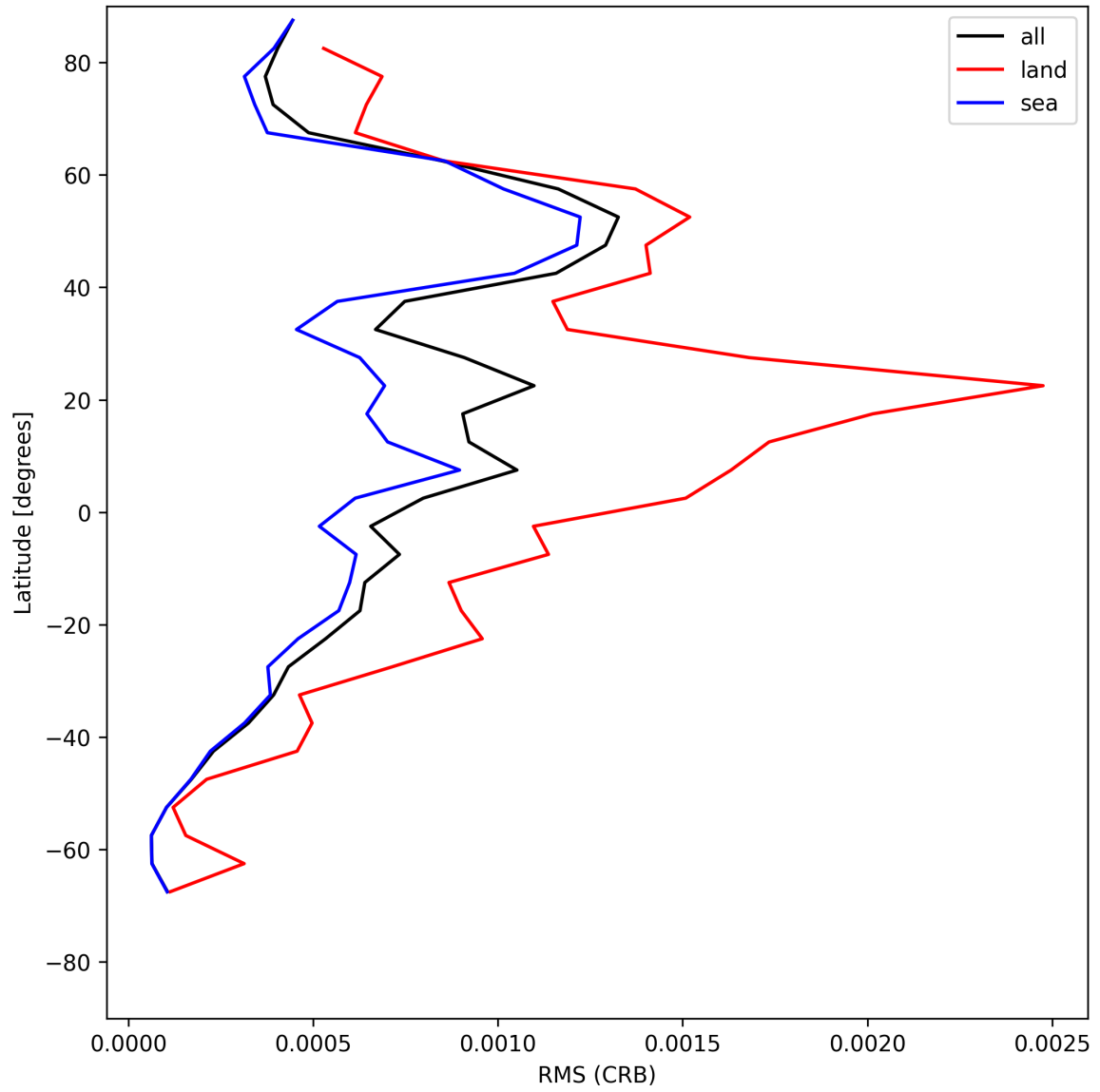
Figure 32: Zonal average of “RMS (CRB)” for 2025-07-27 to 2025-07-29.
