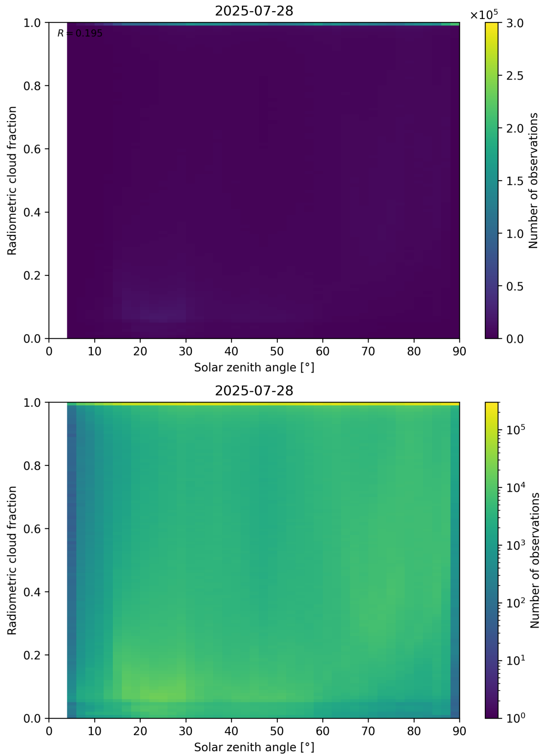
Figure 99: Scatter density plot of “Solar zenith angle” against “Radiometric cloud fraction” for 2025-07-27 to 2025-07-29.
