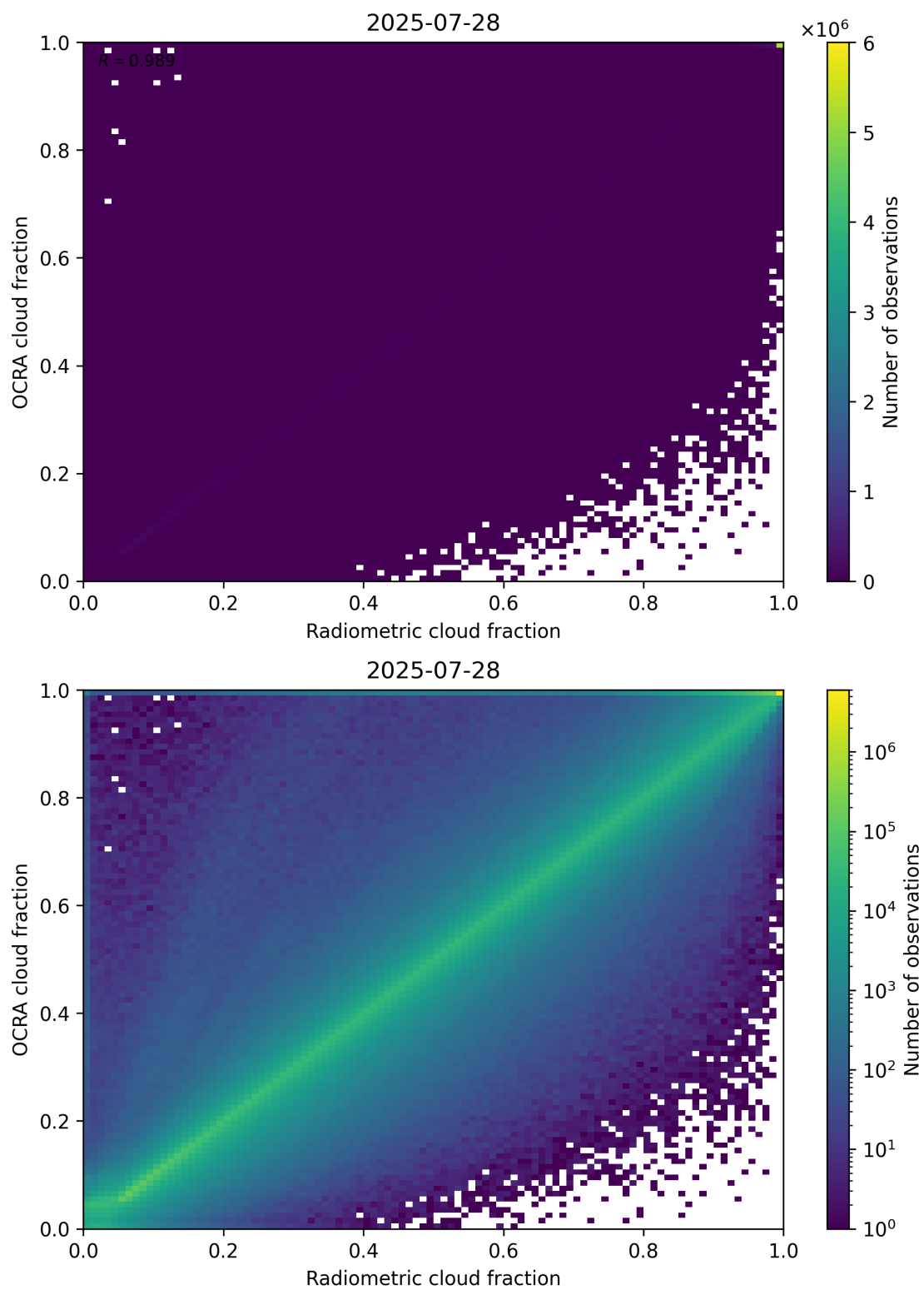
Figure 72: Scatter density plot of “Radiometric cloud fraction” against “OCRA cloud fraction” for 2025-07-27 to 2025-07-29.
