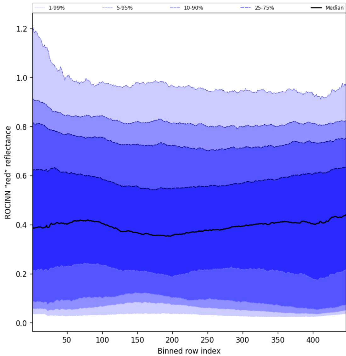
Figure 69: Along track statistics of "ROCINN "red" reflectance" for 2025-07-27 to 2025-07-29
