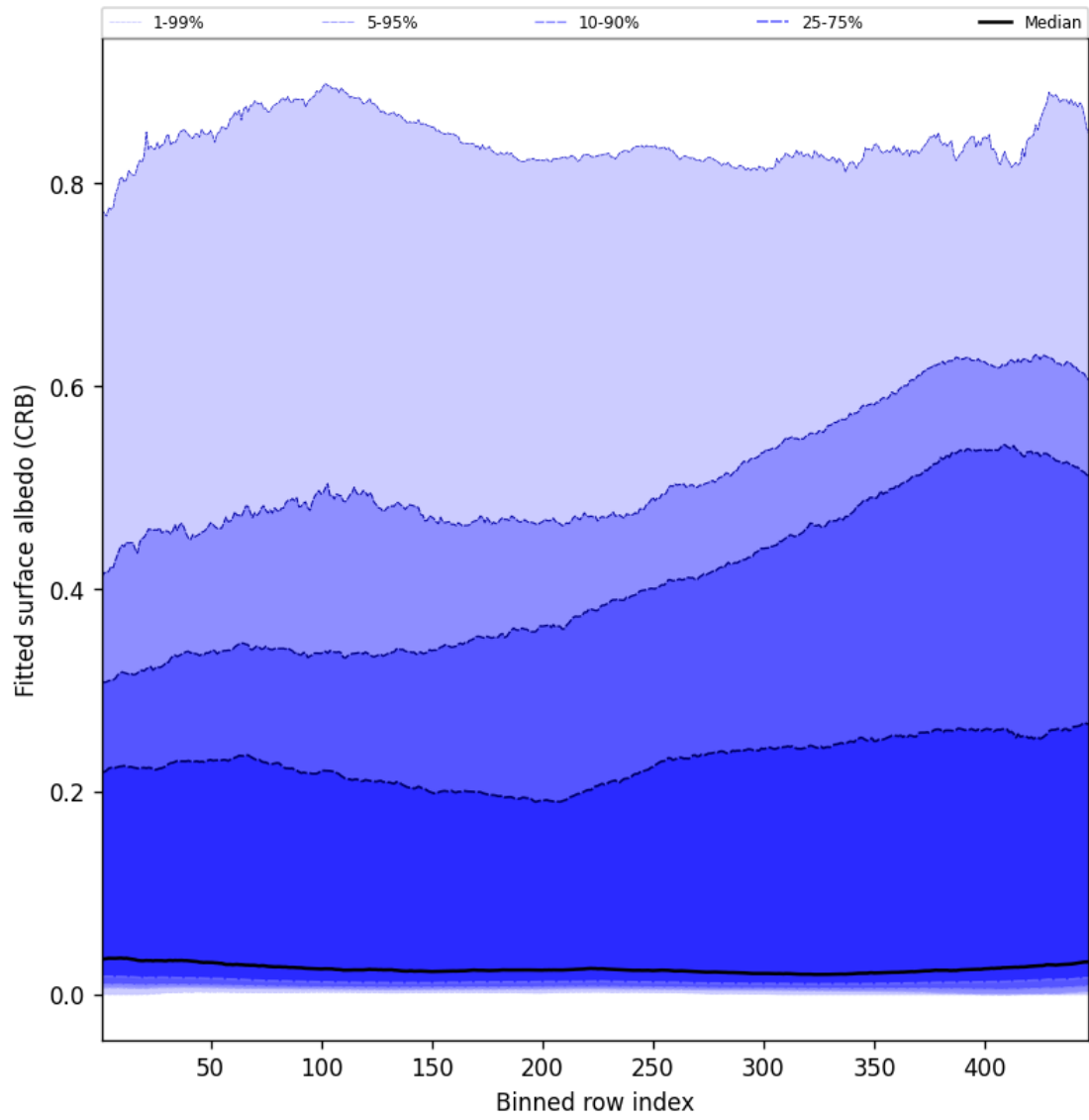
Figure 62: Along track statistics of “Fitted surface albedo (CRB)” for 2025-07-27 to 2025-07-29
