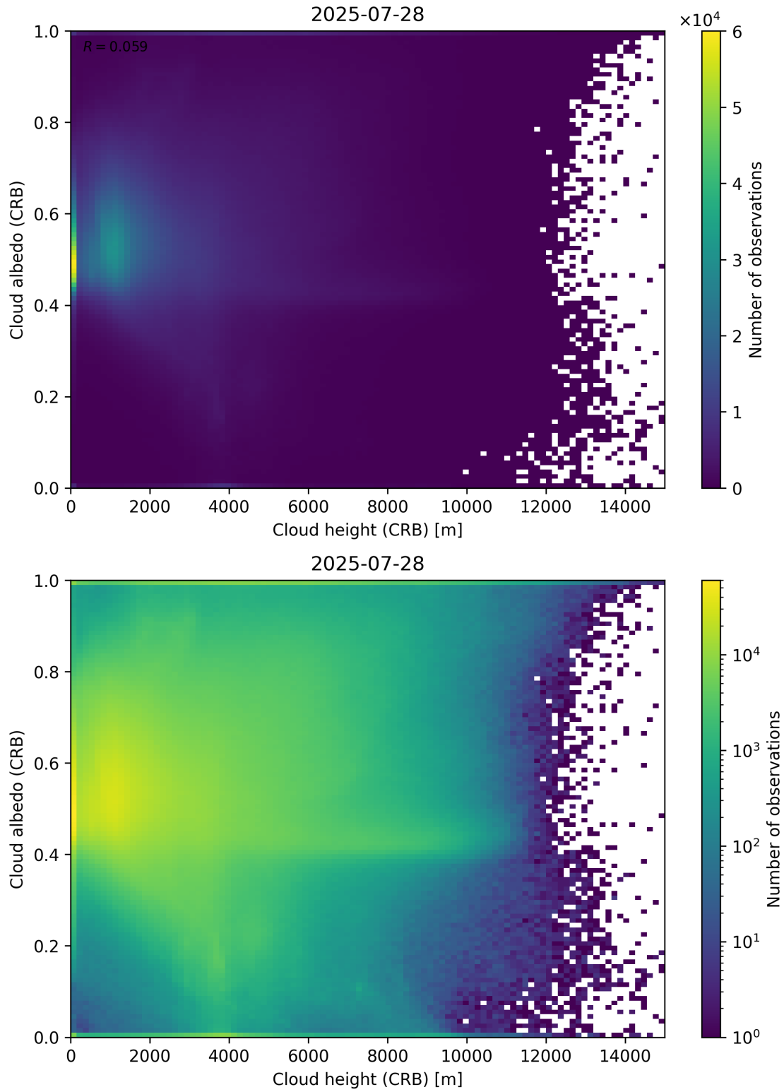
Figure 80: Scatter density plot of “Cloud height (CRB)” against “Cloud albedo (CRB)” for 2025-07-27 to 2025-07-29.
