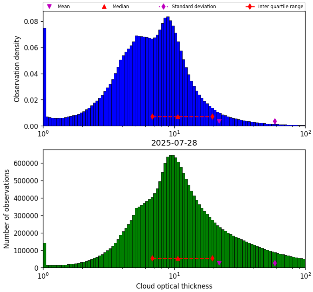
Figure 41: Histogram of “Cloud optical thickness” for 2025-07-27 to 2025-07-29
