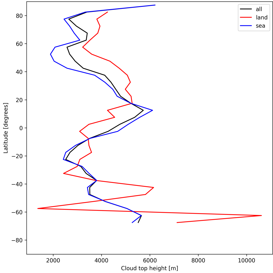
Figure 24: Zonal average of “Cloud top height” for 2025-07-27 to 2025-07-29.
