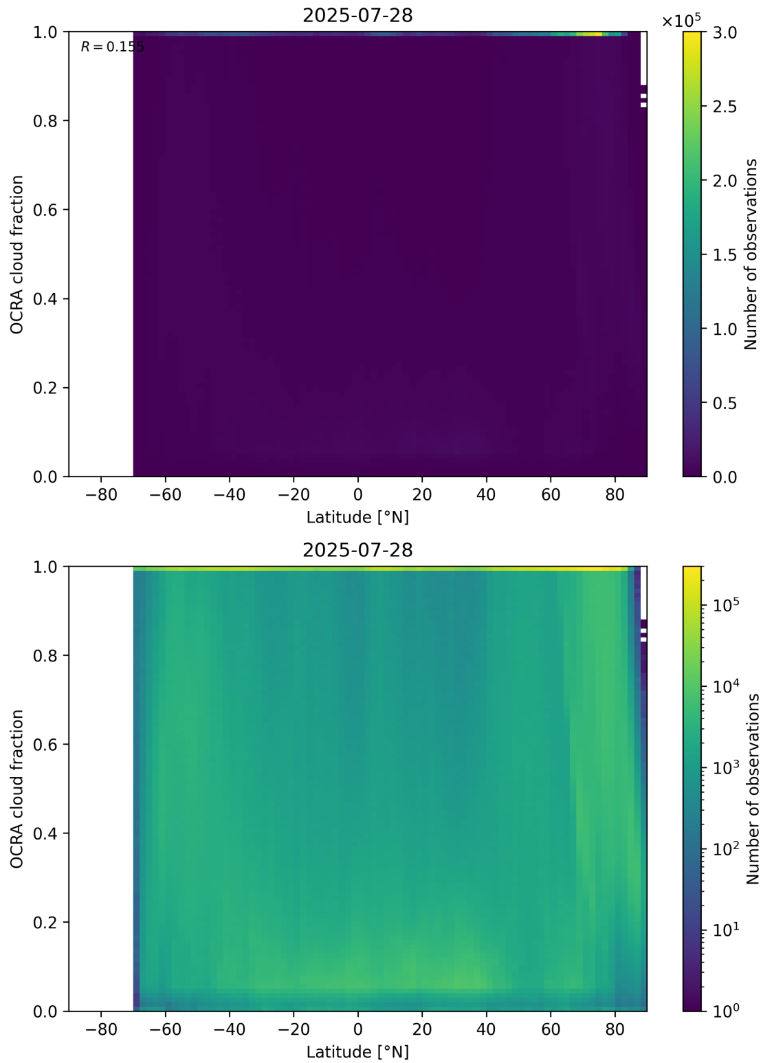
Figure 93: Scatter density plot of “Latitude” against “OCRA cloud fraction” for 2025-07-27 to 2025-07-29.
