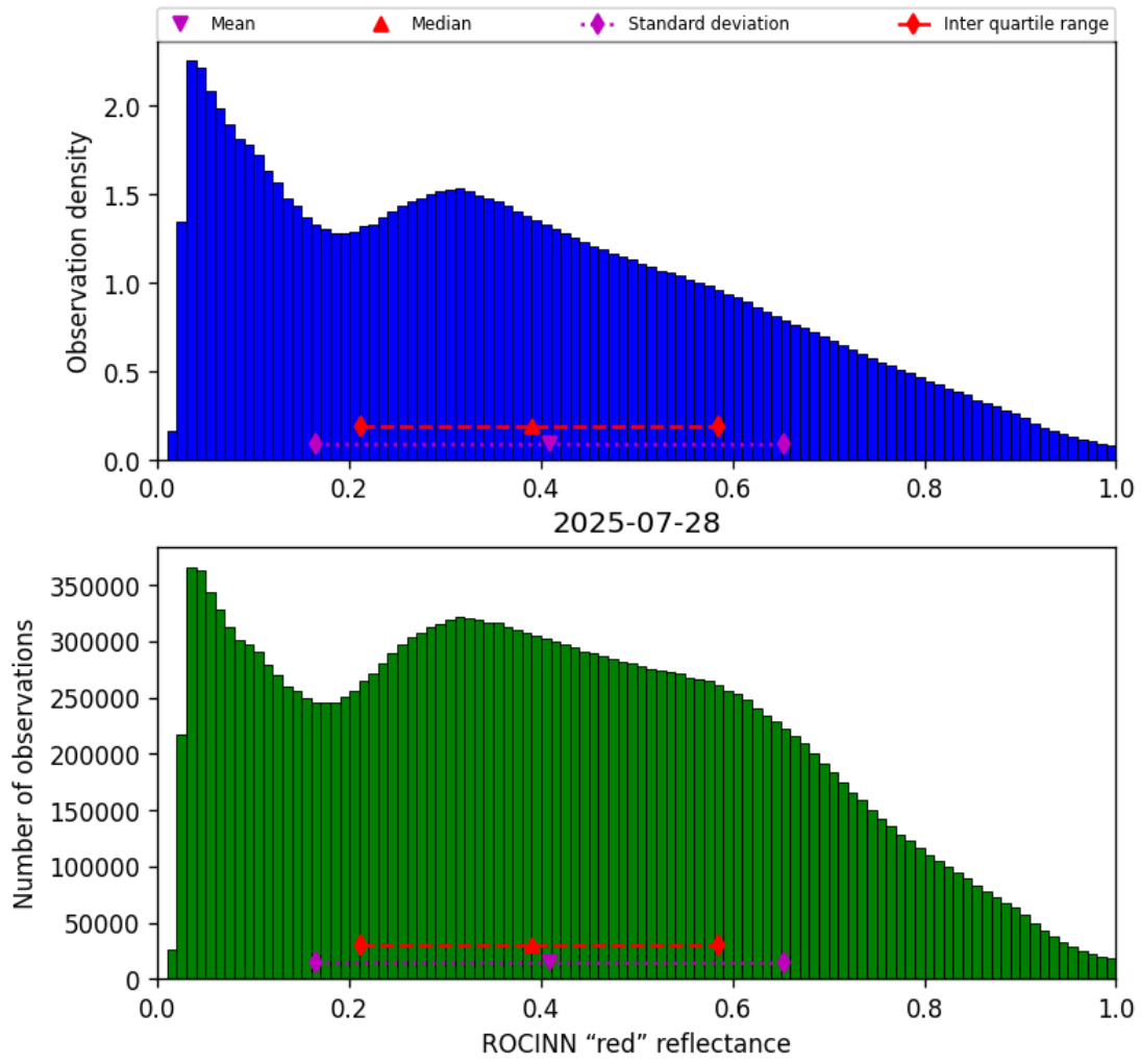
Figure 53: Histogram of “ROCINN “red” reflectance” for 2025-07-27 to 2025-07-29
