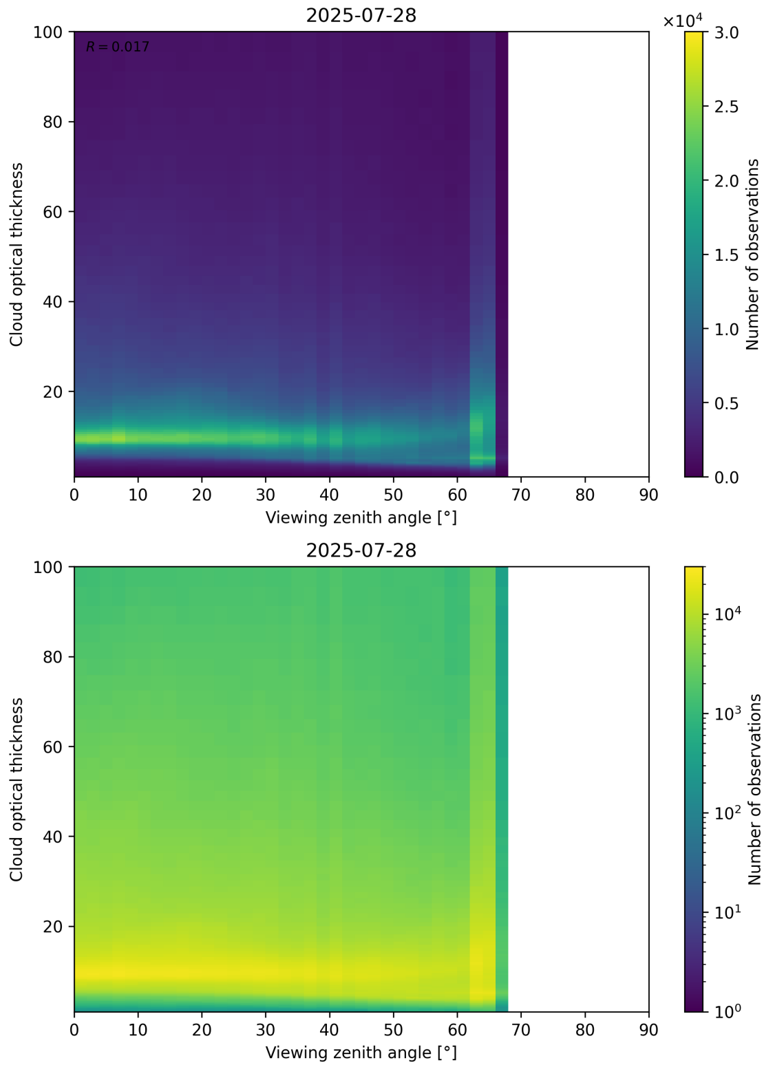
Figure 111: Scatter density plot of “Viewing zenith angle” against “Cloud optical thickness” for 2025-07-27 to 2025-07-29.
