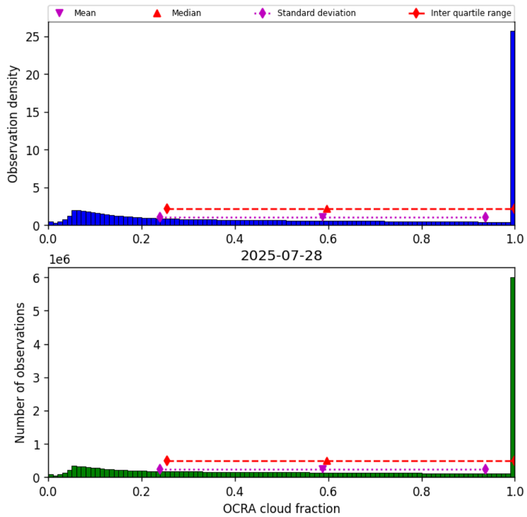
Figure 50: Histogram of “OCRA cloud fraction” for 2025-07-27 to 2025-07-29
