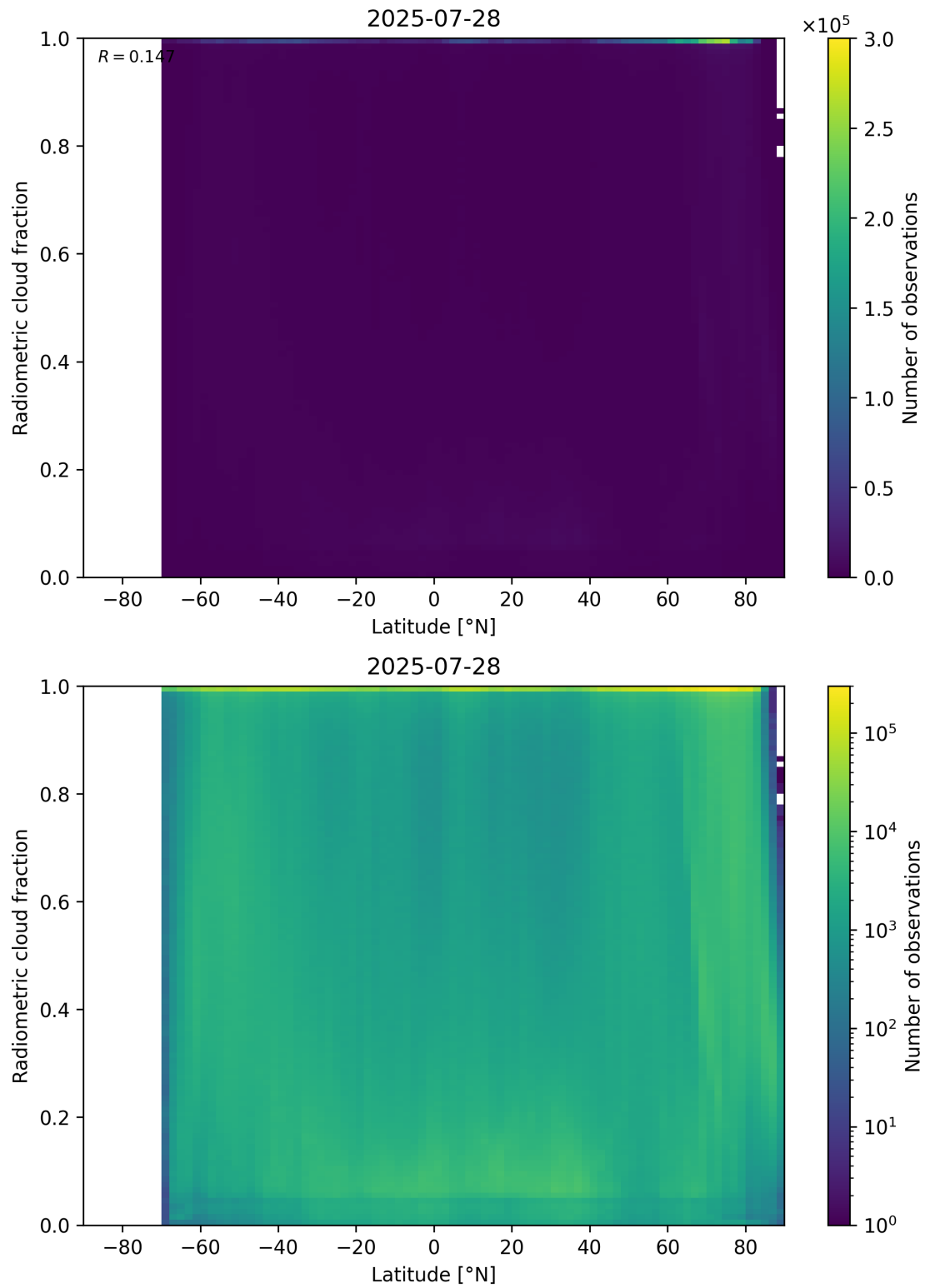
Figure 92: Scatter density plot of “Latitude” against “Radiometric cloud fraction” for 2025-07-27 to 2025-07-29.
