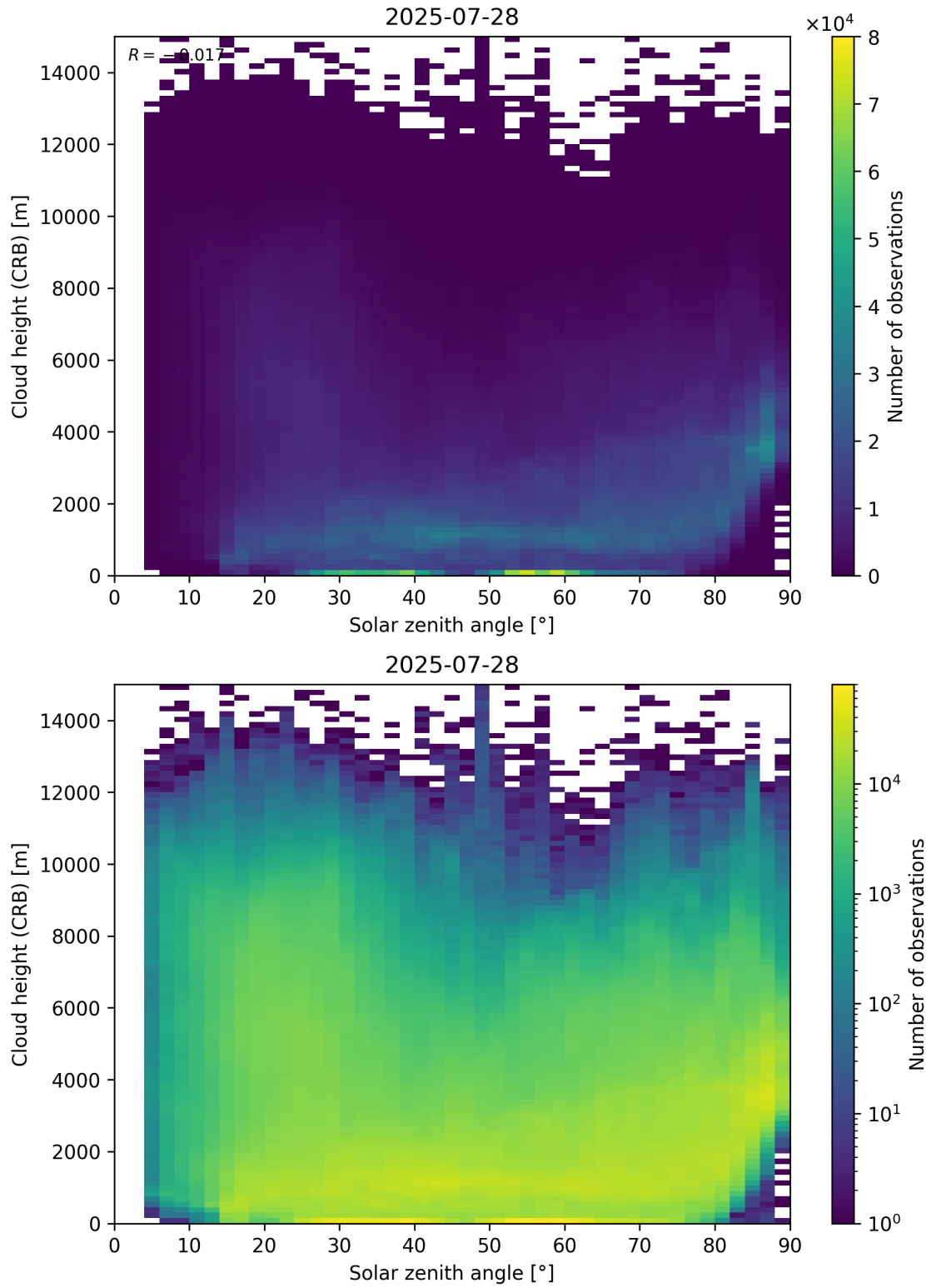
Figure 102: Scatter density plot of “Solar zenith angle” against “Cloud height (CRB)” for 2025-07-27 to 2025-07-29.
