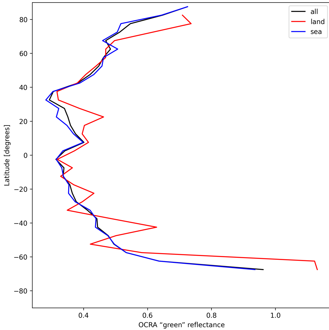
Figure 36: Zonal average of “OCRA “green” reflectance” for 2025-07-27 to 2025-07-29.
