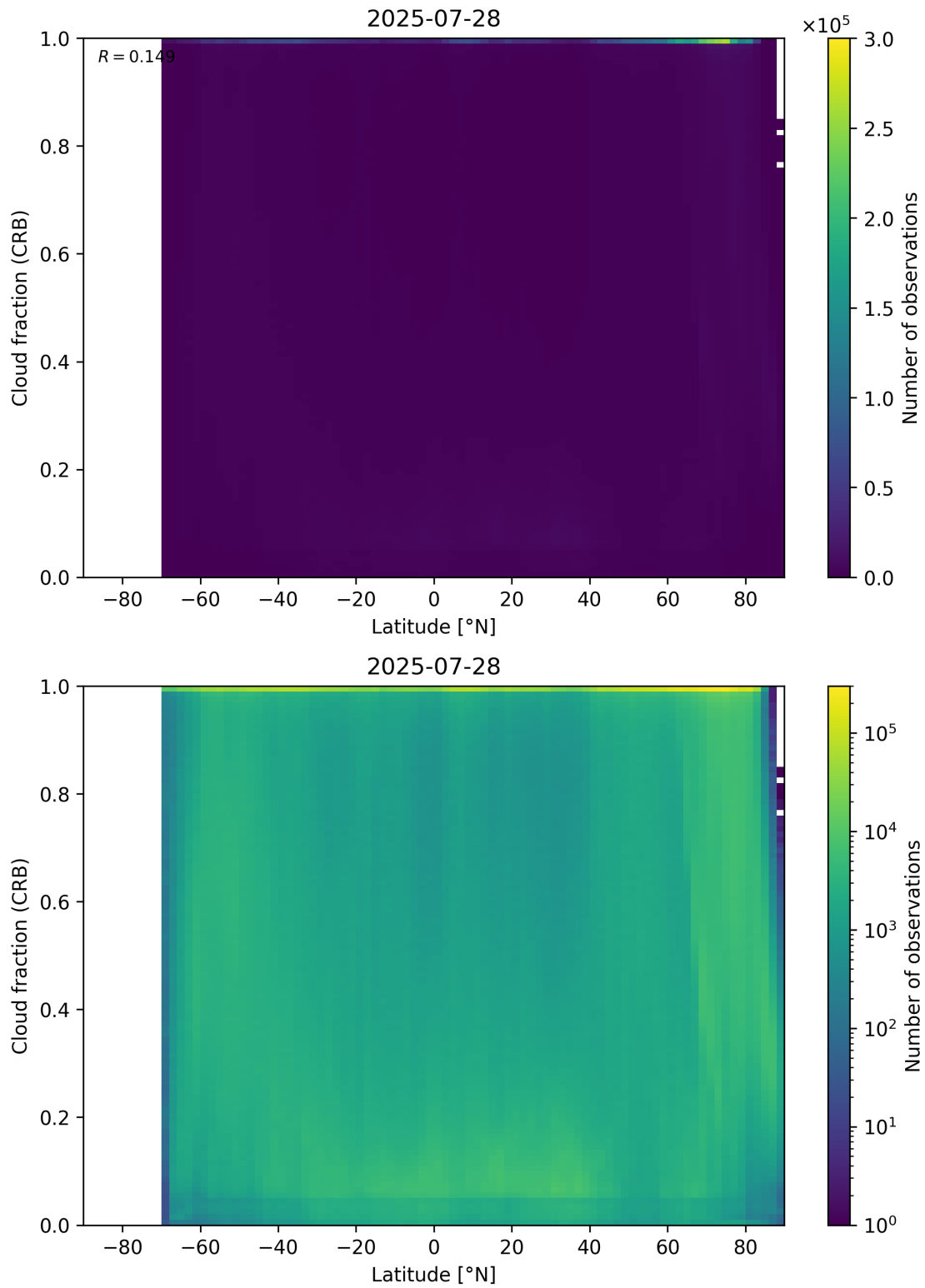
Figure 94: Scatter density plot of “Latitude” against “Cloud fraction (CRB)” for 2025-07-27 to 2025-07-29.
