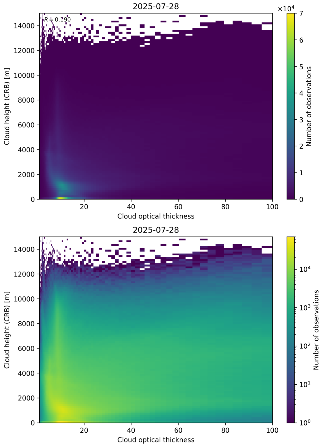
Figure 85: Scatter density plot of “Cloud optical thickness” against “Cloud height (CRB)” for 2025-07-27 to 2025-07-29.
