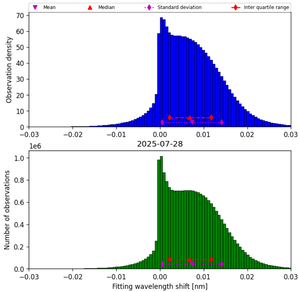
Figure 49: Histogram of “Fitting wavelength shift” for 2025-07-27 to 2025-07-29
