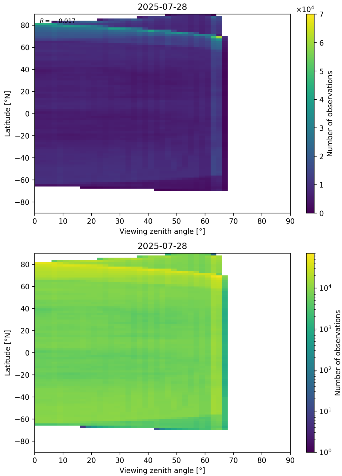
Figure 113: Scatter density plot of “Viewing zenith angle” against “Latitude” for 2025-07-27 to 2025-07-29.
