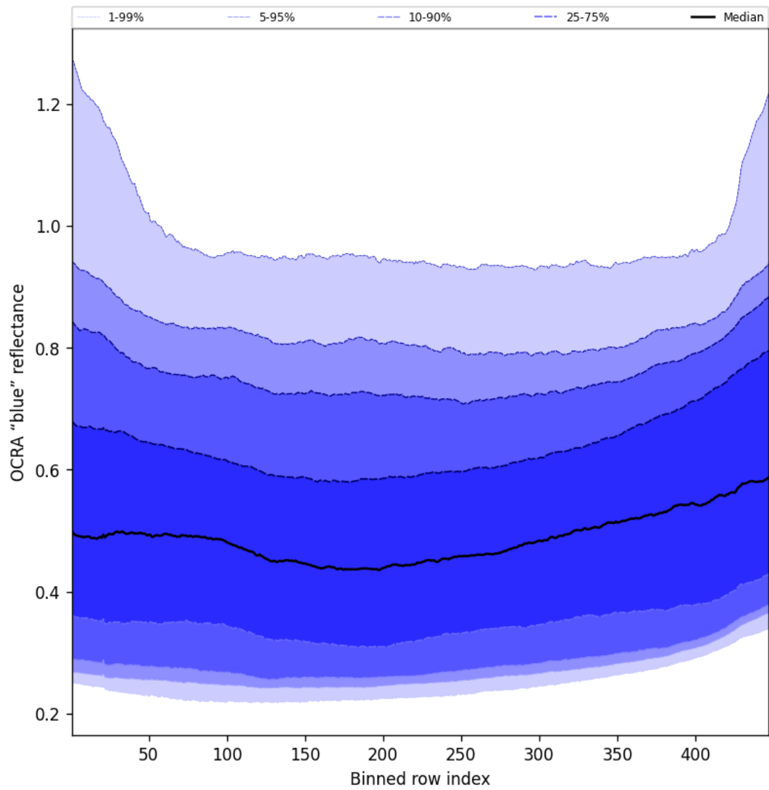
Figure 67: Along track statistics of “OCRA “blue” reflectance” for 2025-07-27 to 2025-07-29
