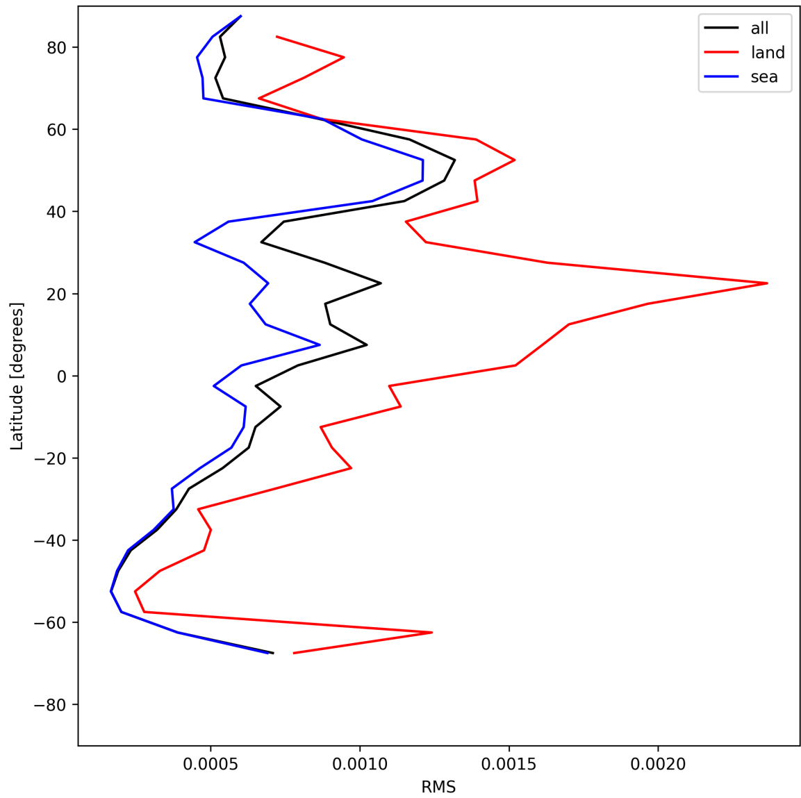
Figure 31: Zonal average of “RMS” for 2025-07-27 to 2025-07-29.
