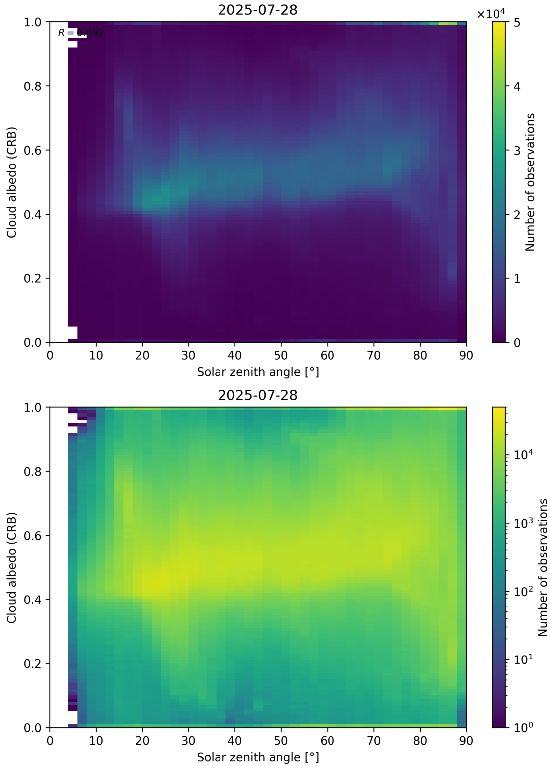
Figure 98: Scatter density plot of “Solar zenith angle” against “Cloud albedo (CRB)” for 2025-07-27 to 2025-07-29.
