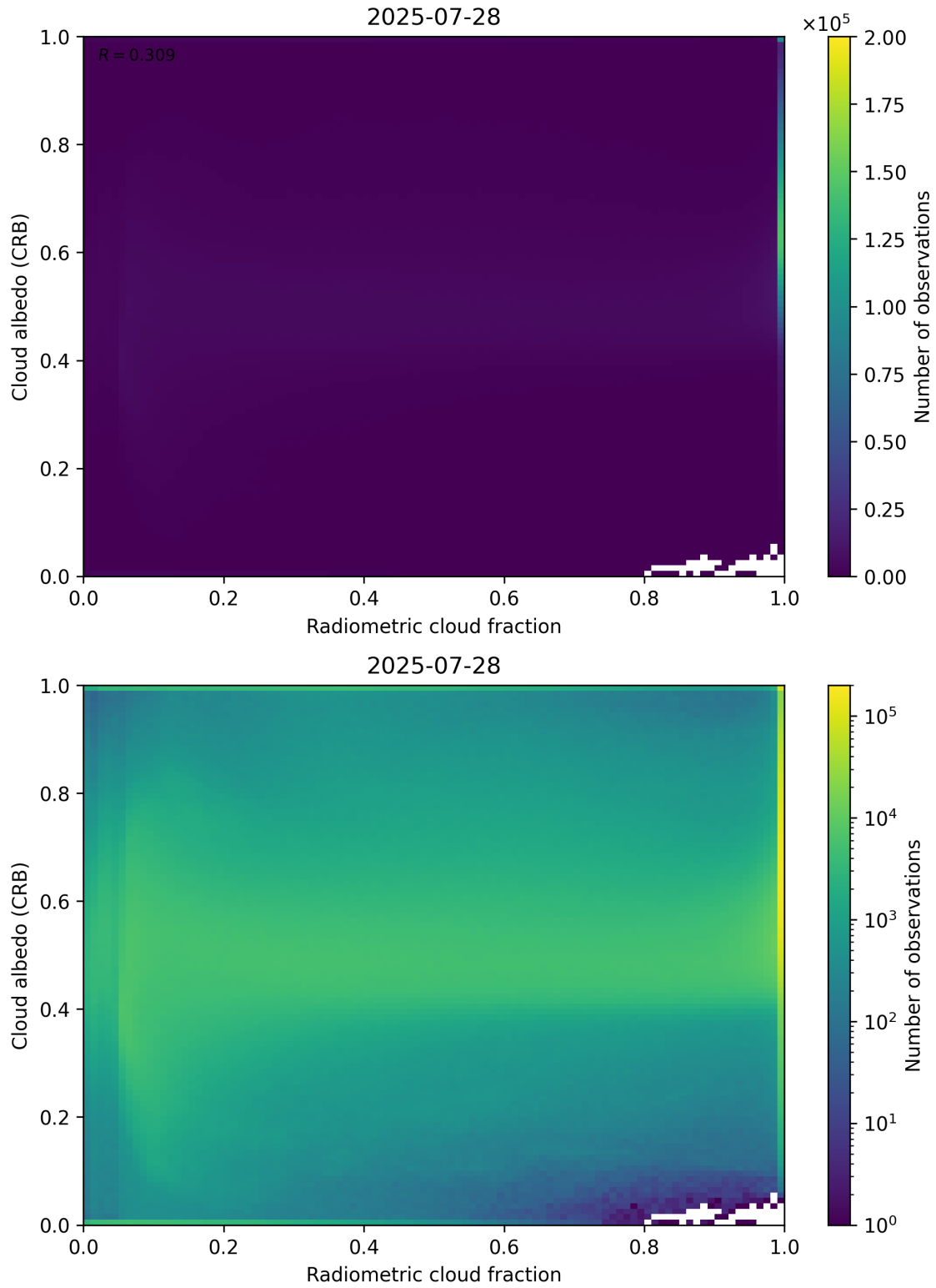
Figure 71: Scatter density plot of “Radiometric cloud fraction” against “Cloud albedo (CRB)” for 2025-07-27 to 2025-07-29.
