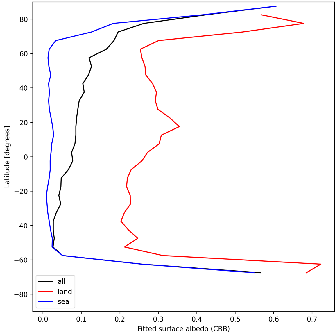
Figure 30: Zonal average of “Fitted surface albedo (CRB)” for 2025-07-27 to 2025-07-29.
