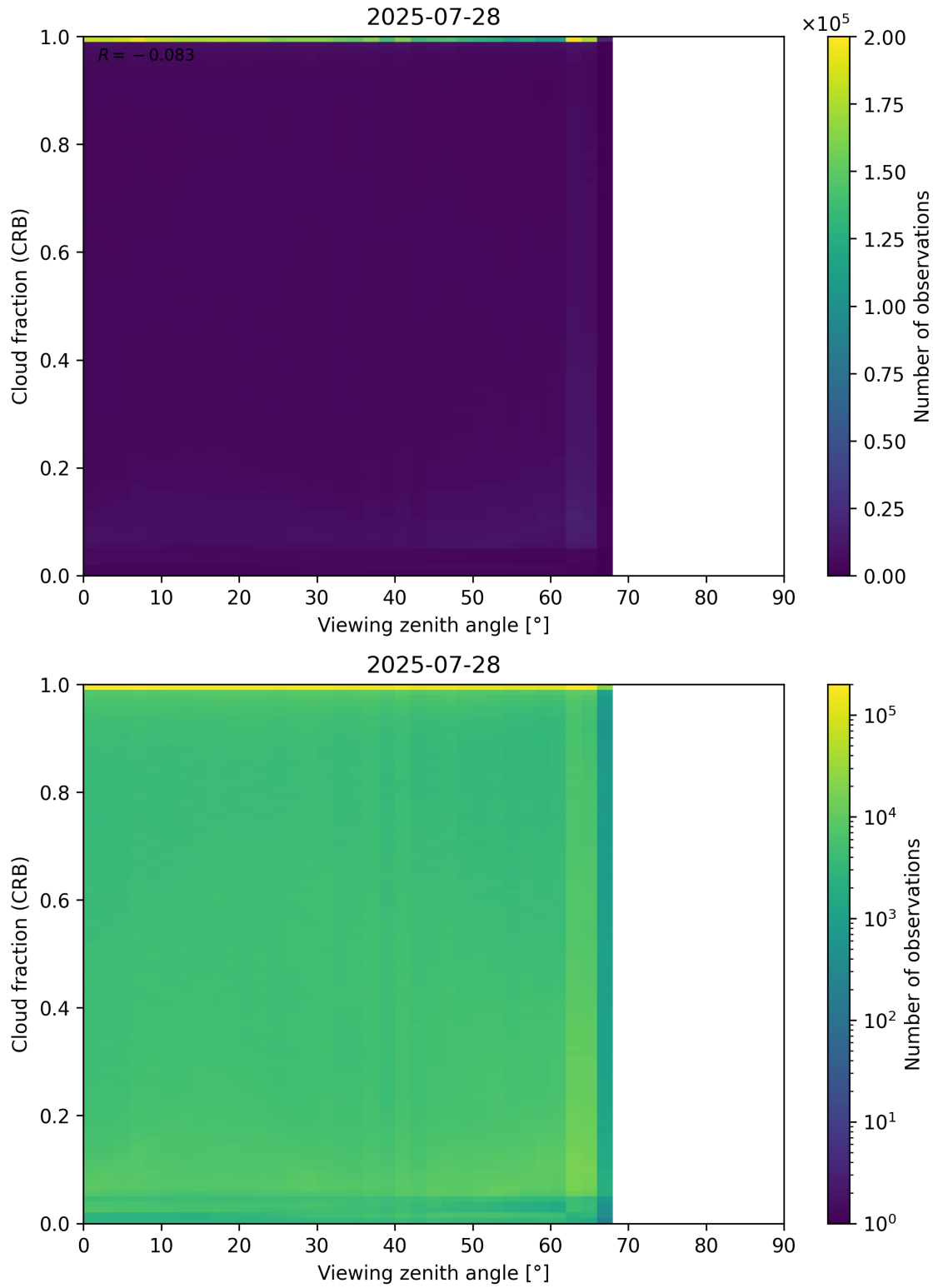
Figure 109: Scatter density plot of “Viewing zenith angle” against “Cloud fraction (CRB)” for 2025-07-27 to 2025-07-29.
