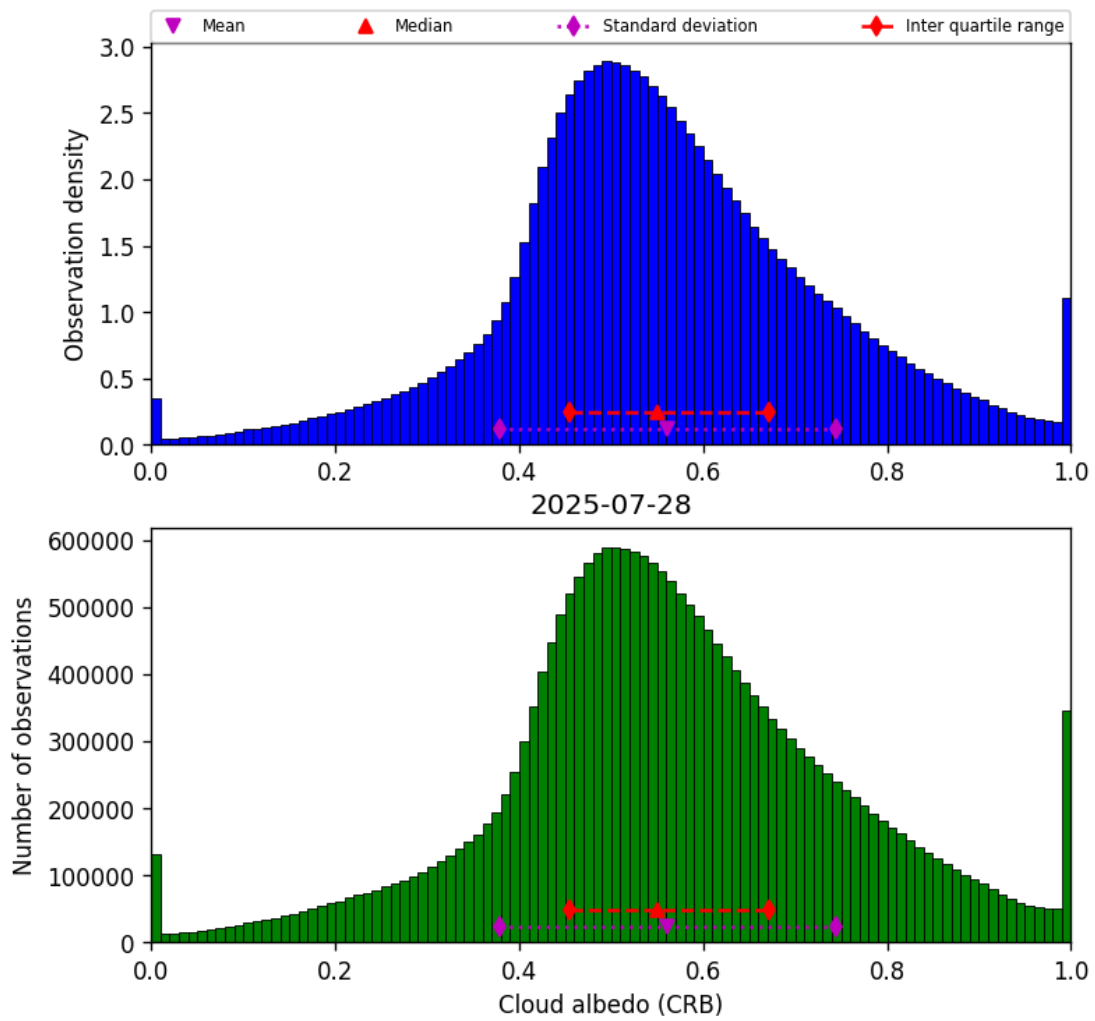
Figure 44: Histogram of “Cloud albedo (CRB)” for 2025-07-27 to 2025-07-29
