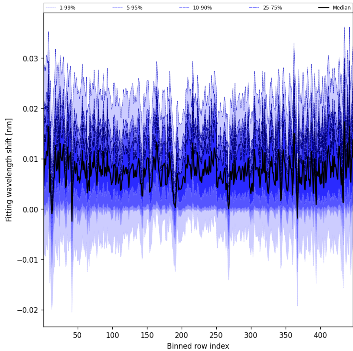
Figure 65: Along track statistics of “Fitting wavelength shift” for 2025-07-27 to 2025-07-29
