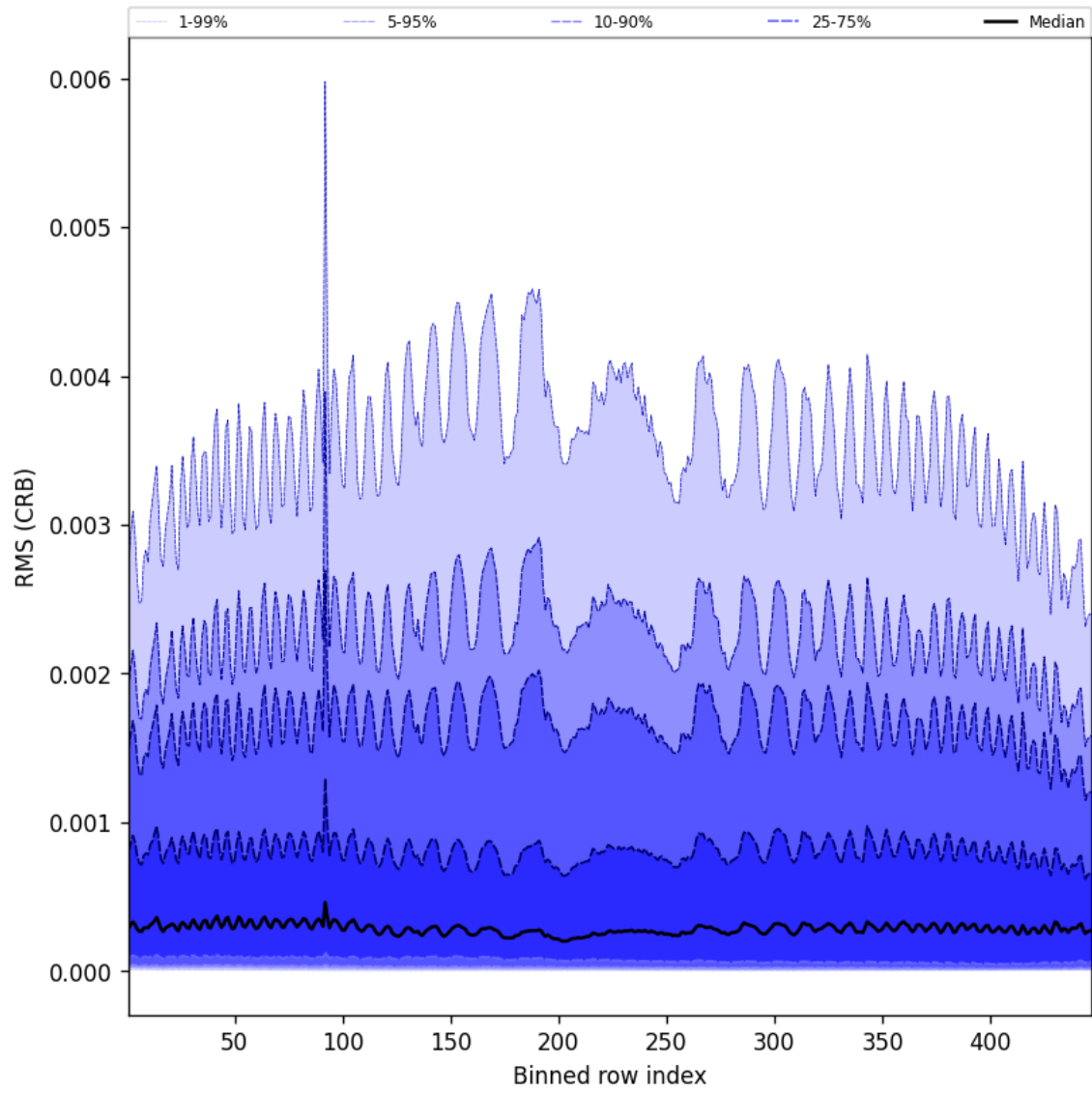
Figure 64: Along track statistics of “RMS (CRB)” for 2025-07-27 to 2025-07-29
