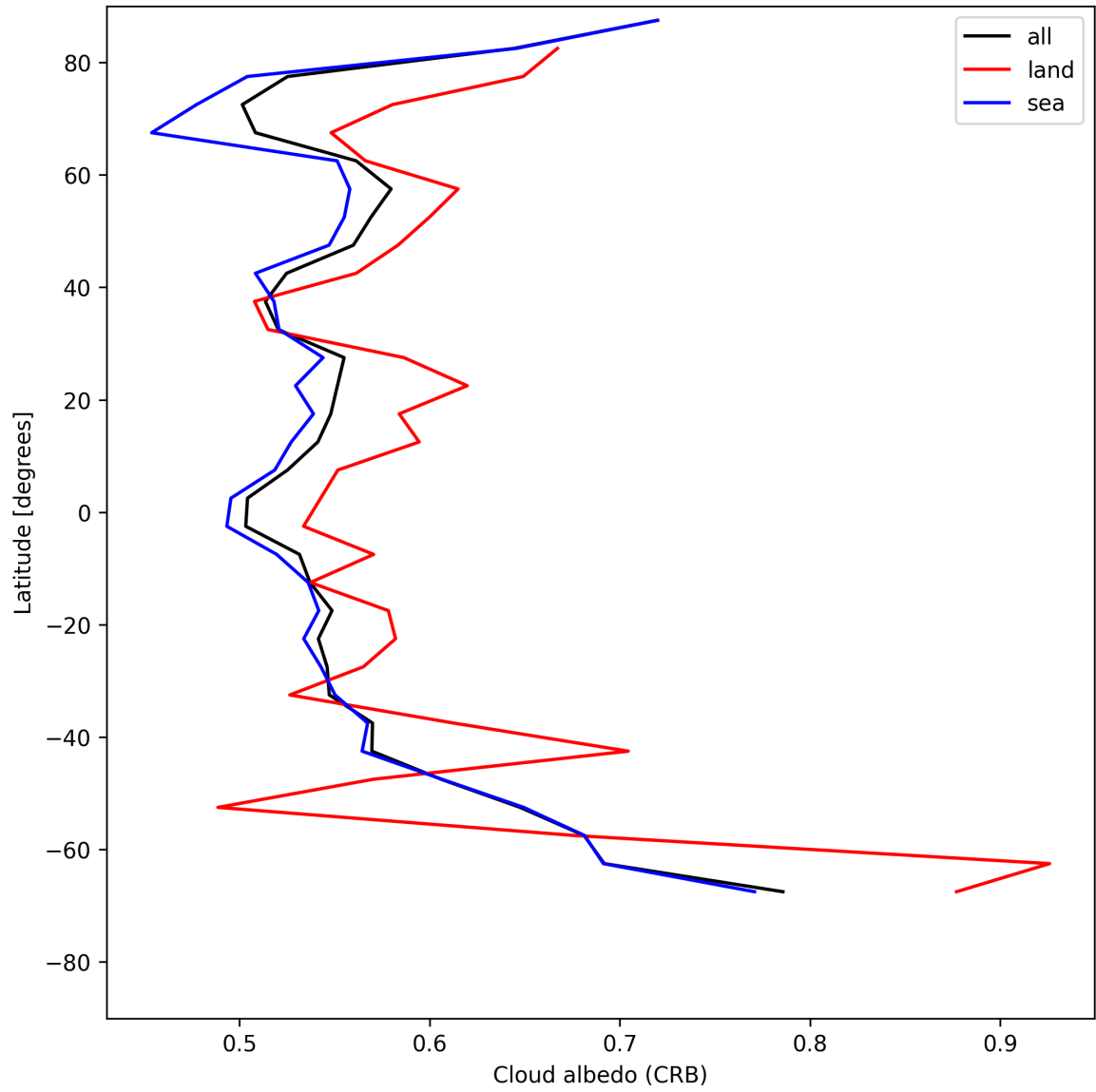
Figure 28: Zonal average of “Cloud albedo (CRB)” for 2025-07-27 to 2025-07-29.
