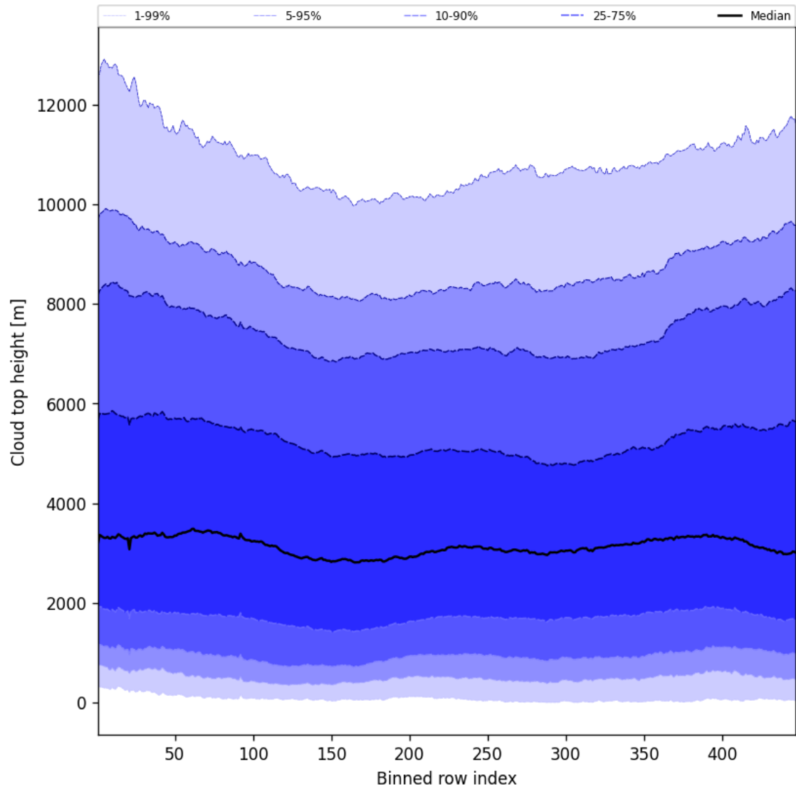
Figure 56: Along track statistics of “Cloud top height” for 2025-07-27 to 2025-07-29
