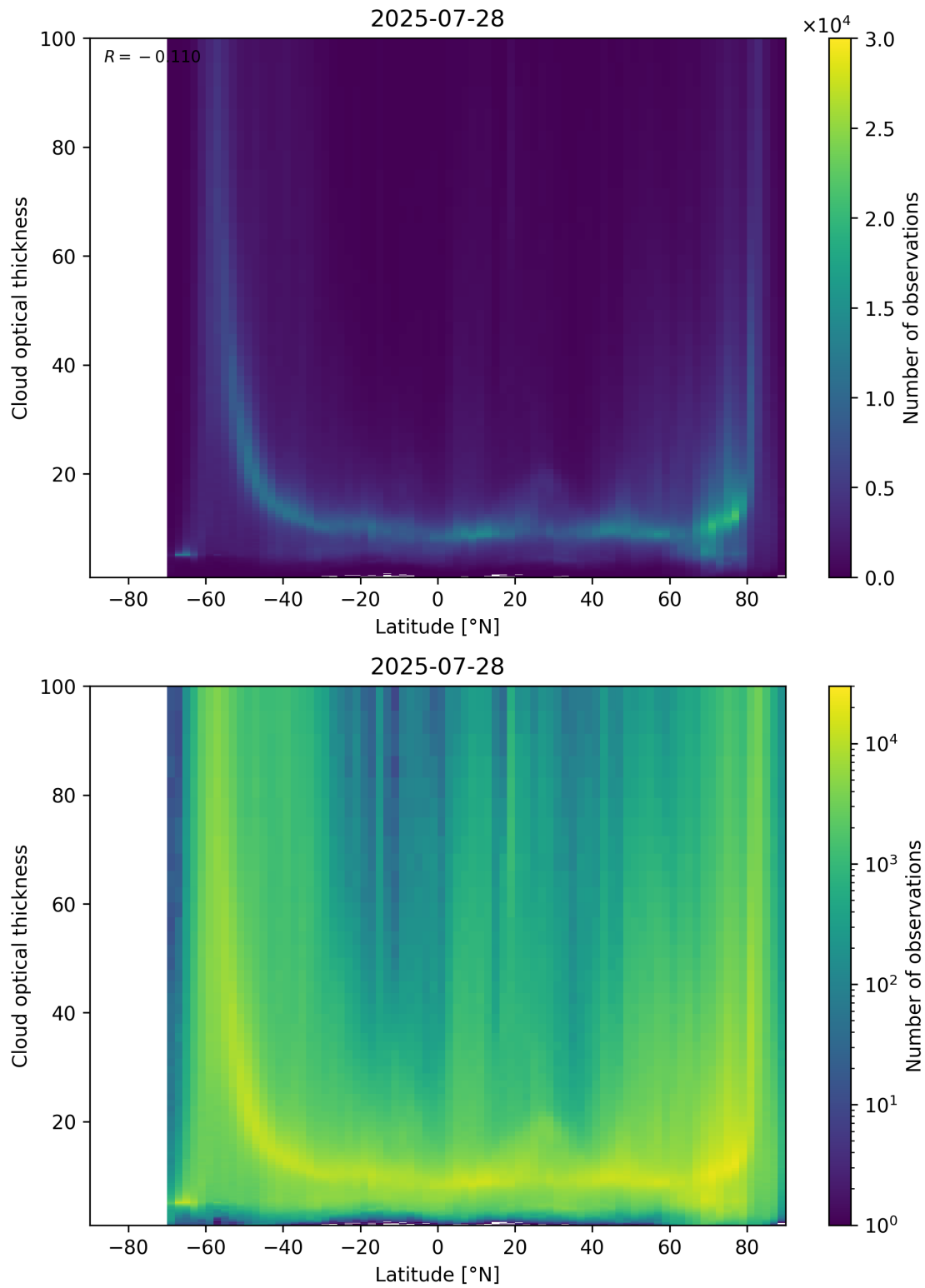
Figure 96: Scatter density plot of “Latitude” against “Cloud optical thickness” for 2025-07-27 to 2025-07-29.
