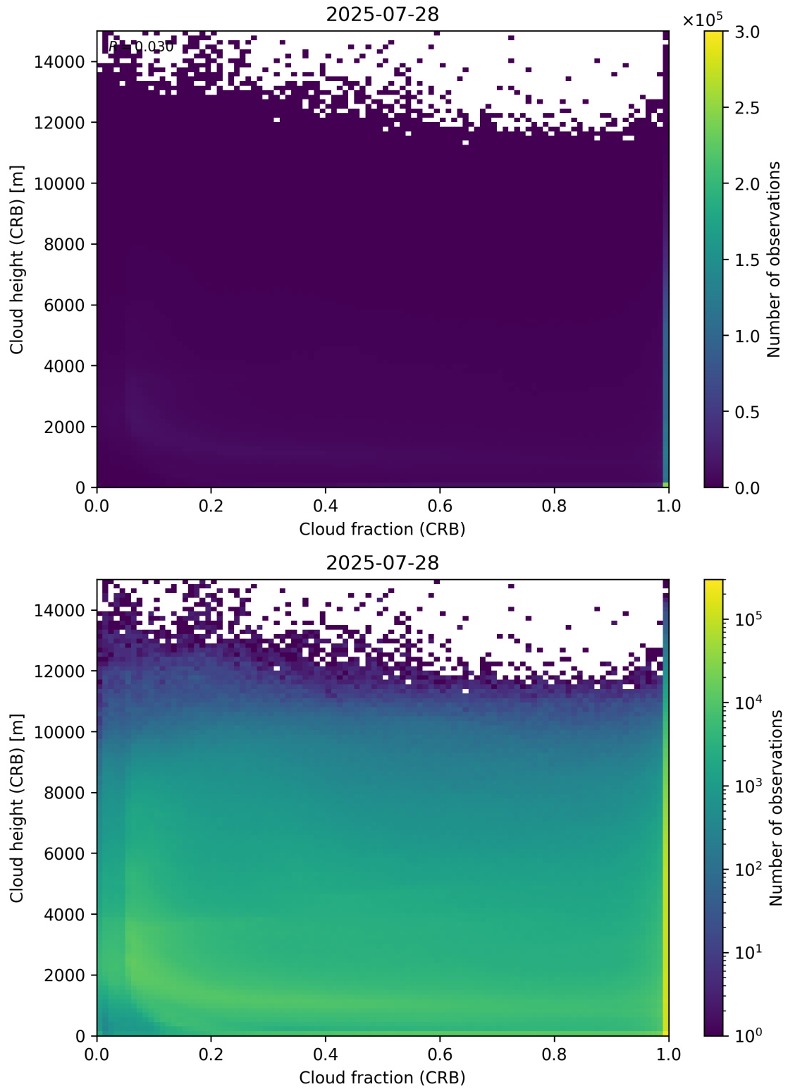
Figure 79: Scatter density plot of “Cloud fraction (CRB)” against “Cloud height (CRB)” for 2025-07-27 to 2025-07-29.
