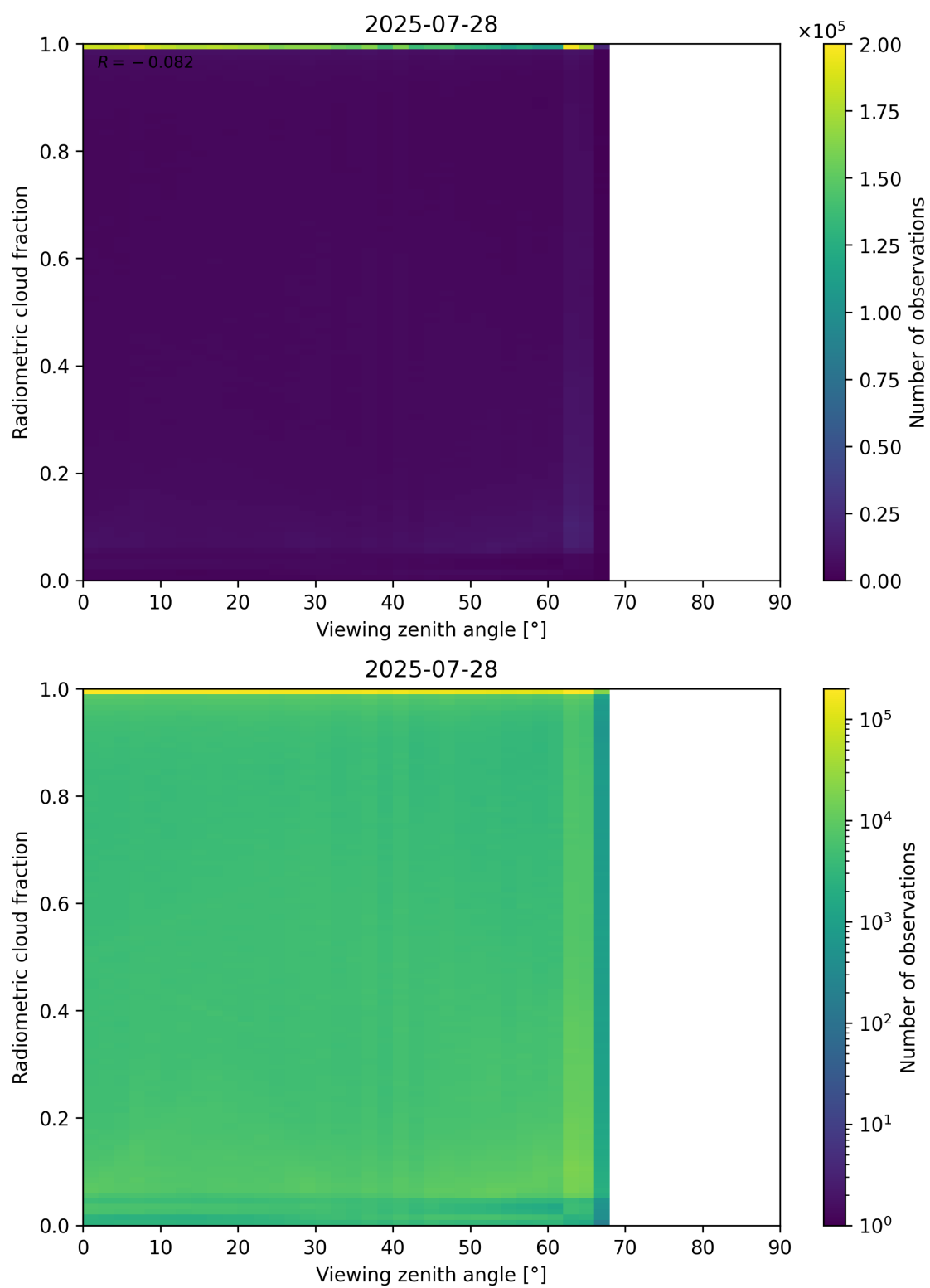
Figure 107: Scatter density plot of “Viewing zenith angle” against “Radiometric cloud fraction” for 2025-07-27 to 2025-07-29.
