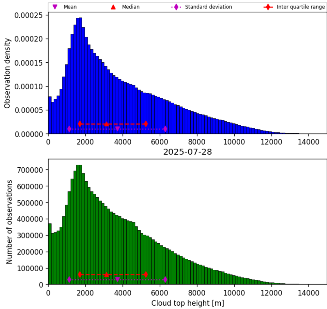
Figure 40: Histogram of “Cloud top height” for 2025-07-27 to 2025-07-29
