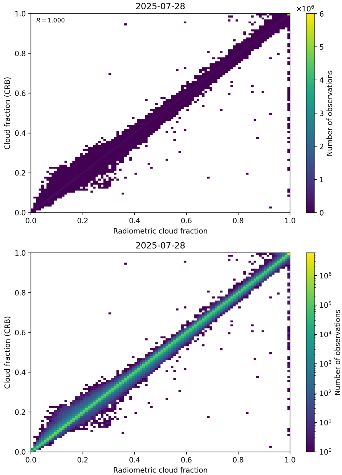
Figure 73: Scatter density plot of “Radiometric cloud fraction” against “Cloud fraction (CRB)” for 2025-07-27 to 2025-07-29.
