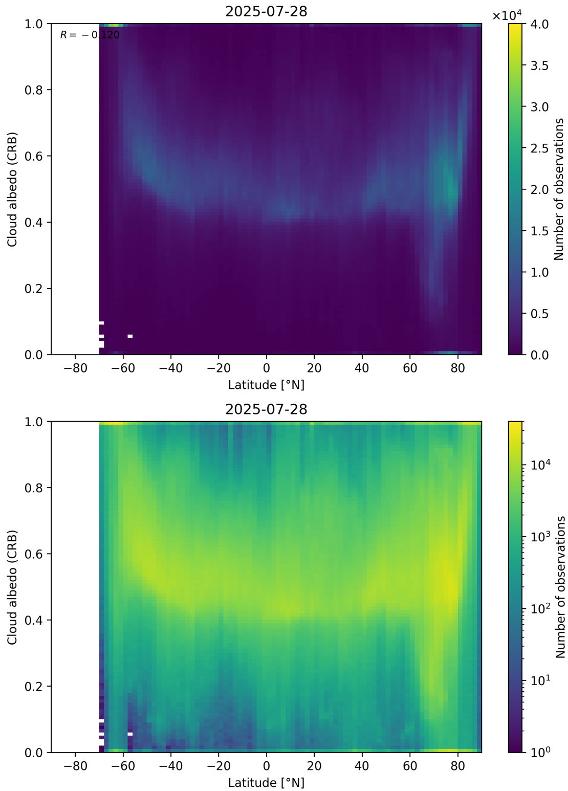
Figure 91: Scatter density plot of “Latitude” against “Cloud albedo (CRB)” for 2025-07-27 to 2025-07-29.
