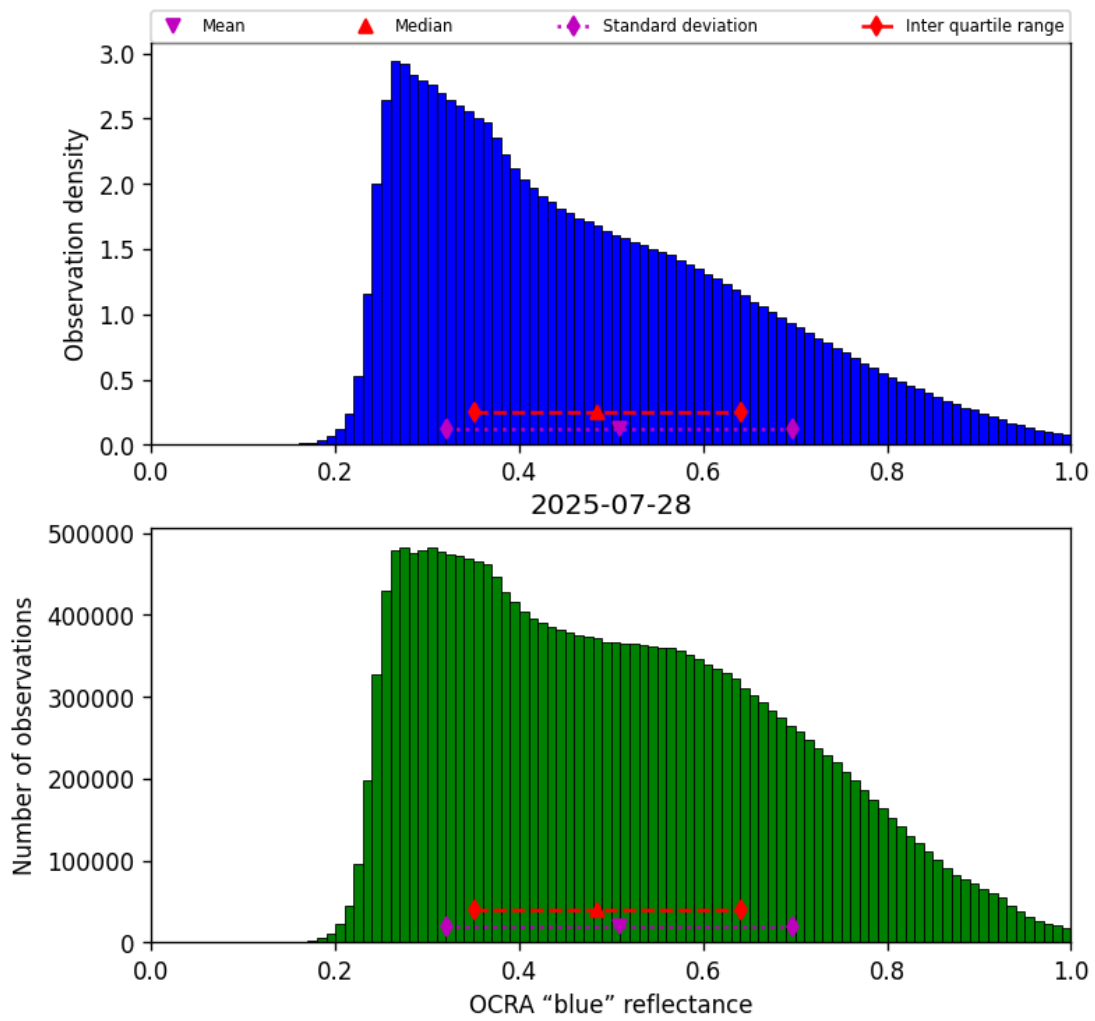
Figure 51: Histogram of “OCRA “blue” reflectance” for 2025-07-27 to 2025-07-29
