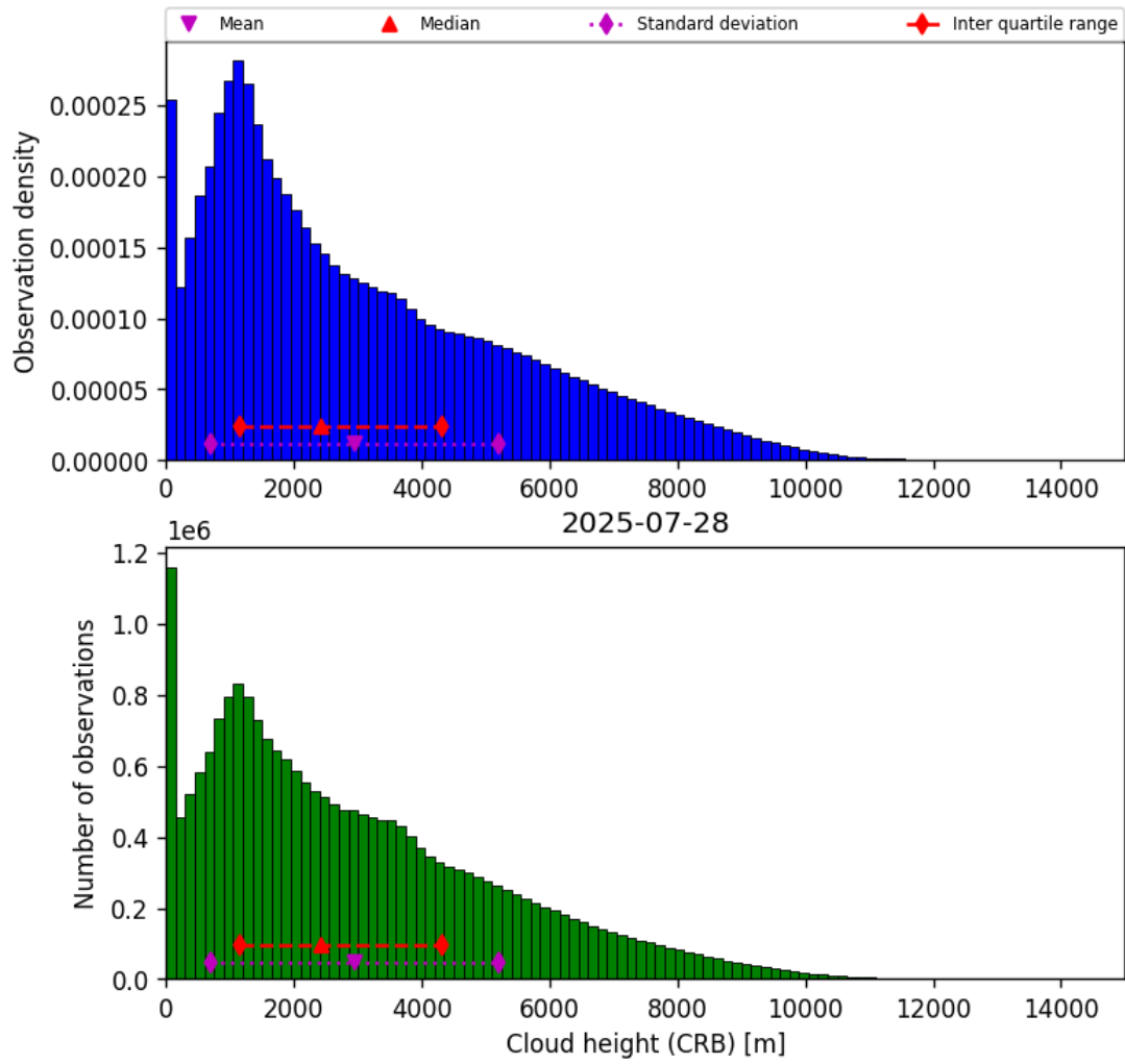
Figure 43: Histogram of “Cloud height (CRB)” for 2025-07-27 to 2025-07-29
