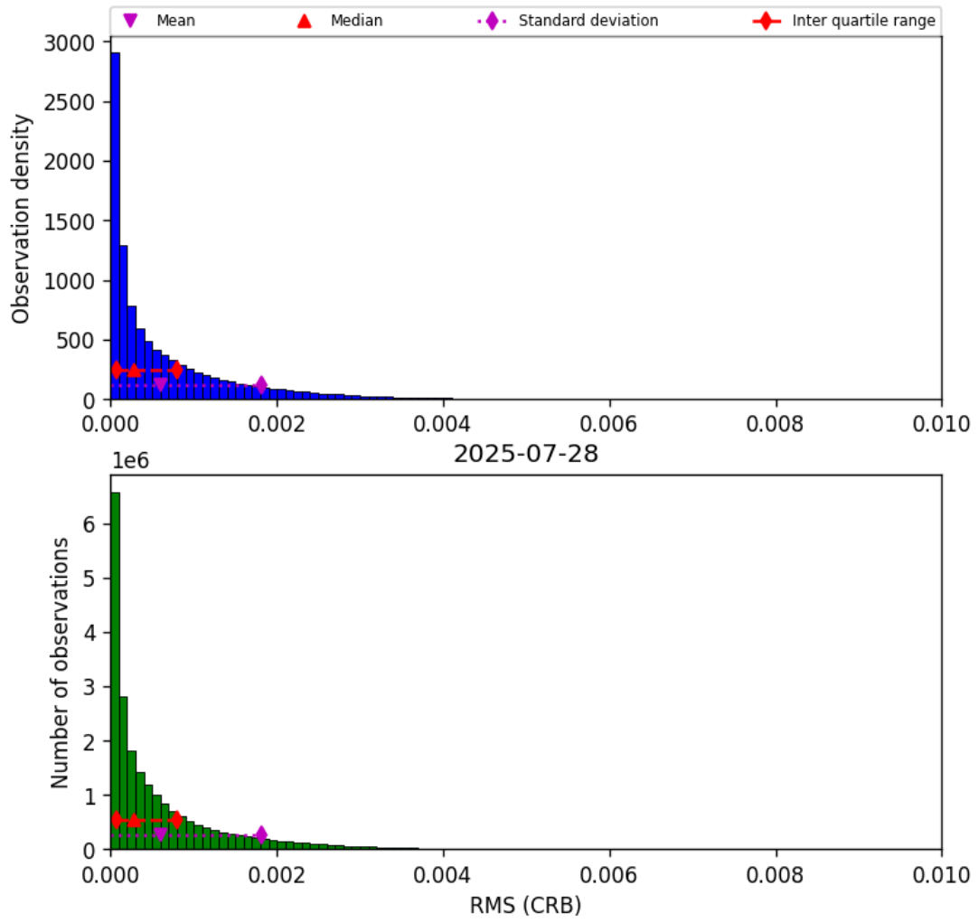
Figure 48: Histogram of “RMS (CRB)” for 2025-07-27 to 2025-07-29
