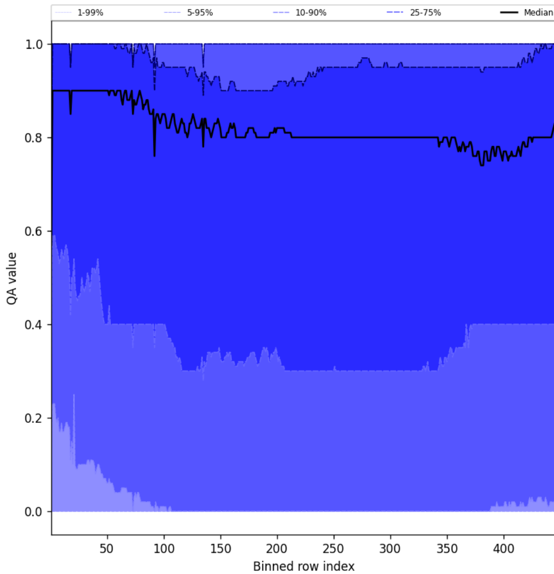
Figure 54: Along track statistics of “QA value” for 2025-07-27 to 2025-07-29
