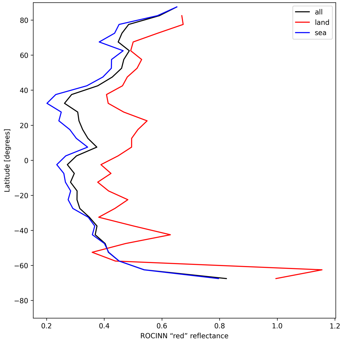
Figure 37: Zonal average of "ROCINN "red" reflectance" for 2025-07-27 to 2025-07-29.
