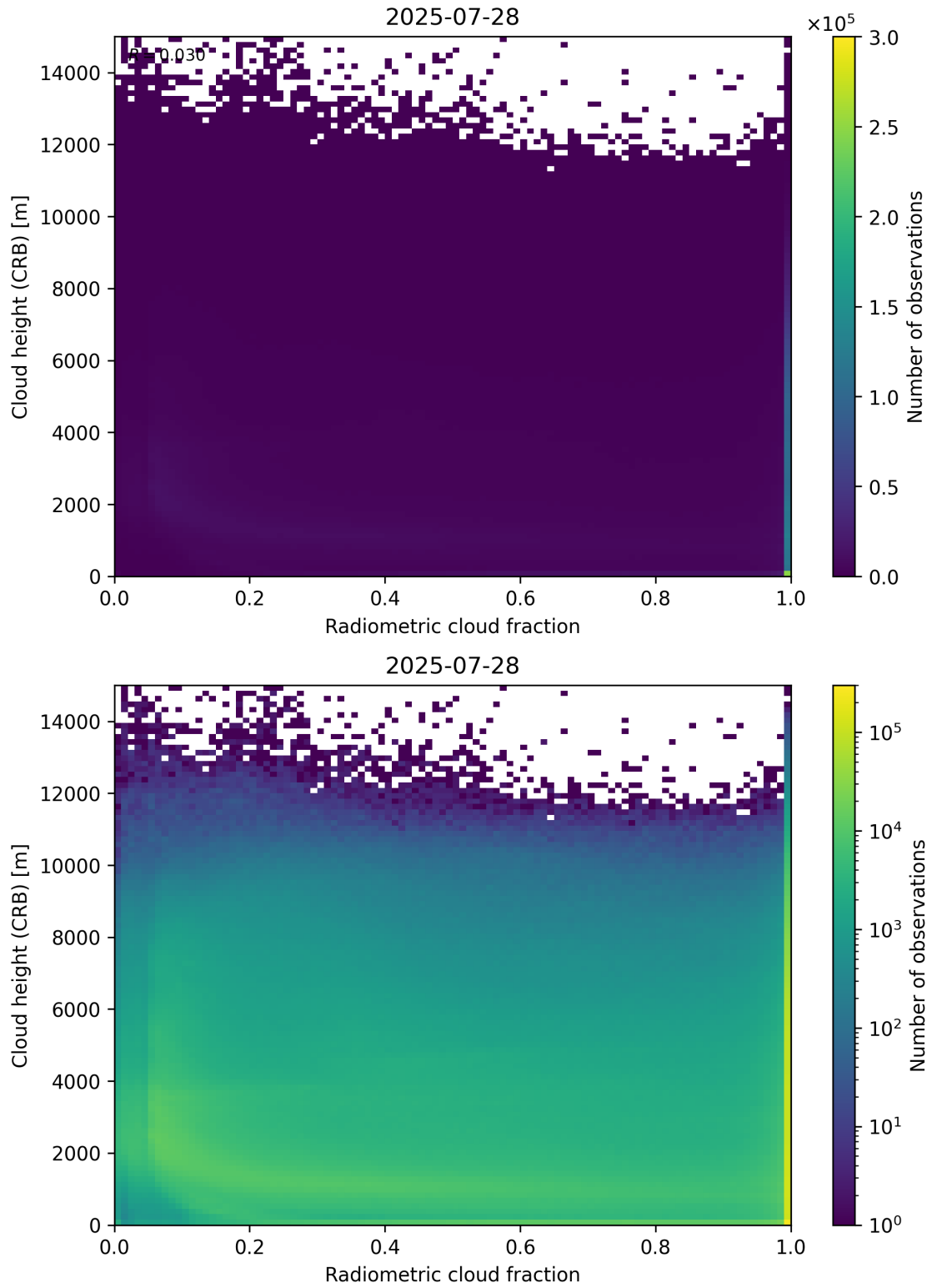
Figure 74: Scatter density plot of “Radiometric cloud fraction” against “Cloud height (CRB)” for 2025-07-27 to 2025-07-29.
