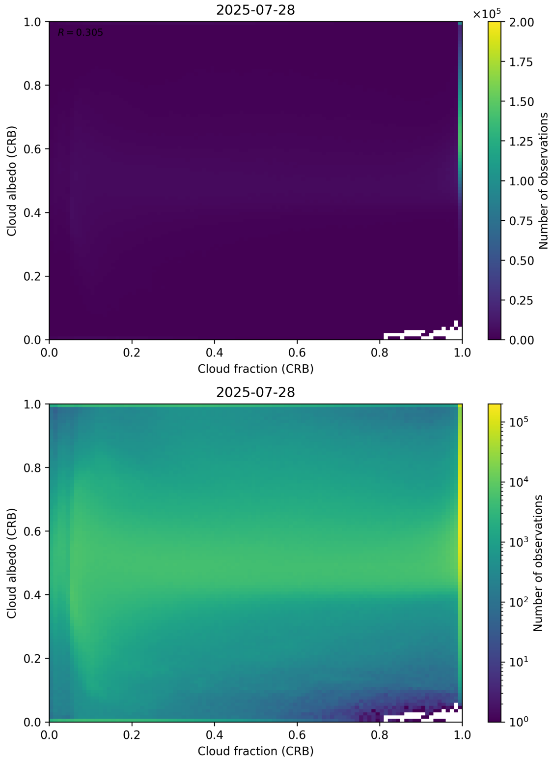
Figure 77: Scatter density plot of “Cloud fraction (CRB)” against “Cloud albedo (CRB)” for 2025-07-27 to 2025-07-29.
