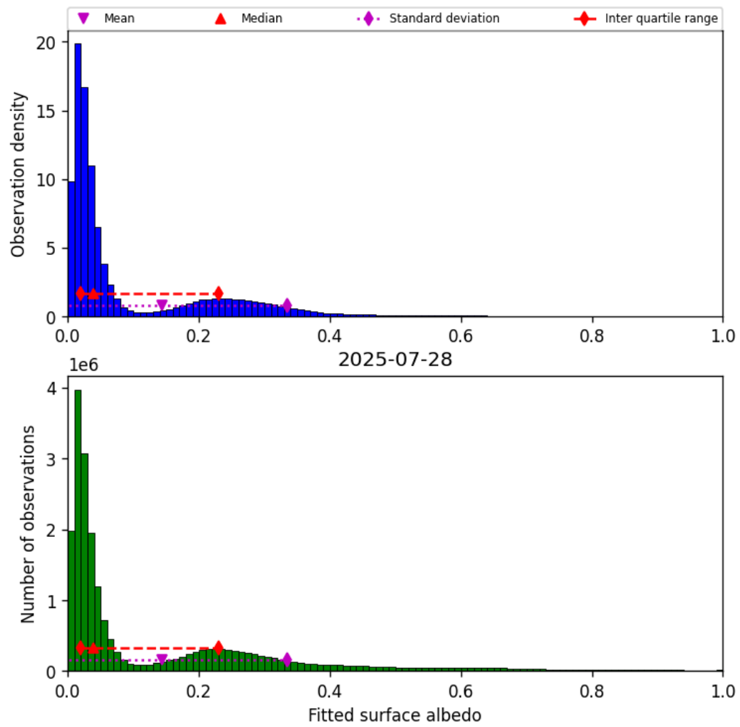
Figure 45: Histogram of “Fitted surface albedo” for 2025-07-27 to 2025-07-29
