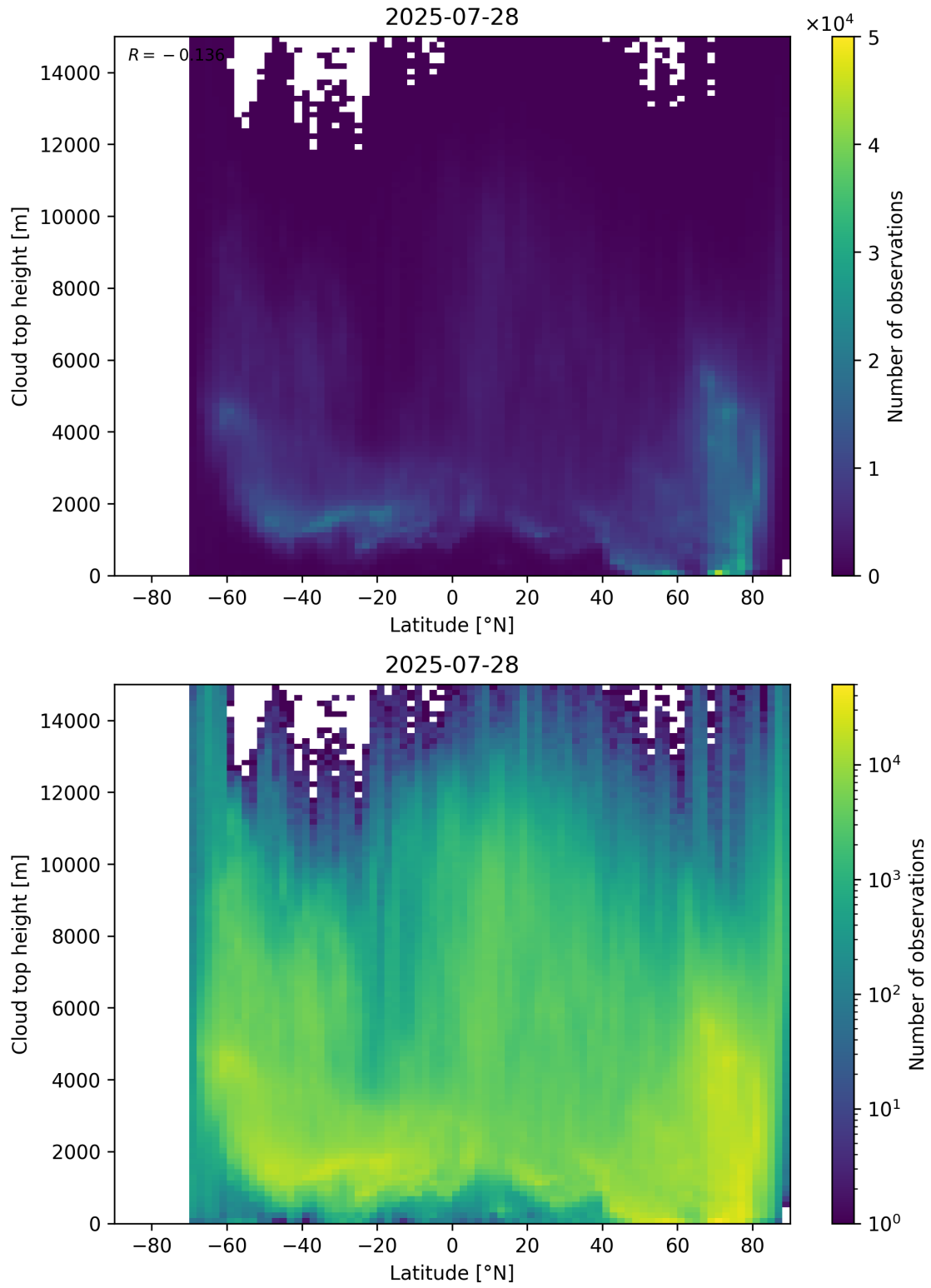
Figure 97: Scatter density plot of “Latitude” against “Cloud top height” for 2025-07-27 to 2025-07-29.
