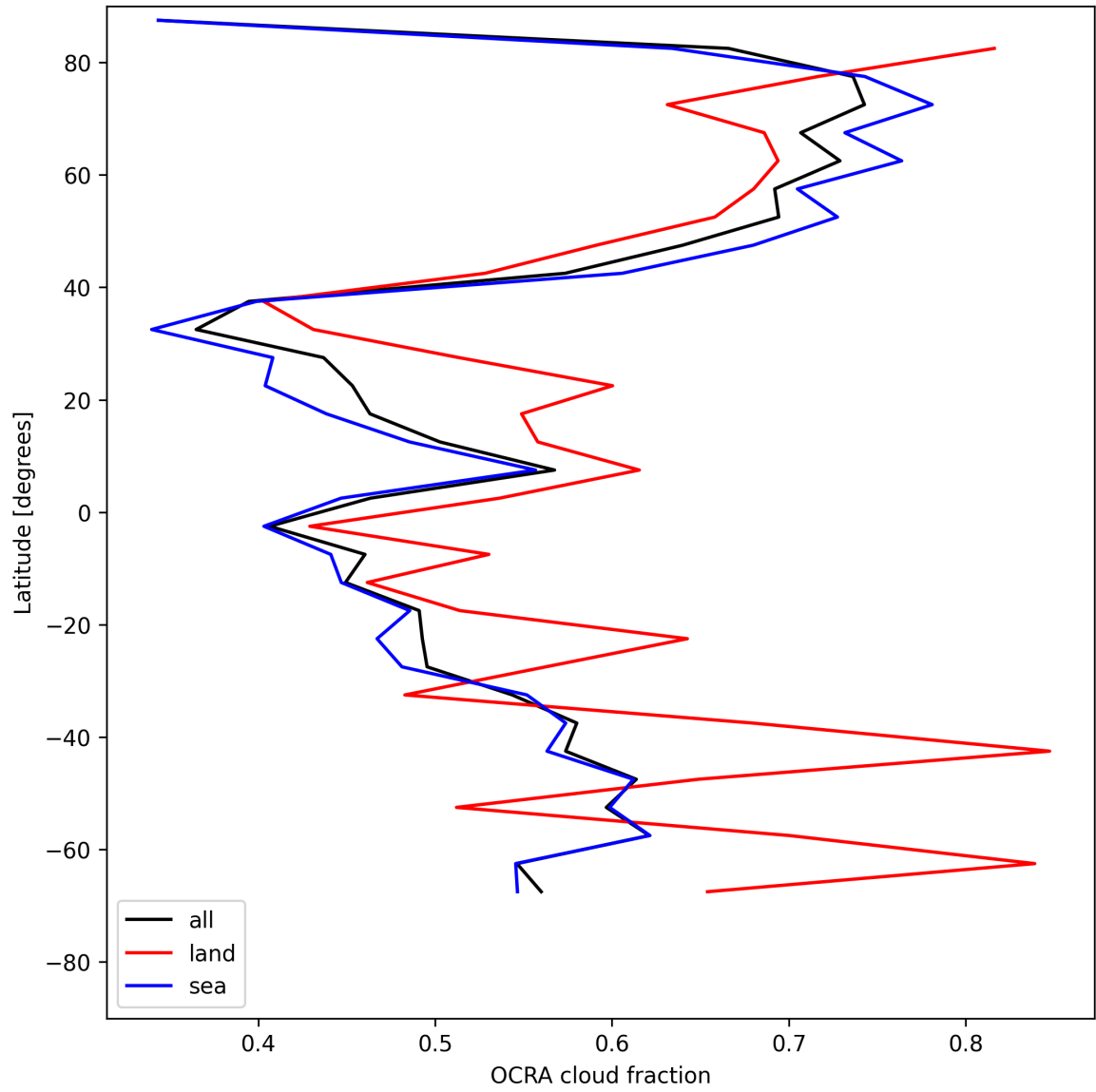
Figure 34: Zonal average of “OCRA cloud fraction” for 2025-07-27 to 2025-07-29.
