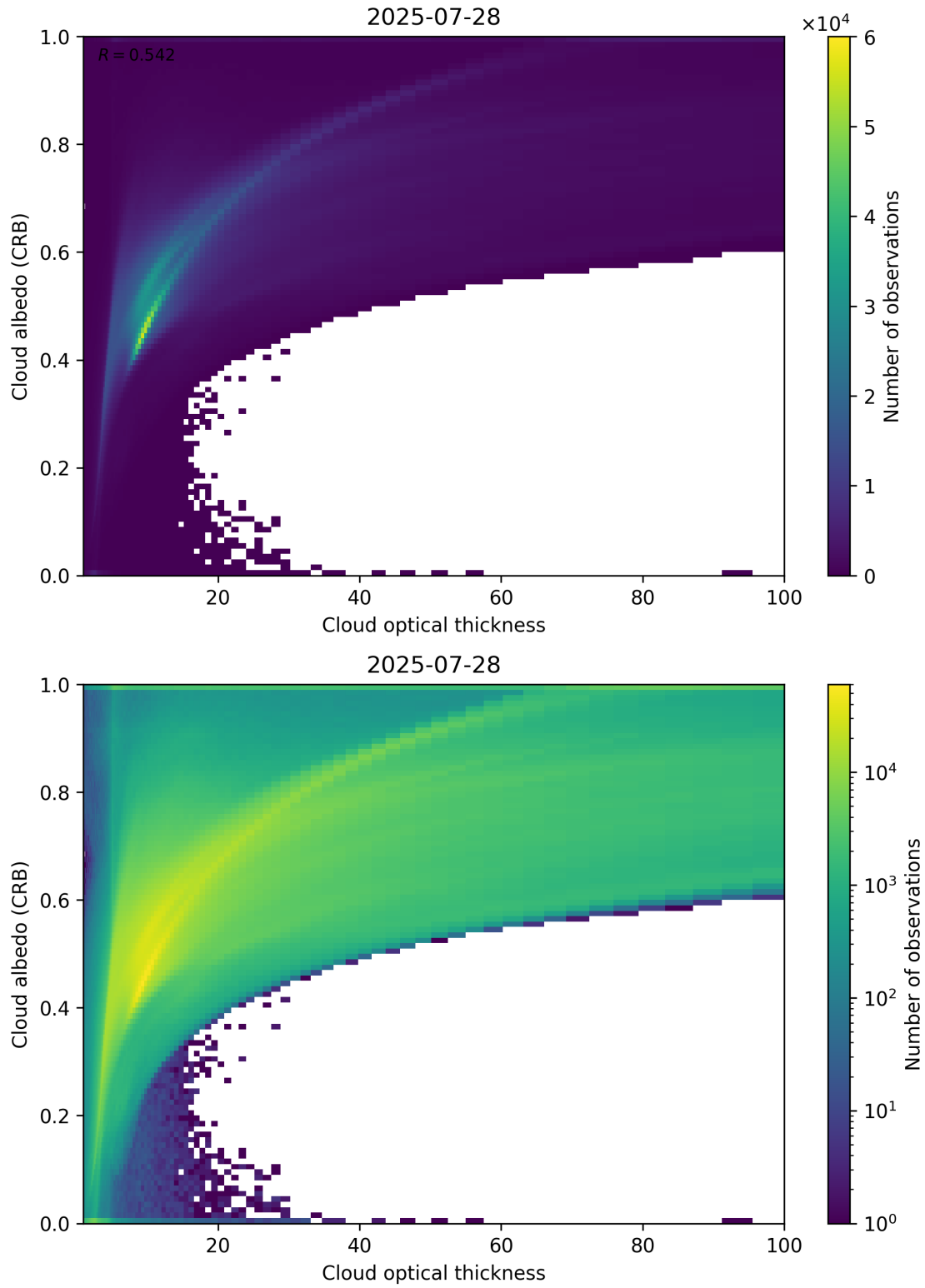
Figure 82: Scatter density plot of “Cloud optical thickness” against “Cloud albedo (CRB)” for 2025-07-27 to 2025-07-29.
