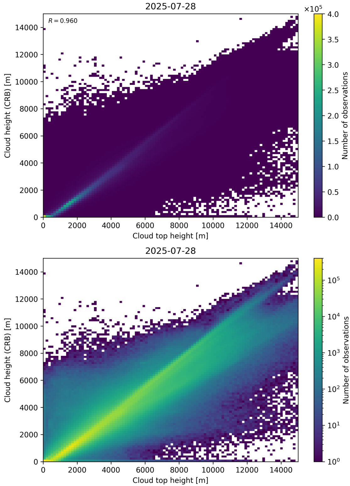
Figure 89: Scatter density plot of “Cloud top height” against “Cloud height (CRB)” for 2025-07-27 to 2025-07-29.
