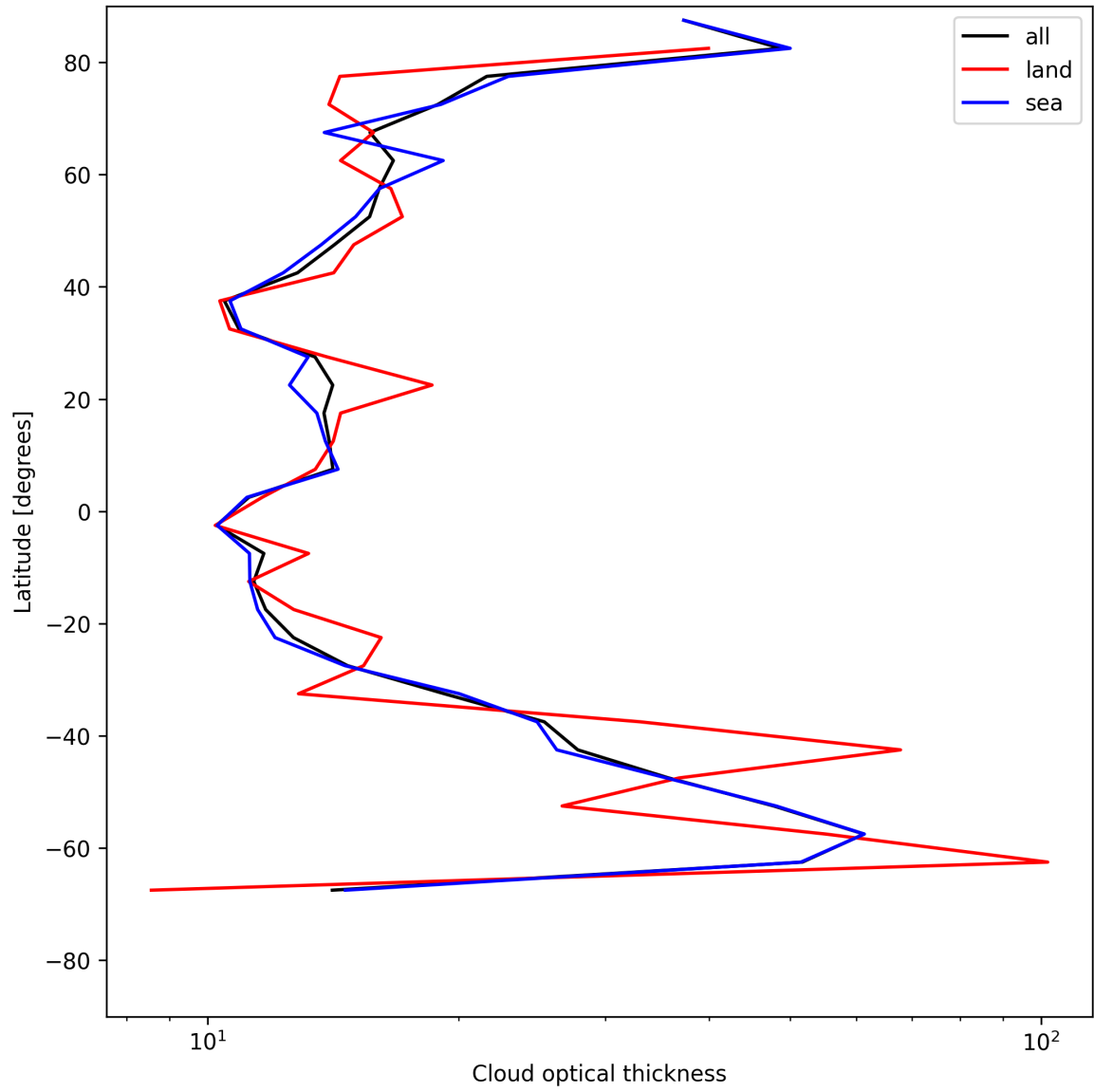
Figure 25: Zonal average of “Cloud optical thickness” for 2025-07-27 to 2025-07-29.
