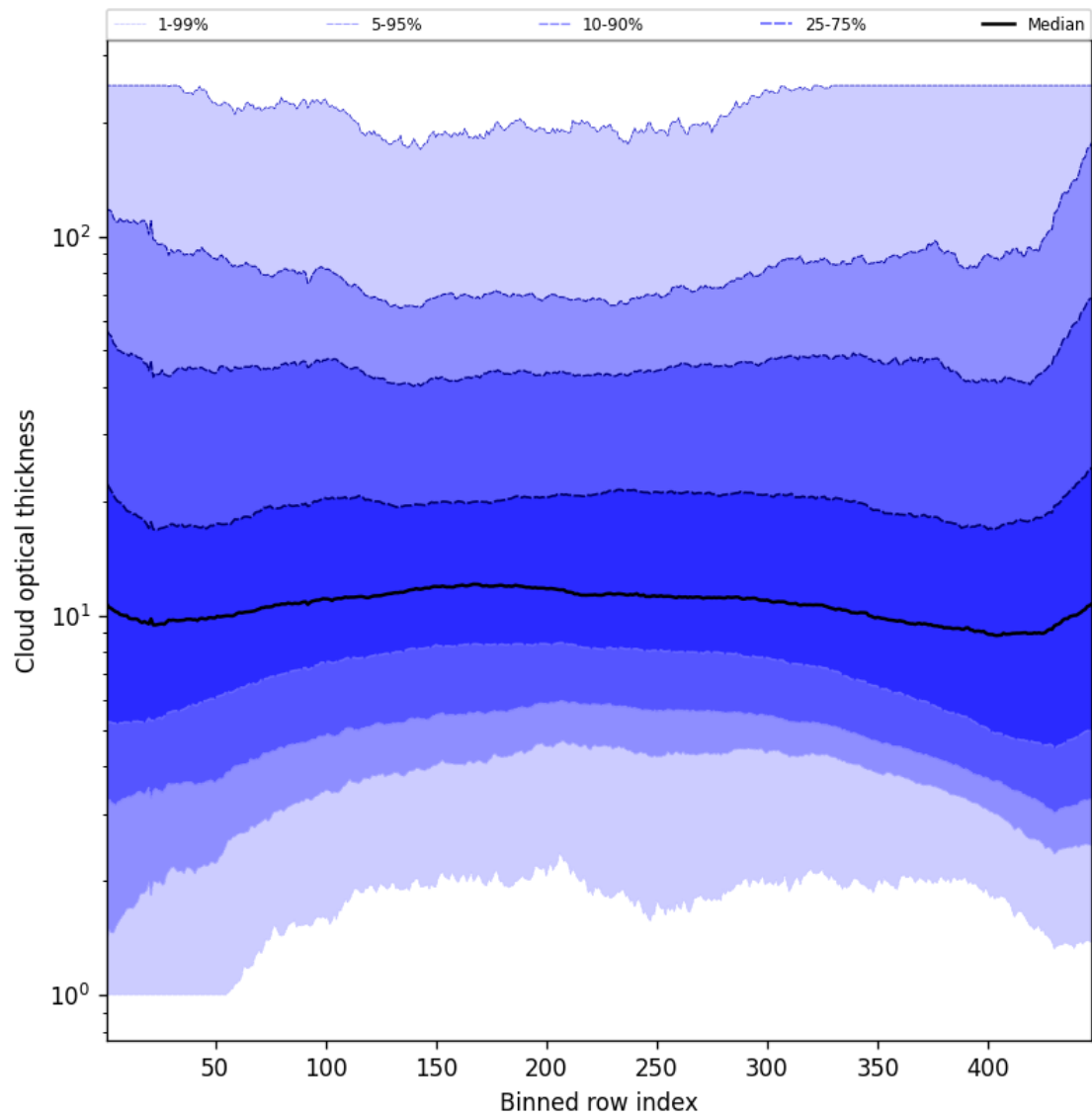
Figure 57: Along track statistics of “Cloud optical thickness” for 2025-07-27 to 2025-07-29
