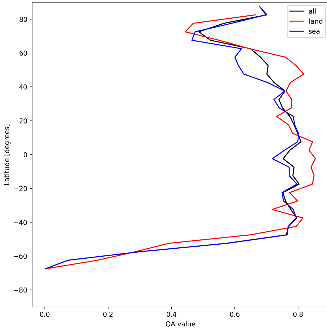
Figure 22: Zonal average of “QA value” for 2025-07-27 to 2025-07-29.
