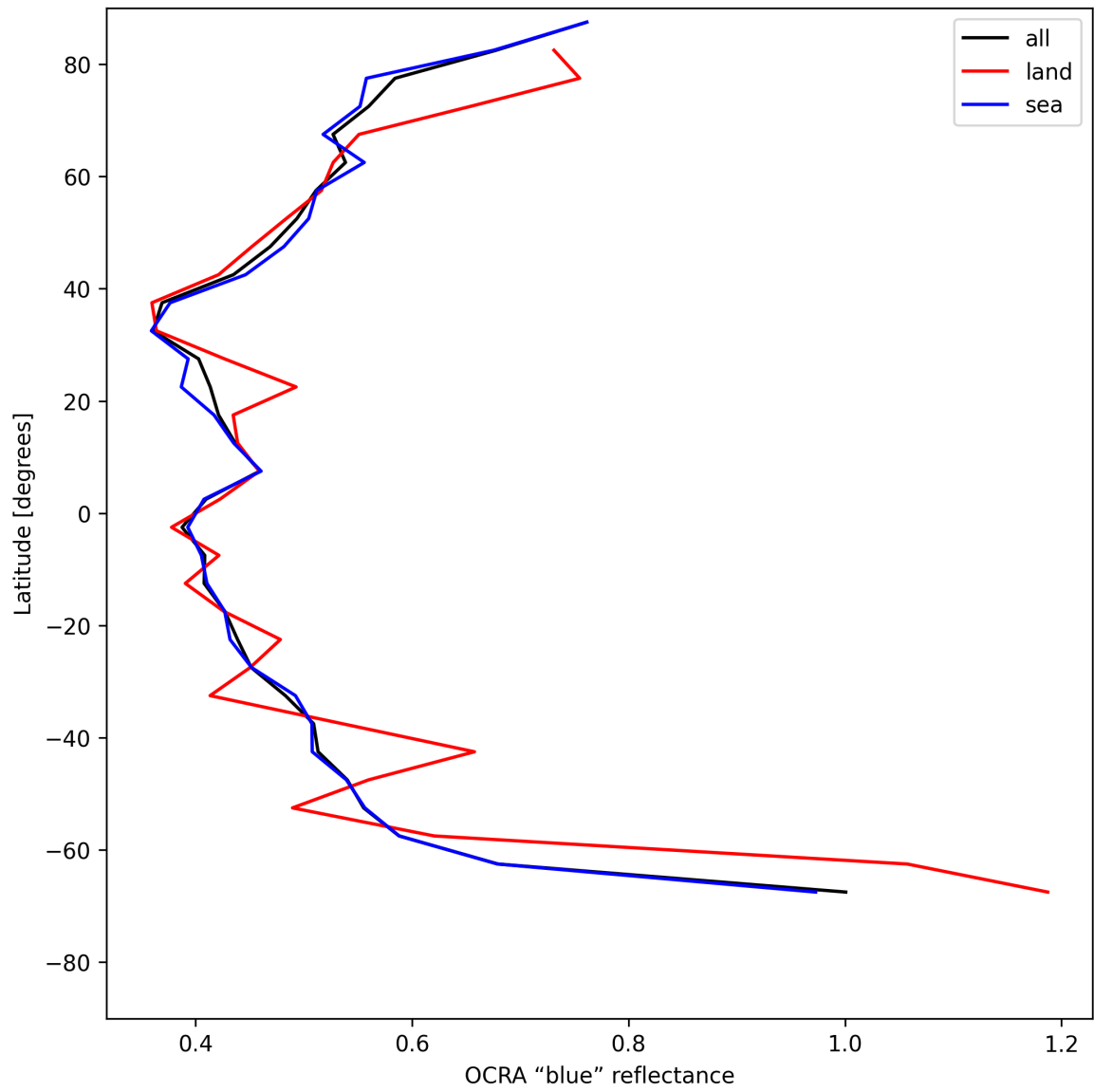
Figure 35: Zonal average of “OCRA “blue” reflectance” for 2025-07-27 to 2025-07-29.
