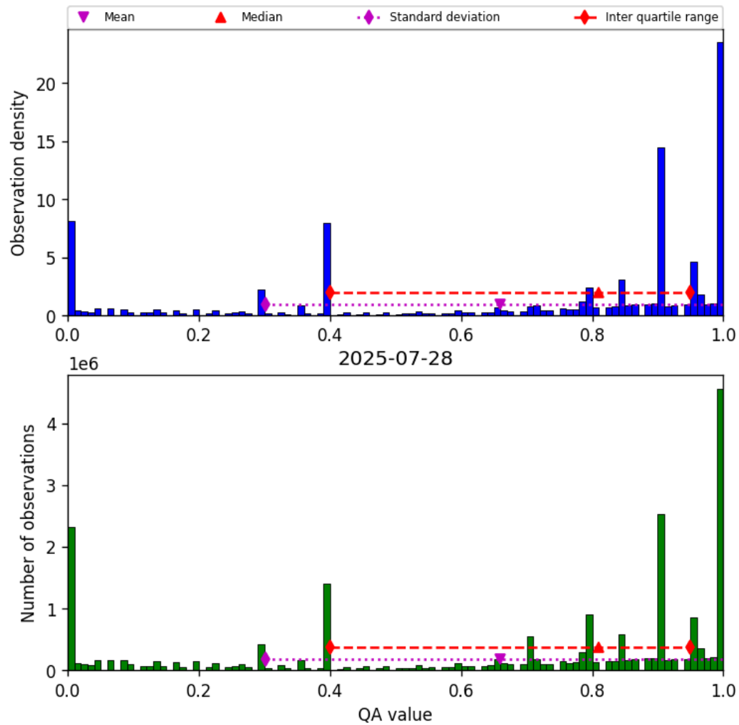
Figure 38: Histogram of “QA value” for 2025-07-27 to 2025-07-29
