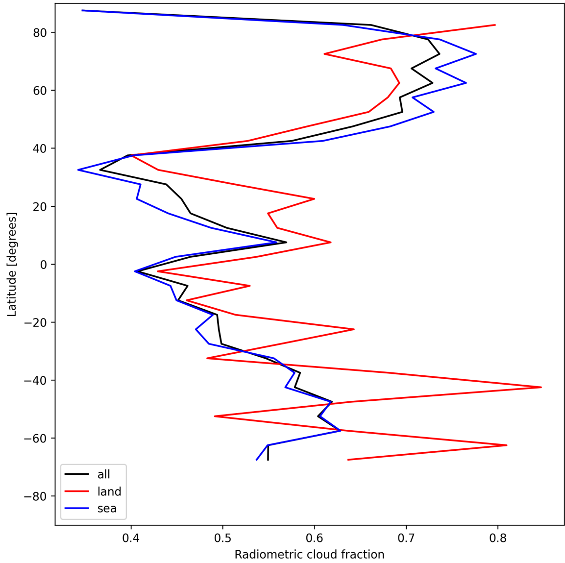
Figure 23: Zonal average of “Radiometric cloud fraction” for 2025-07-27 to 2025-07-29.
