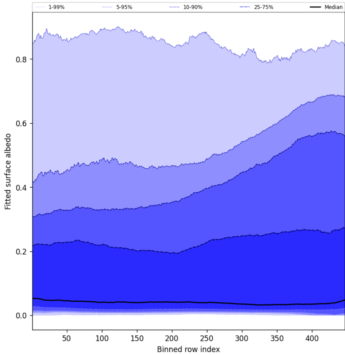
Figure 61: Along track statistics of “Fitted surface albedo” for 2025-07-27 to 2025-07-29
