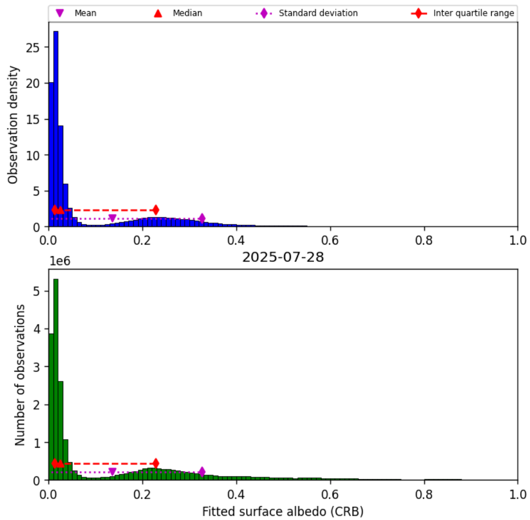
Figure 46: Histogram of “Fitted surface albedo (CRB)” for 2025-07-27 to 2025-07-29
