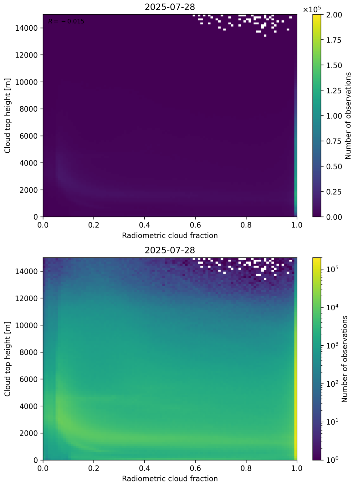
Figure 76: Scatter density plot of “Radiometric cloud fraction” against “Cloud top height” for 2025-07-27 to 2025-07-29.
