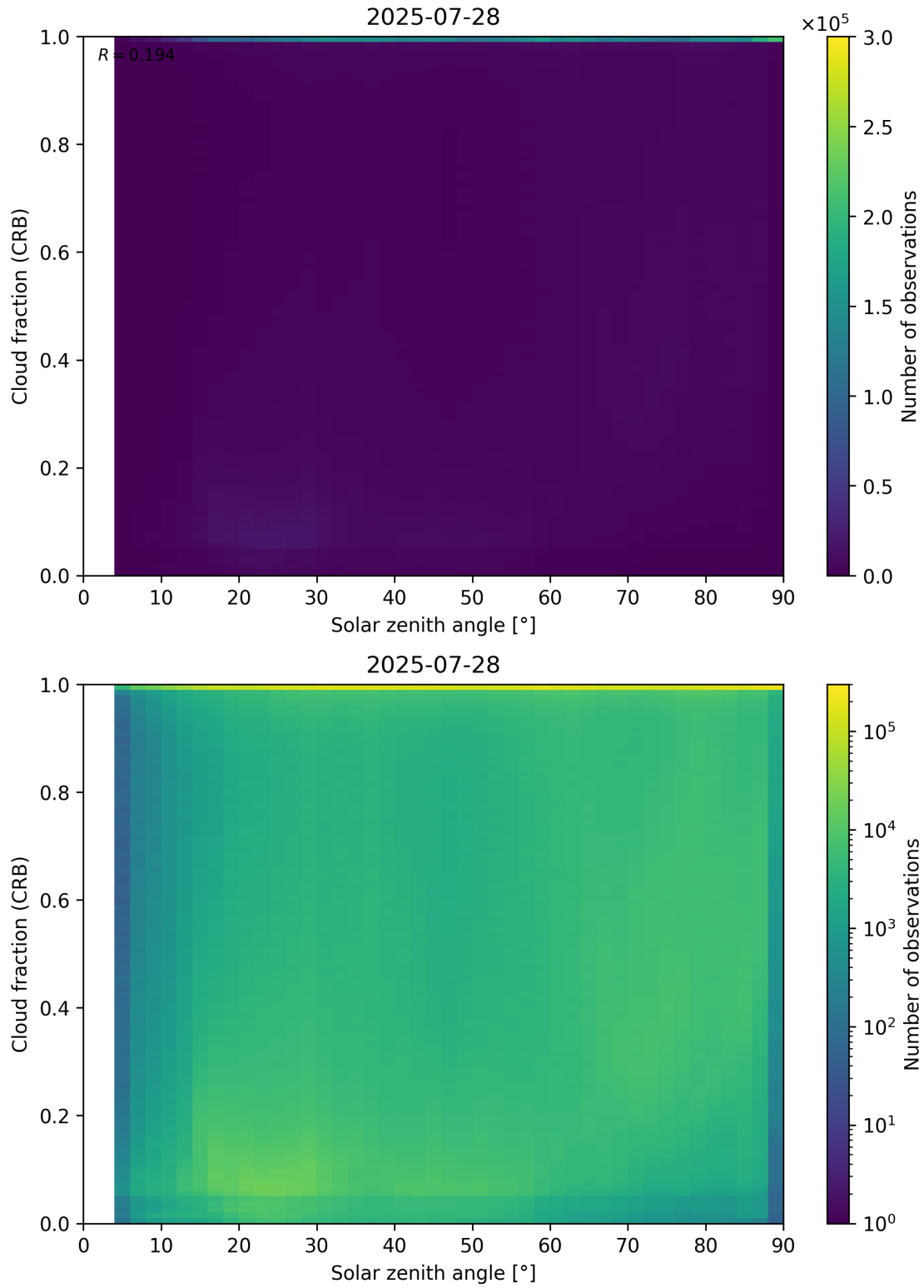
Figure 101: Scatter density plot of “Solar zenith angle” against “Cloud fraction (CRB)” for 2025-07-27 to 2025-07-29.
