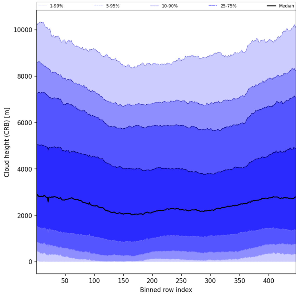
Figure 59: Along track statistics of “Cloud height (CRB)” for 2025-07-27 to 2025-07-29
