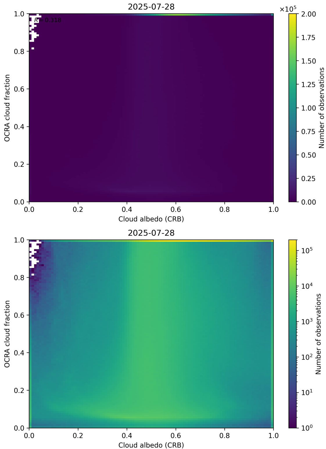
Figure 70: Scatter density plot of “Cloud albedo (CRB)” against “OCRA cloud fraction” for 2025-07-27 to 2025-07-29.
