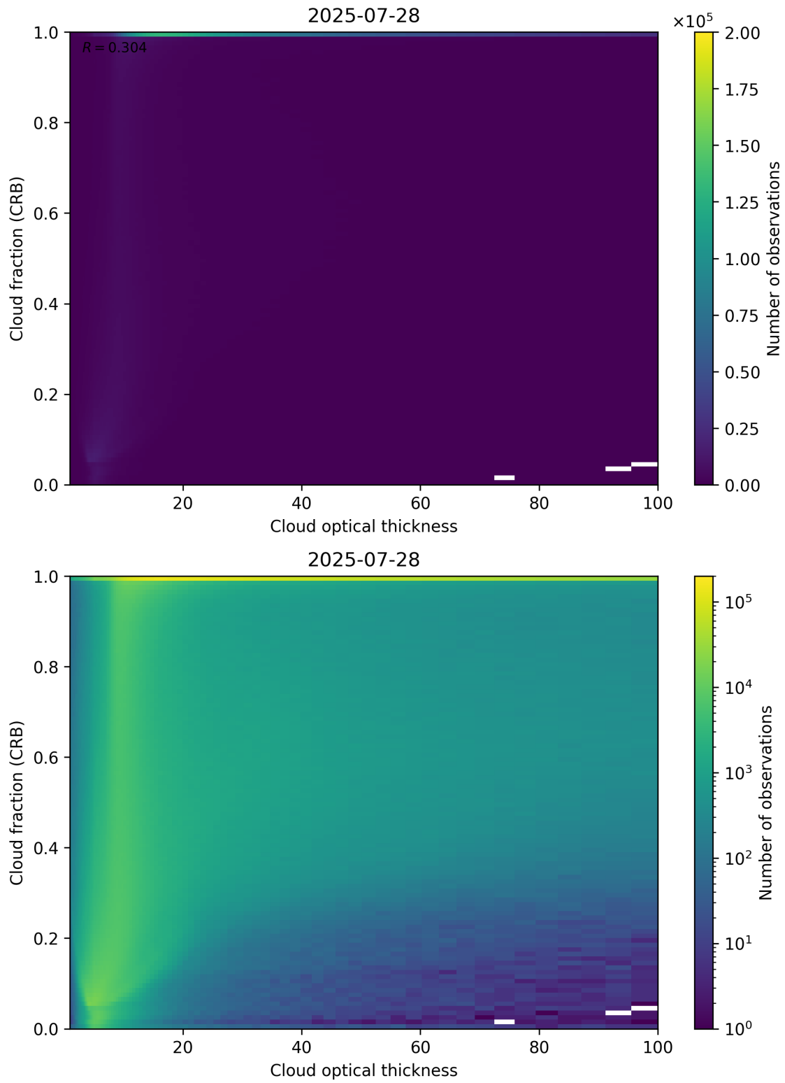
Figure 84: Scatter density plot of “Cloud optical thickness” against “Cloud fraction (CRB)” for 2025-07-27 to 2025-07-29.
