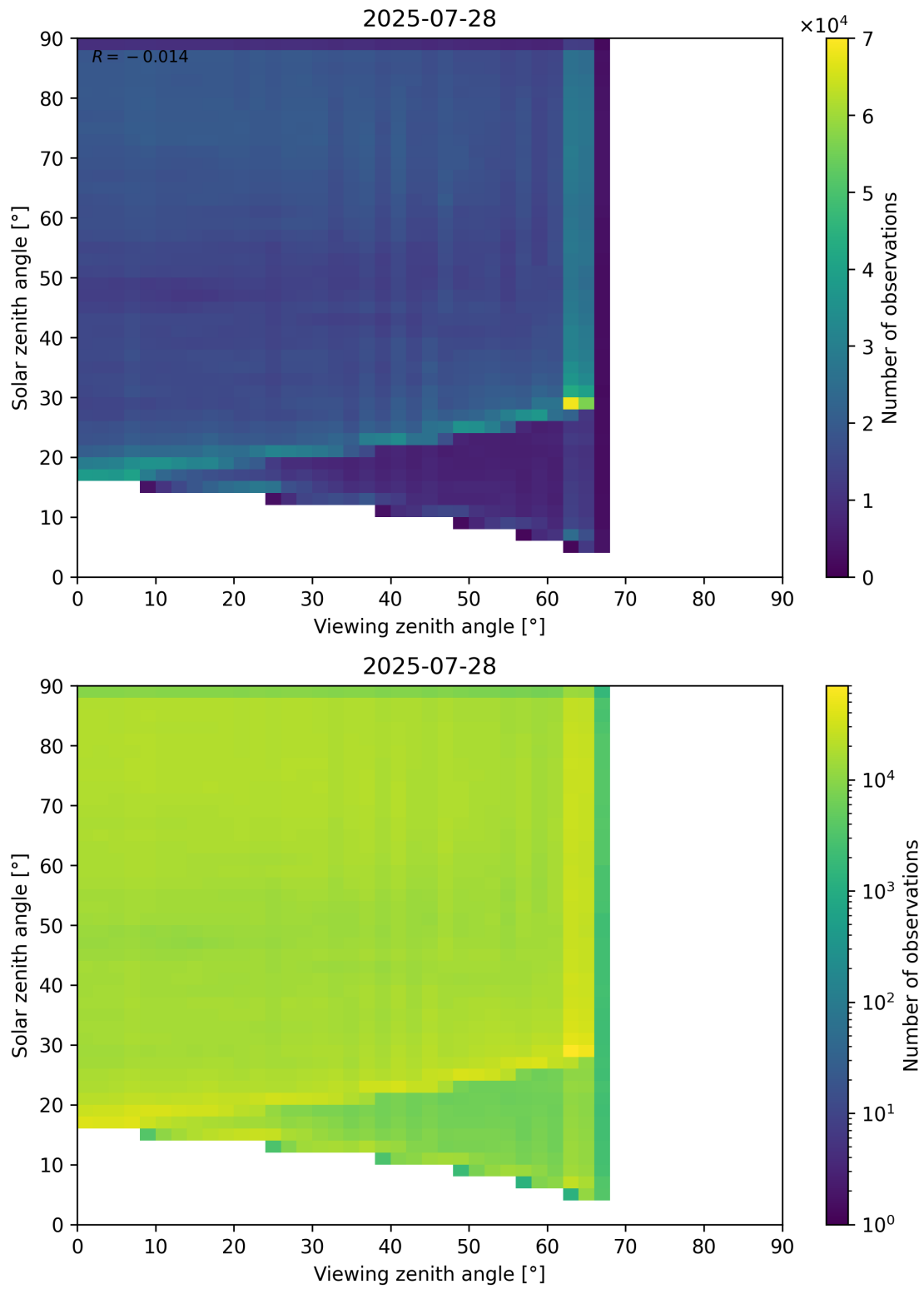
Figure 114: Scatter density plot of “Viewing zenith angle” against “Solar zenith angle” for 2025-07-27 to 2025-07-29.
