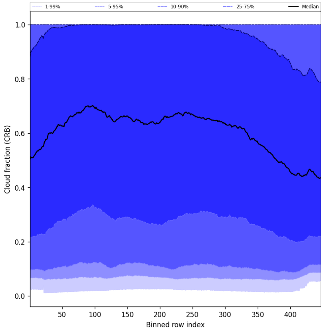
Figure 58: Along track statistics of “Cloud fraction (CRB)” for 2025-07-27 to 2025-07-29
