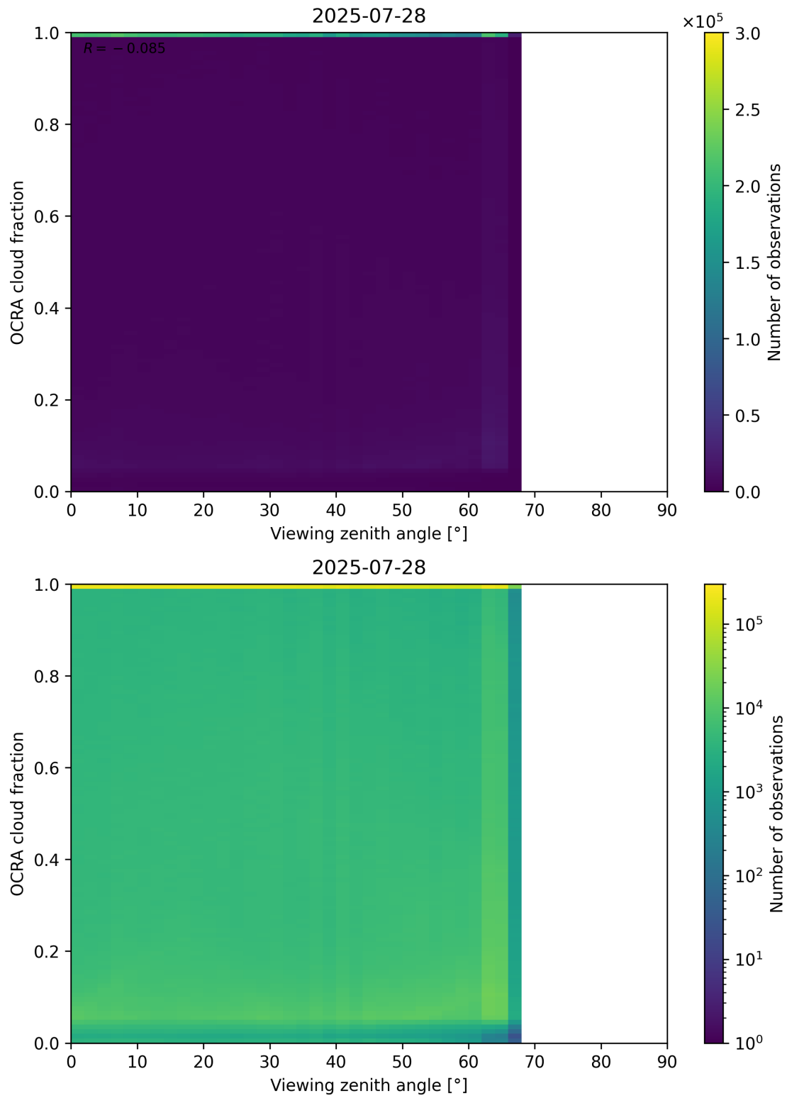
Figure 108: Scatter density plot of “Viewing zenith angle” against “OCRA cloud fraction” for 2025-07-27 to 2025-07-29.
