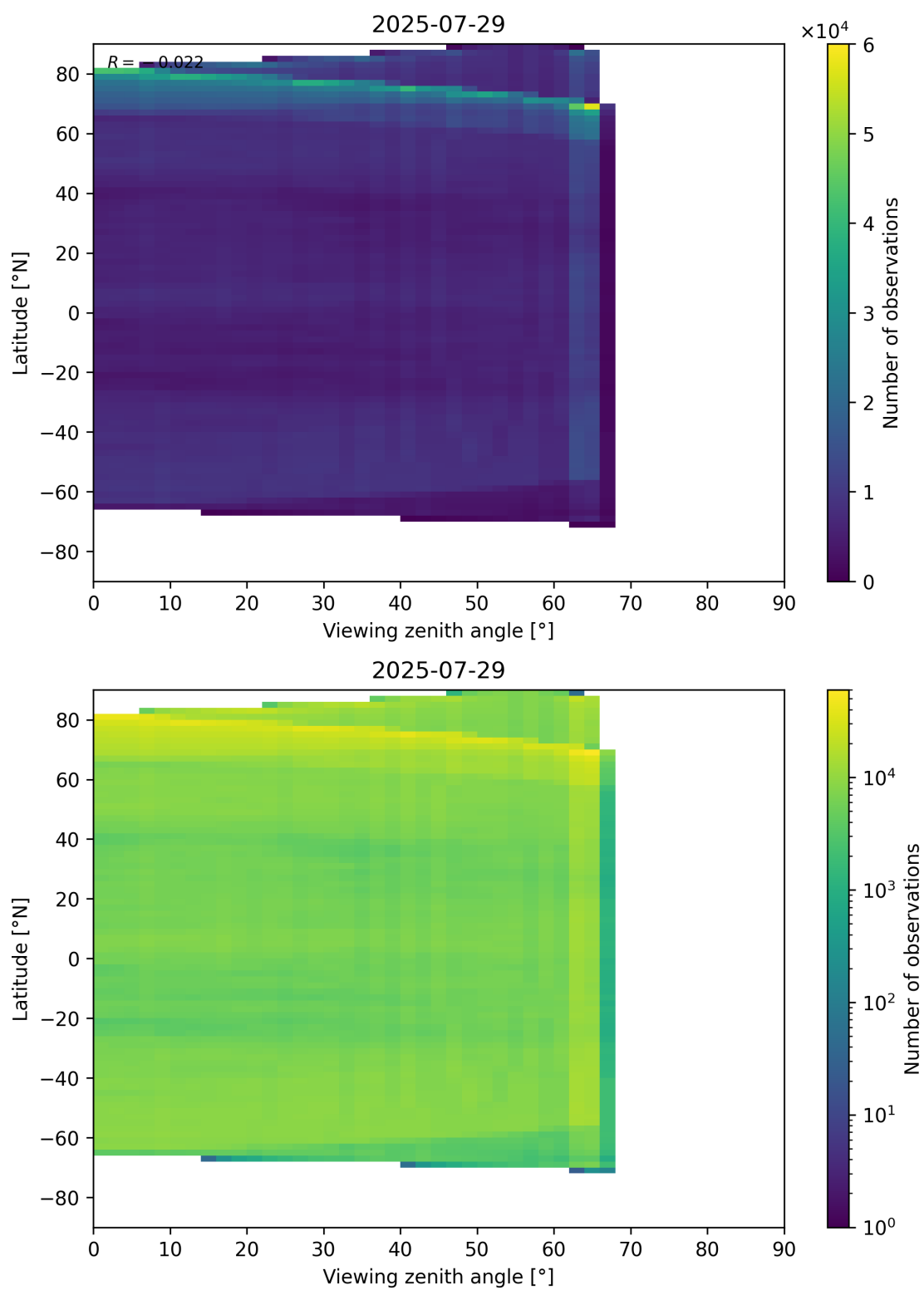
Figure 113: Scatter density plot of “Viewing zenith angle” against “Latitude” for 2025-07-29 to 2025-07-30.
