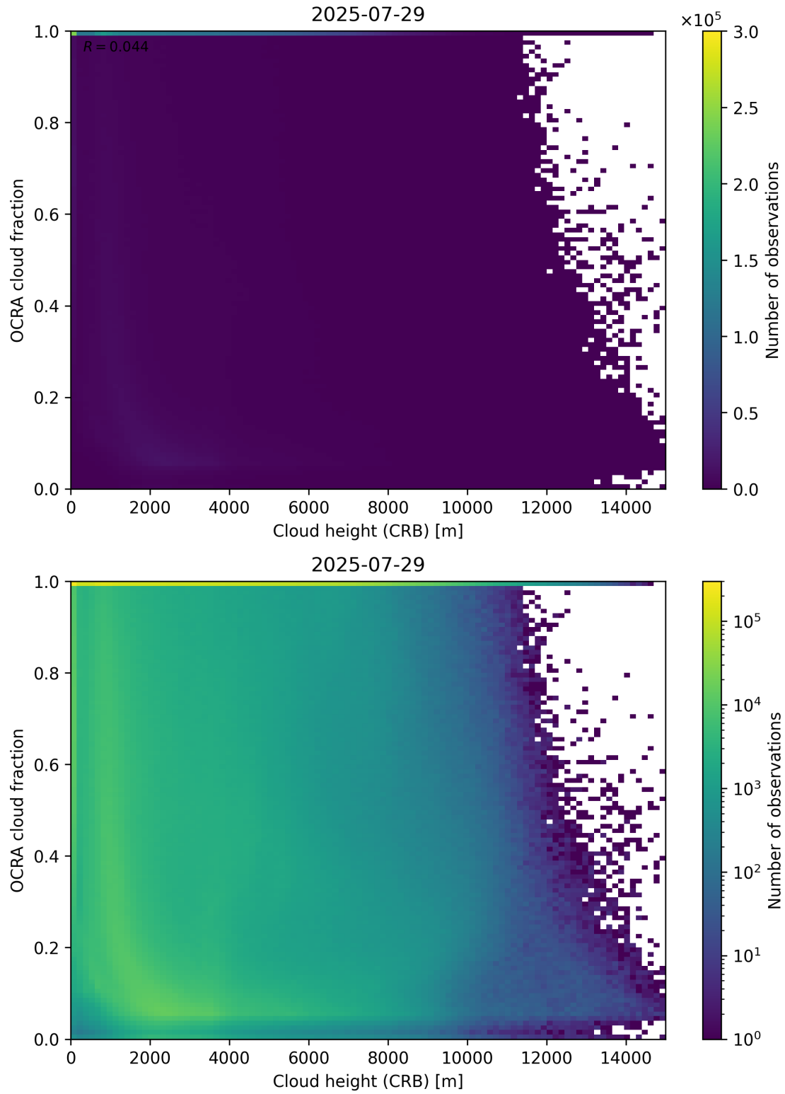
Figure 81: Scatter density plot of “Cloud height (CRB)” against “OCRA cloud fraction” for 2025-07-29 to 2025-07-30.
