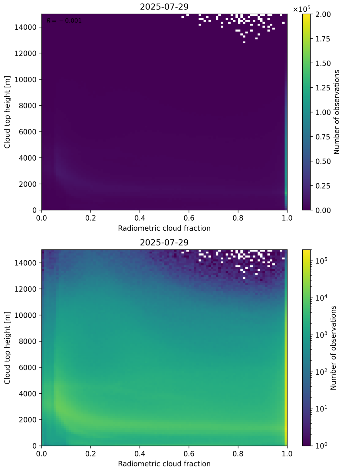
Figure 76: Scatter density plot of “Radiometric cloud fraction” against “Cloud top height” for 2025-07-29 to 2025-07-30.
