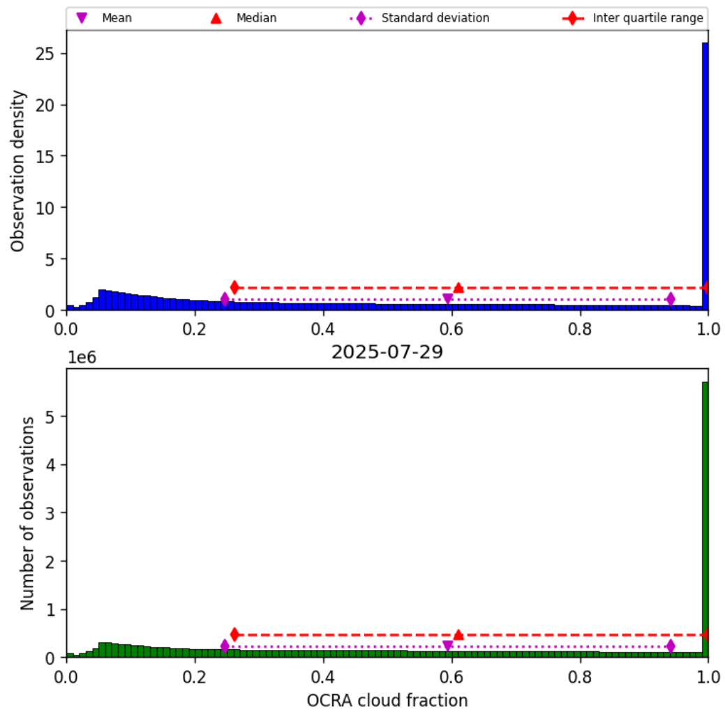
Figure 50: Histogram of “OCRA cloud fraction” for 2025-07-29 to 2025-07-30
