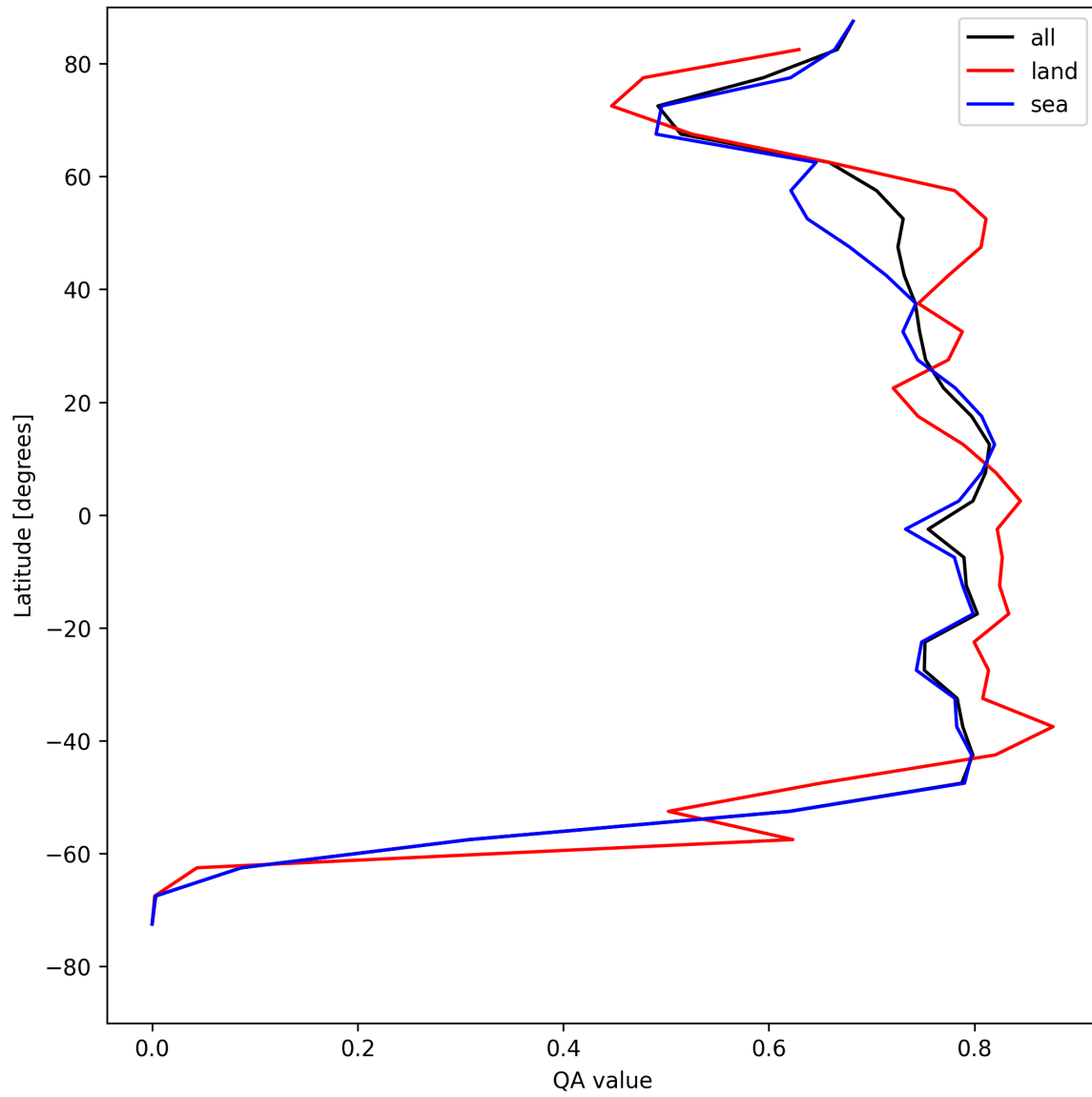
Figure 22: Zonal average of “QA value” for 2025-07-29 to 2025-07-30.
