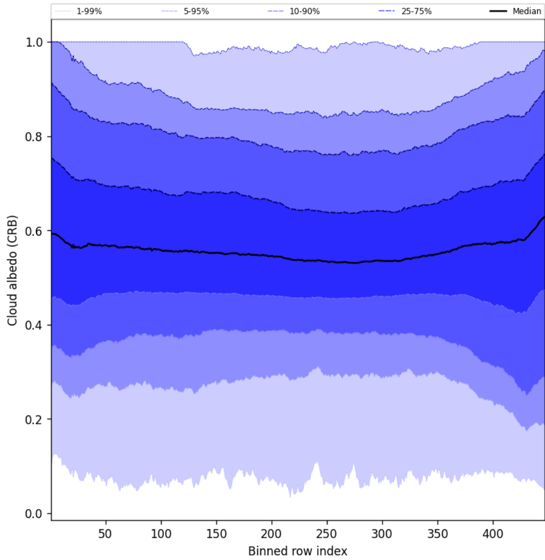
Figure 60: Along track statistics of “Cloud albedo (CRB)” for 2025-07-29 to 2025-07-30
