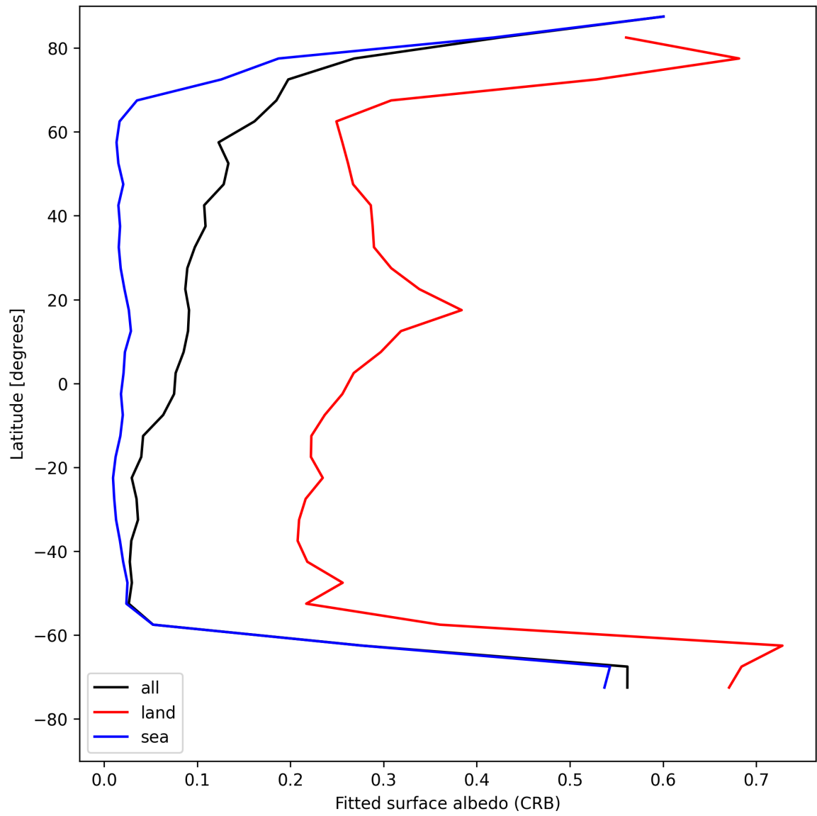
Figure 30: Zonal average of “Fitted surface albedo (CRB)” for 2025-07-29 to 2025-07-30.
