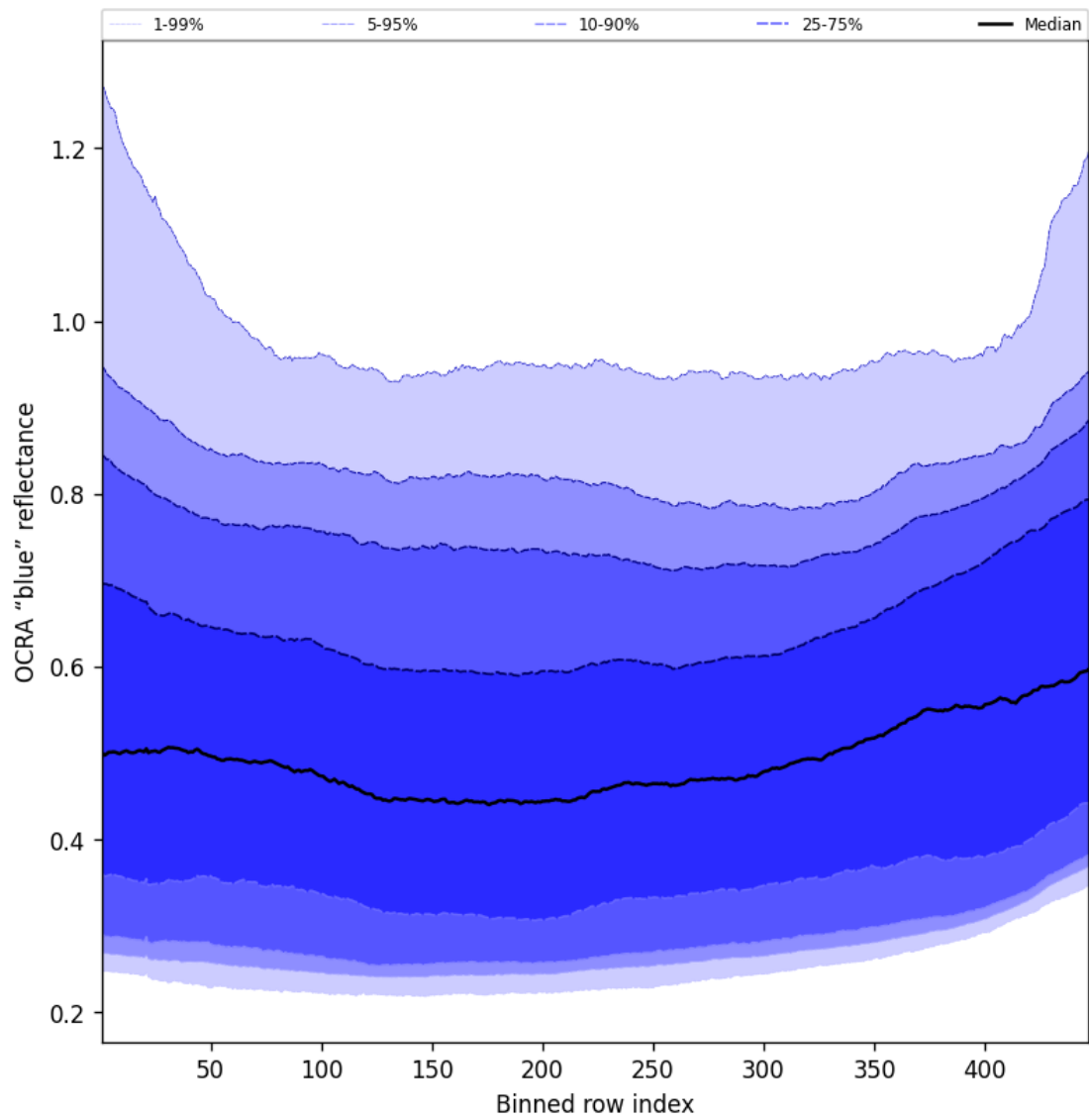
Figure 67: Along track statistics of “OCRA “blue” reflectance” for 2025-07-29 to 2025-07-30
