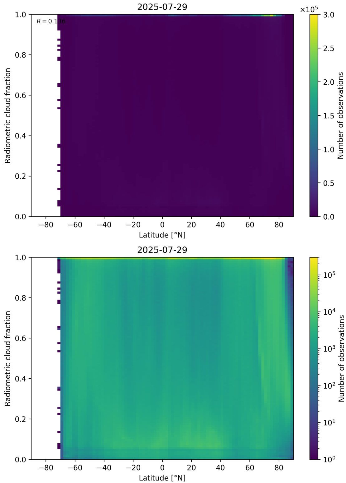
Figure 92: Scatter density plot of “Latitude” against “Radiometric cloud fraction” for 2025-07-29 to 2025-07-30.
