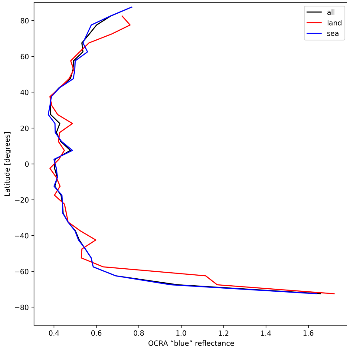
Figure 35: Zonal average of “OCRA “blue” reflectance” for 2025-07-29 to 2025-07-30.
