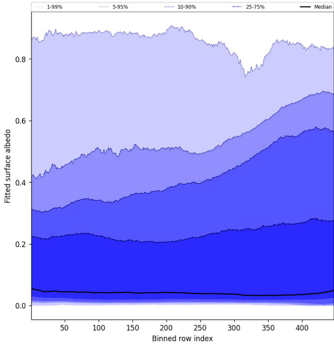
Figure 61: Along track statistics of “Fitted surface albedo” for 2025-07-29 to 2025-07-30
