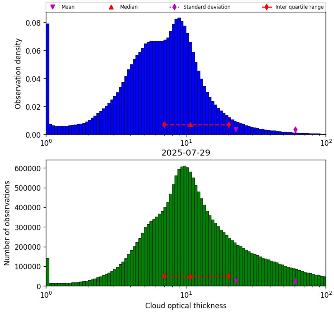
Figure 41: Histogram of “Cloud optical thickness” for 2025-07-29 to 2025-07-30
