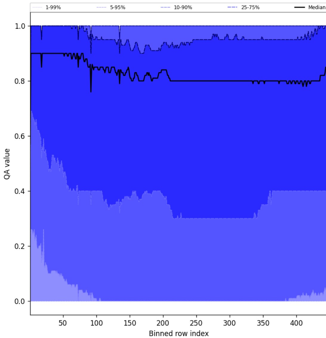
Figure 54: Along track statistics of “QA value” for 2025-07-29 to 2025-07-30
