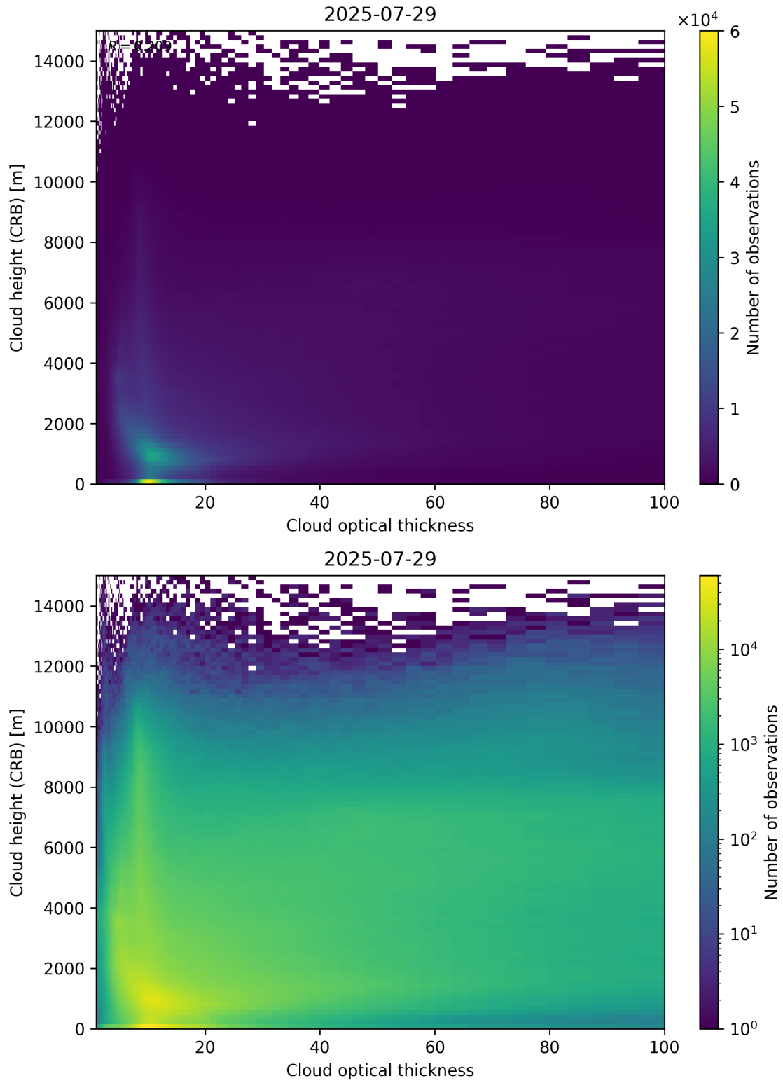
Figure 85: Scatter density plot of “Cloud optical thickness” against “Cloud height (CRB)” for 2025-07-29 to 2025-07-30.
