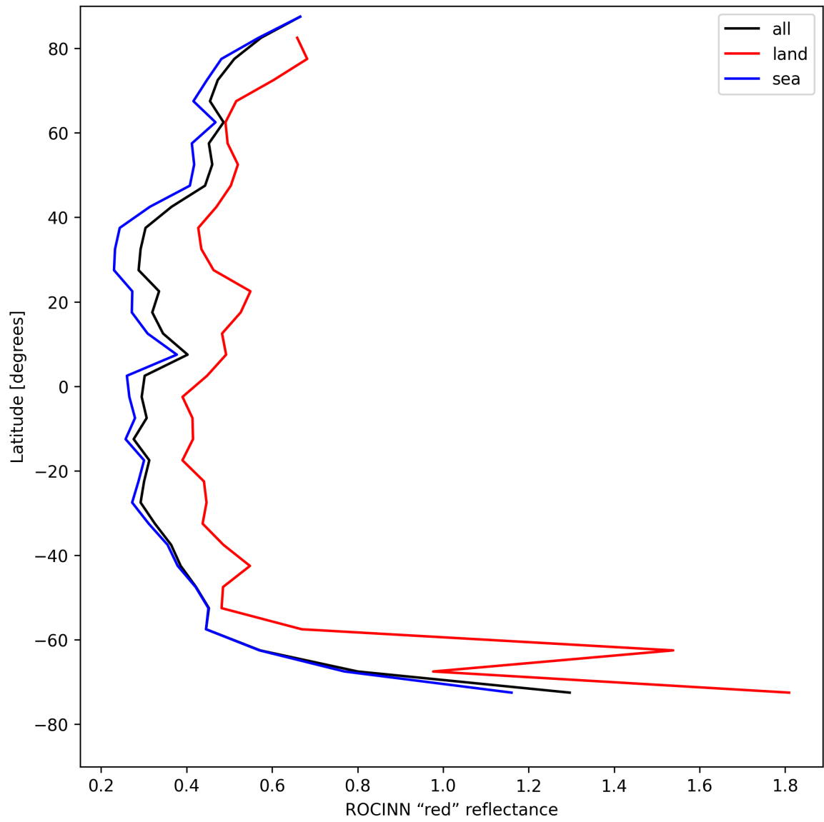
Figure 37: Zonal average of “ROCINN “red” reflectance” for 2025-07-29 to 2025-07-30.
