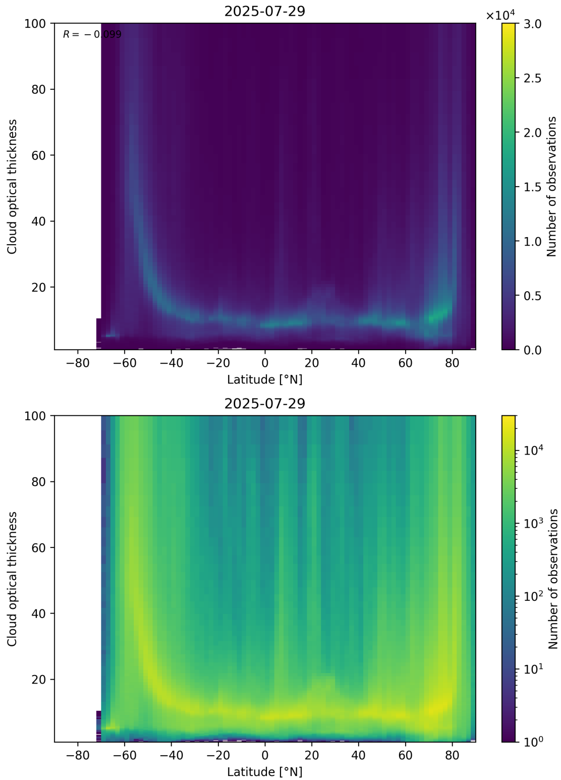
Figure 96: Scatter density plot of “Latitude” against “Cloud optical thickness” for 2025-07-29 to 2025-07-30.
