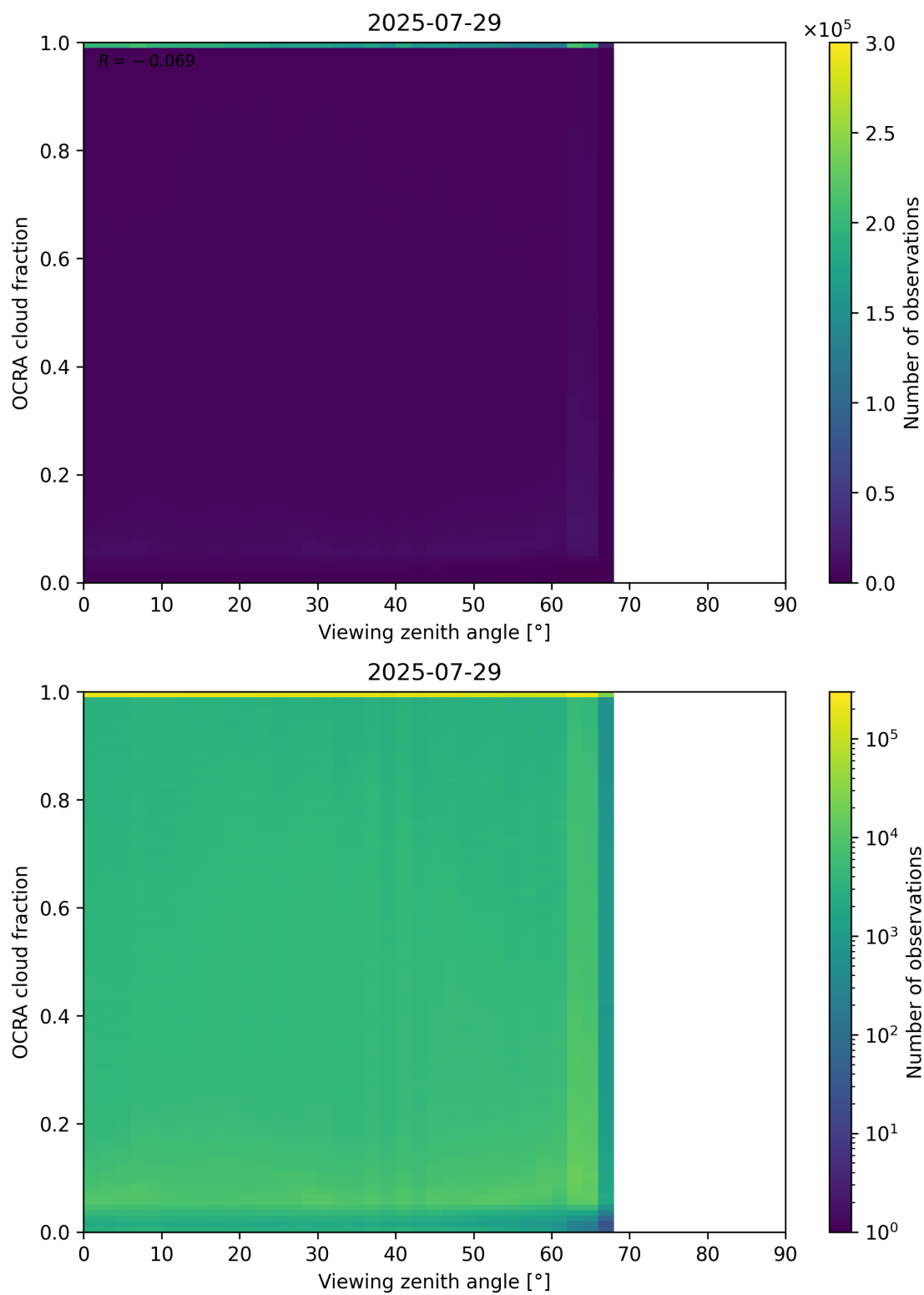
Figure 108: Scatter density plot of “Viewing zenith angle” against “OCRA cloud fraction” for 2025-07-29 to 2025-07-30.
