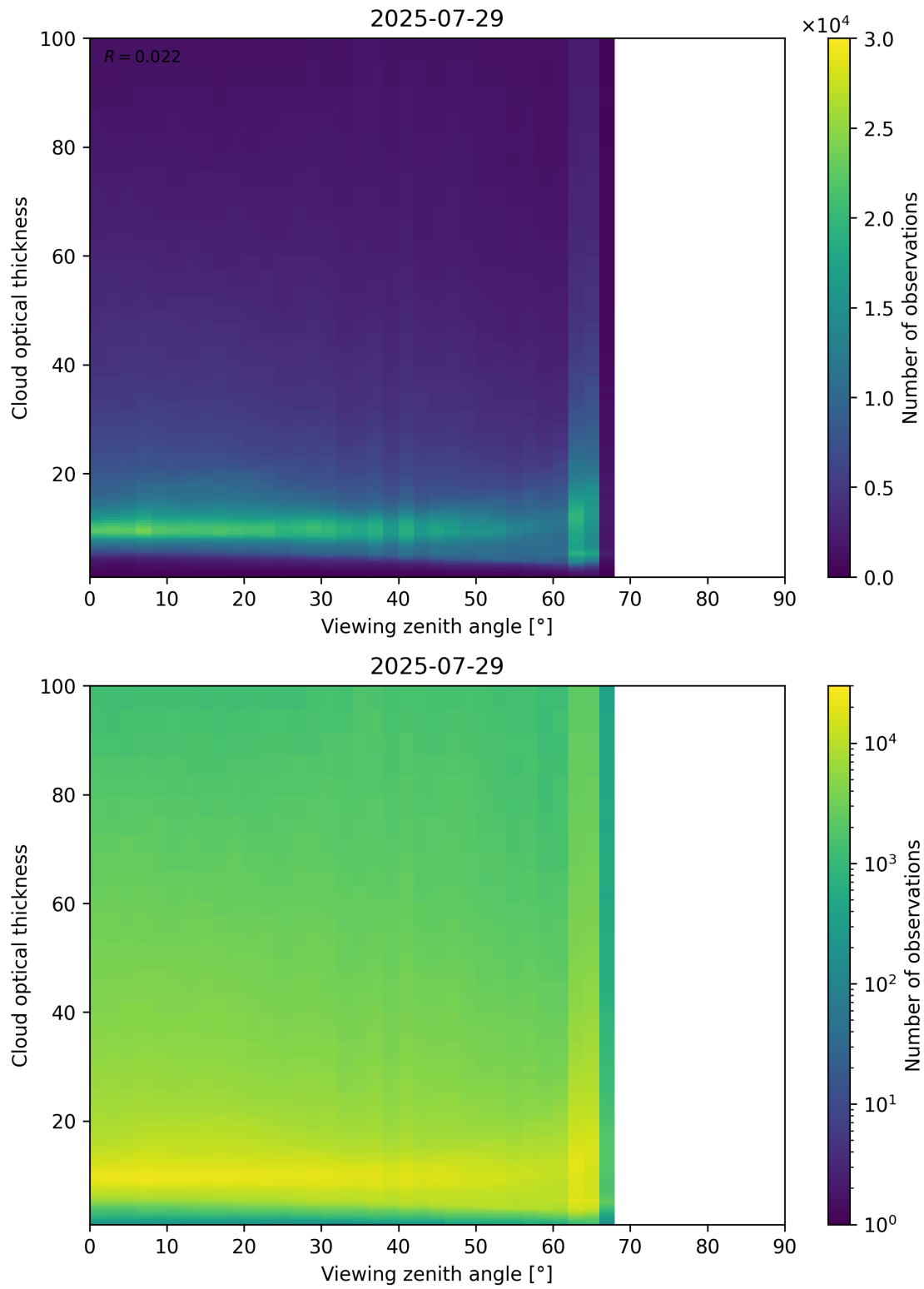
Figure 111: Scatter density plot of “Viewing zenith angle” against “Cloud optical thickness” for 2025-07-29 to 2025-07-30.
