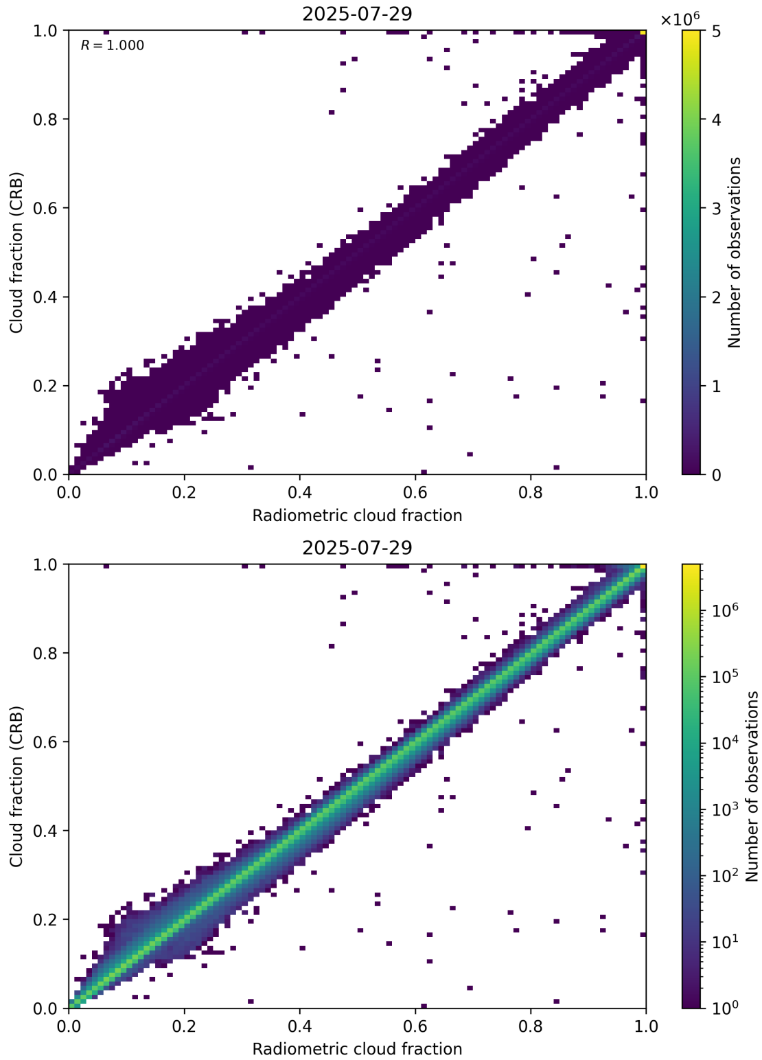
Figure 73: Scatter density plot of “Radiometric cloud fraction” against “Cloud fraction (CRB)” for 2025-07-29 to 2025-07-30.
