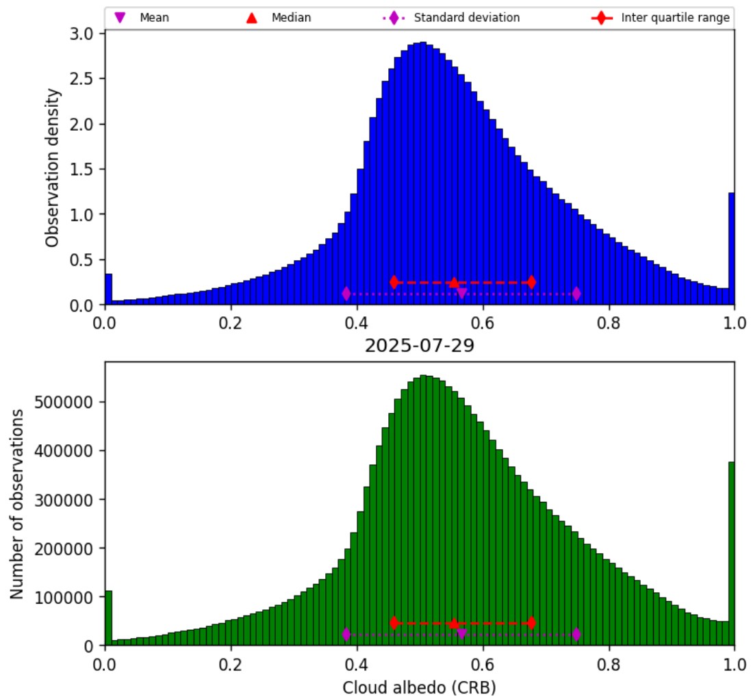
Figure 44: Histogram of “Cloud albedo (CRB)” for 2025-07-29 to 2025-07-30
