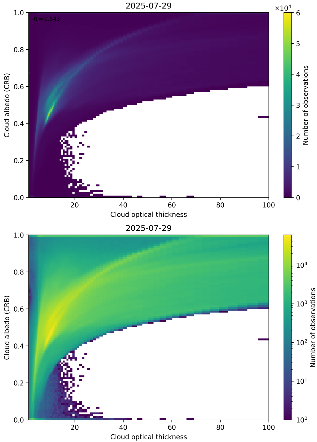
Figure 82: Scatter density plot of “Cloud optical thickness” against “Cloud albedo (CRB)” for 2025-07-29 to 2025-07-30.
