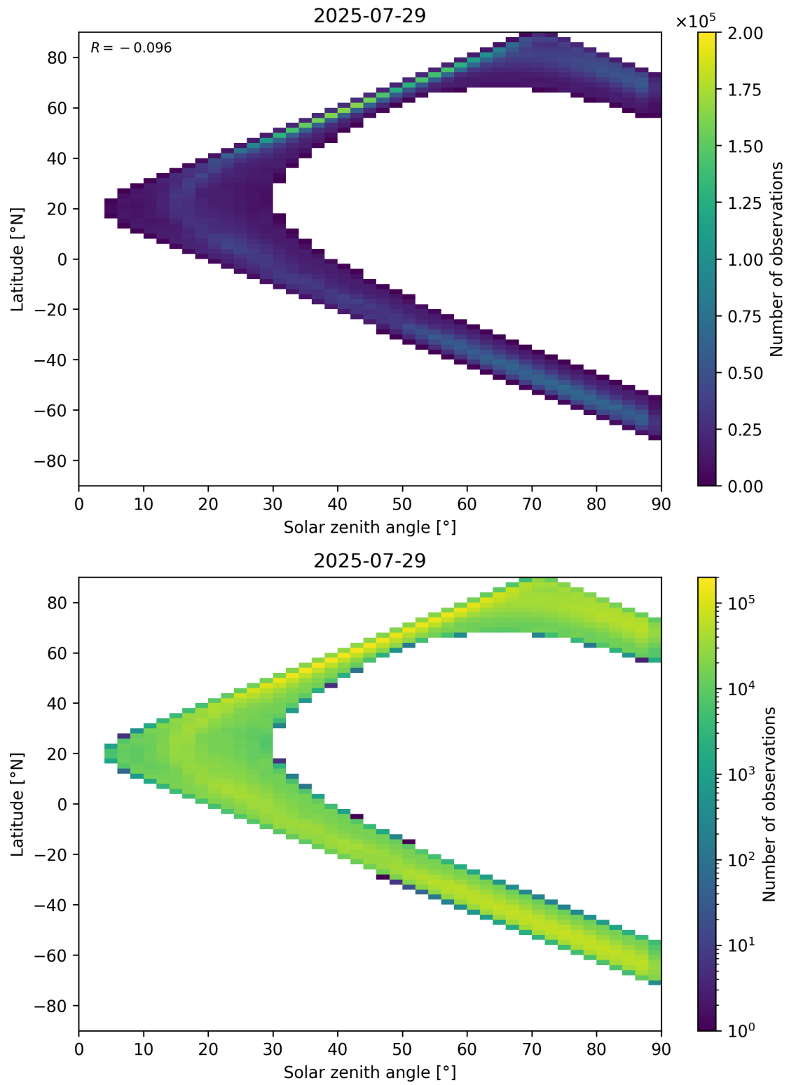
Figure 105: Scatter density plot of “Solar zenith angle” against “Latitude” for 2025-07-29 to 2025-07-30.
