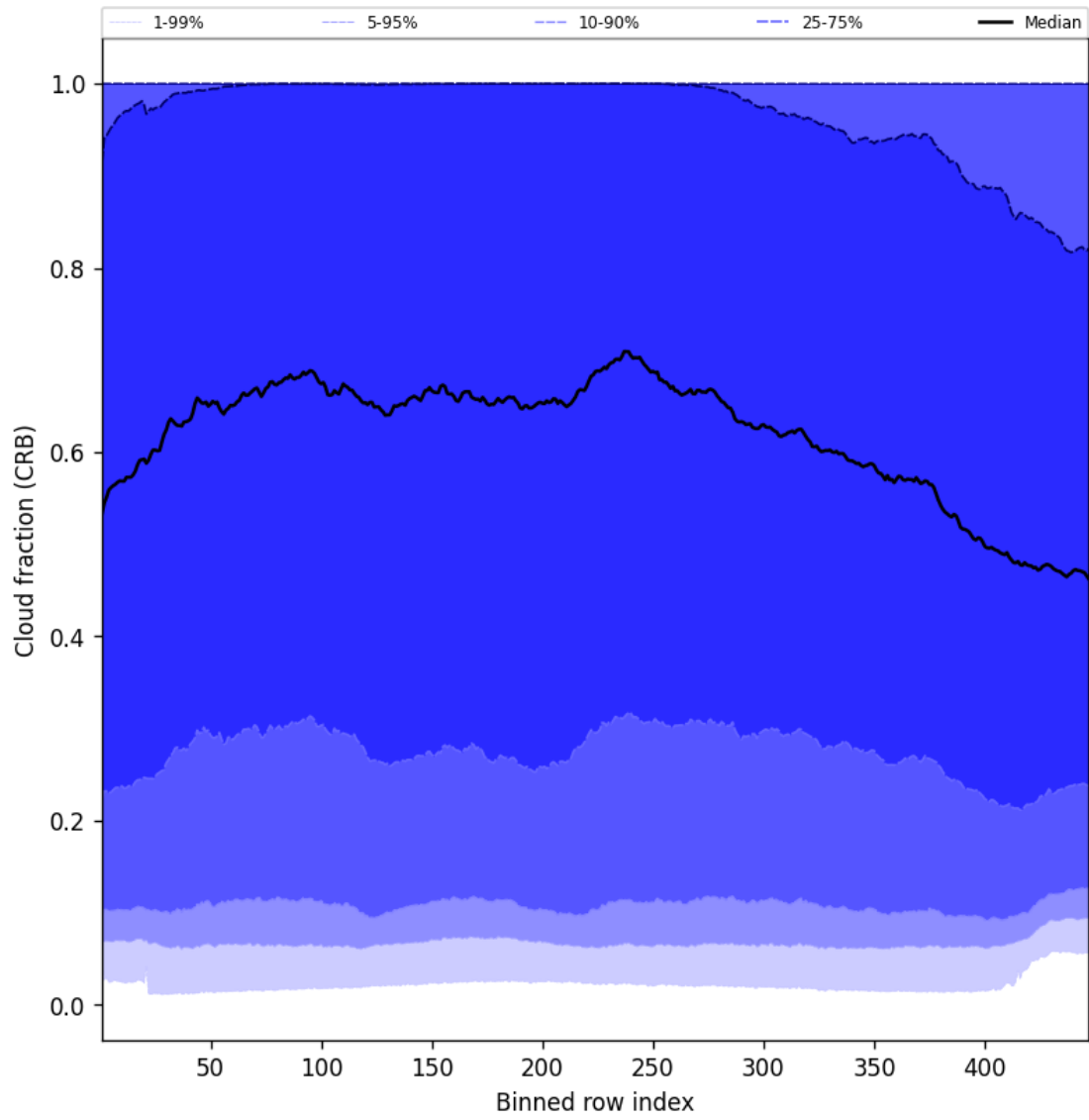
Figure 58: Along track statistics of “Cloud fraction (CRB)” for 2025-07-29 to 2025-07-30
