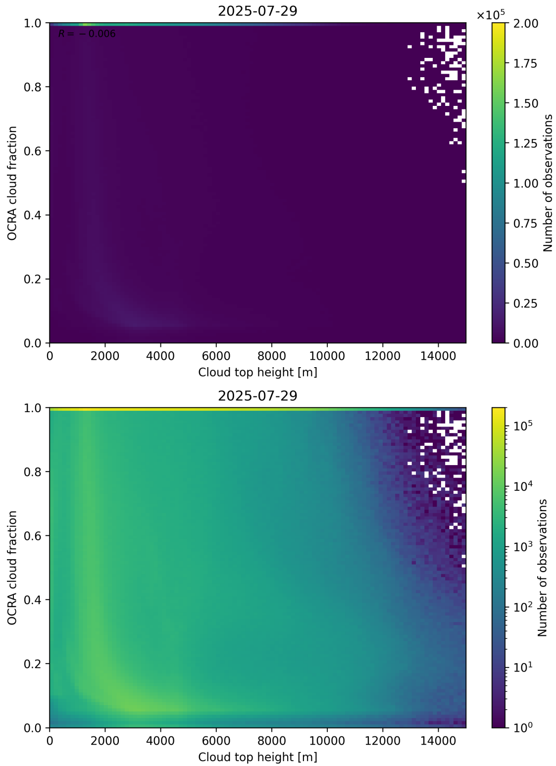
Figure 87: Scatter density plot of “Cloud top height” against “OCRA cloud fraction” for 2025-07-29 to 2025-07-30.
