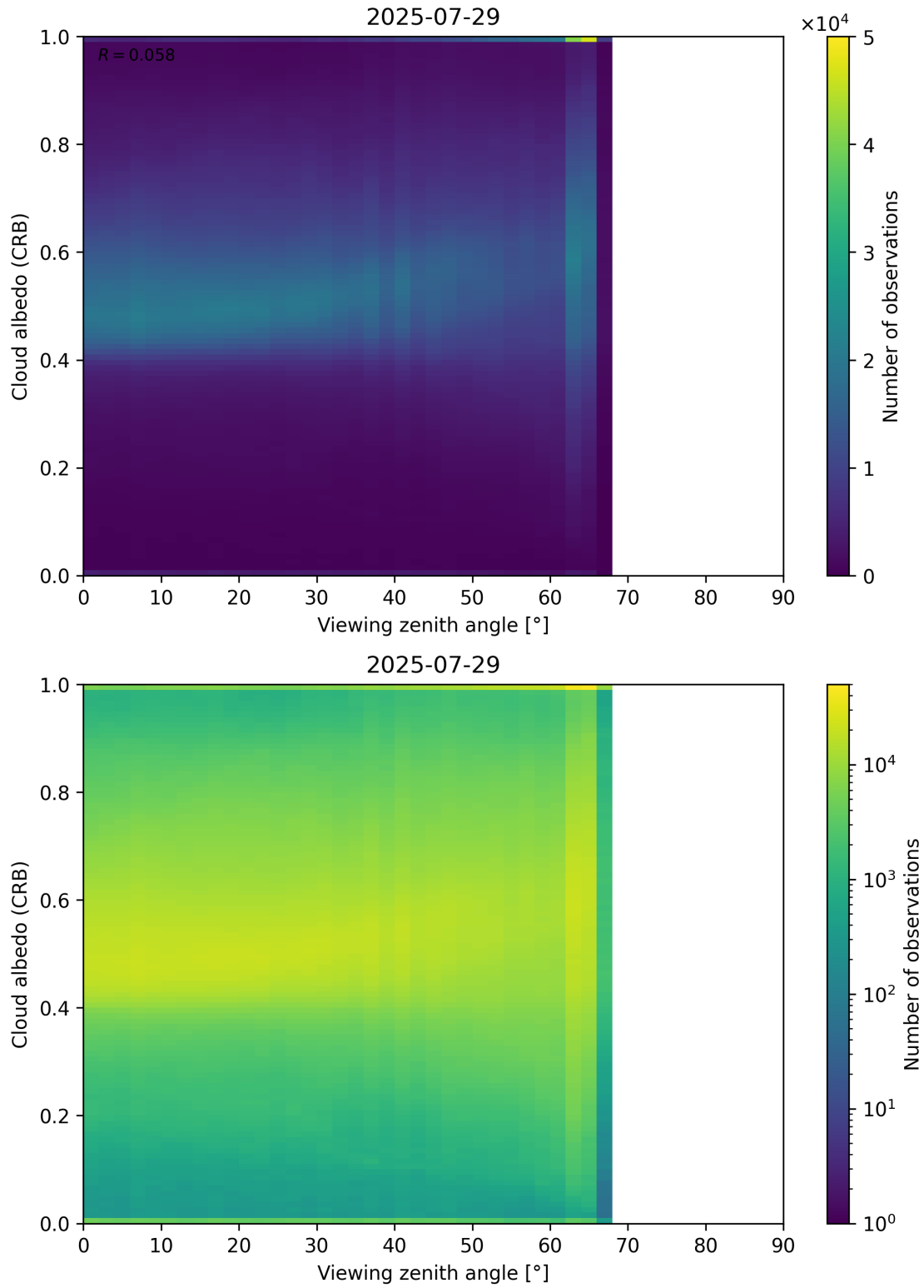
Figure 106: Scatter density plot of “Viewing zenith angle” against “Cloud albedo (CRB)” for 2025-07-29 to 2025-07-30.
