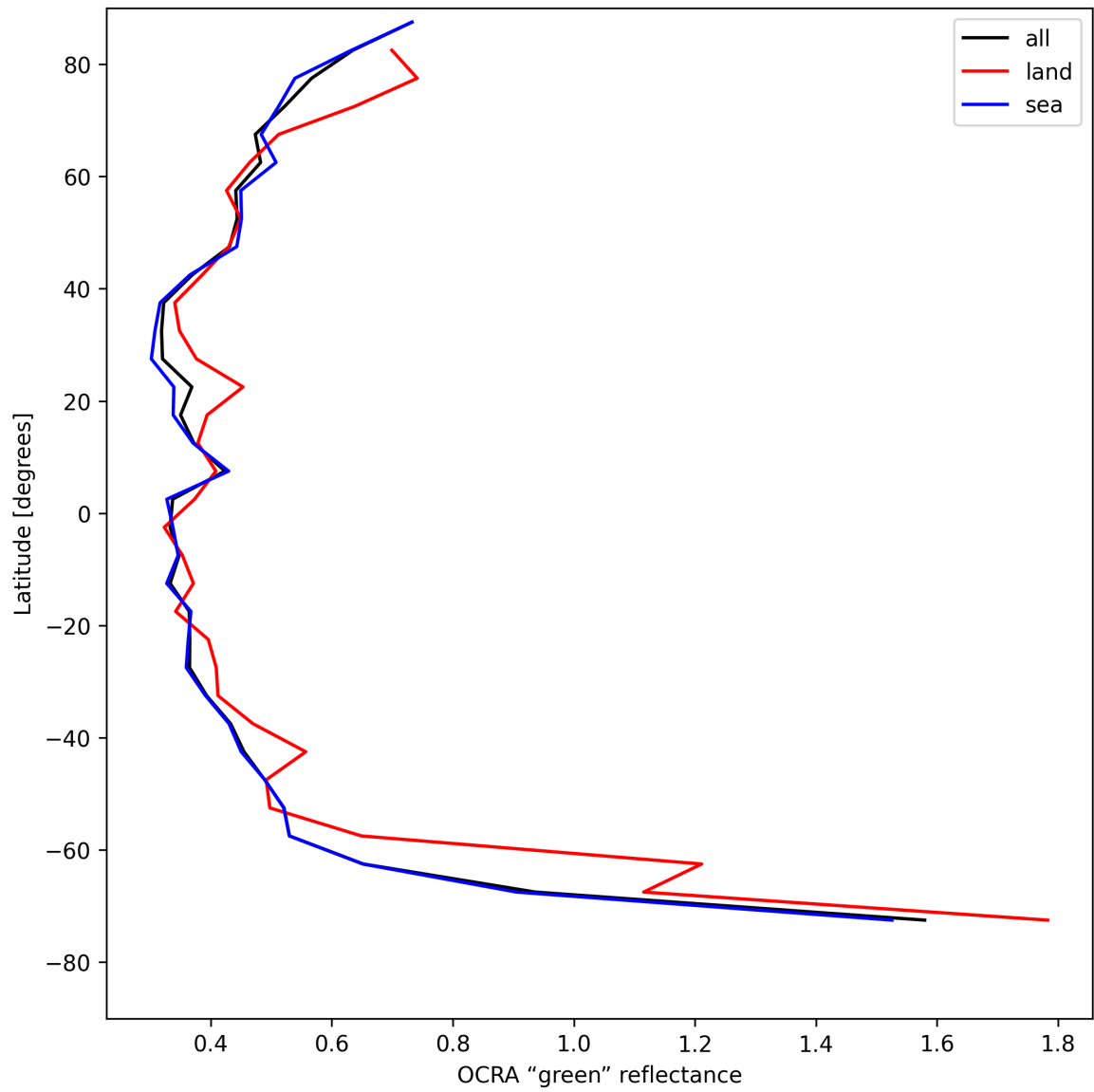
Figure 36: Zonal average of “OCRA “green” reflectance” for 2025-07-29 to 2025-07-30.
