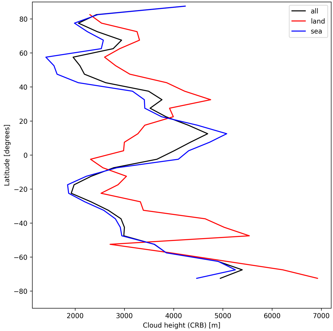
Figure 27: Zonal average of “Cloud height (CRB)” for 2025-07-29 to 2025-07-30.
