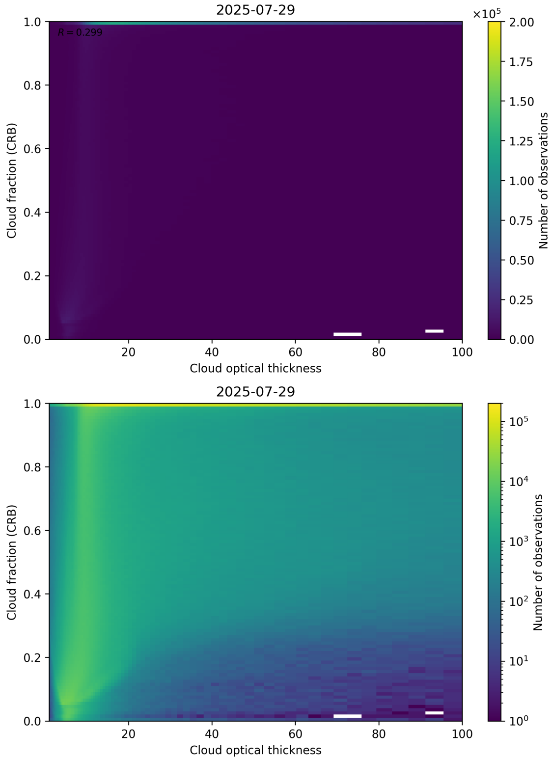
Figure 84: Scatter density plot of “Cloud optical thickness” against “Cloud fraction (CRB)” for 2025-07-29 to 2025-07-30.
