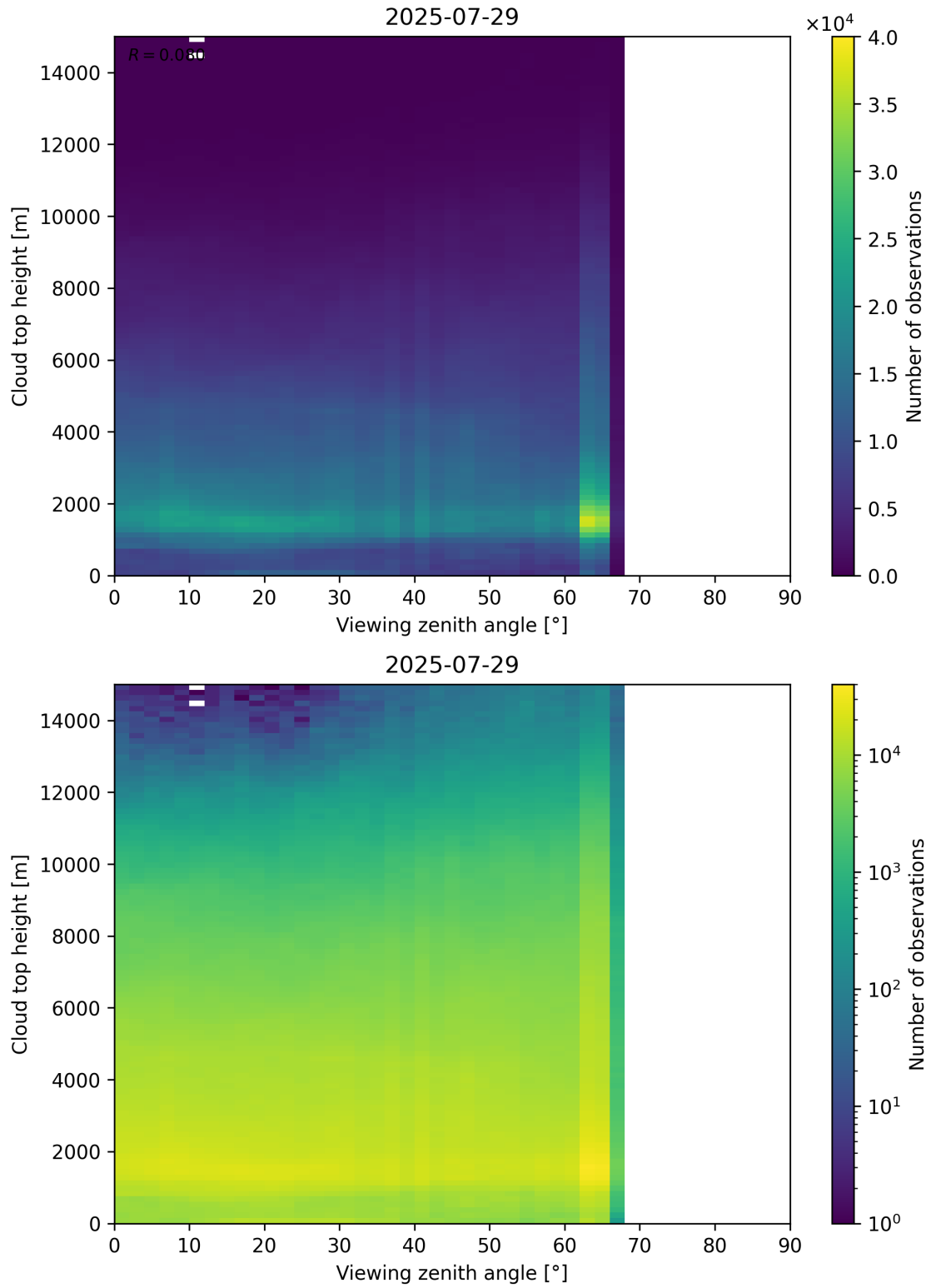
Figure 112: Scatter density plot of “Viewing zenith angle” against “Cloud top height” for 2025-07-29 to 2025-07-30.
