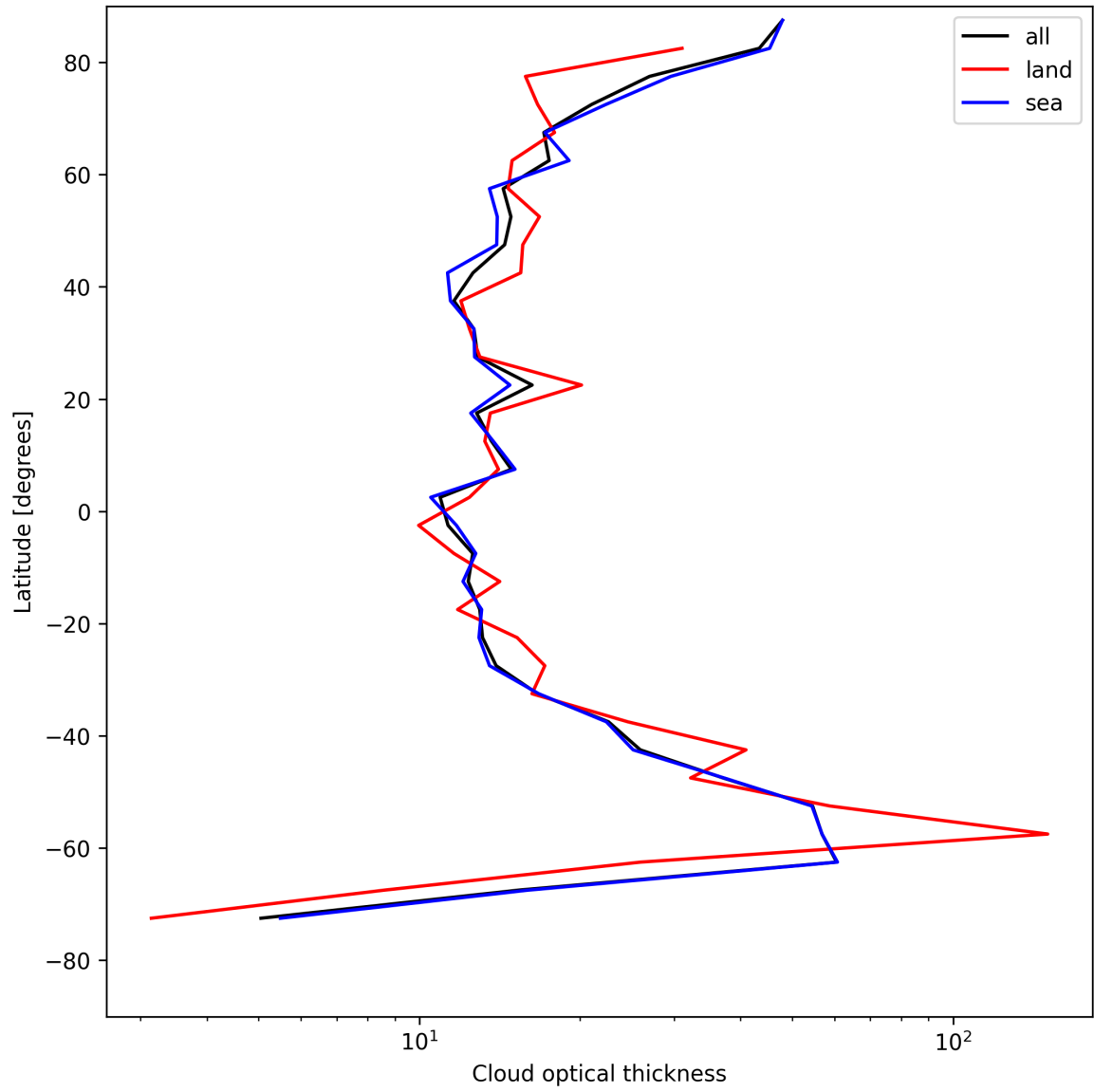
Figure 25: Zonal average of “Cloud optical thickness” for 2025-07-29 to 2025-07-30.
