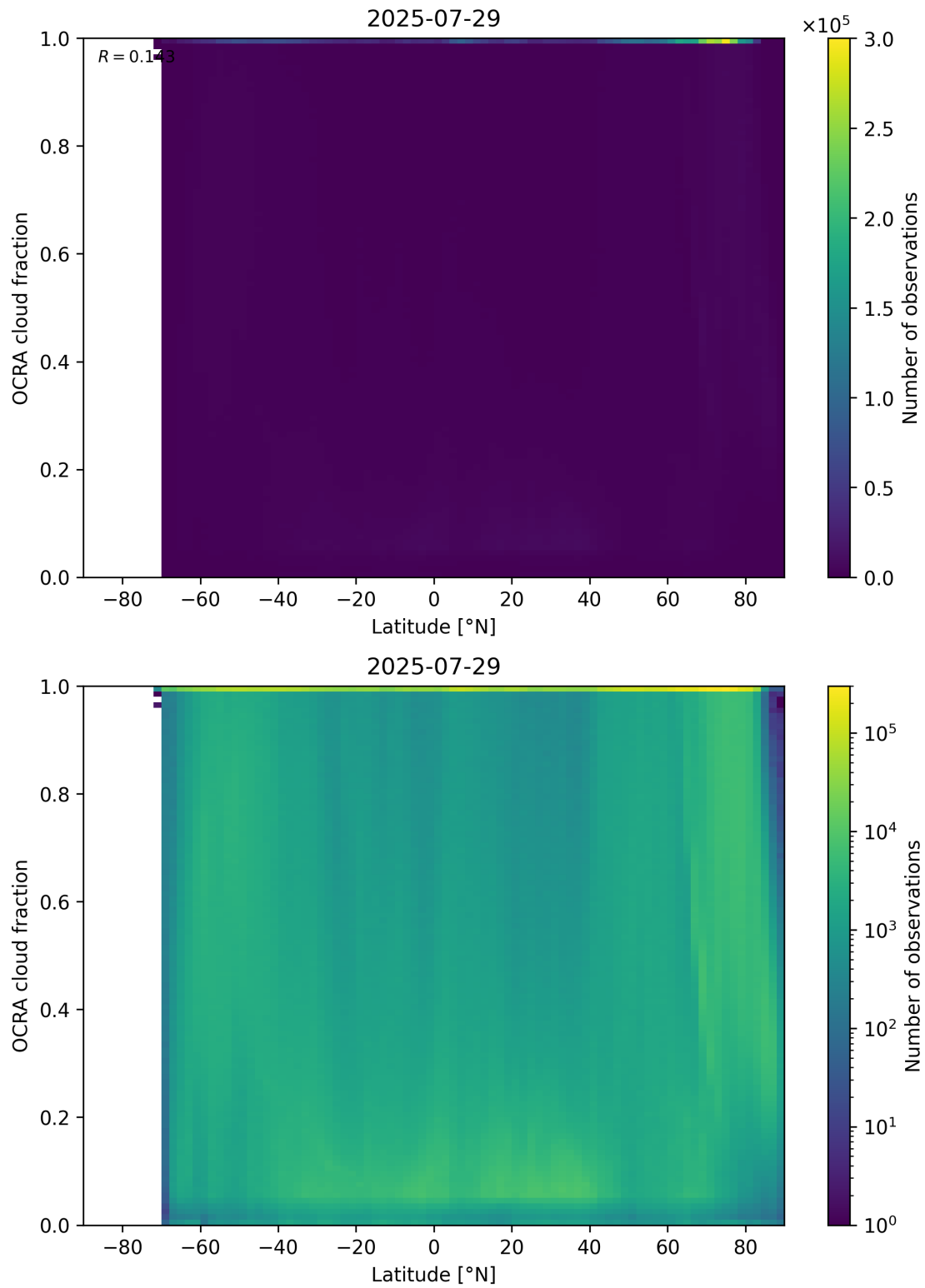
Figure 93: Scatter density plot of “Latitude” against “OCRA cloud fraction” for 2025-07-29 to 2025-07-30.
