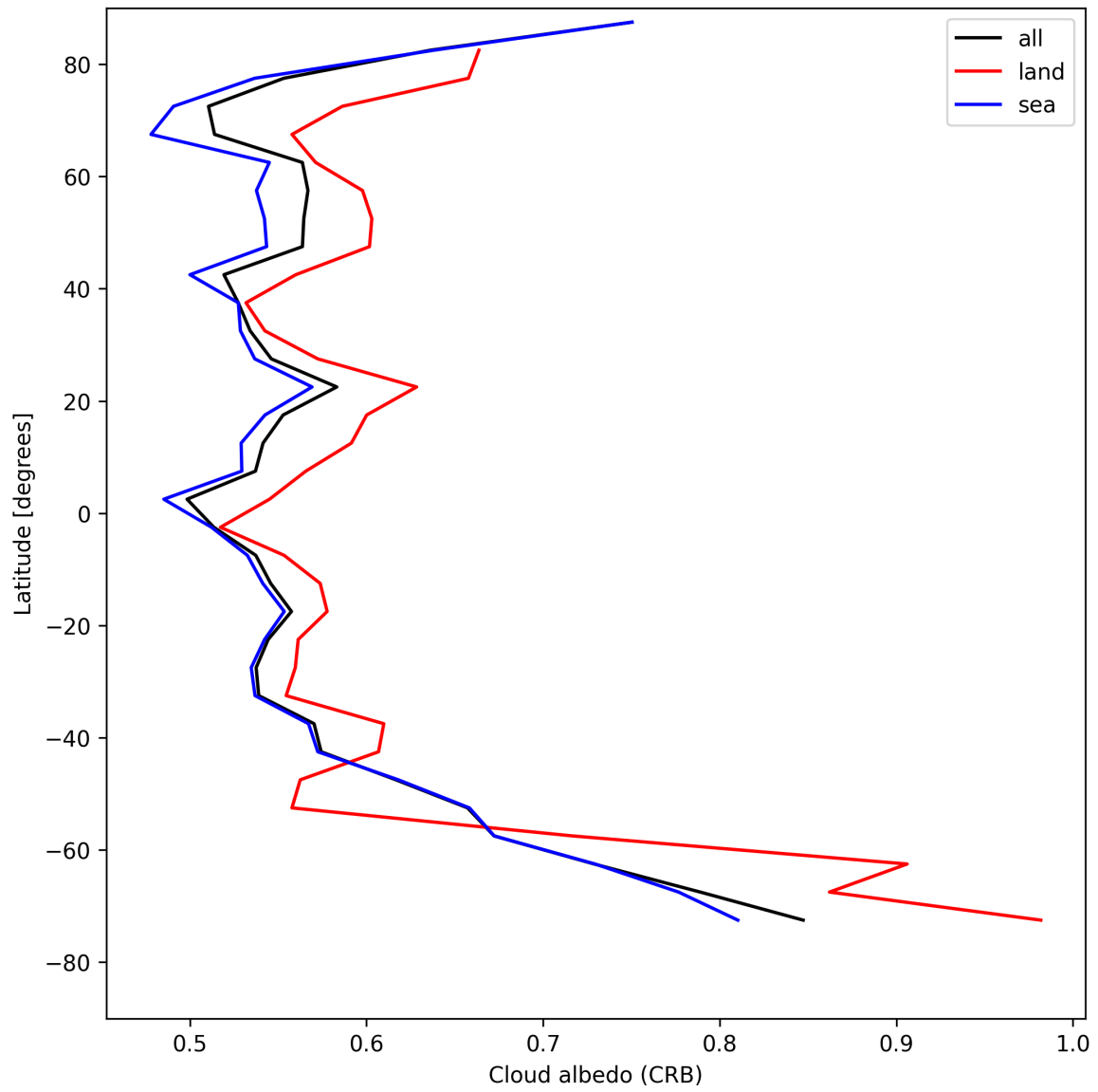
Figure 28: Zonal average of “Cloud albedo (CRB)” for 2025-07-29 to 2025-07-30.
