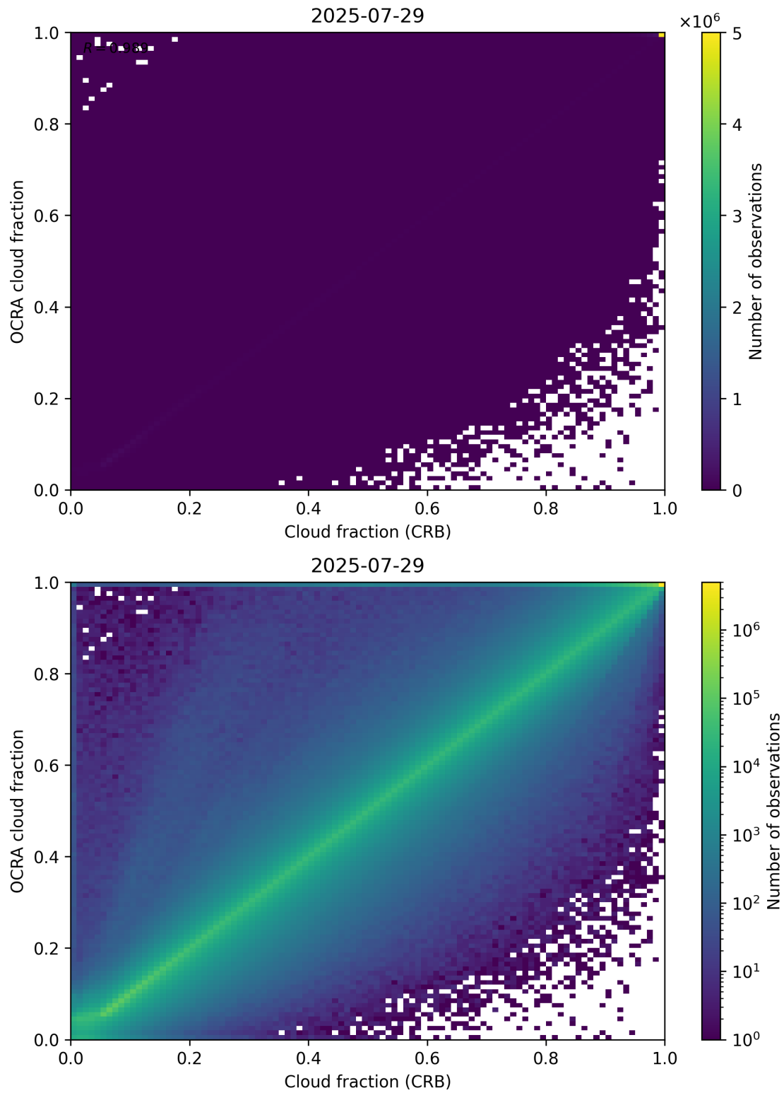
Figure 78: Scatter density plot of “Cloud fraction (CRB)” against “OCRA cloud fraction” for 2025-07-29 to 2025-07-30.
