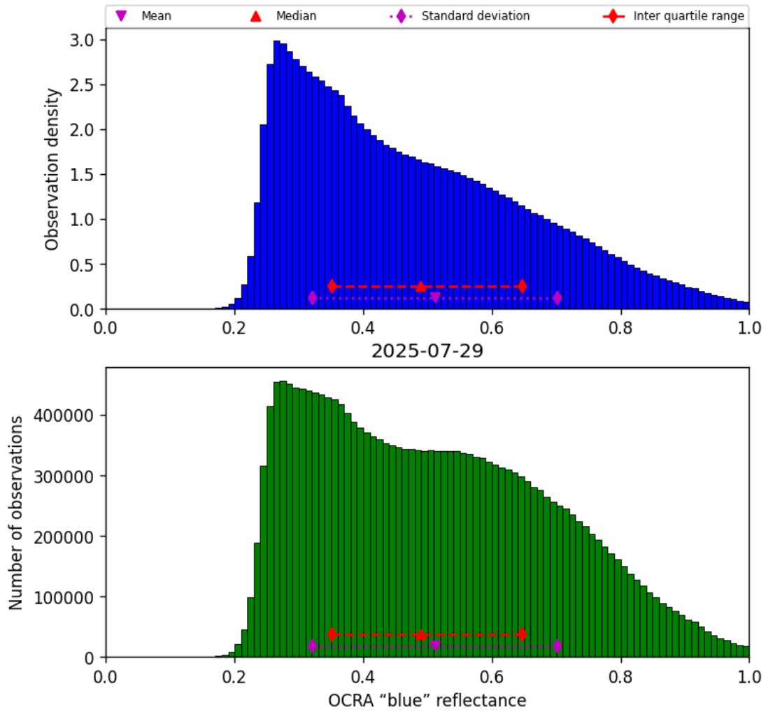
Figure 51: Histogram of “OCRA “blue” reflectance” for 2025-07-29 to 2025-07-30
