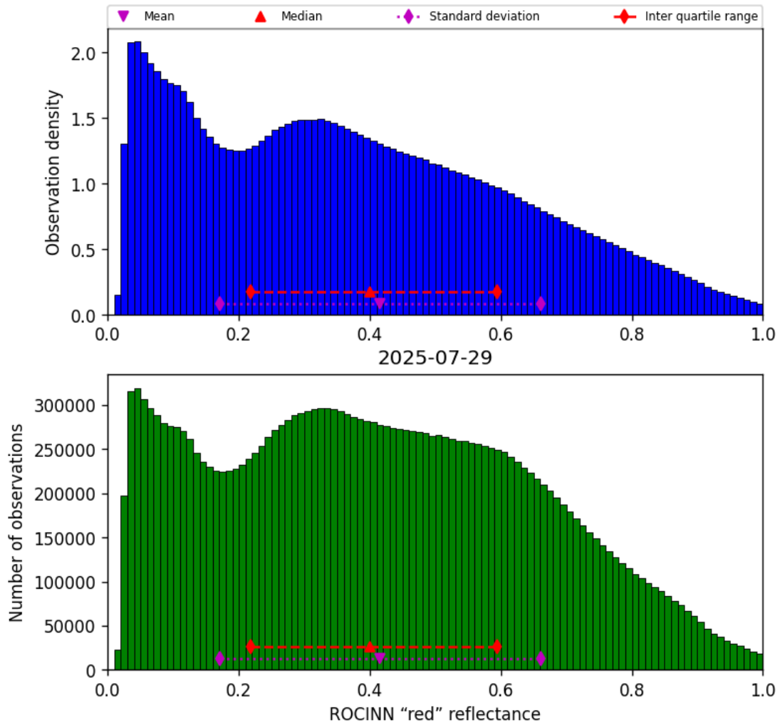
Figure 53: Histogram of “ROCINN “red” reflectance” for 2025-07-29 to 2025-07-30
