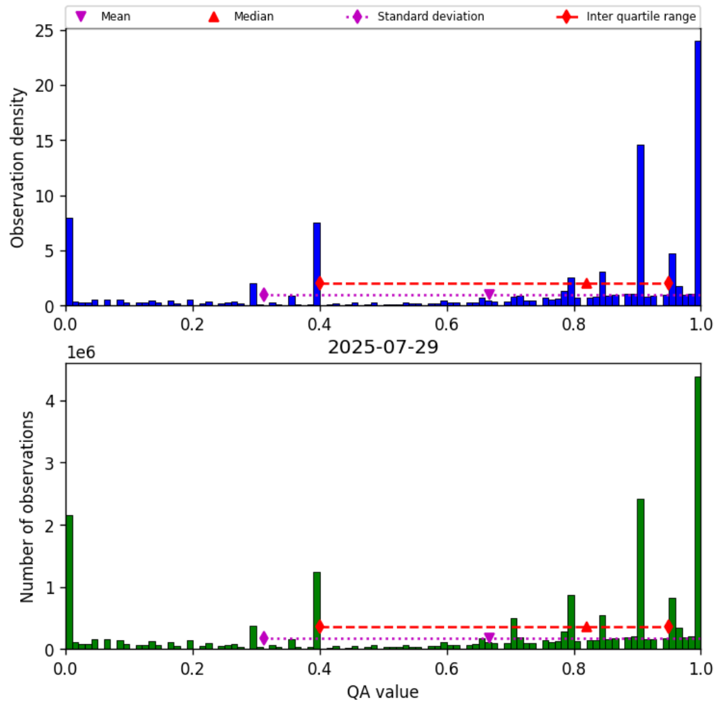
Figure 38: Histogram of “QA value” for 2025-07-29 to 2025-07-30
