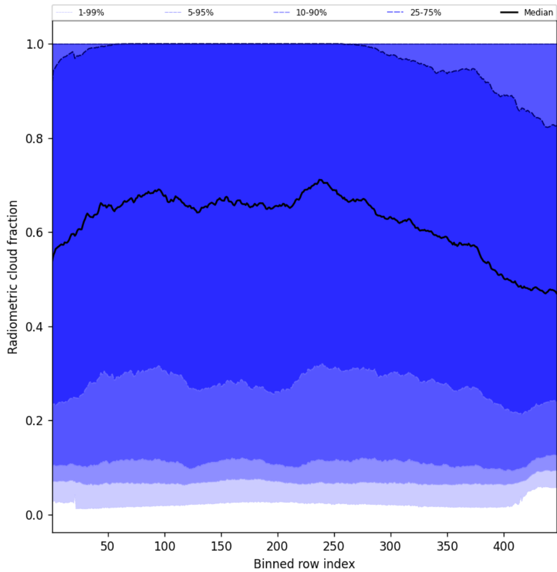
Figure 55: Along track statistics of “Radiometric cloud fraction” for 2025-07-29 to 2025-07-30
