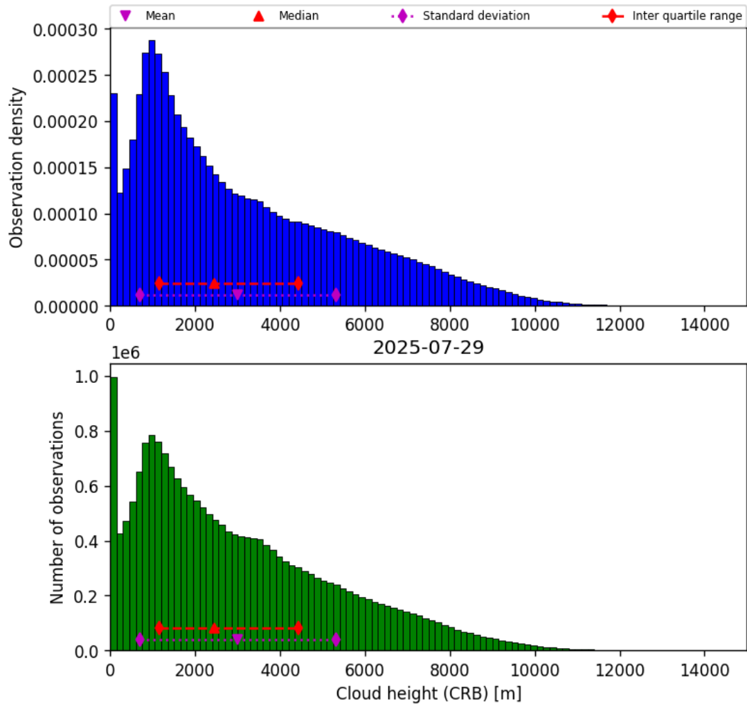
Figure 43: Histogram of “Cloud height (CRB)” for 2025-07-29 to 2025-07-30
