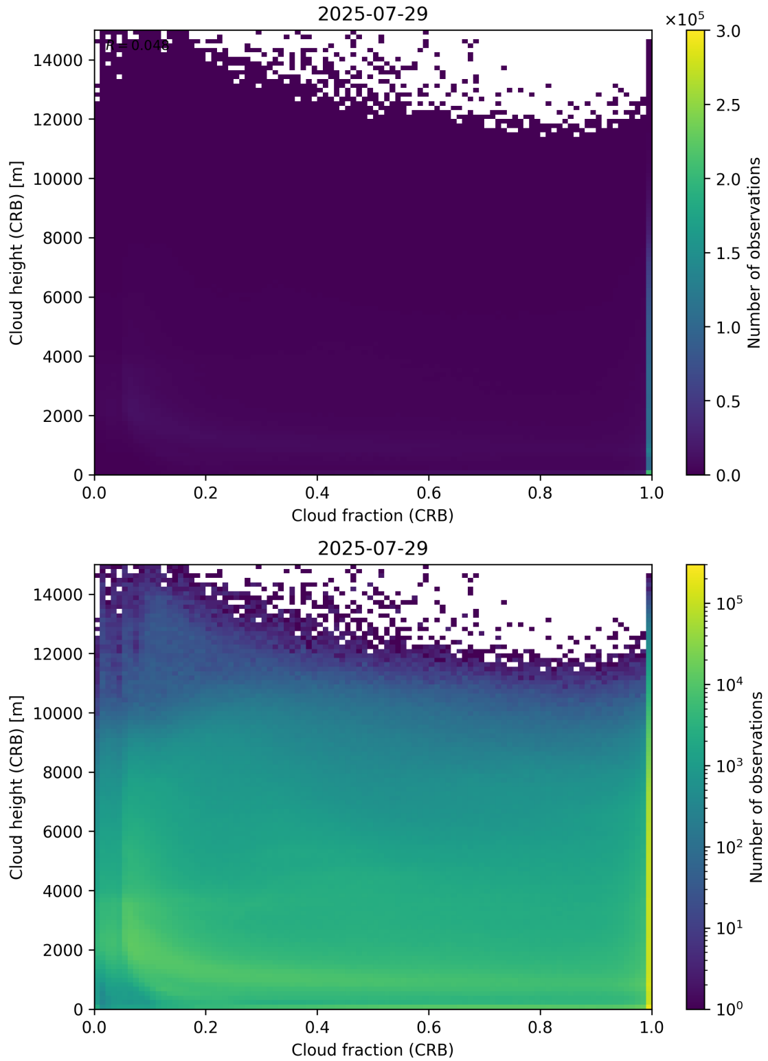
Figure 79: Scatter density plot of “Cloud fraction (CRB)” against “Cloud height (CRB)” for 2025-07-29 to 2025-07-30.
