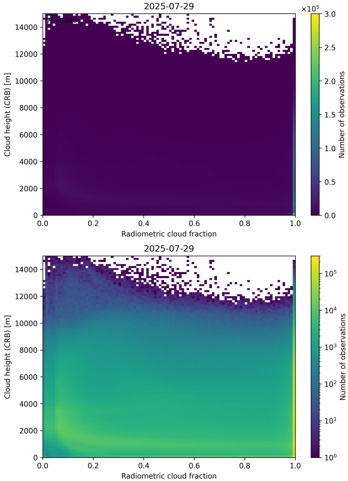
Figure 74: Scatter density plot of “Radiometric cloud fraction” against “Cloud height (CRB)” for 2025-07-29 to 2025-07-30.
