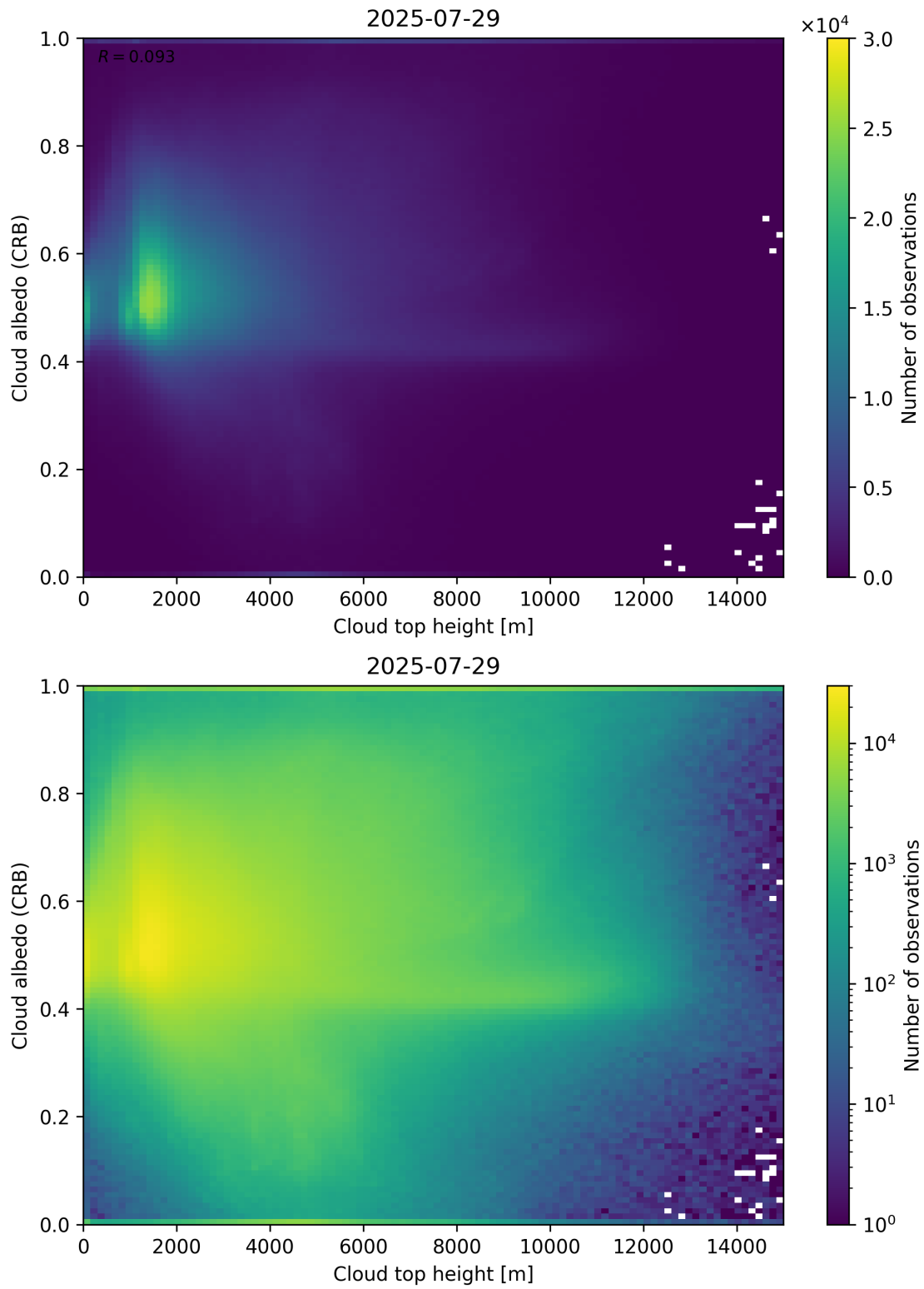
Figure 86: Scatter density plot of “Cloud top height” against “Cloud albedo (CRB)” for 2025-07-29 to 2025-07-30.
