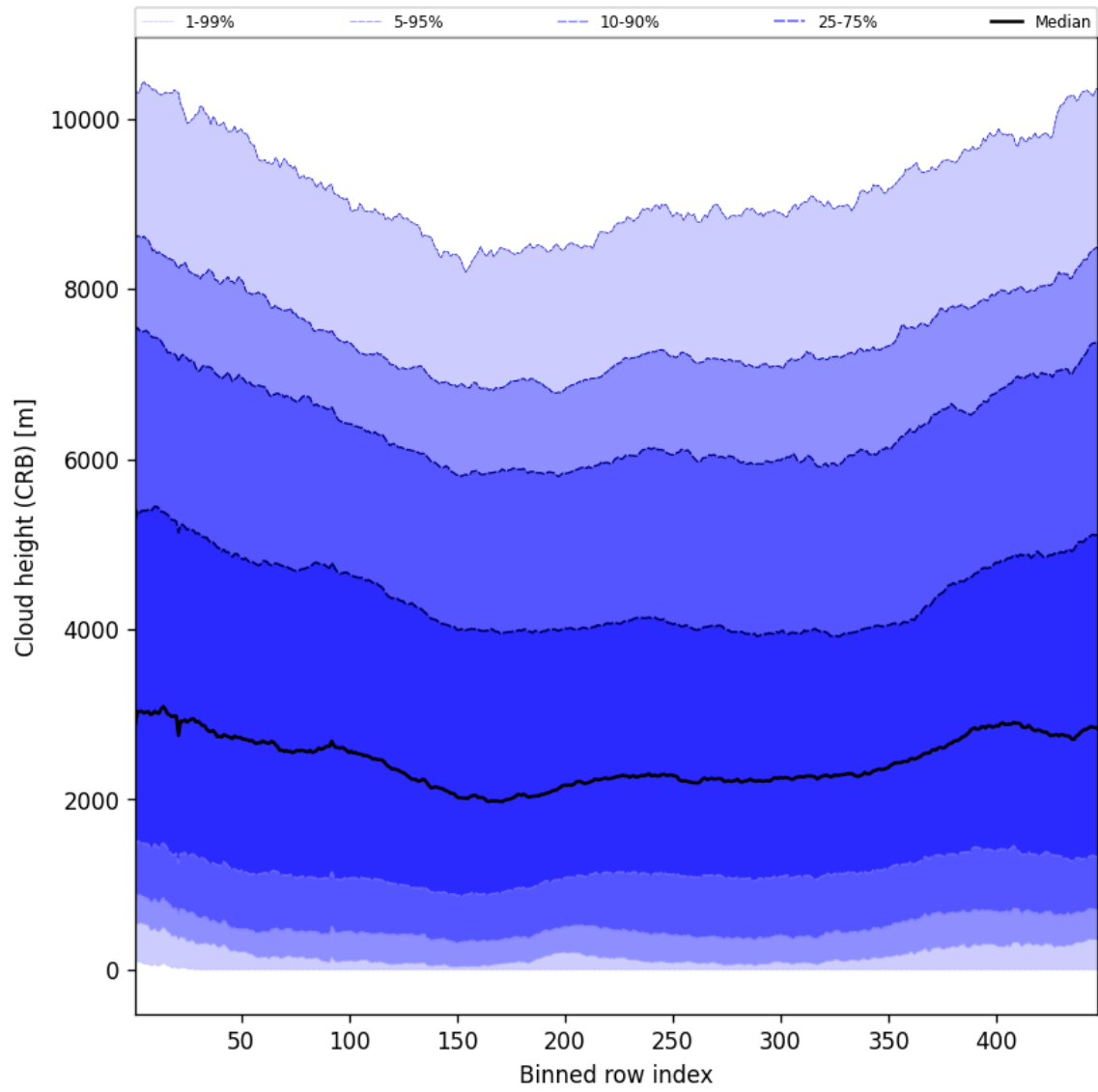
Figure 59: Along track statistics of “Cloud height (CRB)” for 2025-07-29 to 2025-07-30
