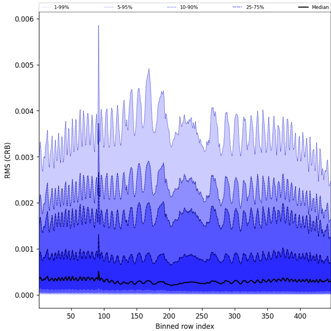
Figure 64: Along track statistics of "RMS (CRB)" for 2025-07-29 to 2025-07-30
