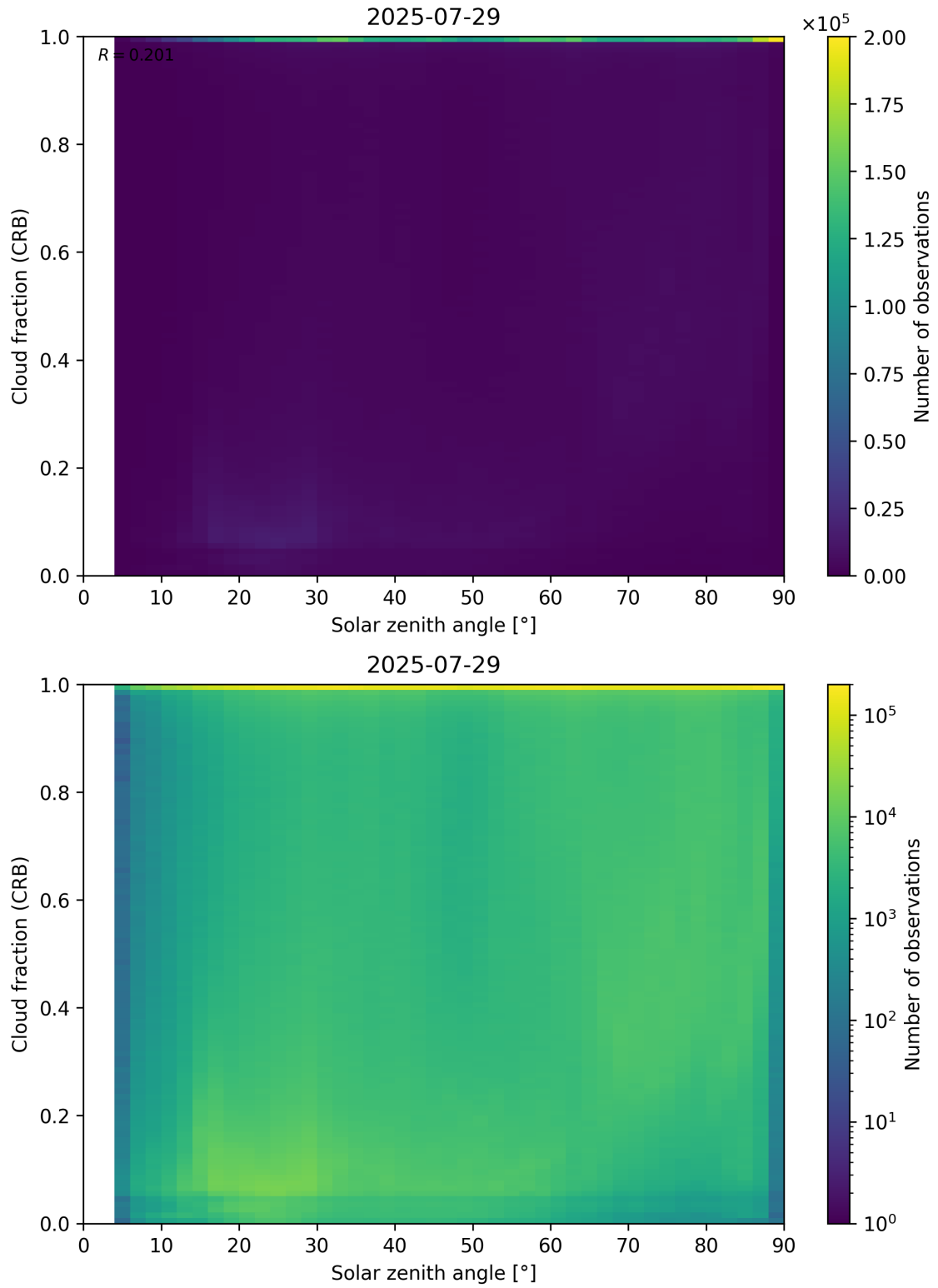
Figure 101: Scatter density plot of “Solar zenith angle” against “Cloud fraction (CRB)” for 2025-07-29 to 2025-07-30.
