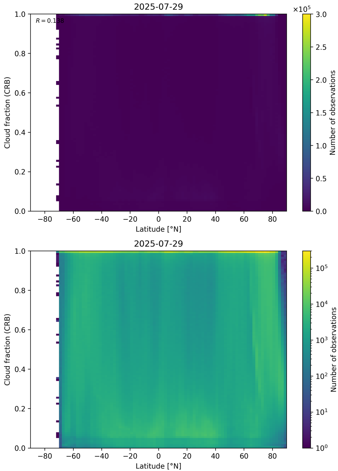
Figure 94: Scatter density plot of “Latitude” against “Cloud fraction (CRB)” for 2025-07-29 to 2025-07-30.
