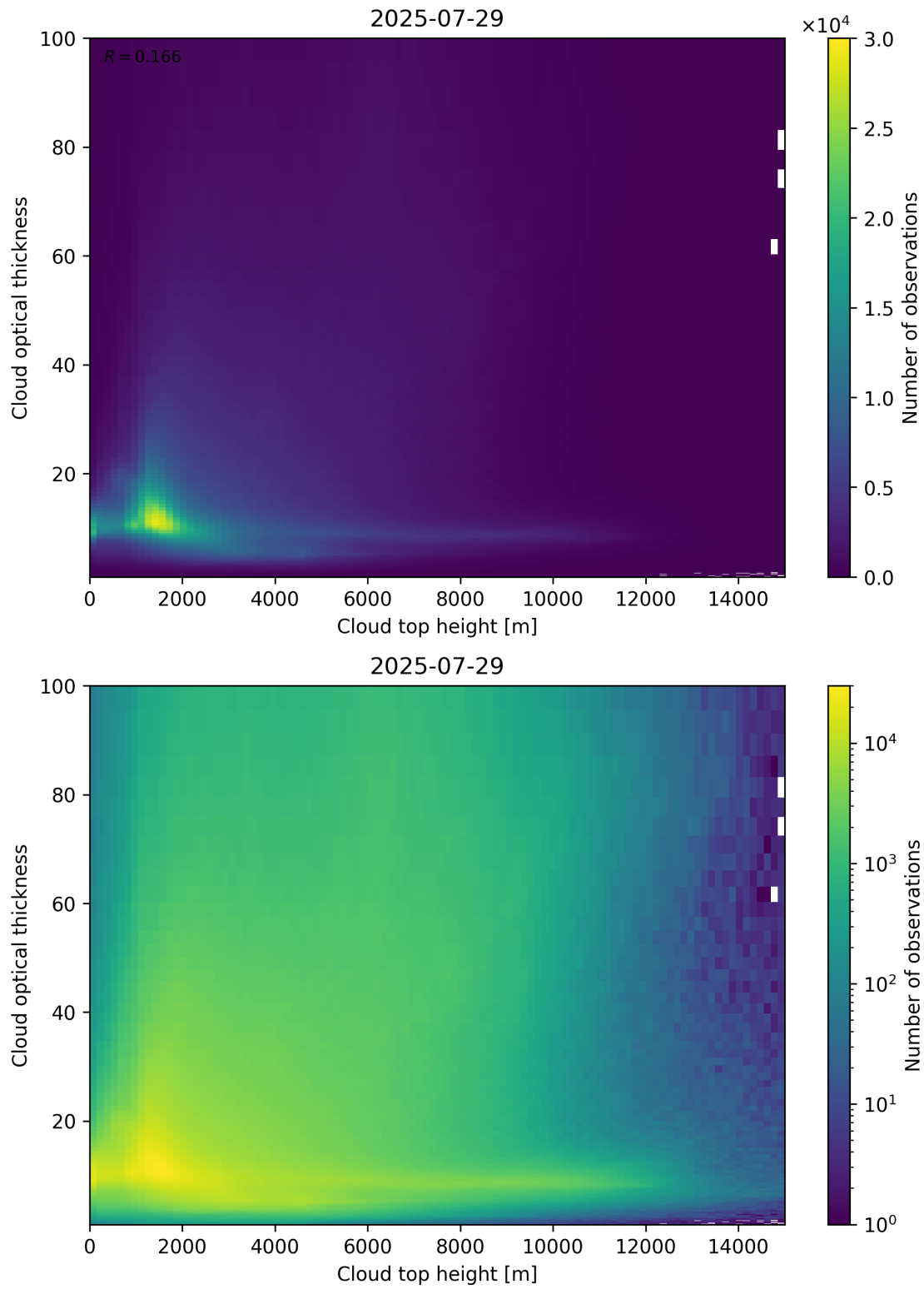
Figure 90: Scatter density plot of “Cloud top height” against “Cloud optical thickness” for 2025-07-29 to 2025-07-30.
