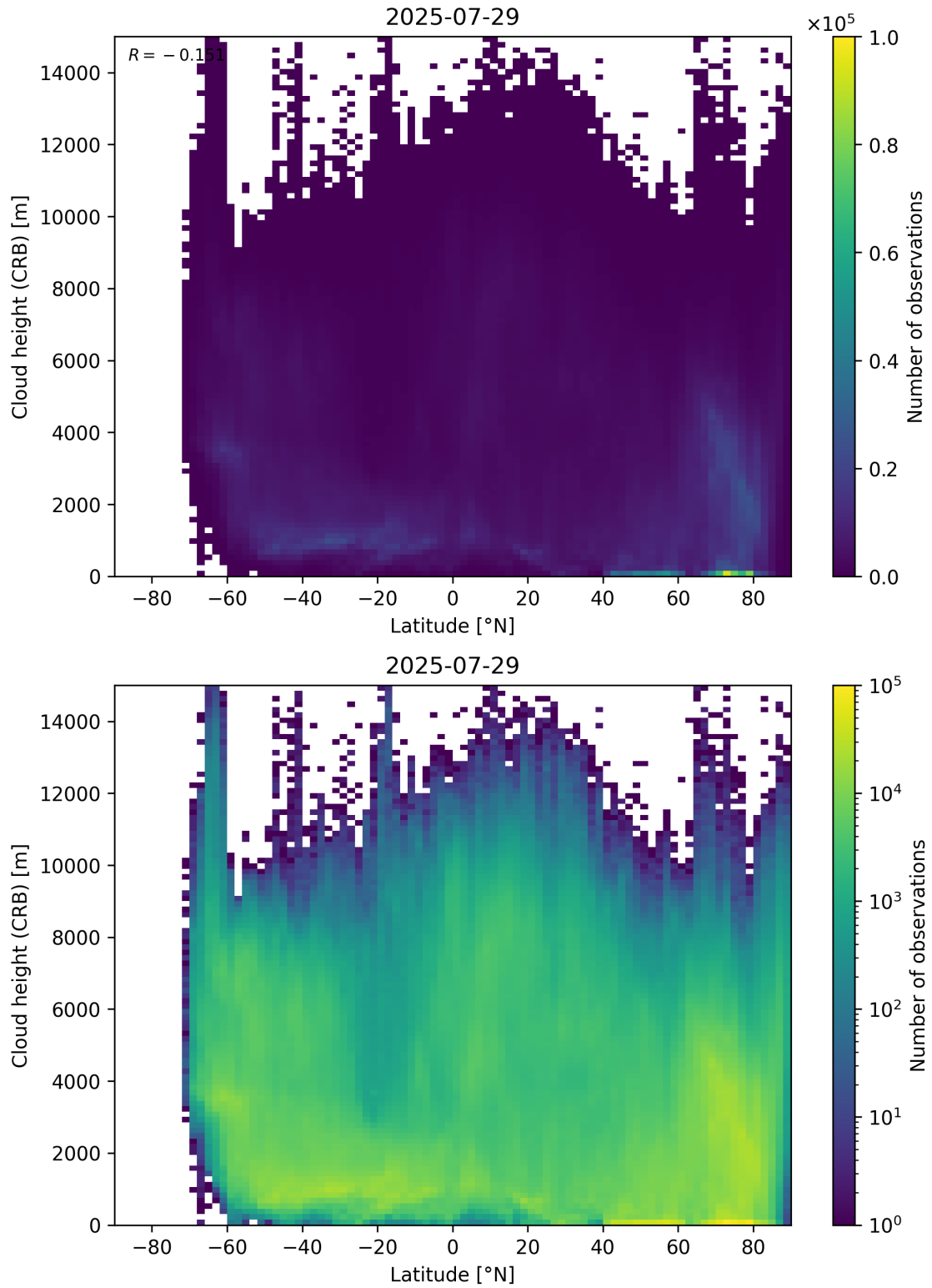
Figure 95: Scatter density plot of “Latitude” against “Cloud height (CRB)” for 2025-07-29 to 2025-07-30.
