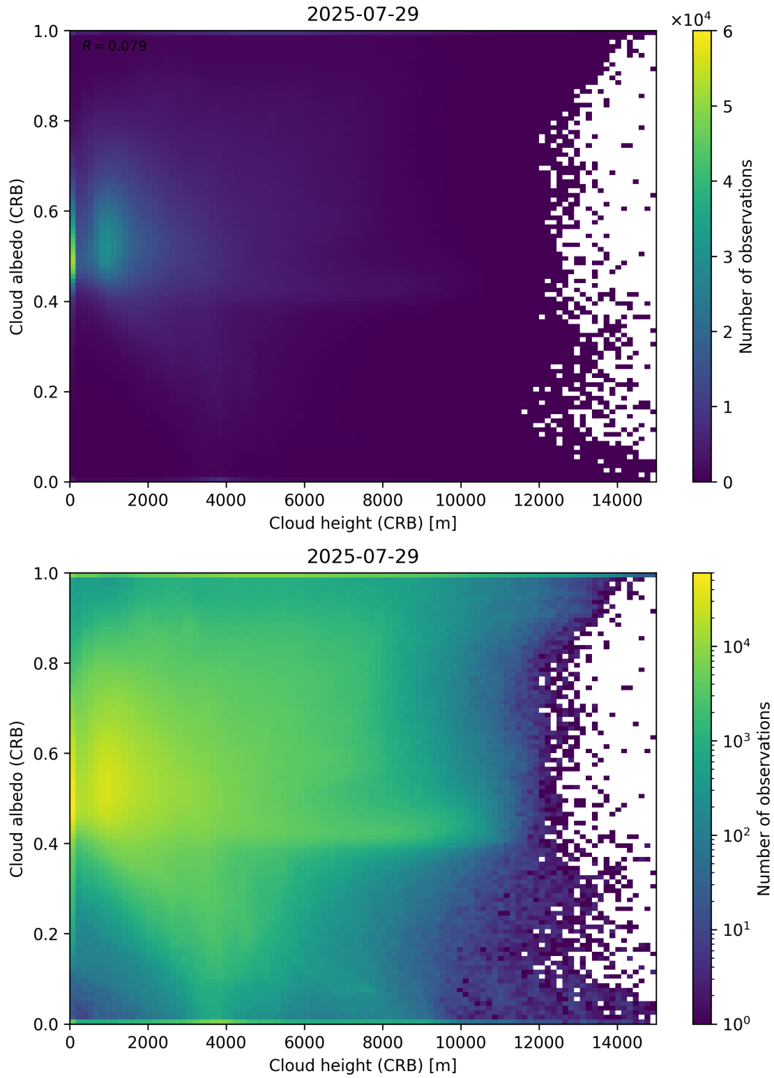
Figure 80: Scatter density plot of “Cloud height (CRB)” against “Cloud albedo (CRB)” for 2025-07-29 to 2025-07-30.
