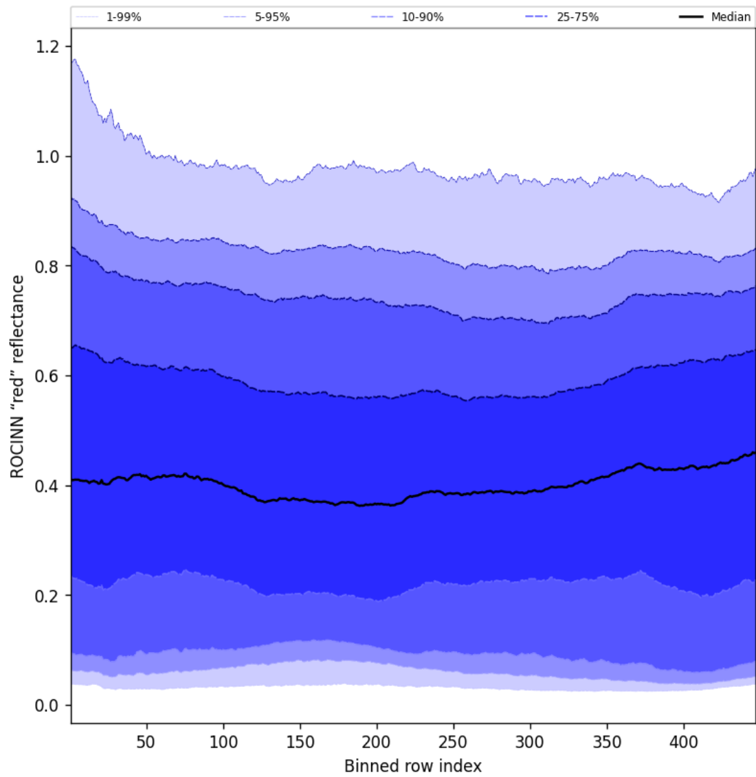
Figure 69: Along track statistics of "ROCINN "red" reflectance" for 2025-07-29 to 2025-07-30
