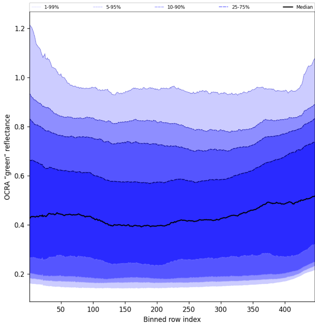
Figure 68: Along track statistics of "OCRA "green" reflectance" for 2025-07-29 to 2025-07-30
