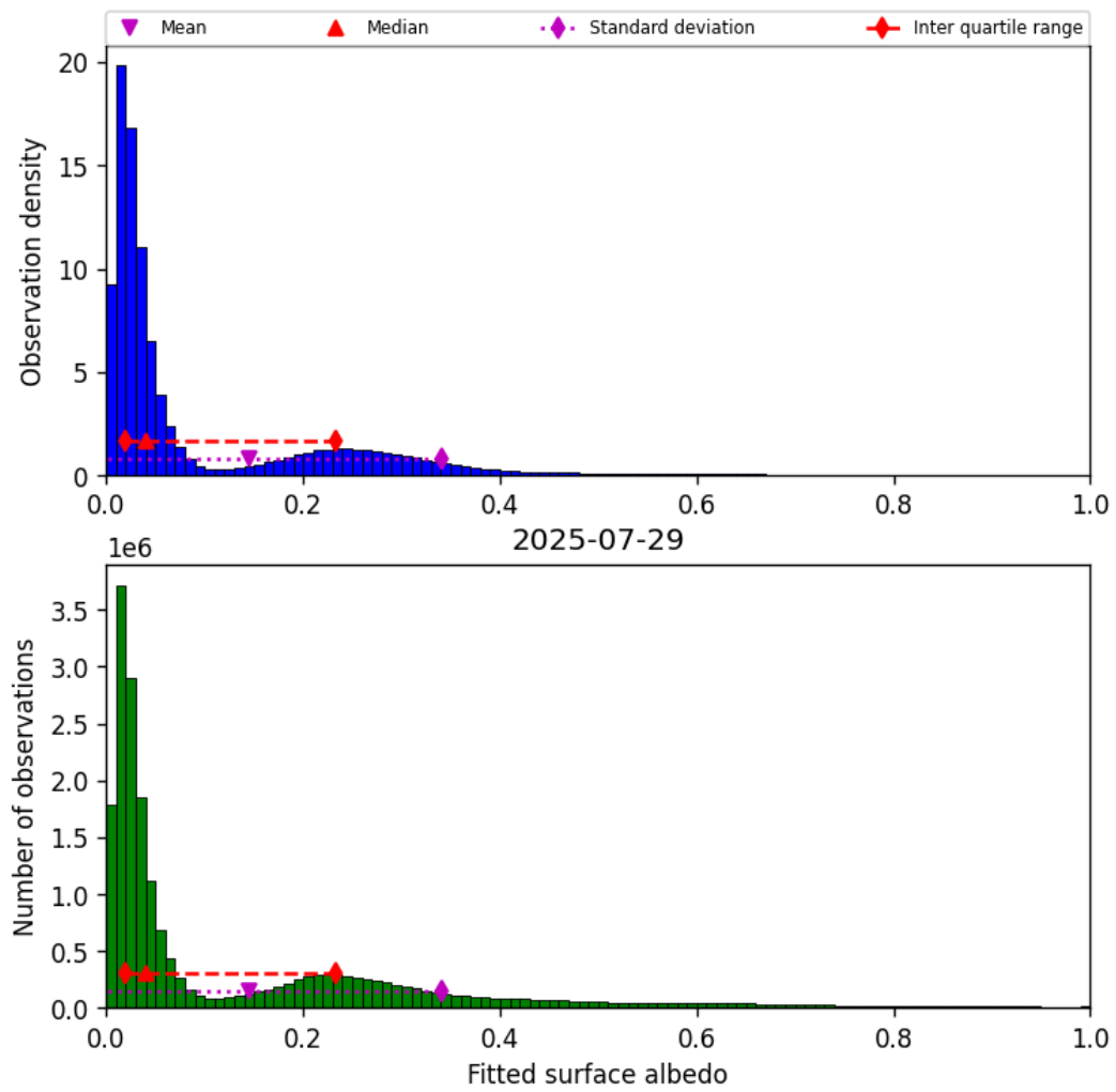
Figure 45: Histogram of “Fitted surface albedo” for 2025-07-29 to 2025-07-30
