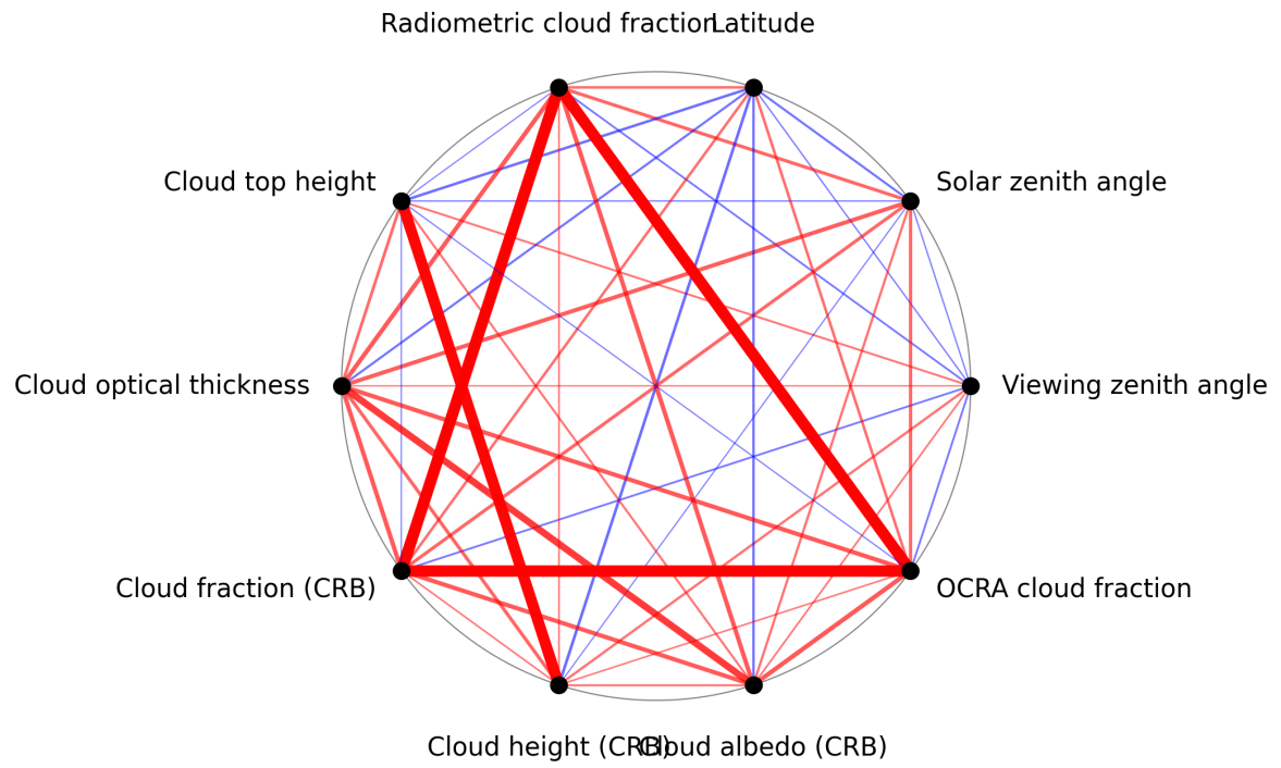
Figure 1: Map of correlation graph for 2025-07-29 to 2025-07-30.
