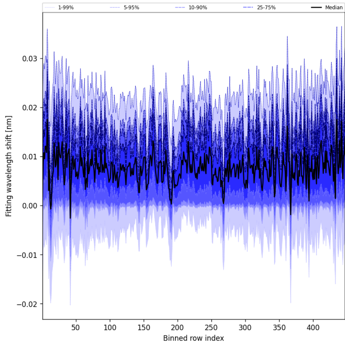
Figure 65: Along track statistics of “Fitting wavelength shift” for 2025-07-29 to 2025-07-30
