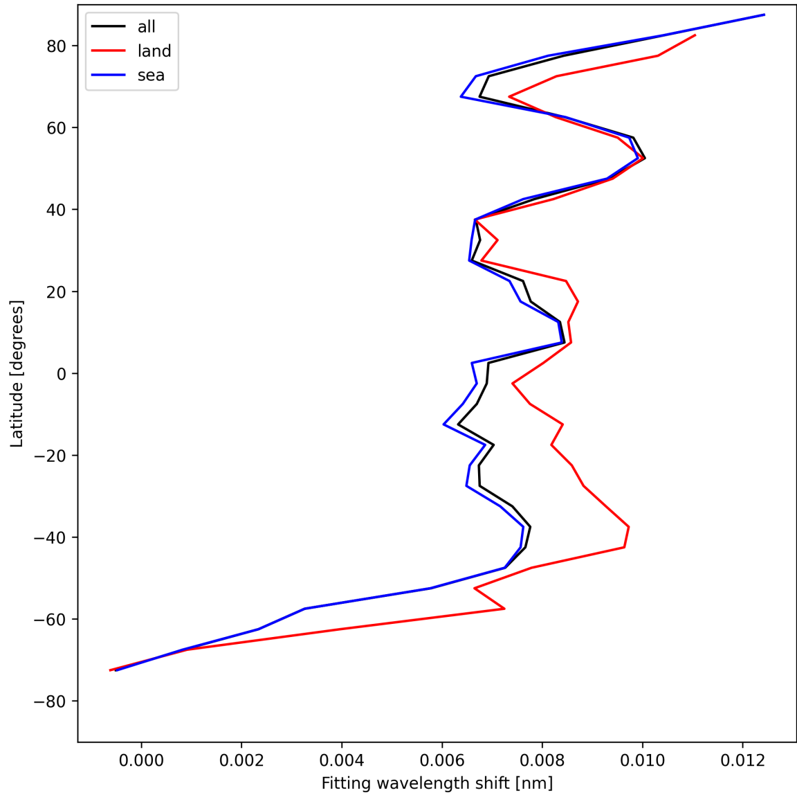
Figure 33: Zonal average of “Fitting wavelength shift” for 2025-07-29 to 2025-07-30.
