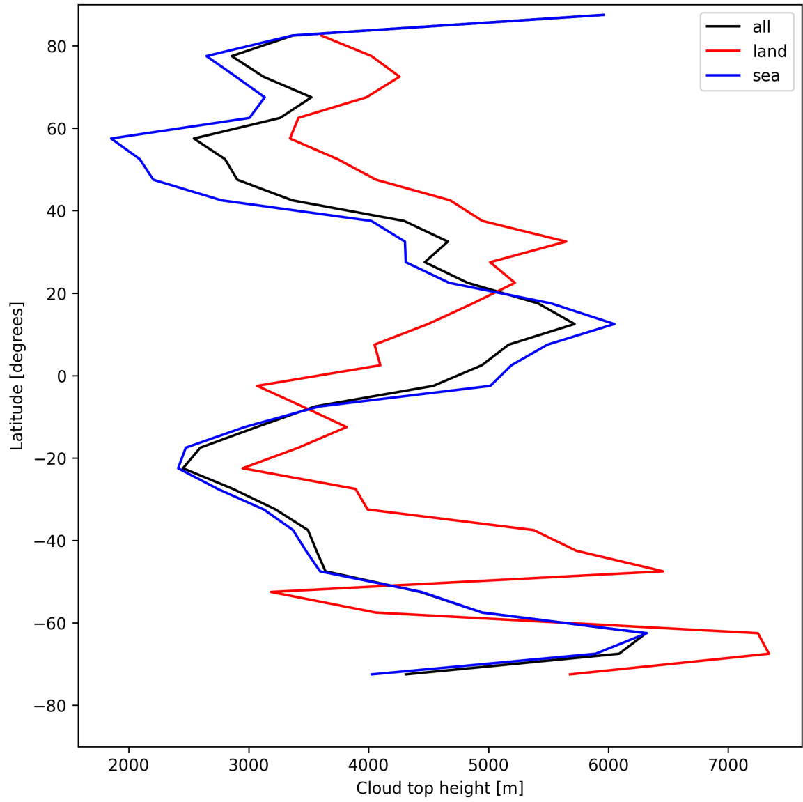
Figure 24: Zonal average of “Cloud top height” for 2025-07-29 to 2025-07-30.
