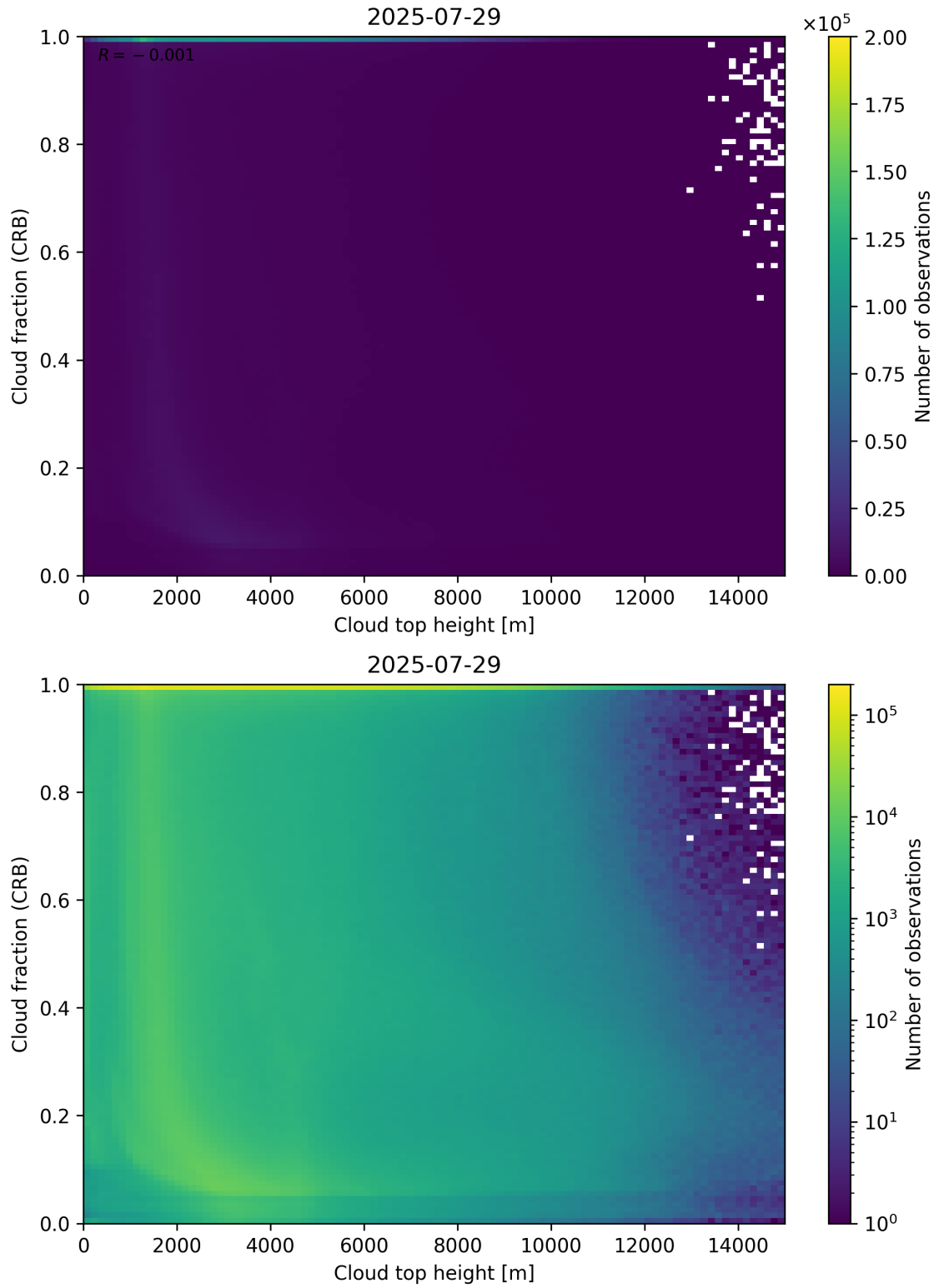
Figure 88: Scatter density plot of “Cloud top height” against “Cloud fraction (CRB)” for 2025-07-29 to 2025-07-30.
