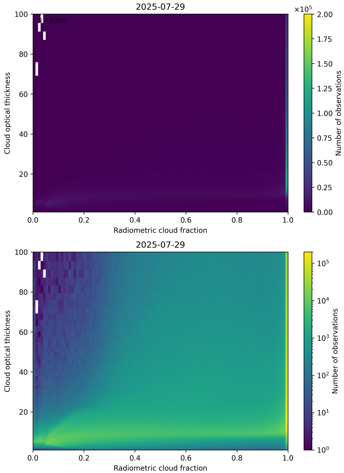
Figure 75: Scatter density plot of “Radiometric cloud fraction” against “Cloud optical thickness” for 2025-07-29 to 2025-07-30.
