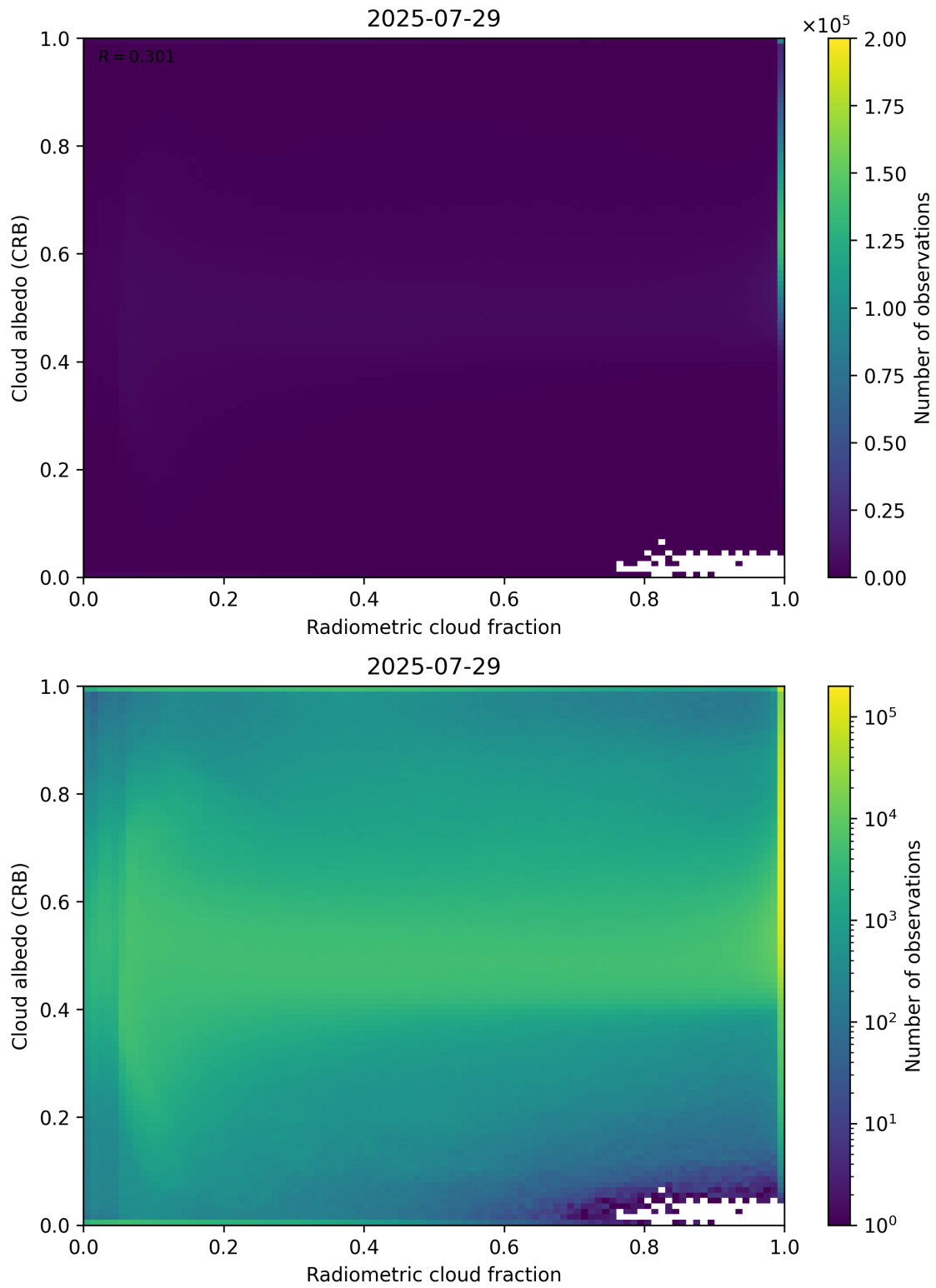
Figure 71: Scatter density plot of “Radiometric cloud fraction” against “Cloud albedo (CRB)” for 2025-07-29 to 2025-07-30.
