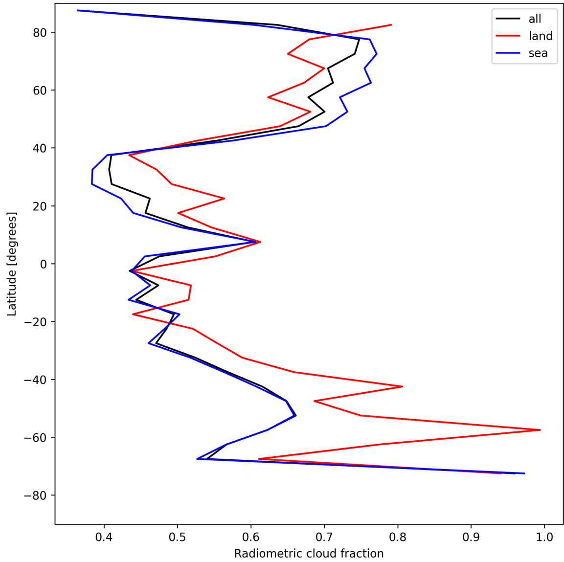
Figure 23: Zonal average of “Radiometric cloud fraction” for 2025-07-29 to 2025-07-30.
