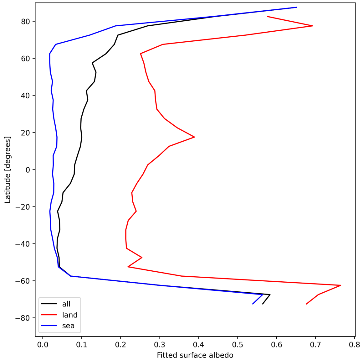
Figure 29: Zonal average of “Fitted surface albedo” for 2025-07-29 to 2025-07-30.
