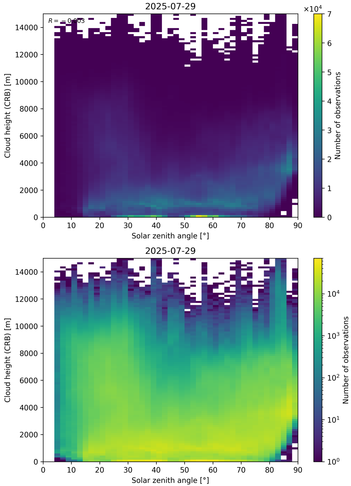
Figure 102: Scatter density plot of “Solar zenith angle” against “Cloud height (CRB)” for 2025-07-29 to 2025-07-30.
