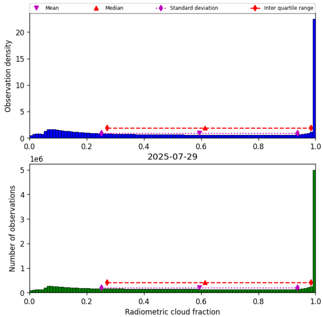
Figure 39: Histogram of “Radiometric cloud fraction” for 2025-07-29 to 2025-07-30
