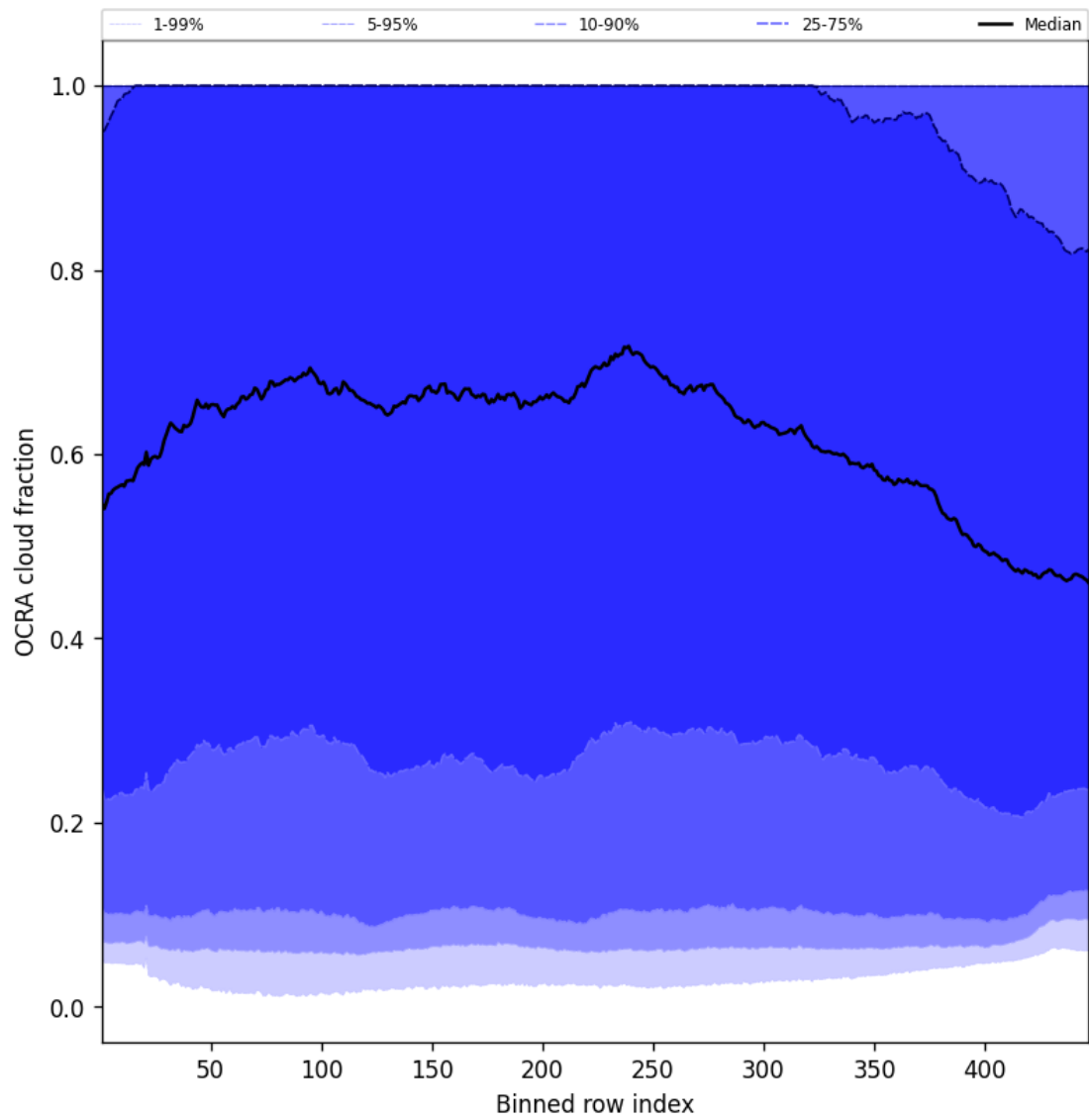
Figure 66: Along track statistics of “OCRA cloud fraction” for 2025-07-29 to 2025-07-30
