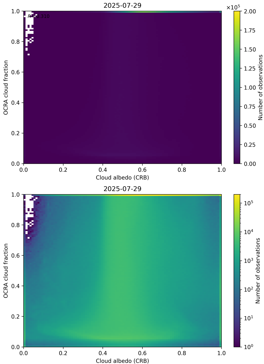
Figure 70: Scatter density plot of “Cloud albedo (CRB)” against “OCRA cloud fraction” for 2025-07-29 to 2025-07-30.
