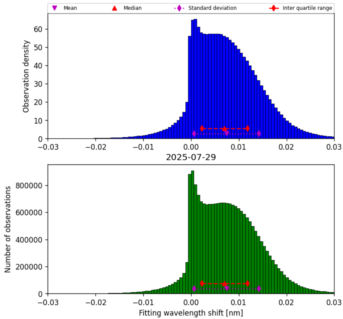
Figure 49: Histogram of “Fitting wavelength shift” for 2025-07-29 to 2025-07-30
