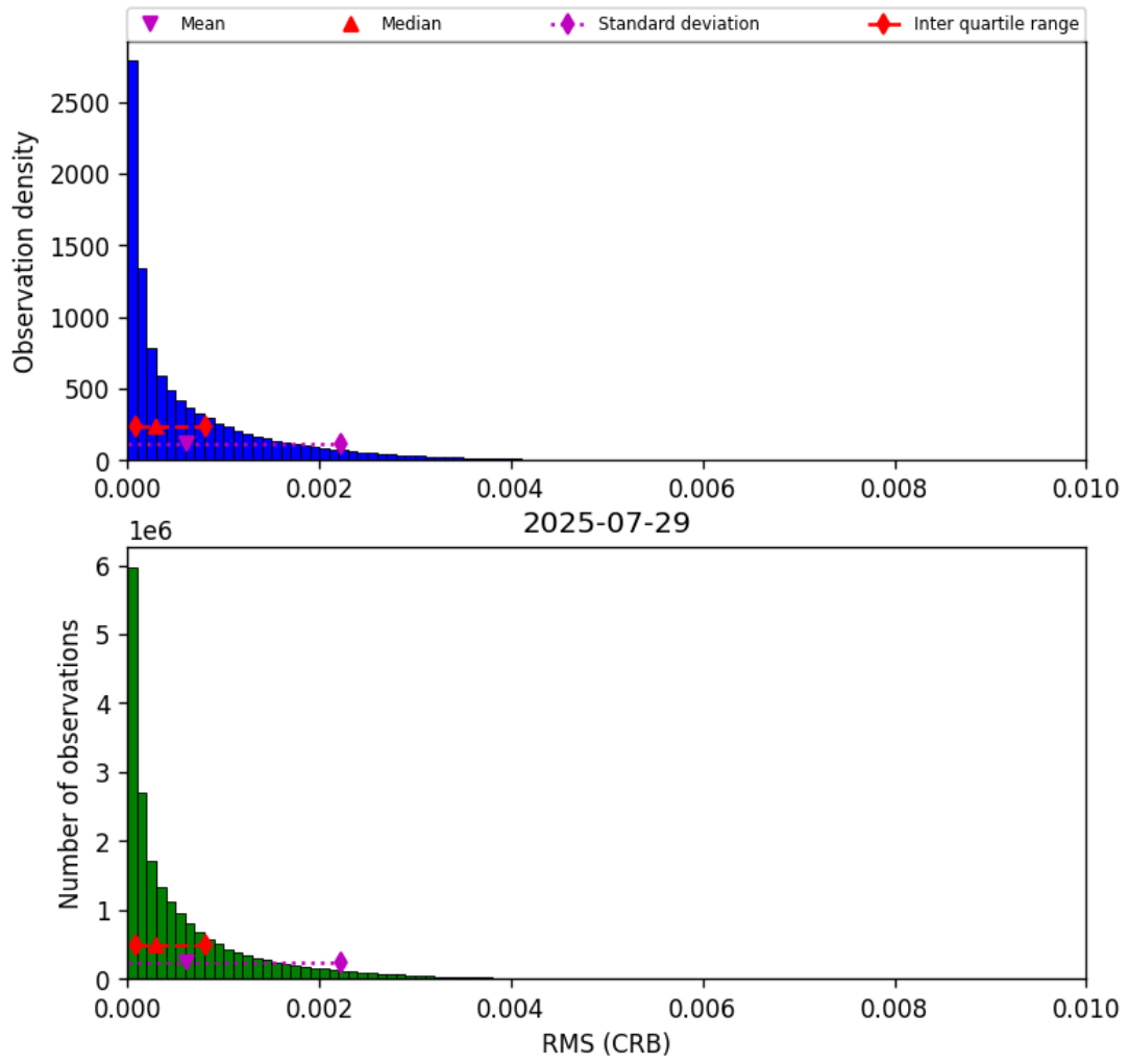
Figure 48: Histogram of “RMS (CRB)” for 2025-07-29 to 2025-07-30
