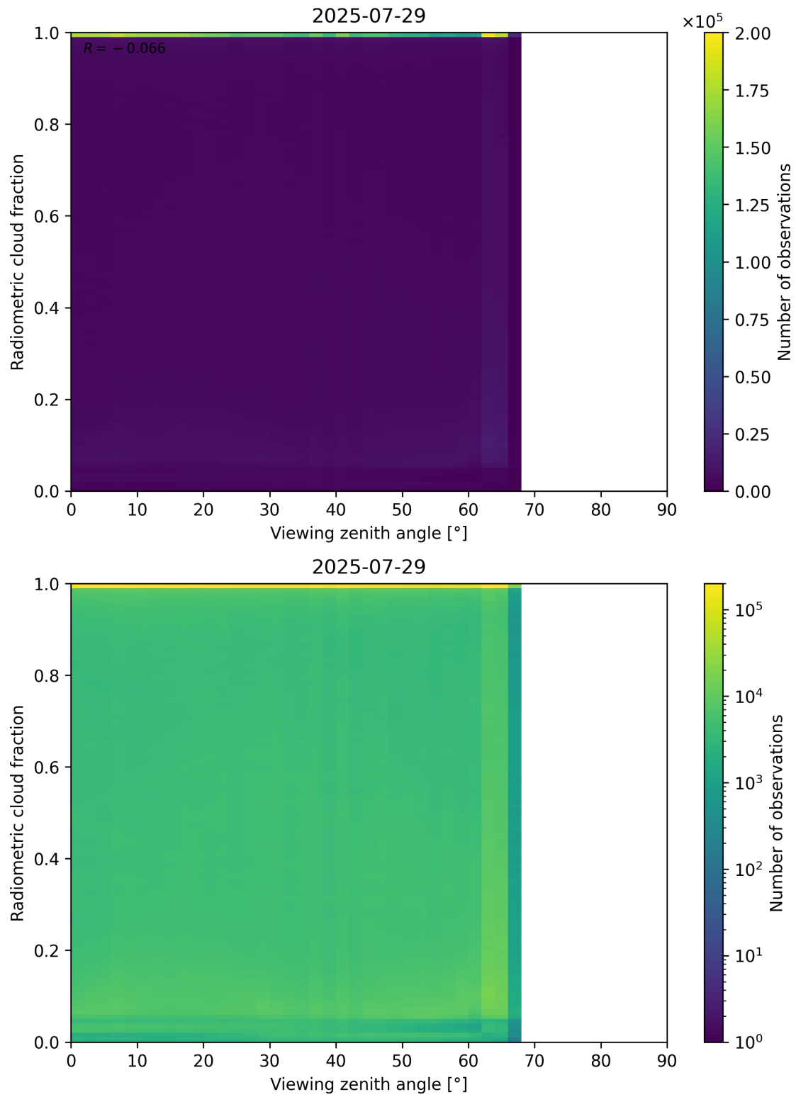
Figure 107: Scatter density plot of “Viewing zenith angle” against “Radiometric cloud fraction” for 2025-07-29 to 2025-07-30.
