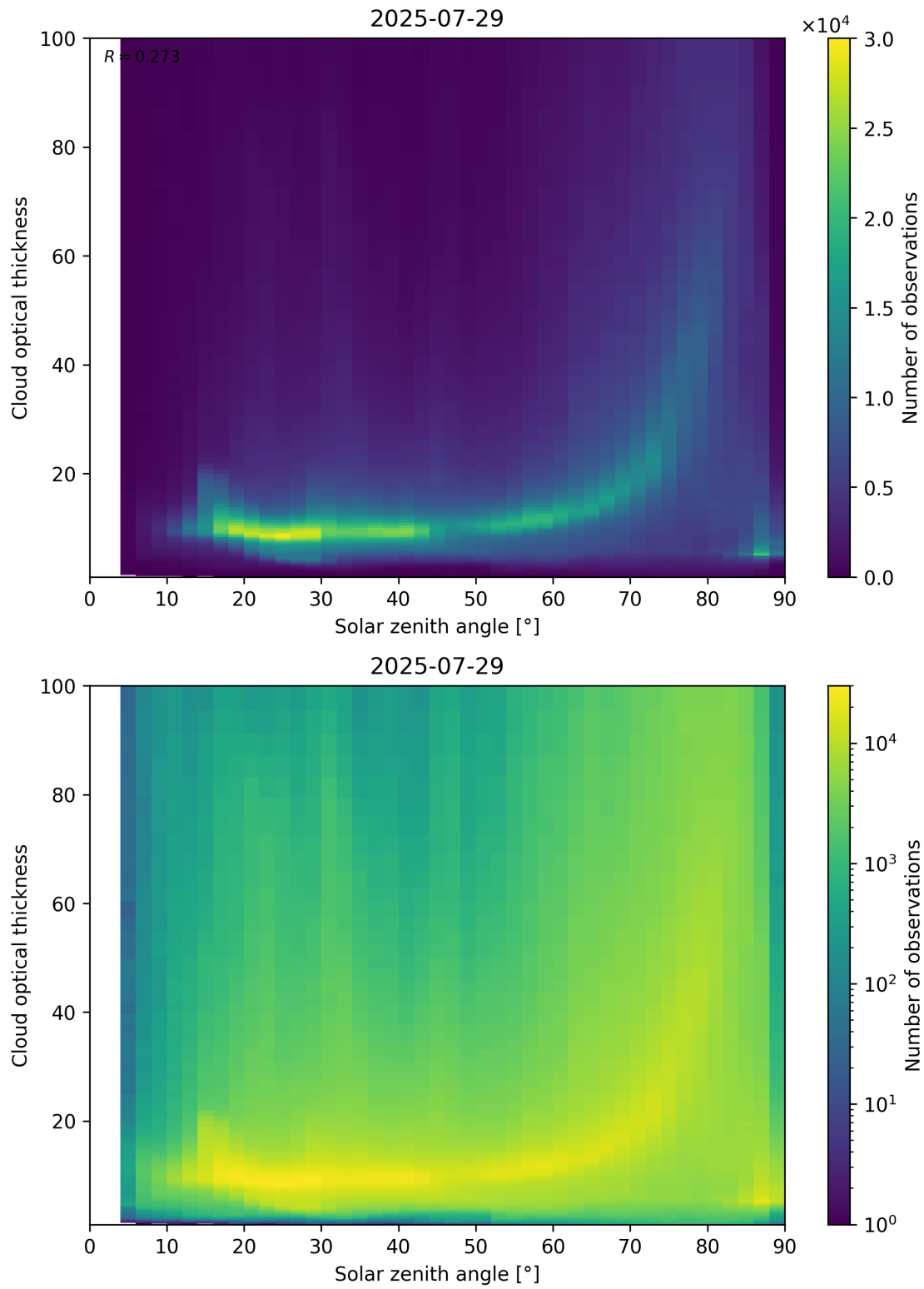
Figure 103: Scatter density plot of “Solar zenith angle” against “Cloud optical thickness” for 2025-07-29 to 2025-07-30.
