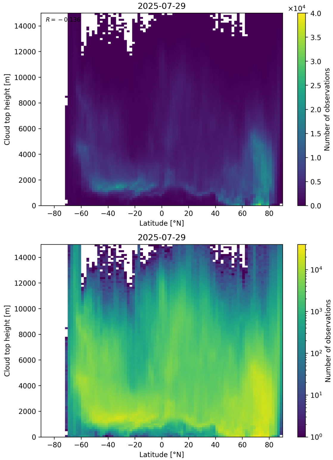
Figure 97: Scatter density plot of “Latitude” against “Cloud top height” for 2025-07-29 to 2025-07-30.
