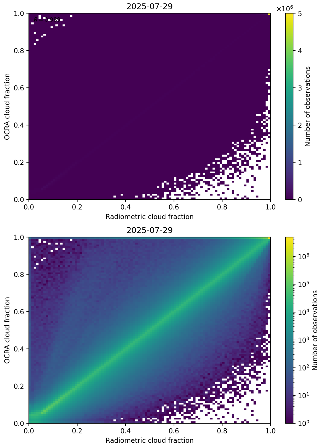
Figure 72: Scatter density plot of “Radiometric cloud fraction” against “OCRA cloud fraction” for 2025-07-29 to 2025-07-30.
