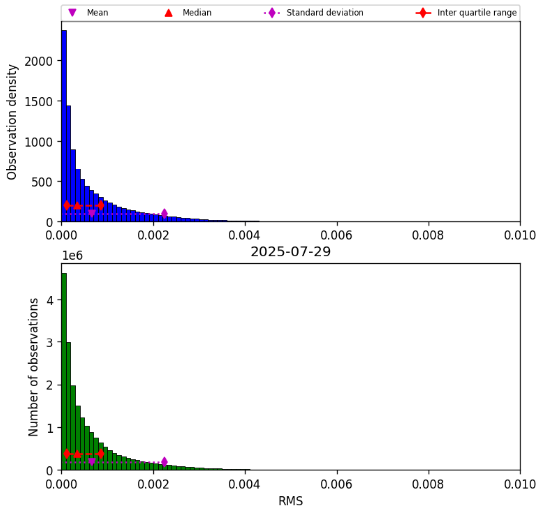
Figure 47: Histogram of “RMS” for 2025-07-29 to 2025-07-30
