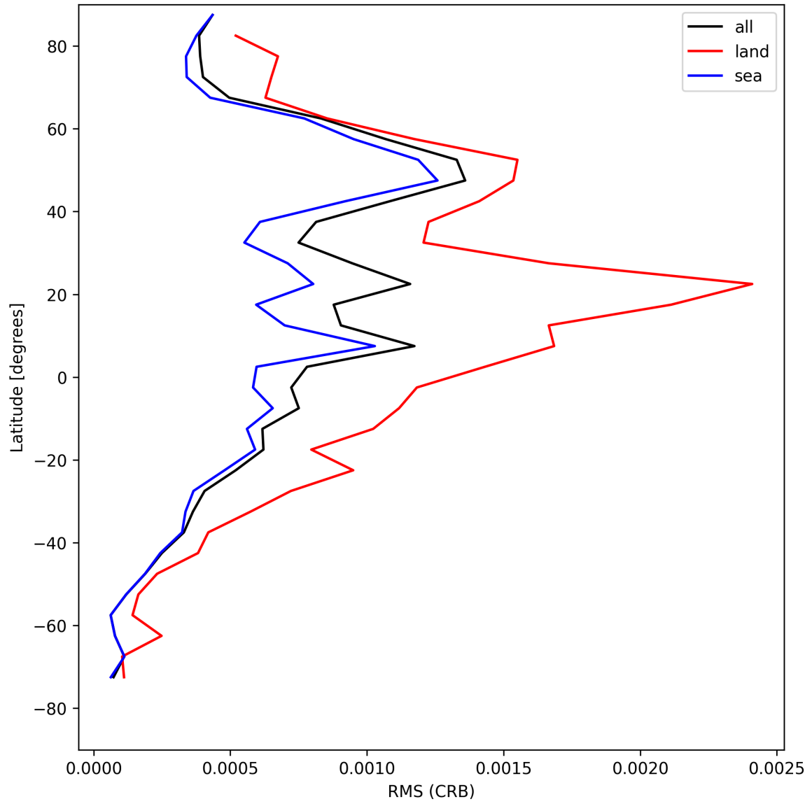
Figure 32: Zonal average of “RMS (CRB)” for 2025-07-29 to 2025-07-30.
