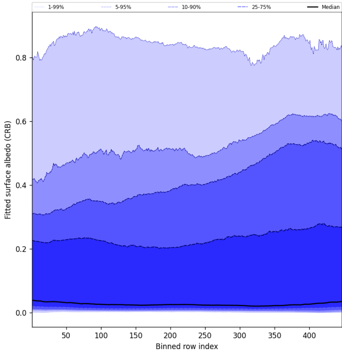
Figure 62: Along track statistics of “Fitted surface albedo (CRB)” for 2025-07-29 to 2025-07-30
