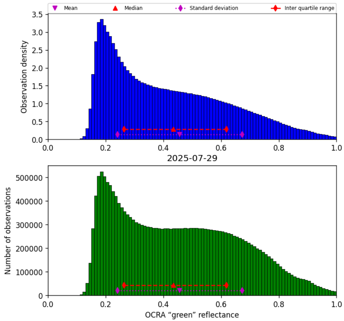
Figure 52: Histogram of “OCRA “green” reflectance” for 2025-07-29 to 2025-07-30
