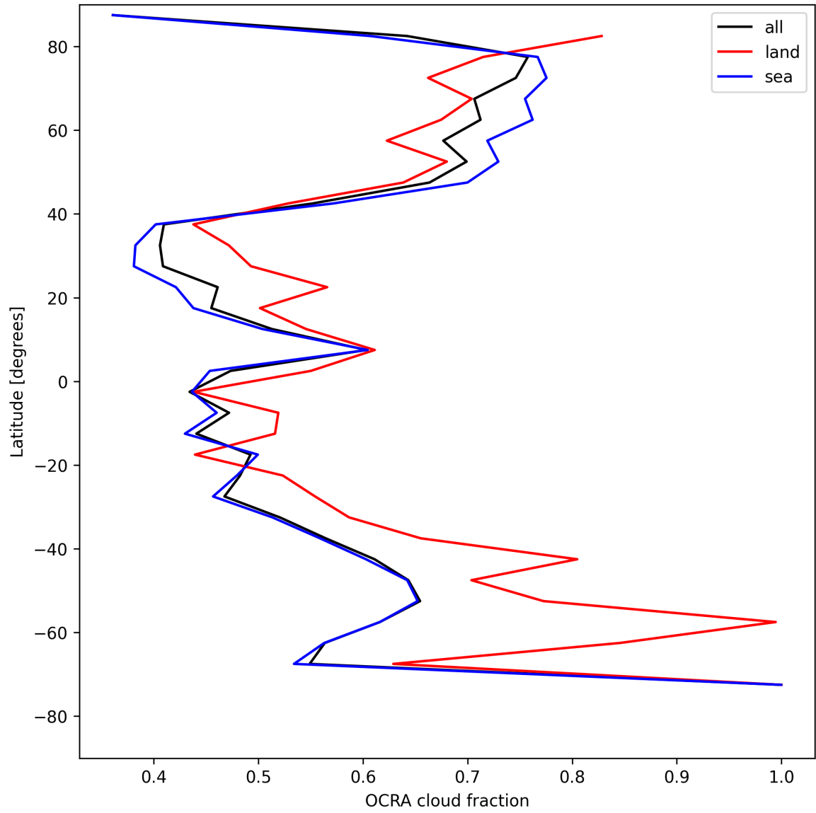
Figure 34: Zonal average of “OCRA cloud fraction” for 2025-07-29 to 2025-07-30.
