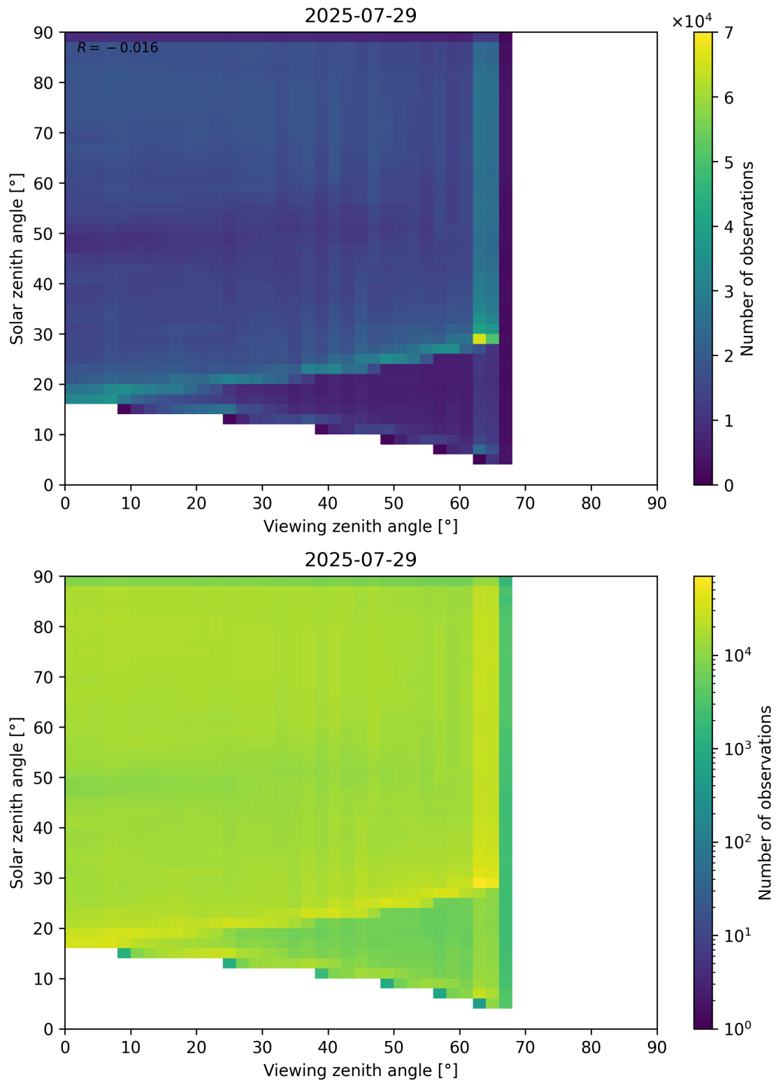
Figure 114: Scatter density plot of “Viewing zenith angle” against “Solar zenith angle” for 2025-07-29 to 2025-07-30.
