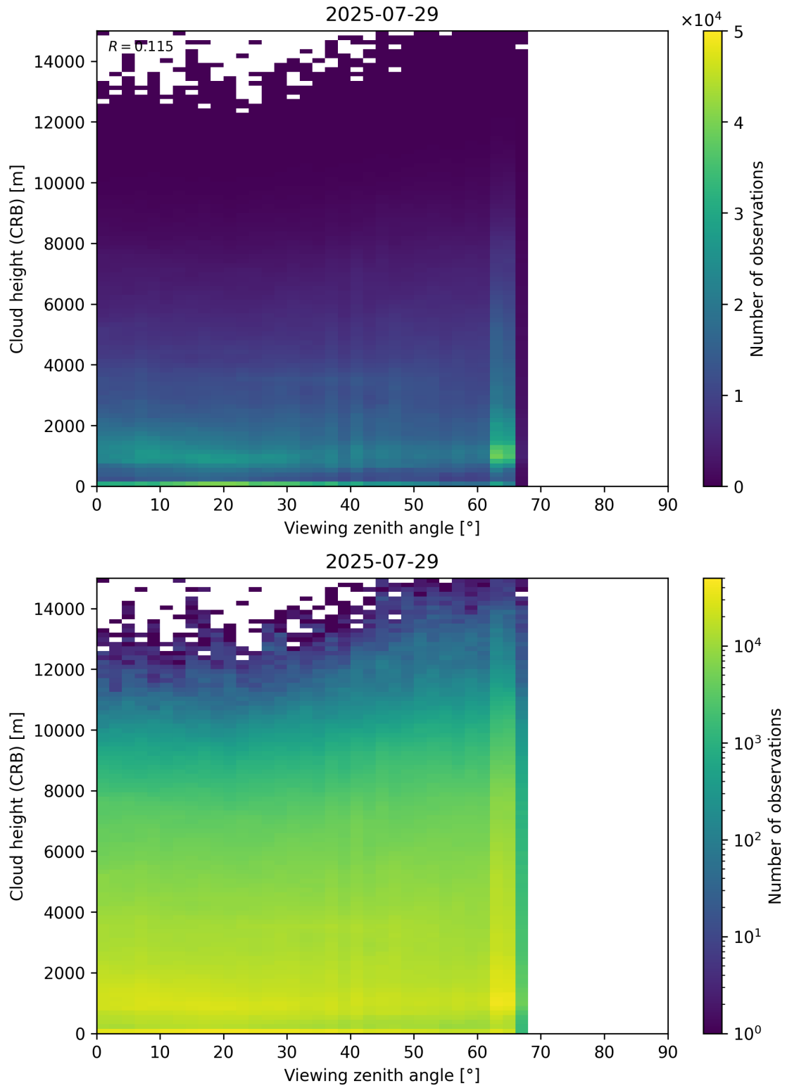
Figure 110: Scatter density plot of “Viewing zenith angle” against “Cloud height (CRB)” for 2025-07-29 to 2025-07-30.
