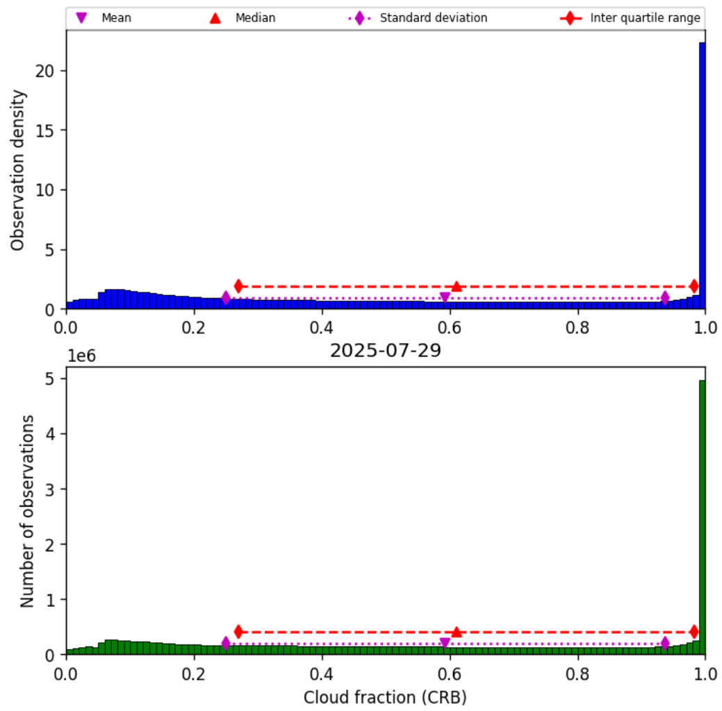
Figure 42: Histogram of “Cloud fraction (CRB)” for 2025-07-29 to 2025-07-30
