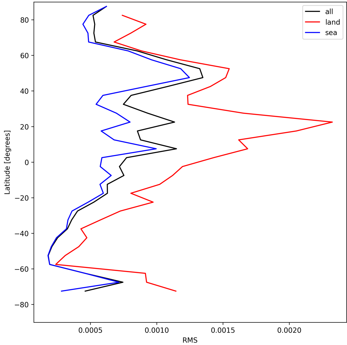
Figure 31: Zonal average of “RMS” for 2025-07-29 to 2025-07-30.
