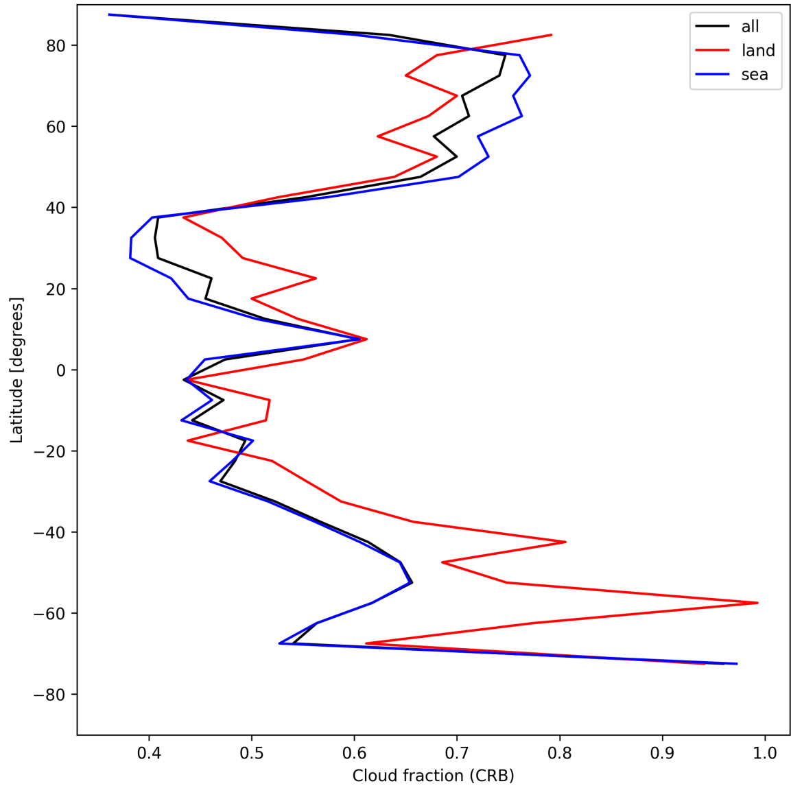
Figure 26: Zonal average of “Cloud fraction (CRB)” for 2025-07-29 to 2025-07-30.
