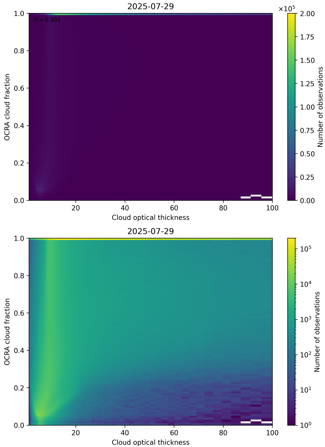
Figure 83: Scatter density plot of “Cloud optical thickness” against “OCRA cloud fraction” for 2025-07-29 to 2025-07-30.
