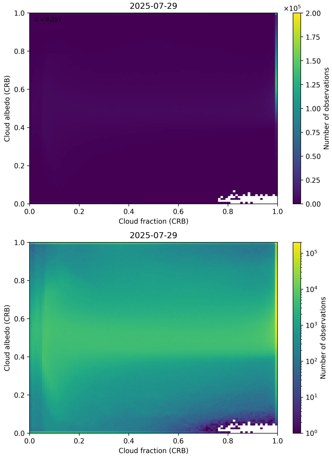
Figure 77: Scatter density plot of “Cloud fraction (CRB)” against “Cloud albedo (CRB)” for 2025-07-29 to 2025-07-30.
