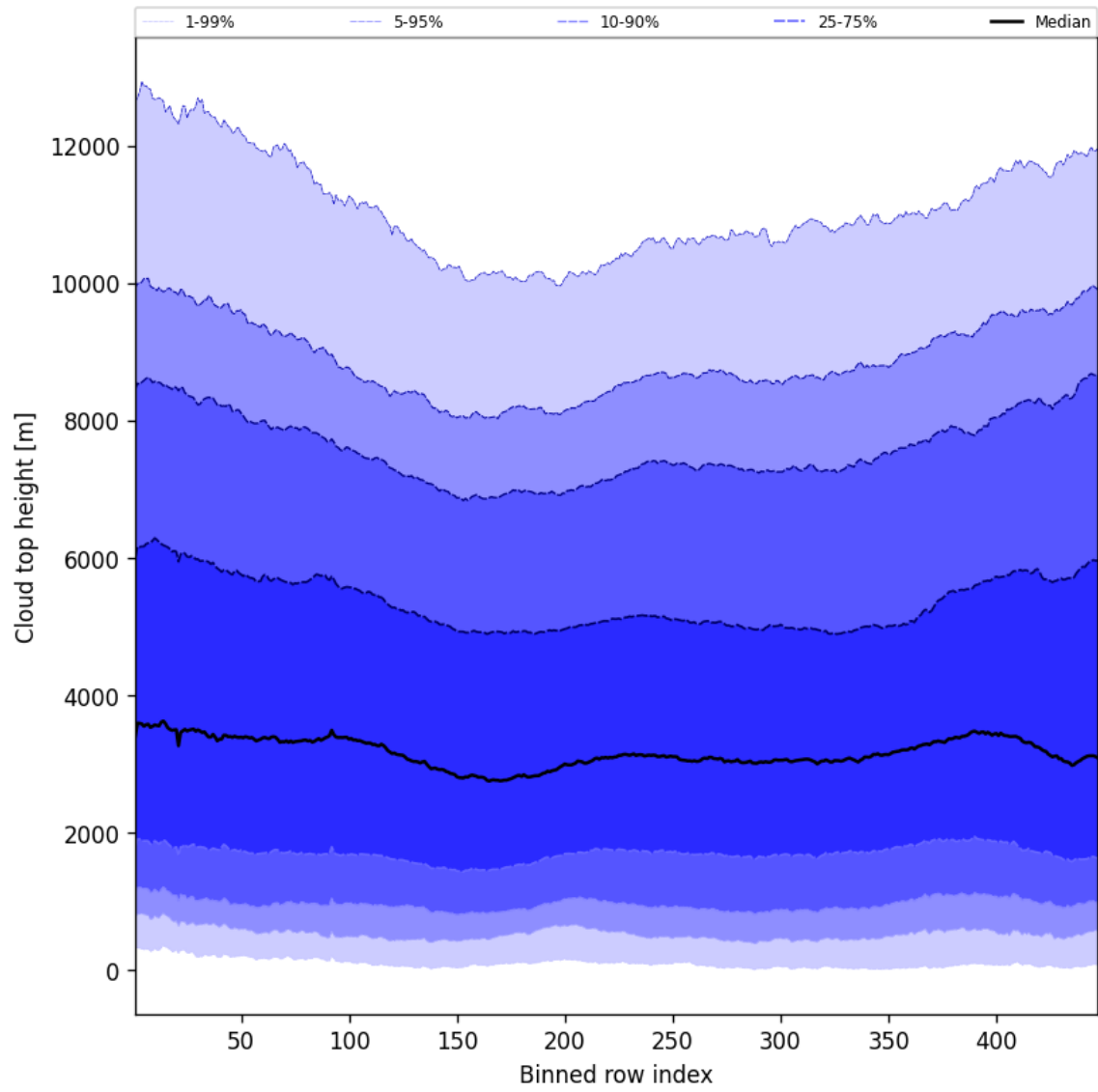
Figure 56: Along track statistics of “Cloud top height” for 2025-07-29 to 2025-07-30
