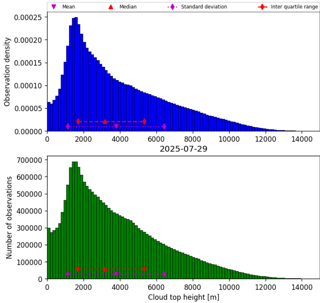
Figure 40: Histogram of “Cloud top height” for 2025-07-29 to 2025-07-30
