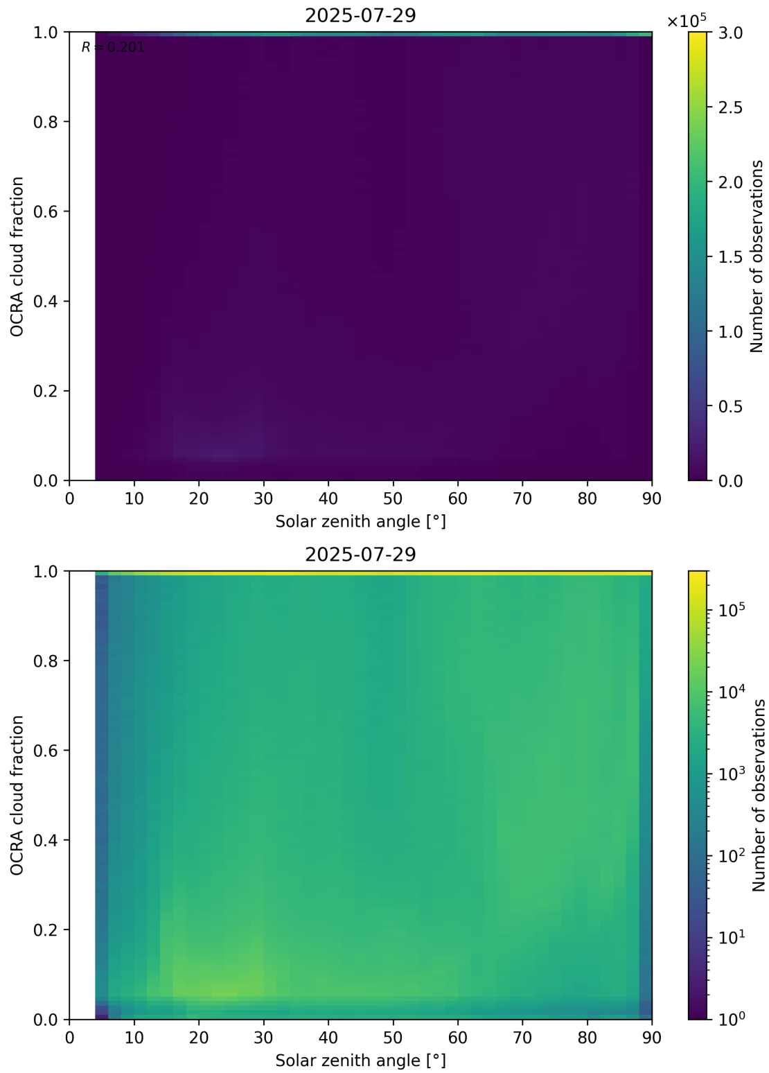
Figure 100: Scatter density plot of “Solar zenith angle” against “OCRA cloud fraction” for 2025-07-29 to 2025-07-30.
