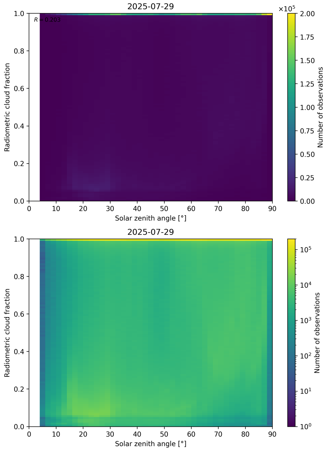
Figure 99: Scatter density plot of “Solar zenith angle” against “Radiometric cloud fraction” for 2025-07-29 to 2025-07-30.
