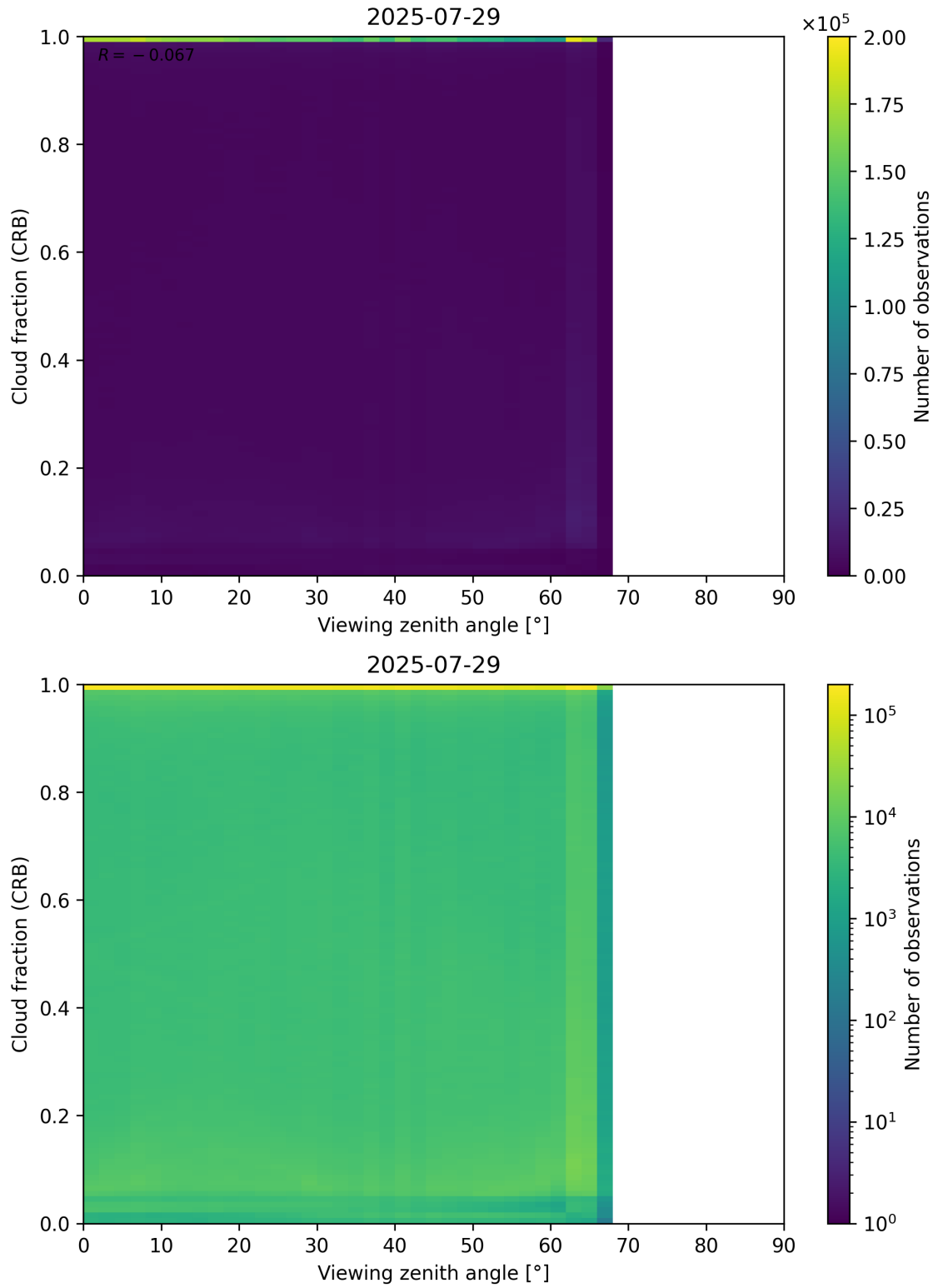
Figure 109: Scatter density plot of “Viewing zenith angle” against “Cloud fraction (CRB)” for 2025-07-29 to 2025-07-30.
