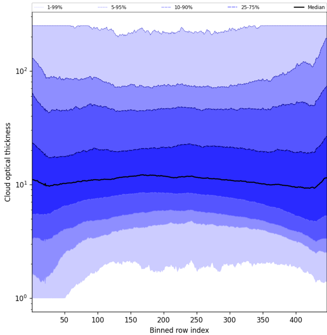
Figure 57: Along track statistics of “Cloud optical thickness” for 2025-07-29 to 2025-07-30
