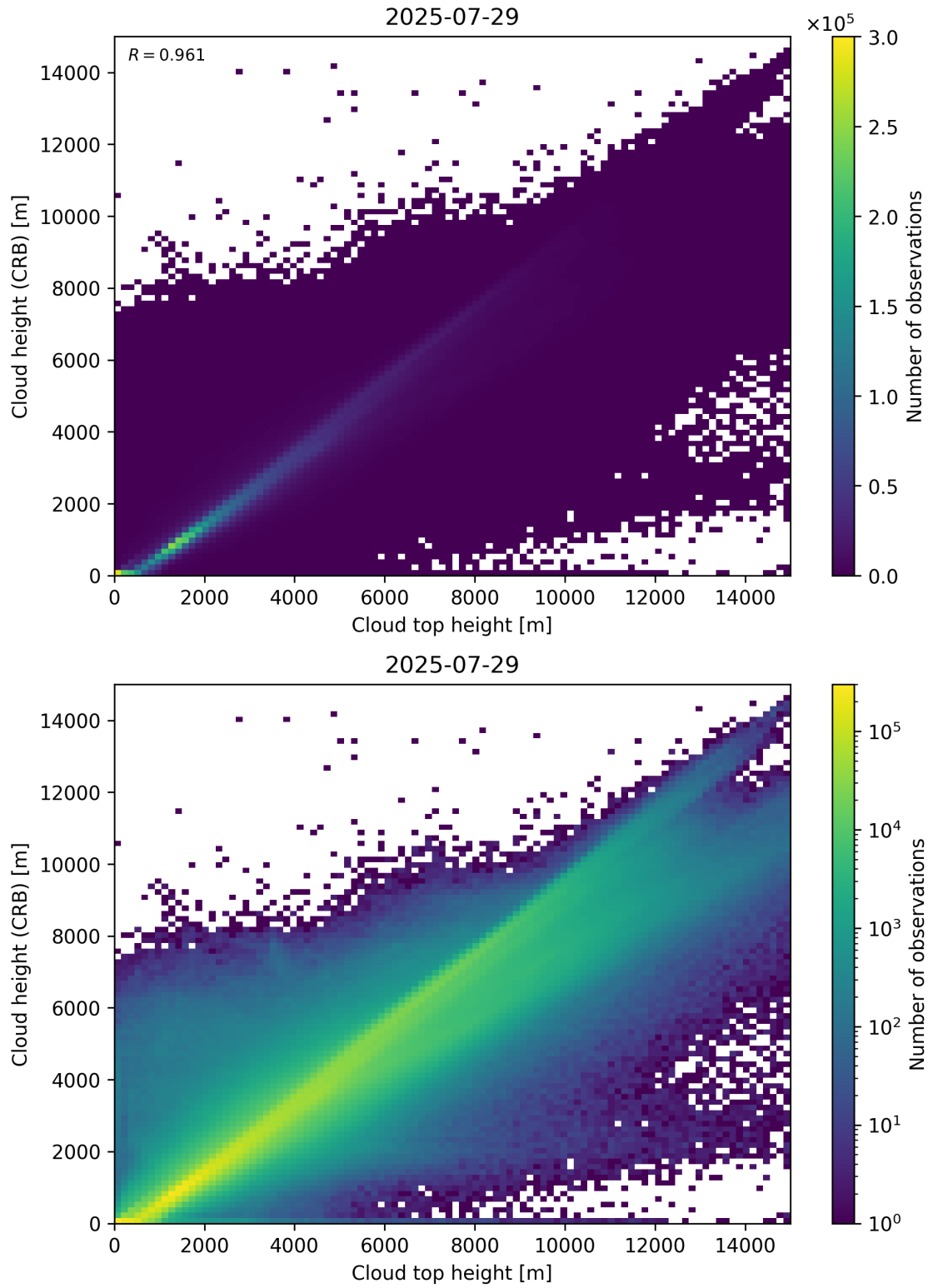
Figure 89: Scatter density plot of “Cloud top height” against “Cloud height (CRB)” for 2025-07-29 to 2025-07-30.
