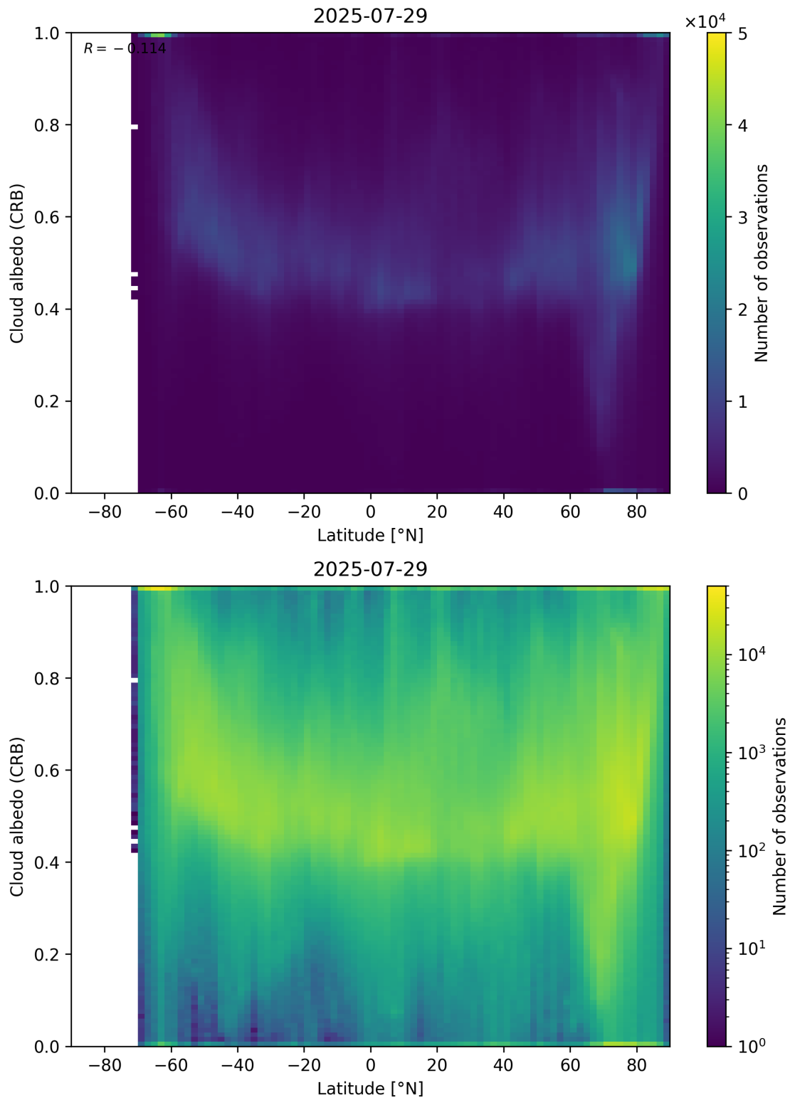
Figure 91: Scatter density plot of “Latitude” against “Cloud albedo (CRB)” for 2025-07-29 to 2025-07-30.
