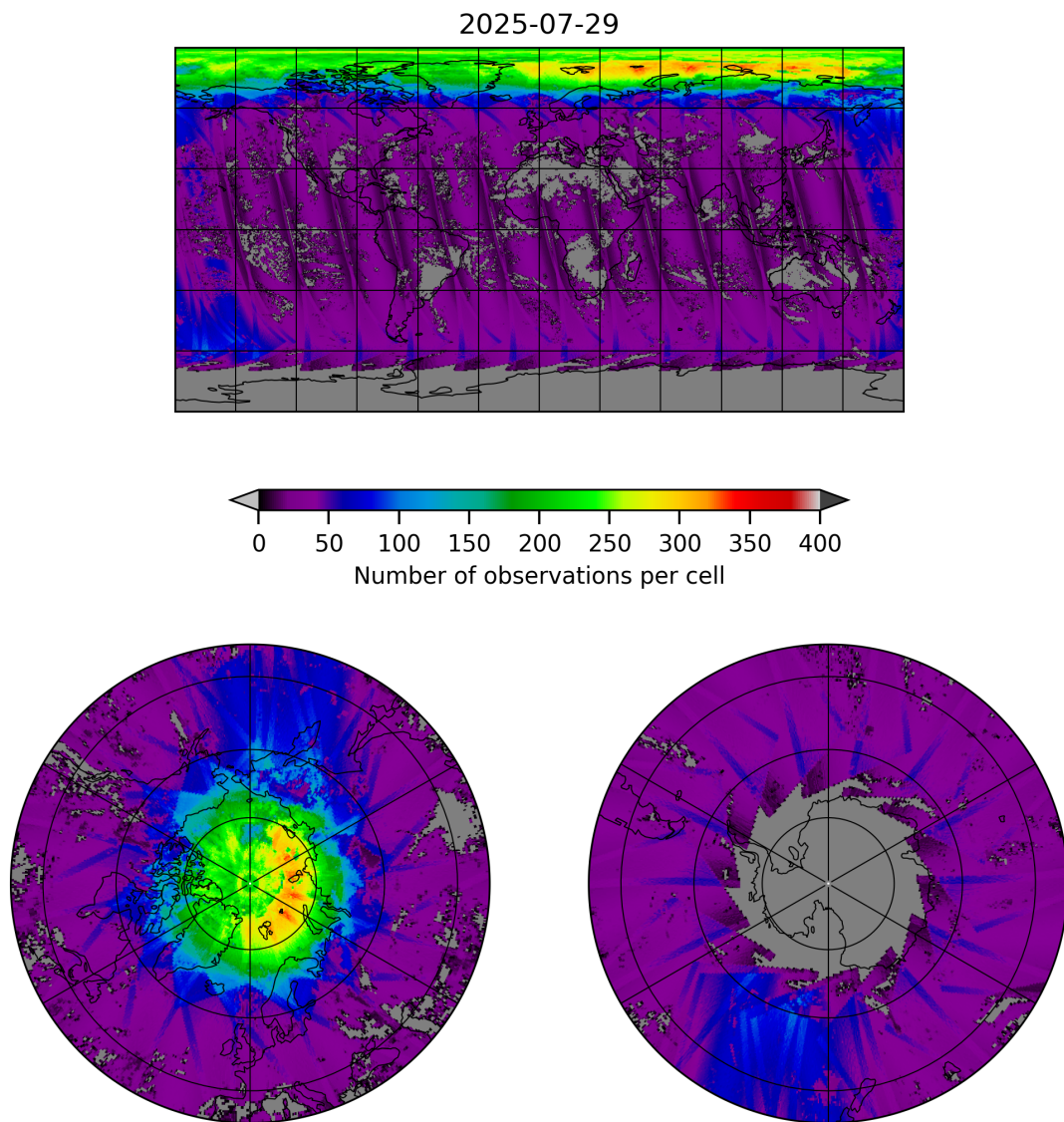
Figure 21: Map of the number of observations for 2025-07-29 to 2025-07-30
