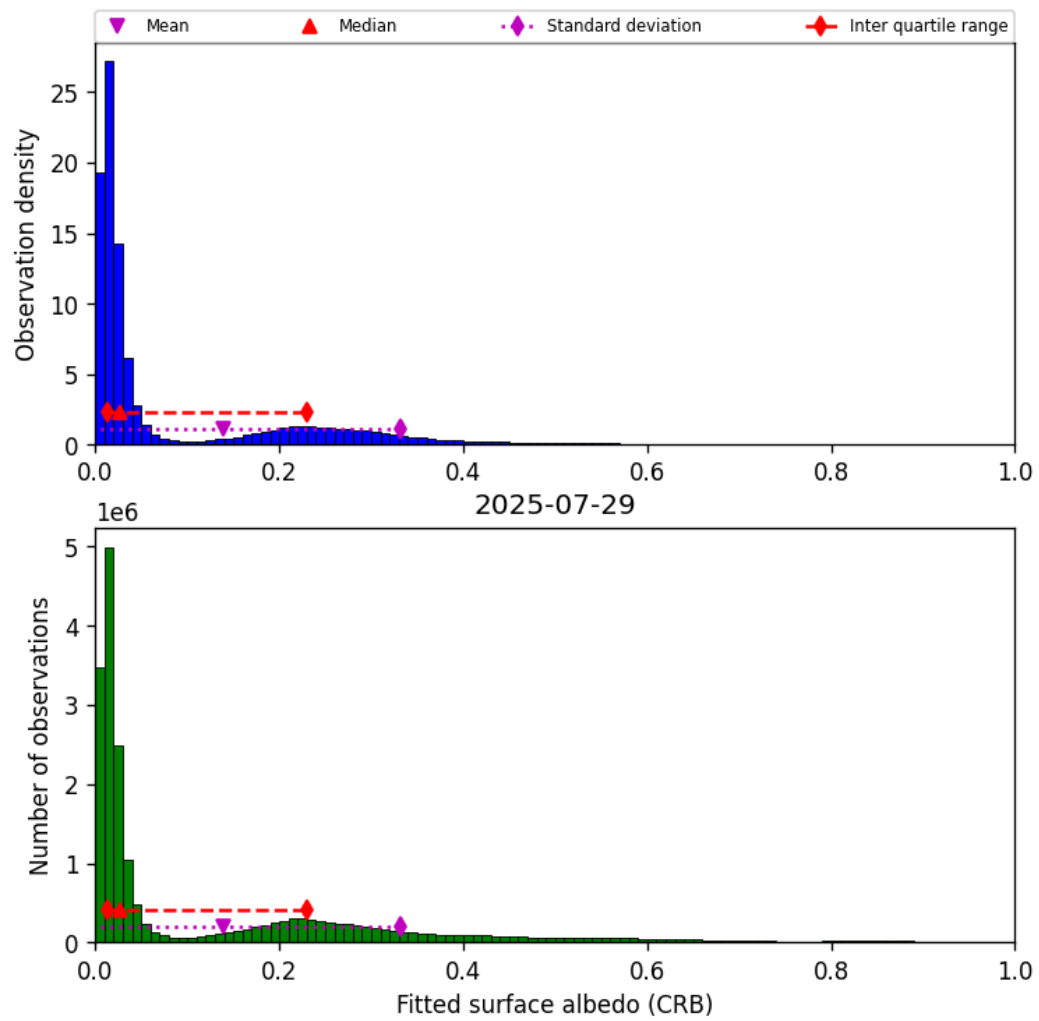
Figure 46: Histogram of “Fitted surface albedo (CRB)” for 2025-07-29 to 2025-07-30
