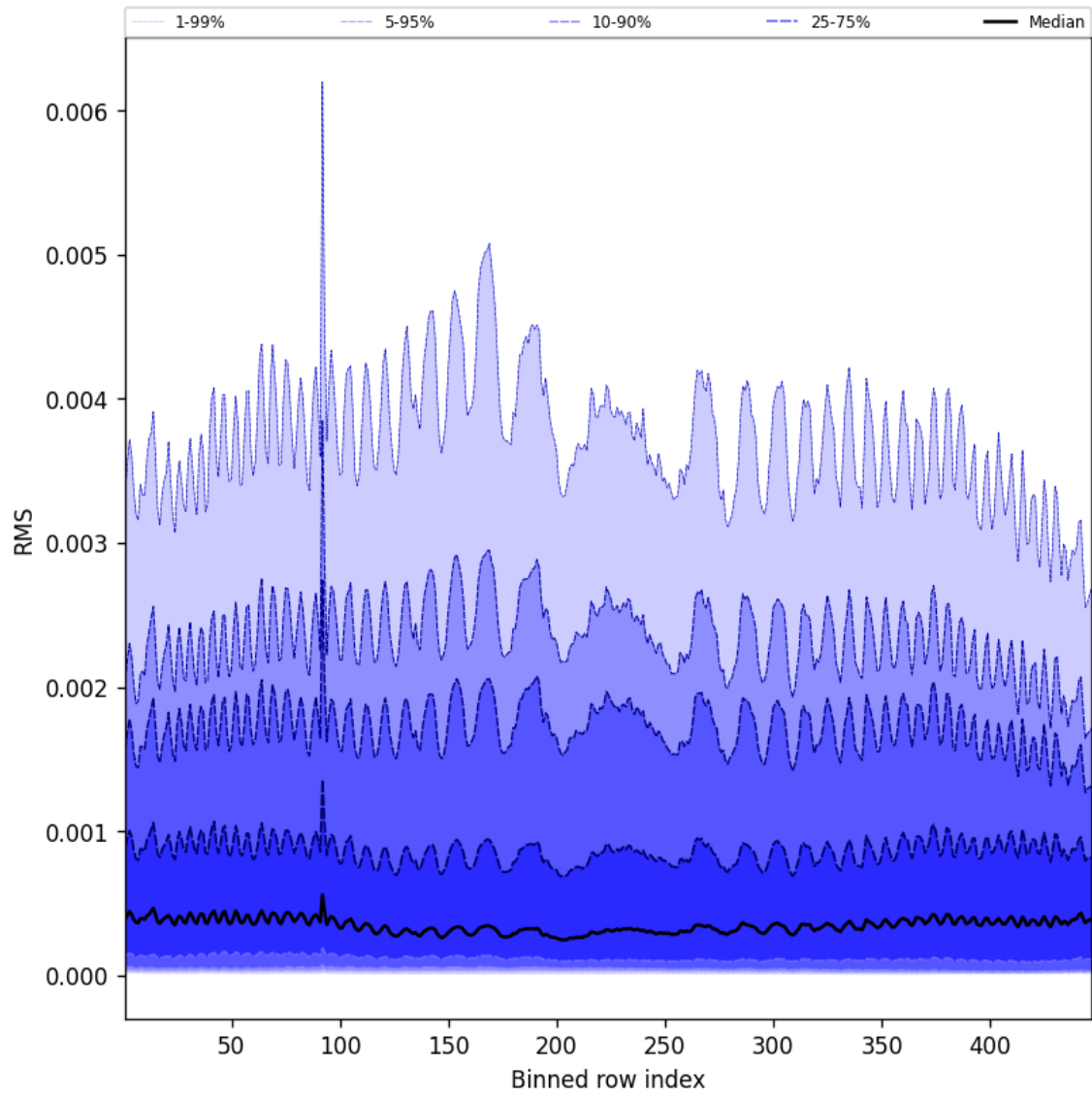
Figure 63: Along track statistics of “RMS” for 2025-07-29 to 2025-07-30
