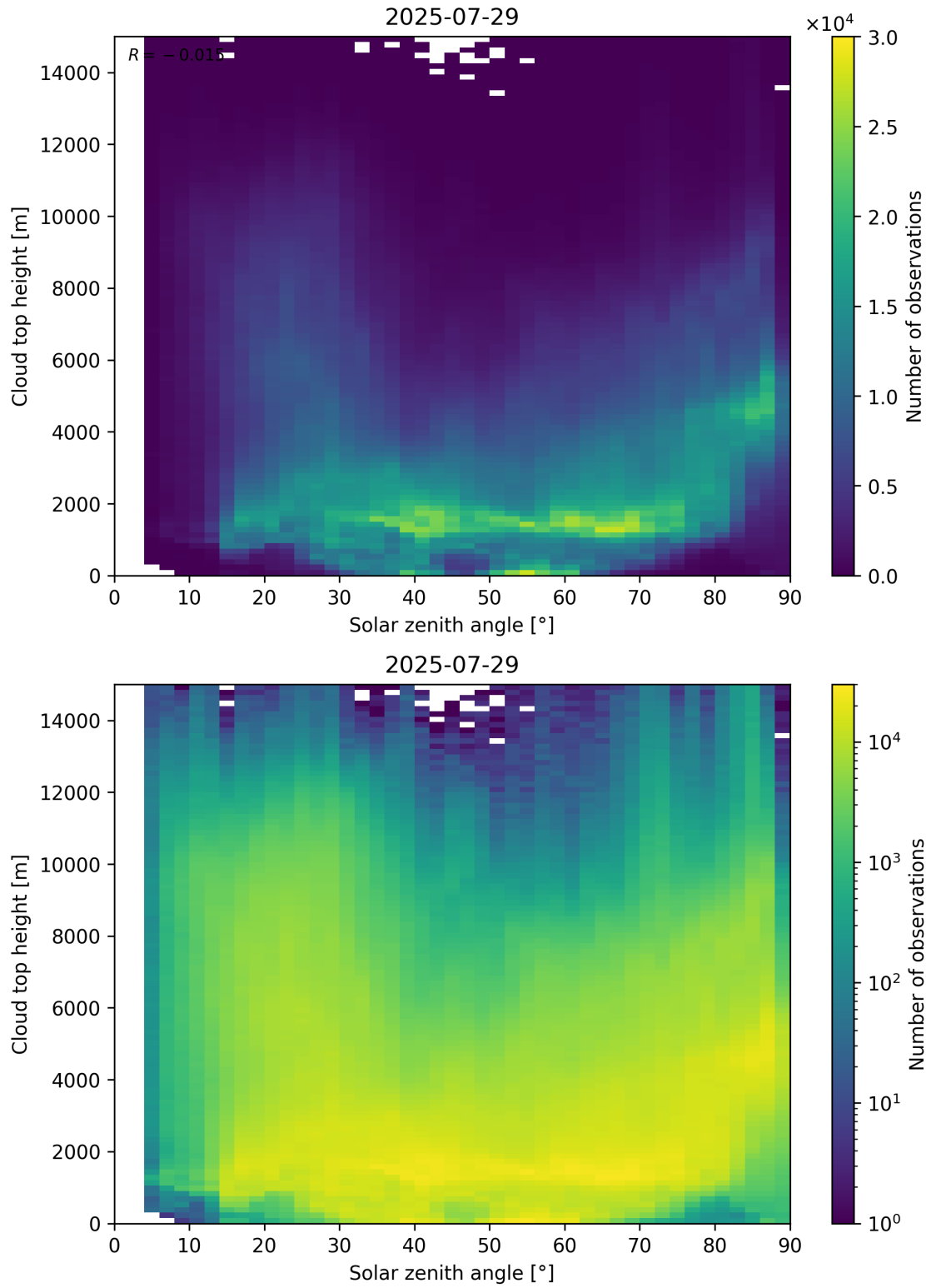
Figure 104: Scatter density plot of “Solar zenith angle” against “Cloud top height” for 2025-07-29 to 2025-07-30.
