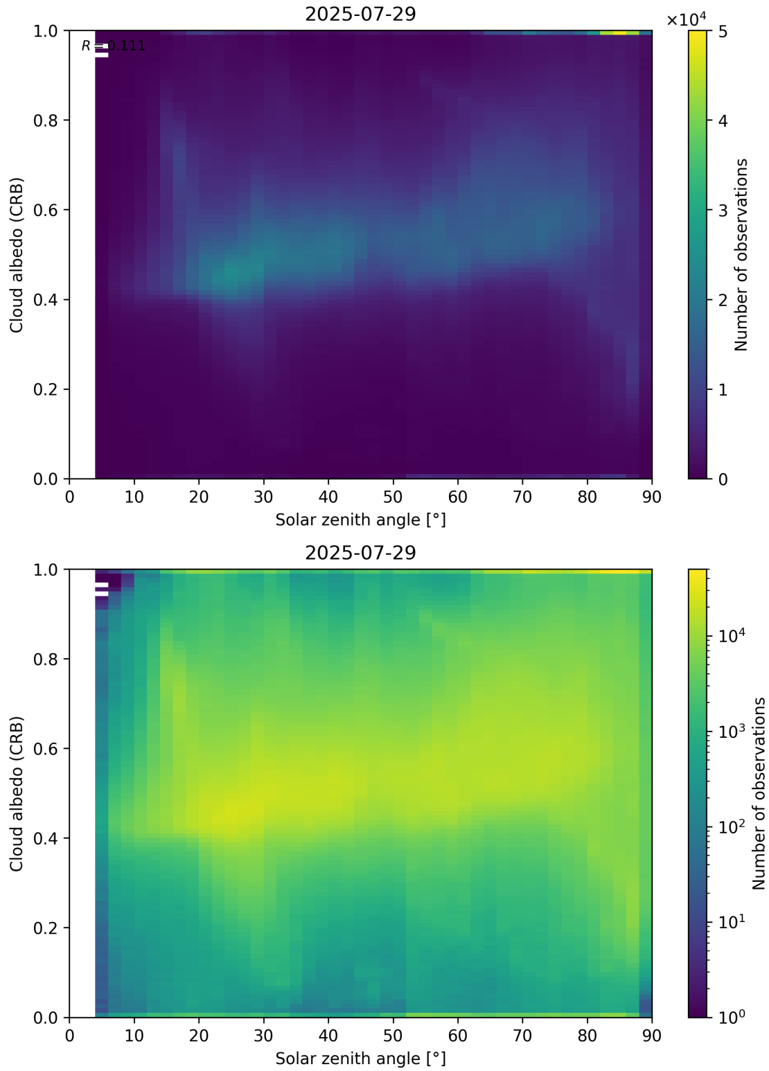
Figure 98: Scatter density plot of “Solar zenith angle” against “Cloud albedo (CRB)” for 2025-07-29 to 2025-07-30.
