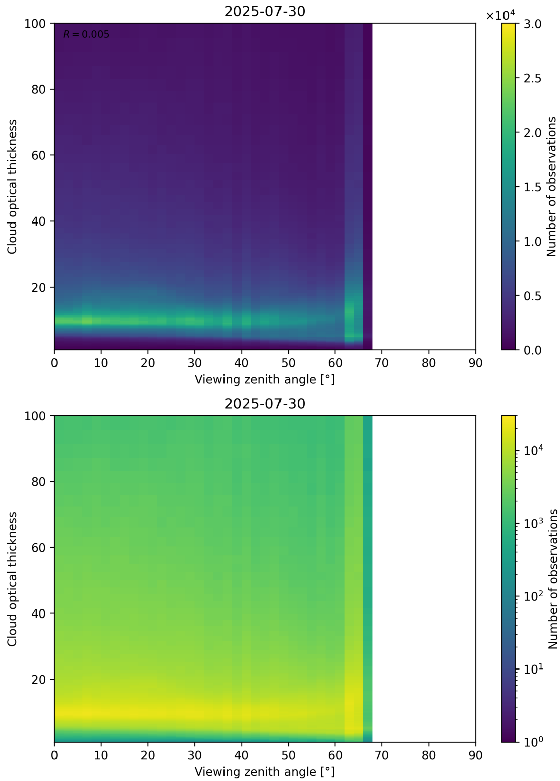
Figure 111: Scatter density plot of “Viewing zenith angle” against “Cloud optical thickness” for 2025-07-29 to 2025-07-31.
