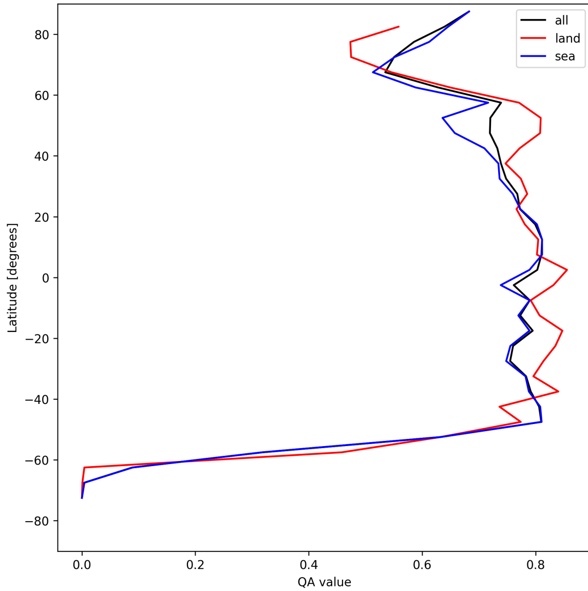
Figure 22: Zonal average of “QA value” for 2025-07-29 to 2025-07-31.
