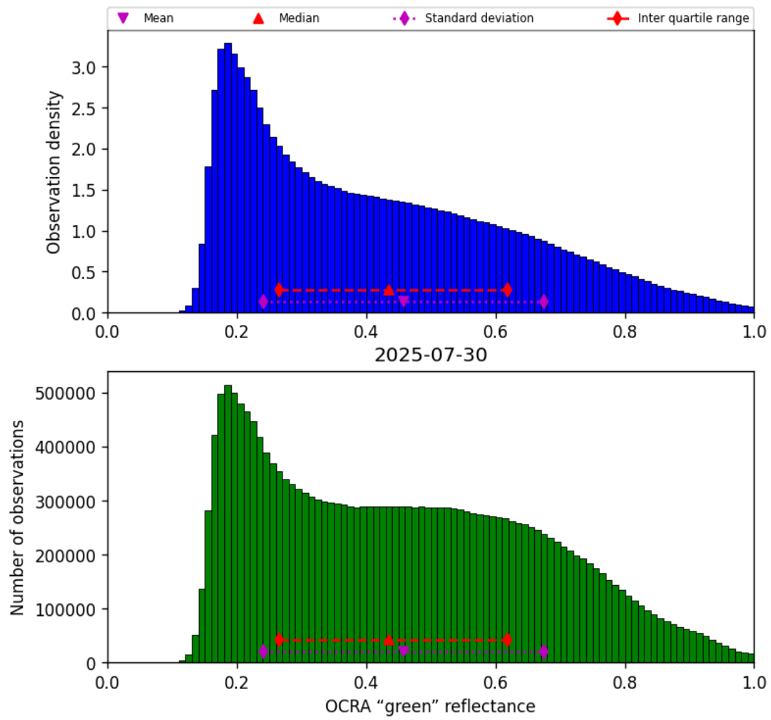
Figure 52: Histogram of “OCRA “green” reflectance” for 2025-07-29 to 2025-07-31
