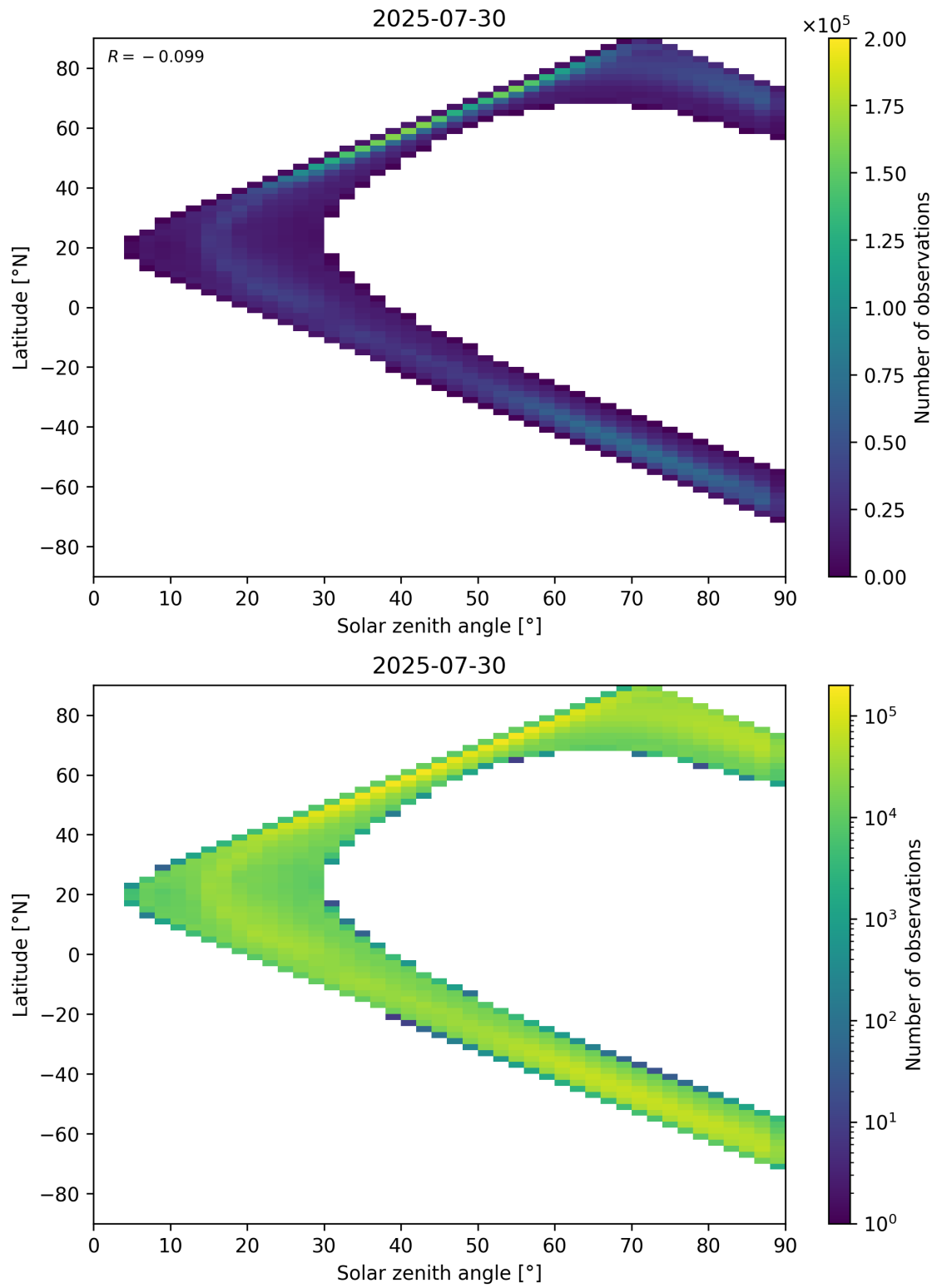
Figure 105: Scatter density plot of “Solar zenith angle” against “Latitude” for 2025-07-29 to 2025-07-31.
