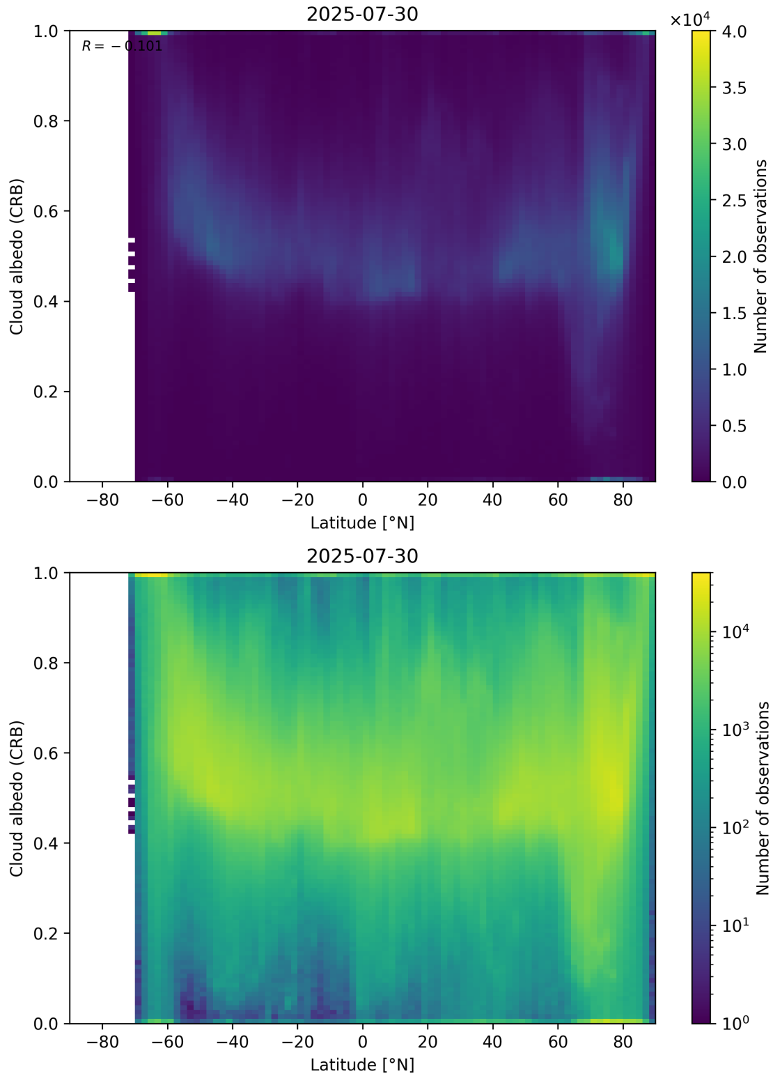
Figure 91: Scatter density plot of “Latitude” against “Cloud albedo (CRB)” for 2025-07-29 to 2025-07-31.
