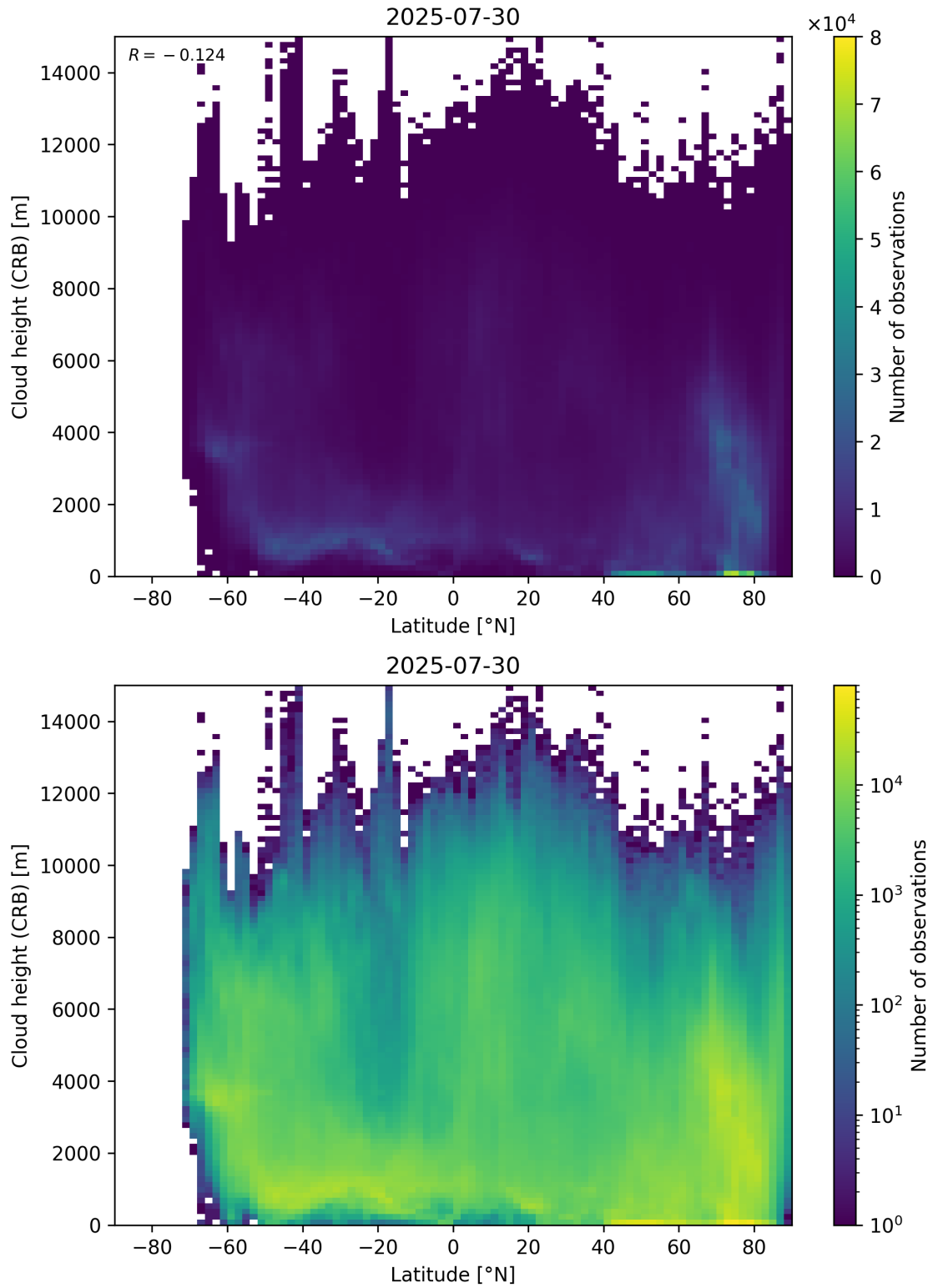
Figure 95: Scatter density plot of “Latitude” against “Cloud height (CRB)” for 2025-07-29 to 2025-07-31.
