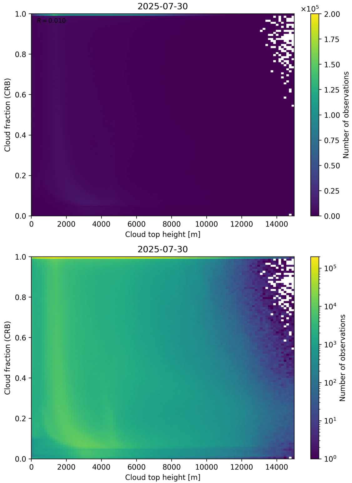
Figure 88: Scatter density plot of “Cloud top height” against “Cloud fraction (CRB)” for 2025-07-29 to 2025-07-31.
