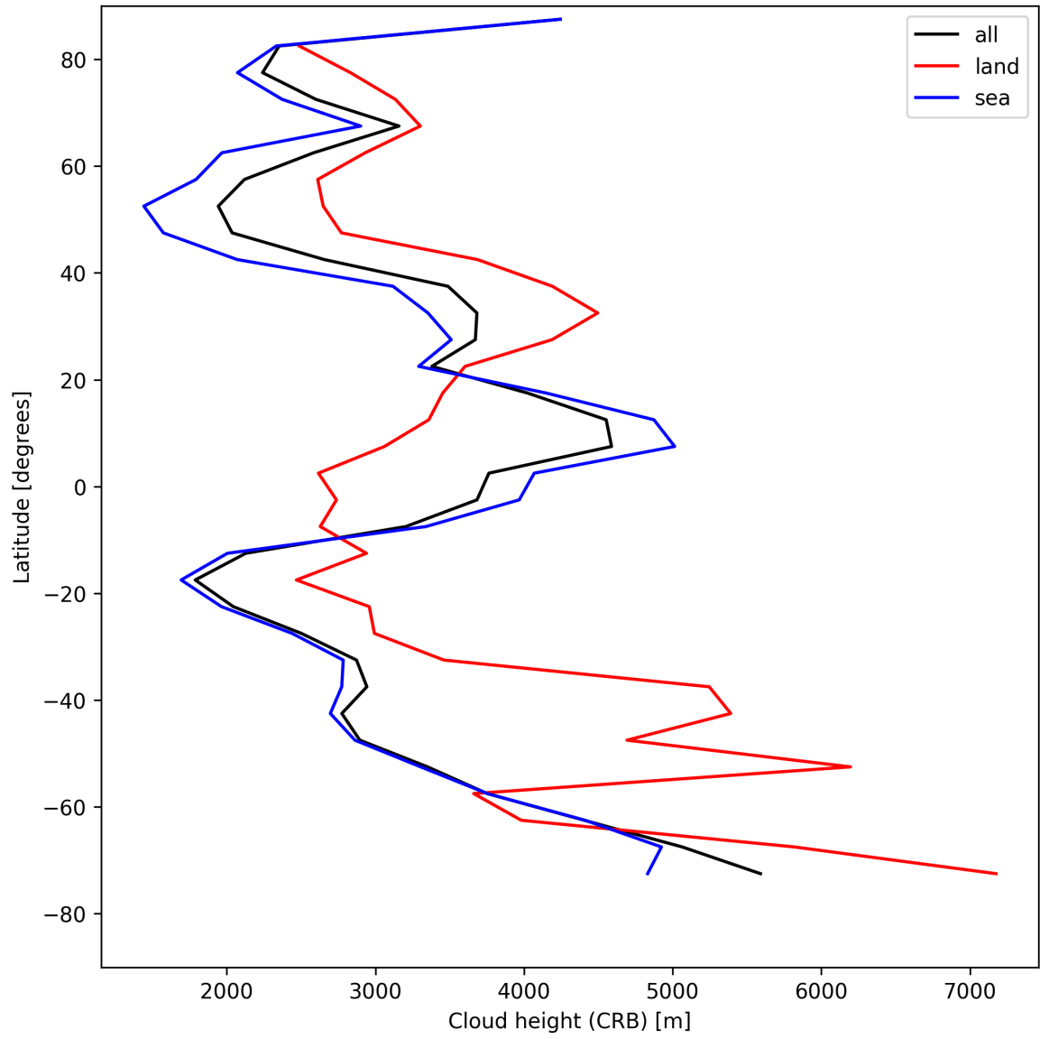
Figure 27: Zonal average of “Cloud height (CRB)” for 2025-07-29 to 2025-07-31.
