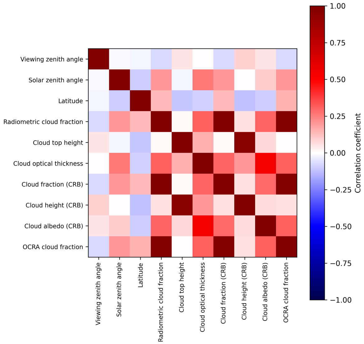
Figure 2: Map of correlation matrix for 2025-07-29 to 2025-07-31.
