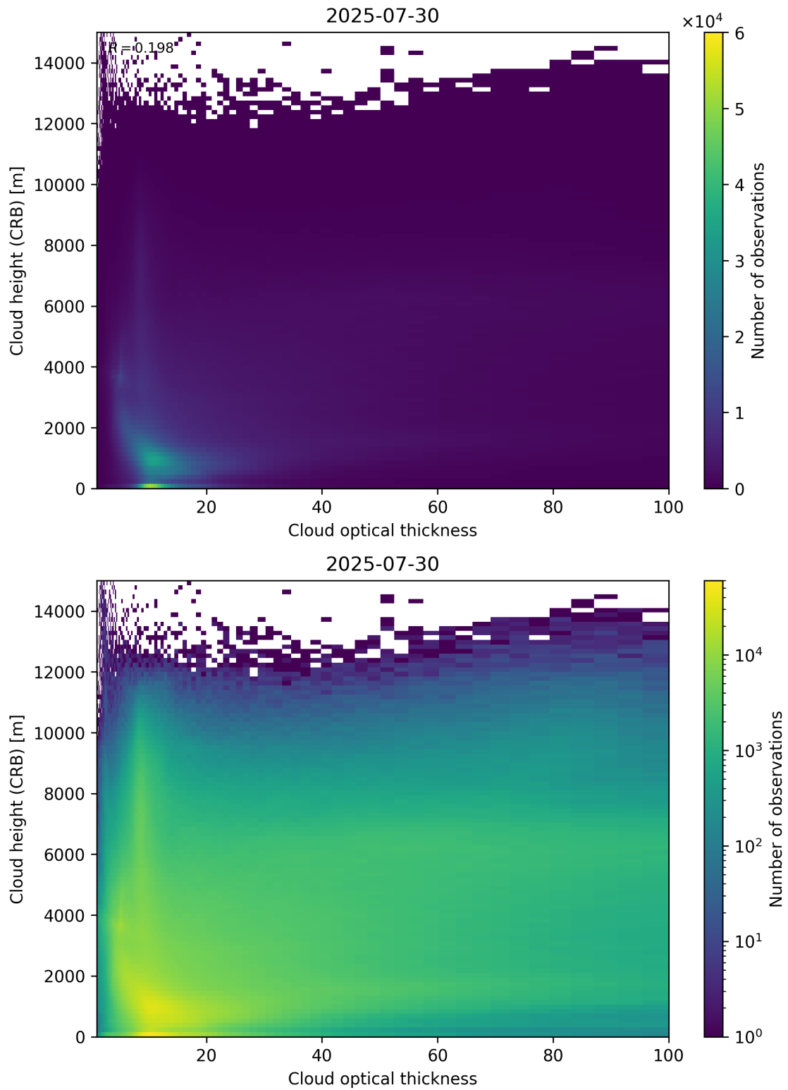
Figure 85: Scatter density plot of “Cloud optical thickness” against “Cloud height (CRB)” for 2025-07-29 to 2025-07-31.
