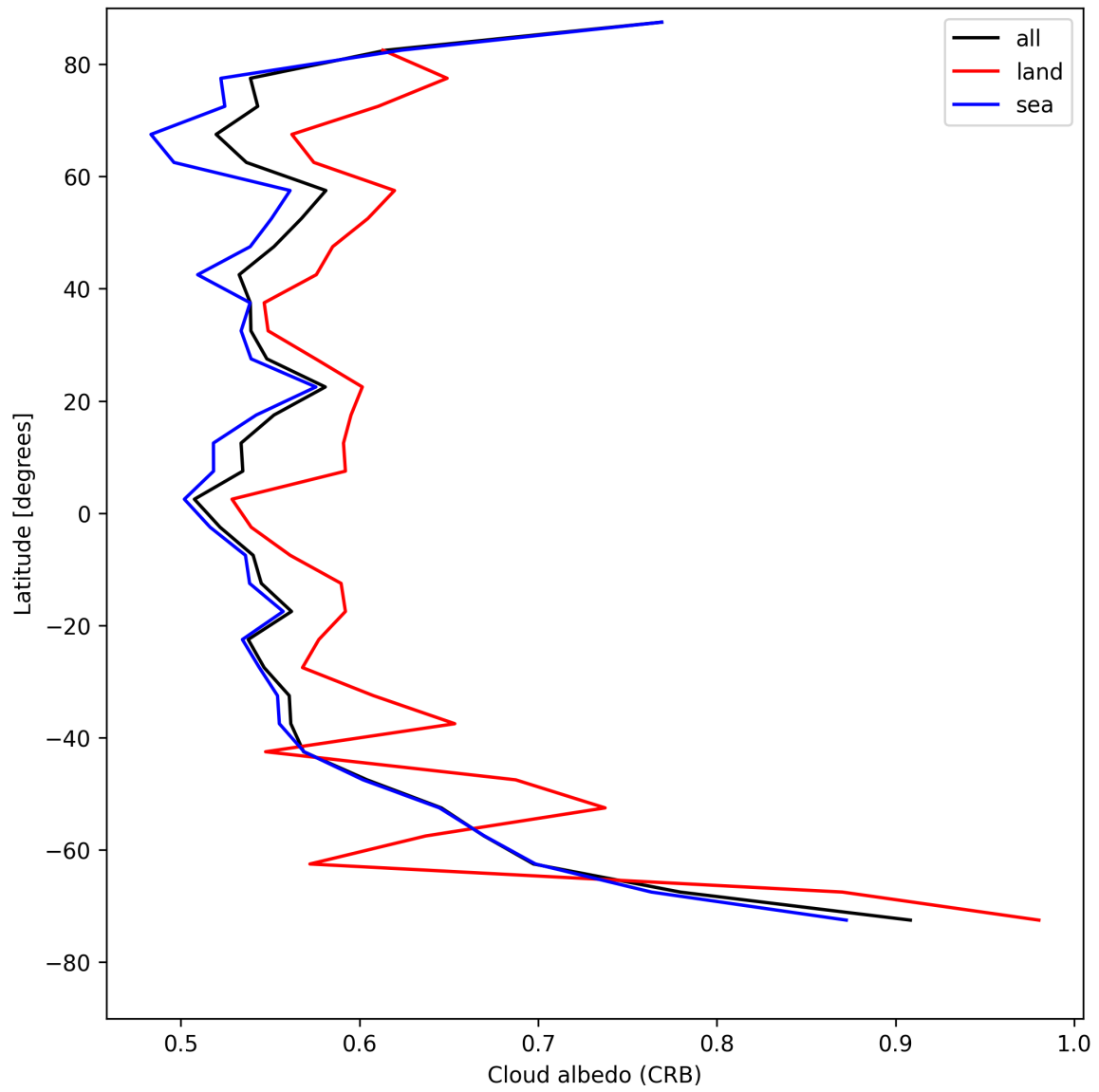
Figure 28: Zonal average of “Cloud albedo (CRB)” for 2025-07-29 to 2025-07-31.
