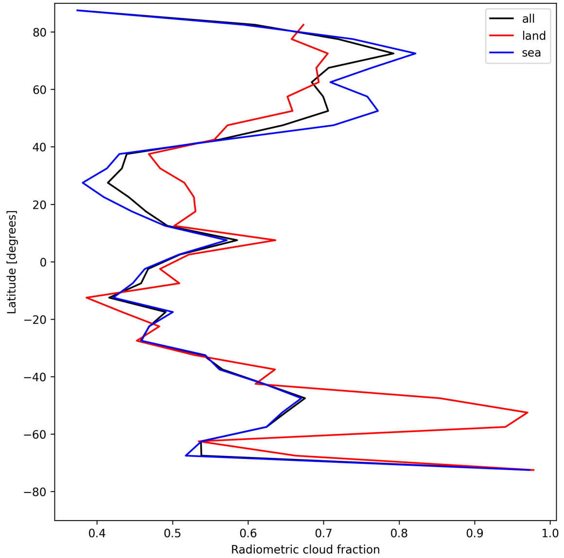
Figure 23: Zonal average of “Radiometric cloud fraction” for 2025-07-29 to 2025-07-31.
