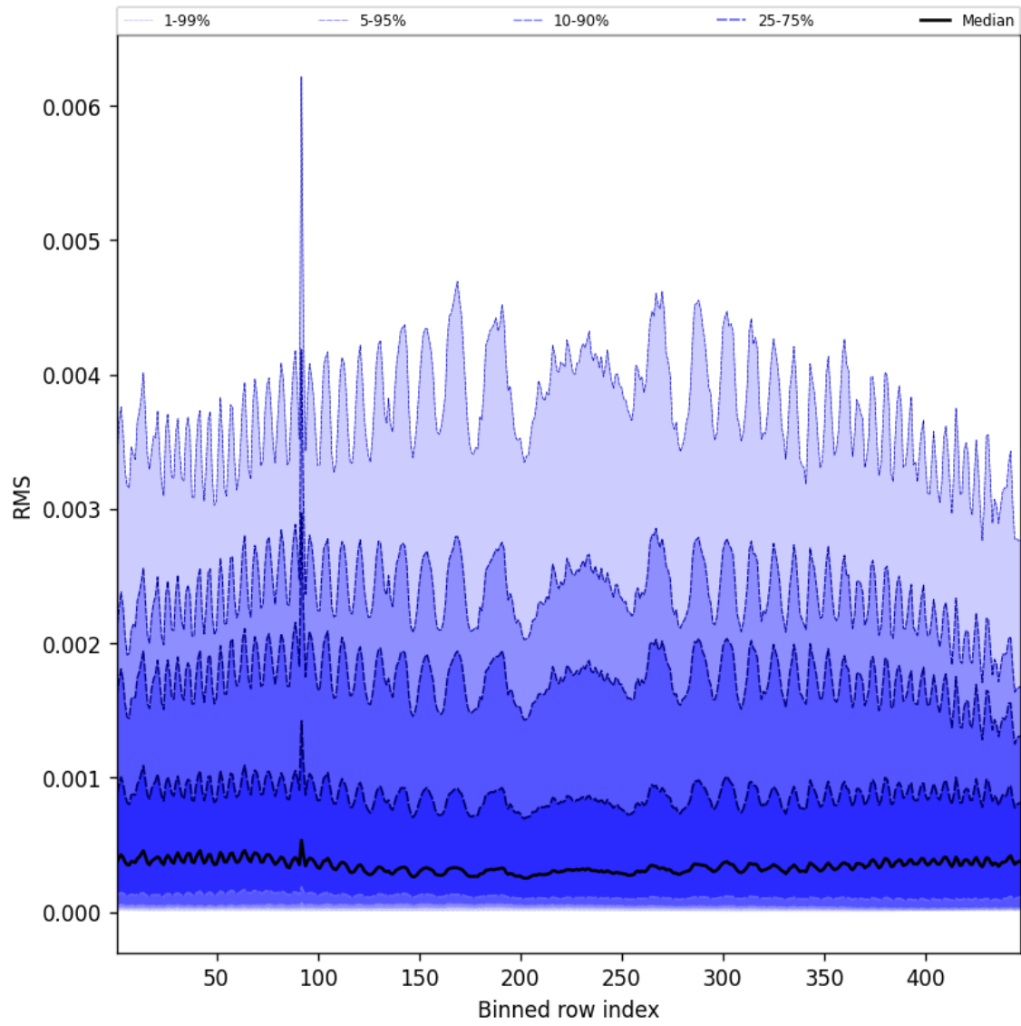
Figure 63: Along track statistics of “RMS” for 2025-07-29 to 2025-07-31
