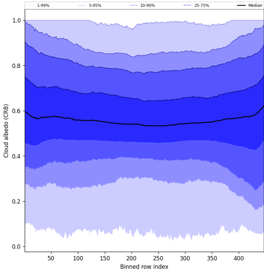
Figure 60: Along track statistics of “Cloud albedo (CRB)” for 2025-07-29 to 2025-07-31
