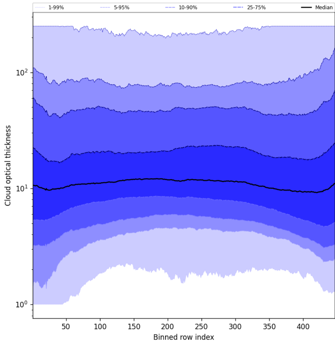
Figure 57: Along track statistics of “Cloud optical thickness” for 2025-07-29 to 2025-07-31
