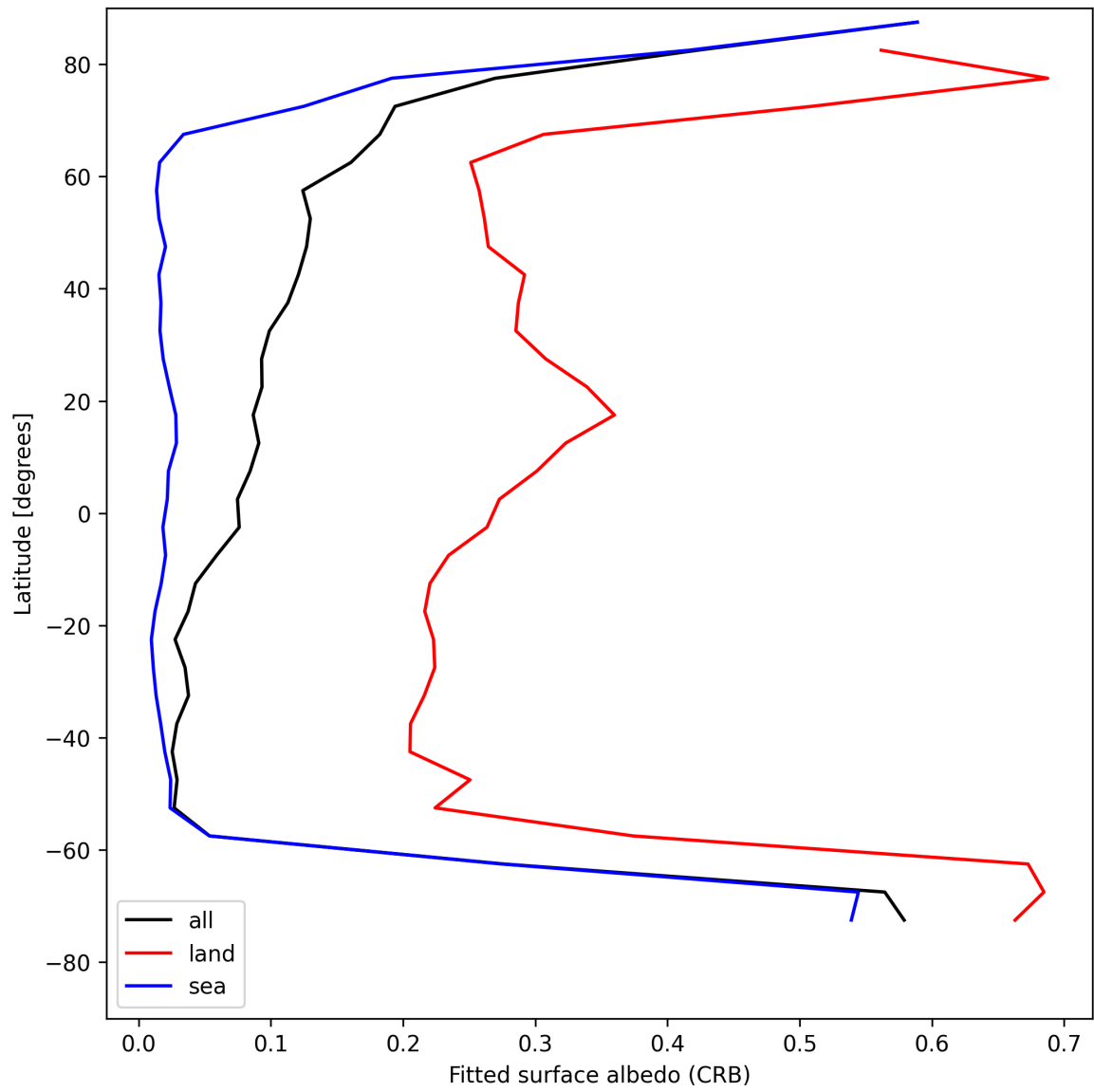
Figure 30: Zonal average of “Fitted surface albedo (CRB)” for 2025-07-29 to 2025-07-31.
