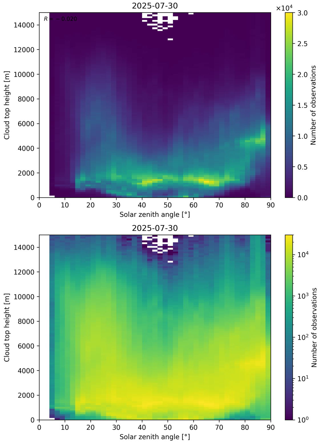
Figure 104: Scatter density plot of “Solar zenith angle” against “Cloud top height” for 2025-07-29 to 2025-07-31.
