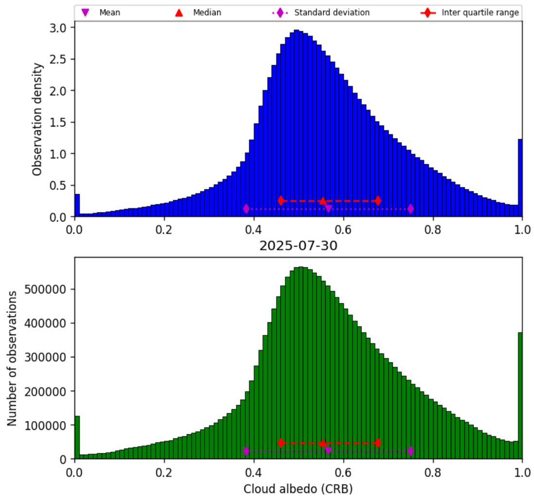
Figure 44: Histogram of “Cloud albedo (CRB)” for 2025-07-29 to 2025-07-31
