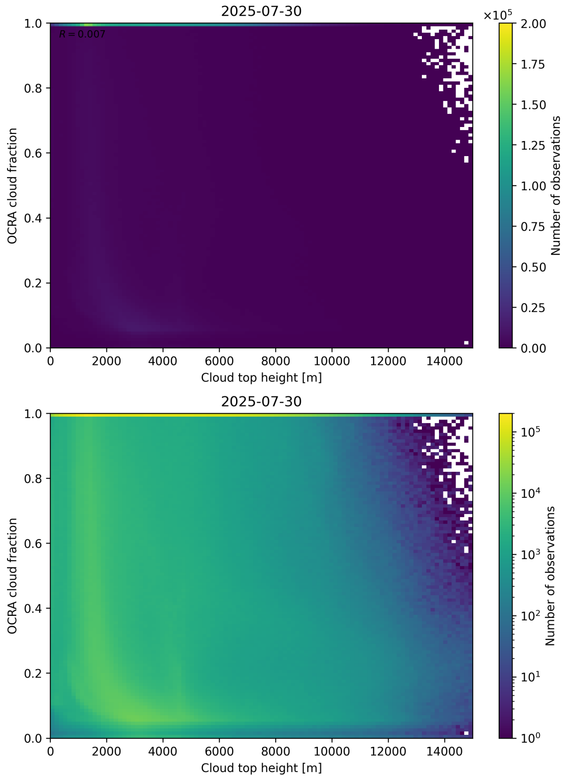
Figure 87: Scatter density plot of “Cloud top height” against “OCRA cloud fraction” for 2025-07-29 to 2025-07-31.
