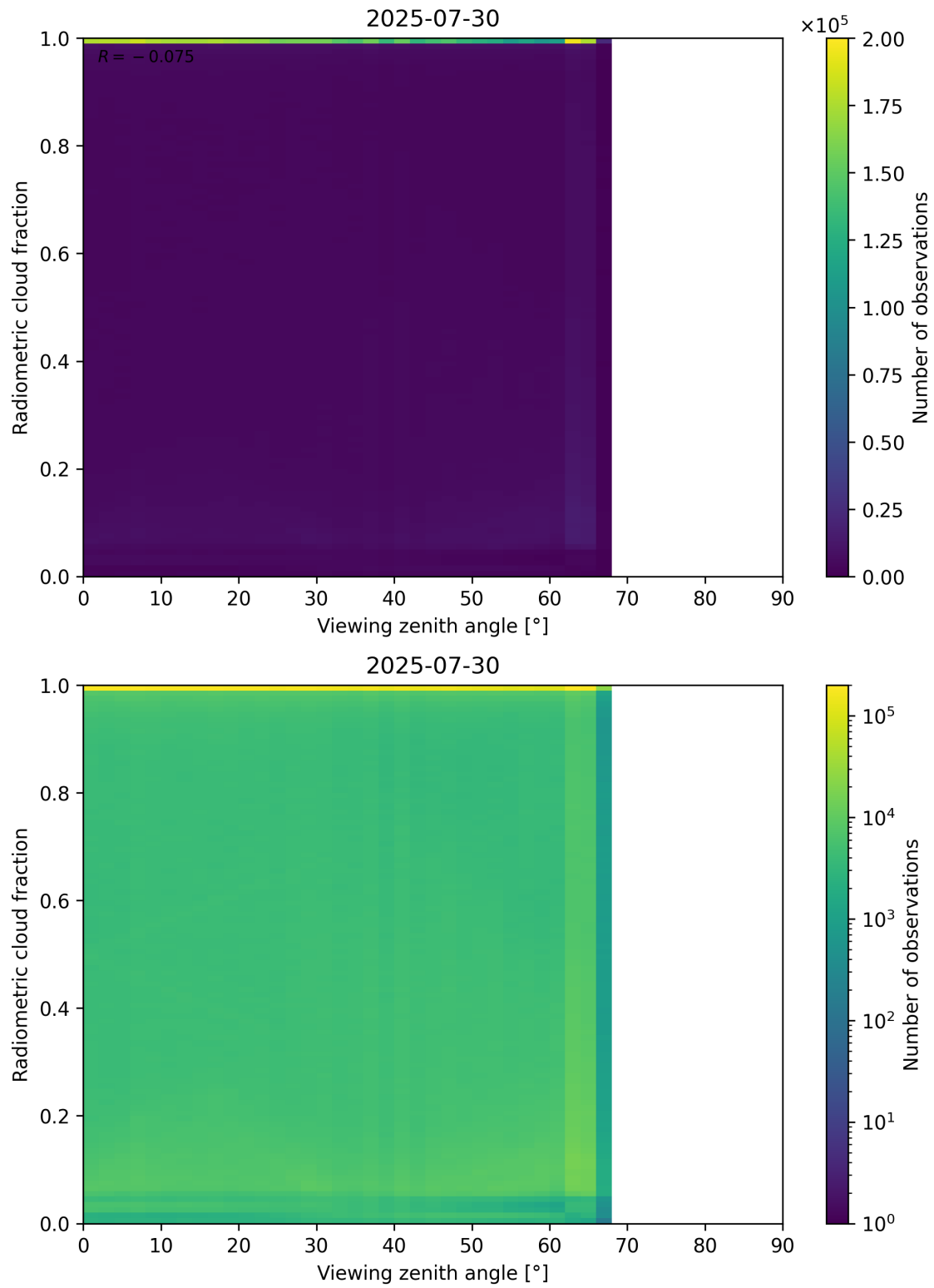
Figure 107: Scatter density plot of “Viewing zenith angle” against “Radiometric cloud fraction” for 2025-07-29 to 2025-07-31.
