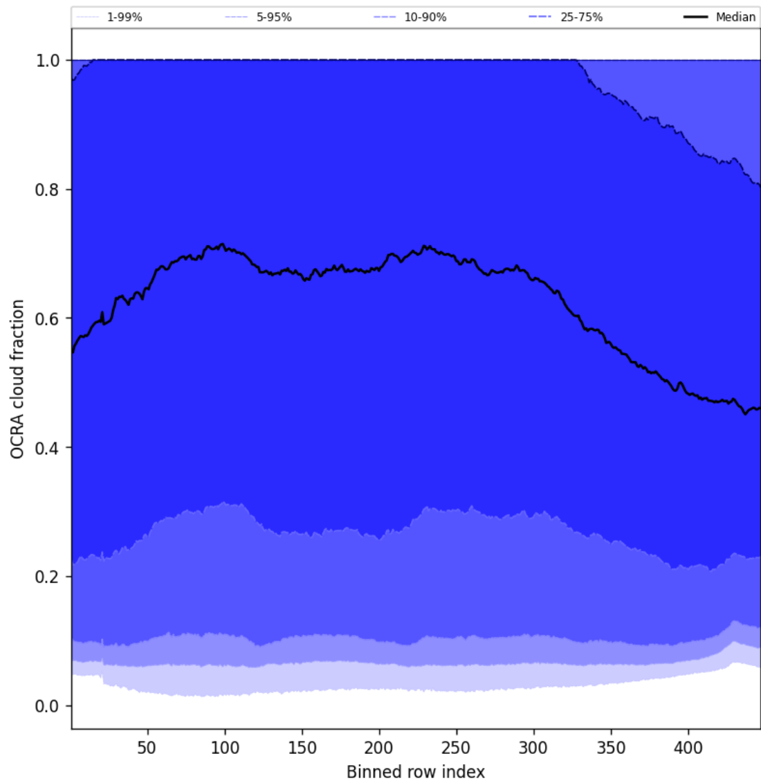
Figure 66: Along track statistics of “OCRA cloud fraction” for 2025-07-29 to 2025-07-31
