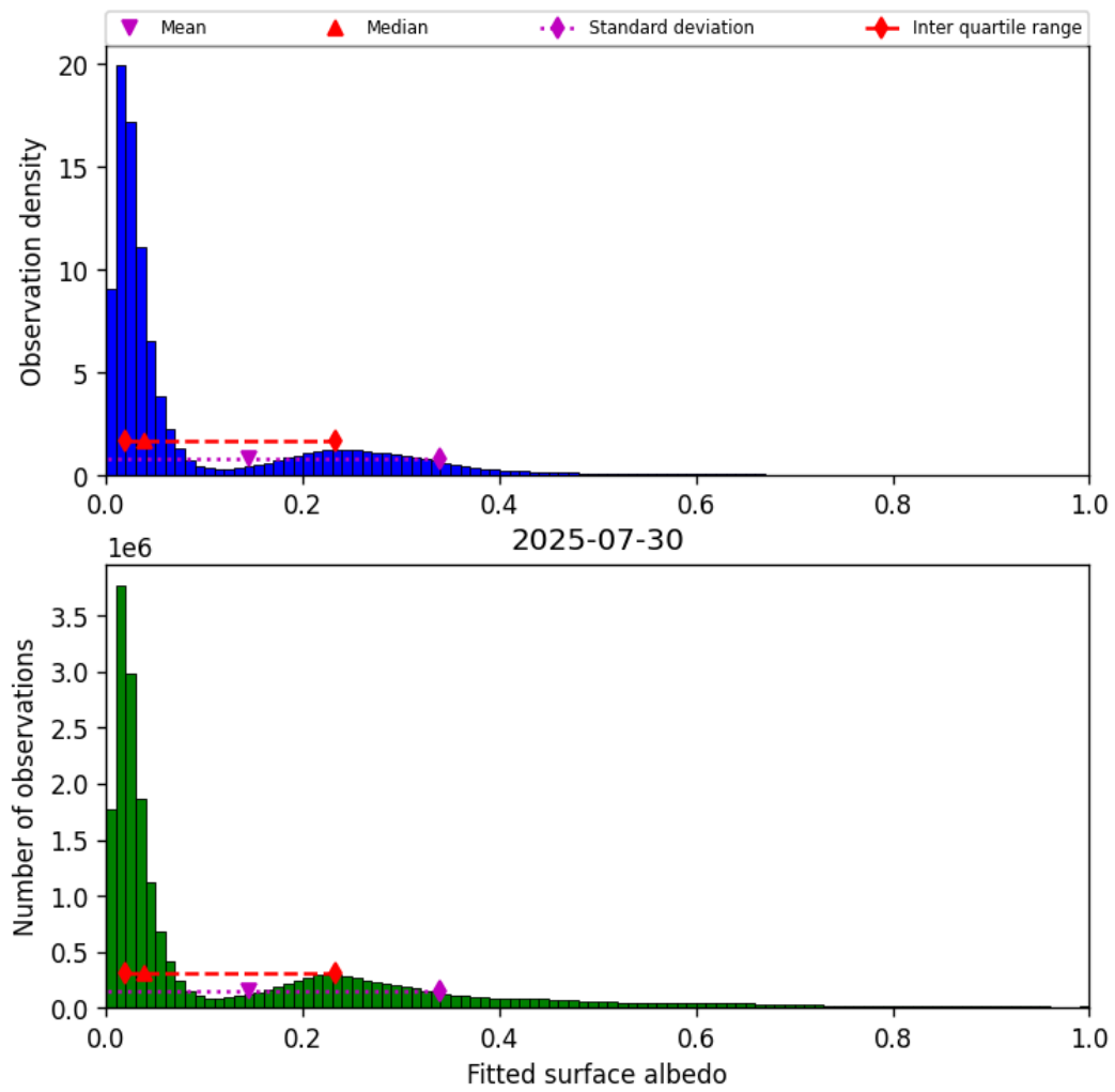
Figure 45: Histogram of “Fitted surface albedo” for 2025-07-29 to 2025-07-31
