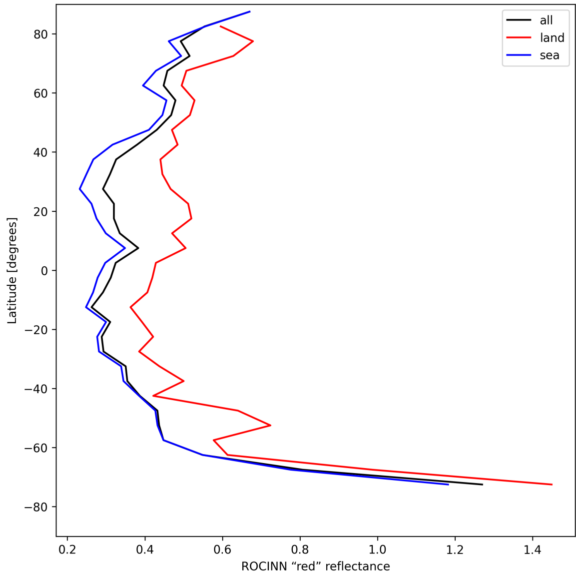
Figure 37: Zonal average of "ROCINN "red" reflectance" for 2025-07-29 to 2025-07-31.
