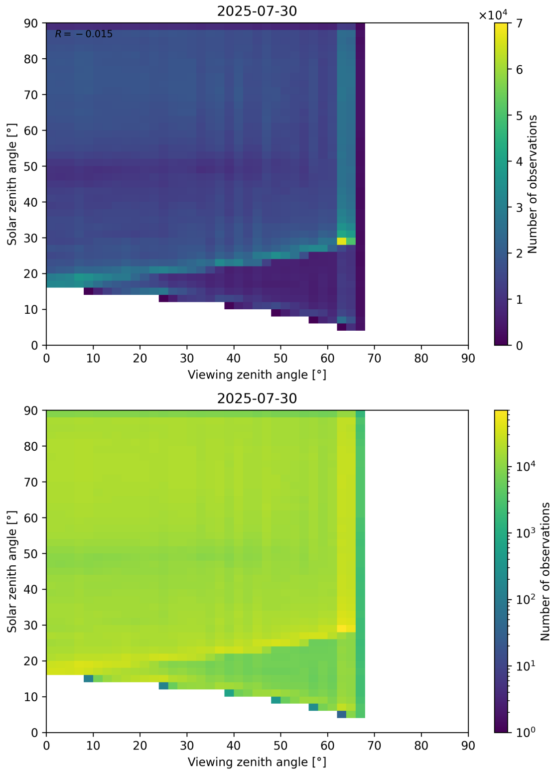
Figure 114: Scatter density plot of “Viewing zenith angle” against “Solar zenith angle” for 2025-07-29 to 2025-07-31.
