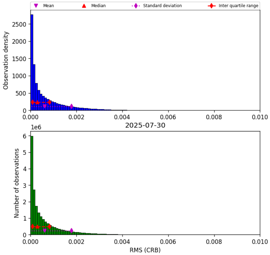
Figure 48: Histogram of “RMS (CRB)” for 2025-07-29 to 2025-07-31
