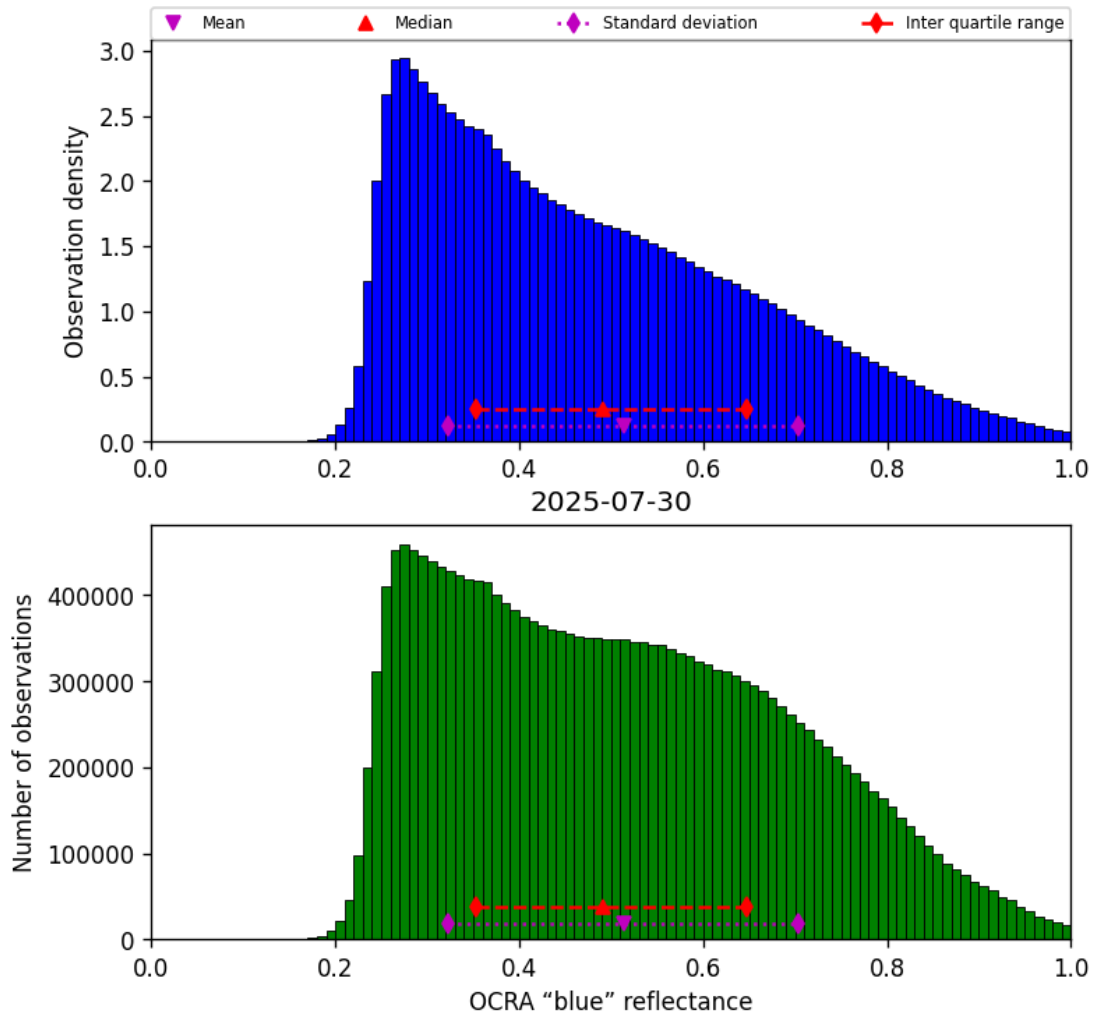
Figure 51: Histogram of “OCRA “blue” reflectance” for 2025-07-29 to 2025-07-31
