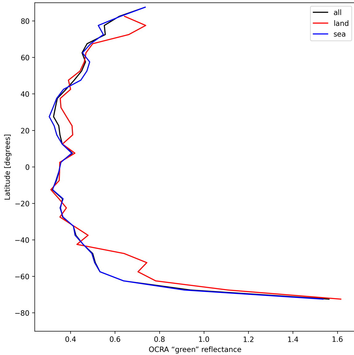
Figure 36: Zonal average of “OCRA “green” reflectance” for 2025-07-29 to 2025-07-31.
