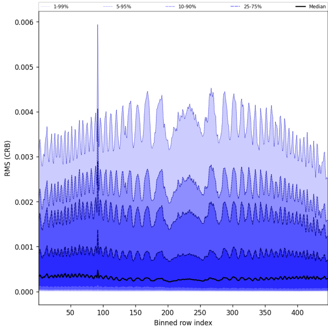
Figure 64: Along track statistics of “RMS (CRB)” for 2025-07-29 to 2025-07-31
