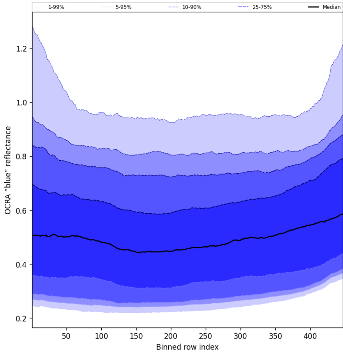
Figure 67: Along track statistics of "OCRA "blue" reflectance" for 2025-07-29 to 2025-07-31
