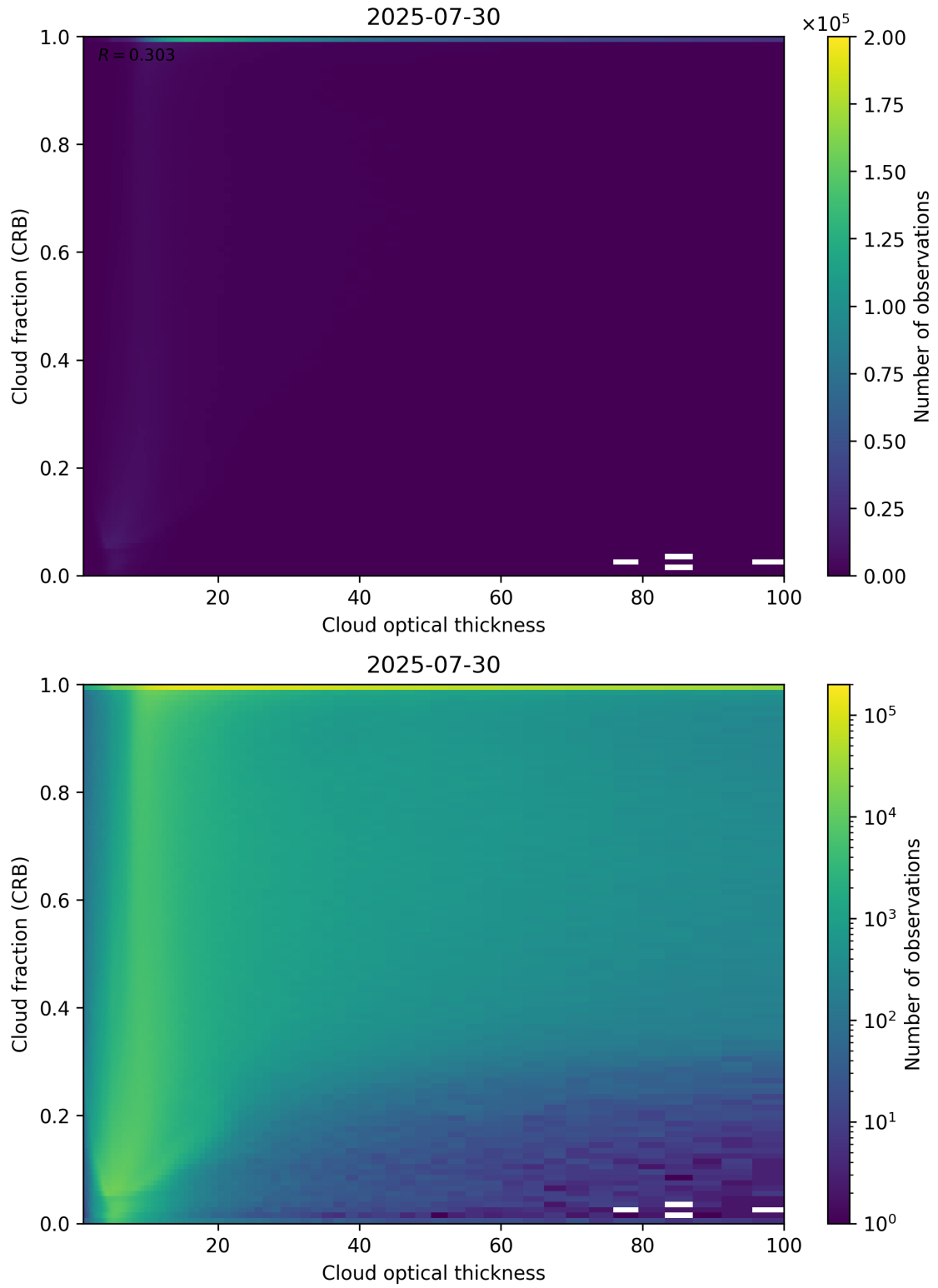
Figure 84: Scatter density plot of “Cloud optical thickness” against “Cloud fraction (CRB)” for 2025-07-29 to 2025-07-31.
