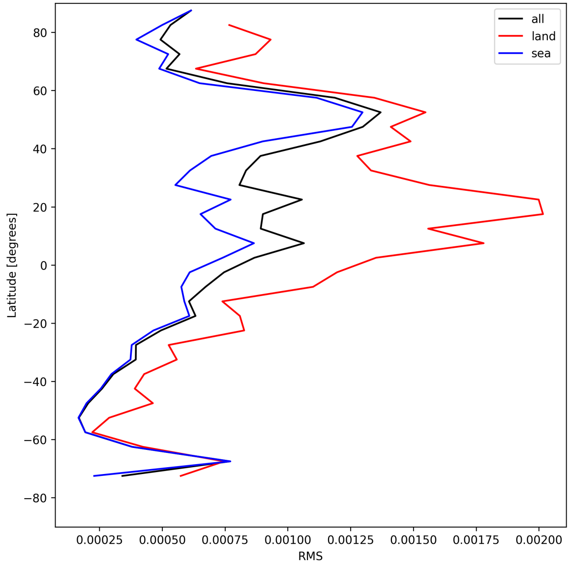
Figure 31: Zonal average of “RMS” for 2025-07-29 to 2025-07-31.
