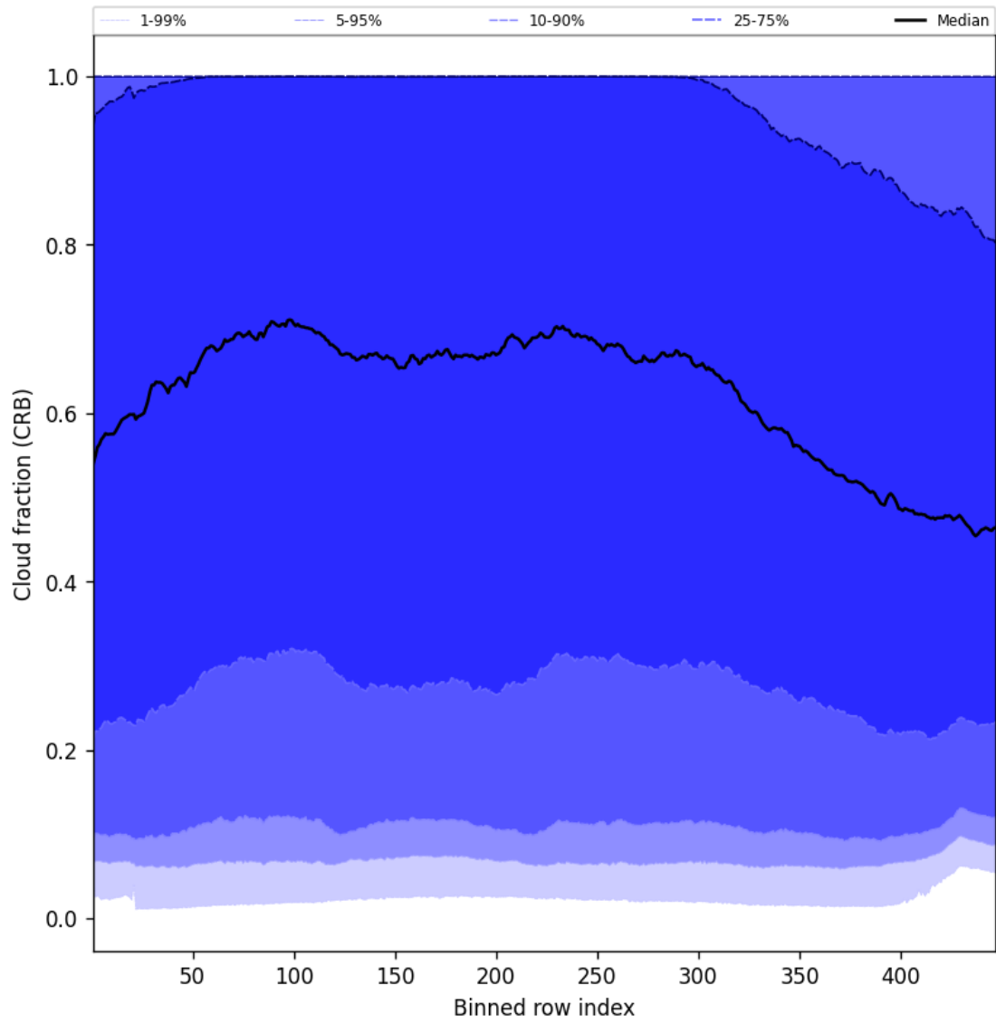
Figure 58: Along track statistics of “Cloud fraction (CRB)” for 2025-07-29 to 2025-07-31
