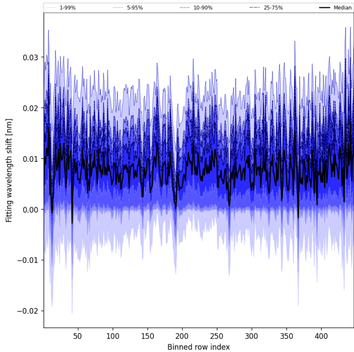
Figure 65: Along track statistics of “Fitting wavelength shift” for 2025-07-29 to 2025-07-31
