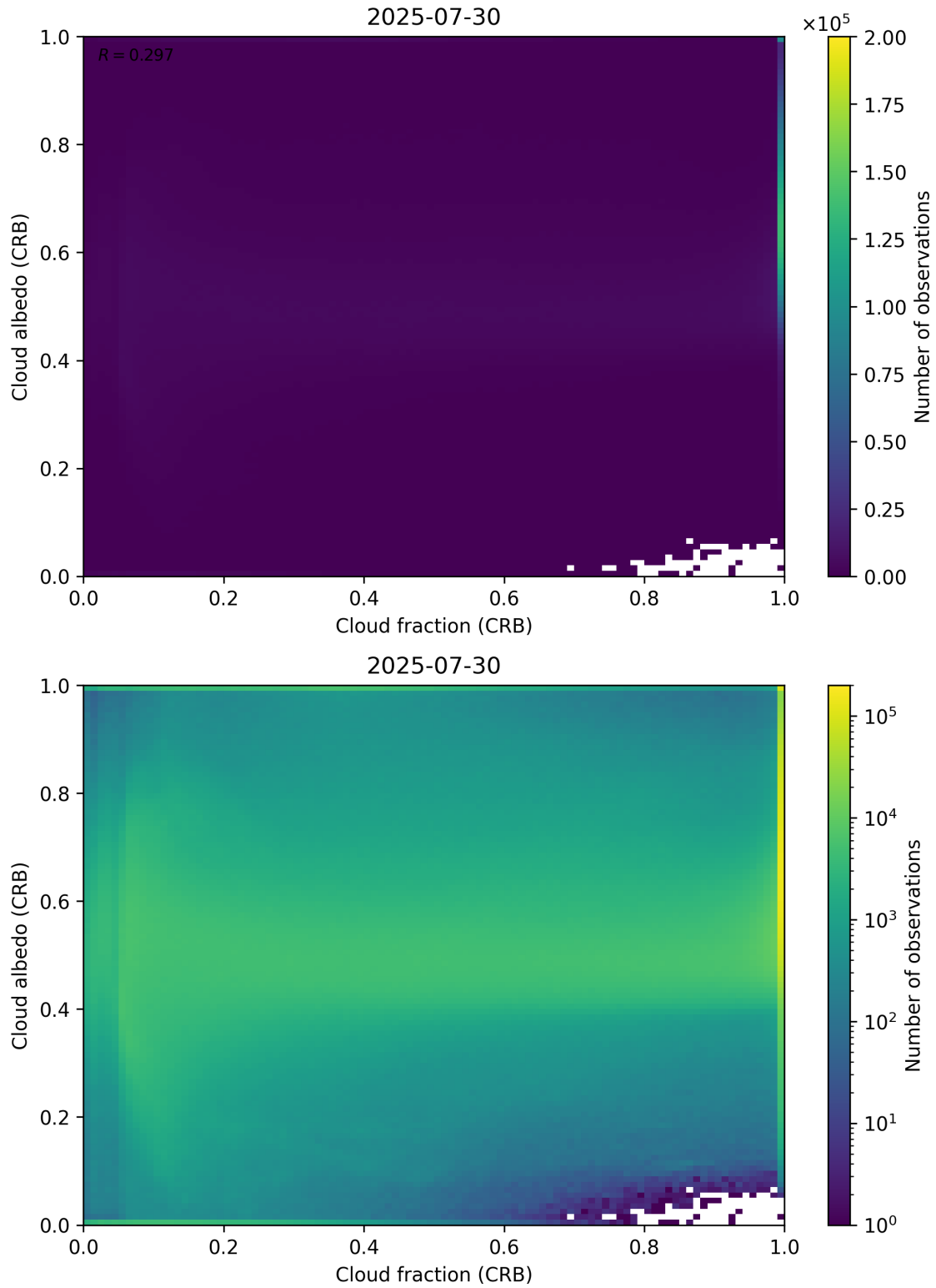
Figure 77: Scatter density plot of “Cloud fraction (CRB)” against “Cloud albedo (CRB)” for 2025-07-29 to 2025-07-31.
