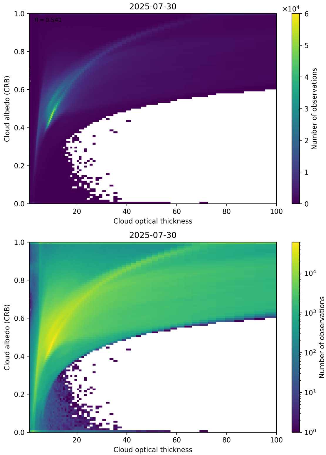
Figure 82: Scatter density plot of “Cloud optical thickness” against “Cloud albedo (CRB)” for 2025-07-29 to 2025-07-31.
