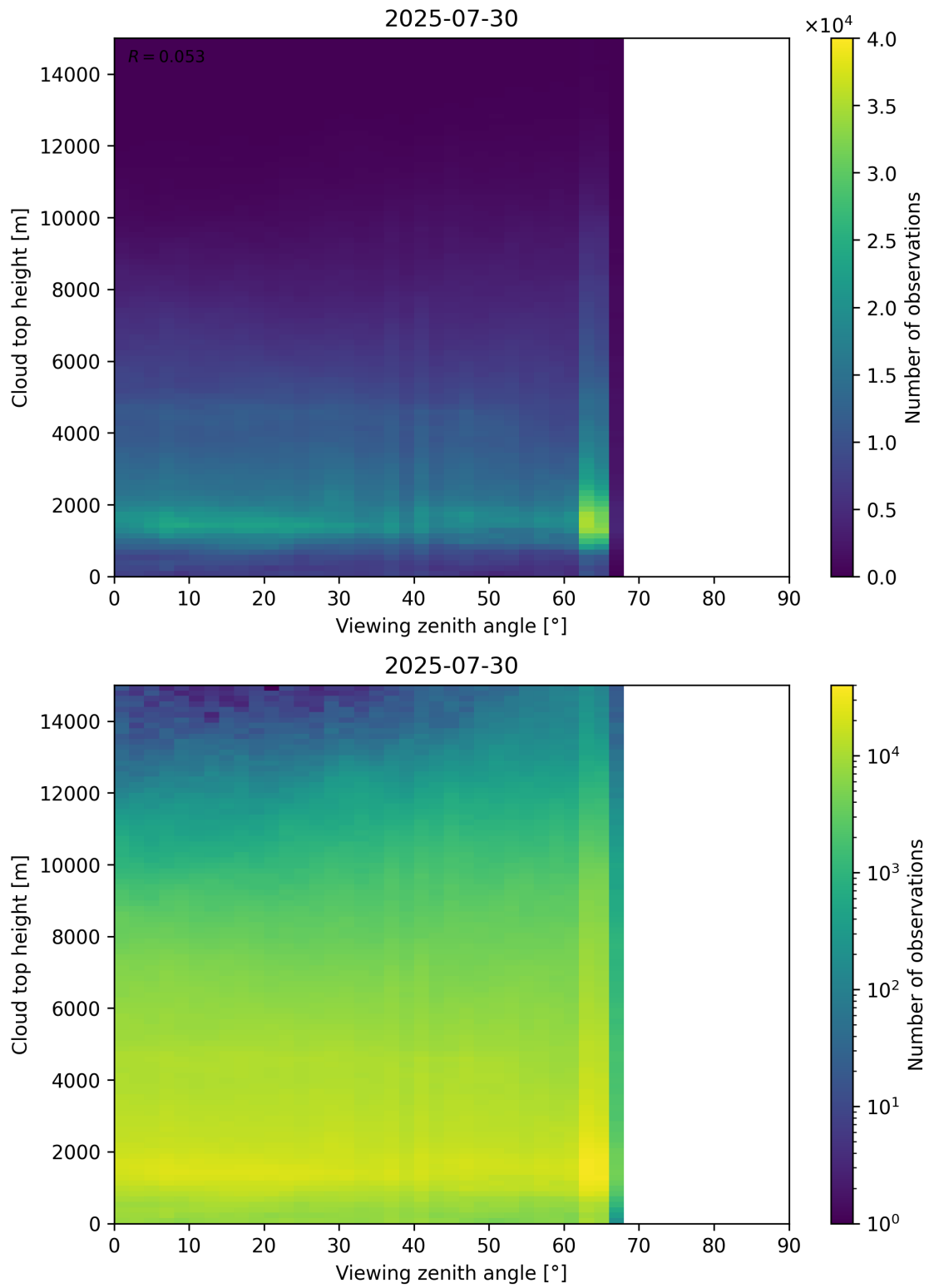
Figure 112: Scatter density plot of “Viewing zenith angle” against “Cloud top height” for 2025-07-29 to 2025-07-31.
