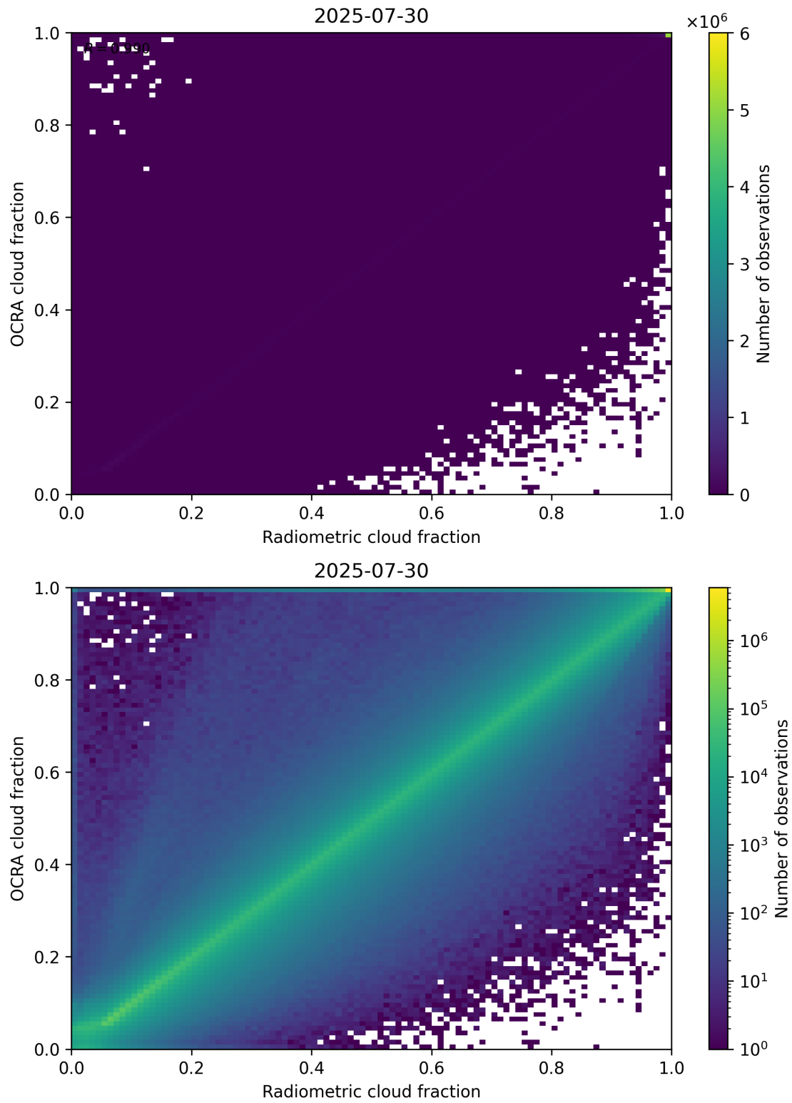
Figure 72: Scatter density plot of “Radiometric cloud fraction” against “OCRA cloud fraction” for 2025-07-29 to 2025-07-31.
