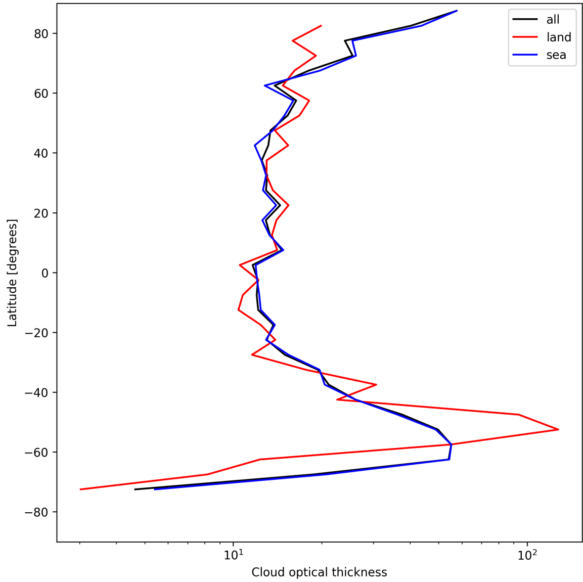
Figure 25: Zonal average of “Cloud optical thickness” for 2025-07-29 to 2025-07-31.
