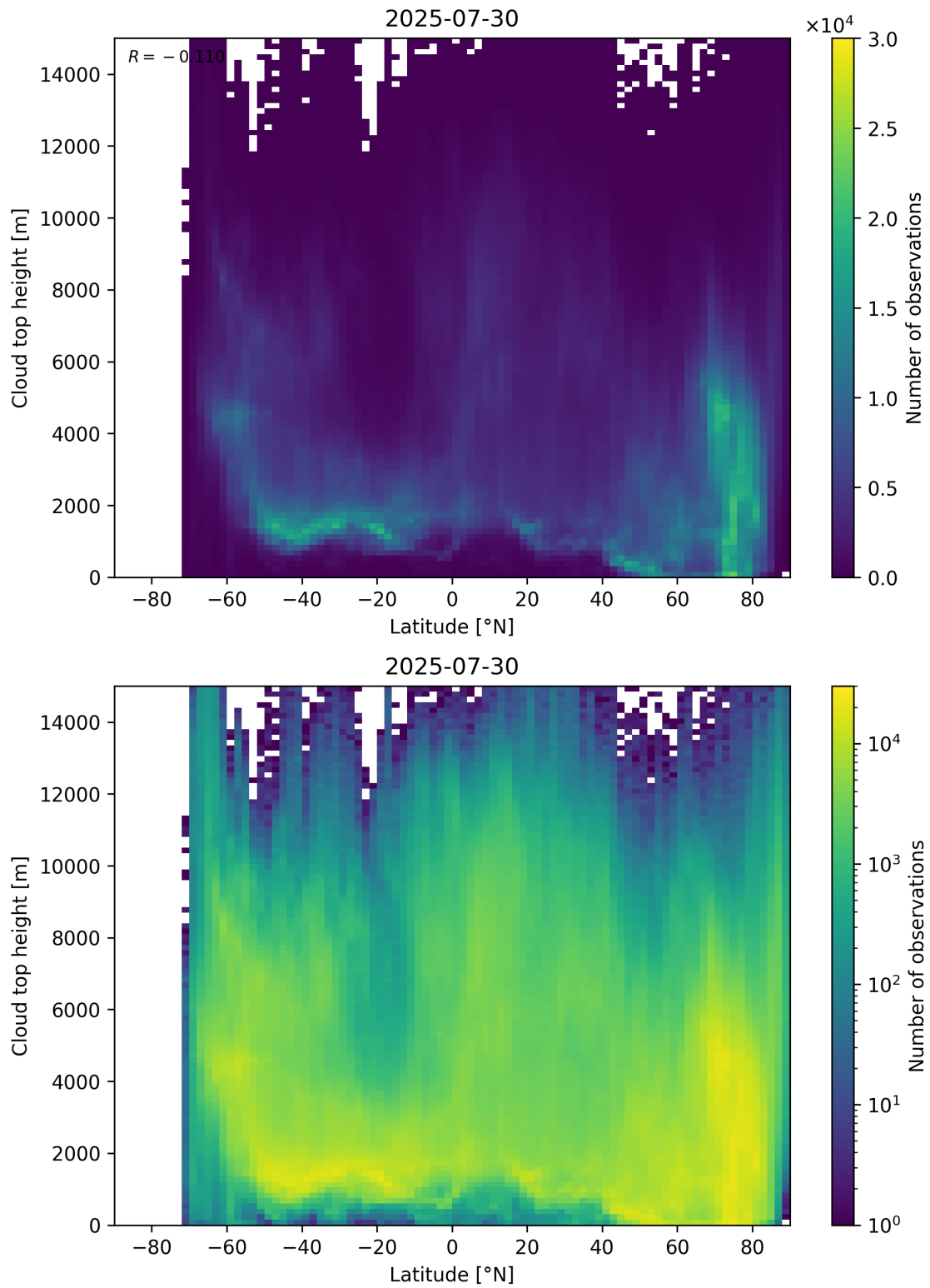
Figure 97: Scatter density plot of “Latitude” against “Cloud top height” for 2025-07-29 to 2025-07-31.
