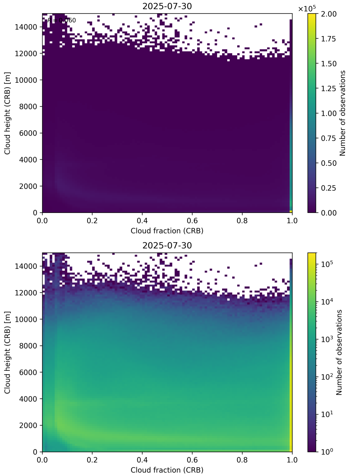
Figure 79: Scatter density plot of “Cloud fraction (CRB)” against “Cloud height (CRB)” for 2025-07-29 to 2025-07-31.
