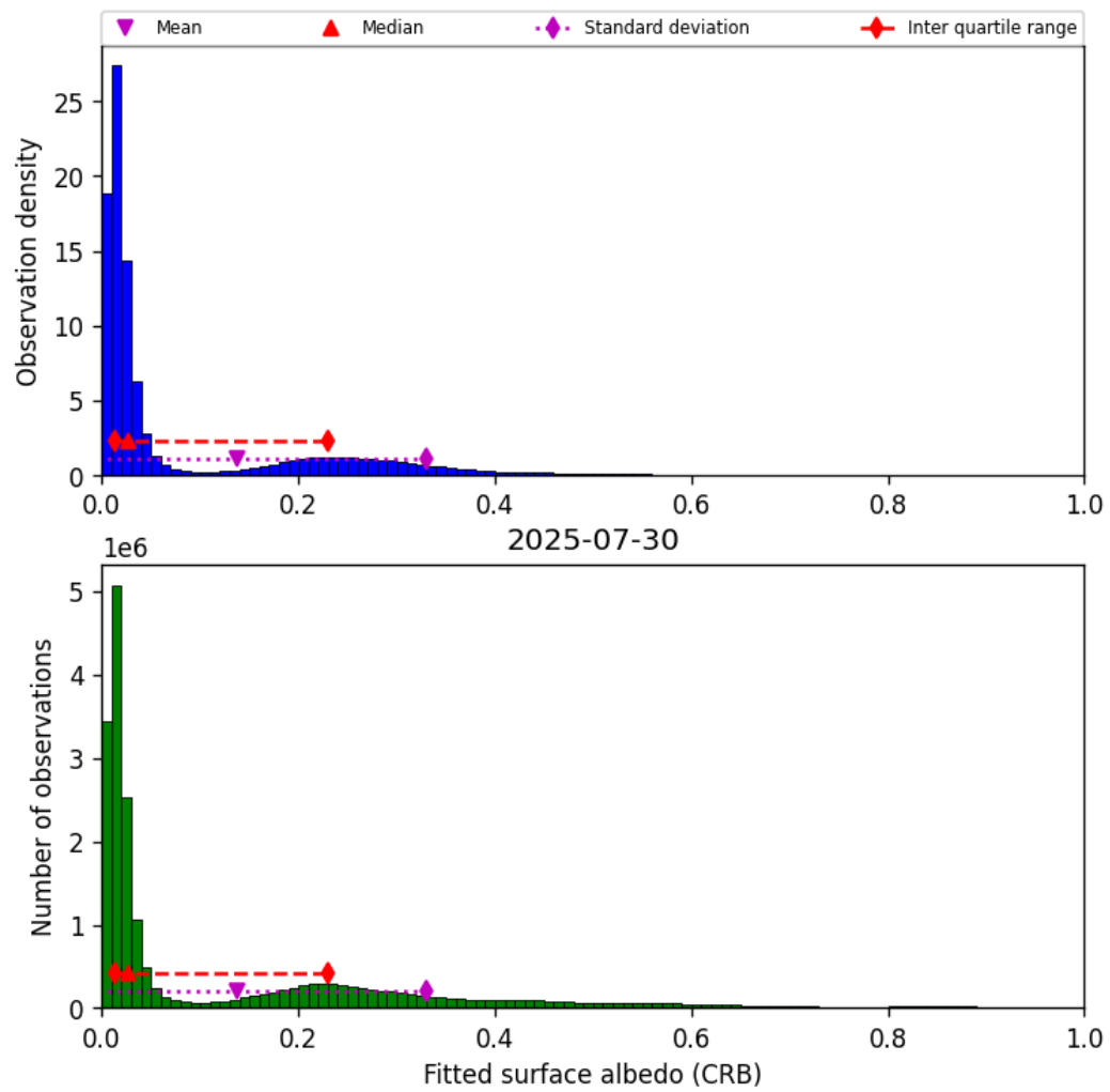
Figure 46: Histogram of “Fitted surface albedo (CRB)” for 2025-07-29 to 2025-07-31
