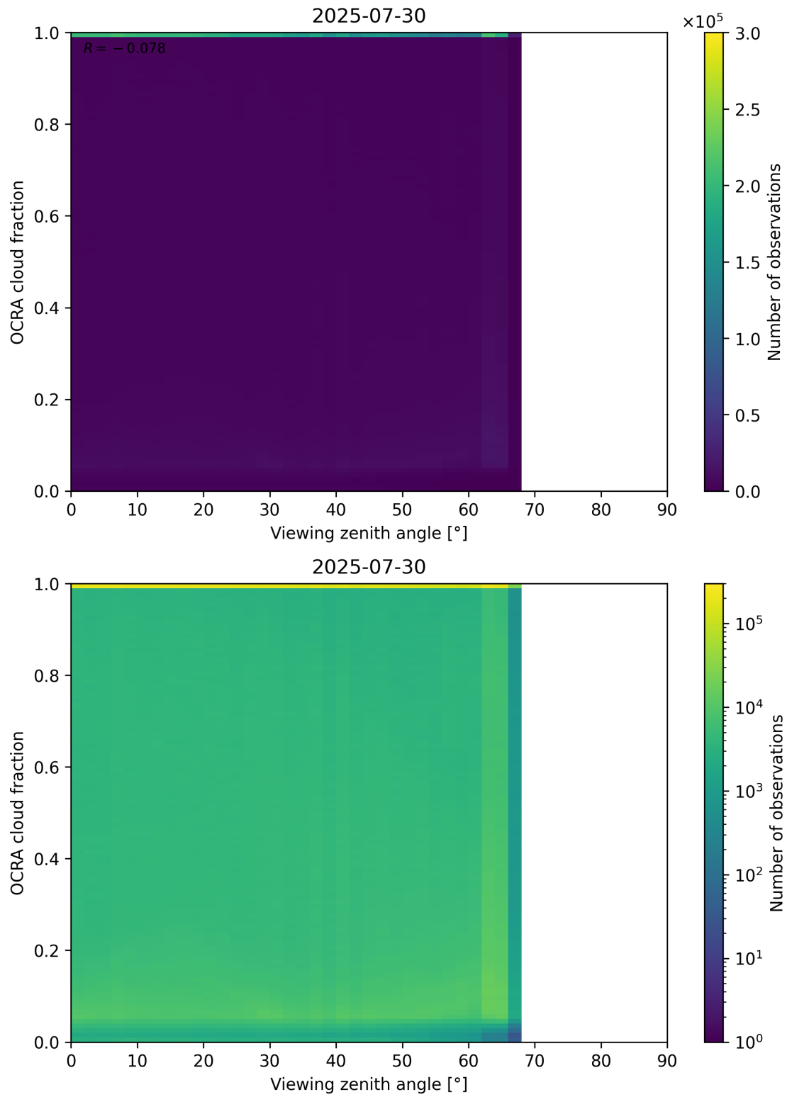
Figure 108: Scatter density plot of “Viewing zenith angle” against “OCRA cloud fraction” for 2025-07-29 to 2025-07-31.
