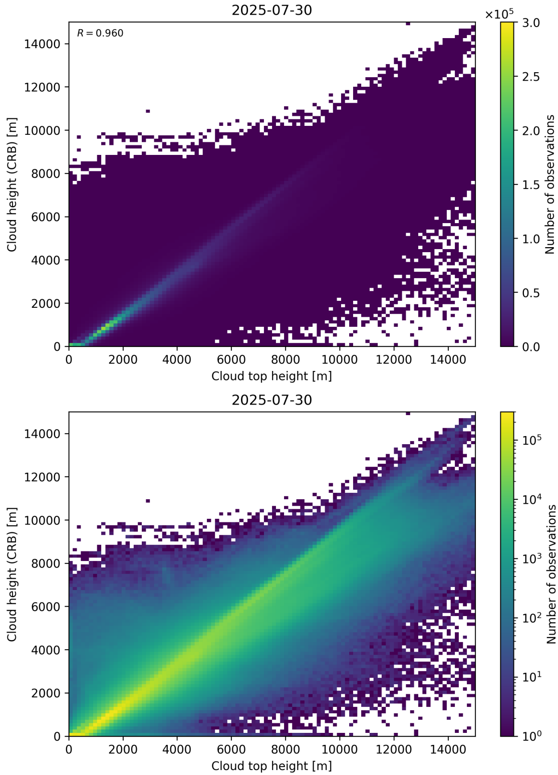
Figure 89: Scatter density plot of “Cloud top height” against “Cloud height (CRB)” for 2025-07-29 to 2025-07-31.
