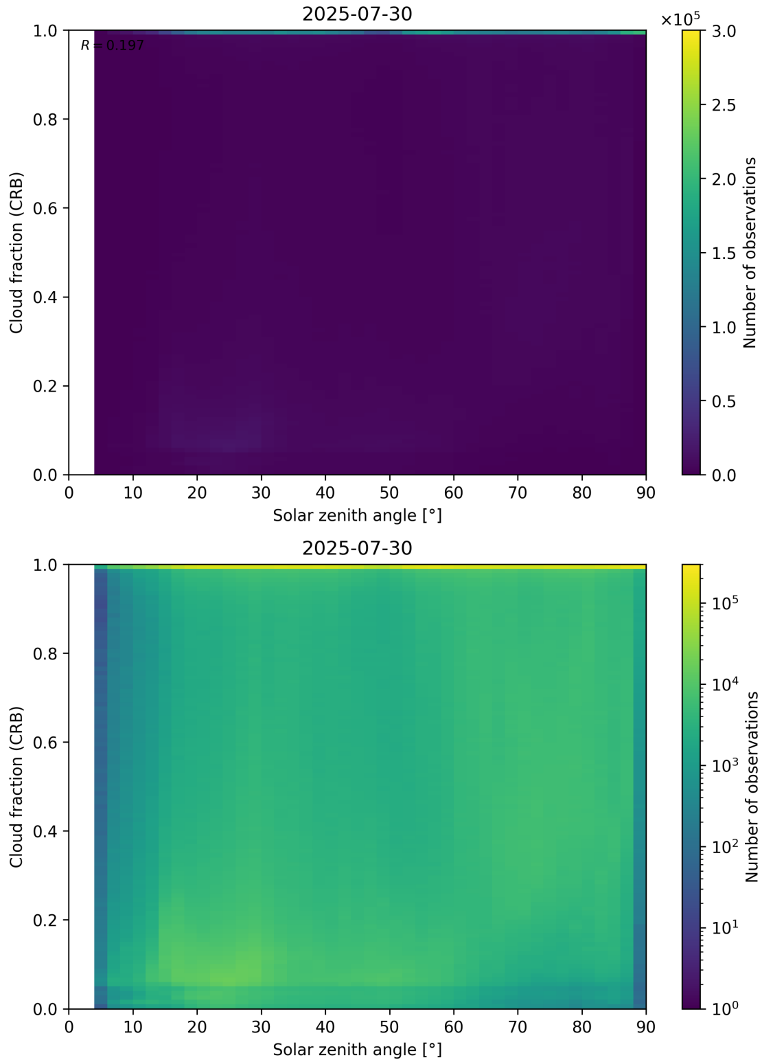
Figure 101: Scatter density plot of “Solar zenith angle” against “Cloud fraction (CRB)” for 2025-07-29 to 2025-07-31.
