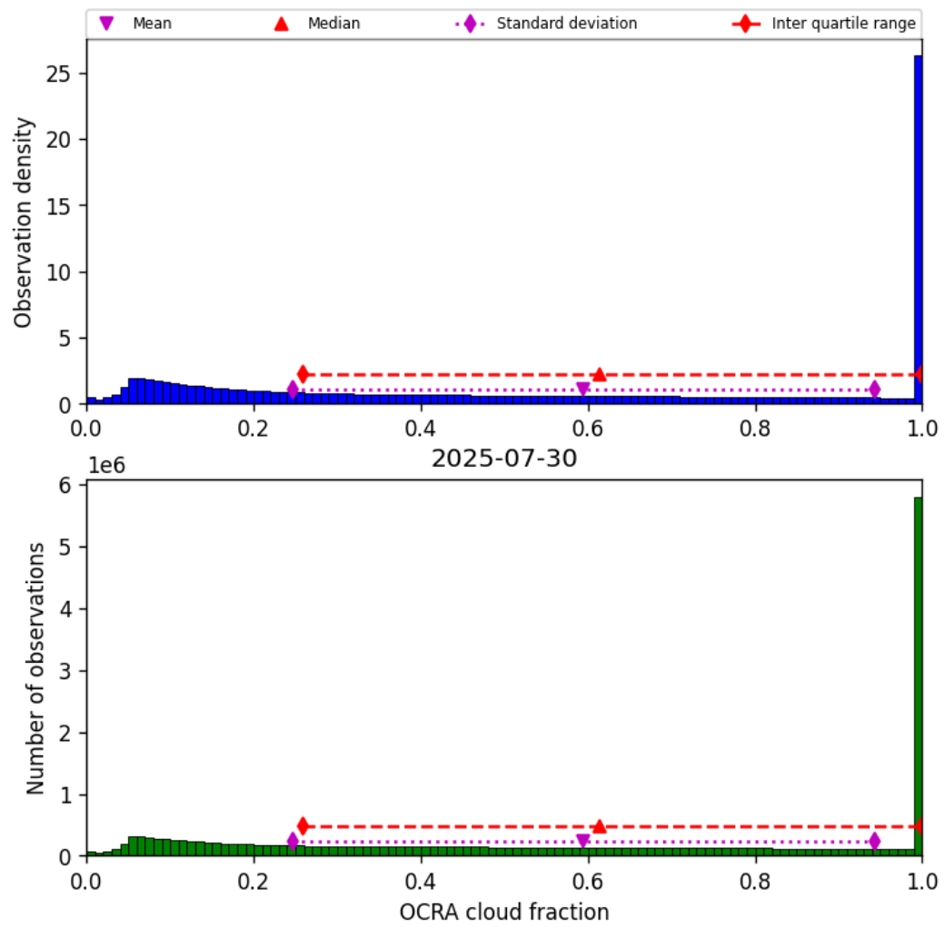
Figure 50: Histogram of “OCRA cloud fraction” for 2025-07-29 to 2025-07-31
