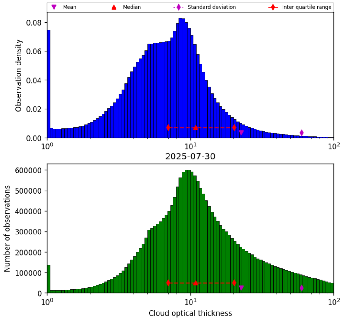
Figure 41: Histogram of “Cloud optical thickness” for 2025-07-29 to 2025-07-31
