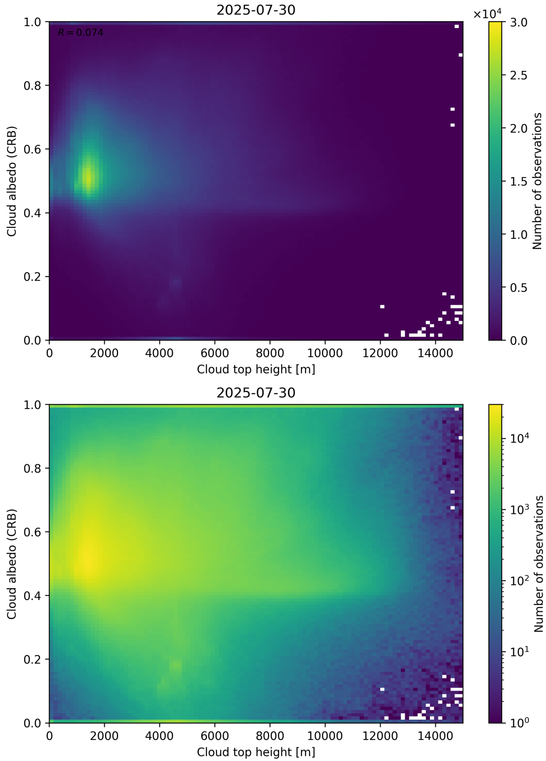
Figure 86: Scatter density plot of “Cloud top height” against “Cloud albedo (CRB)” for 2025-07-29 to 2025-07-31.
