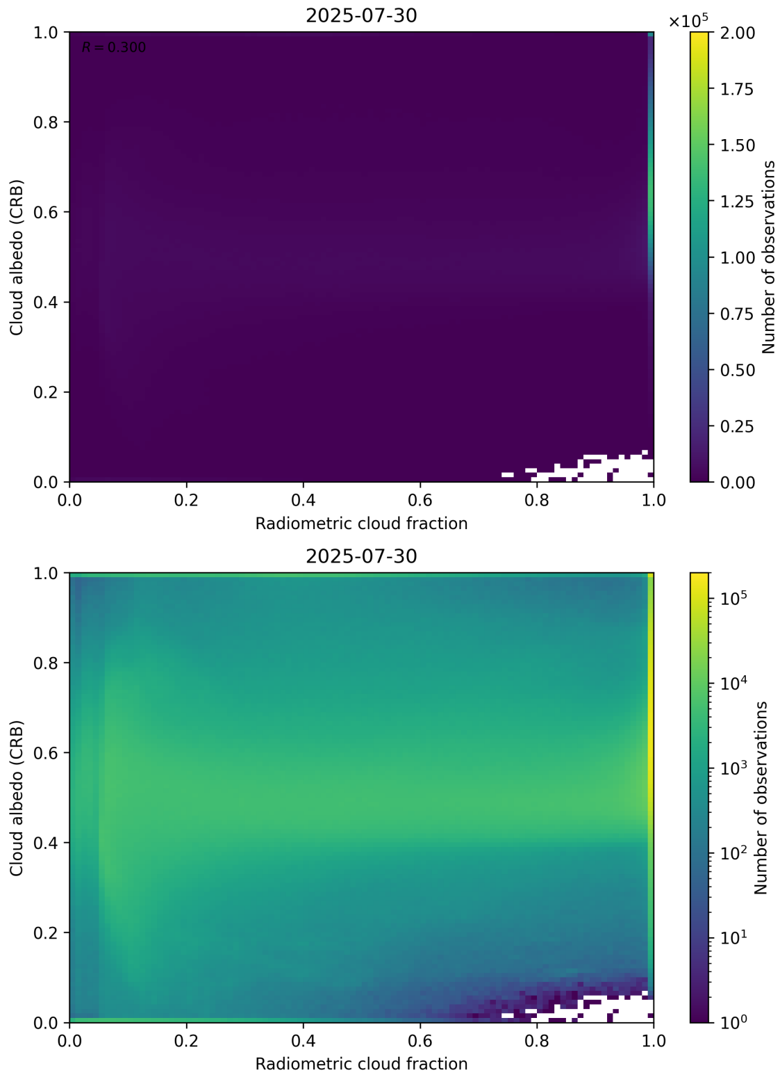
Figure 71: Scatter density plot of “Radiometric cloud fraction” against “Cloud albedo (CRB)” for 2025-07-29 to 2025-07-31.
