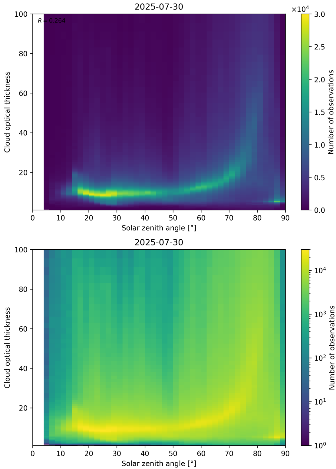
Figure 103: Scatter density plot of “Solar zenith angle” against “Cloud optical thickness” for 2025-07-29 to 2025-07-31.
