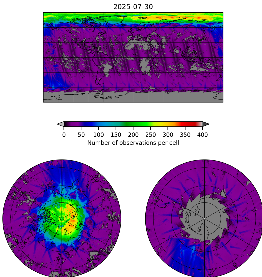
Figure 21: Map of the number of observations for 2025-07-29 to 2025-07-31
