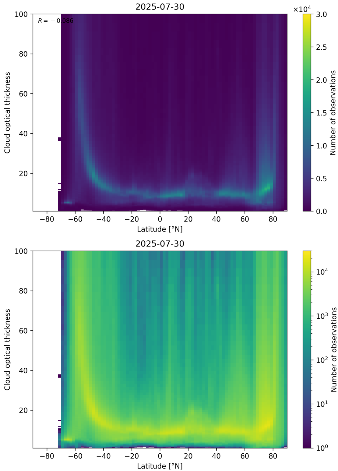
Figure 96: Scatter density plot of “Latitude” against “Cloud optical thickness” for 2025-07-29 to 2025-07-31.
