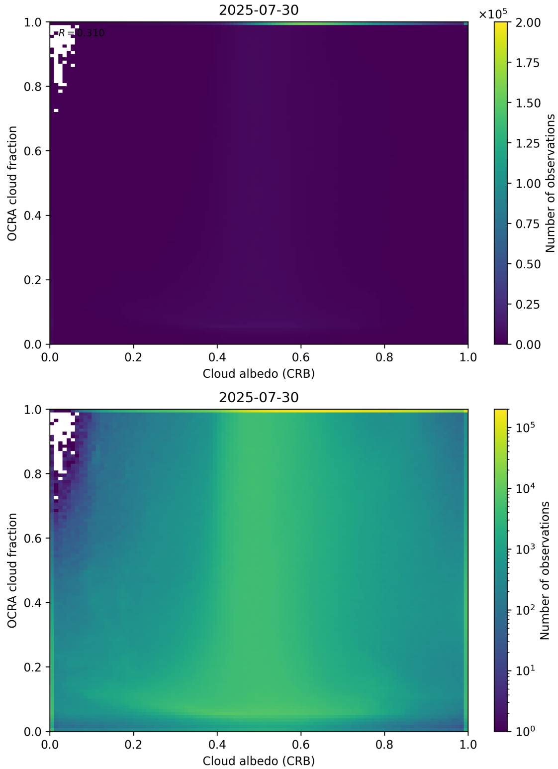
Figure 70: Scatter density plot of “Cloud albedo (CRB)” against “OCRA cloud fraction” for 2025-07-29 to 2025-07-31.
