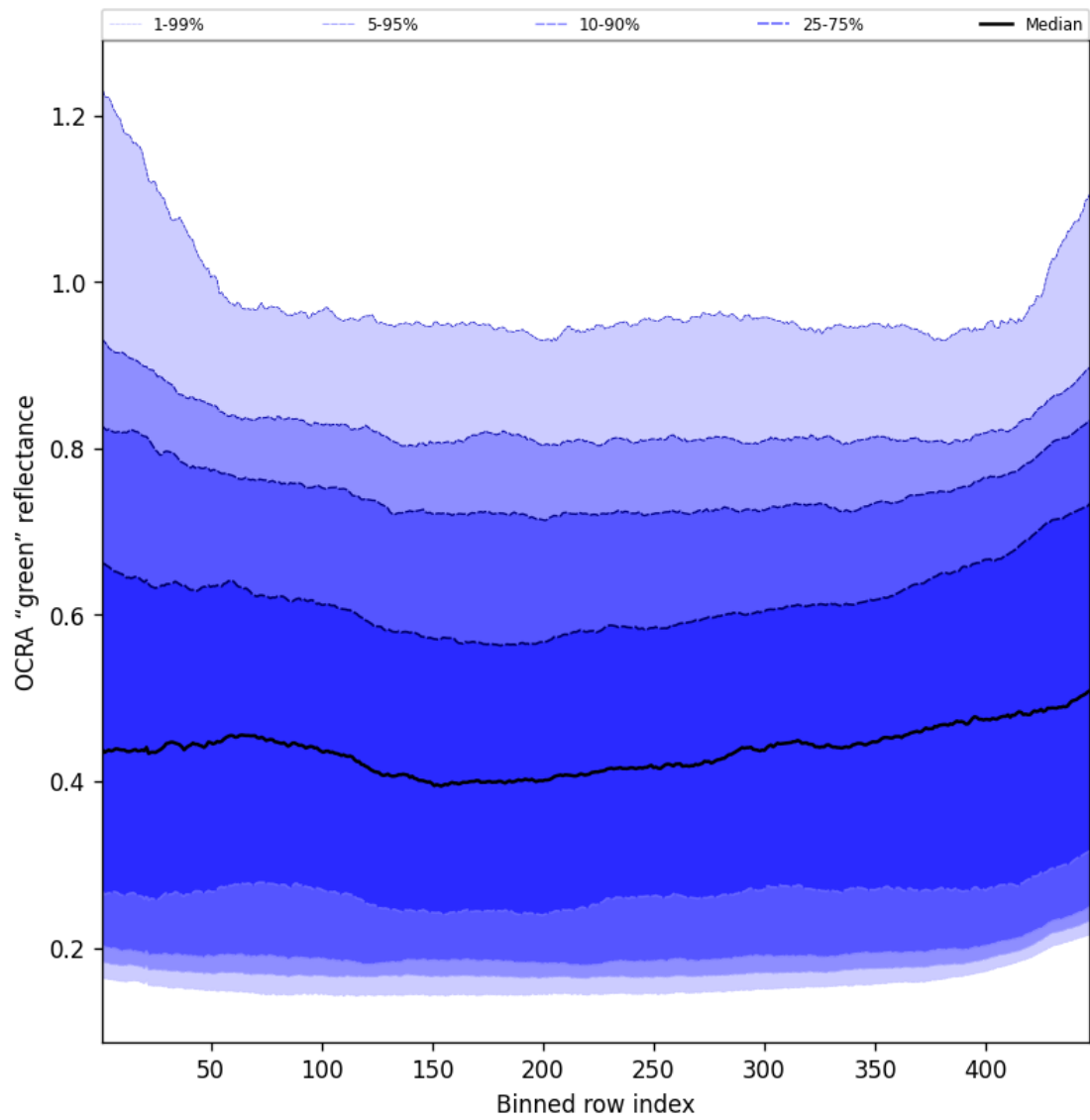
Figure 68: Along track statistics of “OCRA “green” reflectance” for 2025-07-29 to 2025-07-31
