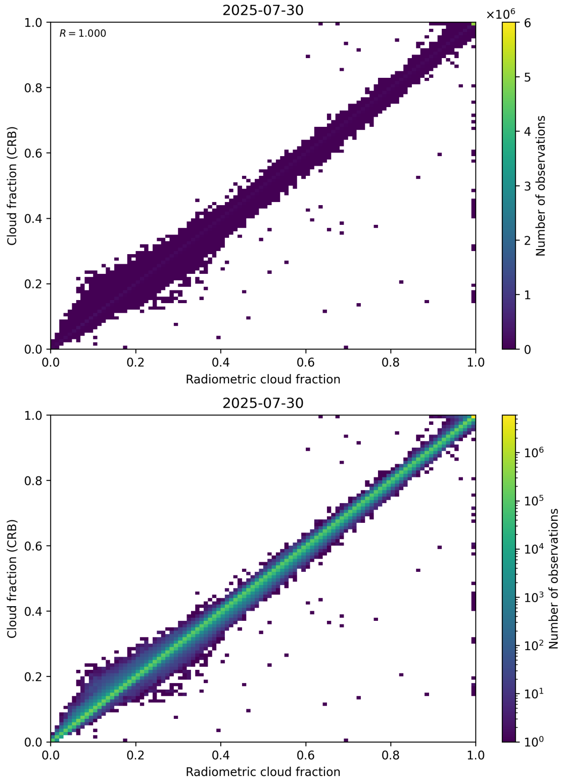
Figure 73: Scatter density plot of “Radiometric cloud fraction” against “Cloud fraction (CRB)” for 2025-07-29 to 2025-07-31.
