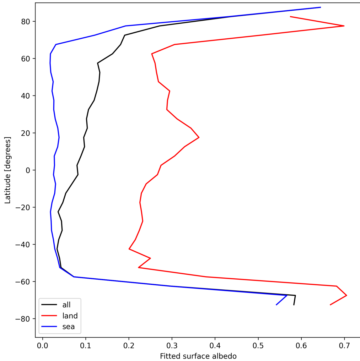
Figure 29: Zonal average of “Fitted surface albedo” for 2025-07-29 to 2025-07-31.
