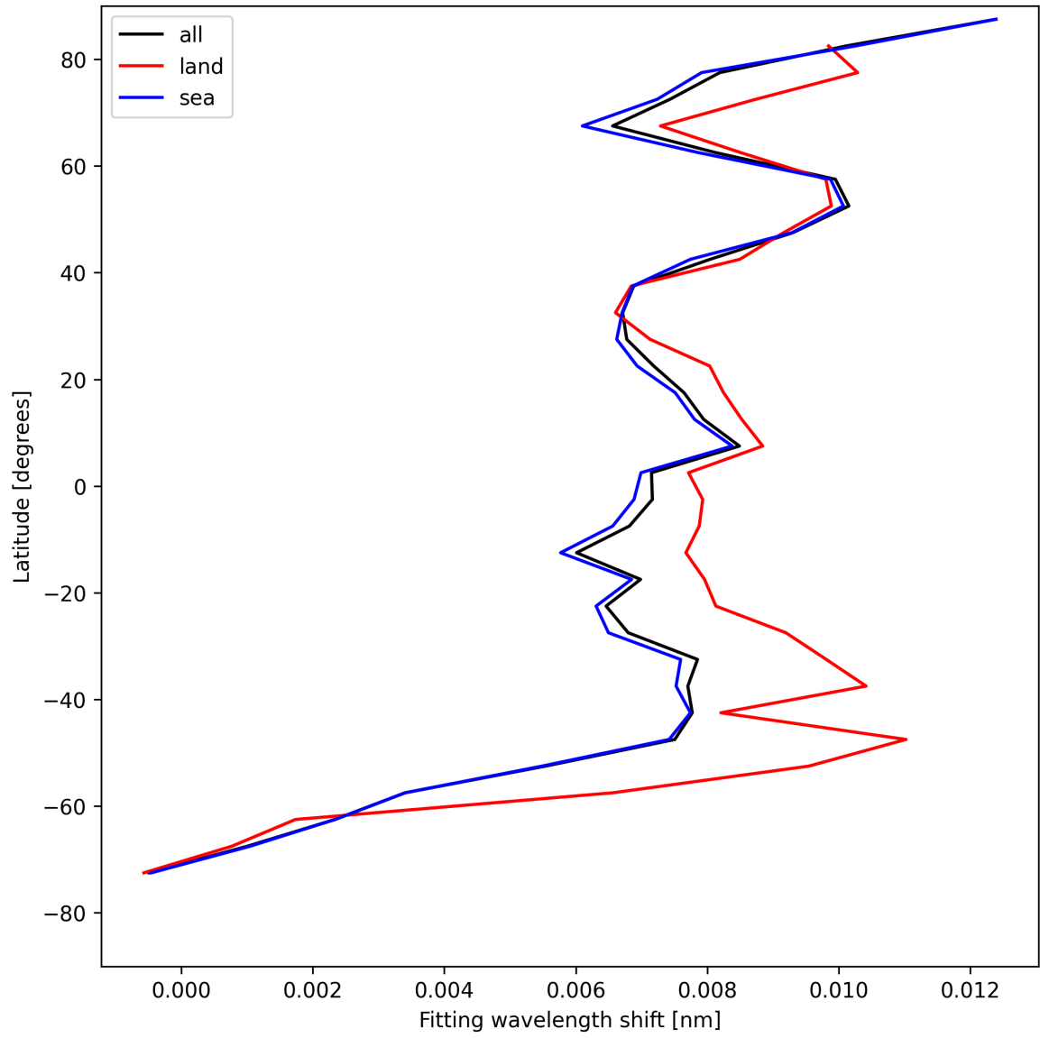
Figure 33: Zonal average of “Fitting wavelength shift” for 2025-07-29 to 2025-07-31.
