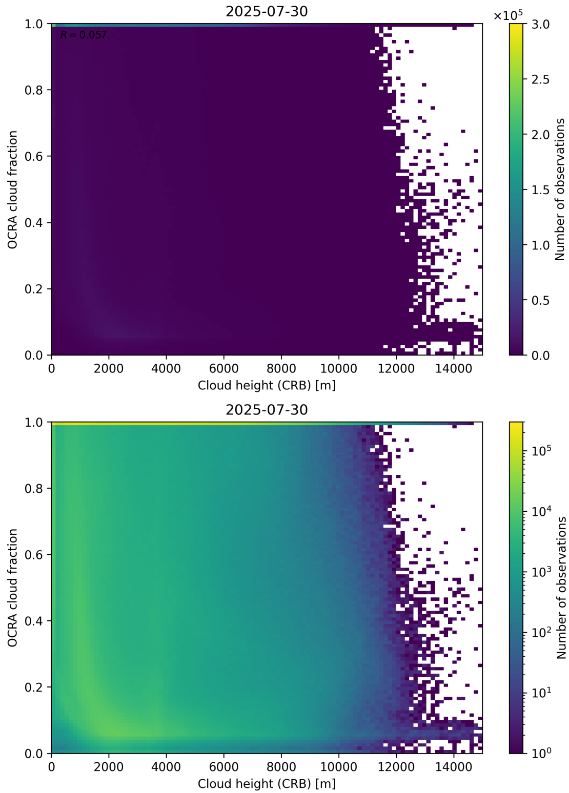
Figure 81: Scatter density plot of “Cloud height (CRB)” against “OCRA cloud fraction” for 2025-07-29 to 2025-07-31.
