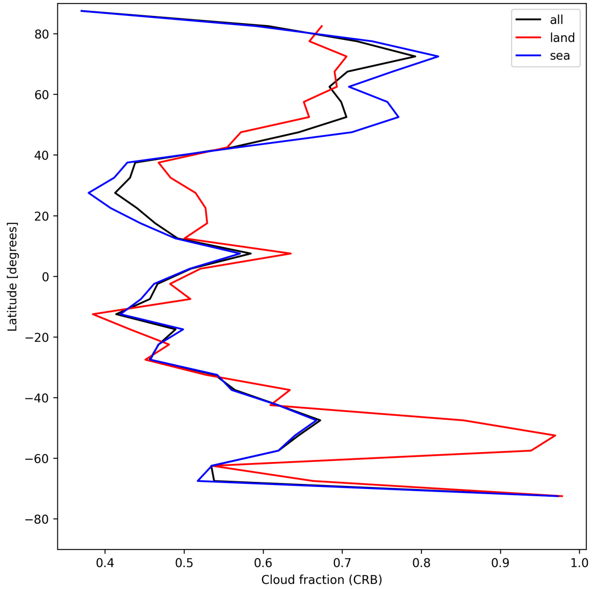
Figure 26: Zonal average of “Cloud fraction (CRB)” for 2025-07-29 to 2025-07-31.
