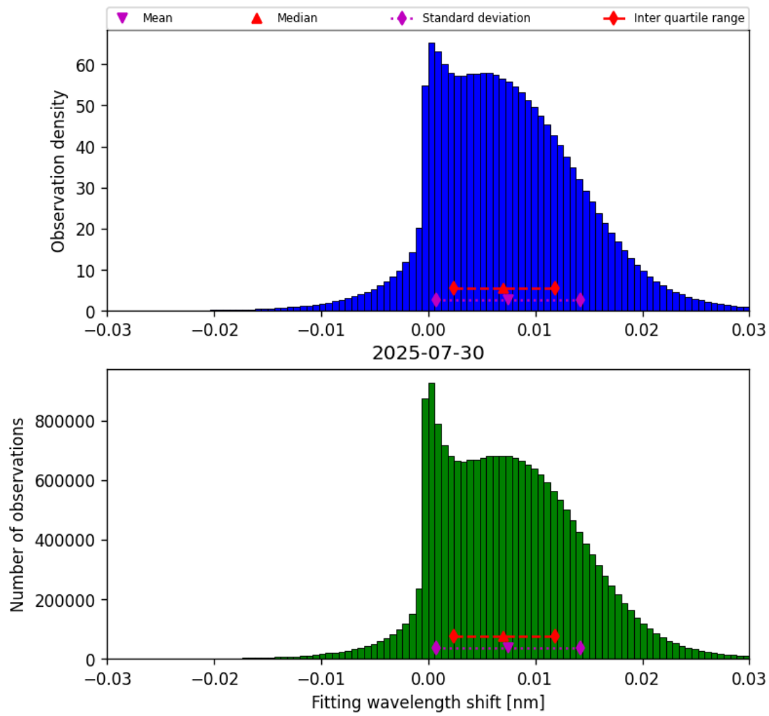
Figure 49: Histogram of “Fitting wavelength shift” for 2025-07-29 to 2025-07-31
