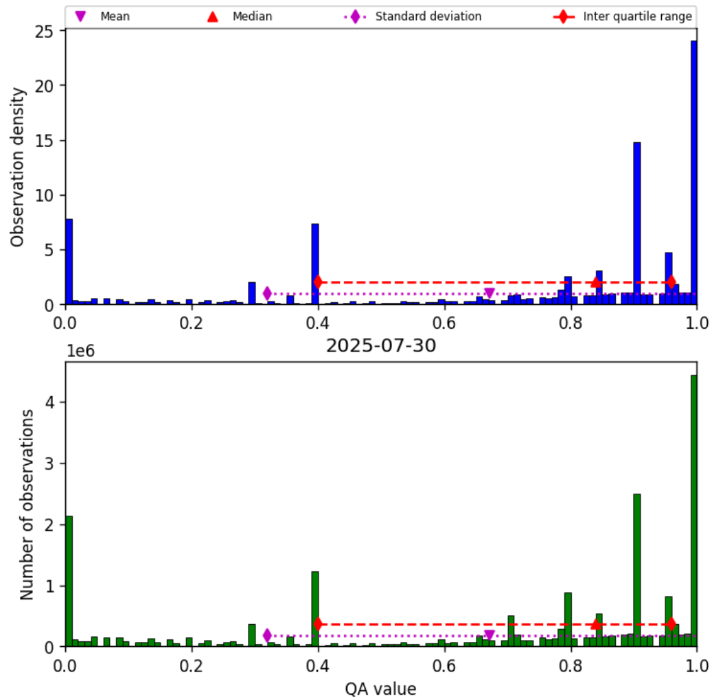
Figure 38: Histogram of “QA value” for 2025-07-29 to 2025-07-31
