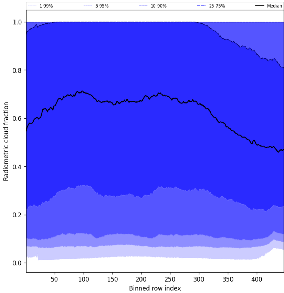
Figure 55: Along track statistics of “Radiometric cloud fraction” for 2025-07-29 to 2025-07-31
