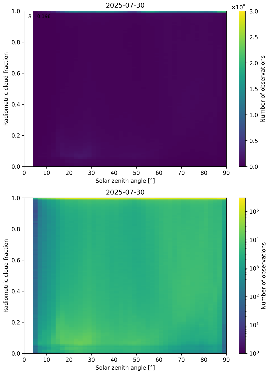
Figure 99: Scatter density plot of “Solar zenith angle” against “Radiometric cloud fraction” for 2025-07-29 to 2025-07-31.
