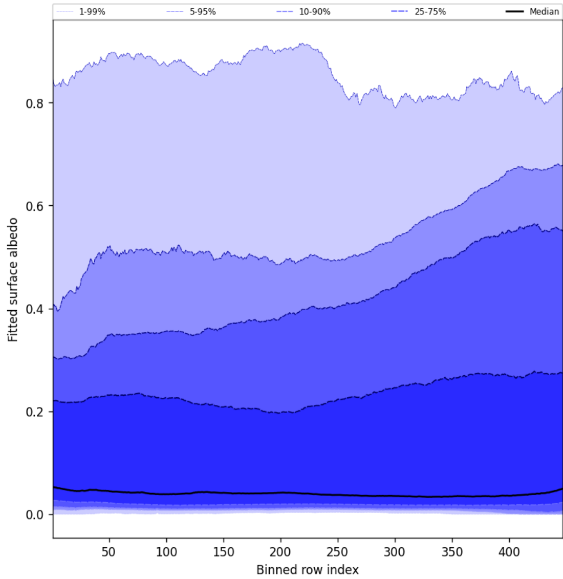
Figure 61: Along track statistics of “Fitted surface albedo” for 2025-07-29 to 2025-07-31
