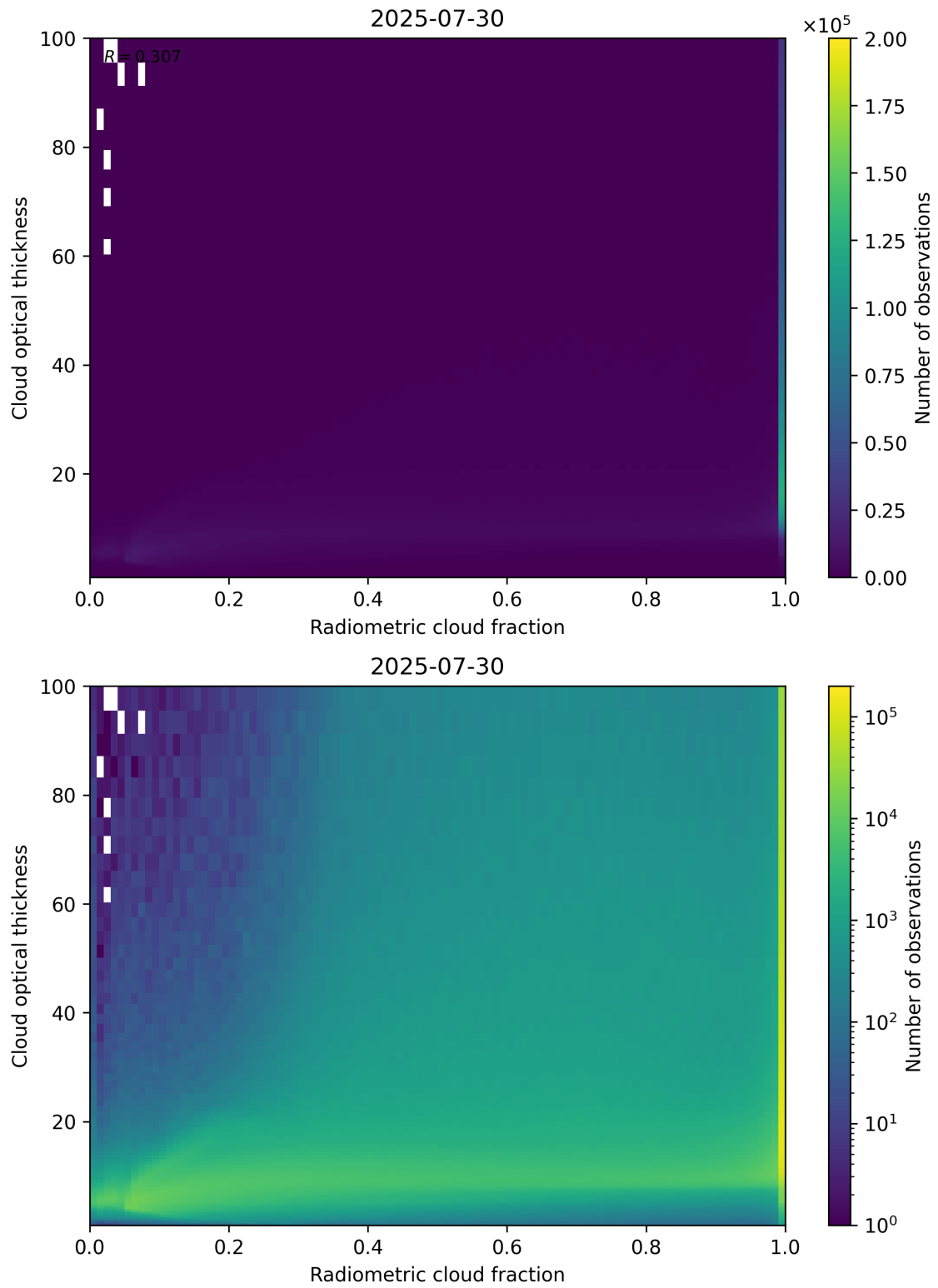
Figure 75: Scatter density plot of “Radiometric cloud fraction” against “Cloud optical thickness” for 2025-07-29 to 2025-07-31.
