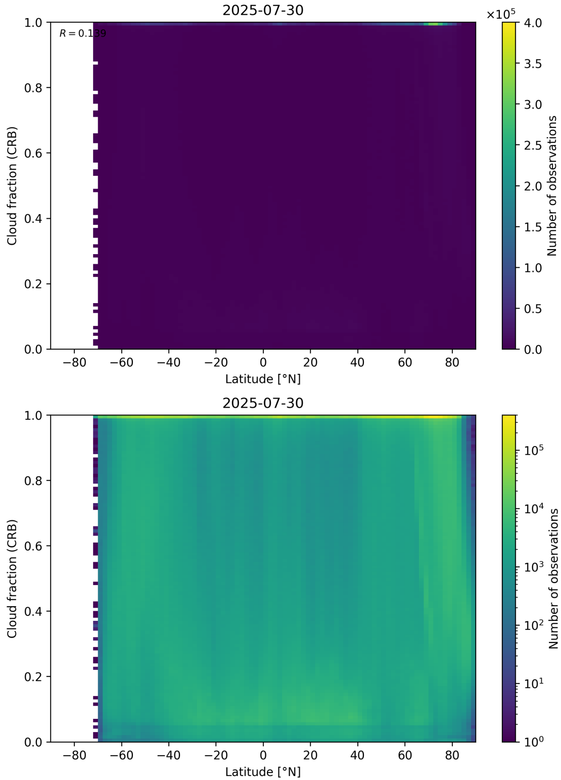
Figure 94: Scatter density plot of “Latitude” against “Cloud fraction (CRB)” for 2025-07-29 to 2025-07-31.
