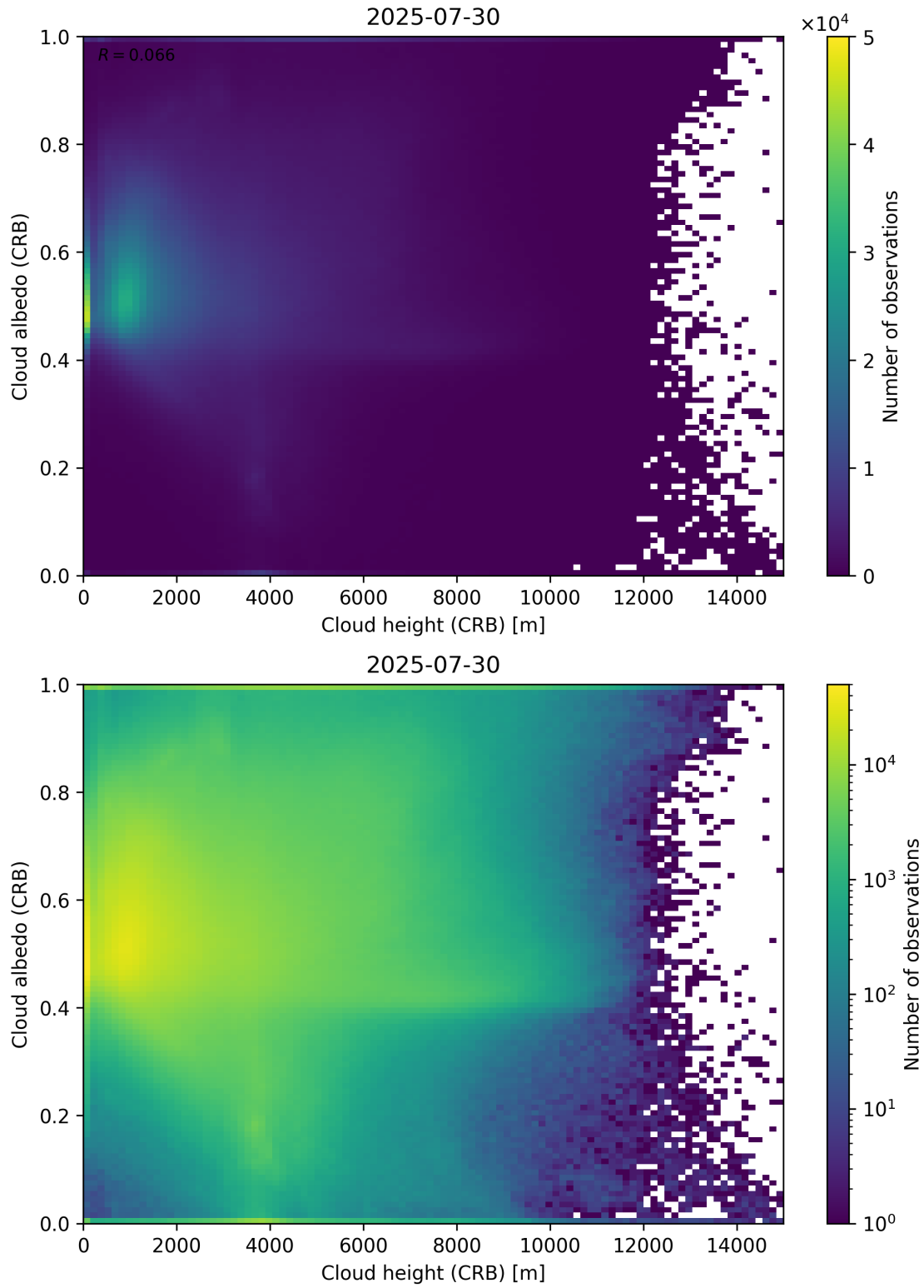
Figure 80: Scatter density plot of “Cloud height (CRB)” against “Cloud albedo (CRB)” for 2025-07-29 to 2025-07-31.
