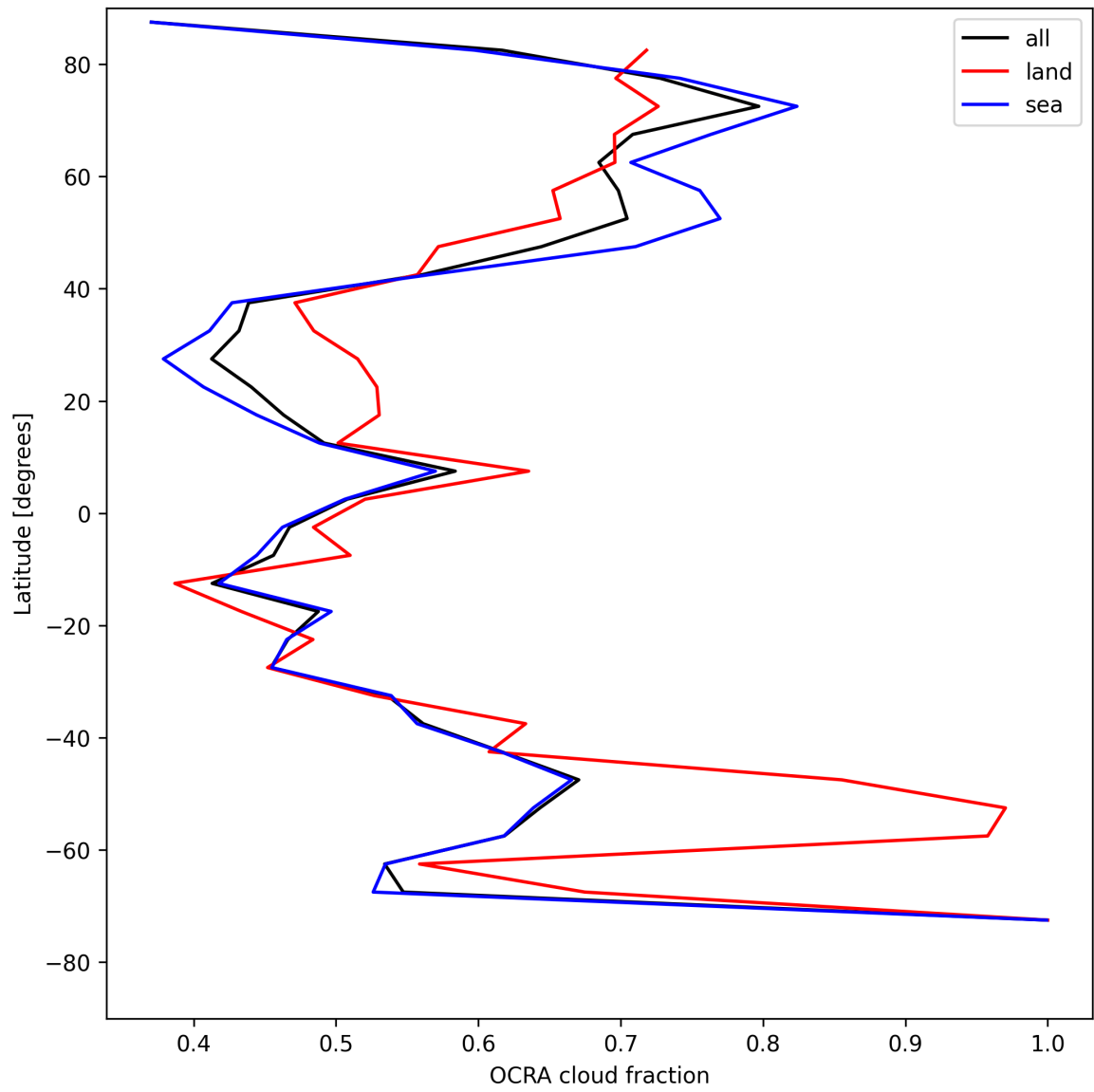
Figure 34: Zonal average of “OCRA cloud fraction” for 2025-07-29 to 2025-07-31.
