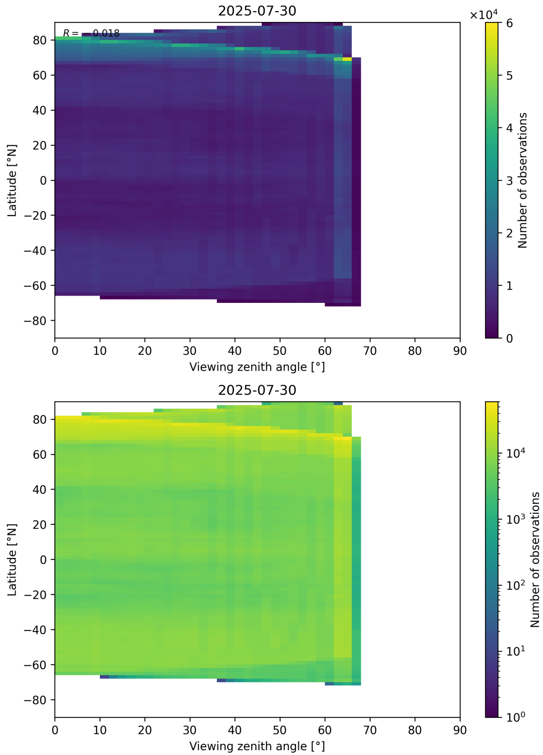
Figure 113: Scatter density plot of “Viewing zenith angle” against “Latitude” for 2025-07-29 to 2025-07-31.
