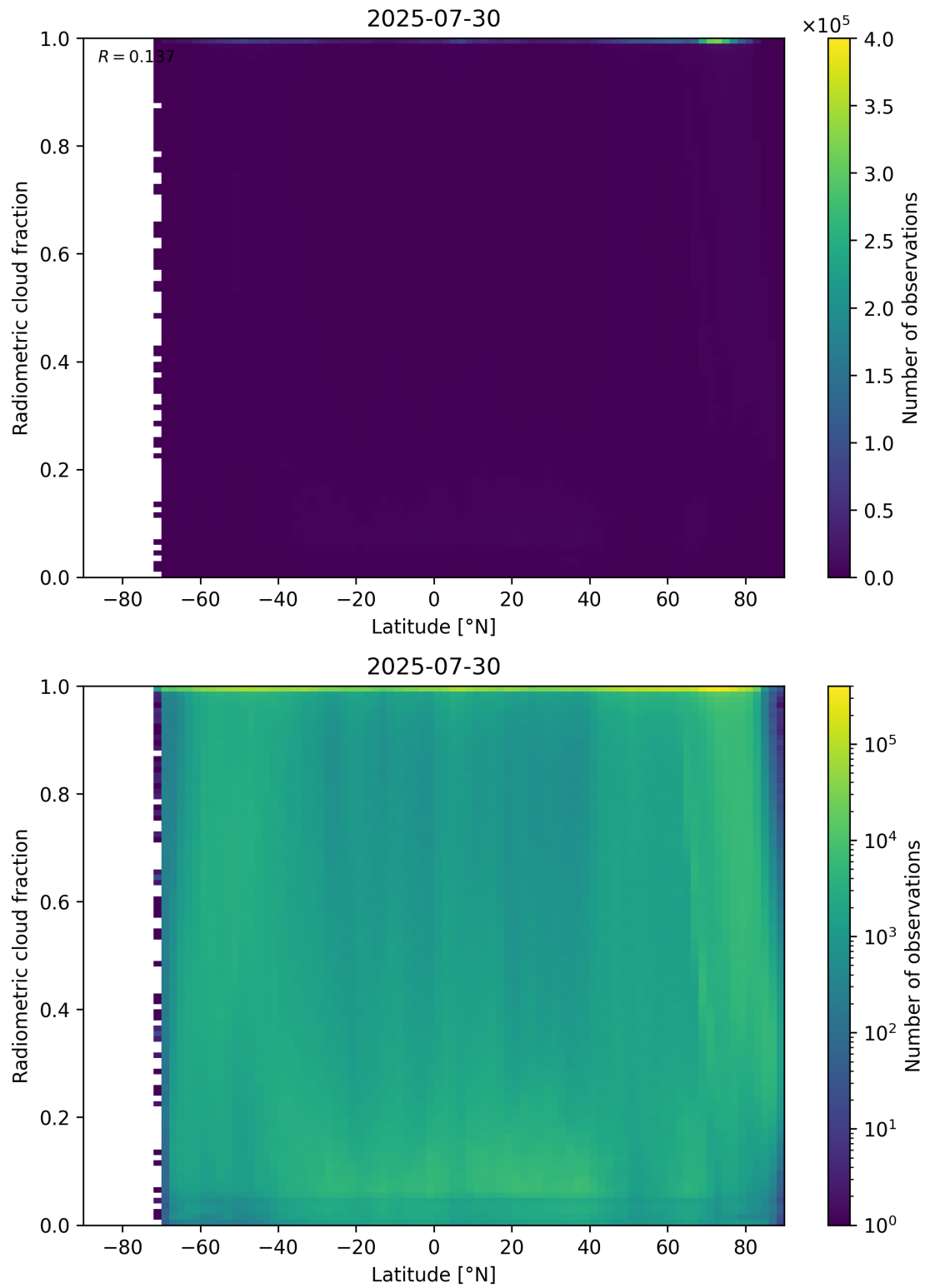
Figure 92: Scatter density plot of “Latitude” against “Radiometric cloud fraction” for 2025-07-29 to 2025-07-31.
