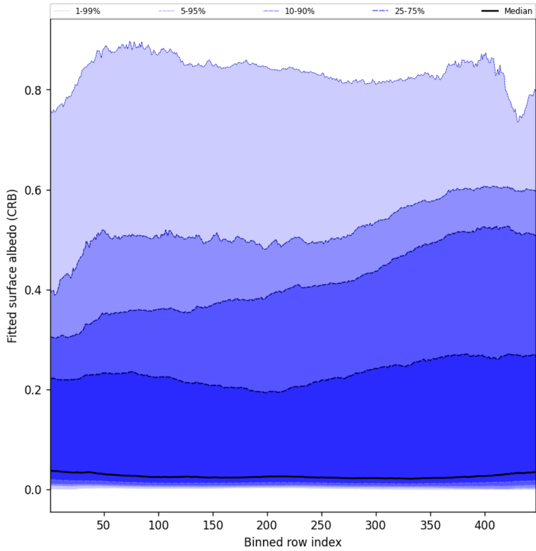
Figure 62: Along track statistics of “Fitted surface albedo (CRB)” for 2025-07-29 to 2025-07-31
