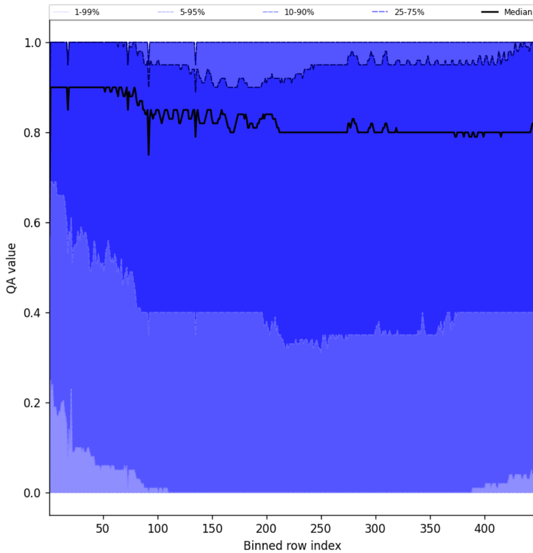
Figure 54: Along track statistics of “QA value” for 2025-07-29 to 2025-07-31
