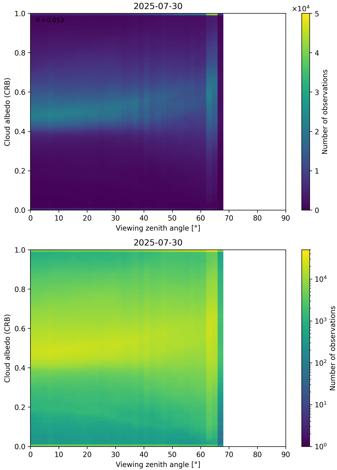
Figure 106: Scatter density plot of “Viewing zenith angle” against “Cloud albedo (CRB)” for 2025-07-29 to 2025-07-31.
