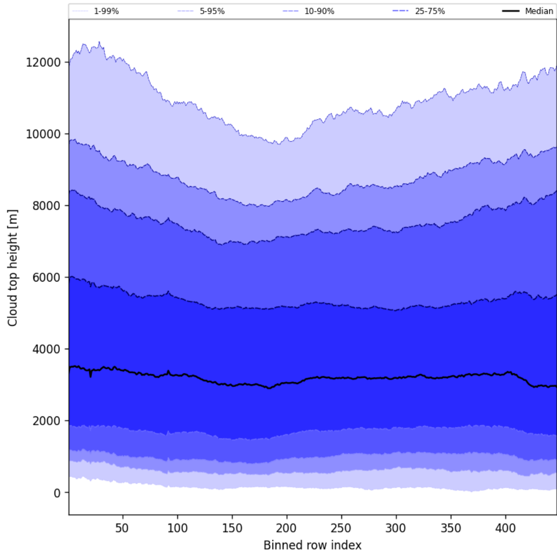
Figure 56: Along track statistics of "Cloud top height" for 2025-07-29 to 2025-07-31
