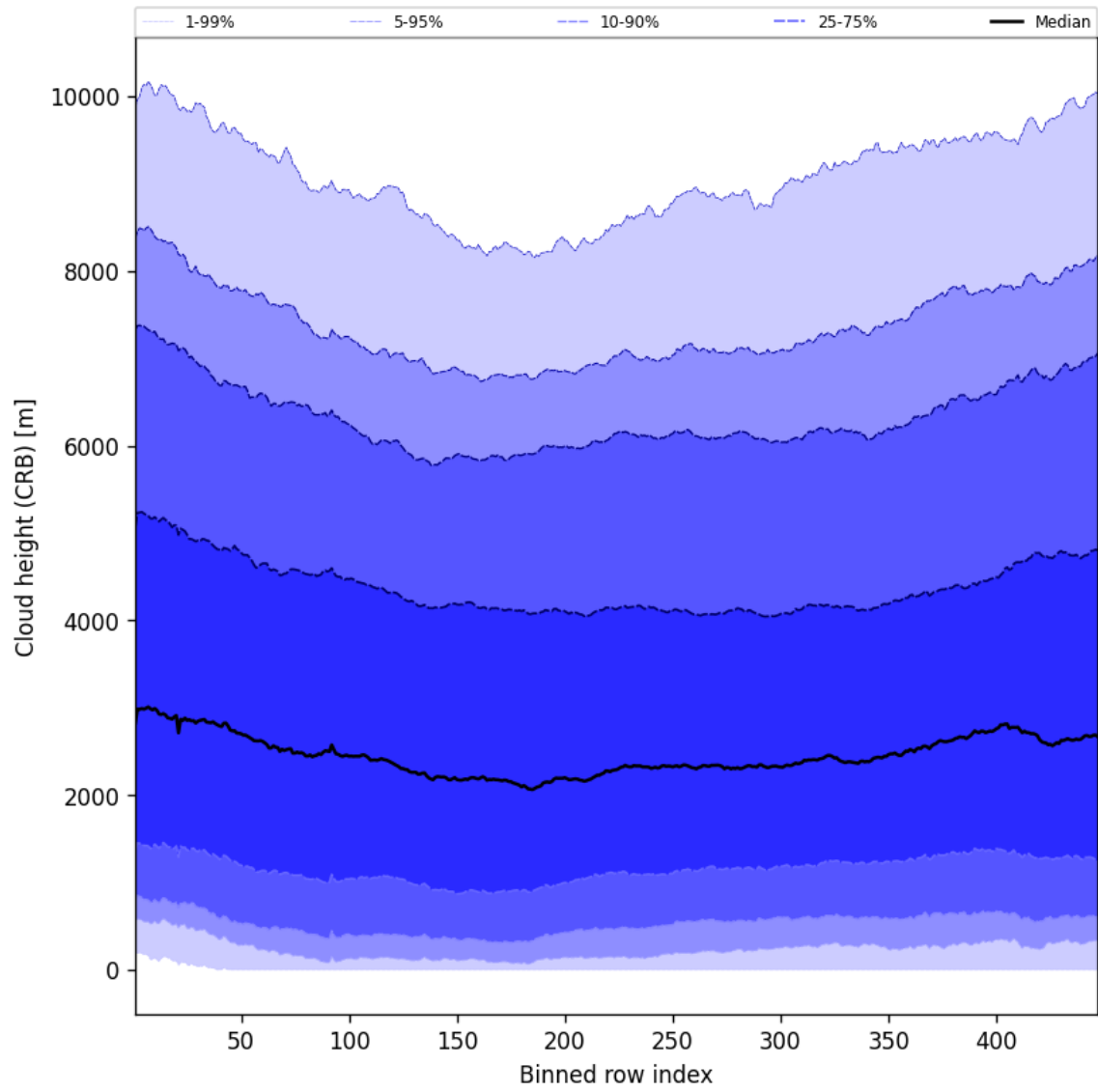
Figure 59: Along track statistics of “Cloud height (CRB)” for 2025-07-29 to 2025-07-31
