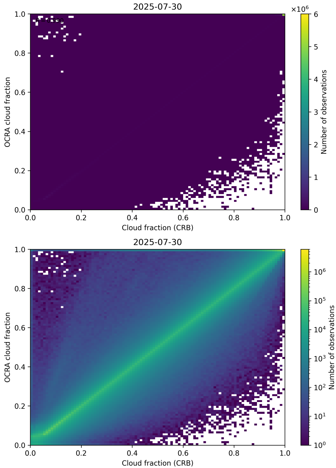
Figure 78: Scatter density plot of “Cloud fraction (CRB)” against “OCRA cloud fraction” for 2025-07-29 to 2025-07-31.
