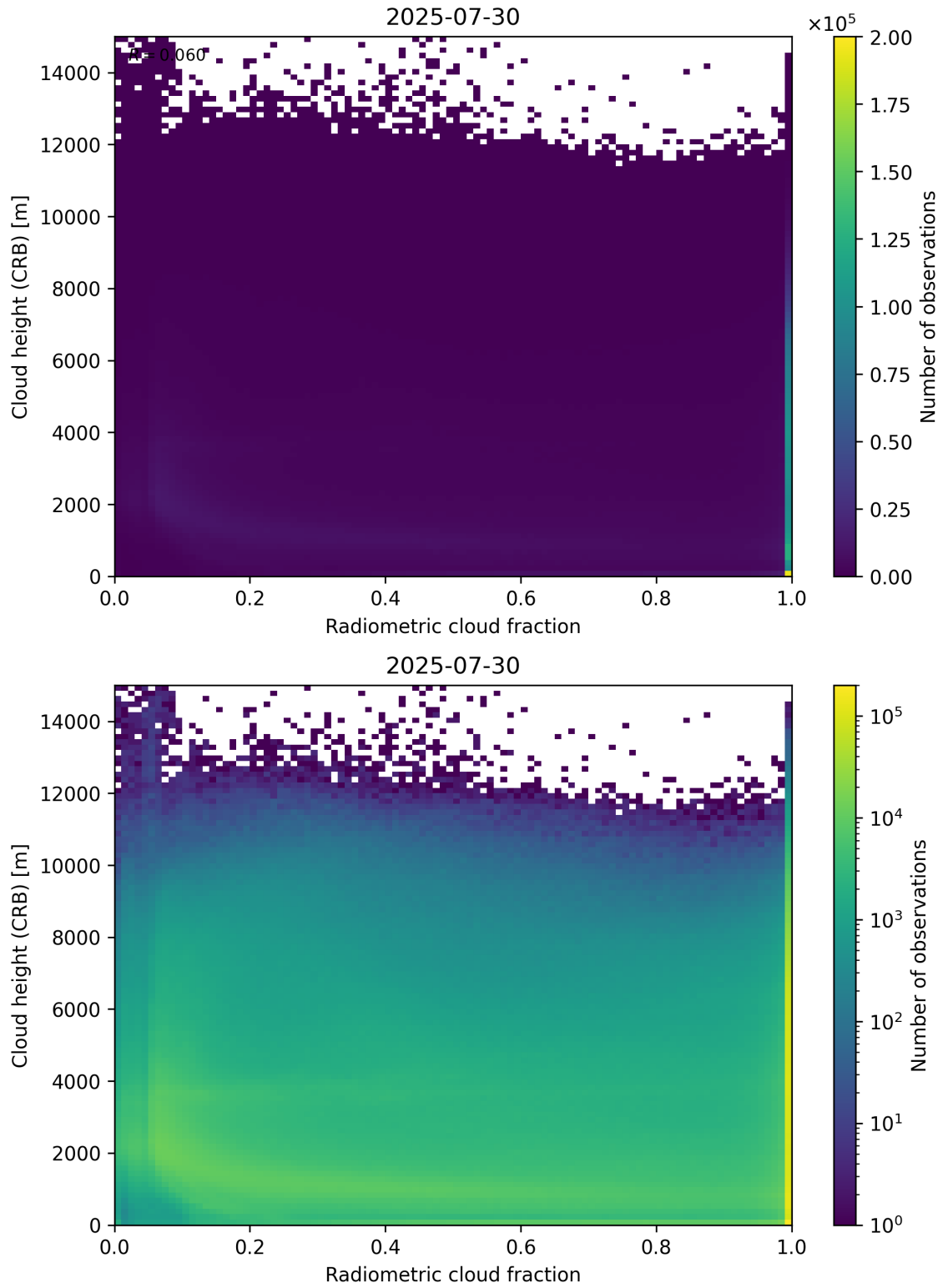
Figure 74: Scatter density plot of “Radiometric cloud fraction” against “Cloud height (CRB)” for 2025-07-29 to 2025-07-31.
