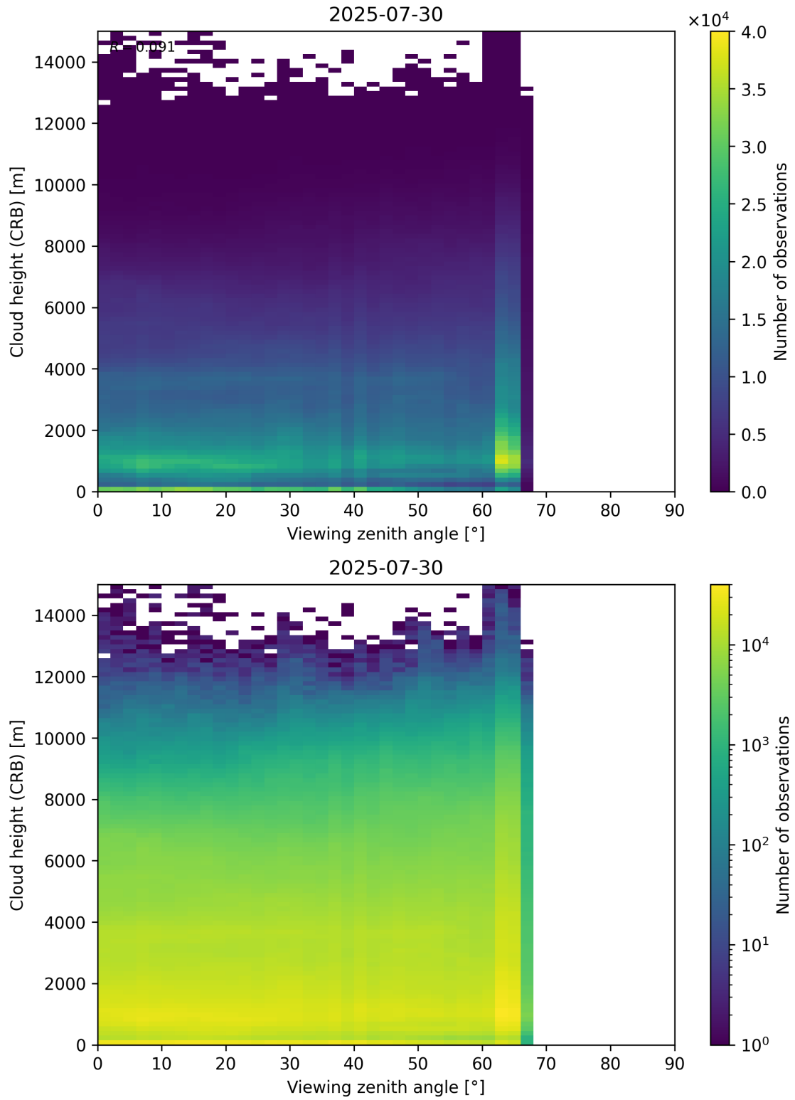
Figure 110: Scatter density plot of “Viewing zenith angle” against “Cloud height (CRB)” for 2025-07-29 to 2025-07-31.
