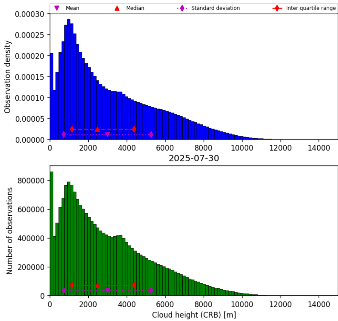
Figure 43: Histogram of “Cloud height (CRB)” for 2025-07-29 to 2025-07-31
