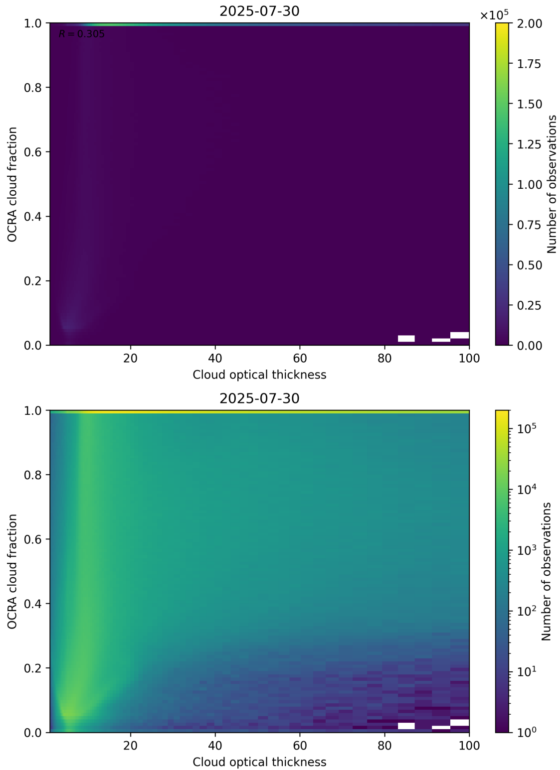
Figure 83: Scatter density plot of “Cloud optical thickness” against “OCRA cloud fraction” for 2025-07-29 to 2025-07-31.
