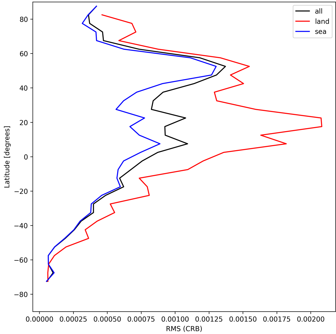
Figure 32: Zonal average of “RMS (CRB)” for 2025-07-29 to 2025-07-31.
