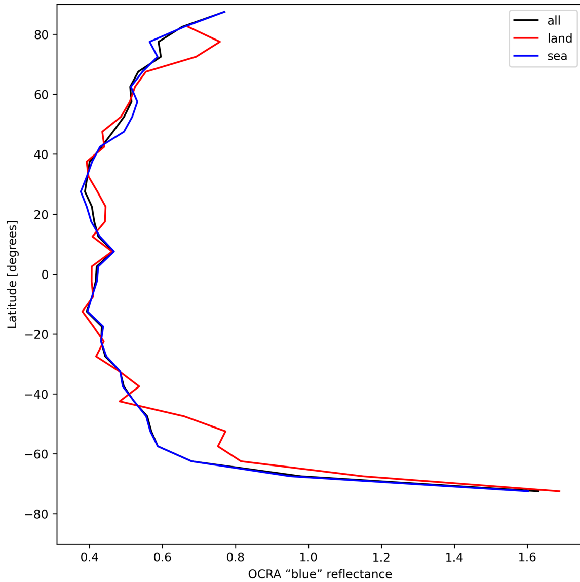
Figure 35: Zonal average of “OCRA “blue” reflectance” for 2025-07-29 to 2025-07-31.
