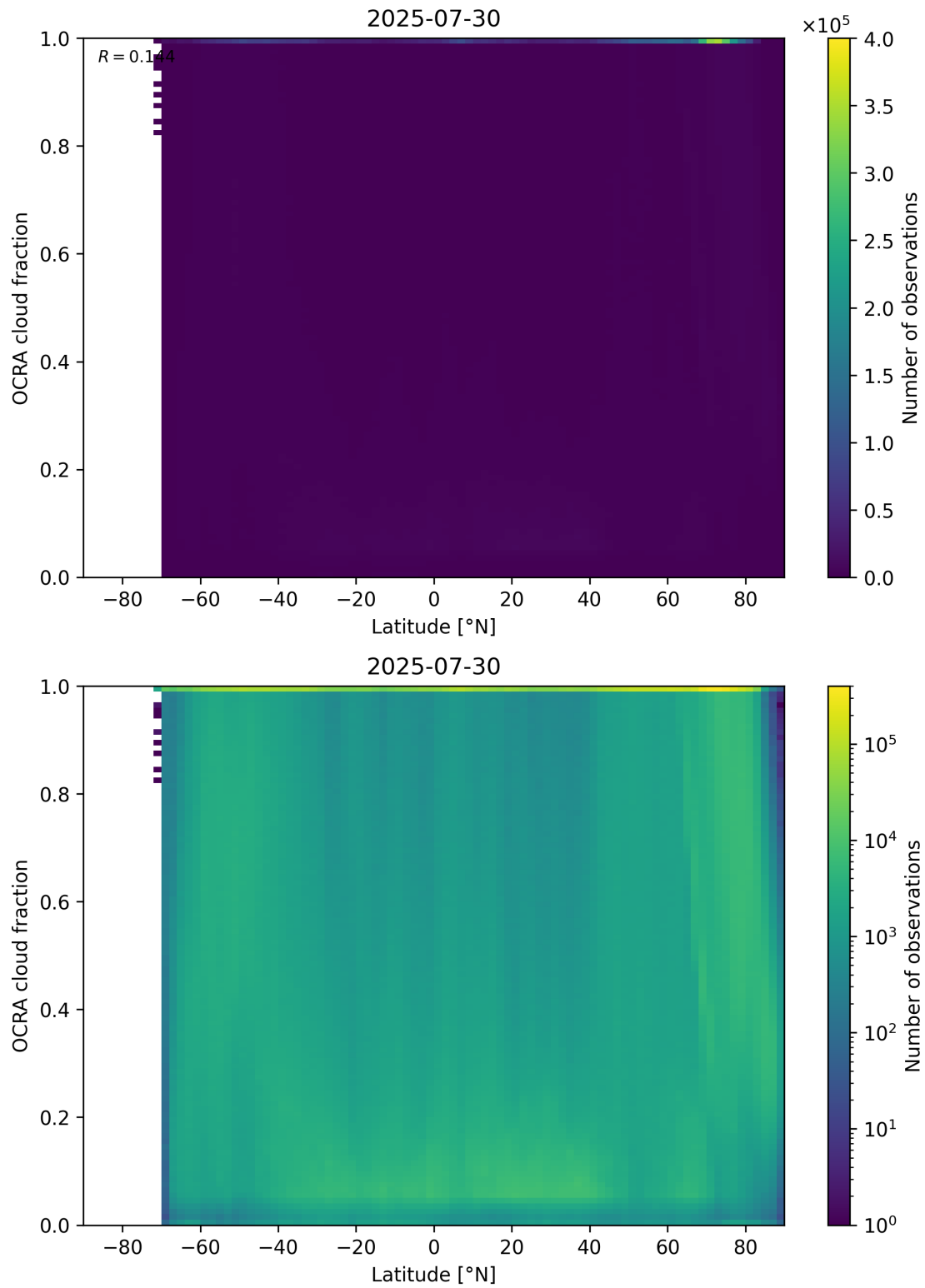
Figure 93: Scatter density plot of “Latitude” against “OCRA cloud fraction” for 2025-07-29 to 2025-07-31.
