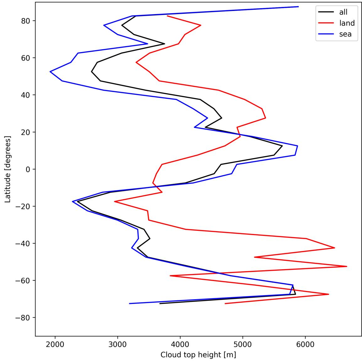
Figure 24: Zonal average of “Cloud top height” for 2025-07-29 to 2025-07-31.
