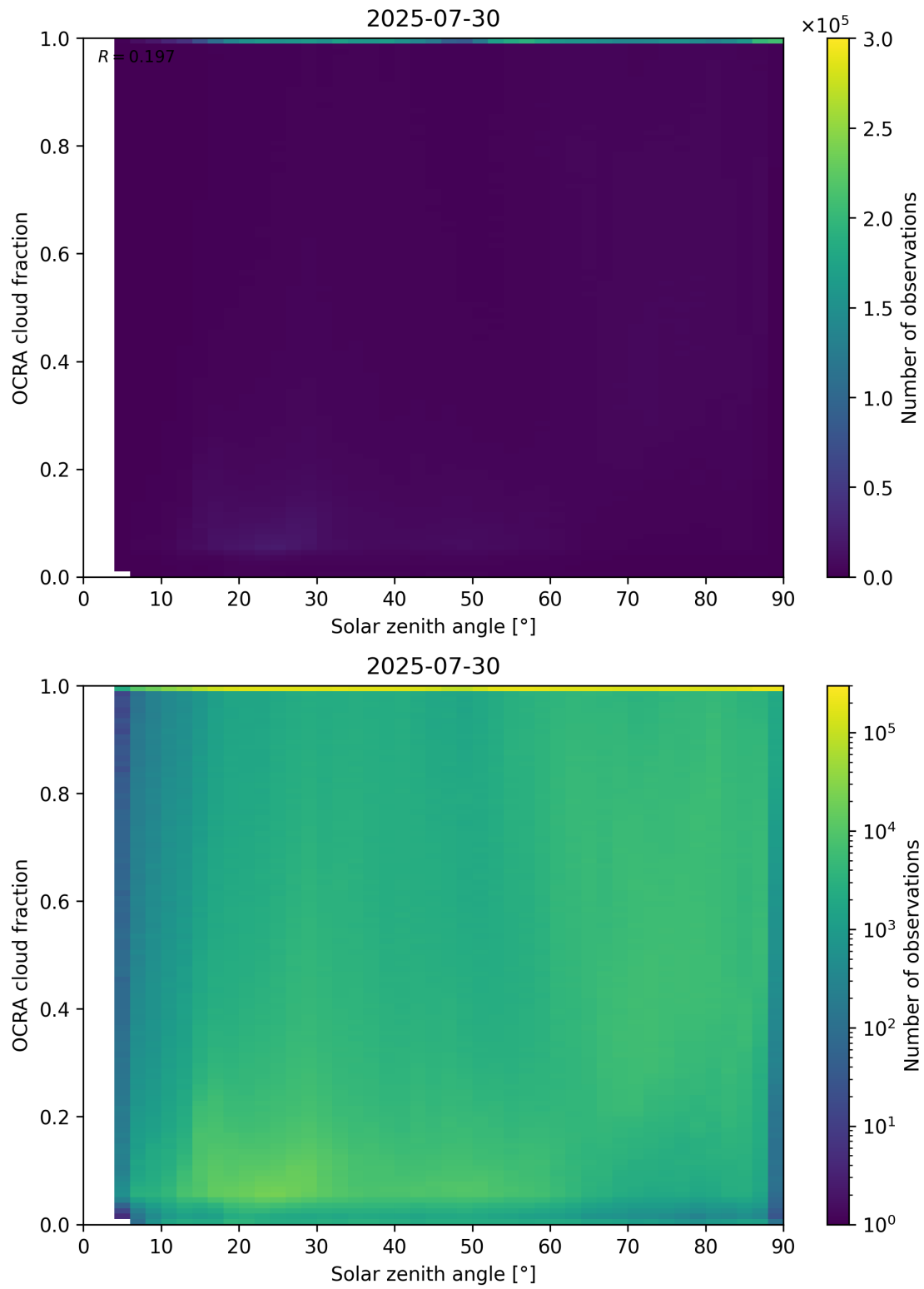
Figure 100: Scatter density plot of “Solar zenith angle” against “OCRA cloud fraction” for 2025-07-29 to 2025-07-31.
