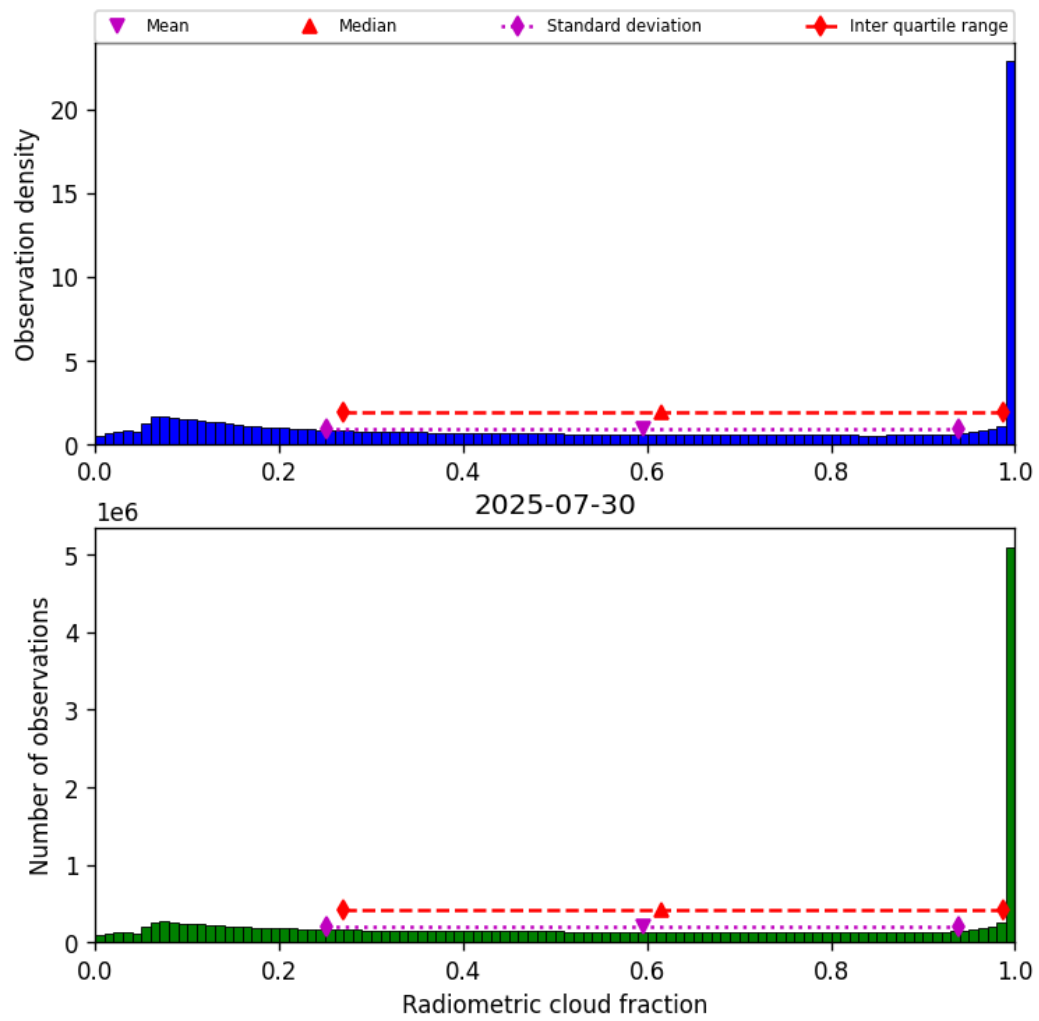
Figure 39: Histogram of “Radiometric cloud fraction” for 2025-07-29 to 2025-07-31
