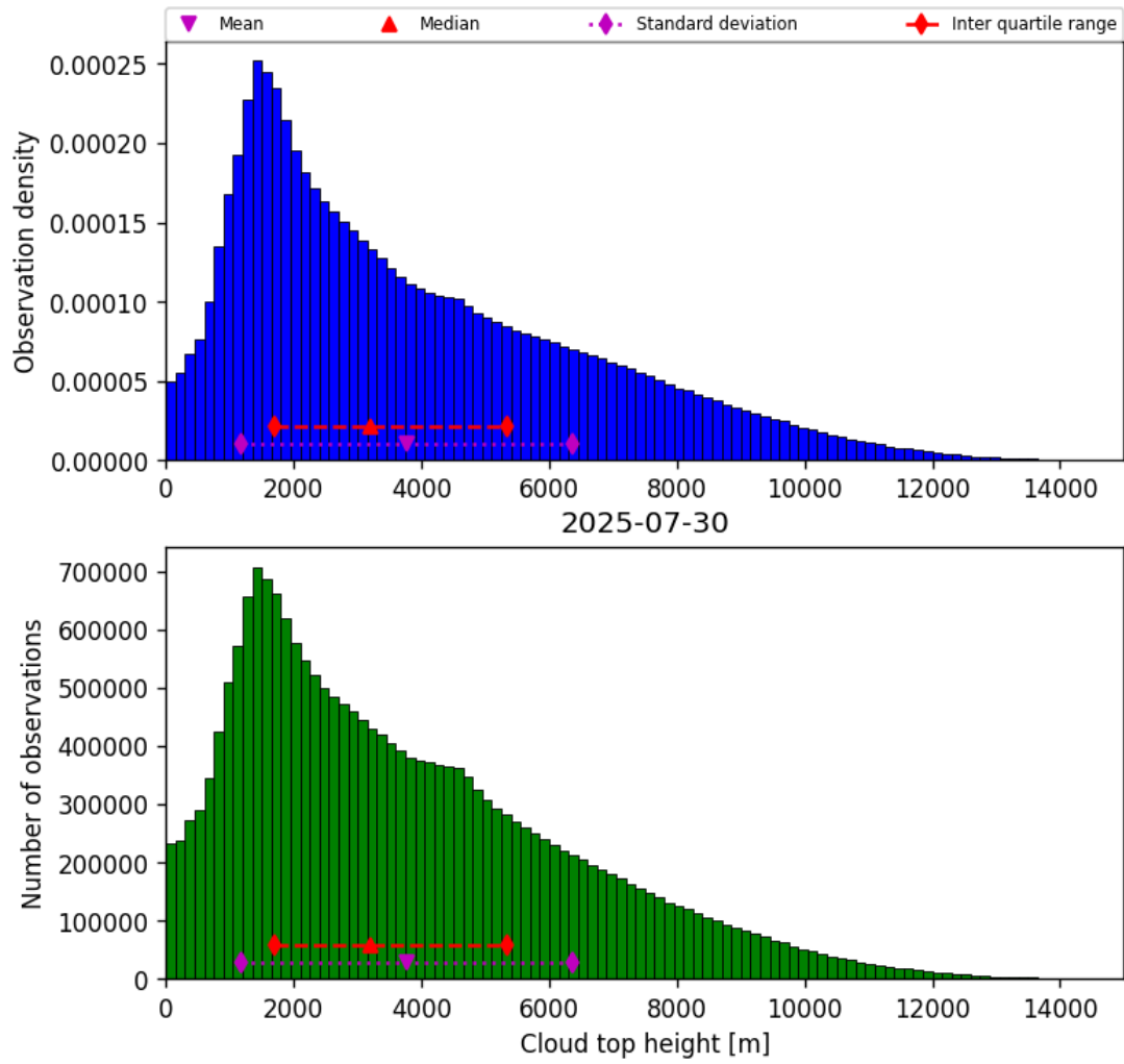
Figure 40: Histogram of “Cloud top height” for 2025-07-29 to 2025-07-31
