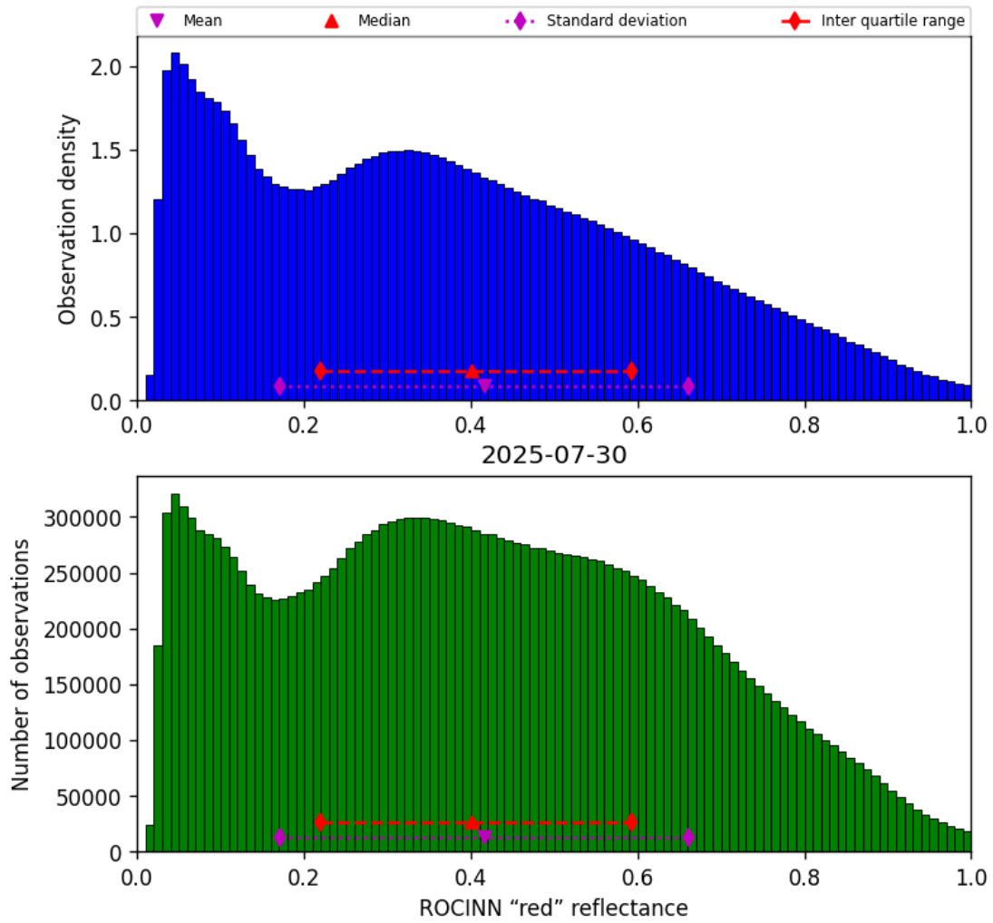
Figure 53: Histogram of “ROCINN “red” reflectance” for 2025-07-29 to 2025-07-31
