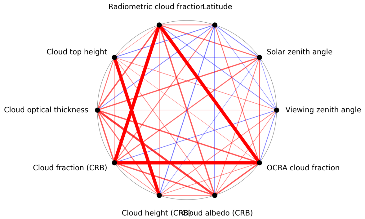
Figure 1: Map of correlation graph for 2025-07-29 to 2025-07-31.
