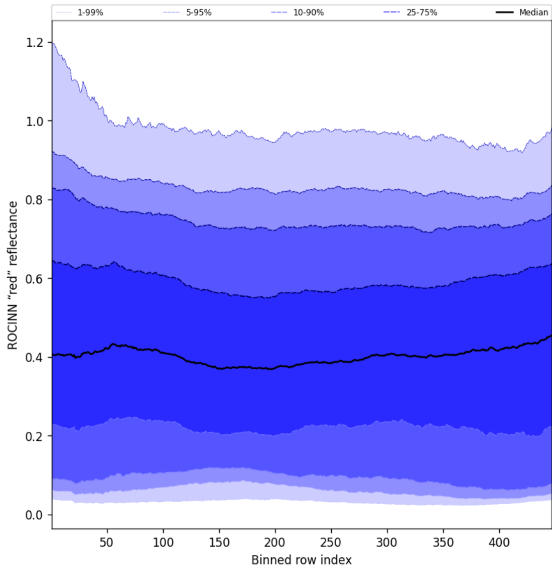
Figure 69: Along track statistics of “ROCINN “red” reflectance” for 2025-07-29 to 2025-07-31
