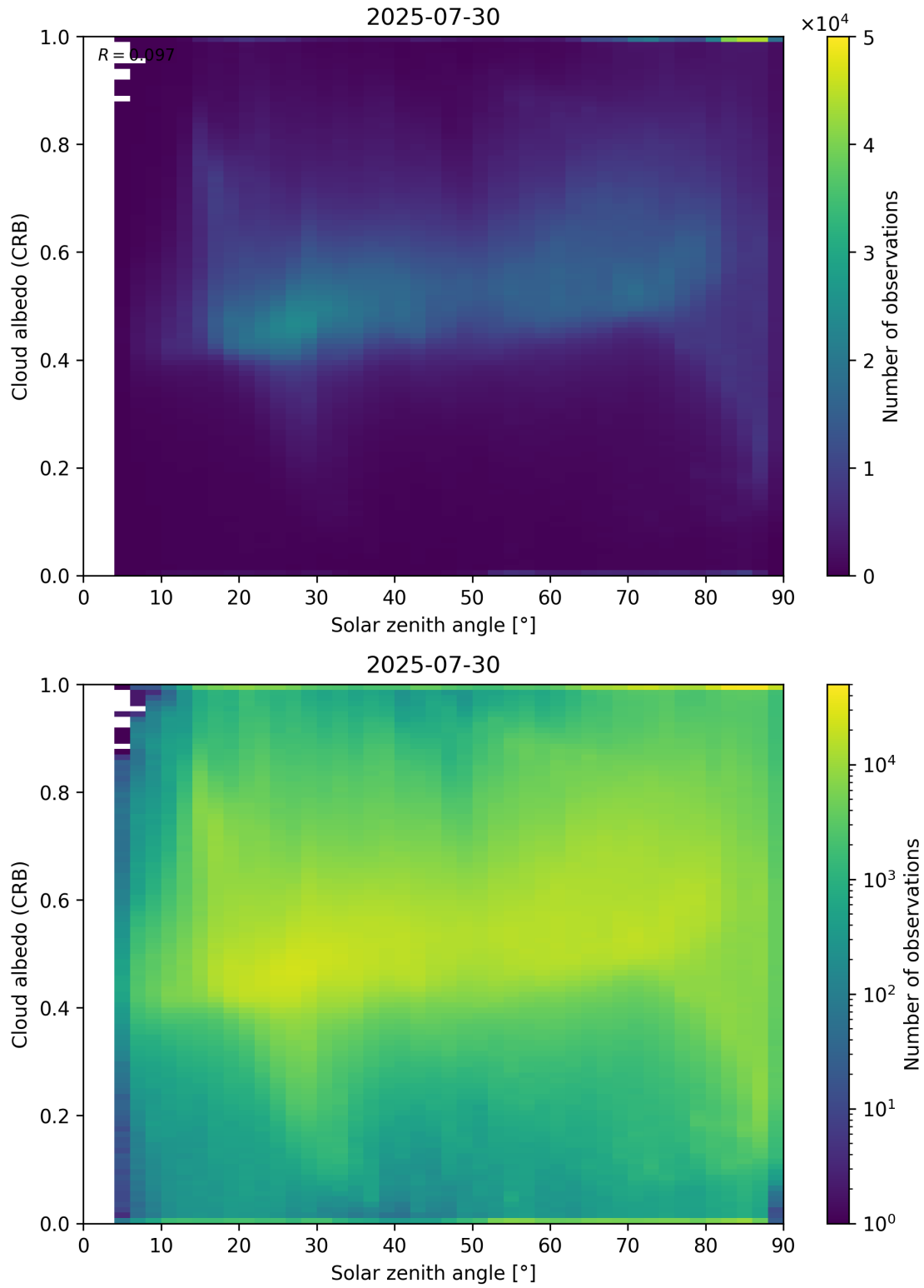
Figure 98: Scatter density plot of “Solar zenith angle” against “Cloud albedo (CRB)” for 2025-07-29 to 2025-07-31.
