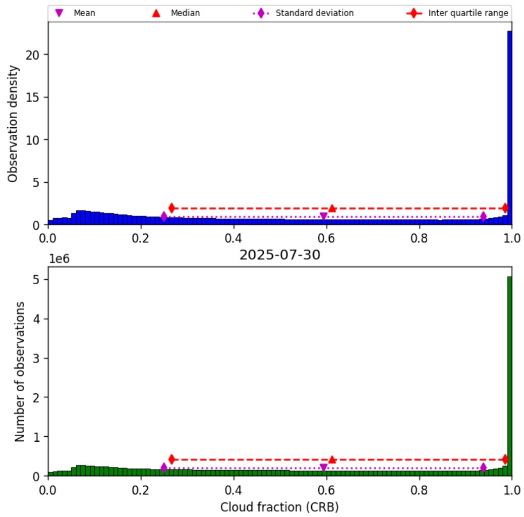
Figure 42: Histogram of “Cloud fraction (CRB)” for 2025-07-29 to 2025-07-31
