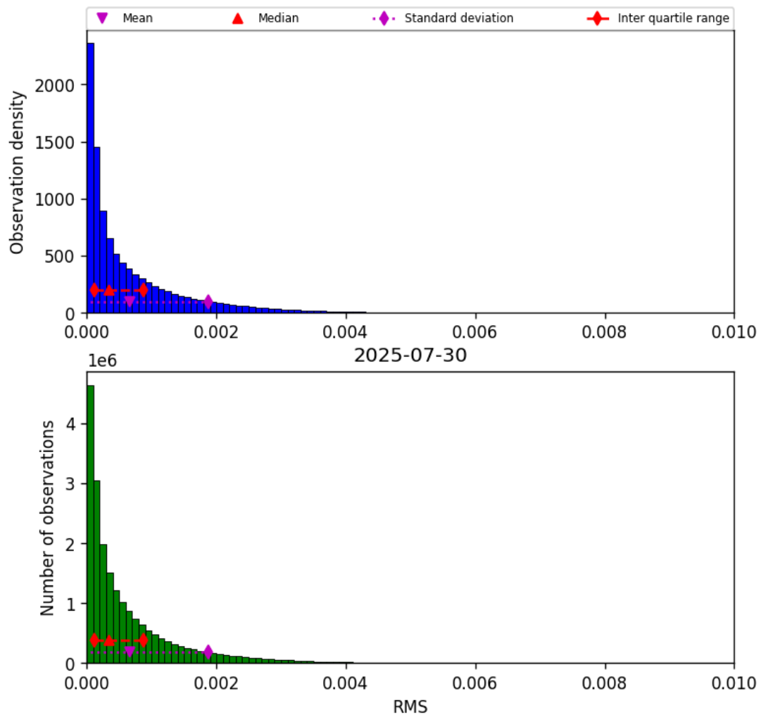
Figure 47: Histogram of “RMS” for 2025-07-29 to 2025-07-31
