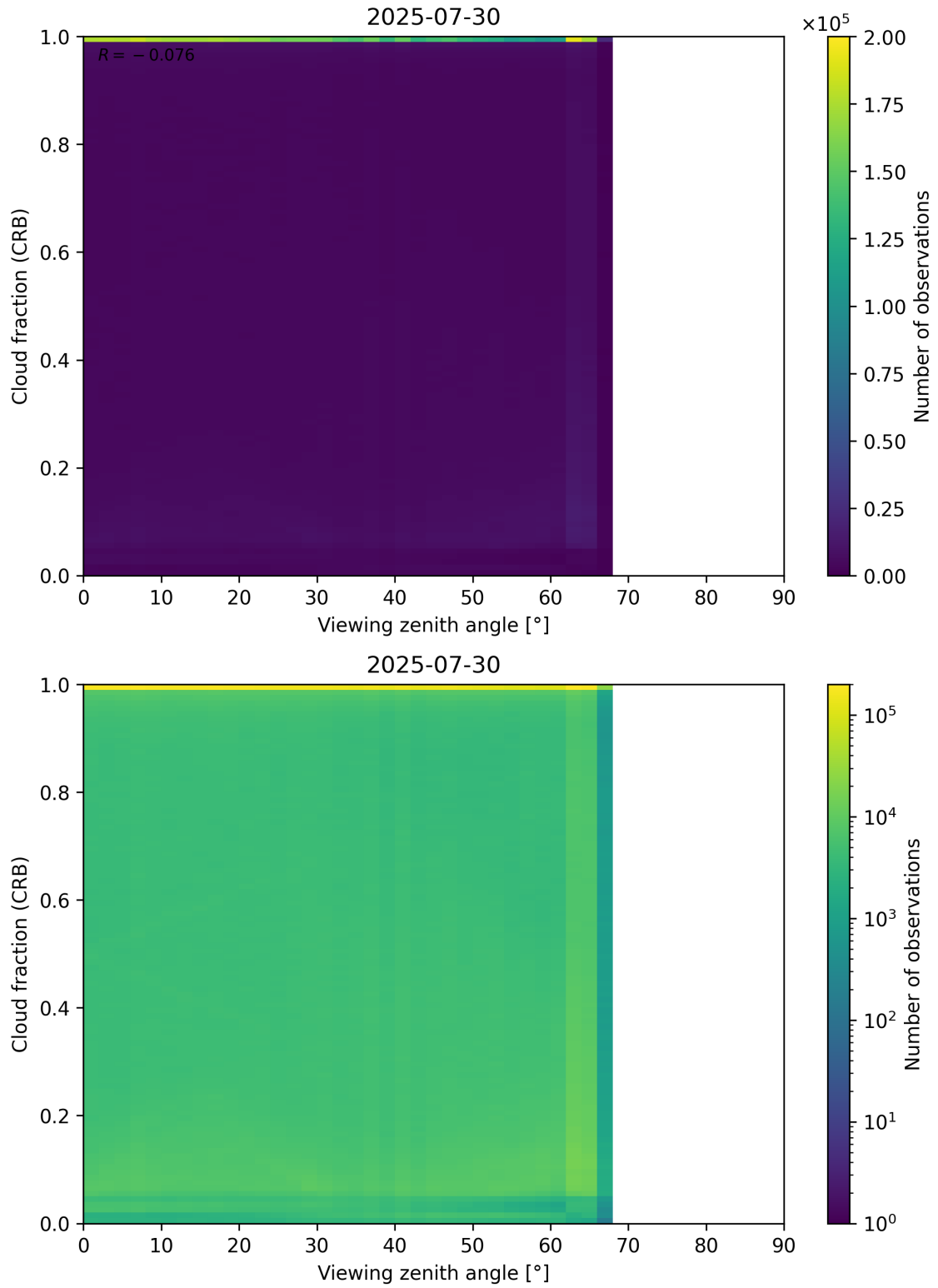
Figure 109: Scatter density plot of “Viewing zenith angle” against “Cloud fraction (CRB)” for 2025-07-29 to 2025-07-31.
