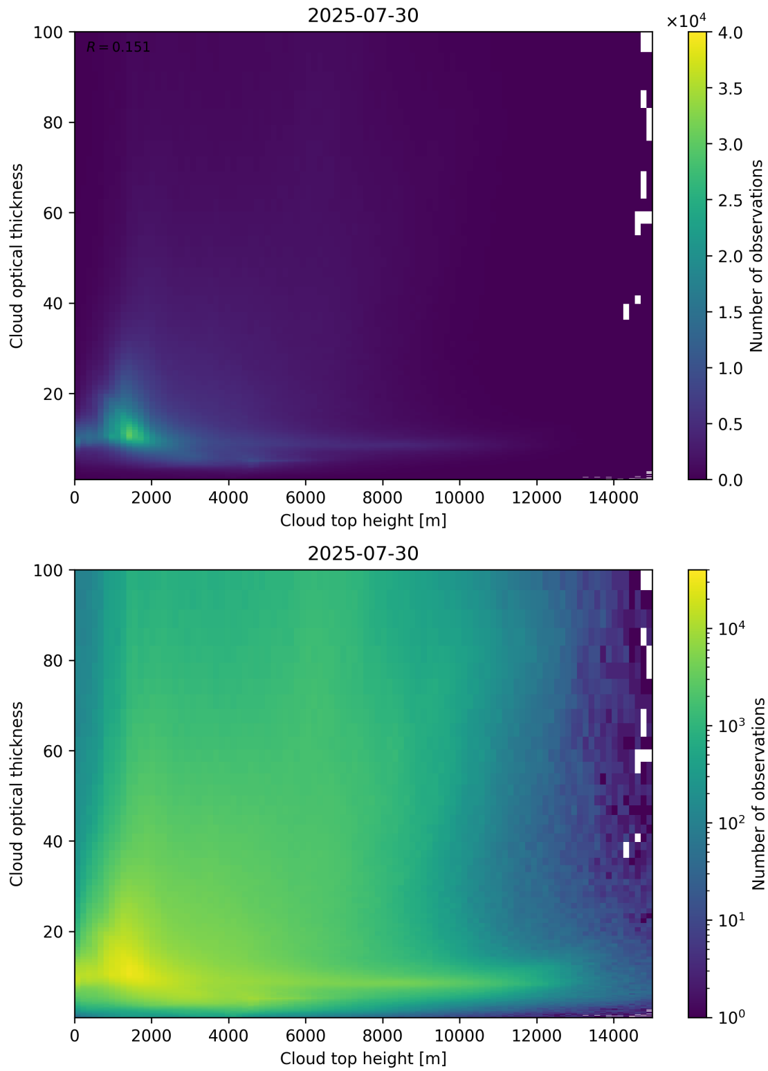
Figure 90: Scatter density plot of “Cloud top height” against “Cloud optical thickness” for 2025-07-29 to 2025-07-31.
