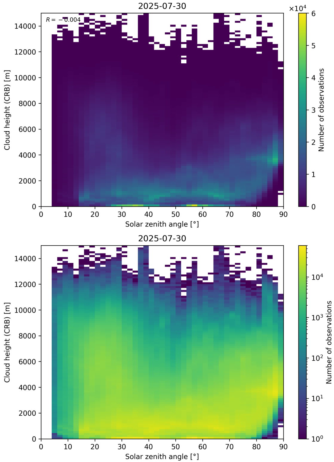
Figure 102: Scatter density plot of “Solar zenith angle” against “Cloud height (CRB)” for 2025-07-29 to 2025-07-31.
