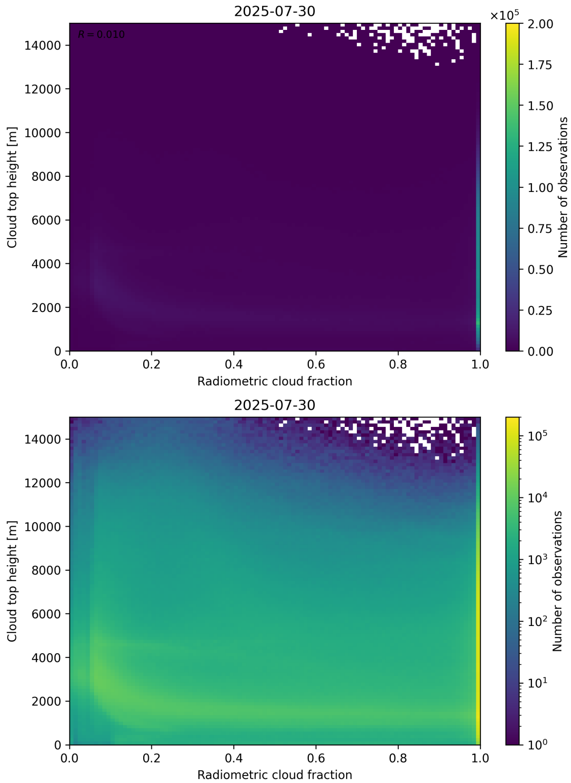
Figure 76: Scatter density plot of “Radiometric cloud fraction” against “Cloud top height” for 2025-07-29 to 2025-07-31.
