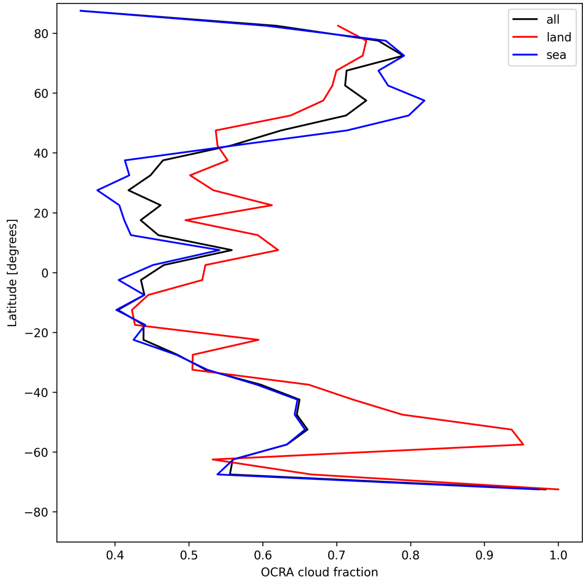
Figure 34: Zonal average of “OCRA cloud fraction” for 2025-07-30 to 2025-08-01.
