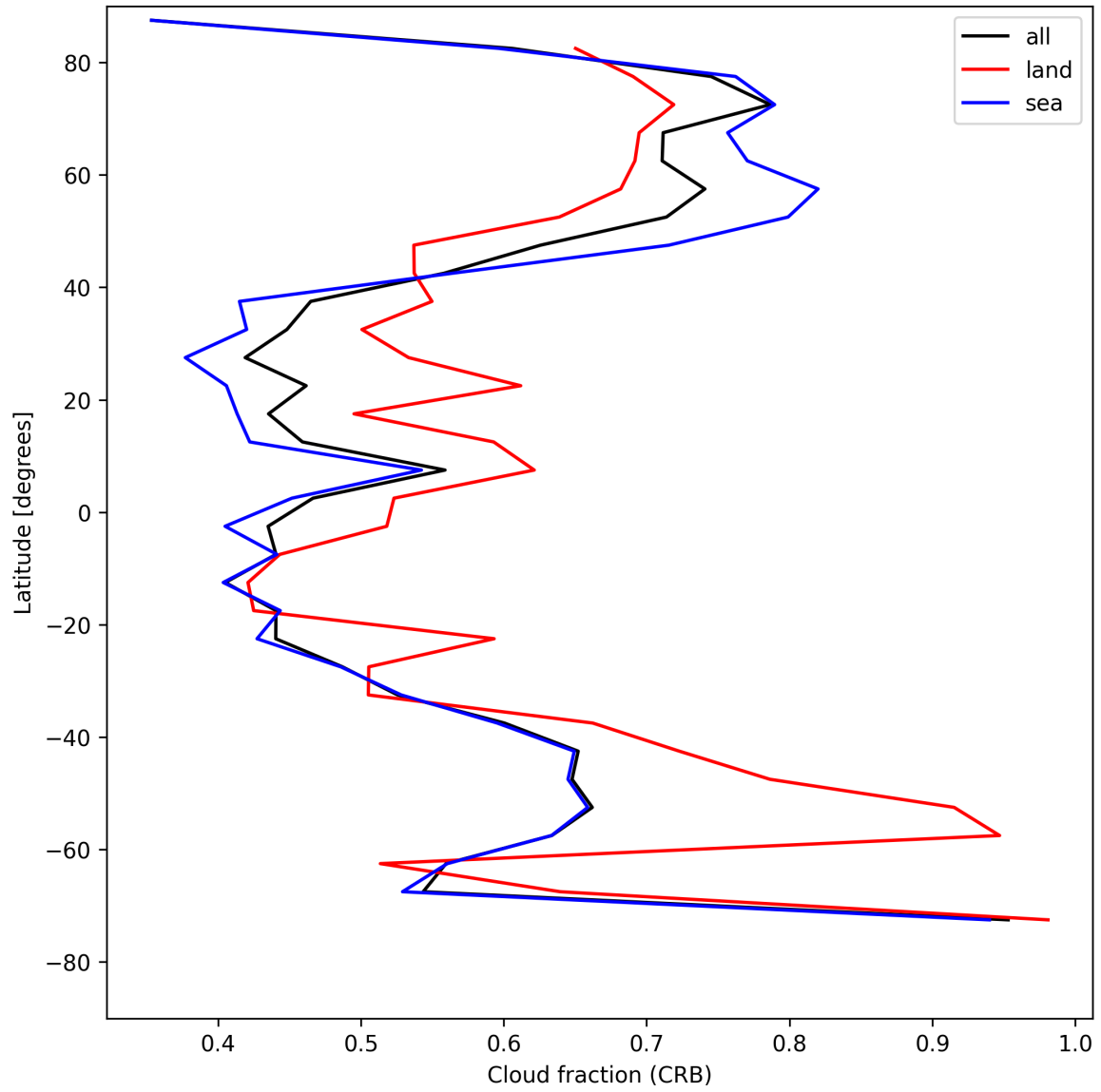
Figure 26: Zonal average of “Cloud fraction (CRB)” for 2025-07-30 to 2025-08-01.
