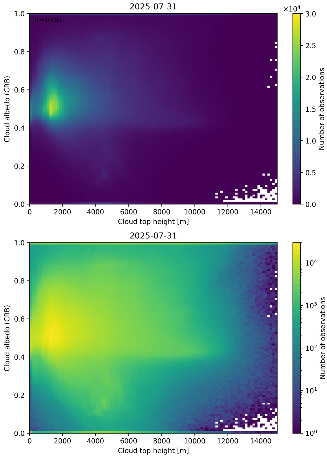
Figure 86: Scatter density plot of “Cloud top height” against “Cloud albedo (CRB)” for 2025-07-30 to 2025-08-01.
