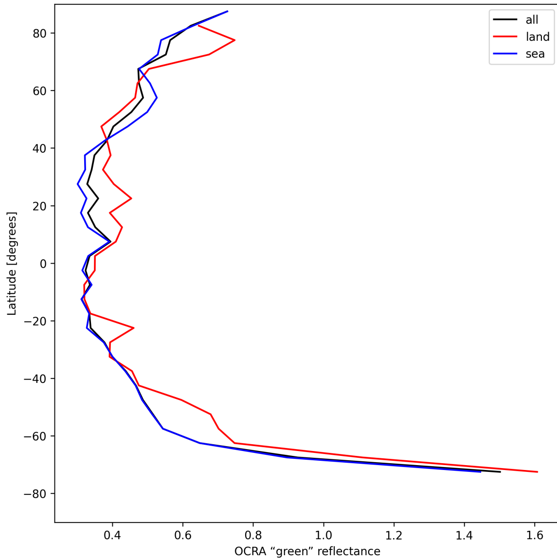
Figure 36: Zonal average of “OCRA “green” reflectance” for 2025-07-30 to 2025-08-01.
