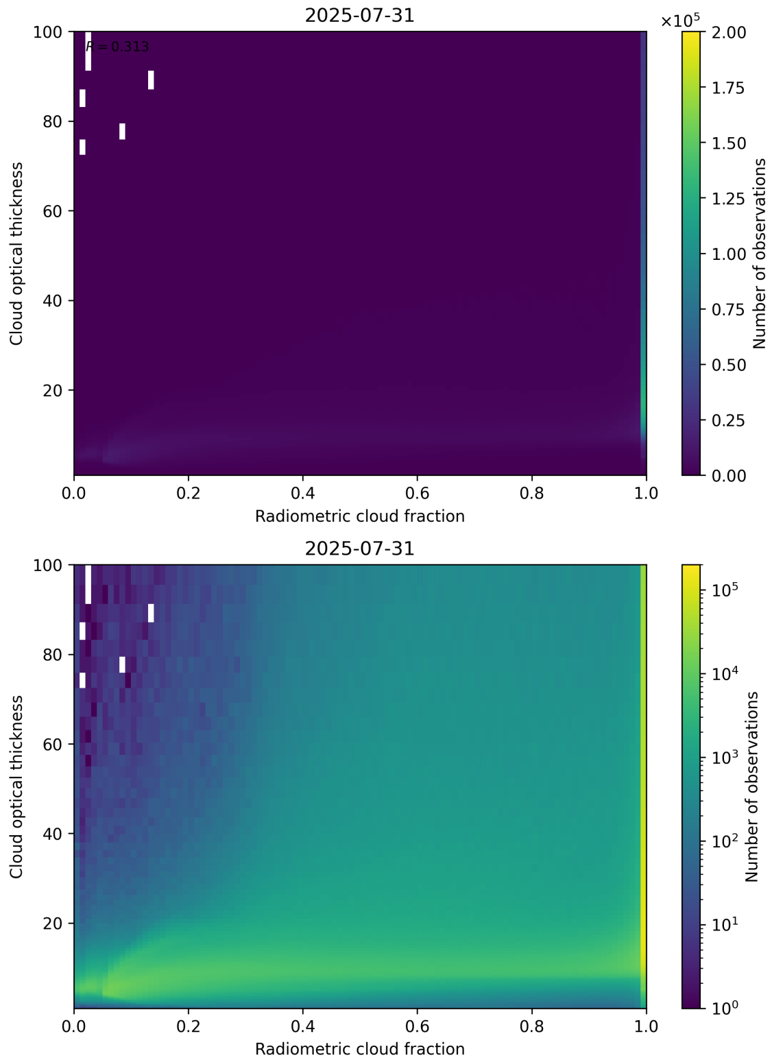
Figure 75: Scatter density plot of “Radiometric cloud fraction” against “Cloud optical thickness” for 2025-07-30 to 2025-08-01.
