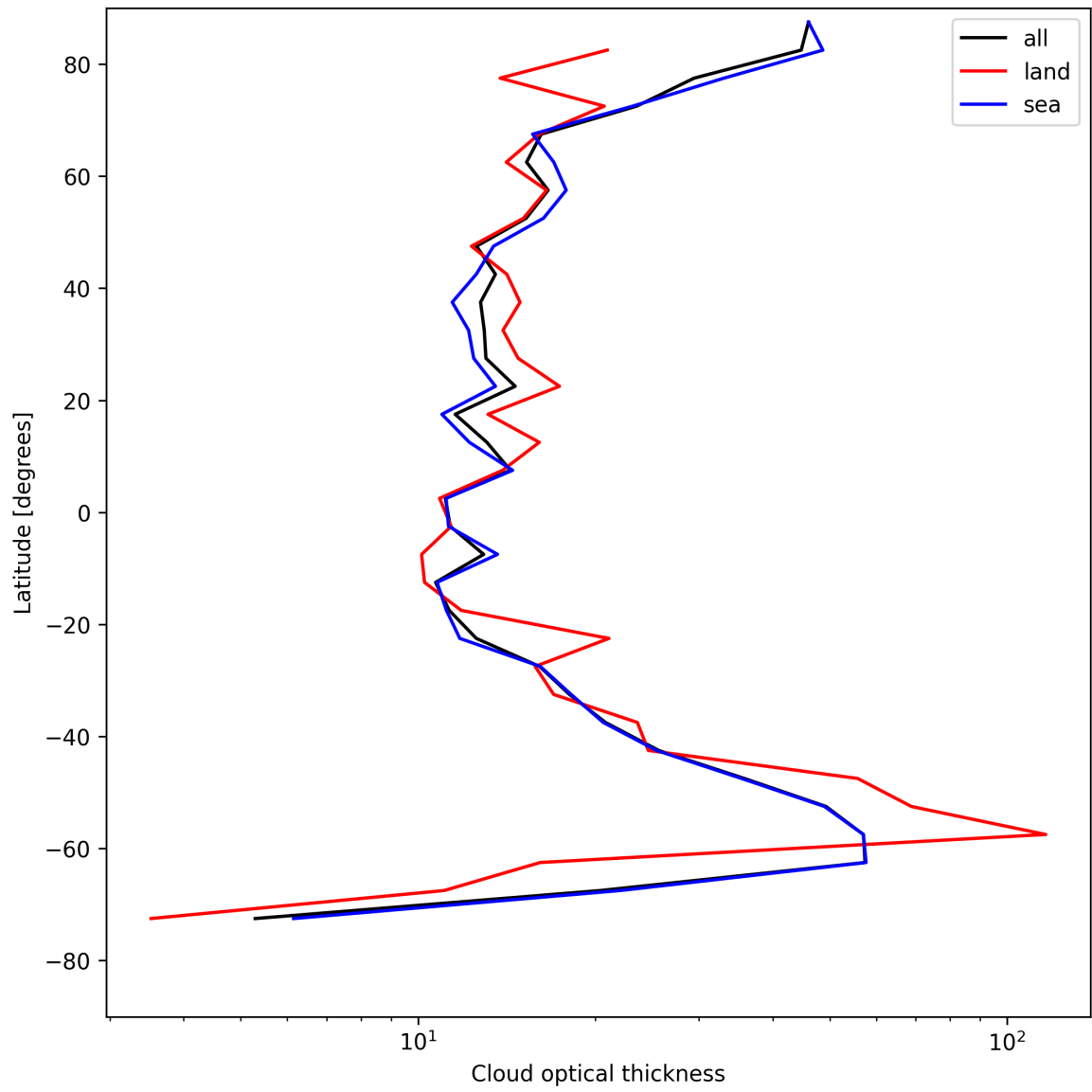
Figure 25: Zonal average of “Cloud optical thickness” for 2025-07-30 to 2025-08-01.
