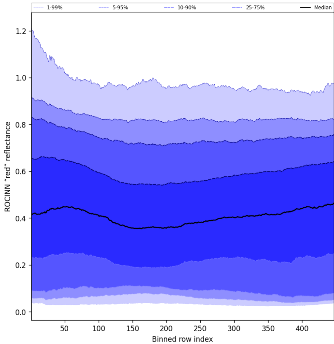
Figure 69: Along track statistics of "ROCINN "red" reflectance" for 2025-07-30 to 2025-08-01
