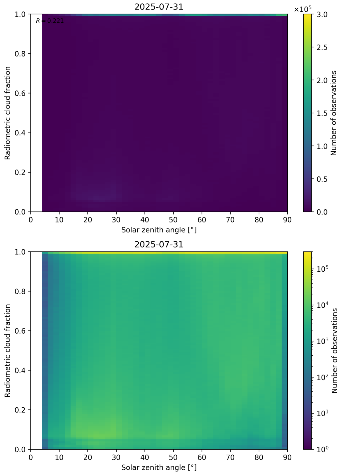
Figure 99: Scatter density plot of “Solar zenith angle” against “Radiometric cloud fraction” for 2025-07-30 to 2025-08-01.
