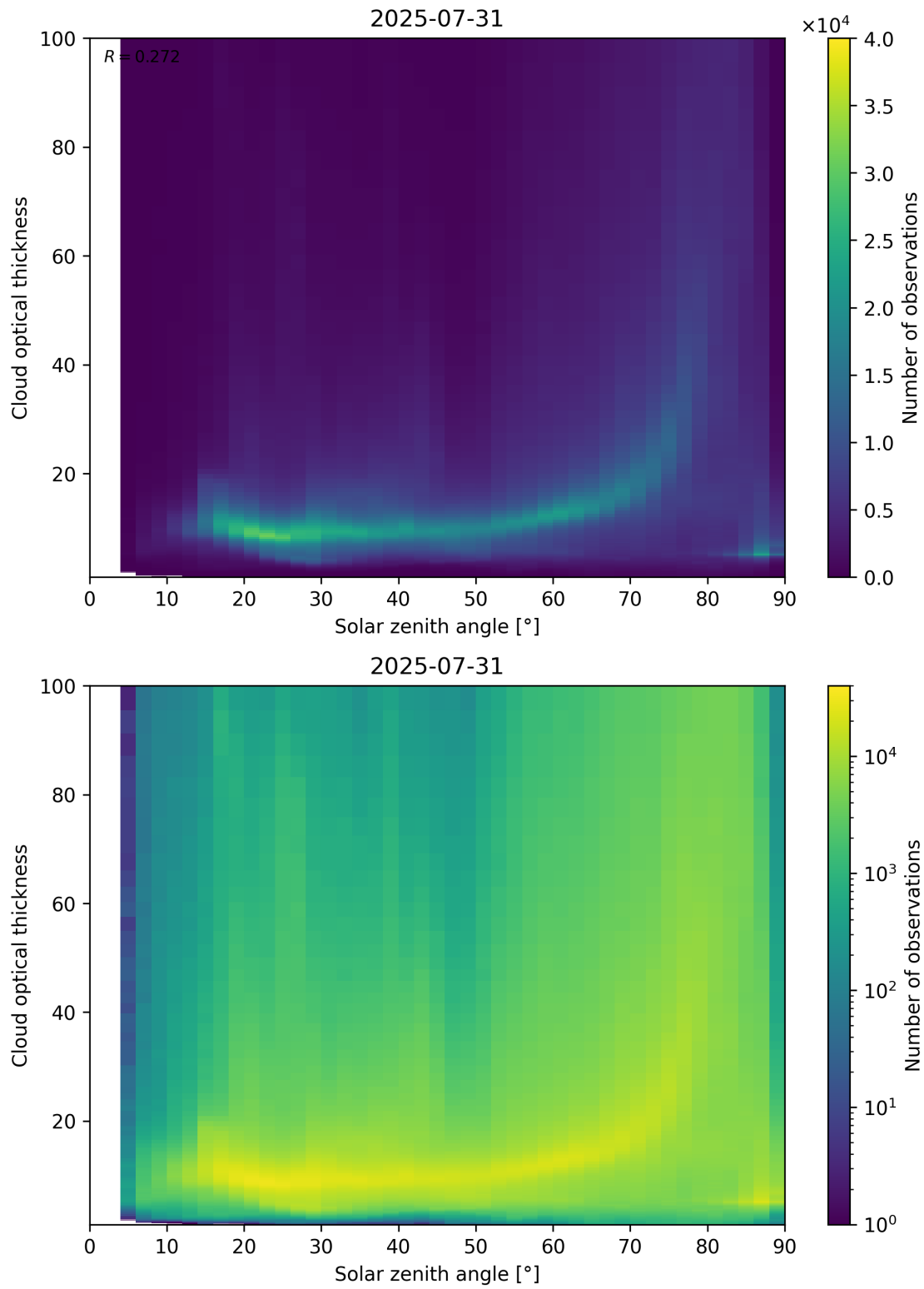
Figure 103: Scatter density plot of “Solar zenith angle” against “Cloud optical thickness” for 2025-07-30 to 2025-08-01.
