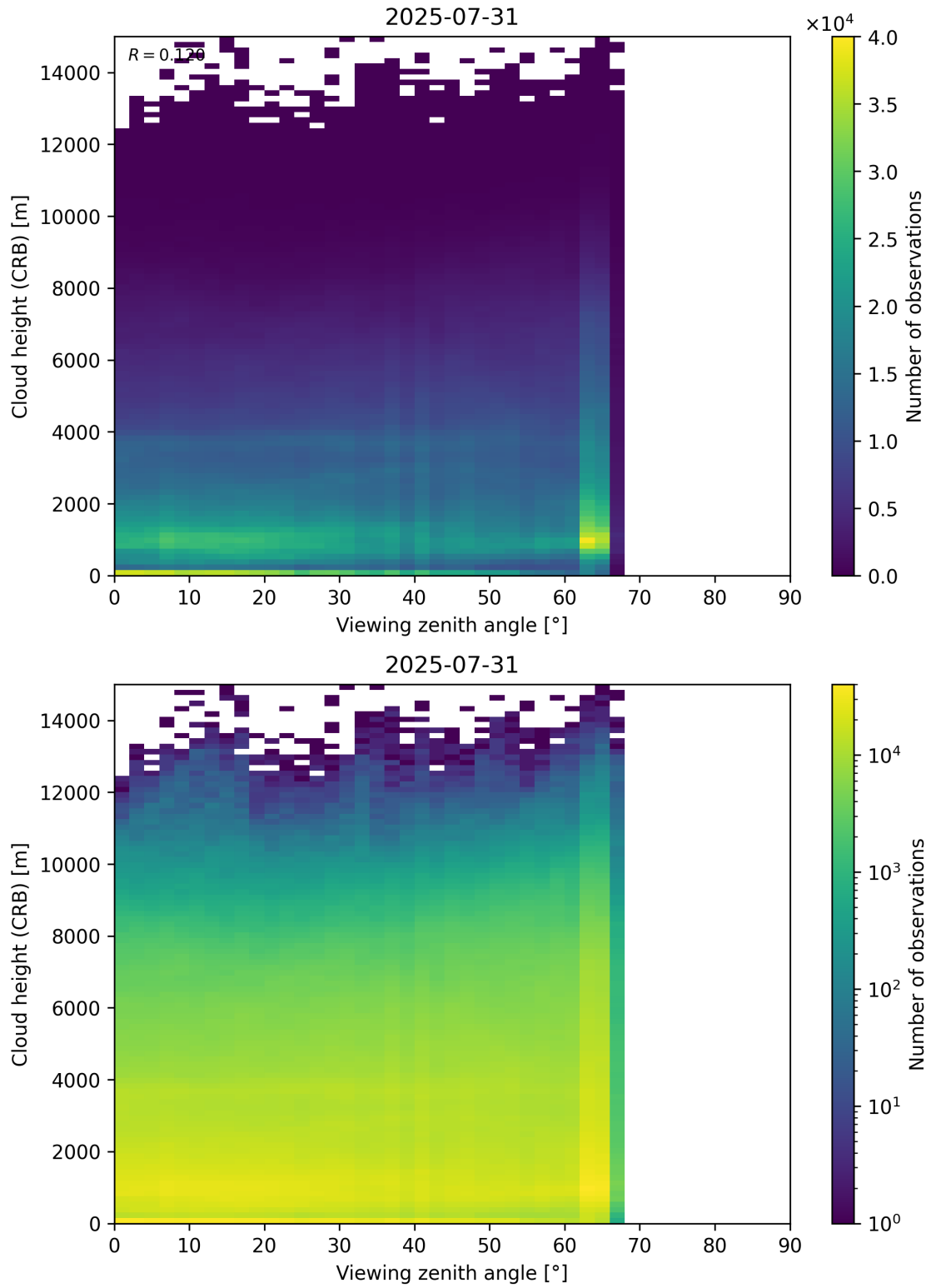
Figure 110: Scatter density plot of “Viewing zenith angle” against “Cloud height (CRB)” for 2025-07-30 to 2025-08-01.
