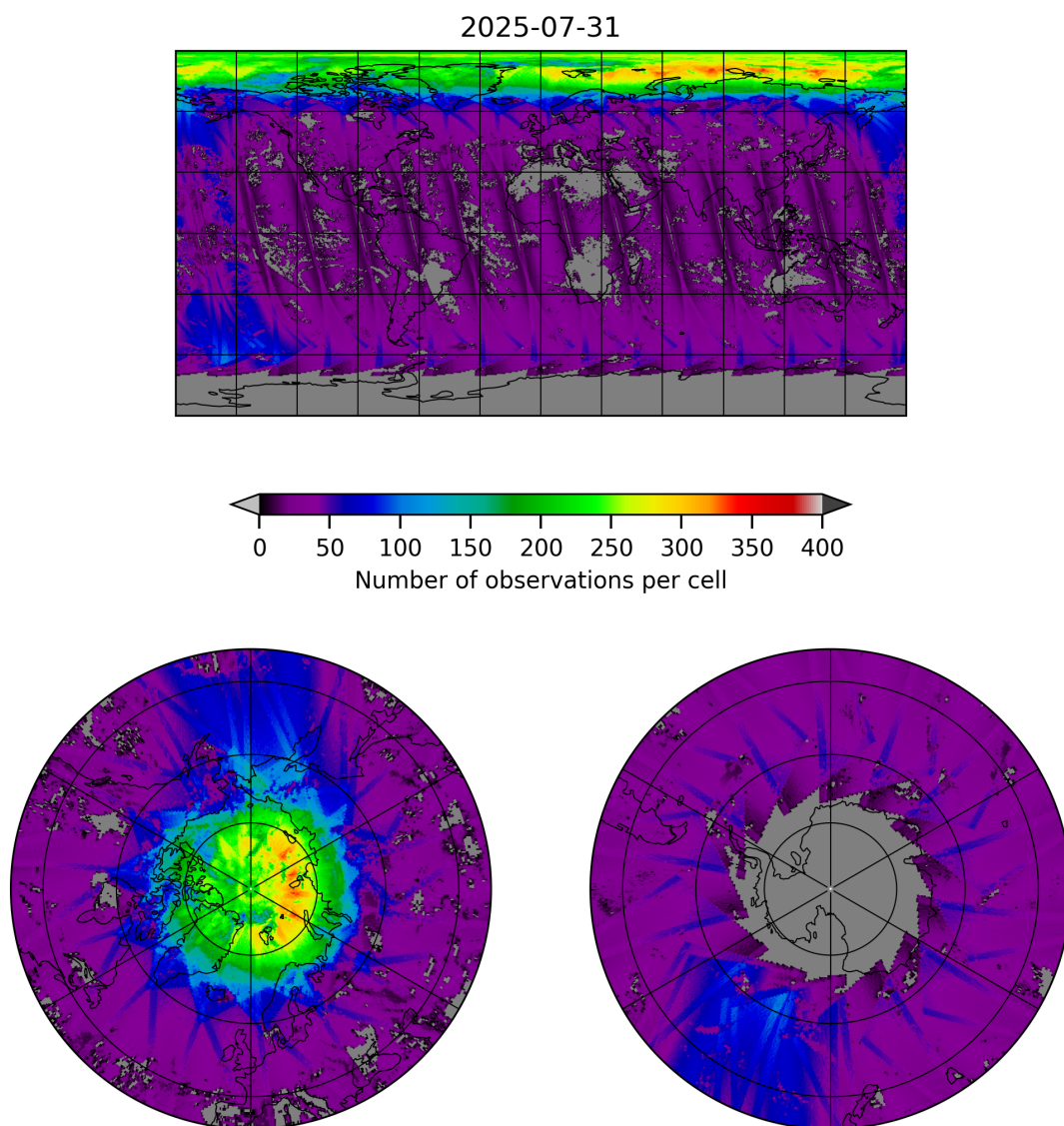
Figure 21: Map of the number of observations for 2025-07-30 to 2025-08-01
