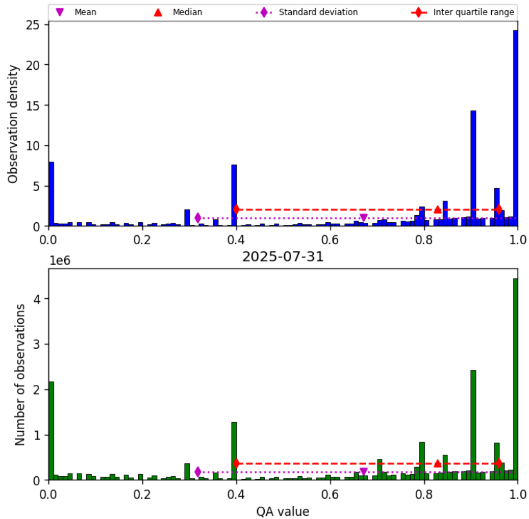
Figure 38: Histogram of “QA value” for 2025-07-30 to 2025-08-01
