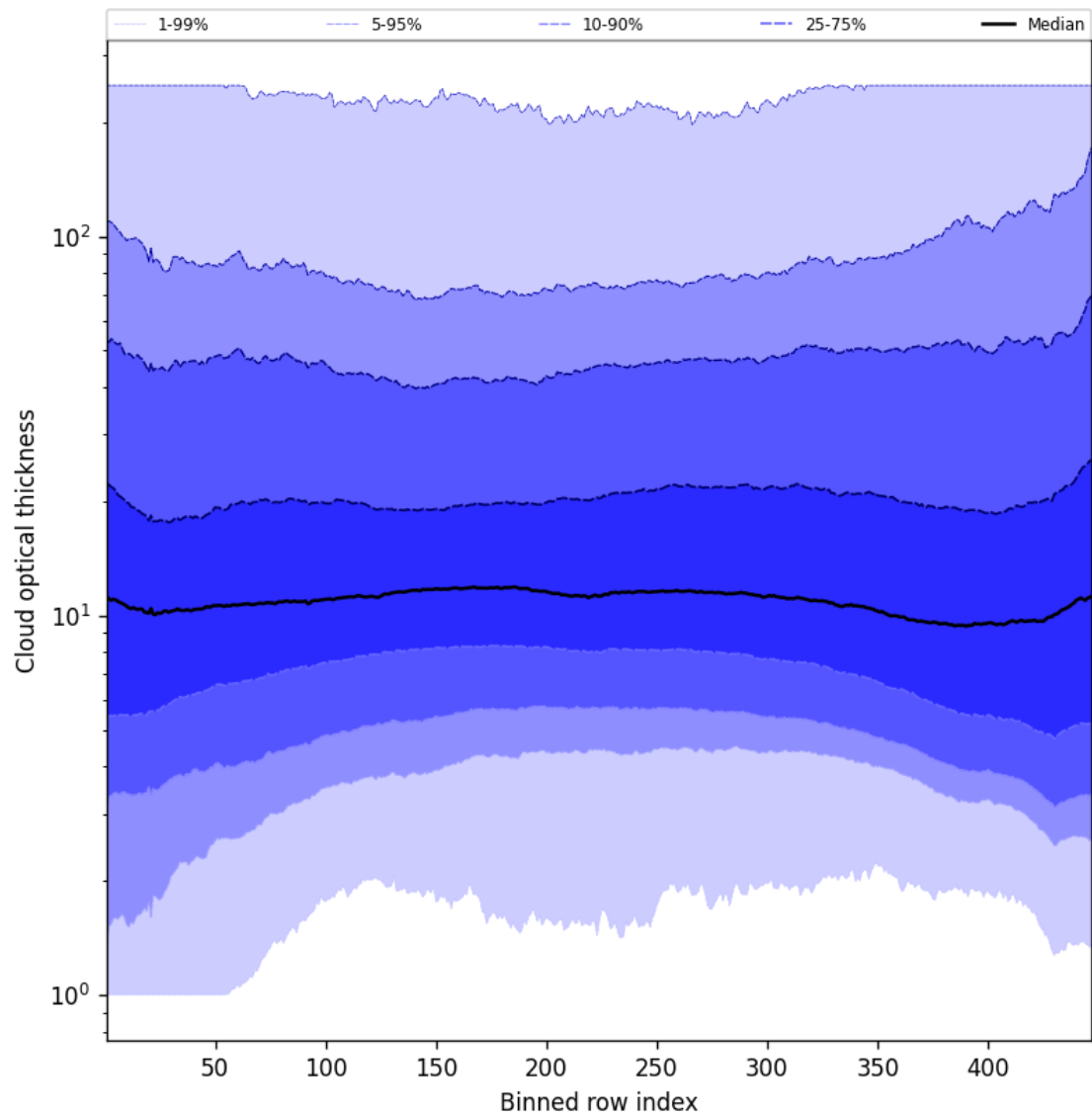
Figure 57: Along track statistics of “Cloud optical thickness” for 2025-07-30 to 2025-08-01
