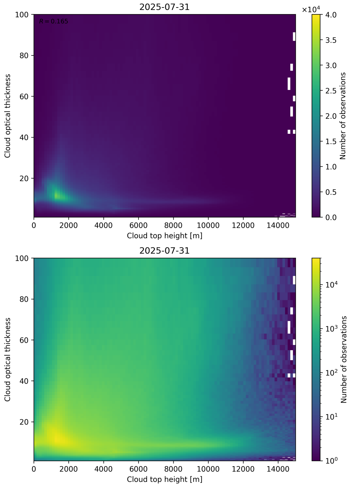
Figure 90: Scatter density plot of “Cloud top height” against “Cloud optical thickness” for 2025-07-30 to 2025-08-01.
