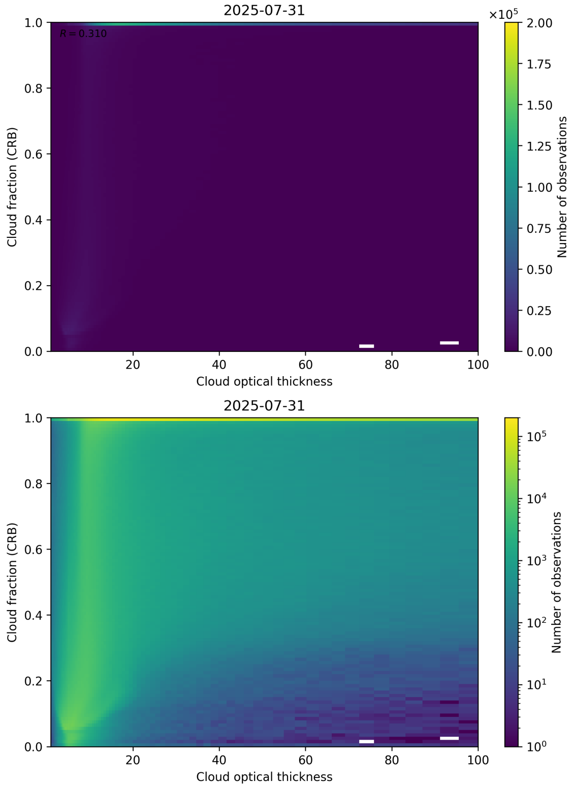
Figure 84: Scatter density plot of “Cloud optical thickness” against “Cloud fraction (CRB)” for 2025-07-30 to 2025-08-01.
