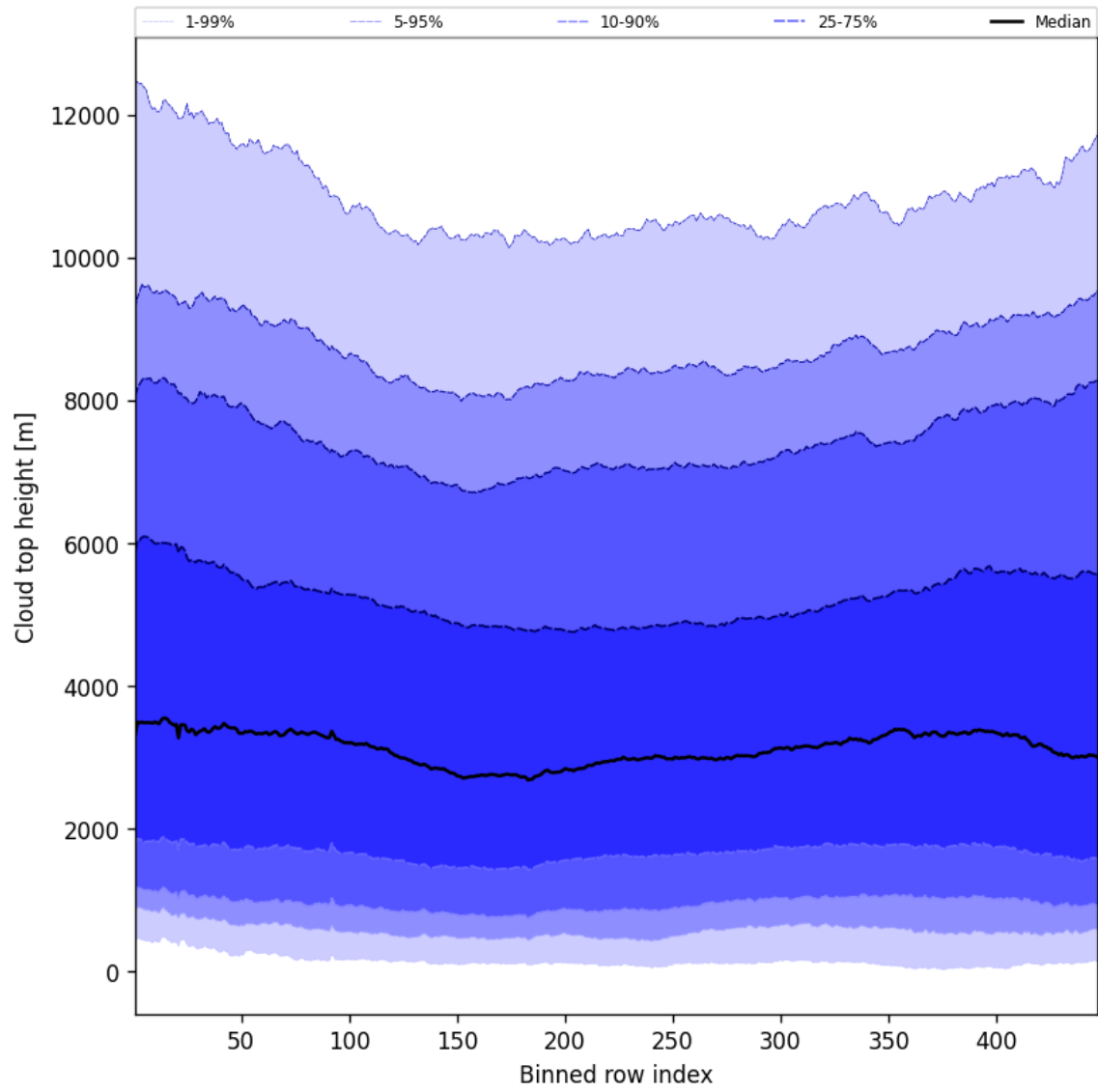
Figure 56: Along track statistics of “Cloud top height” for 2025-07-30 to 2025-08-01
