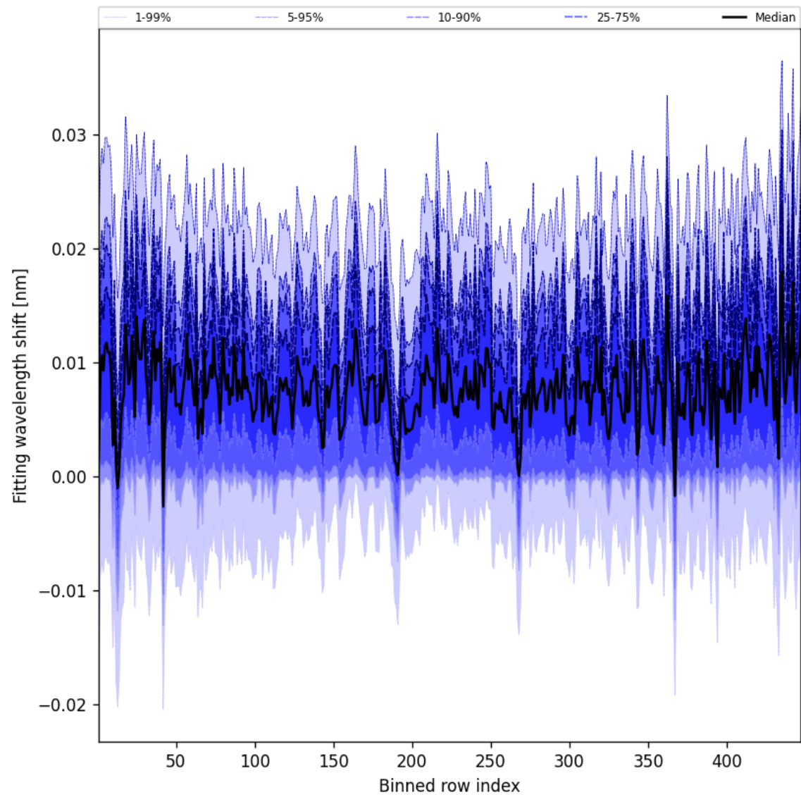
Figure 65: Along track statistics of “Fitting wavelength shift” for 2025-07-30 to 2025-08-01
