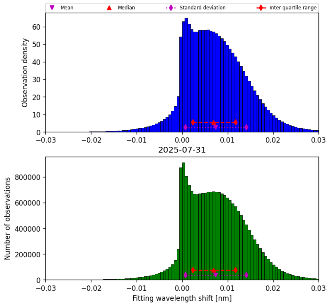
Figure 49: Histogram of “Fitting wavelength shift” for 2025-07-30 to 2025-08-01
