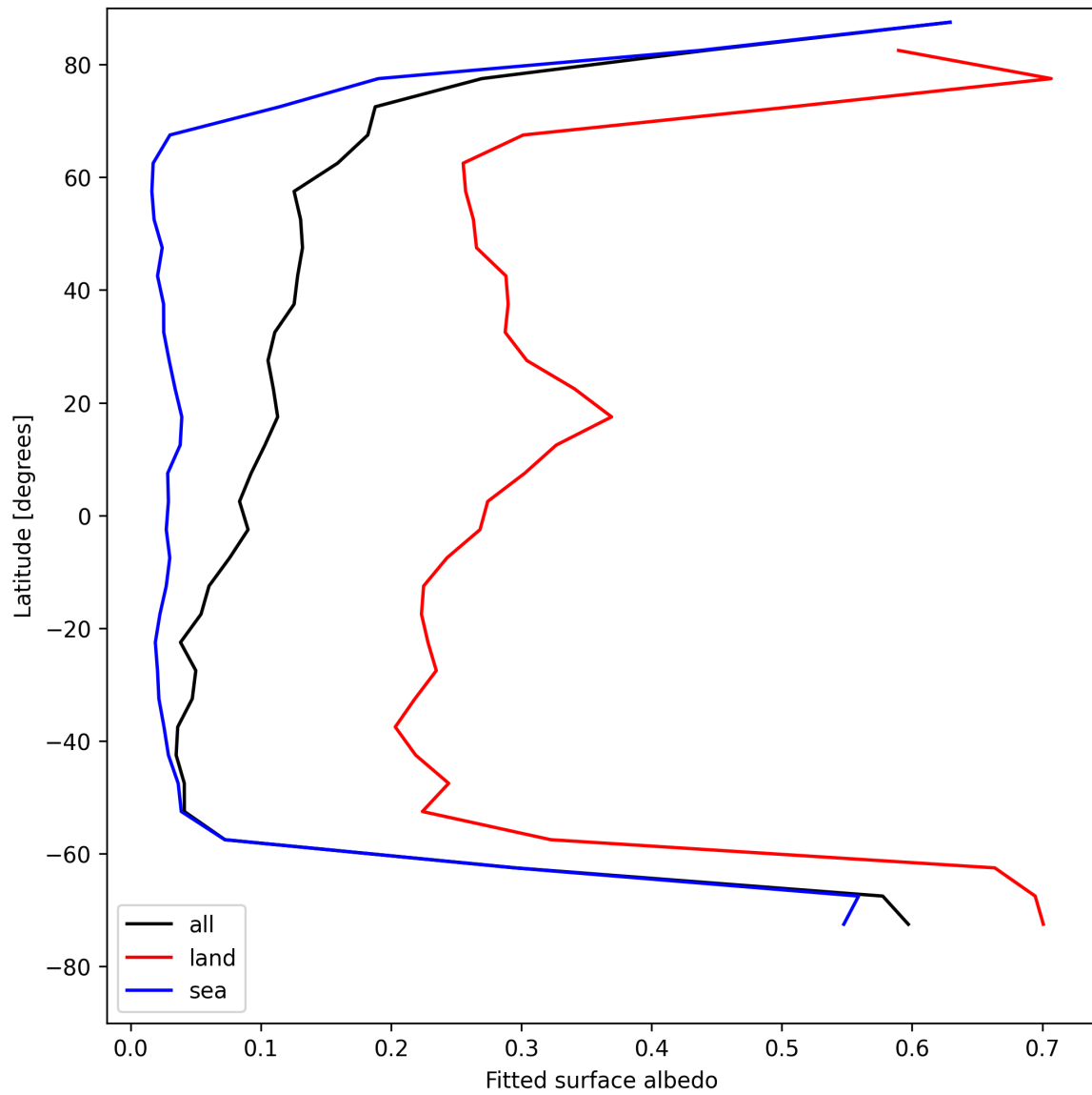
Figure 29: Zonal average of “Fitted surface albedo” for 2025-07-30 to 2025-08-01.
