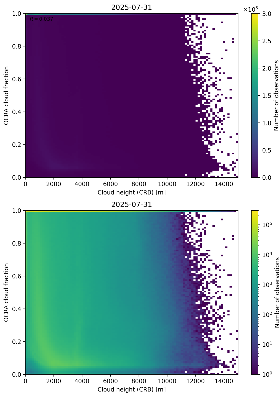
Figure 81: Scatter density plot of “Cloud height (CRB)” against “OCRA cloud fraction” for 2025-07-30 to 2025-08-01.
