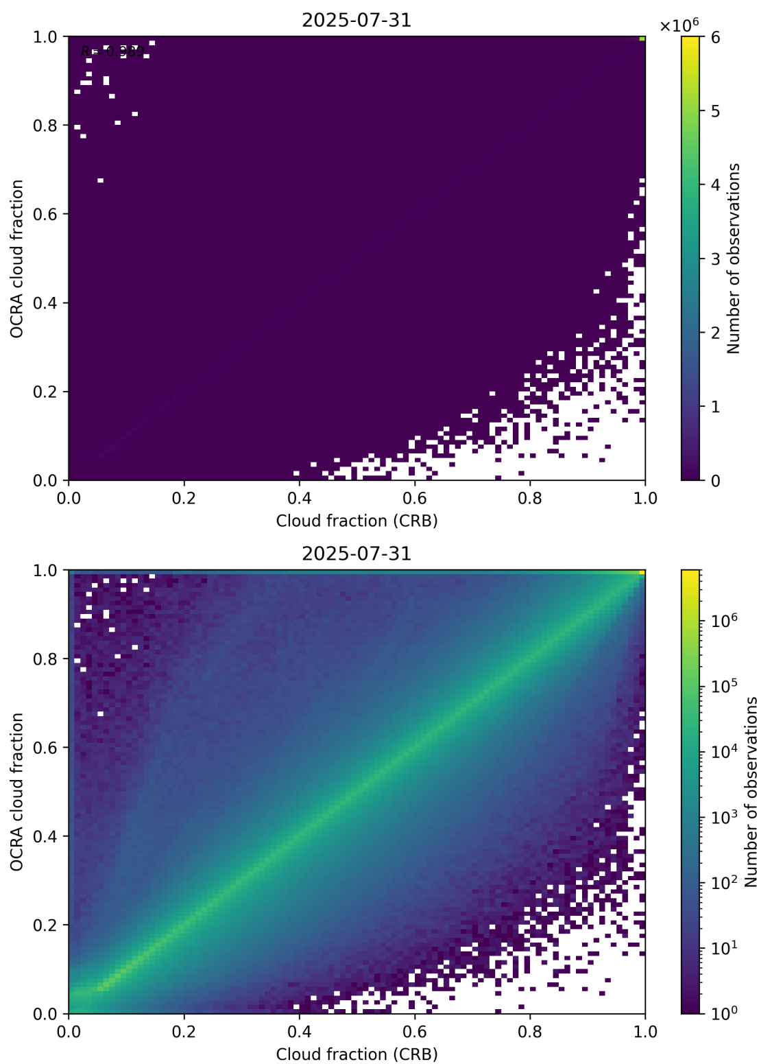
Figure 78: Scatter density plot of “Cloud fraction (CRB)” against “OCRA cloud fraction” for 2025-07-30 to 2025-08-01.
