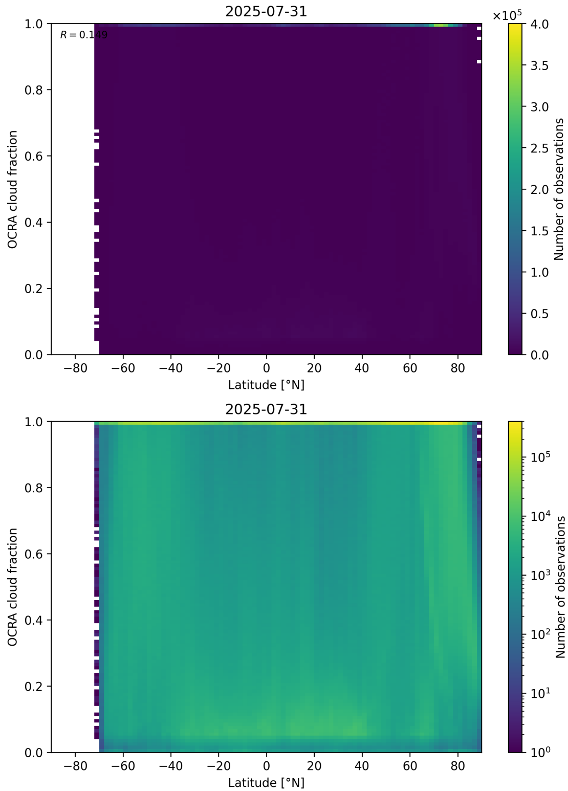
Figure 93: Scatter density plot of “Latitude” against “OCRA cloud fraction” for 2025-07-30 to 2025-08-01.
