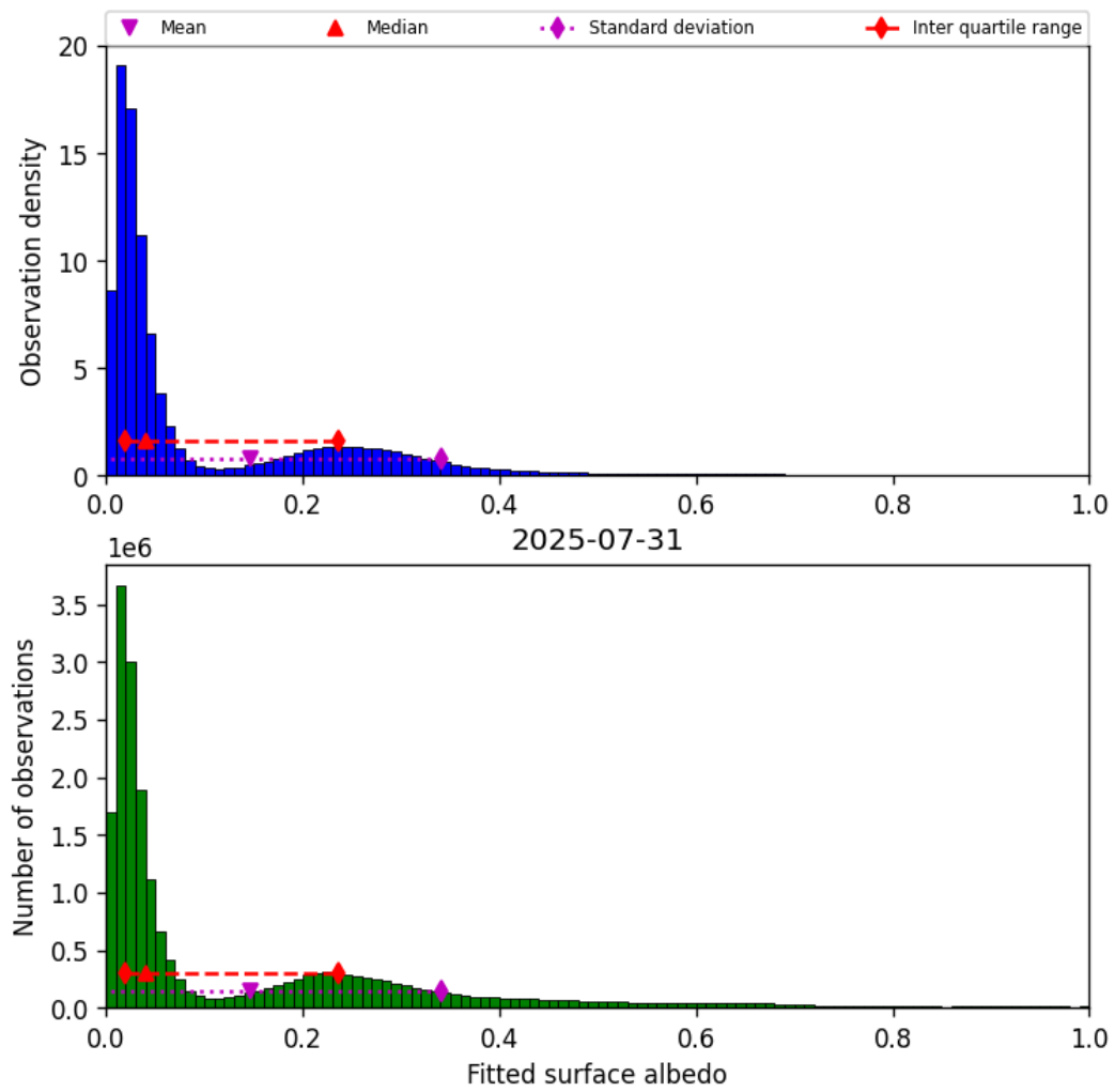
Figure 45: Histogram of “Fitted surface albedo” for 2025-07-30 to 2025-08-01
