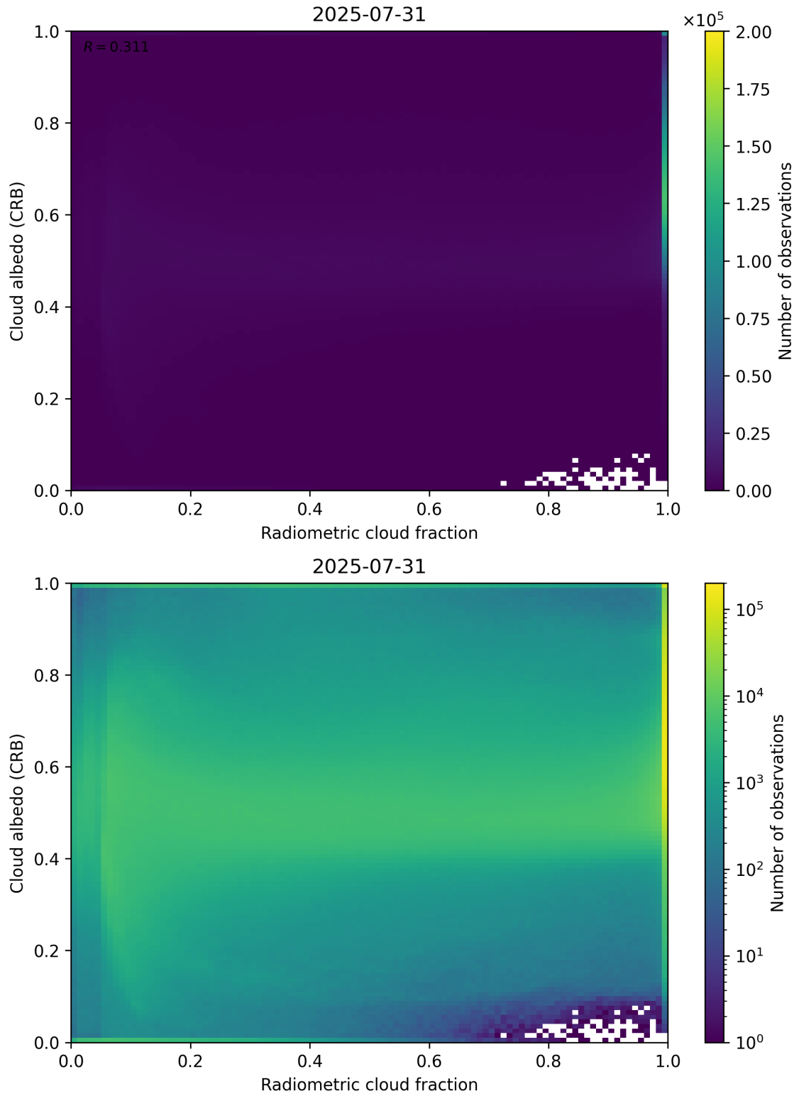
Figure 71: Scatter density plot of “Radiometric cloud fraction” against “Cloud albedo (CRB)” for 2025-07-30 to 2025-08-01.
