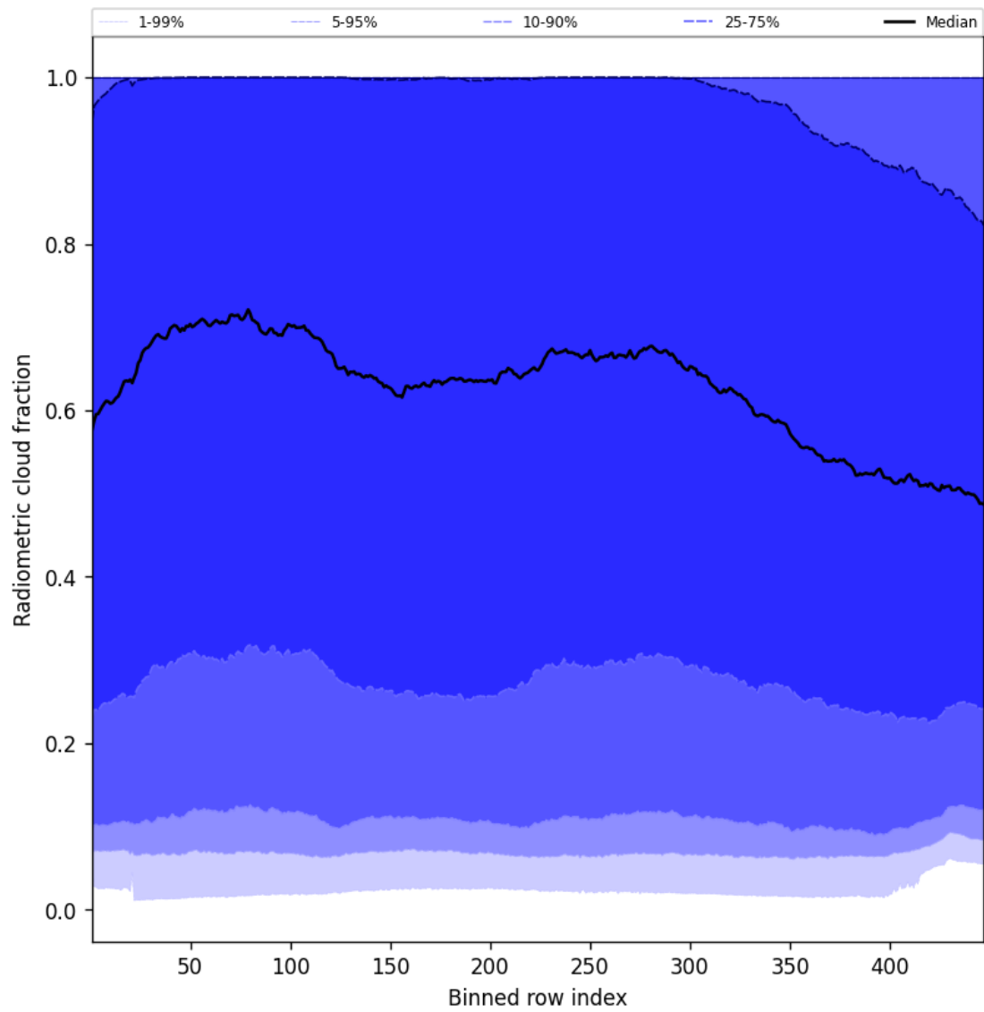
Figure 55: Along track statistics of “Radiometric cloud fraction” for 2025-07-30 to 2025-08-01
