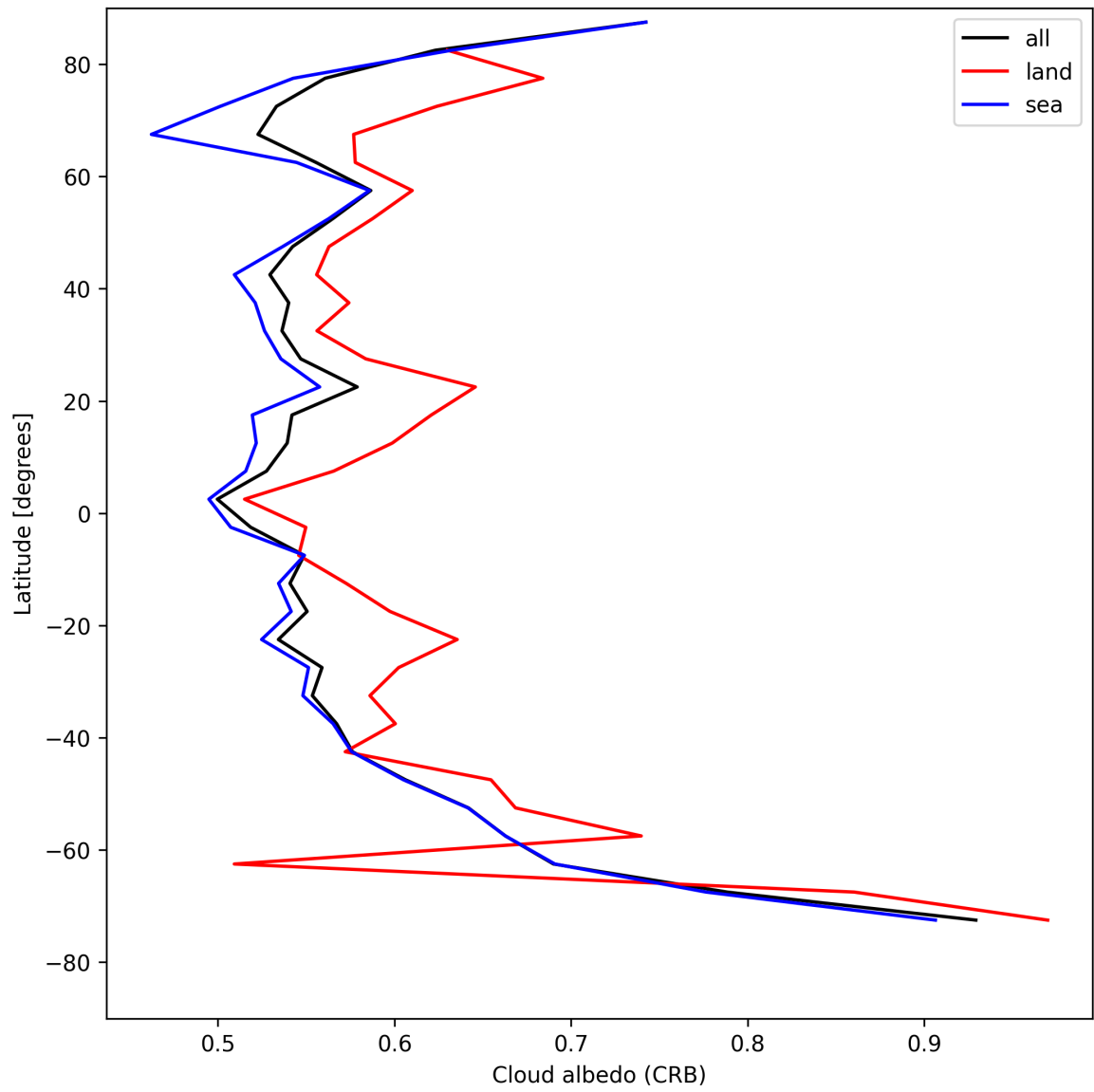
Figure 28: Zonal average of “Cloud albedo (CRB)” for 2025-07-30 to 2025-08-01.
