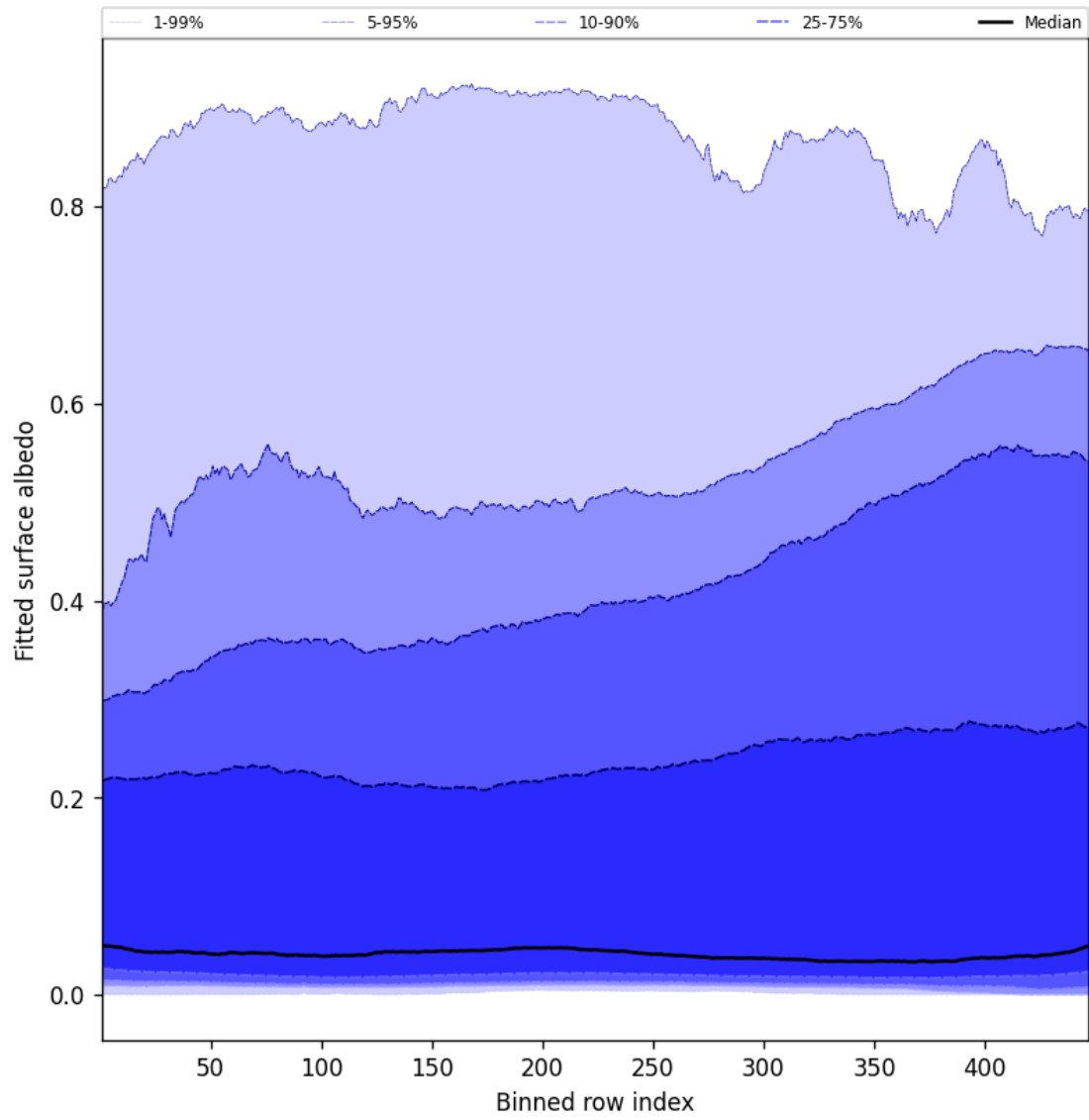
Figure 61: Along track statistics of “Fitted surface albedo” for 2025-07-30 to 2025-08-01
