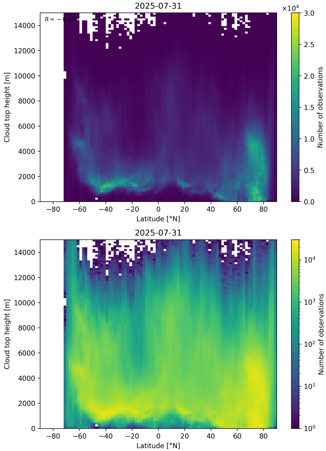
Figure 97: Scatter density plot of “Latitude” against “Cloud top height” for 2025-07-30 to 2025-08-01.
