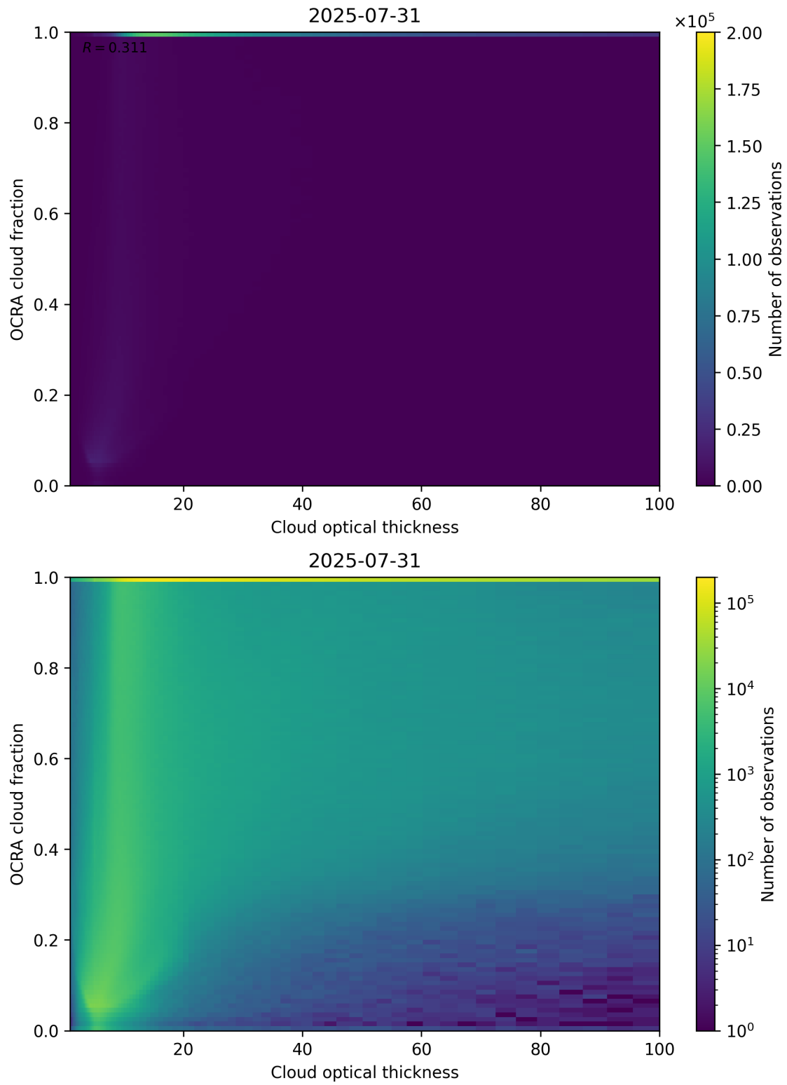
Figure 83: Scatter density plot of “Cloud optical thickness” against “OCRA cloud fraction” for 2025-07-30 to 2025-08-01.
