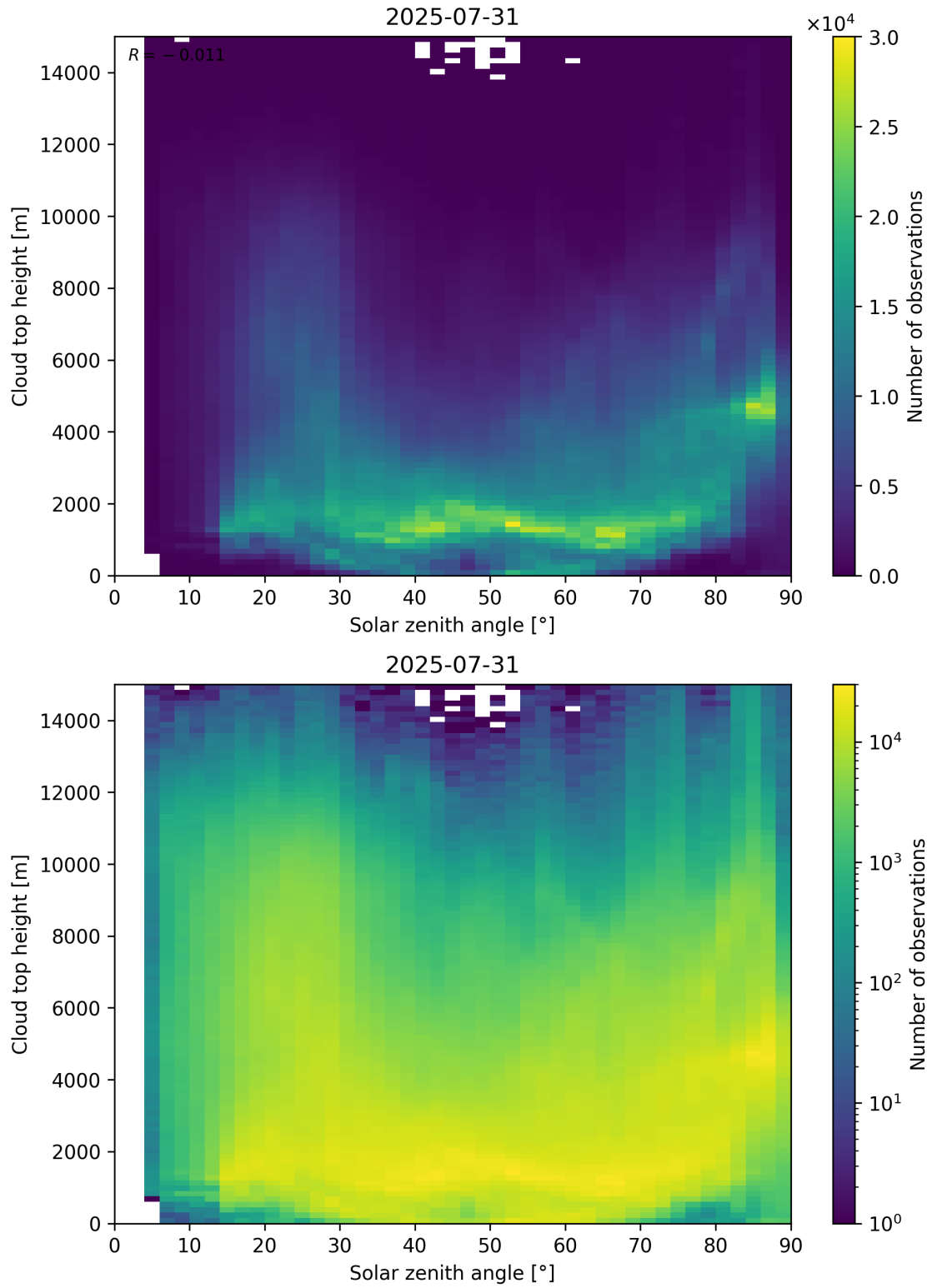
Figure 104: Scatter density plot of “Solar zenith angle” against “Cloud top height” for 2025-07-30 to 2025-08-01.
