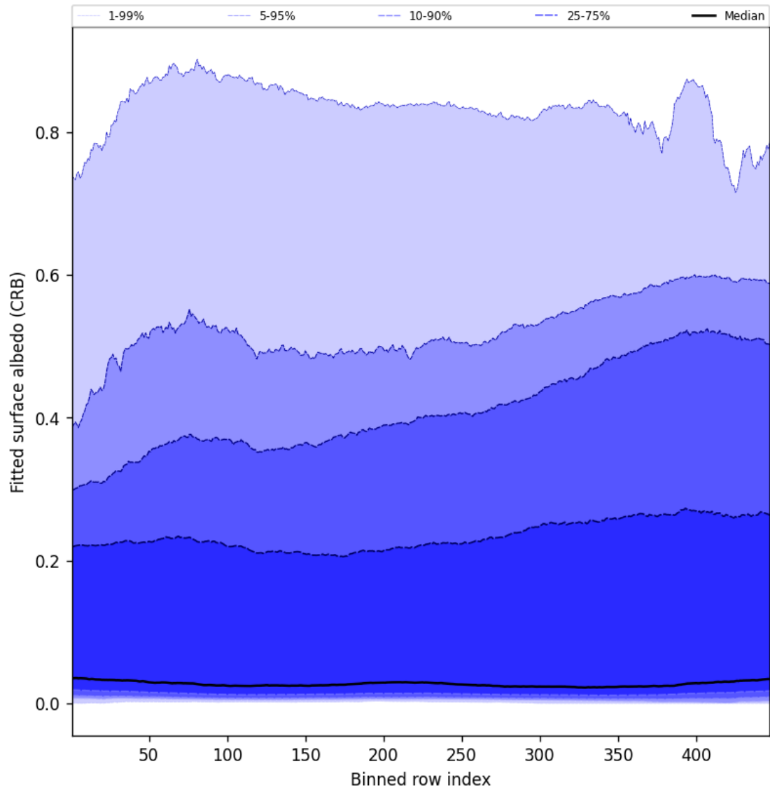
Figure 62: Along track statistics of “Fitted surface albedo (CRB)” for 2025-07-30 to 2025-08-01
