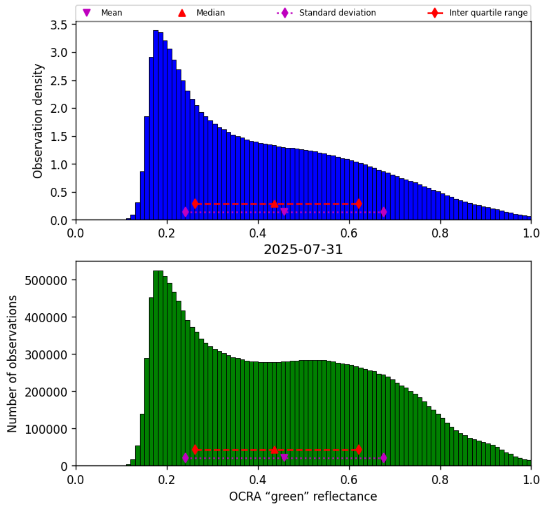
Figure 52: Histogram of “OCRA “green” reflectance” for 2025-07-30 to 2025-08-01
