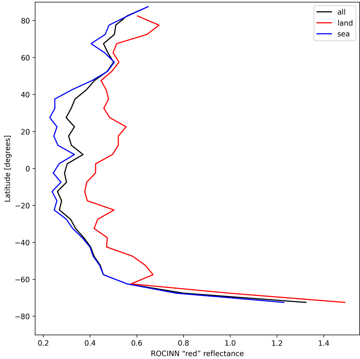
Figure 37: Zonal average of “ROCINN “red” reflectance” for 2025-07-30 to 2025-08-01.
