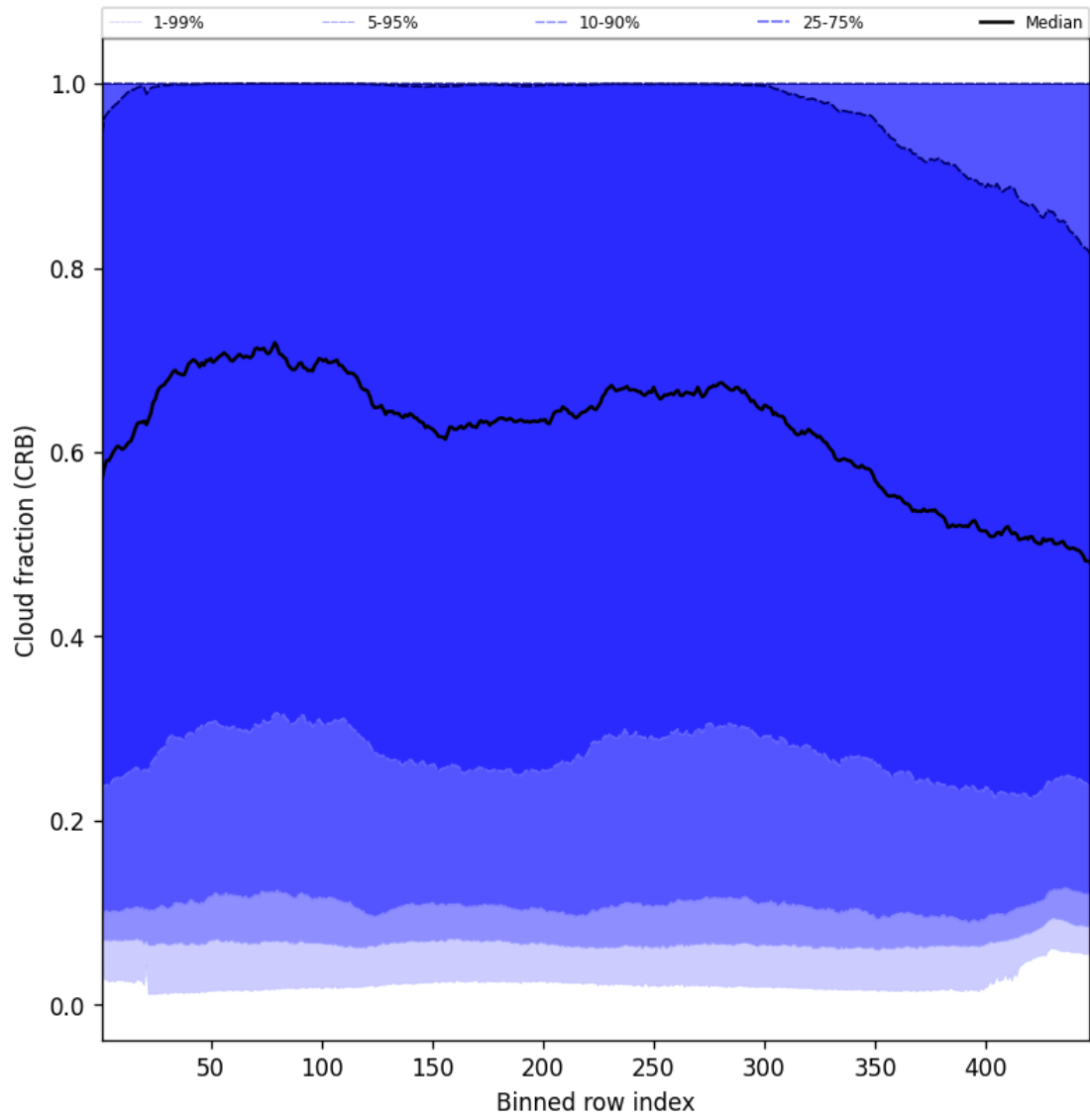
Figure 58: Along track statistics of “Cloud fraction (CRB)” for 2025-07-30 to 2025-08-01
