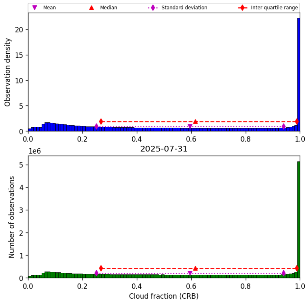
Figure 42: Histogram of “Cloud fraction (CRB)” for 2025-07-30 to 2025-08-01
