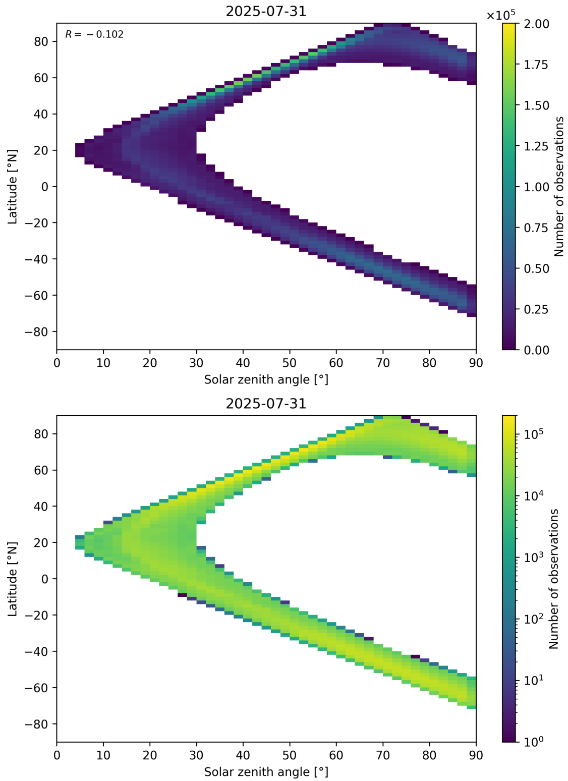
Figure 105: Scatter density plot of “Solar zenith angle” against “Latitude” for 2025-07-30 to 2025-08-01.
