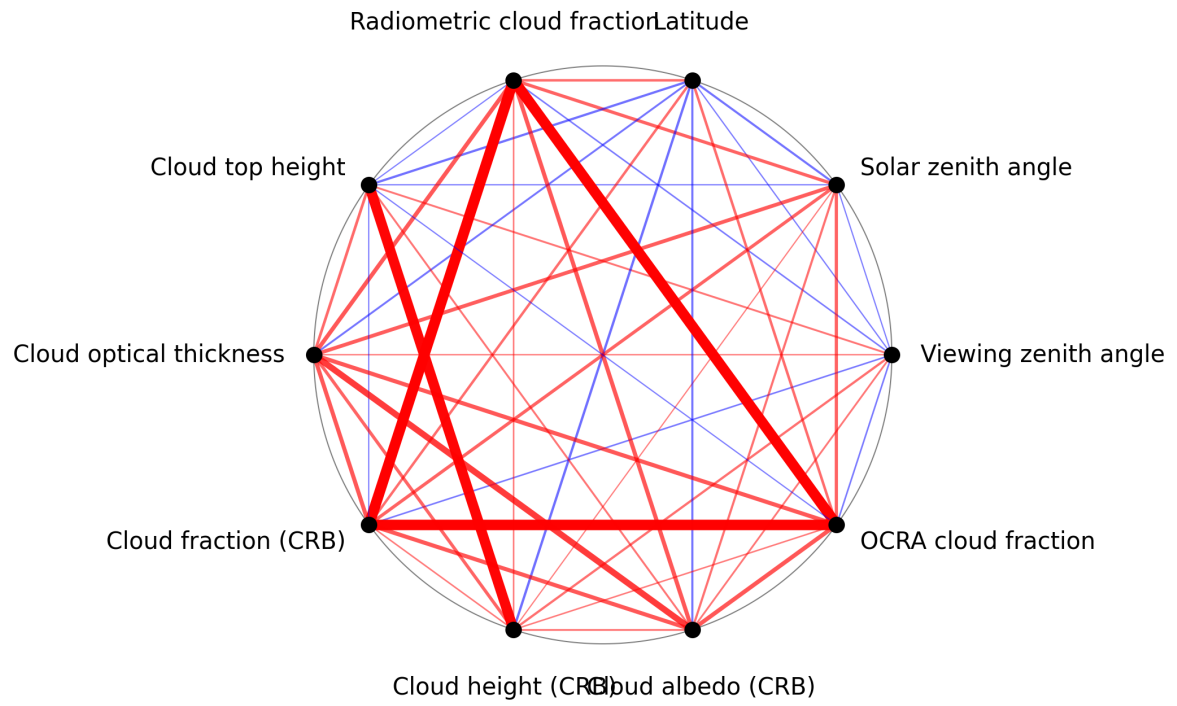
Figure 1: Map of correlation graph for 2025-07-30 to 2025-08-01.
