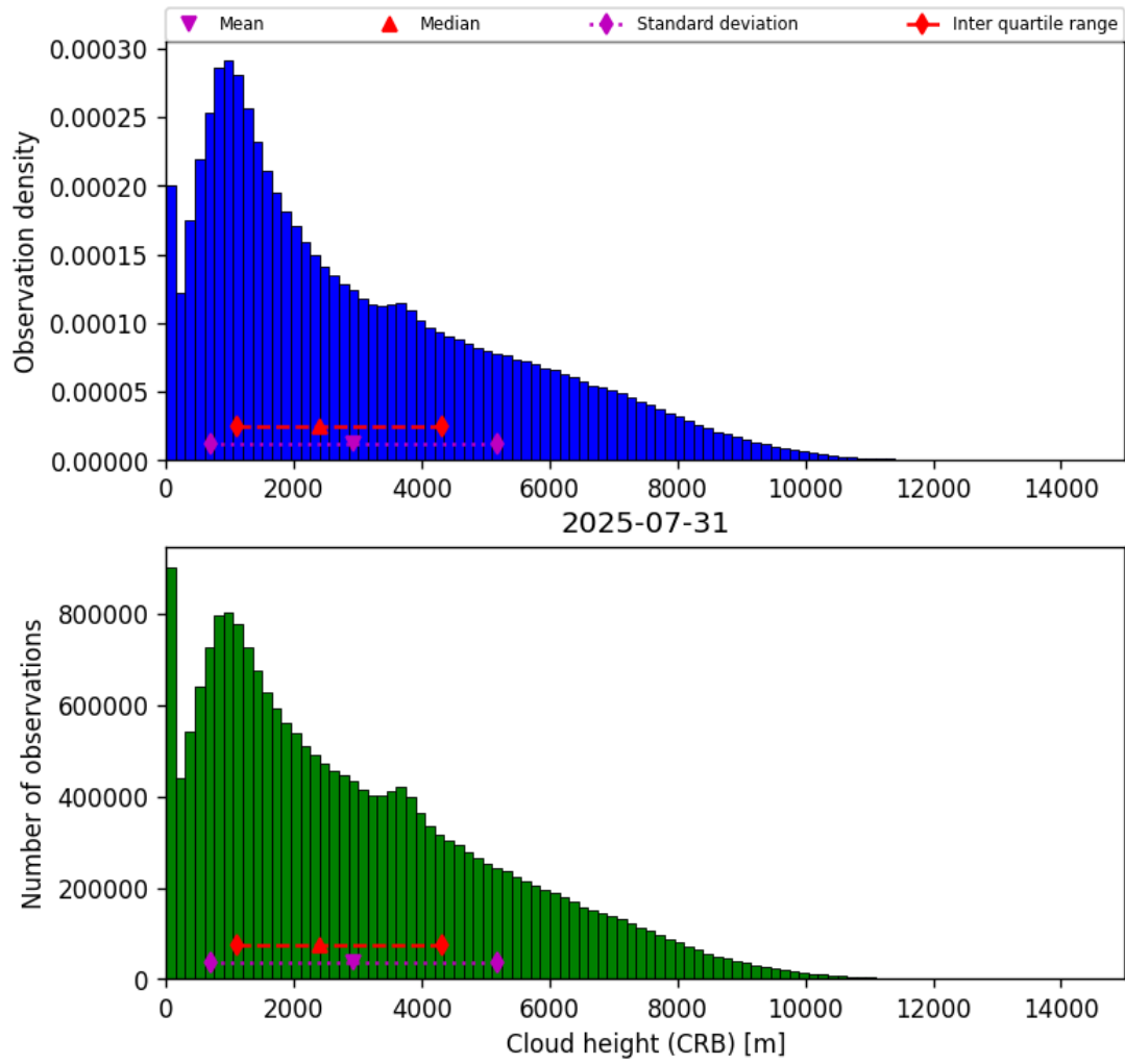
Figure 43: Histogram of “Cloud height (CRB)” for 2025-07-30 to 2025-08-01
