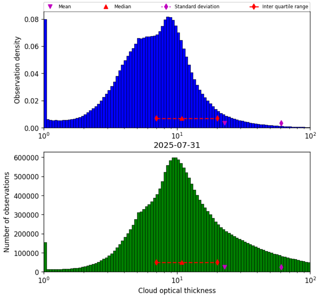
Figure 41: Histogram of “Cloud optical thickness” for 2025-07-30 to 2025-08-01
