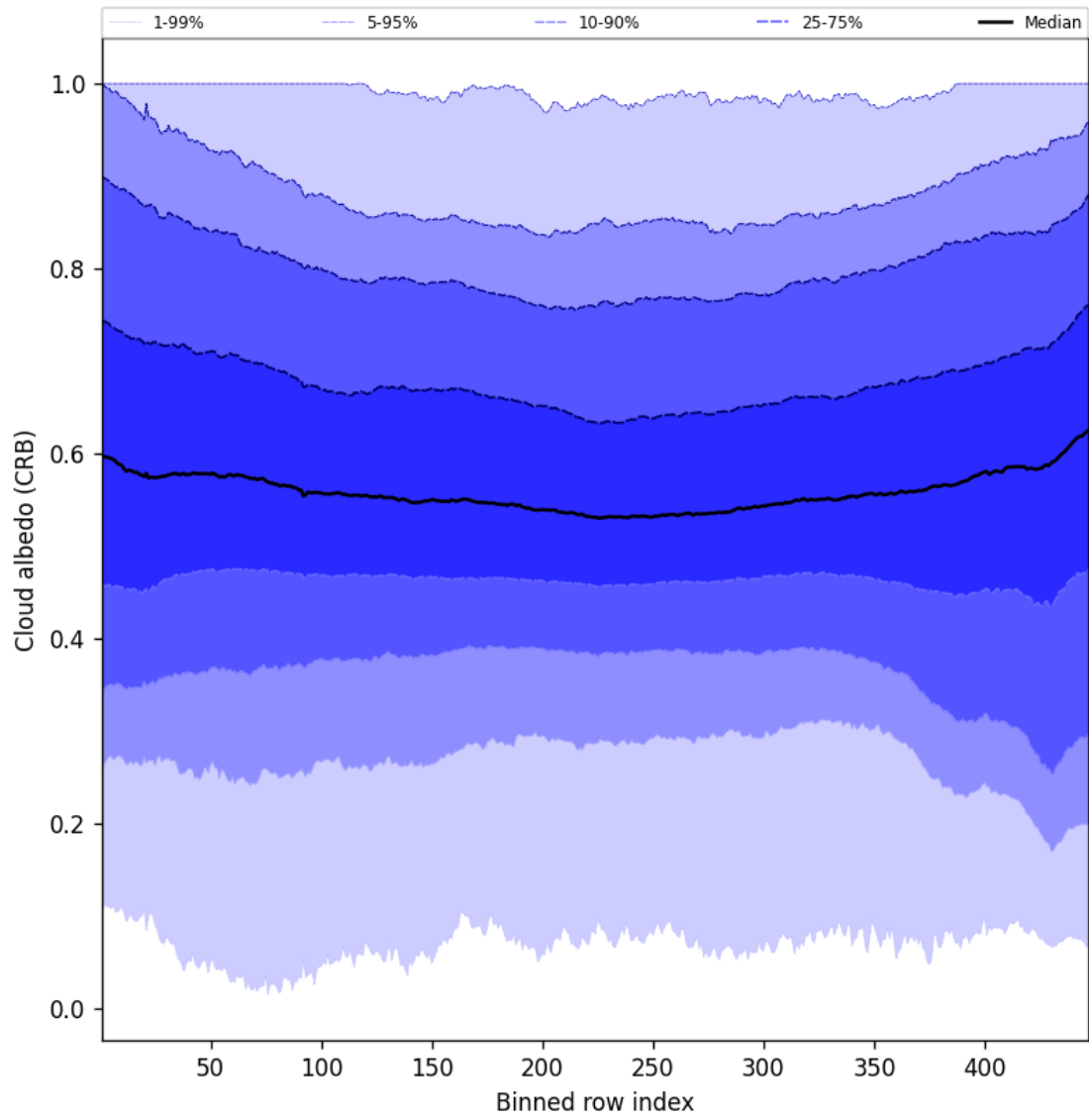
Figure 60: Along track statistics of “Cloud albedo (CRB)” for 2025-07-30 to 2025-08-01
