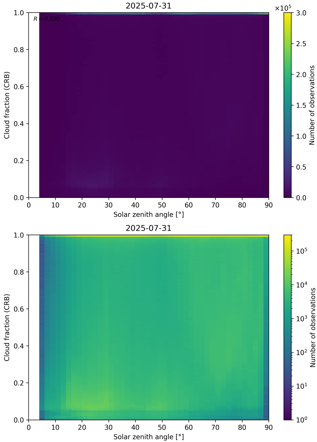
Figure 101: Scatter density plot of “Solar zenith angle” against “Cloud fraction (CRB)” for 2025-07-30 to 2025-08-01.
