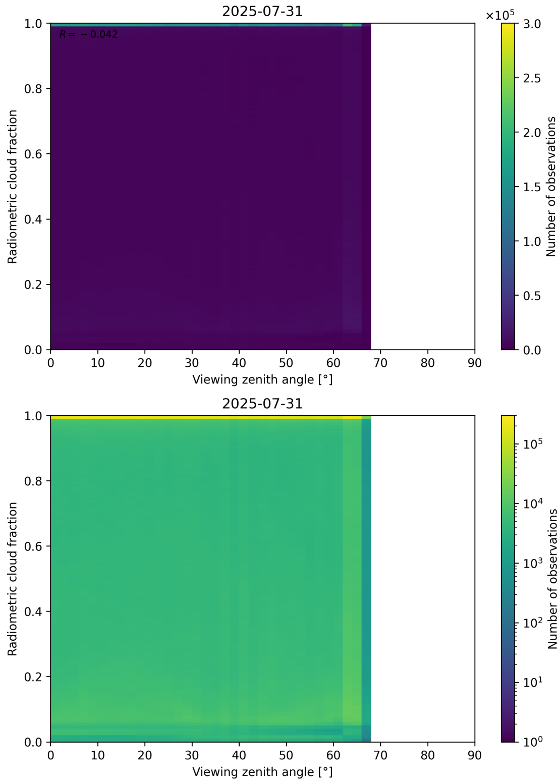
Figure 107: Scatter density plot of “Viewing zenith angle” against “Radiometric cloud fraction” for 2025-07-30 to 2025-08-01.
