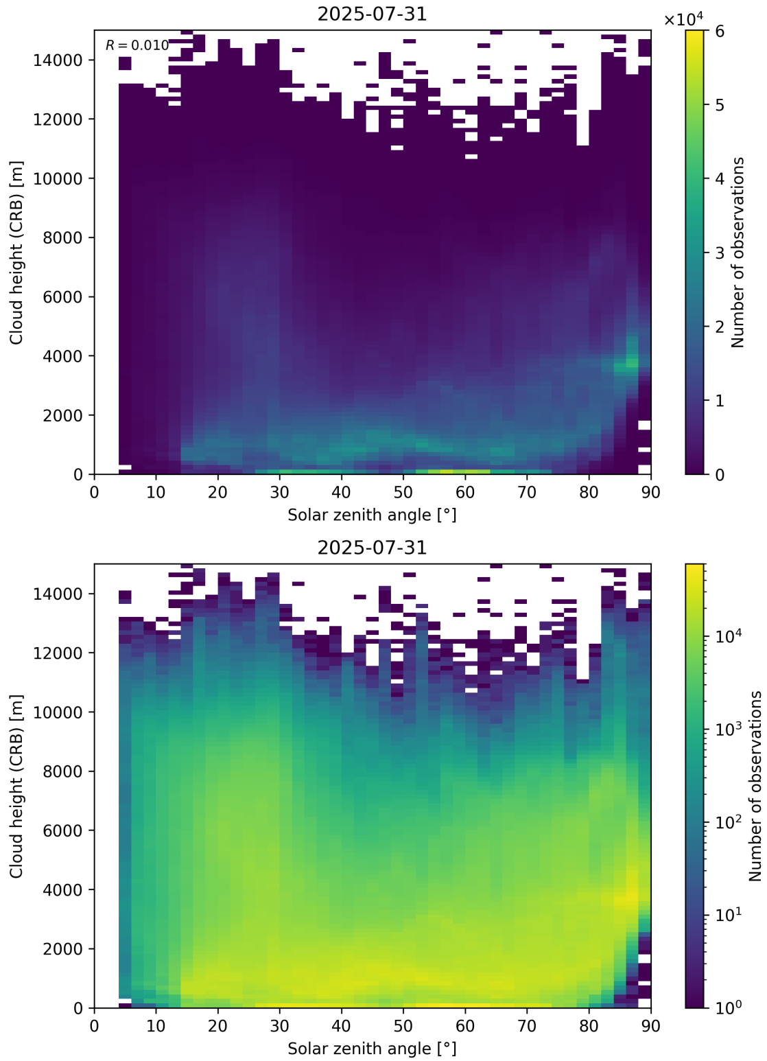
Figure 102: Scatter density plot of “Solar zenith angle” against “Cloud height (CRB)” for 2025-07-30 to 2025-08-01.
