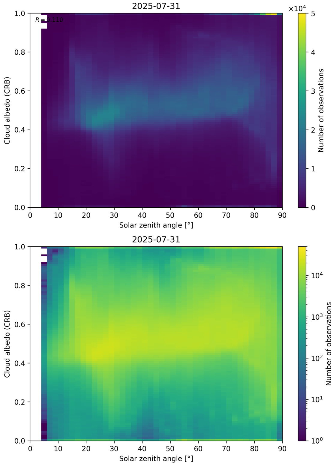
Figure 98: Scatter density plot of “Solar zenith angle” against “Cloud albedo (CRB)” for 2025-07-30 to 2025-08-01.
