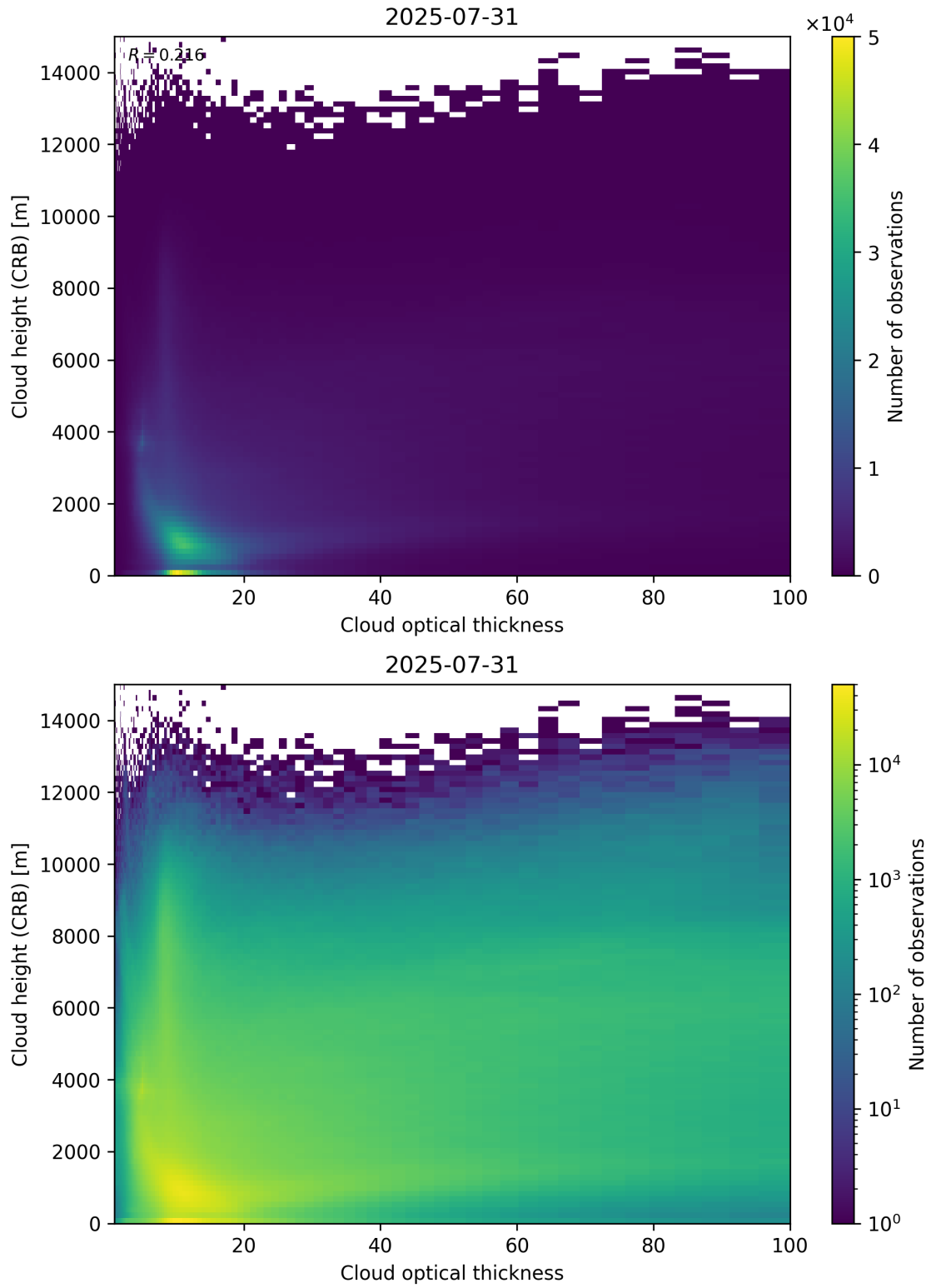
Figure 85: Scatter density plot of “Cloud optical thickness” against “Cloud height (CRB)” for 2025-07-30 to 2025-08-01.
