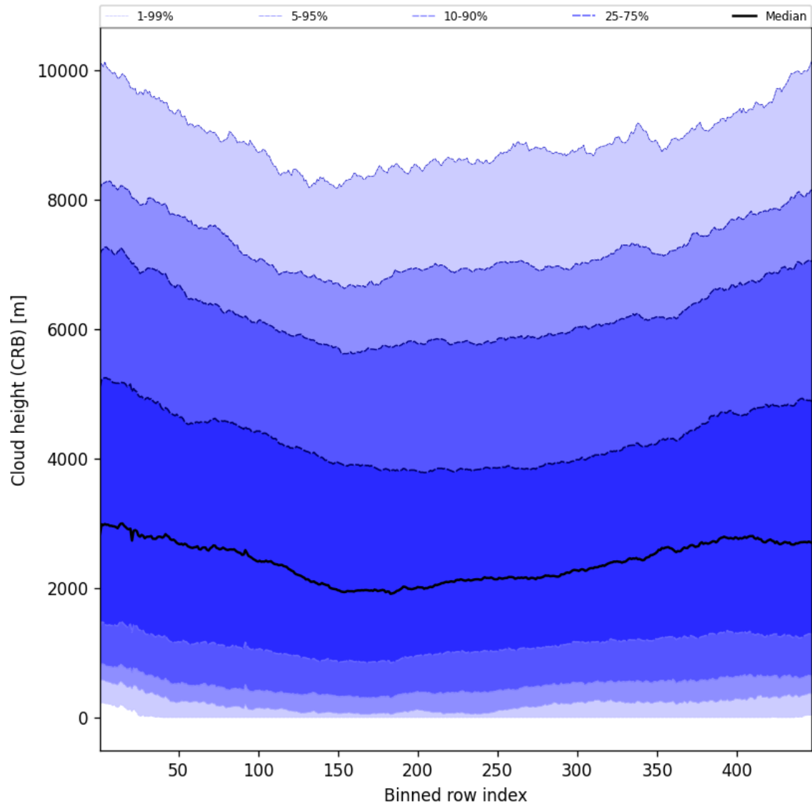
Figure 59: Along track statistics of “Cloud height (CRB)” for 2025-07-30 to 2025-08-01
