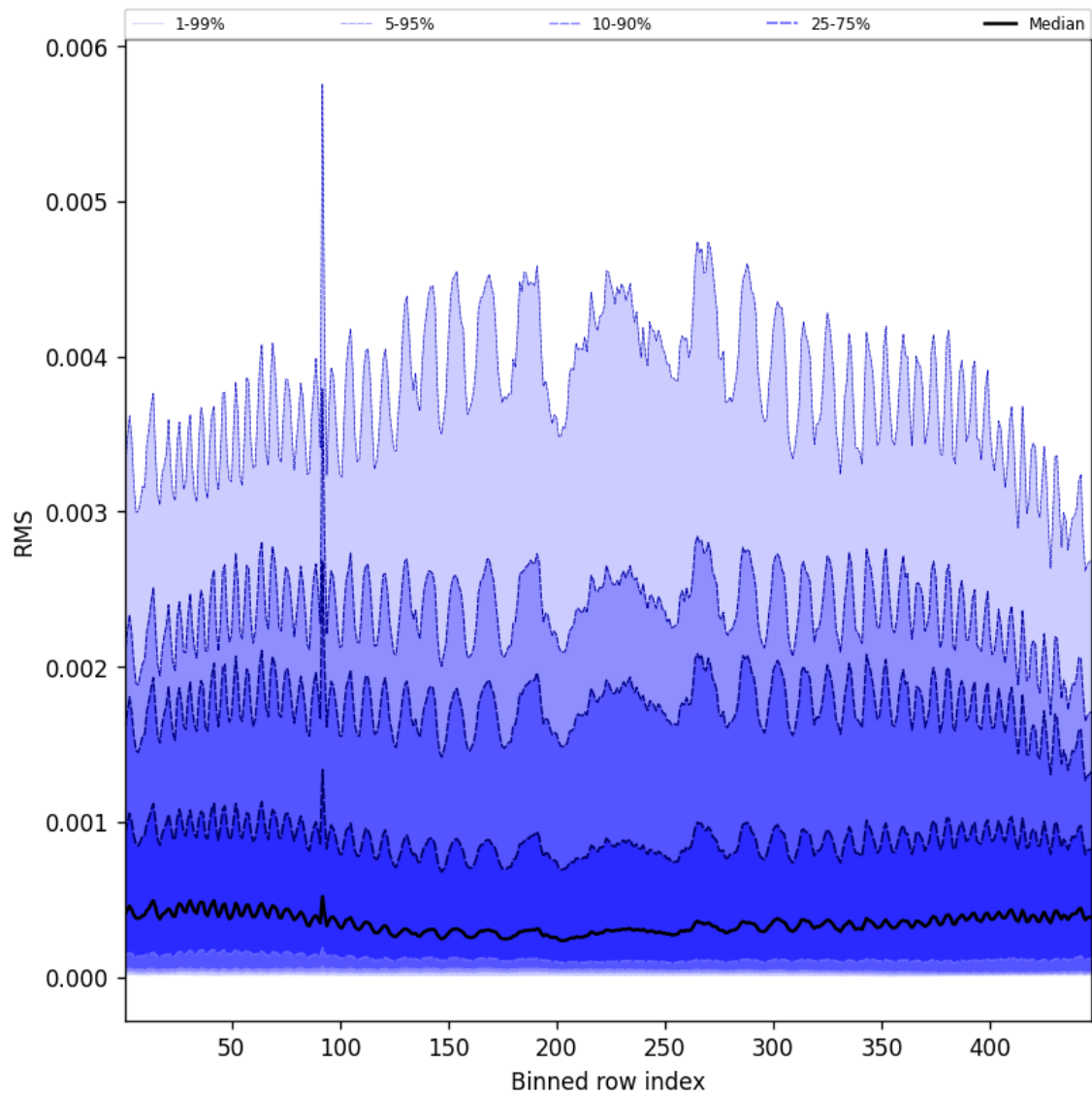
Figure 63: Along track statistics of “RMS” for 2025-07-30 to 2025-08-01
