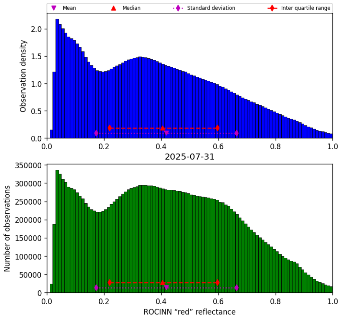
Figure 53: Histogram of “ROCINN “red” reflectance” for 2025-07-30 to 2025-08-01
