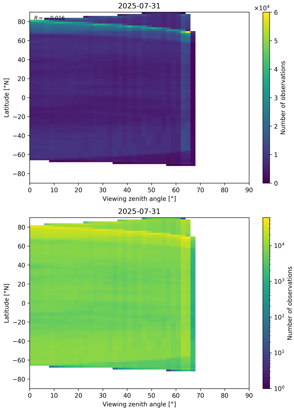
Figure 113: Scatter density plot of “Viewing zenith angle” against “Latitude” for 2025-07-30 to 2025-08-01.
