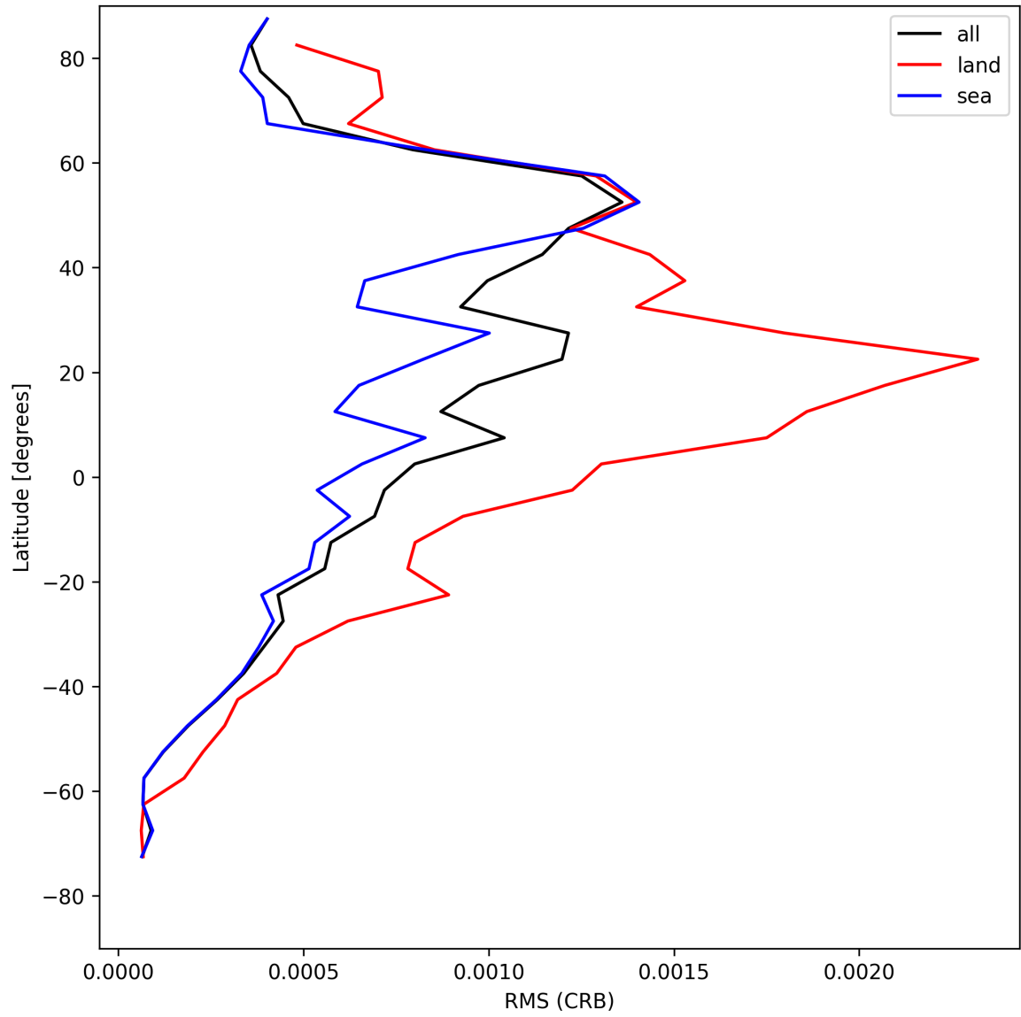
Figure 32: Zonal average of “RMS (CRB)” for 2025-07-30 to 2025-08-01.
