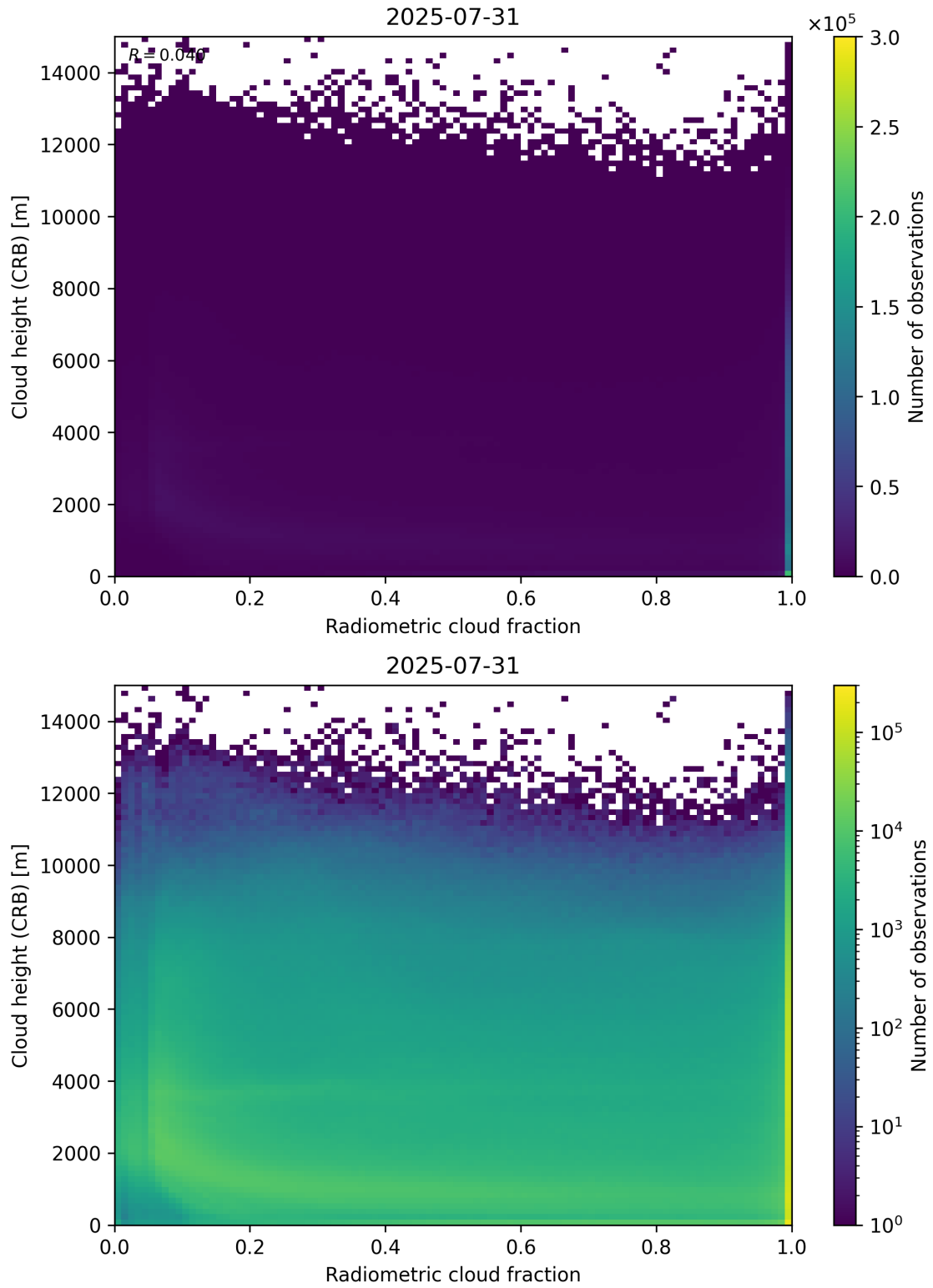
Figure 74: Scatter density plot of “Radiometric cloud fraction” against “Cloud height (CRB)” for 2025-07-30 to 2025-08-01.
