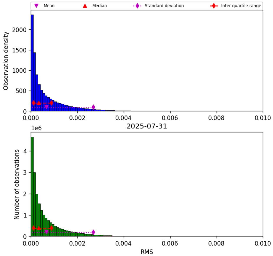
Figure 47: Histogram of “RMS” for 2025-07-30 to 2025-08-01
