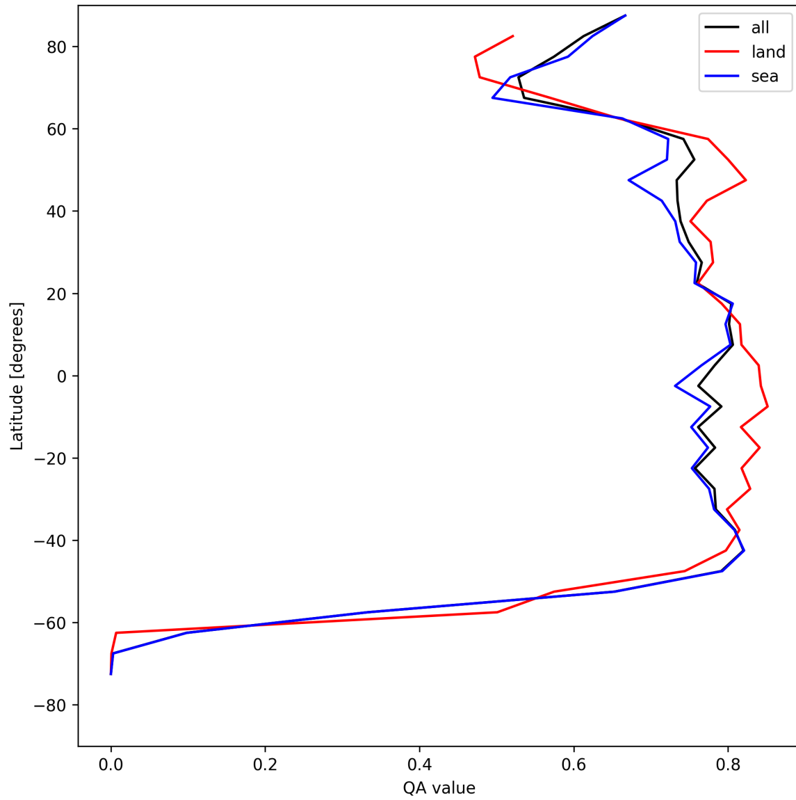
Figure 22: Zonal average of “QA value” for 2025-07-30 to 2025-08-01.
