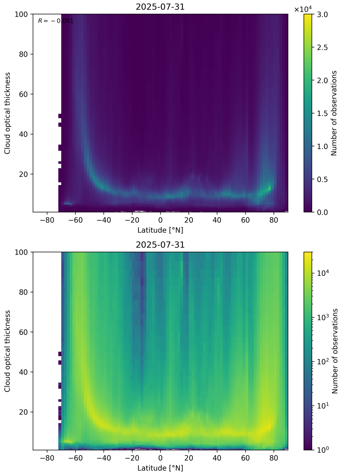
Figure 96: Scatter density plot of “Latitude” against “Cloud optical thickness” for 2025-07-30 to 2025-08-01.
