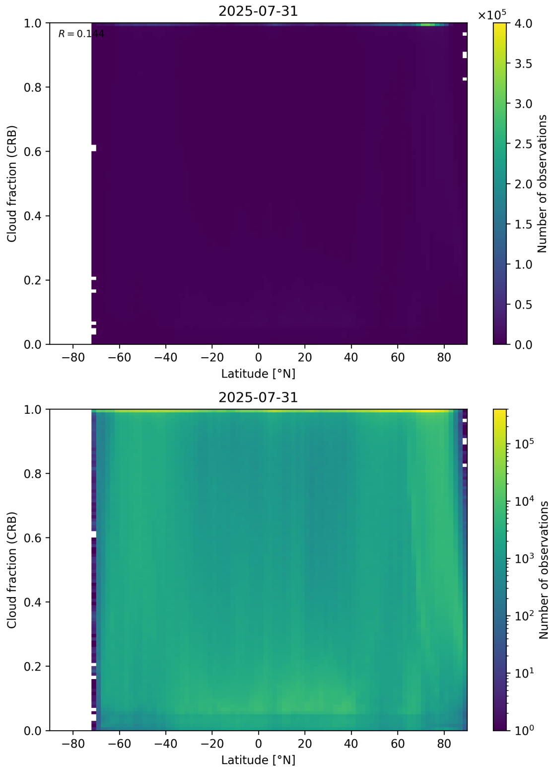
Figure 94: Scatter density plot of “Latitude” against “Cloud fraction (CRB)” for 2025-07-30 to 2025-08-01.
