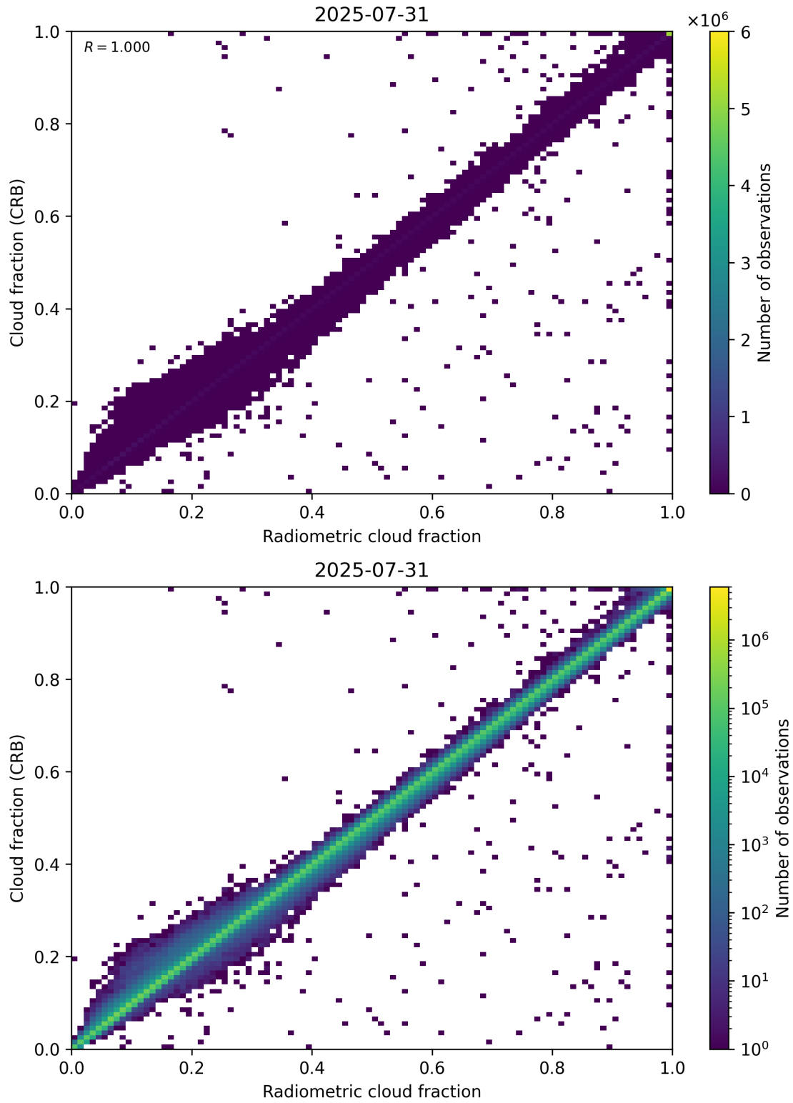
Figure 73: Scatter density plot of “Radiometric cloud fraction” against “Cloud fraction (CRB)” for 2025-07-30 to 2025-08-01.
