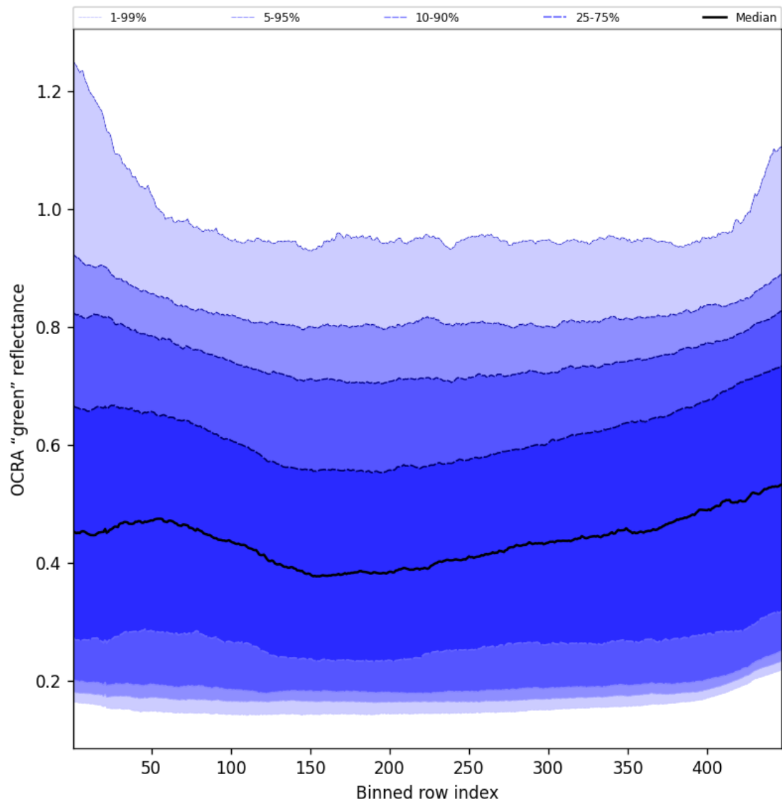
Figure 68: Along track statistics of “OCRA “green” reflectance” for 2025-07-30 to 2025-08-01
