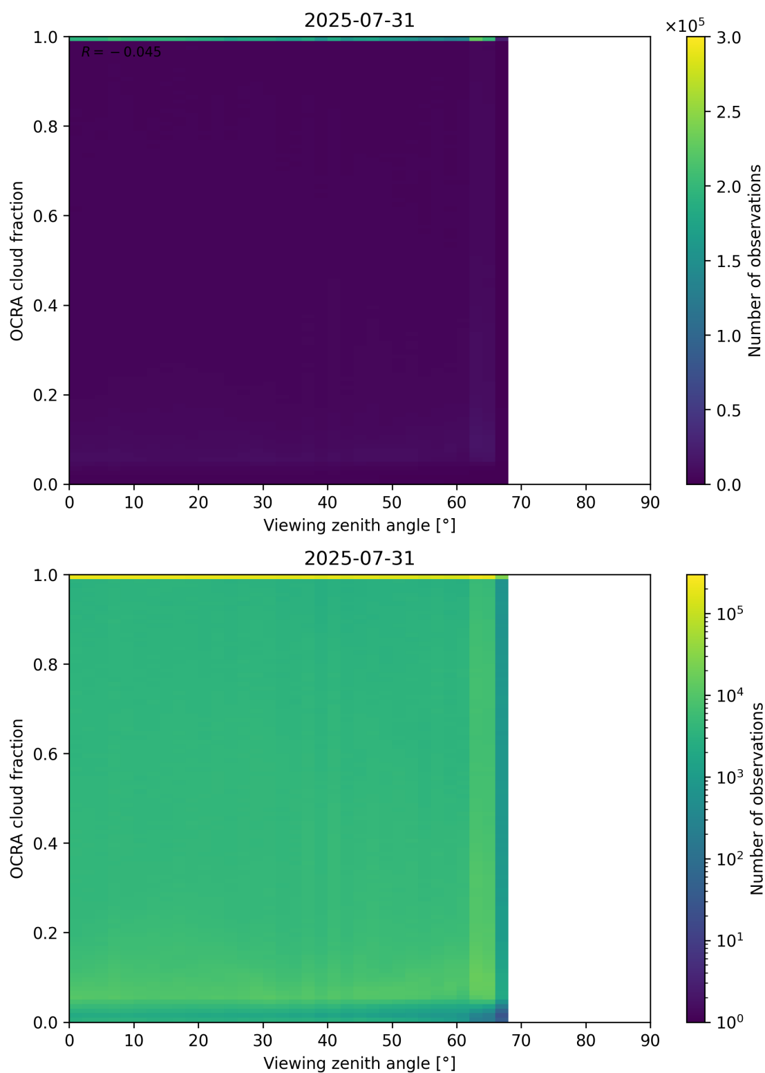
Figure 108: Scatter density plot of “Viewing zenith angle” against “OCRA cloud fraction” for 2025-07-30 to 2025-08-01.
