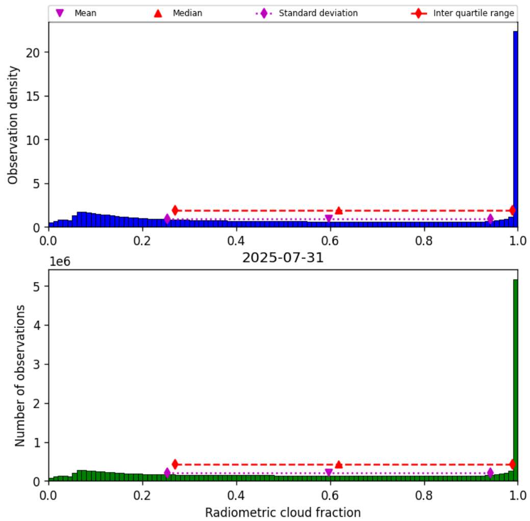
Figure 39: Histogram of “Radiometric cloud fraction” for 2025-07-30 to 2025-08-01
