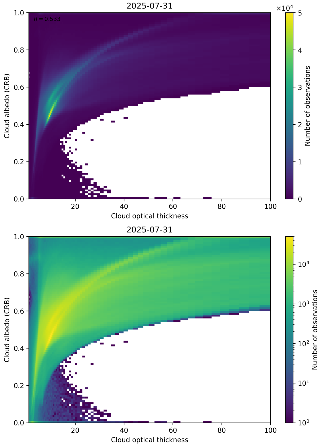
Figure 82: Scatter density plot of “Cloud optical thickness” against “Cloud albedo (CRB)” for 2025-07-30 to 2025-08-01.
