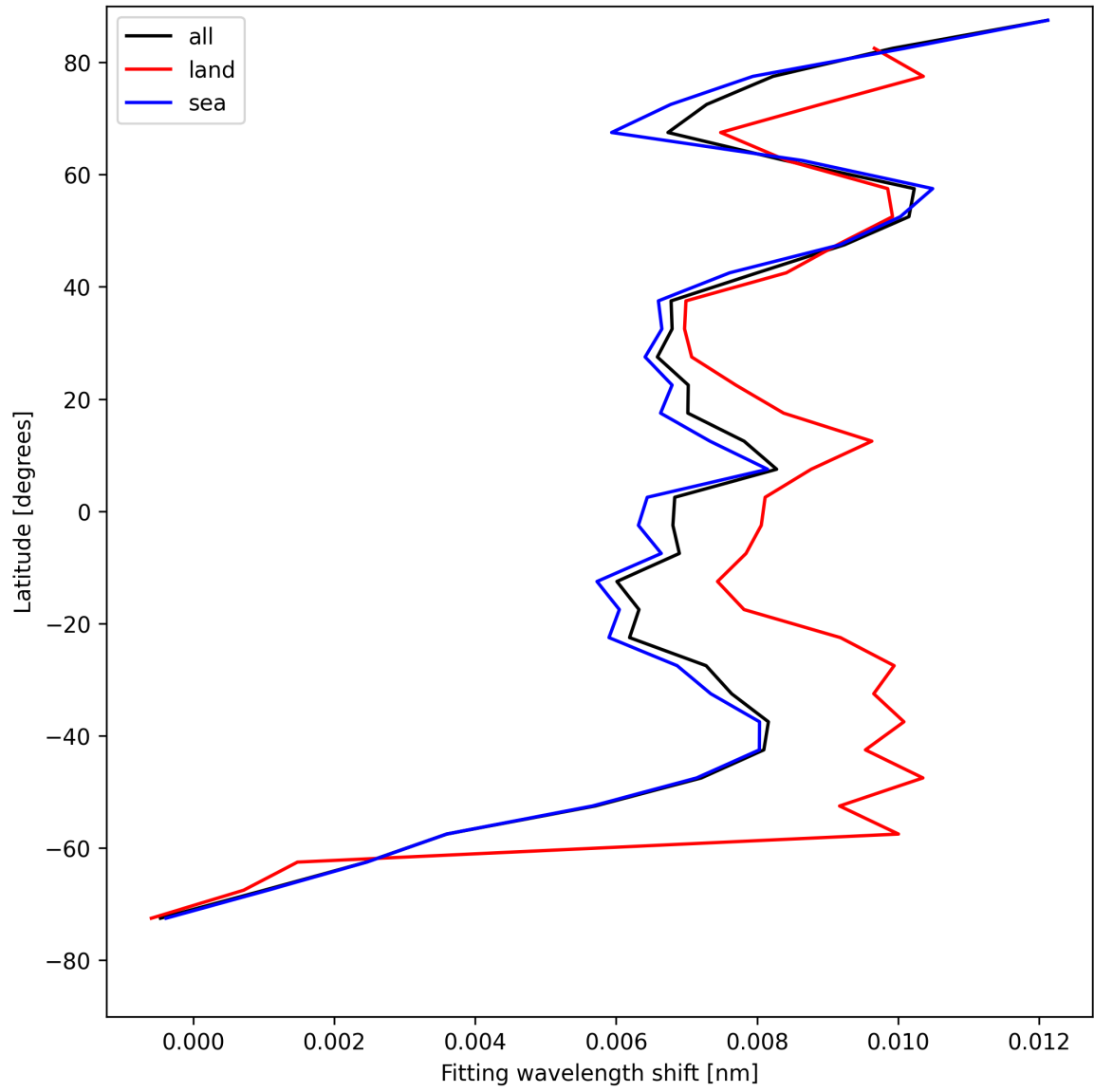
Figure 33: Zonal average of “Fitting wavelength shift” for 2025-07-30 to 2025-08-01.
