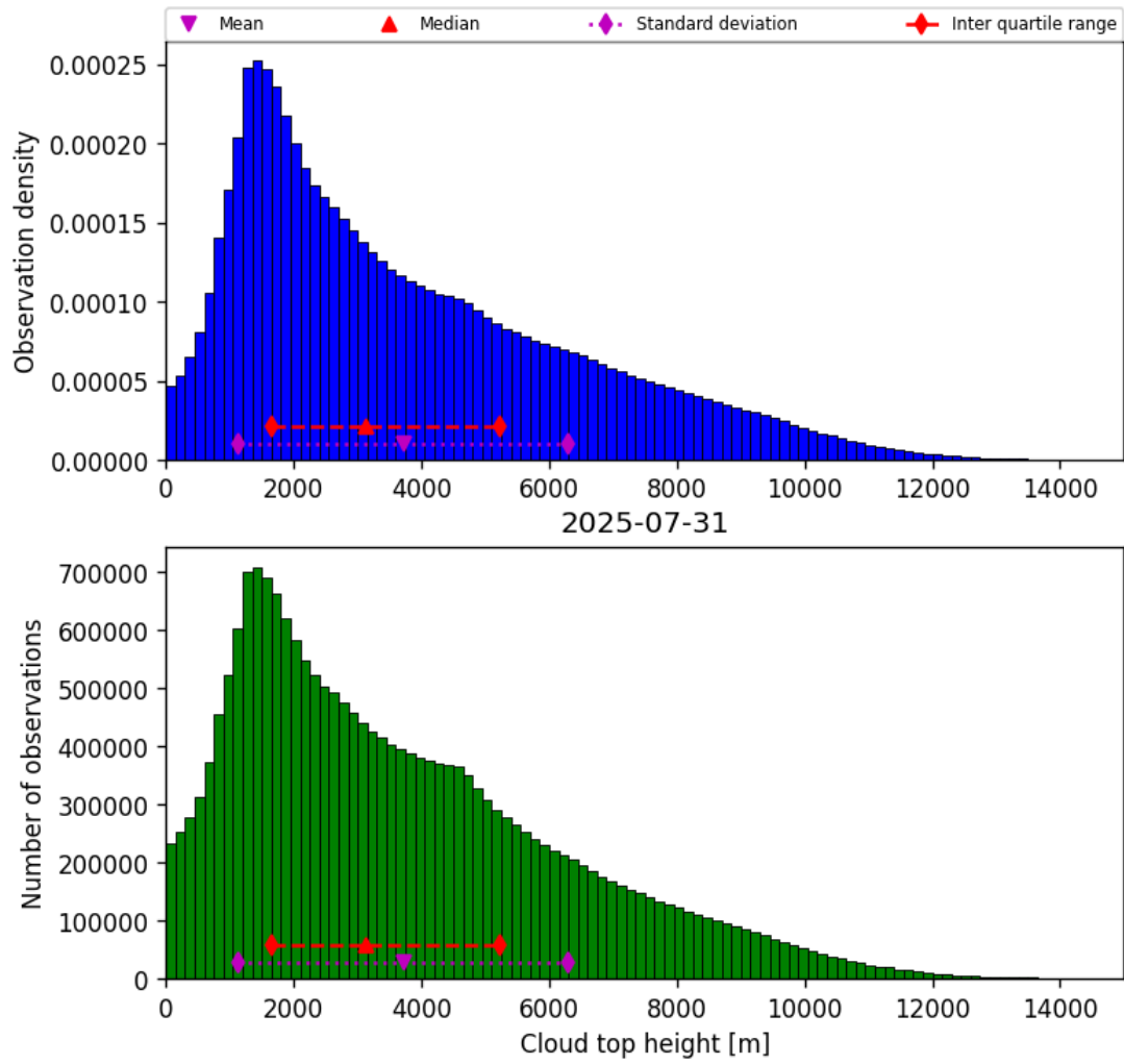
Figure 40: Histogram of “Cloud top height” for 2025-07-30 to 2025-08-01
