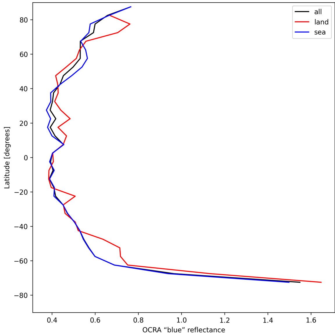
Figure 35: Zonal average of "OCRA "blue" reflectance" for 2025-07-30 to 2025-08-01.
