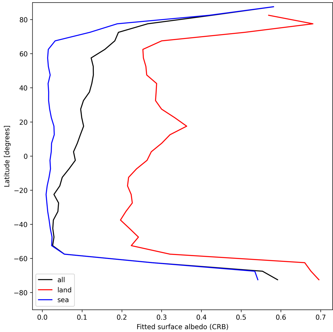
Figure 30: Zonal average of “Fitted surface albedo (CRB)” for 2025-07-30 to 2025-08-01.
