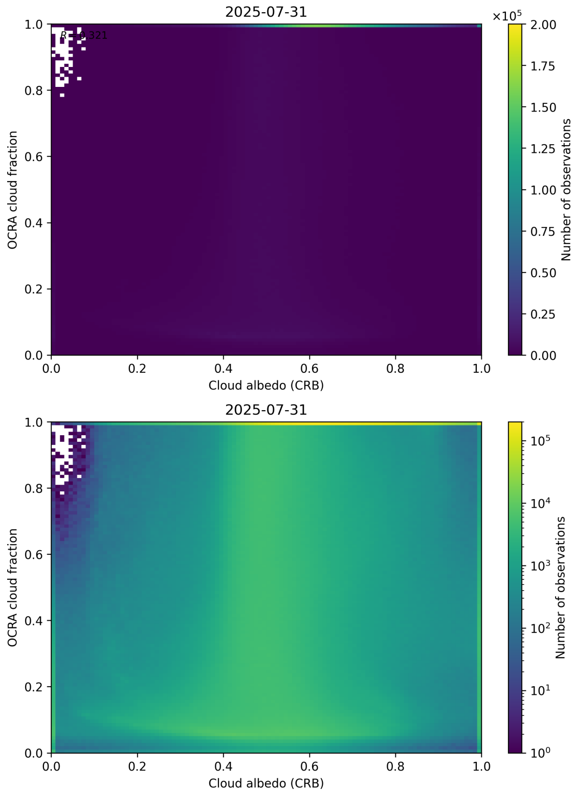
Figure 70: Scatter density plot of “Cloud albedo (CRB)” against “OCRA cloud fraction” for 2025-07-30 to 2025-08-01.
