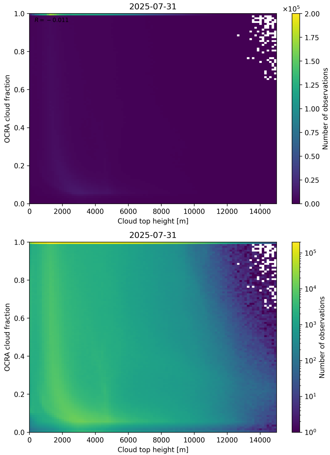
Figure 87: Scatter density plot of “Cloud top height” against “OCRA cloud fraction” for 2025-07-30 to 2025-08-01.
