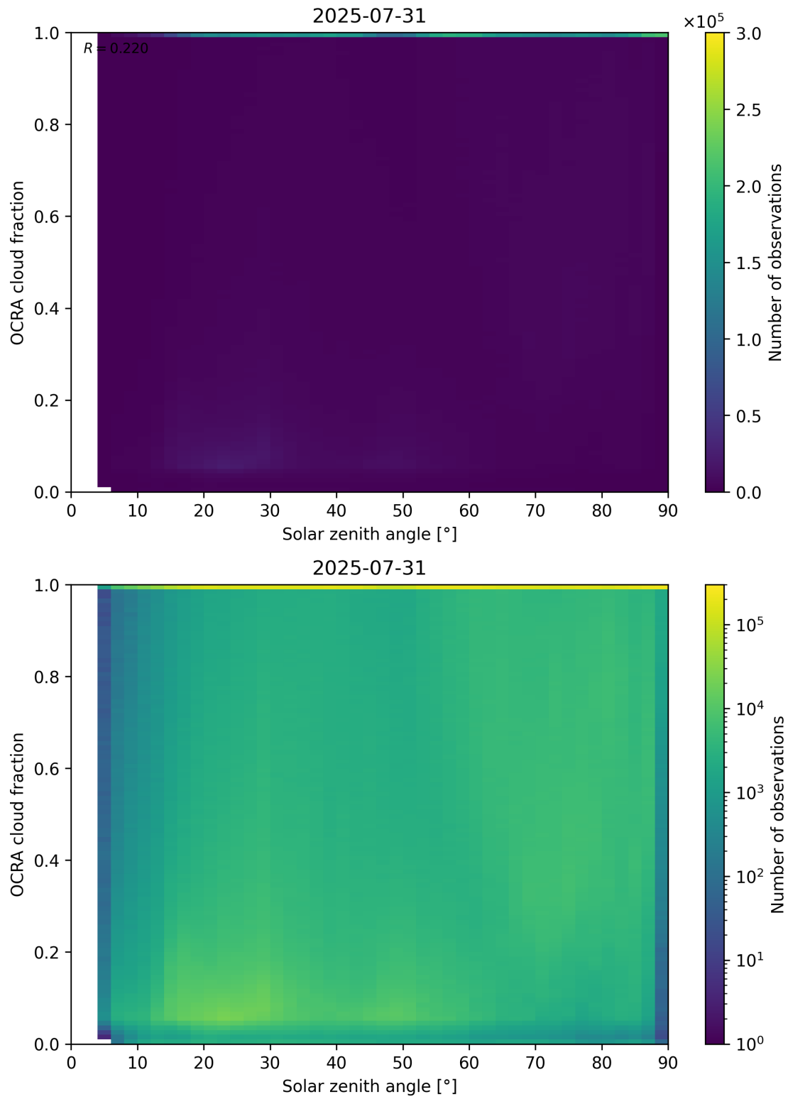
Figure 100: Scatter density plot of “Solar zenith angle” against “OCRA cloud fraction” for 2025-07-30 to 2025-08-01.
