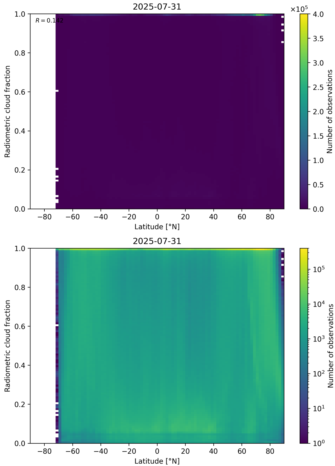
Figure 92: Scatter density plot of “Latitude” against “Radiometric cloud fraction” for 2025-07-30 to 2025-08-01.
