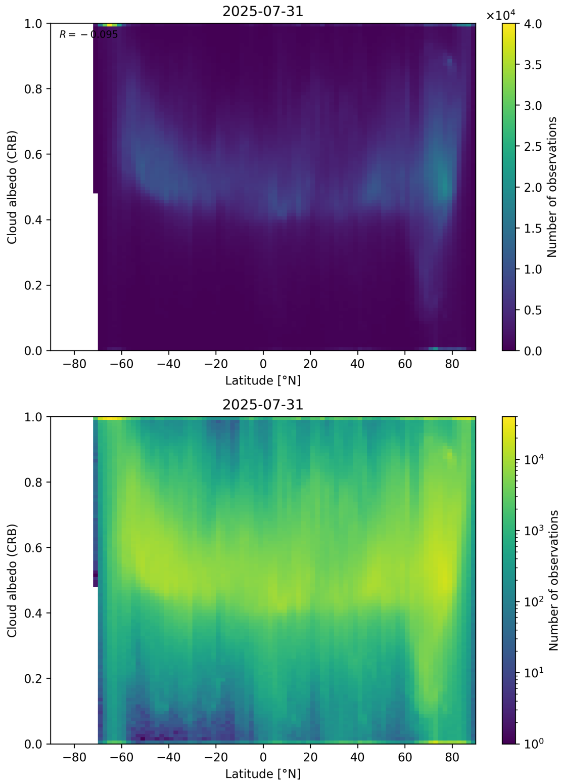
Figure 91: Scatter density plot of “Latitude” against “Cloud albedo (CRB)” for 2025-07-30 to 2025-08-01.
