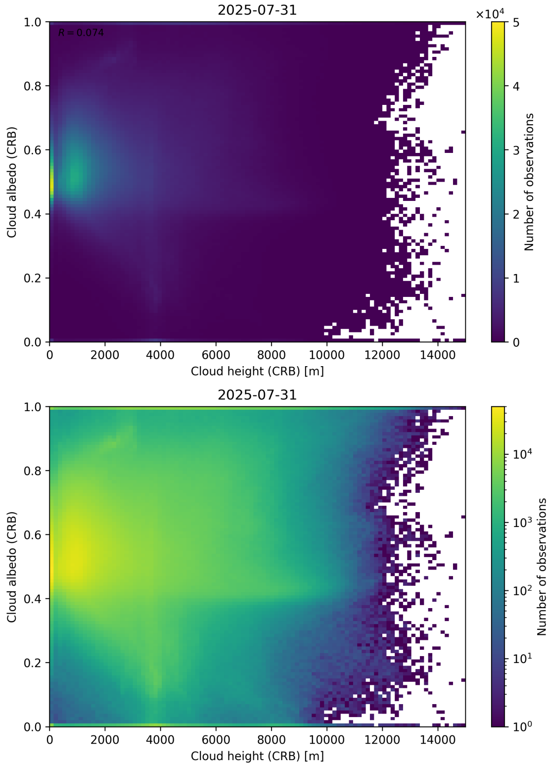
Figure 80: Scatter density plot of “Cloud height (CRB)” against “Cloud albedo (CRB)” for 2025-07-30 to 2025-08-01.
