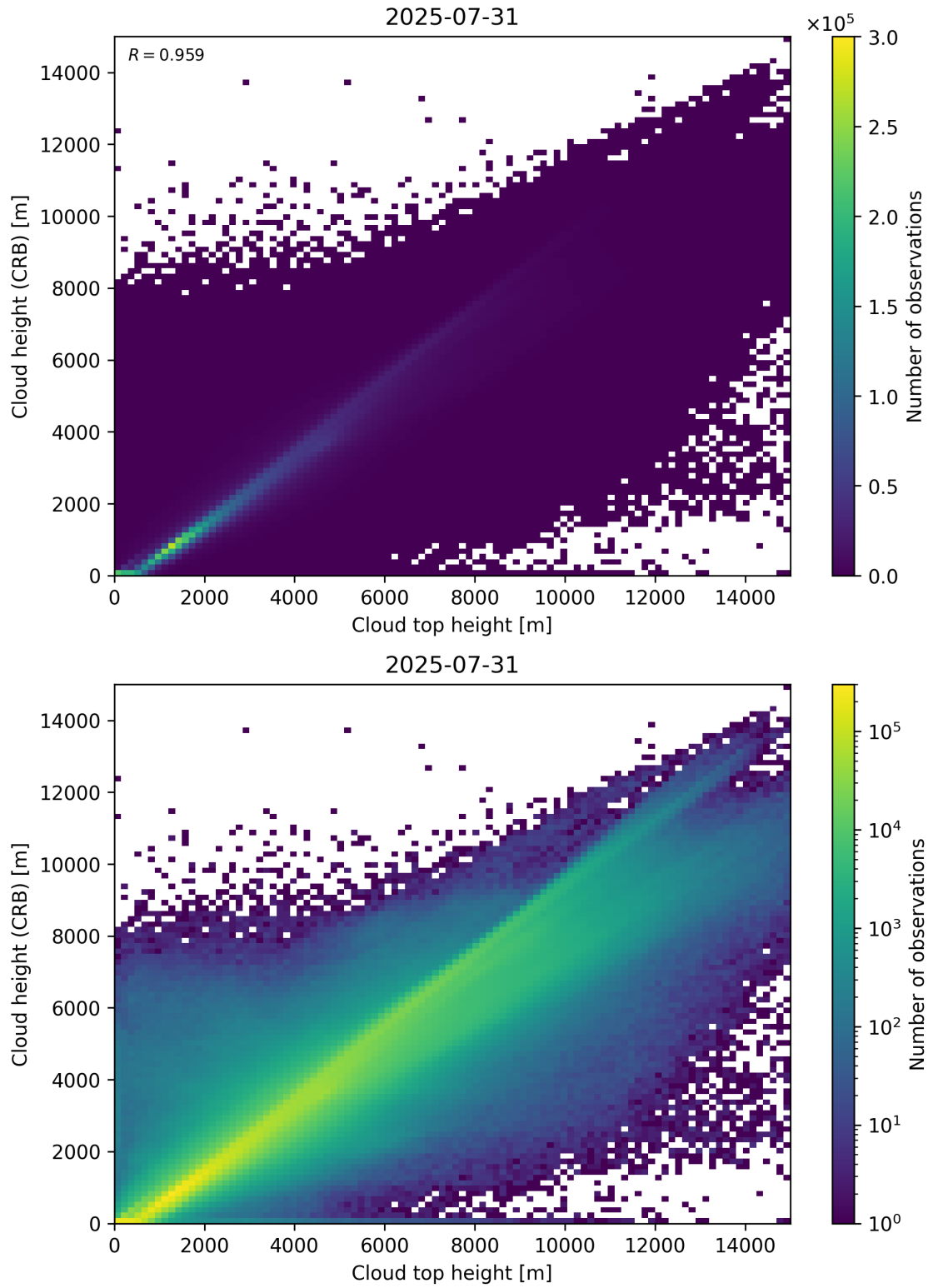
Figure 89: Scatter density plot of “Cloud top height” against “Cloud height (CRB)” for 2025-07-30 to 2025-08-01.
