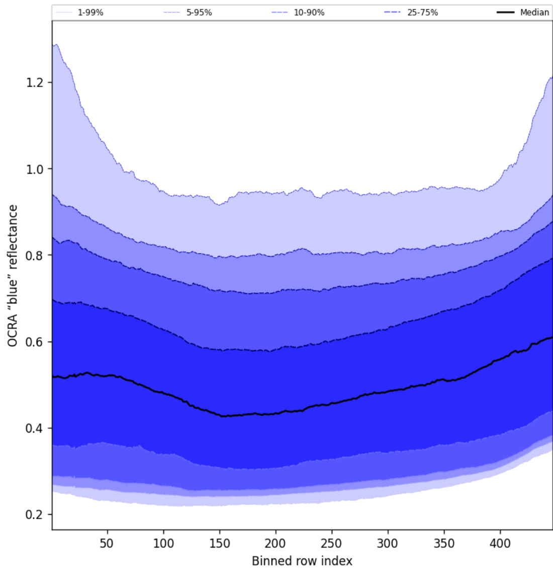
Figure 67: Along track statistics of “OCRA “blue” reflectance” for 2025-07-30 to 2025-08-01
