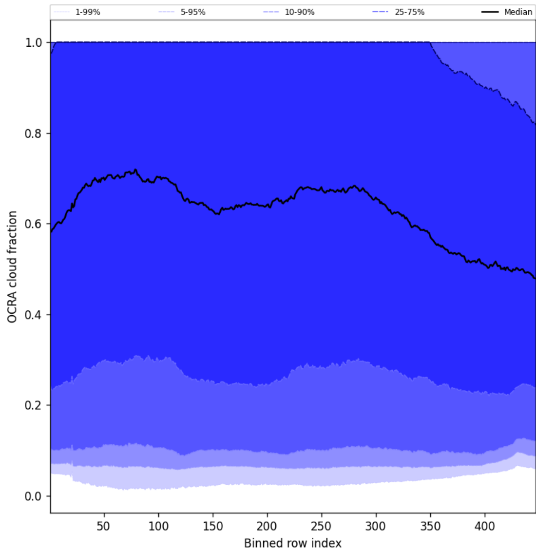
Figure 66: Along track statistics of “OCRA cloud fraction” for 2025-07-30 to 2025-08-01
