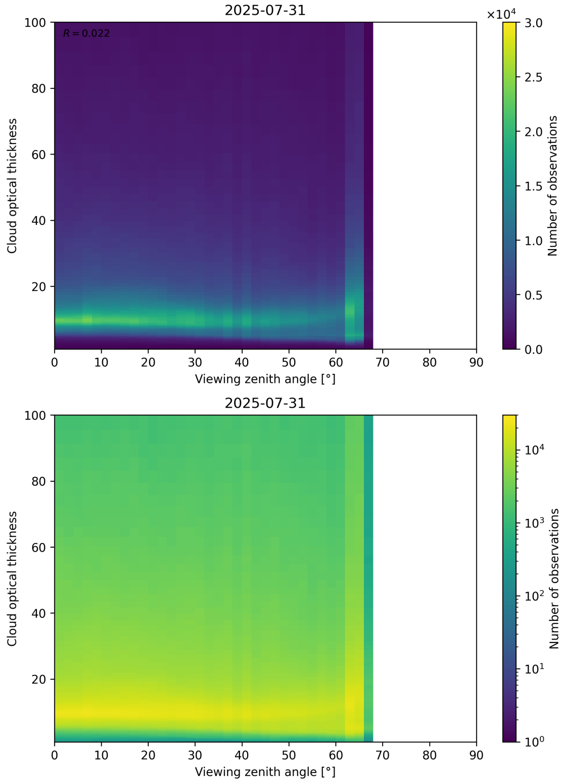
Figure 111: Scatter density plot of “Viewing zenith angle” against “Cloud optical thickness” for 2025-07-30 to 2025-08-01.
