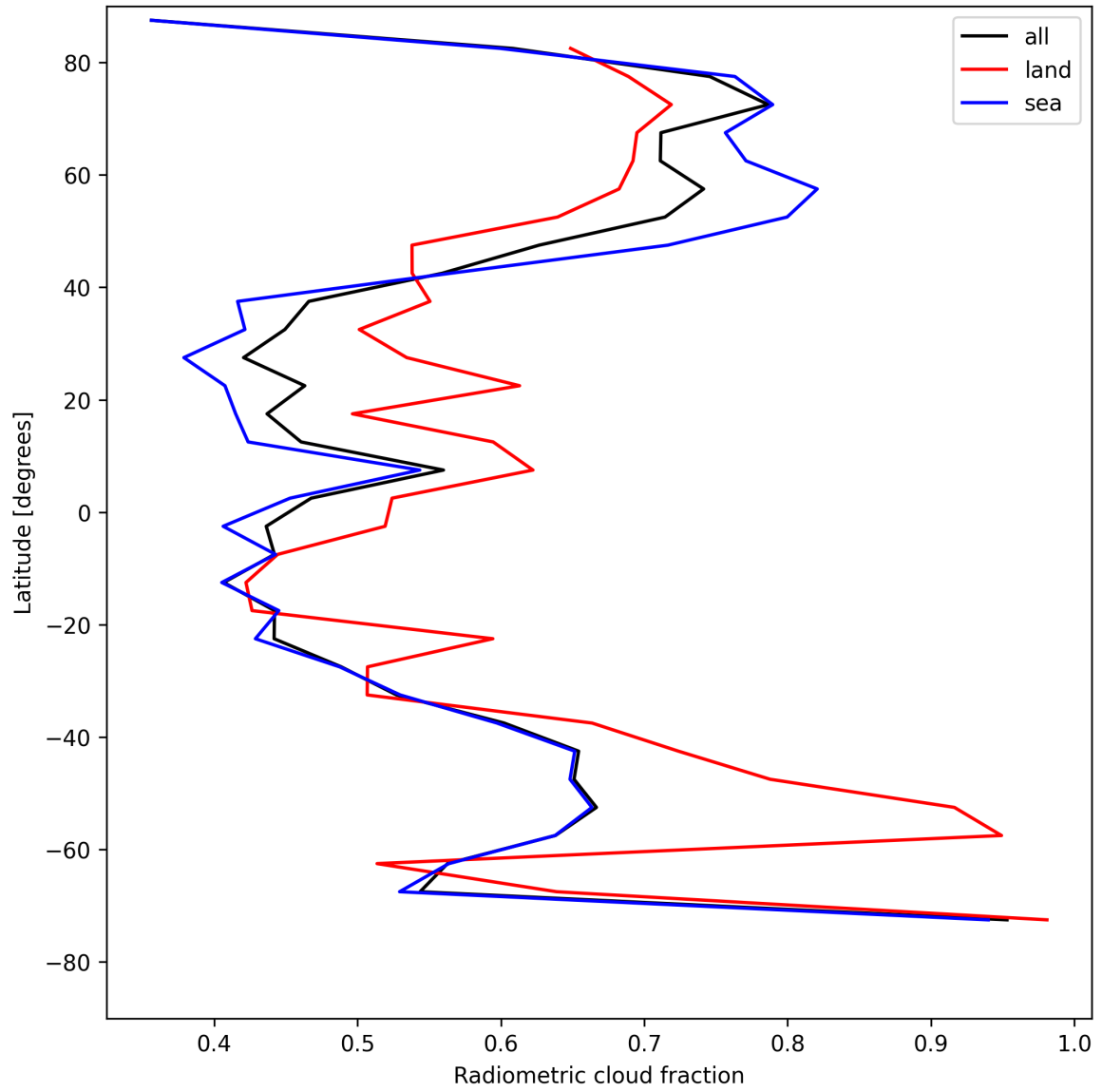
Figure 23: Zonal average of “Radiometric cloud fraction” for 2025-07-30 to 2025-08-01.
