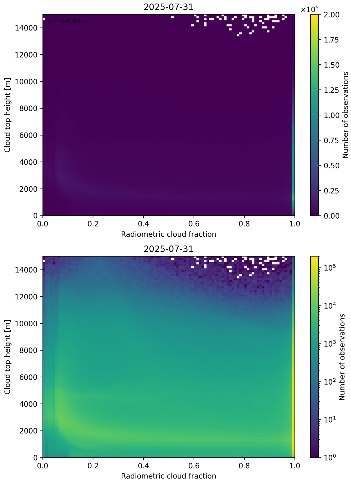
Figure 76: Scatter density plot of “Radiometric cloud fraction” against “Cloud top height” for 2025-07-30 to 2025-08-01.
