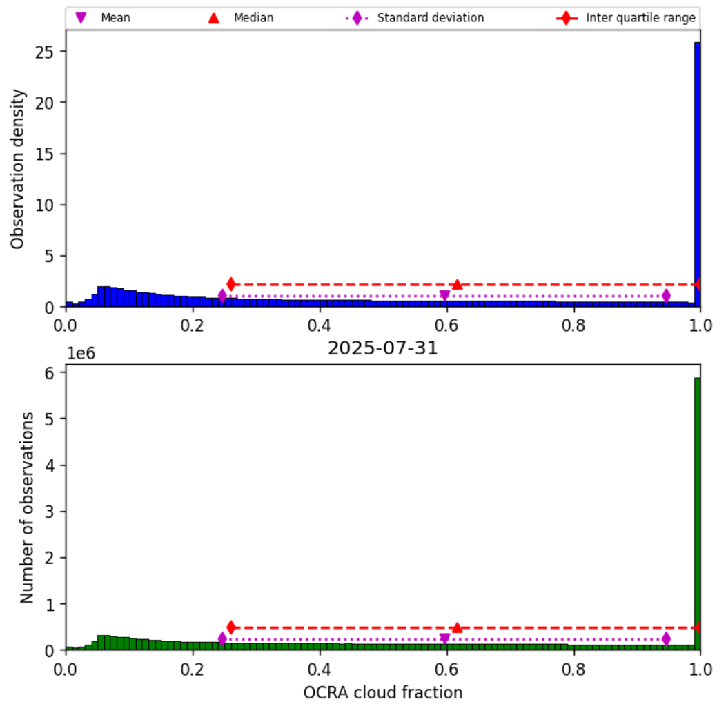
Figure 50: Histogram of “OCRA cloud fraction” for 2025-07-30 to 2025-08-01
