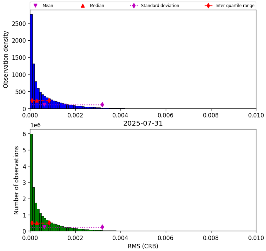
Figure 48: Histogram of “RMS (CRB)” for 2025-07-30 to 2025-08-01
