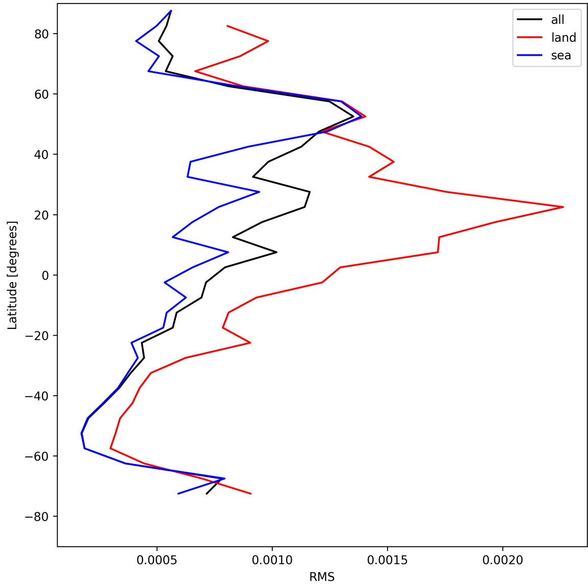
Figure 31: Zonal average of “RMS” for 2025-07-30 to 2025-08-01.
