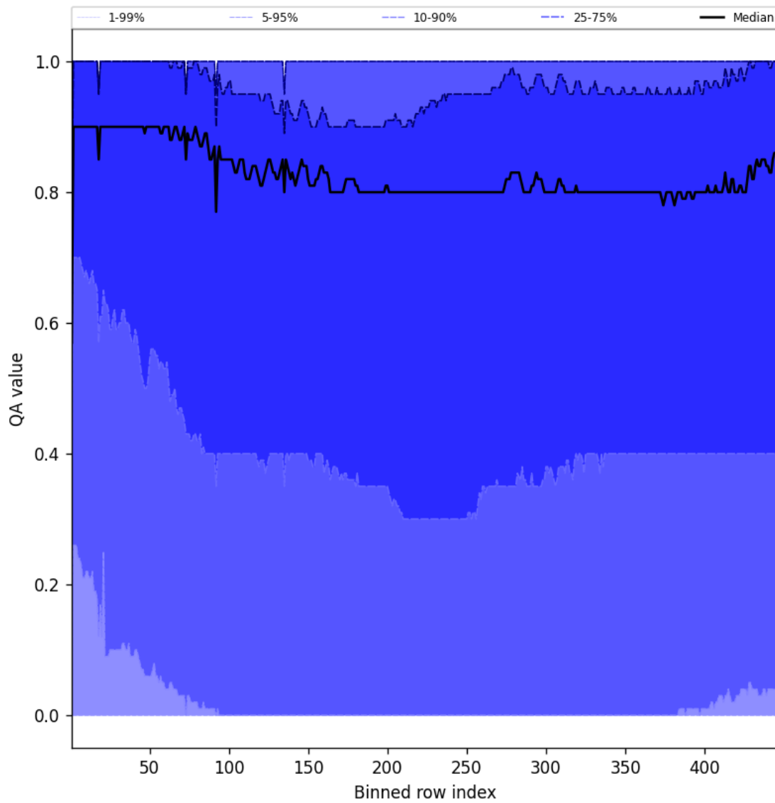
Figure 54: Along track statistics of “QA value” for 2025-07-30 to 2025-08-01
