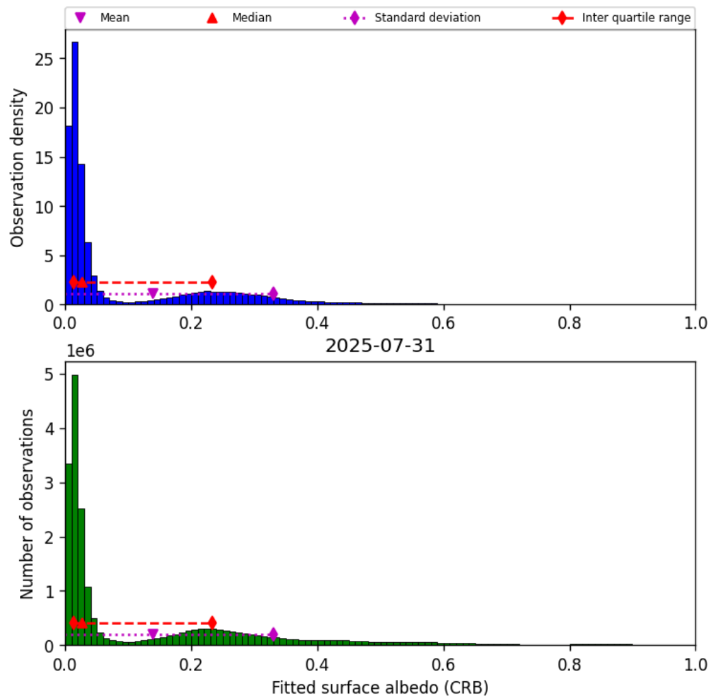
Figure 46: Histogram of “Fitted surface albedo (CRB)” for 2025-07-30 to 2025-08-01
