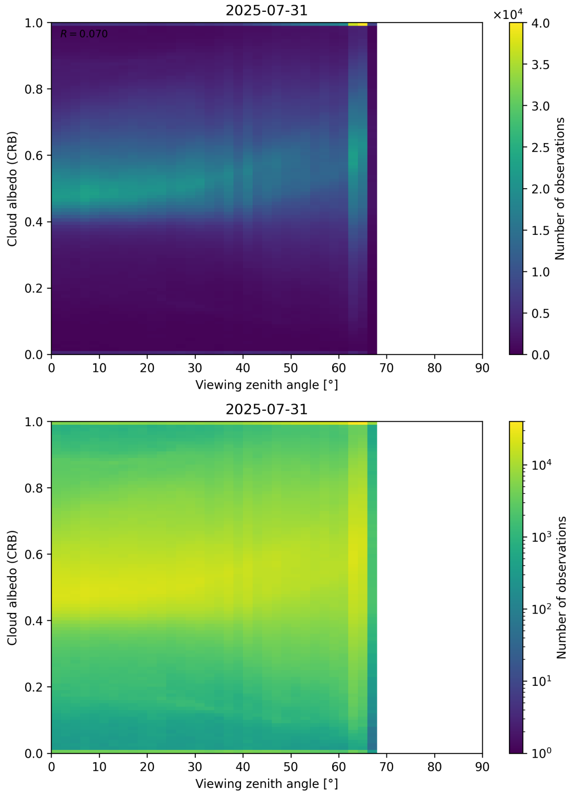
Figure 106: Scatter density plot of “Viewing zenith angle” against “Cloud albedo (CRB)” for 2025-07-30 to 2025-08-01.
