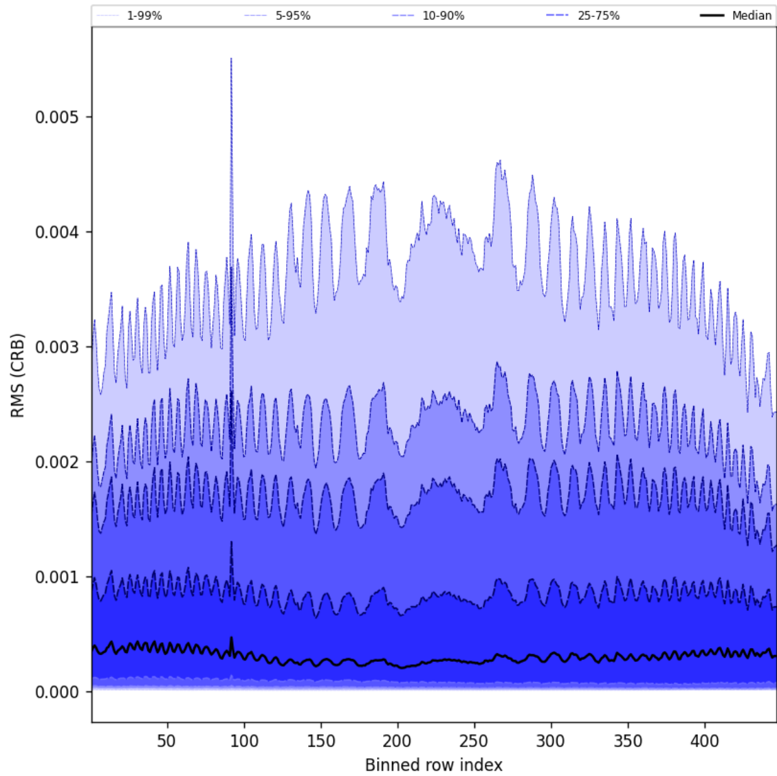
Figure 64: Along track statistics of “RMS (CRB)” for 2025-07-30 to 2025-08-01
