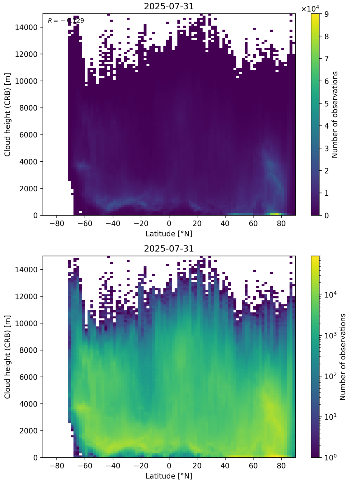
Figure 95: Scatter density plot of “Latitude” against “Cloud height (CRB)” for 2025-07-30 to 2025-08-01.
