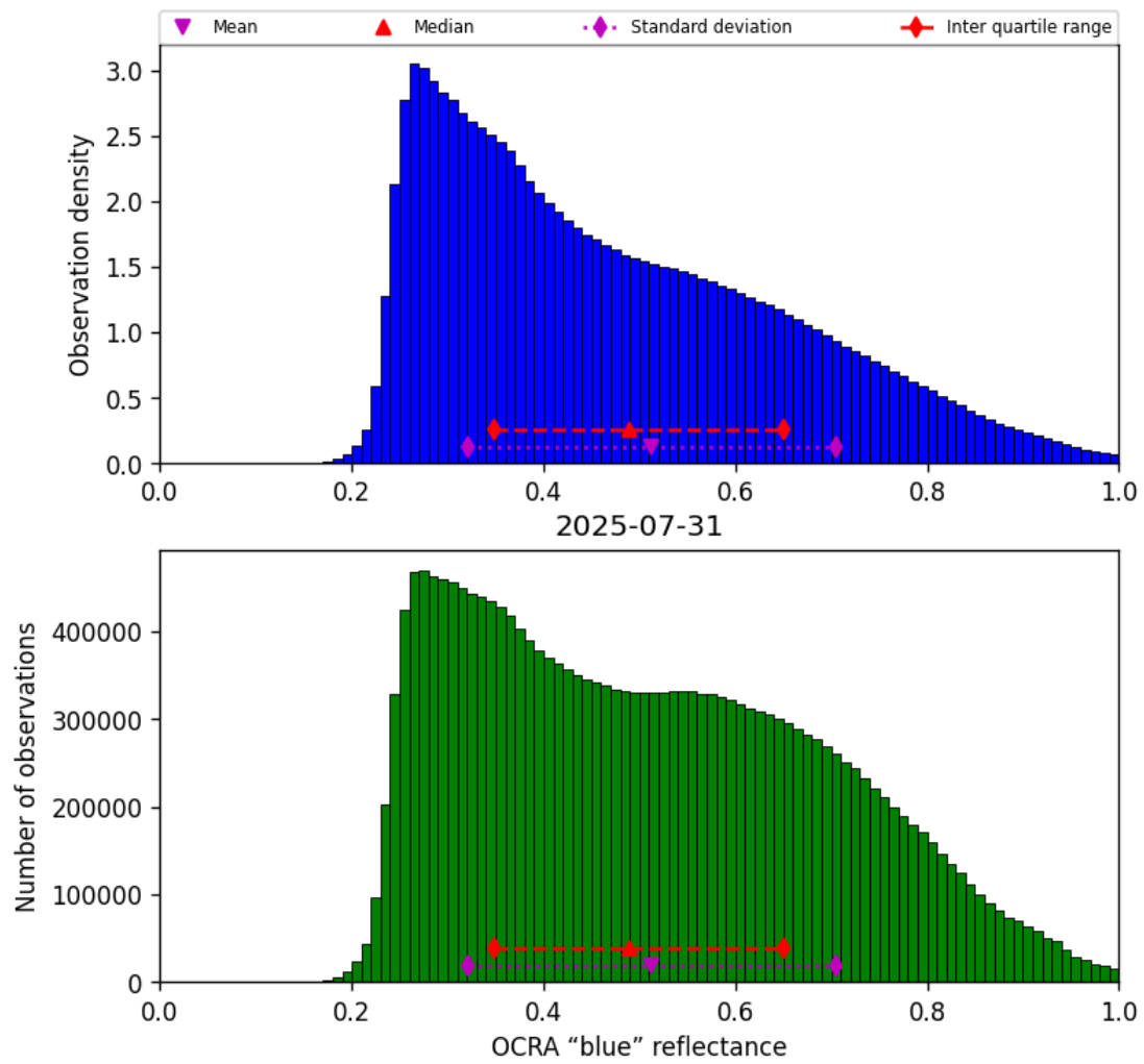
Figure 51: Histogram of “OCRA “blue” reflectance” for 2025-07-30 to 2025-08-01
