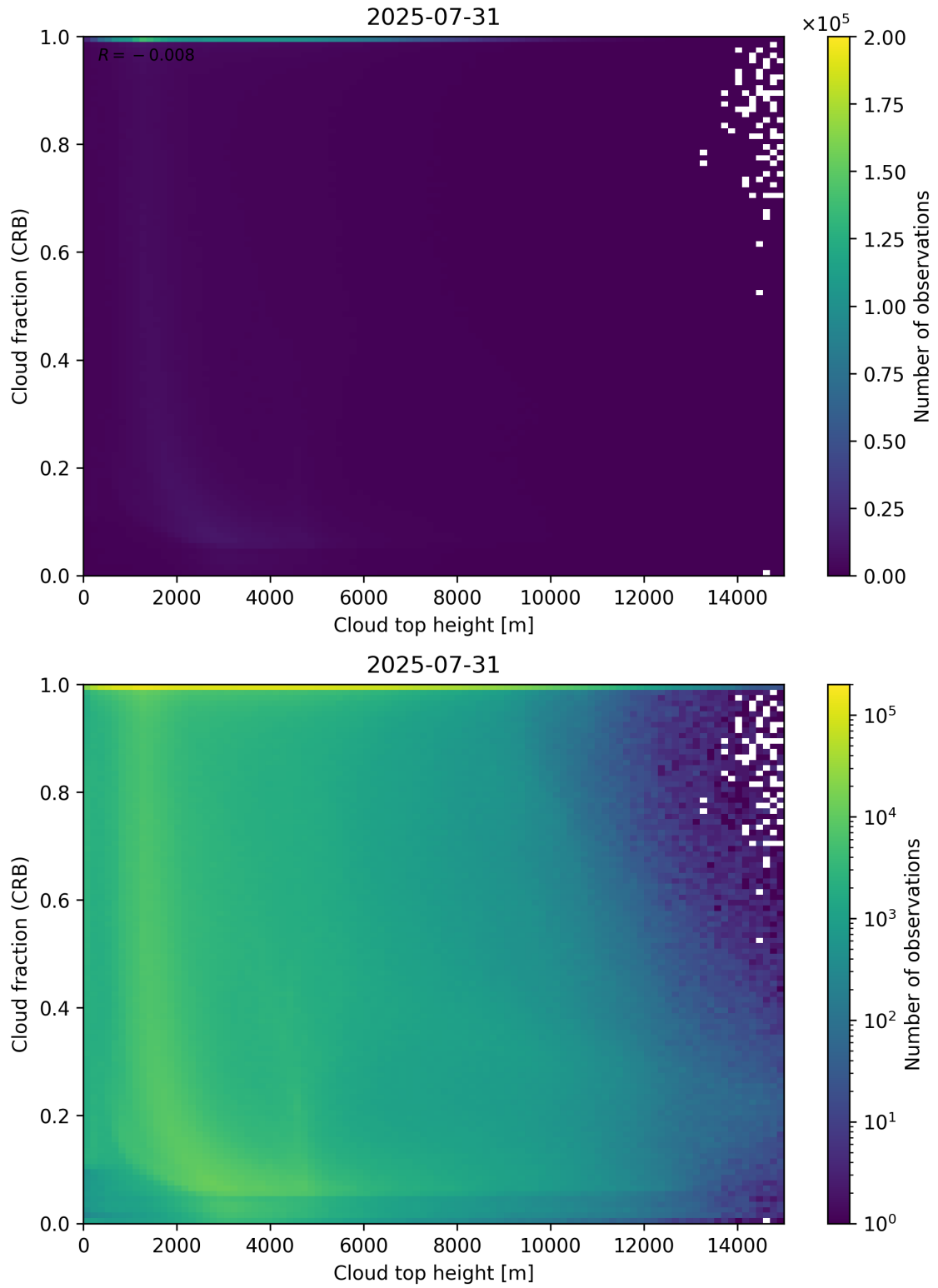
Figure 88: Scatter density plot of “Cloud top height” against “Cloud fraction (CRB)” for 2025-07-30 to 2025-08-01.
