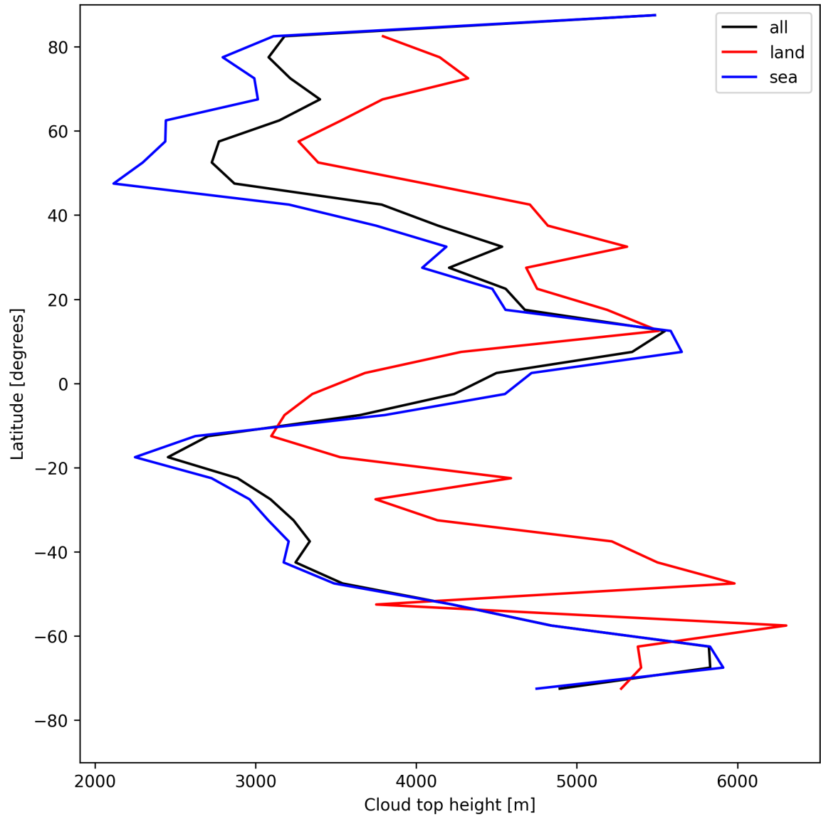
Figure 24: Zonal average of “Cloud top height” for 2025-07-30 to 2025-08-01.
