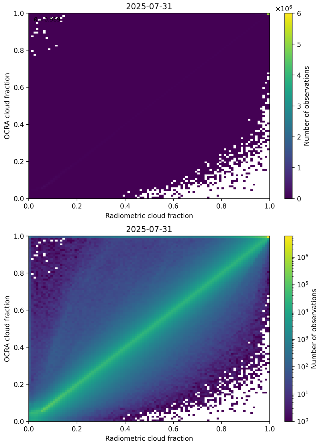
Figure 72: Scatter density plot of “Radiometric cloud fraction” against “OCRA cloud fraction” for 2025-07-30 to 2025-08-01.
