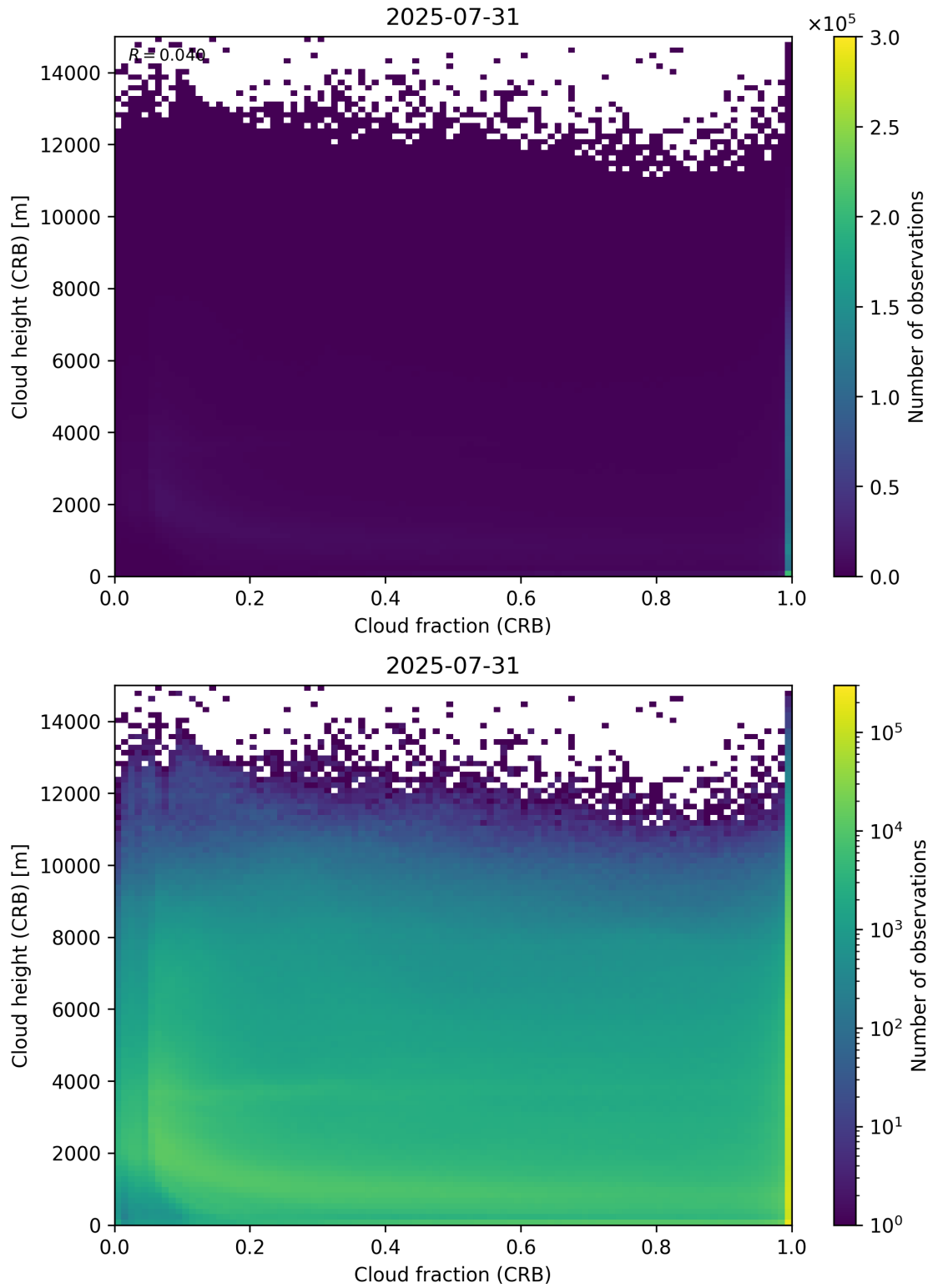
Figure 79: Scatter density plot of “Cloud fraction (CRB)” against “Cloud height (CRB)” for 2025-07-30 to 2025-08-01.
