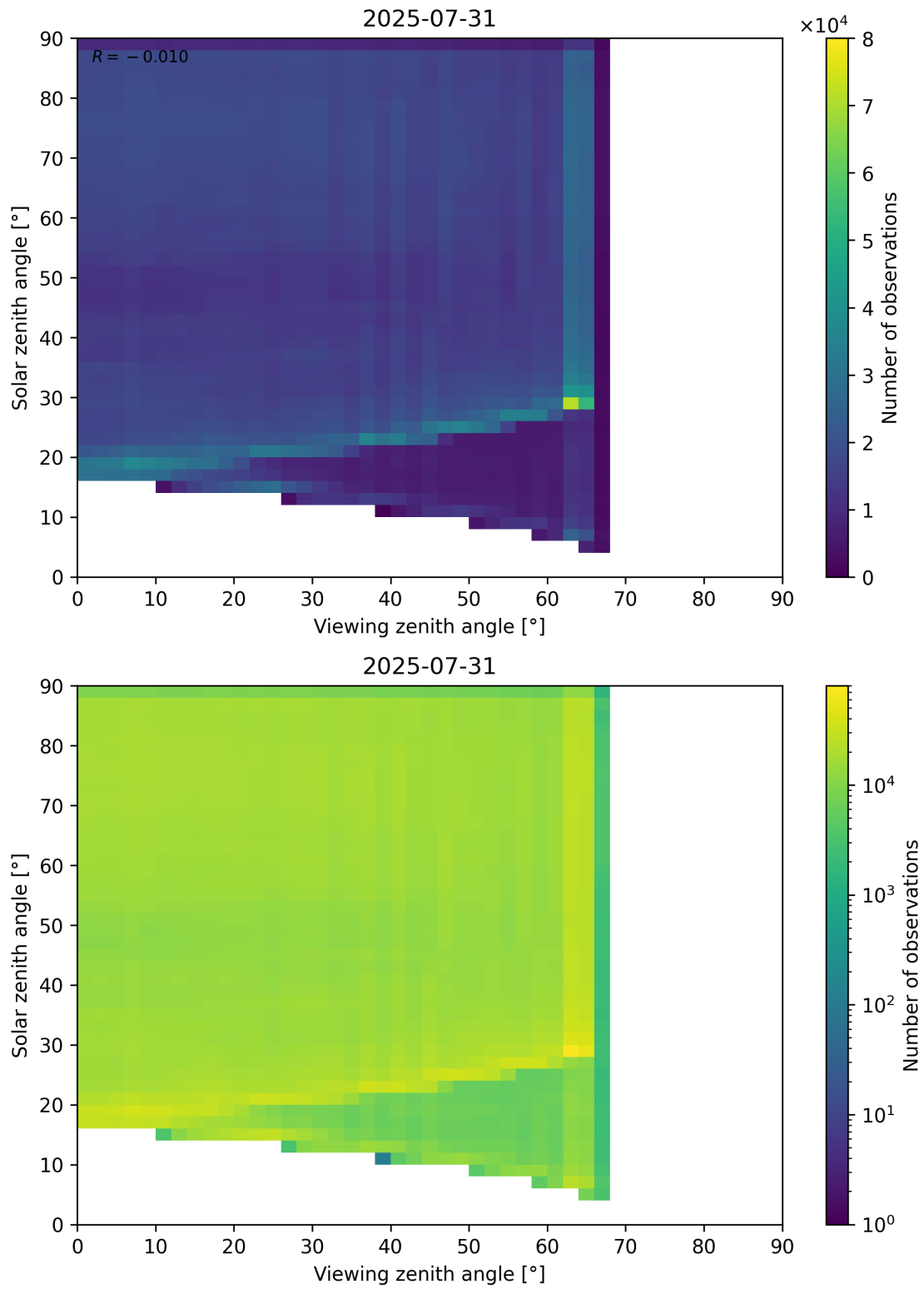
Figure 114: Scatter density plot of “Viewing zenith angle” against “Solar zenith angle” for 2025-07-30 to 2025-08-01.
