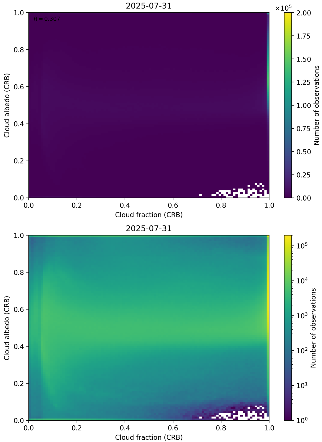
Figure 77: Scatter density plot of “Cloud fraction (CRB)” against “Cloud albedo (CRB)” for 2025-07-30 to 2025-08-01.
