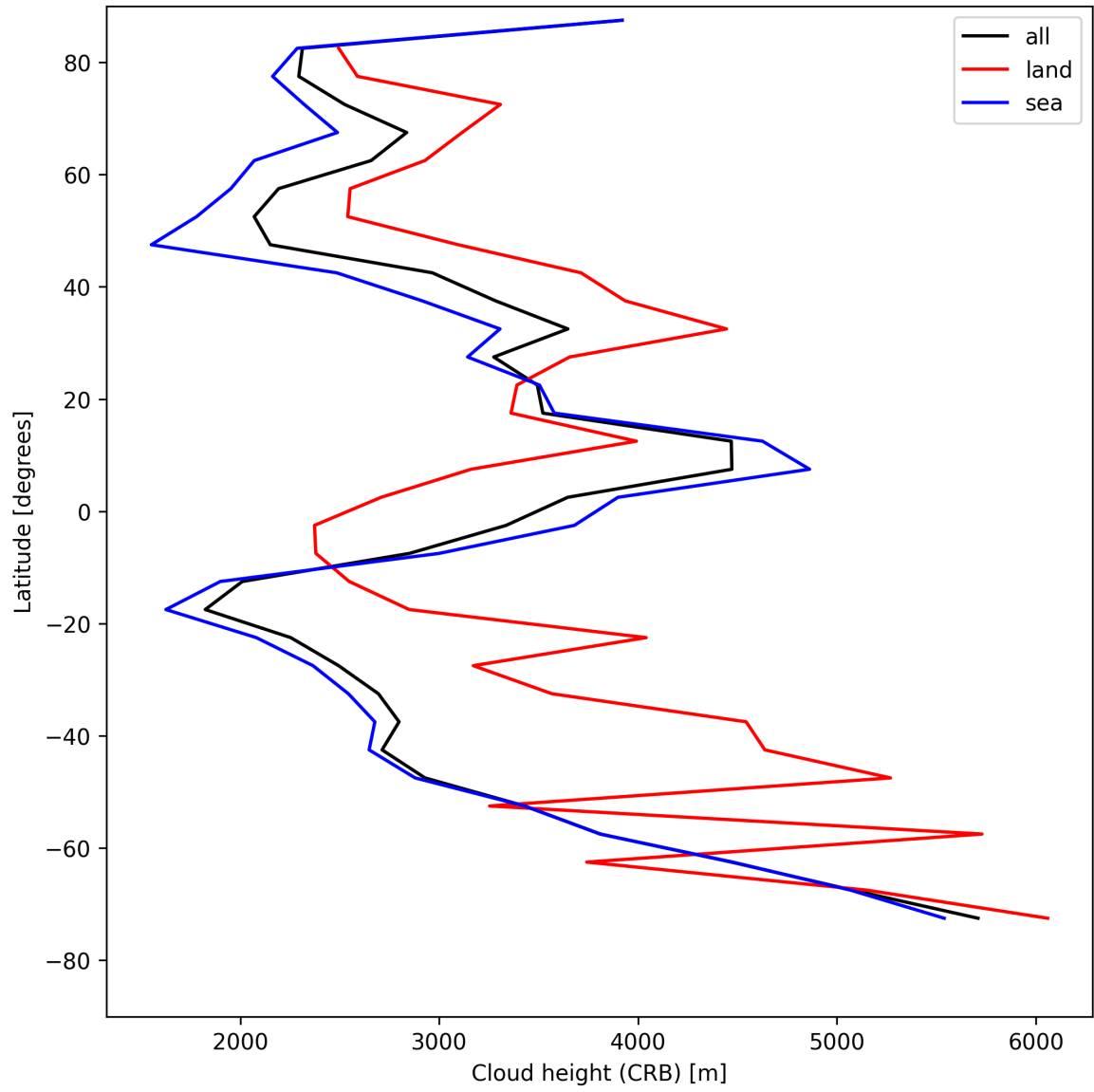
Figure 27: Zonal average of “Cloud height (CRB)” for 2025-07-30 to 2025-08-01.
