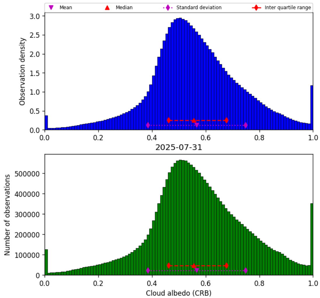
Figure 44: Histogram of “Cloud albedo (CRB)” for 2025-07-30 to 2025-08-01
