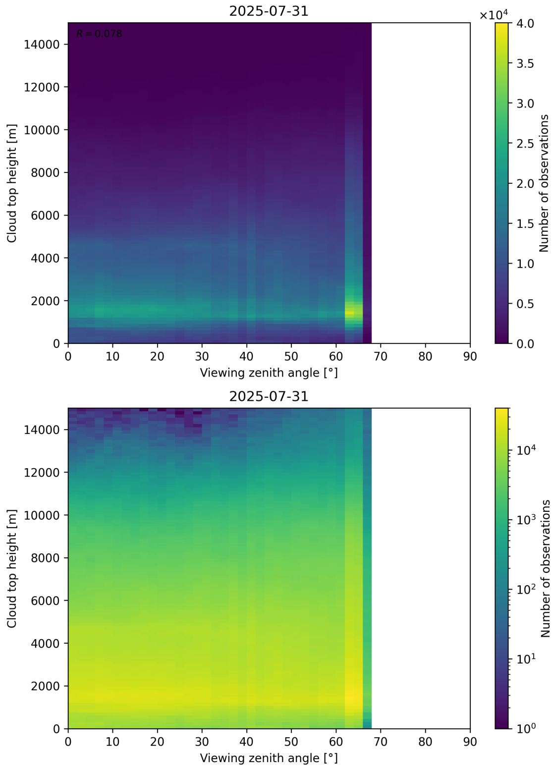
Figure 112: Scatter density plot of “Viewing zenith angle” against “Cloud top height” for 2025-07-30 to 2025-08-01.
