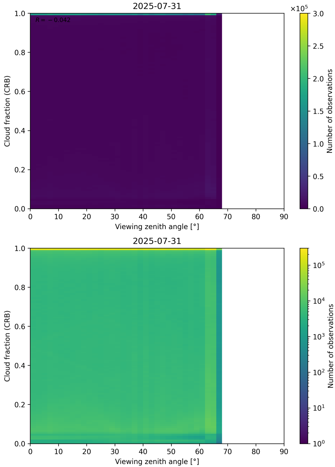
Figure 109: Scatter density plot of “Viewing zenith angle” against “Cloud fraction (CRB)” for 2025-07-30 to 2025-08-01.
